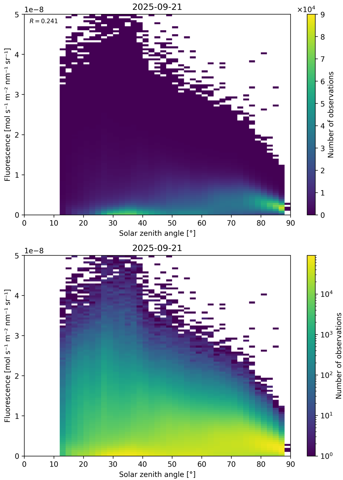
Figure 112: Scatter density plot of “Solar zenith angle” against “Fluorescence” for 2025-09-20 to 2025-09-22.
