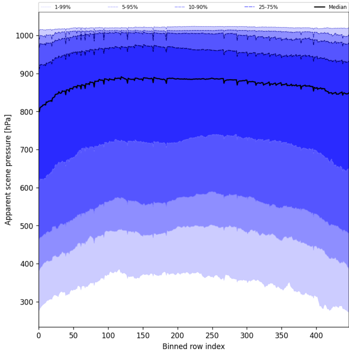
Figure 53: Along track statistics of “Apparent scene pressure” for 2025-09-20 to 2025-09-22
