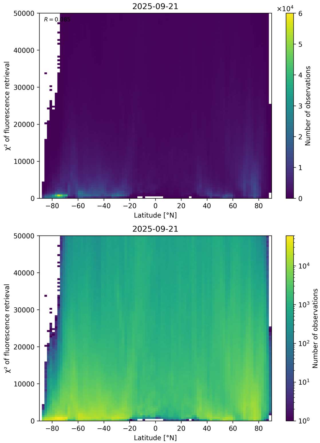
Figure 89: Scatter density plot of “Latitude” against “ \chi^2 of fluorescence retrieval” for 2025-09-20 to 2025-09-22.
