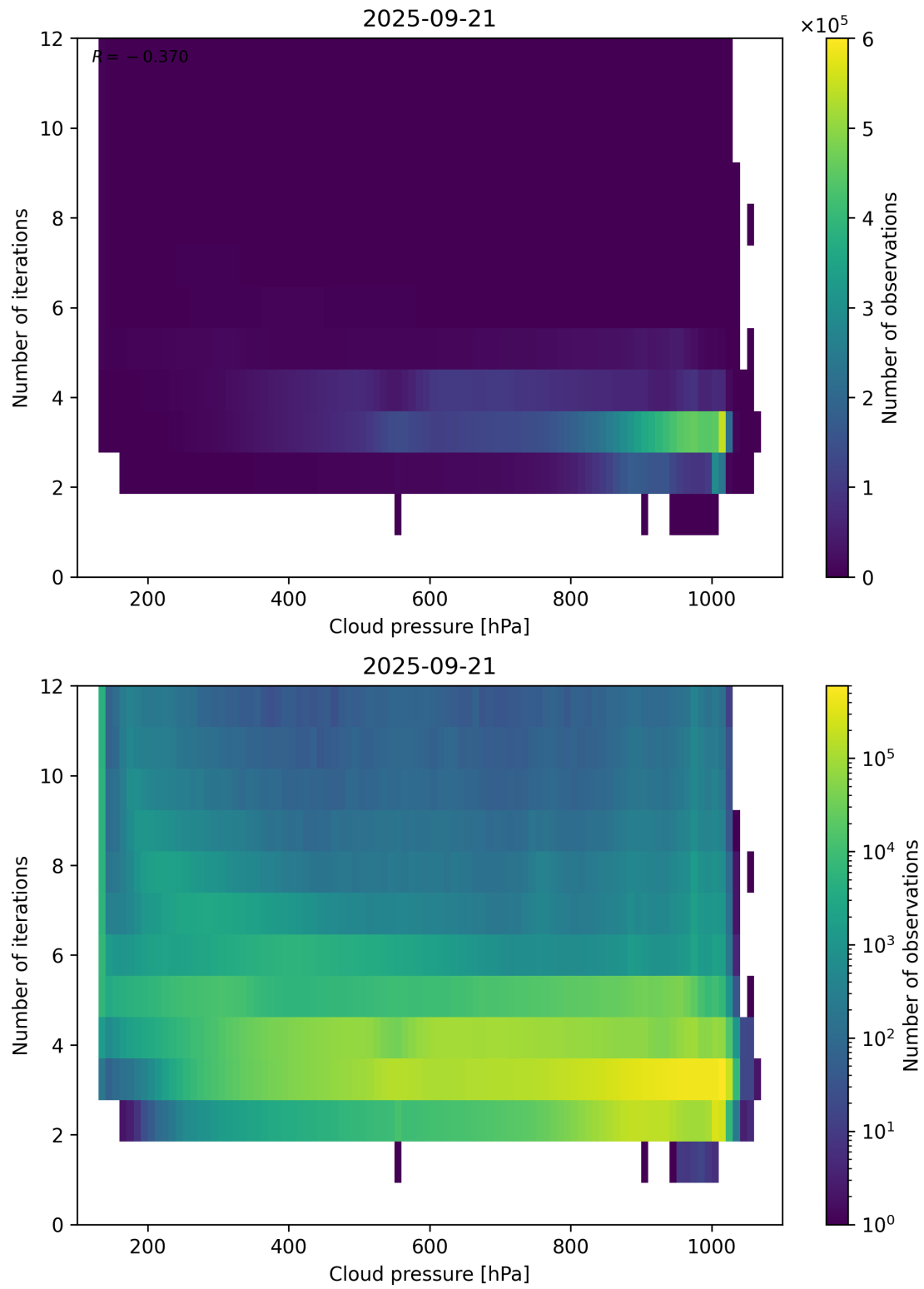
Figure 81: Scatter density plot of “Cloud pressure” against “Number of iterations” for 2025-09-20 to 2025-09-22.
