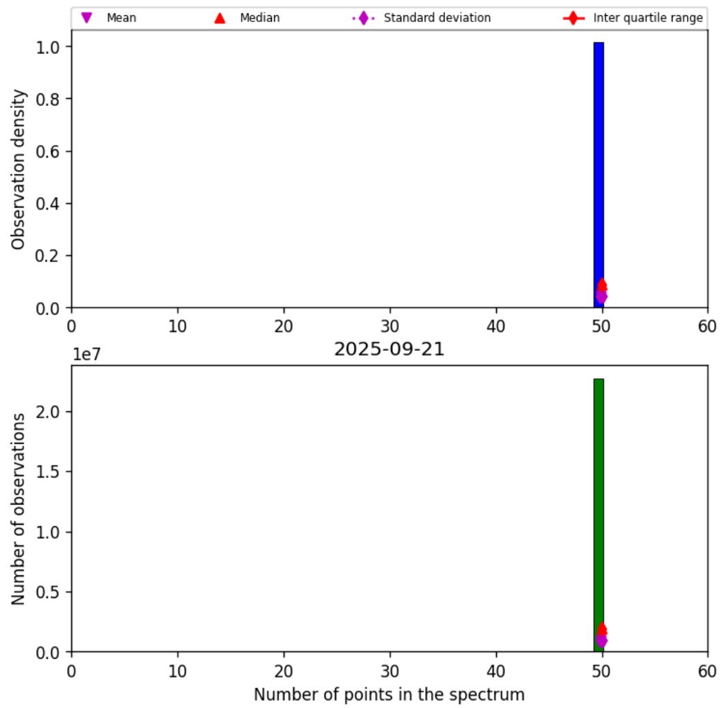
Figure 44: Histogram of "Number of points in the spectrum" for 2025-09-20 to 2025-09-22
