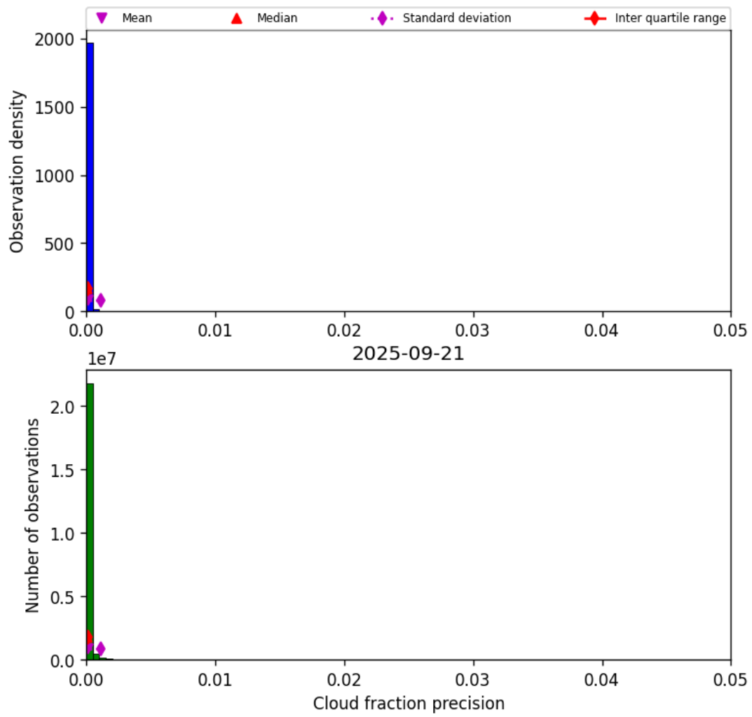
Figure 33: Histogram of “Cloud fraction precision” for 2025-09-20 to 2025-09-22
