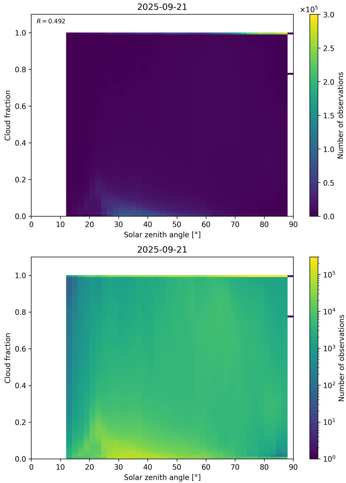
Figure 110: Scatter density plot of “Solar zenith angle” against “Cloud fraction” for 2025-09-20 to 2025-09-22.
