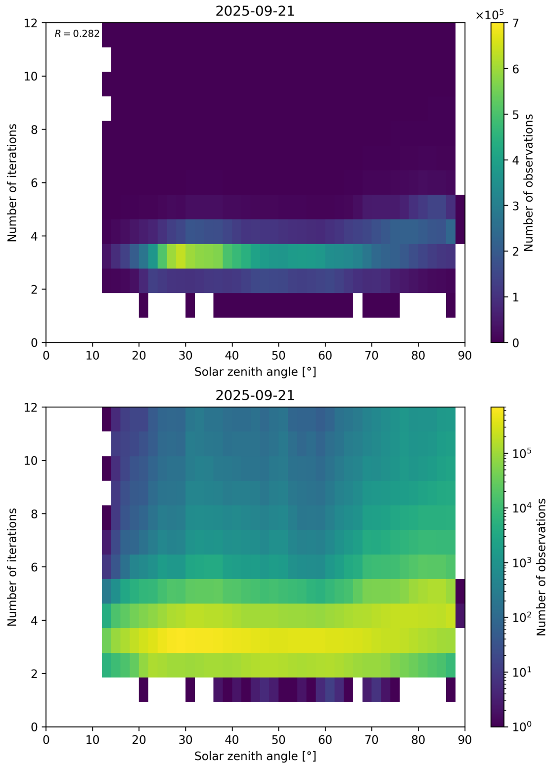
Figure 114: Scatter density plot of “Solar zenith angle” against “Number of iterations” for 2025-09-20 to 2025-09-22.
