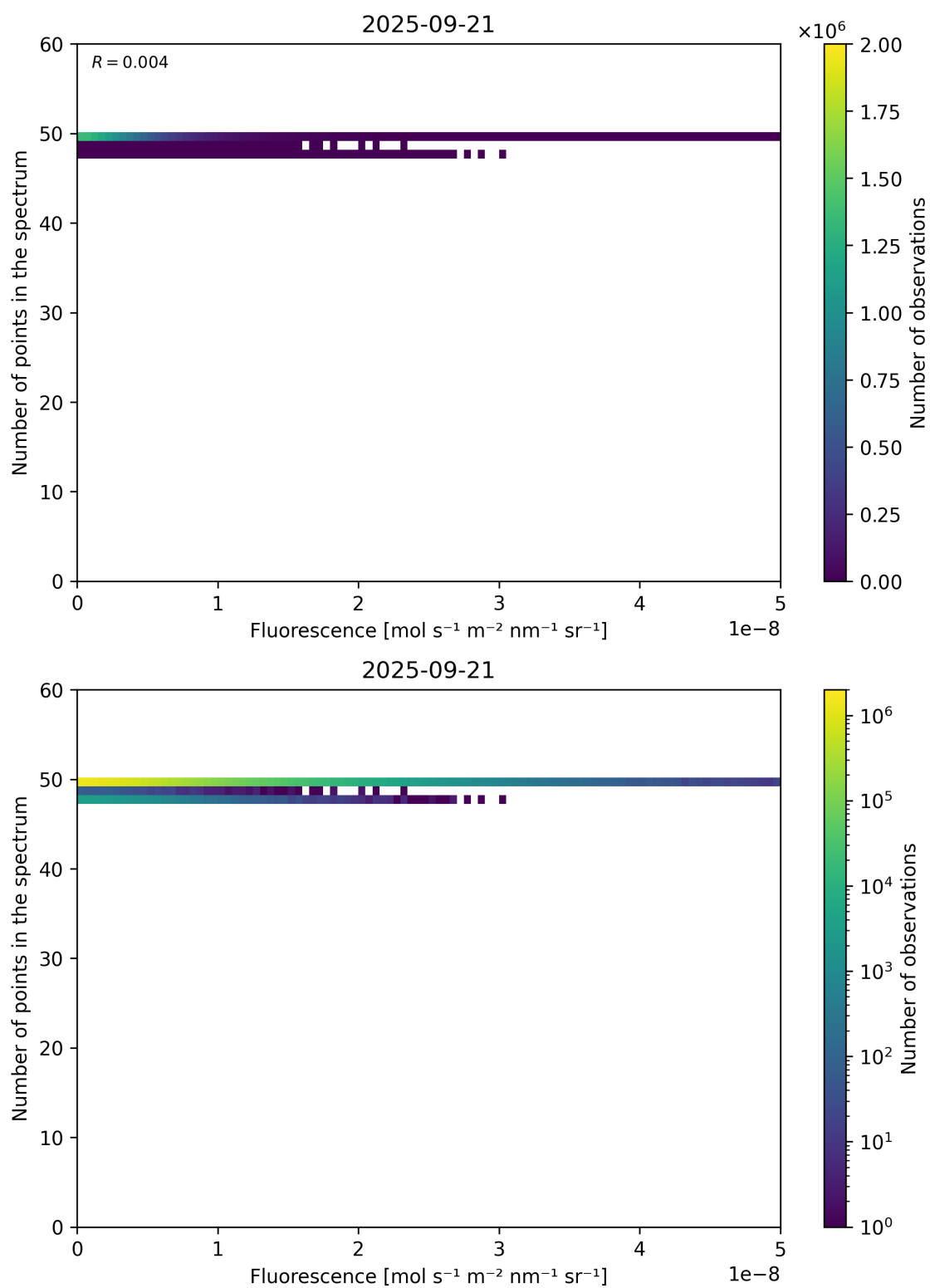
Figure 86: Scatter density plot of “Fluorescence” against “Number of points in the spectrum” for 2025-09-20 to 2025-09-22.
