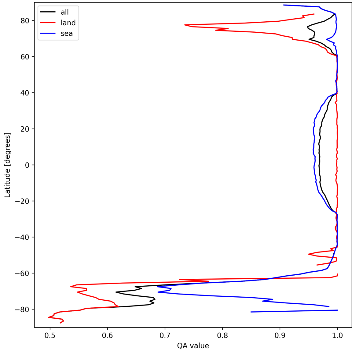
Figure 12: Zonal average of "QA value" for 2025-09-20 to 2025-09-22.
