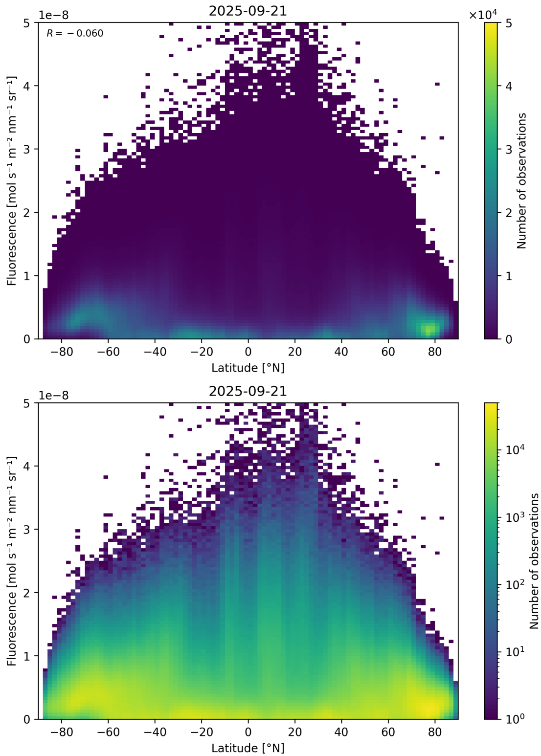
Figure 92: Scatter density plot of “Latitude” against “Fluorescence” for 2025-09-20 to 2025-09-22.
