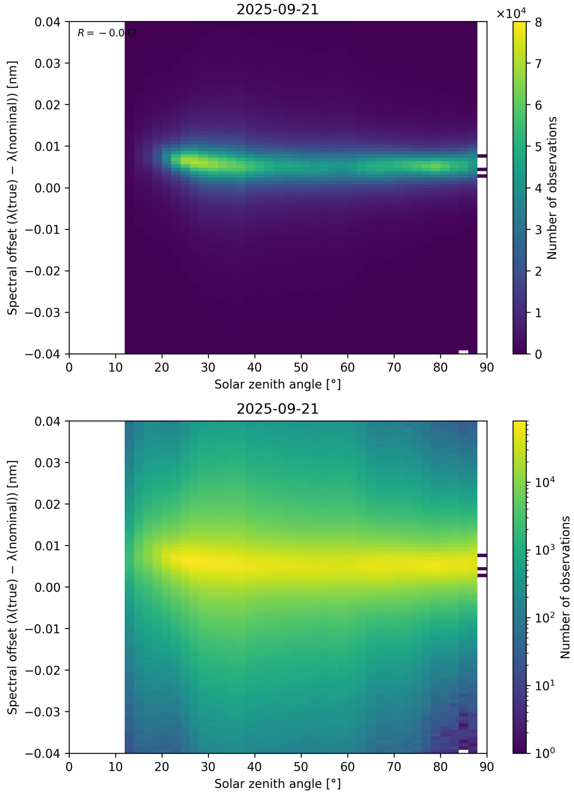
Figure 117: Scatter density plot of “Solar zenith angle” against “Spectral offset ( \lambda_{\text{true}} - \lambda_{\text{nominal}} )” for 2025-09-20 to 2025-09-22.
