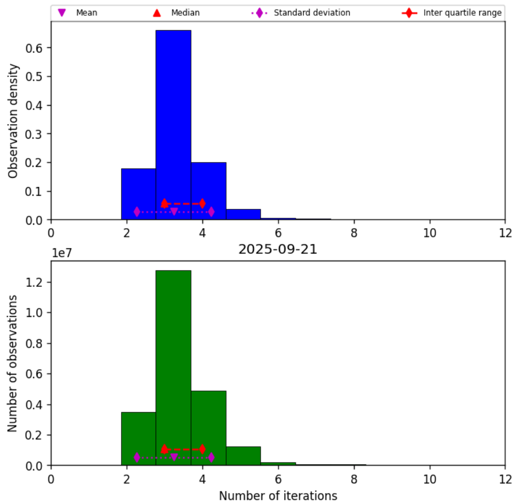
Figure 39: Histogram of “Number of iterations” for 2025-09-20 to 2025-09-22
