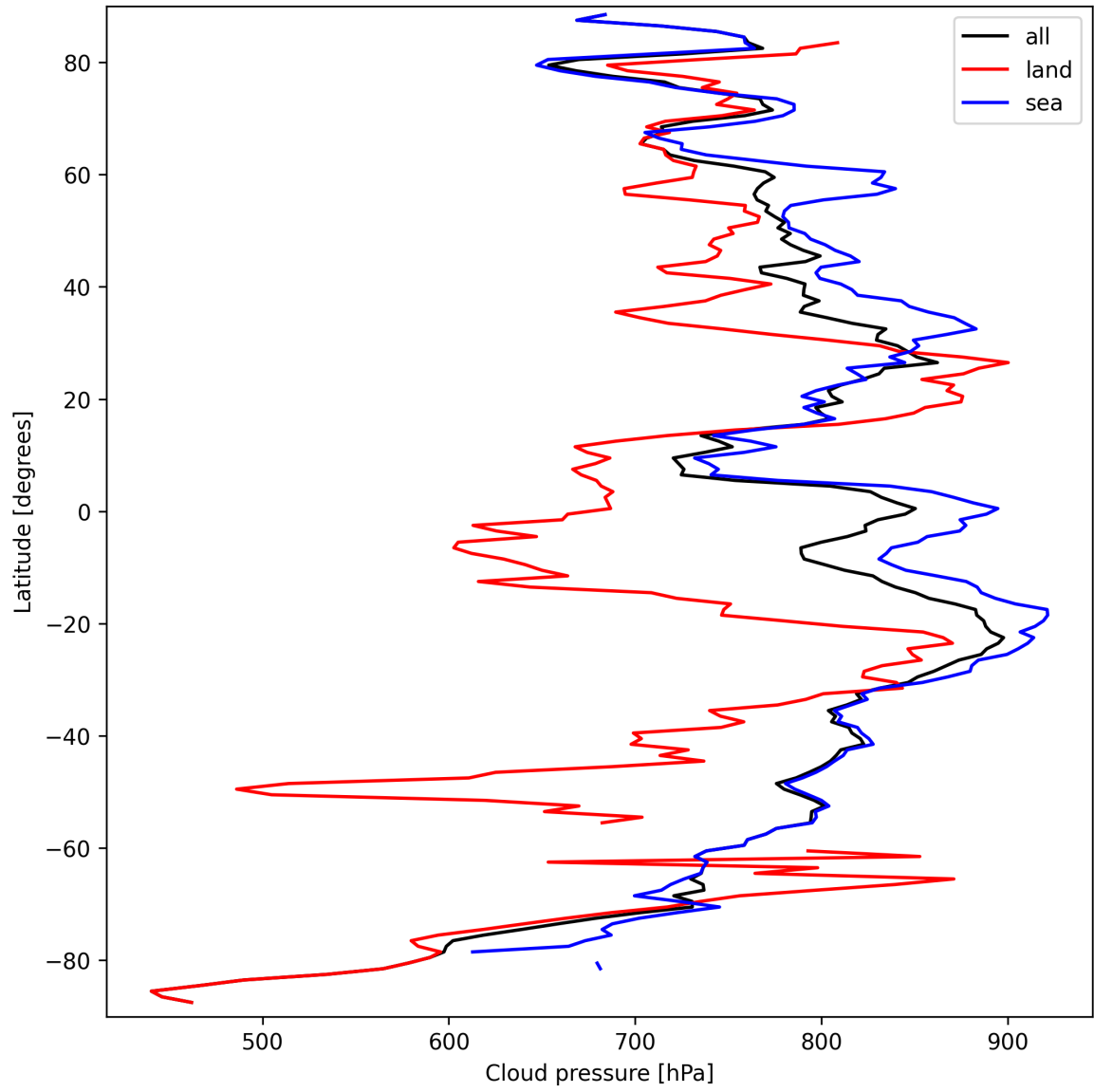
Figure 13: Zonal average of “Cloud pressure” for 2025-09-20 to 2025-09-22.
