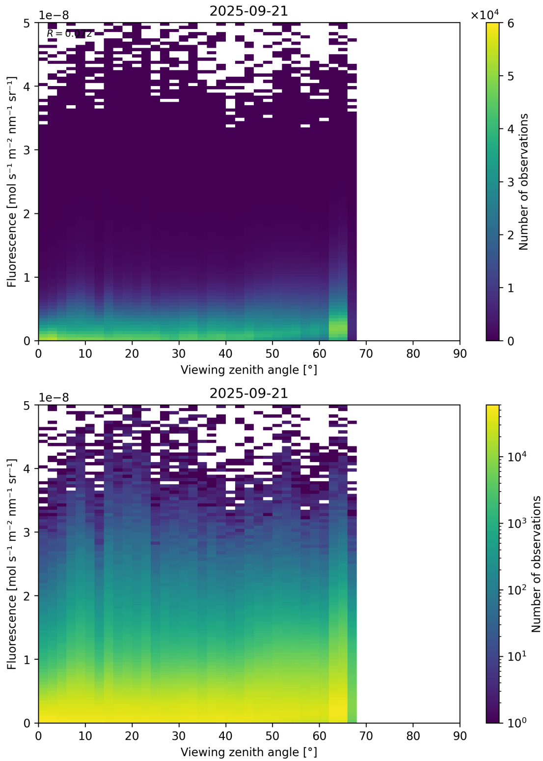
Figure 122: Scatter density plot of “Viewing zenith angle” against “Fluorescence” for 2025-09-20 to 2025-09-22.
