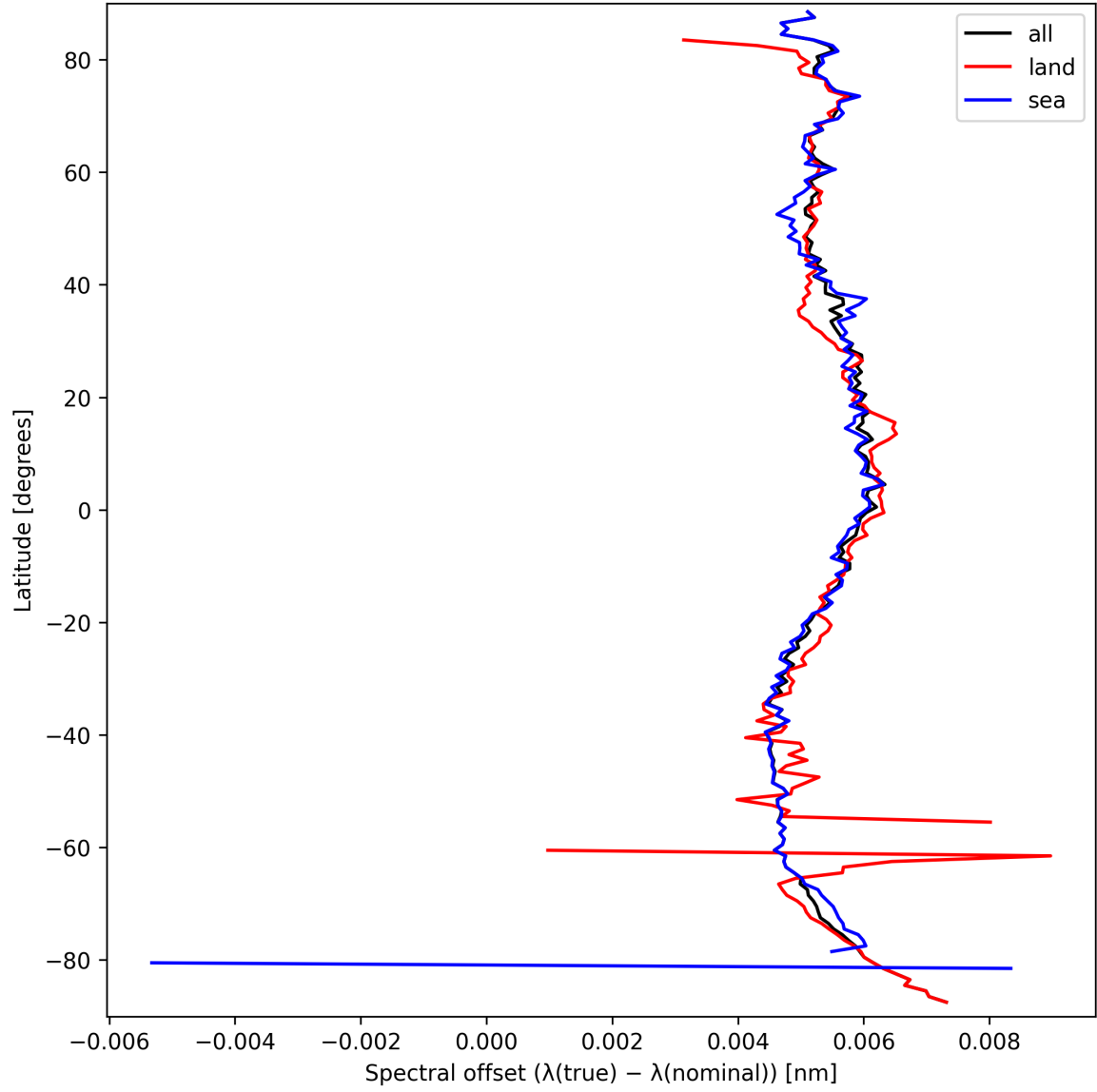
Figure 28: Zonal average of “Spectral offset ( \lambda_{\text{true}} - \lambda_{\text{nominal}} )” for 2025-09-20 to 2025-09-22.
