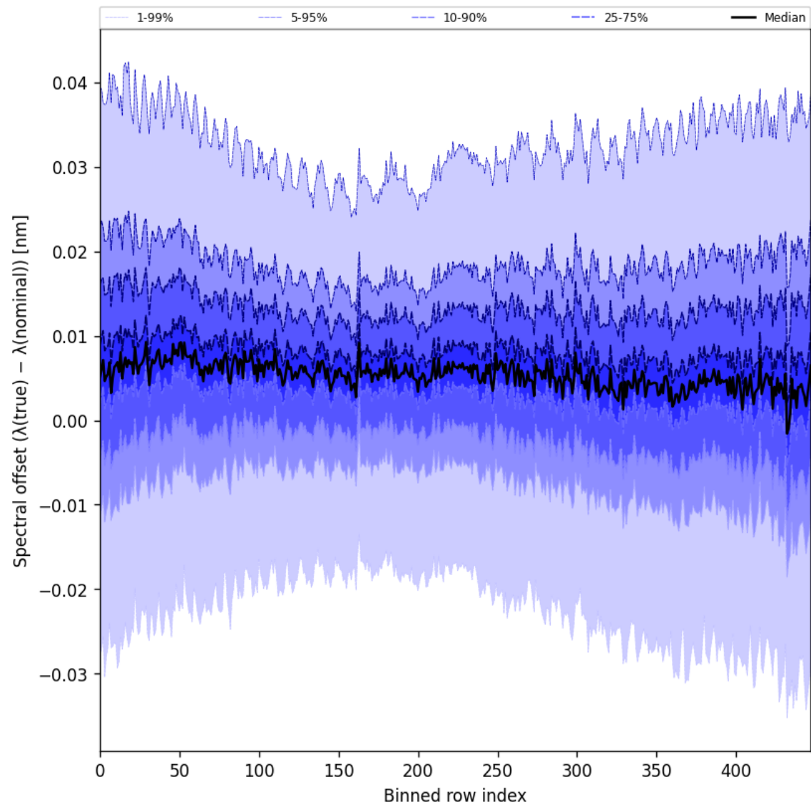
Figure 62: Along track statistics of “Spectral offset ( \lambda_{\text{true}} - \lambda_{\text{nominal}} )” for 2025-09-20 to 2025-09-22
