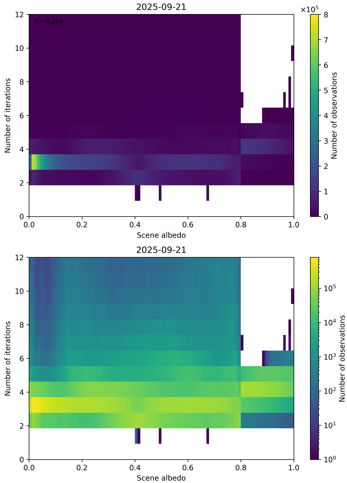
Figure 105: Scatter density plot of “Scene albedo” against “Number of iterations” for 2025-09-20 to 2025-09-22.
