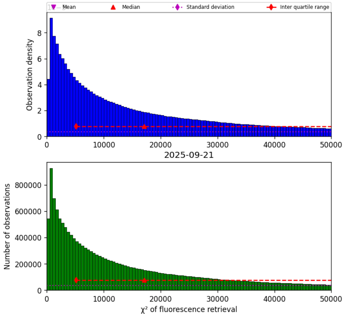
Figure 42: Histogram of “ \chi^2 of fluorescence retrieval” for 2025-09-20 to 2025-09-22
