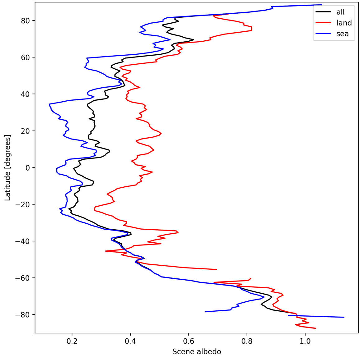
Figure 17: Zonal average of “Scene albedo” for 2025-09-20 to 2025-09-22.
