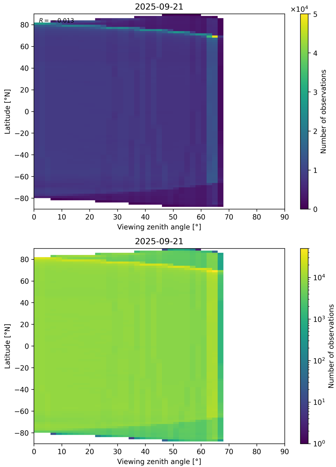
Figure 123: Scatter density plot of “Viewing zenith angle” against “Latitude” for 2025-09-20 to 2025-09-22.
