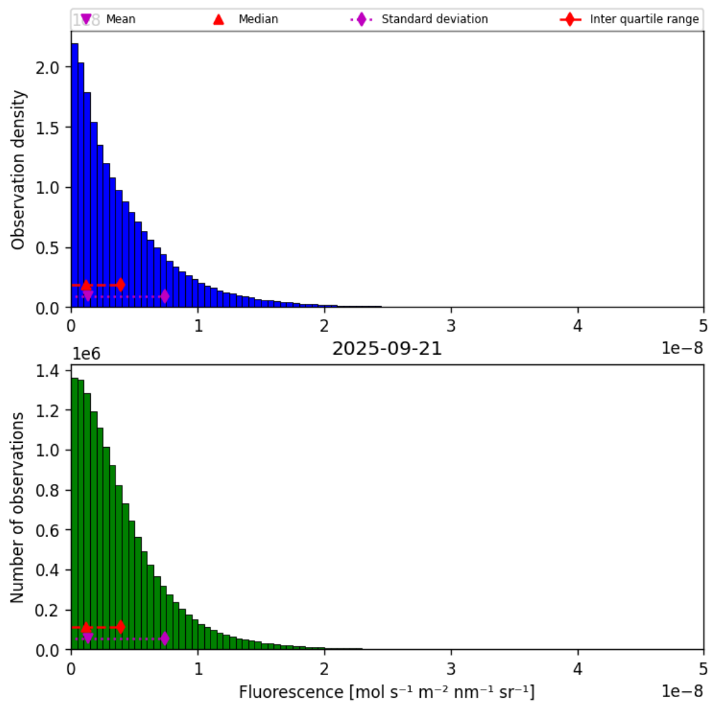
Figure 40: Histogram of “Fluorescence” for 2025-09-20 to 2025-09-22
