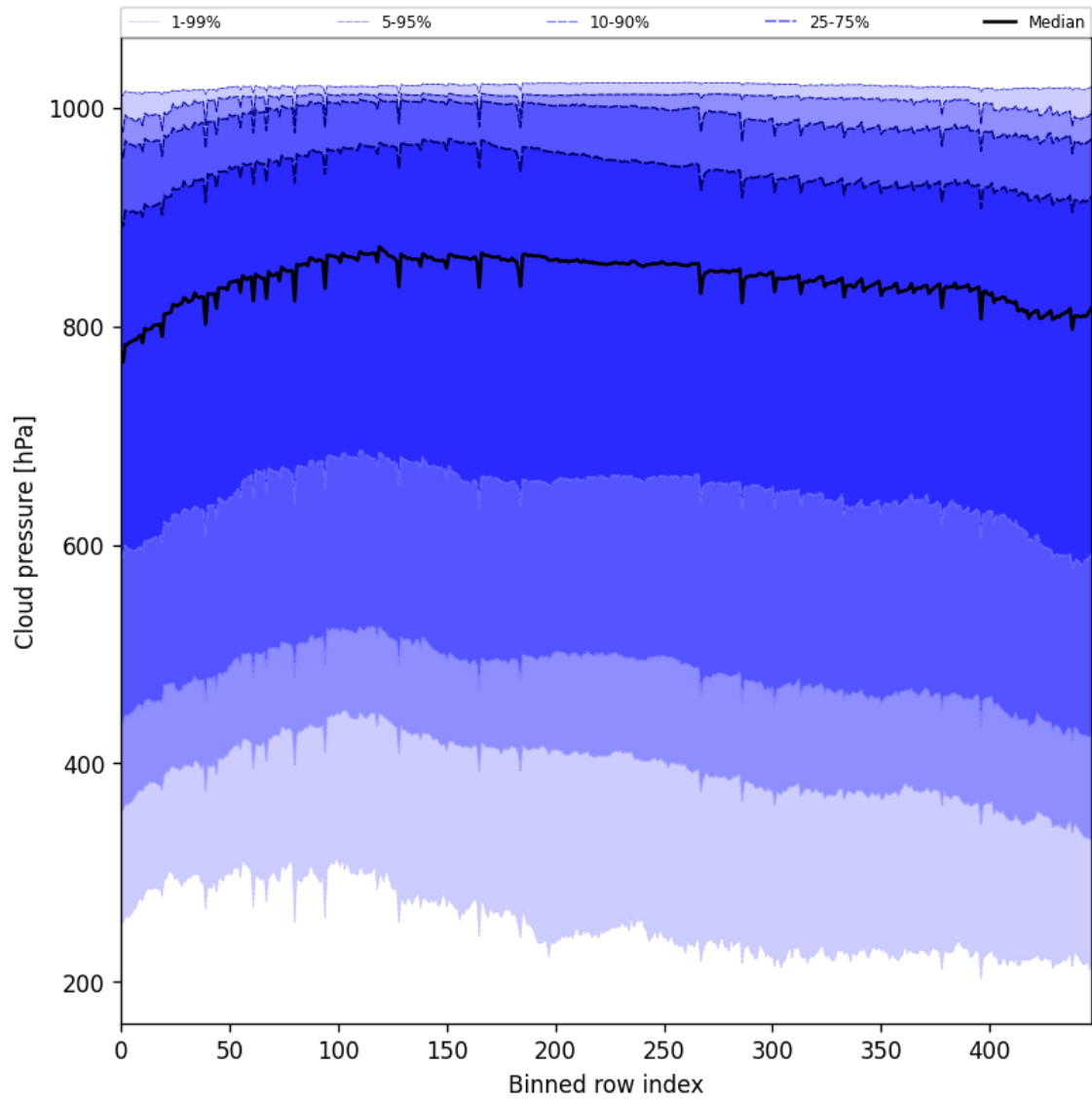
Figure 47: Along track statistics of “Cloud pressure” for 2025-09-20 to 2025-09-22
