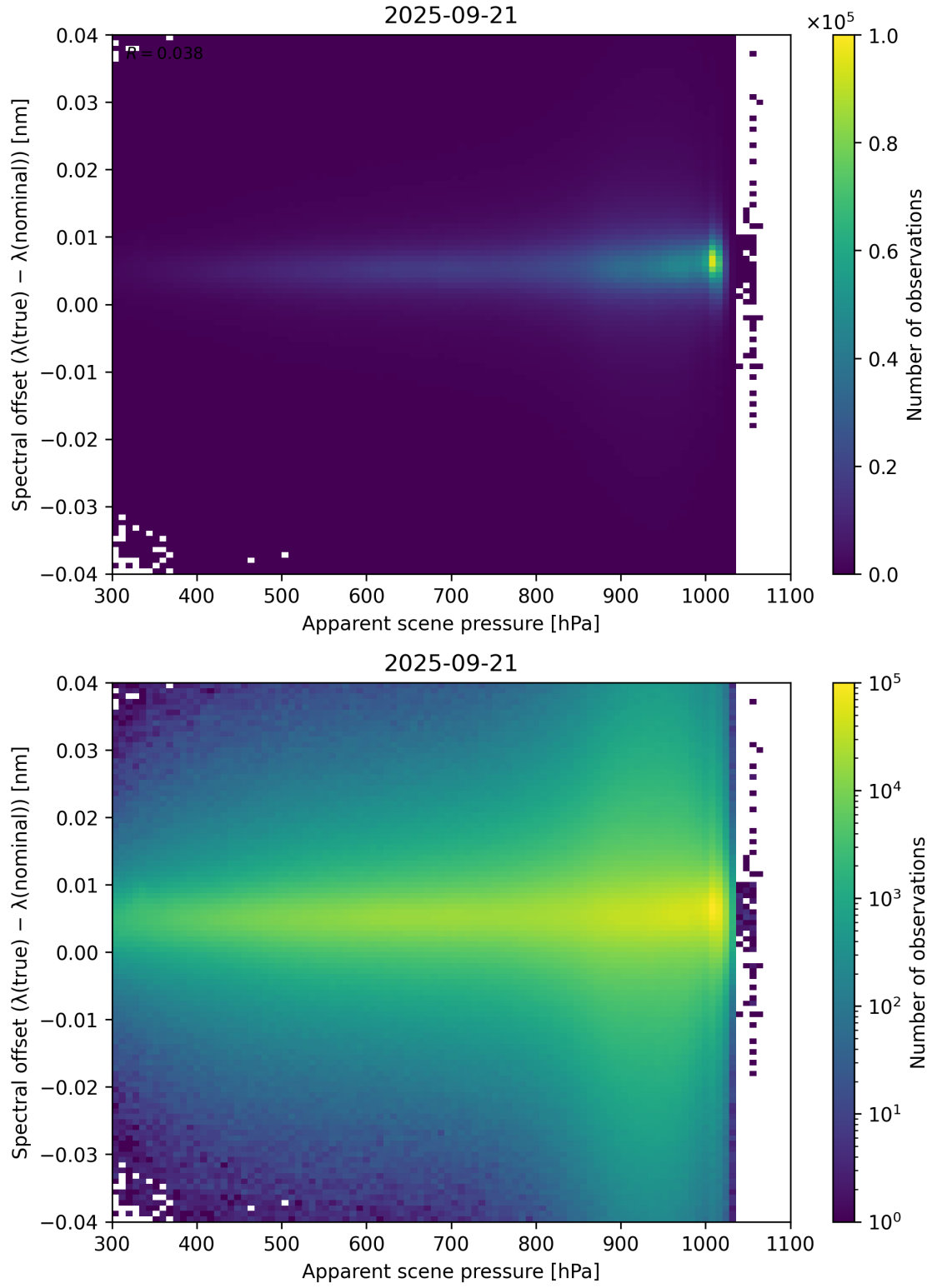
Figure 67: Scatter density plot of “Apparent scene pressure” against “Spectral offset ( \lambda_{\text{true}} - \lambda_{\text{nominal}} )” for 2025-09-20 to 2025-09-22.
