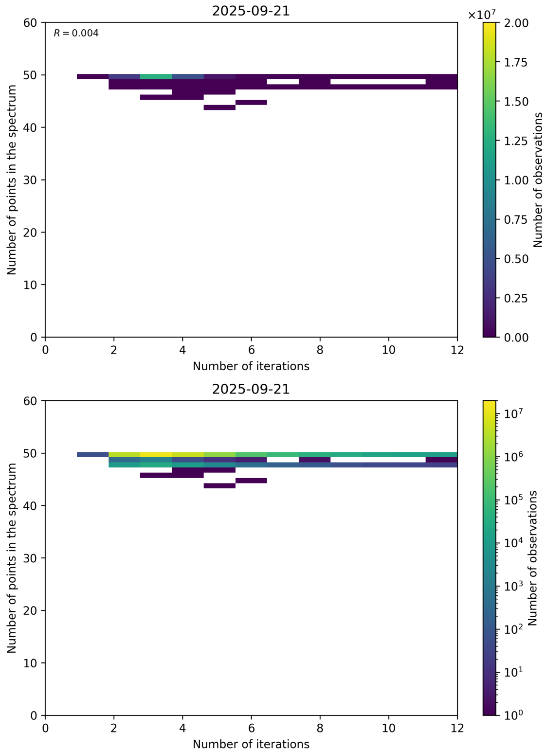
Figure 99: Scatter density plot of “Number of iterations” against “Number of points in the spectrum” for 2025-09-20 to 2025-09-22.
