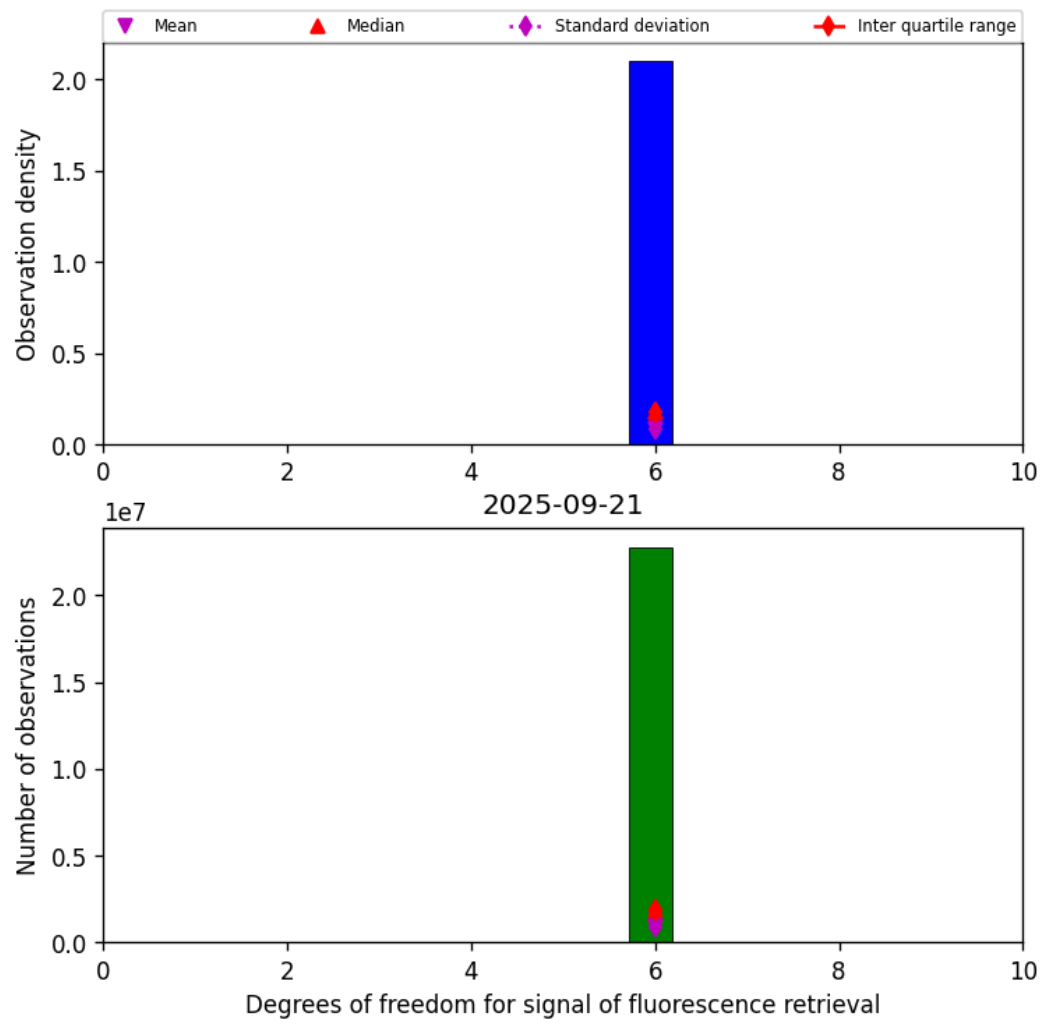
Figure 43: Histogram of "Degrees of freedom for signal of fluorescence retrieval" for 2025-09-20 to 2025-09-22
