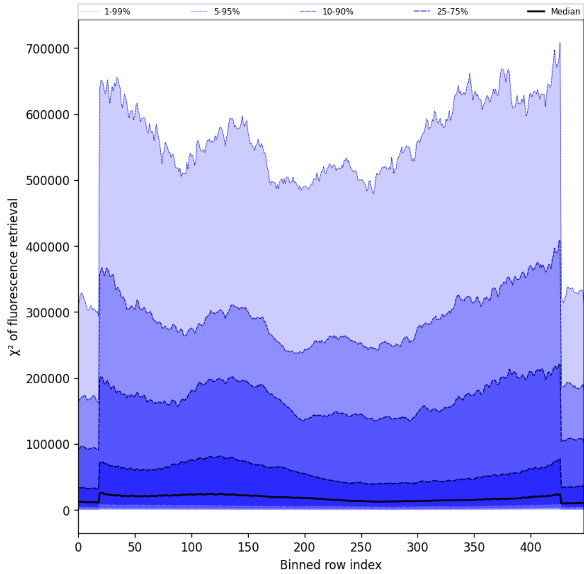
Figure 59: Along track statistics of “ \chi^2 of fluorescence retrieval” for 2025-09-20 to 2025-09-22
