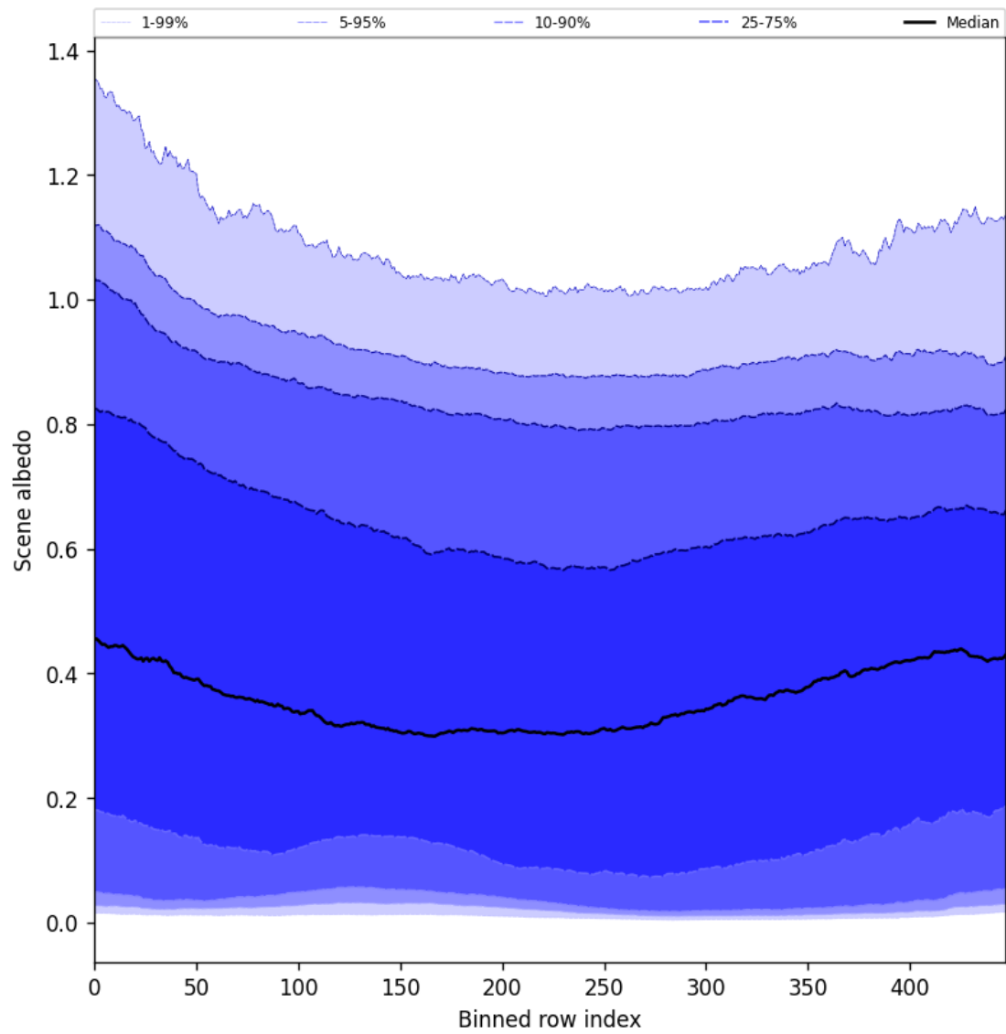
Figure 51: Along track statistics of “Scene albedo” for 2025-09-20 to 2025-09-22
