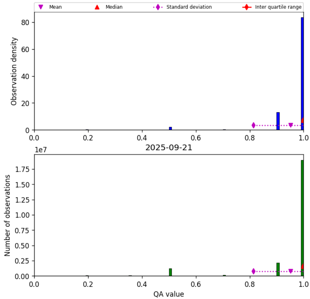
Figure 29: Histogram of “QA value” for 2025-09-20 to 2025-09-22
