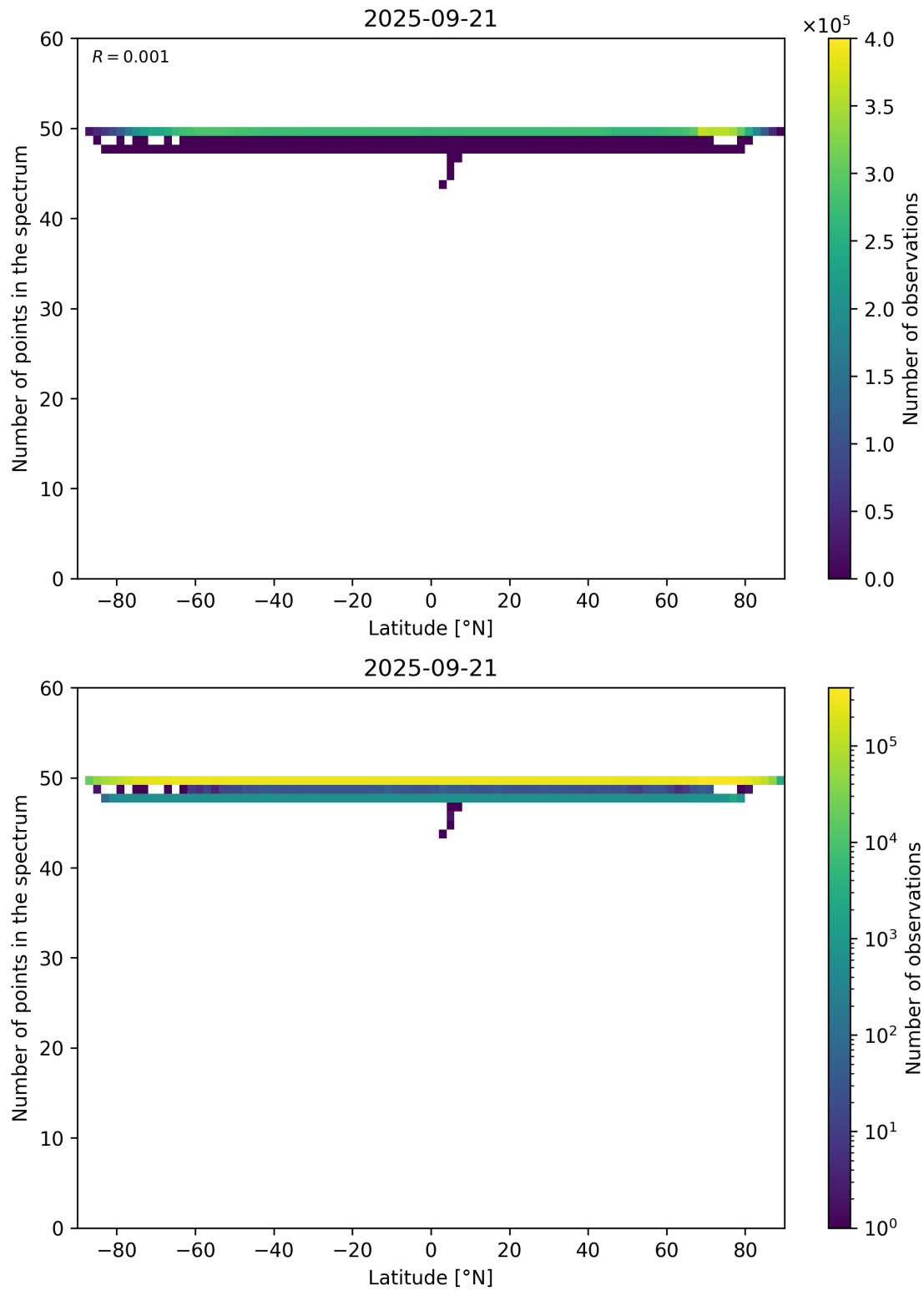
Figure 94: Scatter density plot of “Latitude” against “Number of points in the spectrum” for 2025-09-20 to 2025-09-22.
