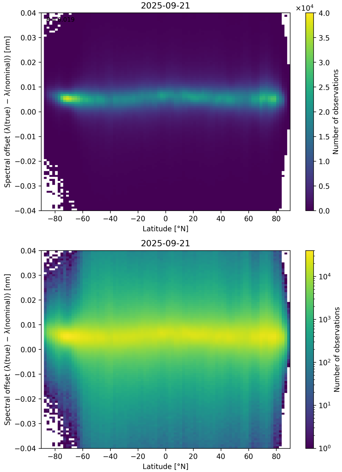
Figure 96: Scatter density plot of “Latitude” against “Spectral offset ( \lambda_{\text{true}} - \lambda_{\text{nominal}} )” for 2025-09-20 to 2025-09-22.
