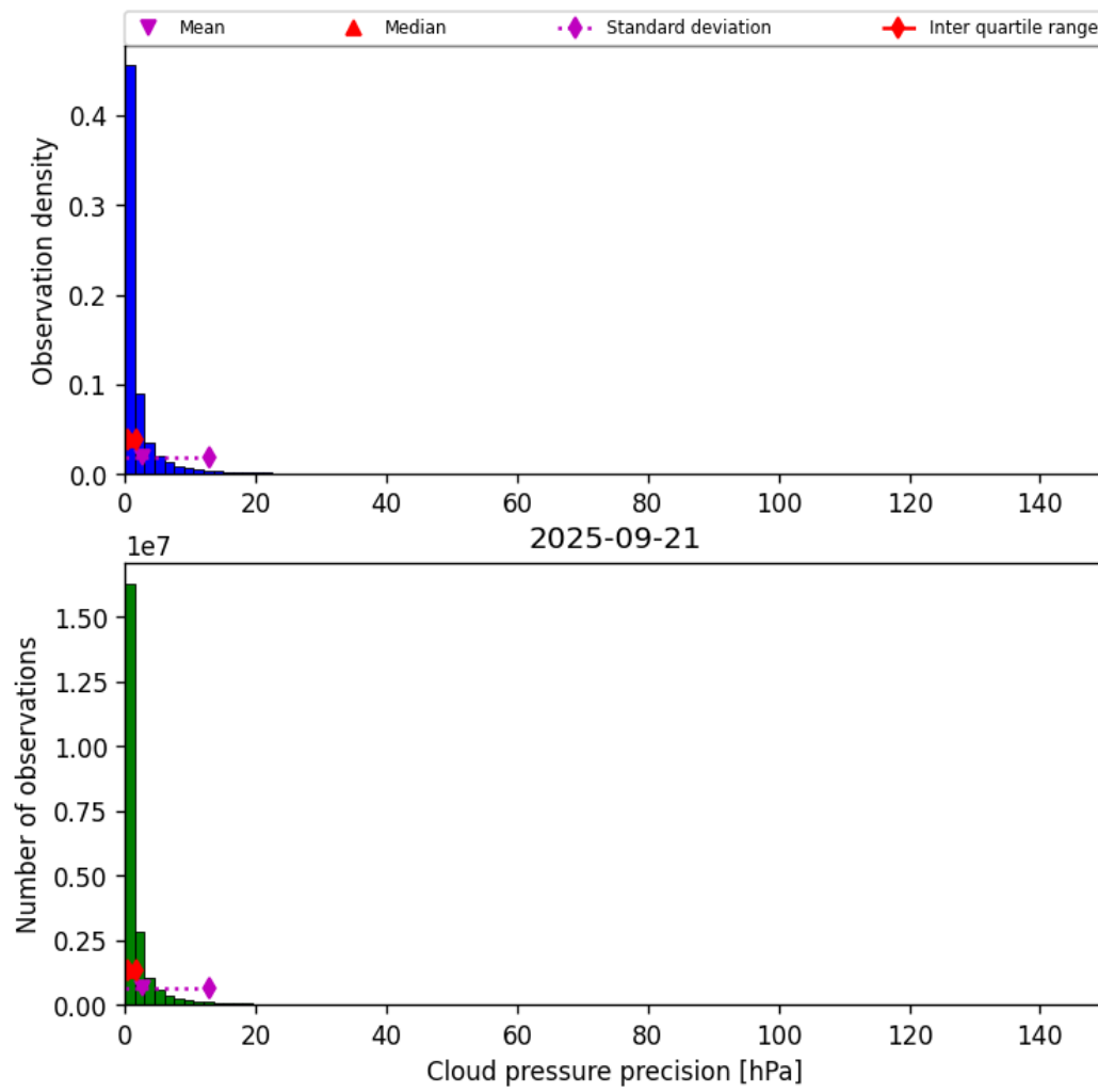
Figure 31: Histogram of “Cloud pressure precision” for 2025-09-20 to 2025-09-22
