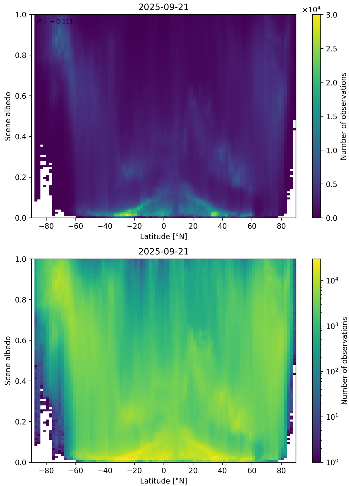
Figure 95: Scatter density plot of “Latitude” against “Scene albedo” for 2025-09-20 to 2025-09-22.
