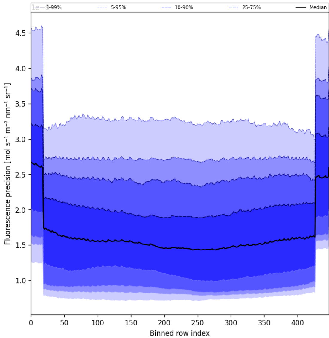
Figure 58: Along track statistics of “Fluorescence precision” for 2025-09-20 to 2025-09-22
