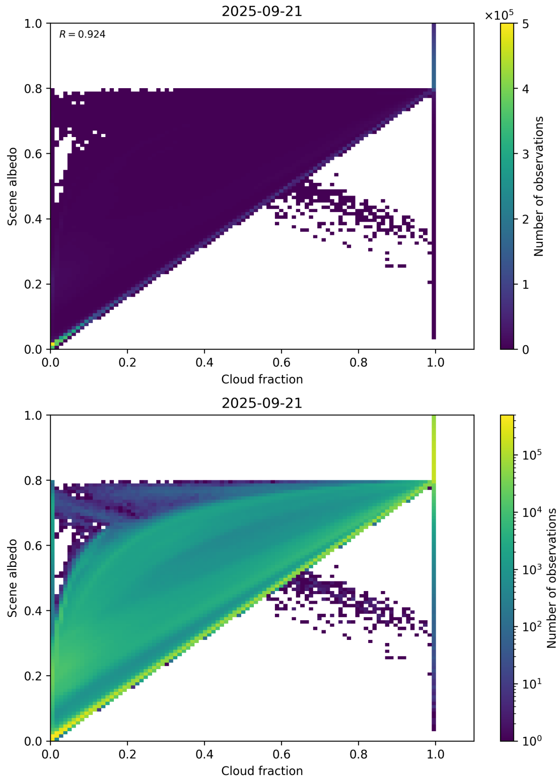
Figure 75: Scatter density plot of “Cloud fraction” against “Scene albedo” for 2025-09-20 to 2025-09-22.
