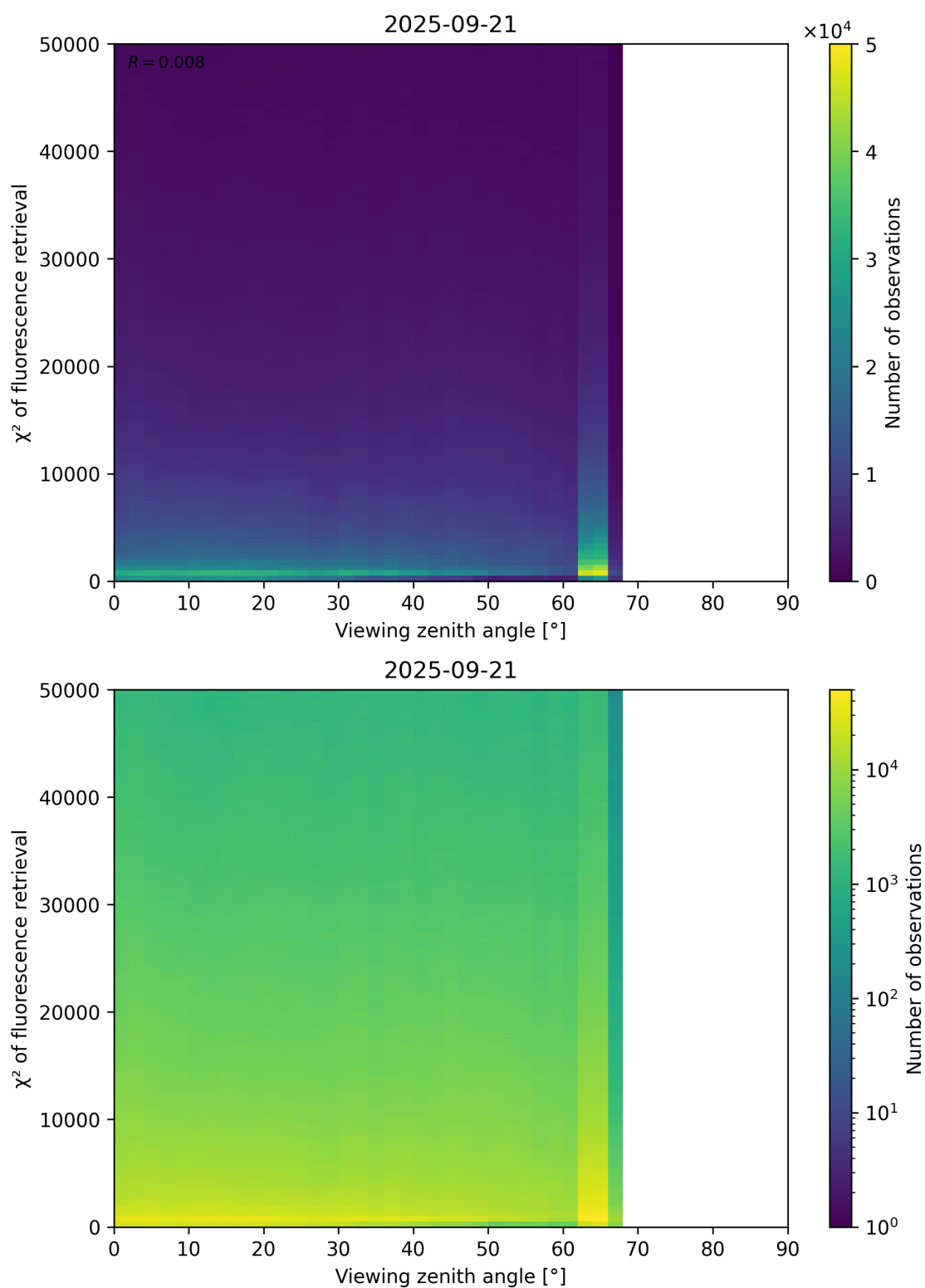
Figure 119: Scatter density plot of “Viewing zenith angle” against “ \chi^2 of fluorescence retrieval” for 2025-09-20 to 2025-09-22.
