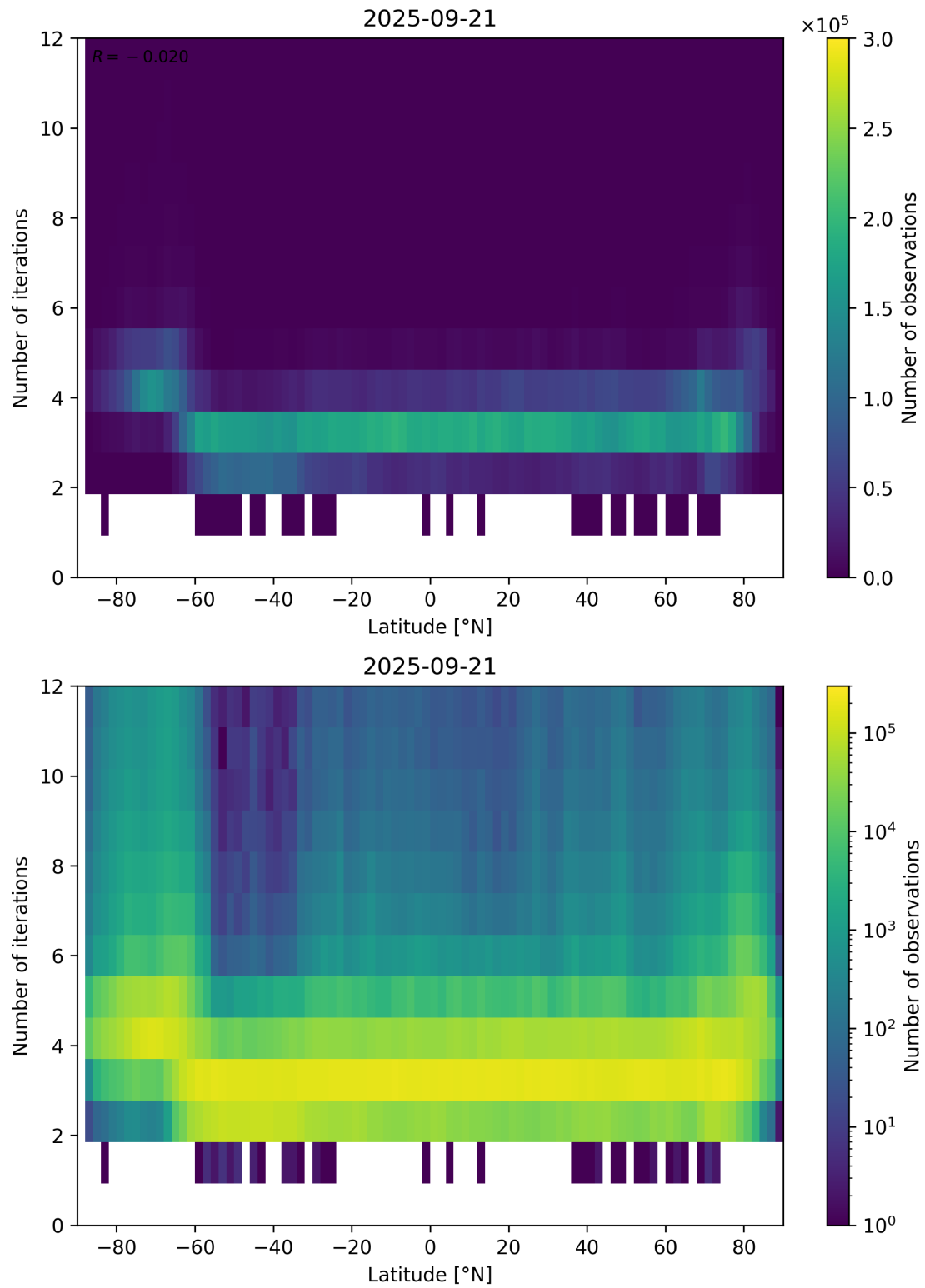
Figure 93: Scatter density plot of “Latitude” against “Number of iterations” for 2025-09-20 to 2025-09-22.
