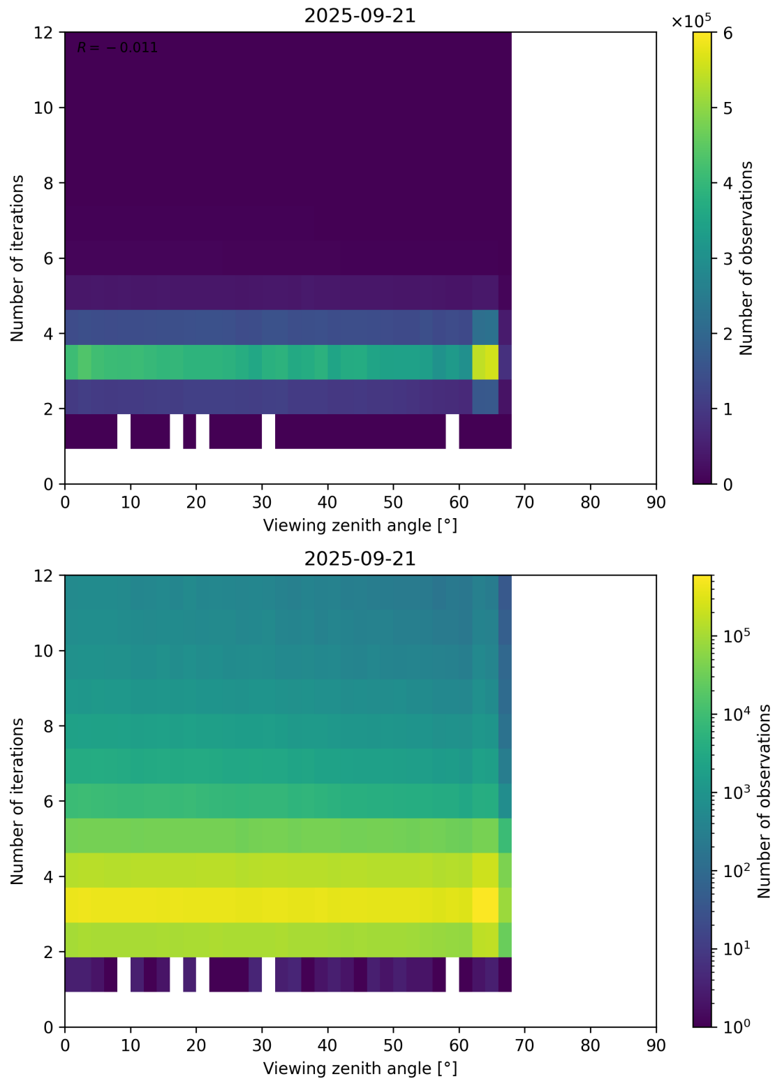
Figure 124: Scatter density plot of “Viewing zenith angle” against “Number of iterations” for 2025-09-20 to 2025-09-22.
