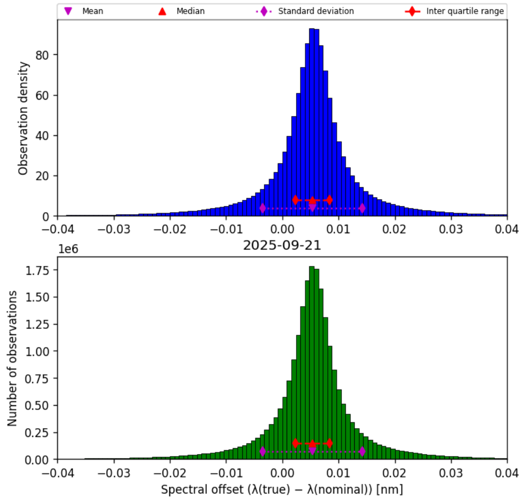
Figure 45: Histogram of “Spectral offset ( \lambda_{\text{true}} - \lambda_{\text{nominal}} )” for 2025-09-20 to 2025-09-22
