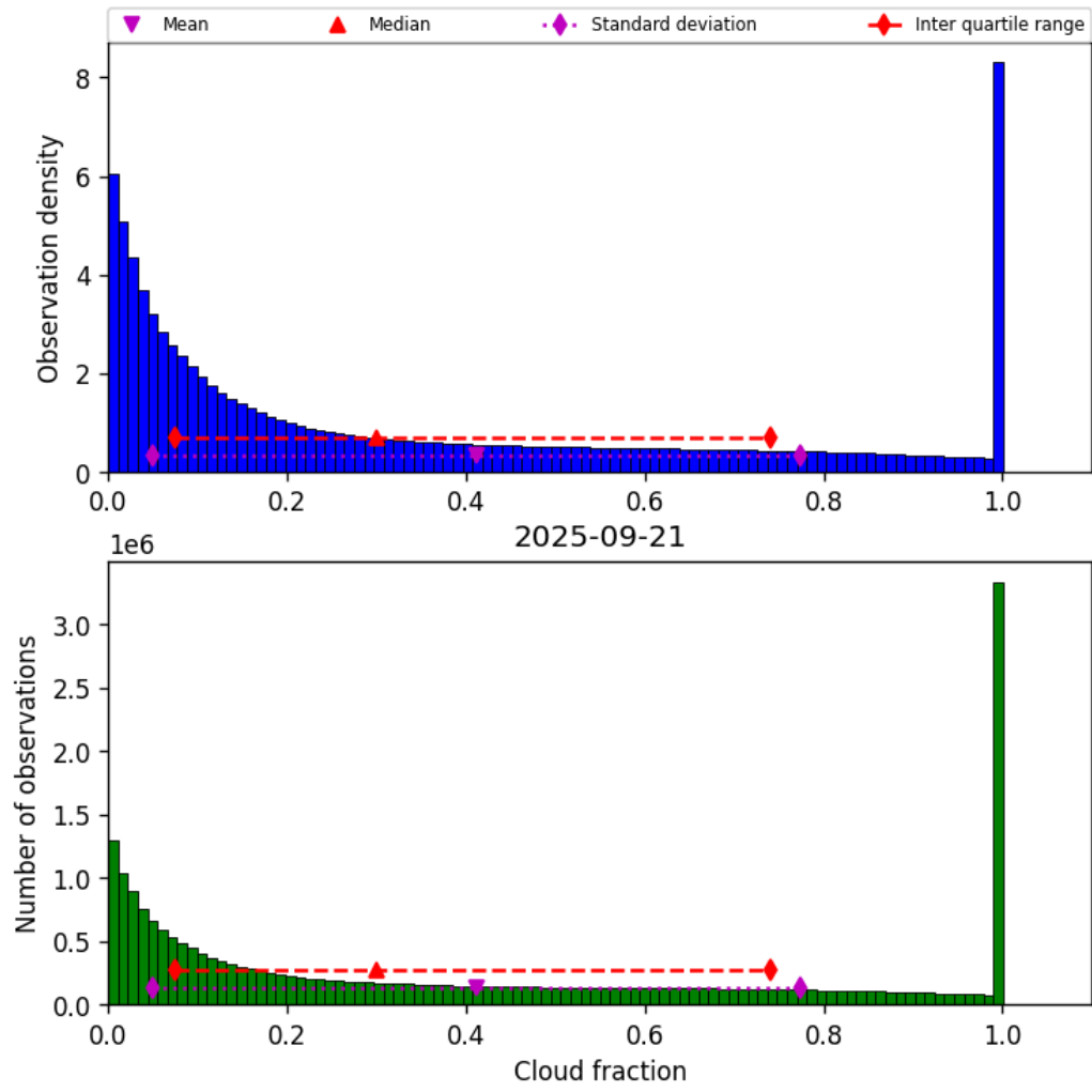
Figure 32: Histogram of “Cloud fraction” for 2025-09-20 to 2025-09-22
