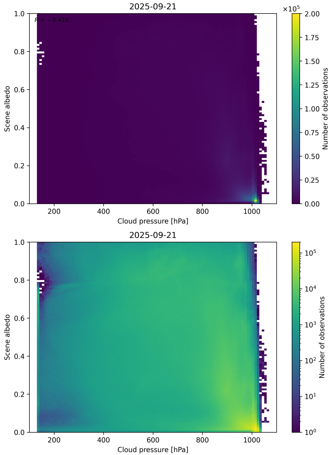
Figure 83: Scatter density plot of “Cloud pressure” against “Scene albedo” for 2025-09-20 to 2025-09-22.
