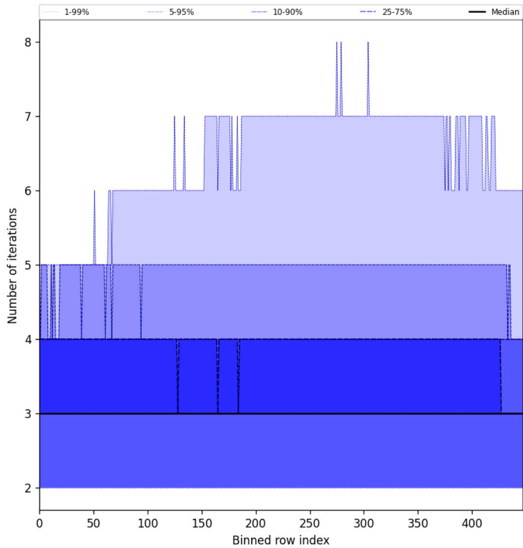
Figure 56: Along track statistics of “Number of iterations” for 2025-09-20 to 2025-09-22
