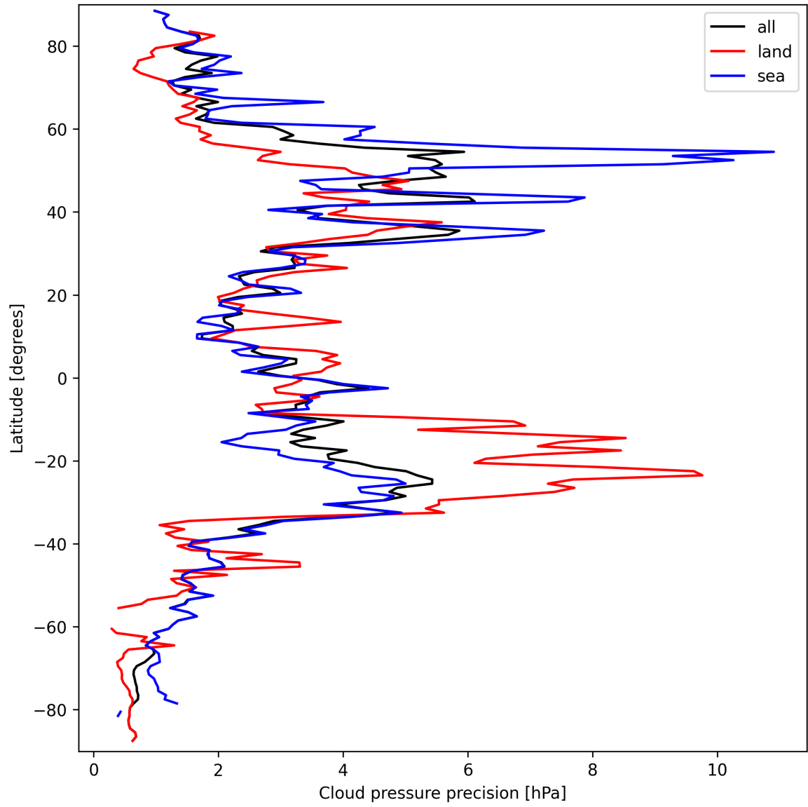
Figure 14: Zonal average of “Cloud pressure precision” for 2025-09-20 to 2025-09-22.
