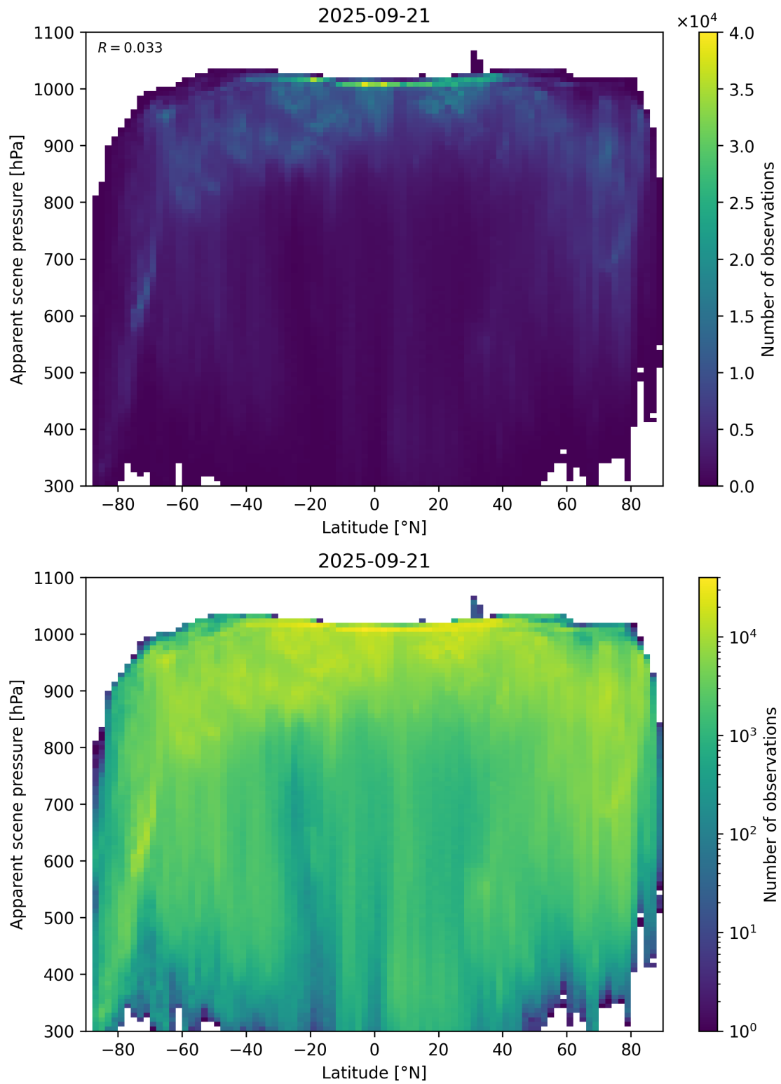
Figure 88: Scatter density plot of “Latitude” against “Apparent scene pressure” for 2025-09-20 to 2025-09-22.
