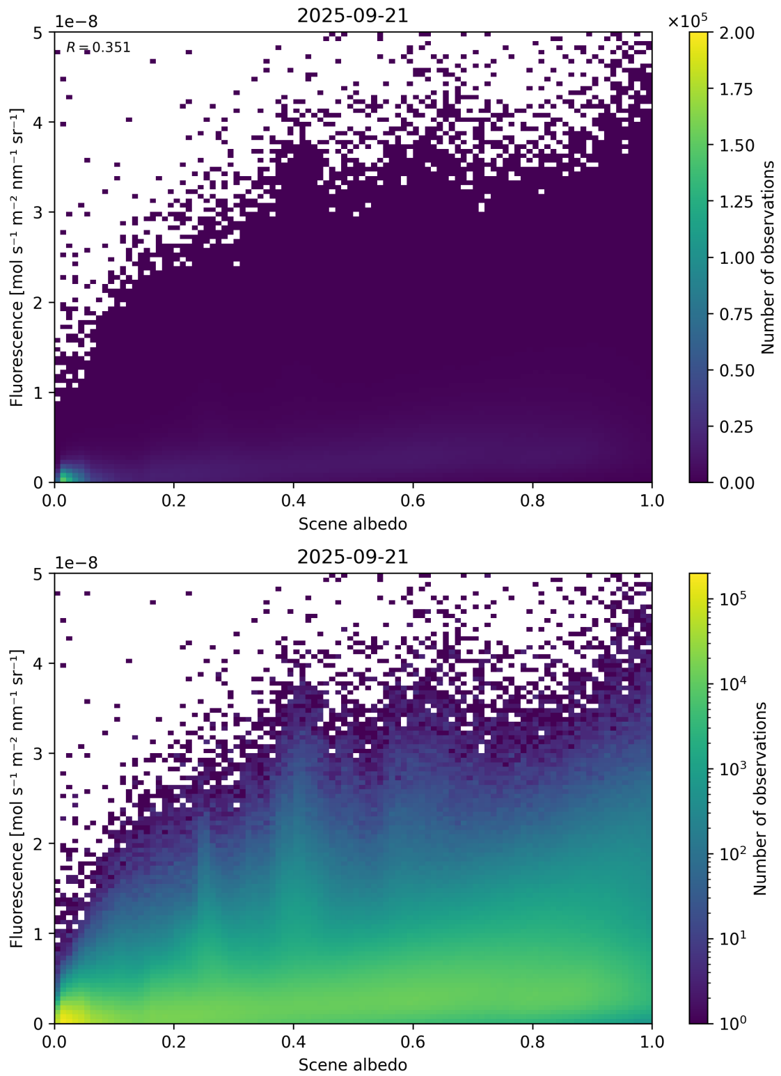
Figure 104: Scatter density plot of “Scene albedo” against “Fluorescence” for 2025-09-20 to 2025-09-22.
