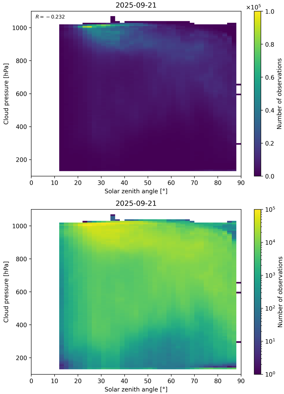
Figure 111: Scatter density plot of “Solar zenith angle” against “Cloud pressure” for 2025-09-20 to 2025-09-22.
