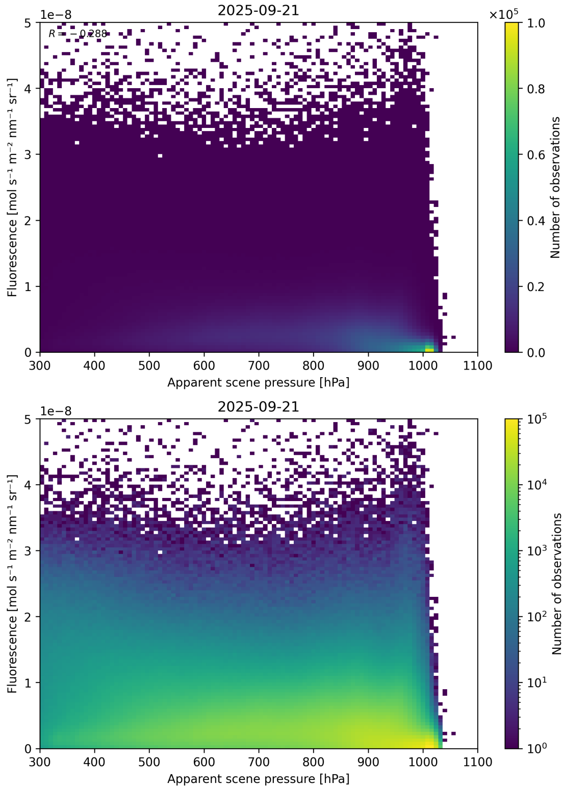
Figure 64: Scatter density plot of “Apparent scene pressure” against “Fluorescence” for 2025-09-20 to 2025-09-22.
