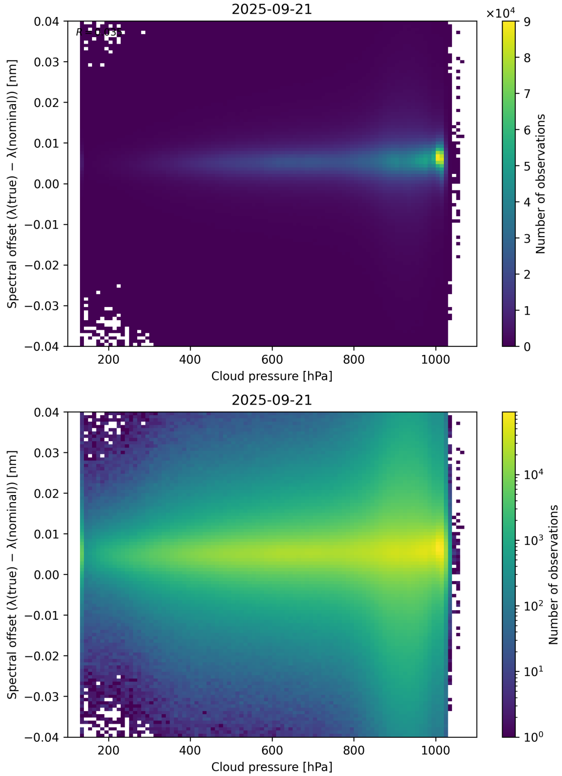
Figure 84: Scatter density plot of “Cloud pressure” against “Spectral offset ( \lambda_{\text{true}} - \lambda_{\text{nominal}} )” for 2025-09-20 to 2025-09-22.
