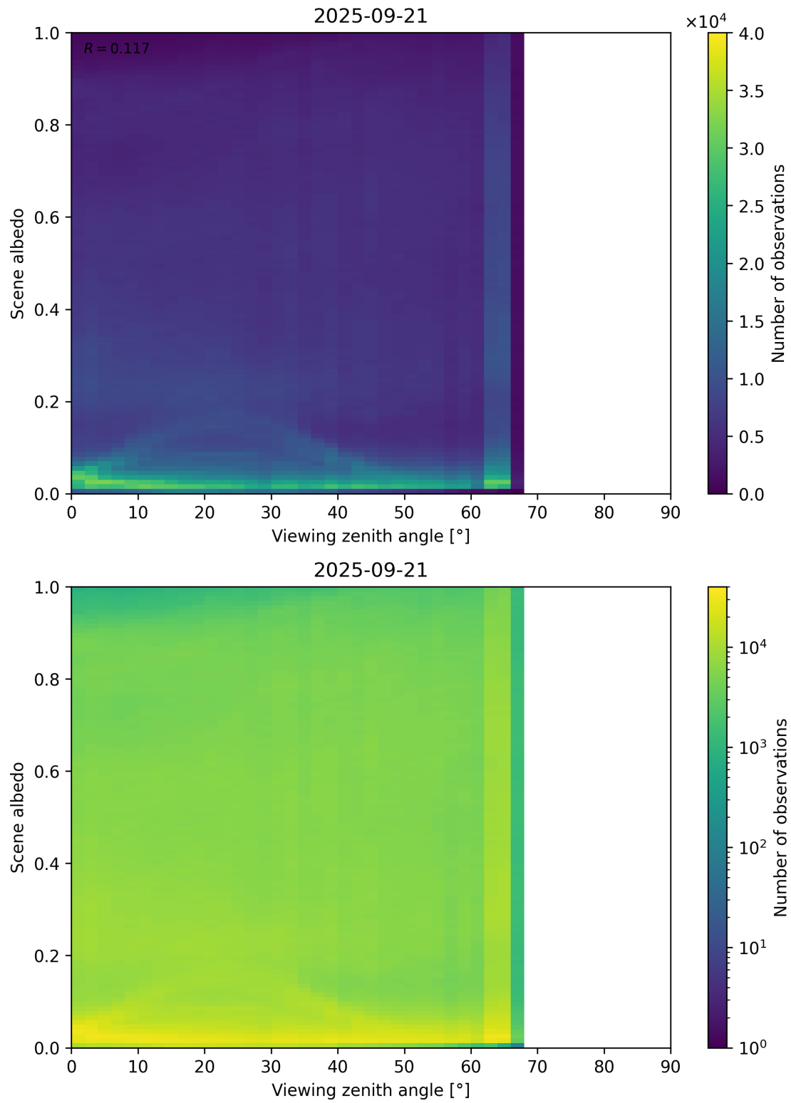
Figure 126: Scatter density plot of “Viewing zenith angle” against “Scene albedo” for 2025-09-20 to 2025-09-22.
