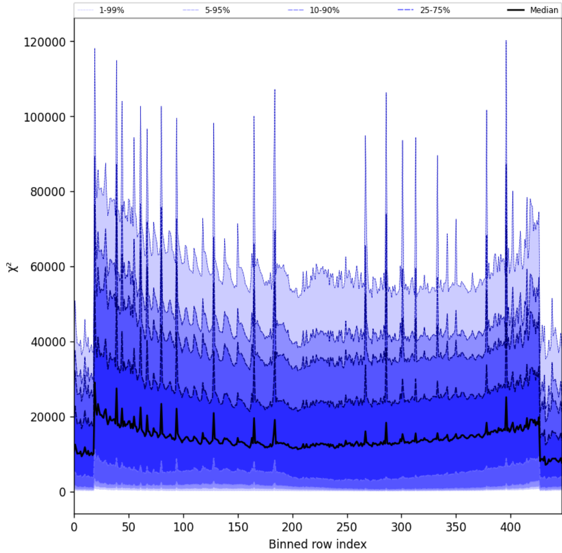
Figure 55: Along track statistics of “ \chi^2 ” for 2025-09-20 to 2025-09-22
