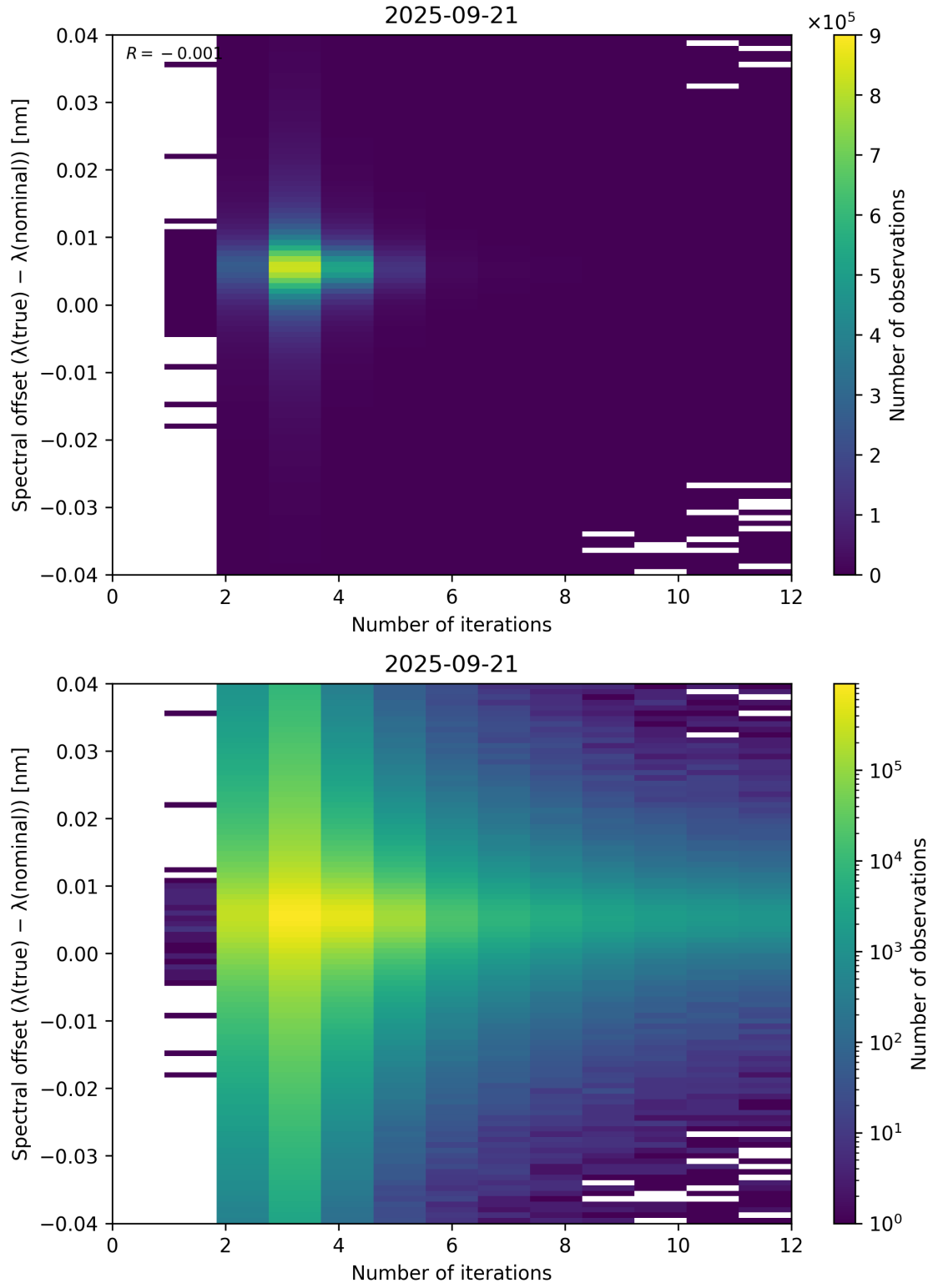
Figure 100: Scatter density plot of “Number of iterations” against “Spectral offset ( \lambda_{\text{true}} - \lambda_{\text{nominal}} )” for 2025-09-20 to 2025-09-22.
