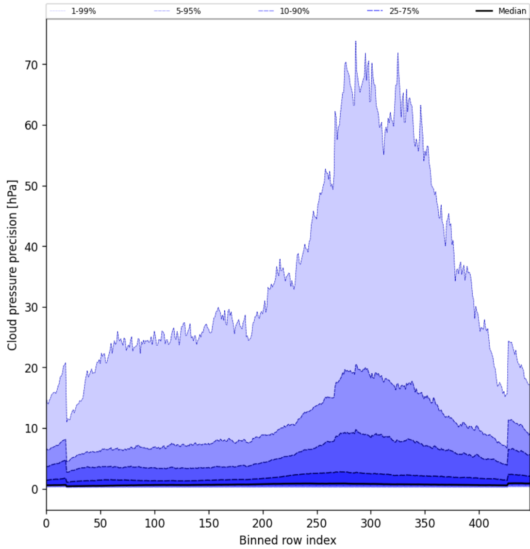
Figure 48: Along track statistics of “Cloud pressure precision” for 2025-09-20 to 2025-09-22
