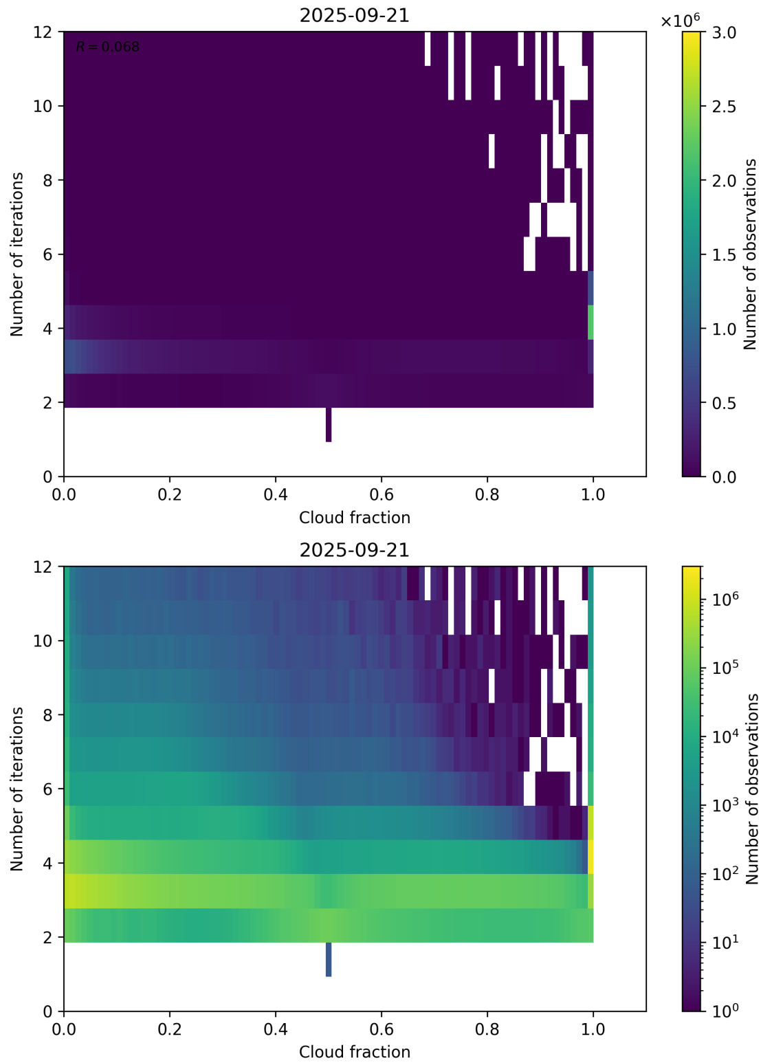
Figure 73: Scatter density plot of “Cloud fraction” against “Number of iterations” for 2025-09-20 to 2025-09-22.
