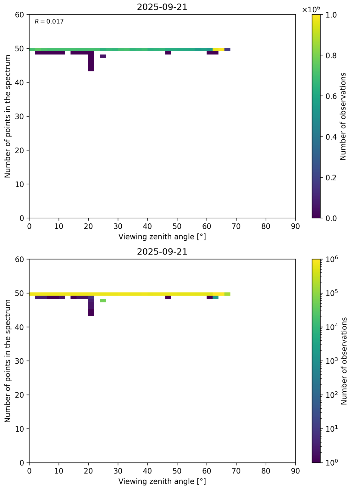
Figure 125: Scatter density plot of “Viewing zenith angle” against “Number of points in the spectrum” for 2025-09-20 to 2025-09-22.
