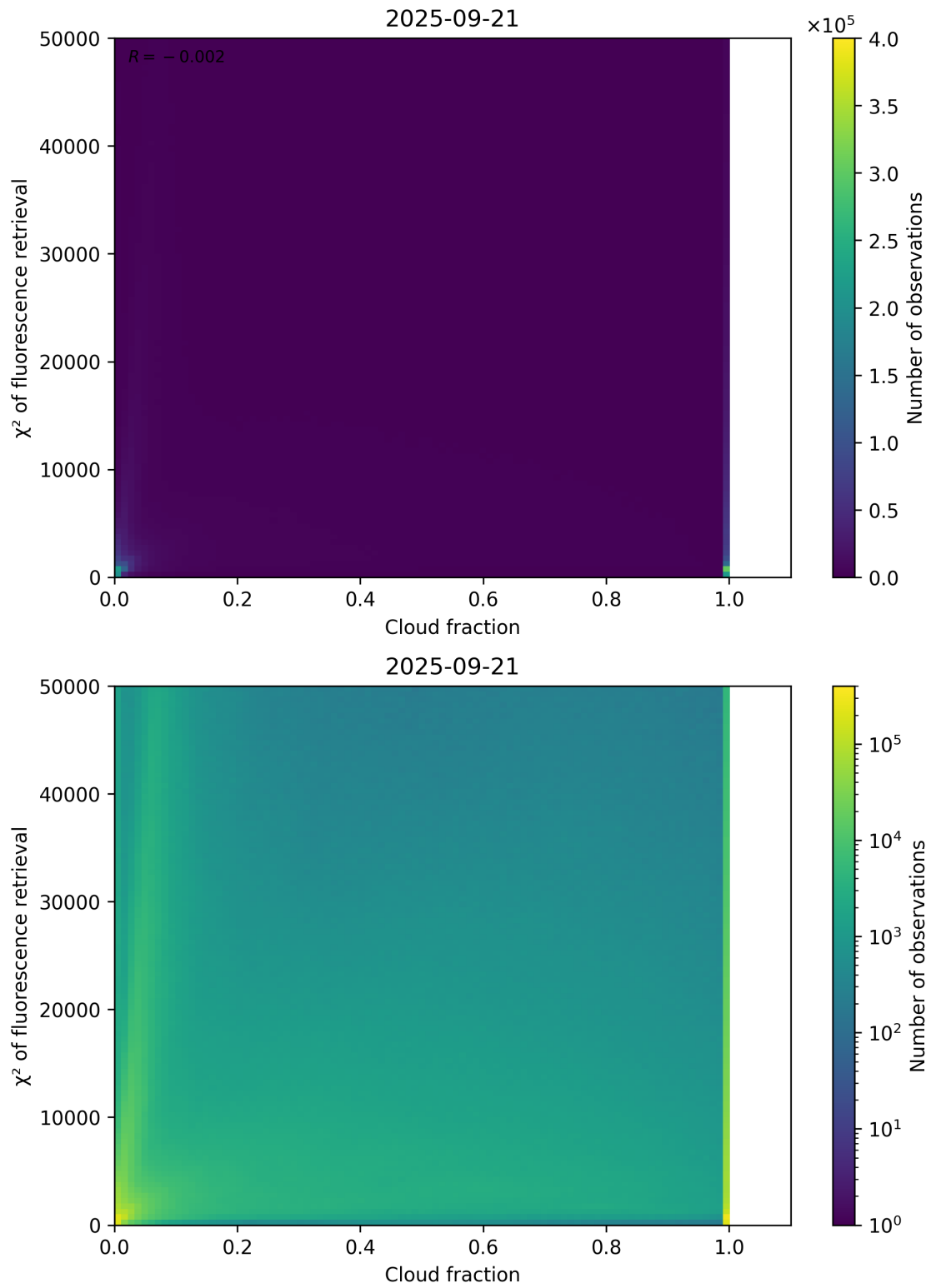
Figure 71: Scatter density plot of “Cloud fraction” against “ \chi^2 of fluorescence retrieval” for 2025-09-20 to 2025-09-22.
