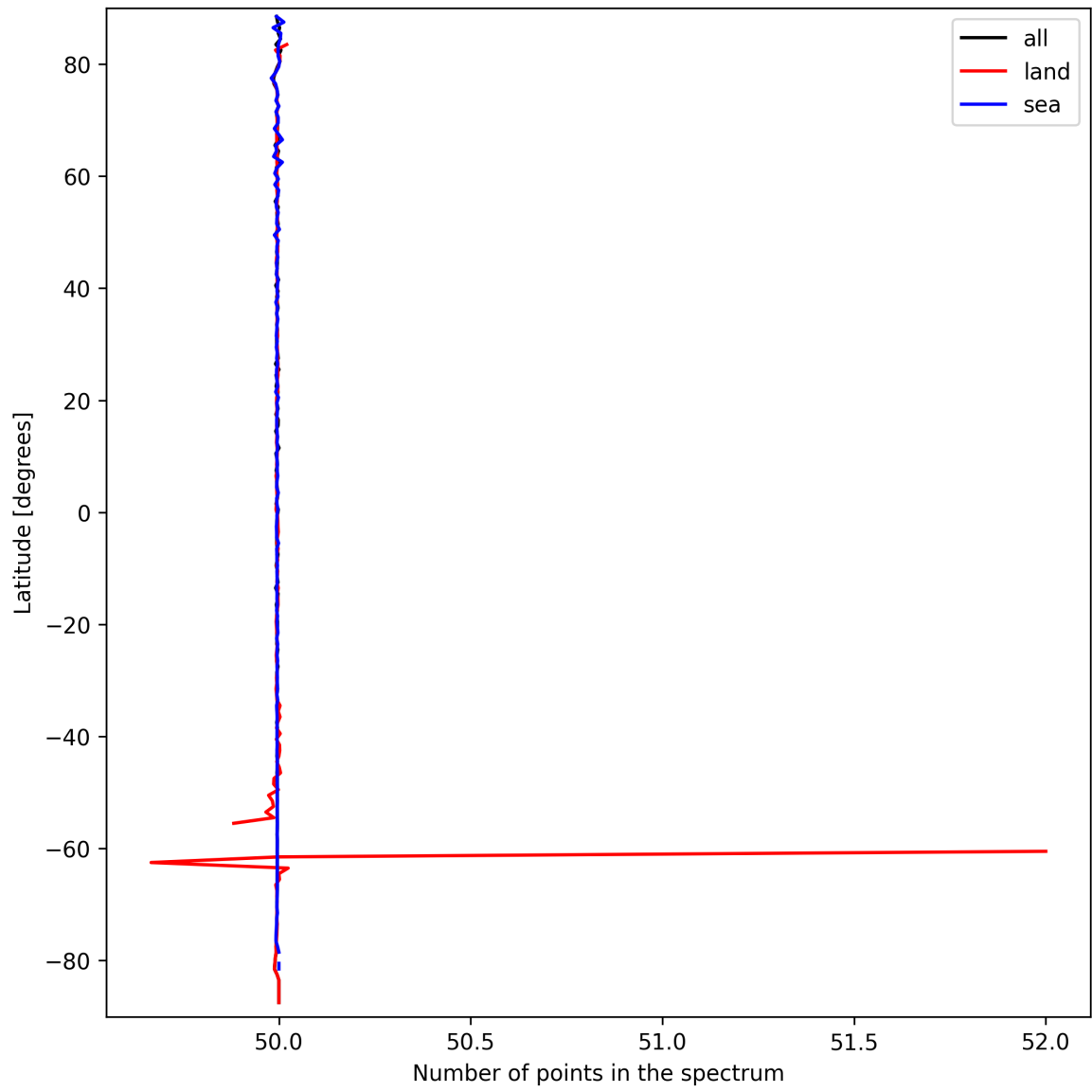
Figure 27: Zonal average of “Number of points in the spectrum” for 2025-09-20 to 2025-09-22.
