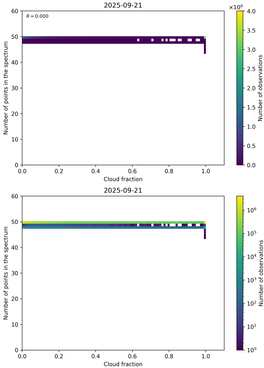
Figure 74: Scatter density plot of “Cloud fraction” against “Number of points in the spectrum” for 2025-09-20 to 2025-09-22.
