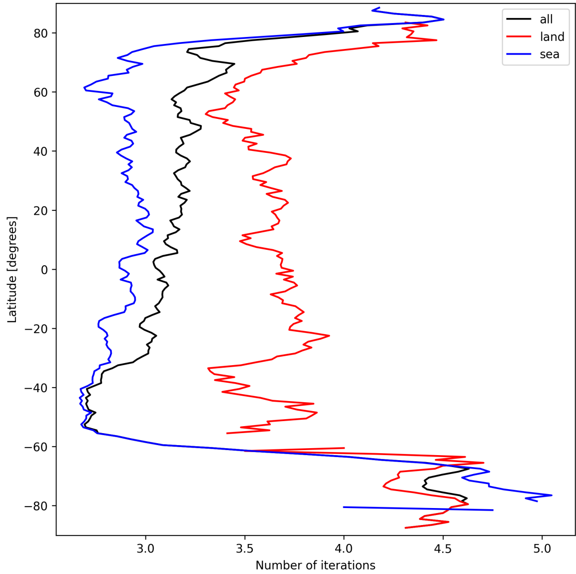
Figure 22: Zonal average of “Number of iterations” for 2025-09-20 to 2025-09-22.
