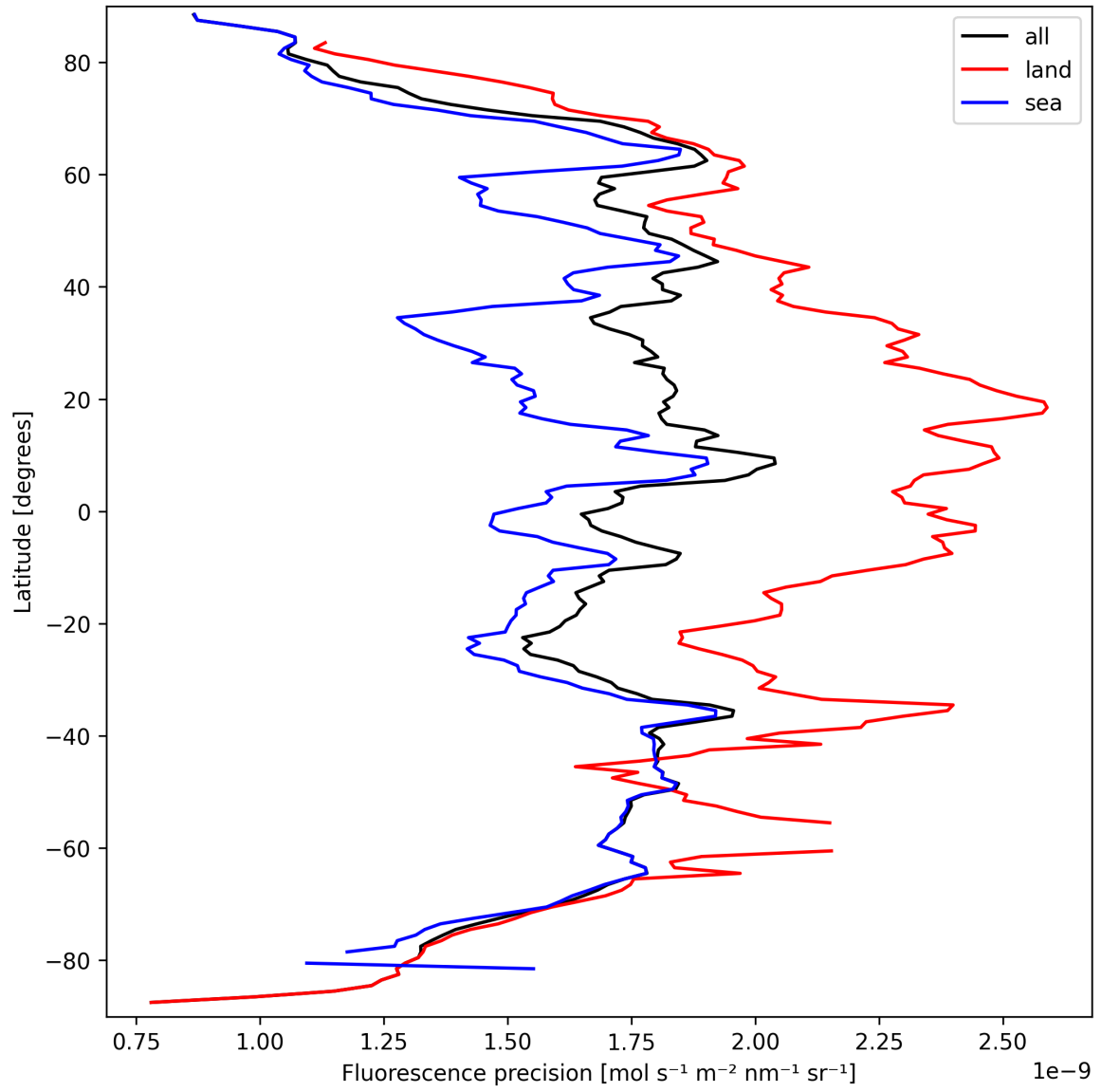
Figure 24: Zonal average of “Fluorescence precision” for 2025-09-20 to 2025-09-22.
