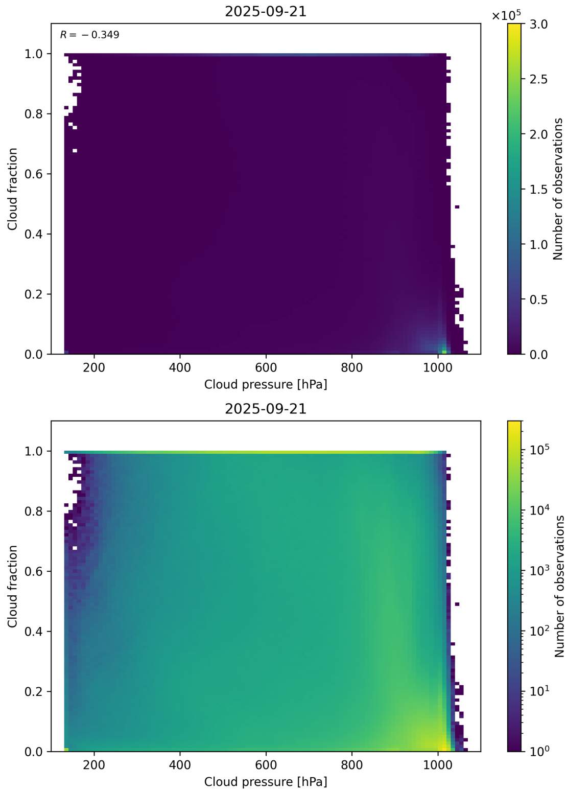
Figure 79: Scatter density plot of “Cloud pressure” against “Cloud fraction” for 2025-09-20 to 2025-09-22.
