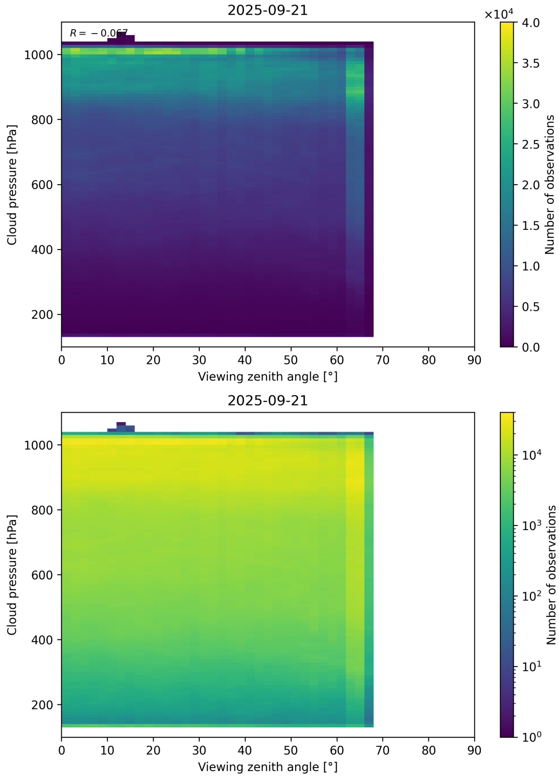
Figure 121: Scatter density plot of “Viewing zenith angle” against “Cloud pressure” for 2025-09-20 to 2025-09-22.
