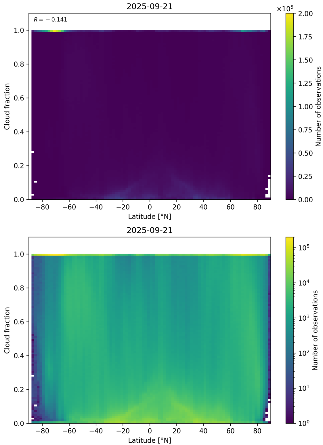
Figure 90: Scatter density plot of “Latitude” against “Cloud fraction” for 2025-09-20 to 2025-09-22.
