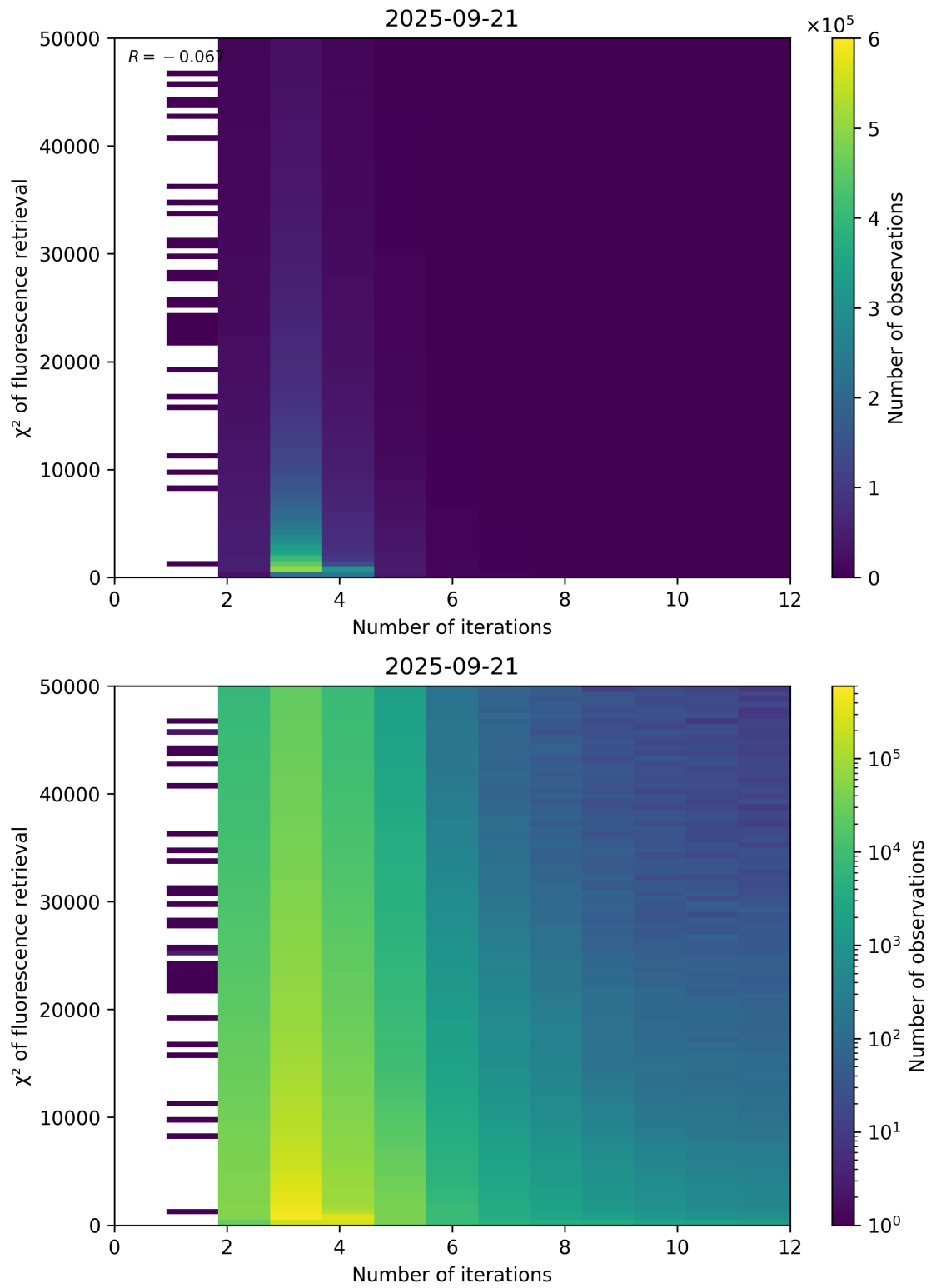
Figure 97: Scatter density plot of “Number of iterations” against “ \chi^2 of fluorescence retrieval” for 2025-09-20 to 2025-09-22.
