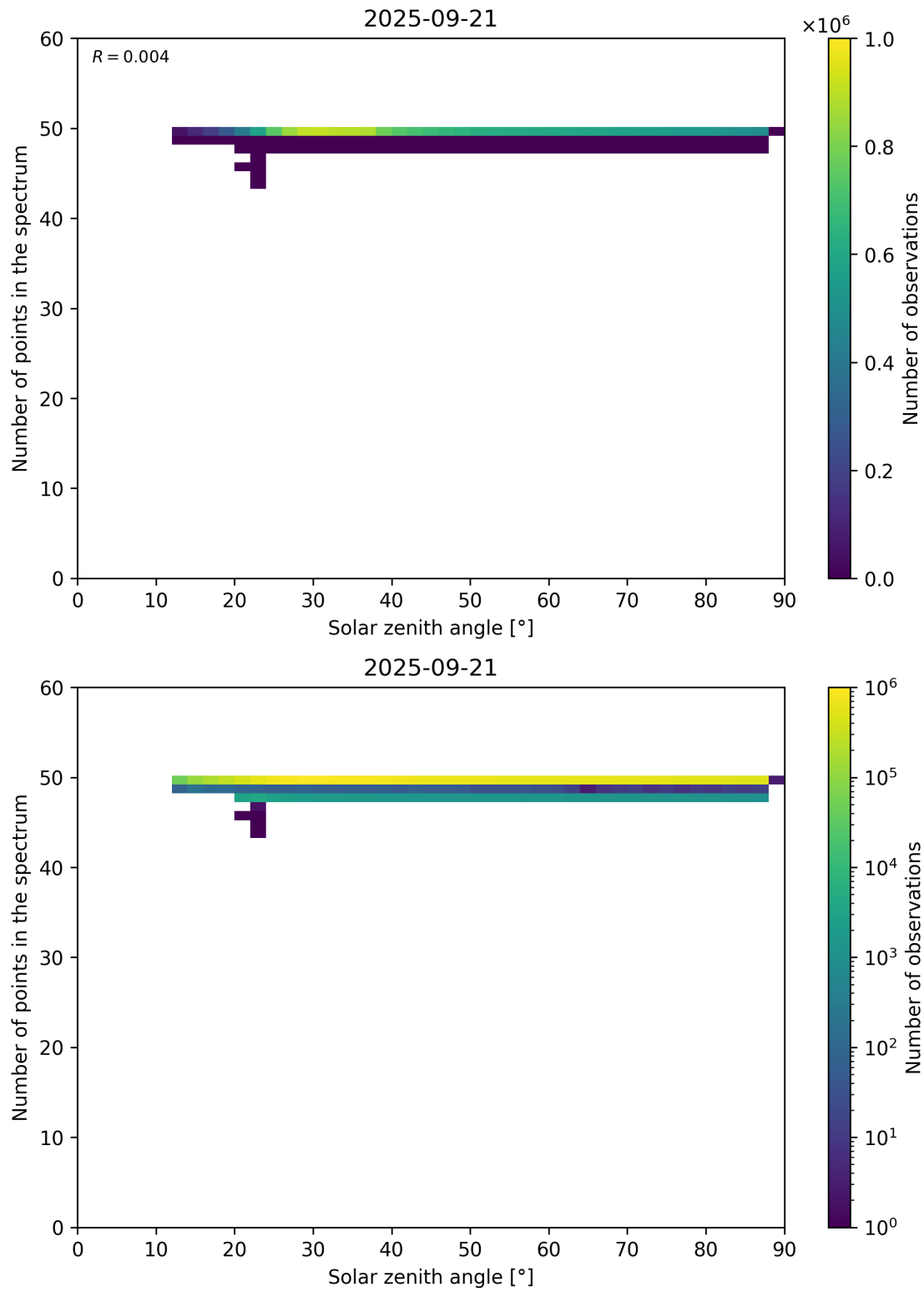
Figure 115: Scatter density plot of “Solar zenith angle” against “Number of points in the spectrum” for 2025-09-20 to 2025-09-22.
