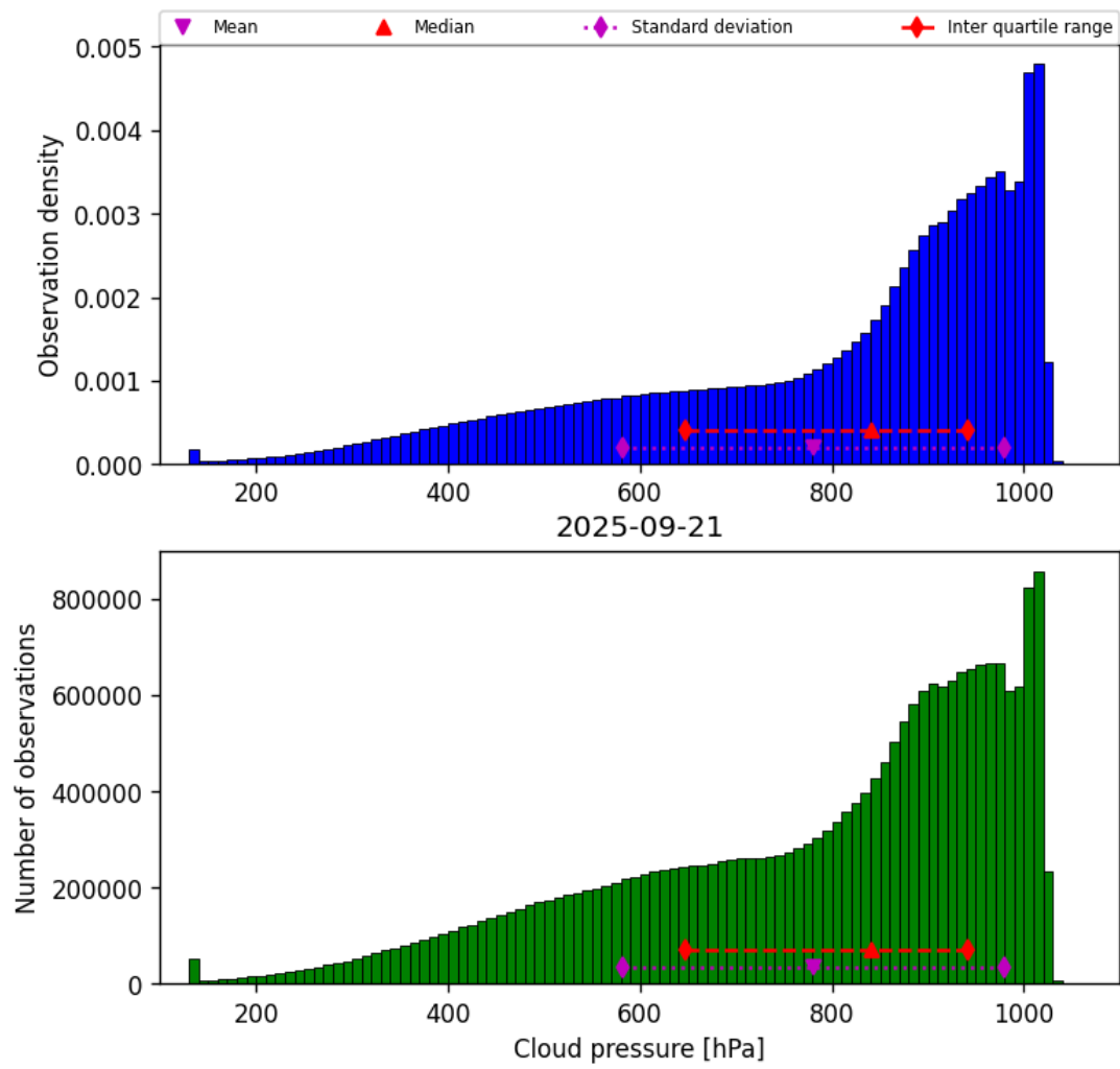
Figure 30: Histogram of “Cloud pressure” for 2025-09-20 to 2025-09-22
