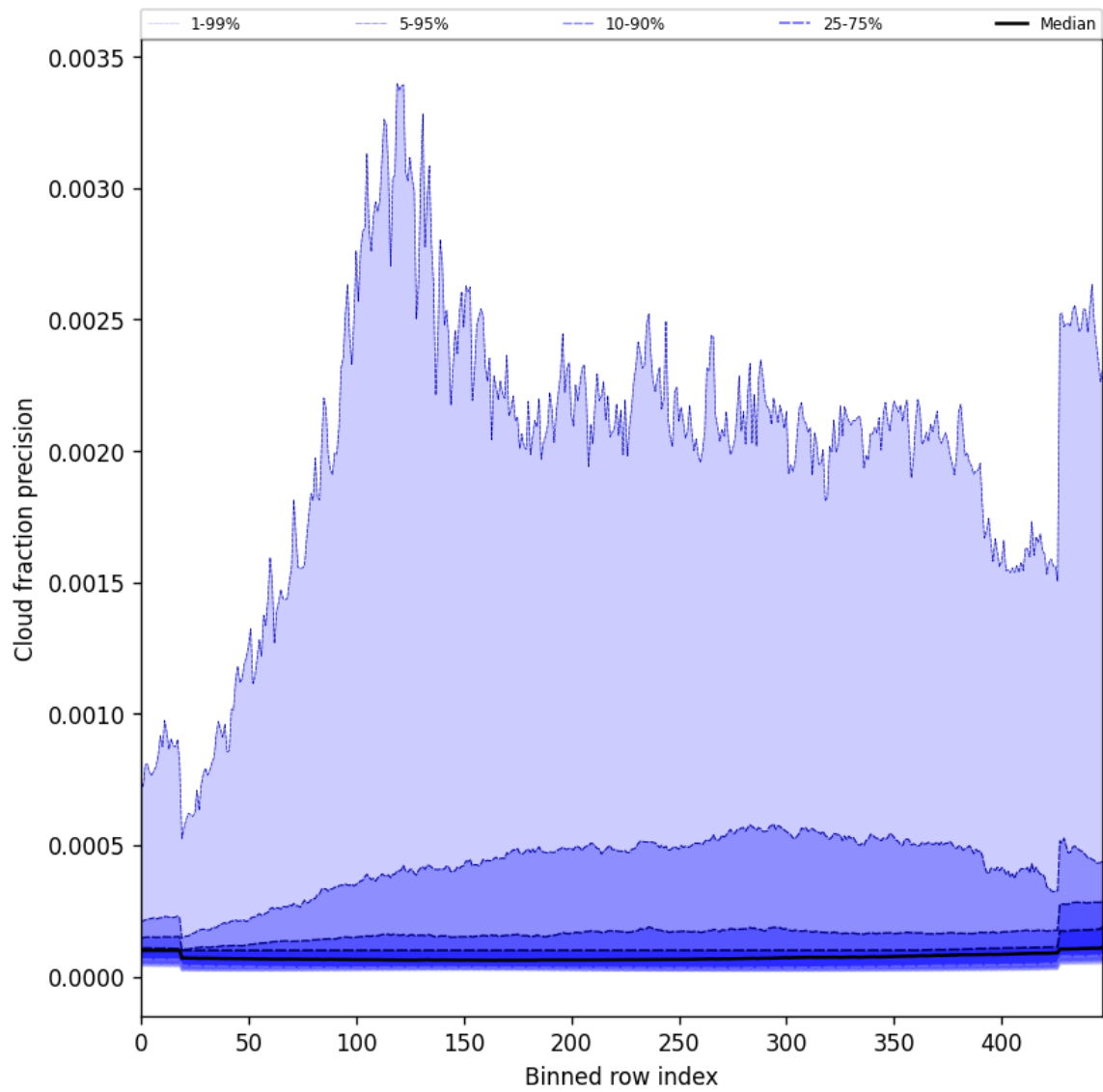
Figure 50: Along track statistics of “Cloud fraction precision” for 2025-09-20 to 2025-09-22
