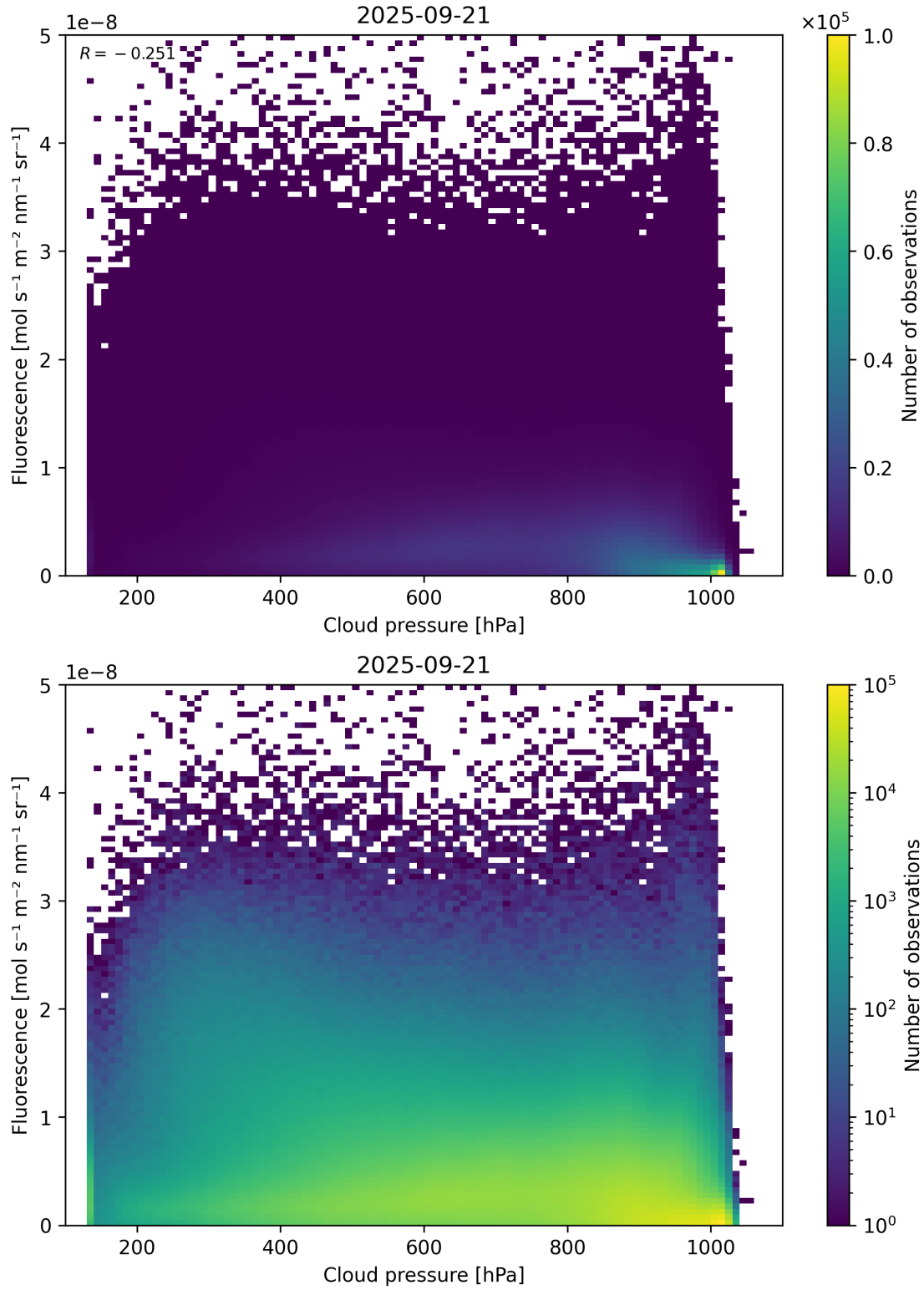
Figure 80: Scatter density plot of “Cloud pressure” against “Fluorescence” for 2025-09-20 to 2025-09-22.
