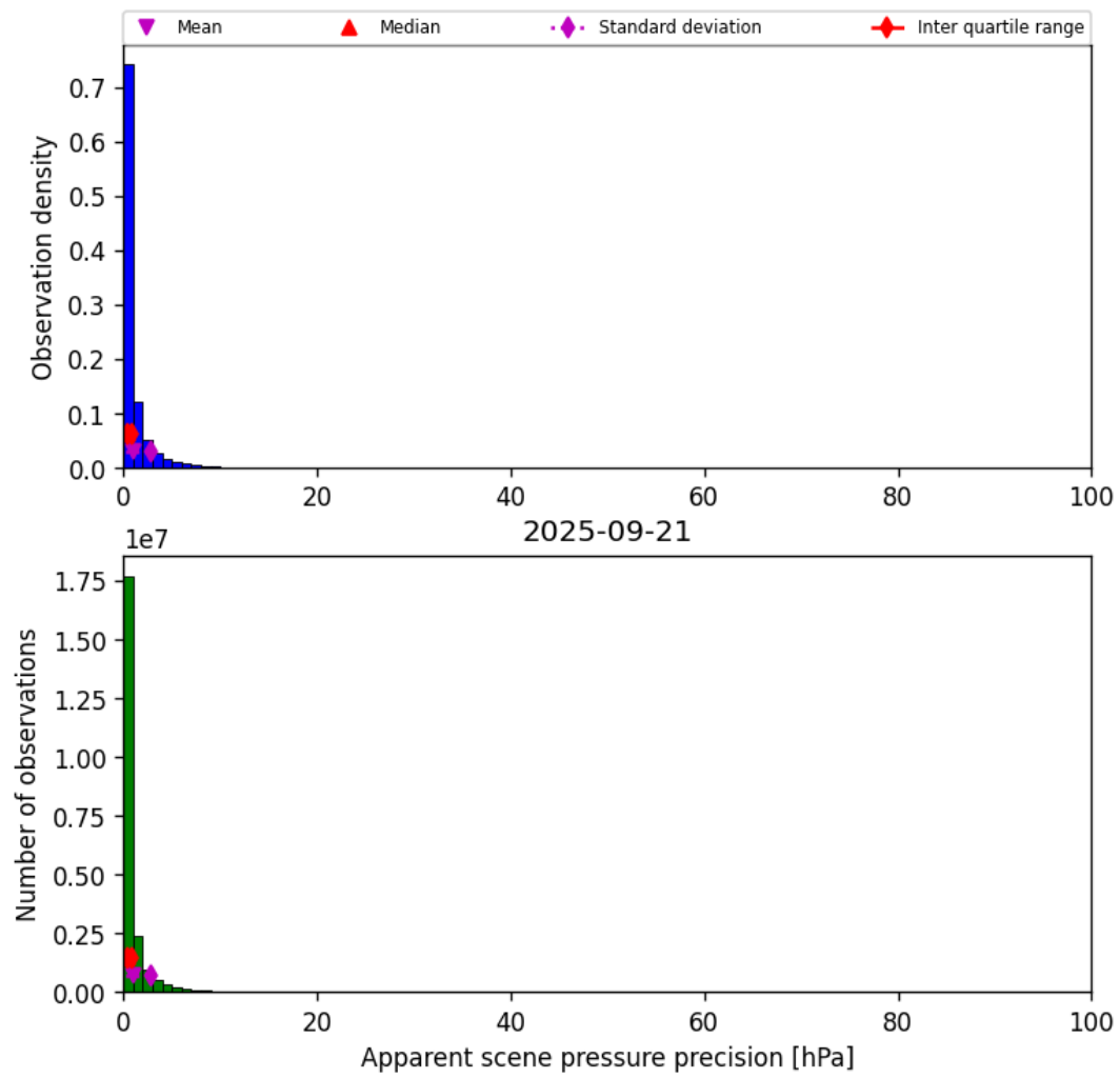
Figure 37: Histogram of “Apparent scene pressure precision” for 2025-09-20 to 2025-09-22
