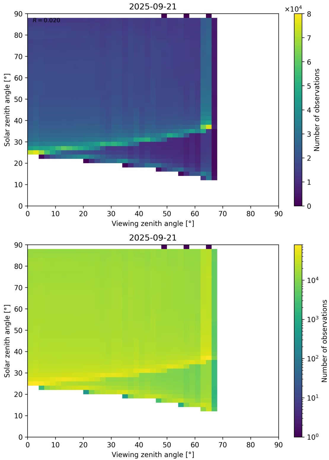
Figure 127: Scatter density plot of “Viewing zenith angle” against “Solar zenith angle” for 2025-09-20 to 2025-09-22.
