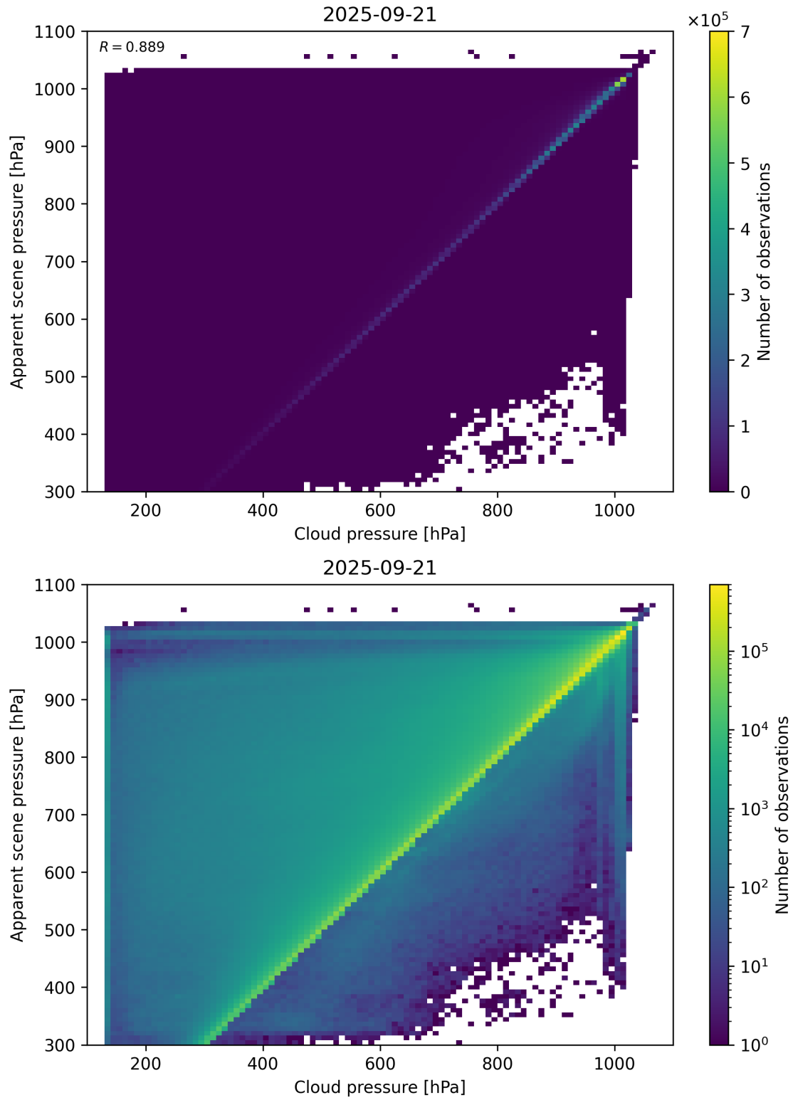
Figure 77: Scatter density plot of “Cloud pressure” against “Apparent scene pressure” for 2025-09-20 to 2025-09-22.
