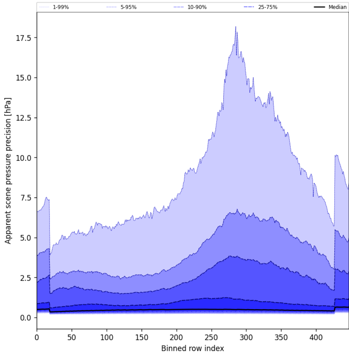
Figure 54: Along track statistics of “Apparent scene pressure precision” for 2025-09-20 to 2025-09-22
