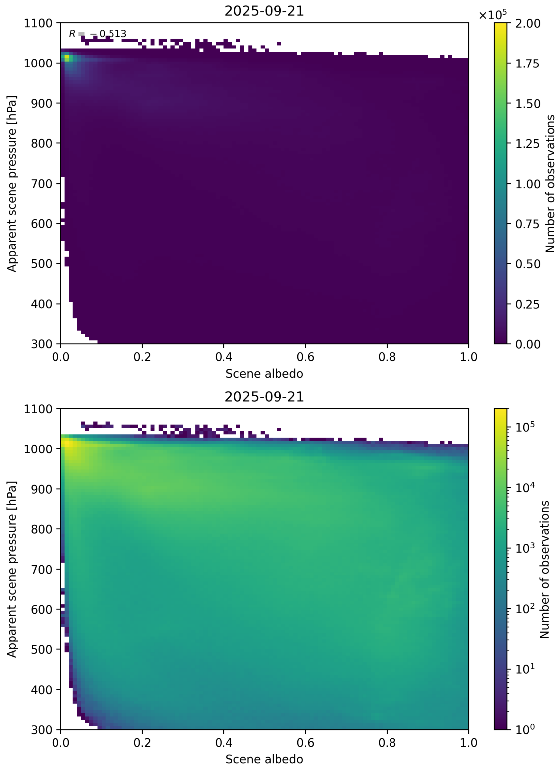
Figure 102: Scatter density plot of “Scene albedo” against “Apparent scene pressure” for 2025-09-20 to 2025-09-22.
