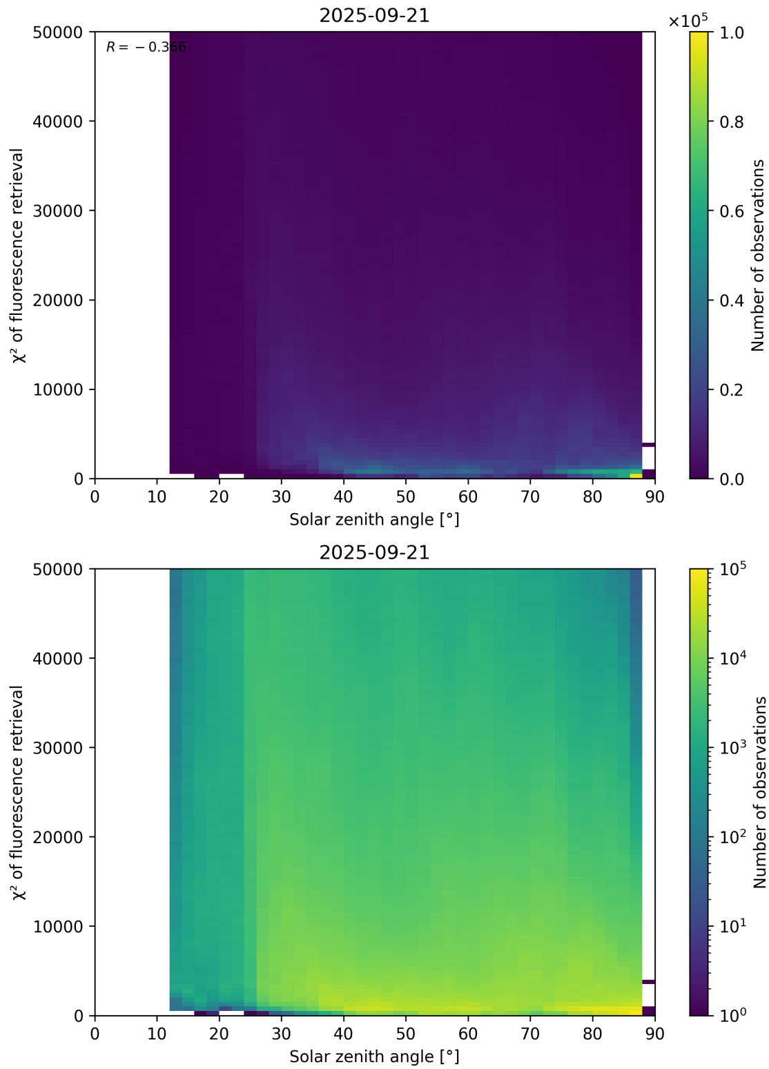
Figure 109: Scatter density plot of “Solar zenith angle” against “ \chi^2 of fluorescence retrieval” for 2025-09-20 to 2025-09-22.
