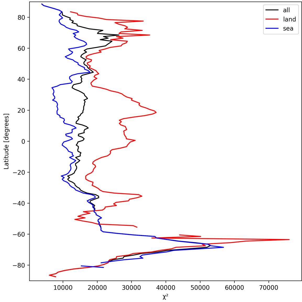
Figure 21: Zonal average of “ \chi^2 ” for 2025-09-20 to 2025-09-22.
