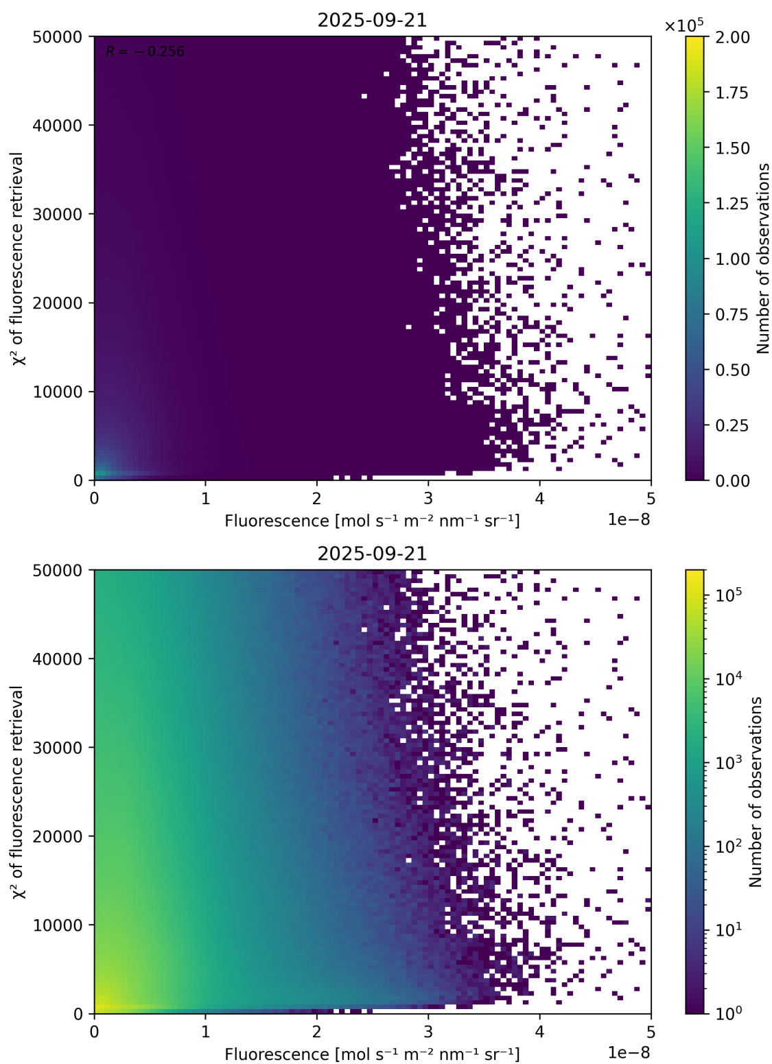
Figure 85: Scatter density plot of “Fluorescence” against “ \chi^2 of fluorescence retrieval” for 2025-09-20 to 2025-09-22.
