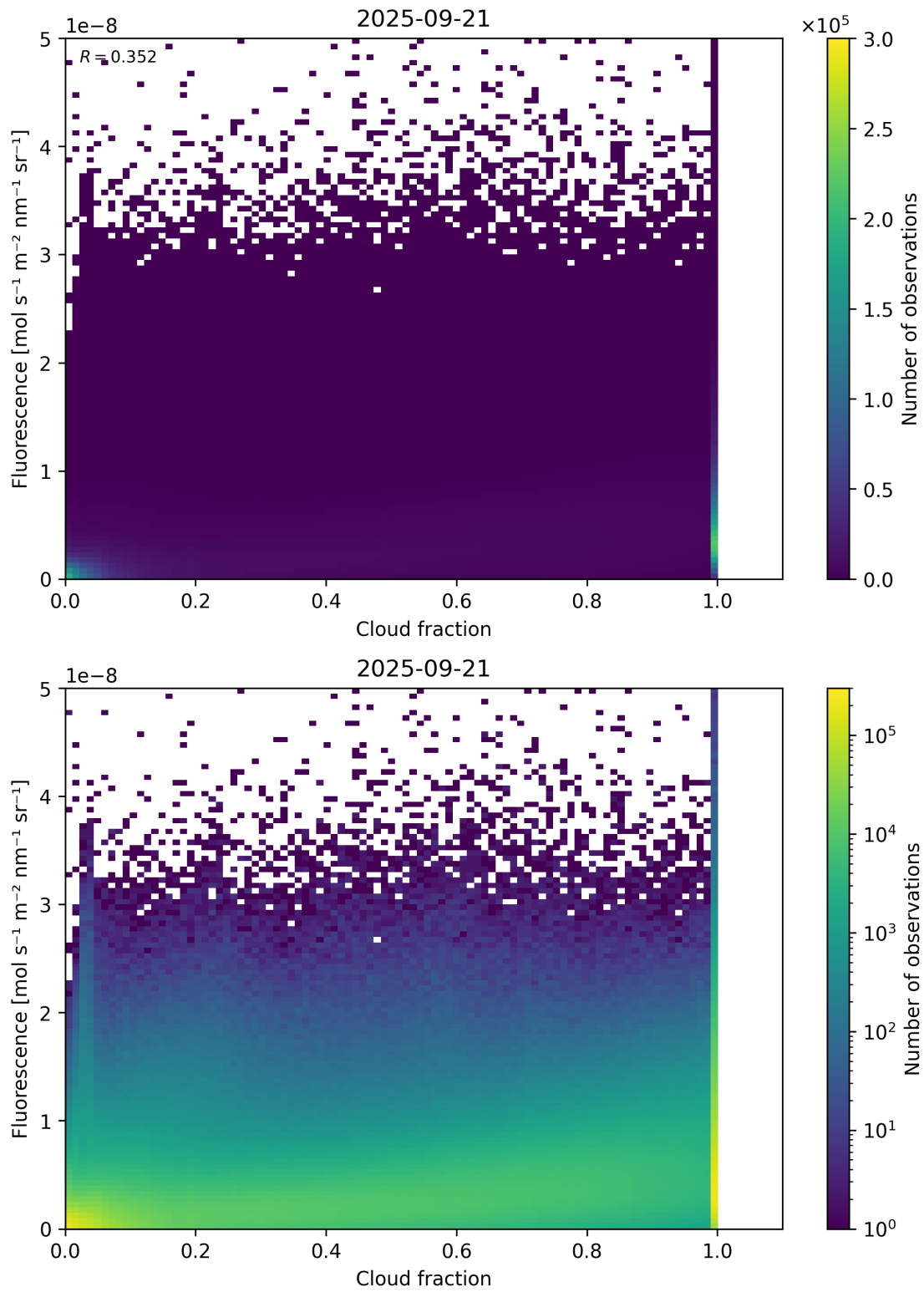
Figure 72: Scatter density plot of “Cloud fraction” against “Fluorescence” for 2025-09-20 to 2025-09-22.
