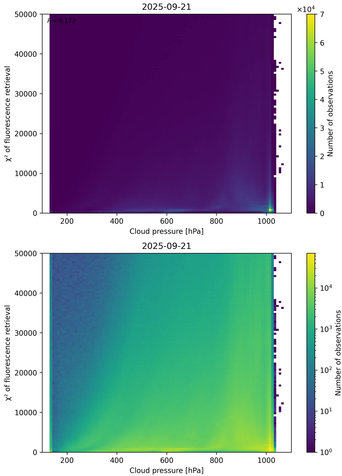
Figure 78: Scatter density plot of “Cloud pressure” against “ \chi^2 of fluorescence retrieval” for 2025-09-20 to 2025-09-22.
