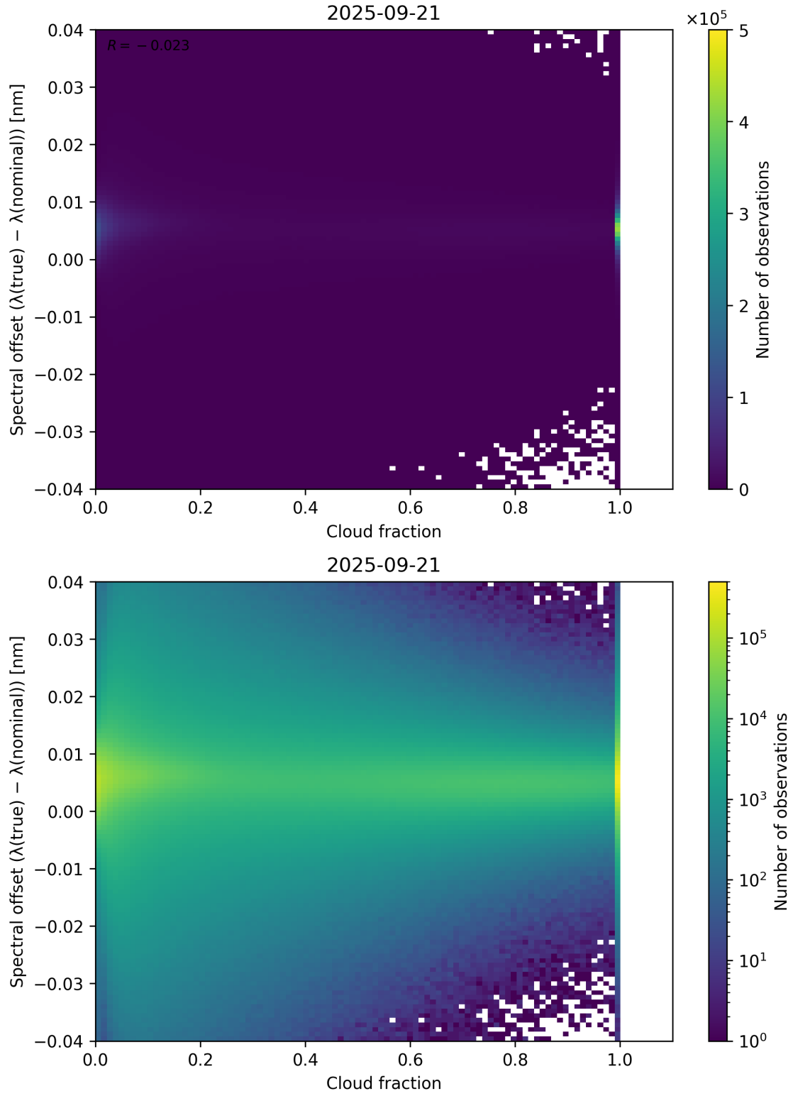
Figure 76: Scatter density plot of “Cloud fraction” against “Spectral offset ( \lambda_{\text{true}} - \lambda_{\text{nominal}} )” for 2025-09-20 to 2025-09-22.
