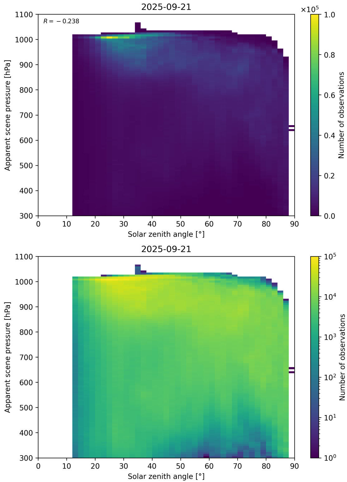
Figure 108: Scatter density plot of “Solar zenith angle” against “Apparent scene pressure” for 2025-09-20 to 2025-09-22.
