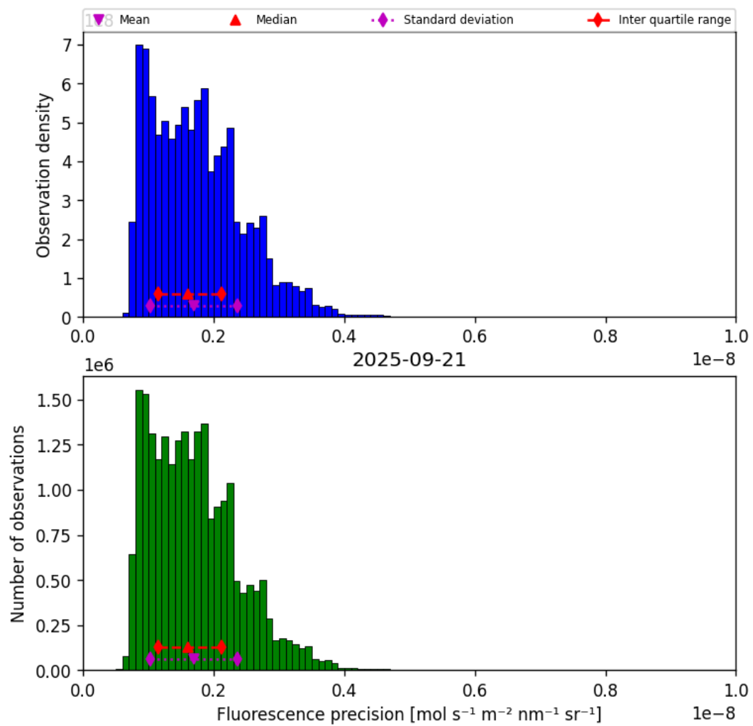
Figure 41: Histogram of “Fluorescence precision” for 2025-09-20 to 2025-09-22
