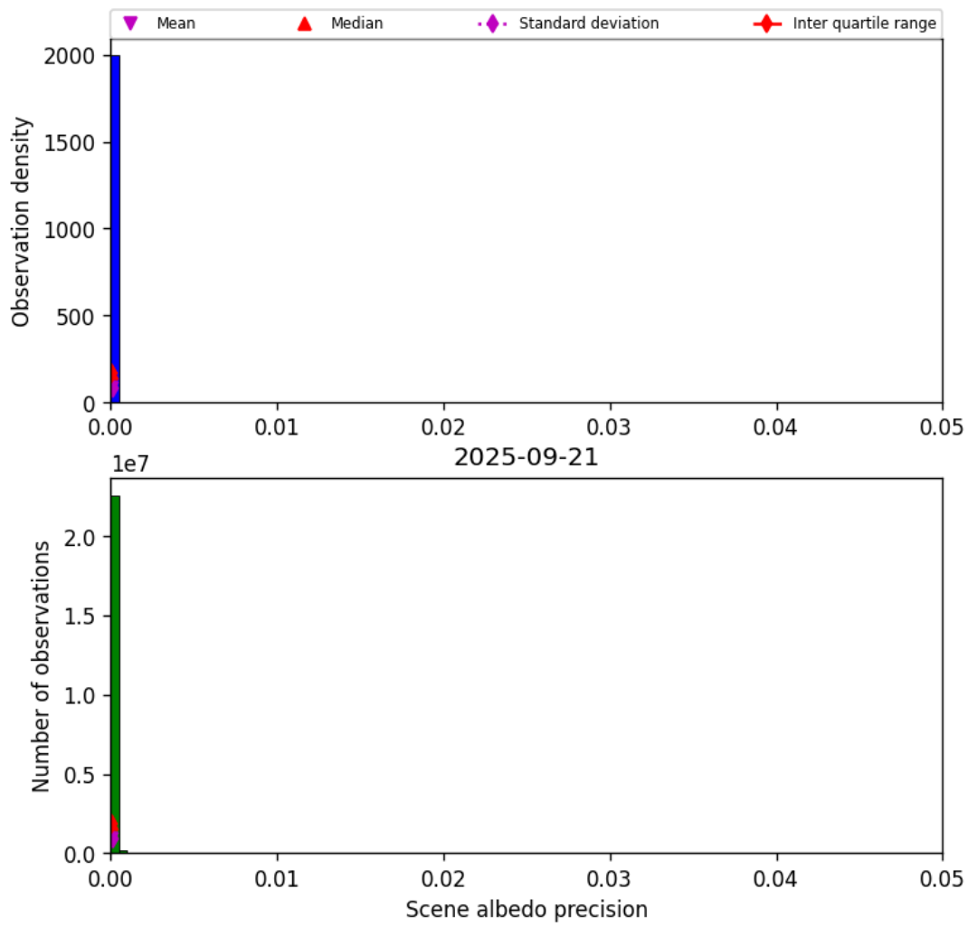
Figure 35: Histogram of “Scene albedo precision” for 2025-09-20 to 2025-09-22
