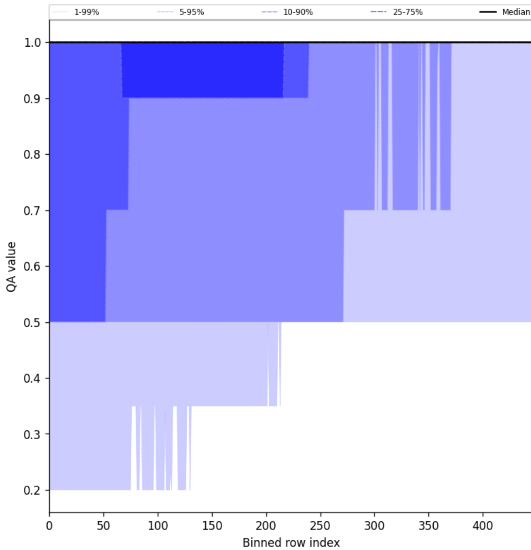
Figure 46: Along track statistics of “QA value” for 2025-09-20 to 2025-09-22
