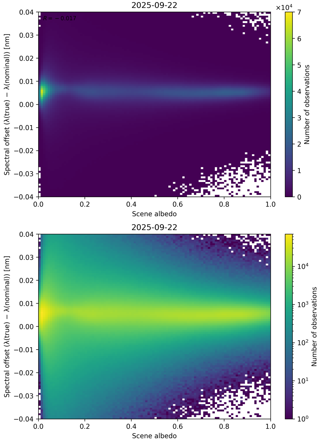
Figure 107: Scatter density plot of “Scene albedo” against “Spectral offset ( \lambda_{\text{true}} - \lambda_{\text{nominal}} )” for 2025-09-22 to 2025-09-23.
