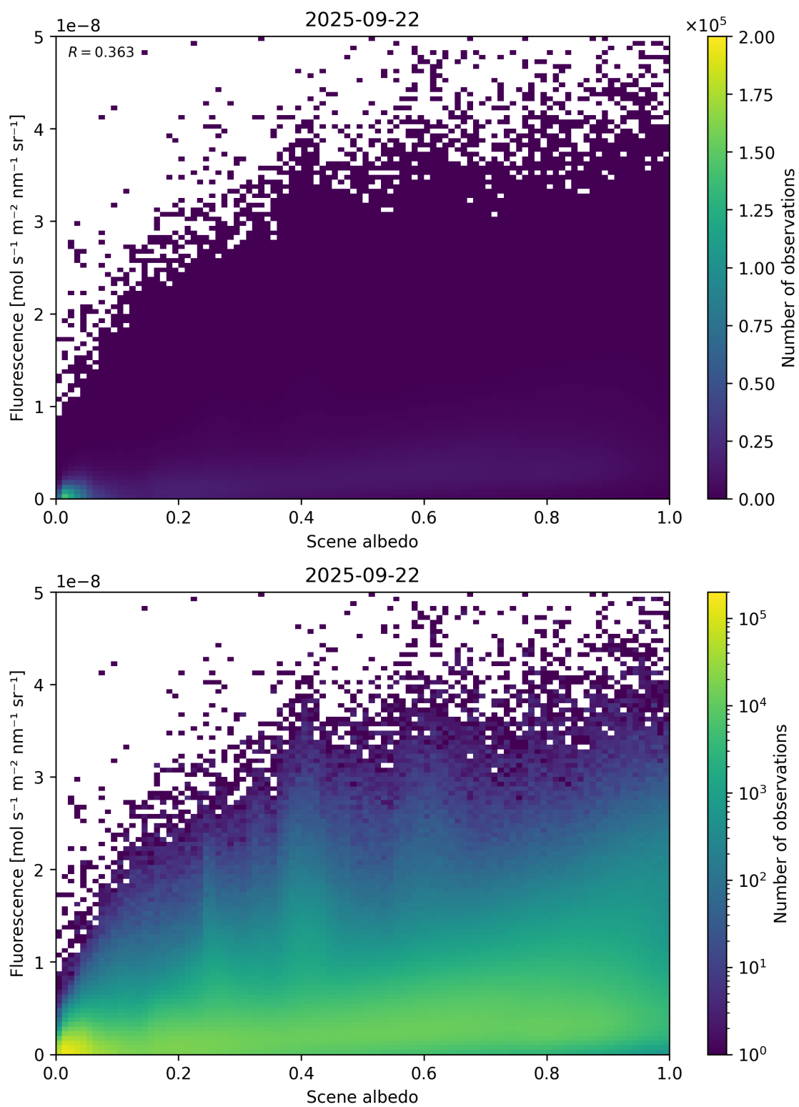
Figure 104: Scatter density plot of “Scene albedo” against “Fluorescence” for 2025-09-22 to 2025-09-23.
