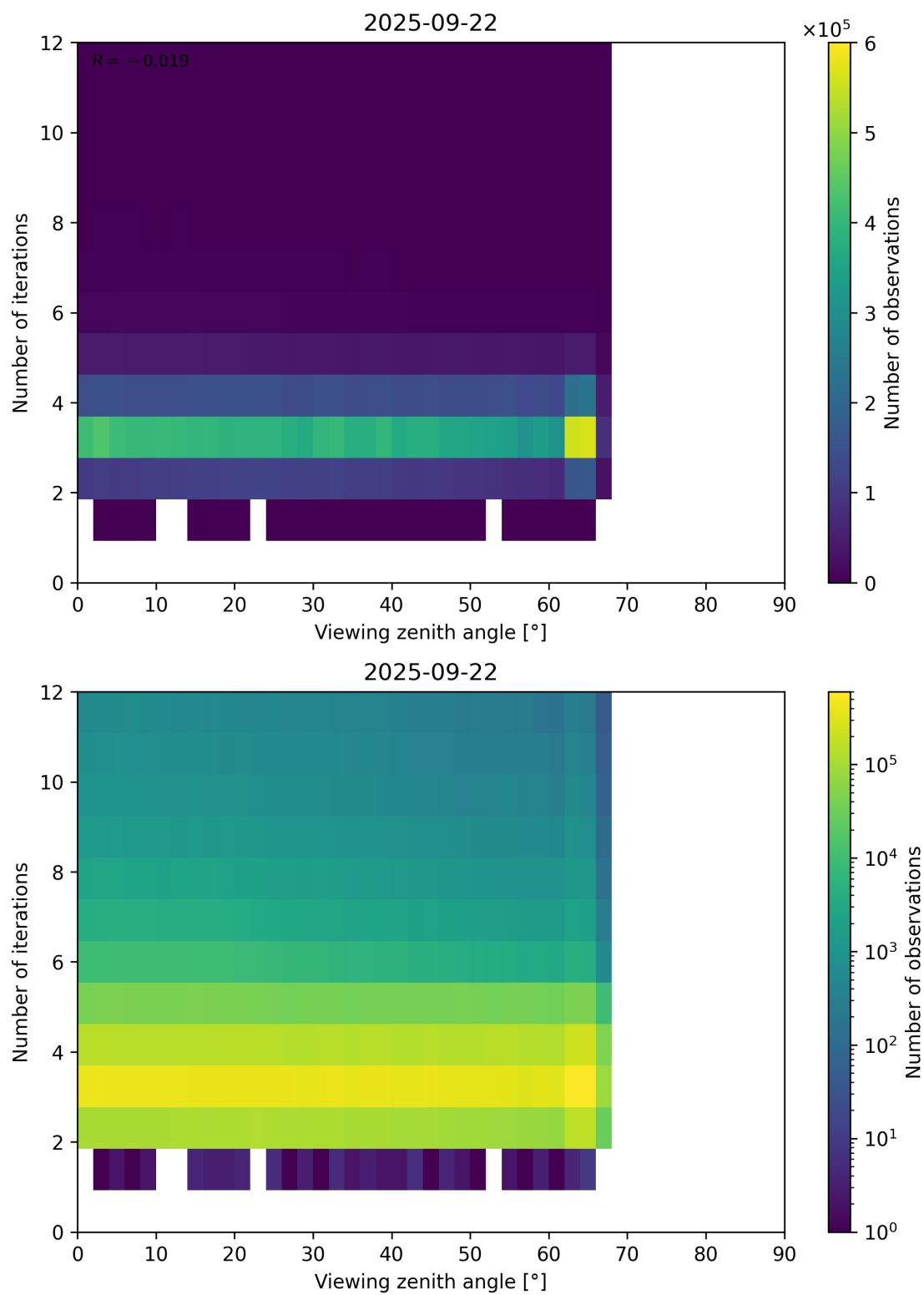
Figure 124: Scatter density plot of “Viewing zenith angle” against “Number of iterations” for 2025-09-22 to 2025-09-23.
