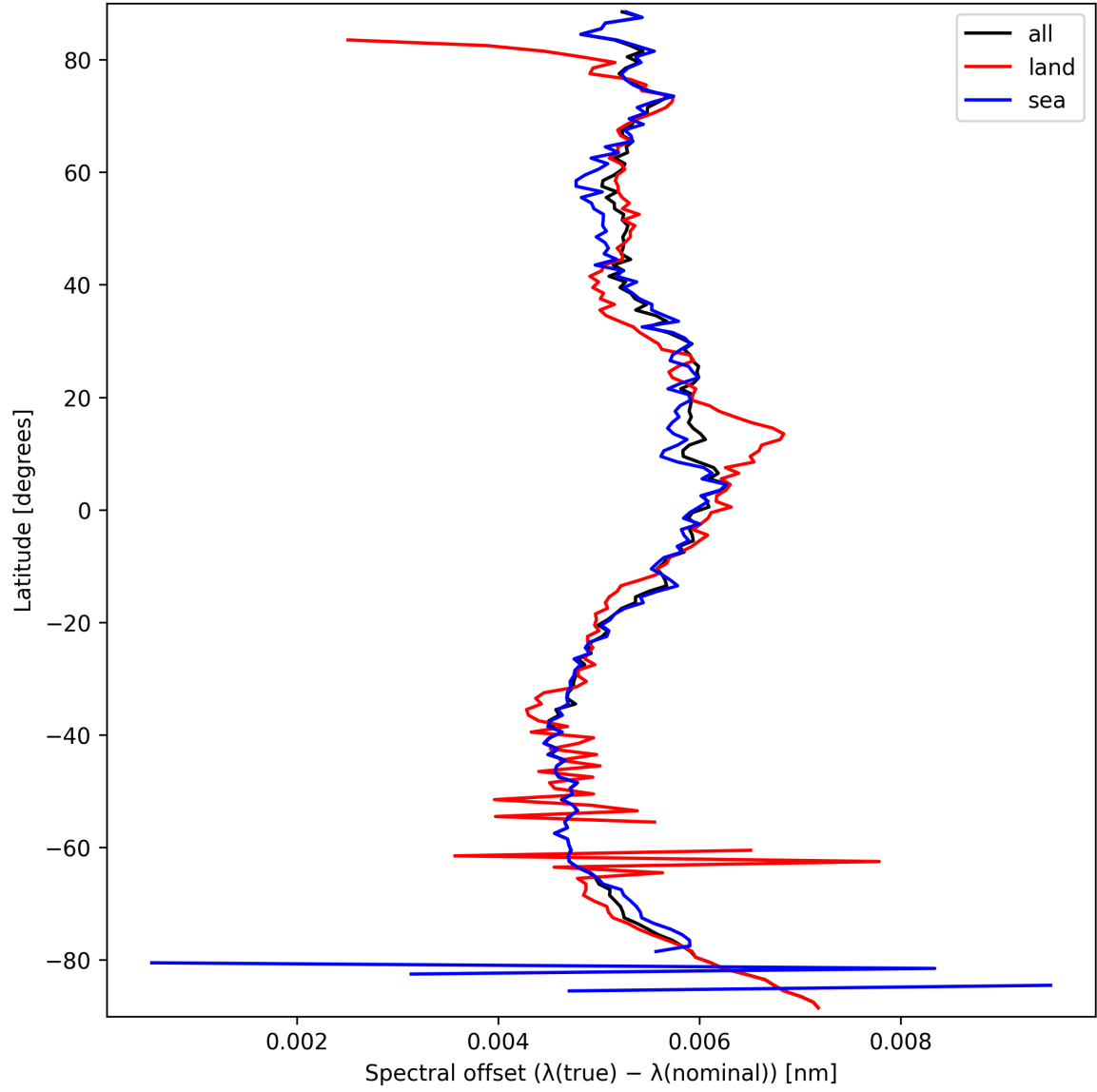
Figure 28: Zonal average of “Spectral offset ( \lambda_{\text{true}} - \lambda_{\text{nominal}} )” for 2025-09-22 to 2025-09-23.
