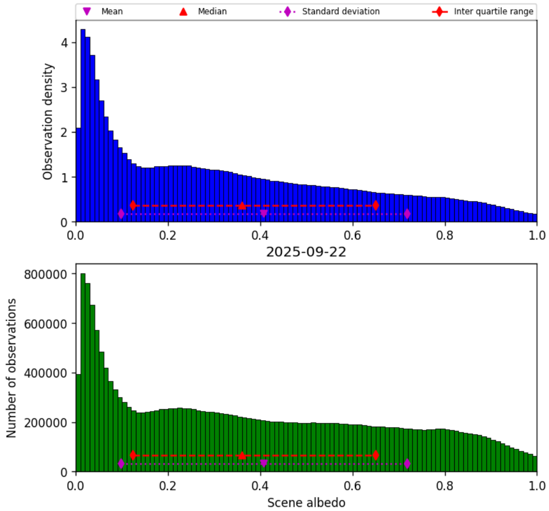
Figure 34: Histogram of “Scene albedo” for 2025-09-22 to 2025-09-23
