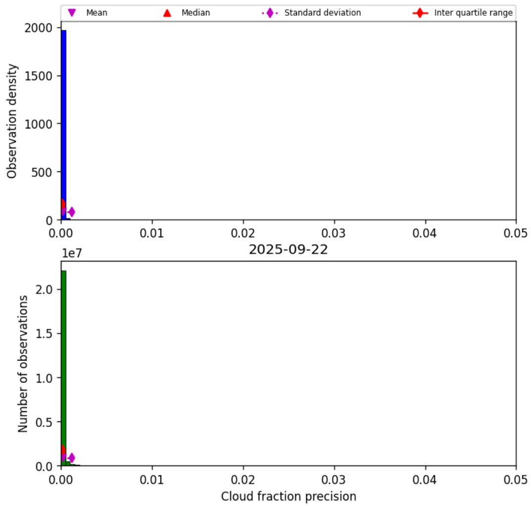
Figure 33: Histogram of “Cloud fraction precision” for 2025-09-22 to 2025-09-23
