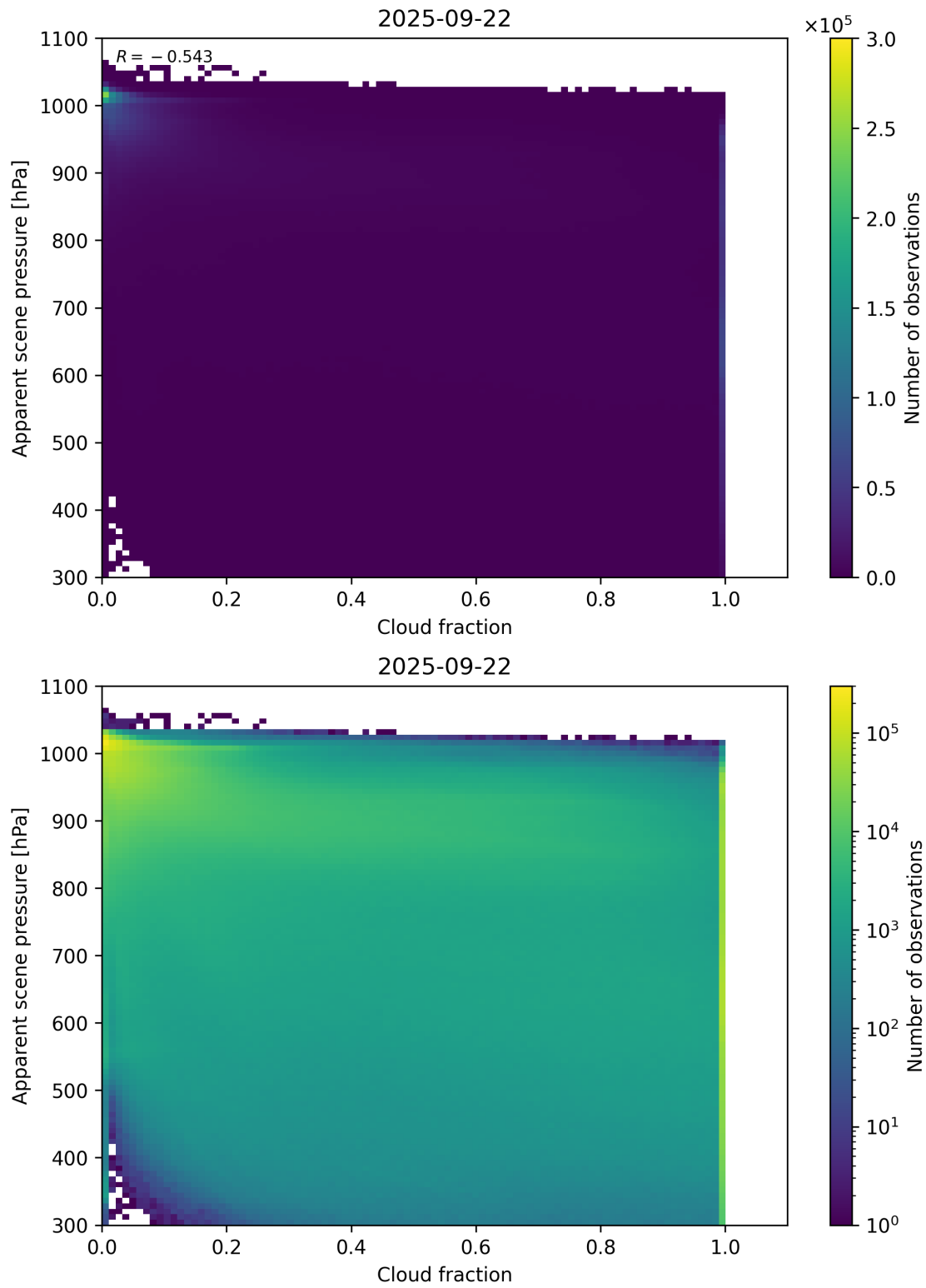
Figure 70: Scatter density plot of “Cloud fraction” against “Apparent scene pressure” for 2025-09-22 to 2025-09-23.
