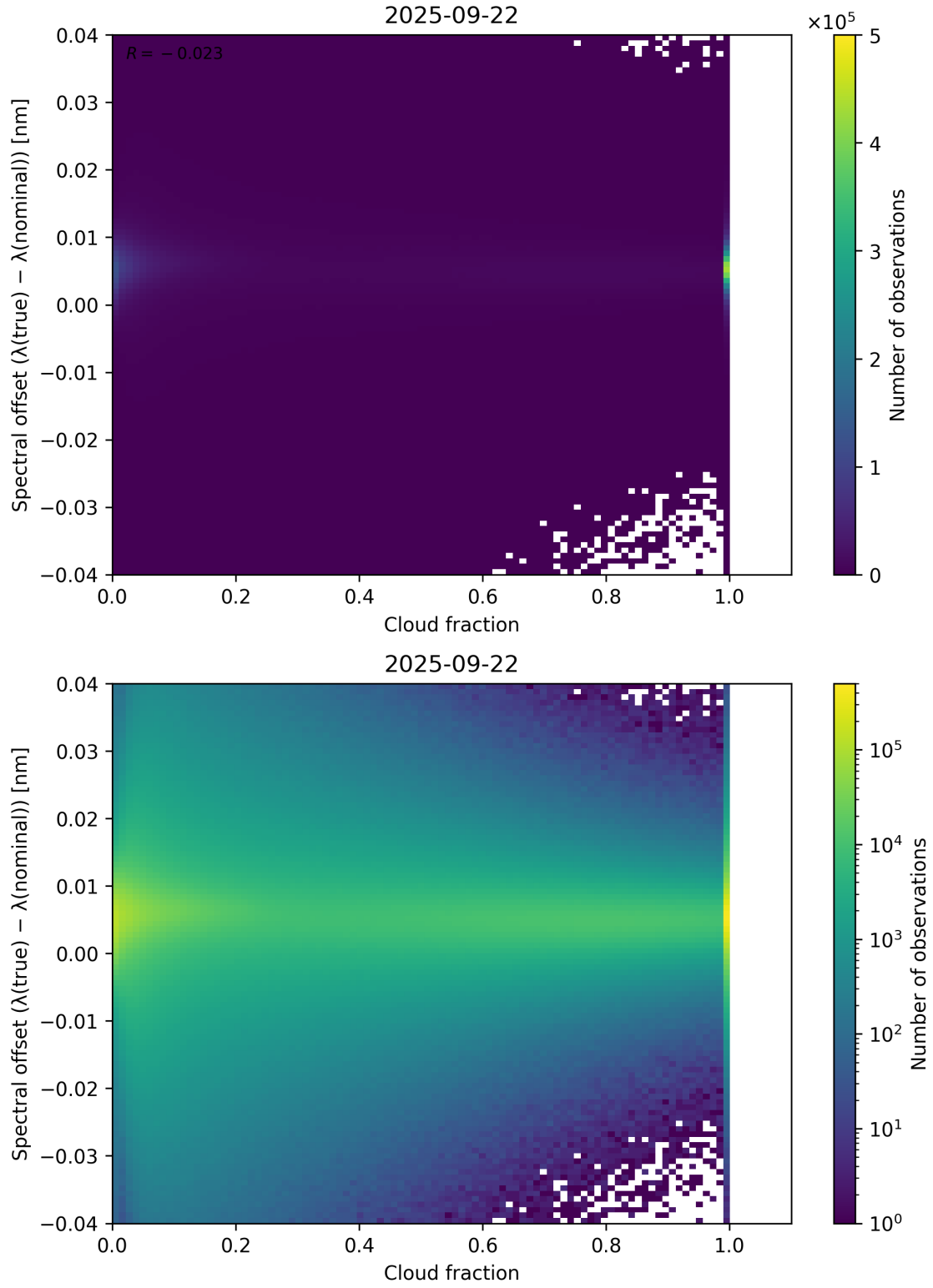
Figure 76: Scatter density plot of “Cloud fraction” against “Spectral offset ( \lambda_{\text{true}} - \lambda_{\text{nominal}} )” for 2025-09-22 to 2025-09-23.
