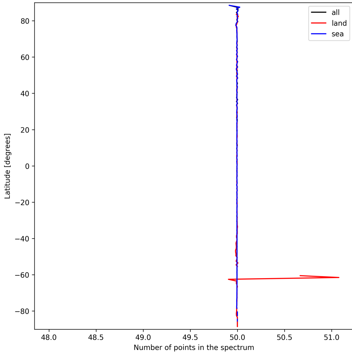
Figure 27: Zonal average of “Number of points in the spectrum” for 2025-09-22 to 2025-09-23.
