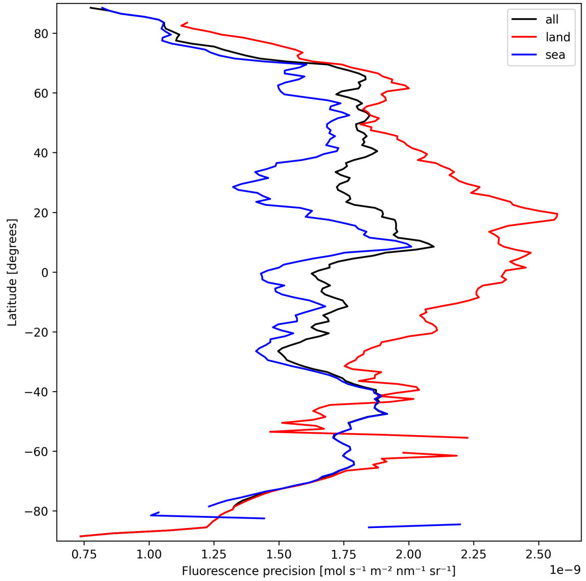
Figure 24: Zonal average of “Fluorescence precision” for 2025-09-22 to 2025-09-23.
