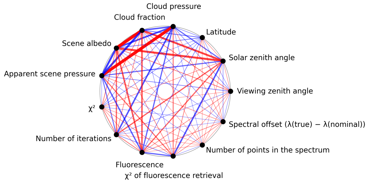
Figure 1: Map of correlation graph for 2025-09-22 to 2025-09-23.
