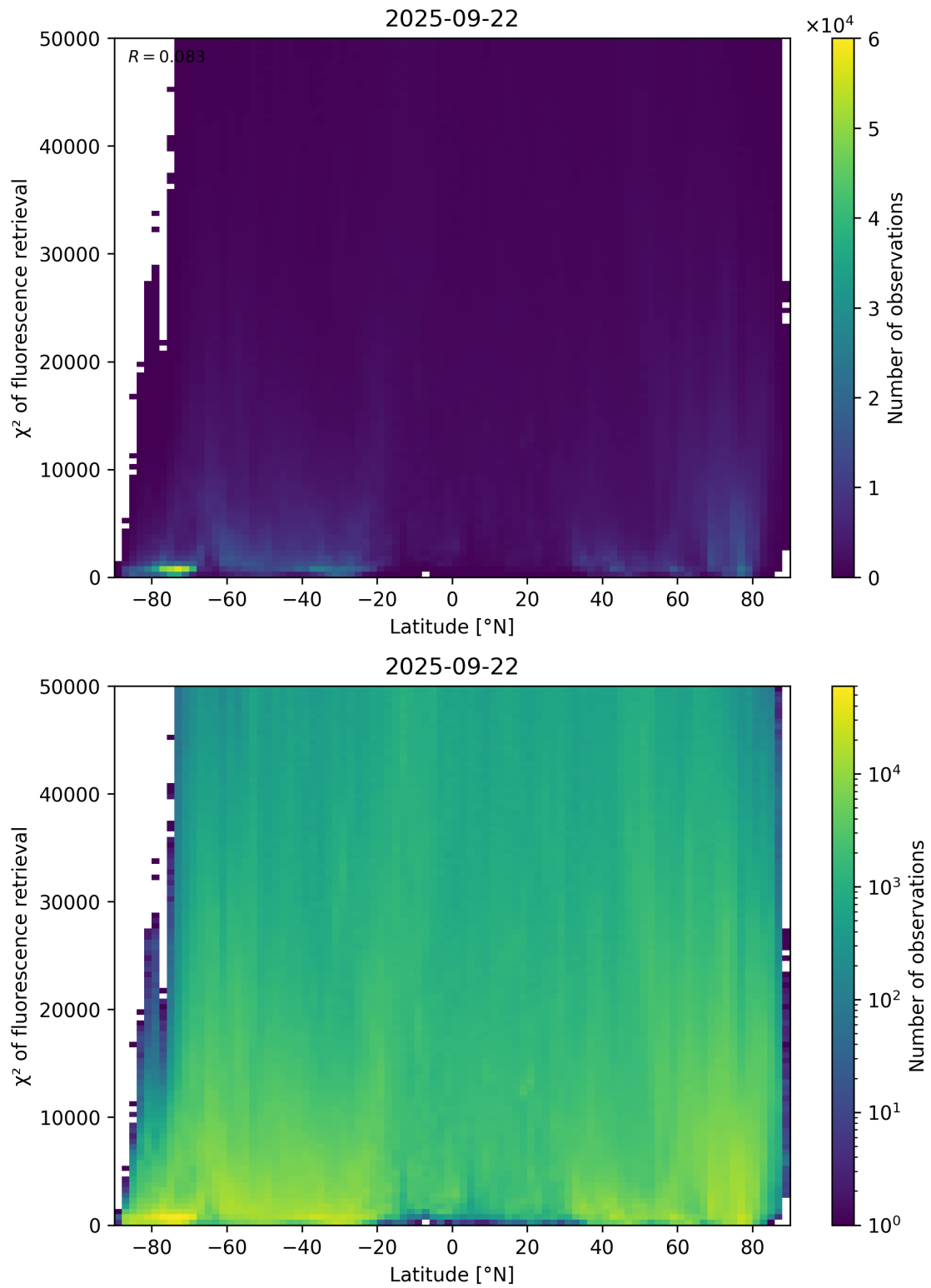
Figure 89: Scatter density plot of “Latitude” against “ \chi^2 of fluorescence retrieval” for 2025-09-22 to 2025-09-23.
