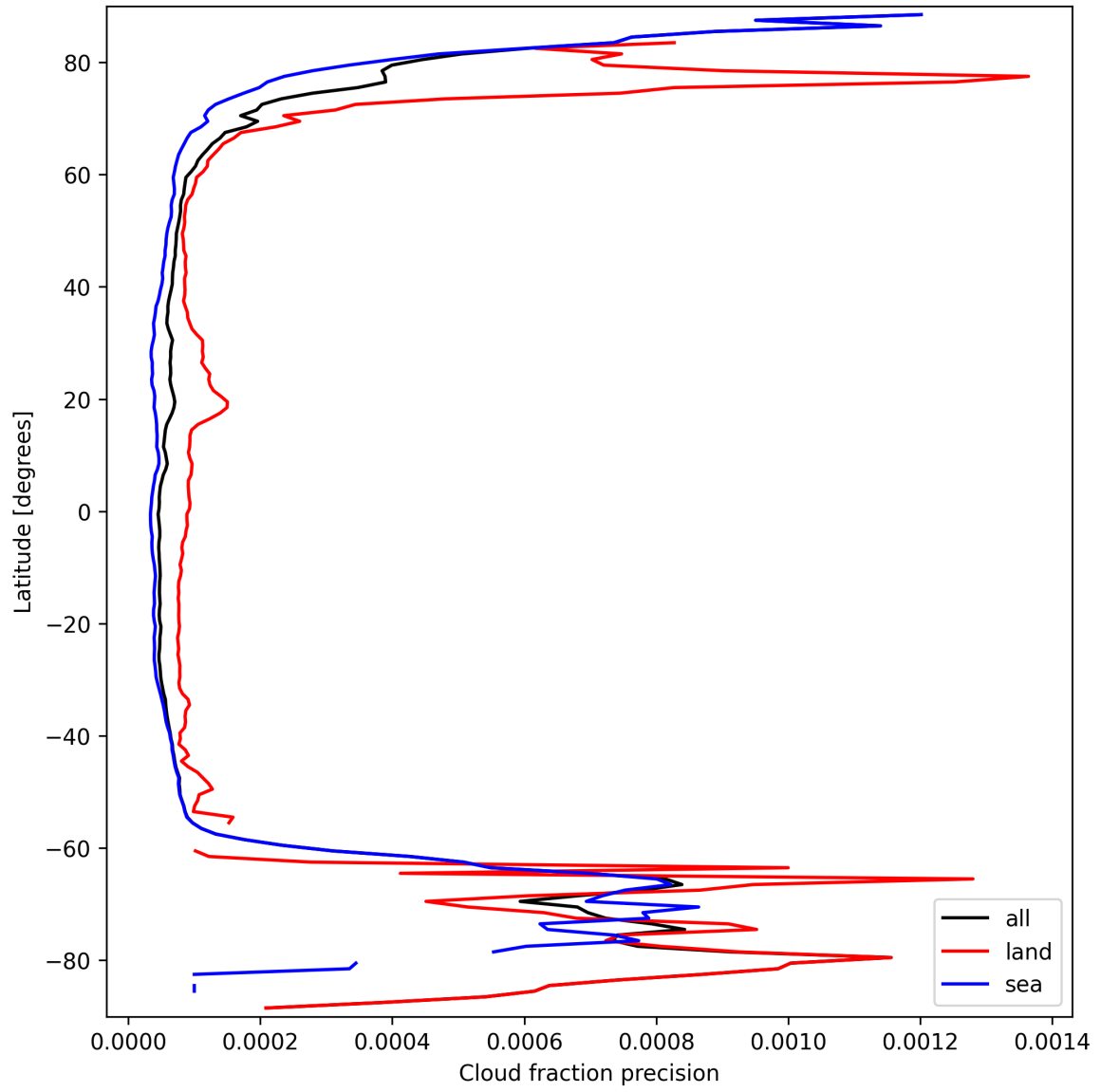
Figure 16: Zonal average of “Cloud fraction precision” for 2025-09-22 to 2025-09-23.
