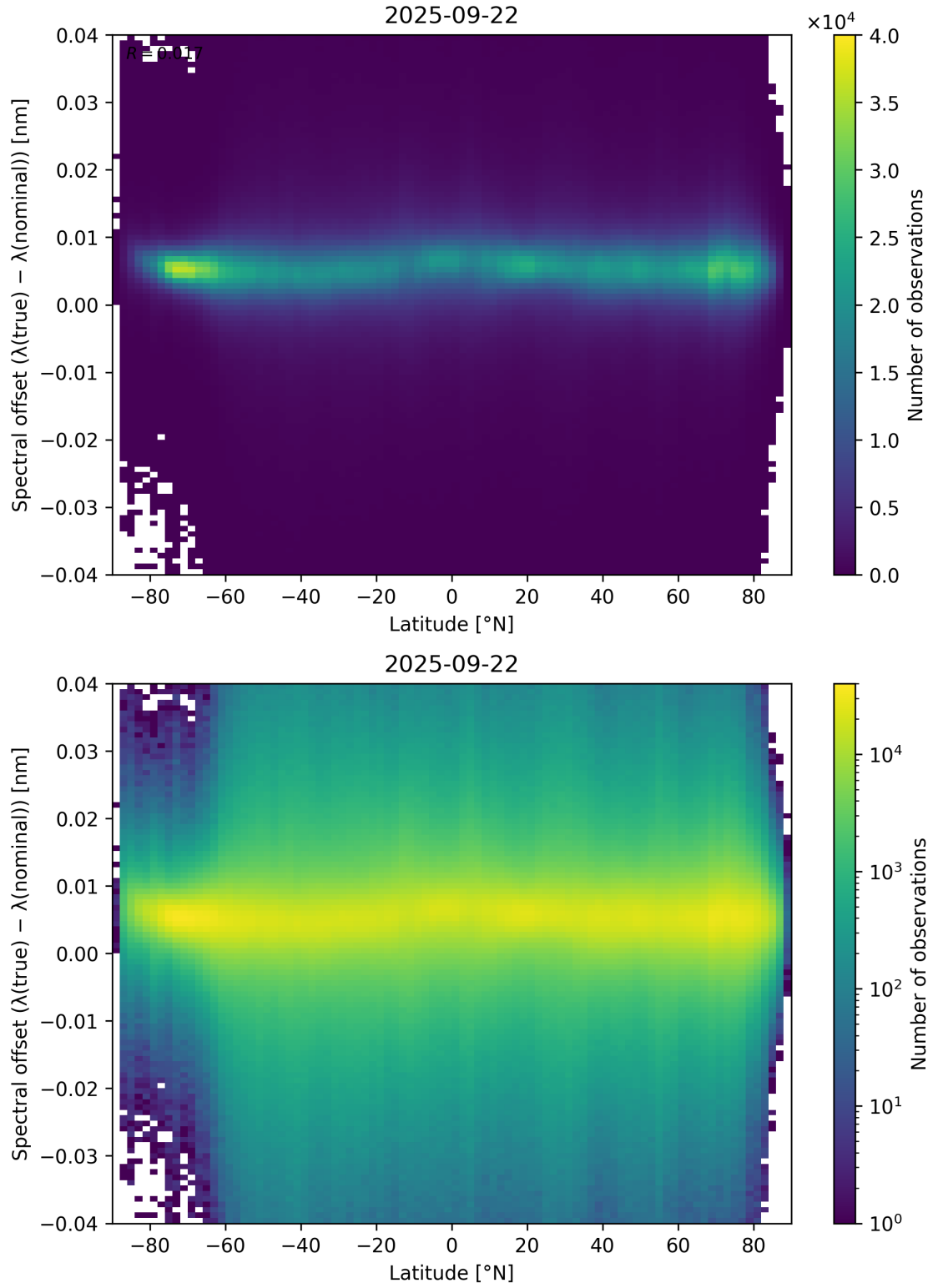
Figure 96: Scatter density plot of “Latitude” against “Spectral offset ( \lambda_{\text{true}} - \lambda_{\text{nominal}} )” for 2025-09-22 to 2025-09-23.
