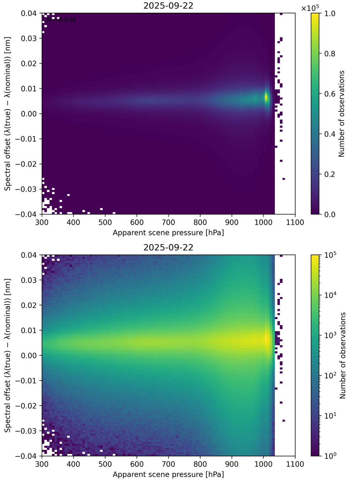
Figure 67: Scatter density plot of “Apparent scene pressure” against “Spectral offset ( \lambda_{\text{true}} - \lambda_{\text{nominal}} )” for 2025-09-22 to 2025-09-23.
