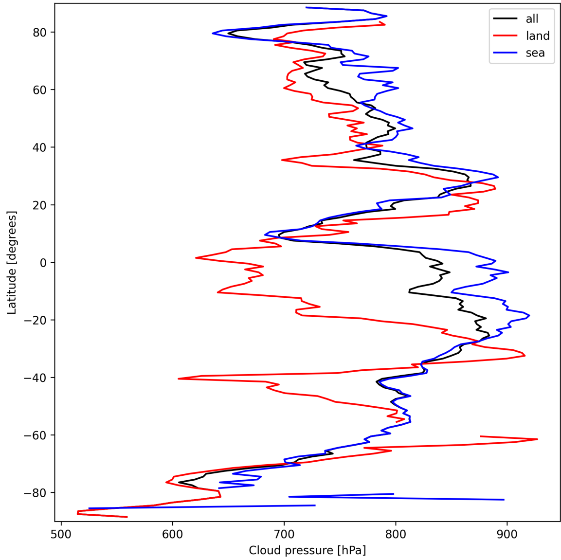
Figure 13: Zonal average of “Cloud pressure” for 2025-09-22 to 2025-09-23.
