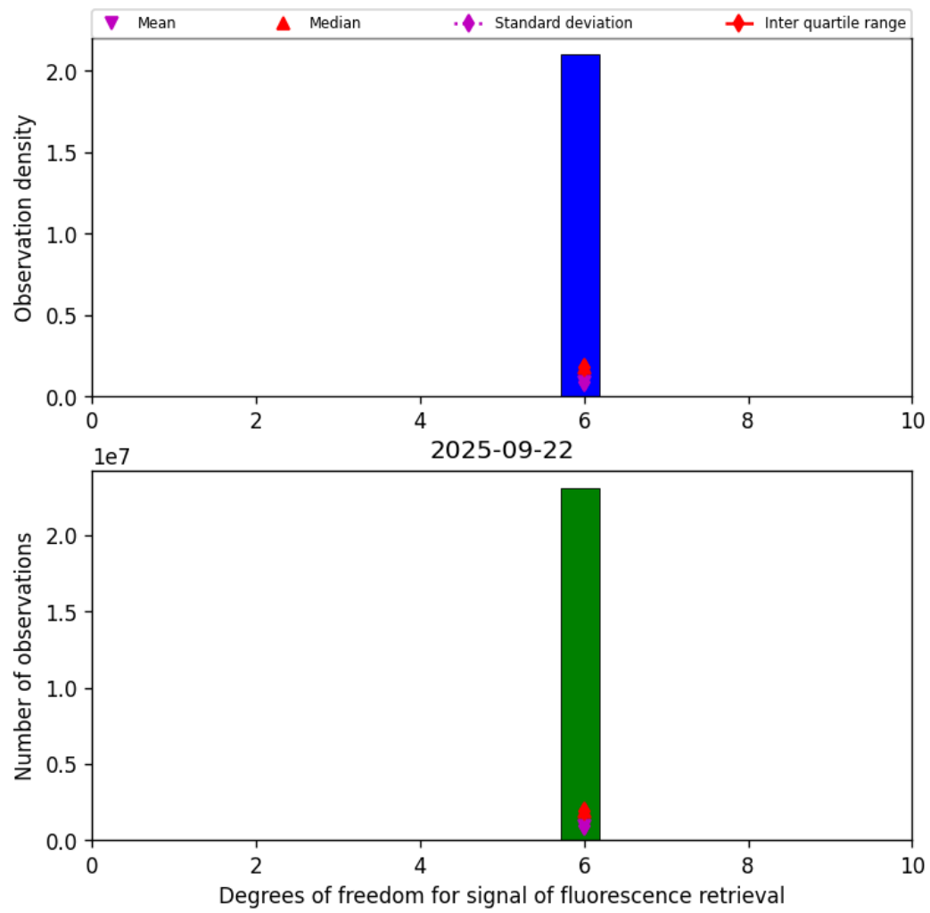
Figure 43: Histogram of “Degrees of freedom for signal of fluorescence retrieval” for 2025-09-22 to 2025-09-23
