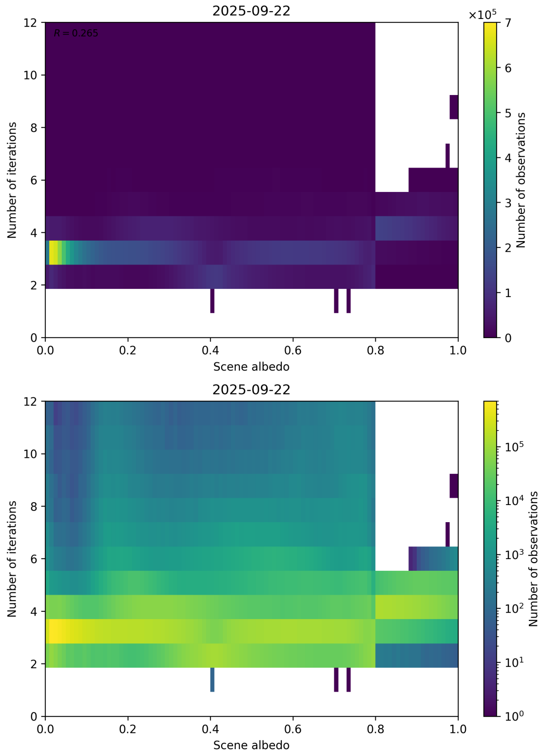
Figure 105: Scatter density plot of “Scene albedo” against “Number of iterations” for 2025-09-22 to 2025-09-23.
