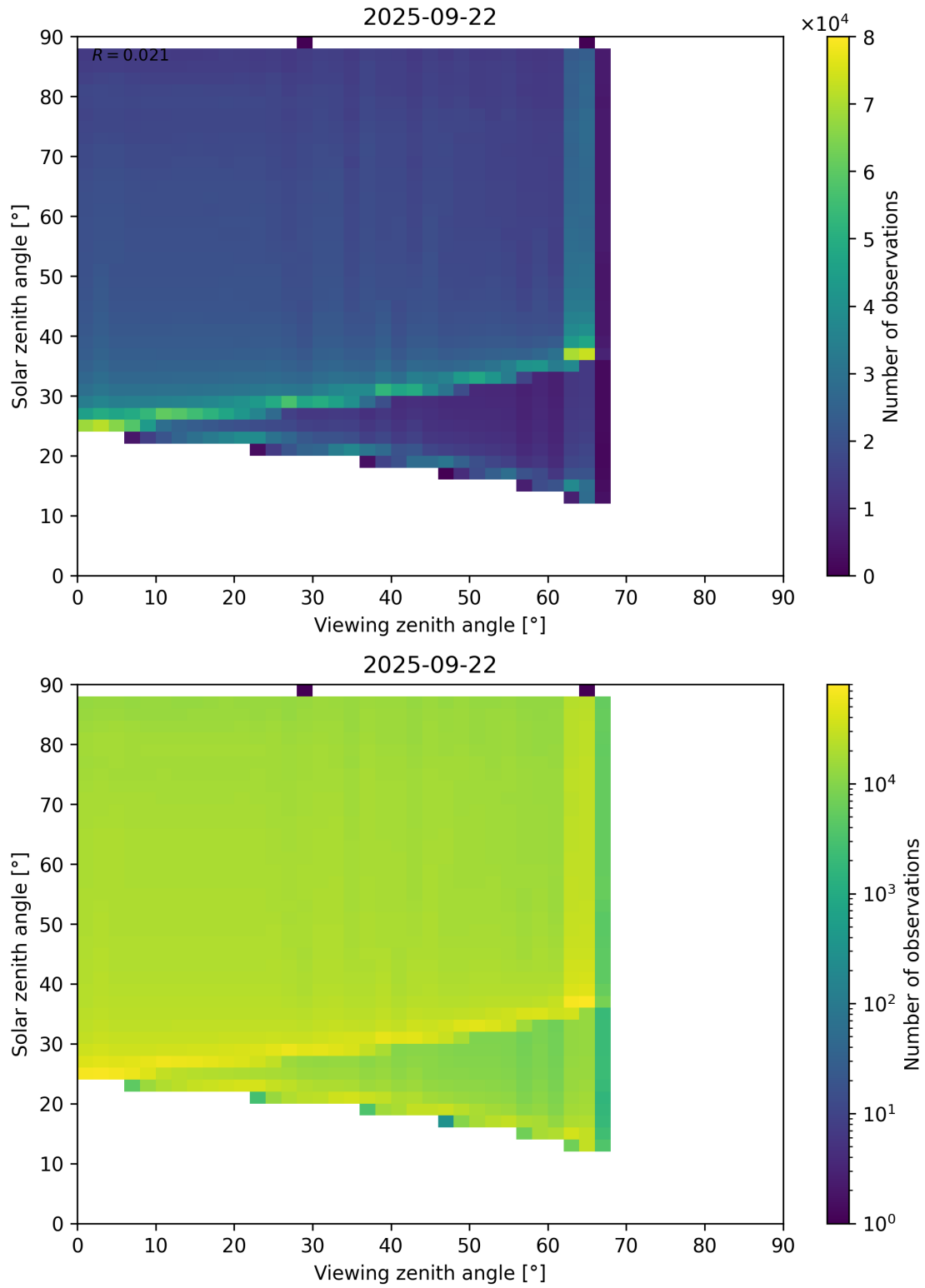
Figure 127: Scatter density plot of “Viewing zenith angle” against “Solar zenith angle” for 2025-09-22 to 2025-09-23.
