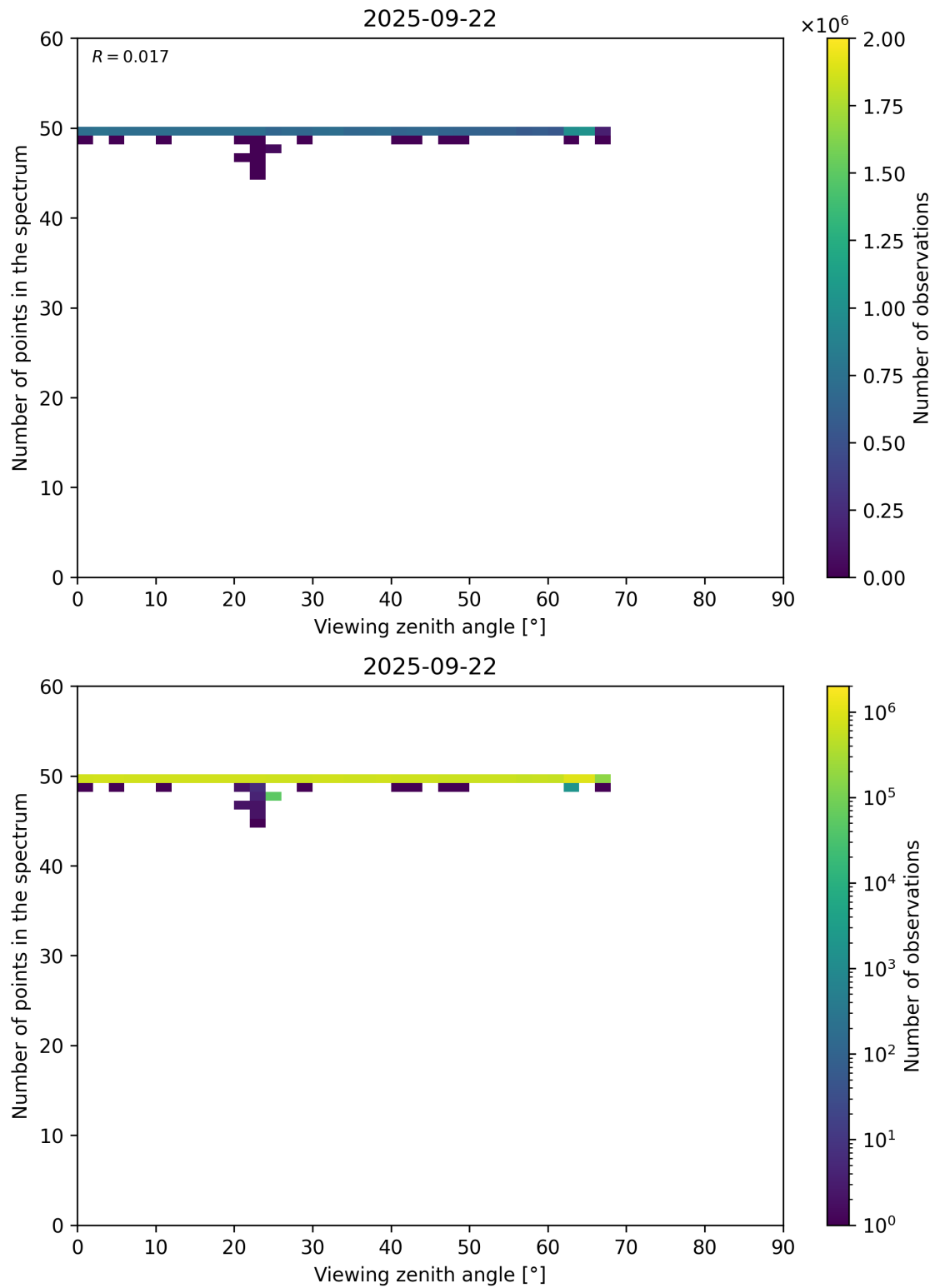
Figure 125: Scatter density plot of “Viewing zenith angle” against “Number of points in the spectrum” for 2025-09-22 to 2025-09-23.
