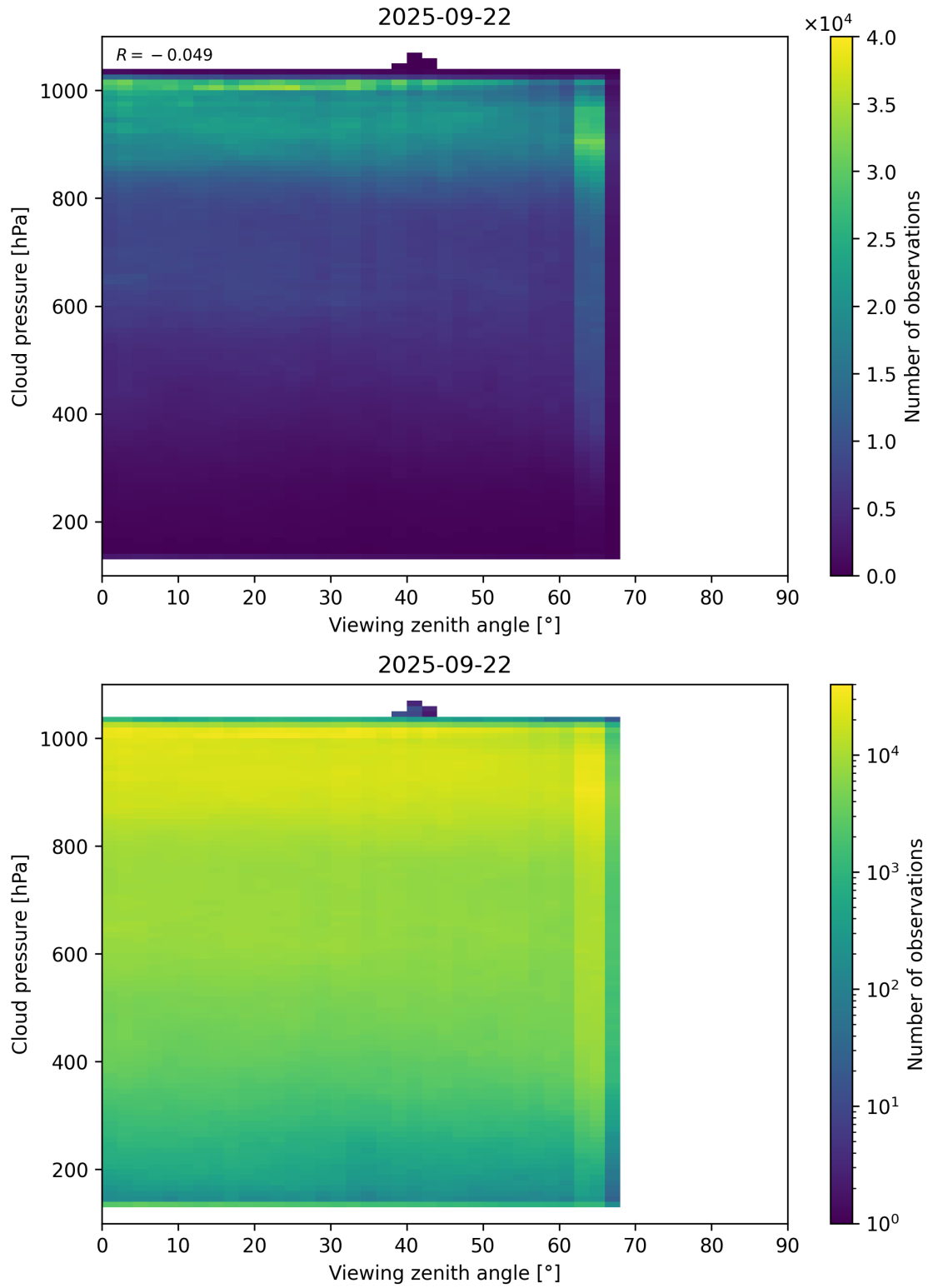
Figure 121: Scatter density plot of “Viewing zenith angle” against “Cloud pressure” for 2025-09-22 to 2025-09-23.
