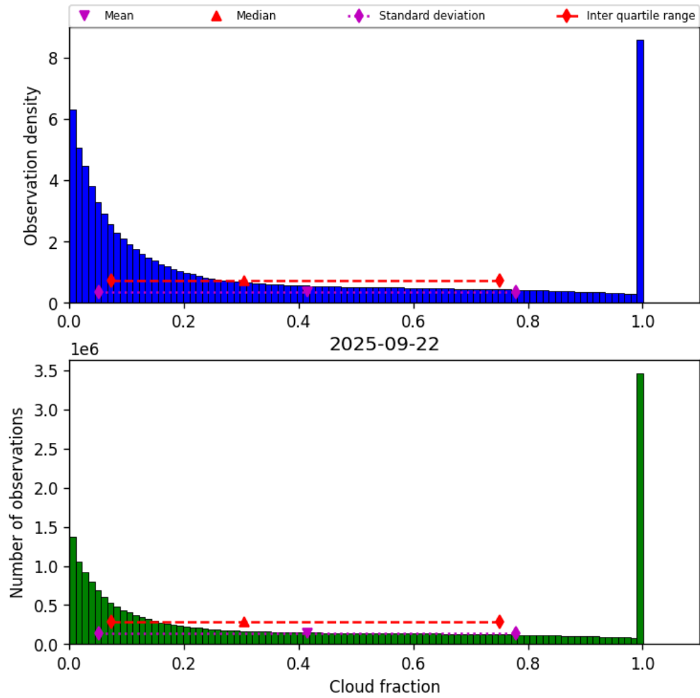
Figure 32: Histogram of “Cloud fraction” for 2025-09-22 to 2025-09-23
