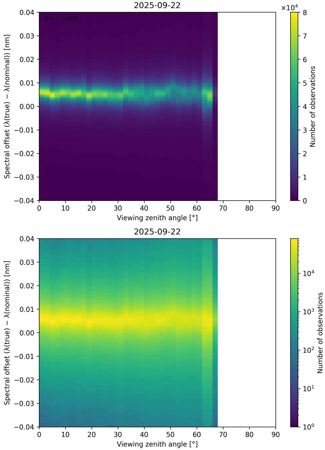
Figure 128: Scatter density plot of “Viewing zenith angle” against “Spectral offset ( \lambda_{\text{true}} - \lambda_{\text{nominal}} )” for 2025-09-22 to 2025-09-23.
