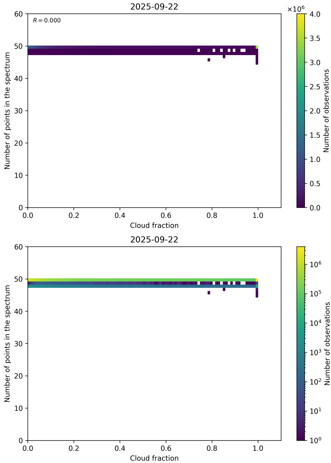
Figure 74: Scatter density plot of “Cloud fraction” against “Number of points in the spectrum” for 2025-09-22 to 2025-09-23.
