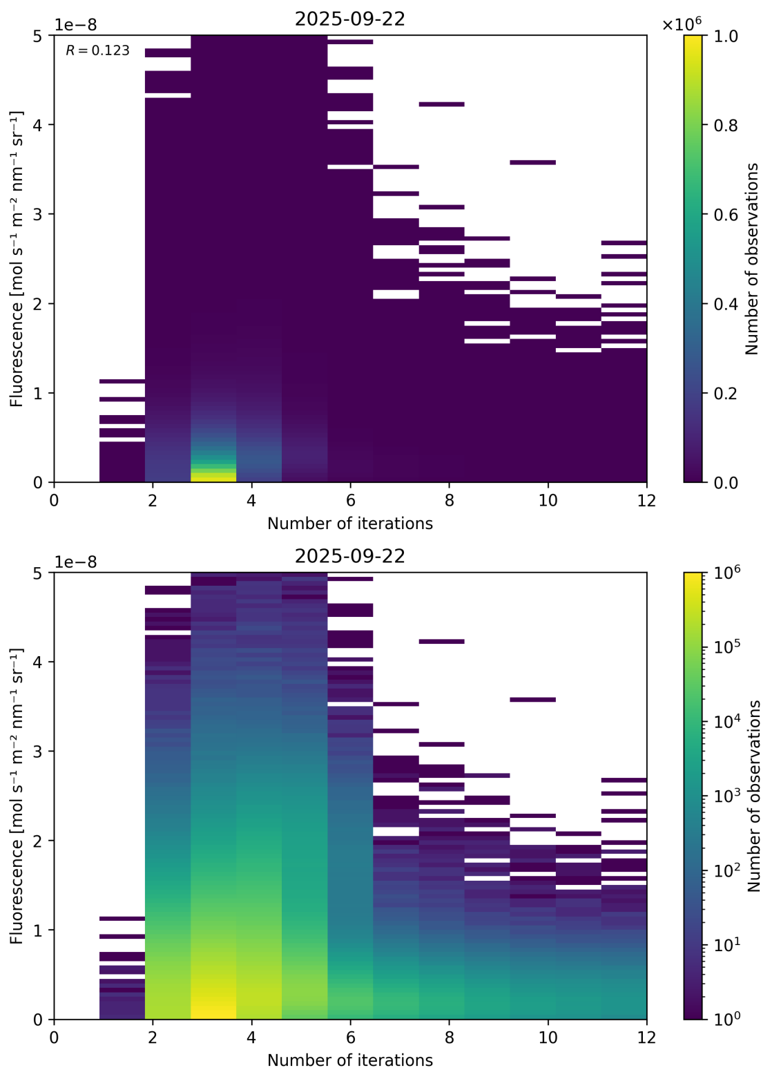
Figure 98: Scatter density plot of “Number of iterations” against “Fluorescence” for 2025-09-22 to 2025-09-23.
