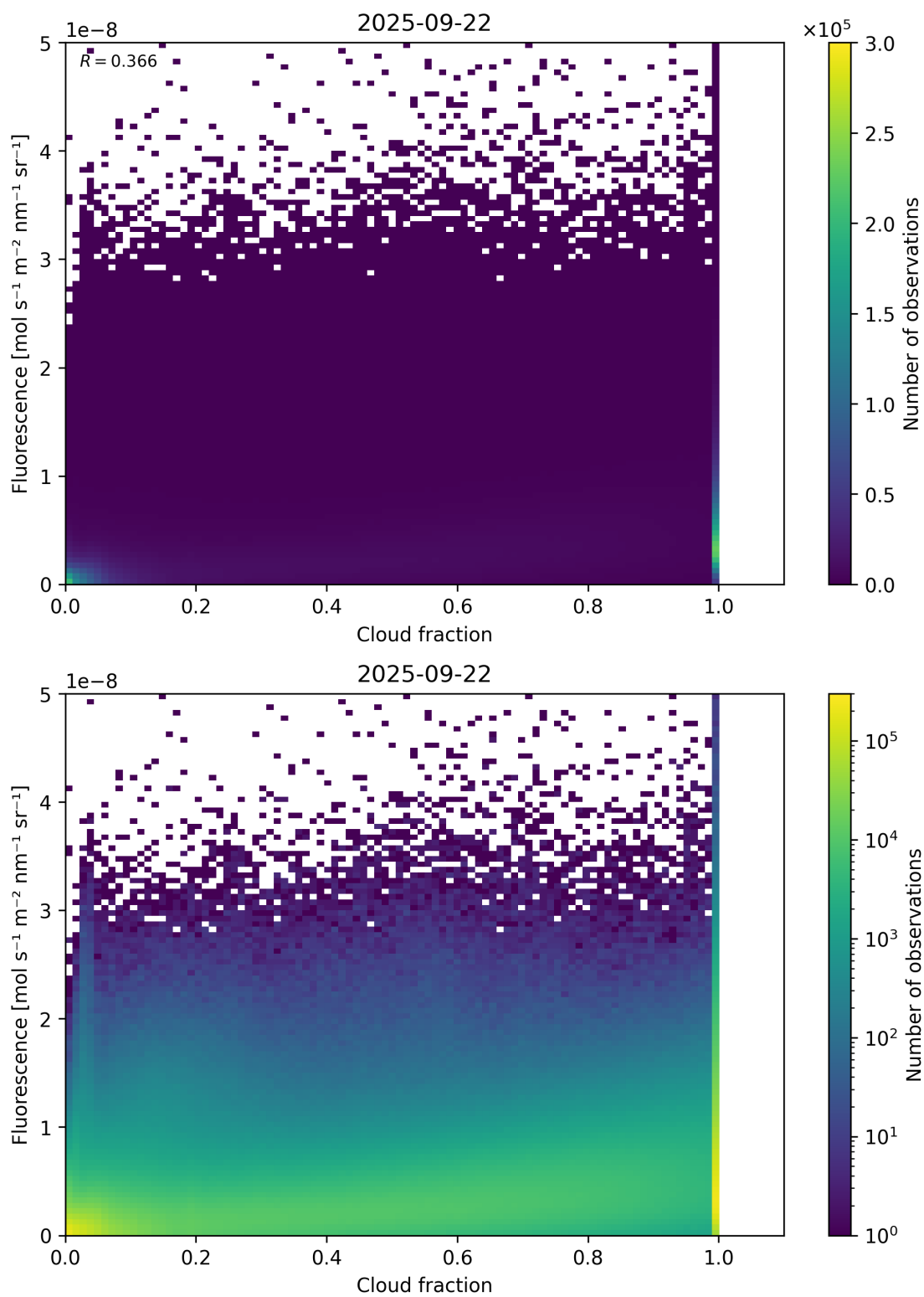
Figure 72: Scatter density plot of “Cloud fraction” against “Fluorescence” for 2025-09-22 to 2025-09-23.
