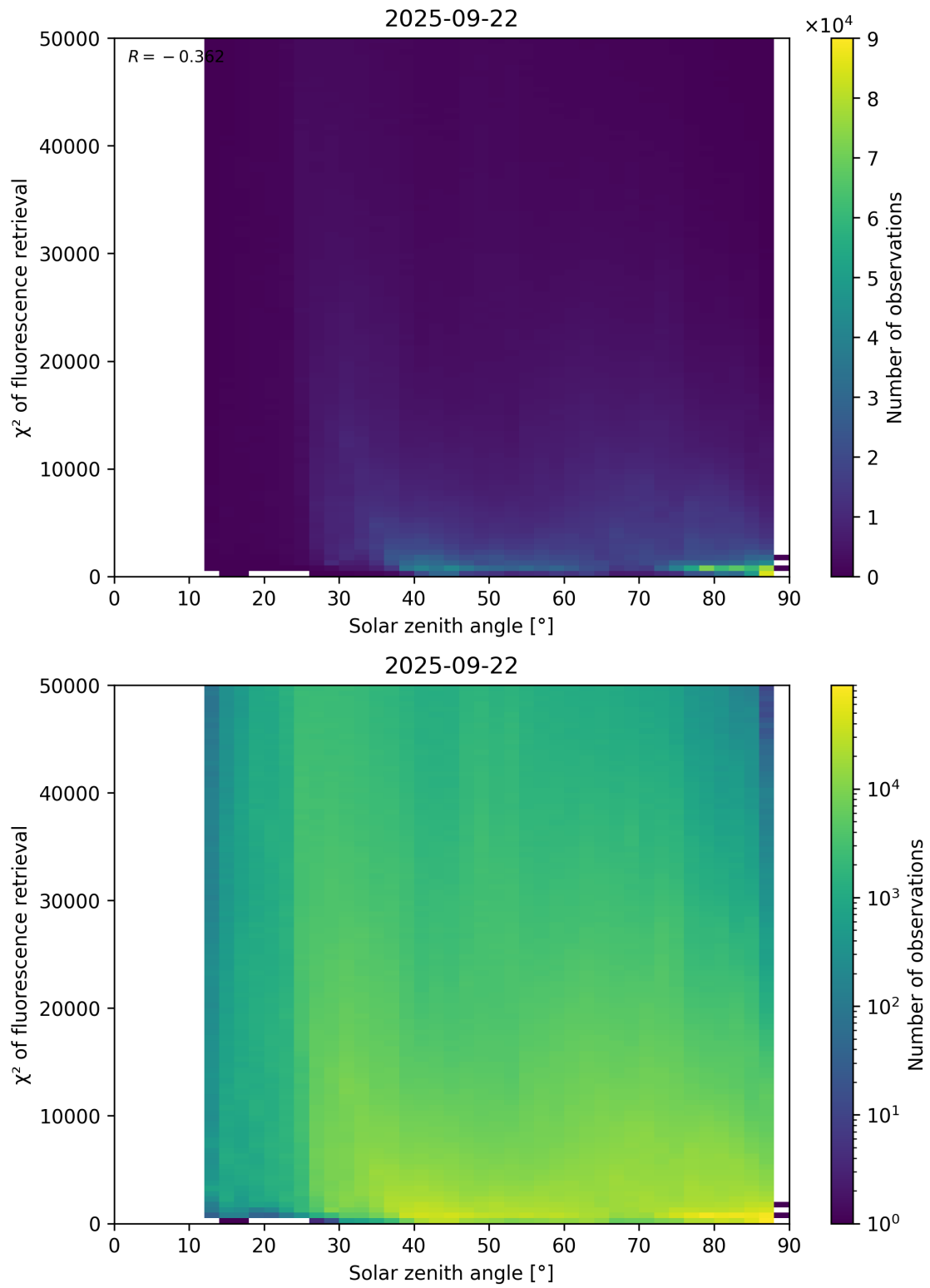
Figure 109: Scatter density plot of “Solar zenith angle” against “ \chi^2 of fluorescence retrieval” for 2025-09-22 to 2025-09-23.
