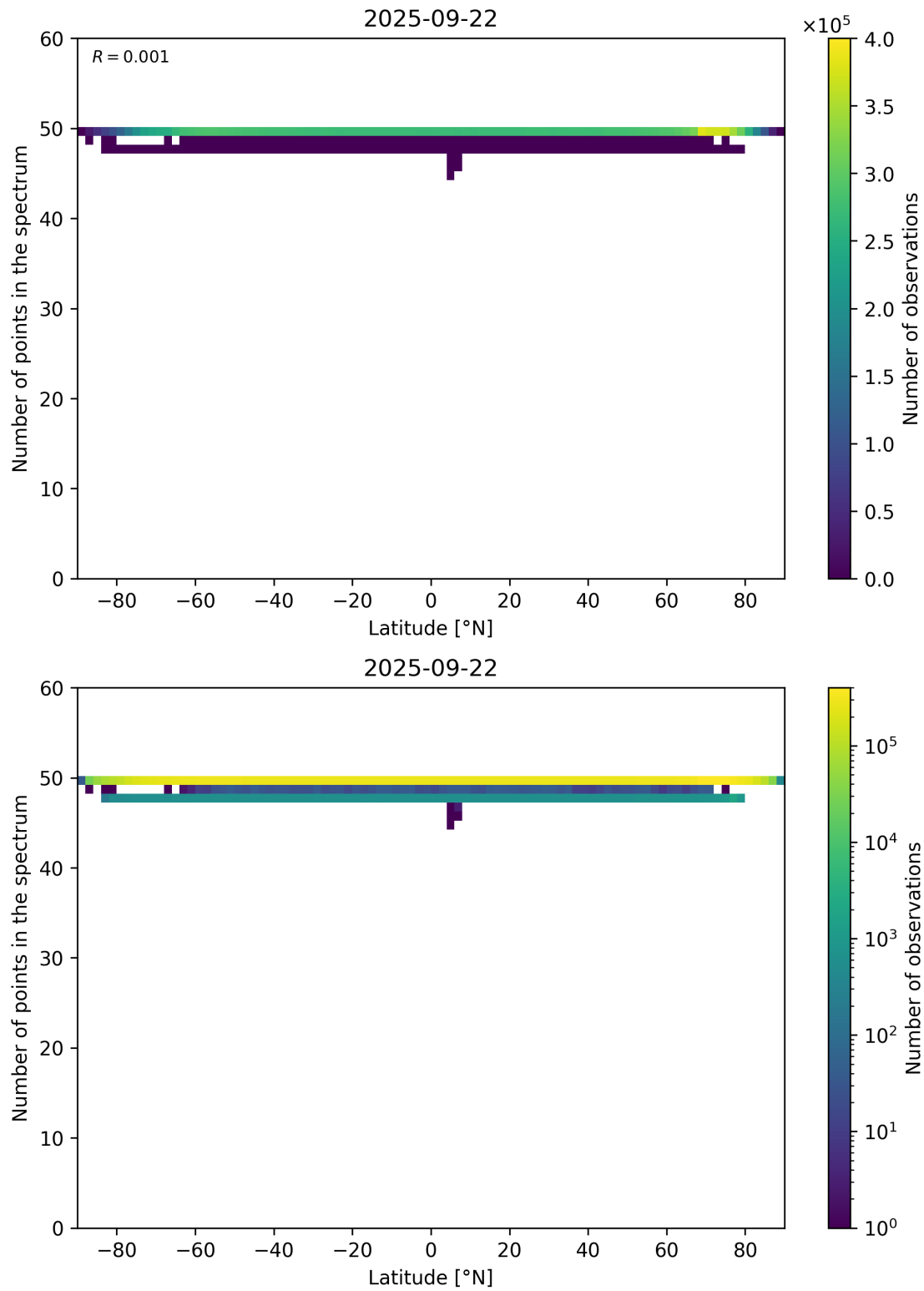
Figure 94: Scatter density plot of “Latitude” against “Number of points in the spectrum” for 2025-09-22 to 2025-09-23.
