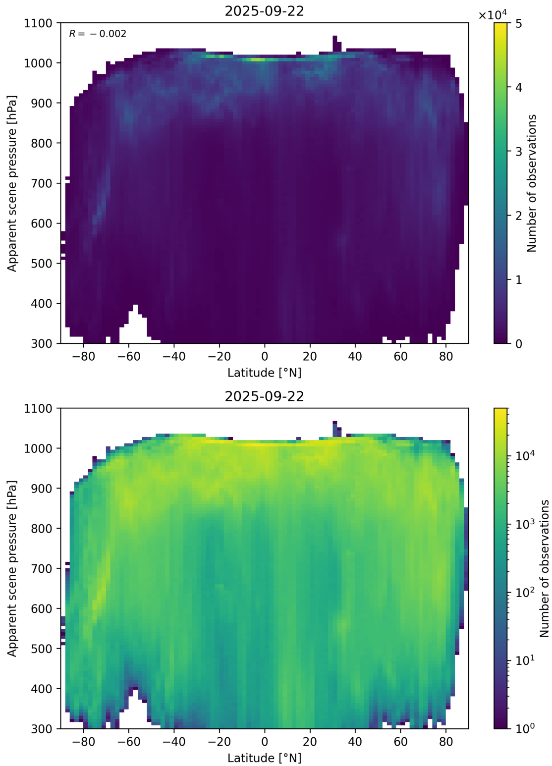
Figure 88: Scatter density plot of “Latitude” against “Apparent scene pressure” for 2025-09-22 to 2025-09-23.
