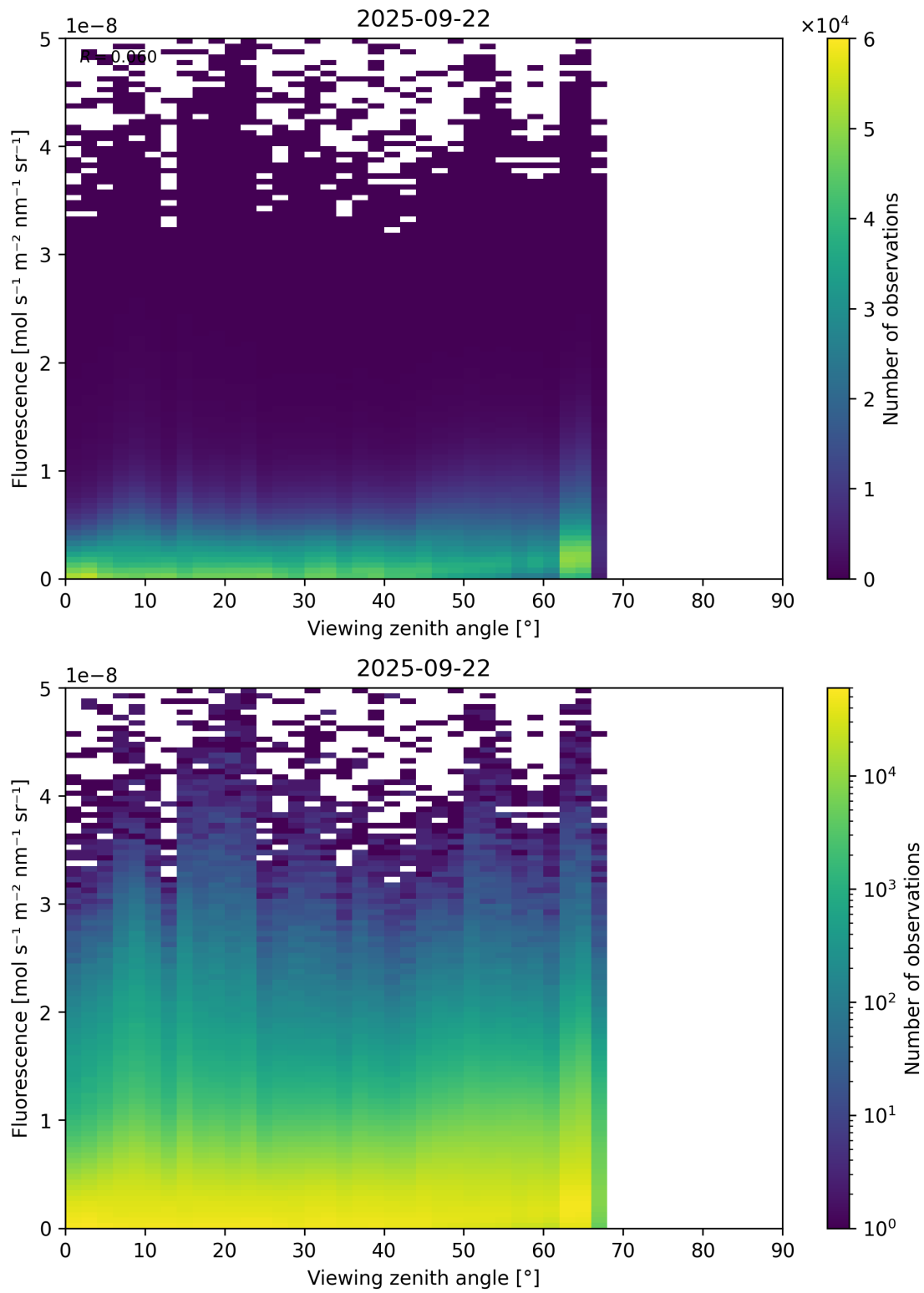
Figure 122: Scatter density plot of “Viewing zenith angle” against “Fluorescence” for 2025-09-22 to 2025-09-23.
