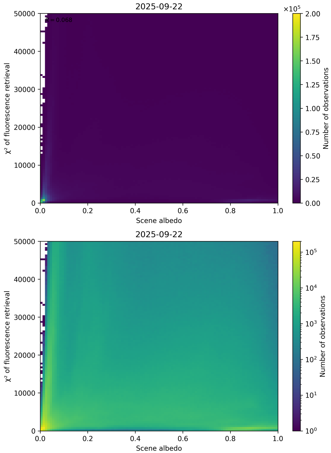
Figure 103: Scatter density plot of “Scene albedo” against “ \chi^2 of fluorescence retrieval” for 2025-09-22 to 2025-09-23.
