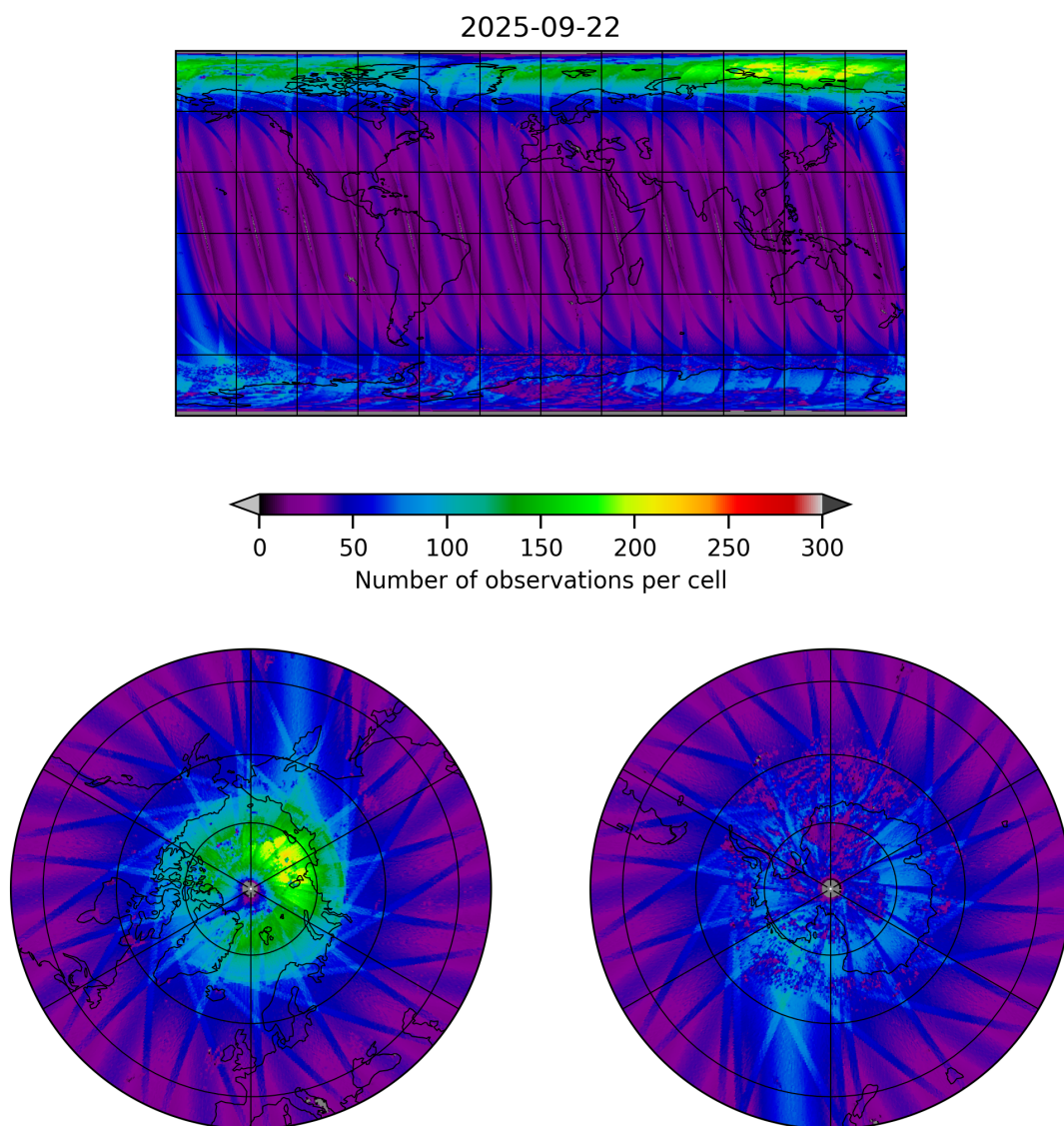
Figure 11: Map of the number of observations for 2025-09-22 to 2025-09-23
