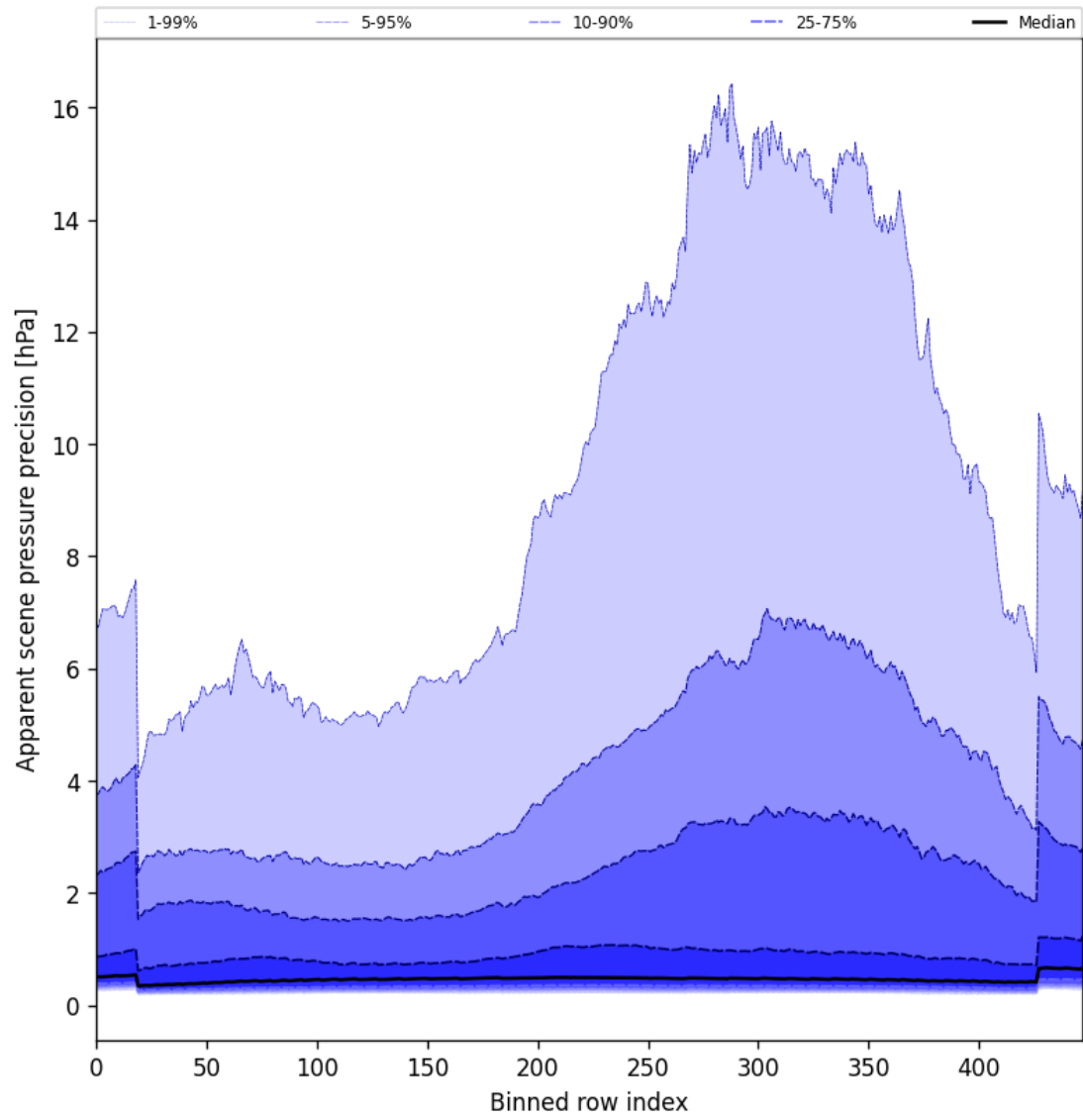
Figure 54: Along track statistics of “Apparent scene pressure precision” for 2025-09-22 to 2025-09-23
