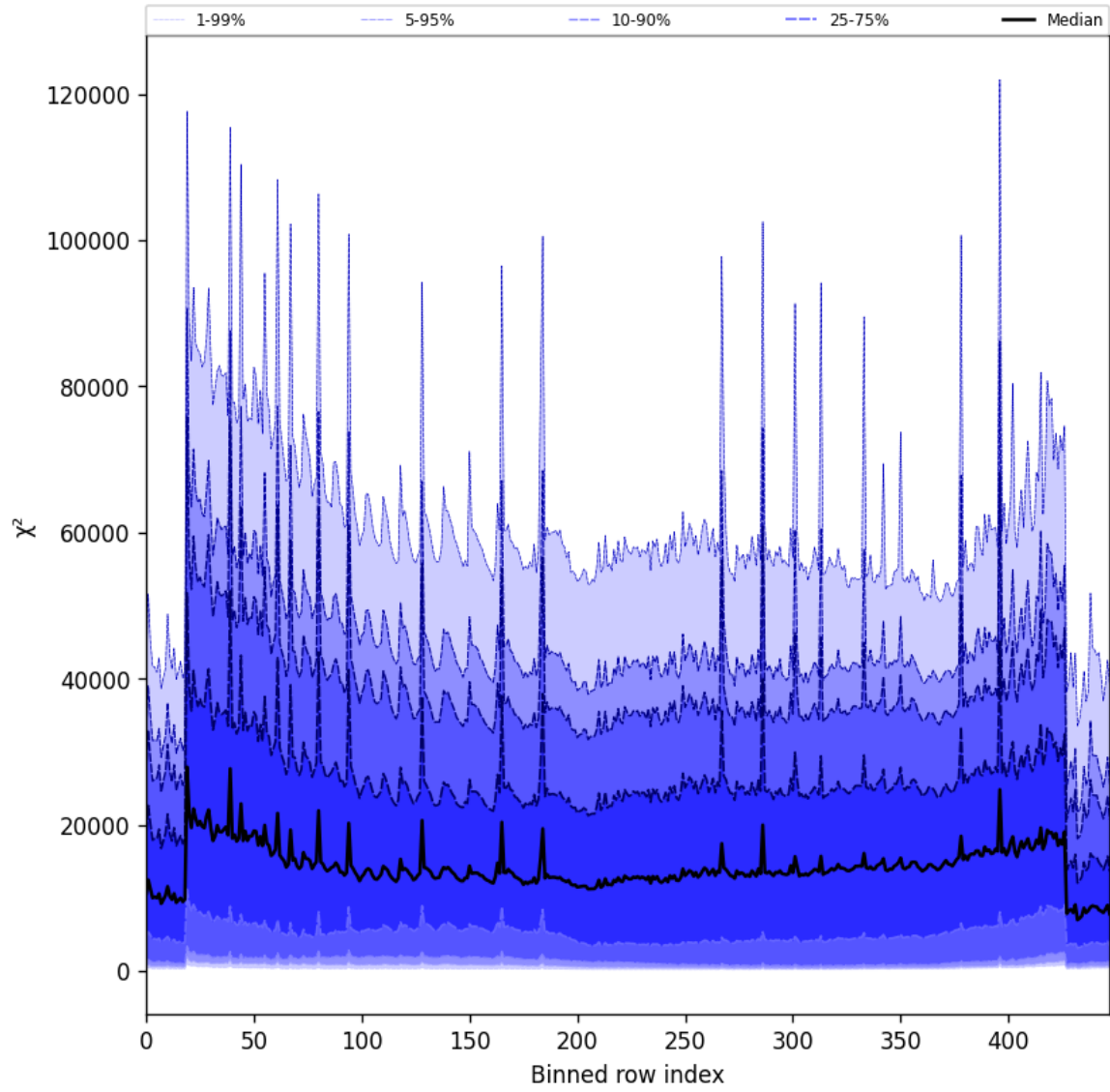
Figure 55: Along track statistics of “ \chi^2 ” for 2025-09-22 to 2025-09-23
