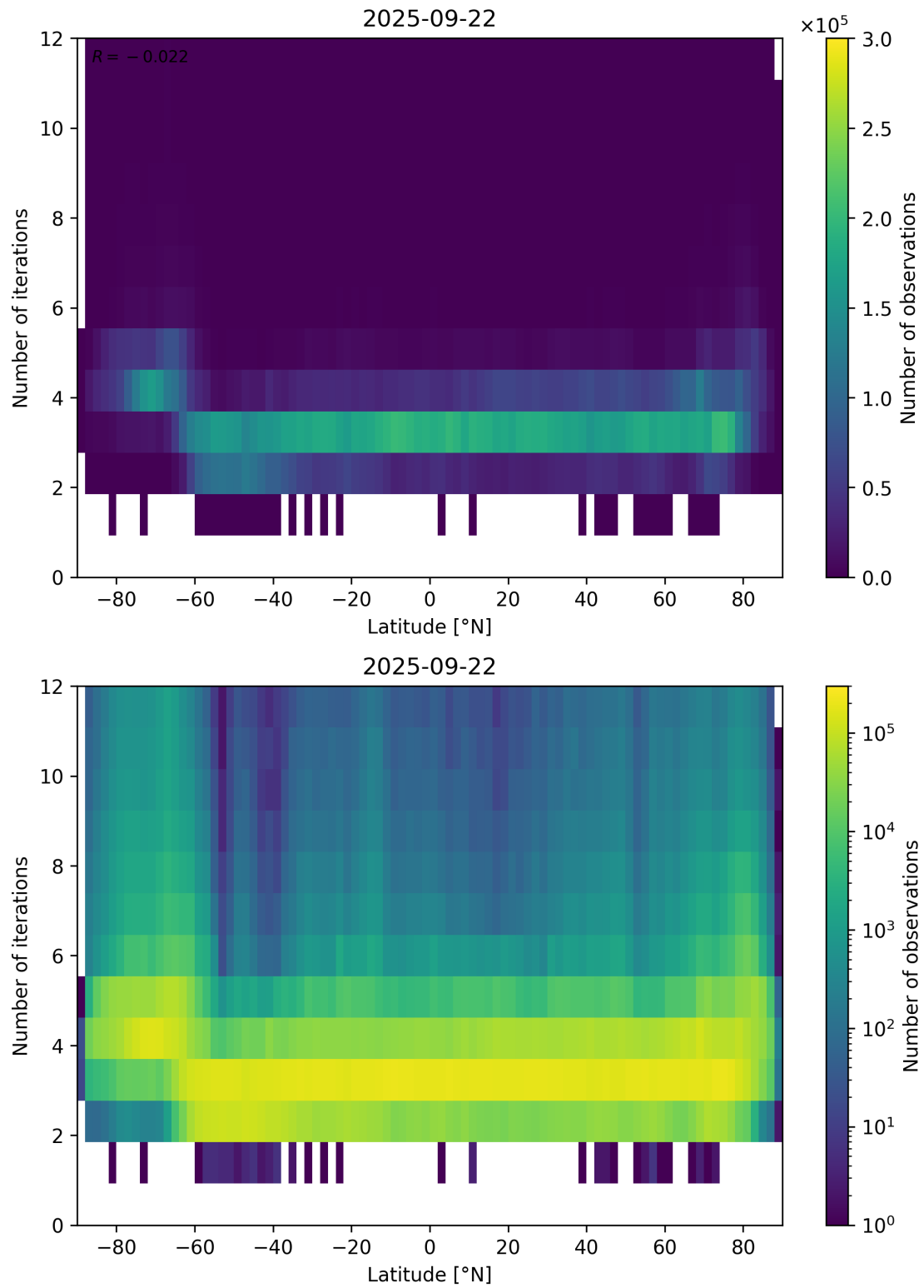
Figure 93: Scatter density plot of “Latitude” against “Number of iterations” for 2025-09-22 to 2025-09-23.
