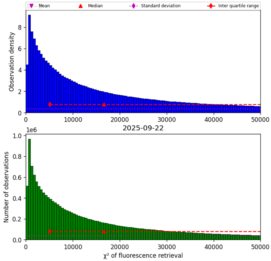
Figure 42: Histogram of “ \chi^2 of fluorescence retrieval” for 2025-09-22 to 2025-09-23
