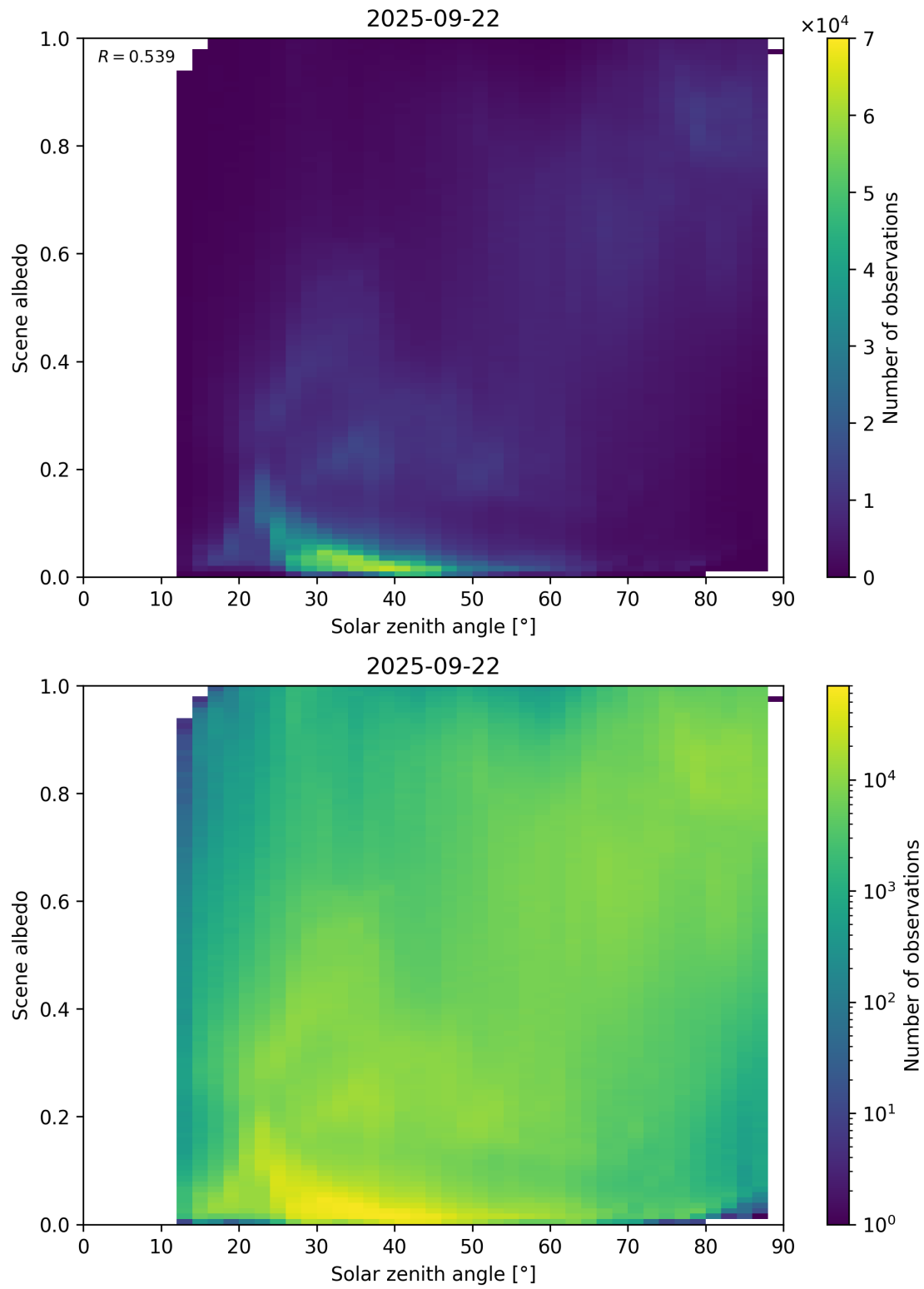
Figure 116: Scatter density plot of “Solar zenith angle” against “Scene albedo” for 2025-09-22 to 2025-09-23.
