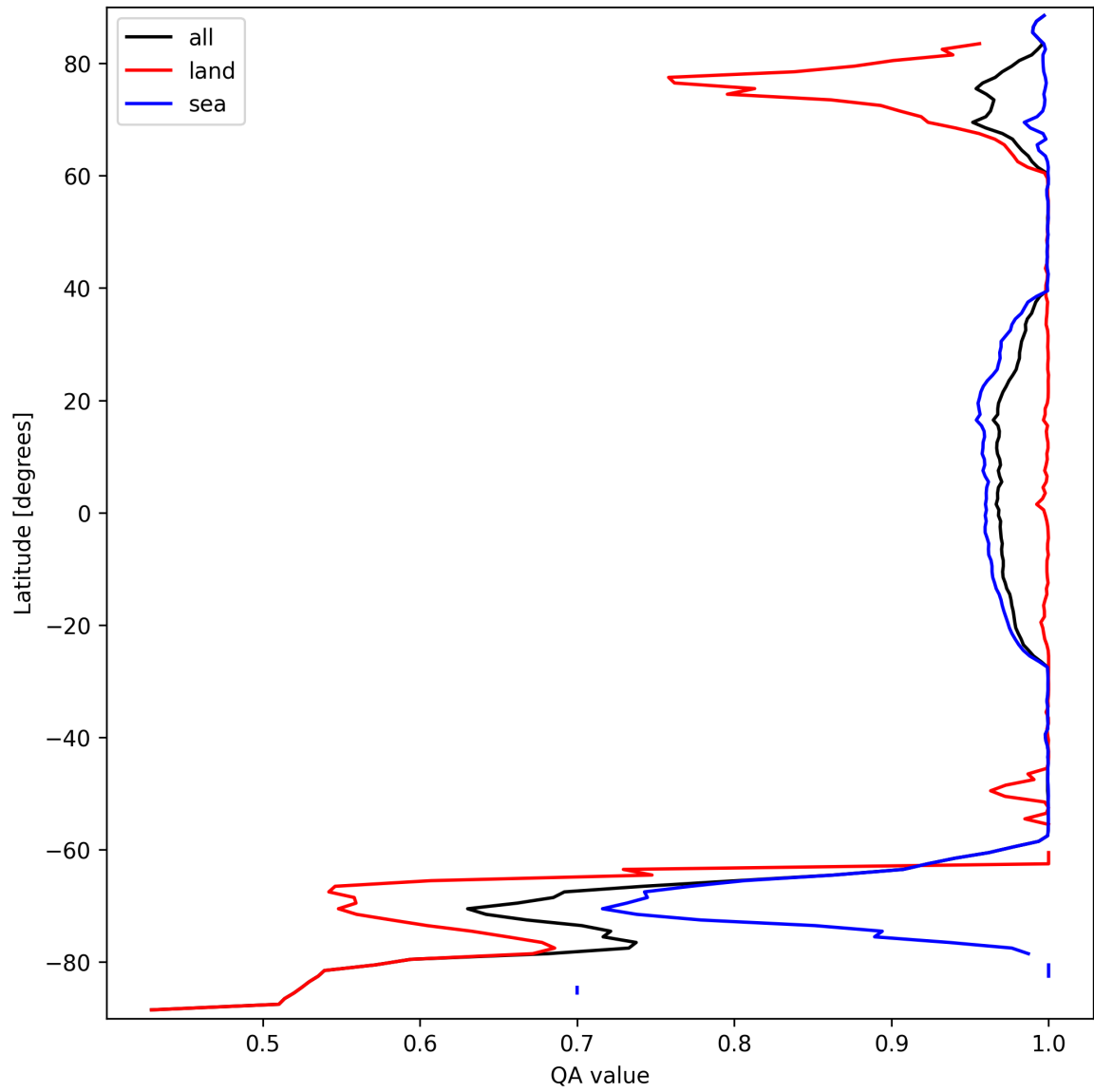
Figure 12: Zonal average of “QA value” for 2025-09-22 to 2025-09-23.
