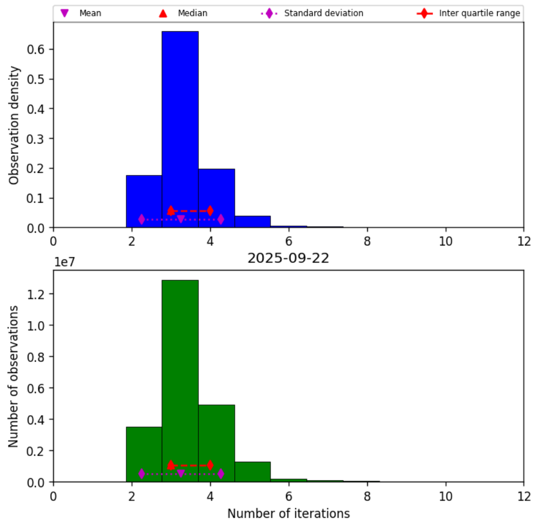
Figure 39: Histogram of “Number of iterations” for 2025-09-22 to 2025-09-23
