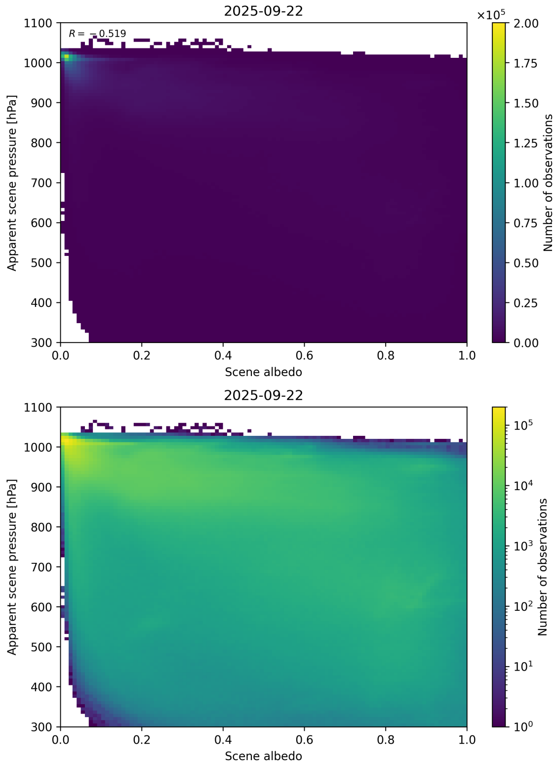
Figure 102: Scatter density plot of “Scene albedo” against “Apparent scene pressure” for 2025-09-22 to 2025-09-23.
