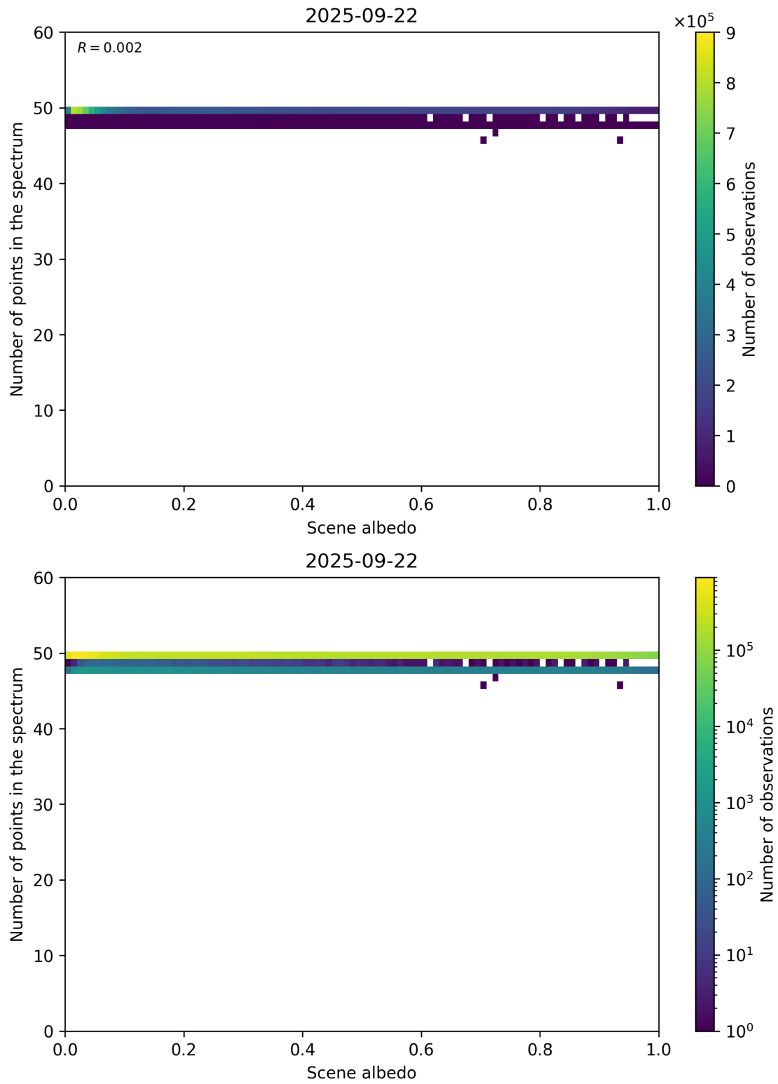
Figure 106: Scatter density plot of “Scene albedo” against “Number of points in the spectrum” for 2025-09-22 to 2025-09-23.
