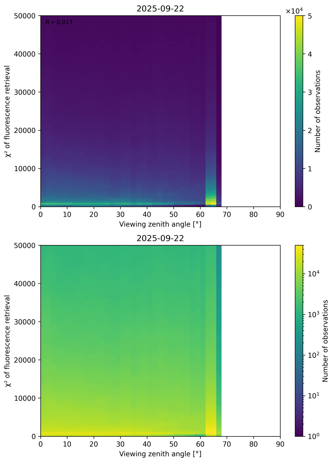
Figure 119: Scatter density plot of “Viewing zenith angle” against “ \chi^2 of fluorescence retrieval” for 2025-09-22 to 2025-09-23.
