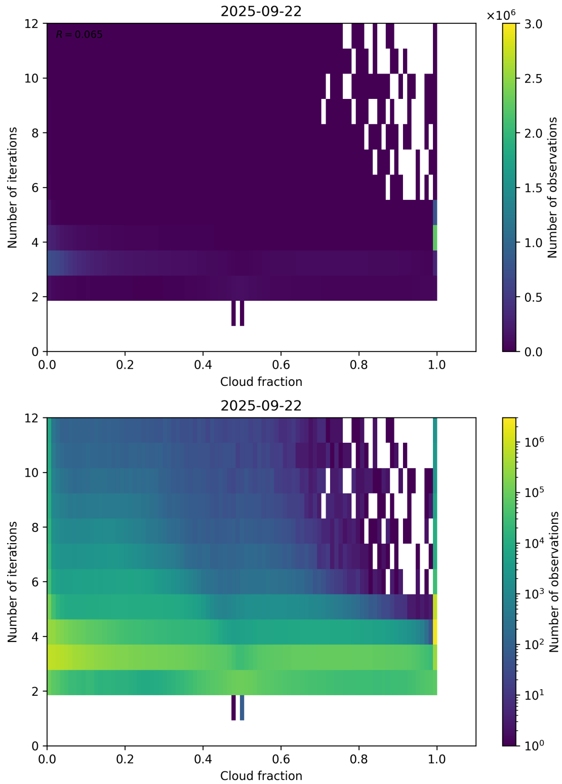
Figure 73: Scatter density plot of “Cloud fraction” against “Number of iterations” for 2025-09-22 to 2025-09-23.
