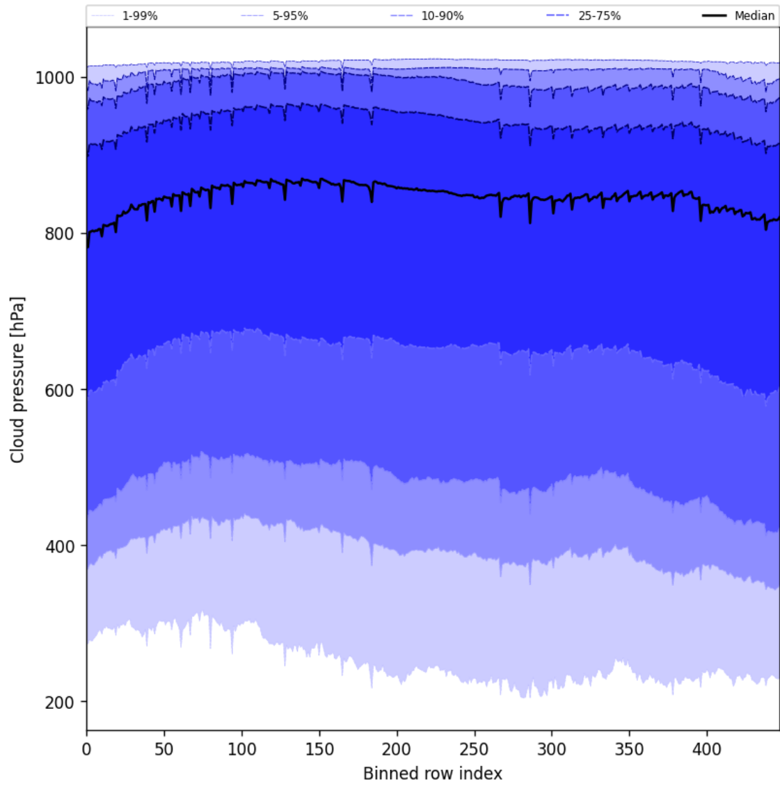
Figure 47: Along track statistics of “Cloud pressure” for 2025-09-22 to 2025-09-23
