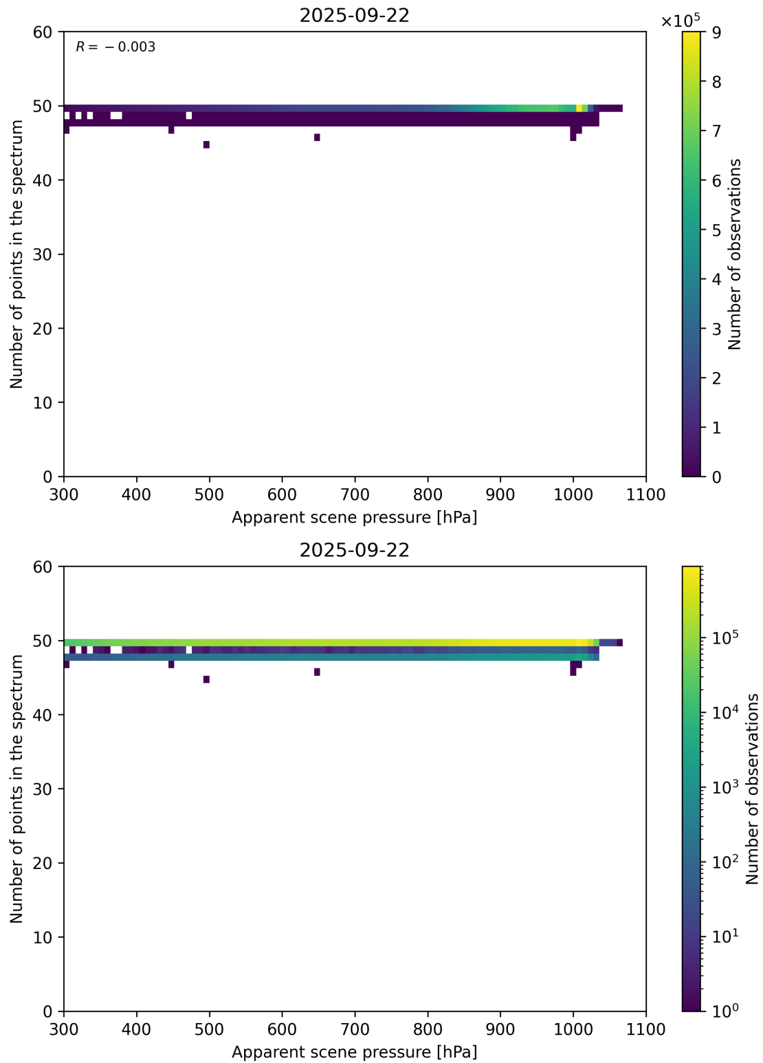
Figure 66: Scatter density plot of “Apparent scene pressure” against “Number of points in the spectrum” for 2025-09-22 to 2025-09-23.
