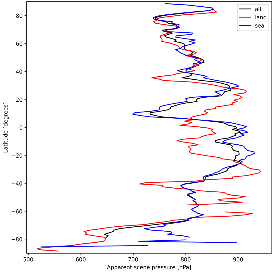
Figure 19: Zonal average of “Apparent scene pressure” for 2025-09-22 to 2025-09-23.
