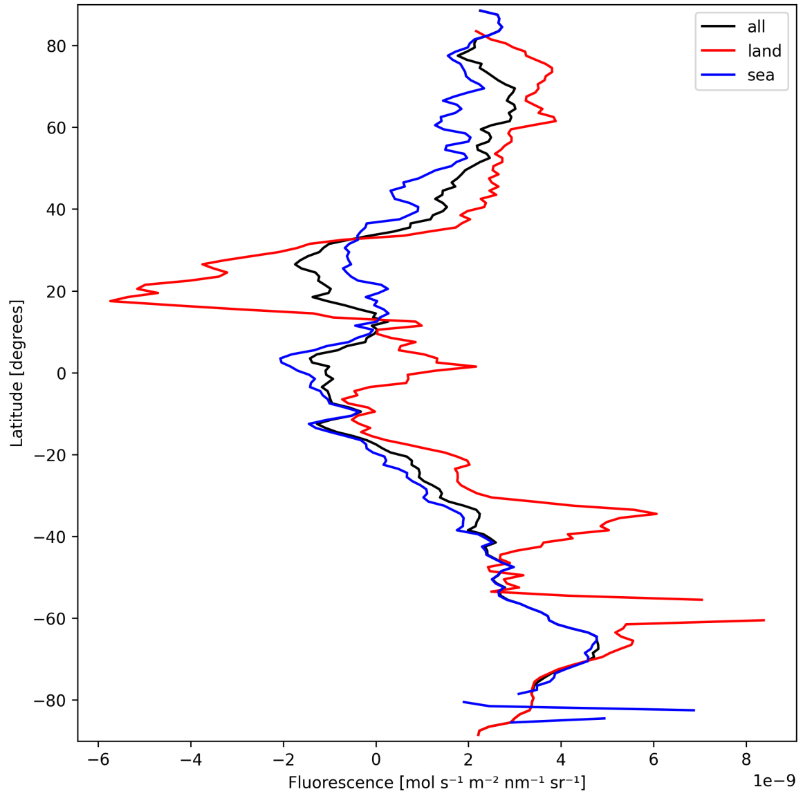
Figure 23: Zonal average of “Fluorescence” for 2025-09-22 to 2025-09-23.
