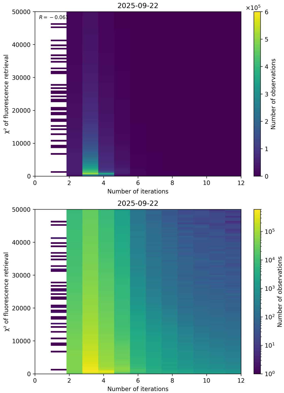
Figure 97: Scatter density plot of “Number of iterations” against “ \chi^2 of fluorescence retrieval” for 2025-09-22 to 2025-09-23.
