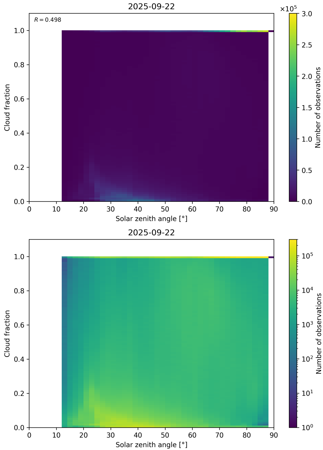
Figure 110: Scatter density plot of “Solar zenith angle” against “Cloud fraction” for 2025-09-22 to 2025-09-23.
