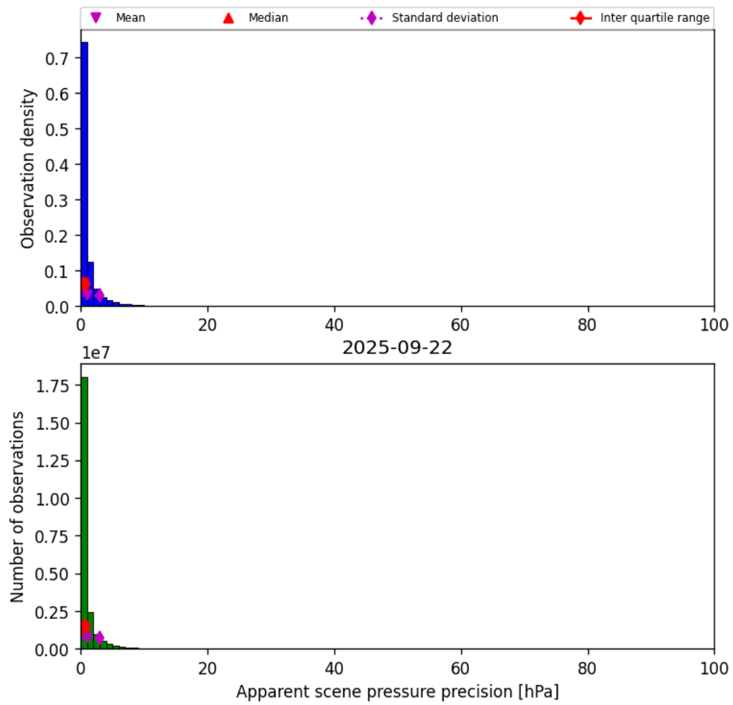
Figure 37: Histogram of “Apparent scene pressure precision” for 2025-09-22 to 2025-09-23
