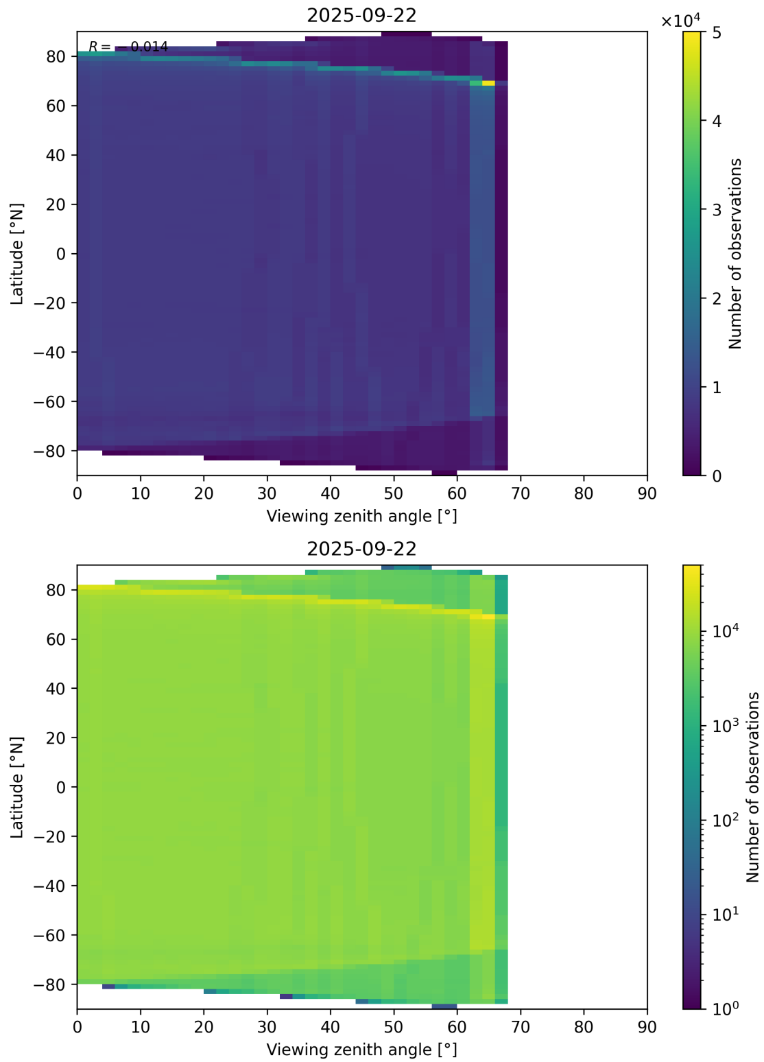
Figure 123: Scatter density plot of “Viewing zenith angle” against “Latitude” for 2025-09-22 to 2025-09-23.
