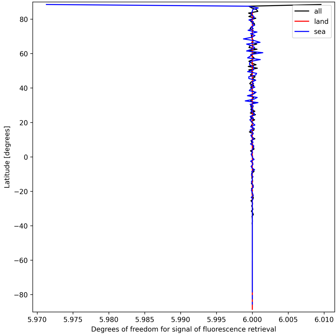
Figure 26: Zonal average of “Degrees of freedom for signal of fluorescence retrieval” for 2025-09-22 to 2025-09-23.
