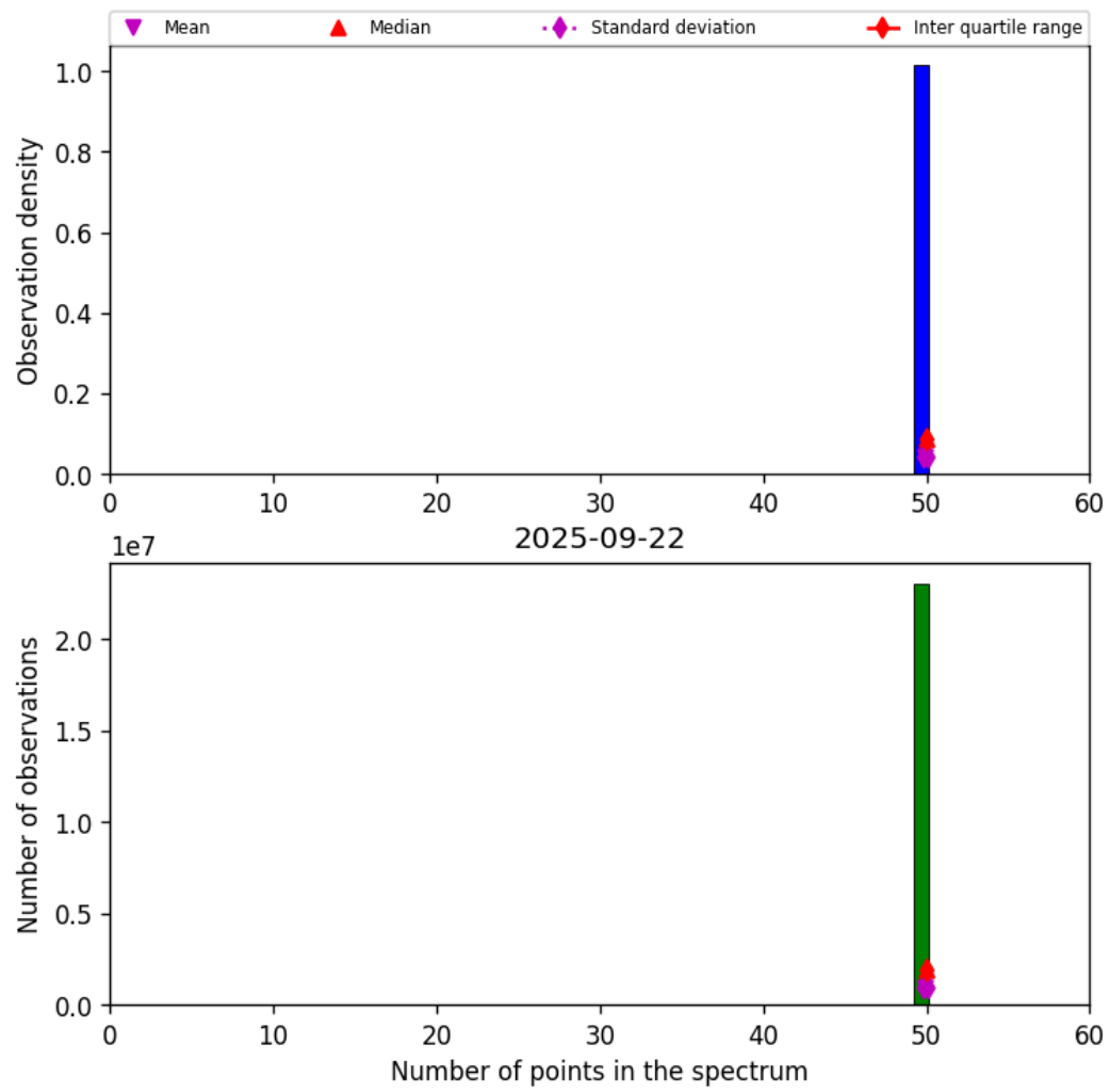
Figure 44: Histogram of “Number of points in the spectrum” for 2025-09-22 to 2025-09-23
