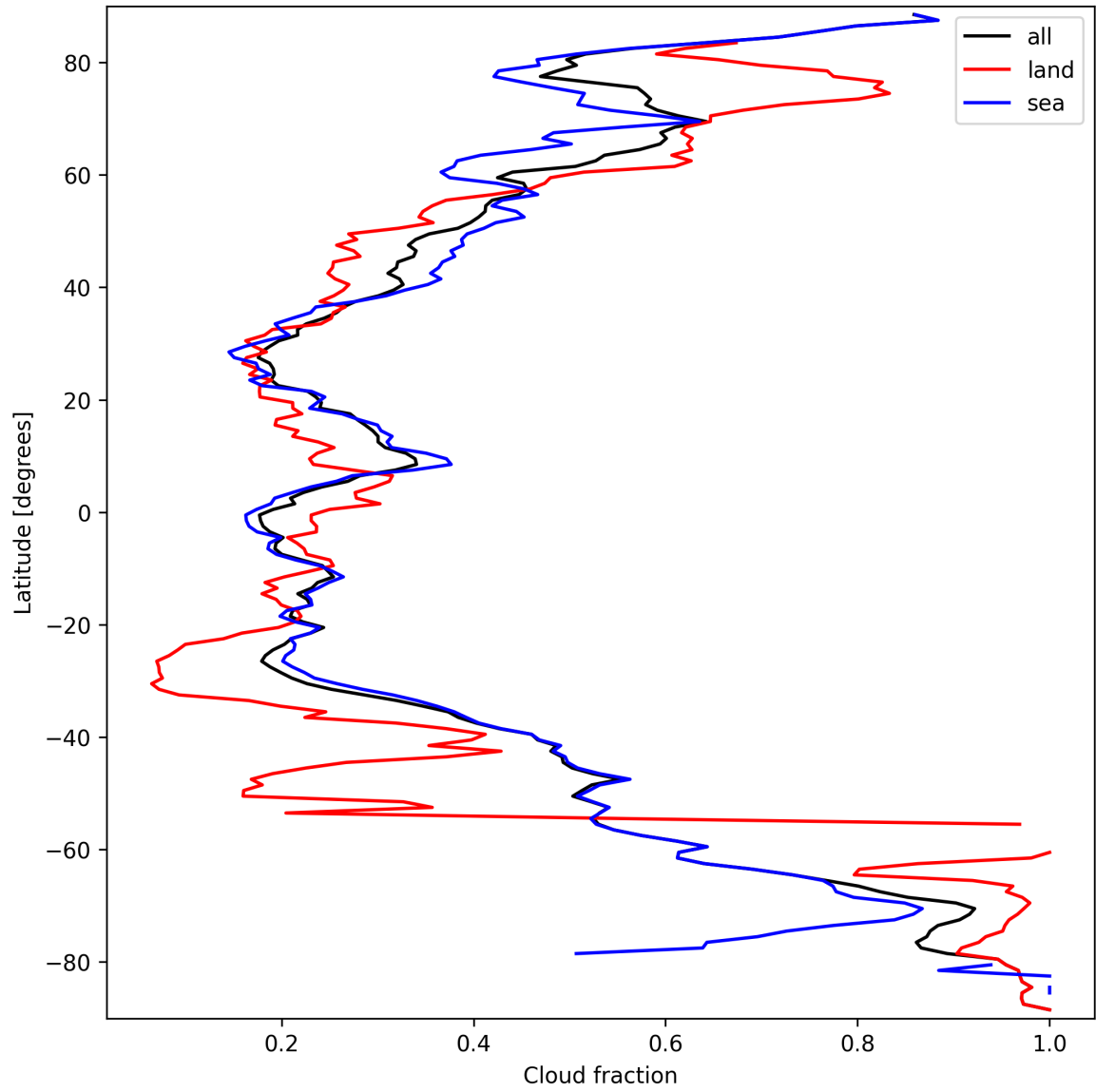
Figure 15: Zonal average of “Cloud fraction” for 2025-09-22 to 2025-09-23.
