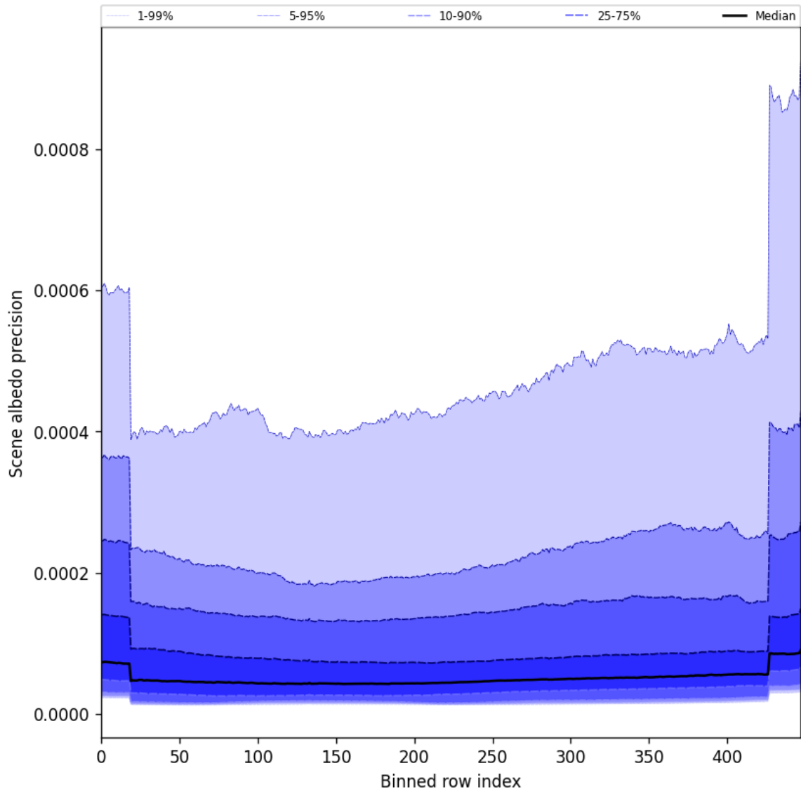
Figure 52: Along track statistics of “Scene albedo precision” for 2025-09-22 to 2025-09-23
