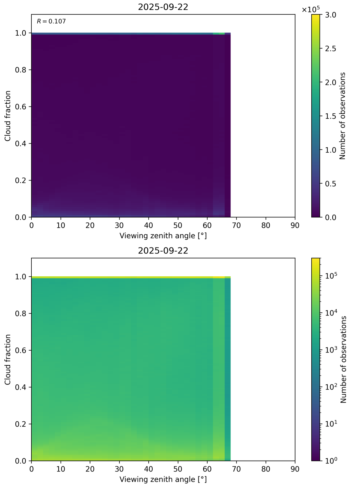
Figure 120: Scatter density plot of “Viewing zenith angle” against “Cloud fraction” for 2025-09-22 to 2025-09-23.
