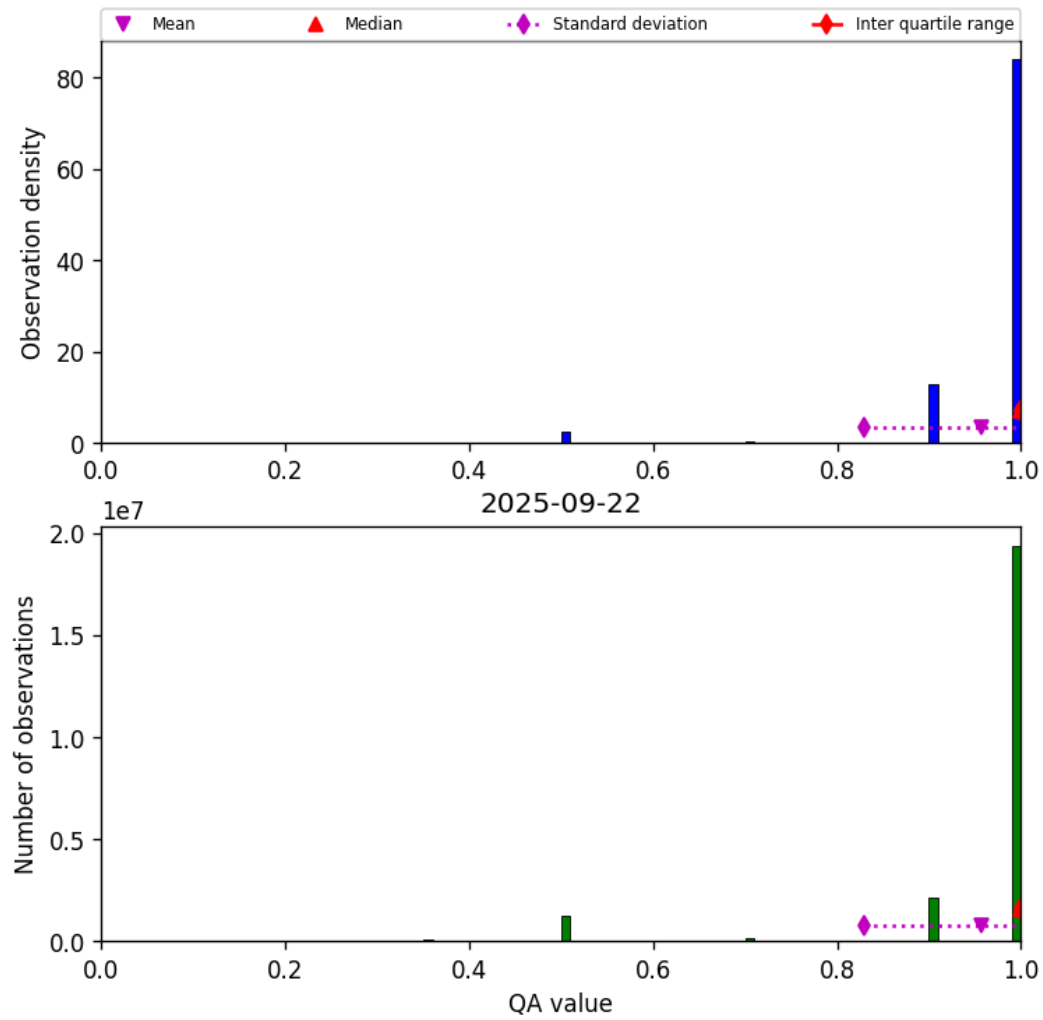
Figure 29: Histogram of “QA value” for 2025-09-22 to 2025-09-23
