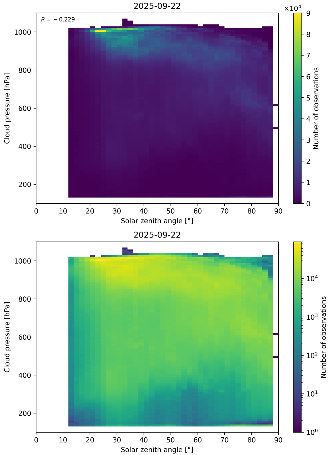
Figure 111: Scatter density plot of “Solar zenith angle” against “Cloud pressure” for 2025-09-22 to 2025-09-23.
