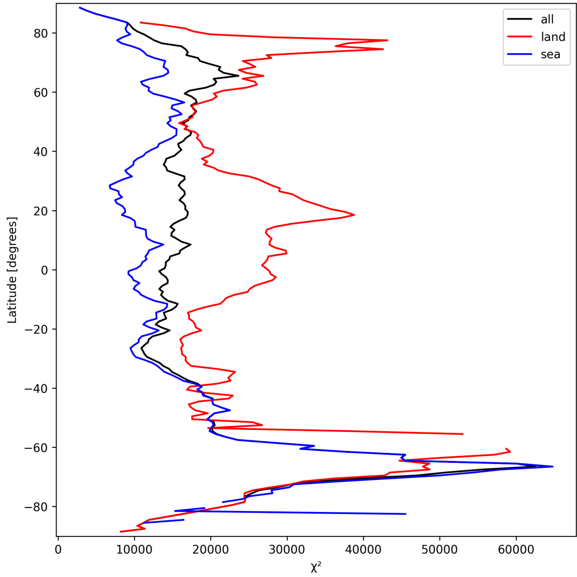
Figure 21: Zonal average of “ \chi^2 ” for 2025-09-22 to 2025-09-23.
