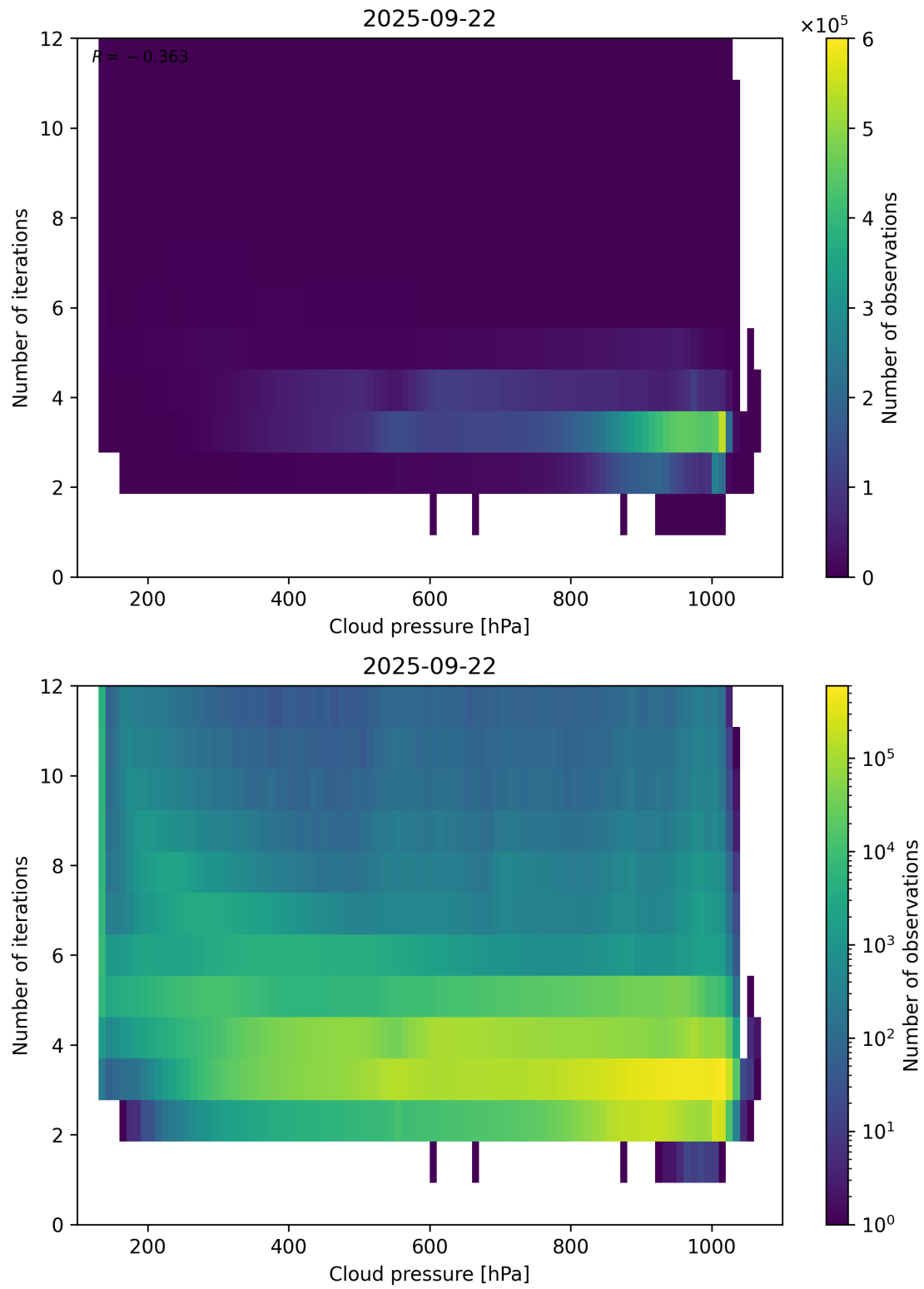
Figure 81: Scatter density plot of “Cloud pressure” against “Number of iterations” for 2025-09-22 to 2025-09-23.
