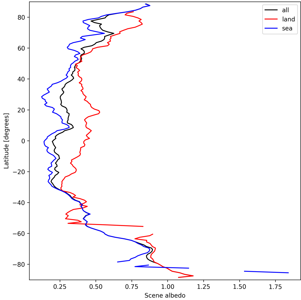
Figure 17: Zonal average of “Scene albedo” for 2025-09-22 to 2025-09-23.
