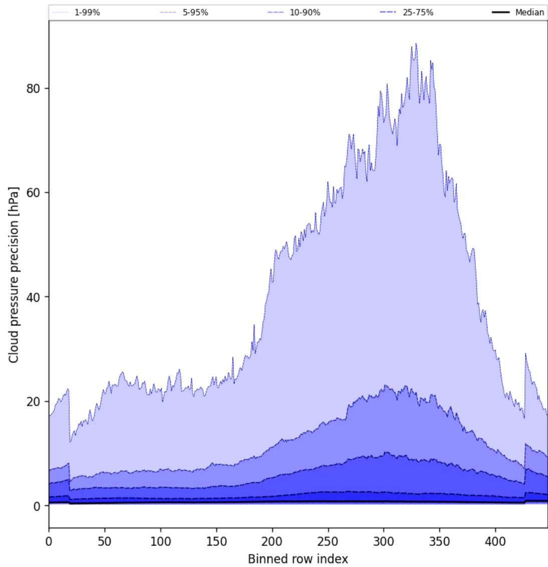
Figure 48: Along track statistics of “Cloud pressure precision” for 2025-09-22 to 2025-09-23
