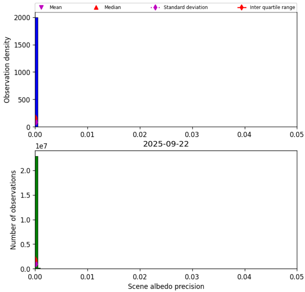
Figure 35: Histogram of “Scene albedo precision” for 2025-09-22 to 2025-09-23
