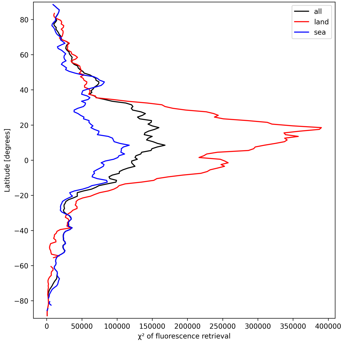
Figure 25: Zonal average of “ \chi^2 of fluorescence retrieval” for 2025-09-22 to 2025-09-23.
