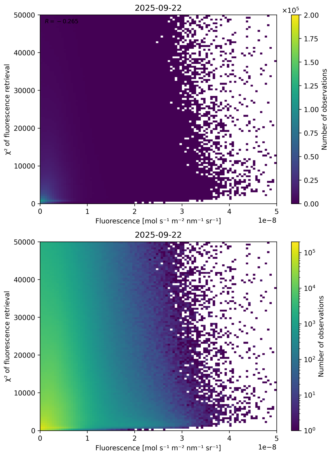
Figure 85: Scatter density plot of “Fluorescence” against “ \chi^2 of fluorescence retrieval” for 2025-09-22 to 2025-09-23.
