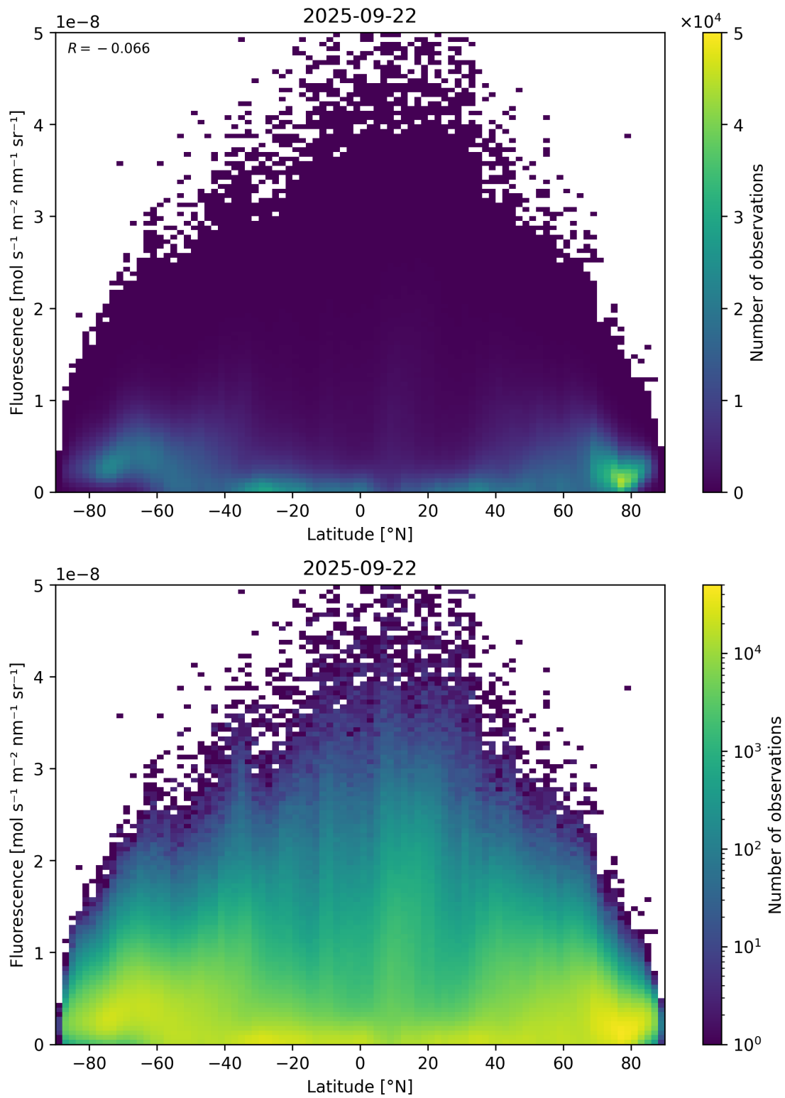
Figure 92: Scatter density plot of “Latitude” against “Fluorescence” for 2025-09-22 to 2025-09-23.
