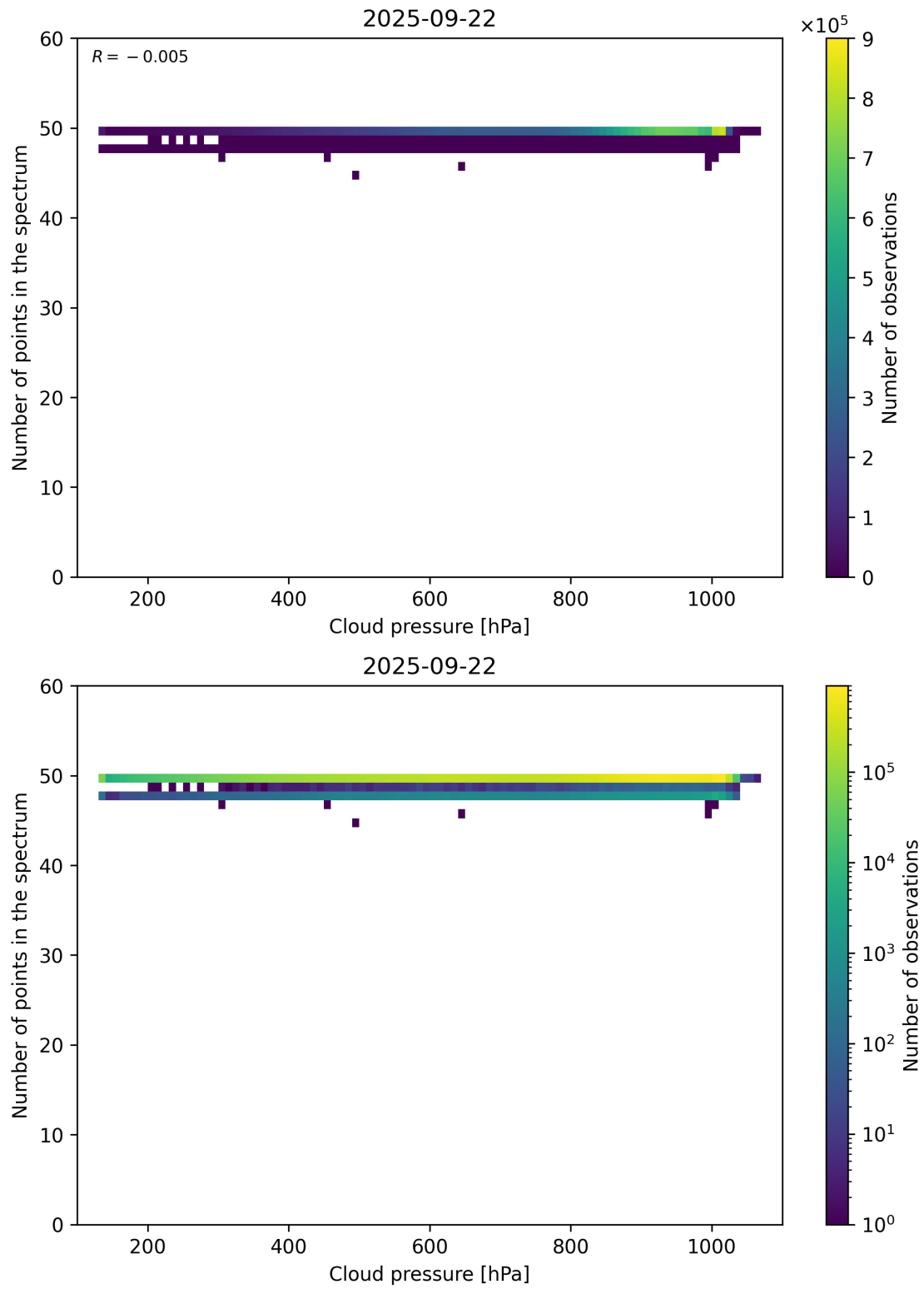
Figure 82: Scatter density plot of “Cloud pressure” against “Number of points in the spectrum” for 2025-09-22 to 2025-09-23.
