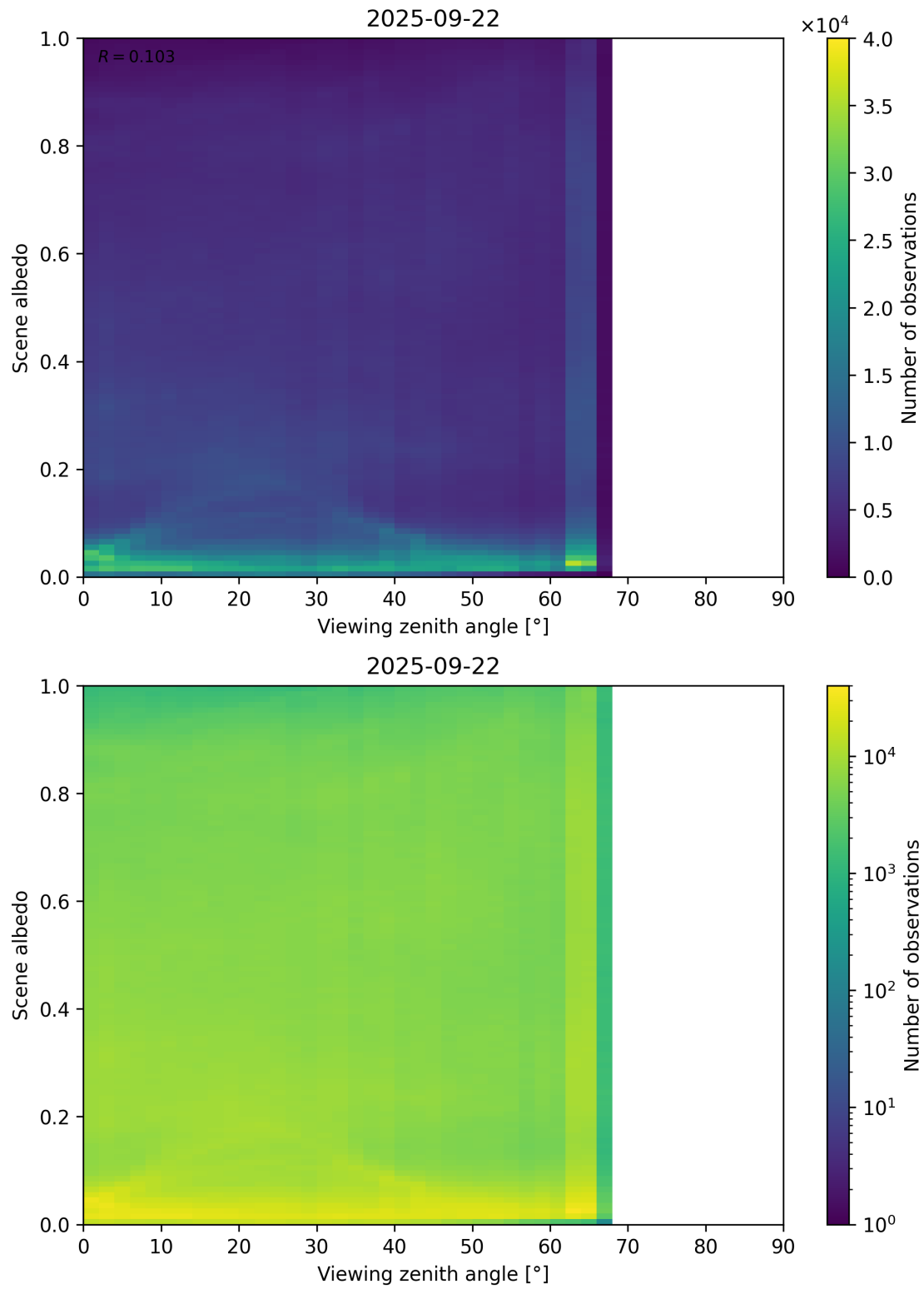
Figure 126: Scatter density plot of “Viewing zenith angle” against “Scene albedo” for 2025-09-22 to 2025-09-23.
