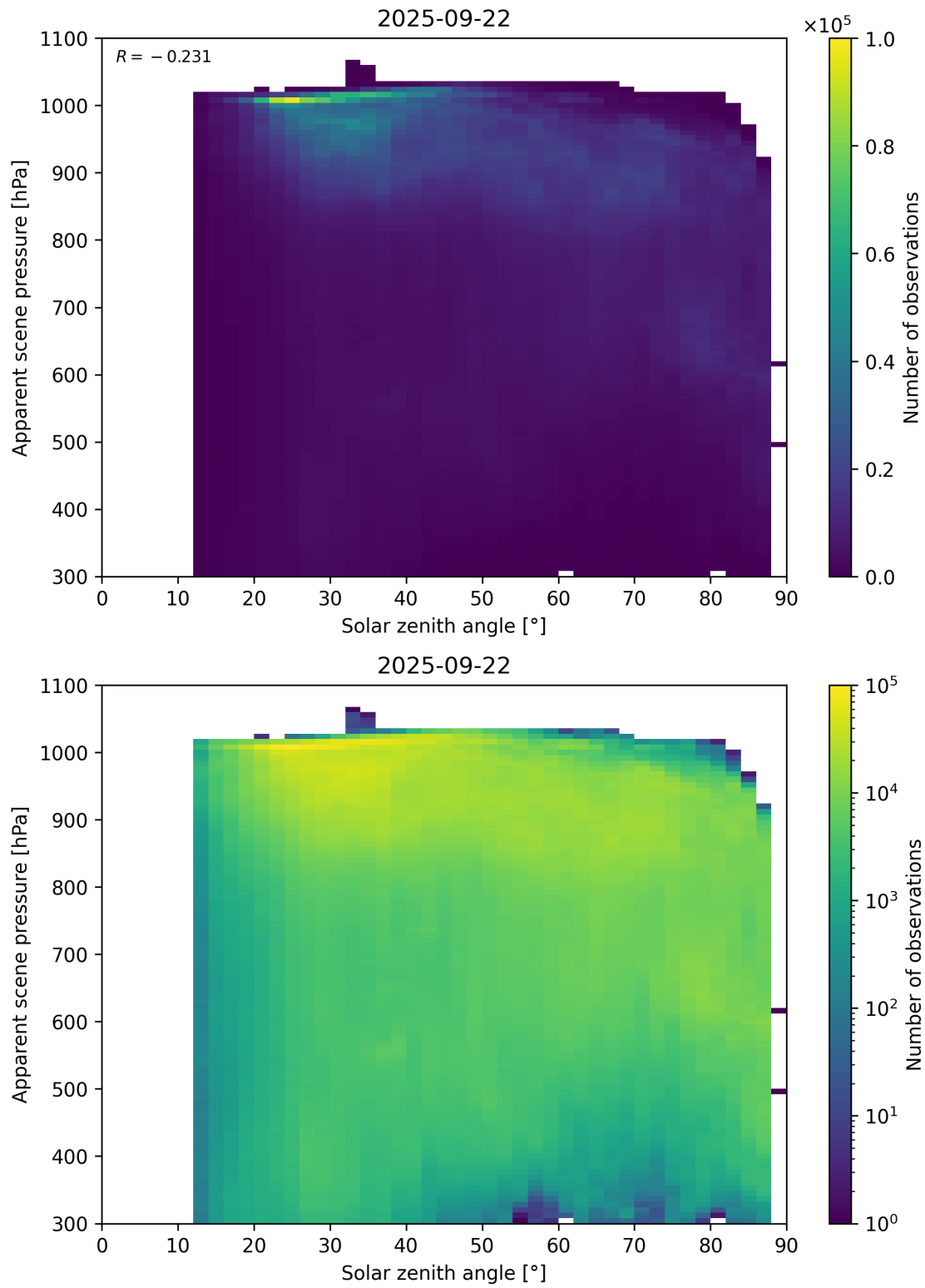
Figure 108: Scatter density plot of “Solar zenith angle” against “Apparent scene pressure” for 2025-09-22 to 2025-09-23.
