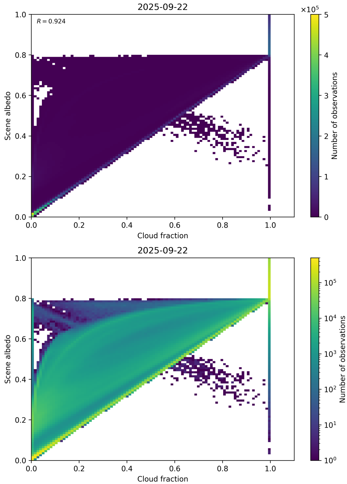
Figure 75: Scatter density plot of “Cloud fraction” against “Scene albedo” for 2025-09-22 to 2025-09-23.
