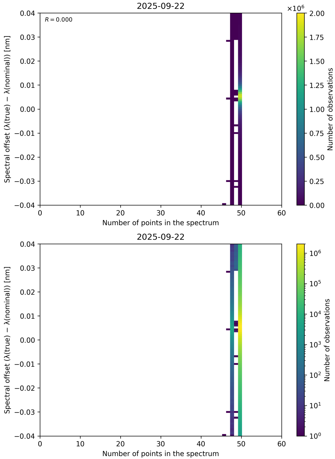
Figure 101: Scatter density plot of “Number of points in the spectrum” against “Spectral offset ( \lambda_{\text{true}} - \lambda_{\text{nominal}} )” for 2025-09-22 to 2025-09-23.
