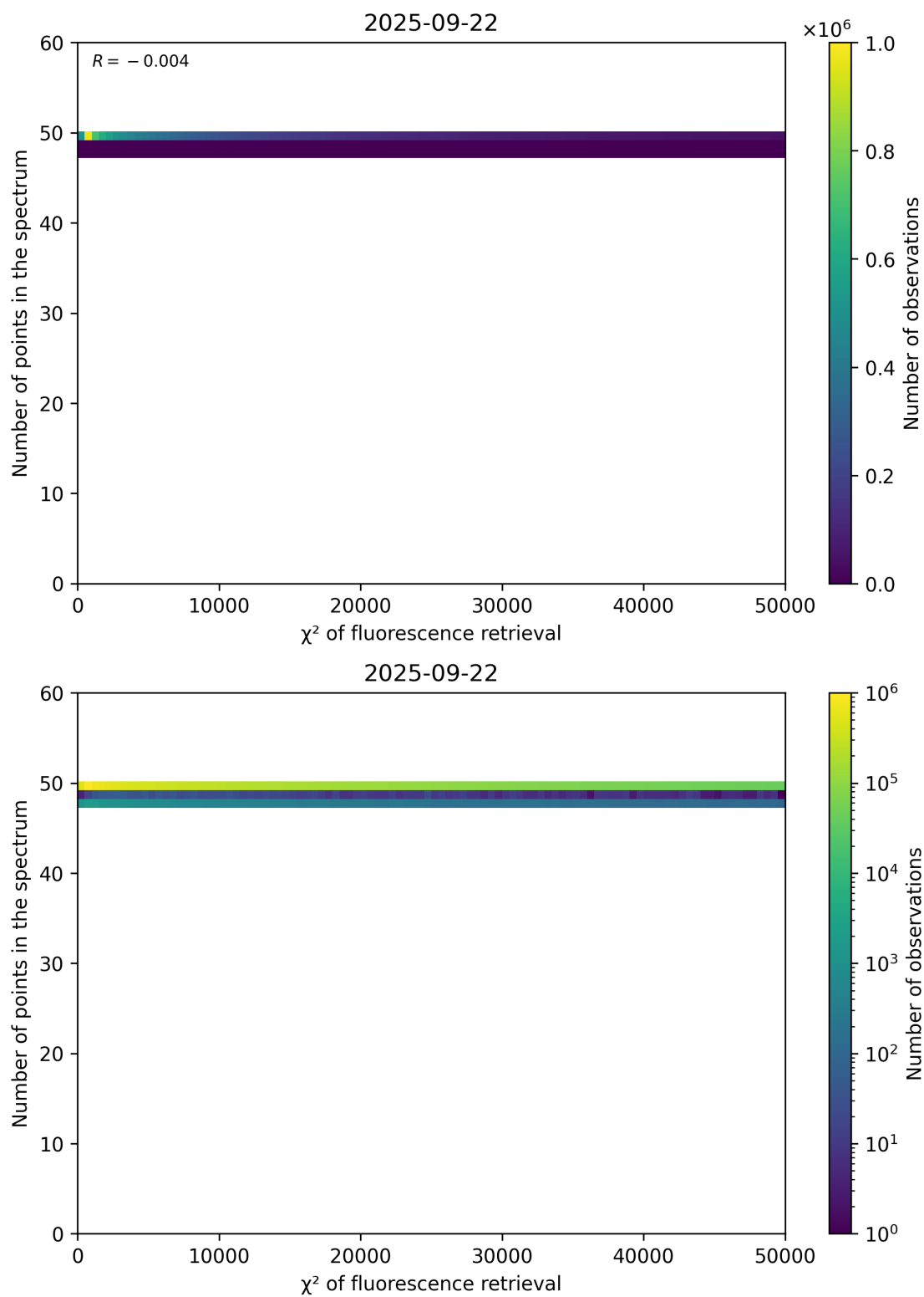
Figure 68: Scatter density plot of “ \chi^2 of fluorescence retrieval” against “Number of points in the spectrum” for 2025-09-22 to 2025-09-23.
