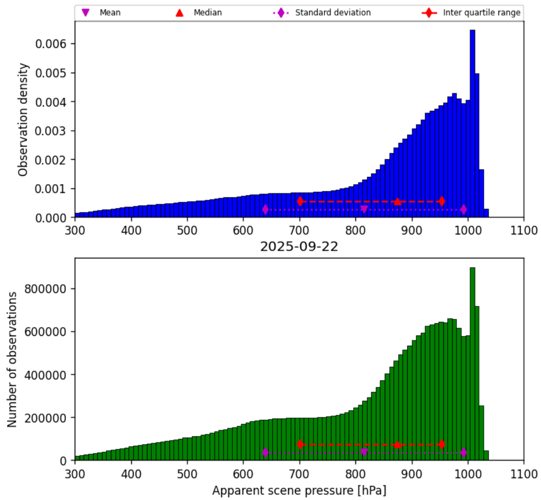
Figure 36: Histogram of “Apparent scene pressure” for 2025-09-22 to 2025-09-23
