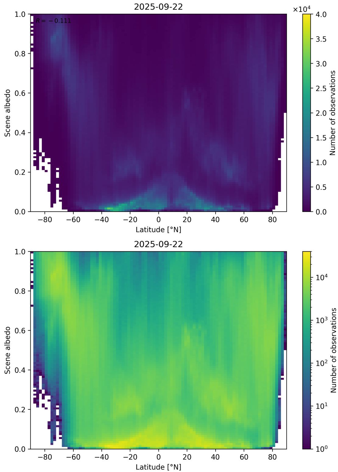
Figure 95: Scatter density plot of “Latitude” against “Scene albedo” for 2025-09-22 to 2025-09-23.
