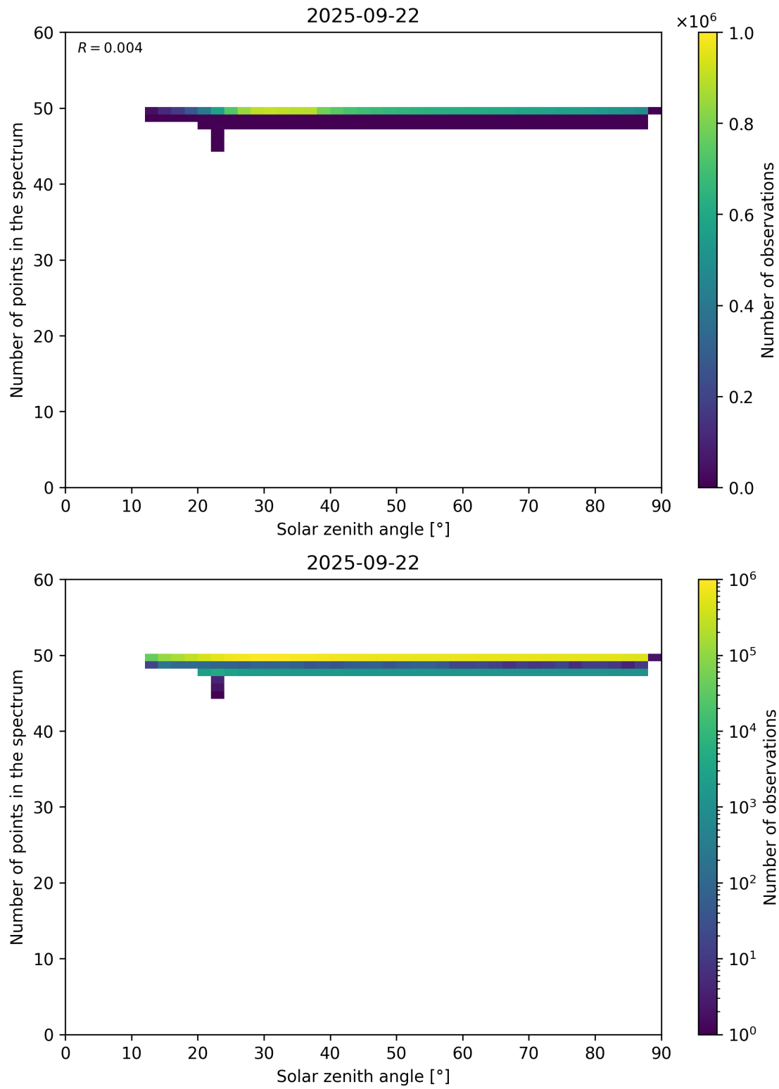
Figure 115: Scatter density plot of “Solar zenith angle” against “Number of points in the spectrum” for 2025-09-22 to 2025-09-23.
