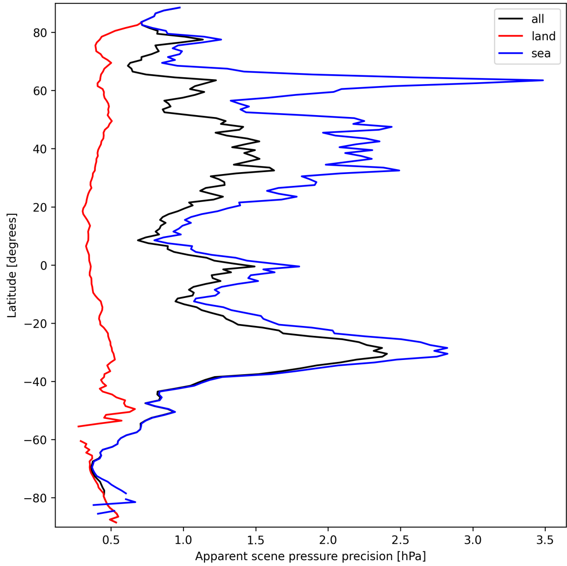
Figure 20: Zonal average of “Apparent scene pressure precision” for 2025-09-22 to 2025-09-23.
