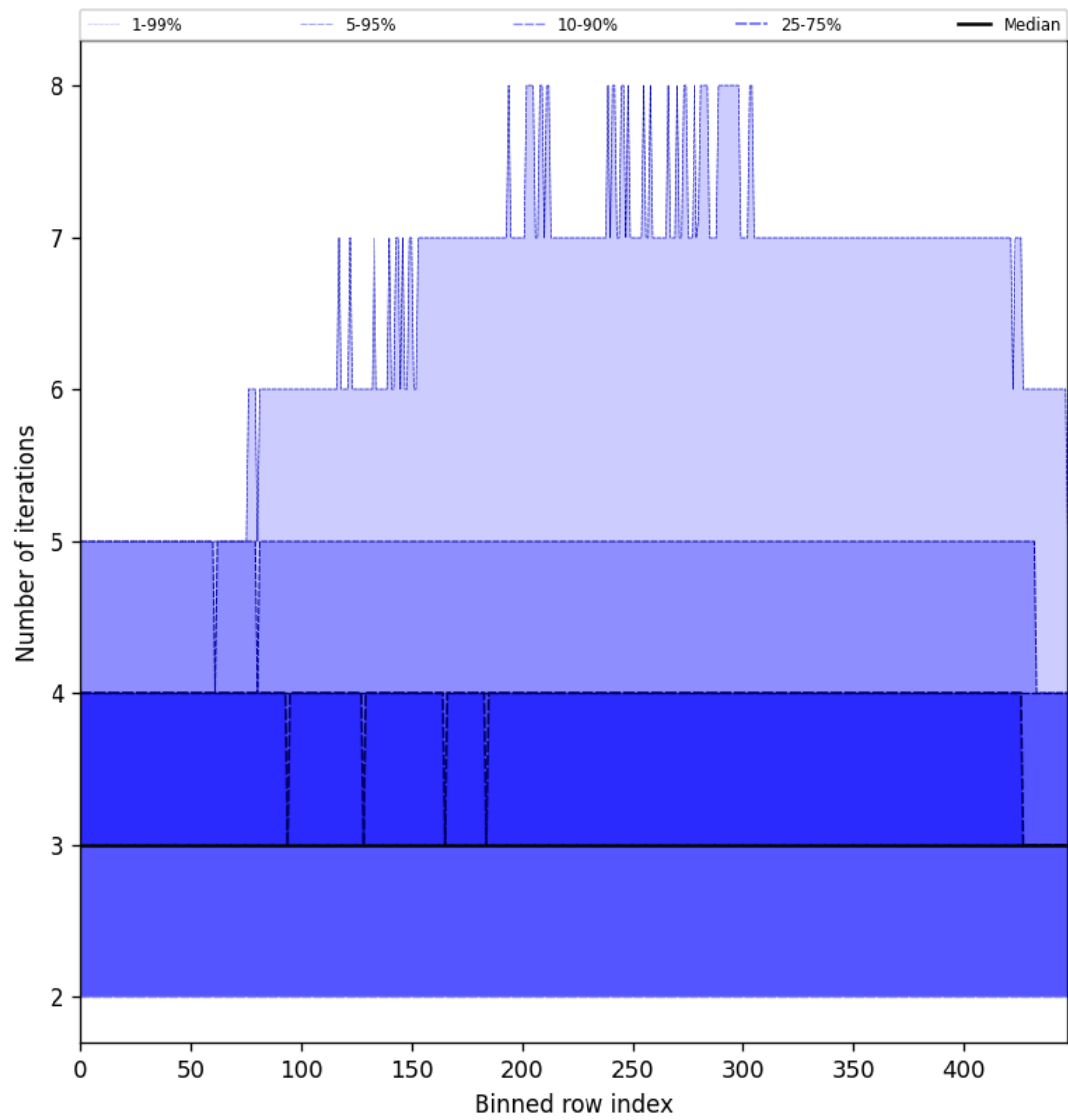
Figure 56: Along track statistics of “Number of iterations” for 2025-09-22 to 2025-09-23
