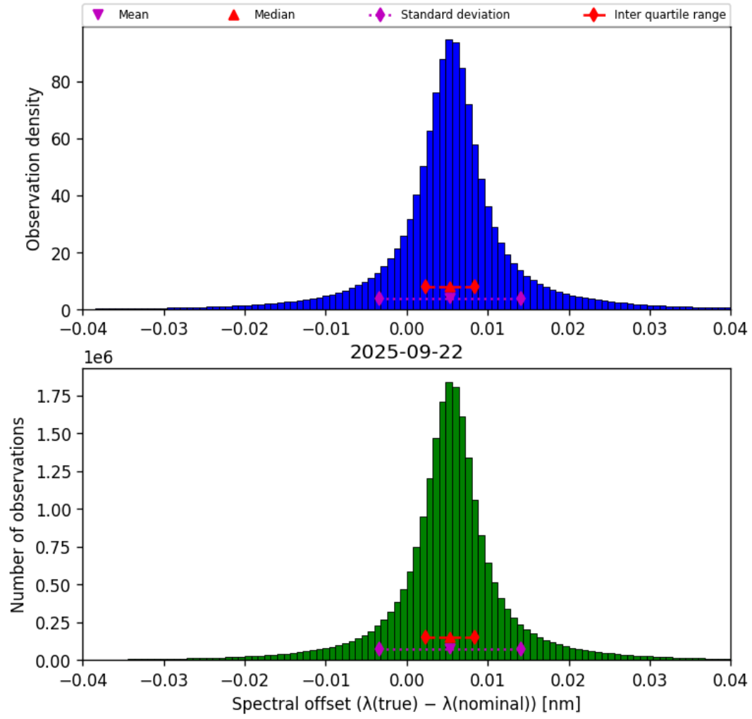
Figure 45: Histogram of “Spectral offset ( \lambda_{\text{true}} - \lambda_{\text{nominal}} )” for 2025-09-22 to 2025-09-23
