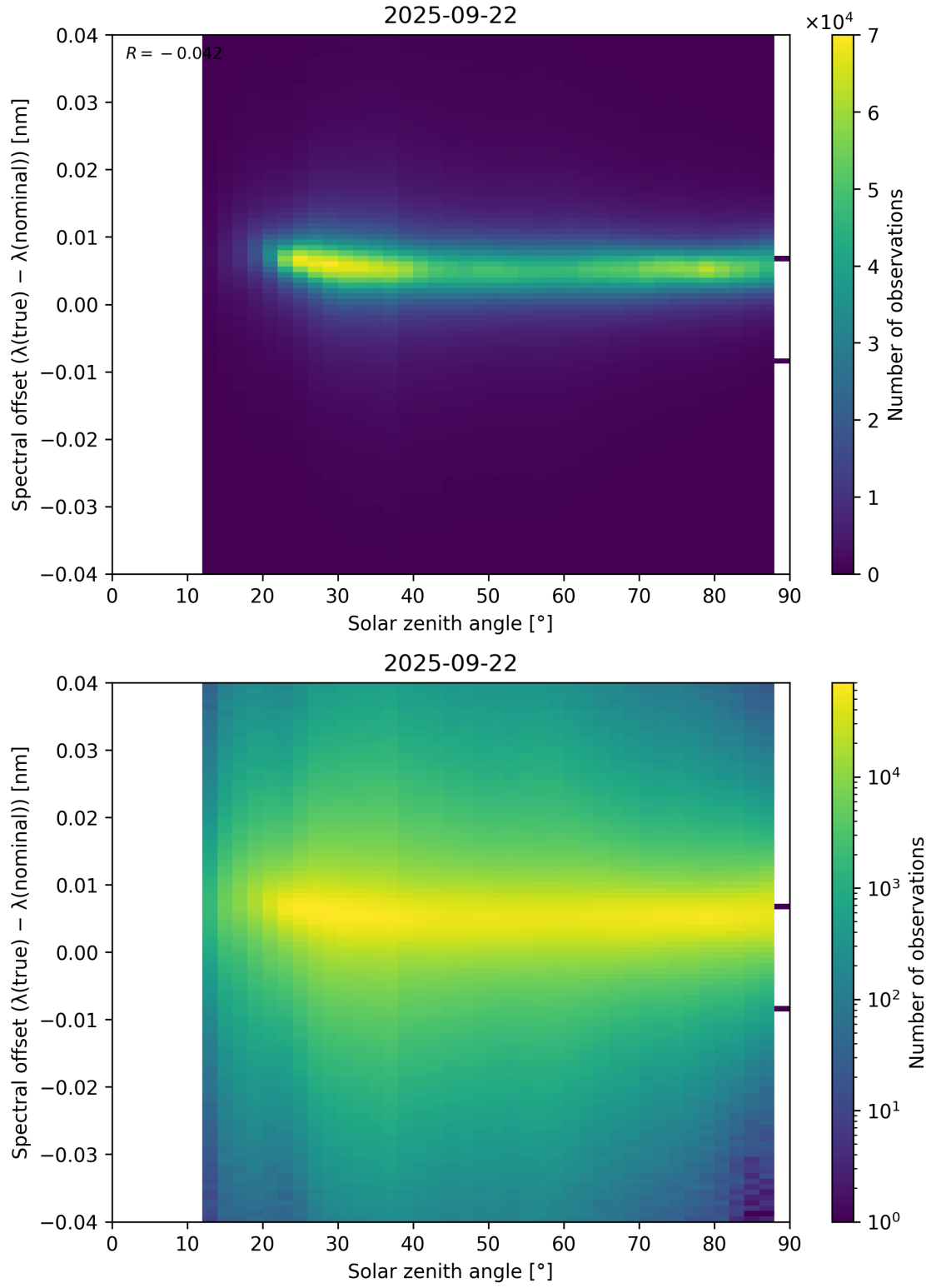
Figure 117: Scatter density plot of “Solar zenith angle” against “Spectral offset ( \lambda_{\text{true}} - \lambda_{\text{nominal}} )” for 2025-09-22 to 2025-09-23.
