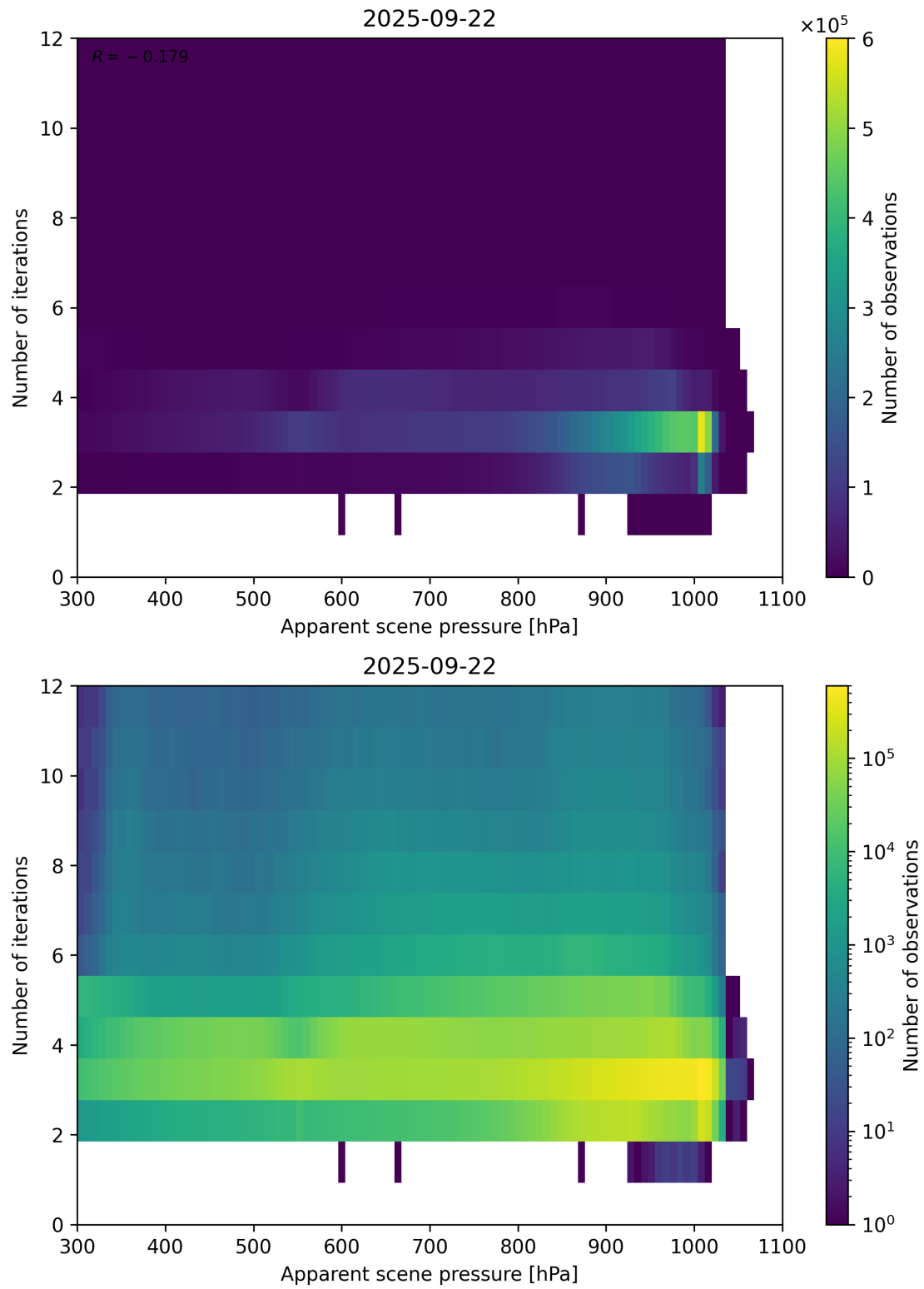
Figure 65: Scatter density plot of “Apparent scene pressure” against “Number of iterations” for 2025-09-22 to 2025-09-23.
