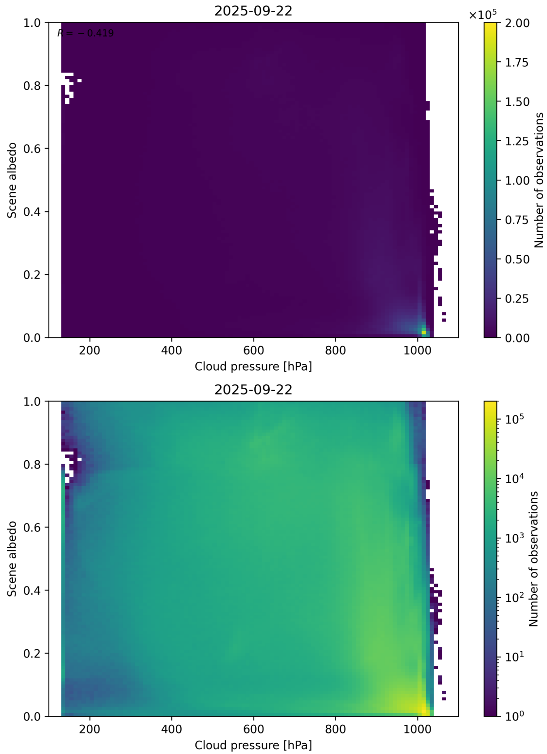
Figure 83: Scatter density plot of “Cloud pressure” against “Scene albedo” for 2025-09-22 to 2025-09-23.
