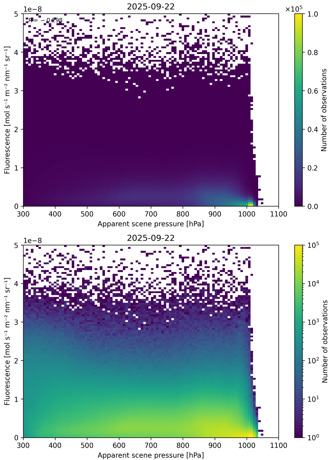
Figure 64: Scatter density plot of “Apparent scene pressure” against “Fluorescence” for 2025-09-22 to 2025-09-23.
