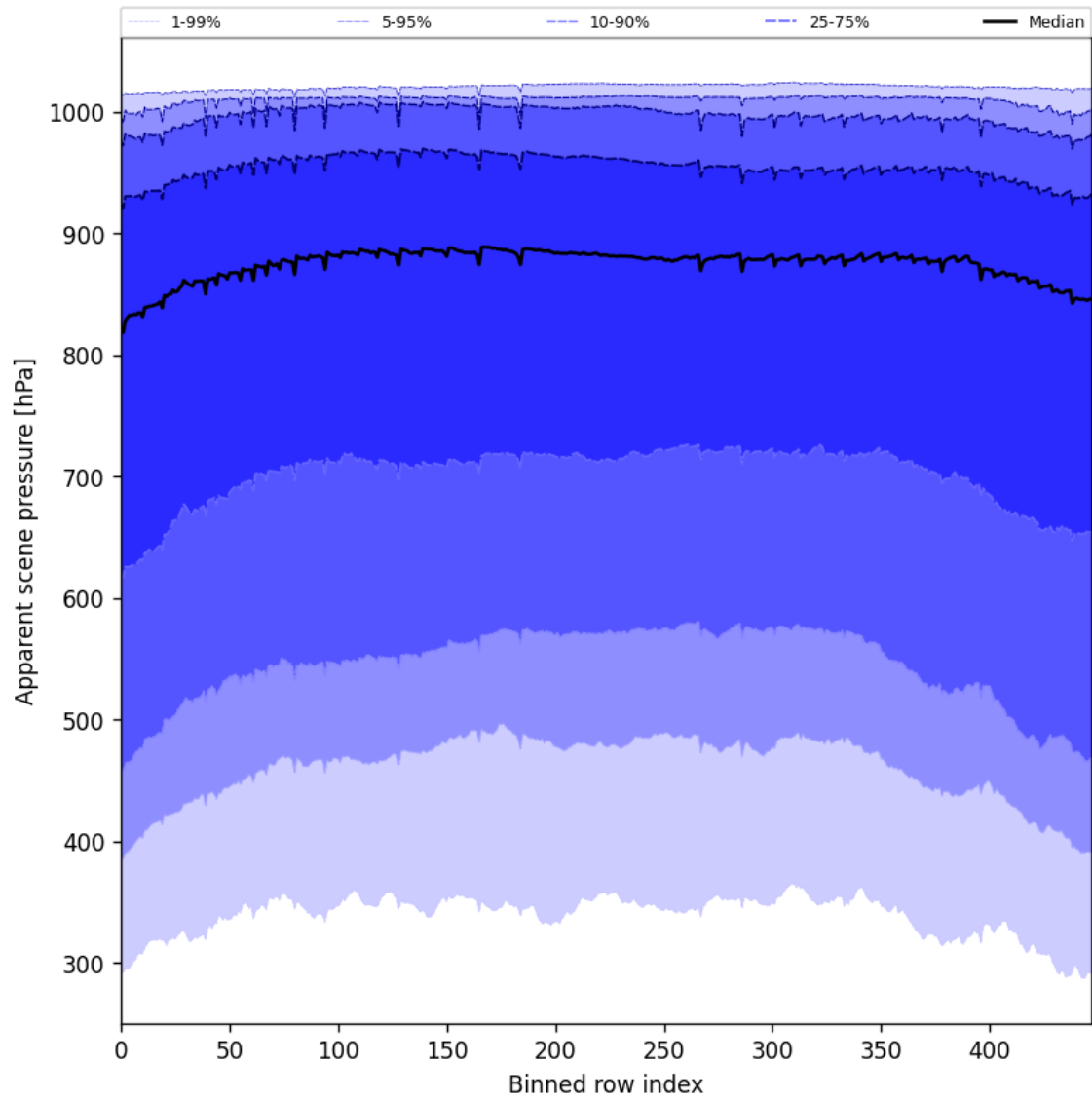
Figure 53: Along track statistics of “Apparent scene pressure” for 2025-09-22 to 2025-09-23
