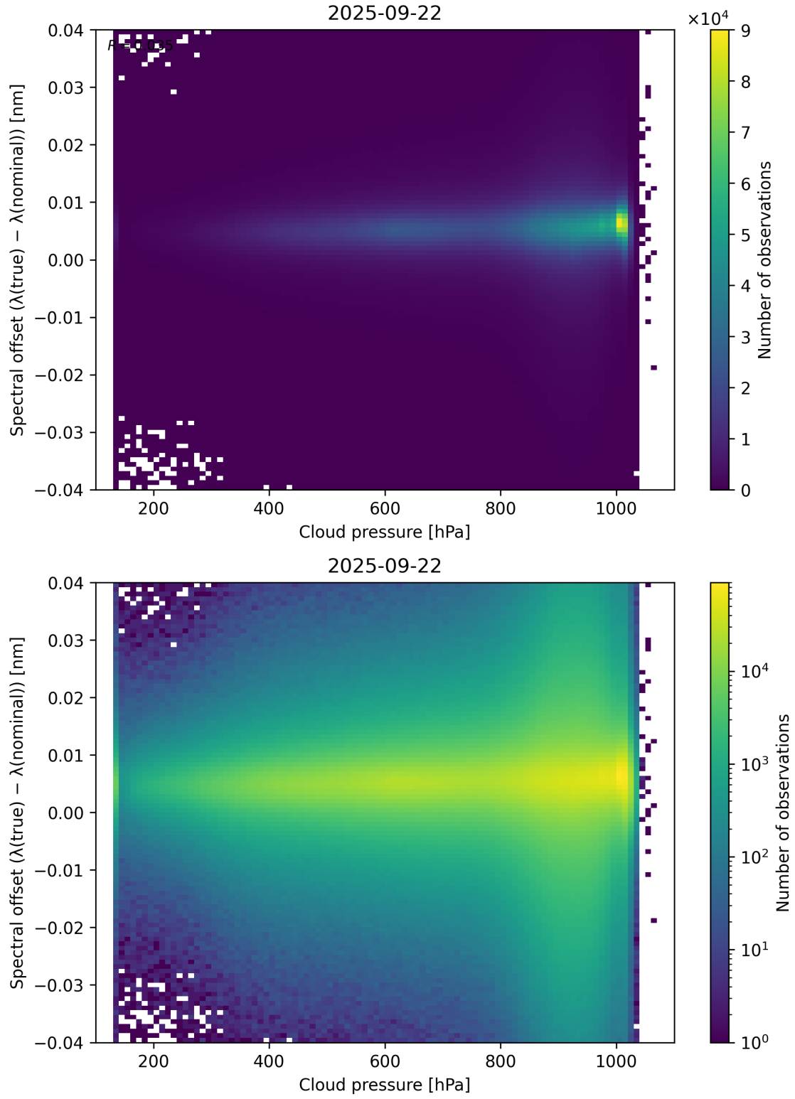
Figure 84: Scatter density plot of “Cloud pressure” against “Spectral offset ( \lambda_{\text{true}} - \lambda_{\text{nominal}} )” for 2025-09-22 to 2025-09-23.
