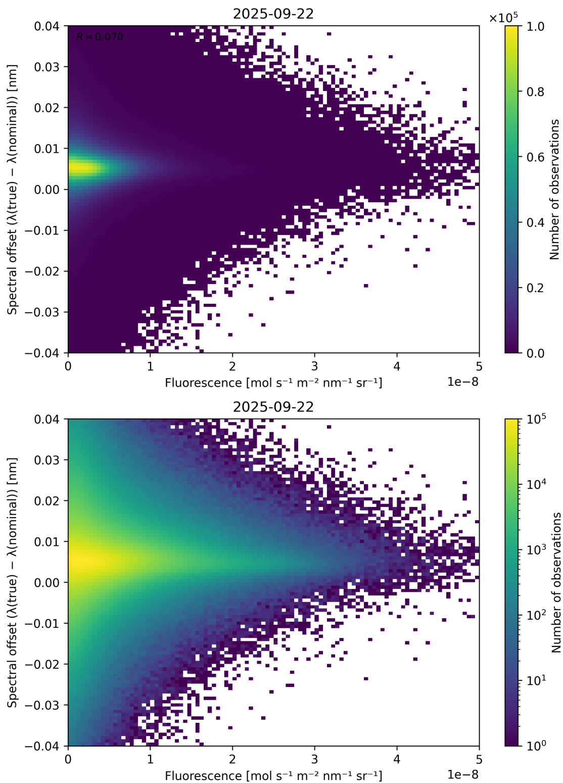
Figure 87: Scatter density plot of “Fluorescence” against “Spectral offset ( \lambda_{\text{true}} - \lambda_{\text{nominal}} )” for 2025-09-22 to 2025-09-23.
