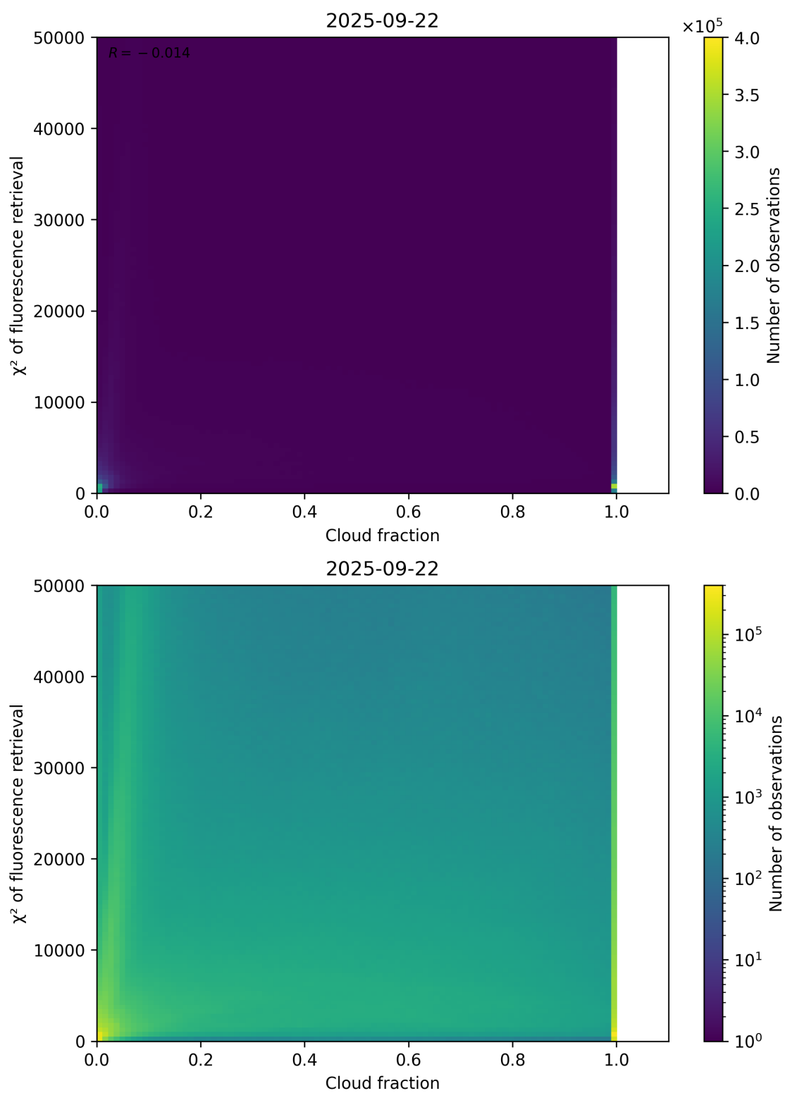
Figure 71: Scatter density plot of “Cloud fraction” against “ \chi^2 of fluorescence retrieval” for 2025-09-22 to 2025-09-23.
