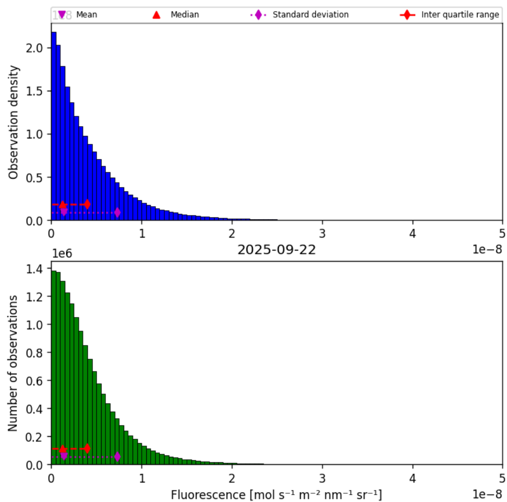
Figure 40: Histogram of “Fluorescence” for 2025-09-22 to 2025-09-23
