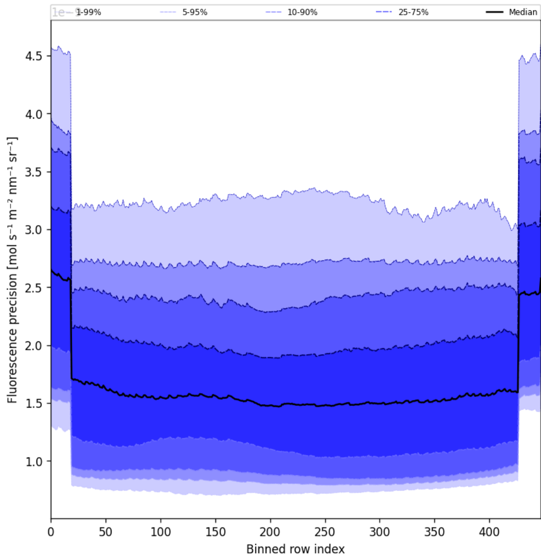
Figure 58: Along track statistics of “Fluorescence precision” for 2025-09-22 to 2025-09-23
