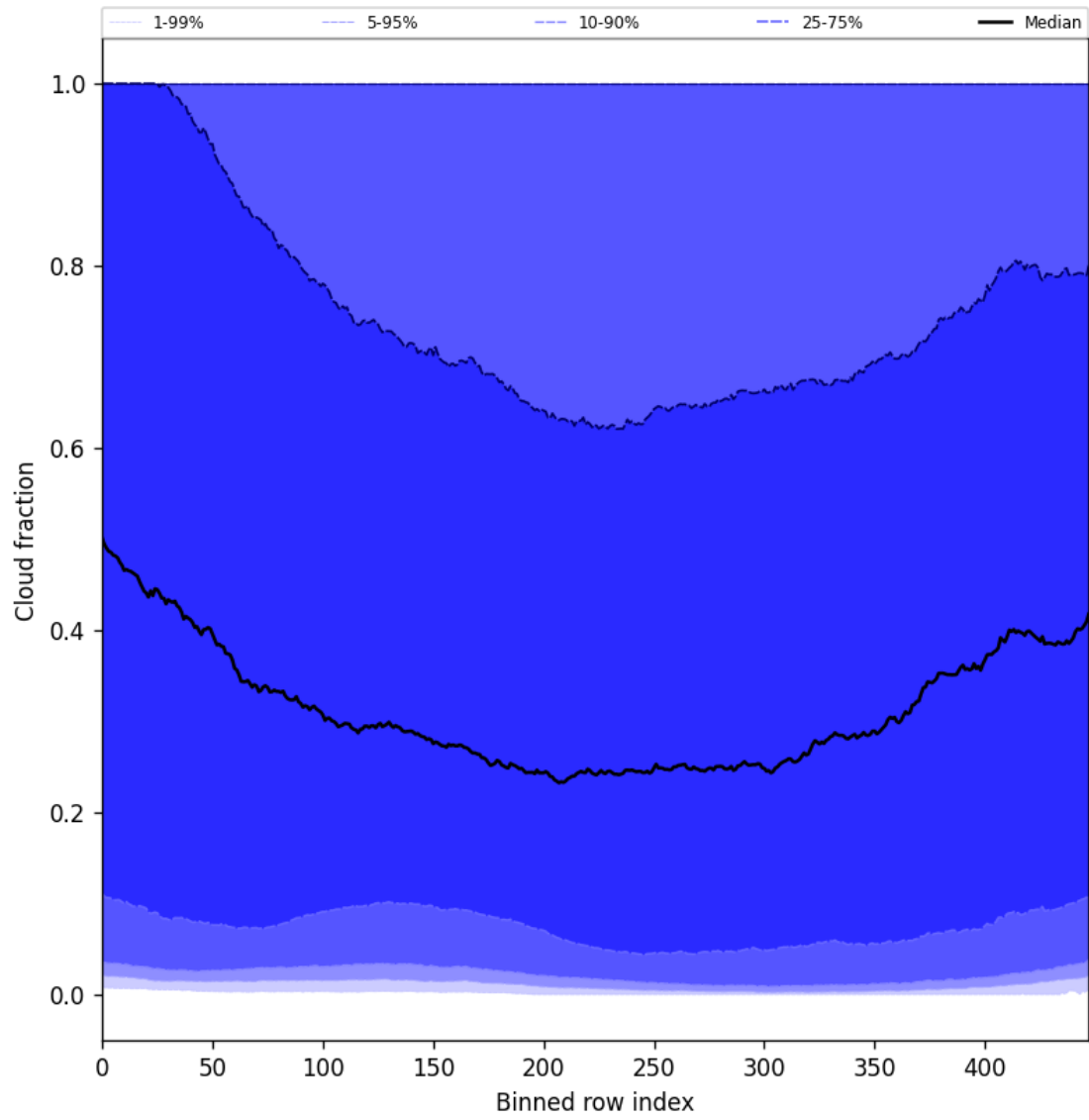
Figure 49: Along track statistics of “Cloud fraction” for 2025-09-22 to 2025-09-23
