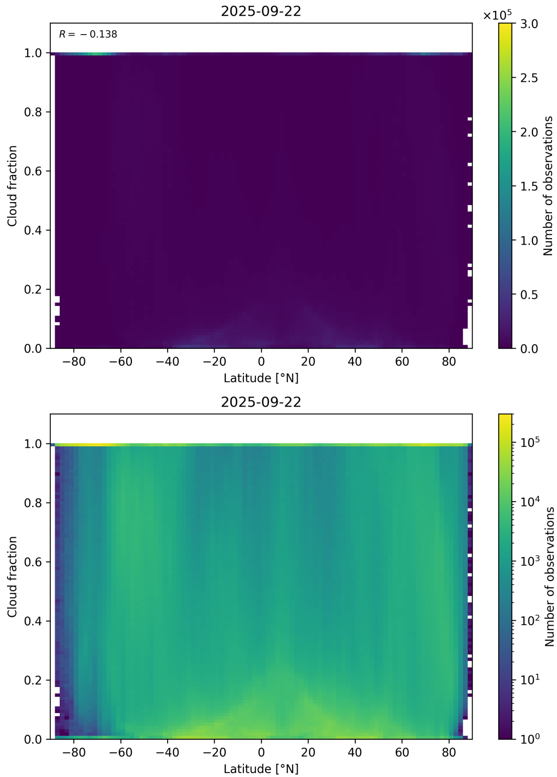
Figure 90: Scatter density plot of “Latitude” against “Cloud fraction” for 2025-09-22 to 2025-09-23.
