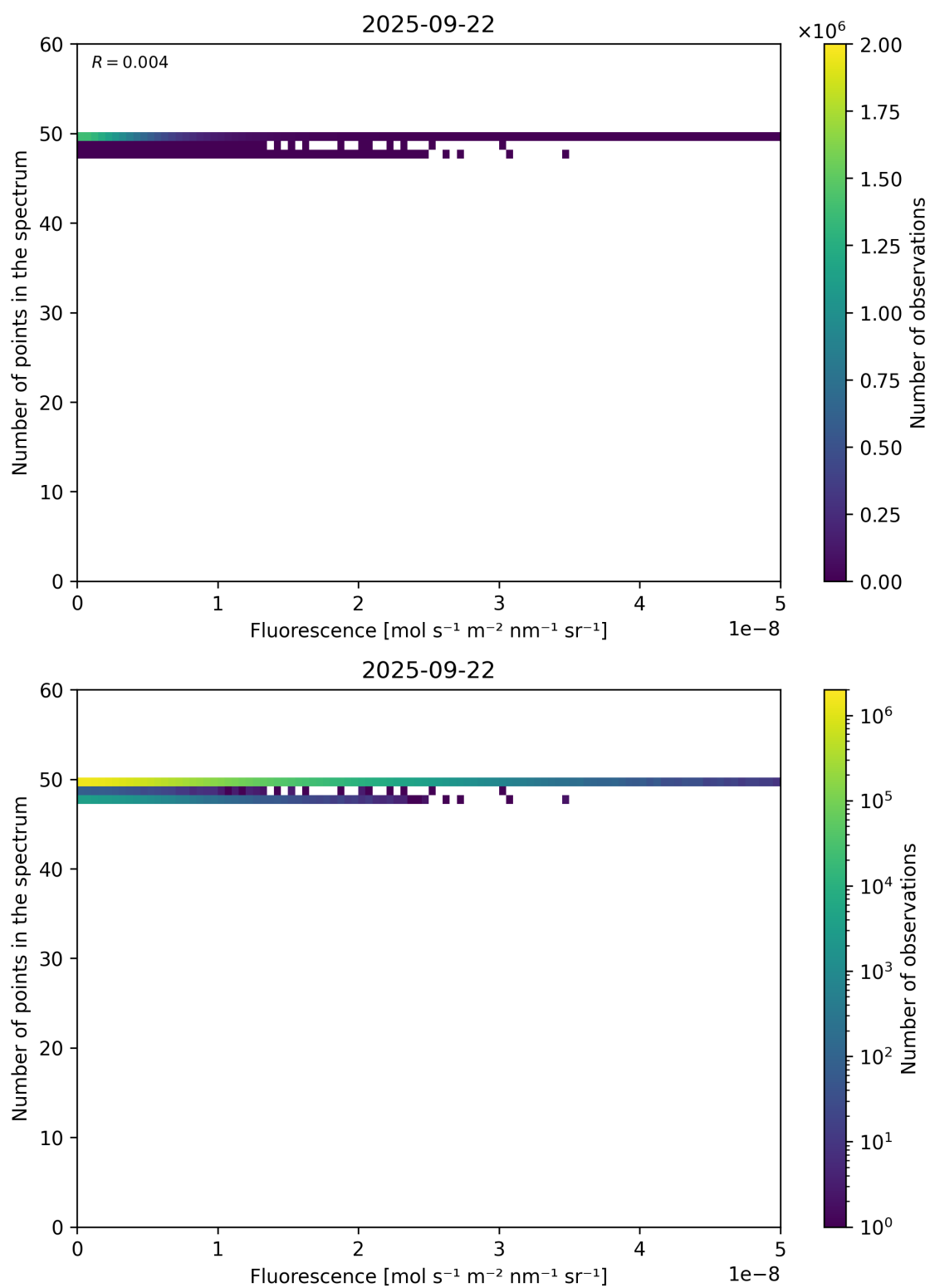
Figure 86: Scatter density plot of “Fluorescence” against “Number of points in the spectrum” for 2025-09-22 to 2025-09-23.
