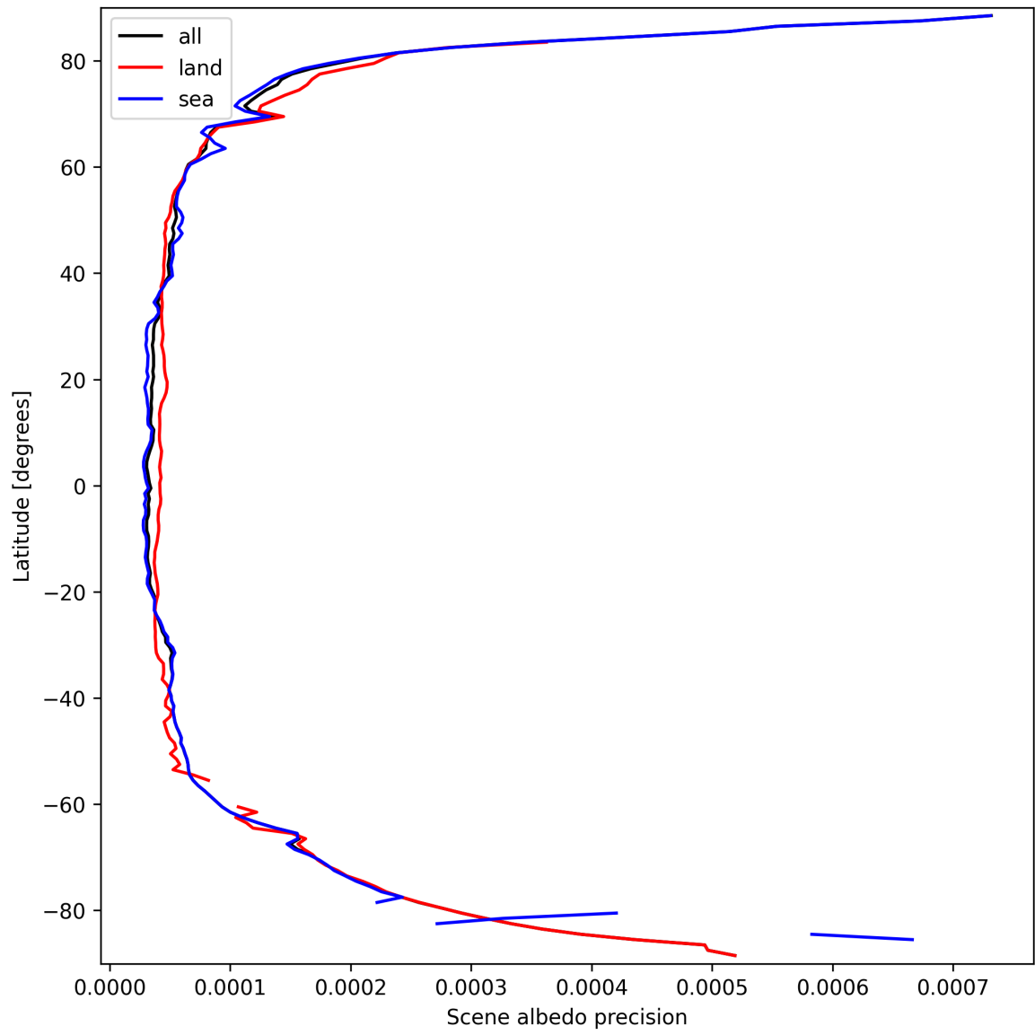
Figure 18: Zonal average of “Scene albedo precision” for 2025-09-22 to 2025-09-23.
