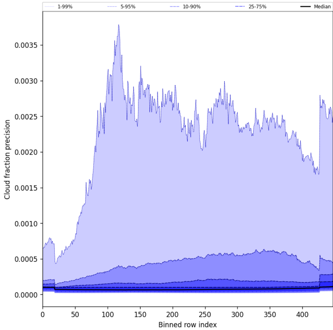
Figure 50: Along track statistics of “Cloud fraction precision” for 2025-09-22 to 2025-09-23
