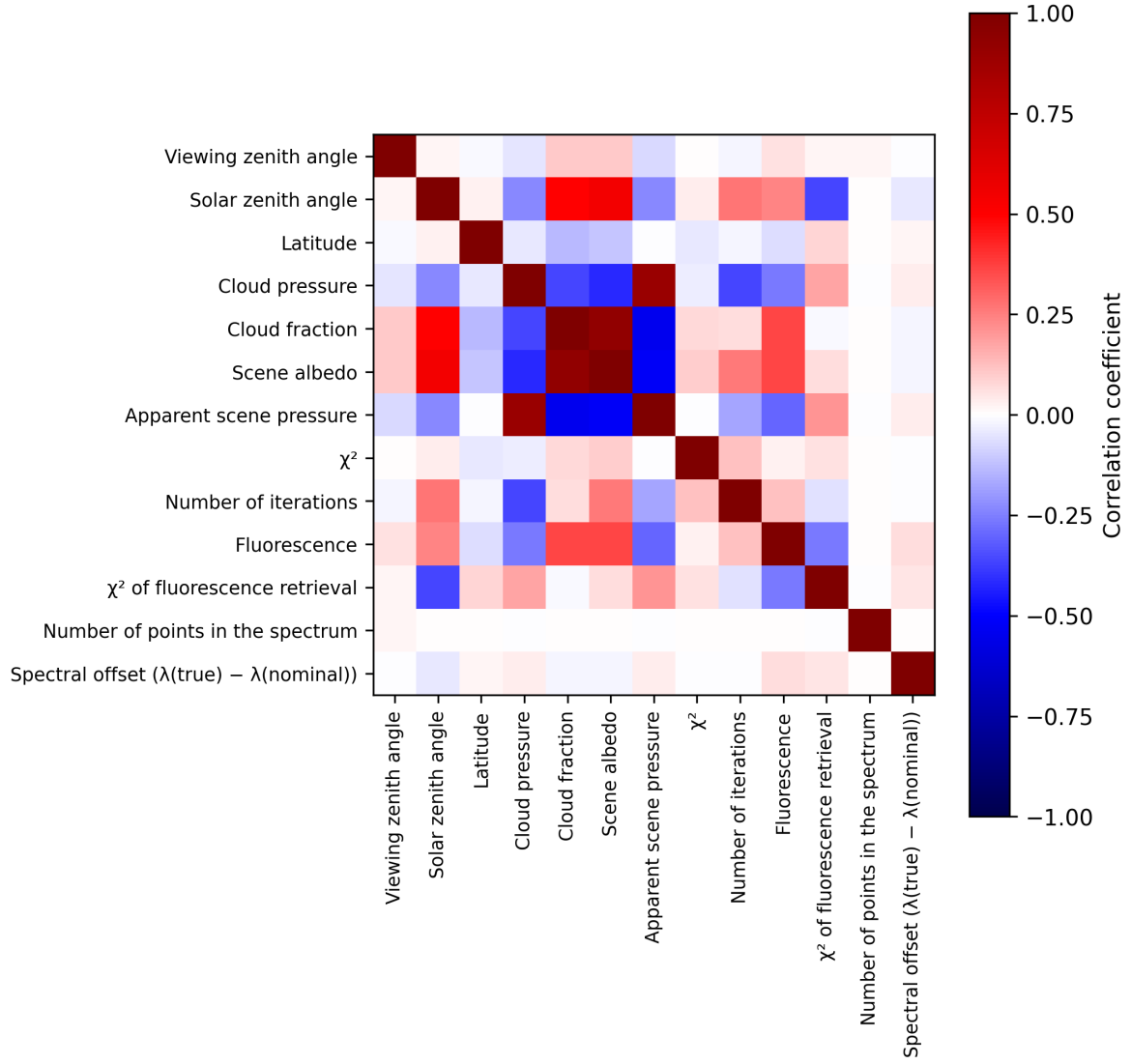
Figure 2: Map of correlation matrix for 2025-09-22 to 2025-09-23.
