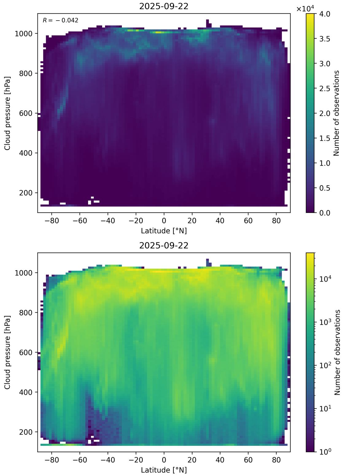
Figure 91: Scatter density plot of “Latitude” against “Cloud pressure” for 2025-09-22 to 2025-09-23.
