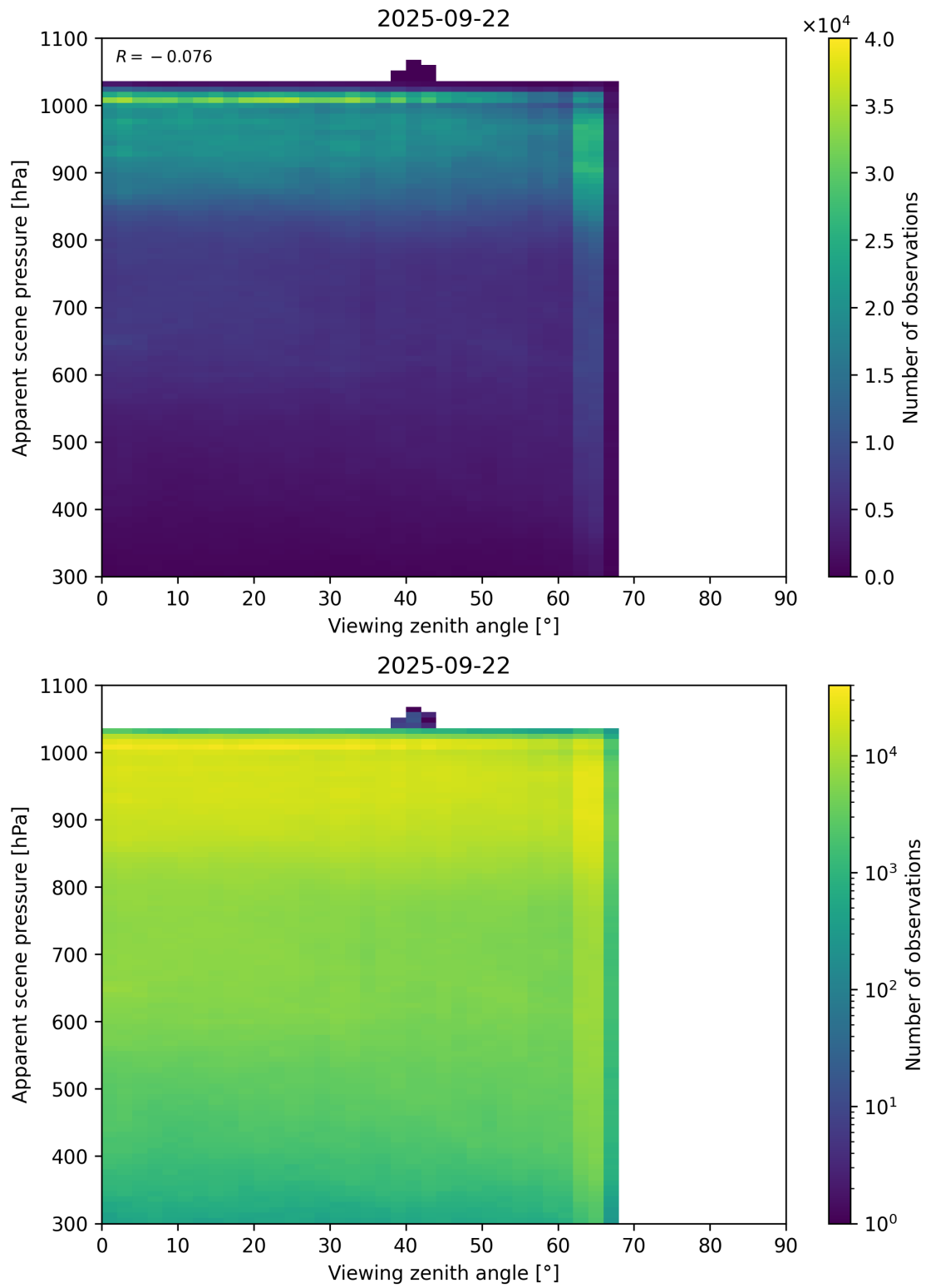
Figure 118: Scatter density plot of “Viewing zenith angle” against “Apparent scene pressure” for 2025-09-22 to 2025-09-23.
