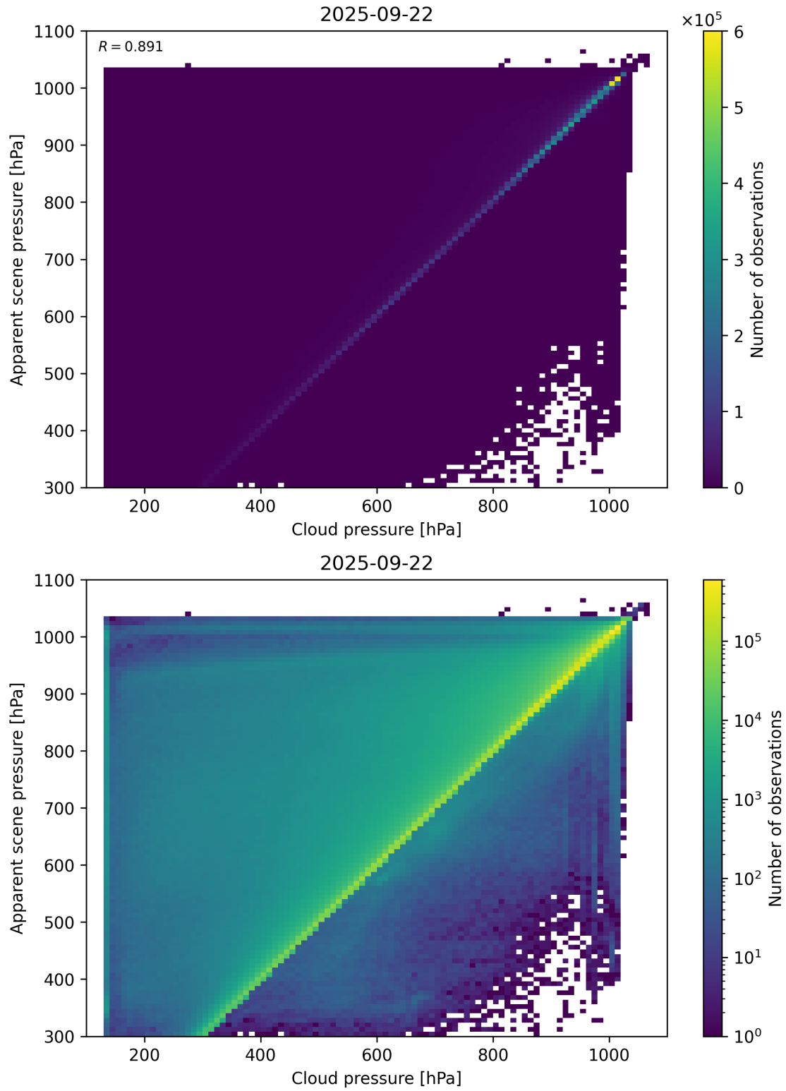
Figure 77: Scatter density plot of “Cloud pressure” against “Apparent scene pressure” for 2025-09-22 to 2025-09-23.
