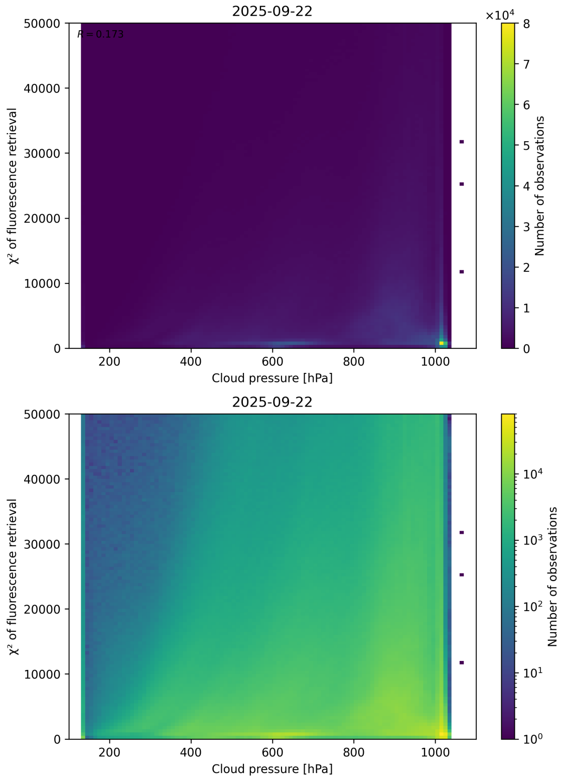
Figure 78: Scatter density plot of “Cloud pressure” against “ \chi^2 of fluorescence retrieval” for 2025-09-22 to 2025-09-23.
