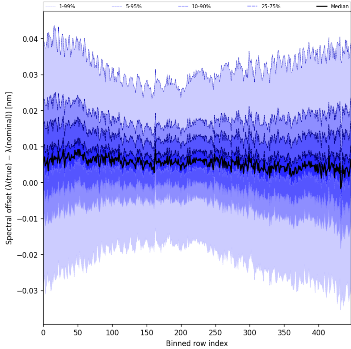
Figure 62: Along track statistics of “Spectral offset ( \lambda_{\text{true}} - \lambda_{\text{nominal}} )” for 2025-09-22 to 2025-09-23
