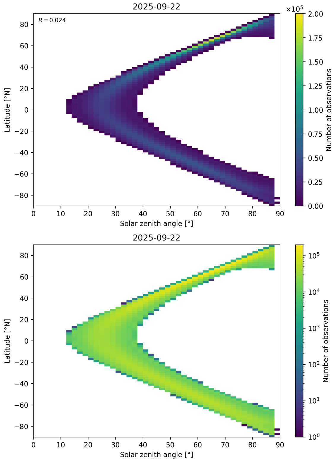
Figure 113: Scatter density plot of “Solar zenith angle” against “Latitude” for 2025-09-22 to 2025-09-23.
