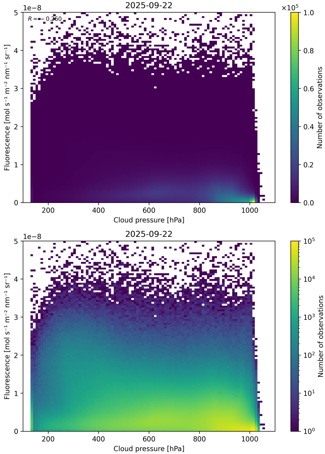
Figure 80: Scatter density plot of “Cloud pressure” against “Fluorescence” for 2025-09-22 to 2025-09-23.
