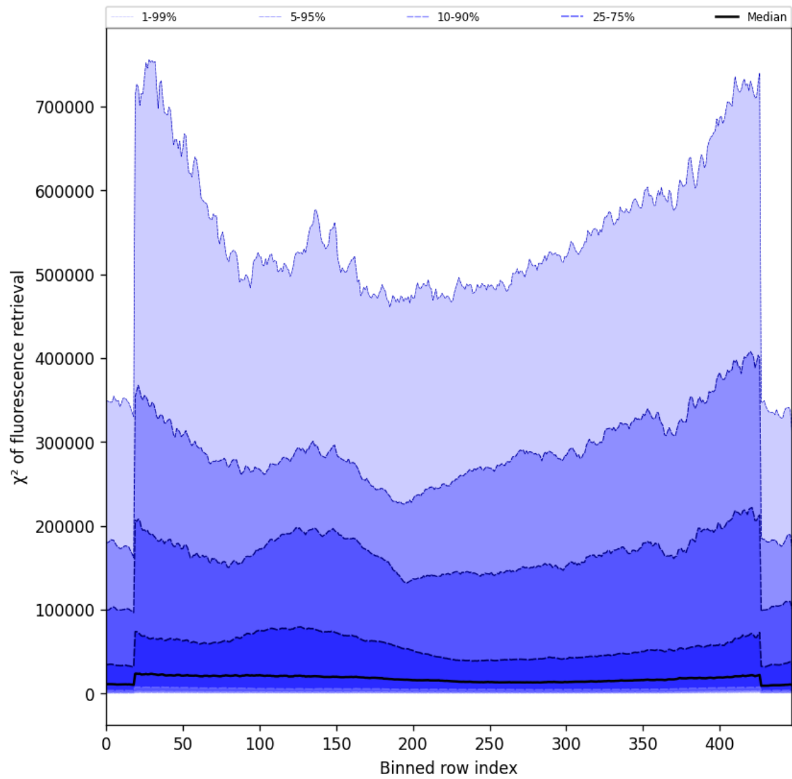
Figure 59: Along track statistics of “ \chi^2 of fluorescence retrieval” for 2025-09-22 to 2025-09-23
