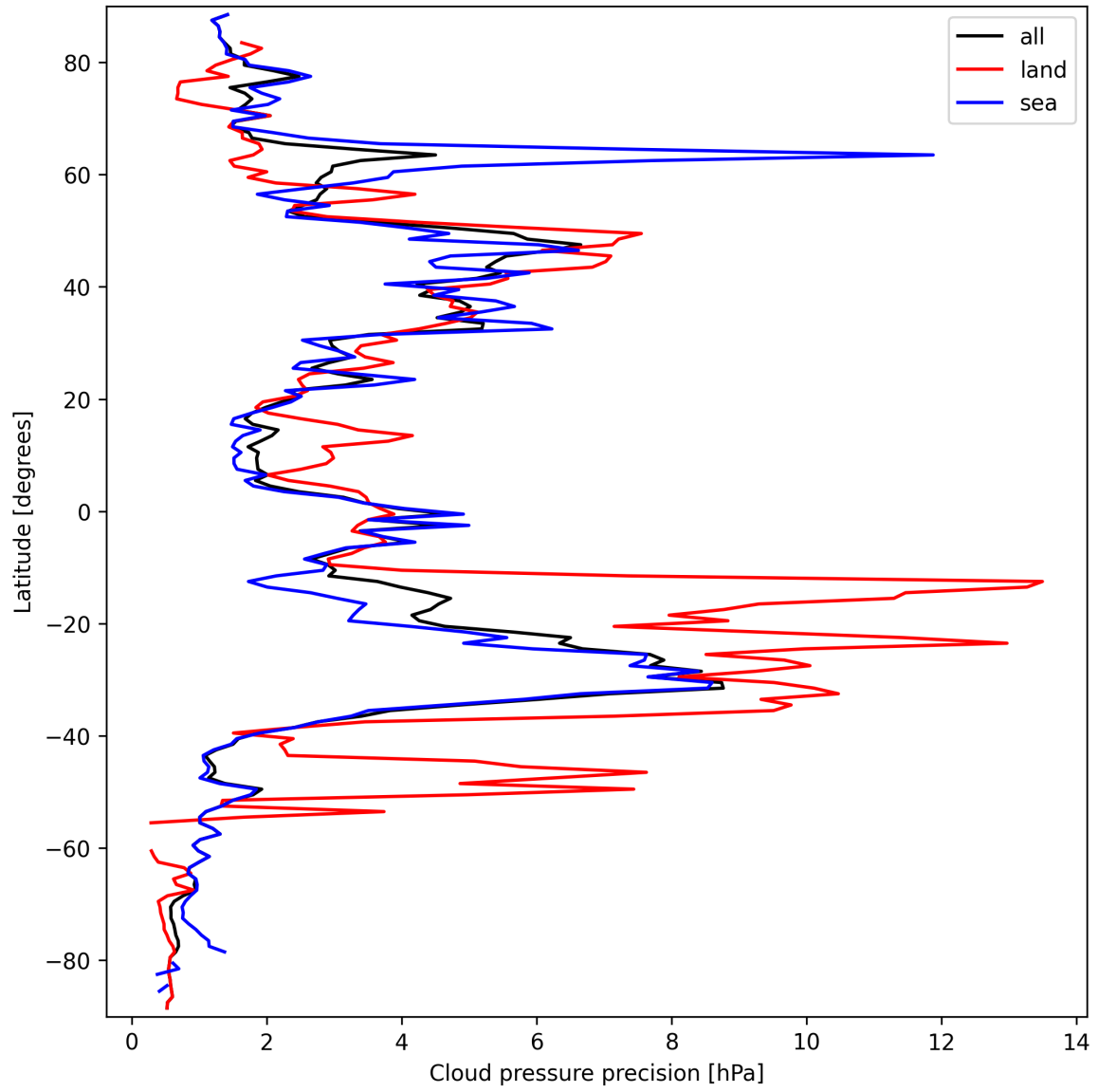
Figure 14: Zonal average of “Cloud pressure precision” for 2025-09-22 to 2025-09-23.
