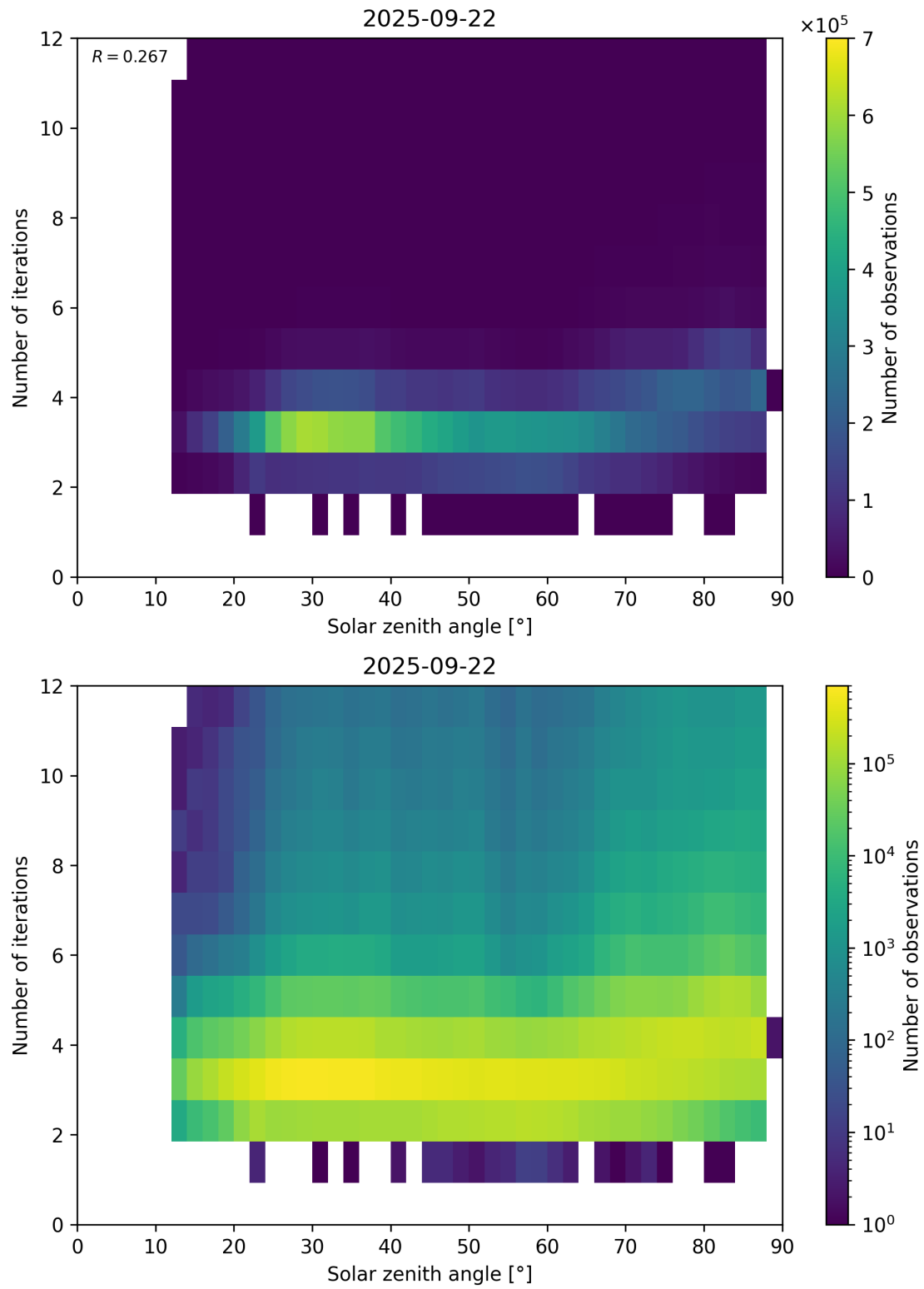
Figure 114: Scatter density plot of “Solar zenith angle” against “Number of iterations” for 2025-09-22 to 2025-09-23.
