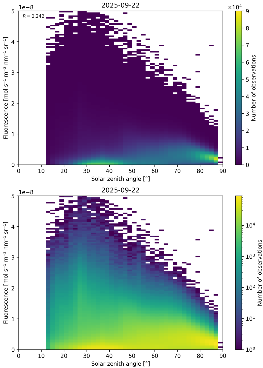
Figure 112: Scatter density plot of “Solar zenith angle” against “Fluorescence” for 2025-09-22 to 2025-09-23.
