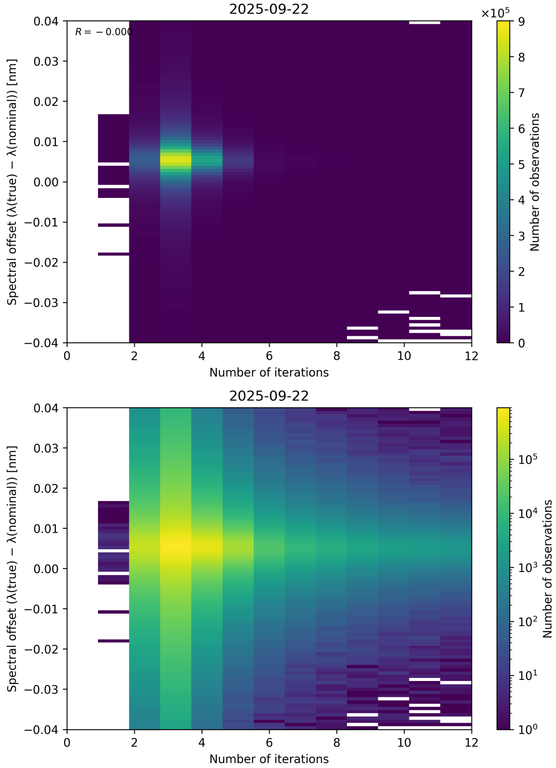
Figure 100: Scatter density plot of “Number of iterations” against “Spectral offset ( \lambda_{\text{true}} - \lambda_{\text{nominal}} )” for 2025-09-22 to 2025-09-23.
