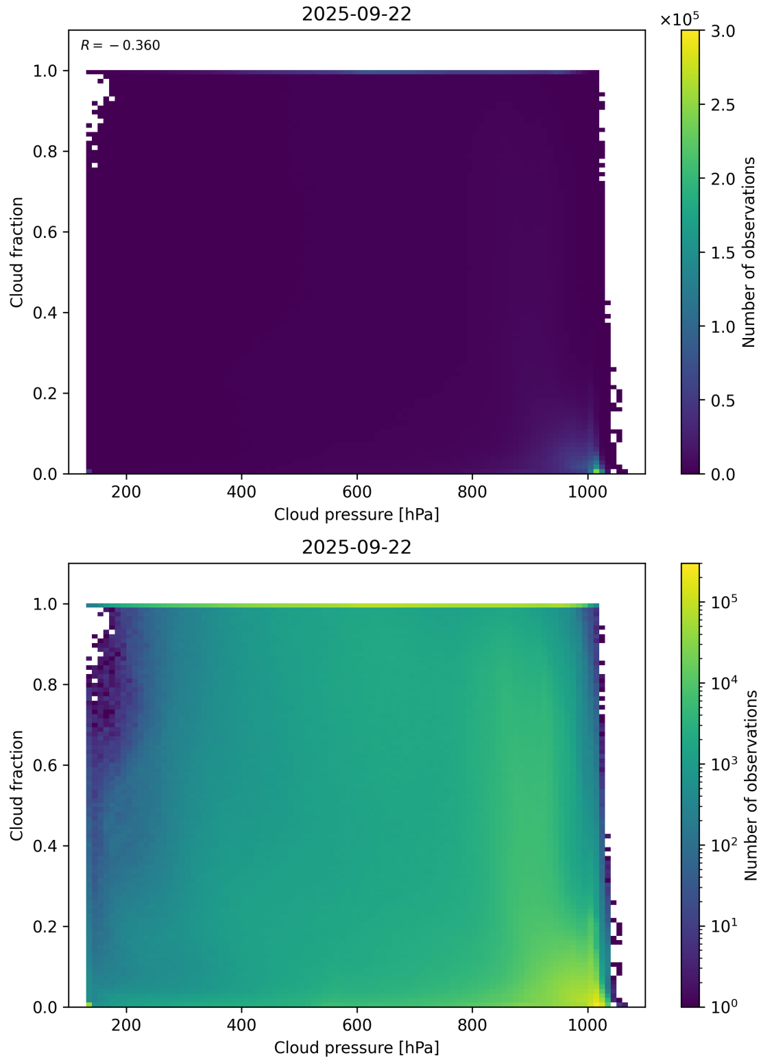
Figure 79: Scatter density plot of “Cloud pressure” against “Cloud fraction” for 2025-09-22 to 2025-09-23.
