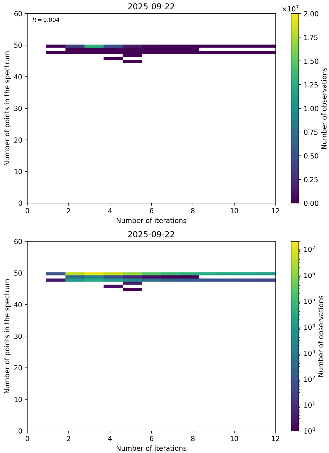
Figure 99: Scatter density plot of “Number of iterations” against “Number of points in the spectrum” for 2025-09-22 to 2025-09-23.
