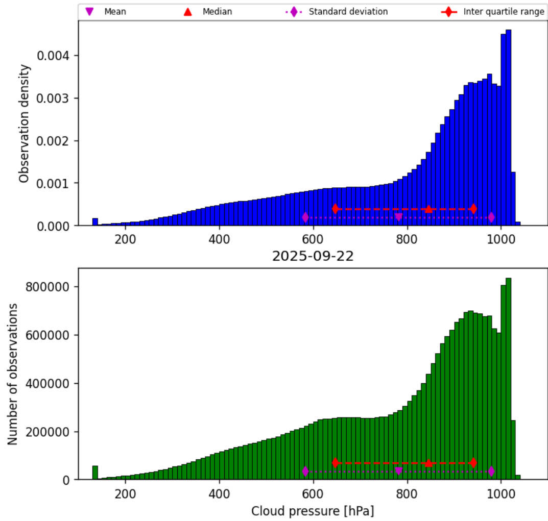
Figure 30: Histogram of “Cloud pressure” for 2025-09-22 to 2025-09-23
