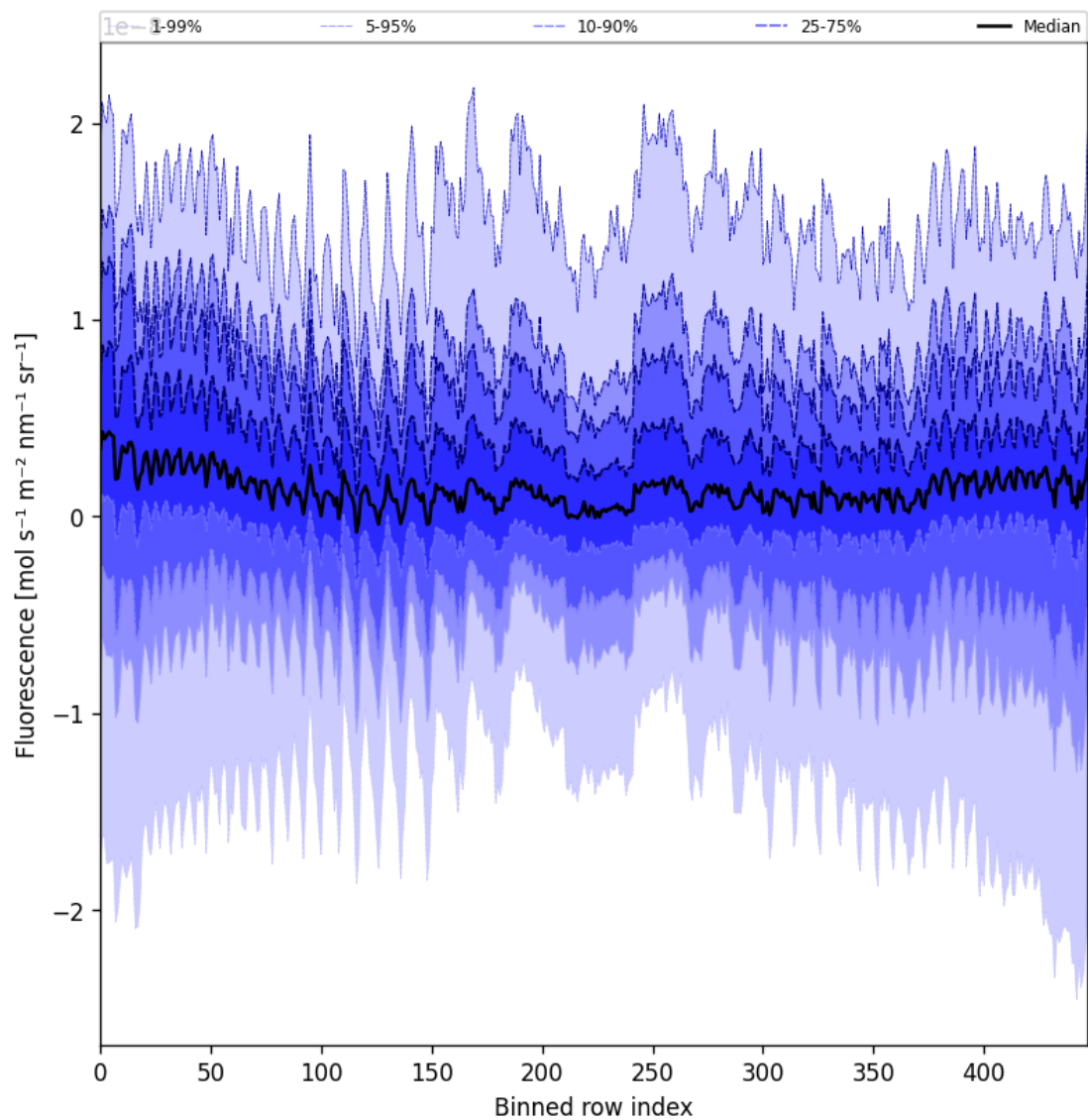
Figure 57: Along track statistics of "Fluorescence" for 2025-09-22 to 2025-09-23
