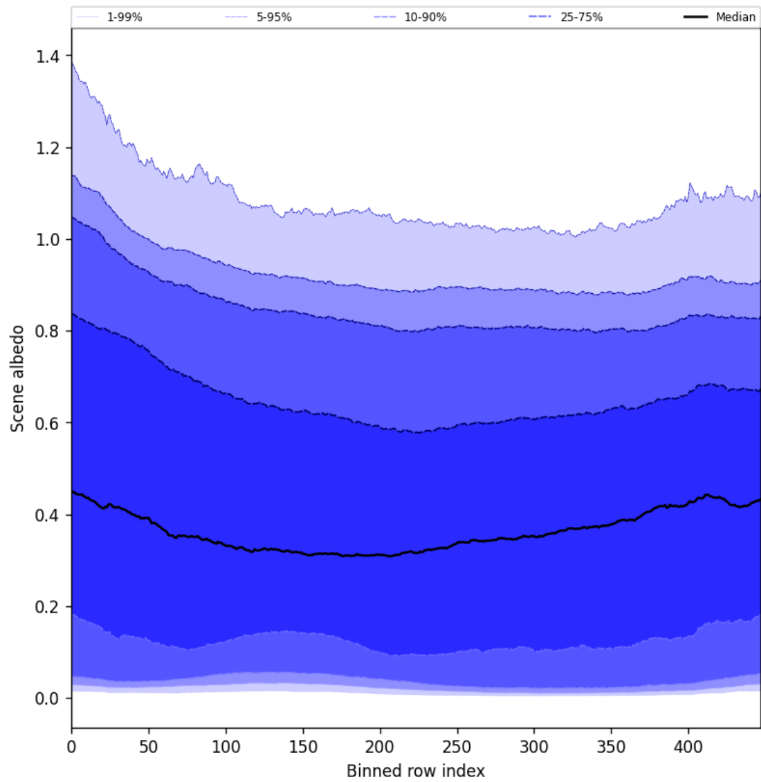
Figure 51: Along track statistics of “Scene albedo” for 2025-09-22 to 2025-09-23
