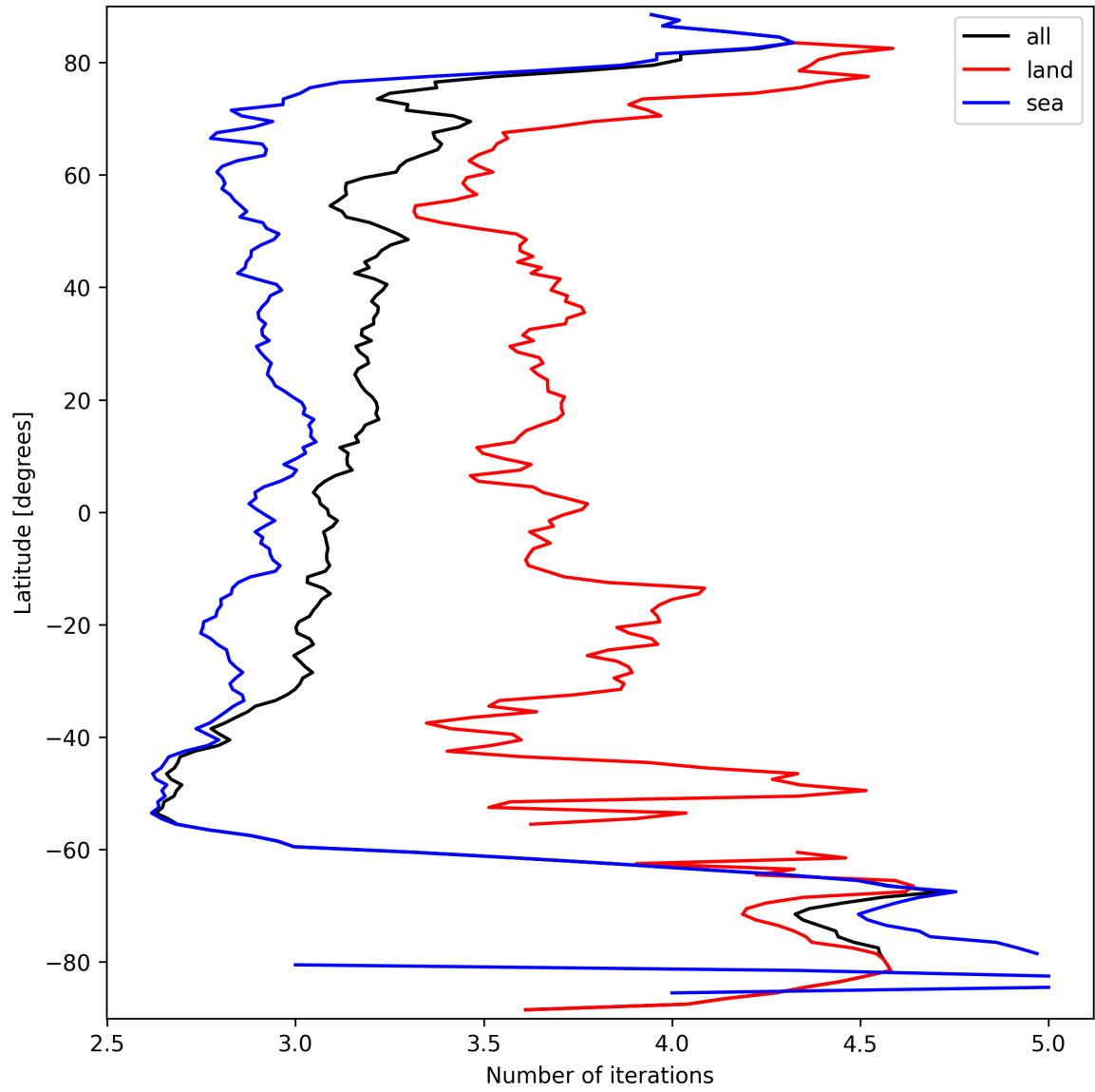
Figure 22: Zonal average of “Number of iterations” for 2025-09-22 to 2025-09-23.
