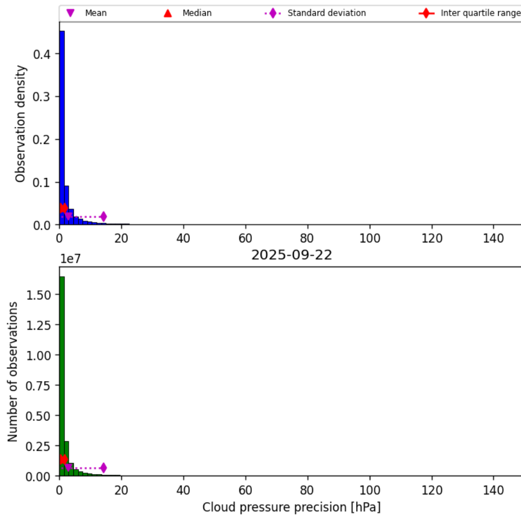
Figure 31: Histogram of "Cloud pressure precision" for 2025-09-22 to 2025-09-23
