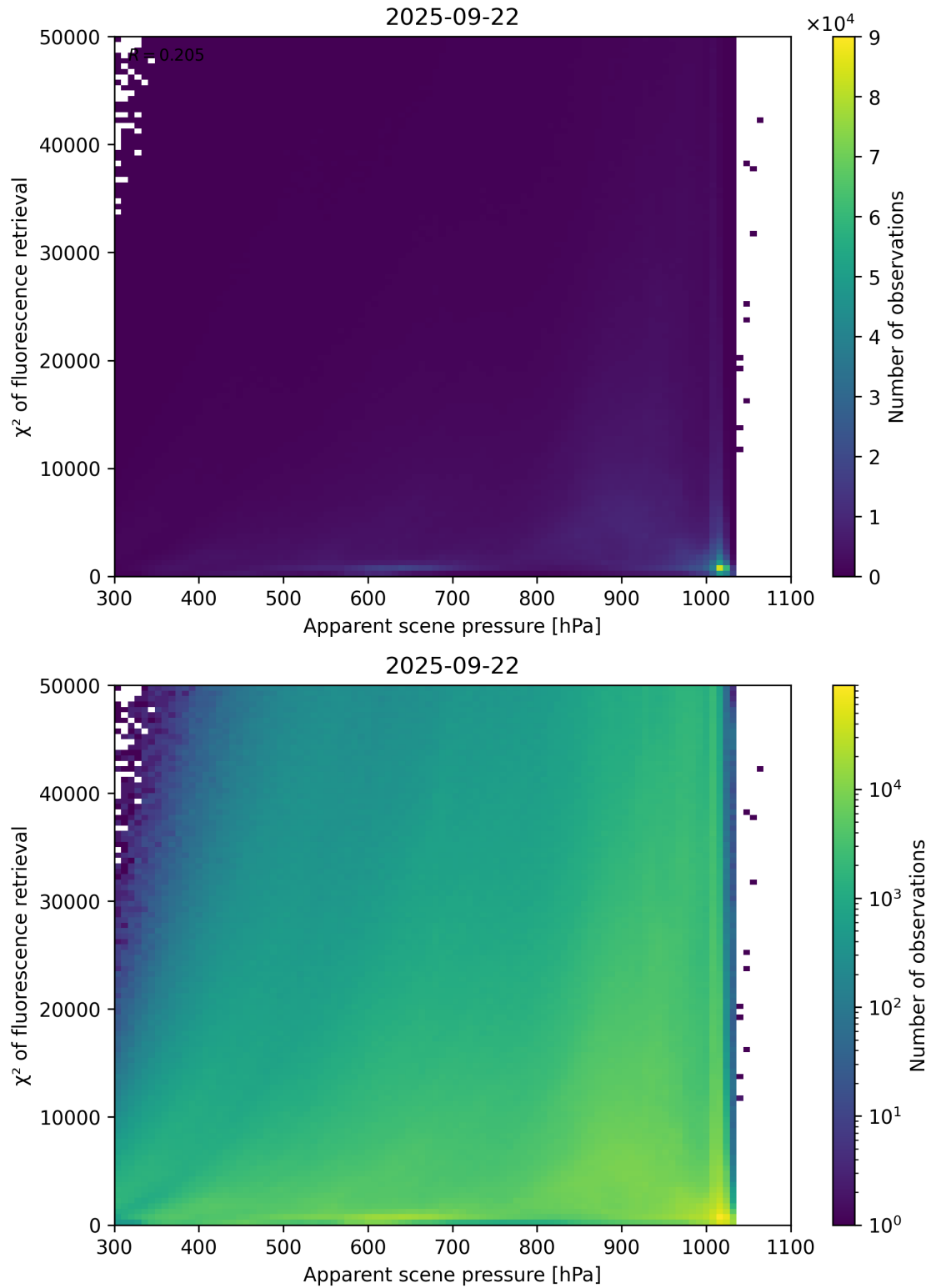
Figure 63: Scatter density plot of “Apparent scene pressure” against “ \chi^2 of fluorescence retrieval” for 2025-09-22 to 2025-09-23.
