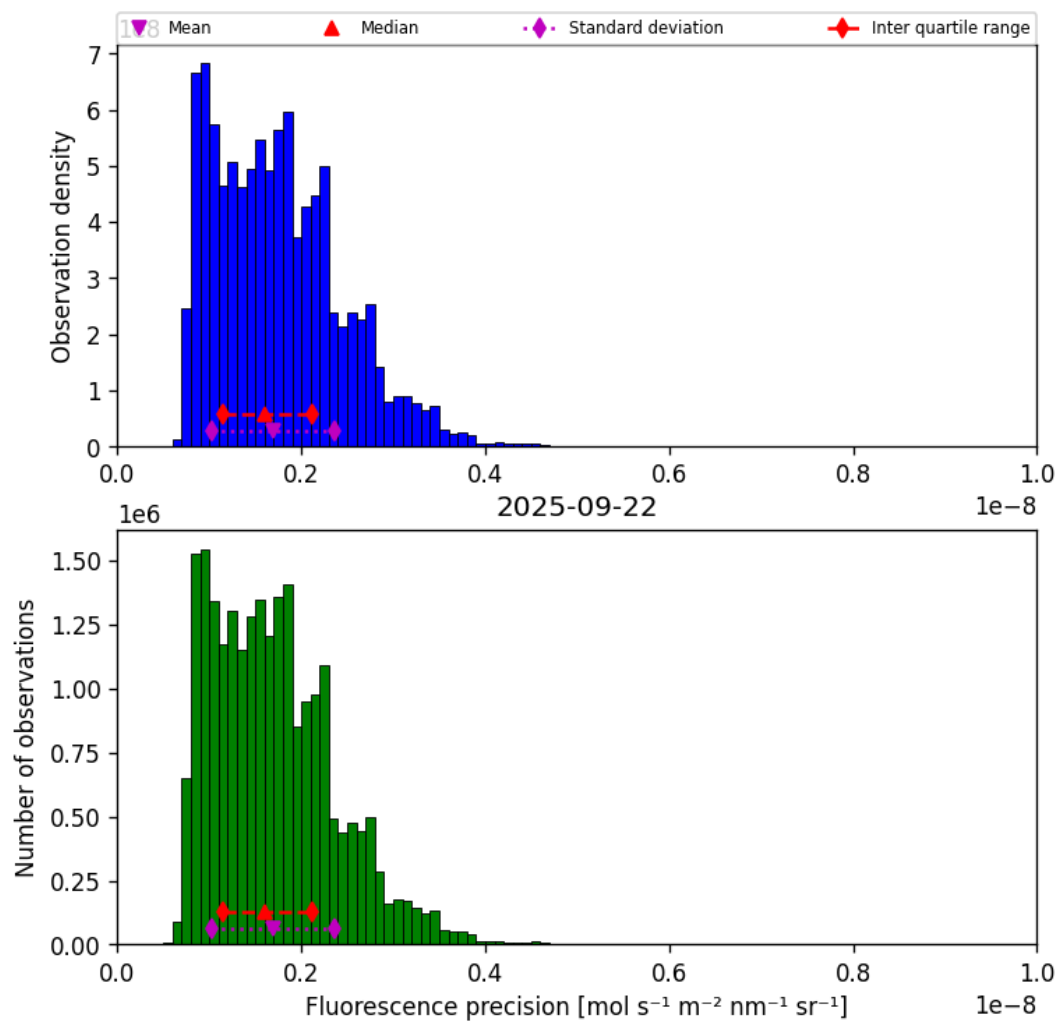
Figure 41: Histogram of “Fluorescence precision” for 2025-09-22 to 2025-09-23
