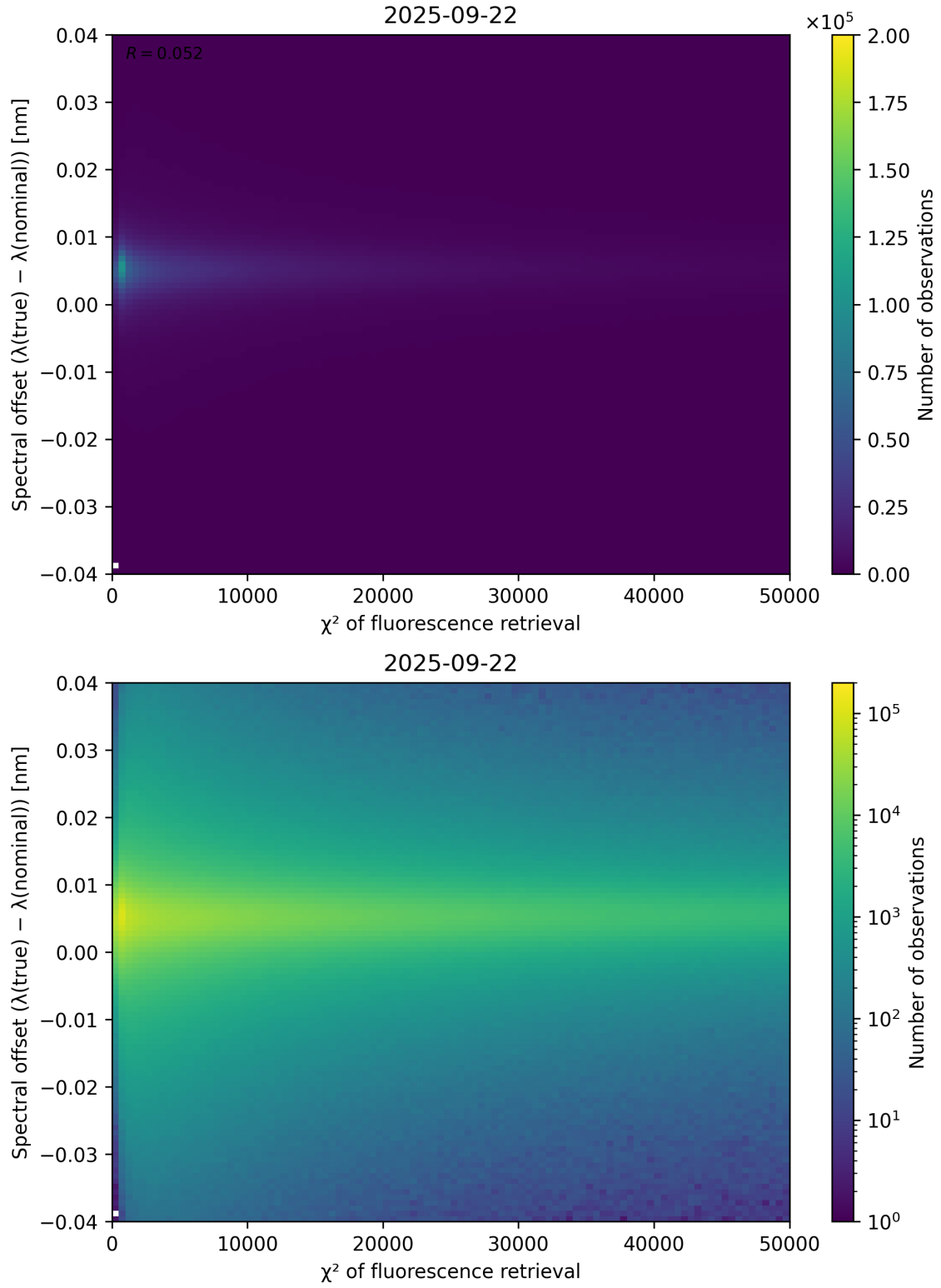
Figure 69: Scatter density plot of “ \chi^2 of fluorescence retrieval” against “Spectral offset ( \lambda_{\text{true}} - \lambda_{\text{nominal}} )” for 2025-09-22 to 2025-09-23.
