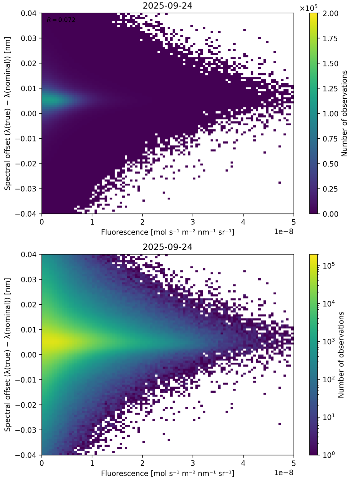
Figure 87: Scatter density plot of “Fluorescence” against “Spectral offset ( \lambda_{\text{true}} - \lambda_{\text{nominal}} )” for 2025-09-23 to 2025-09-25.
