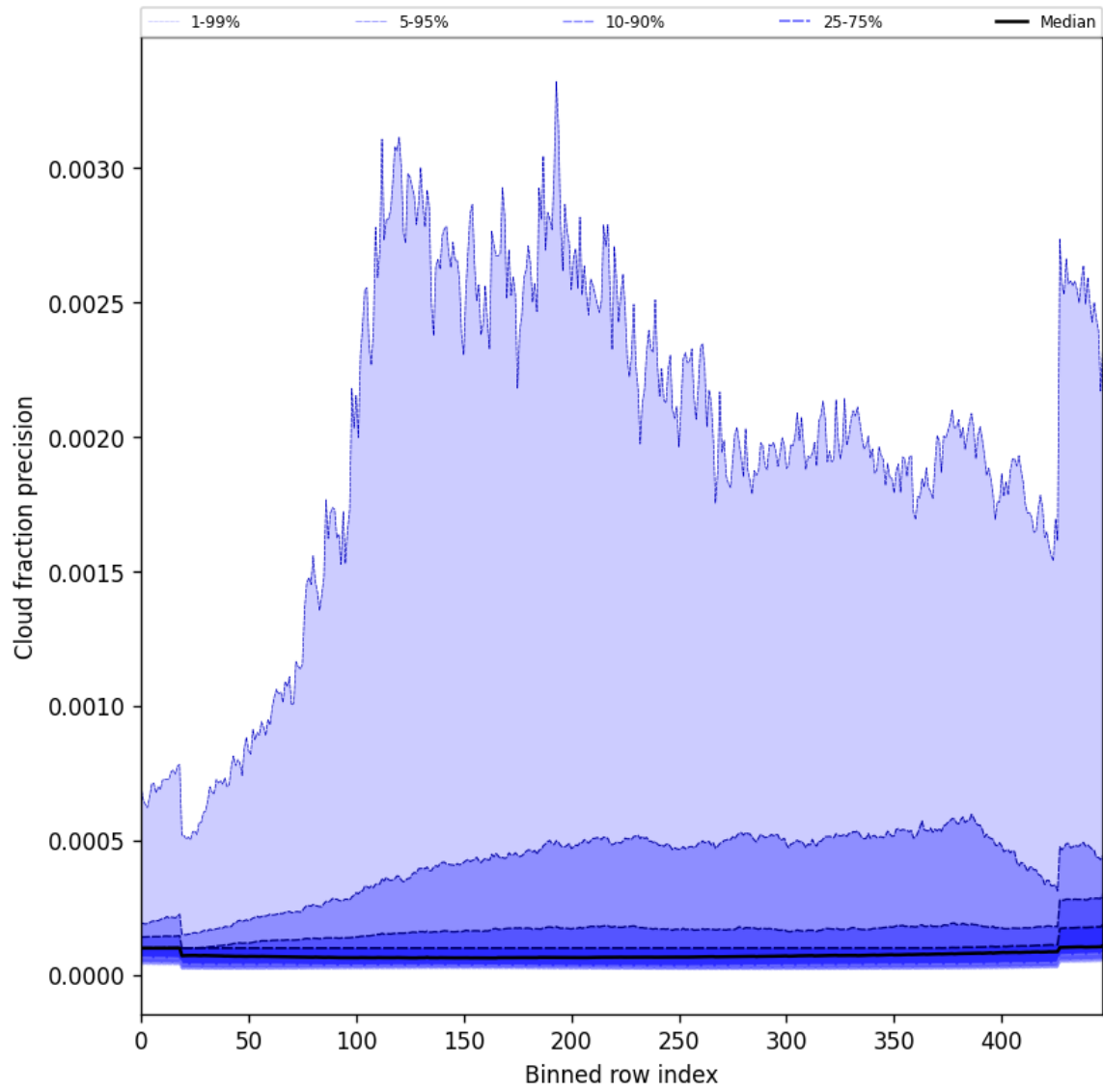
Figure 50: Along track statistics of “Cloud fraction precision” for 2025-09-23 to 2025-09-25
