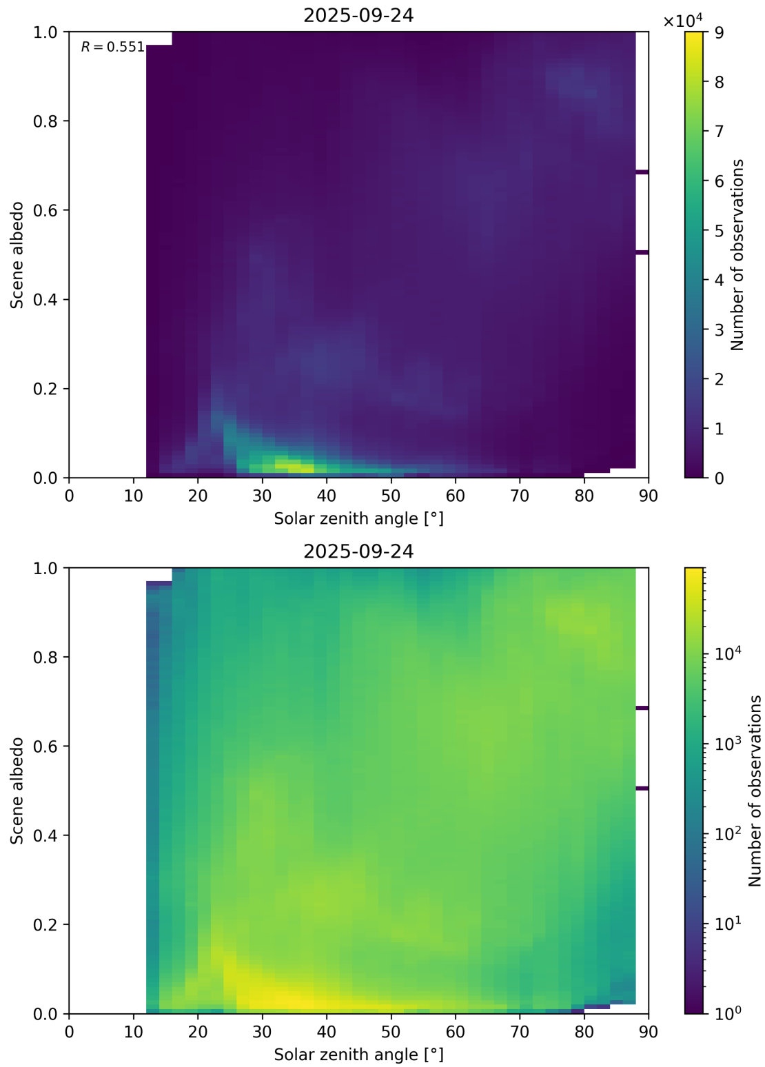
Figure 116: Scatter density plot of “Solar zenith angle” against “Scene albedo” for 2025-09-23 to 2025-09-25.
