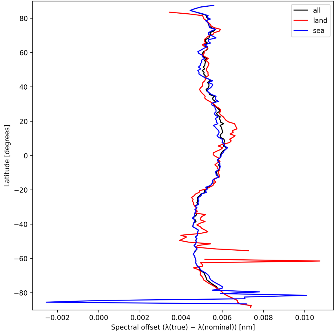
Figure 28: Zonal average of “Spectral offset ( \lambda_{\text{true}} - \lambda_{\text{nominal}} )” for 2025-09-23 to 2025-09-25.
