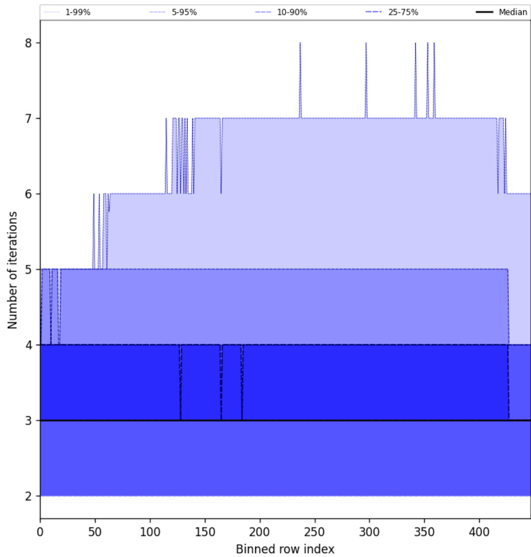
Figure 56: Along track statistics of “Number of iterations” for 2025-09-23 to 2025-09-25
