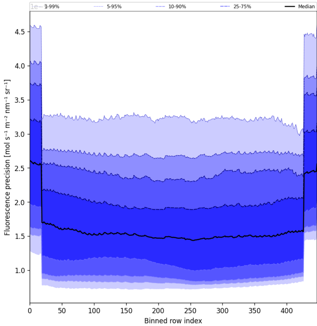
Figure 58: Along track statistics of “Fluorescence precision” for 2025-09-23 to 2025-09-25
