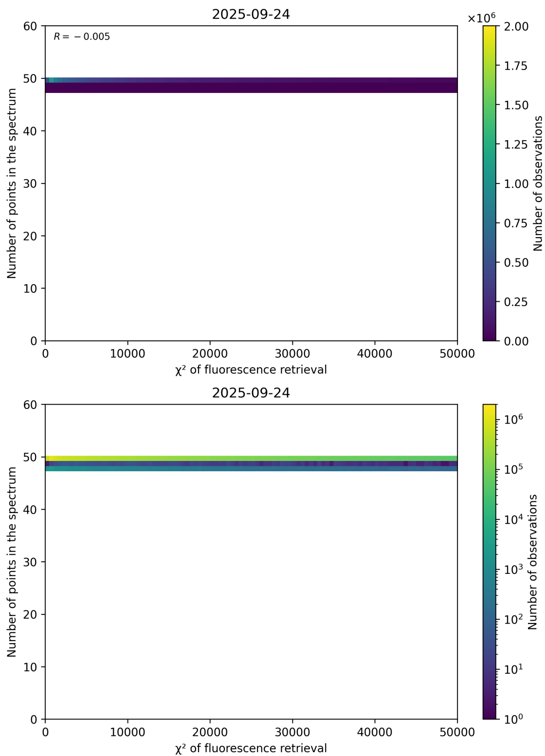
Figure 68: Scatter density plot of “ \chi^2 of fluorescence retrieval” against “Number of points in the spectrum” for 2025-09-23 to 2025-09-25.
