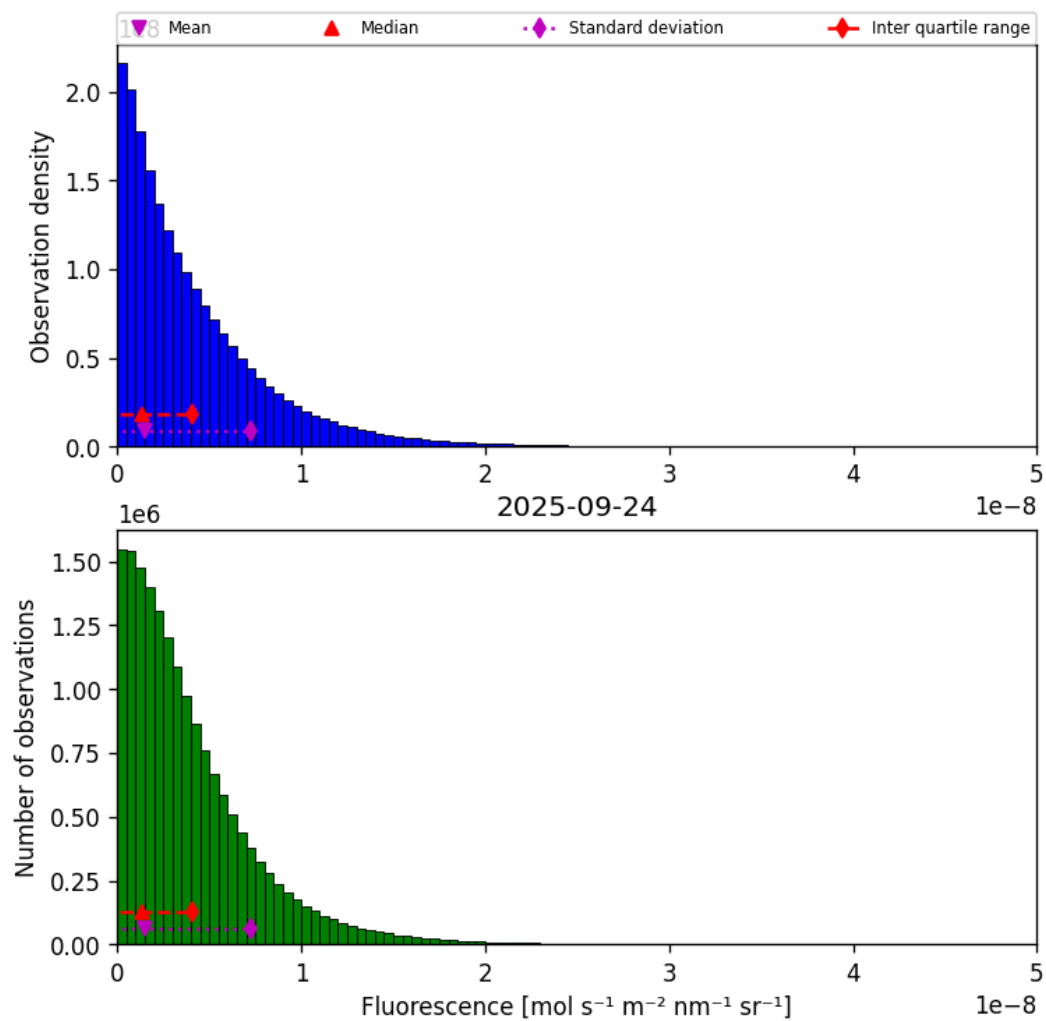
Figure 40: Histogram of “Fluorescence” for 2025-09-23 to 2025-09-25
