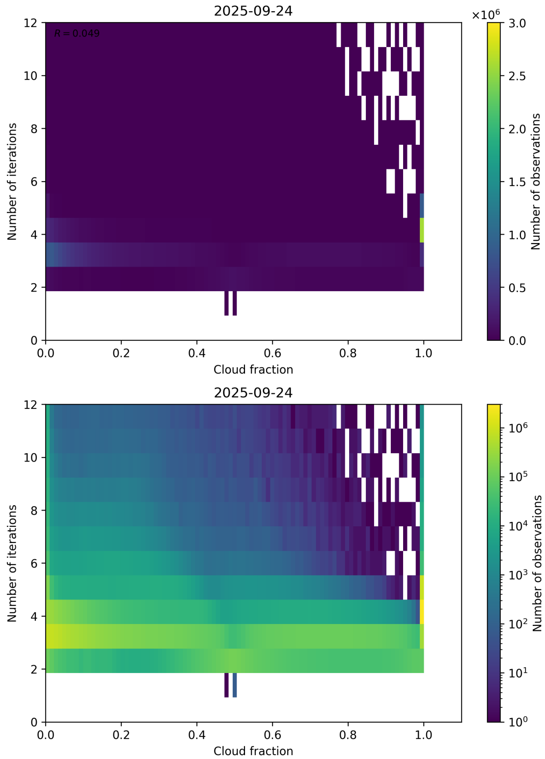
Figure 73: Scatter density plot of “Cloud fraction” against “Number of iterations” for 2025-09-23 to 2025-09-25.
