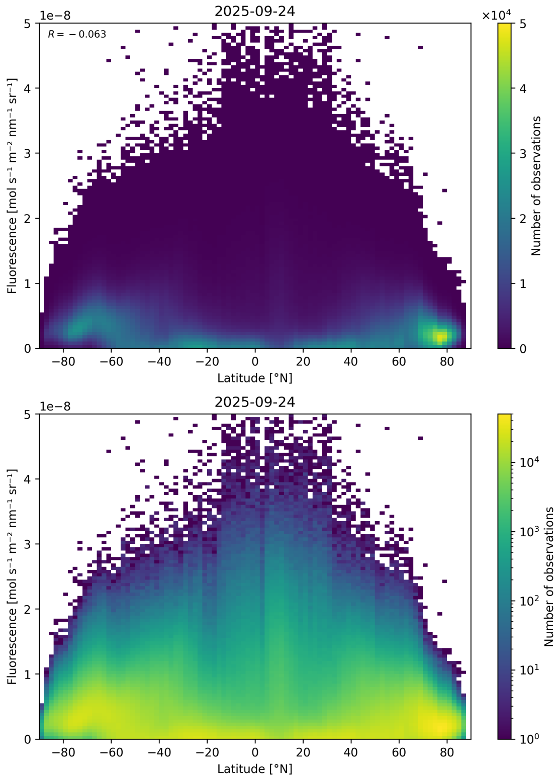
Figure 92: Scatter density plot of “Latitude” against “Fluorescence” for 2025-09-23 to 2025-09-25.
