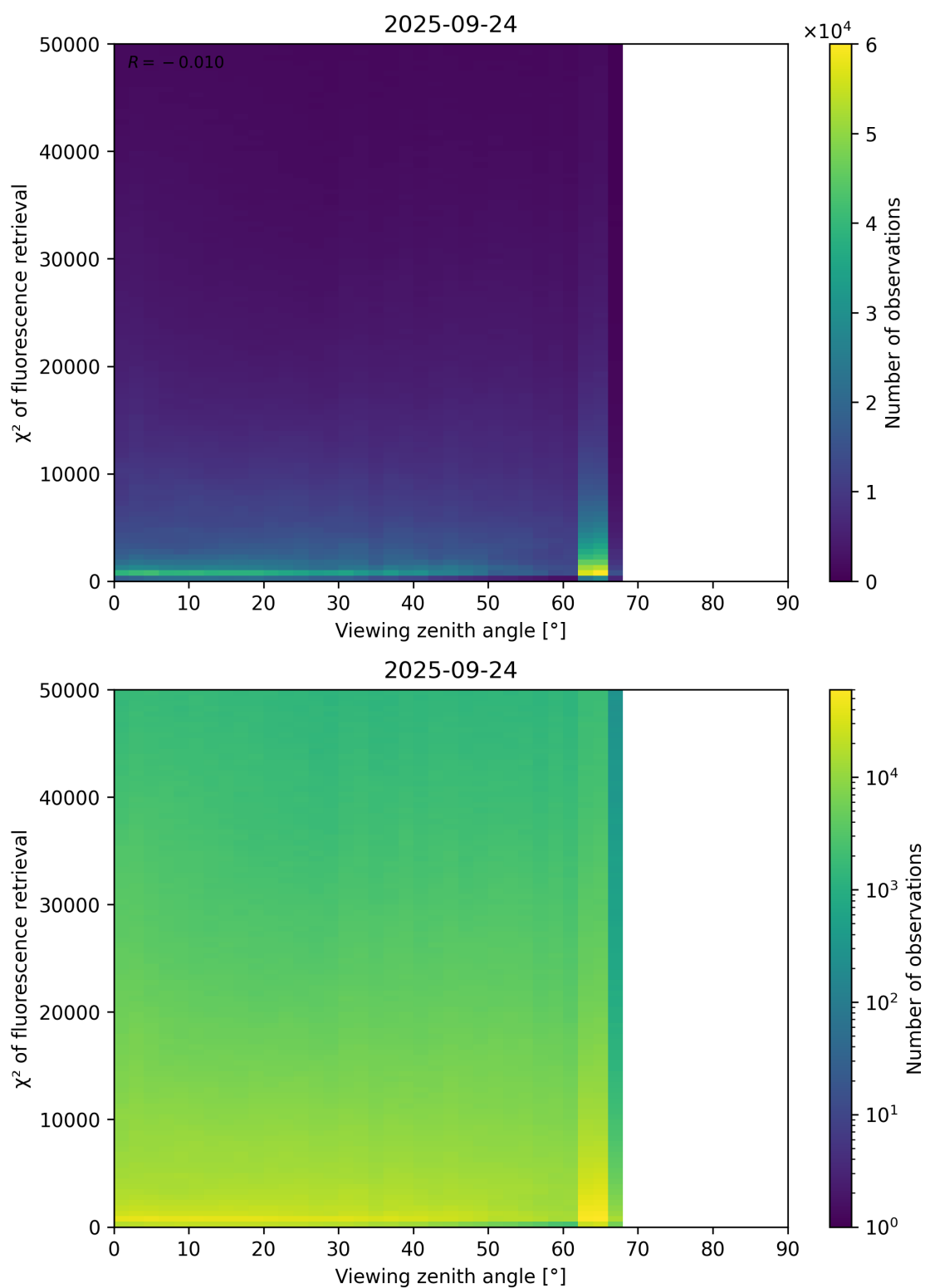
Figure 119: Scatter density plot of “Viewing zenith angle” against “ \chi^2 of fluorescence retrieval” for 2025-09-23 to 2025-09-25.
