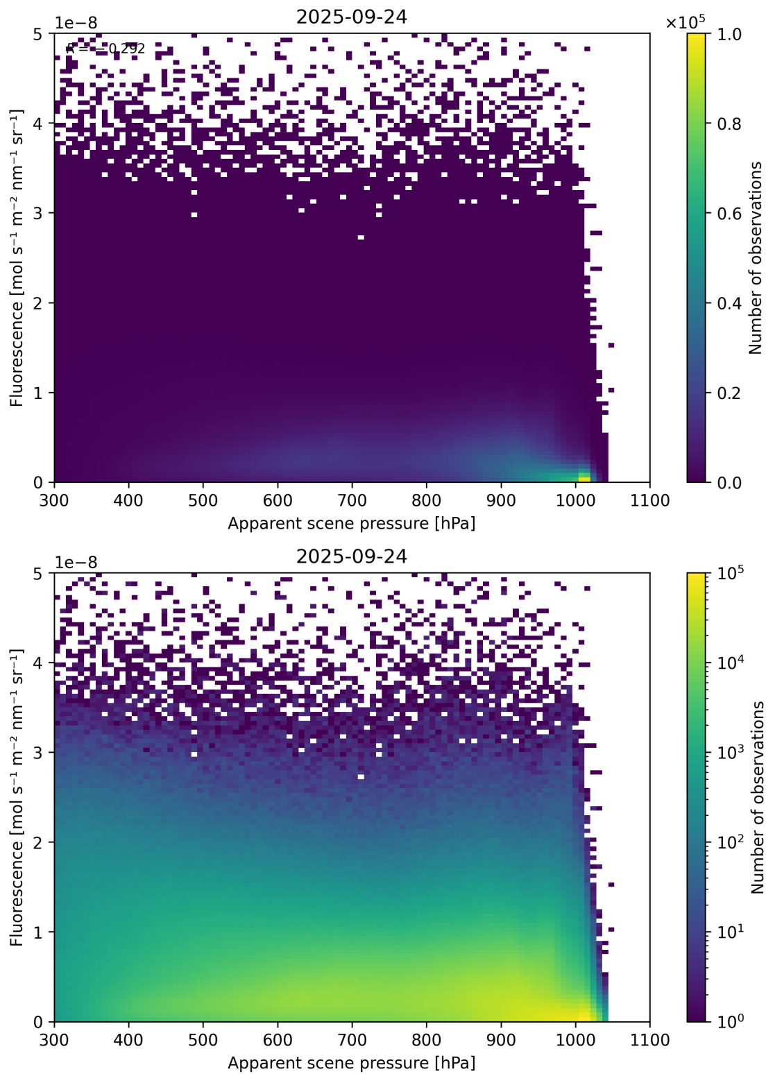
Figure 64: Scatter density plot of “Apparent scene pressure” against “Fluorescence” for 2025-09-23 to 2025-09-25.
