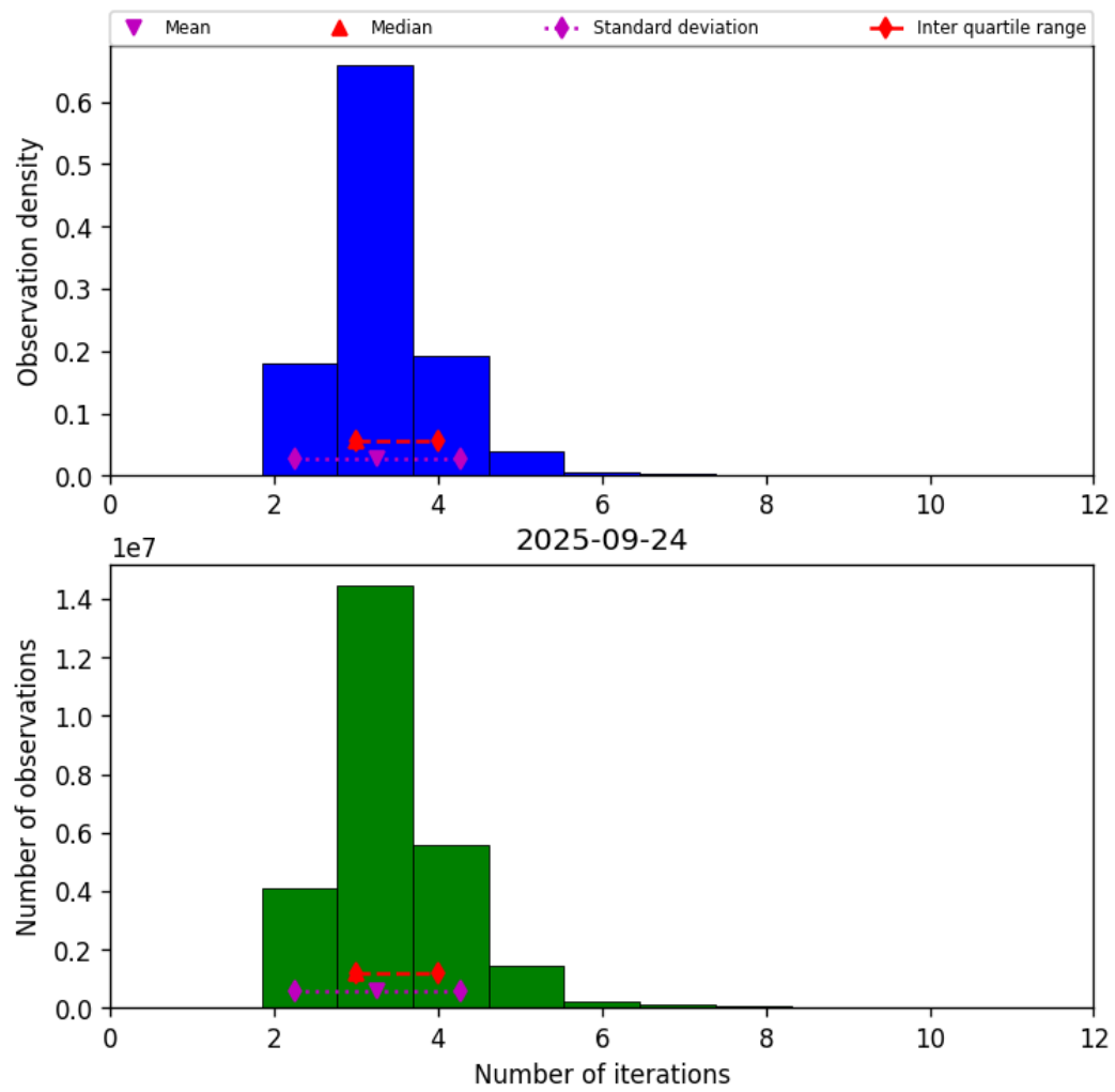
Figure 39: Histogram of “Number of iterations” for 2025-09-23 to 2025-09-25
