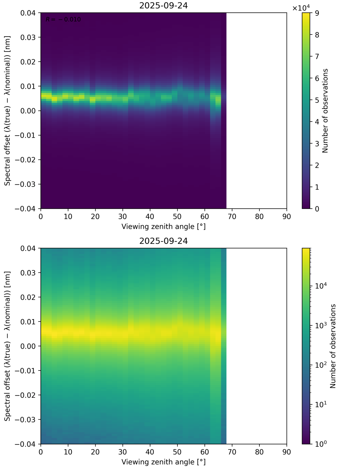
Figure 128: Scatter density plot of “Viewing zenith angle” against “Spectral offset ( \lambda_{\text{true}} - \lambda_{\text{nominal}} )” for 2025-09-23 to 2025-09-25.
