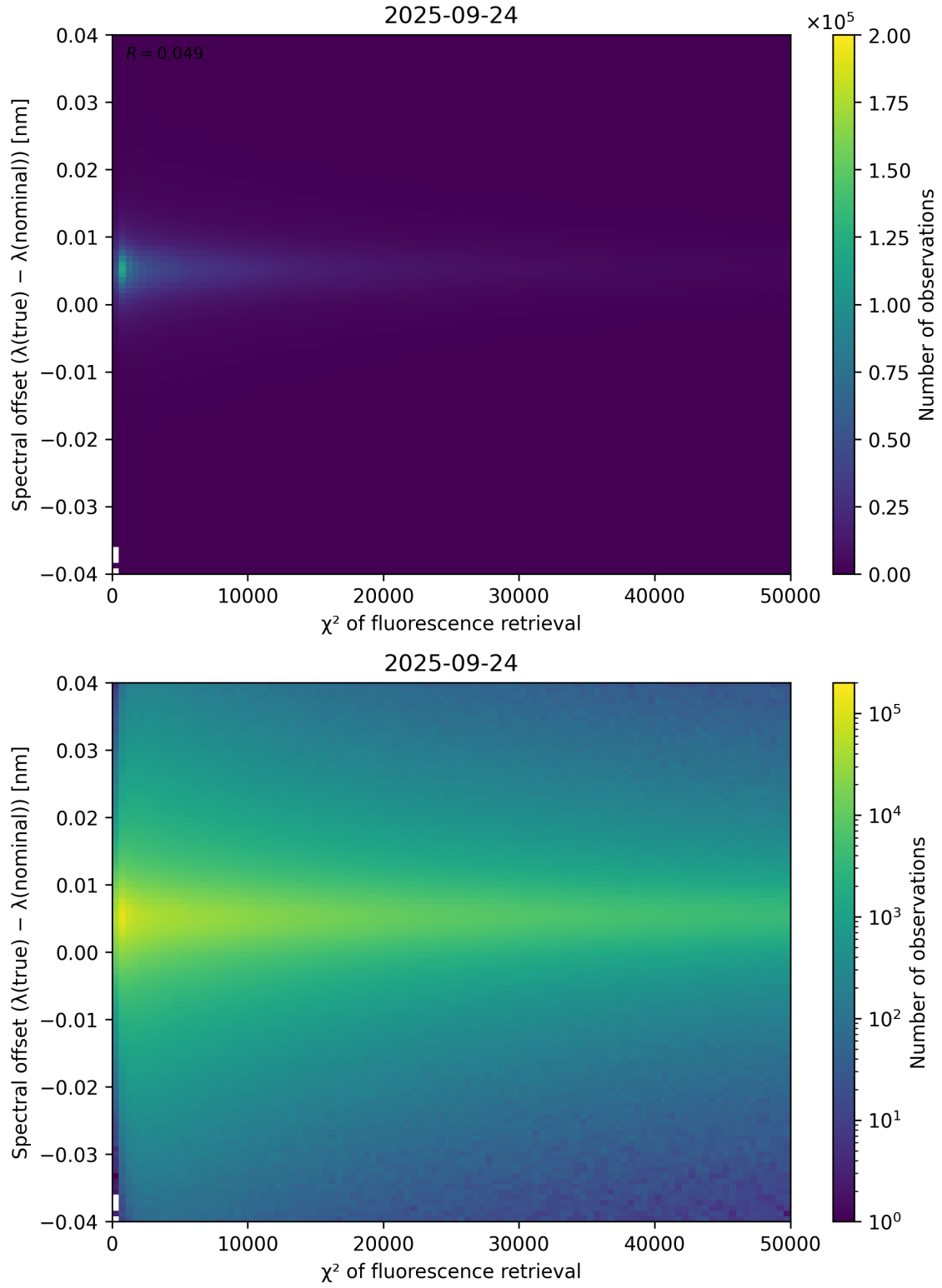
Figure 69: Scatter density plot of “ \chi^2 of fluorescence retrieval” against “Spectral offset ( \lambda_{\text{true}} - \lambda_{\text{nominal}} )” for 2025-09-23 to 2025-09-25.
