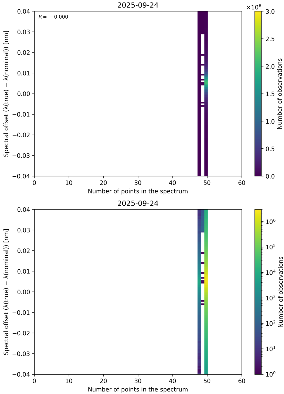
Figure 101: Scatter density plot of “Number of points in the spectrum” against “Spectral offset ( \lambda_{\text{true}} - \lambda_{\text{nominal}} )” for 2025-09-23 to 2025-09-25.
