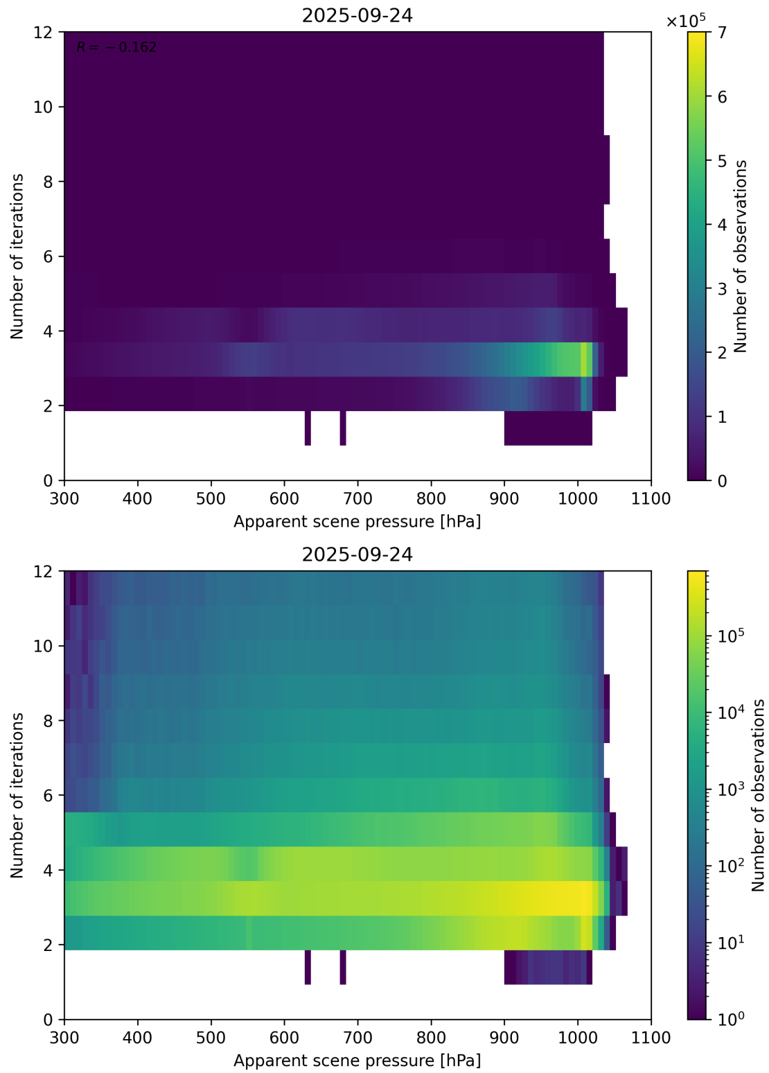
Figure 65: Scatter density plot of “Apparent scene pressure” against “Number of iterations” for 2025-09-23 to 2025-09-25.
