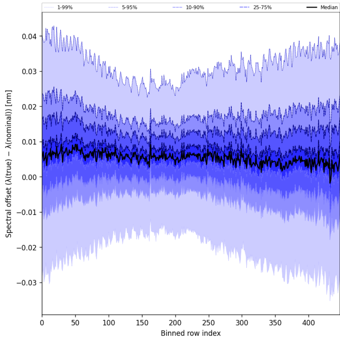
Figure 62: Along track statistics of “Spectral offset ( \lambda_{\text{true}} - \lambda_{\text{nominal}} )” for 2025-09-23 to 2025-09-25
