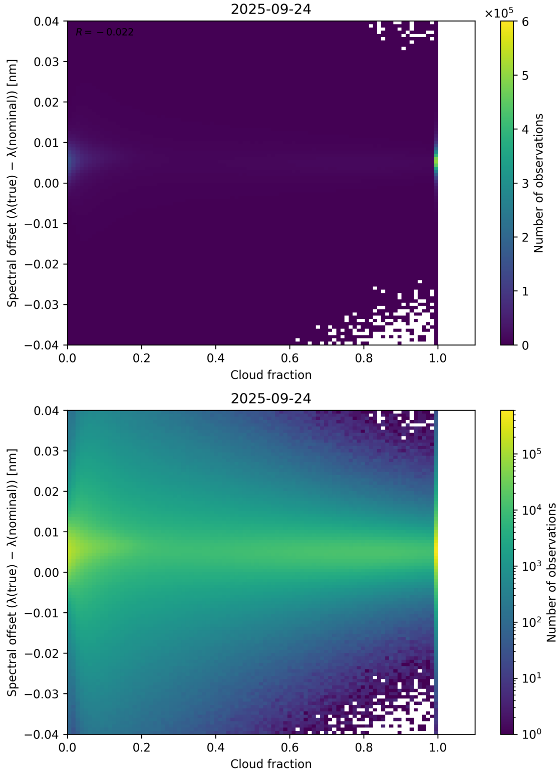
Figure 76: Scatter density plot of “Cloud fraction” against “Spectral offset ( \lambda_{\text{true}} - \lambda_{\text{nominal}} )” for 2025-09-23 to 2025-09-25.
