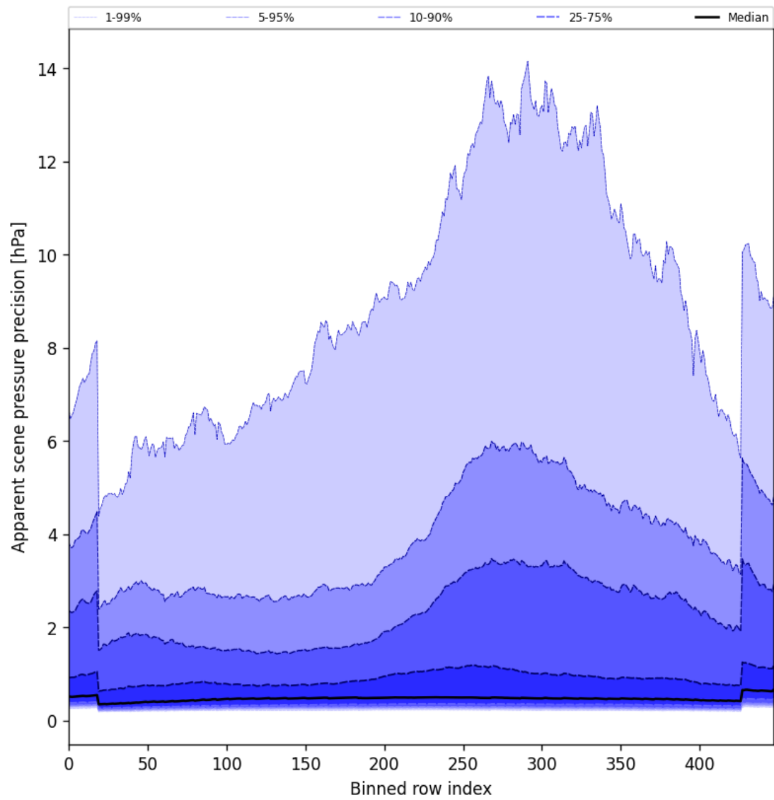
Figure 54: Along track statistics of “Apparent scene pressure precision” for 2025-09-23 to 2025-09-25
