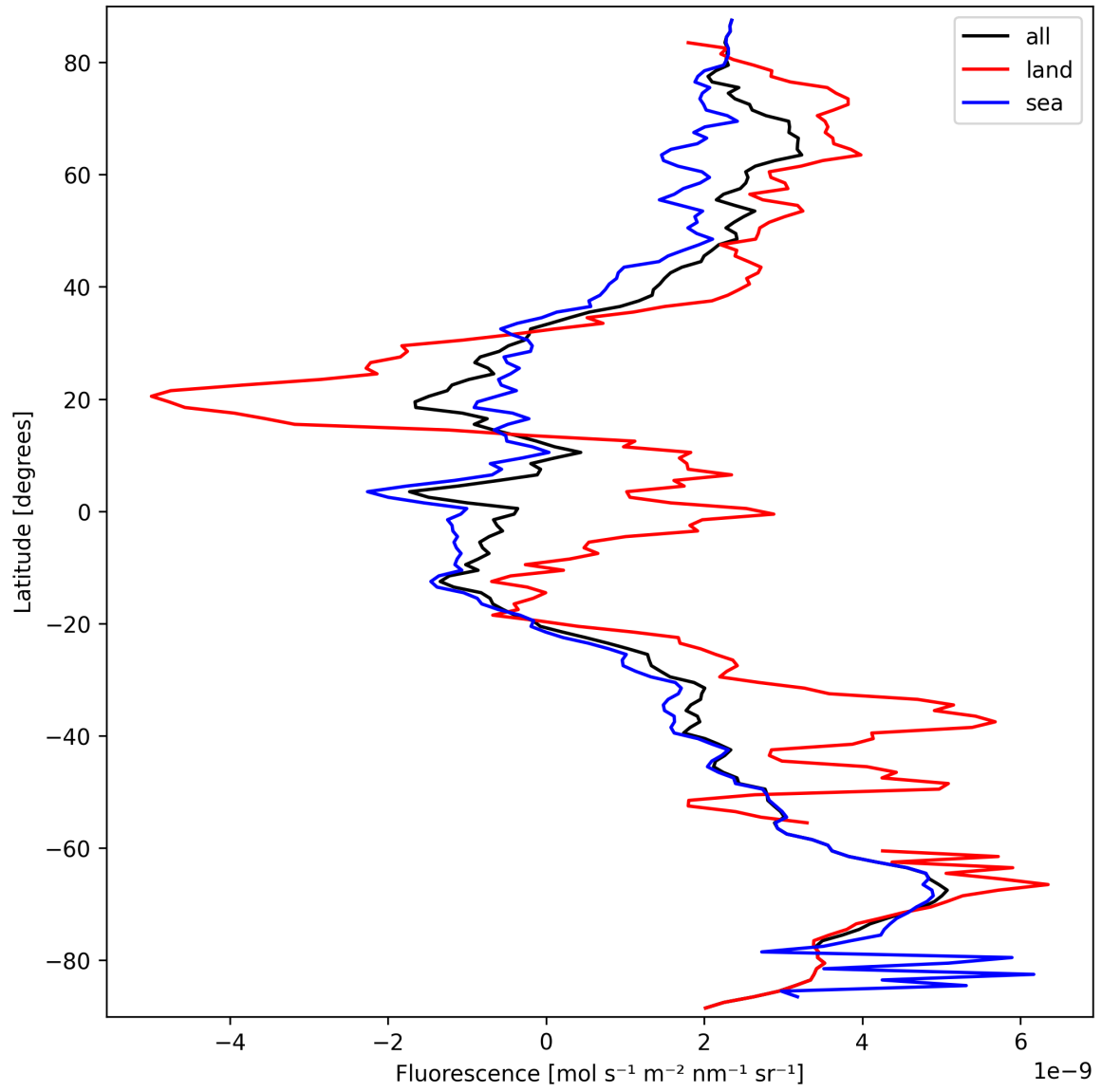
Figure 23: Zonal average of “Fluorescence” for 2025-09-23 to 2025-09-25.
