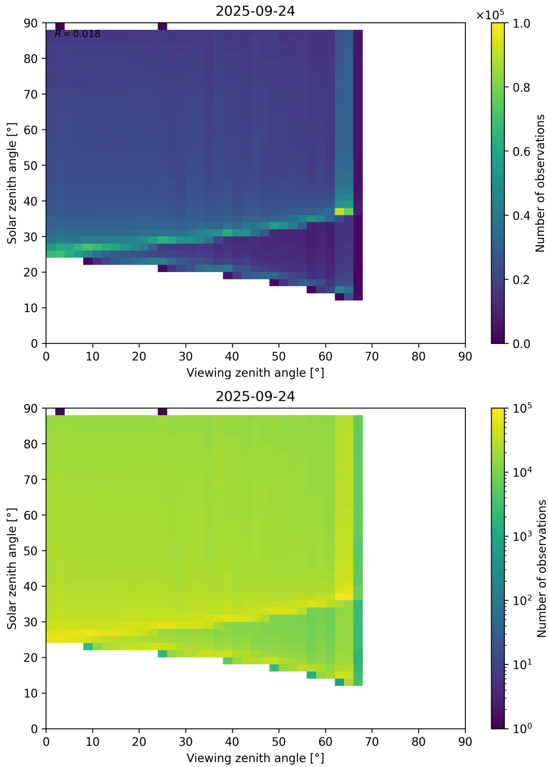
Figure 127: Scatter density plot of “Viewing zenith angle” against “Solar zenith angle” for 2025-09-23 to 2025-09-25.
