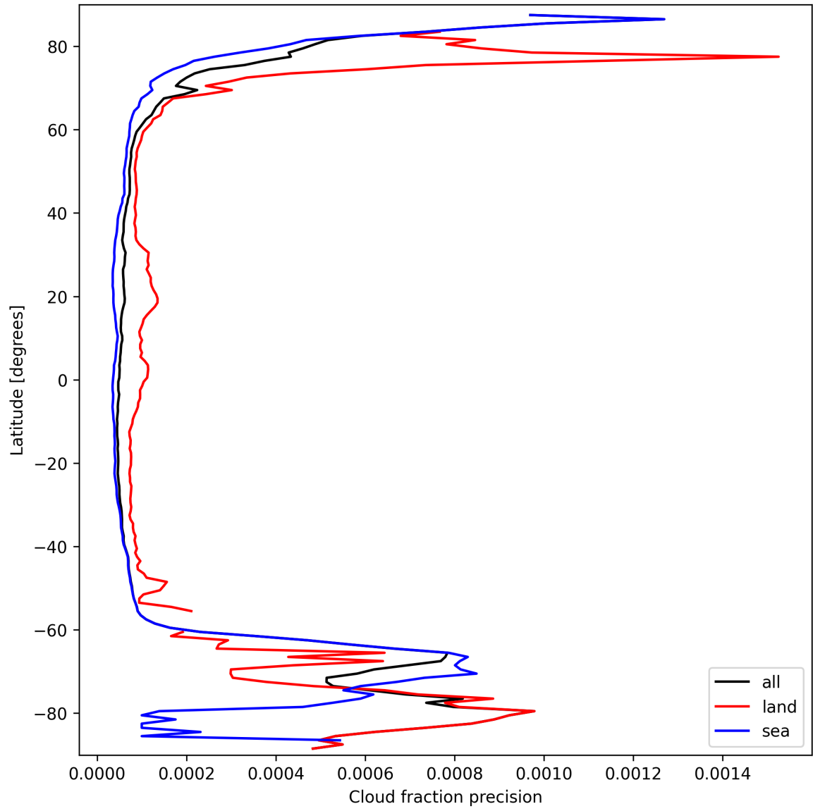
Figure 16: Zonal average of “Cloud fraction precision” for 2025-09-23 to 2025-09-25.
