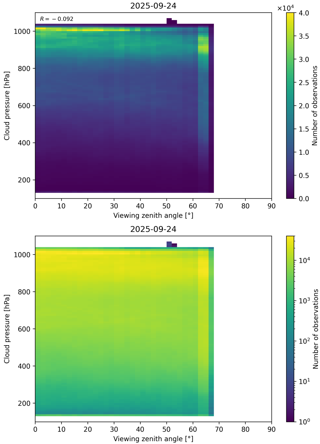
Figure 121: Scatter density plot of “Viewing zenith angle” against “Cloud pressure” for 2025-09-23 to 2025-09-25.
