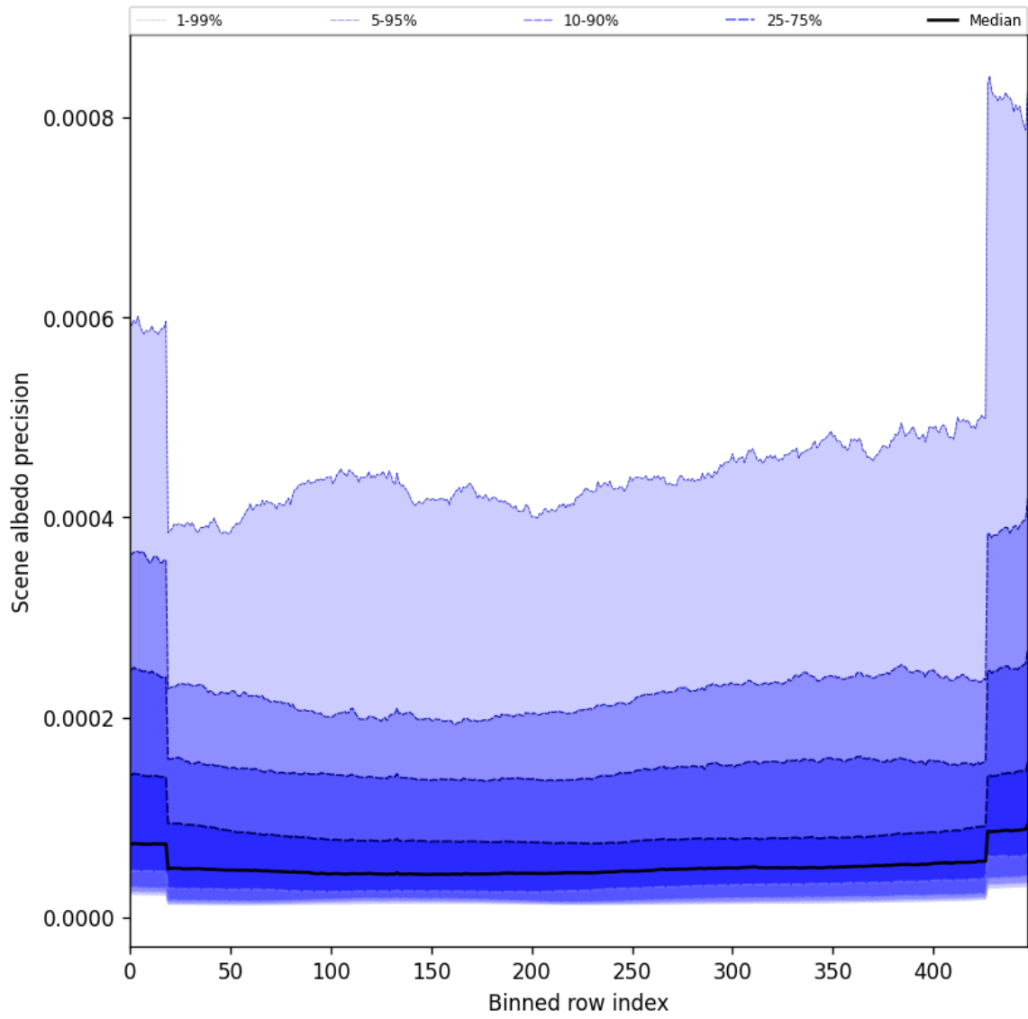
Figure 52: Along track statistics of “Scene albedo precision” for 2025-09-23 to 2025-09-25
