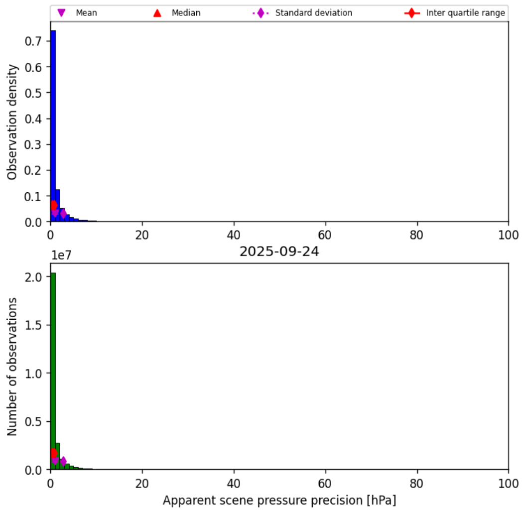
Figure 37: Histogram of “Apparent scene pressure precision” for 2025-09-23 to 2025-09-25
