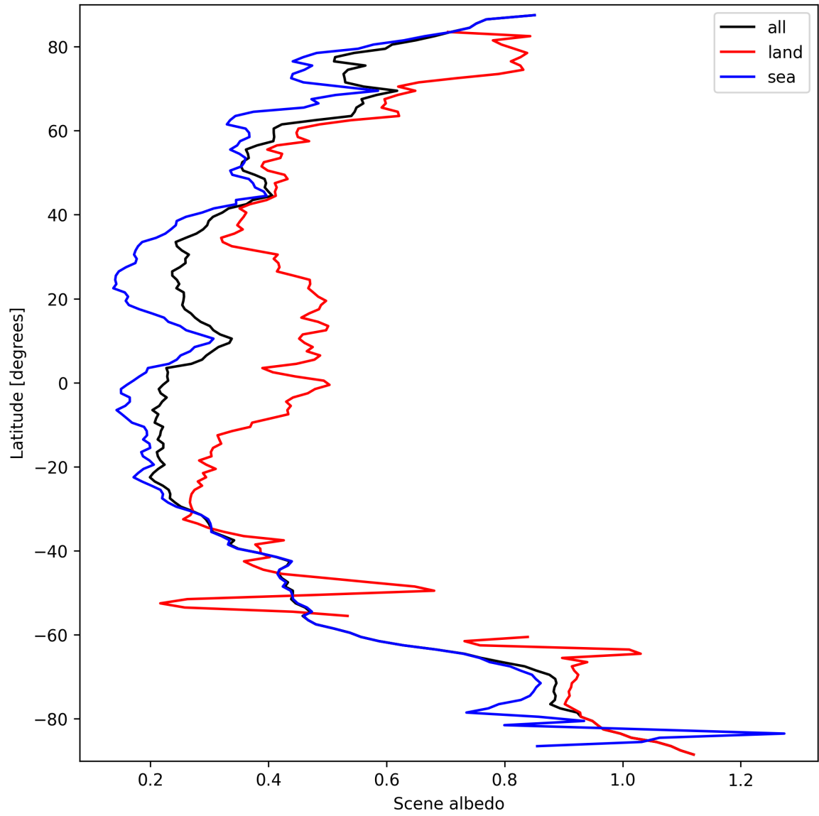
Figure 17: Zonal average of “Scene albedo” for 2025-09-23 to 2025-09-25.
