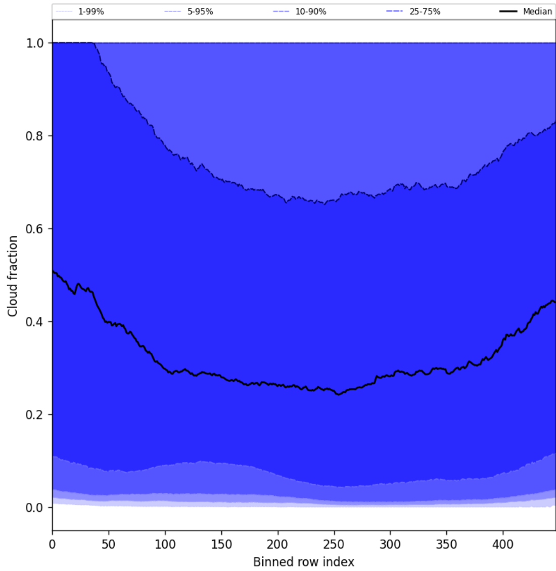
Figure 49: Along track statistics of “Cloud fraction” for 2025-09-23 to 2025-09-25
