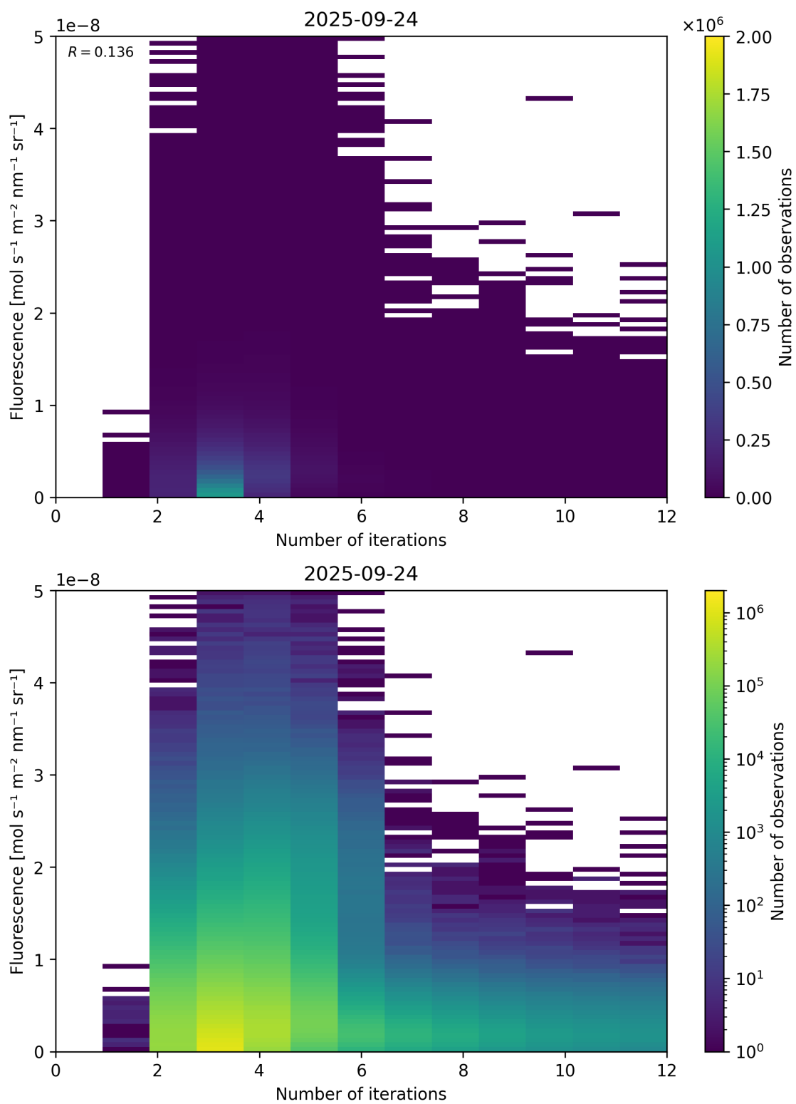
Figure 98: Scatter density plot of “Number of iterations” against “Fluorescence” for 2025-09-23 to 2025-09-25.
