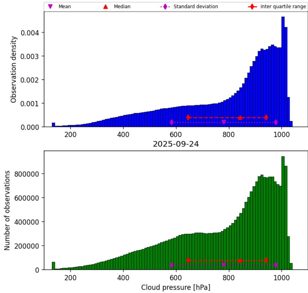
Figure 30: Histogram of “Cloud pressure” for 2025-09-23 to 2025-09-25
