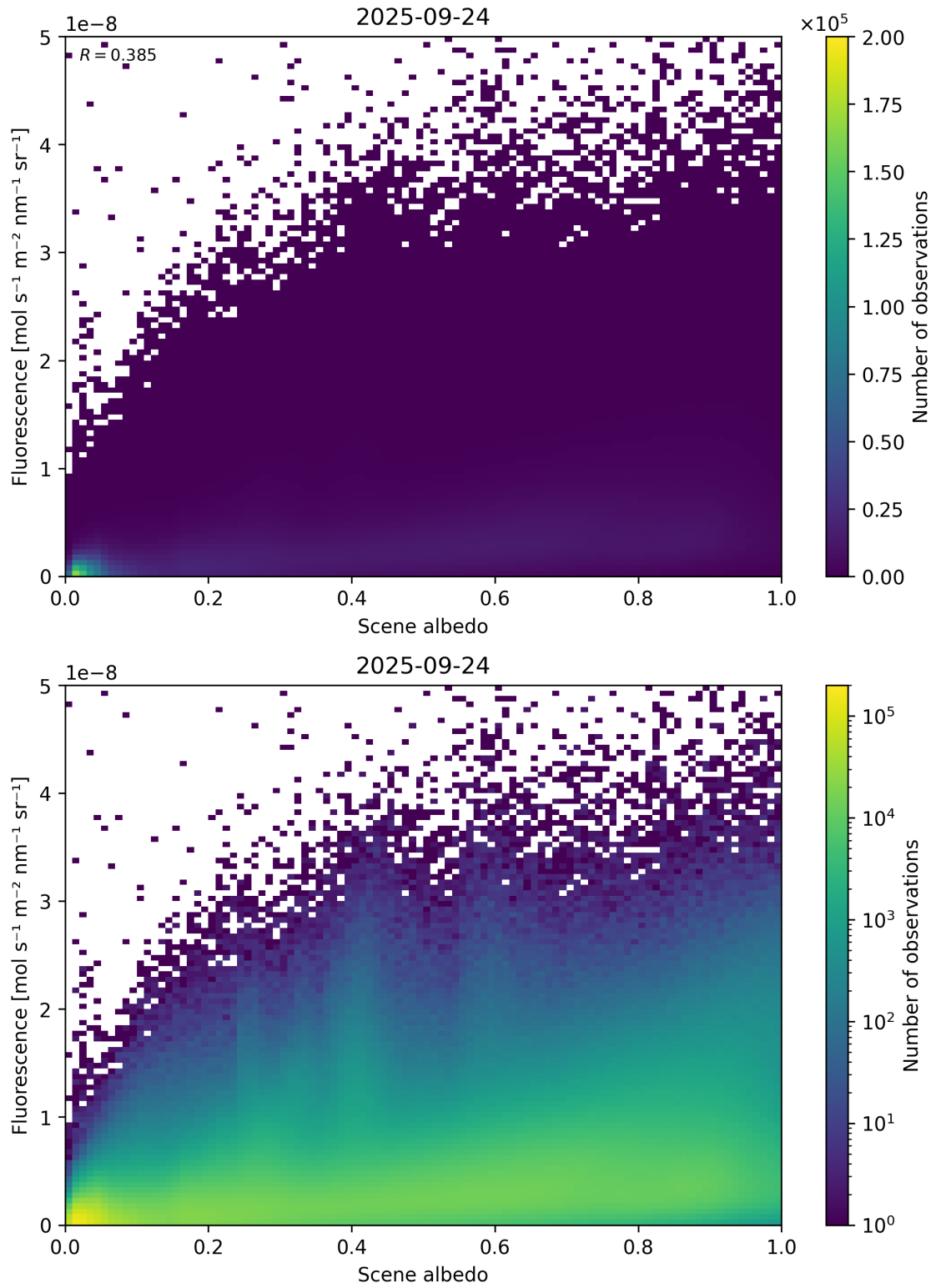
Figure 104: Scatter density plot of “Scene albedo” against “Fluorescence” for 2025-09-23 to 2025-09-25.
