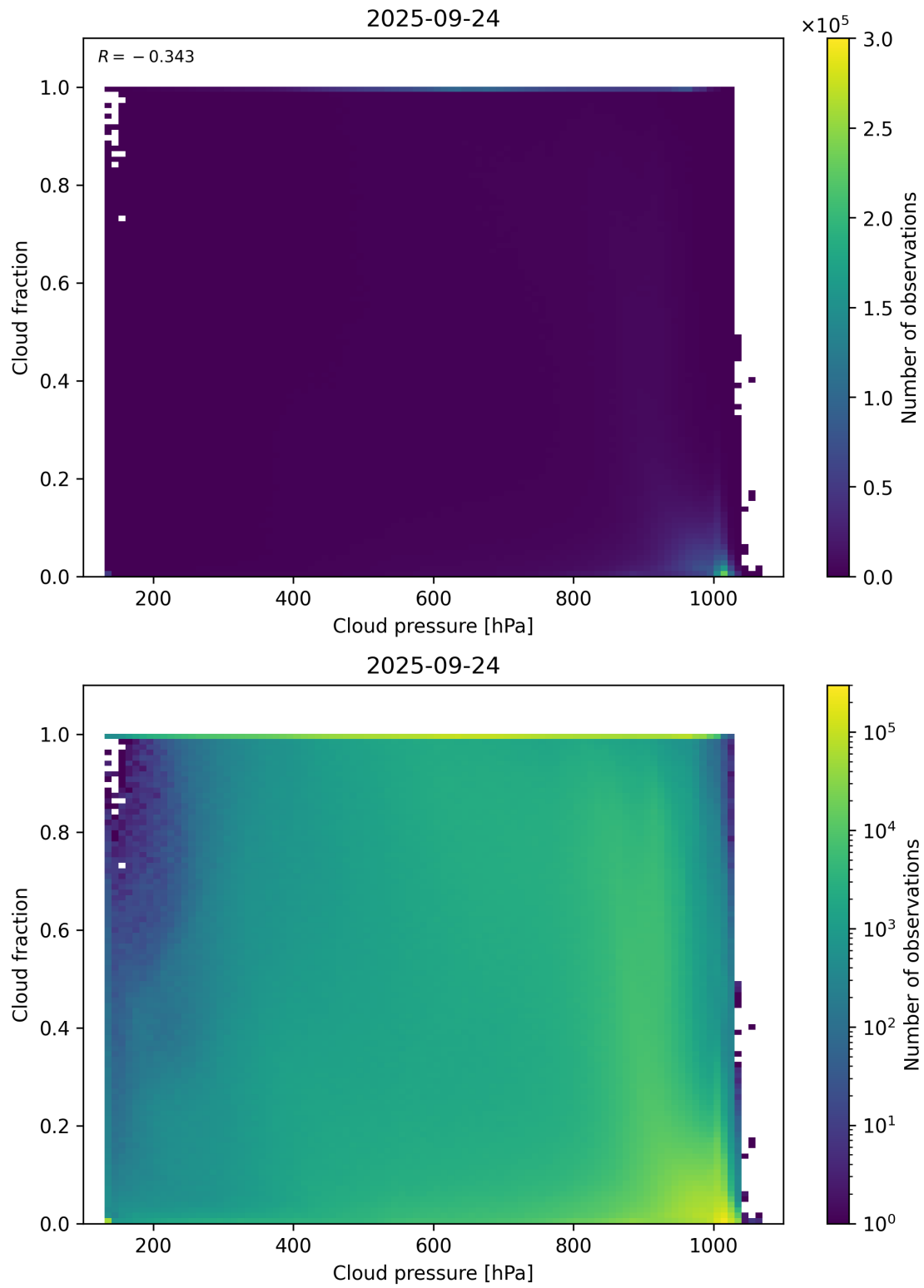
Figure 79: Scatter density plot of “Cloud pressure” against “Cloud fraction” for 2025-09-23 to 2025-09-25.
