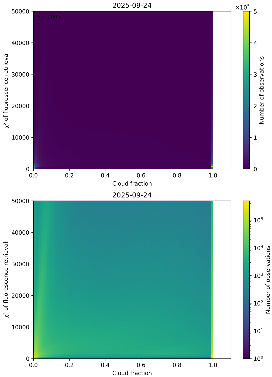
Figure 71: Scatter density plot of “Cloud fraction” against “ \chi^2 of fluorescence retrieval” for 2025-09-23 to 2025-09-25.
