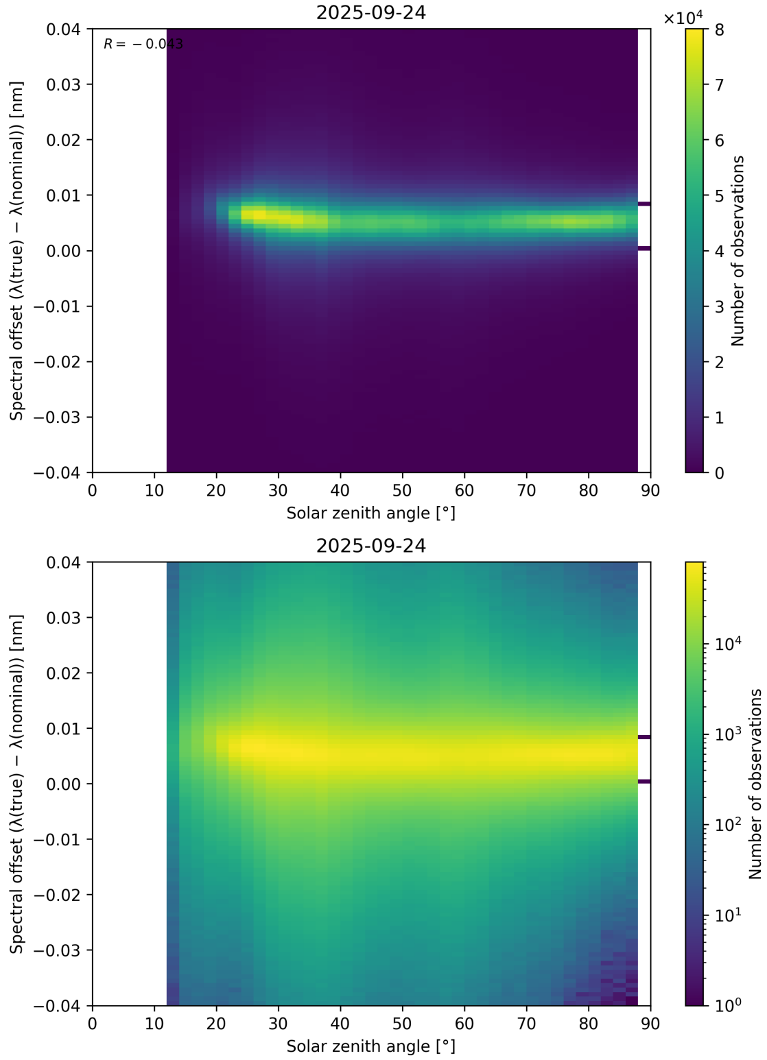
Figure 117: Scatter density plot of “Solar zenith angle” against “Spectral offset ( \lambda_{\text{true}} - \lambda_{\text{nominal}} )” for 2025-09-23 to 2025-09-25.
