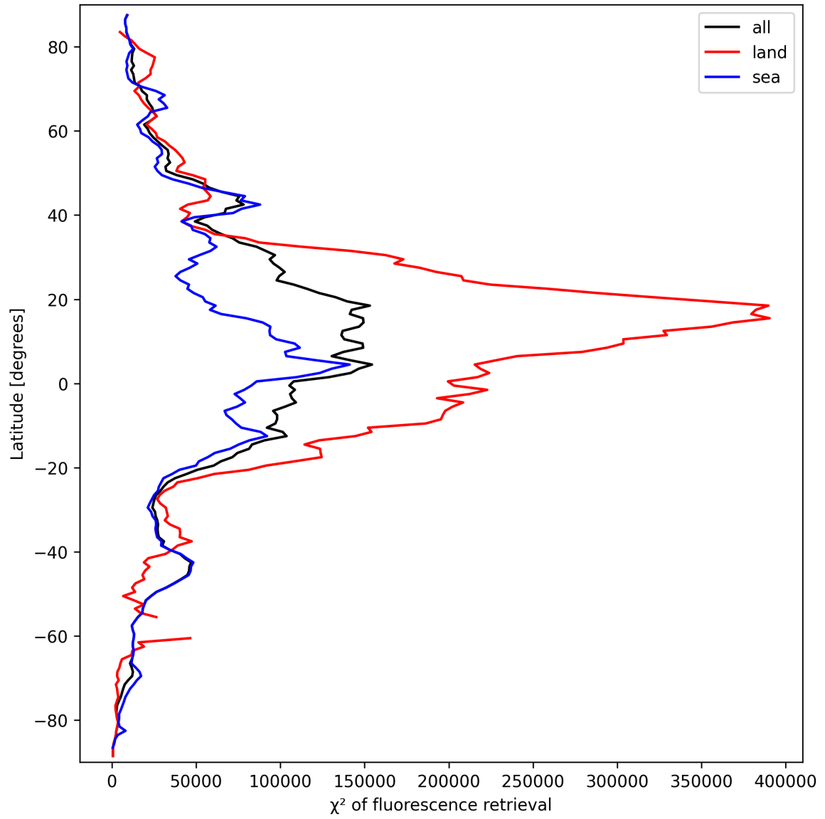
Figure 25: Zonal average of “ \chi^2 of fluorescence retrieval” for 2025-09-23 to 2025-09-25.
