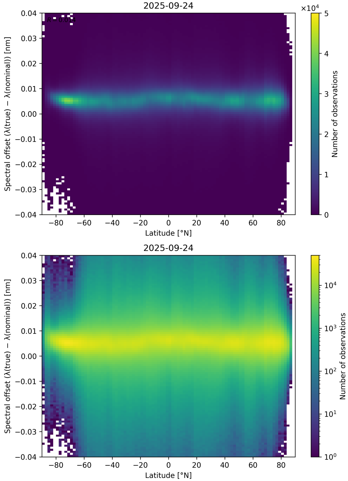
Figure 96: Scatter density plot of “Latitude” against “Spectral offset ( \lambda_{\text{true}} - \lambda_{\text{nominal}} )” for 2025-09-23 to 2025-09-25.
