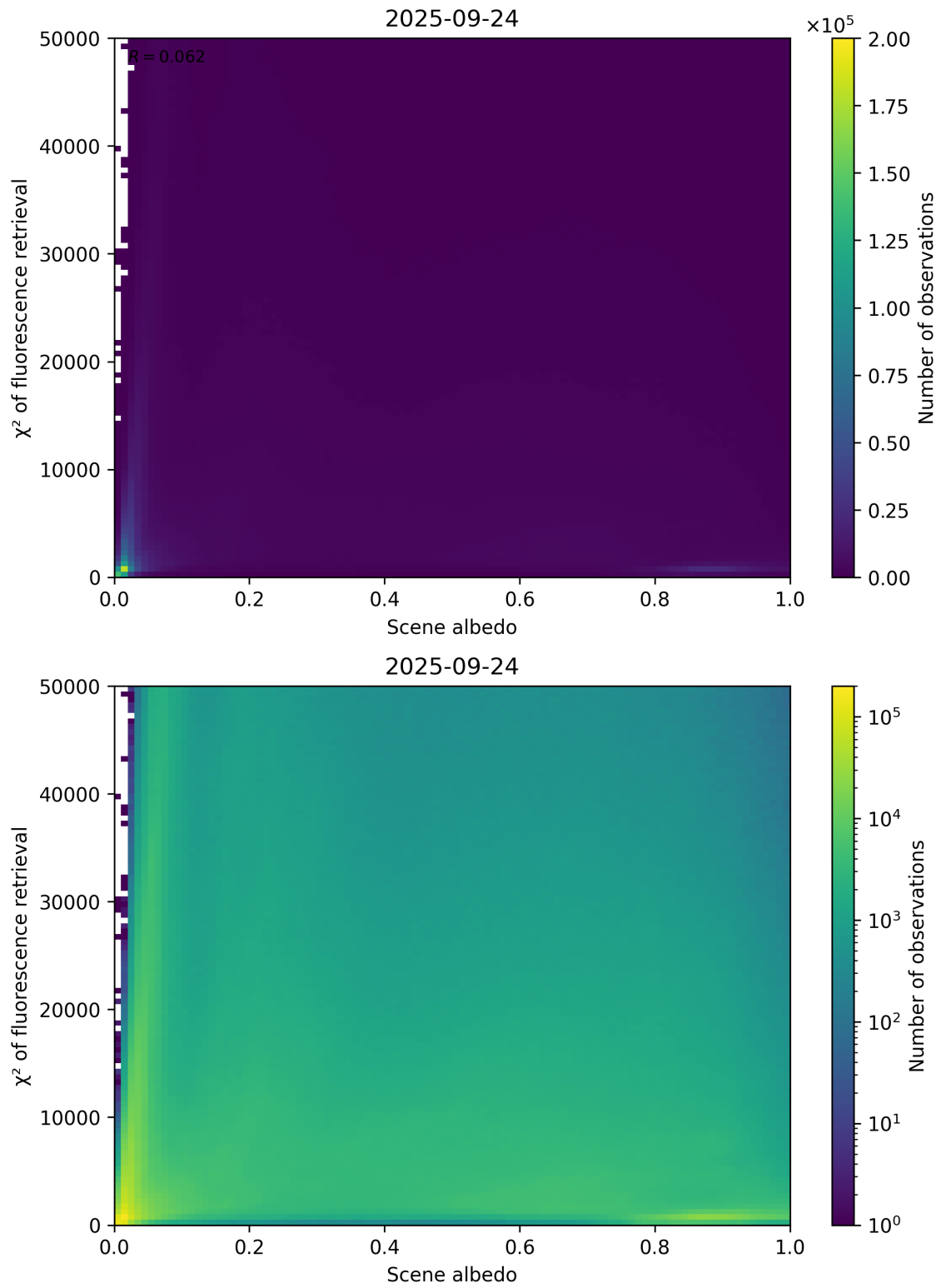
Figure 103: Scatter density plot of “Scene albedo” against “ \chi^2 of fluorescence retrieval” for 2025-09-23 to 2025-09-25.
