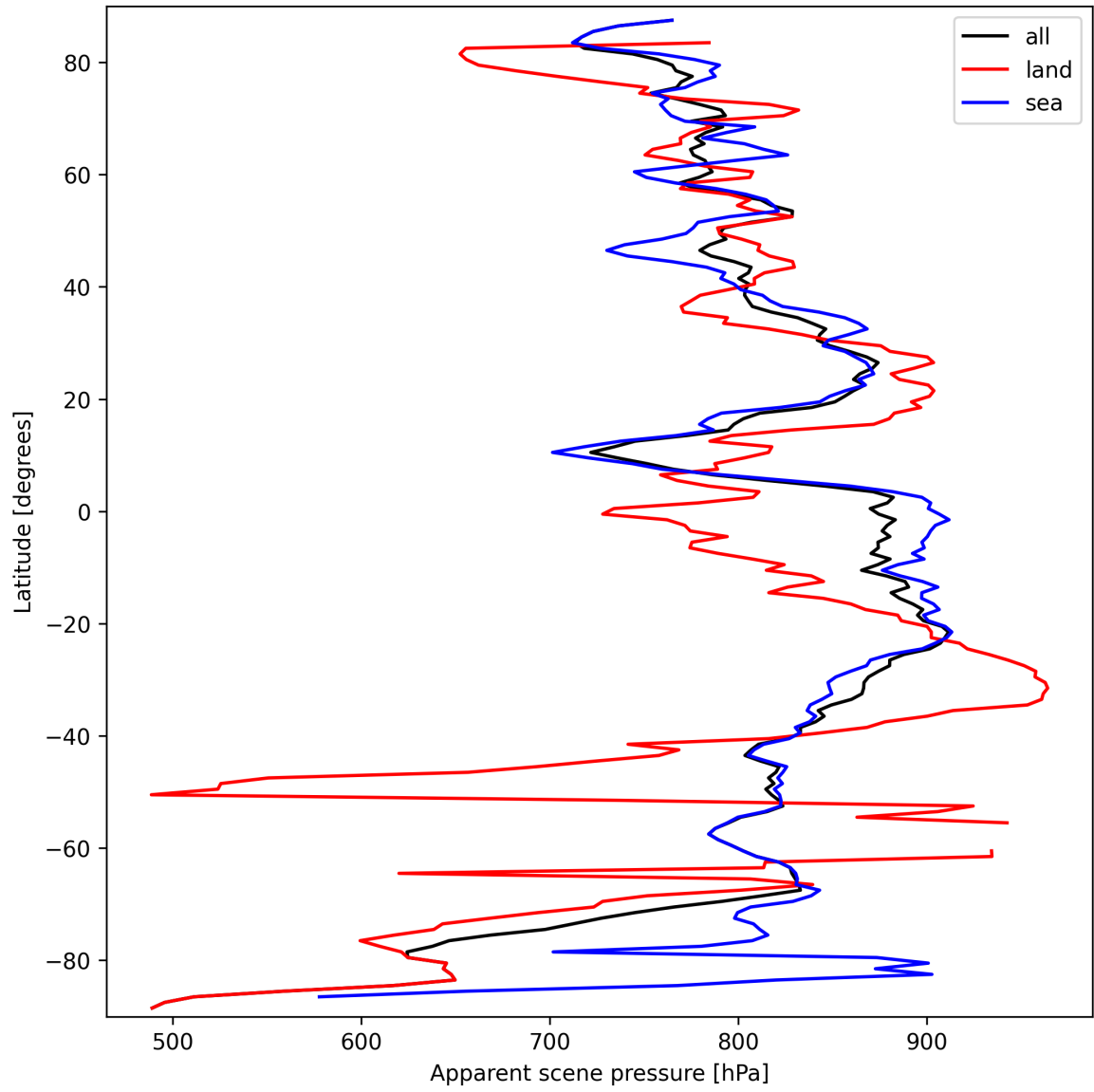
Figure 19: Zonal average of “Apparent scene pressure” for 2025-09-23 to 2025-09-25.
