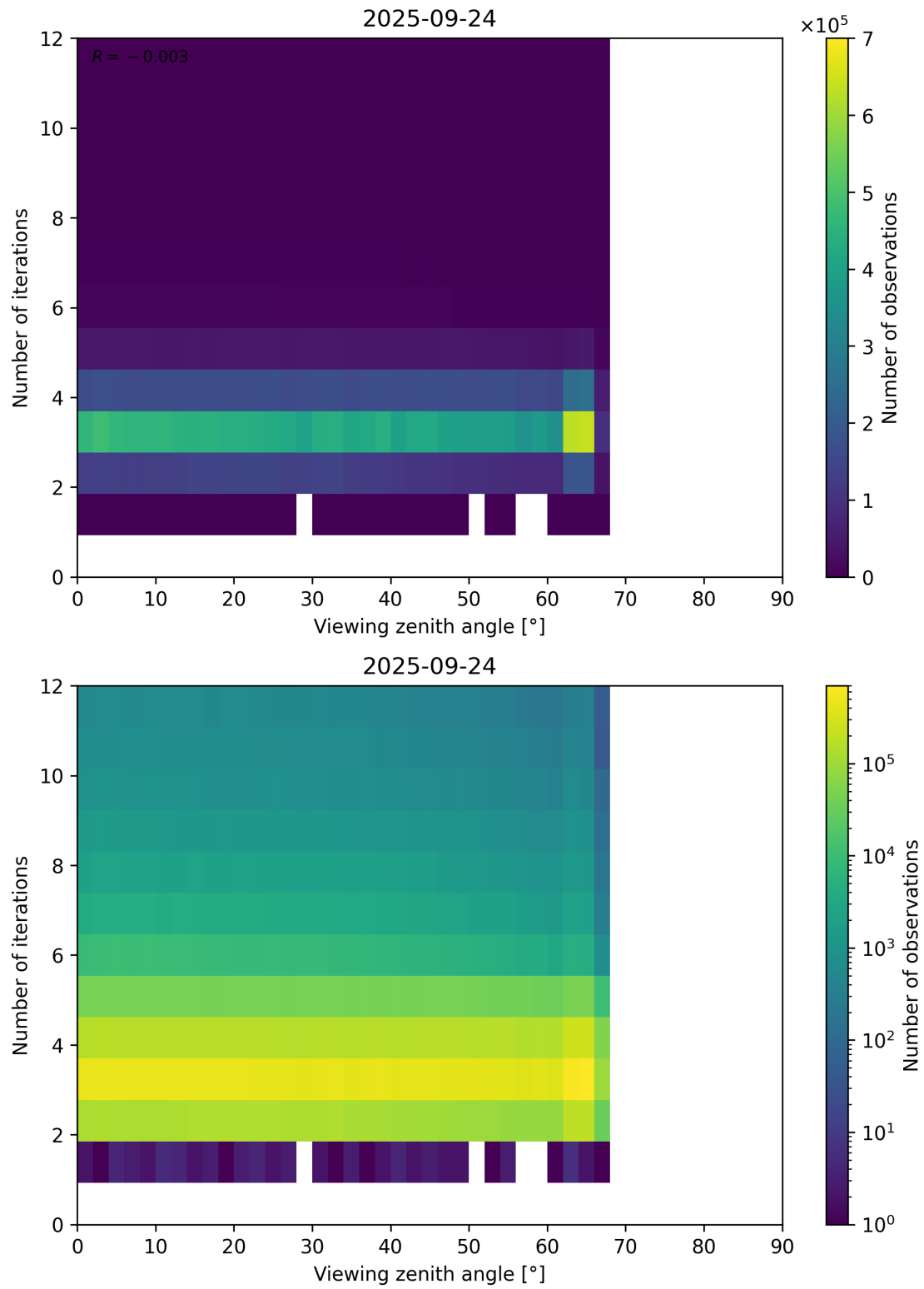
Figure 124: Scatter density plot of “Viewing zenith angle” against “Number of iterations” for 2025-09-23 to 2025-09-25.
