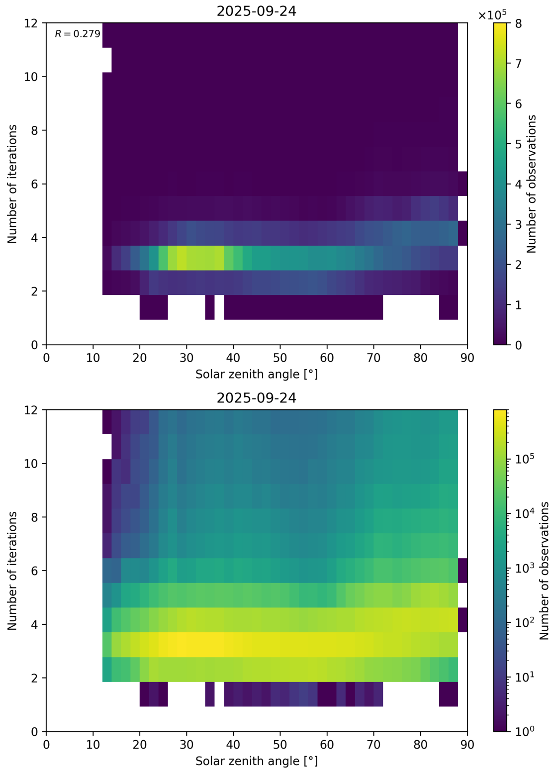
Figure 114: Scatter density plot of “Solar zenith angle” against “Number of iterations” for 2025-09-23 to 2025-09-25.
