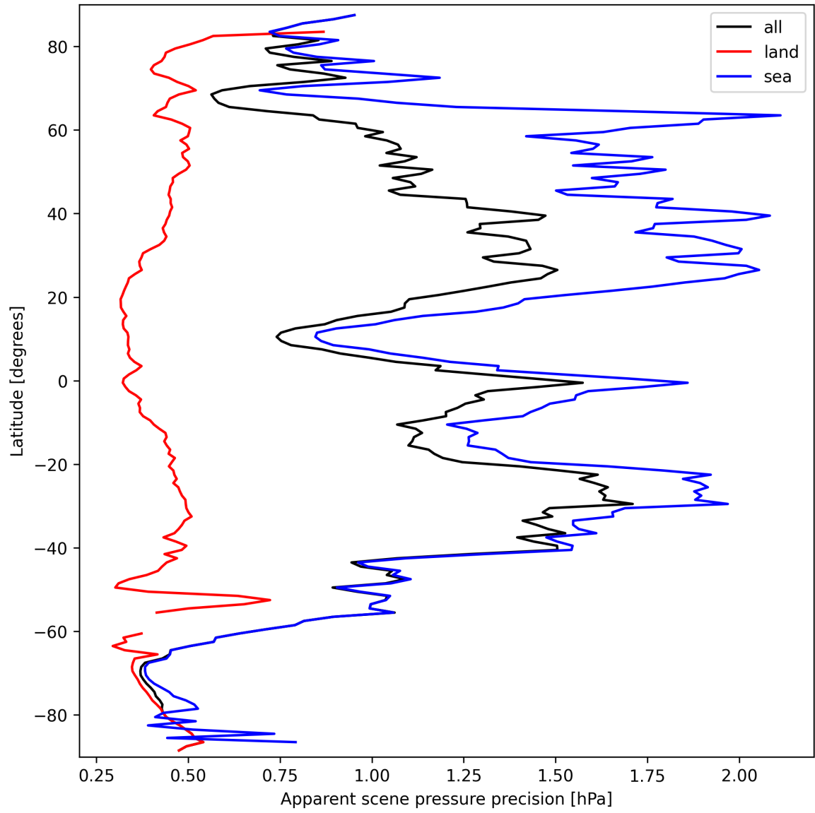
Figure 20: Zonal average of “Apparent scene pressure precision” for 2025-09-23 to 2025-09-25.
