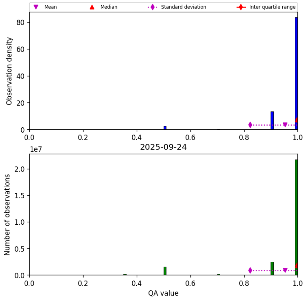
Figure 29: Histogram of “QA value” for 2025-09-23 to 2025-09-25
