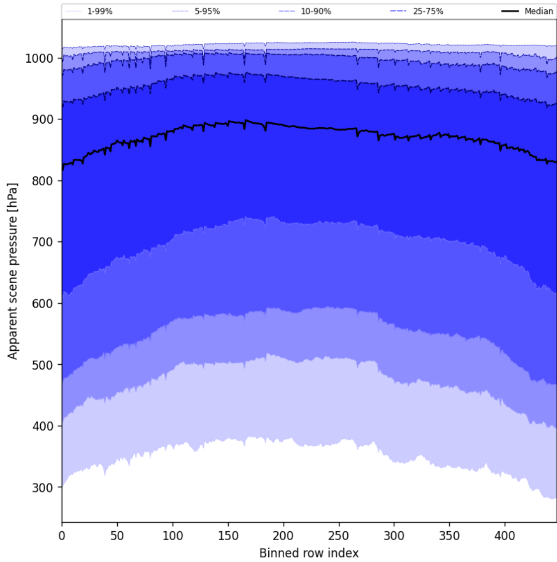
Figure 53: Along track statistics of “Apparent scene pressure” for 2025-09-23 to 2025-09-25
