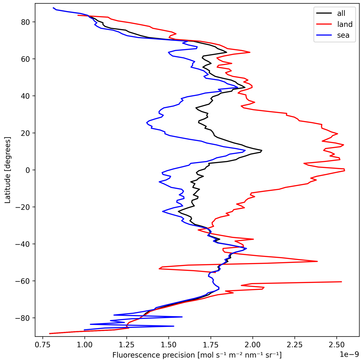
Figure 24: Zonal average of “Fluorescence precision” for 2025-09-23 to 2025-09-25.
