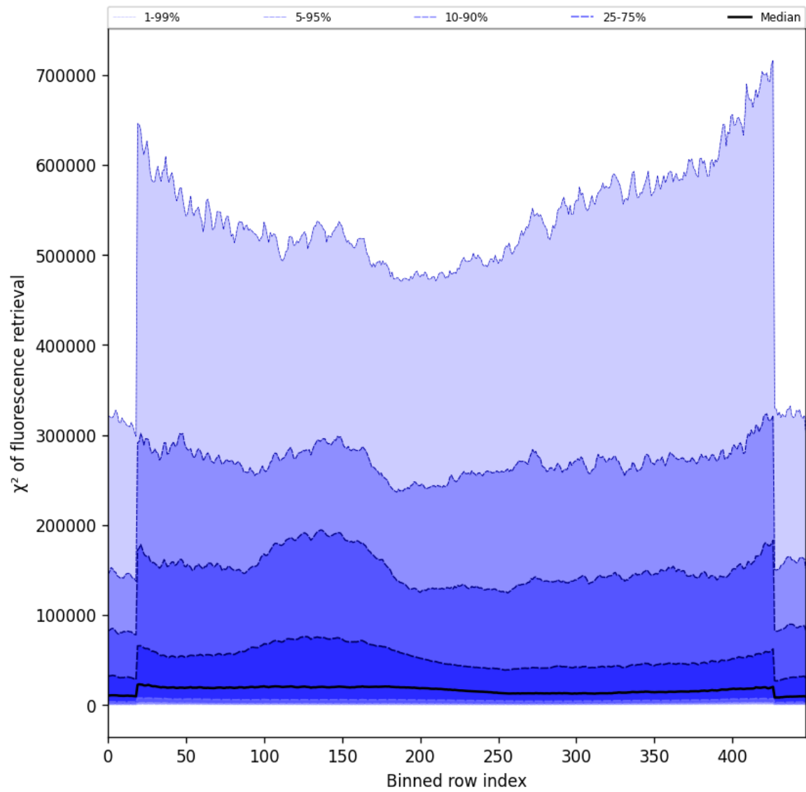
Figure 59: Along track statistics of “ \chi^2 of fluorescence retrieval” for 2025-09-23 to 2025-09-25
