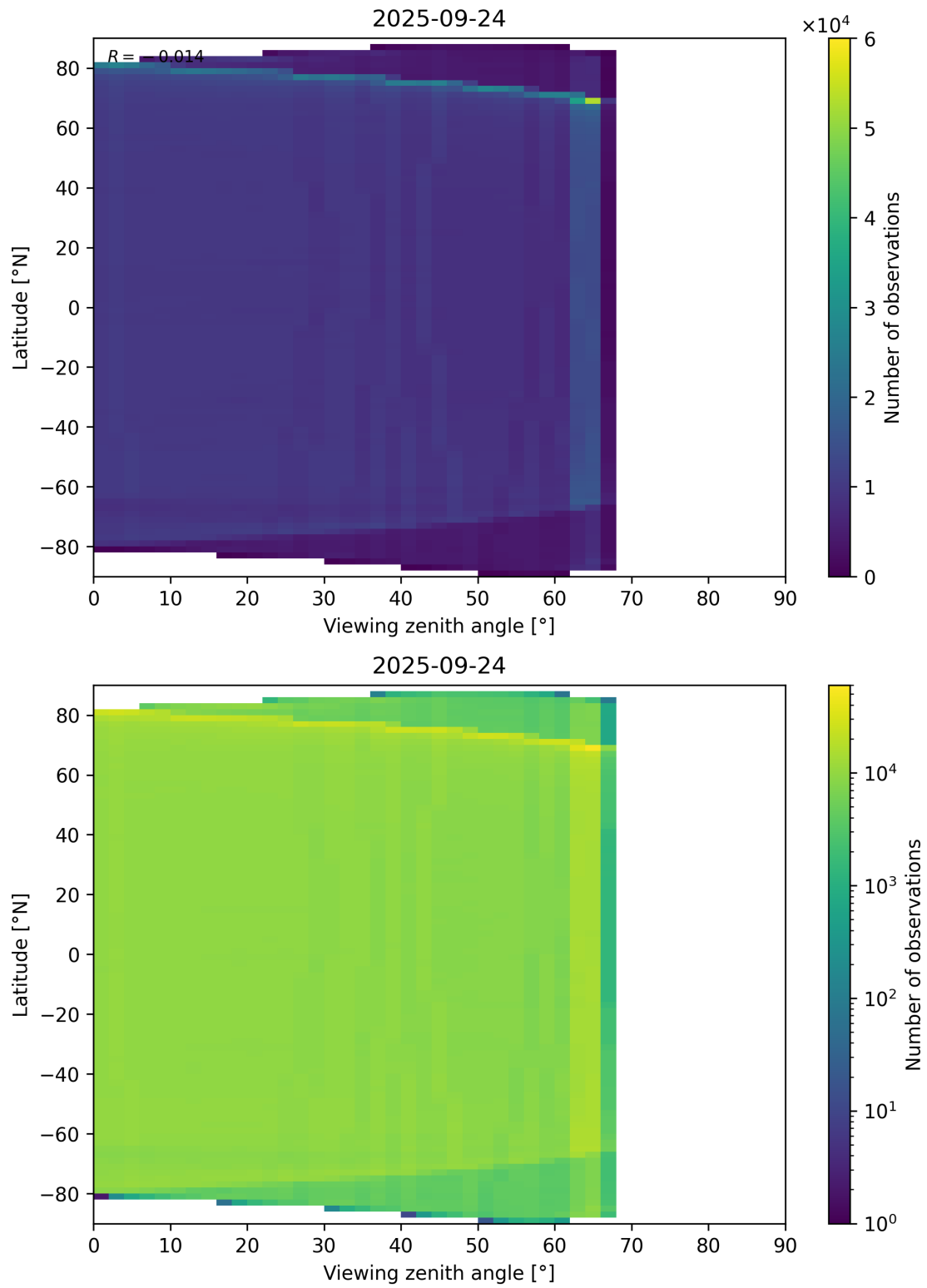
Figure 123: Scatter density plot of “Viewing zenith angle” against “Latitude” for 2025-09-23 to 2025-09-25.
