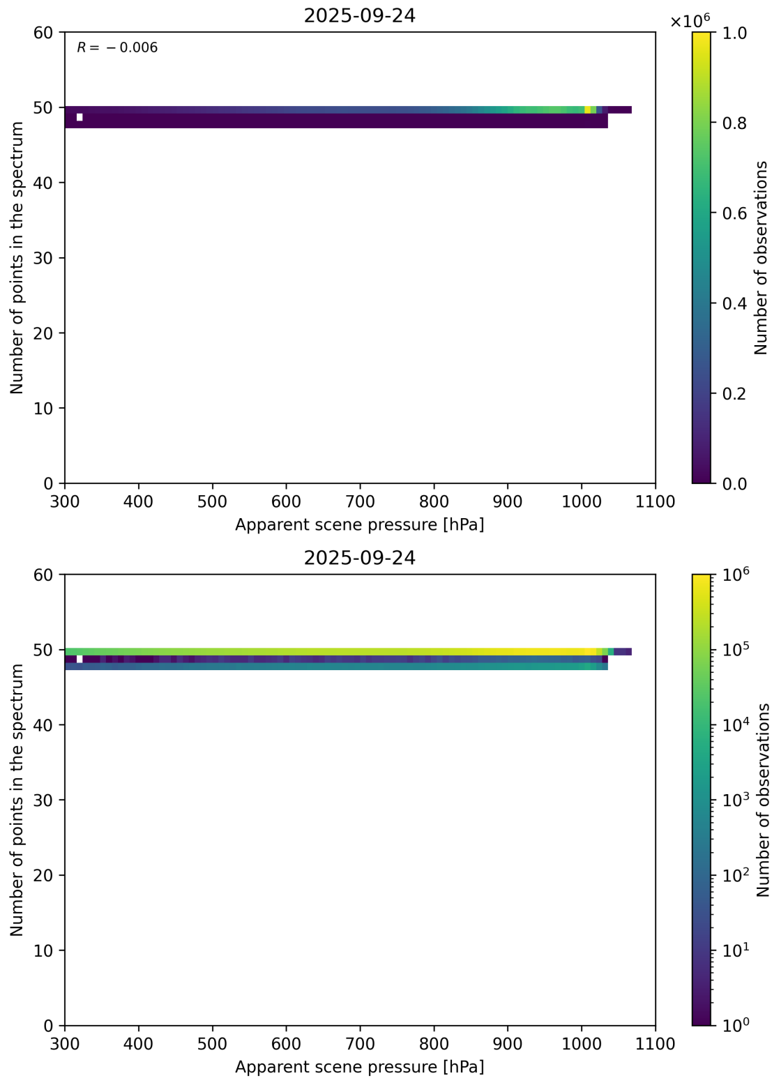
Figure 66: Scatter density plot of “Apparent scene pressure” against “Number of points in the spectrum” for 2025-09-23 to 2025-09-25.
