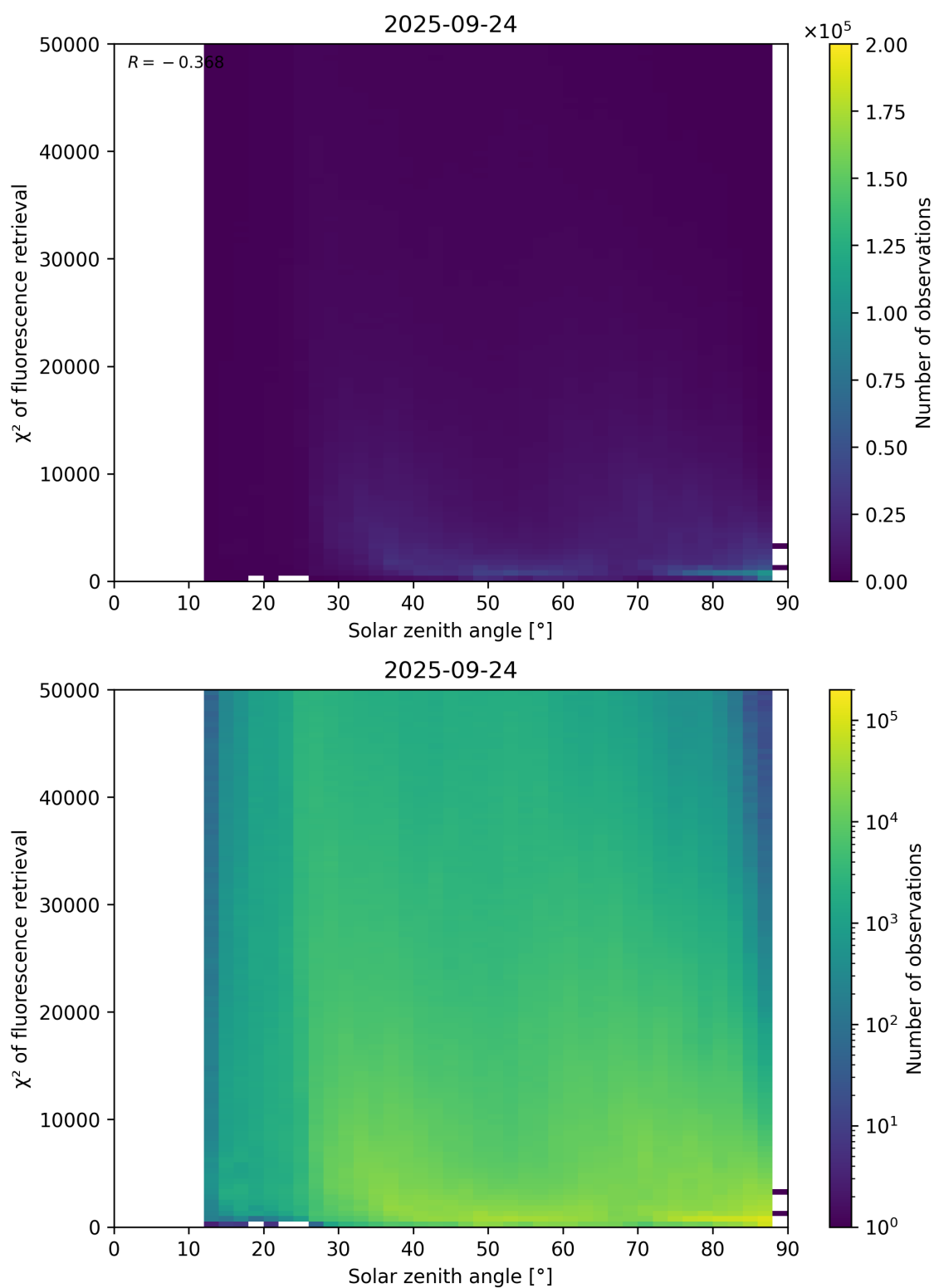
Figure 109: Scatter density plot of “Solar zenith angle” against “ \chi^2 of fluorescence retrieval” for 2025-09-23 to 2025-09-25.
