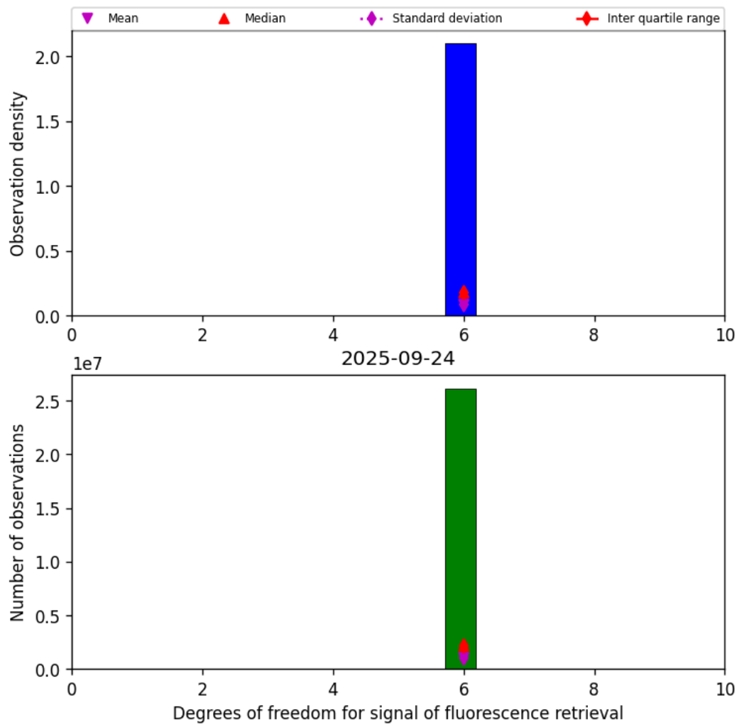
Figure 43: Histogram of “Degrees of freedom for signal of fluorescence retrieval” for 2025-09-23 to 2025-09-25
