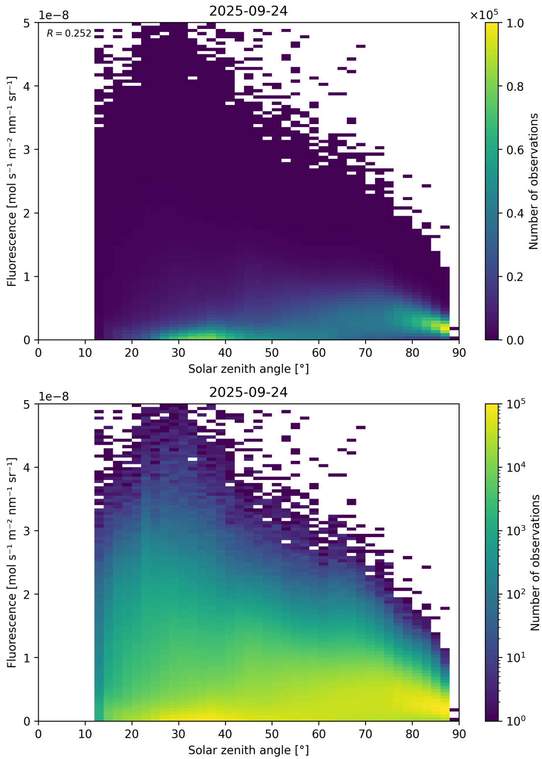
Figure 112: Scatter density plot of “Solar zenith angle” against “Fluorescence” for 2025-09-23 to 2025-09-25.
