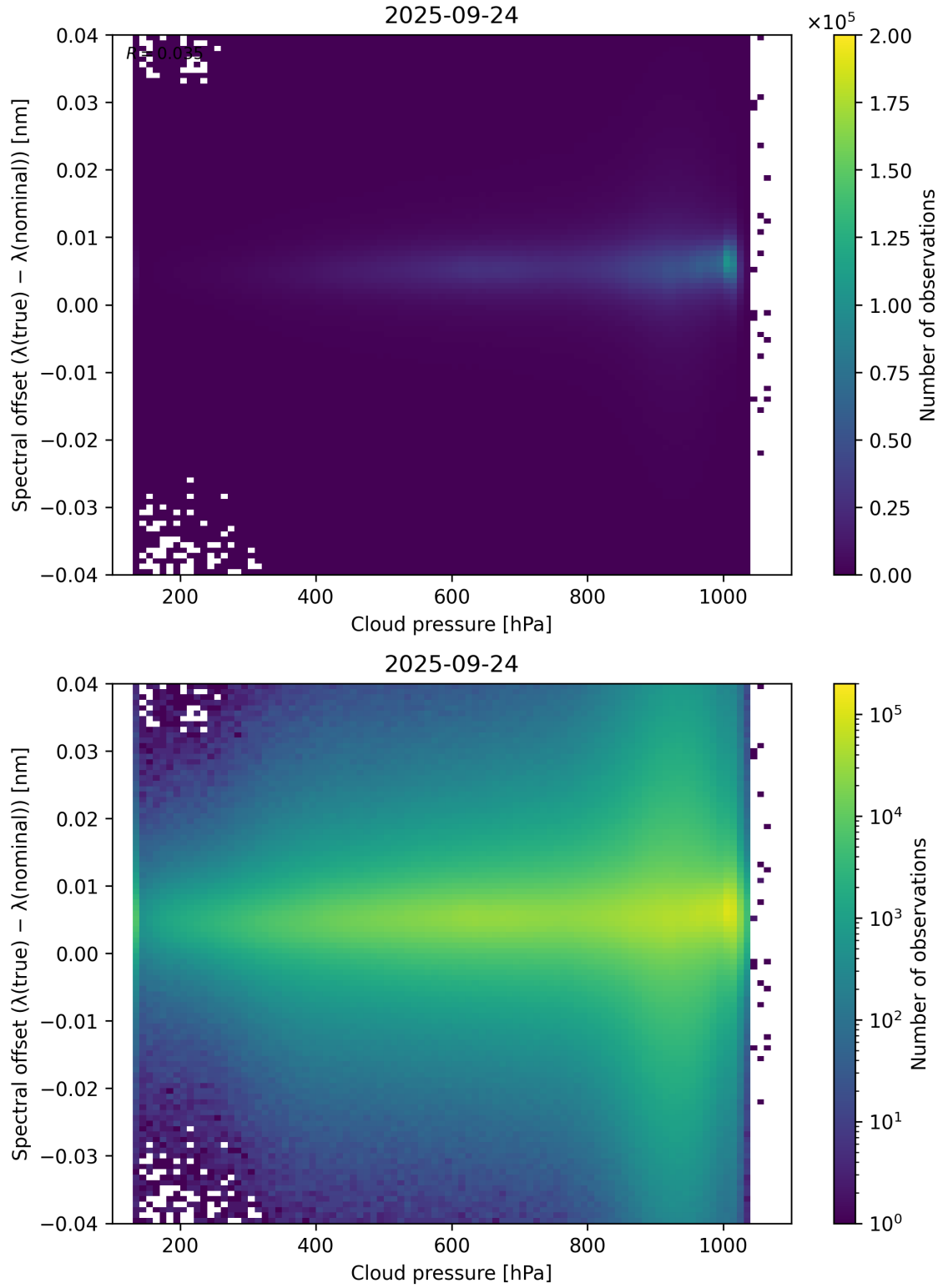
Figure 84: Scatter density plot of “Cloud pressure” against “Spectral offset ( \lambda_{\text{true}} - \lambda_{\text{nominal}} )” for 2025-09-23 to 2025-09-25.
