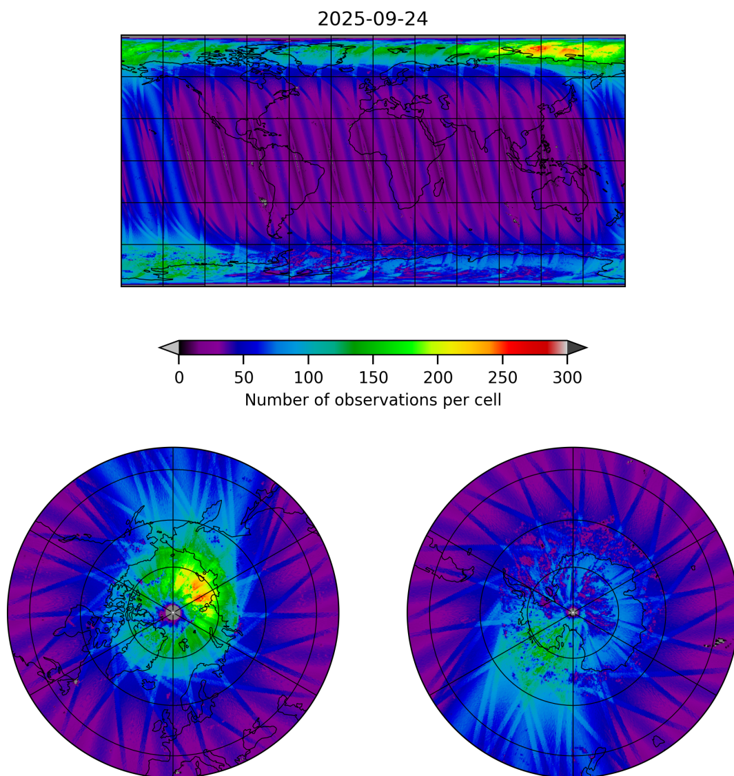
Figure 11: Map of the number of observations for 2025-09-23 to 2025-09-25
