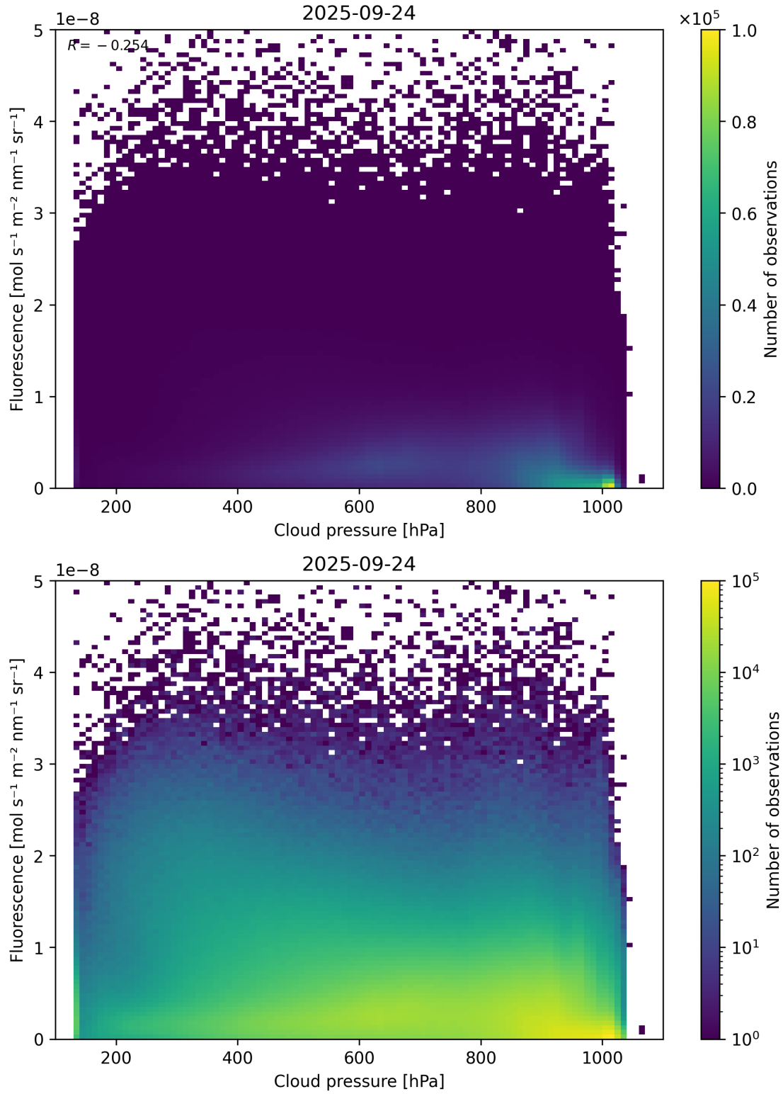
Figure 80: Scatter density plot of “Cloud pressure” against “Fluorescence” for 2025-09-23 to 2025-09-25.
