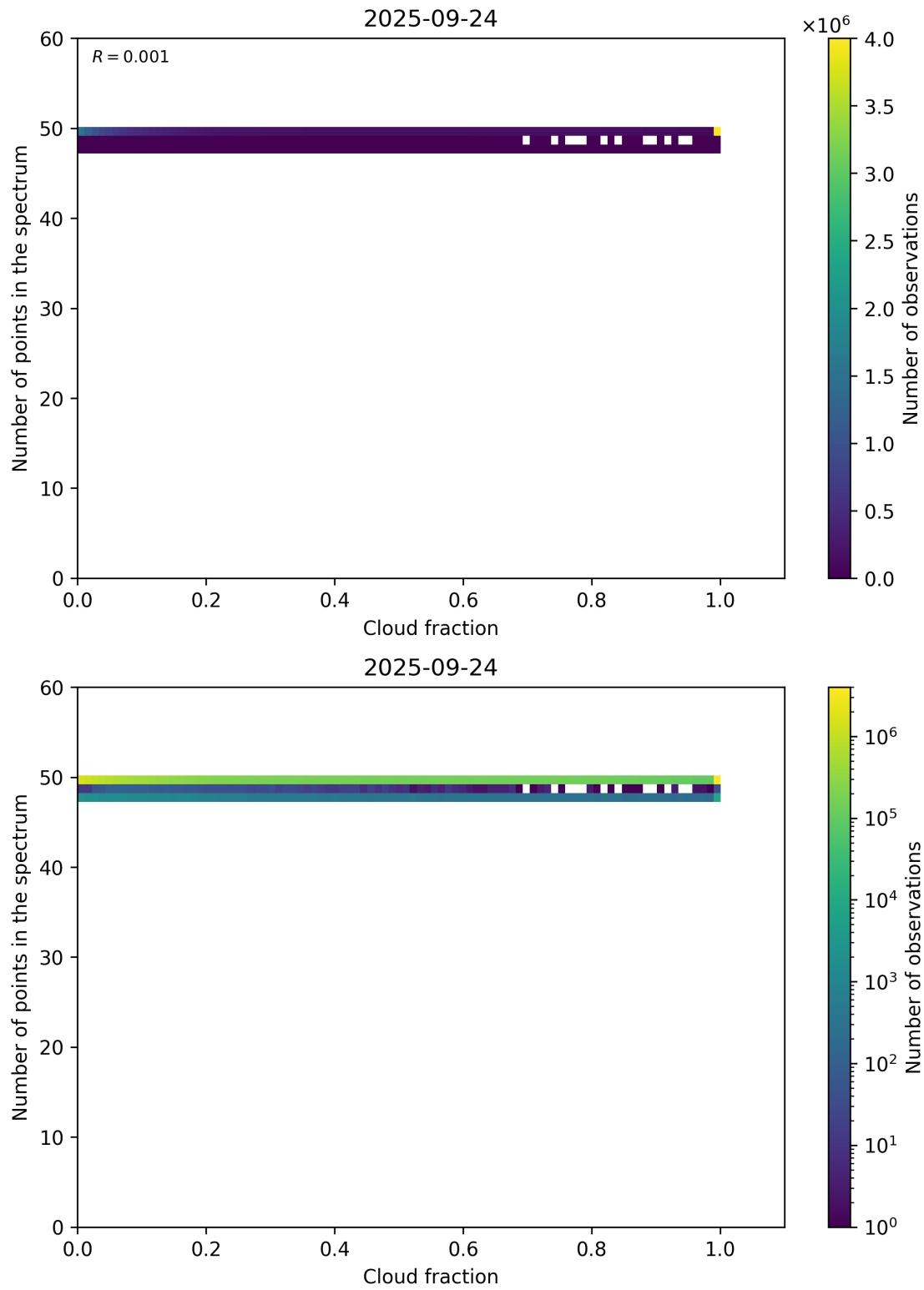
Figure 74: Scatter density plot of “Cloud fraction” against “Number of points in the spectrum” for 2025-09-23 to 2025-09-25.
