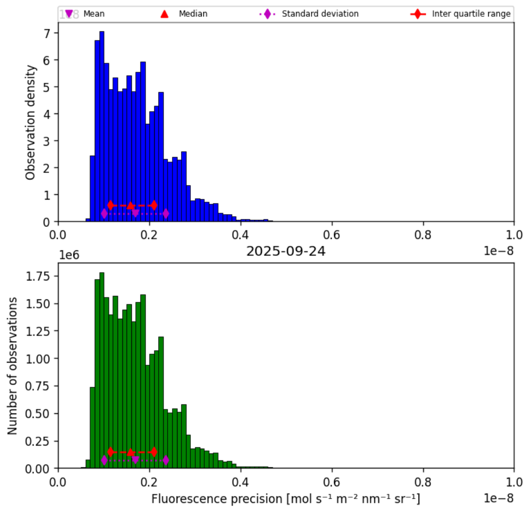
Figure 41: Histogram of “Fluorescence precision” for 2025-09-23 to 2025-09-25
