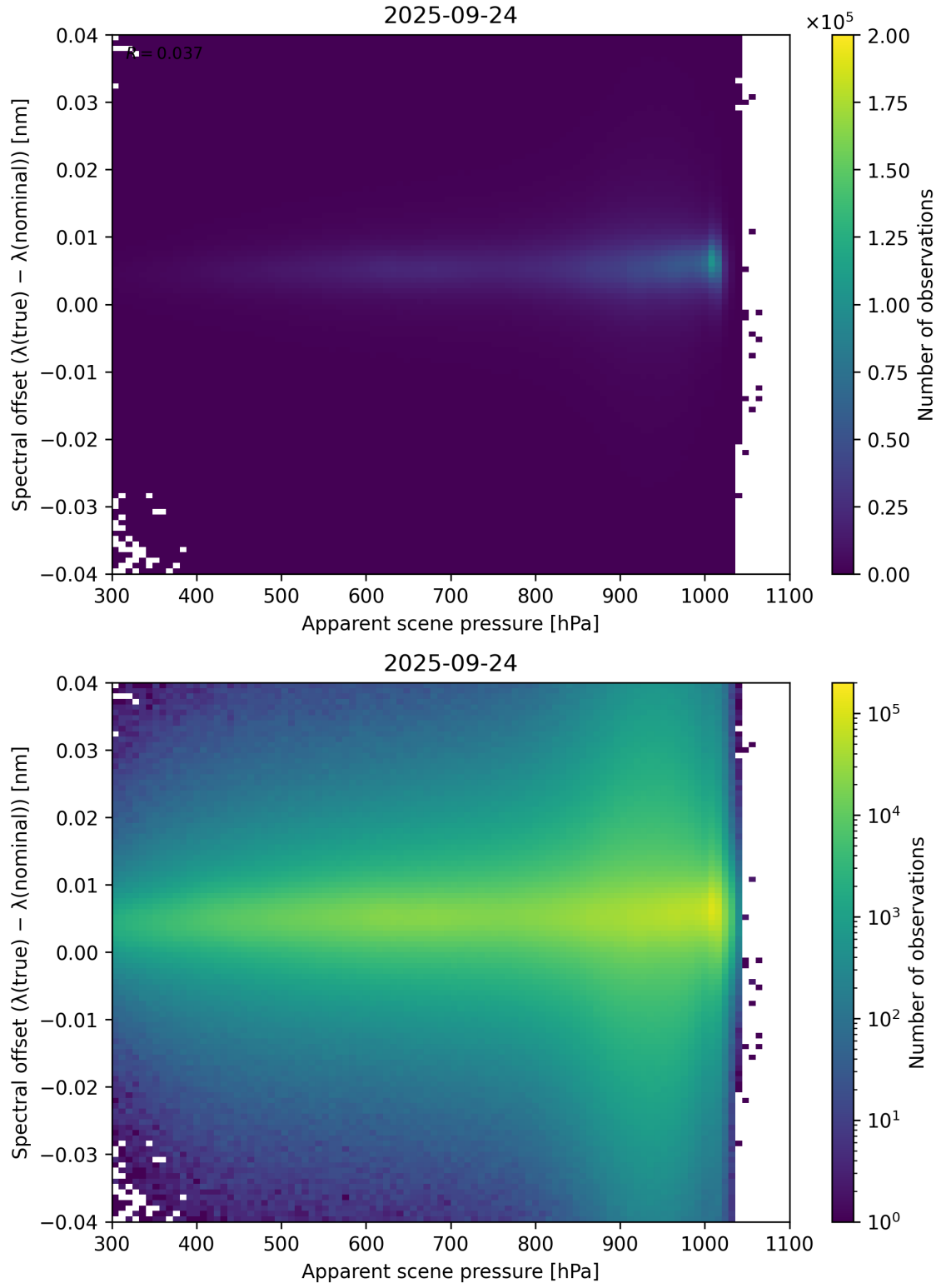
Figure 67: Scatter density plot of “Apparent scene pressure” against “Spectral offset ( \lambda_{\text{true}} - \lambda_{\text{nominal}} )” for 2025-09-23 to 2025-09-25.
