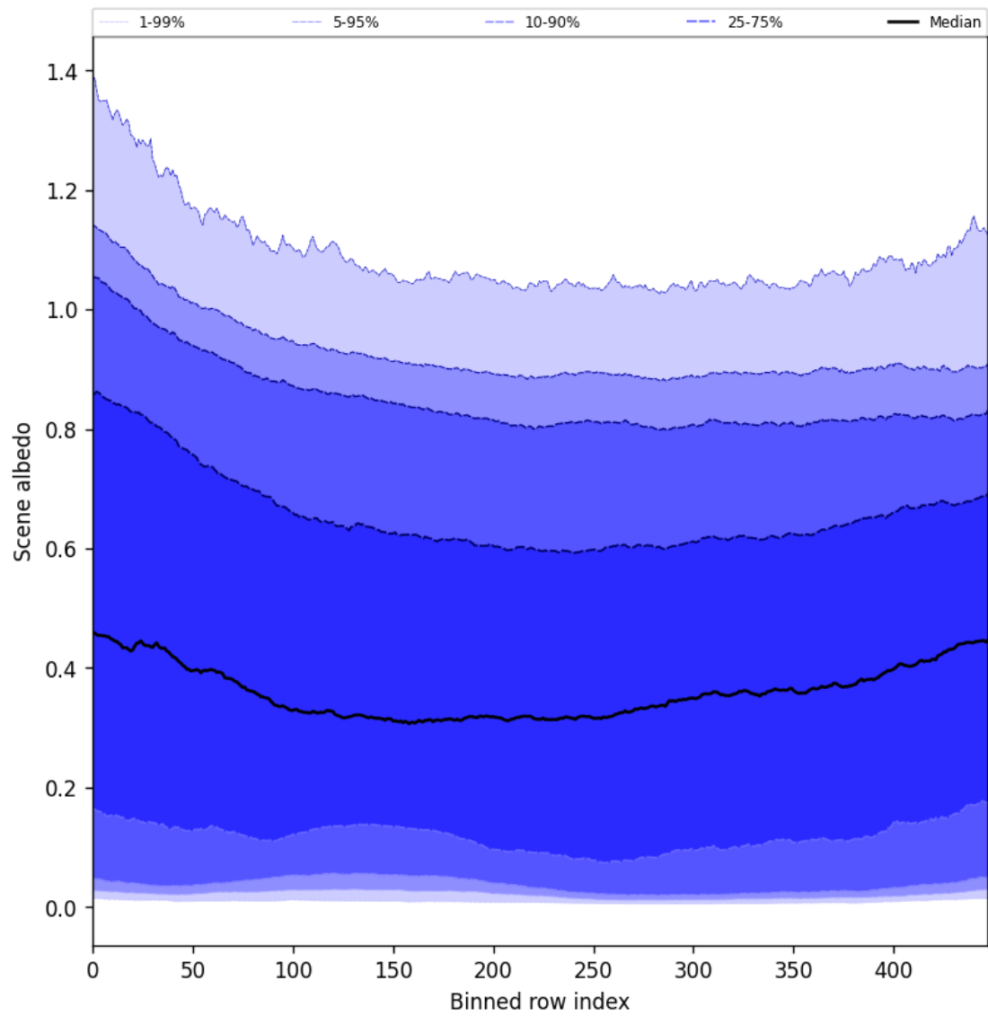
Figure 51: Along track statistics of “Scene albedo” for 2025-09-23 to 2025-09-25
