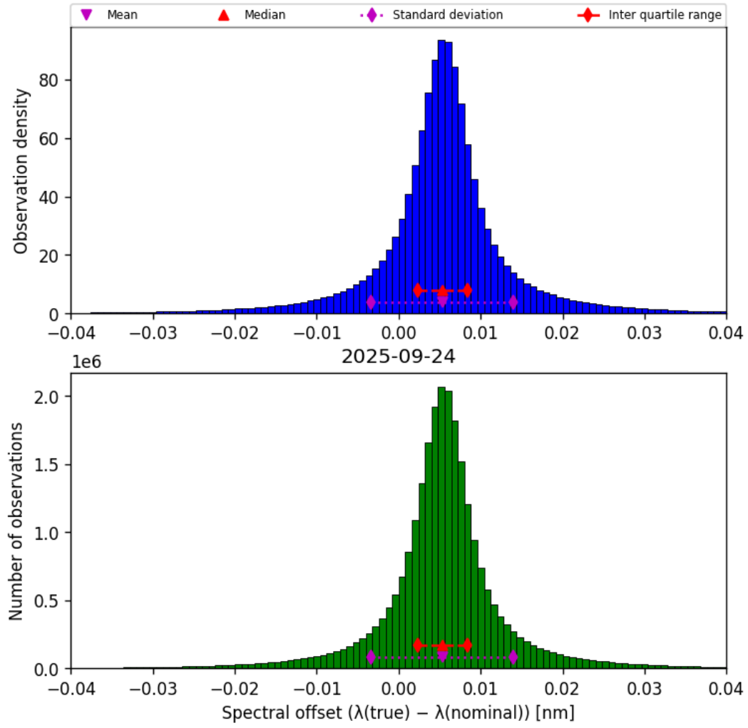
Figure 45: Histogram of “Spectral offset ( \lambda_{\text{true}} - \lambda_{\text{nominal}} )” for 2025-09-23 to 2025-09-25
