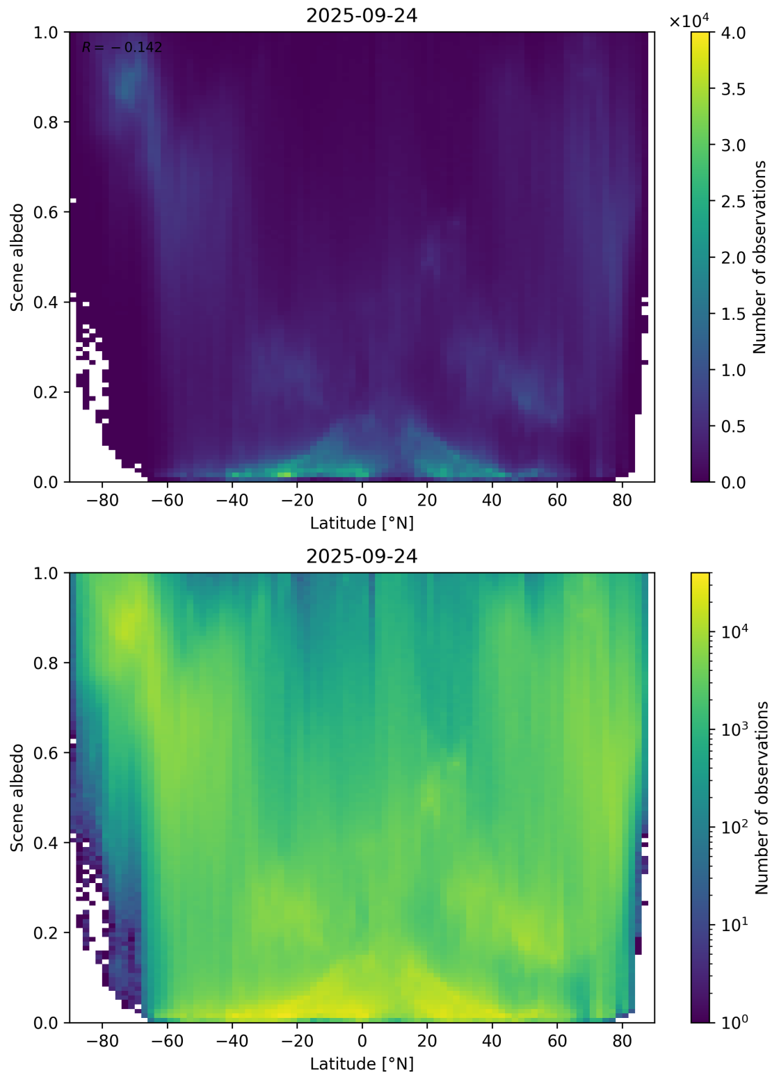
Figure 95: Scatter density plot of “Latitude” against “Scene albedo” for 2025-09-23 to 2025-09-25.
