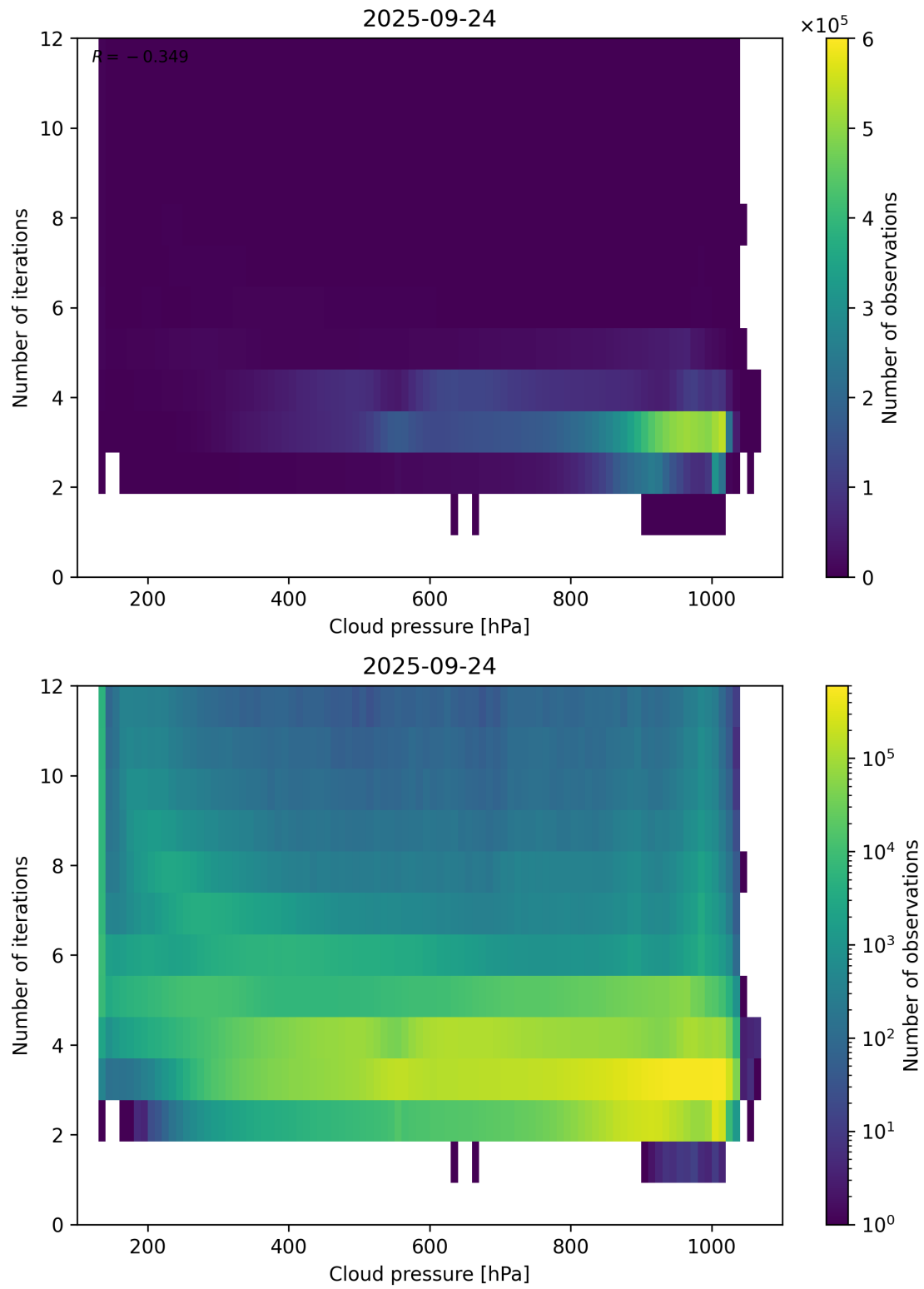
Figure 81: Scatter density plot of “Cloud pressure” against “Number of iterations” for 2025-09-23 to 2025-09-25.
