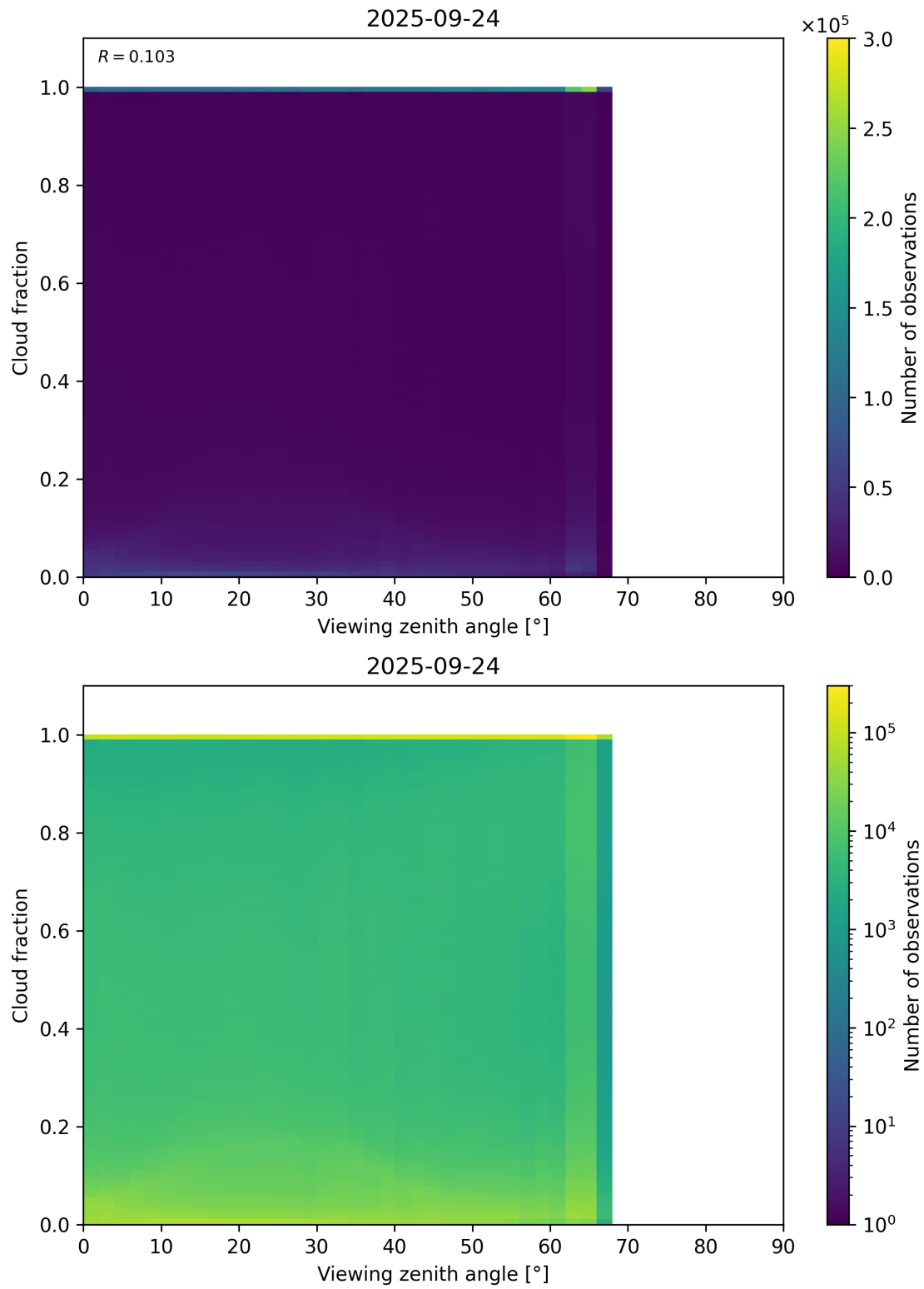
Figure 120: Scatter density plot of “Viewing zenith angle” against “Cloud fraction” for 2025-09-23 to 2025-09-25.
