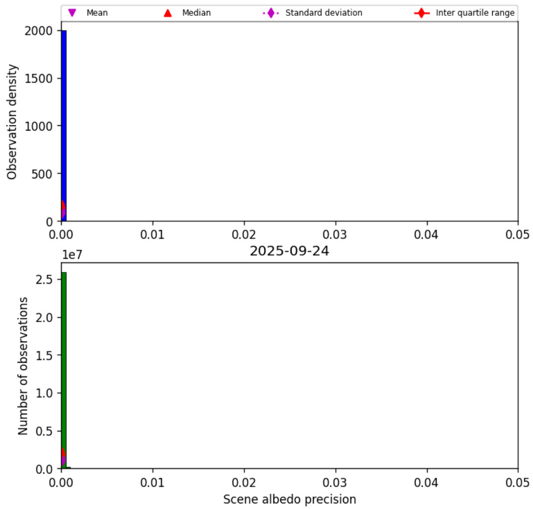
Figure 35: Histogram of “Scene albedo precision” for 2025-09-23 to 2025-09-25
