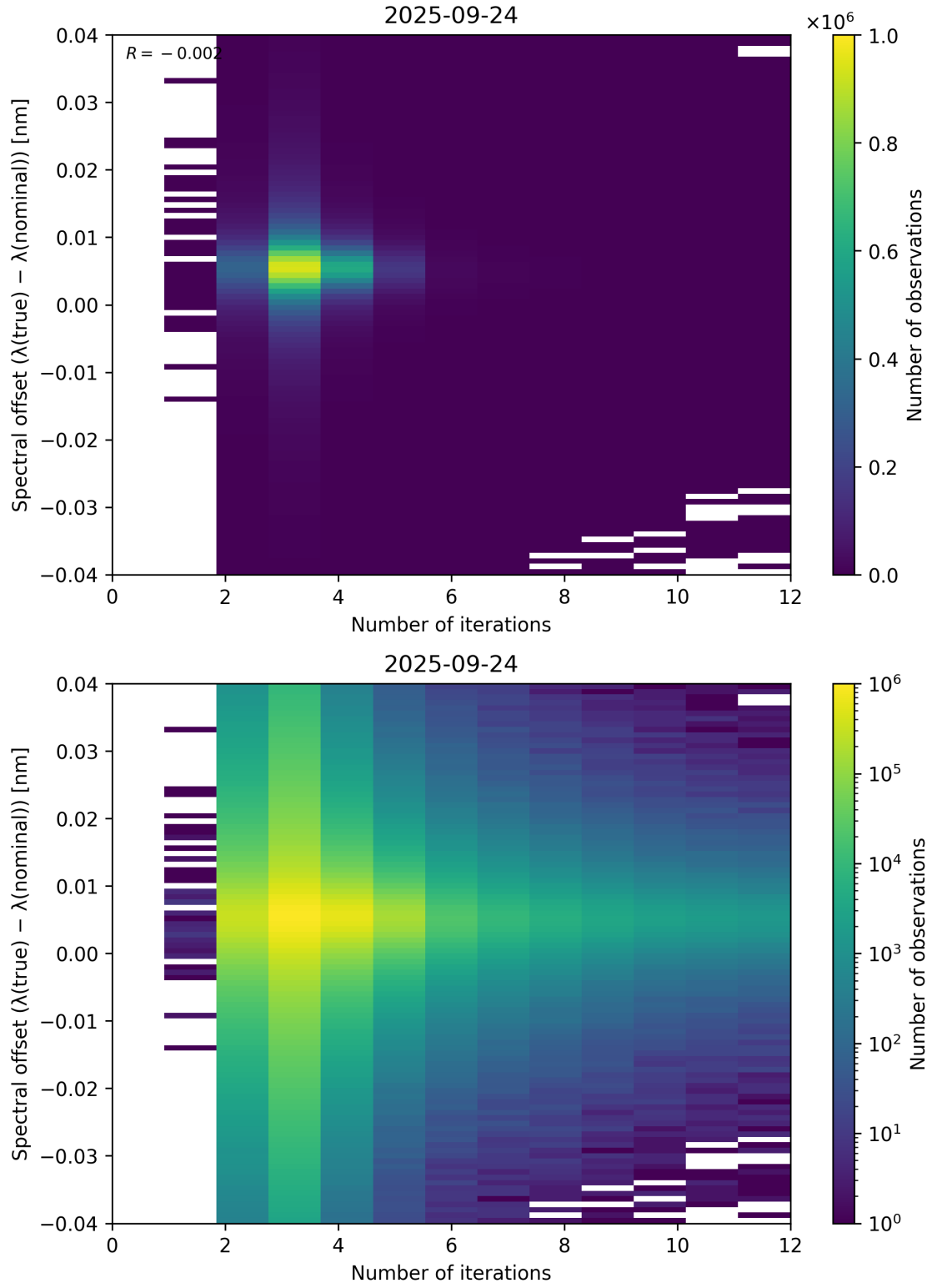
Figure 100: Scatter density plot of “Number of iterations” against “Spectral offset ( \lambda_{\text{true}} - \lambda_{\text{nominal}} )” for 2025-09-23 to 2025-09-25.
