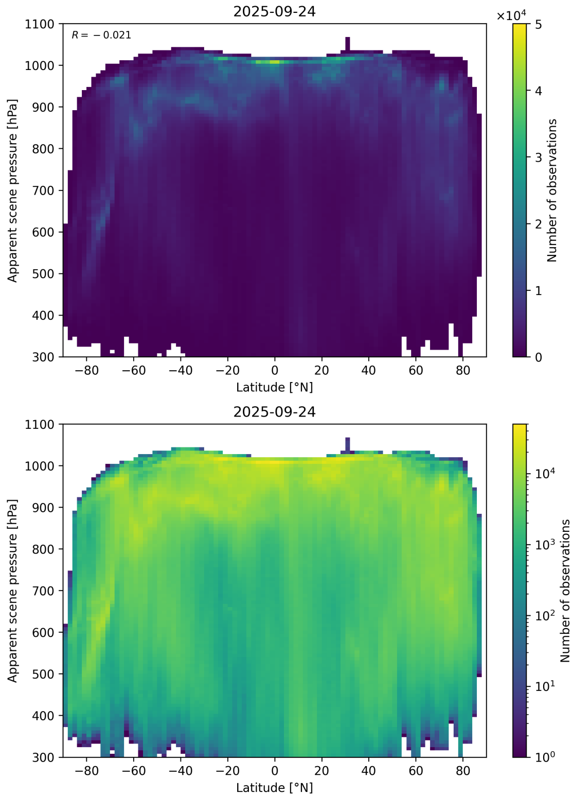
Figure 88: Scatter density plot of “Latitude” against “Apparent scene pressure” for 2025-09-23 to 2025-09-25.
