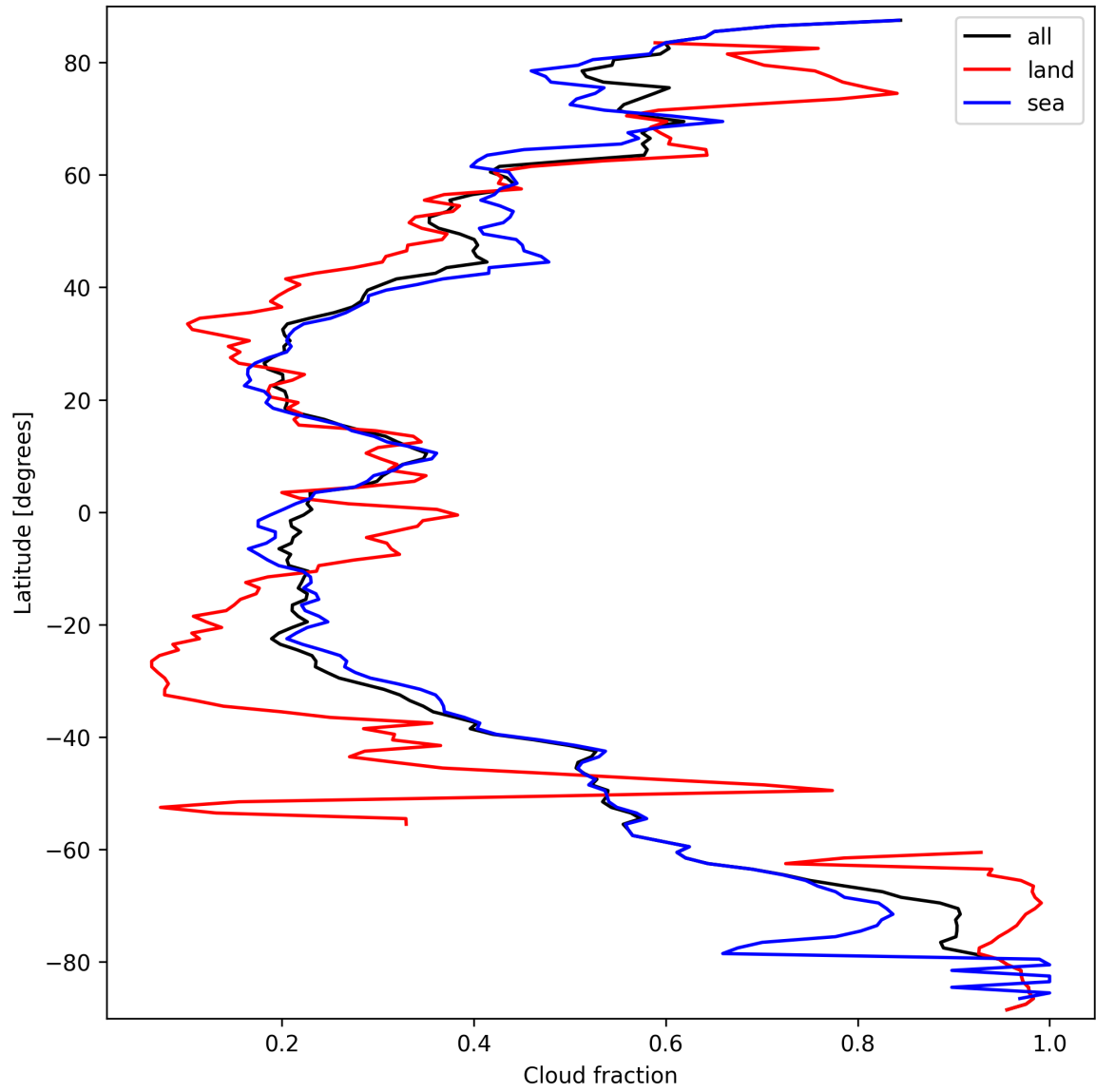
Figure 15: Zonal average of “Cloud fraction” for 2025-09-23 to 2025-09-25.
