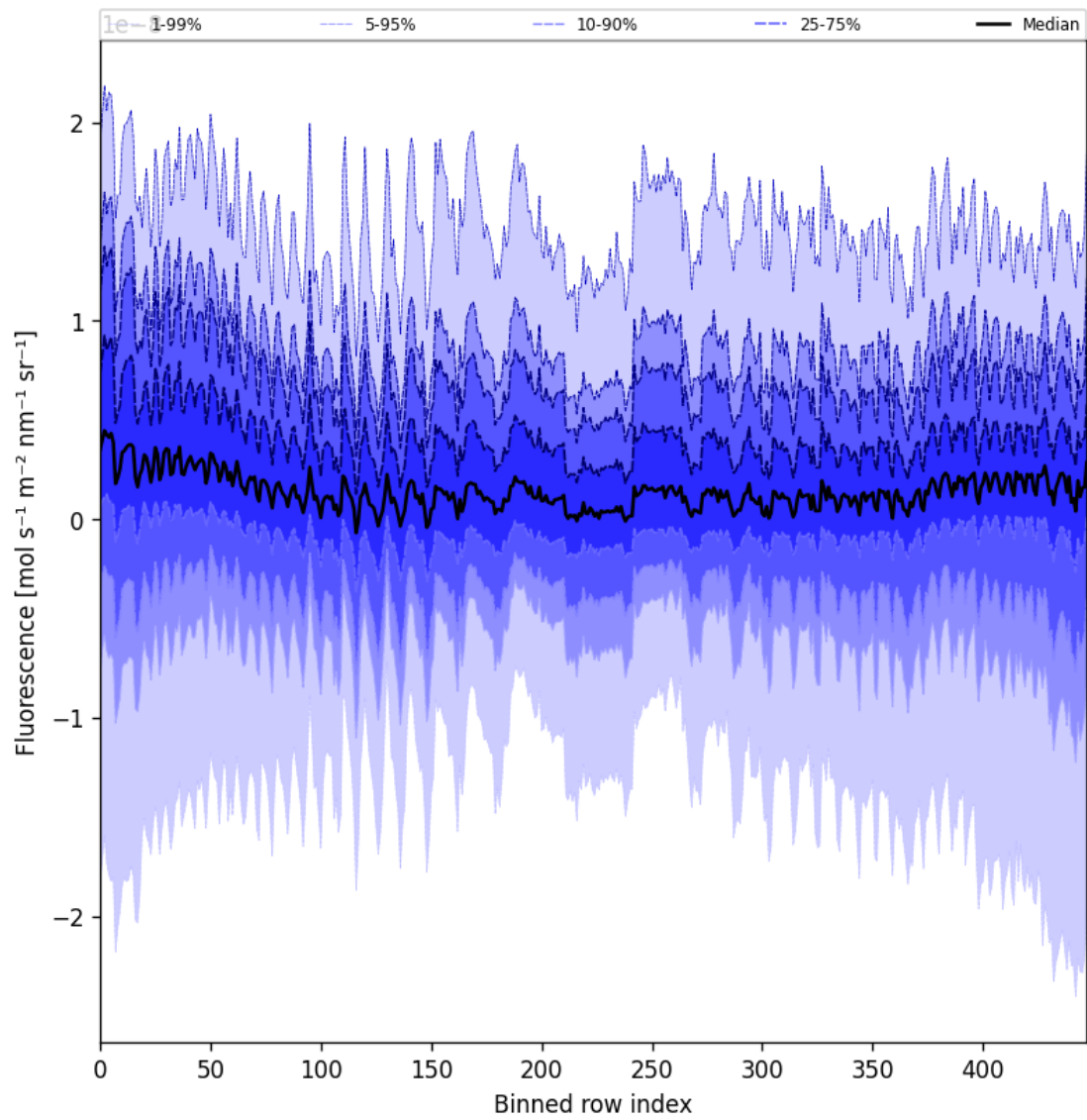
Figure 57: Along track statistics of “Fluorescence” for 2025-09-23 to 2025-09-25
