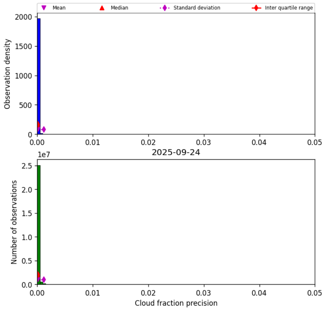
Figure 33: Histogram of “Cloud fraction precision” for 2025-09-23 to 2025-09-25
