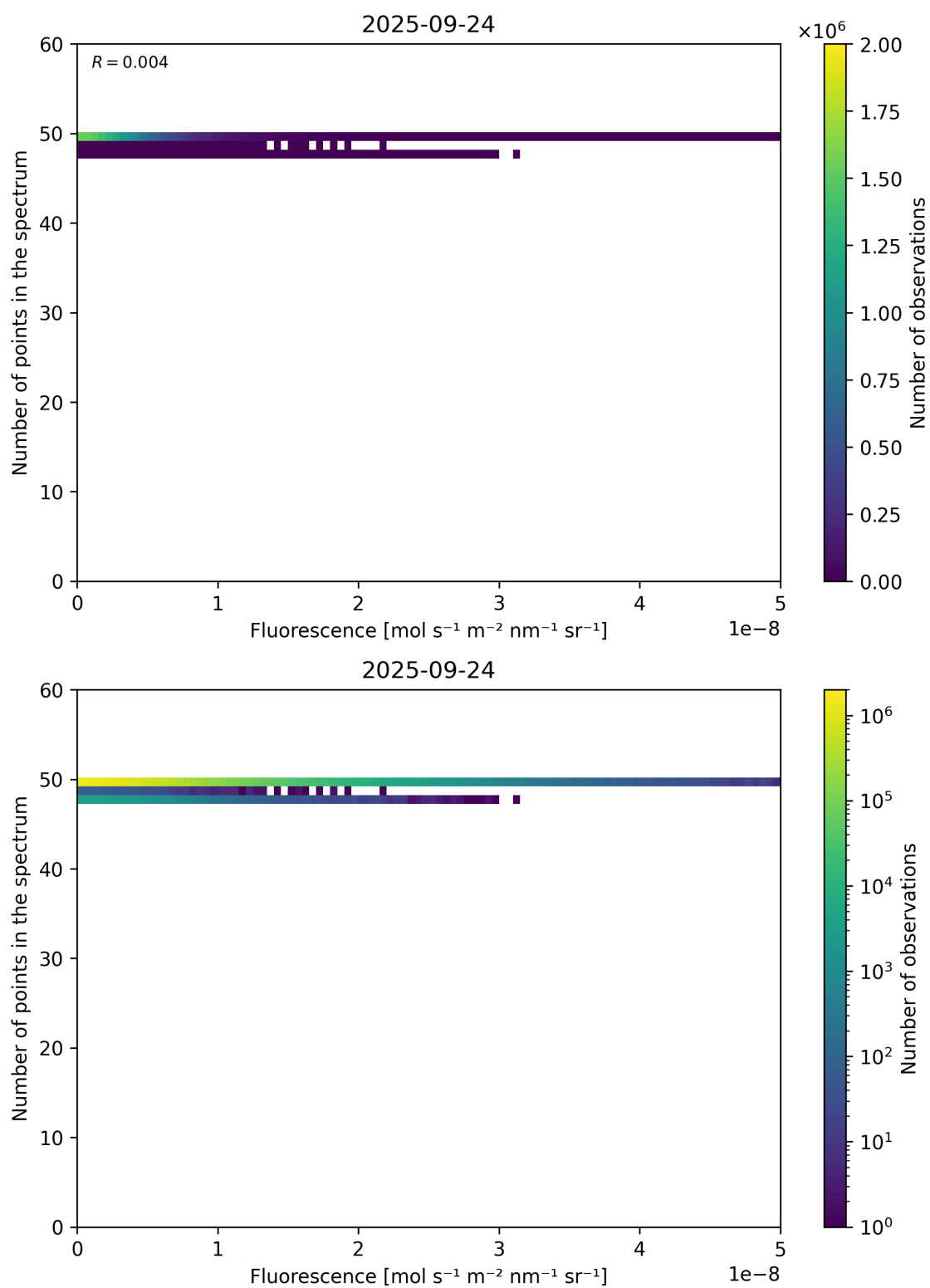
Figure 86: Scatter density plot of “Fluorescence” against “Number of points in the spectrum” for 2025-09-23 to 2025-09-25.
