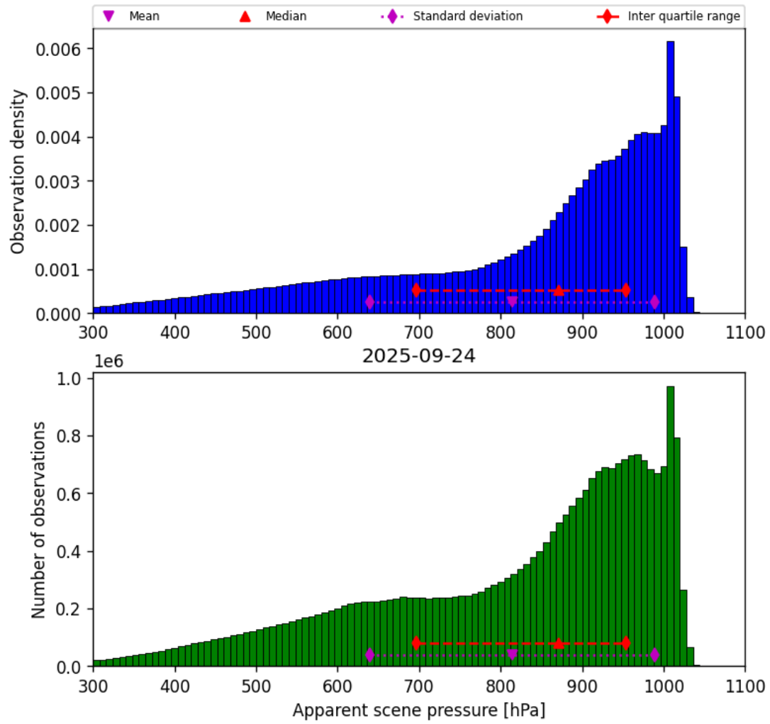
Figure 36: Histogram of “Apparent scene pressure” for 2025-09-23 to 2025-09-25
