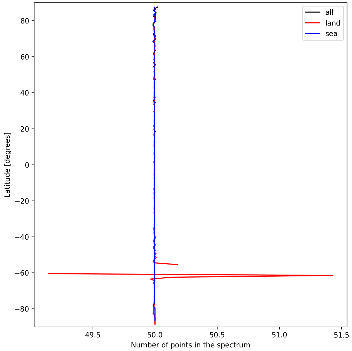
Figure 27: Zonal average of “Number of points in the spectrum” for 2025-09-23 to 2025-09-25.
