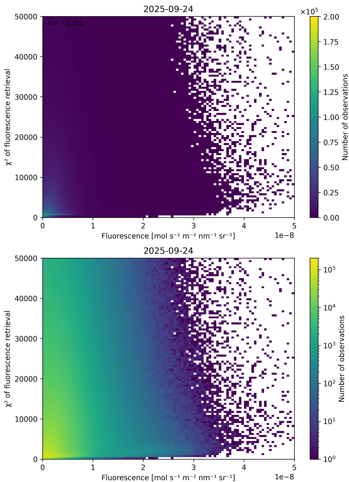
Figure 85: Scatter density plot of “Fluorescence” against “ \chi^2 of fluorescence retrieval” for 2025-09-23 to 2025-09-25.
