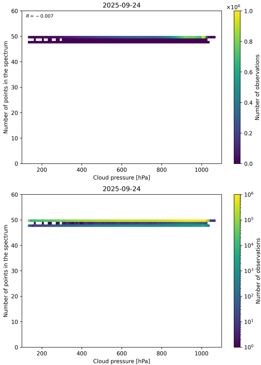
Figure 82: Scatter density plot of “Cloud pressure” against “Number of points in the spectrum” for 2025-09-23 to 2025-09-25.
