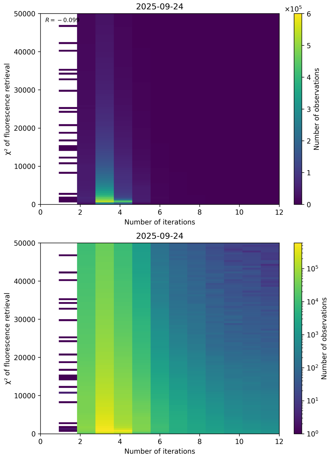
Figure 97: Scatter density plot of “Number of iterations” against “ \chi^2 of fluorescence retrieval” for 2025-09-23 to 2025-09-25.
