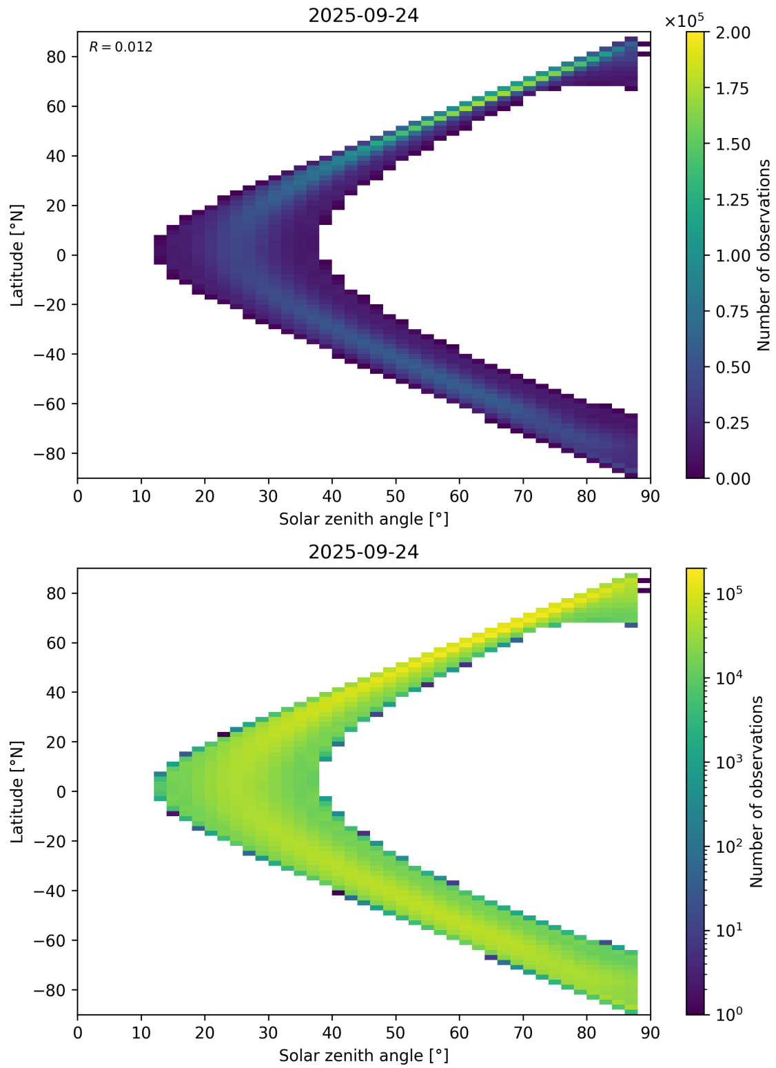
Figure 113: Scatter density plot of “Solar zenith angle” against “Latitude” for 2025-09-23 to 2025-09-25.
