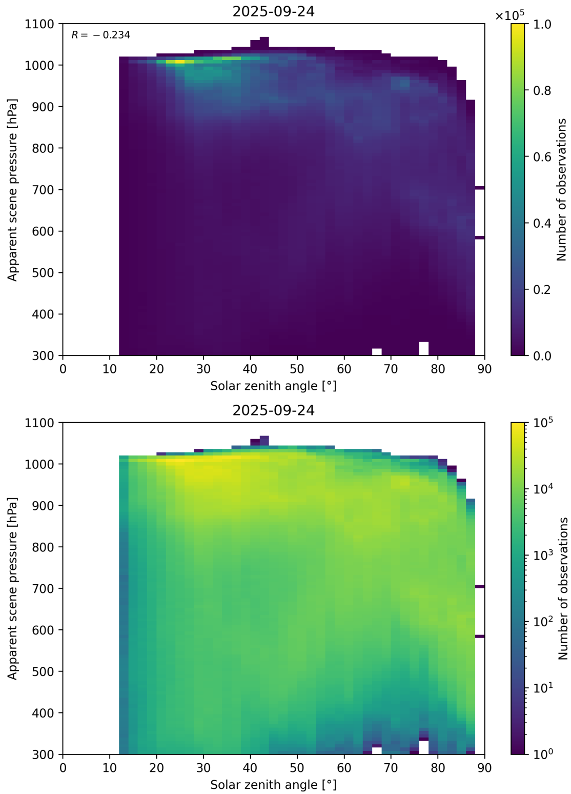
Figure 108: Scatter density plot of “Solar zenith angle” against “Apparent scene pressure” for 2025-09-23 to 2025-09-25.
