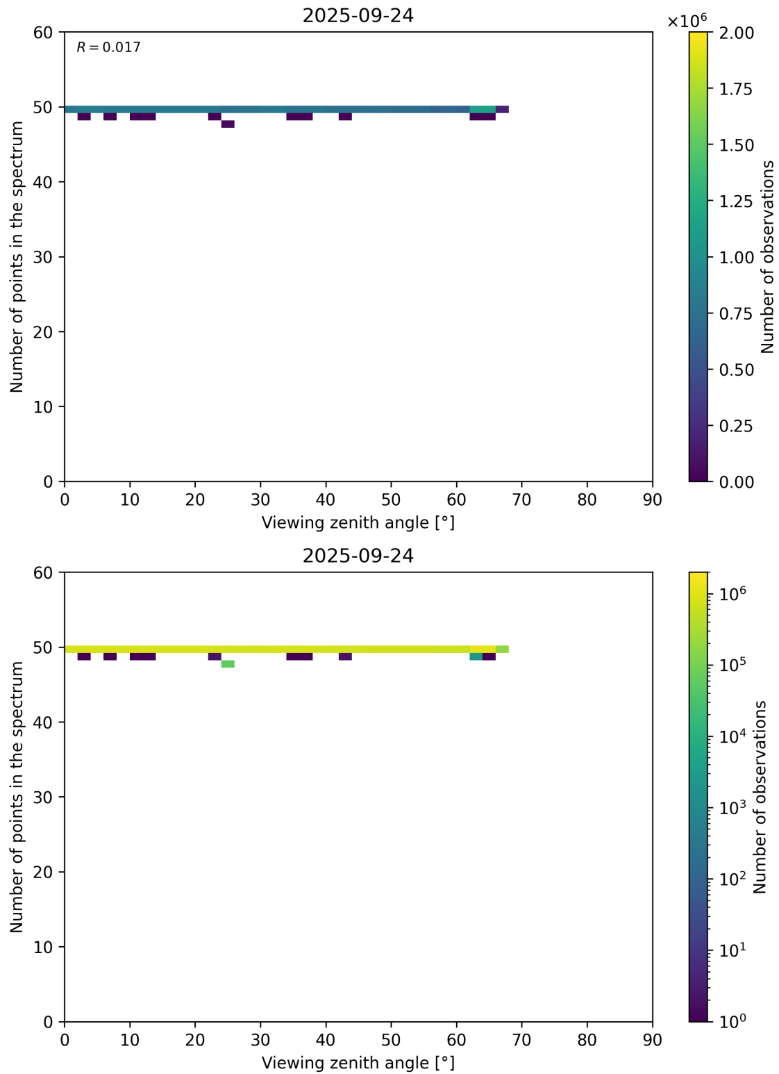
Figure 125: Scatter density plot of “Viewing zenith angle” against “Number of points in the spectrum” for 2025-09-23 to 2025-09-25.
