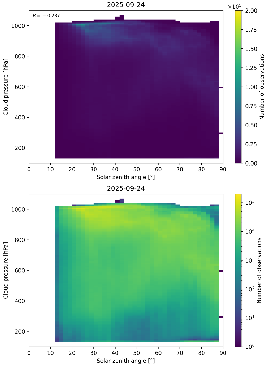
Figure 111: Scatter density plot of “Solar zenith angle” against “Cloud pressure” for 2025-09-23 to 2025-09-25.
