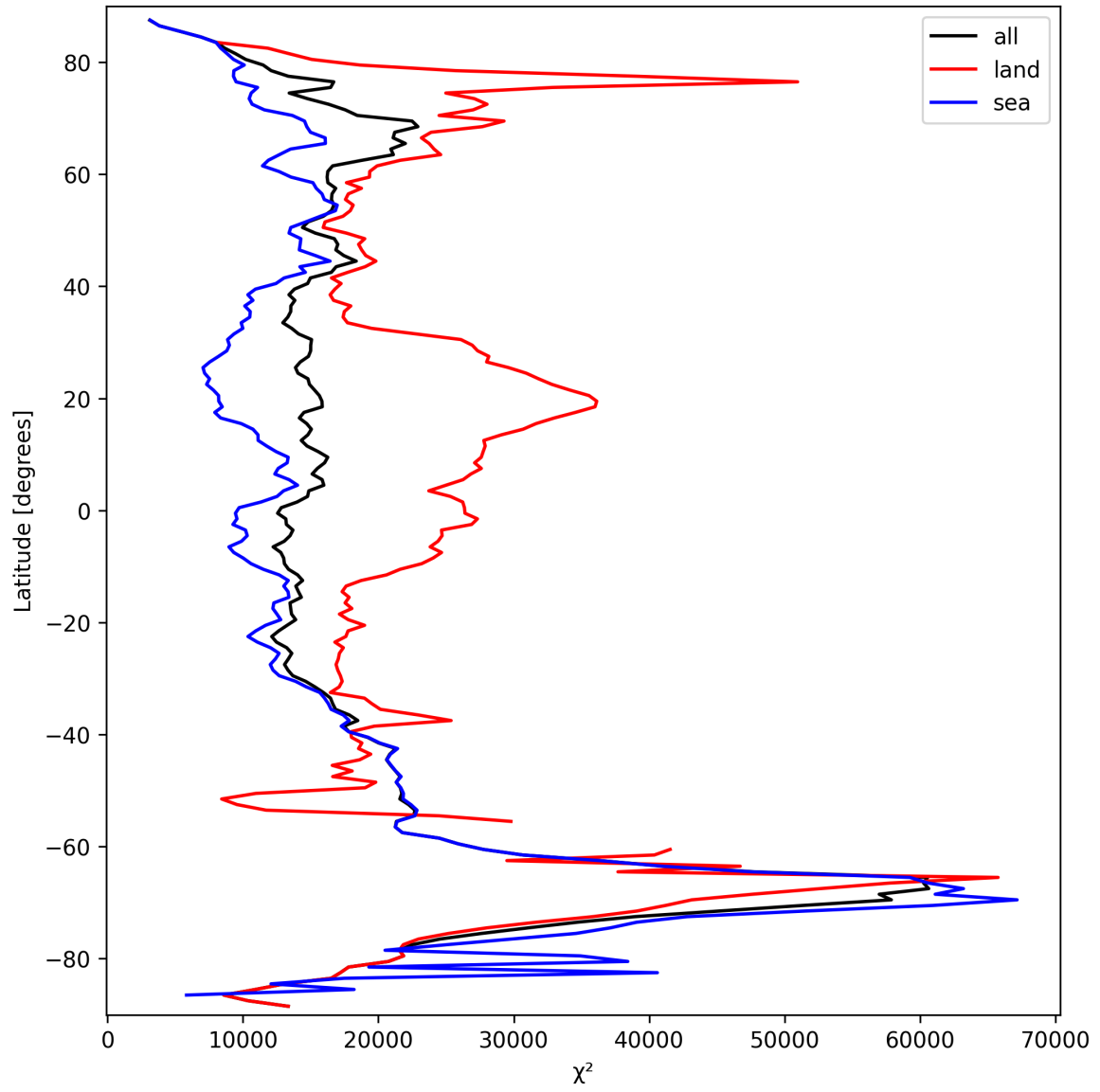
Figure 21: Zonal average of “ \chi^2 ” for 2025-09-23 to 2025-09-25.
