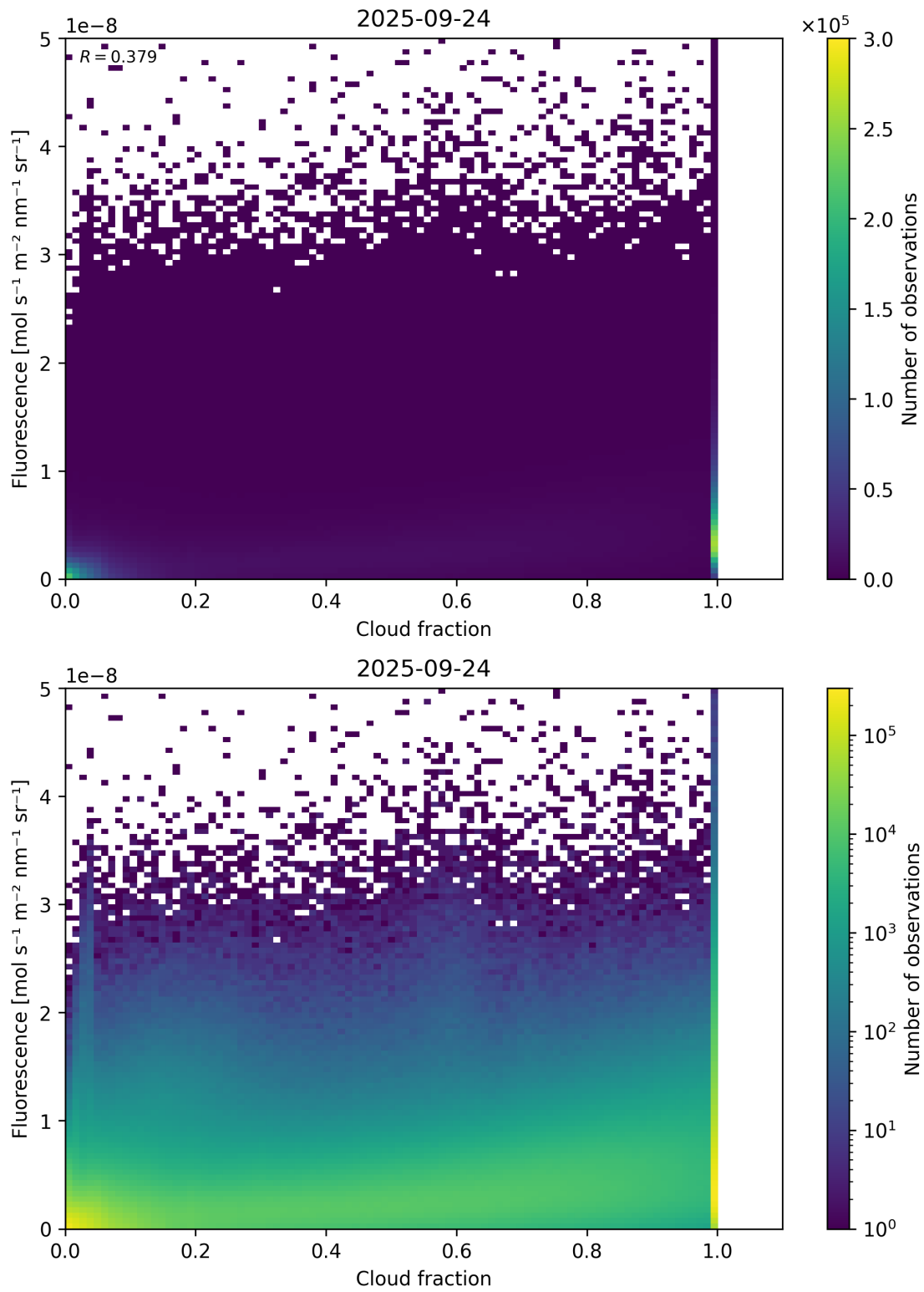
Figure 72: Scatter density plot of “Cloud fraction” against “Fluorescence” for 2025-09-23 to 2025-09-25.
