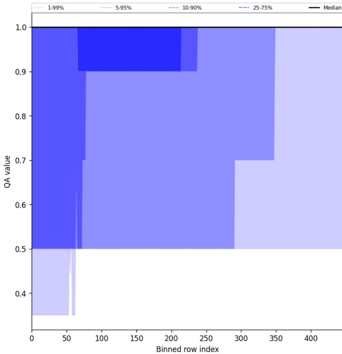
Figure 46: Along track statistics of “QA value” for 2025-09-23 to 2025-09-25
