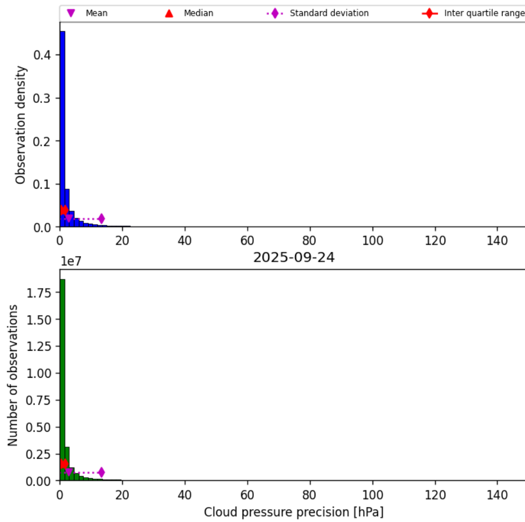
Figure 31: Histogram of “Cloud pressure precision” for 2025-09-23 to 2025-09-25
