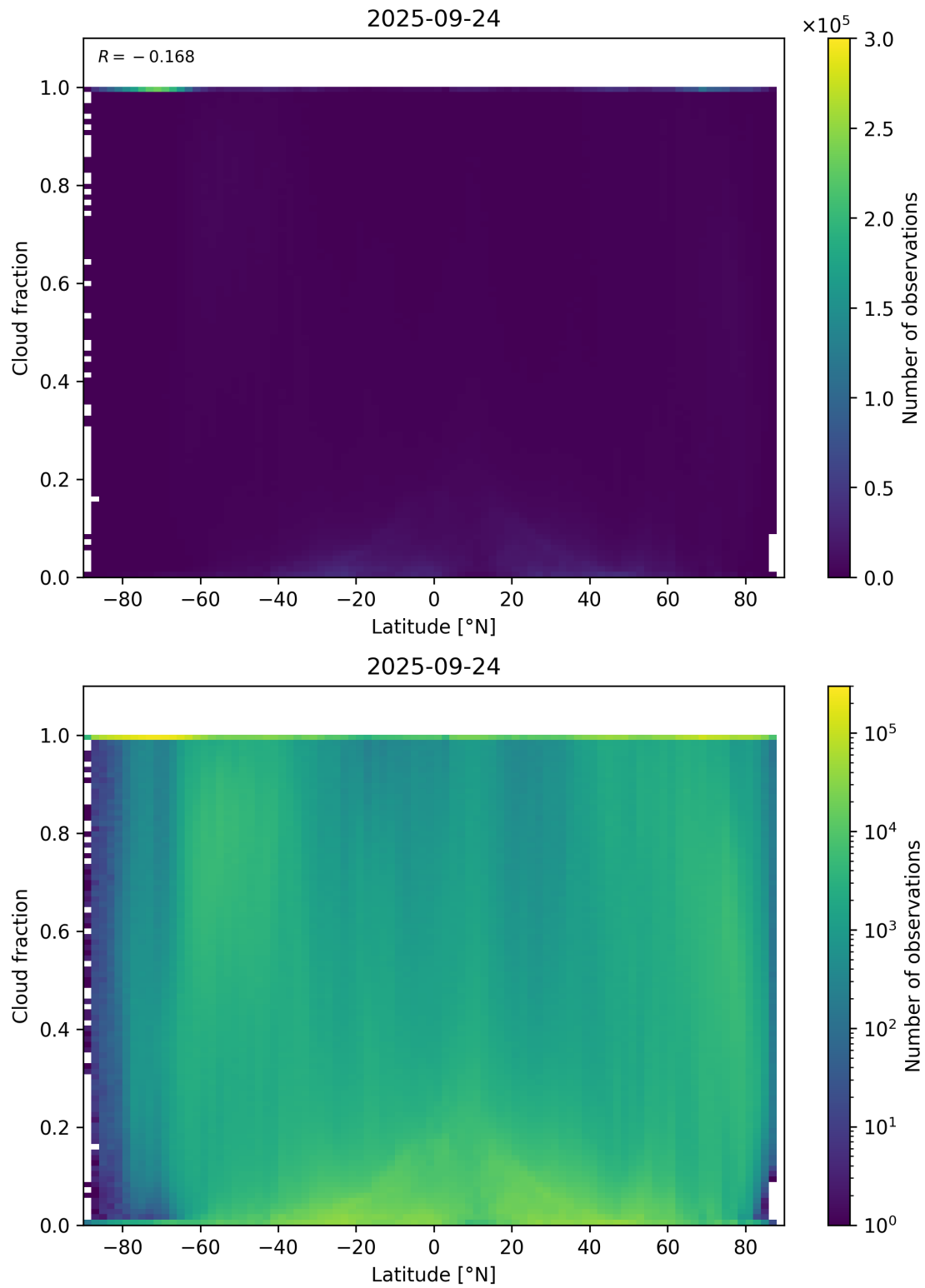
Figure 90: Scatter density plot of “Latitude” against “Cloud fraction” for 2025-09-23 to 2025-09-25.
