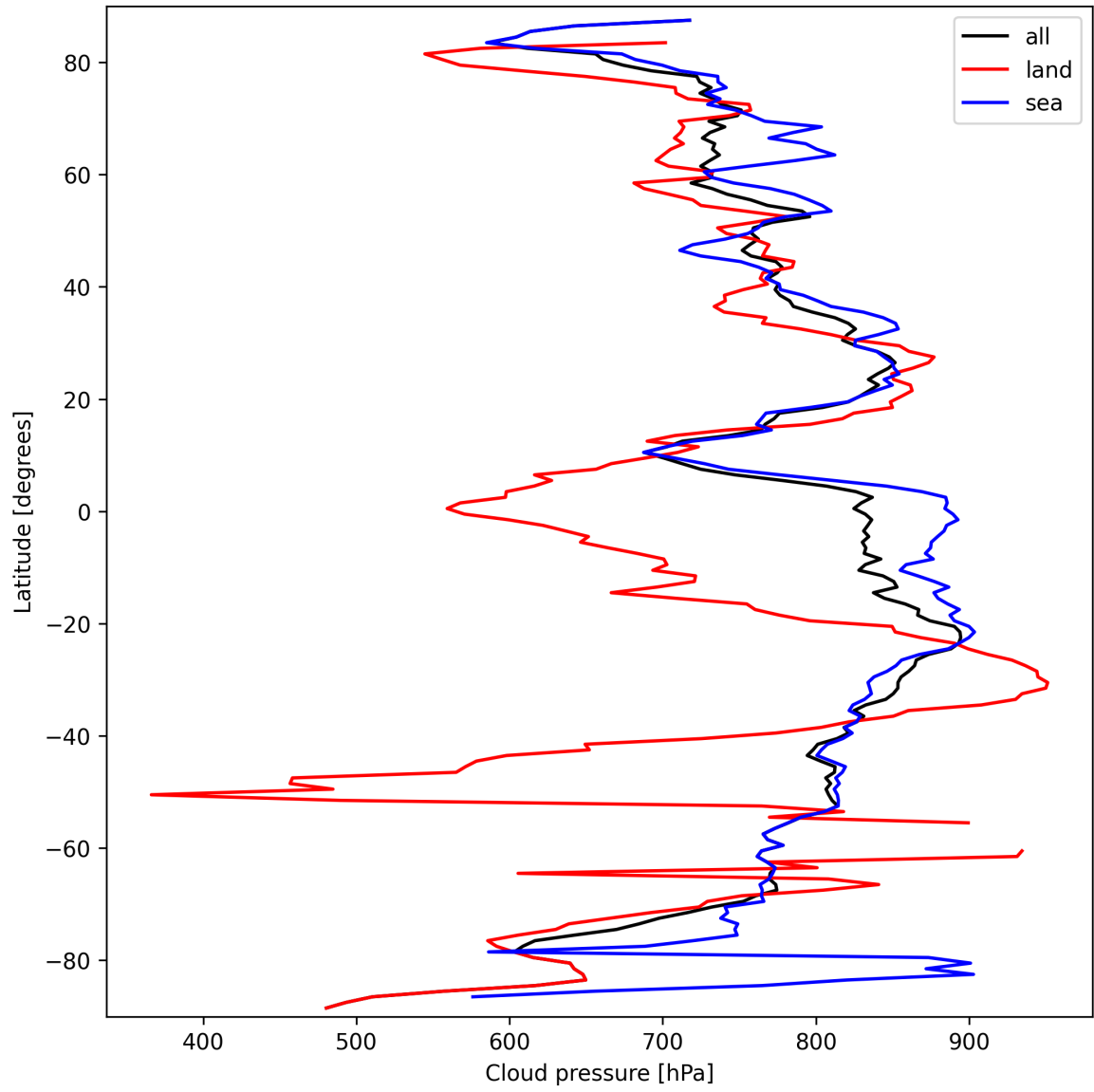
Figure 13: Zonal average of “Cloud pressure” for 2025-09-23 to 2025-09-25.
