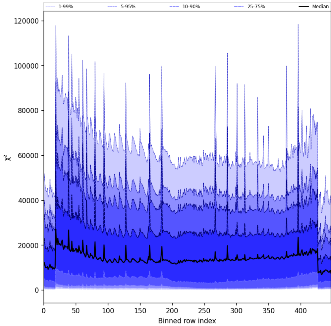
Figure 55: Along track statistics of “ \chi^2 ” for 2025-09-23 to 2025-09-25
