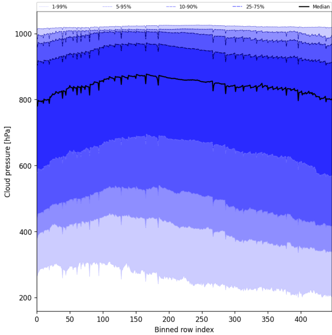
Figure 47: Along track statistics of “Cloud pressure” for 2025-09-23 to 2025-09-25
