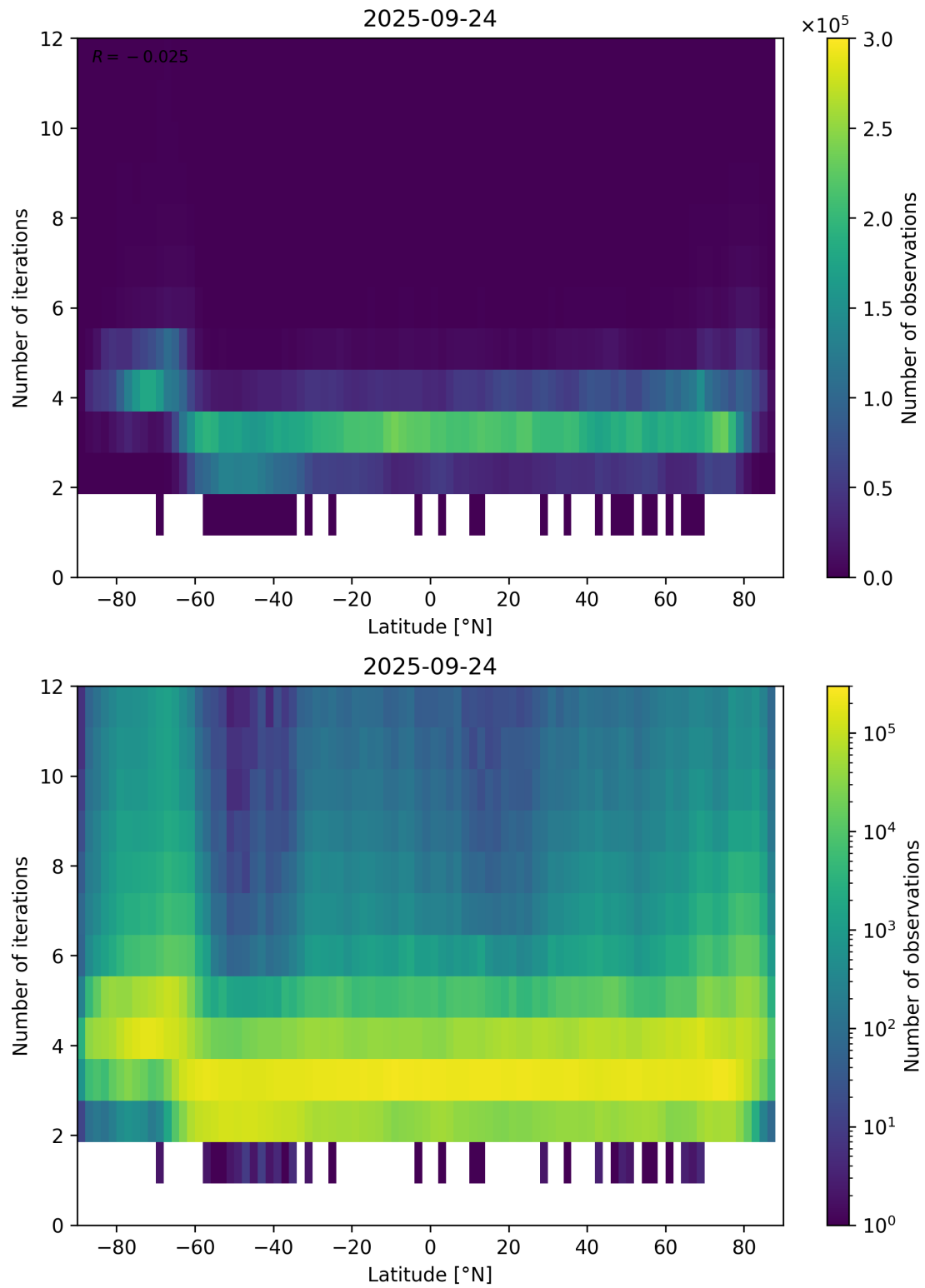
Figure 93: Scatter density plot of “Latitude” against “Number of iterations” for 2025-09-23 to 2025-09-25.
