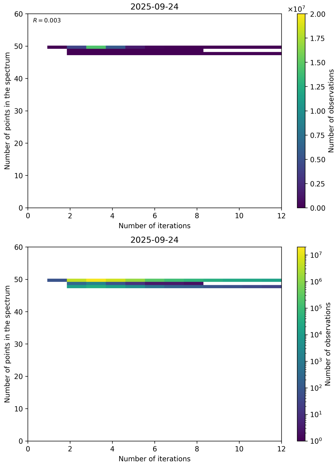
Figure 99: Scatter density plot of “Number of iterations” against “Number of points in the spectrum” for 2025-09-23 to 2025-09-25.
