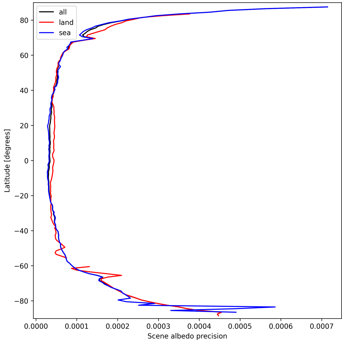
Figure 18: Zonal average of “Scene albedo precision” for 2025-09-23 to 2025-09-25.
