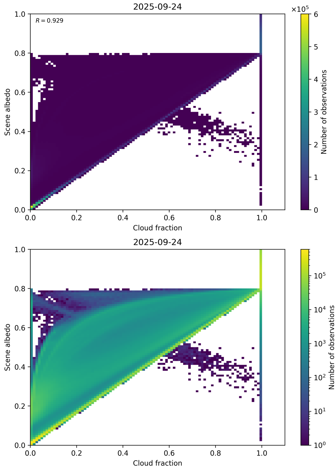
Figure 75: Scatter density plot of “Cloud fraction” against “Scene albedo” for 2025-09-23 to 2025-09-25.
