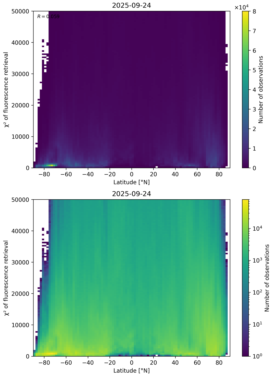
Figure 89: Scatter density plot of “Latitude” against “ \chi^2 of fluorescence retrieval” for 2025-09-23 to 2025-09-25.
