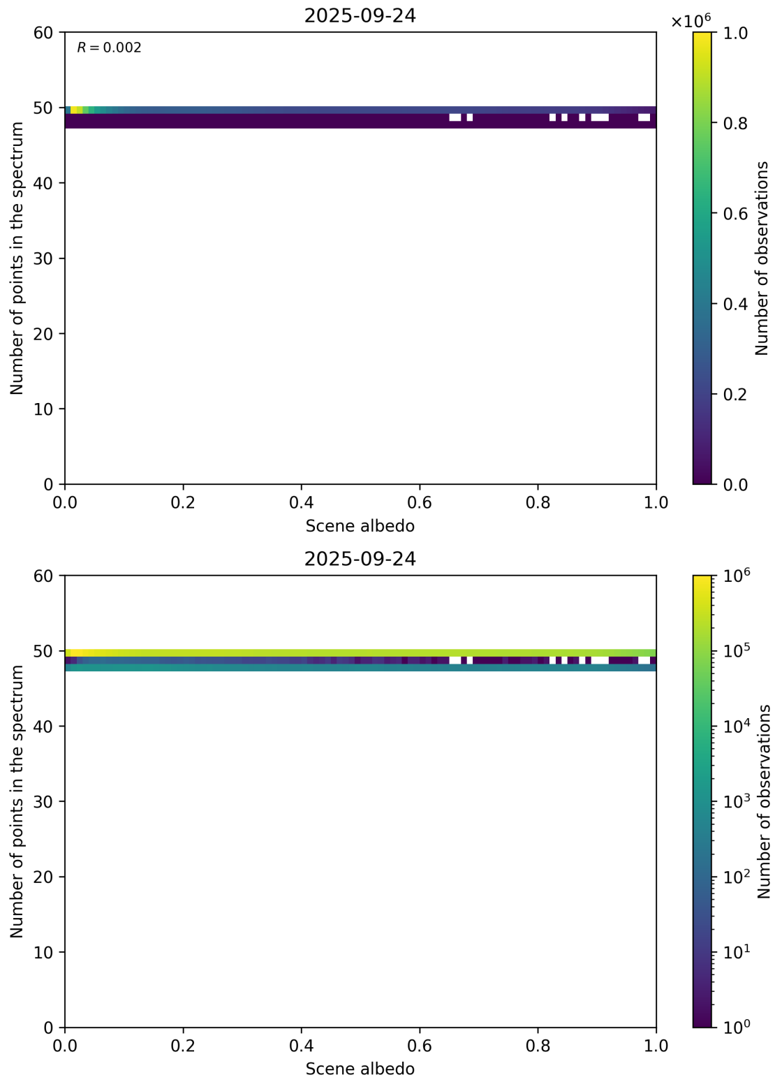
Figure 106: Scatter density plot of “Scene albedo” against “Number of points in the spectrum” for 2025-09-23 to 2025-09-25.
