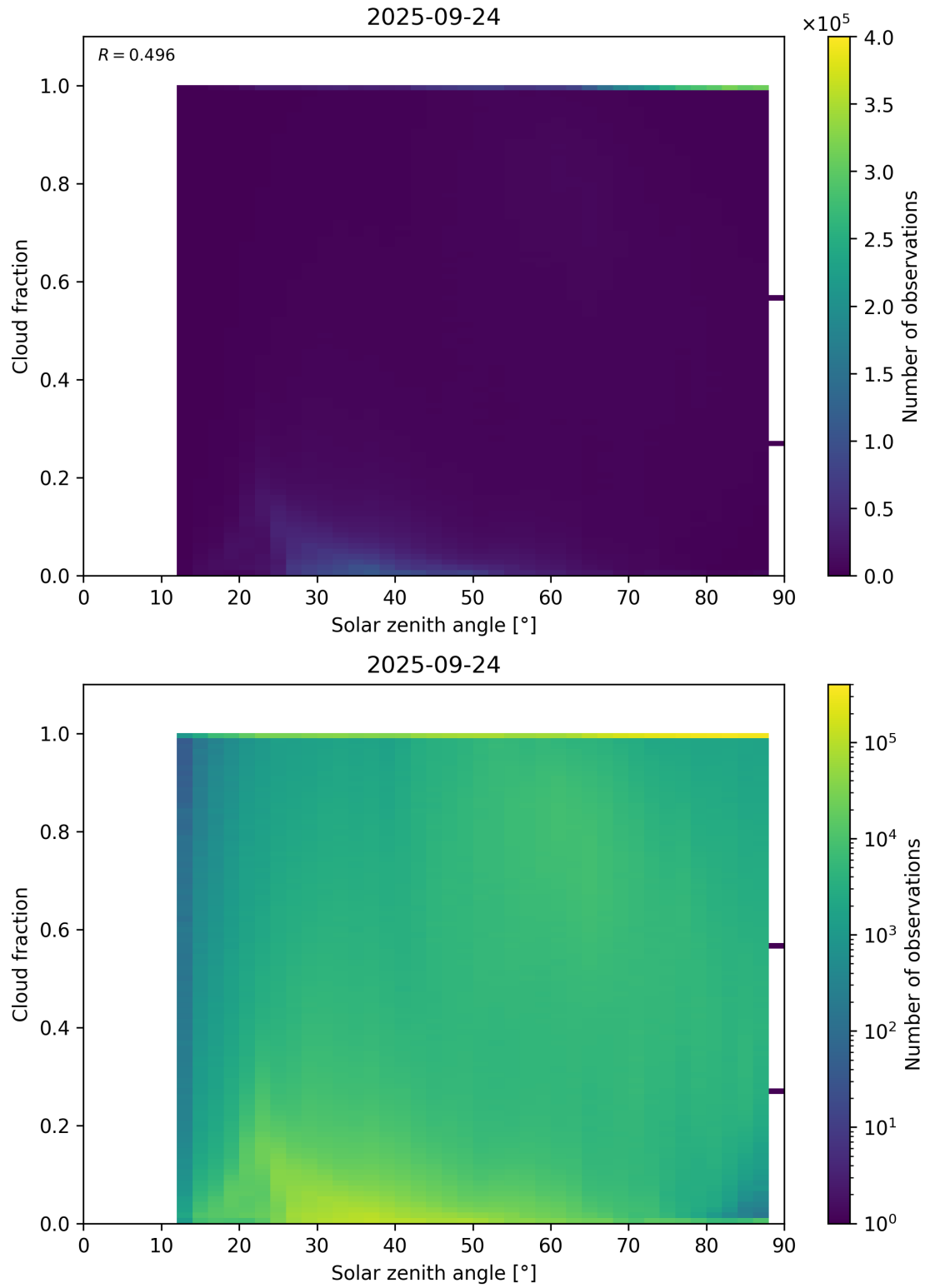
Figure 110: Scatter density plot of “Solar zenith angle” against “Cloud fraction” for 2025-09-23 to 2025-09-25.
