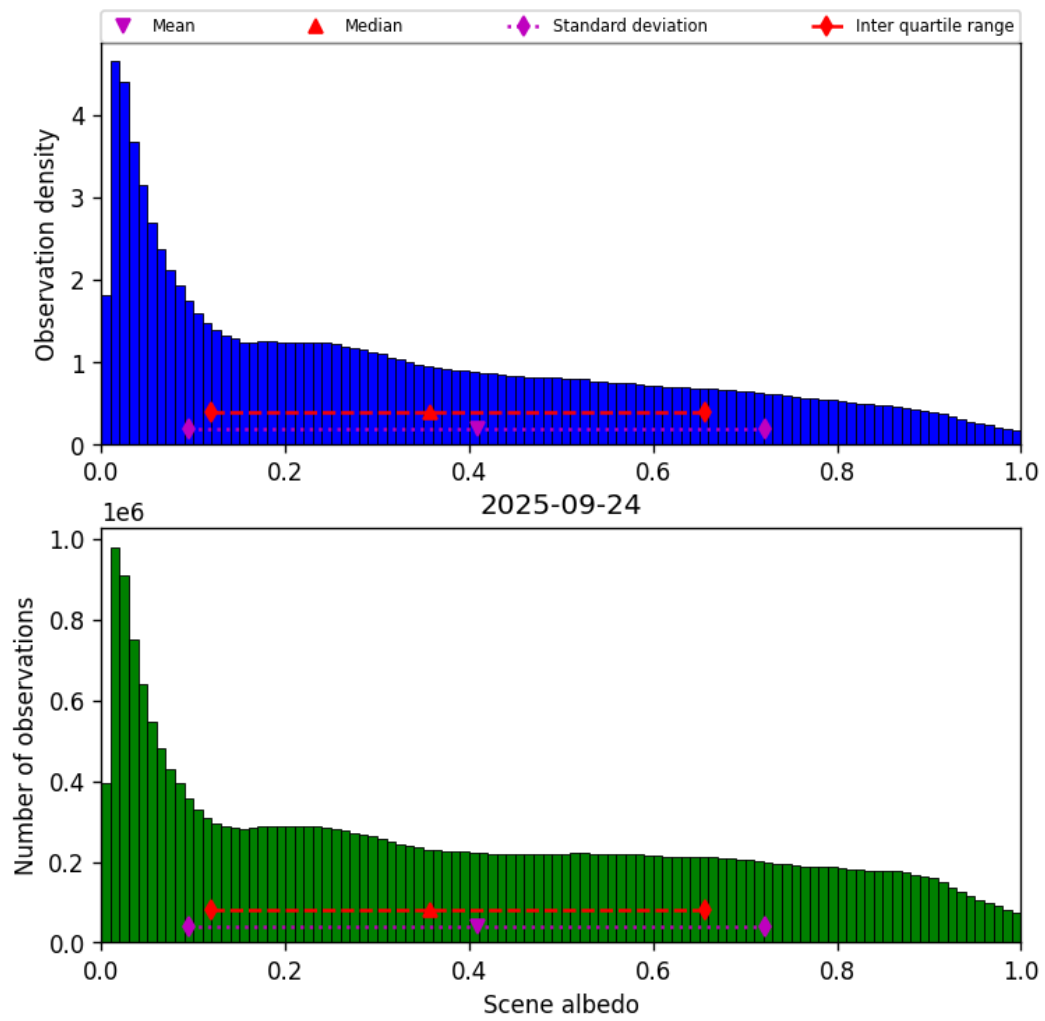
Figure 34: Histogram of “Scene albedo” for 2025-09-23 to 2025-09-25
