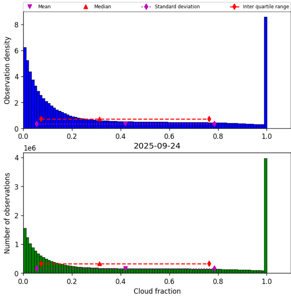
Figure 32: Histogram of “Cloud fraction” for 2025-09-23 to 2025-09-25
