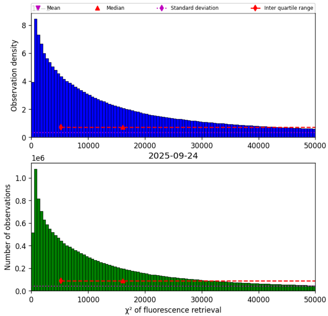
Figure 42: Histogram of “ \chi^2 of fluorescence retrieval” for 2025-09-23 to 2025-09-25
