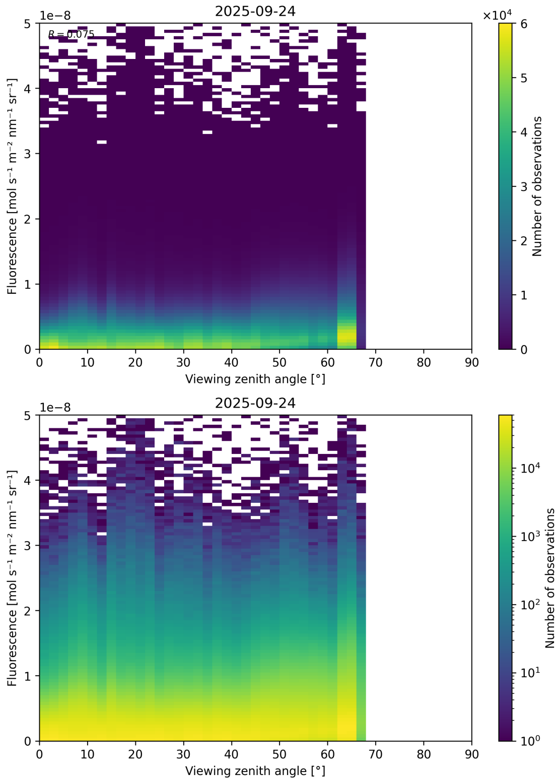
Figure 122: Scatter density plot of “Viewing zenith angle” against “Fluorescence” for 2025-09-23 to 2025-09-25.
