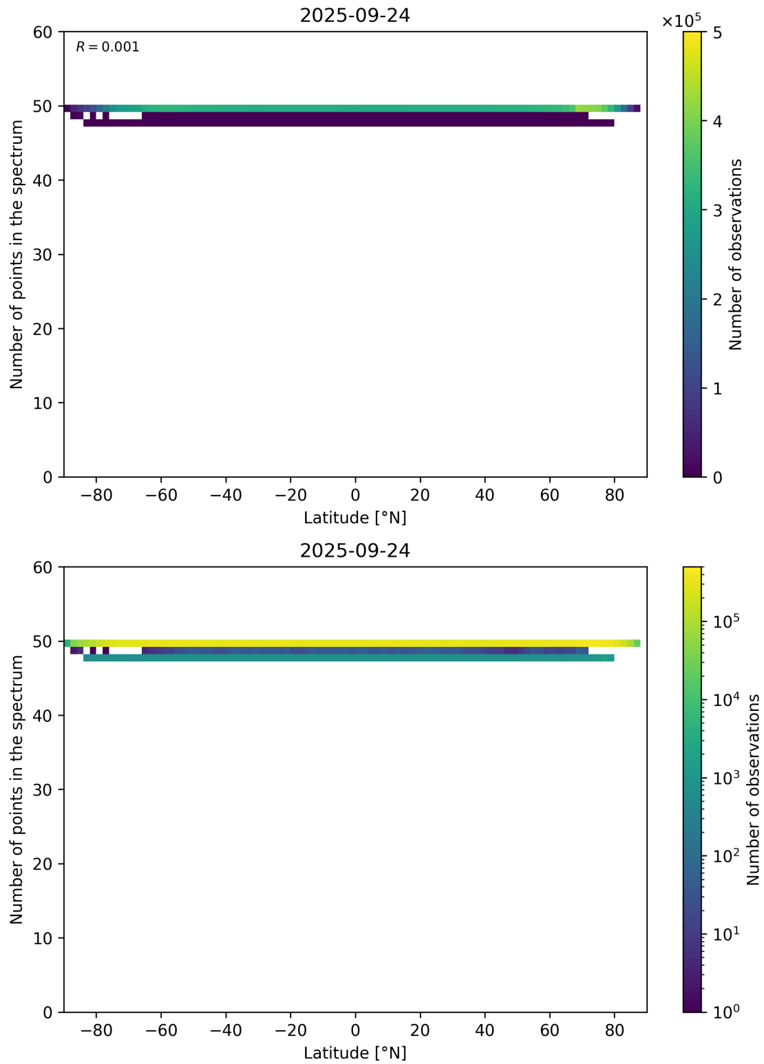
Figure 94: Scatter density plot of “Latitude” against “Number of points in the spectrum” for 2025-09-23 to 2025-09-25.
