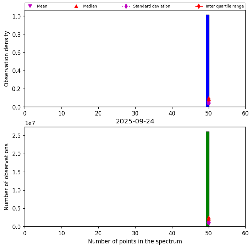
Figure 44: Histogram of “Number of points in the spectrum” for 2025-09-23 to 2025-09-25
