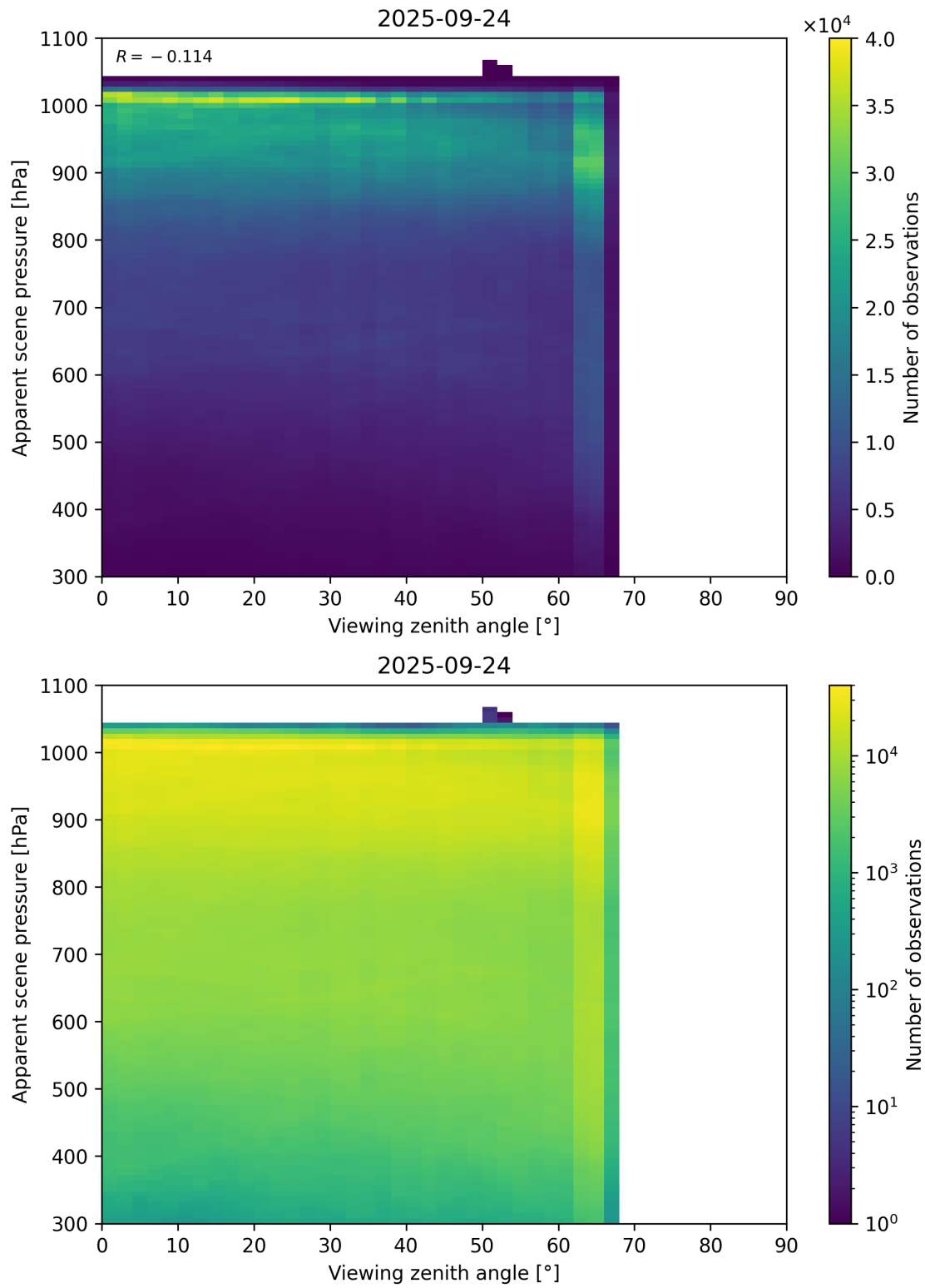
Figure 118: Scatter density plot of “Viewing zenith angle” against “Apparent scene pressure” for 2025-09-23 to 2025-09-25.
