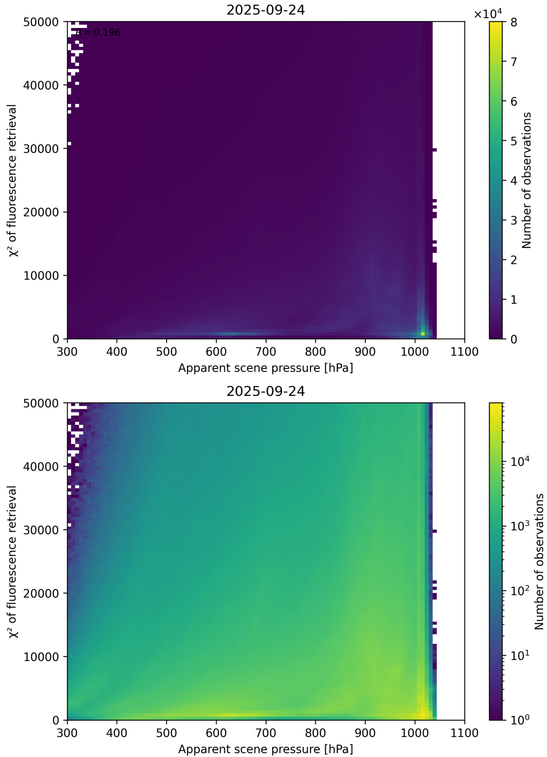
Figure 63: Scatter density plot of “Apparent scene pressure” against “ \chi^2 of fluorescence retrieval” for 2025-09-23 to 2025-09-25.
