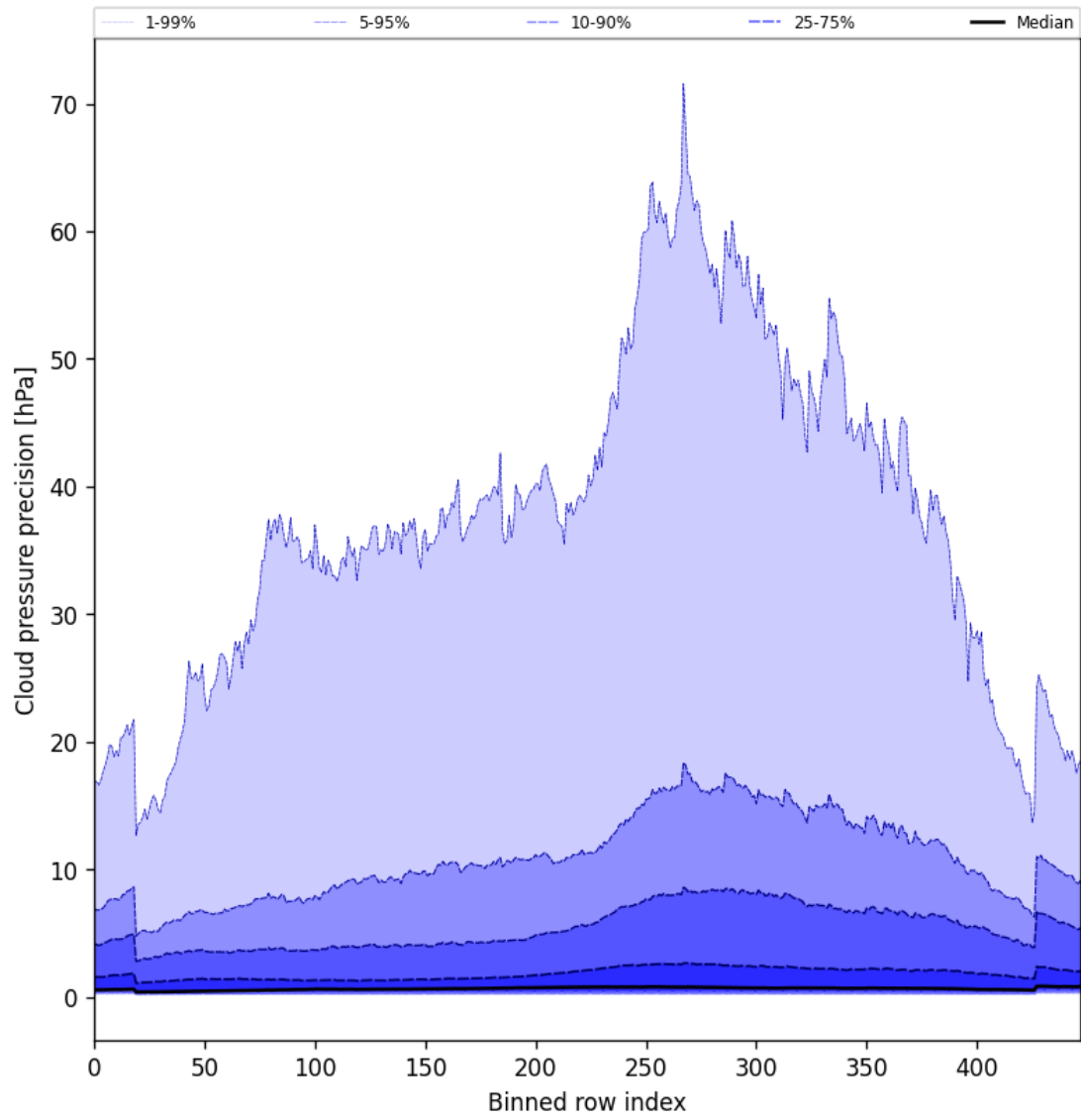
Figure 48: Along track statistics of “Cloud pressure precision” for 2025-09-23 to 2025-09-25
