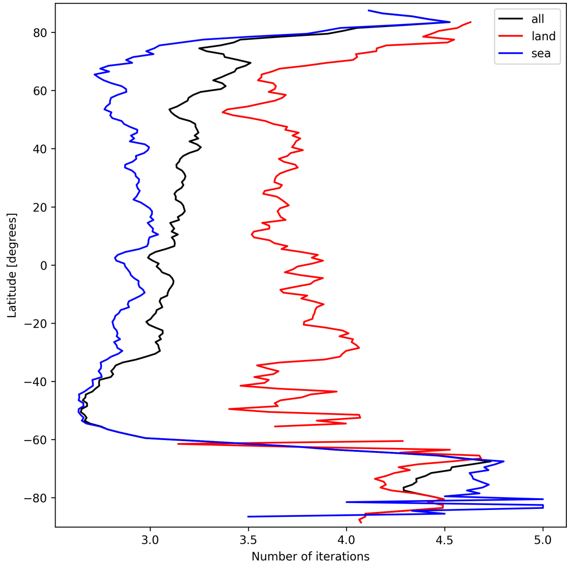
Figure 22: Zonal average of “Number of iterations” for 2025-09-23 to 2025-09-25.
