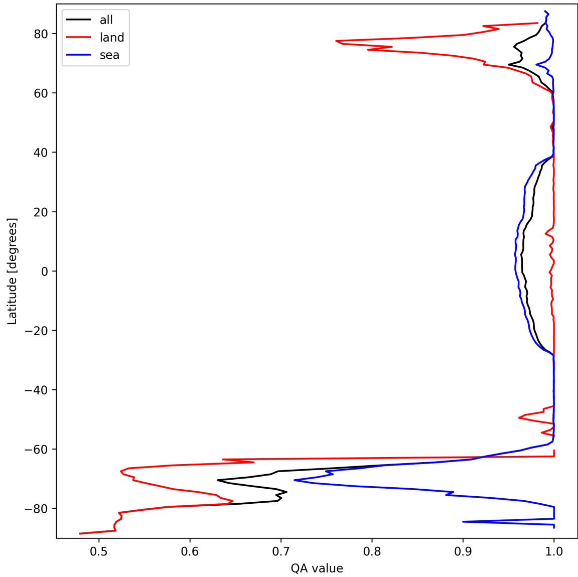
Figure 12: Zonal average of “QA value” for 2025-09-23 to 2025-09-25.
