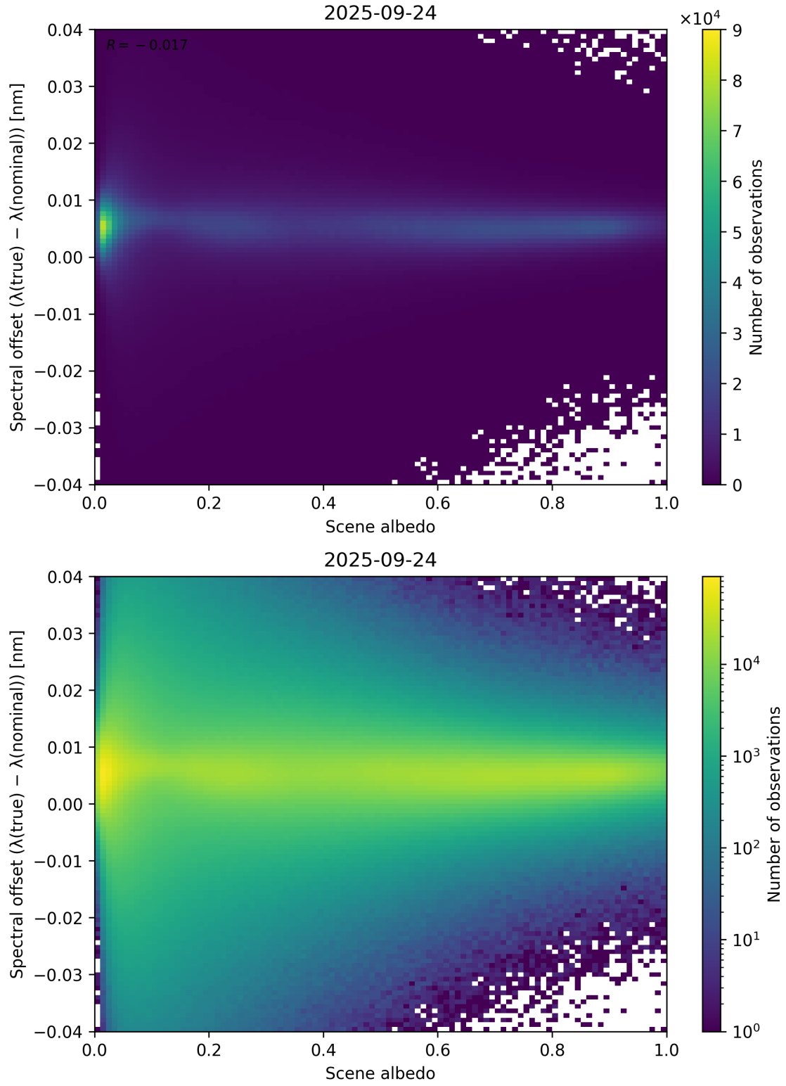
Figure 107: Scatter density plot of “Scene albedo” against “Spectral offset ( \lambda_{\text{true}} - \lambda_{\text{nominal}} )” for 2025-09-23 to 2025-09-25.
