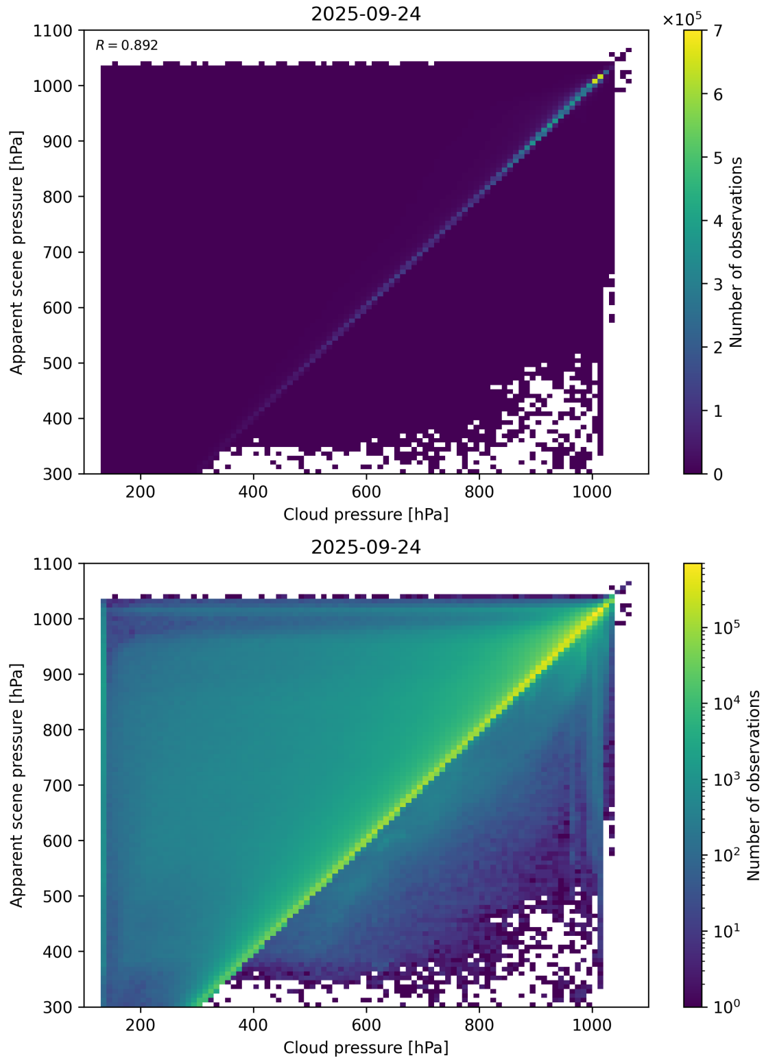
Figure 77: Scatter density plot of “Cloud pressure” against “Apparent scene pressure” for 2025-09-23 to 2025-09-25.
