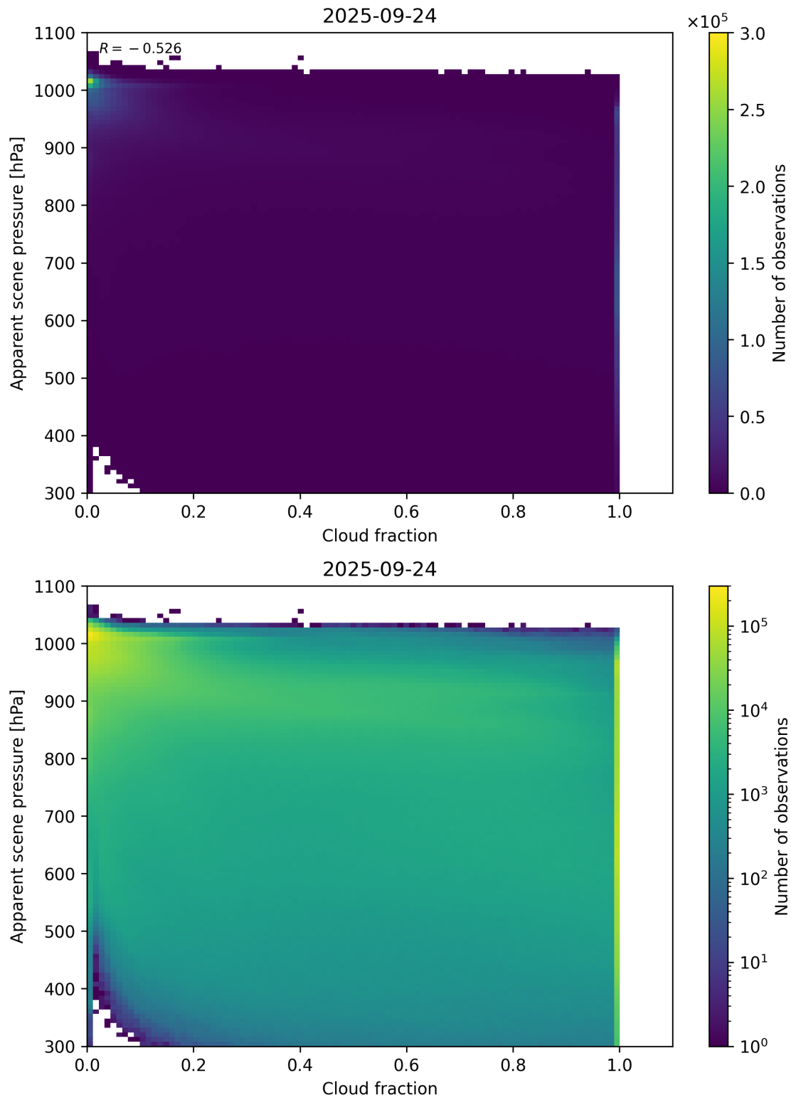
Figure 70: Scatter density plot of “Cloud fraction” against “Apparent scene pressure” for 2025-09-23 to 2025-09-25.
