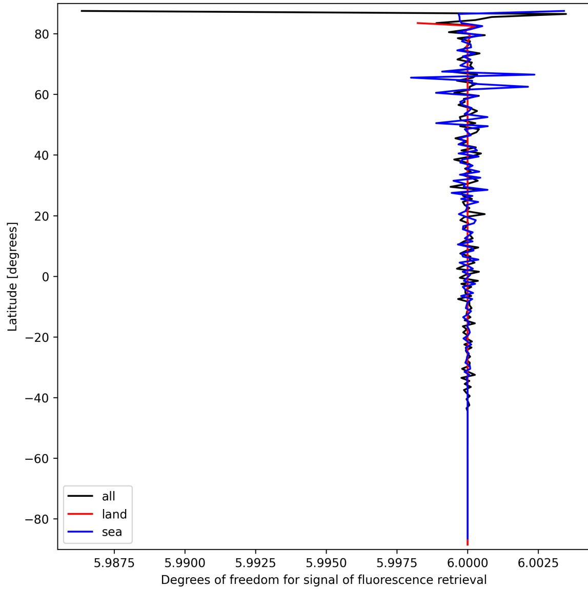
Figure 26: Zonal average of “Degrees of freedom for signal of fluorescence retrieval” for 2025-09-23 to 2025-09-25.
