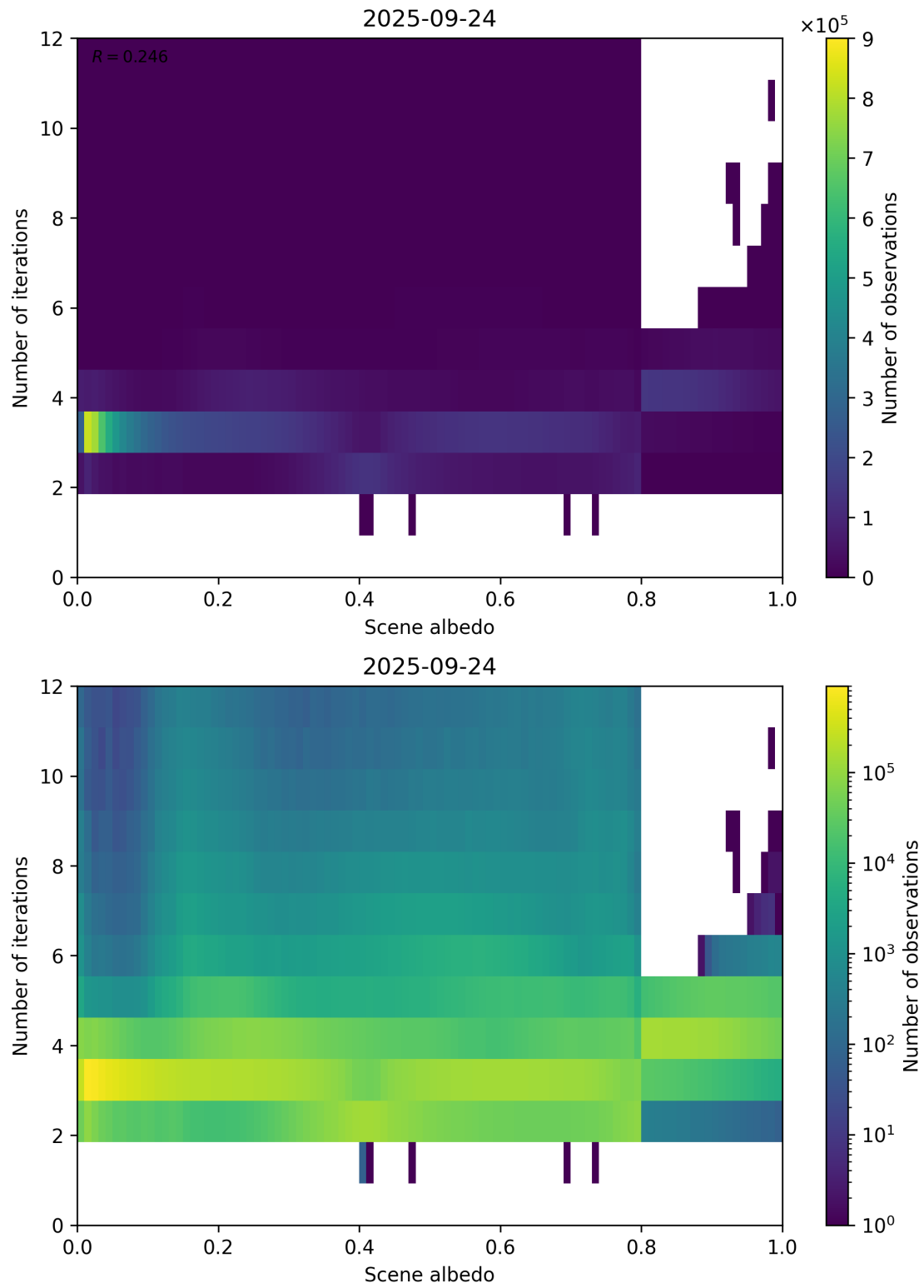
Figure 105: Scatter density plot of “Scene albedo” against “Number of iterations” for 2025-09-23 to 2025-09-25.
