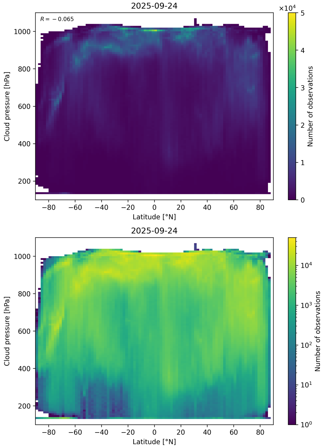
Figure 91: Scatter density plot of “Latitude” against “Cloud pressure” for 2025-09-23 to 2025-09-25.
