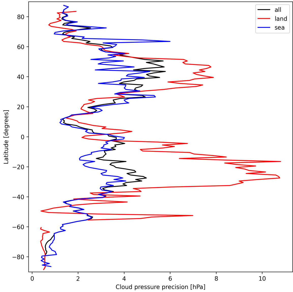
Figure 14: Zonal average of “Cloud pressure precision” for 2025-09-23 to 2025-09-25.
