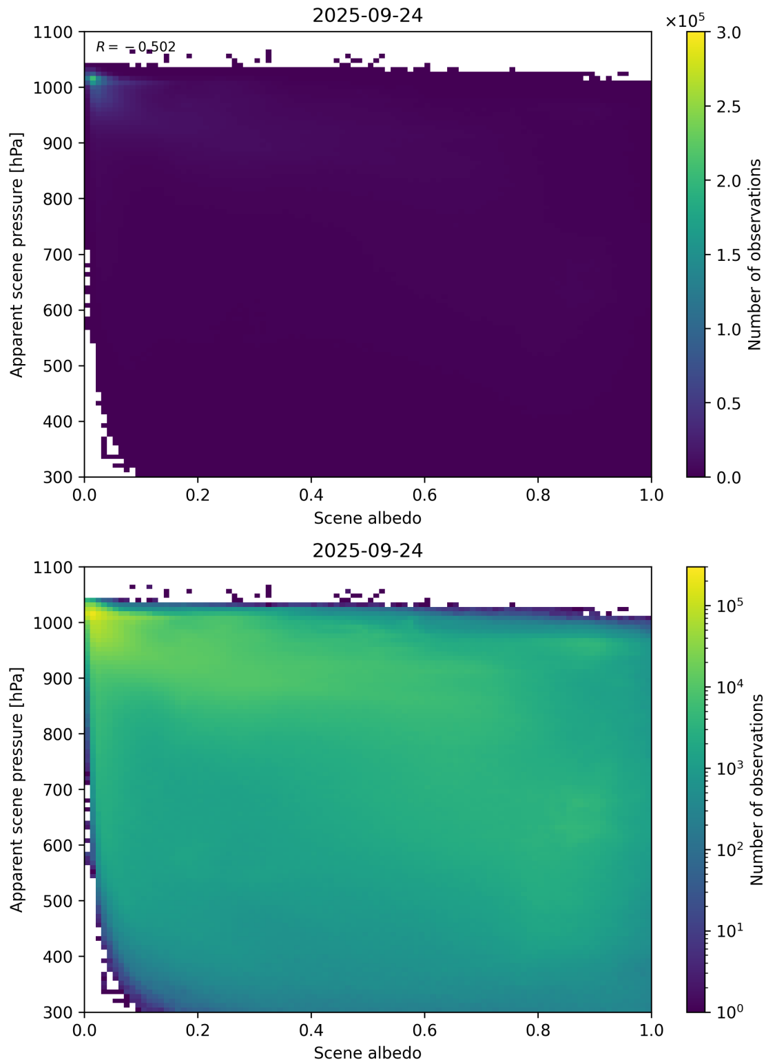
Figure 102: Scatter density plot of “Scene albedo” against “Apparent scene pressure” for 2025-09-23 to 2025-09-25.
