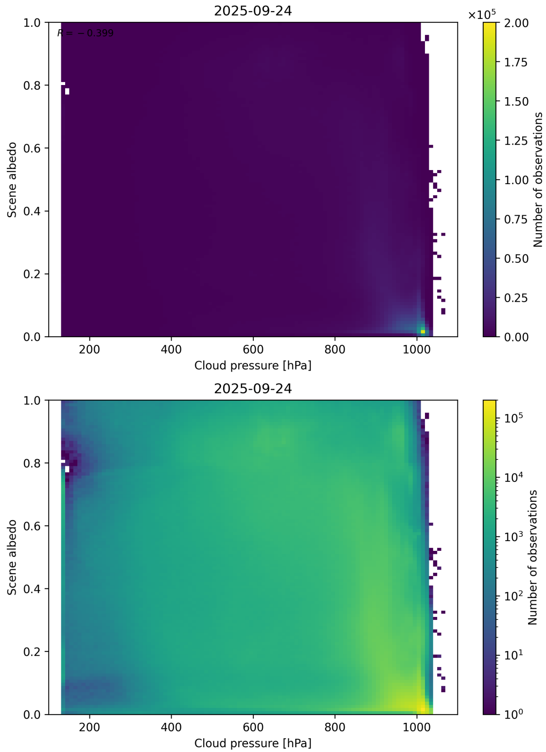
Figure 83: Scatter density plot of “Cloud pressure” against “Scene albedo” for 2025-09-23 to 2025-09-25.
