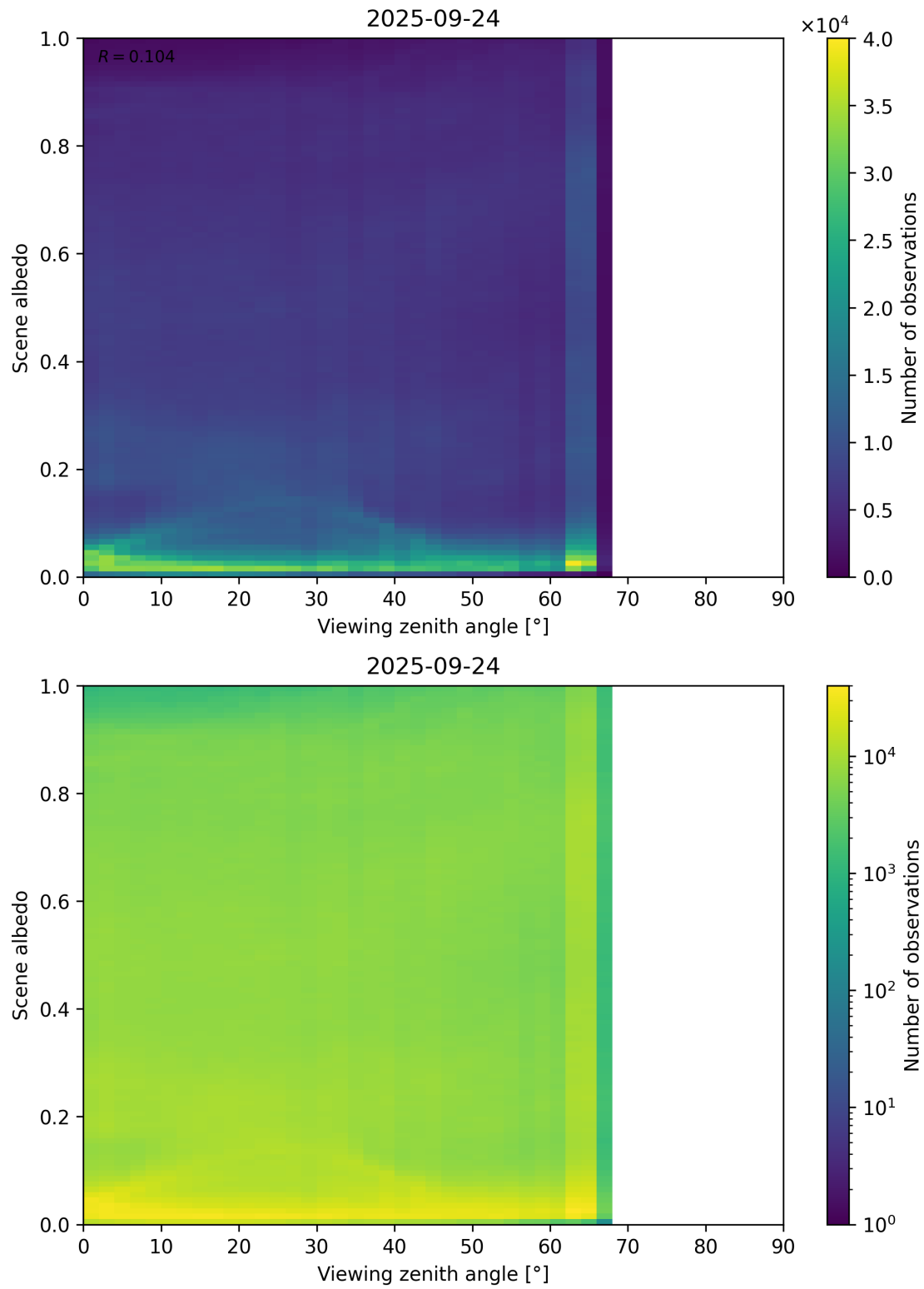
Figure 126: Scatter density plot of “Viewing zenith angle” against “Scene albedo” for 2025-09-23 to 2025-09-25.
