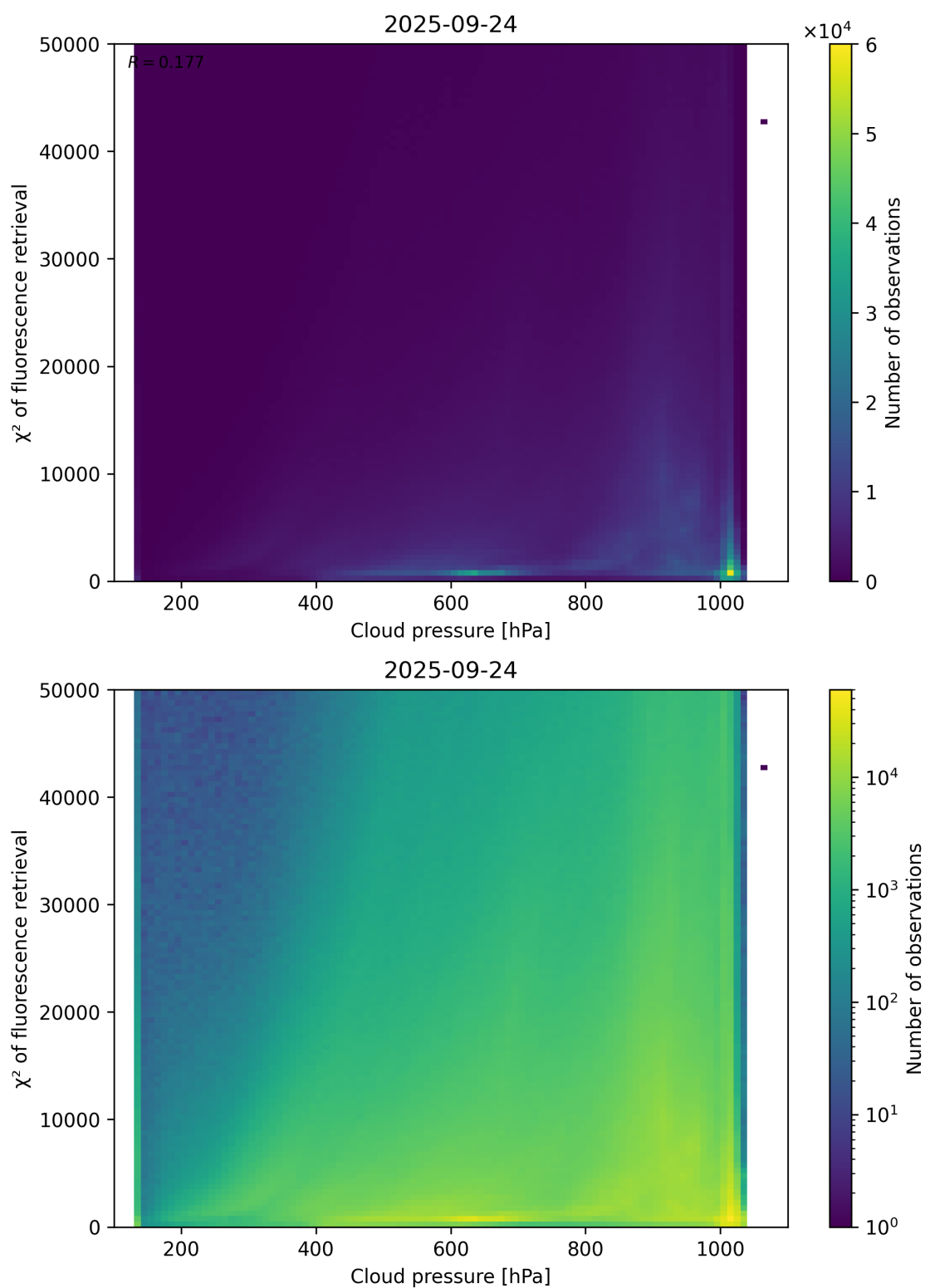
Figure 78: Scatter density plot of “Cloud pressure” against “ \chi^2 of fluorescence retrieval” for 2025-09-23 to 2025-09-25.
