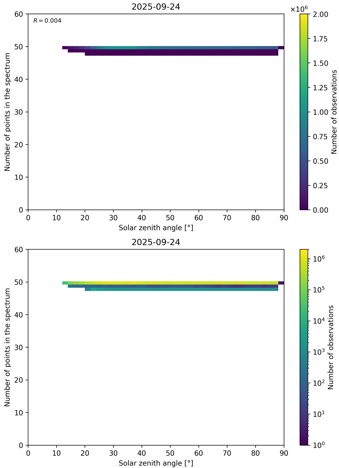
Figure 115: Scatter density plot of “Solar zenith angle” against “Number of points in the spectrum” for 2025-09-23 to 2025-09-25.
