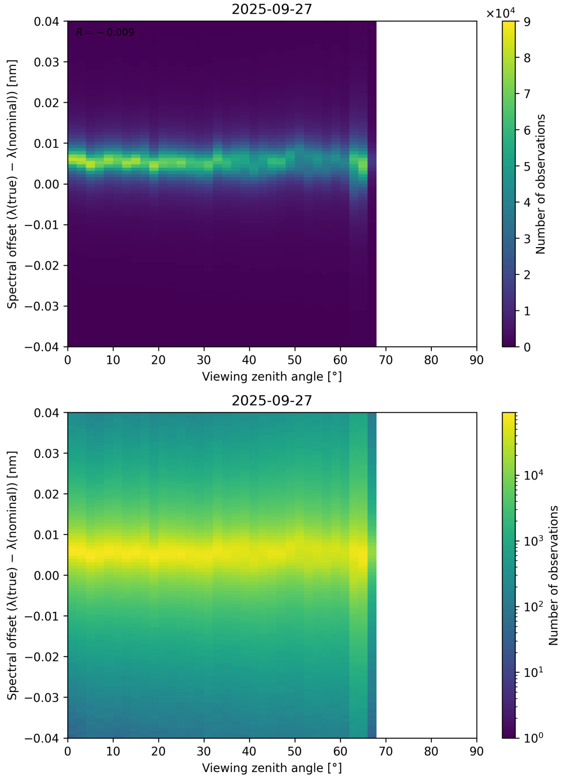
Figure 128: Scatter density plot of “Viewing zenith angle” against “Spectral offset ( \lambda_{\text{true}} - \lambda_{\text{nominal}} )” for 2025-09-26 to 2025-09-28.
