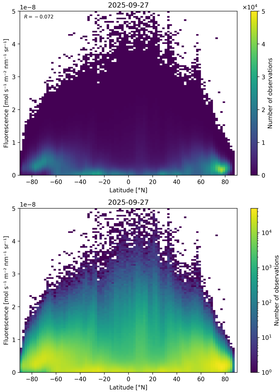
Figure 92: Scatter density plot of “Latitude” against “Fluorescence” for 2025-09-26 to 2025-09-28.
