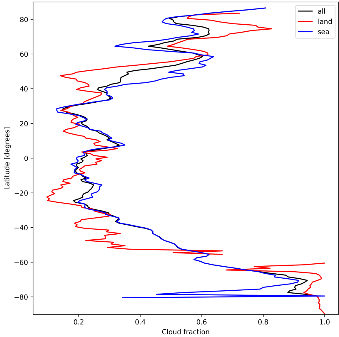
Figure 15: Zonal average of “Cloud fraction” for 2025-09-26 to 2025-09-28.
