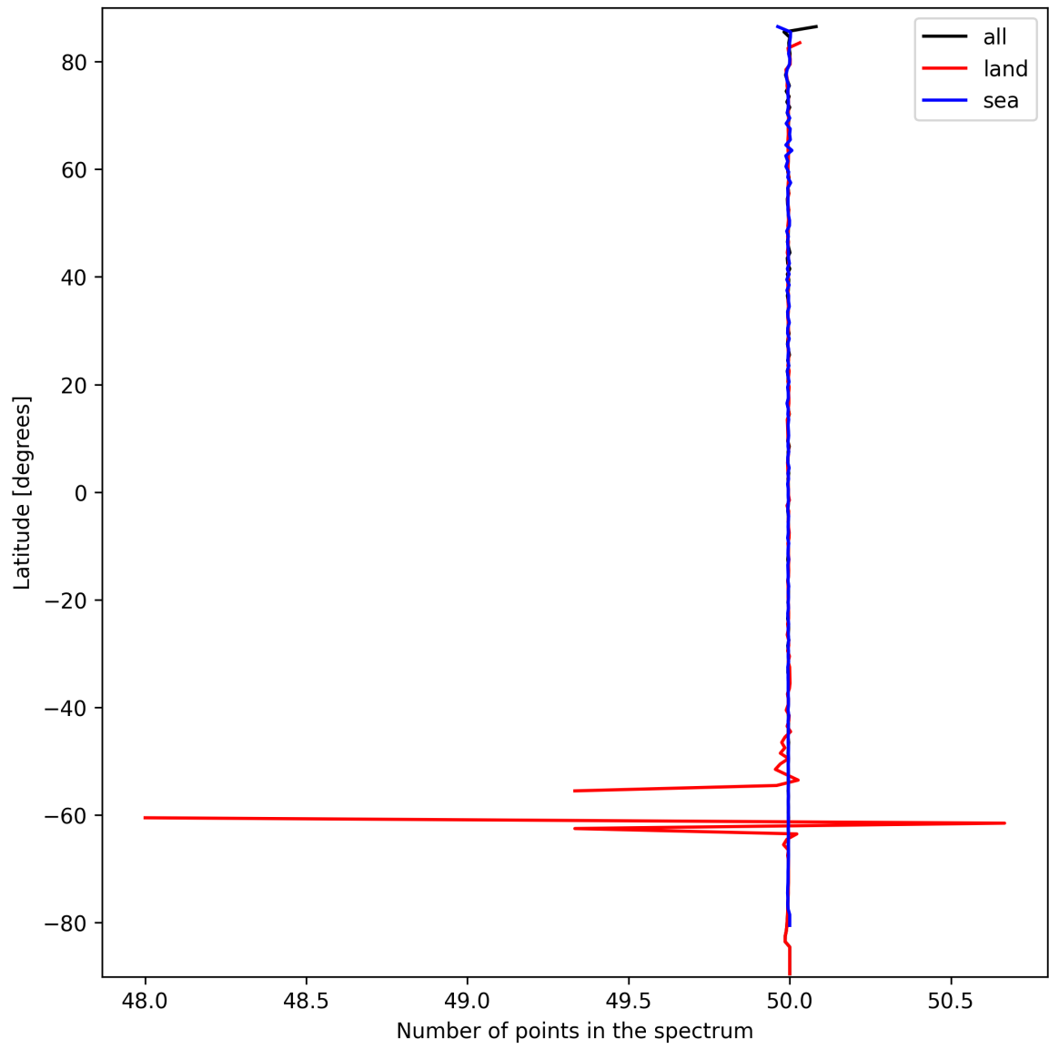
Figure 27: Zonal average of “Number of points in the spectrum” for 2025-09-26 to 2025-09-28.
