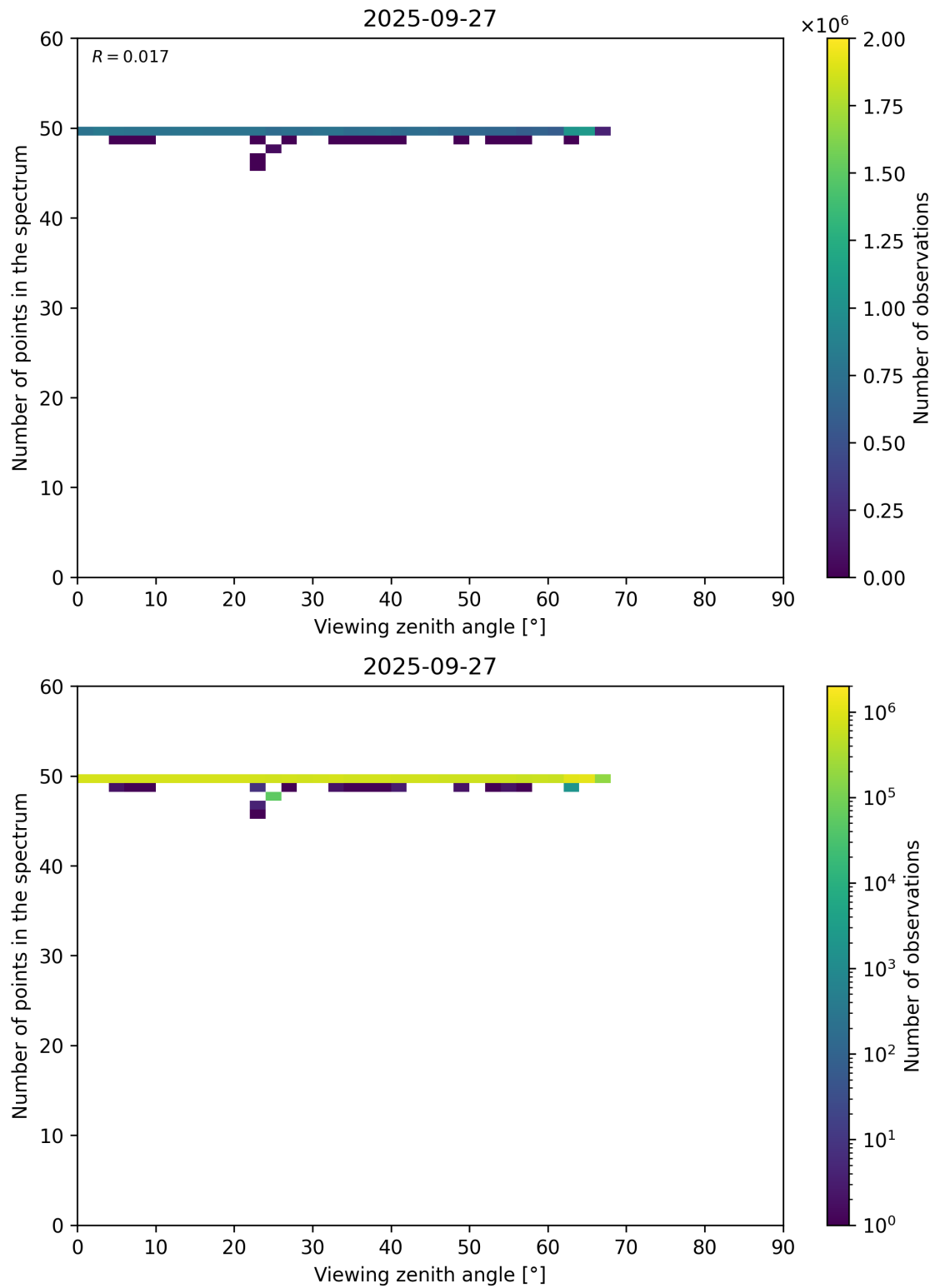
Figure 125: Scatter density plot of “Viewing zenith angle” against “Number of points in the spectrum” for 2025-09-26 to 2025-09-28.
