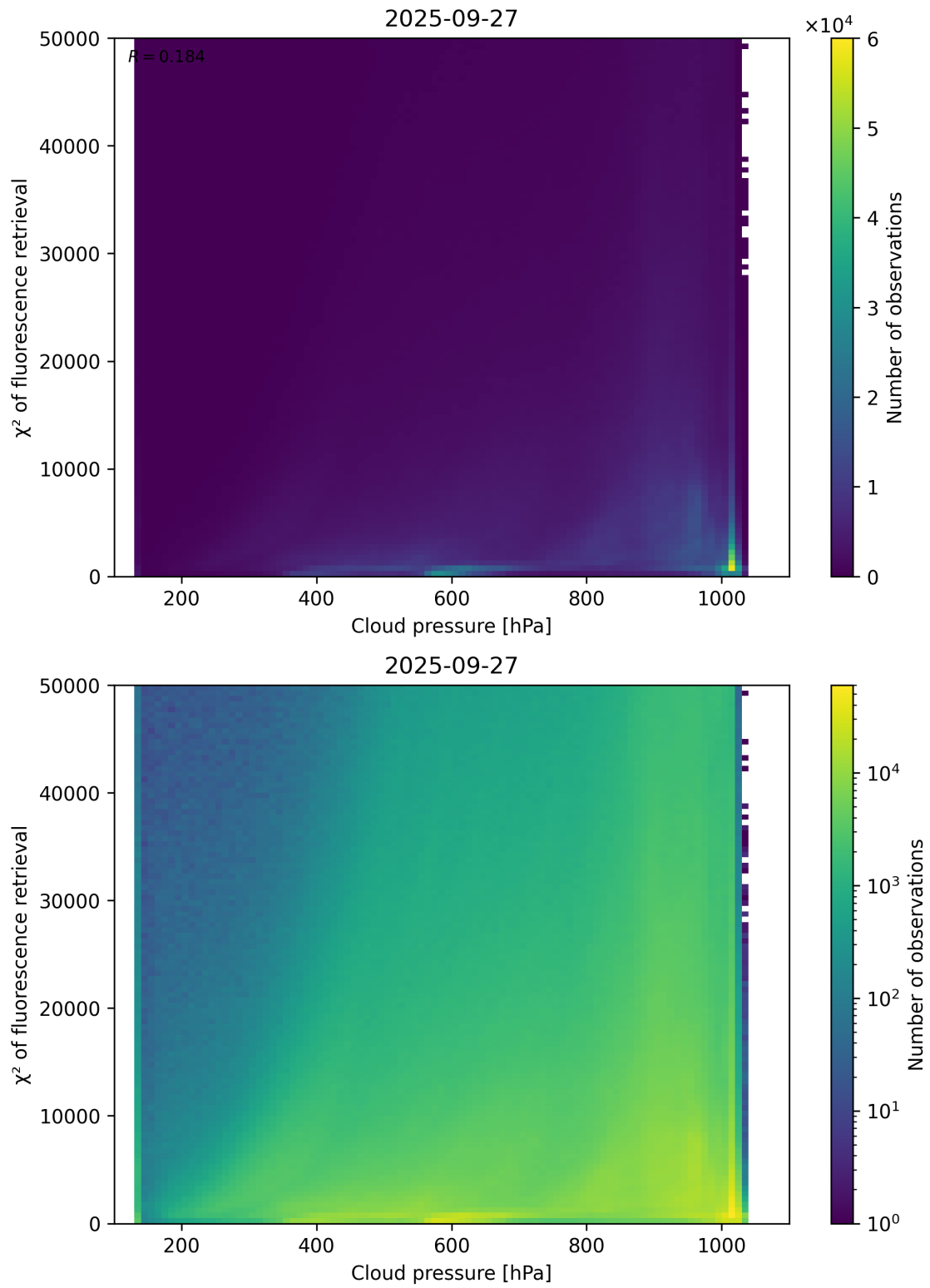
Figure 78: Scatter density plot of “Cloud pressure” against “ \chi^2 of fluorescence retrieval” for 2025-09-26 to 2025-09-28.
