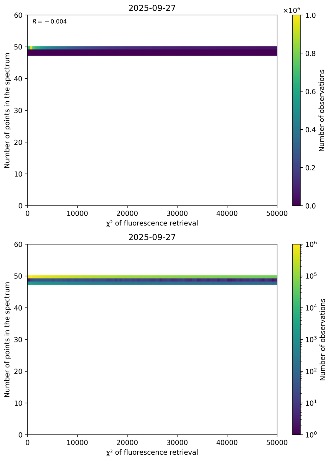
Figure 68: Scatter density plot of " \chi^2 of fluorescence retrieval" against "Number of points in the spectrum" for 2025-09-26 to 2025-09-28.
