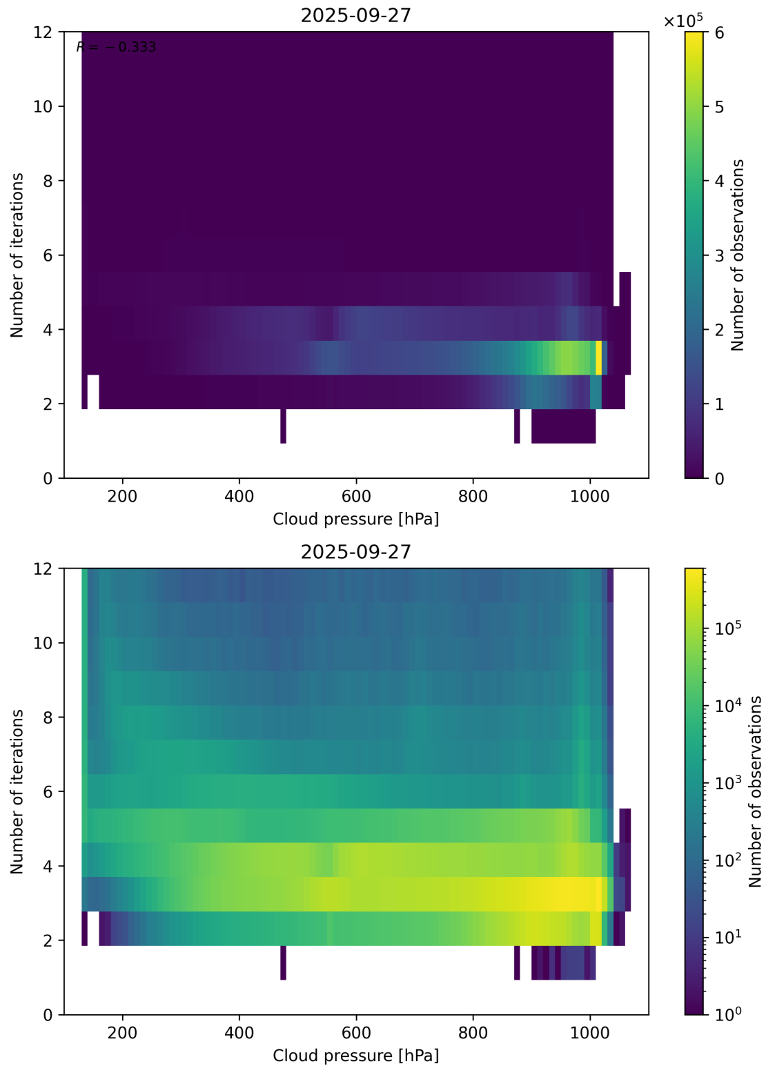
Figure 81: Scatter density plot of “Cloud pressure” against “Number of iterations” for 2025-09-26 to 2025-09-28.
