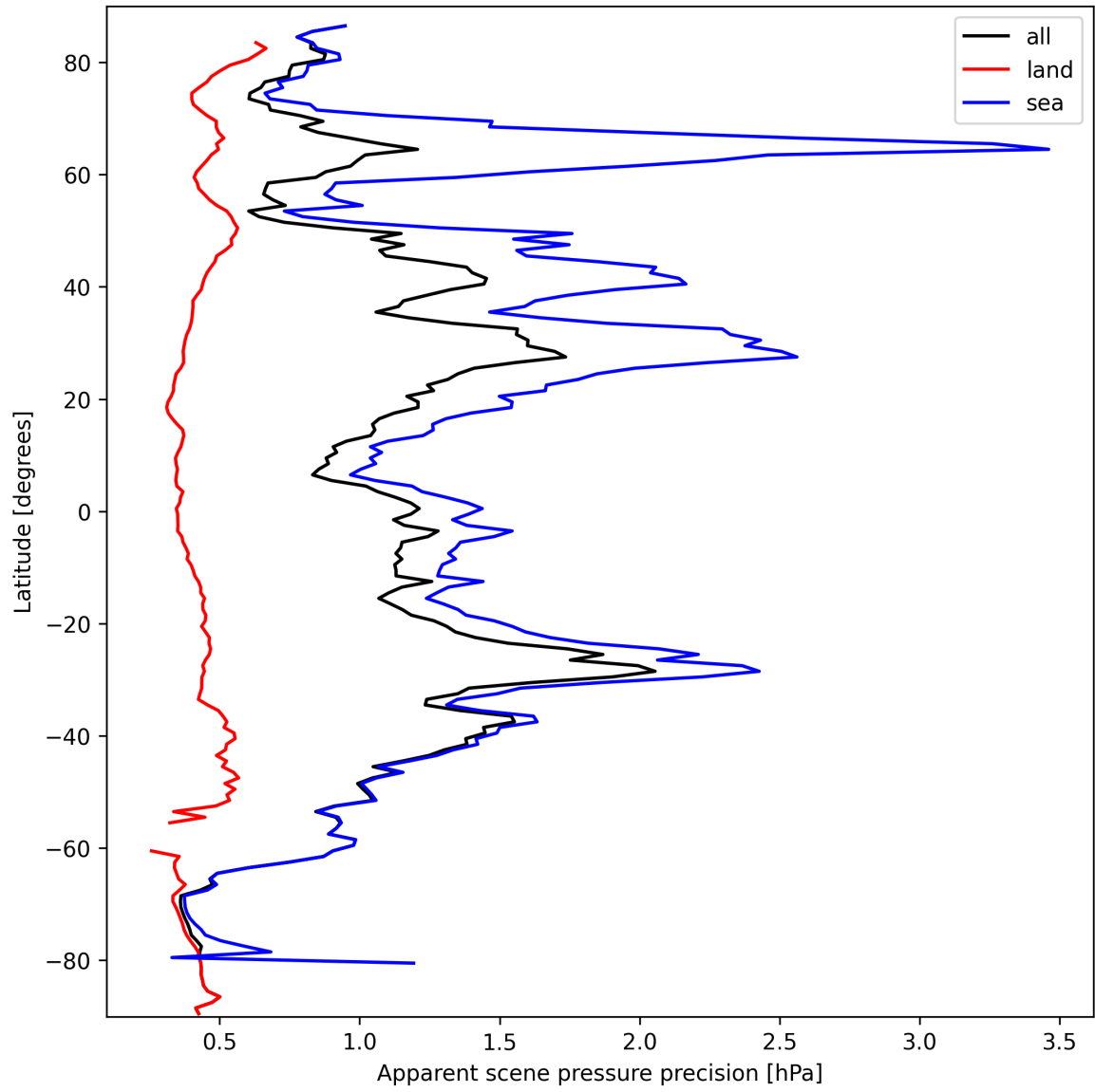
Figure 20: Zonal average of “Apparent scene pressure precision” for 2025-09-26 to 2025-09-28.
