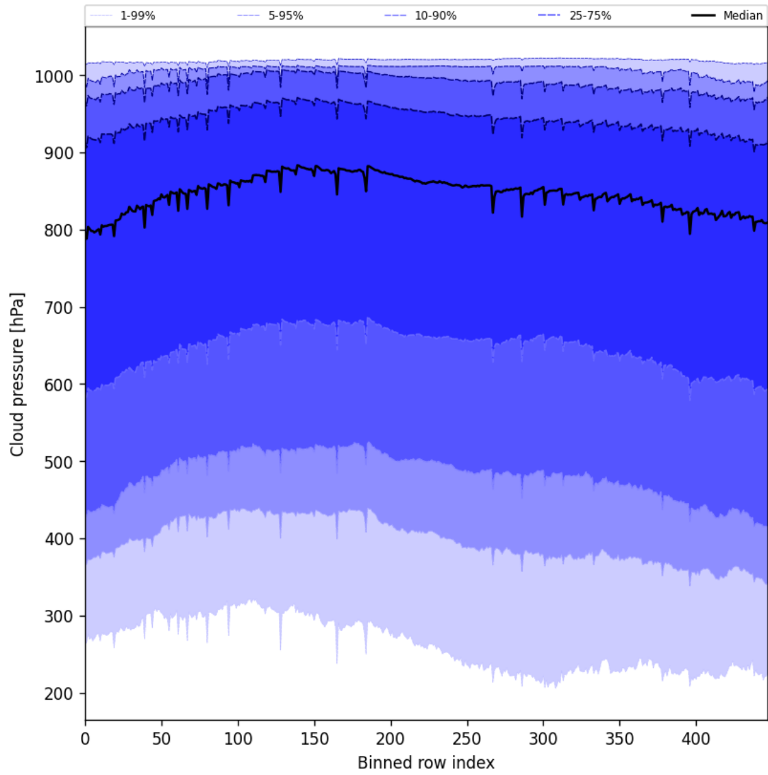
Figure 47: Along track statistics of “Cloud pressure” for 2025-09-26 to 2025-09-28
