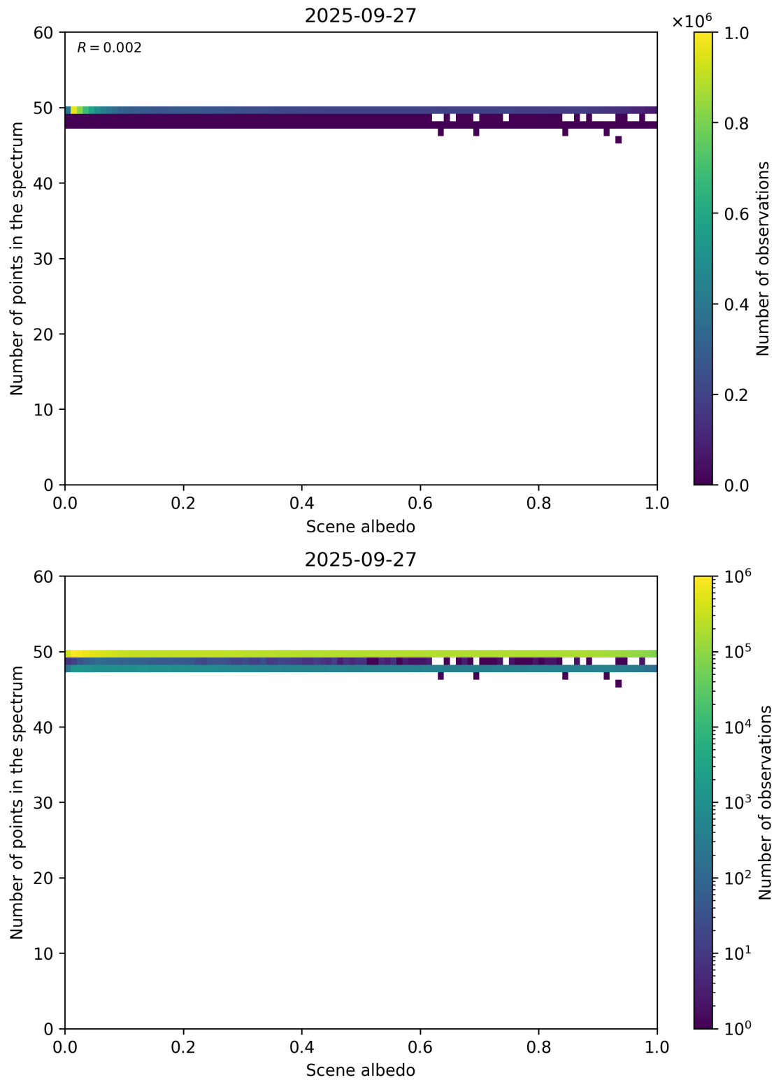
Figure 106: Scatter density plot of “Scene albedo” against “Number of points in the spectrum” for 2025-09-26 to 2025-09-28.
