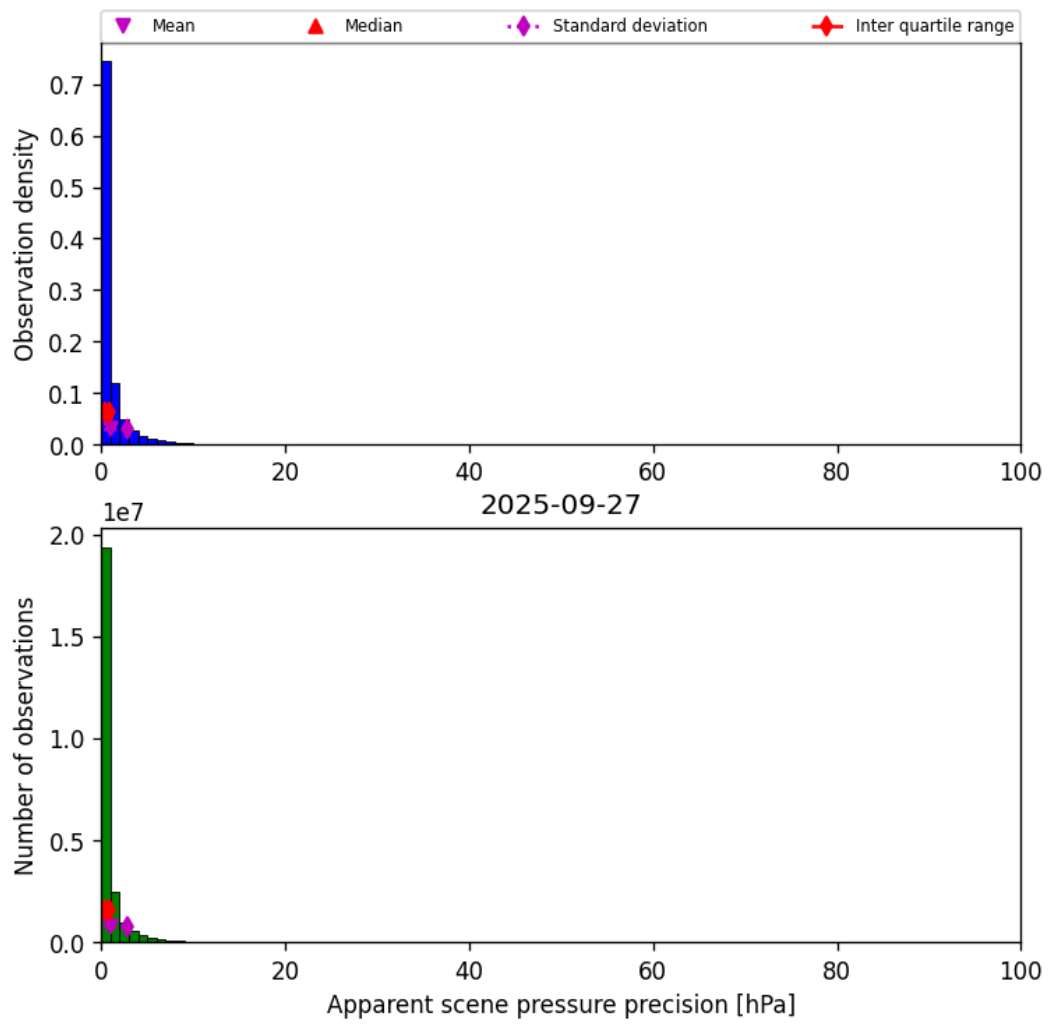
Figure 37: Histogram of “Apparent scene pressure precision” for 2025-09-26 to 2025-09-28
