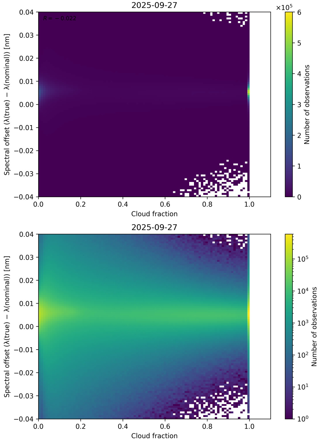
Figure 76: Scatter density plot of “Cloud fraction” against “Spectral offset ( \lambda_{\text{true}} - \lambda_{\text{nominal}} )” for 2025-09-26 to 2025-09-28.
