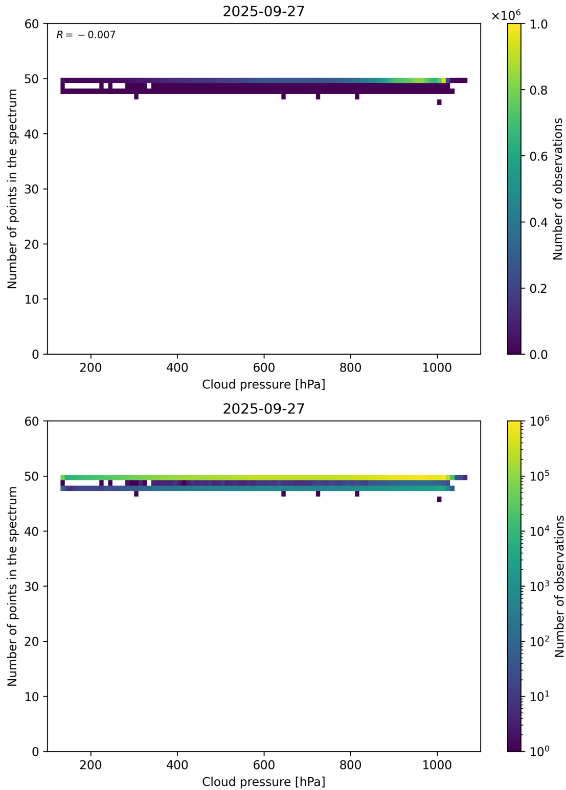
Figure 82: Scatter density plot of “Cloud pressure” against “Number of points in the spectrum” for 2025-09-26 to 2025-09-28.
