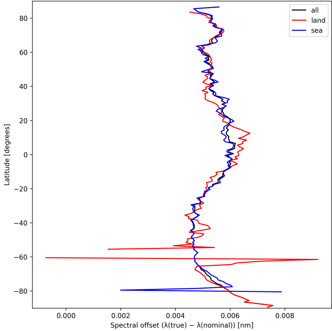
Figure 28: Zonal average of “Spectral offset ( \lambda_{\text{true}} - \lambda_{\text{nominal}} )” for 2025-09-26 to 2025-09-28.
