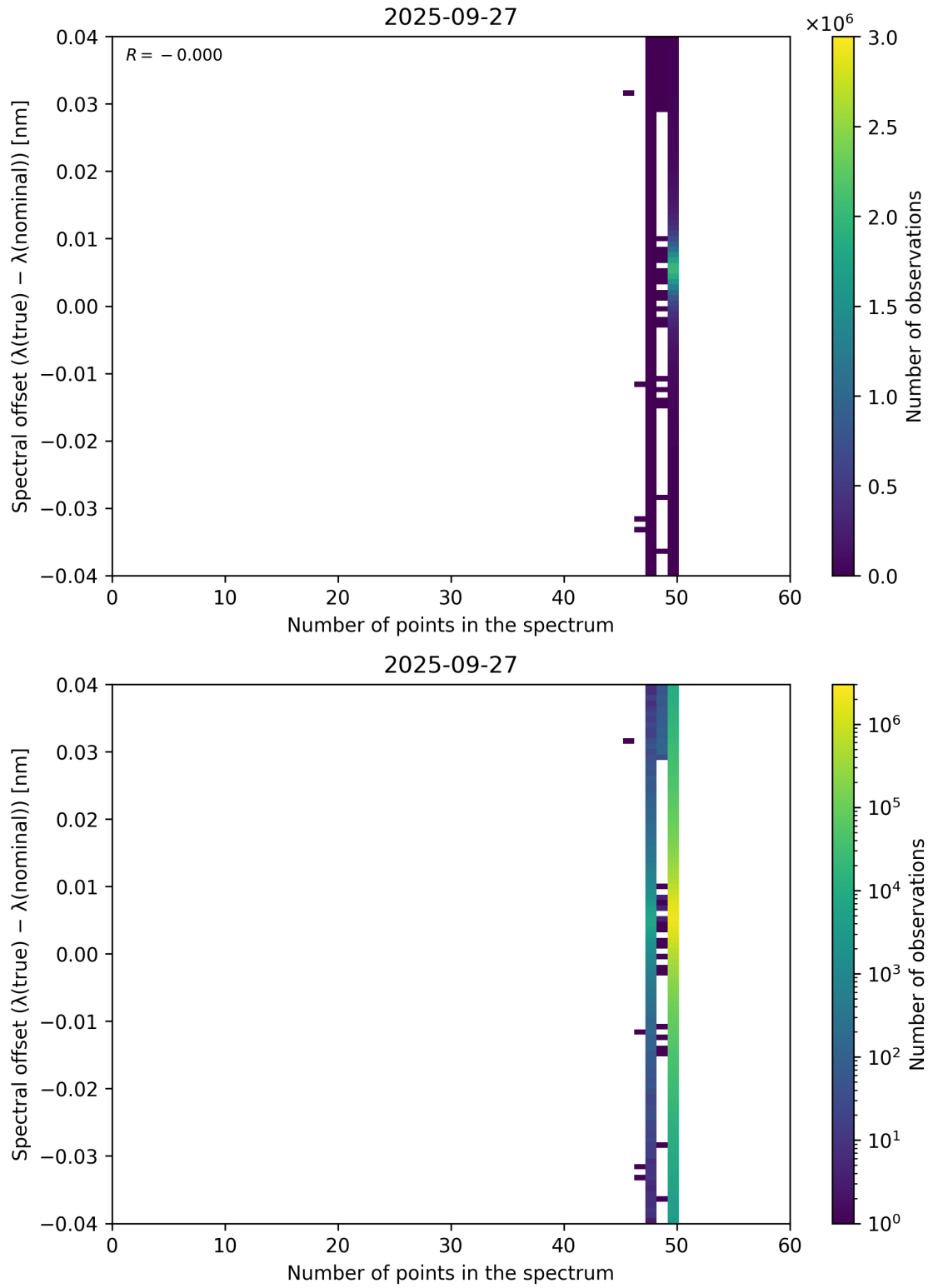
Figure 101: Scatter density plot of “Number of points in the spectrum” against “Spectral offset ( \lambda_{\text{true}} - \lambda_{\text{nominal}} )” for 2025-09-26 to 2025-09-28.
