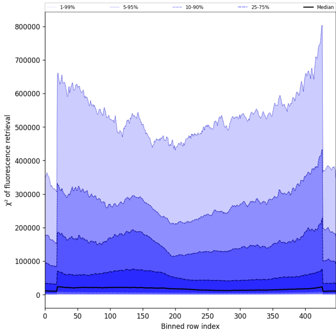
Figure 59: Along track statistics of “ \chi^2 of fluorescence retrieval” for 2025-09-26 to 2025-09-28
