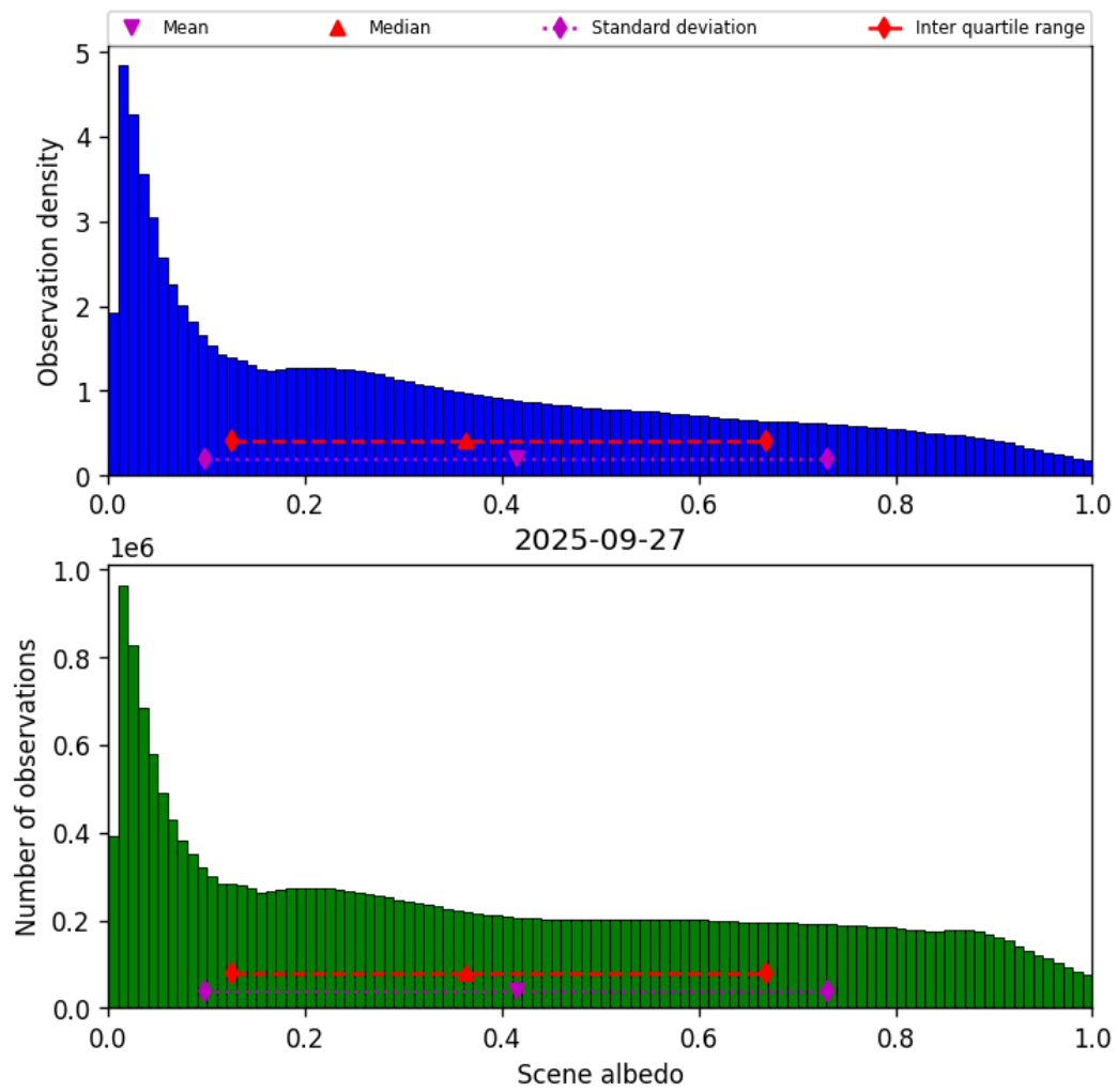
Figure 34: Histogram of “Scene albedo” for 2025-09-26 to 2025-09-28
