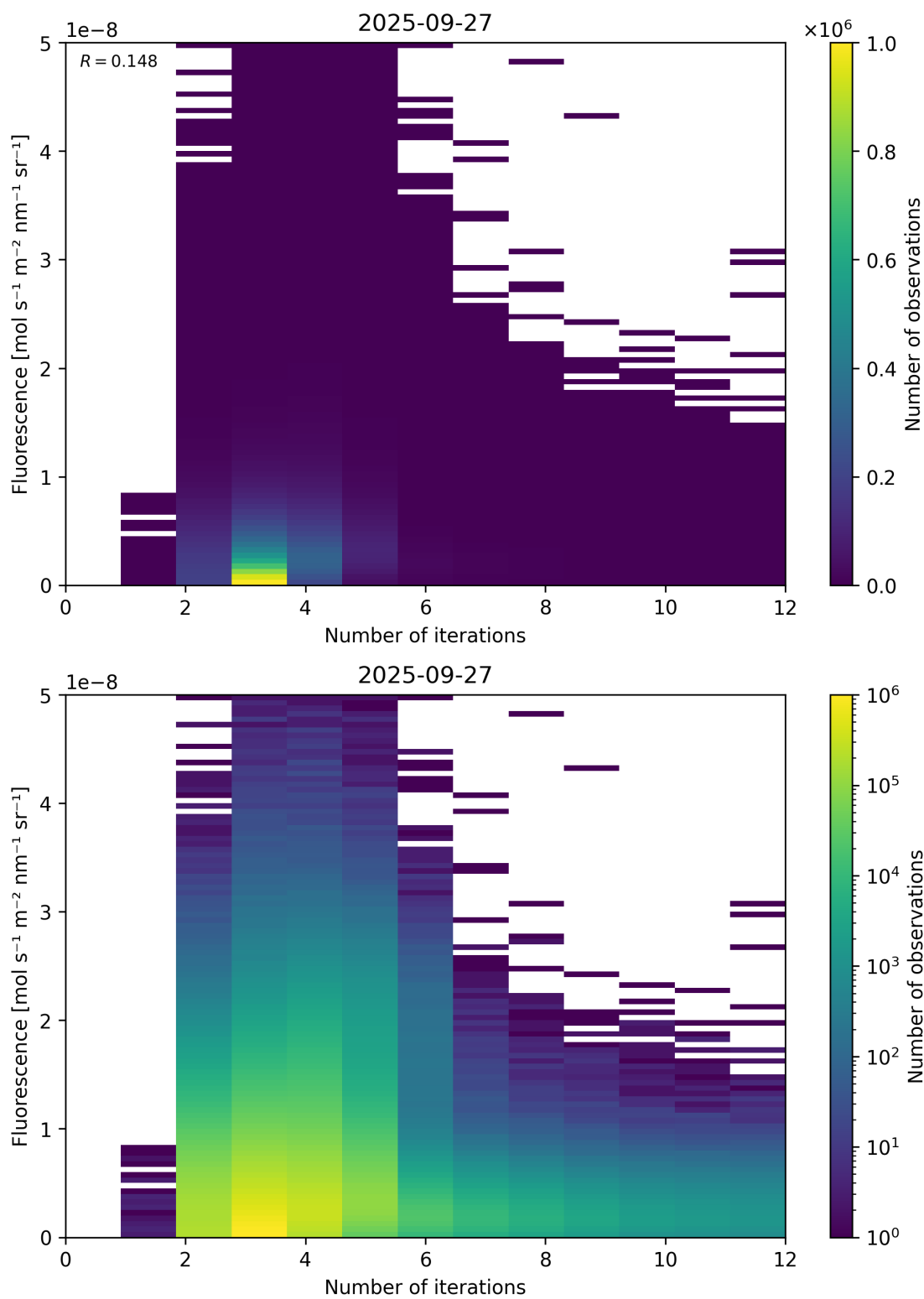
Figure 98: Scatter density plot of “Number of iterations” against “Fluorescence” for 2025-09-26 to 2025-09-28.
