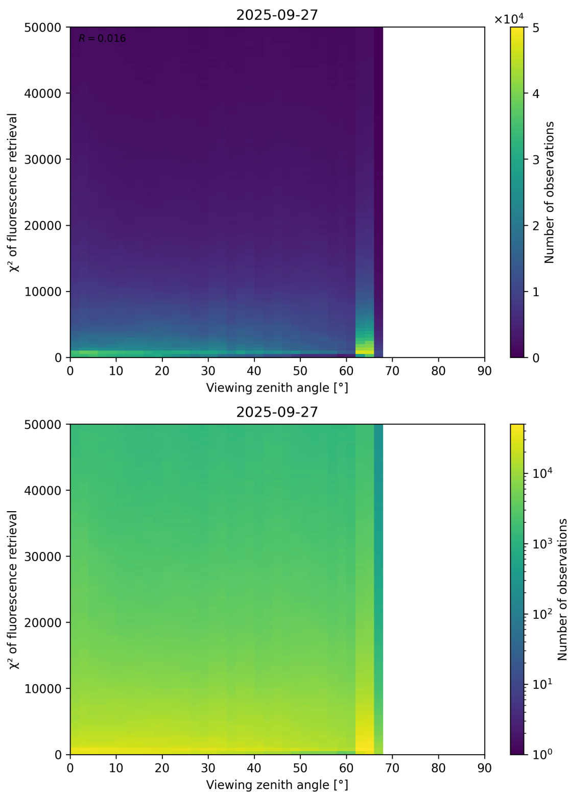
Figure 119: Scatter density plot of “Viewing zenith angle” against “ \chi^2 of fluorescence retrieval” for 2025-09-26 to 2025-09-28.
