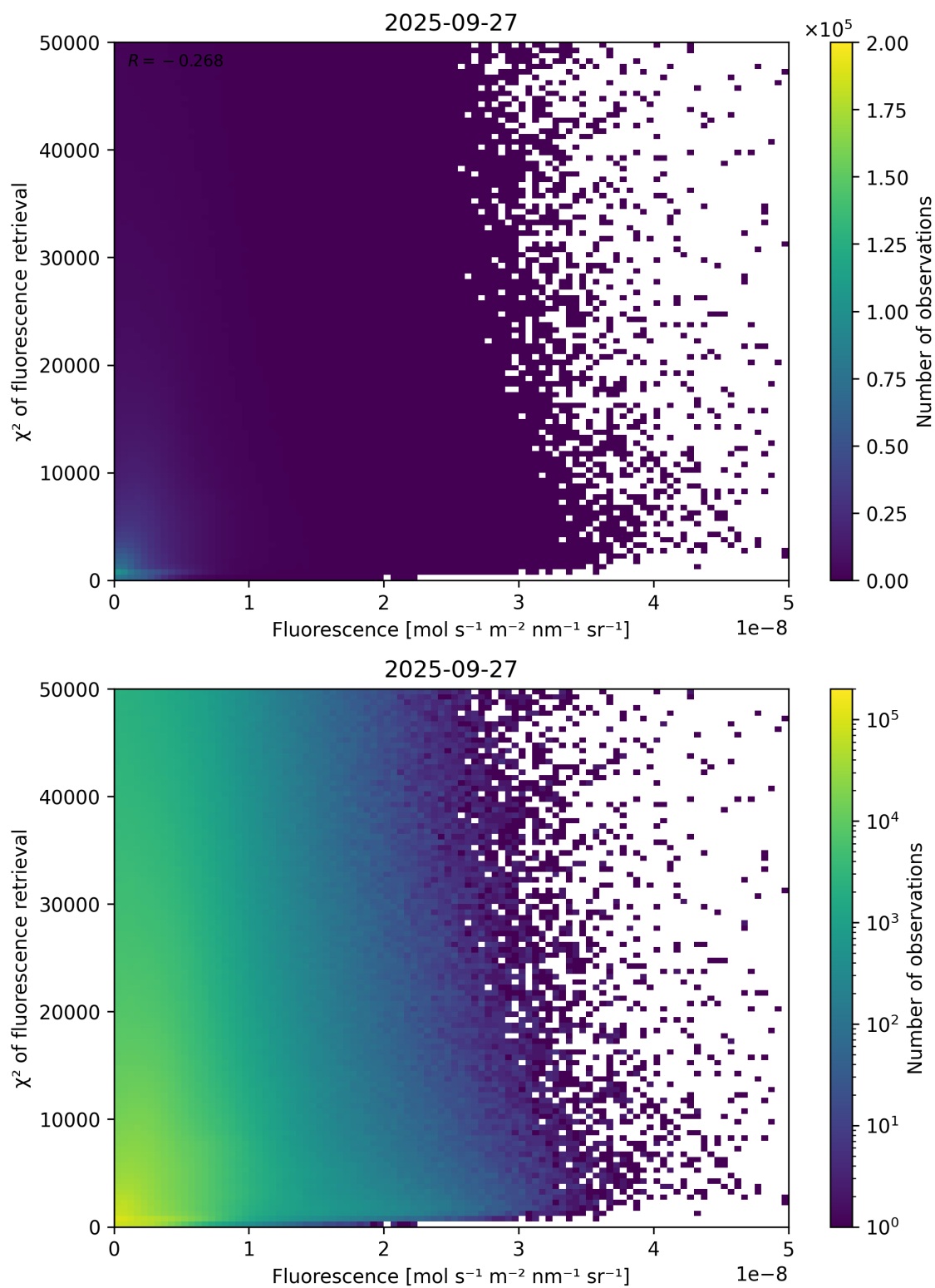
Figure 85: Scatter density plot of “Fluorescence” against “ \chi^2 of fluorescence retrieval” for 2025-09-26 to 2025-09-28.
