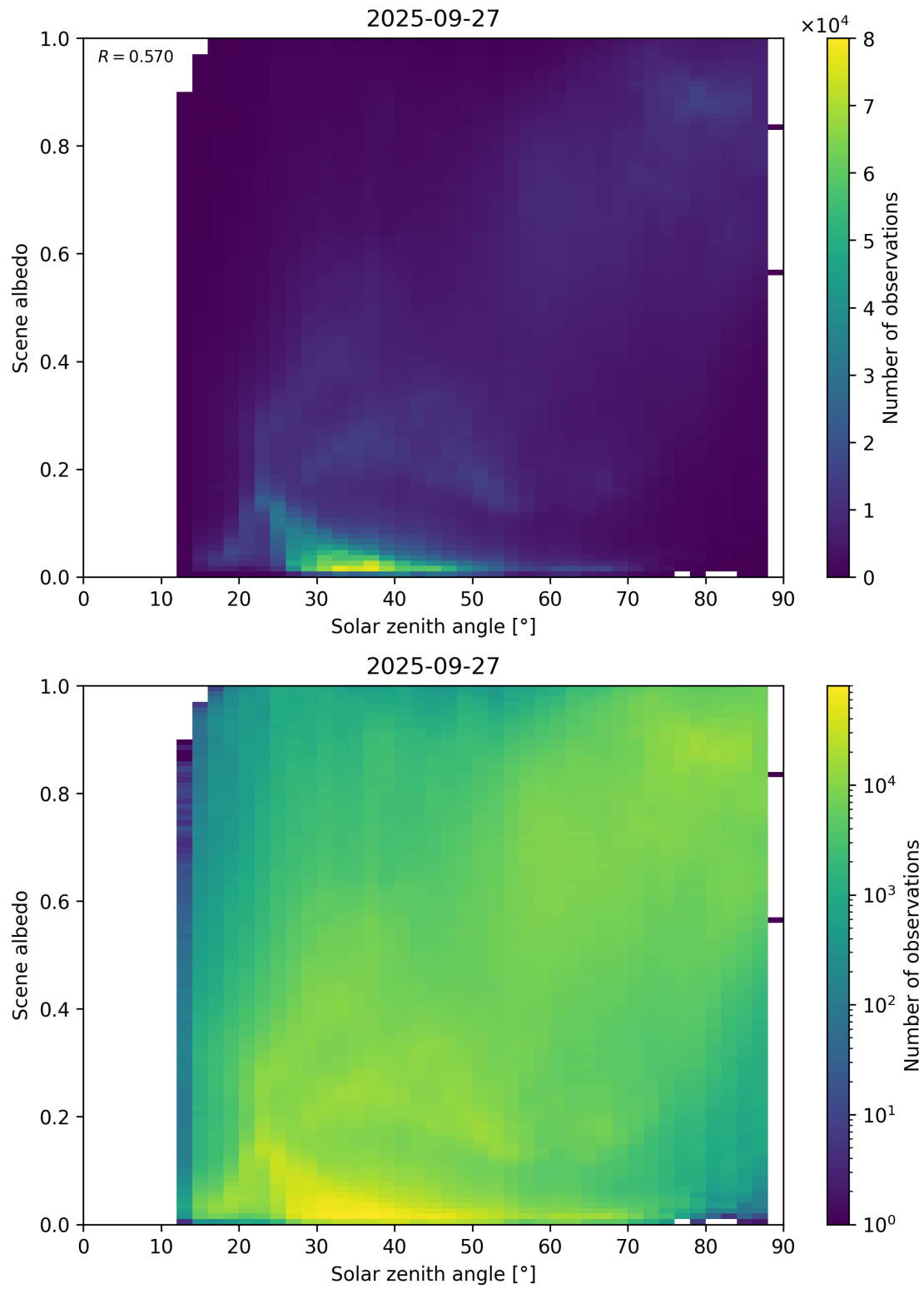
Figure 116: Scatter density plot of “Solar zenith angle” against “Scene albedo” for 2025-09-26 to 2025-09-28.
