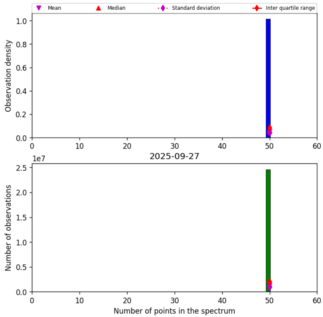
Figure 44: Histogram of "Number of points in the spectrum" for 2025-09-26 to 2025-09-28
