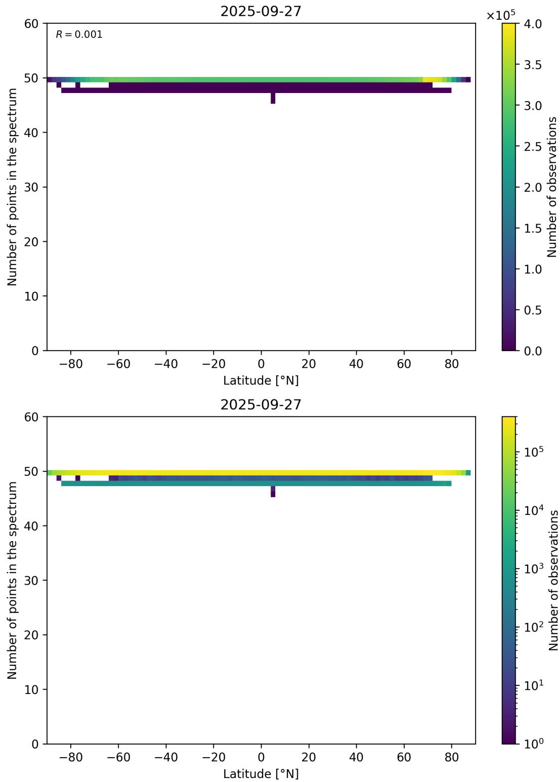
Figure 94: Scatter density plot of “Latitude” against “Number of points in the spectrum” for 2025-09-26 to 2025-09-28.
