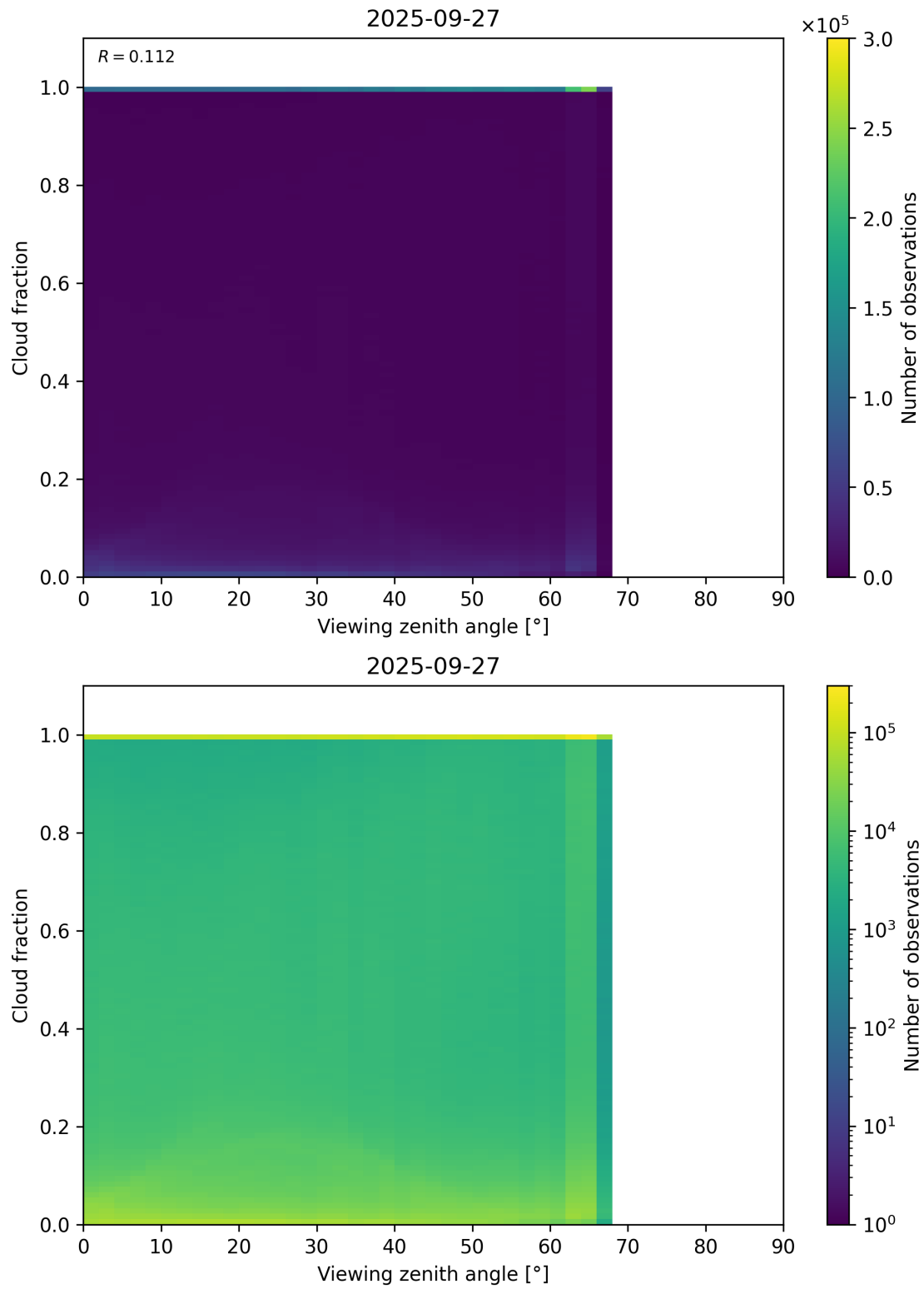
Figure 120: Scatter density plot of “Viewing zenith angle” against “Cloud fraction” for 2025-09-26 to 2025-09-28.
