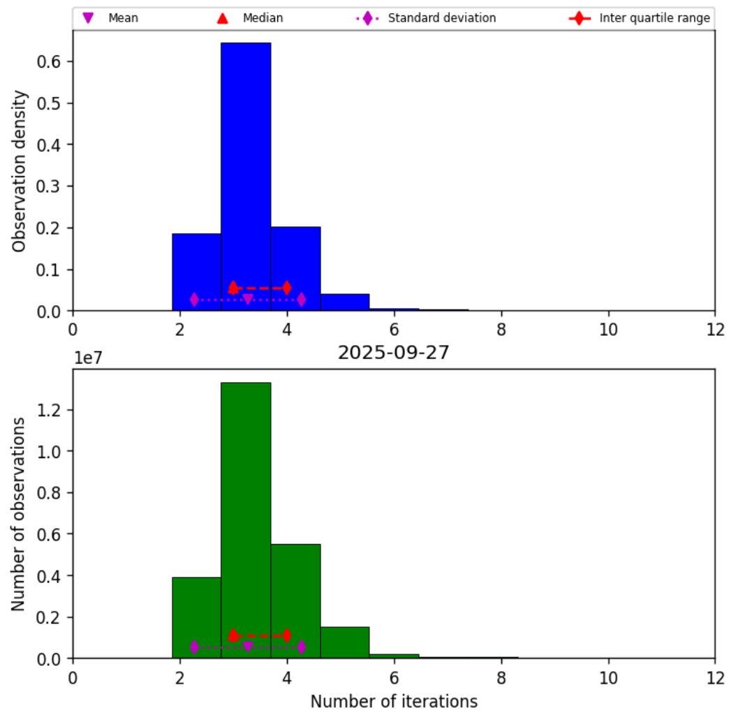
Figure 39: Histogram of “Number of iterations” for 2025-09-26 to 2025-09-28
