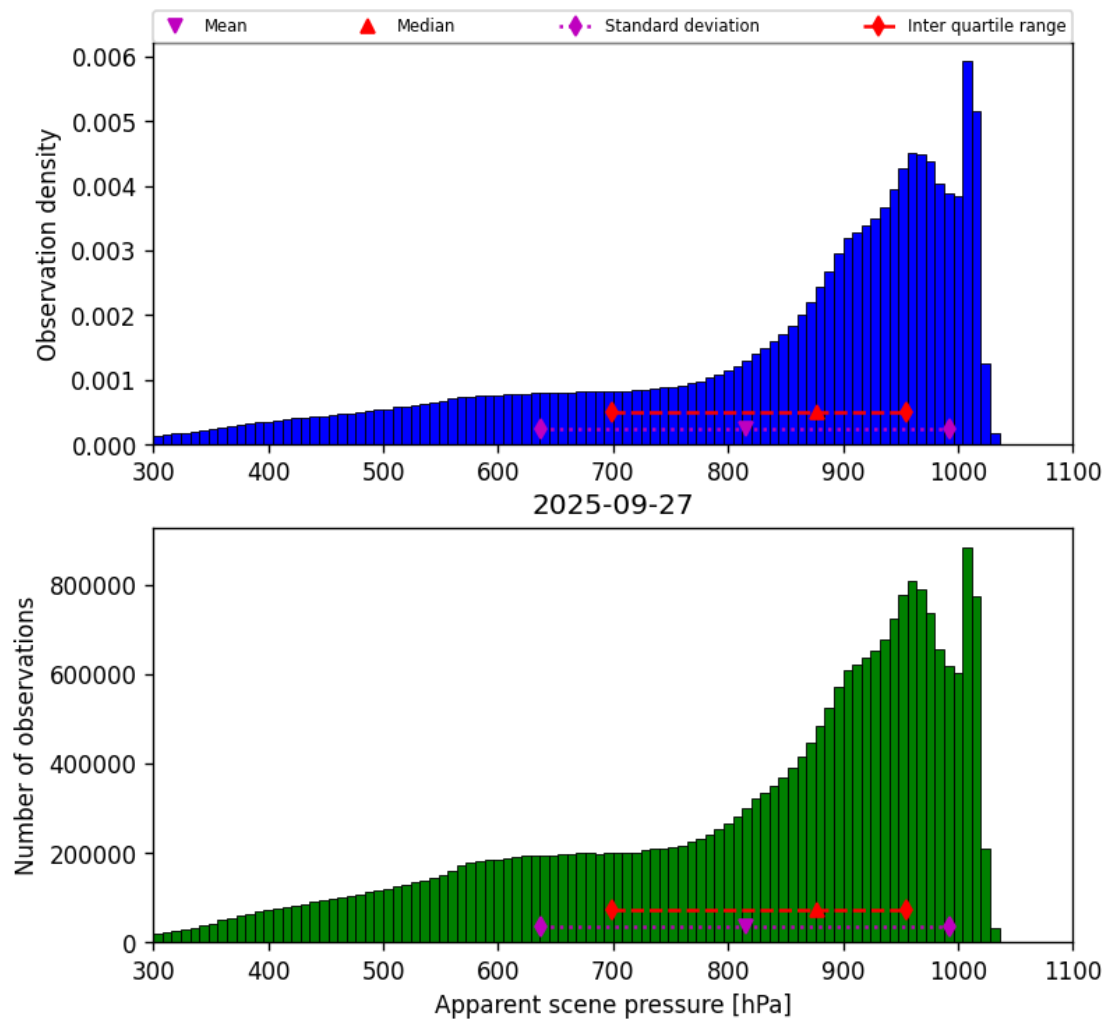
Figure 36: Histogram of “Apparent scene pressure” for 2025-09-26 to 2025-09-28
