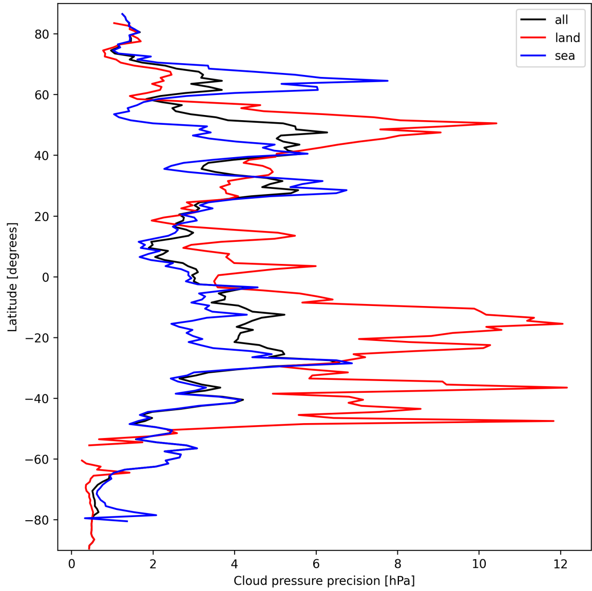
Figure 14: Zonal average of "Cloud pressure precision" for 2025-09-26 to 2025-09-28.
