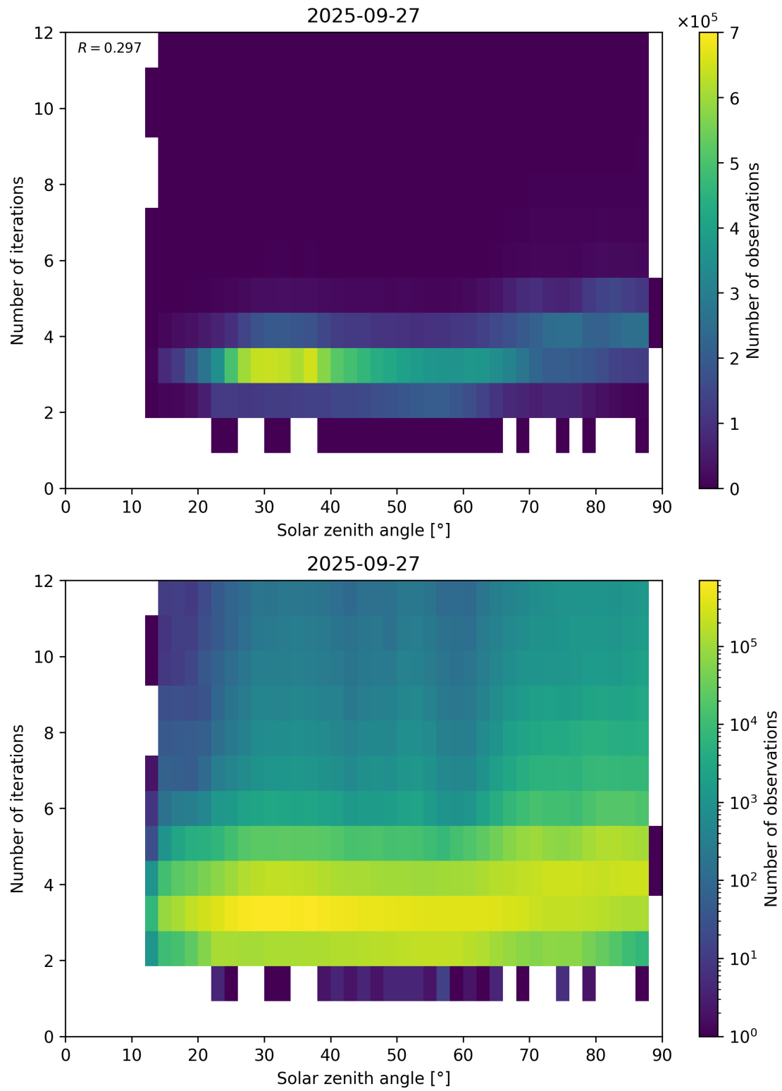
Figure 114: Scatter density plot of “Solar zenith angle” against “Number of iterations” for 2025-09-26 to 2025-09-28.
