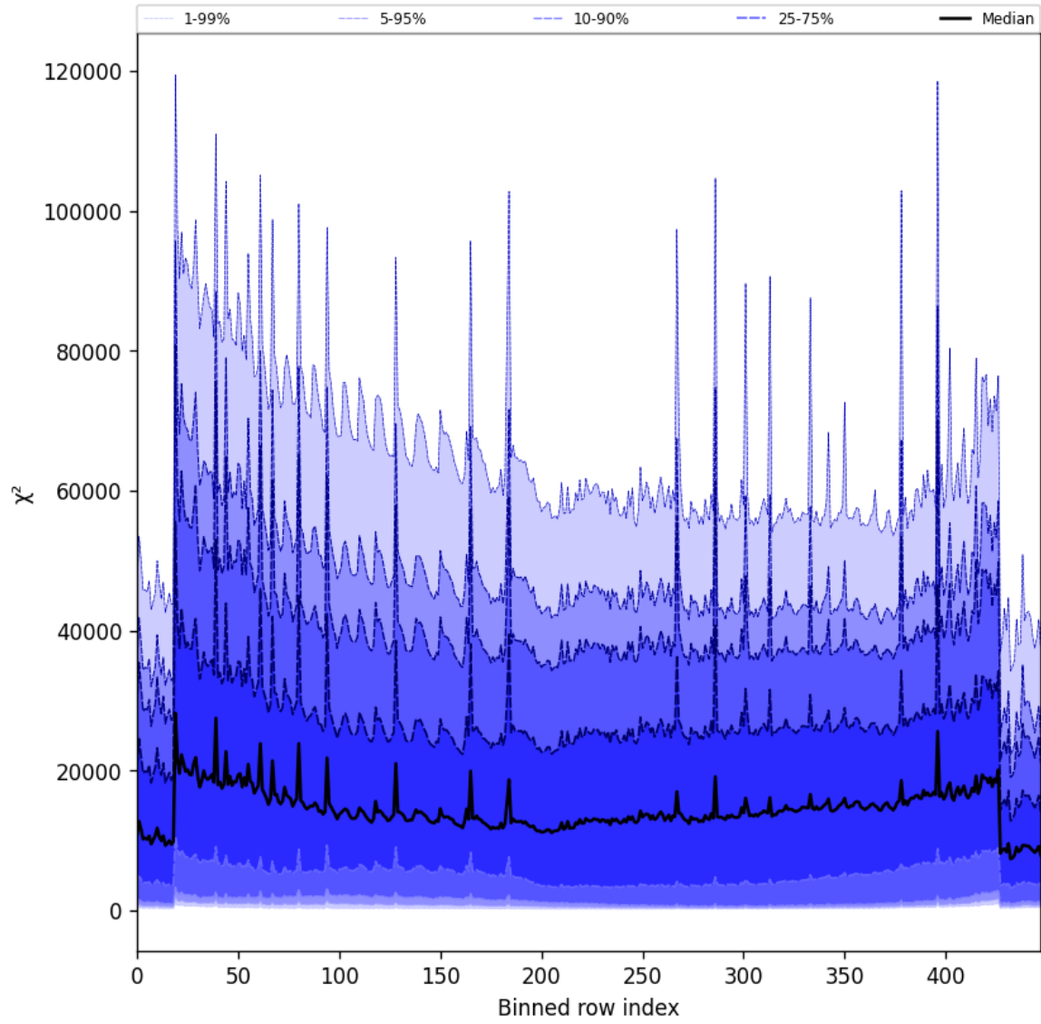
Figure 55: Along track statistics of “ \chi^2 ” for 2025-09-26 to 2025-09-28
