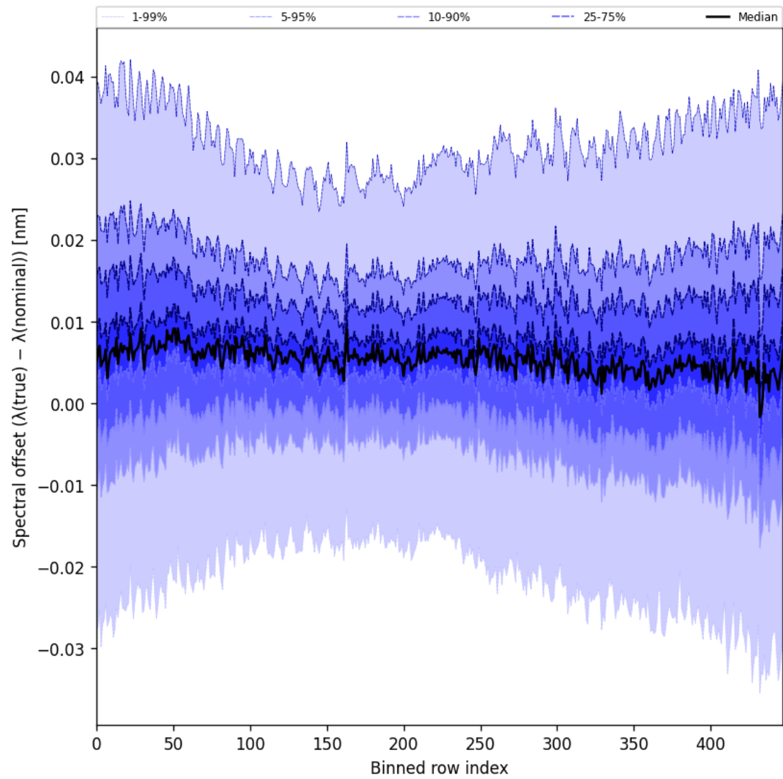
Figure 62: Along track statistics of “Spectral offset ( \lambda_{\text{true}} - \lambda_{\text{nominal}} )” for 2025-09-26 to 2025-09-28
