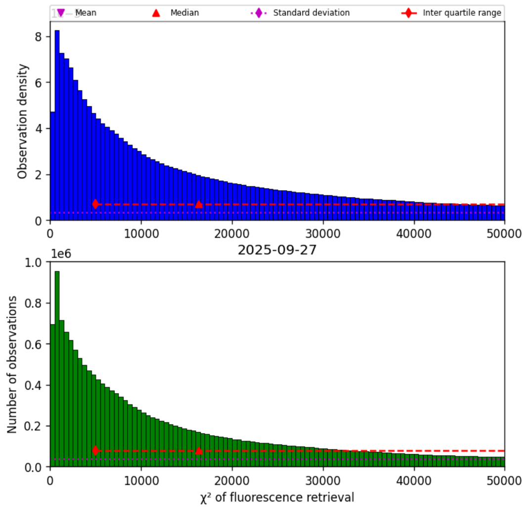
Figure 42: Histogram of “ \chi^2 of fluorescence retrieval” for 2025-09-26 to 2025-09-28
