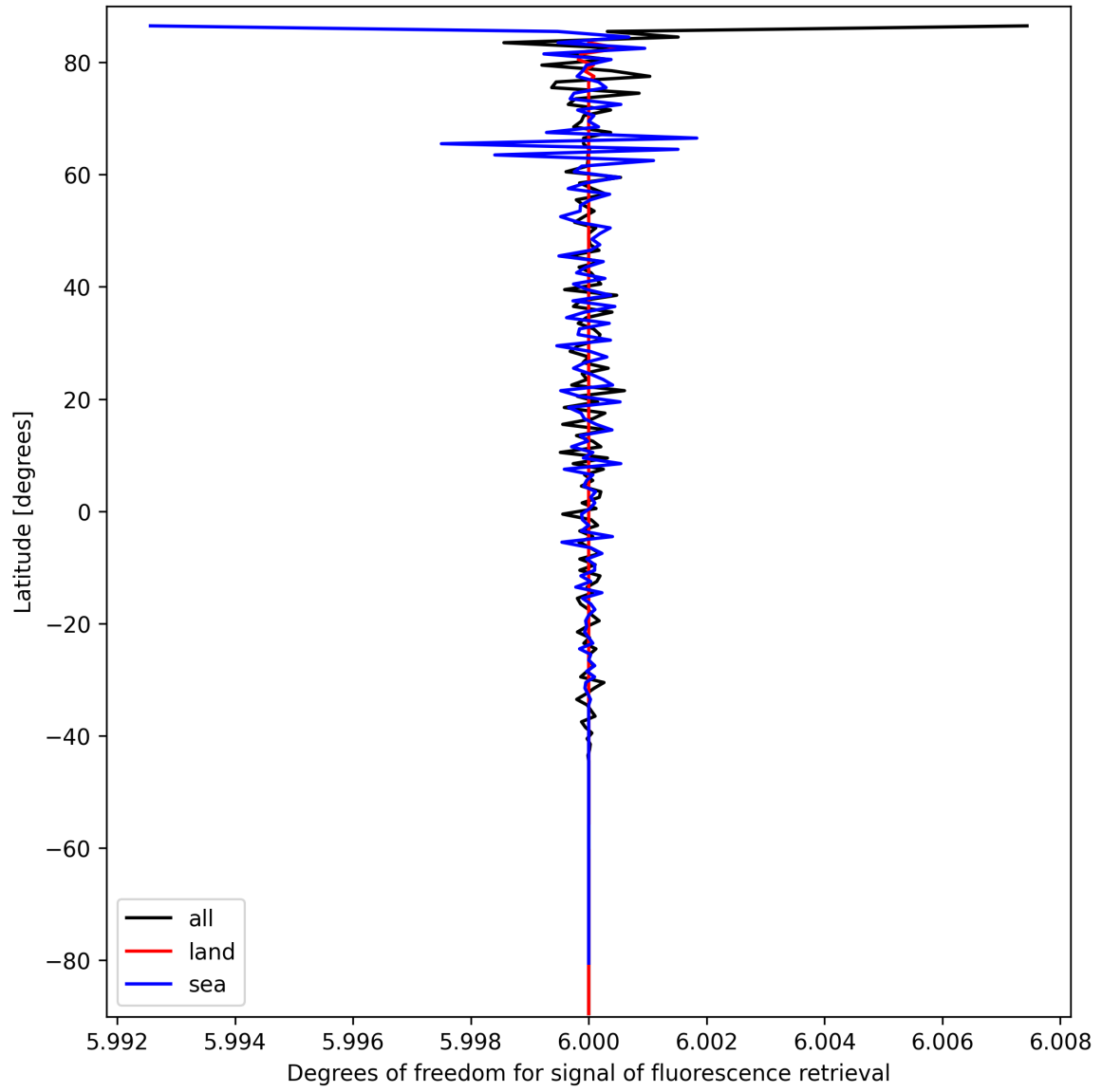
Figure 26: Zonal average of “Degrees of freedom for signal of fluorescence retrieval” for 2025-09-26 to 2025-09-28.
