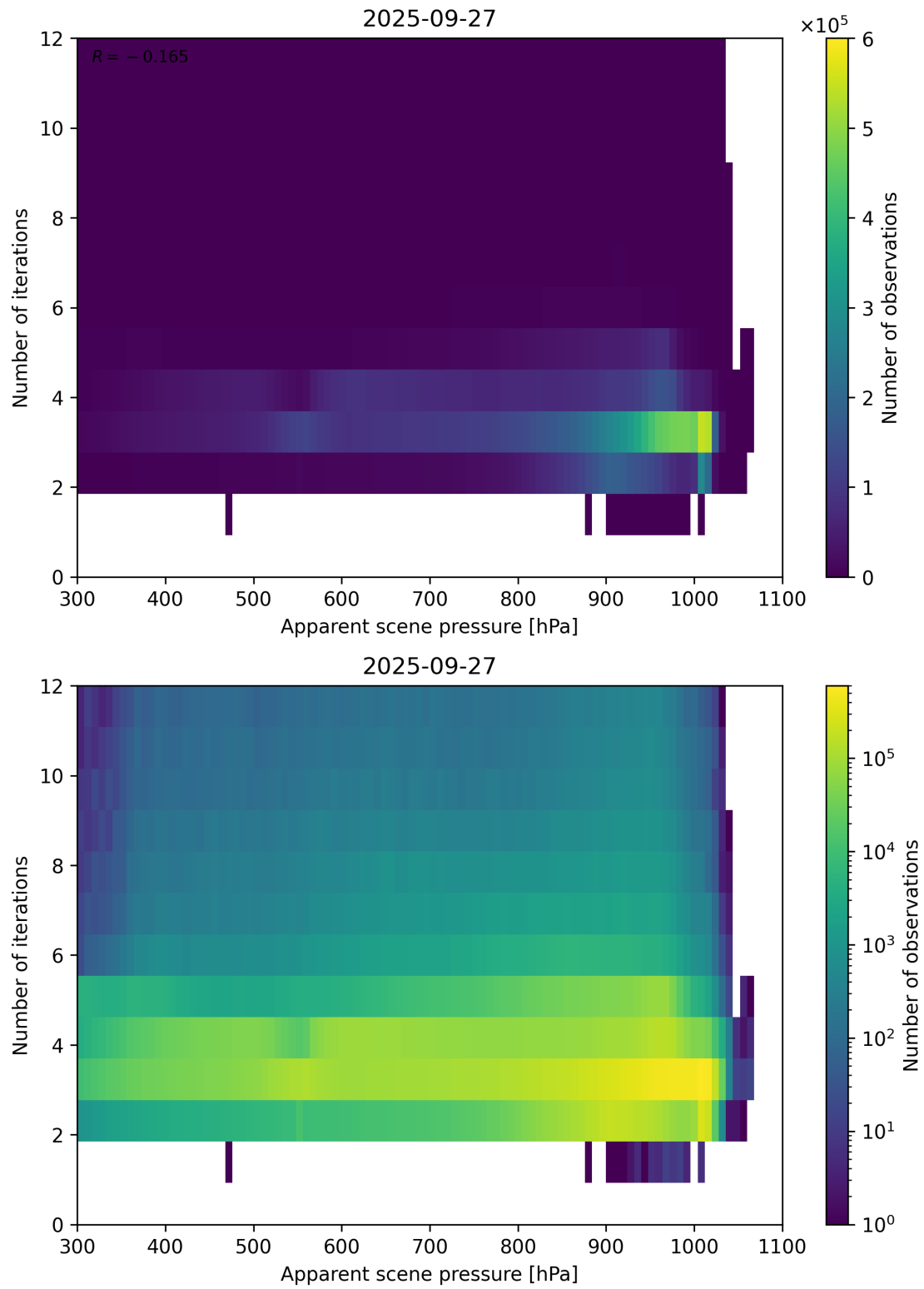
Figure 65: Scatter density plot of “Apparent scene pressure” against “Number of iterations” for 2025-09-26 to 2025-09-28.
