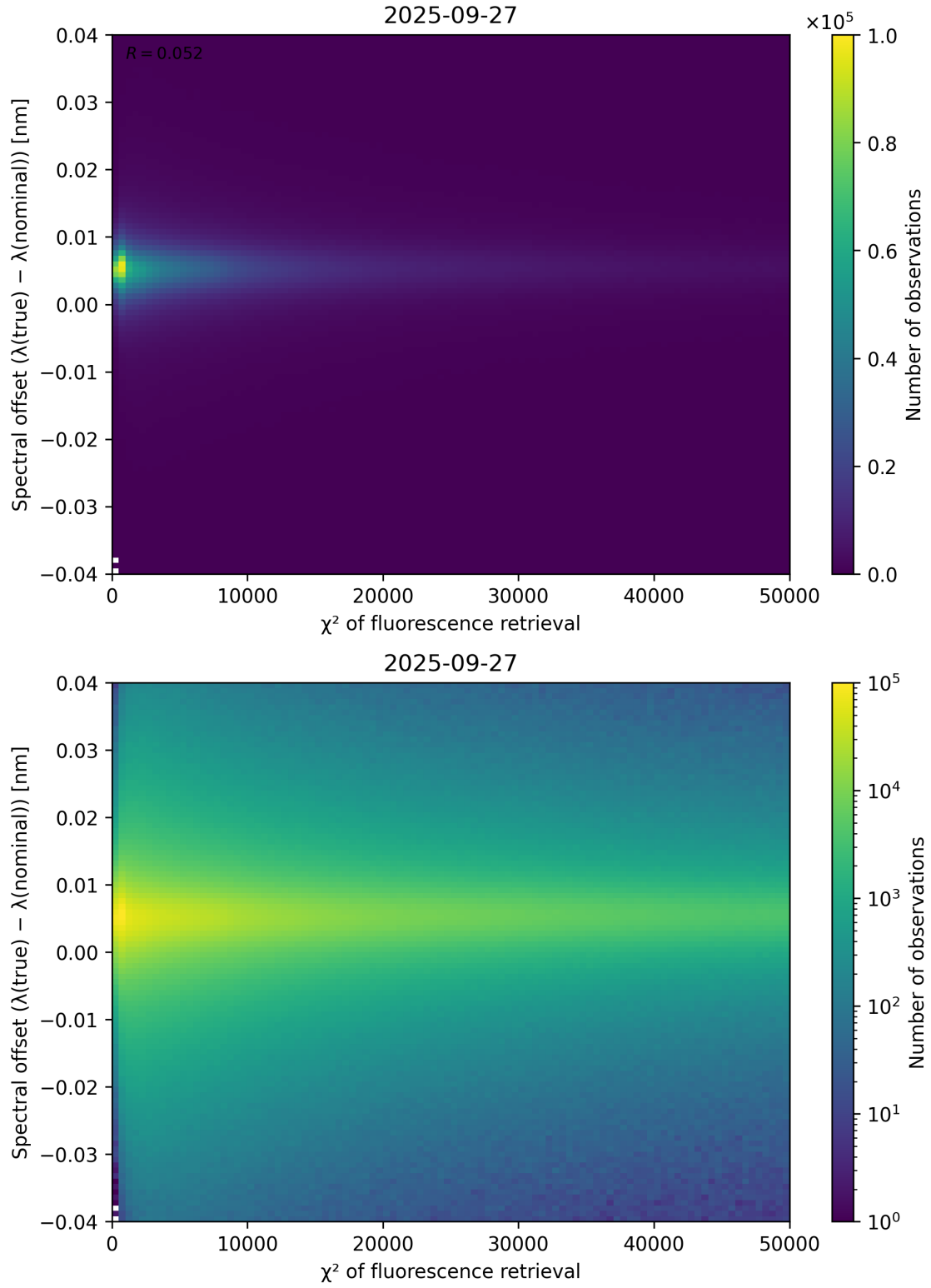
Figure 69: Scatter density plot of “ \chi^2 of fluorescence retrieval” against “Spectral offset ( \lambda_{\text{true}} - \lambda_{\text{nominal}} )” for 2025-09-26 to 2025-09-28.
