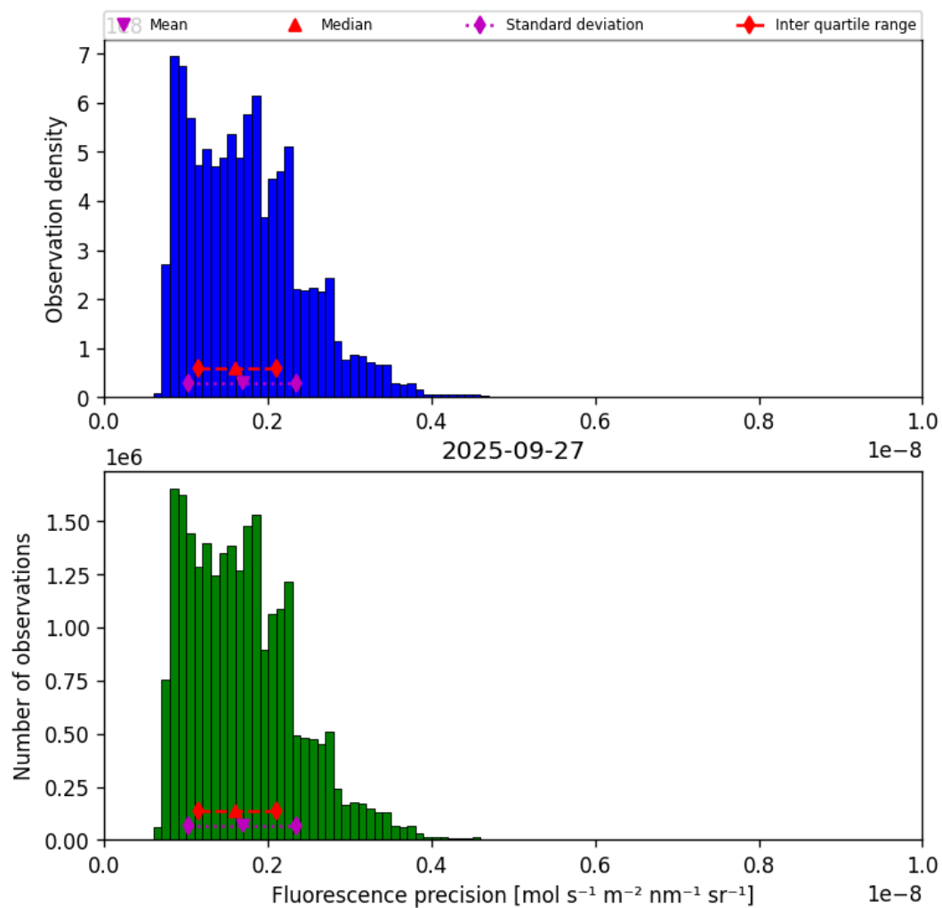
Figure 41: Histogram of “Fluorescence precision” for 2025-09-26 to 2025-09-28
