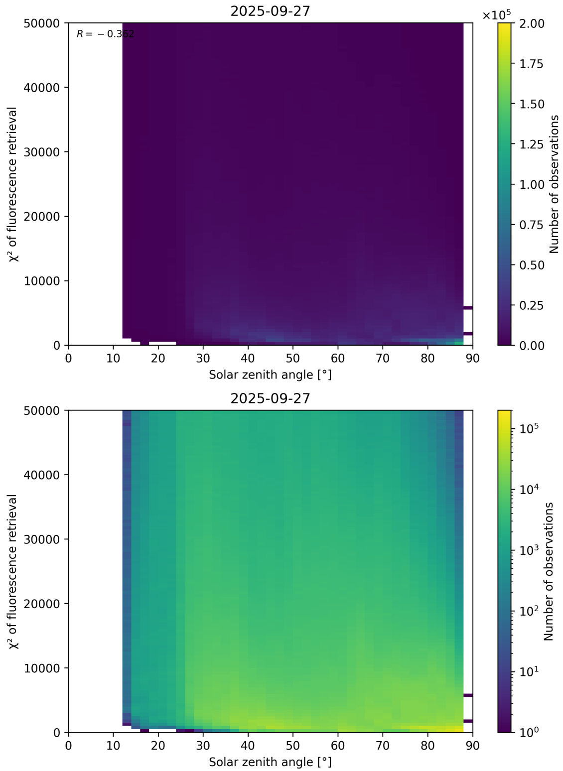
Figure 109: Scatter density plot of “Solar zenith angle” against “ \chi^2 of fluorescence retrieval” for 2025-09-26 to 2025-09-28.
