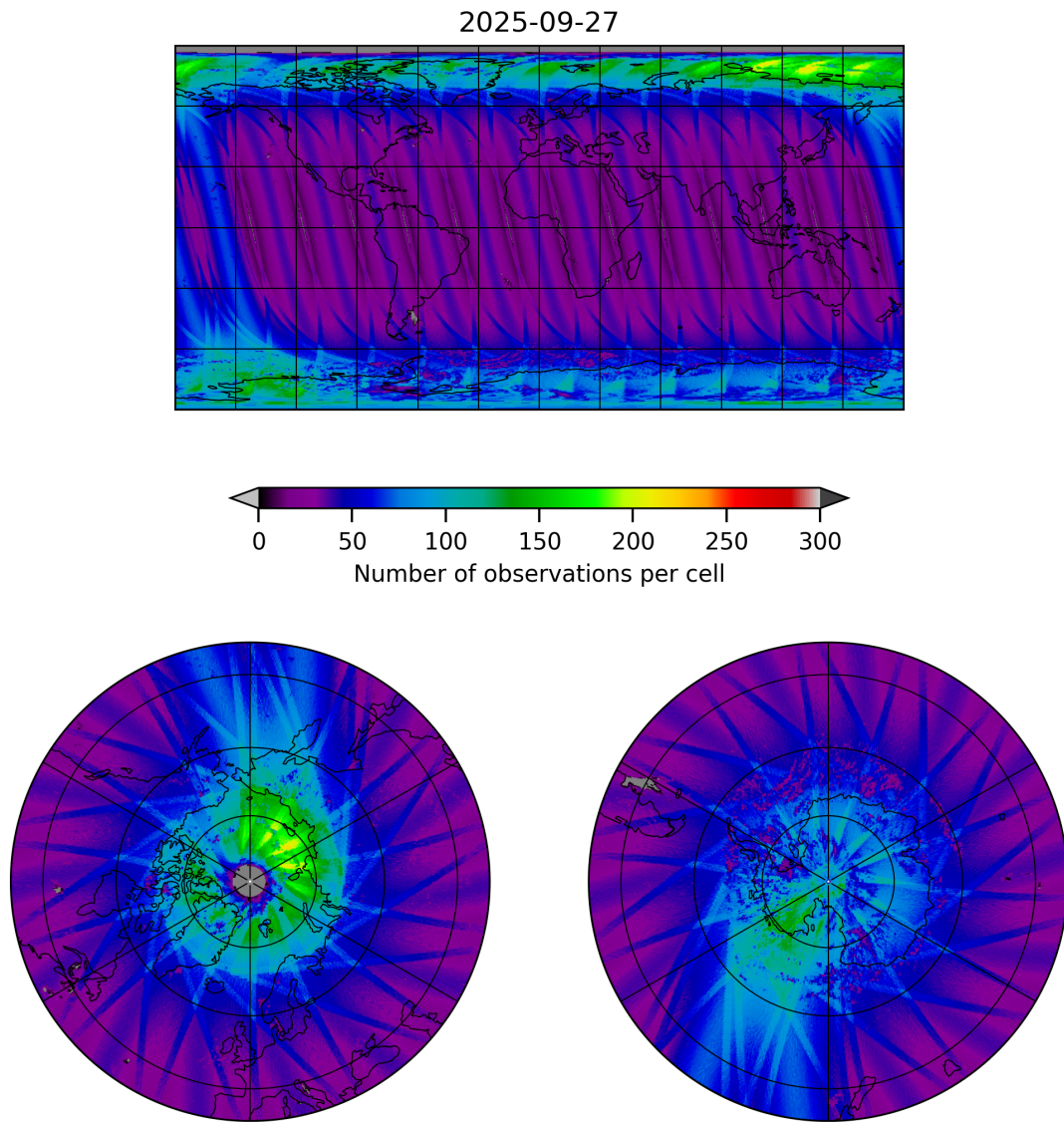
Figure 11: Map of the number of observations for 2025-09-26 to 2025-09-28
