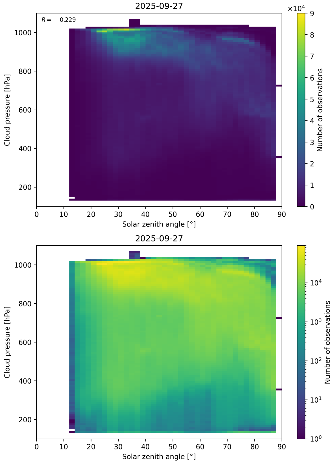
Figure 111: Scatter density plot of “Solar zenith angle” against “Cloud pressure” for 2025-09-26 to 2025-09-28.
