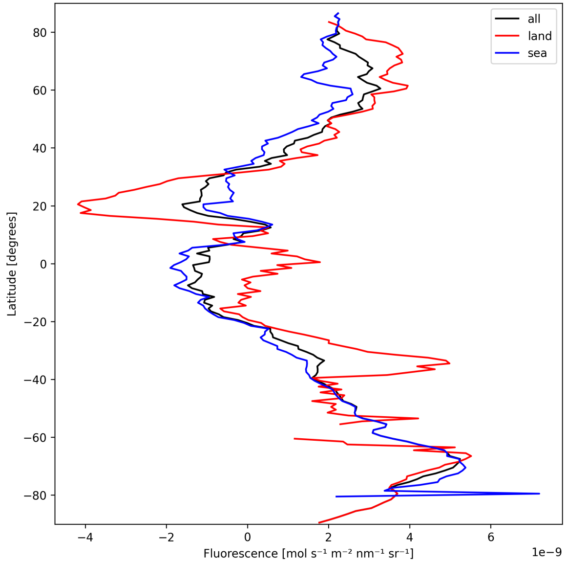
Figure 23: Zonal average of “Fluorescence” for 2025-09-26 to 2025-09-28.
