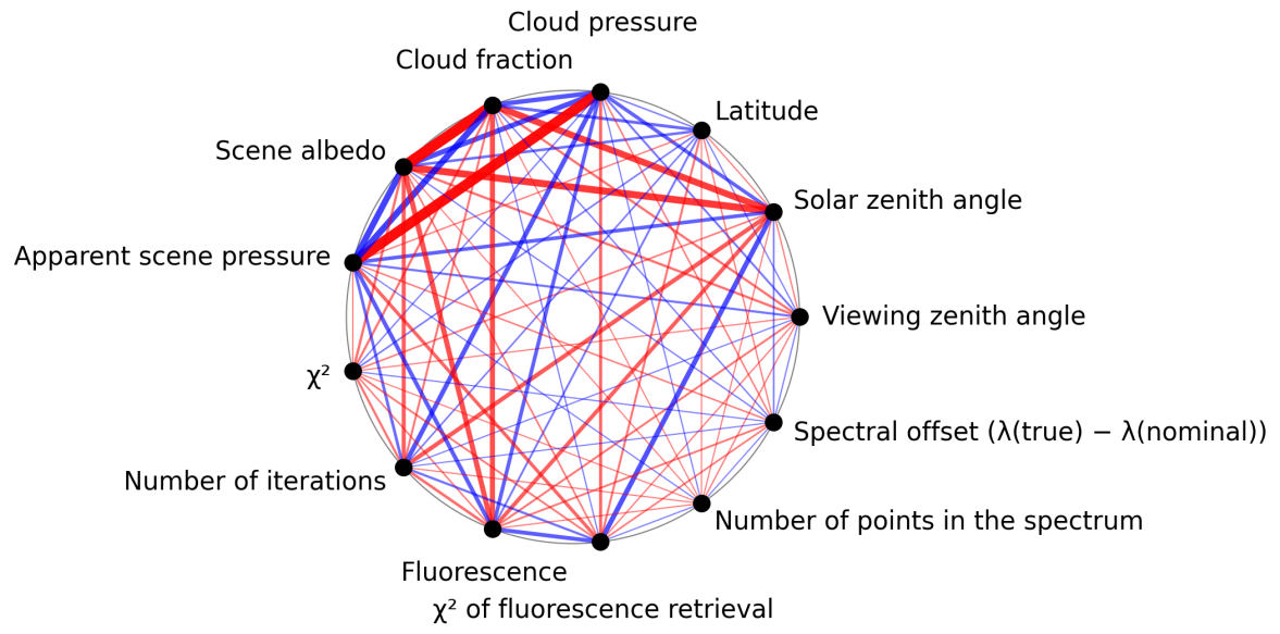
Figure 1: Map of correlation graph for 2025-09-26 to 2025-09-28.
