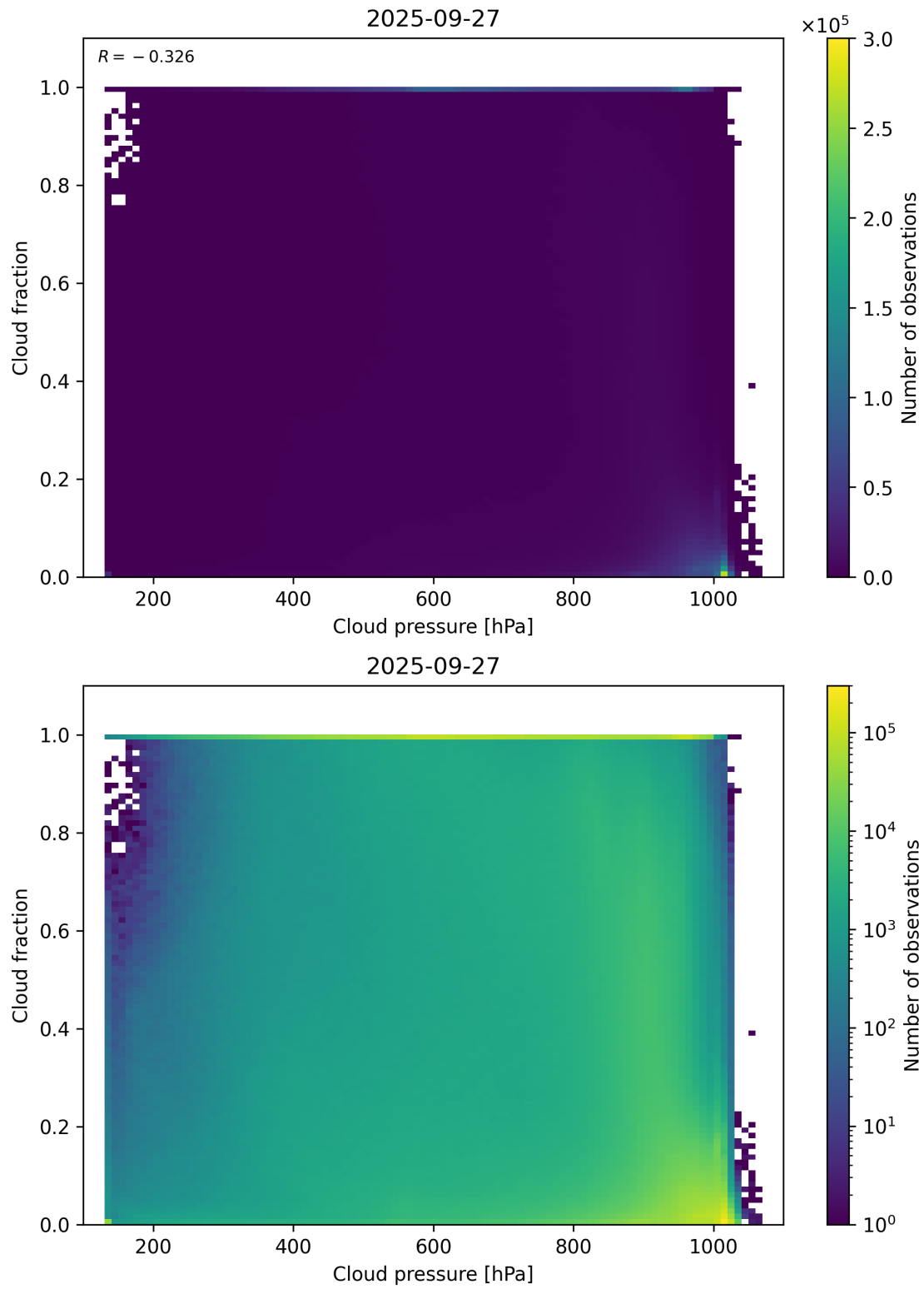
Figure 79: Scatter density plot of “Cloud pressure” against “Cloud fraction” for 2025-09-26 to 2025-09-28.
