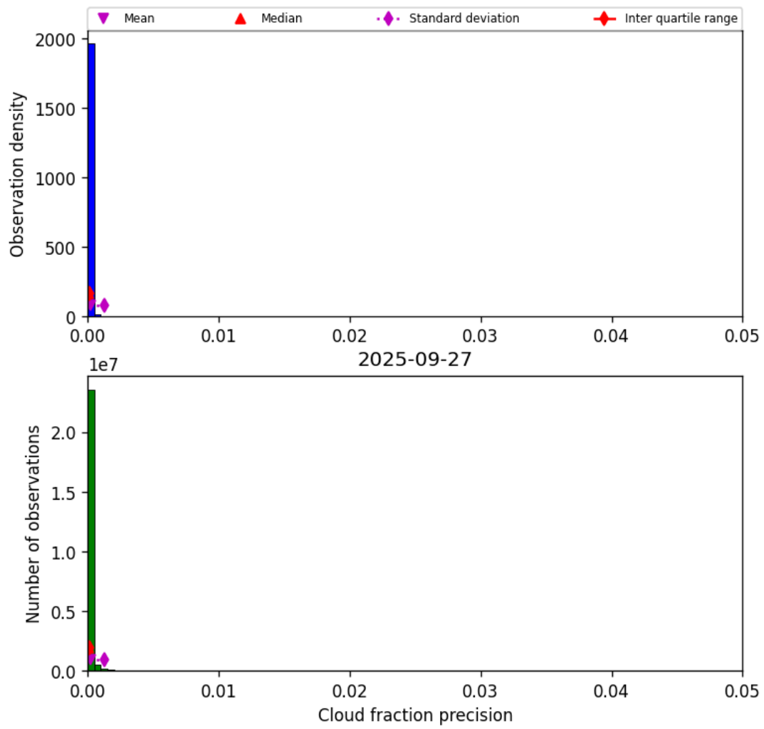
Figure 33: Histogram of “Cloud fraction precision” for 2025-09-26 to 2025-09-28
