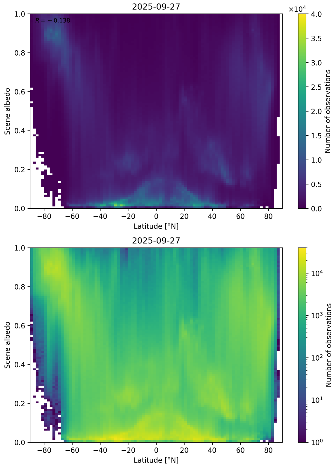
Figure 95: Scatter density plot of “Latitude” against “Scene albedo” for 2025-09-26 to 2025-09-28.
