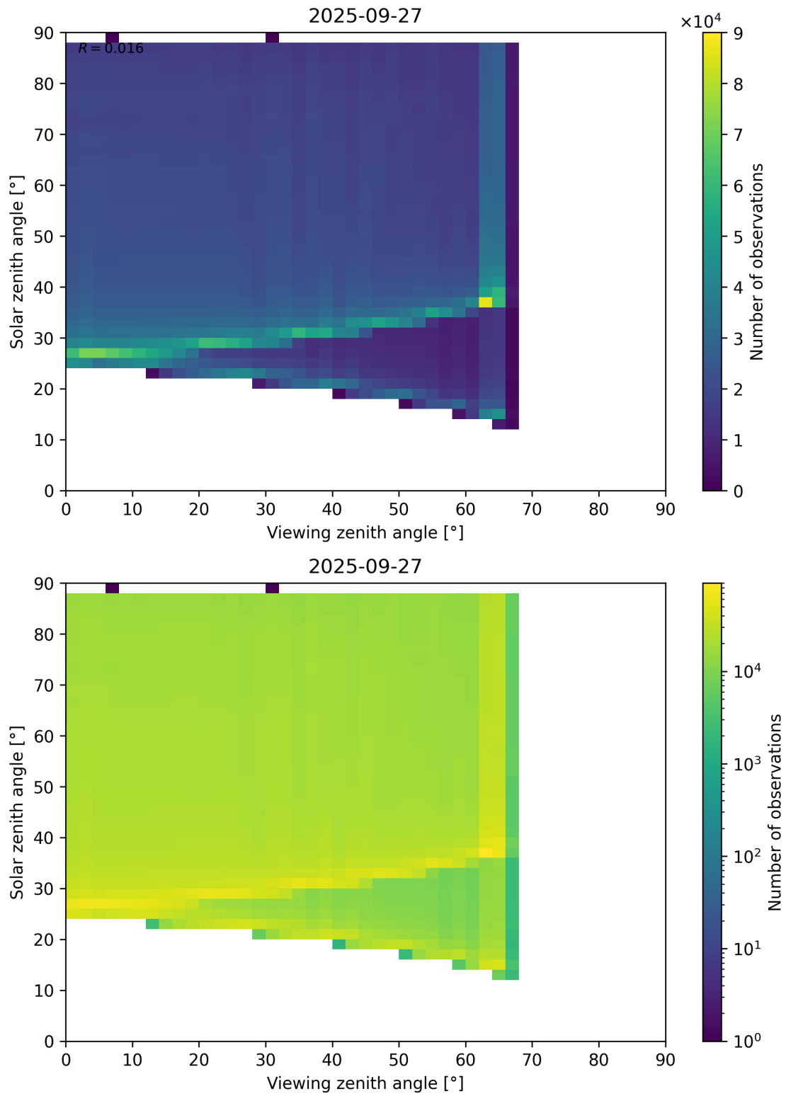
Figure 127: Scatter density plot of “Viewing zenith angle” against “Solar zenith angle” for 2025-09-26 to 2025-09-28.
