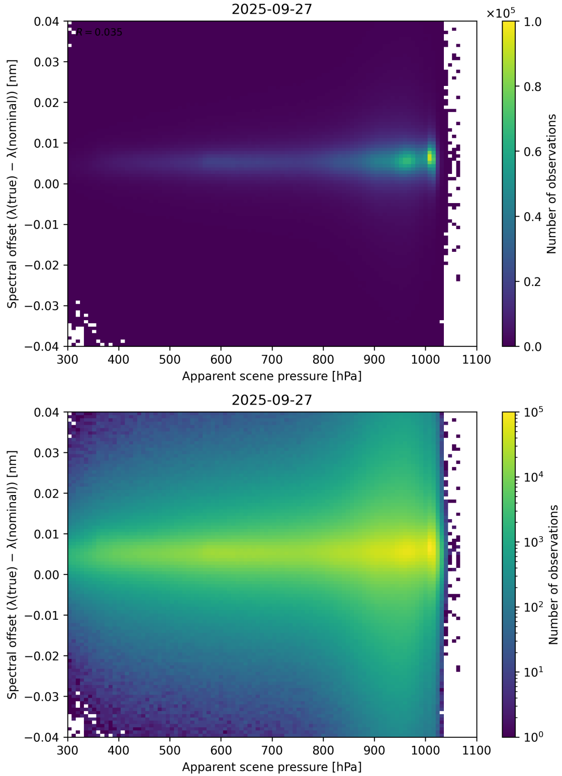
Figure 67: Scatter density plot of “Apparent scene pressure” against “Spectral offset ( \lambda_{\text{true}} - \lambda_{\text{nominal}} )” for 2025-09-26 to 2025-09-28.
