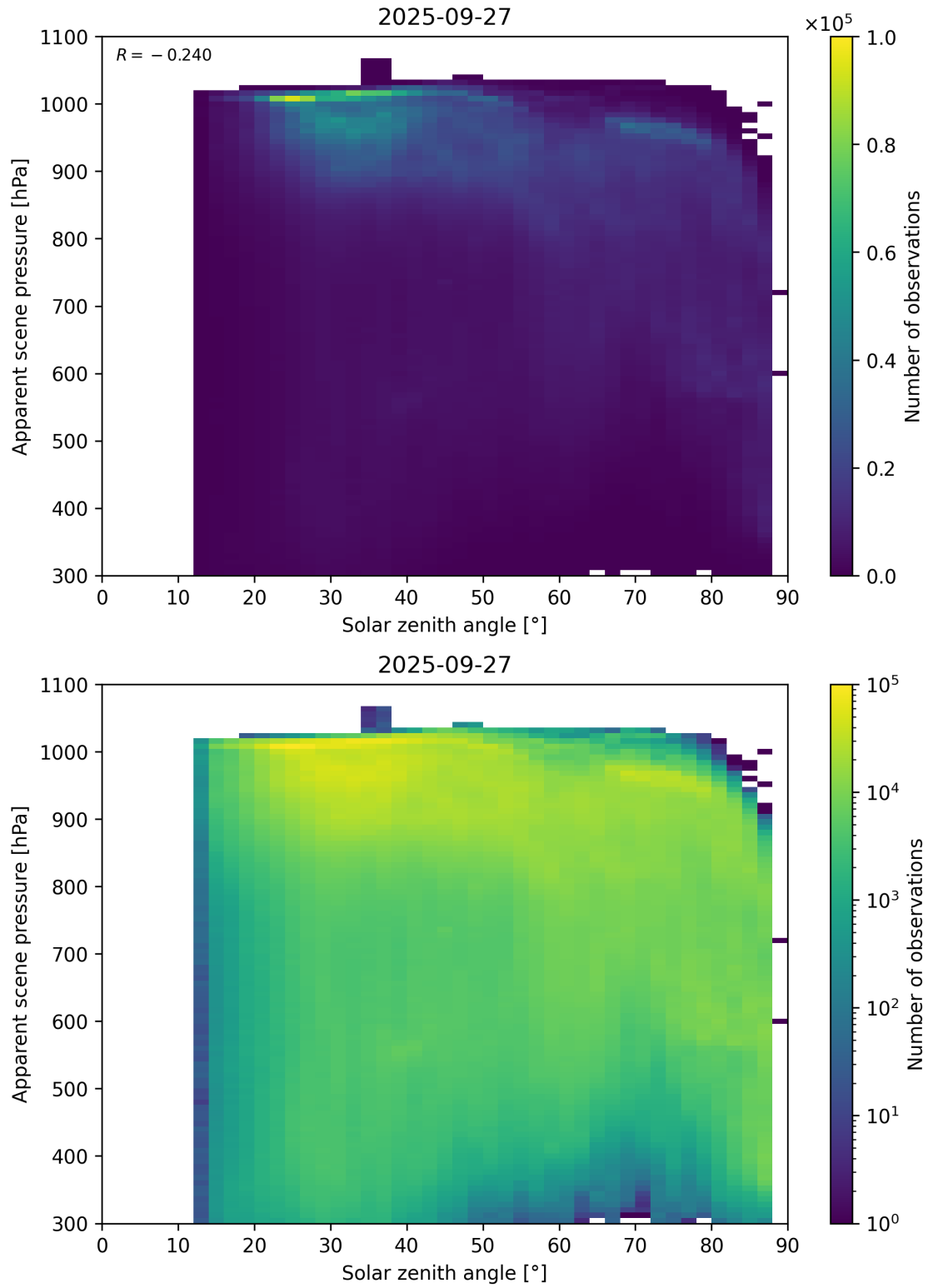
Figure 108: Scatter density plot of “Solar zenith angle” against “Apparent scene pressure” for 2025-09-26 to 2025-09-28.
