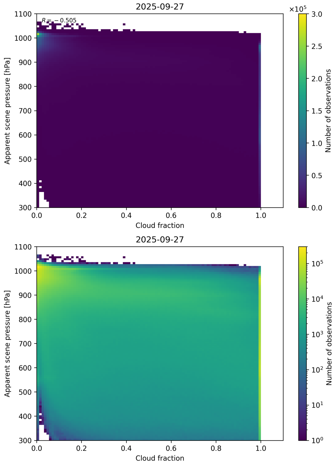
Figure 70: Scatter density plot of “Cloud fraction” against “Apparent scene pressure” for 2025-09-26 to 2025-09-28.
