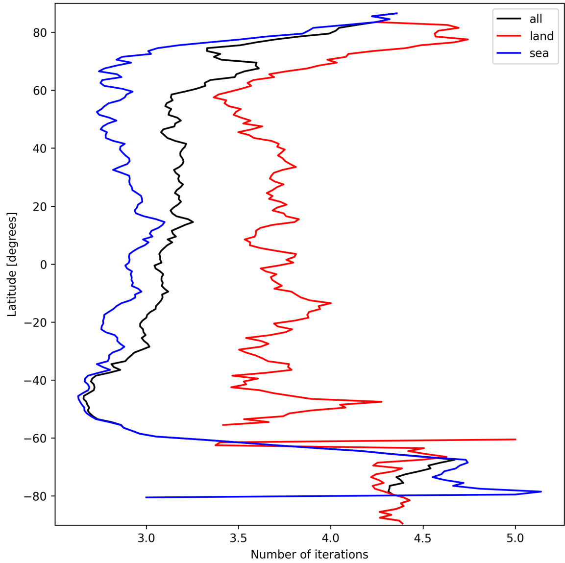
Figure 22: Zonal average of “Number of iterations” for 2025-09-26 to 2025-09-28.
