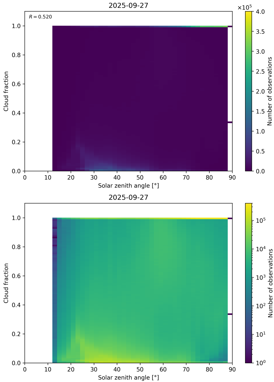
Figure 110: Scatter density plot of “Solar zenith angle” against “Cloud fraction” for 2025-09-26 to 2025-09-28.
