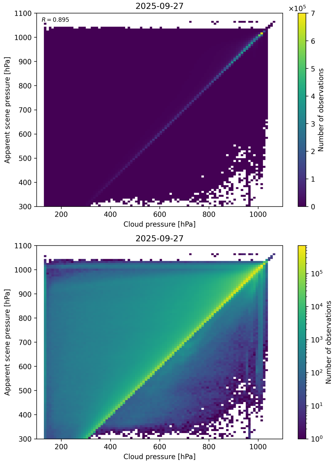
Figure 77: Scatter density plot of “Cloud pressure” against “Apparent scene pressure” for 2025-09-26 to 2025-09-28.
