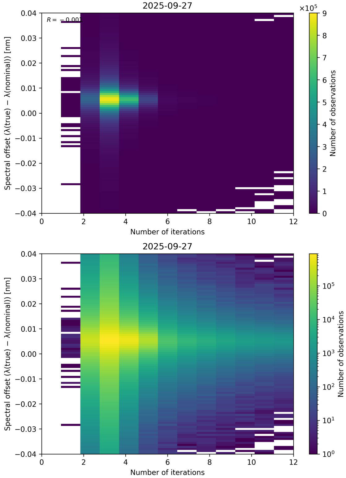
Figure 100: Scatter density plot of “Number of iterations” against “Spectral offset ( \lambda_{\text{true}} - \lambda_{\text{nominal}} )” for 2025-09-26 to 2025-09-28.
