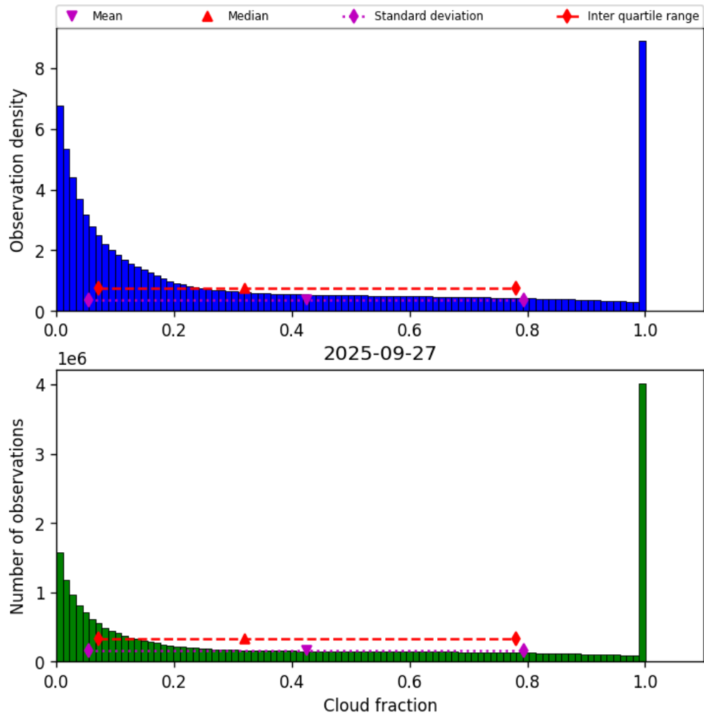
Figure 32: Histogram of “Cloud fraction” for 2025-09-26 to 2025-09-28
