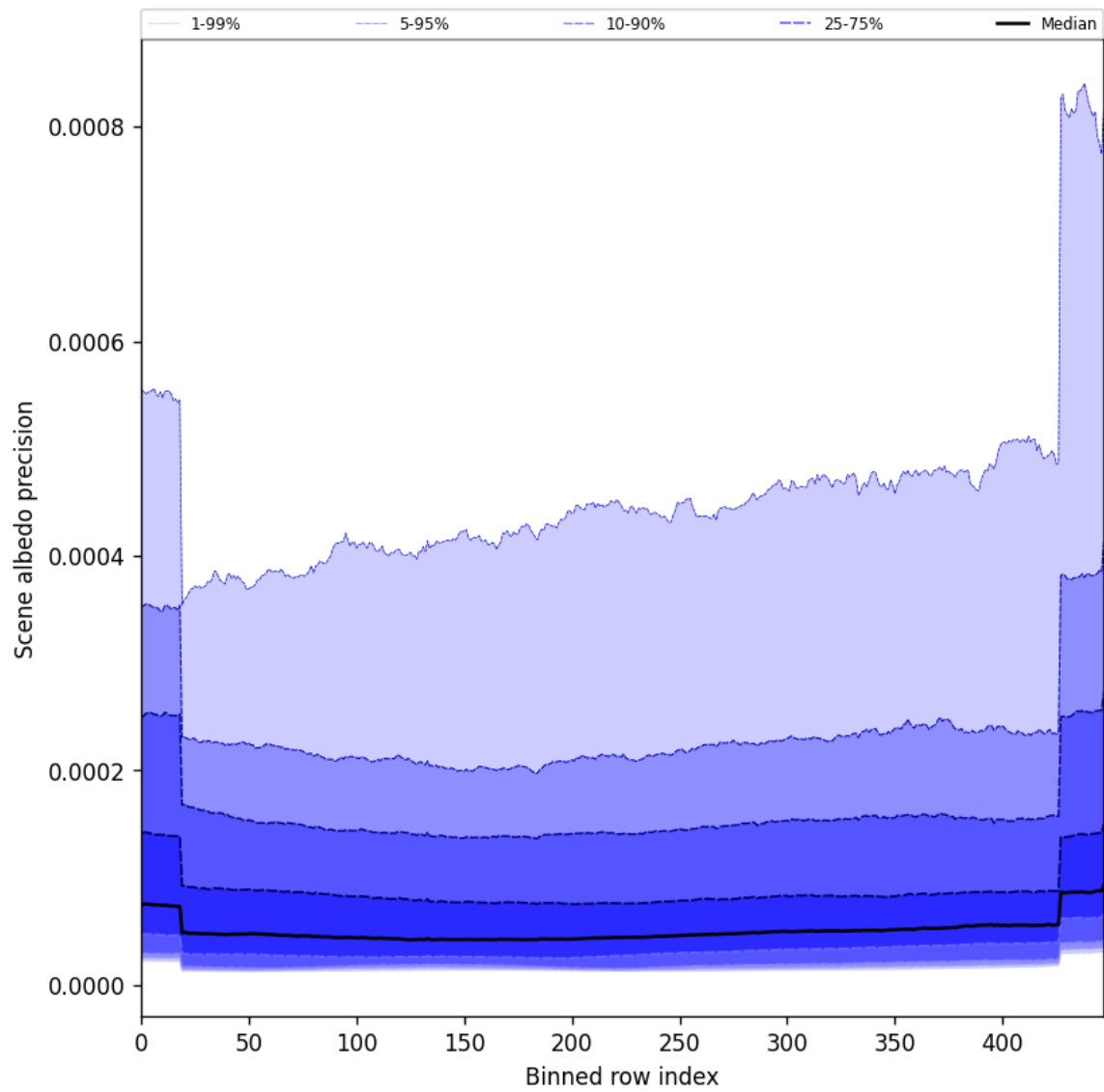
Figure 52: Along track statistics of “Scene albedo precision” for 2025-09-26 to 2025-09-28
