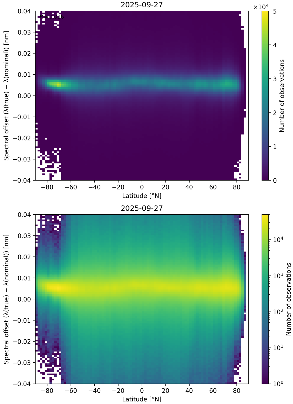
Figure 96: Scatter density plot of “Latitude” against “Spectral offset ( \lambda_{\text{true}} - \lambda_{\text{nominal}} )” for 2025-09-26 to 2025-09-28.
