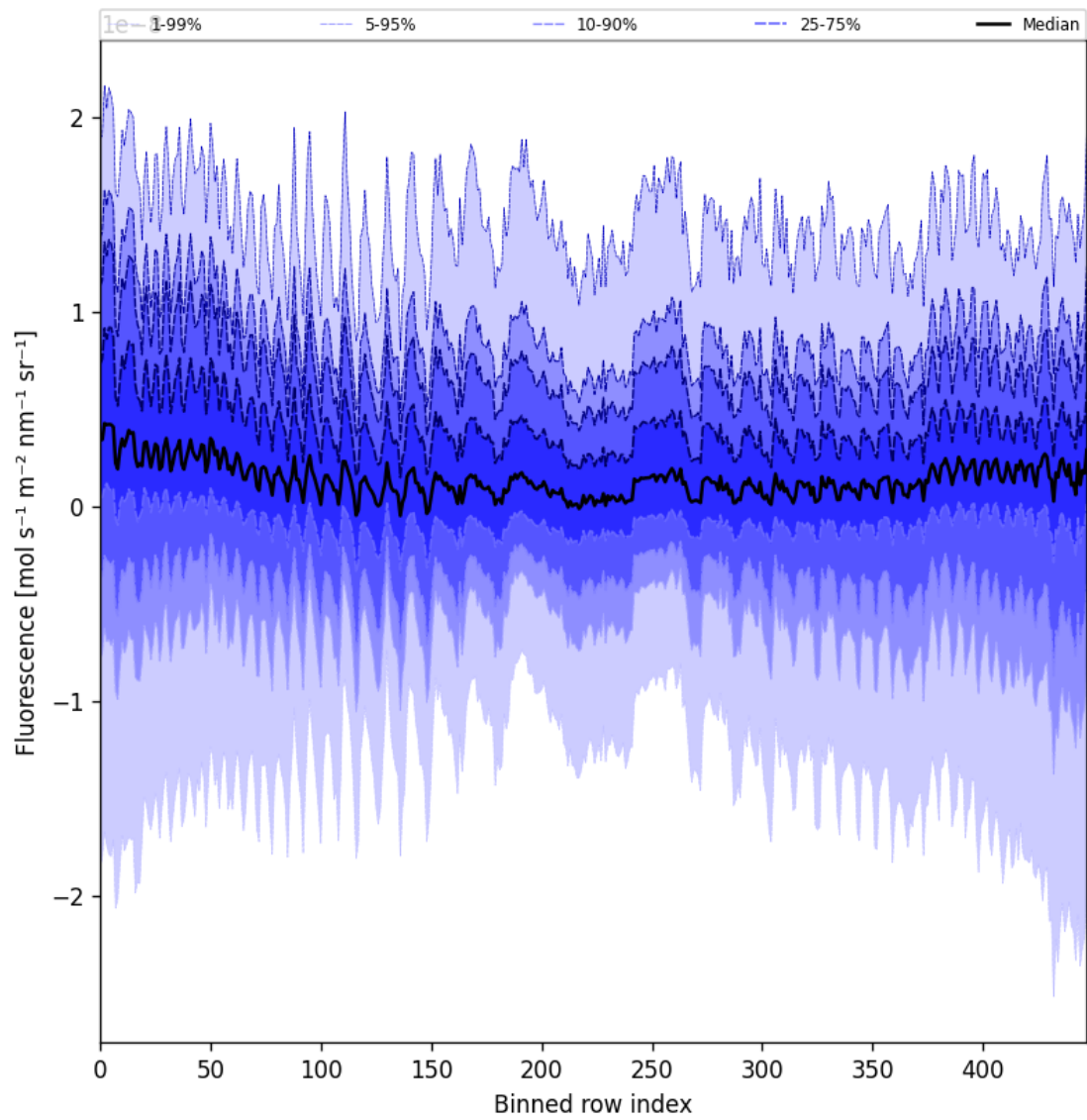
Figure 57: Along track statistics of “Fluorescence” for 2025-09-26 to 2025-09-28
