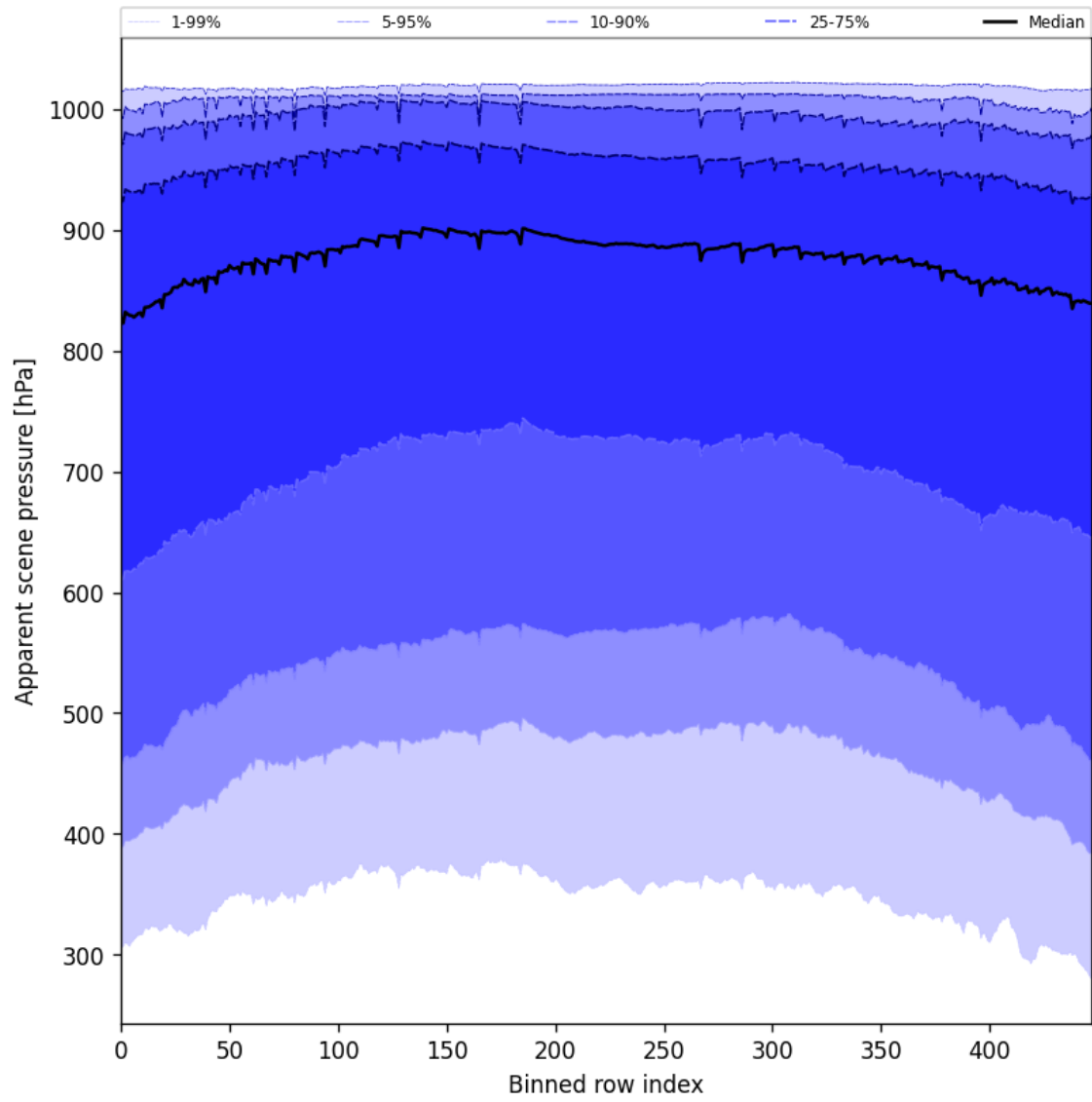
Figure 53: Along track statistics of “Apparent scene pressure” for 2025-09-26 to 2025-09-28
