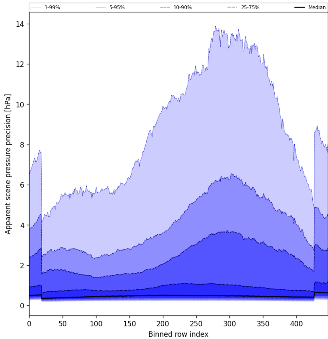
Figure 54: Along track statistics of “Apparent scene pressure precision” for 2025-09-26 to 2025-09-28
