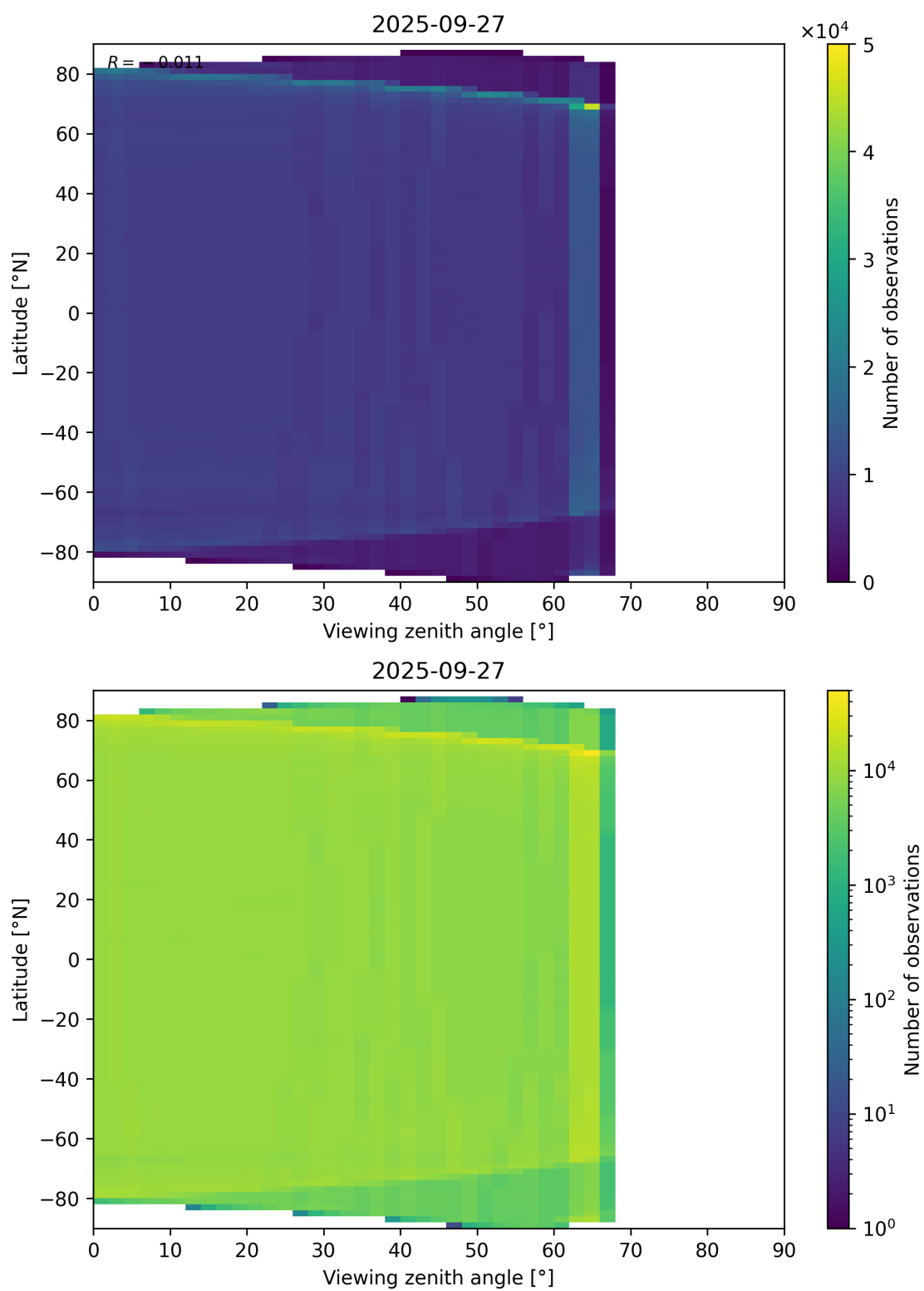
Figure 123: Scatter density plot of “Viewing zenith angle” against “Latitude” for 2025-09-26 to 2025-09-28.
