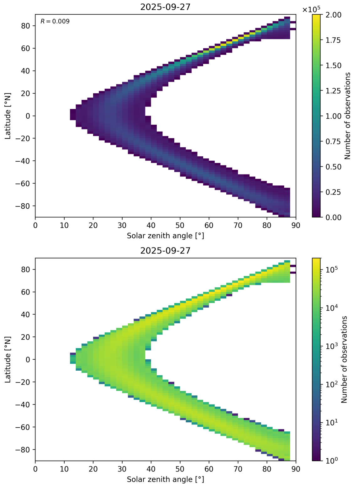
Figure 113: Scatter density plot of “Solar zenith angle” against “Latitude” for 2025-09-26 to 2025-09-28.
