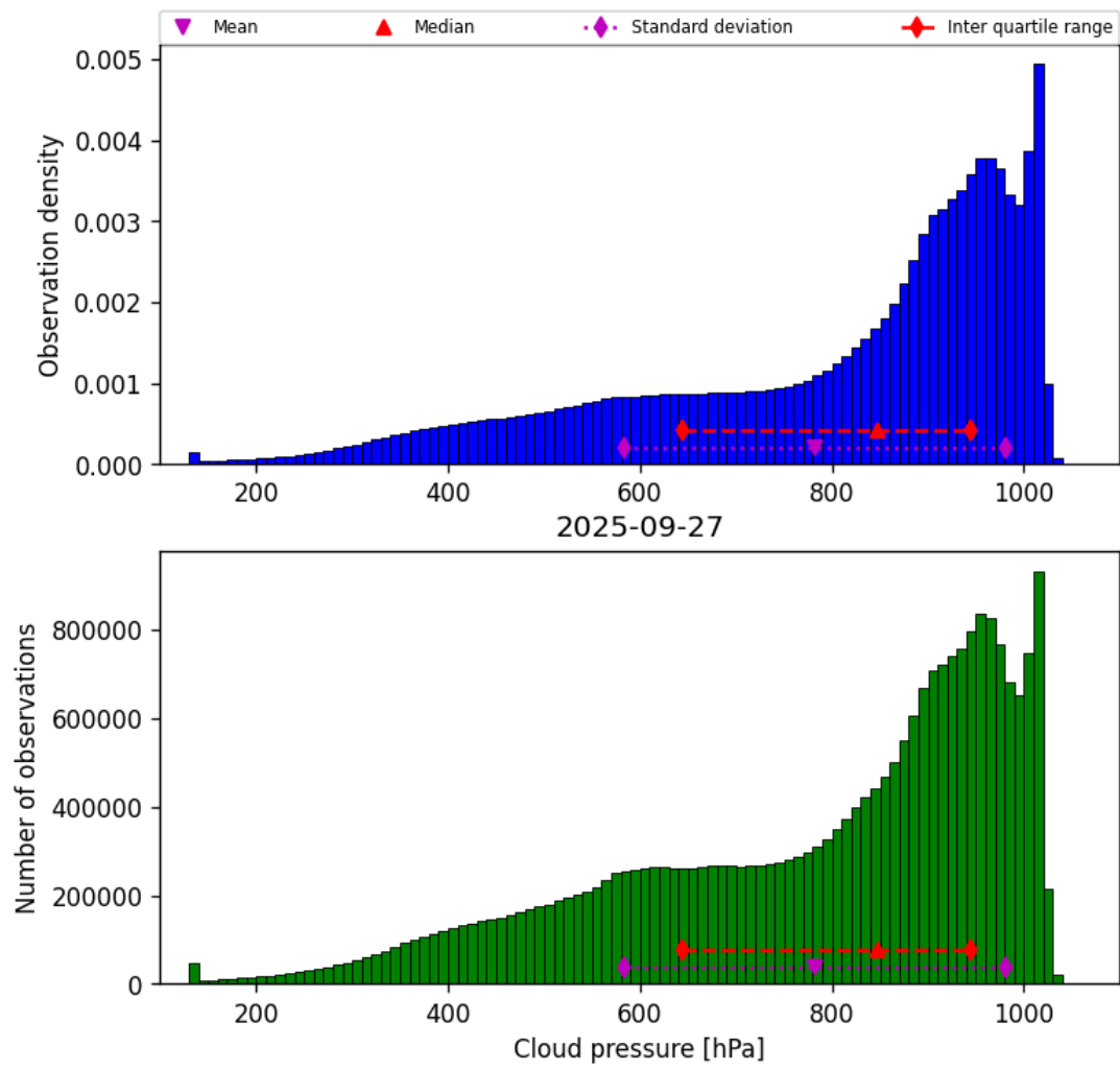
Figure 30: Histogram of “Cloud pressure” for 2025-09-26 to 2025-09-28
