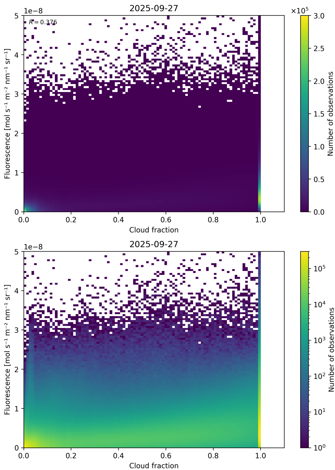
Figure 72: Scatter density plot of “Cloud fraction” against “Fluorescence” for 2025-09-26 to 2025-09-28.
