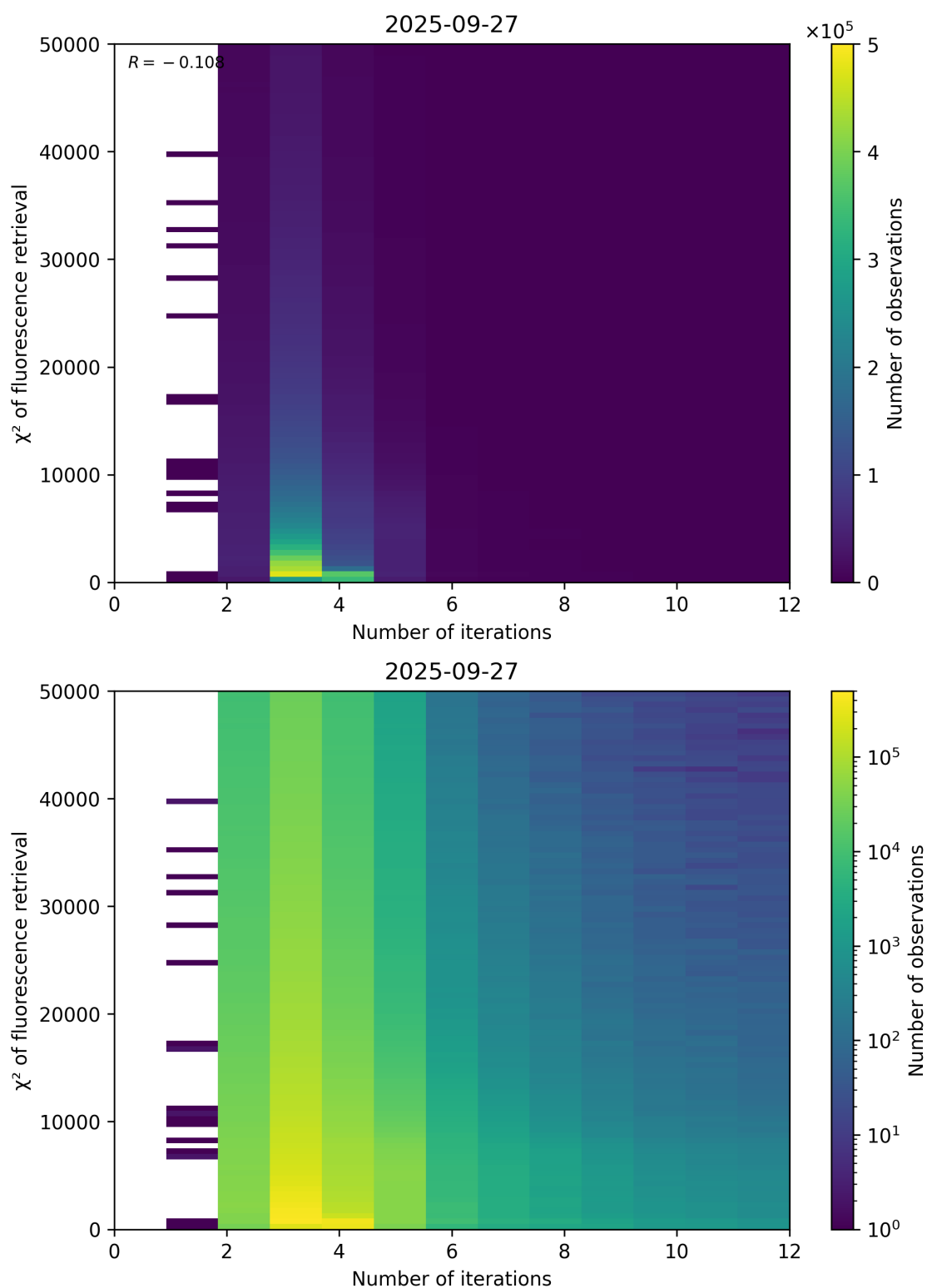
Figure 97: Scatter density plot of “Number of iterations” against “ \chi^2 of fluorescence retrieval” for 2025-09-26 to 2025-09-28.
