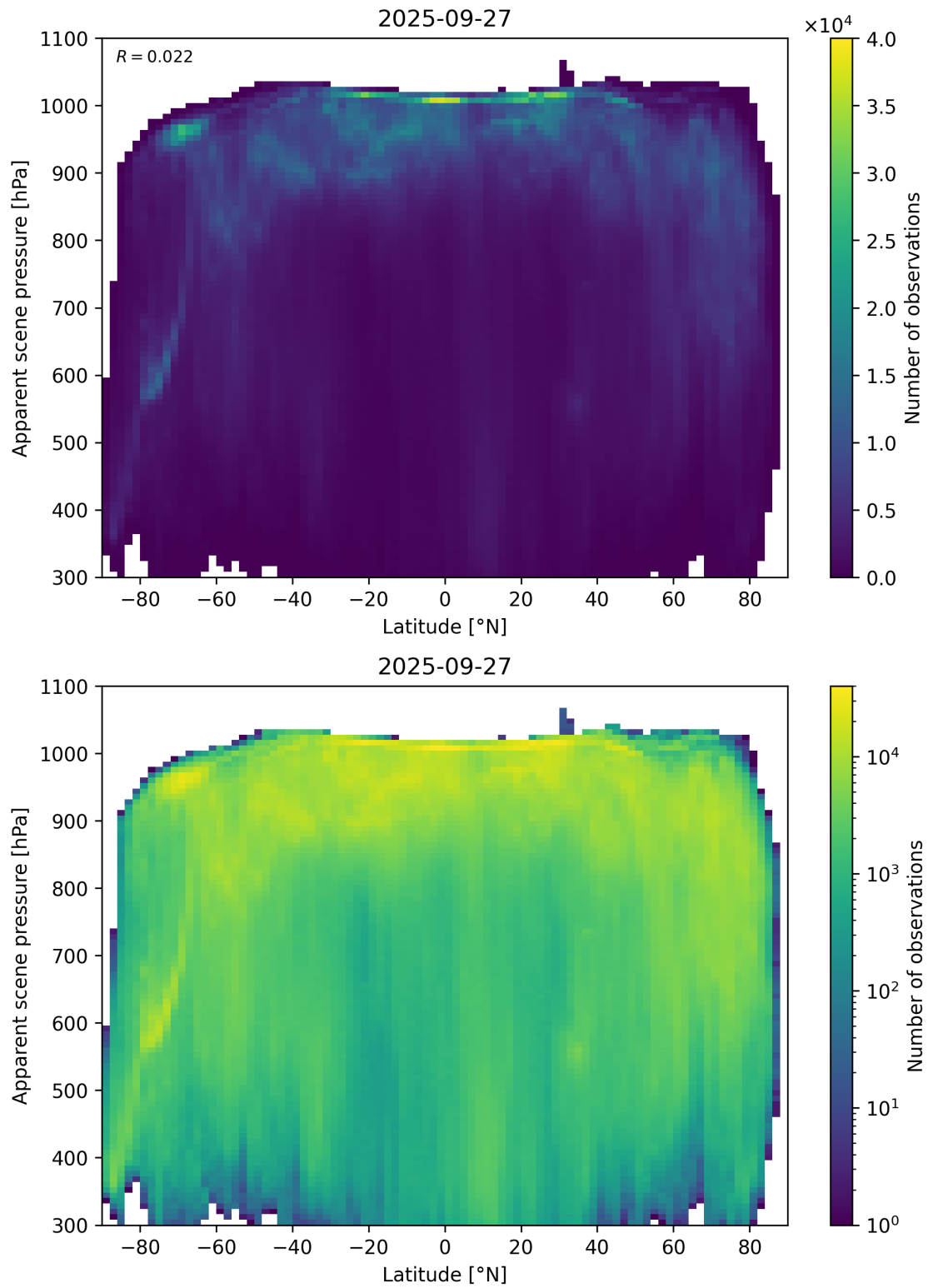
Figure 88: Scatter density plot of “Latitude” against “Apparent scene pressure” for 2025-09-26 to 2025-09-28.
