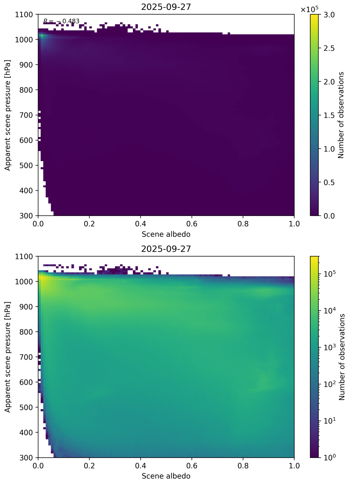
Figure 102: Scatter density plot of “Scene albedo” against “Apparent scene pressure” for 2025-09-26 to 2025-09-28.
