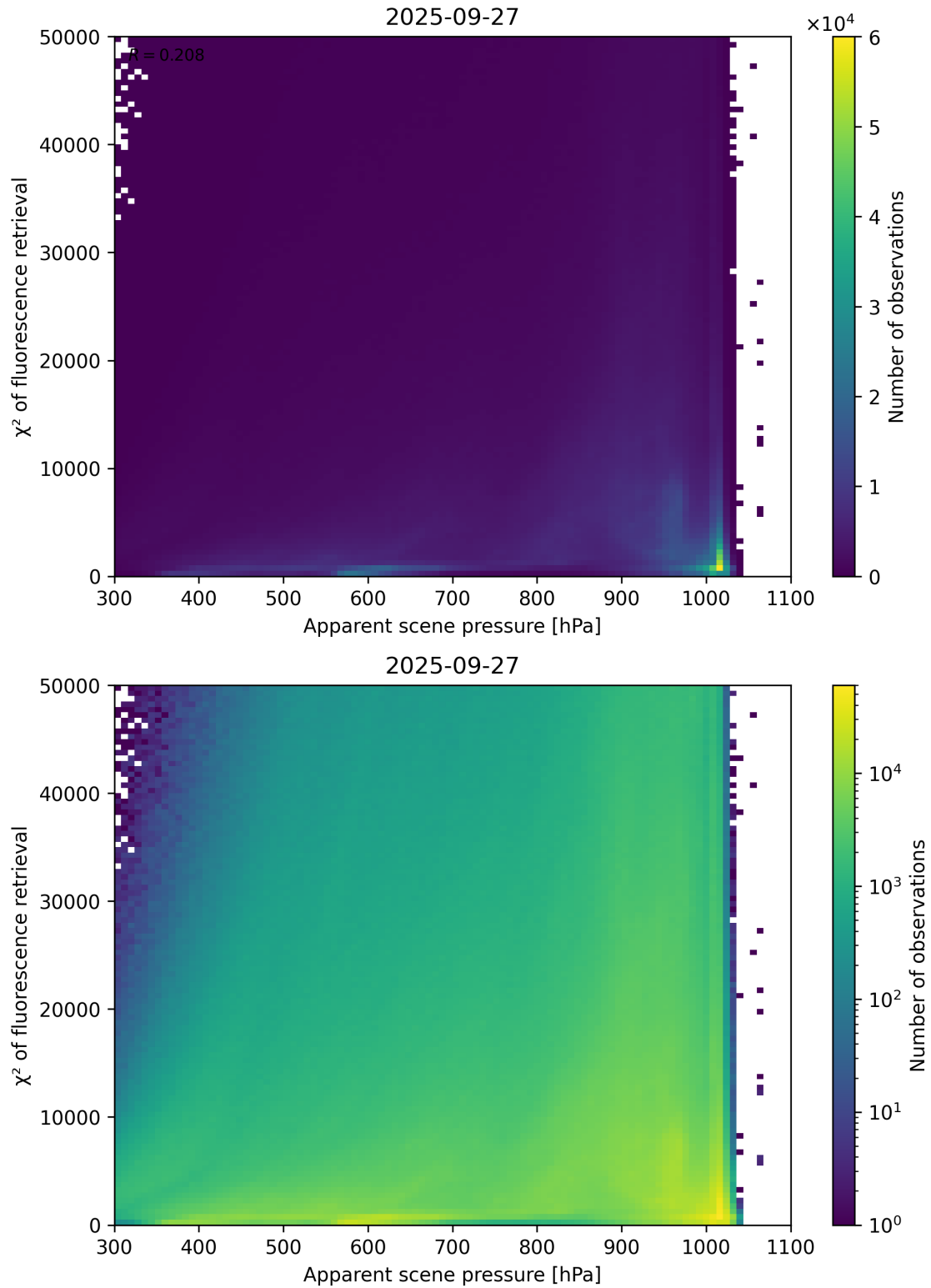
Figure 63: Scatter density plot of “Apparent scene pressure” against “ \chi^2 of fluorescence retrieval” for 2025-09-26 to 2025-09-28.
