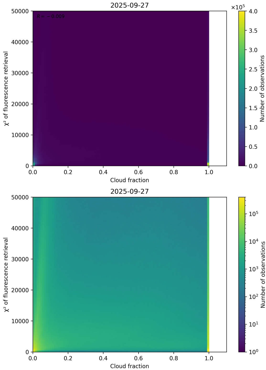
Figure 71: Scatter density plot of “Cloud fraction” against “ \chi^2 of fluorescence retrieval” for 2025-09-26 to 2025-09-28.
