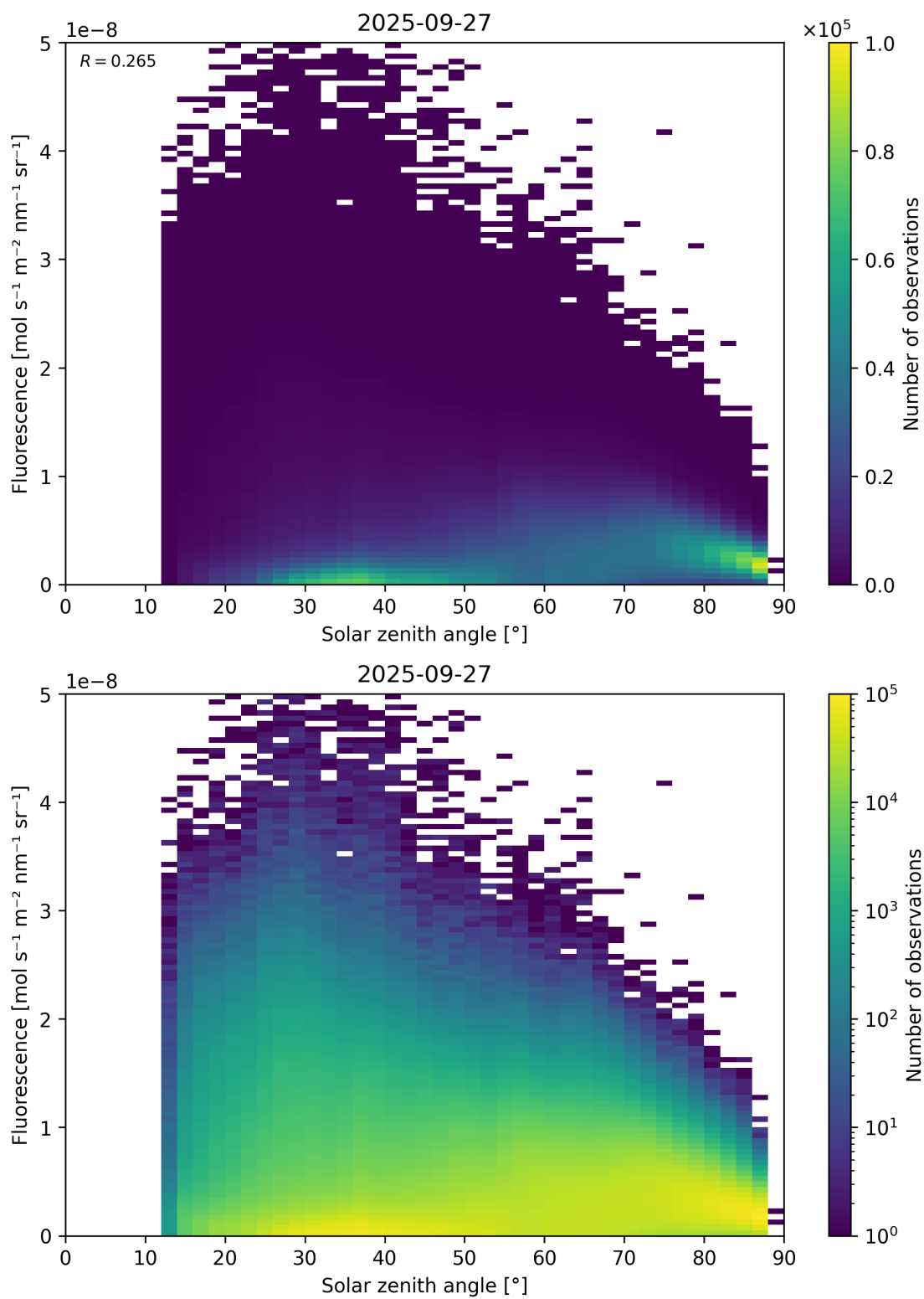
Figure 112: Scatter density plot of “Solar zenith angle” against “Fluorescence” for 2025-09-26 to 2025-09-28.
