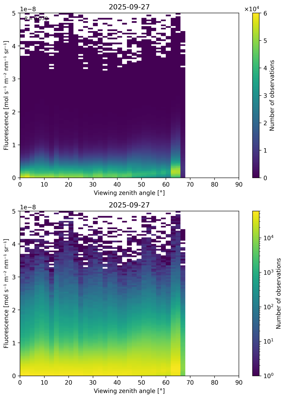
Figure 122: Scatter density plot of “Viewing zenith angle” against “Fluorescence” for 2025-09-26 to 2025-09-28.
