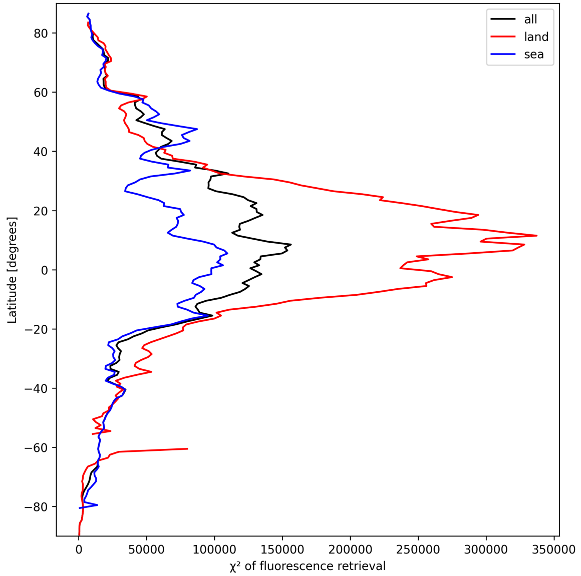
Figure 25: Zonal average of “ \chi^2 of fluorescence retrieval” for 2025-09-26 to 2025-09-28.
