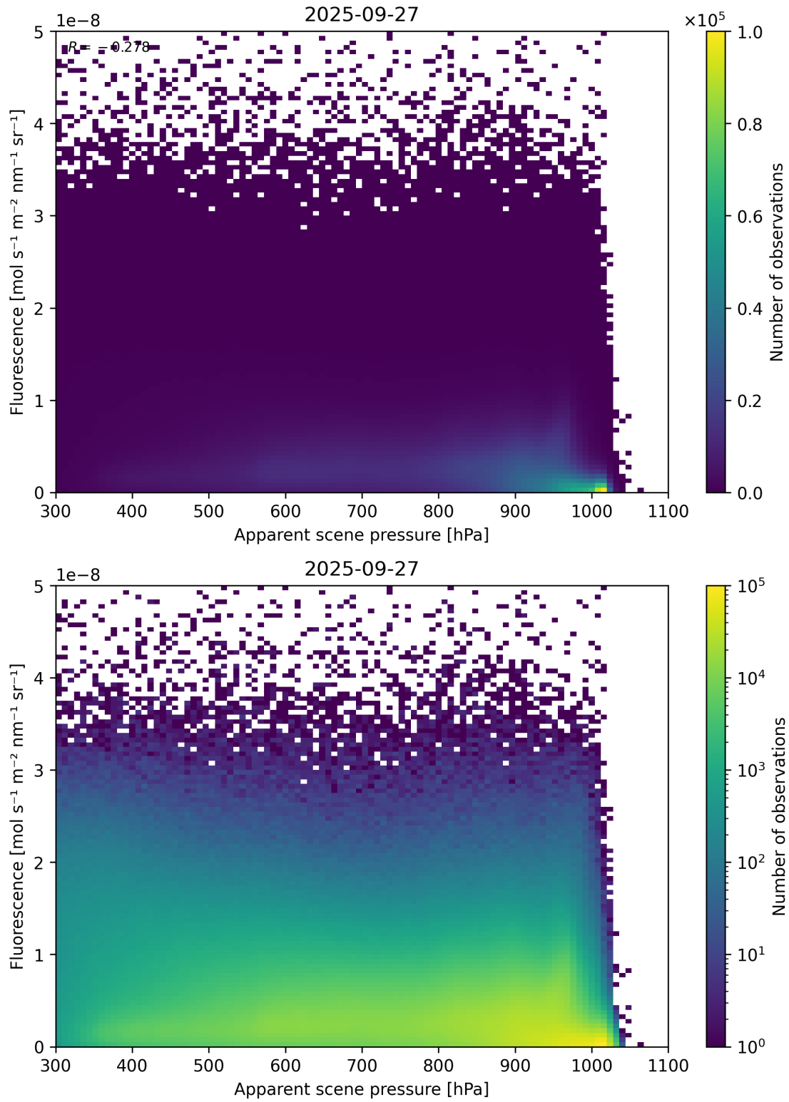
Figure 64: Scatter density plot of “Apparent scene pressure” against “Fluorescence” for 2025-09-26 to 2025-09-28.
