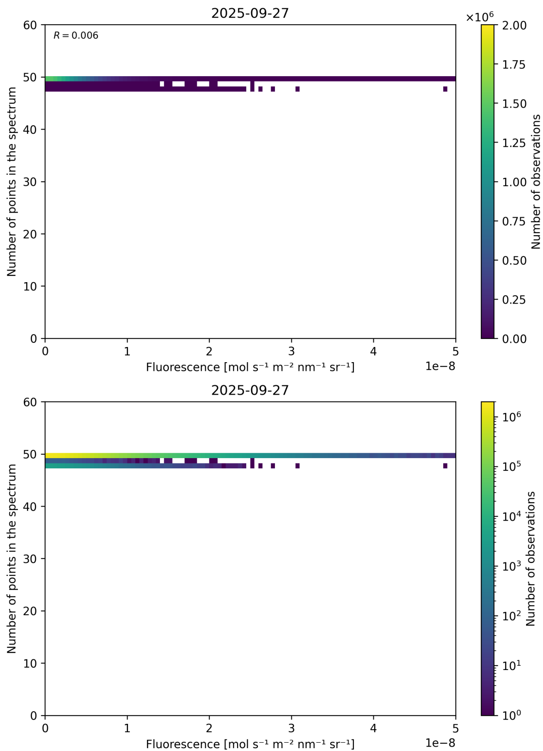
Figure 86: Scatter density plot of “Fluorescence” against “Number of points in the spectrum” for 2025-09-26 to 2025-09-28.
