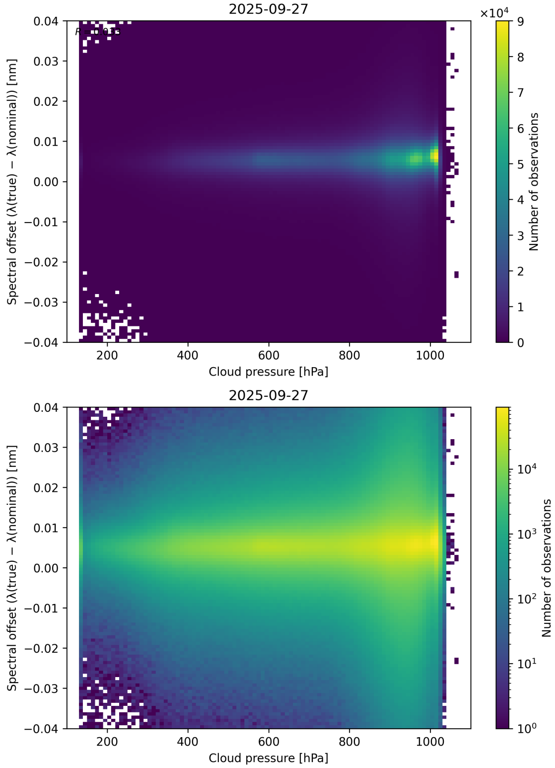
Figure 84: Scatter density plot of “Cloud pressure” against “Spectral offset ( \lambda_{\text{true}} - \lambda_{\text{nominal}} )” for 2025-09-26 to 2025-09-28.
