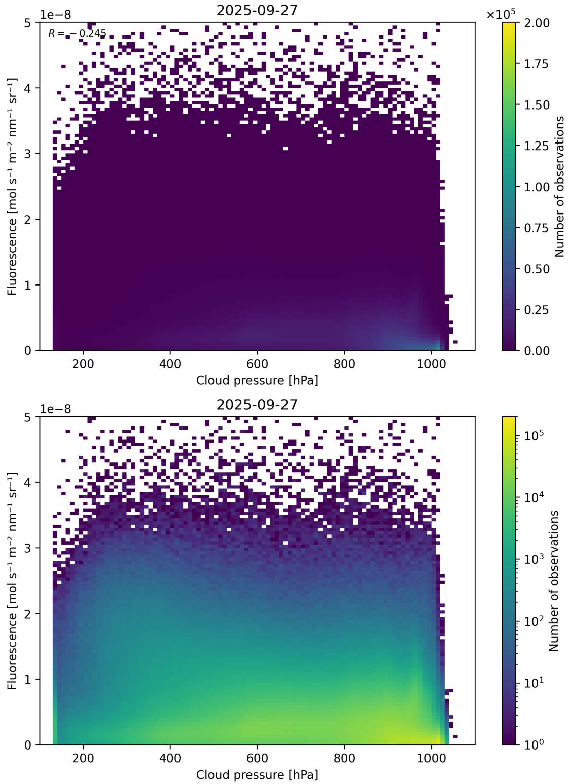
Figure 80: Scatter density plot of “Cloud pressure” against “Fluorescence” for 2025-09-26 to 2025-09-28.
