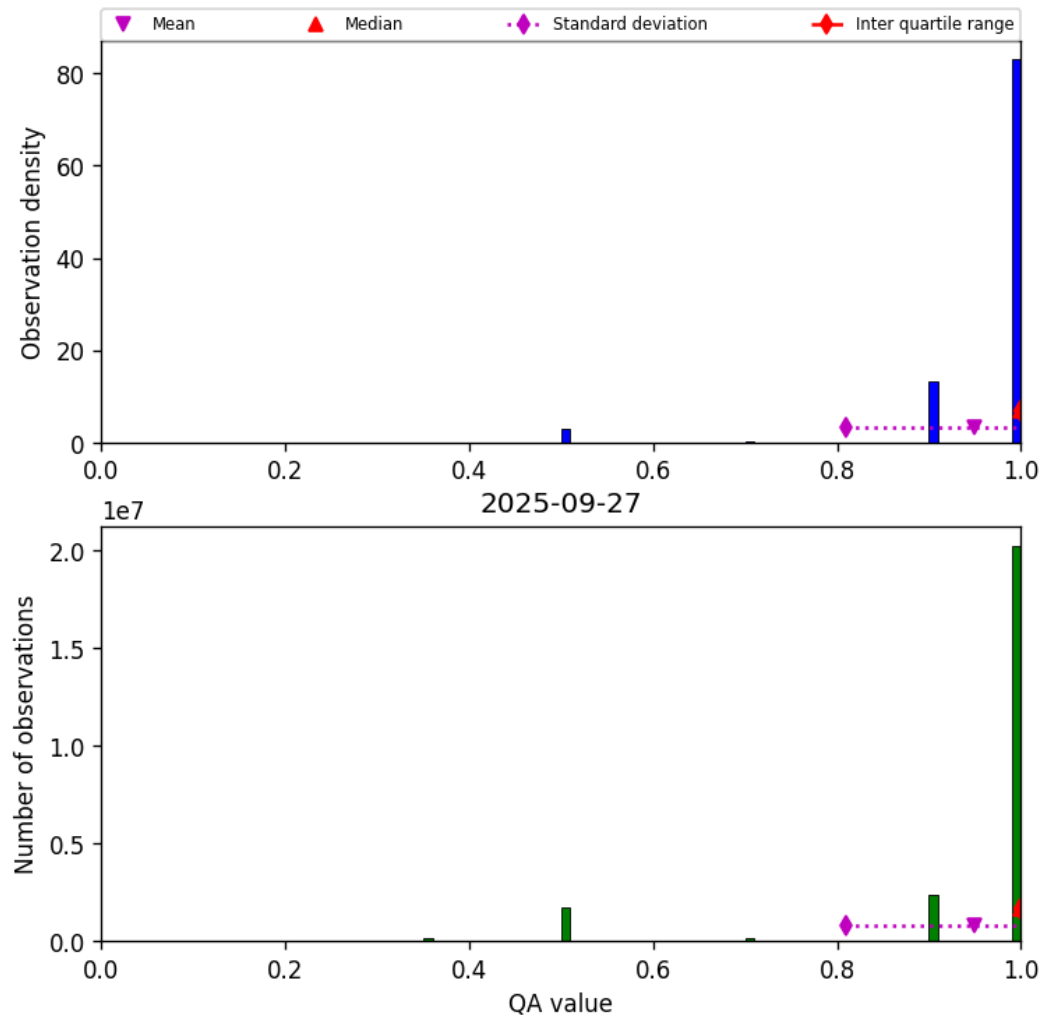
Figure 29: Histogram of “QA value” for 2025-09-26 to 2025-09-28
