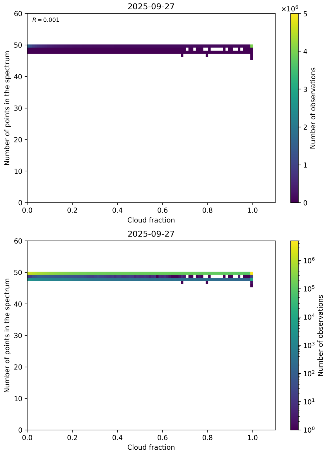
Figure 74: Scatter density plot of “Cloud fraction” against “Number of points in the spectrum” for 2025-09-26 to 2025-09-28.
