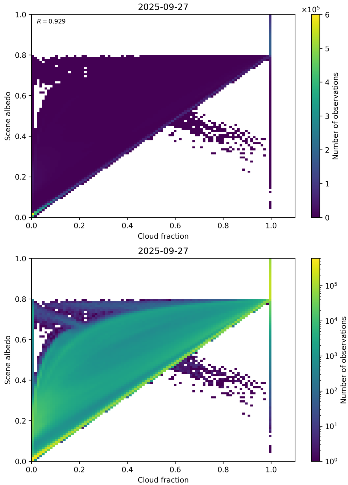
Figure 75: Scatter density plot of “Cloud fraction” against “Scene albedo” for 2025-09-26 to 2025-09-28.
