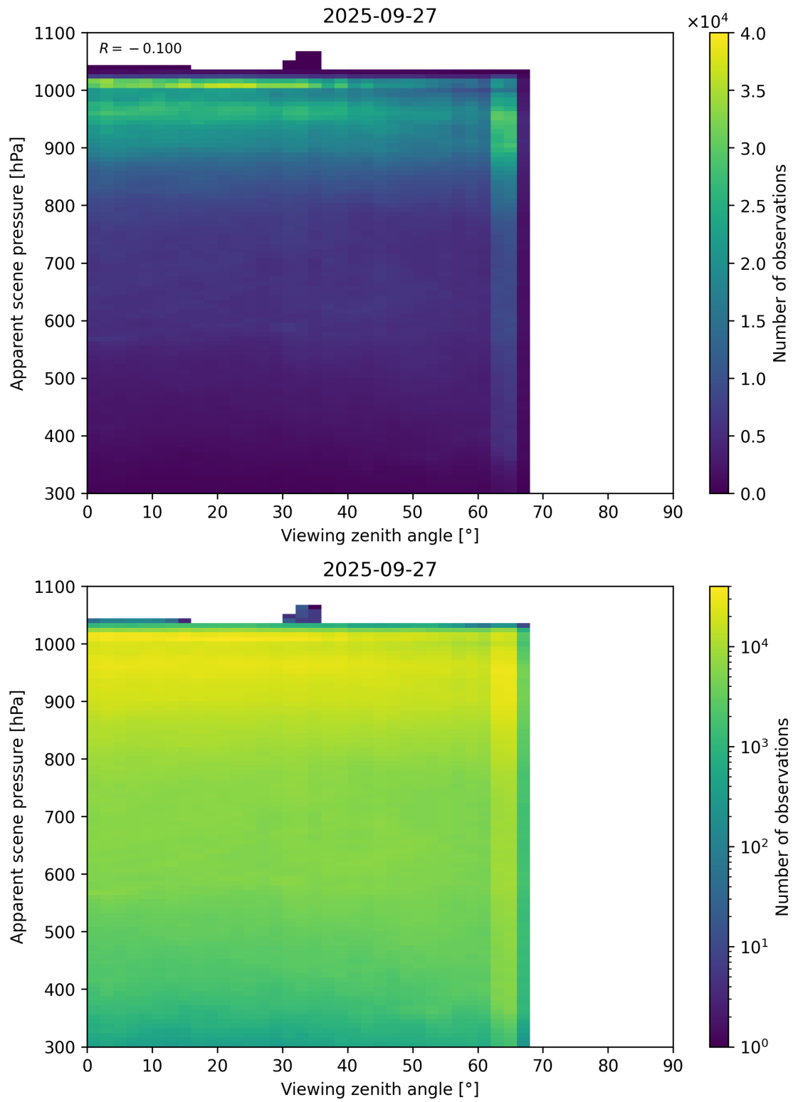
Figure 118: Scatter density plot of “Viewing zenith angle” against “Apparent scene pressure” for 2025-09-26 to 2025-09-28.
