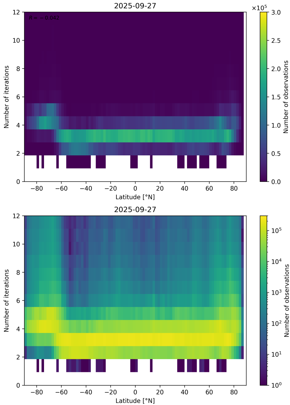
Figure 93: Scatter density plot of “Latitude” against “Number of iterations” for 2025-09-26 to 2025-09-28.
