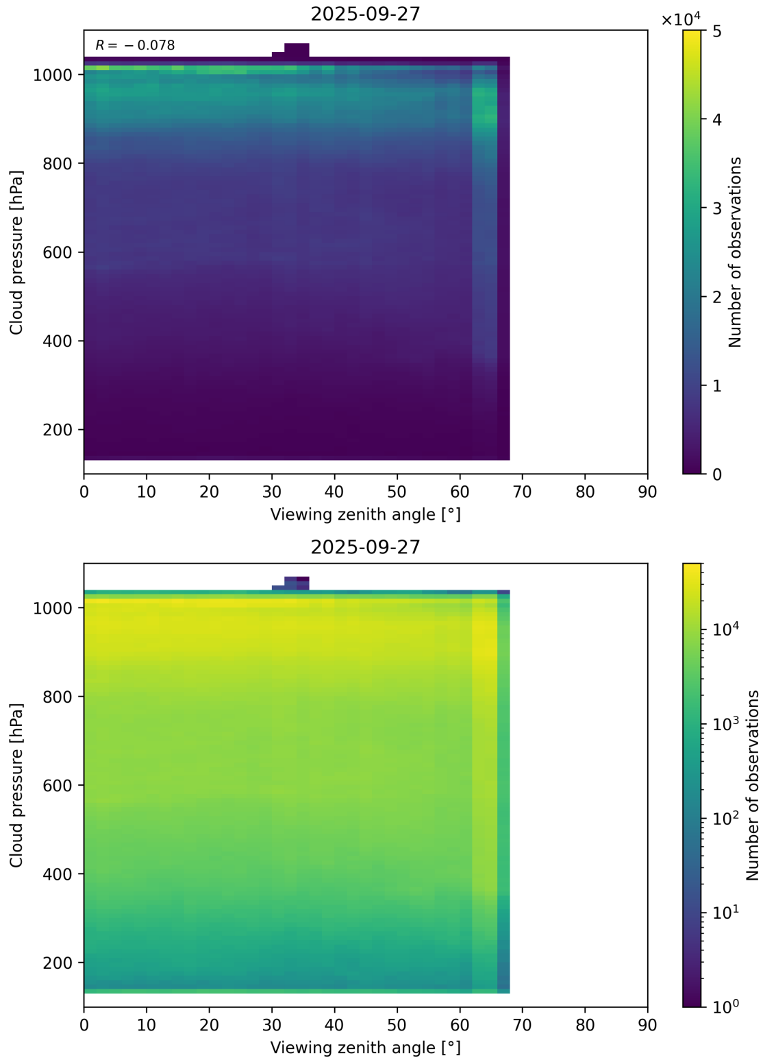
Figure 121: Scatter density plot of “Viewing zenith angle” against “Cloud pressure” for 2025-09-26 to 2025-09-28.
