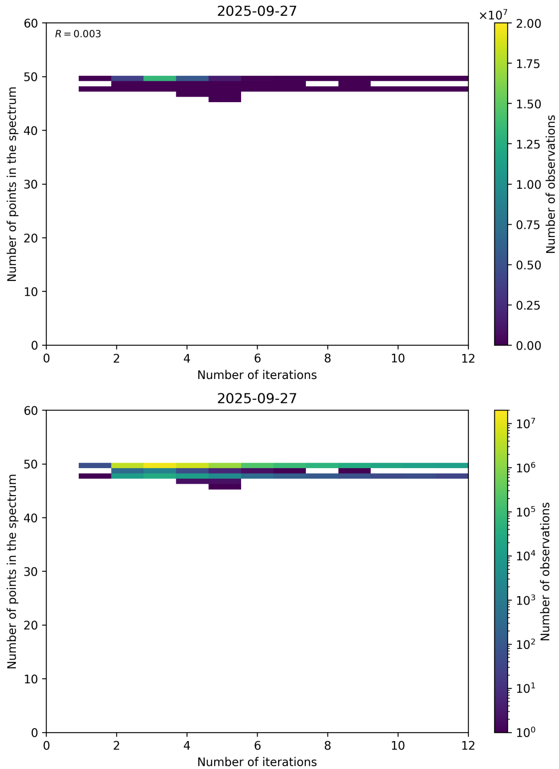
Figure 99: Scatter density plot of “Number of iterations” against “Number of points in the spectrum” for 2025-09-26 to 2025-09-28.
