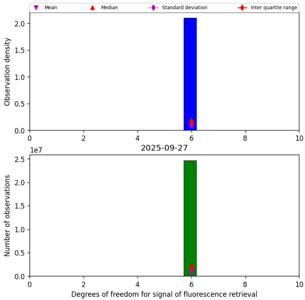
Figure 43: Histogram of “Degrees of freedom for signal of fluorescence retrieval” for 2025-09-26 to 2025-09-28
