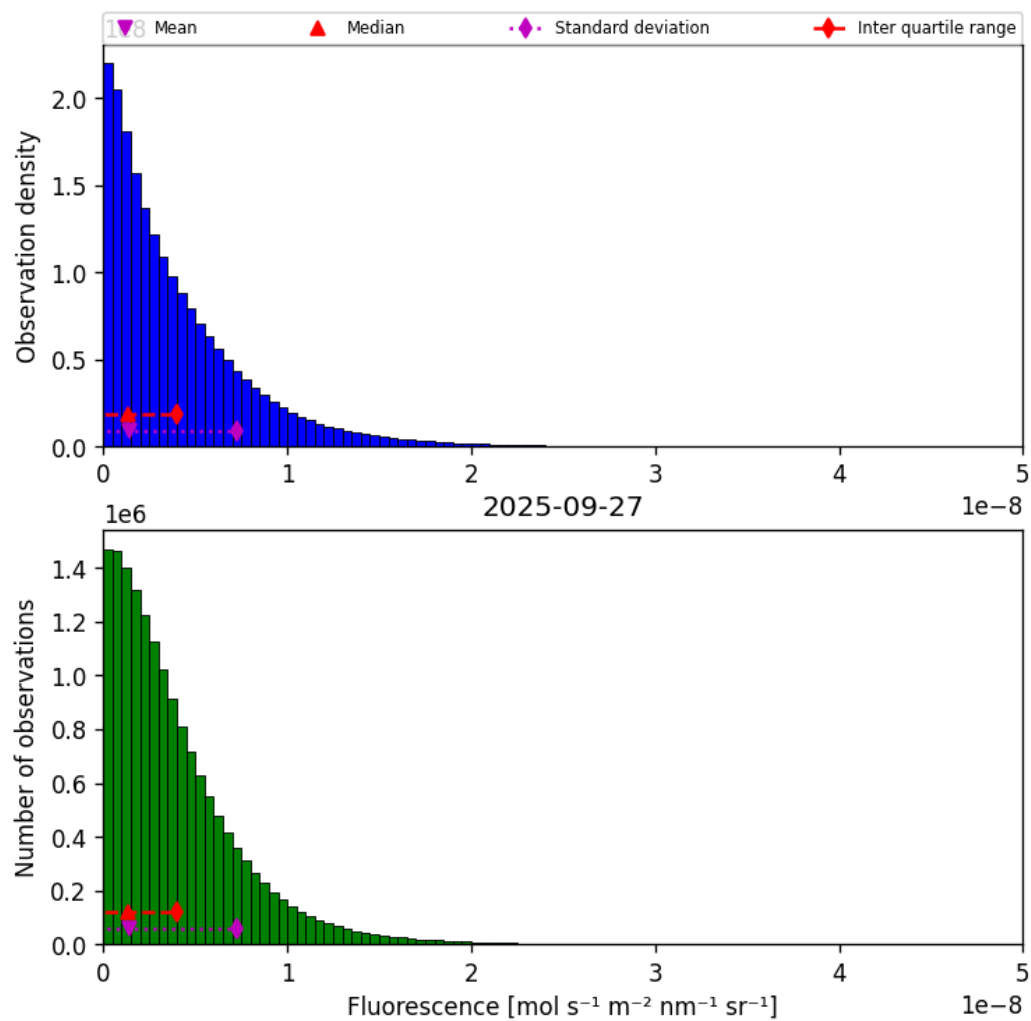
Figure 40: Histogram of “Fluorescence” for 2025-09-26 to 2025-09-28
