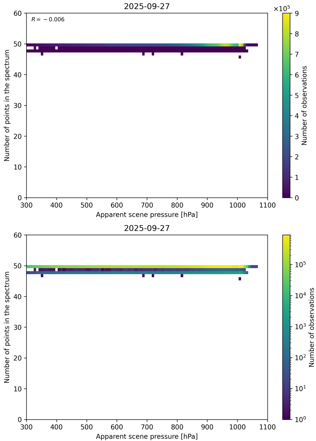
Figure 66: Scatter density plot of “Apparent scene pressure” against “Number of points in the spectrum” for 2025-09-26 to 2025-09-28.
