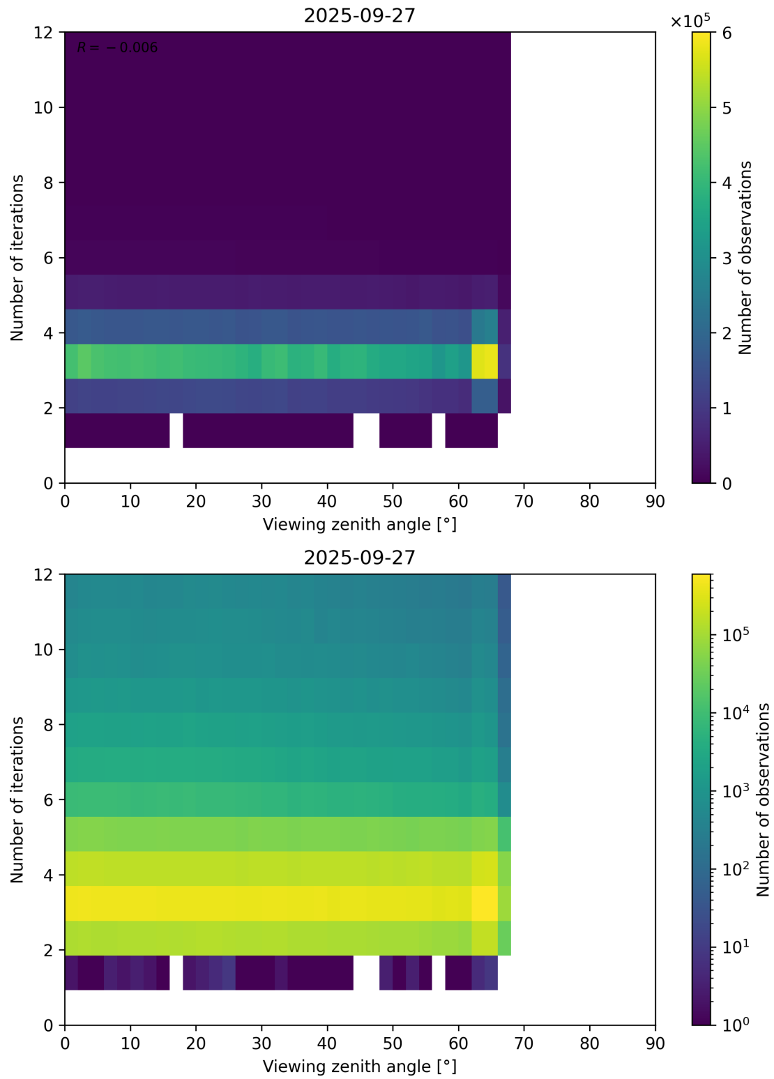
Figure 124: Scatter density plot of “Viewing zenith angle” against “Number of iterations” for 2025-09-26 to 2025-09-28.
