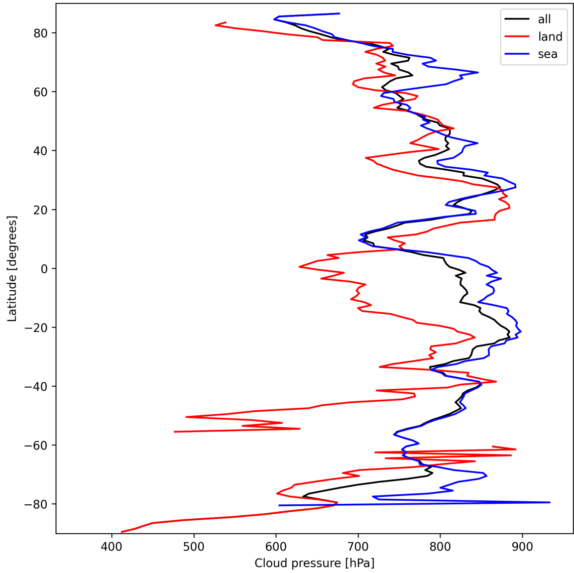
Figure 13: Zonal average of “Cloud pressure” for 2025-09-26 to 2025-09-28.
