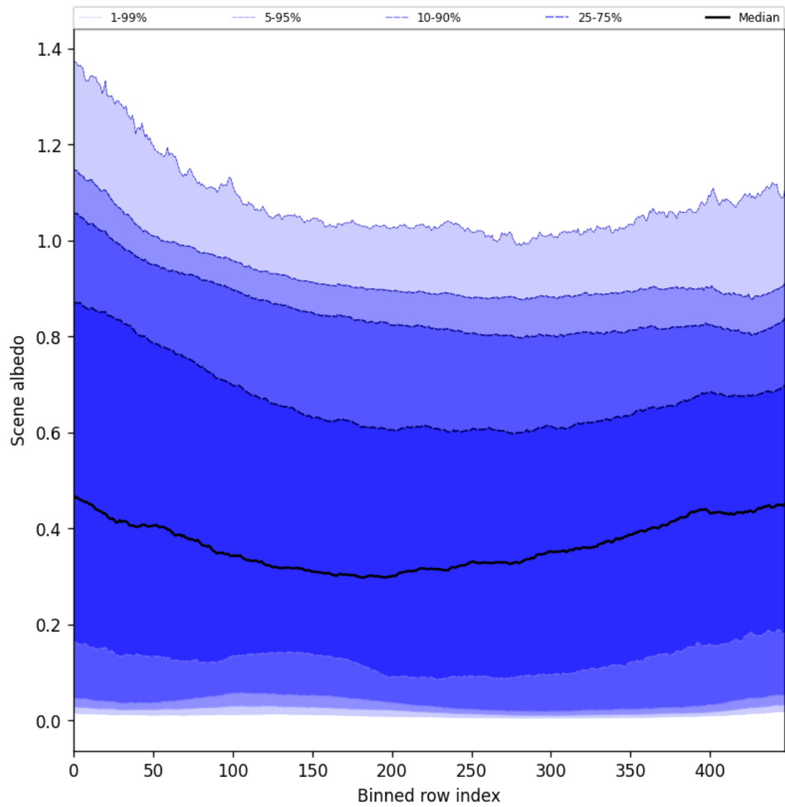
Figure 51: Along track statistics of “Scene albedo” for 2025-09-26 to 2025-09-28
