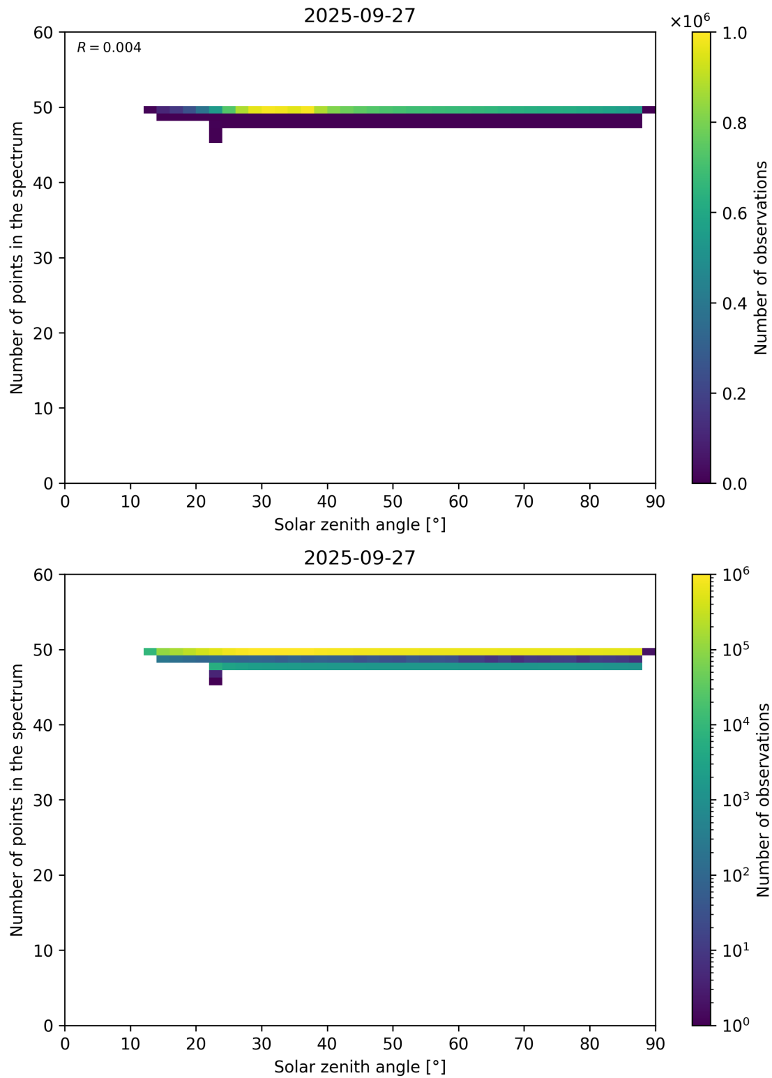
Figure 115: Scatter density plot of “Solar zenith angle” against “Number of points in the spectrum” for 2025-09-26 to 2025-09-28.
