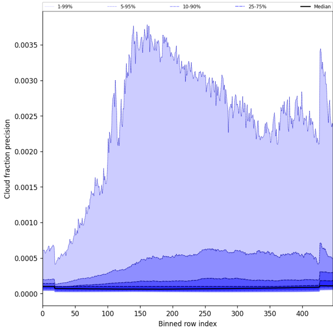
Figure 50: Along track statistics of “Cloud fraction precision” for 2025-09-26 to 2025-09-28
