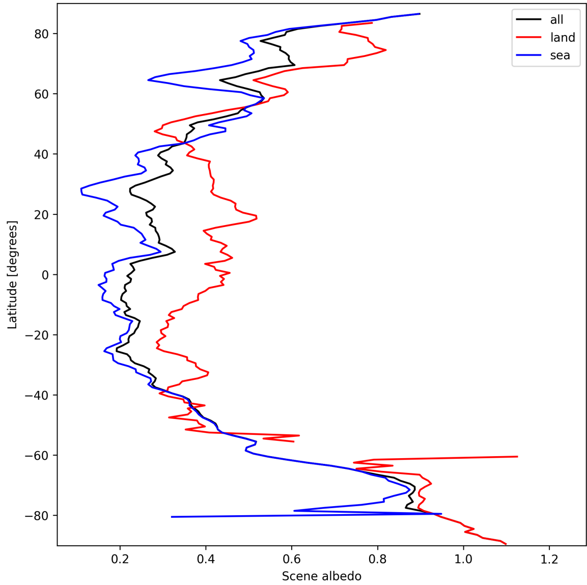
Figure 17: Zonal average of “Scene albedo” for 2025-09-26 to 2025-09-28.
