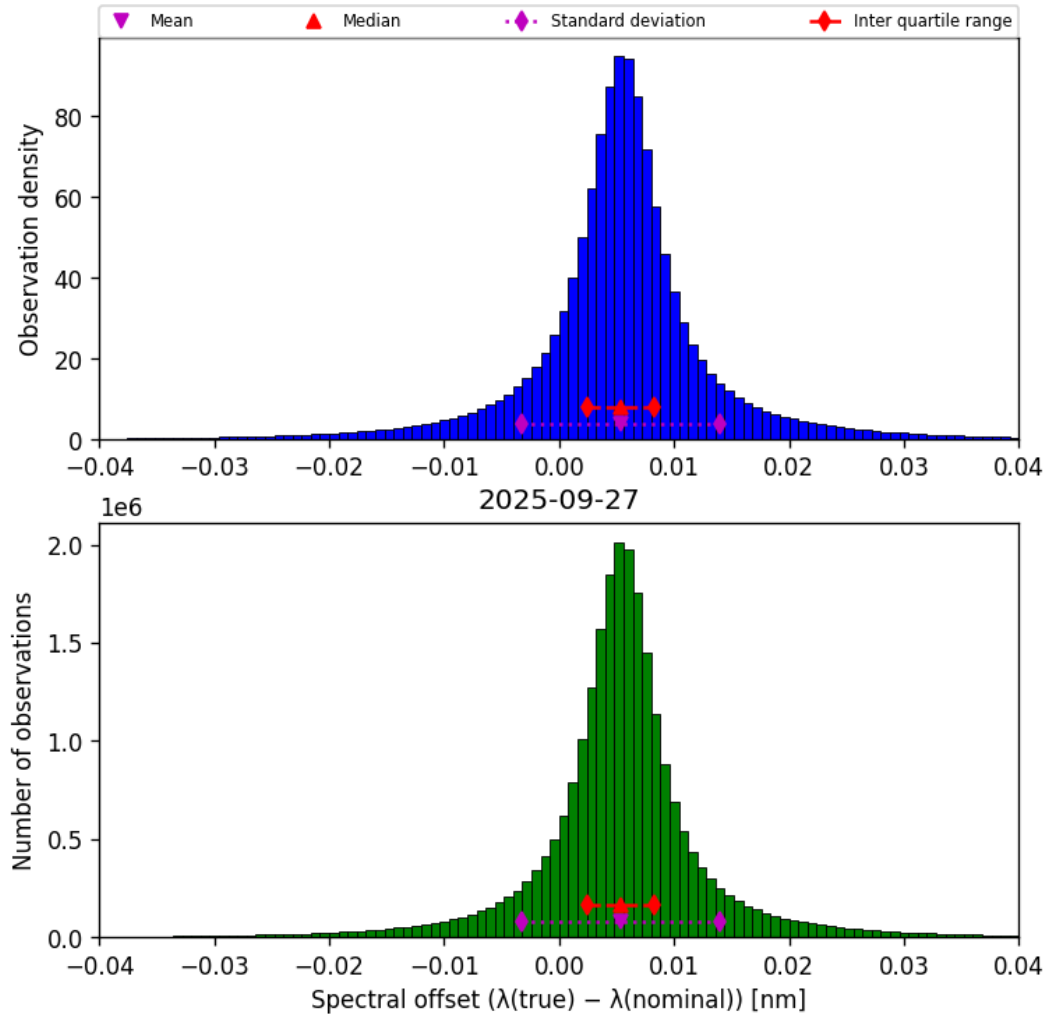
Figure 45: Histogram of “Spectral offset ( \lambda_{\text{true}} - \lambda_{\text{nominal}} )” for 2025-09-26 to 2025-09-28
