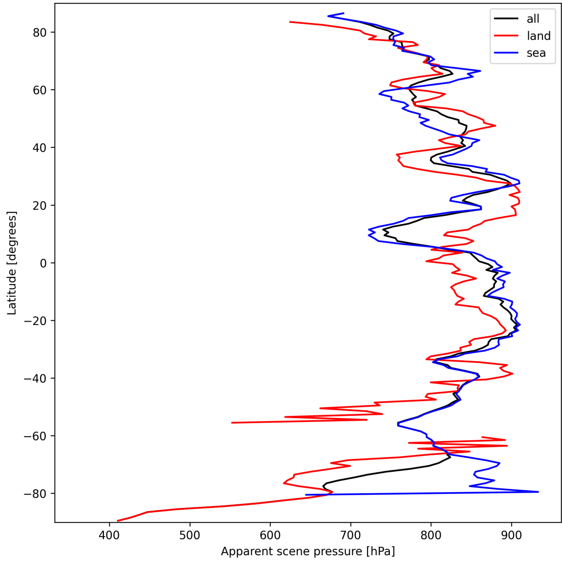
Figure 19: Zonal average of “Apparent scene pressure” for 2025-09-26 to 2025-09-28.
