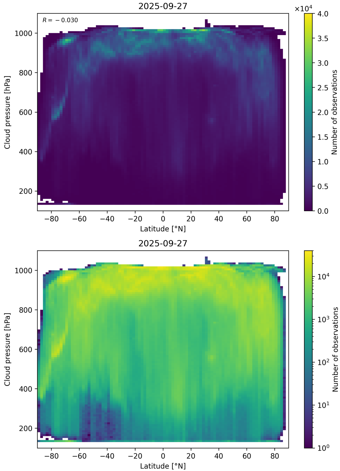
Figure 91: Scatter density plot of “Latitude” against “Cloud pressure” for 2025-09-26 to 2025-09-28.
