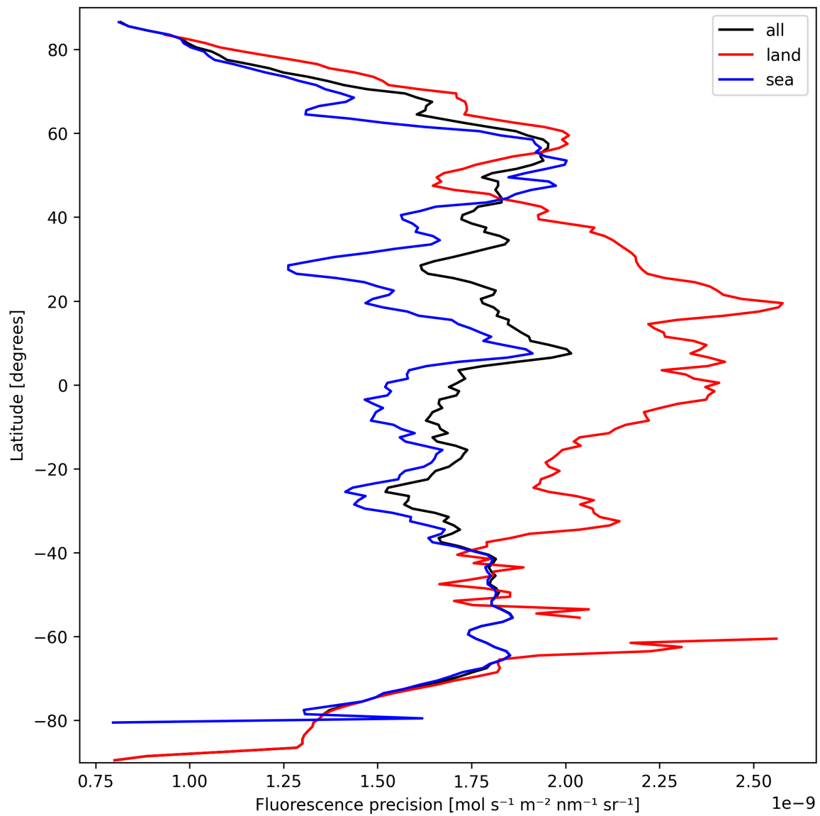
Figure 24: Zonal average of “Fluorescence precision” for 2025-09-26 to 2025-09-28.
