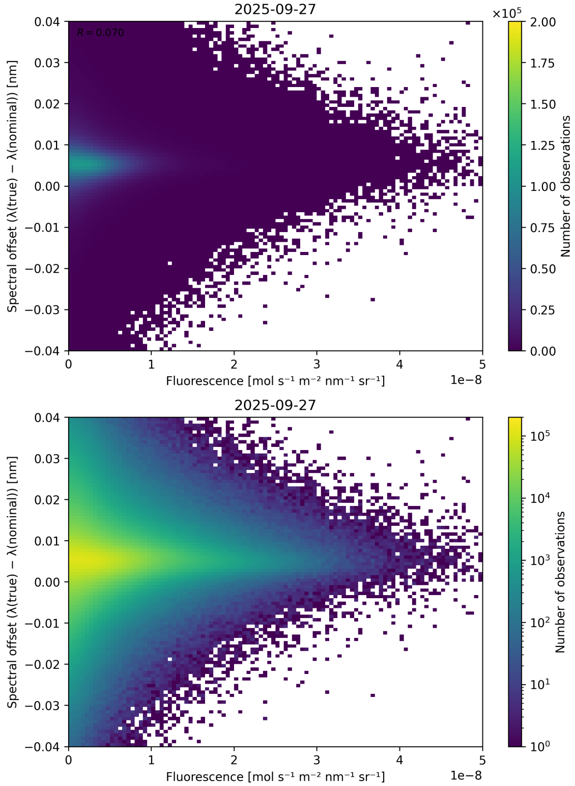
Figure 87: Scatter density plot of “Fluorescence” against “Spectral offset ( \lambda_{\text{true}} - \lambda_{\text{nominal}} )” for 2025-09-26 to 2025-09-28.
