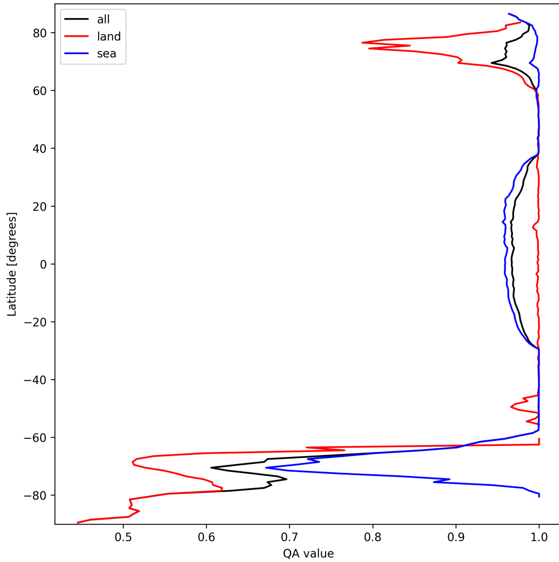
Figure 12: Zonal average of “QA value” for 2025-09-26 to 2025-09-28.
