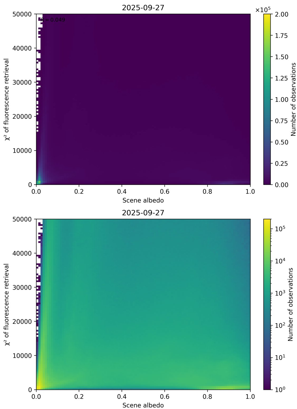
Figure 103: Scatter density plot of “Scene albedo” against “ \chi^2 of fluorescence retrieval” for 2025-09-26 to 2025-09-28.
