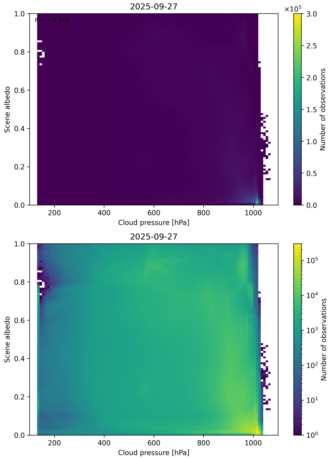
Figure 83: Scatter density plot of “Cloud pressure” against “Scene albedo” for 2025-09-26 to 2025-09-28.
