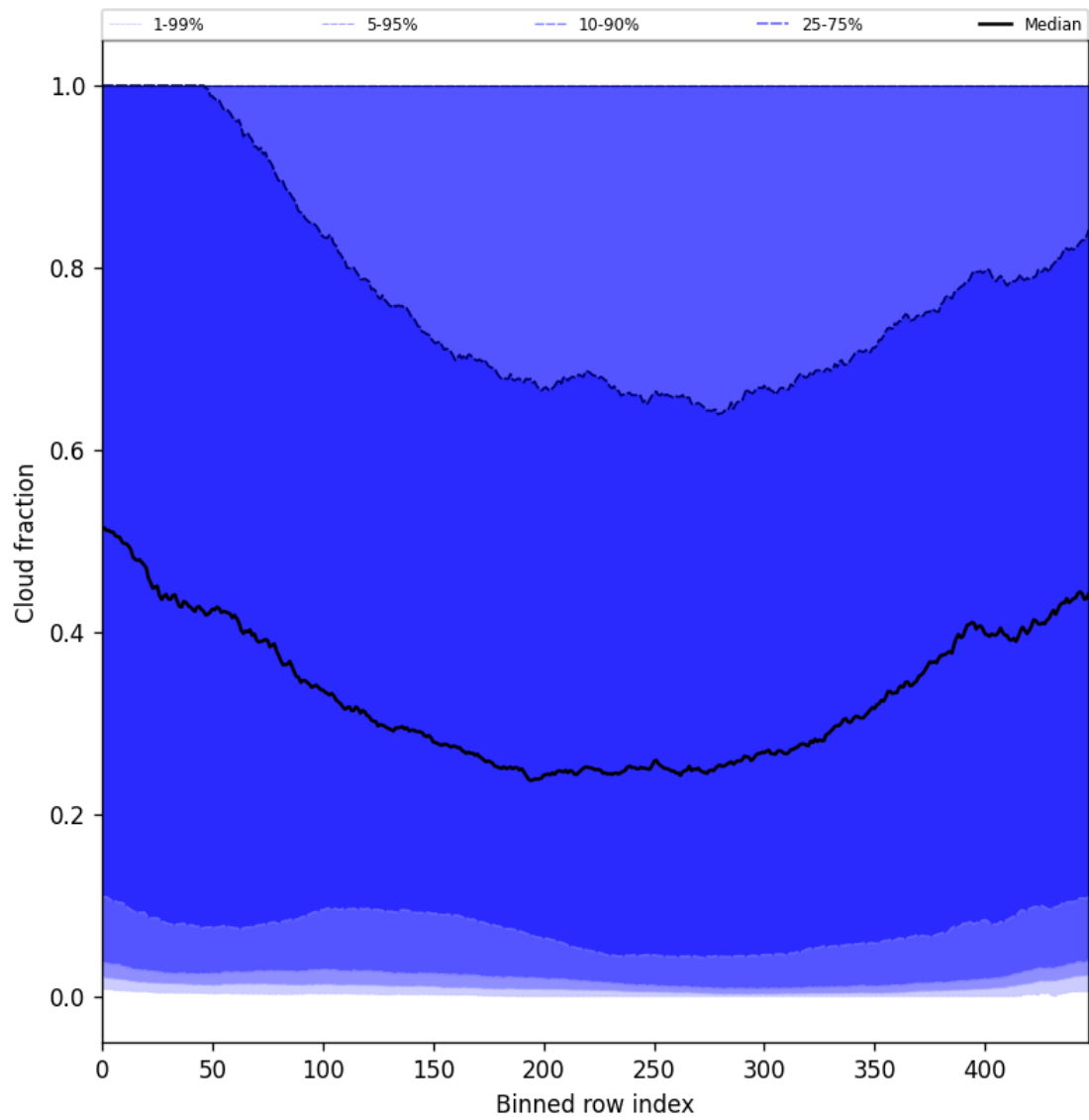
Figure 49: Along track statistics of “Cloud fraction” for 2025-09-26 to 2025-09-28
