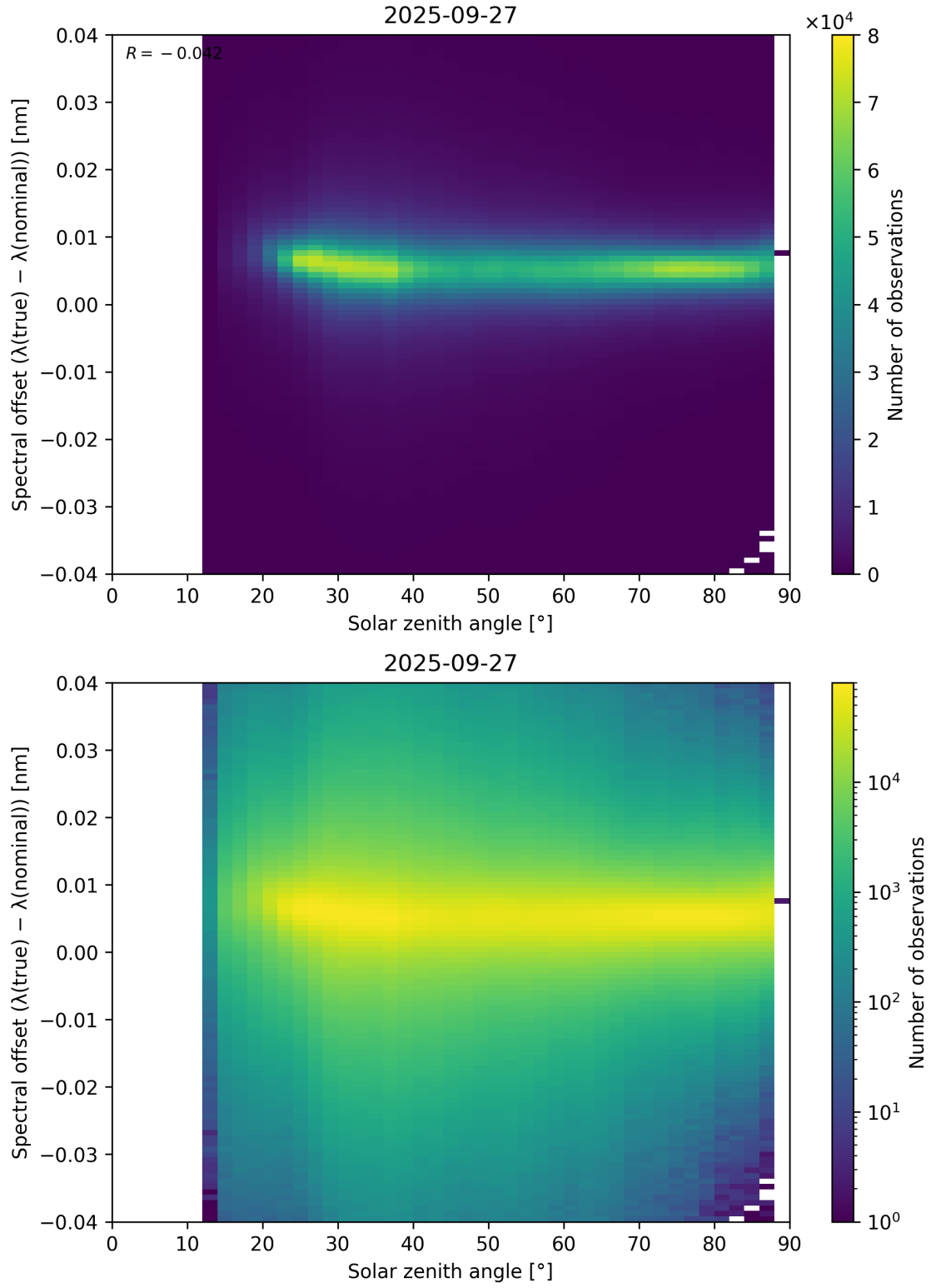
Figure 117: Scatter density plot of “Solar zenith angle” against “Spectral offset ( \lambda_{\text{true}} - \lambda_{\text{nominal}} )” for 2025-09-26 to 2025-09-28.
