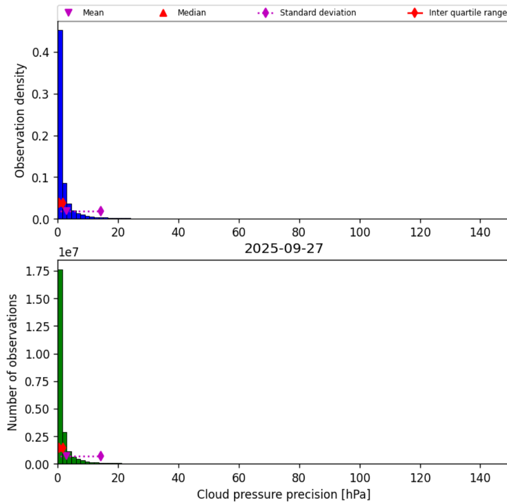
Figure 31: Histogram of “Cloud pressure precision” for 2025-09-26 to 2025-09-28
