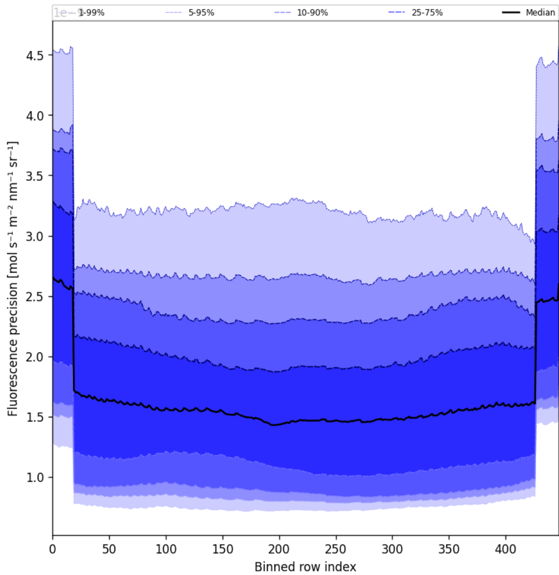
Figure 58: Along track statistics of “Fluorescence precision” for 2025-09-26 to 2025-09-28
