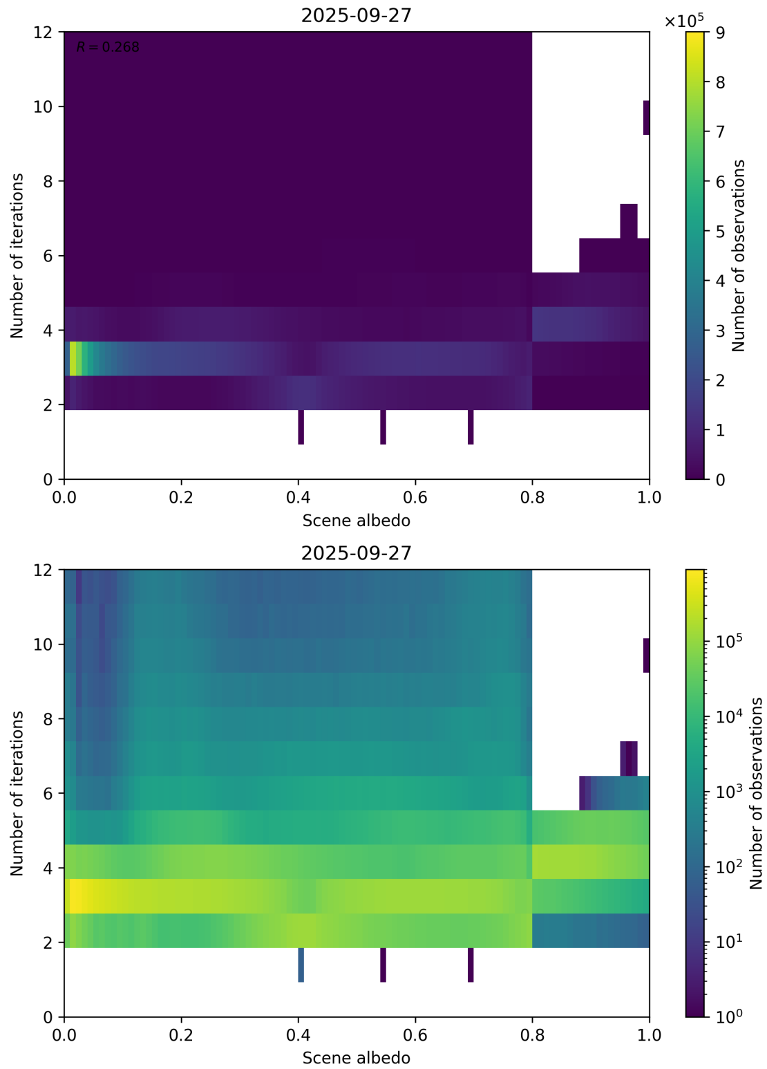
Figure 105: Scatter density plot of “Scene albedo” against “Number of iterations” for 2025-09-26 to 2025-09-28.
