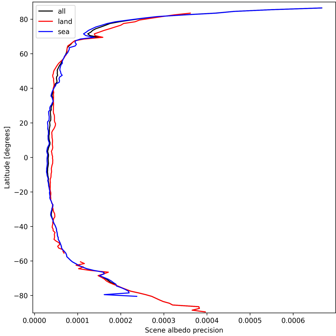
Figure 18: Zonal average of “Scene albedo precision” for 2025-09-26 to 2025-09-28.
