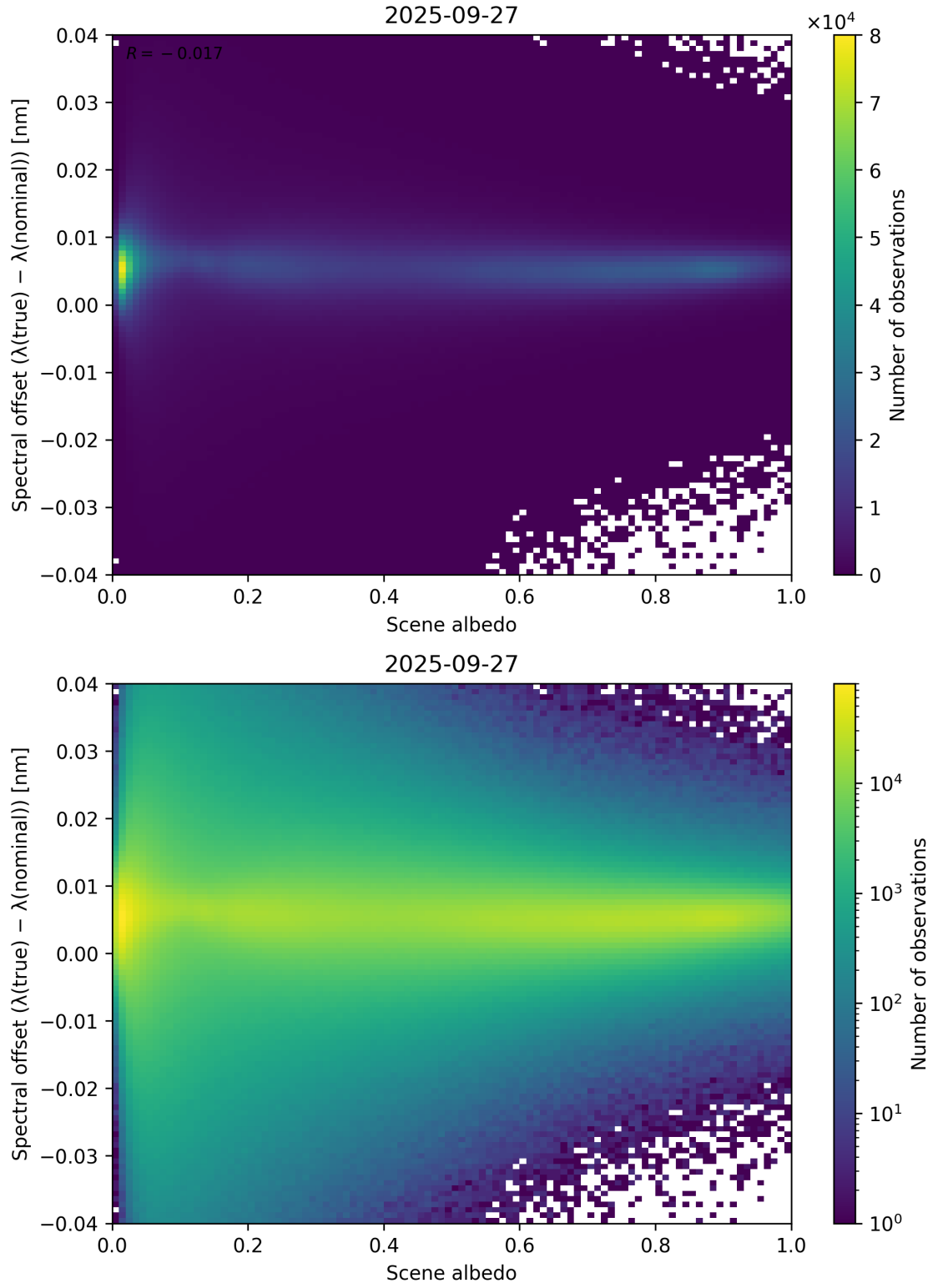
Figure 107: Scatter density plot of “Scene albedo” against “Spectral offset ( \lambda_{\text{true}} - \lambda_{\text{nominal}} )” for 2025-09-26 to 2025-09-28.
