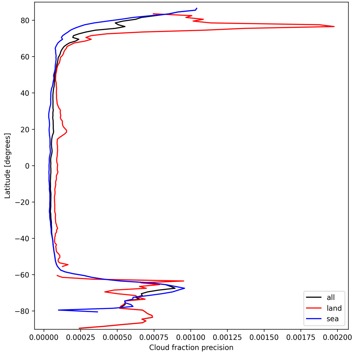
Figure 16: Zonal average of “Cloud fraction precision” for 2025-09-26 to 2025-09-28.
