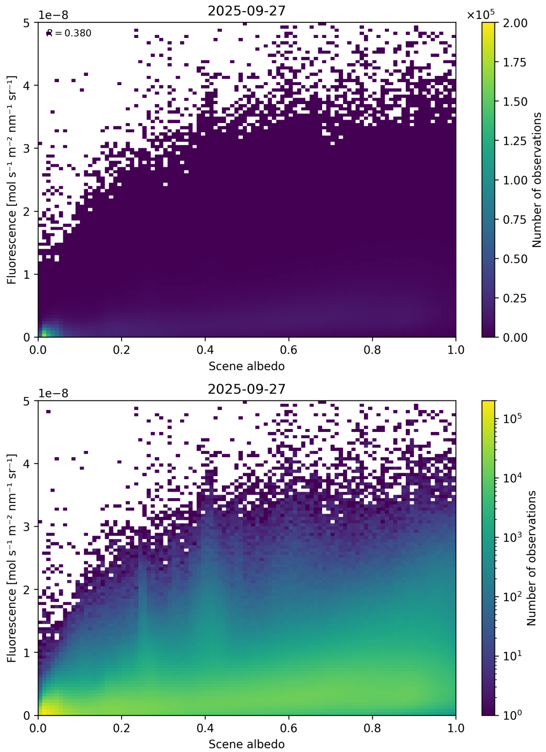
Figure 104: Scatter density plot of “Scene albedo” against “Fluorescence” for 2025-09-26 to 2025-09-28.
