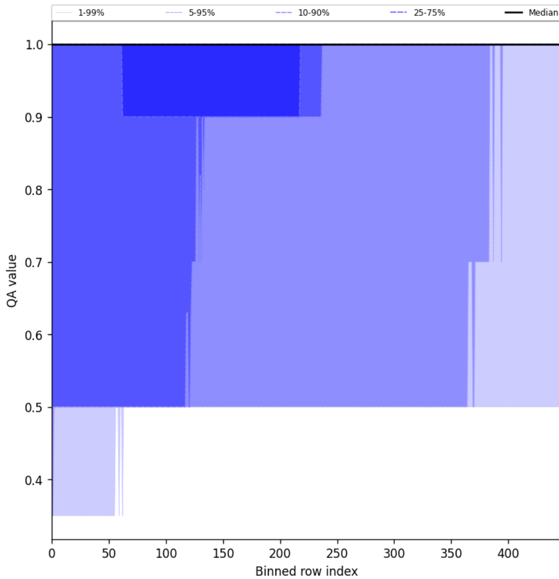
Figure 46: Along track statistics of “QA value” for 2025-09-26 to 2025-09-28
