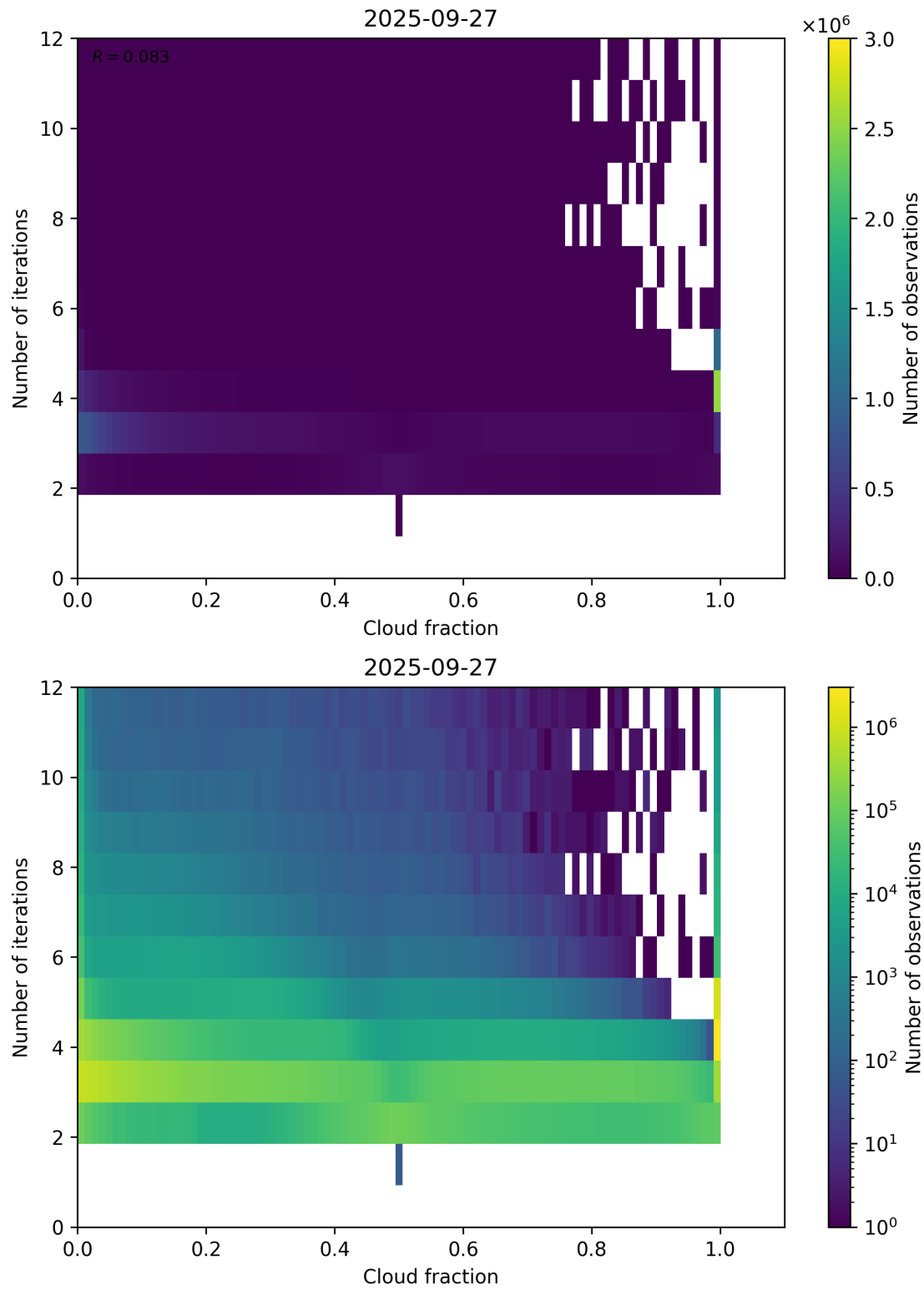
Figure 73: Scatter density plot of “Cloud fraction” against “Number of iterations” for 2025-09-26 to 2025-09-28.
