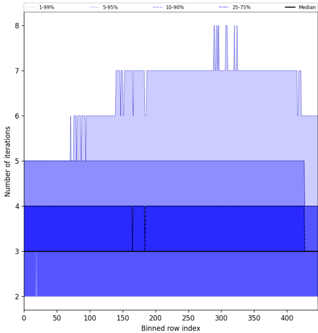
Figure 56: Along track statistics of “Number of iterations” for 2025-09-26 to 2025-09-28
