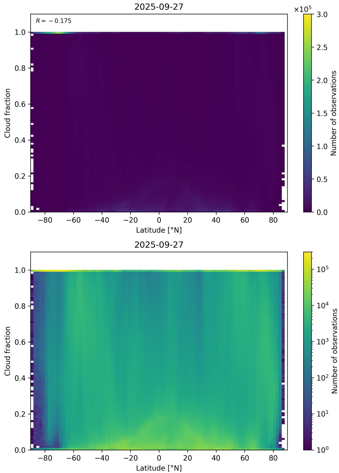
Figure 90: Scatter density plot of “Latitude” against “Cloud fraction” for 2025-09-26 to 2025-09-28.
