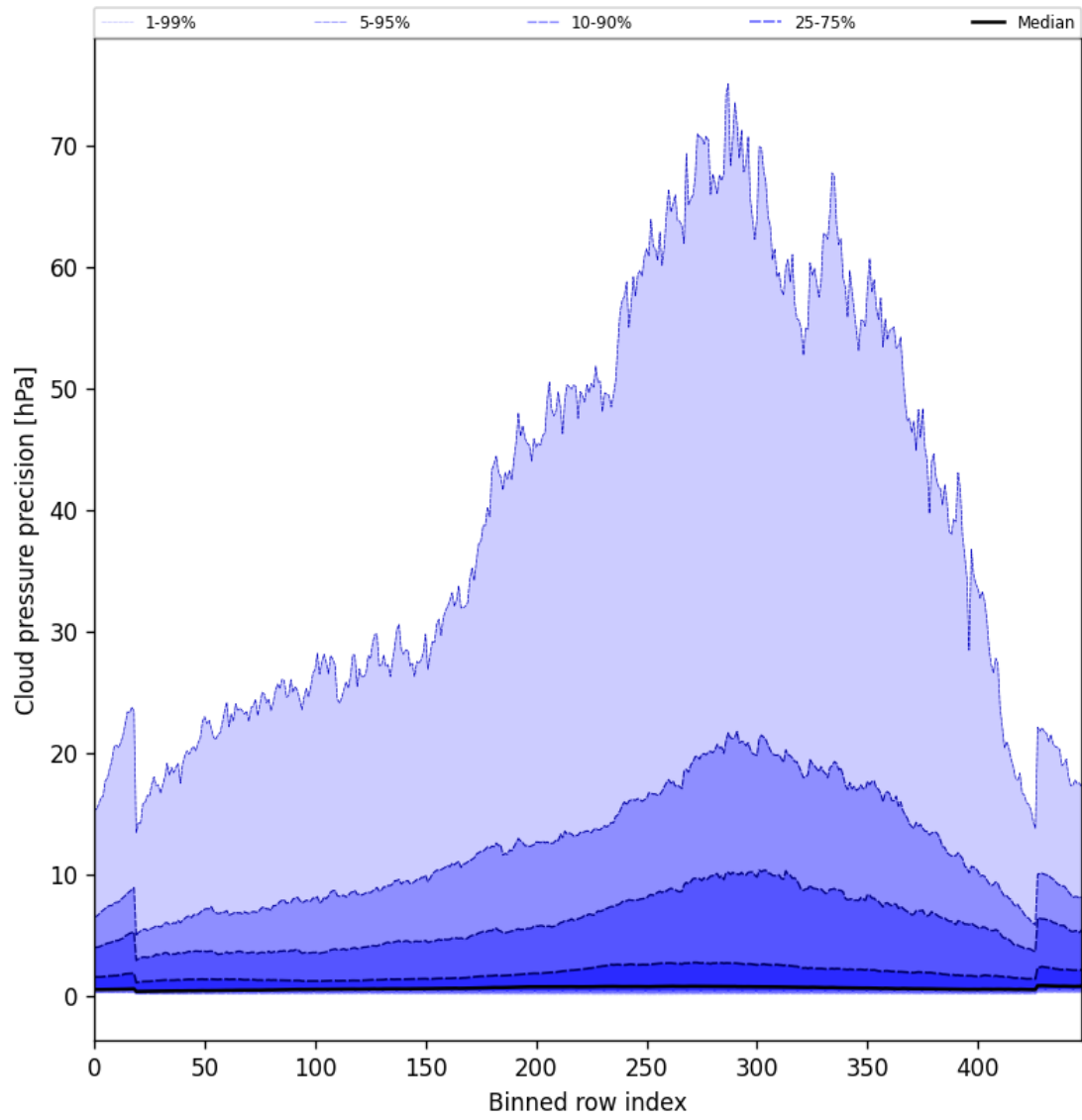
Figure 48: Along track statistics of “Cloud pressure precision” for 2025-09-26 to 2025-09-28
