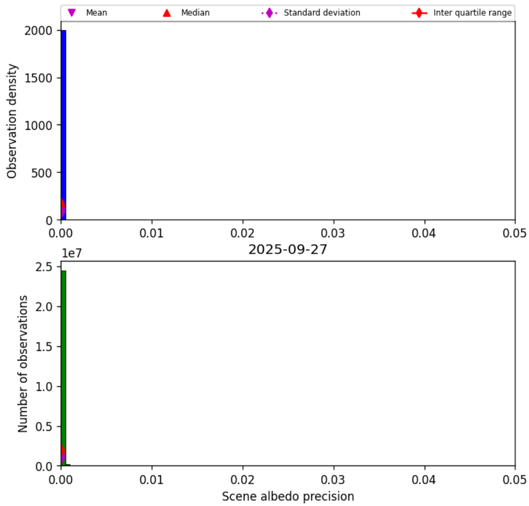
Figure 35: Histogram of “Scene albedo precision” for 2025-09-26 to 2025-09-28
