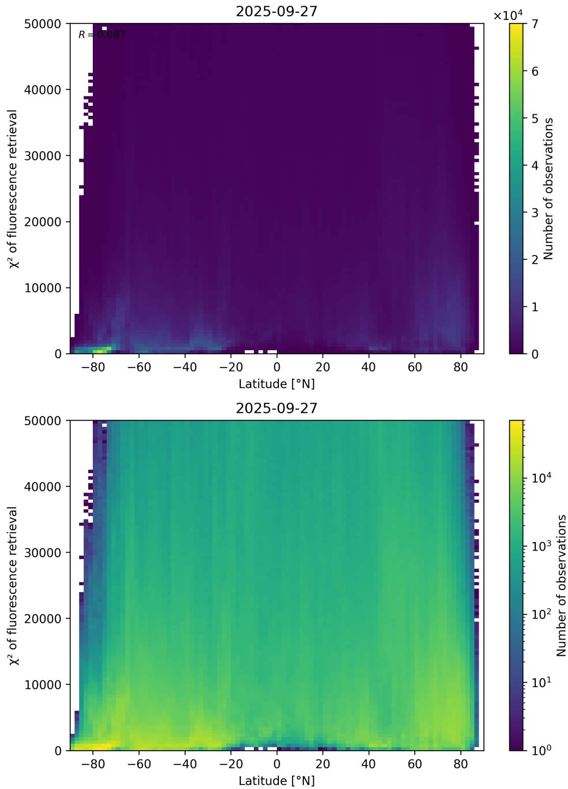
Figure 89: Scatter density plot of “Latitude” against “ \chi^2 of fluorescence retrieval” for 2025-09-26 to 2025-09-28.
