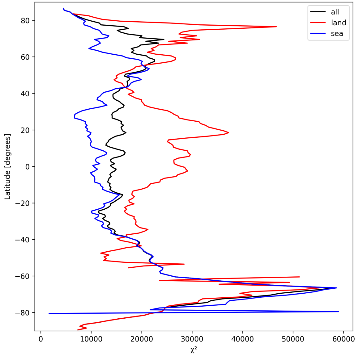
Figure 21: Zonal average of “ \chi^2 ” for 2025-09-26 to 2025-09-28.
