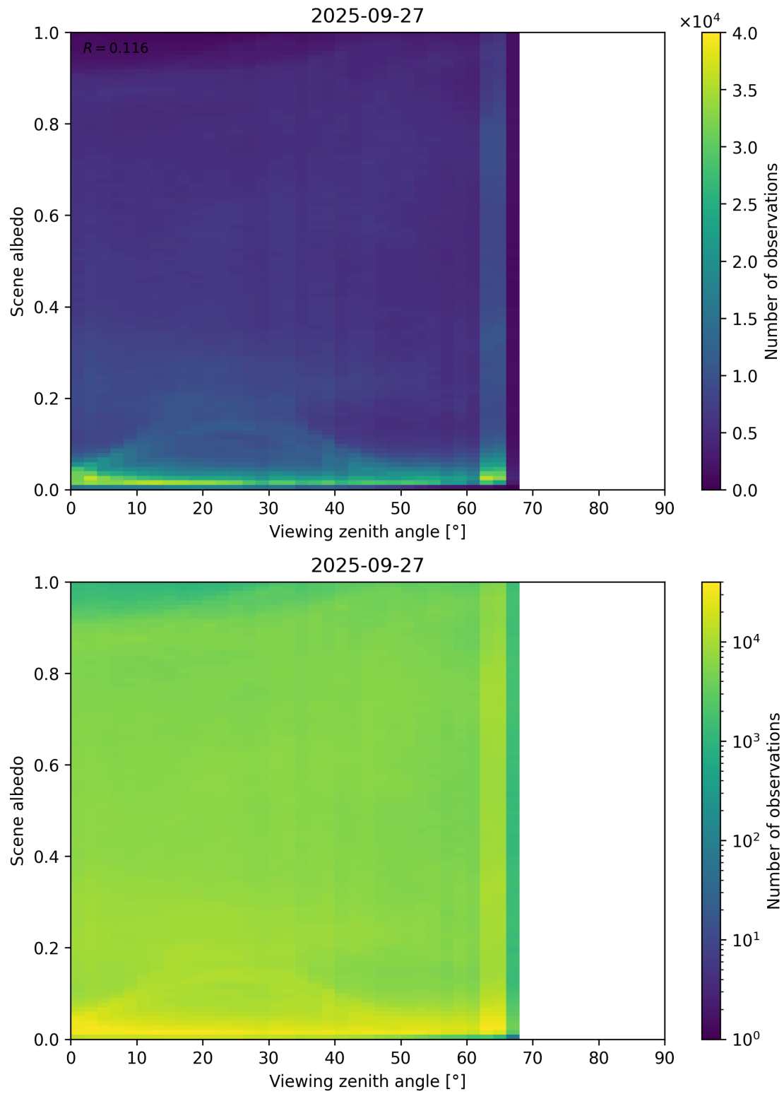
Figure 126: Scatter density plot of “Viewing zenith angle” against “Scene albedo” for 2025-09-26 to 2025-09-28.
