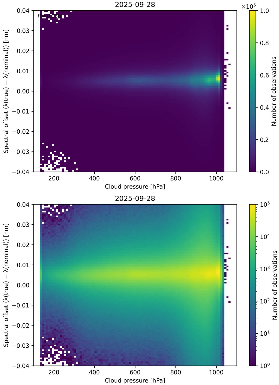
Figure 84: Scatter density plot of “Cloud pressure” against “Spectral offset ( \lambda_{\text{true}} - \lambda_{\text{nominal}} )” for 2025-09-27 to 2025-09-29.
