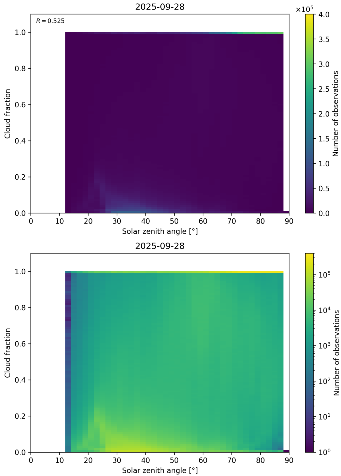
Figure 110: Scatter density plot of “Solar zenith angle” against “Cloud fraction” for 2025-09-27 to 2025-09-29.
