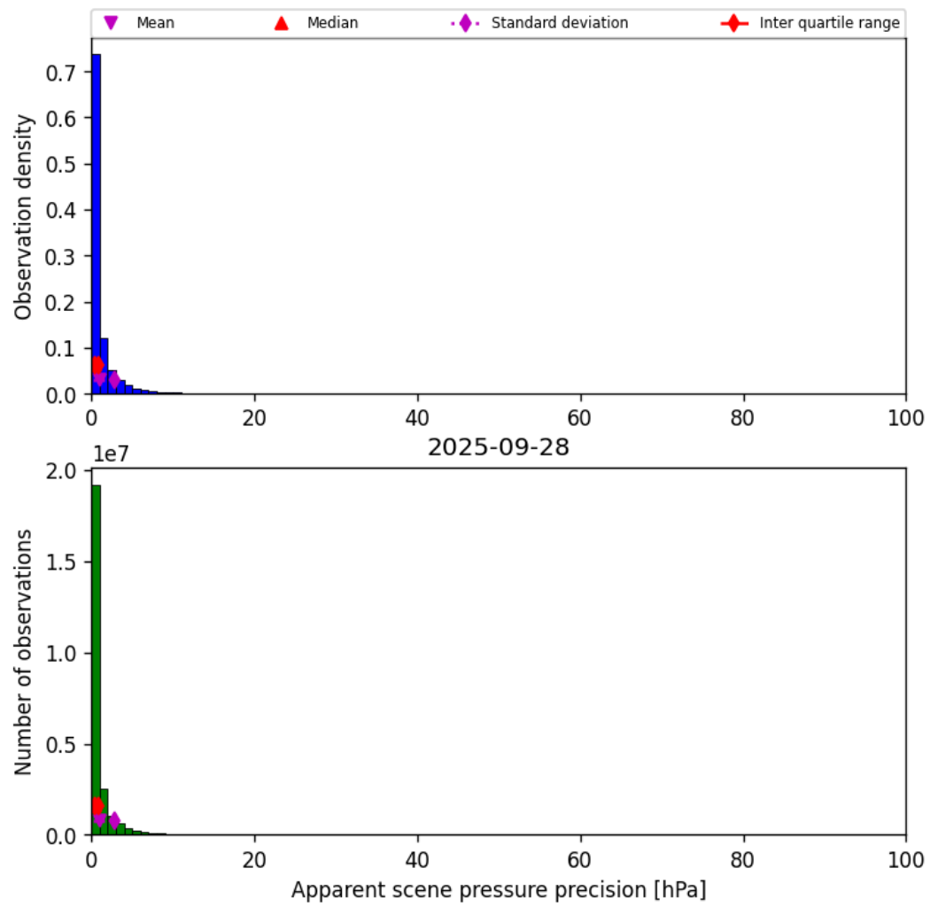
Figure 37: Histogram of “Apparent scene pressure precision” for 2025-09-27 to 2025-09-29
