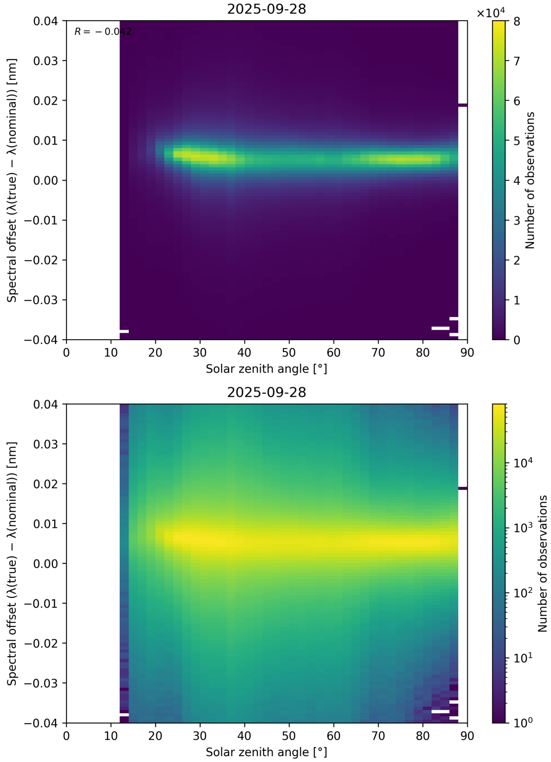
Figure 117: Scatter density plot of “Solar zenith angle” against “Spectral offset ( \lambda_{\text{true}} - \lambda_{\text{nominal}} )” for 2025-09-27 to 2025-09-29.
