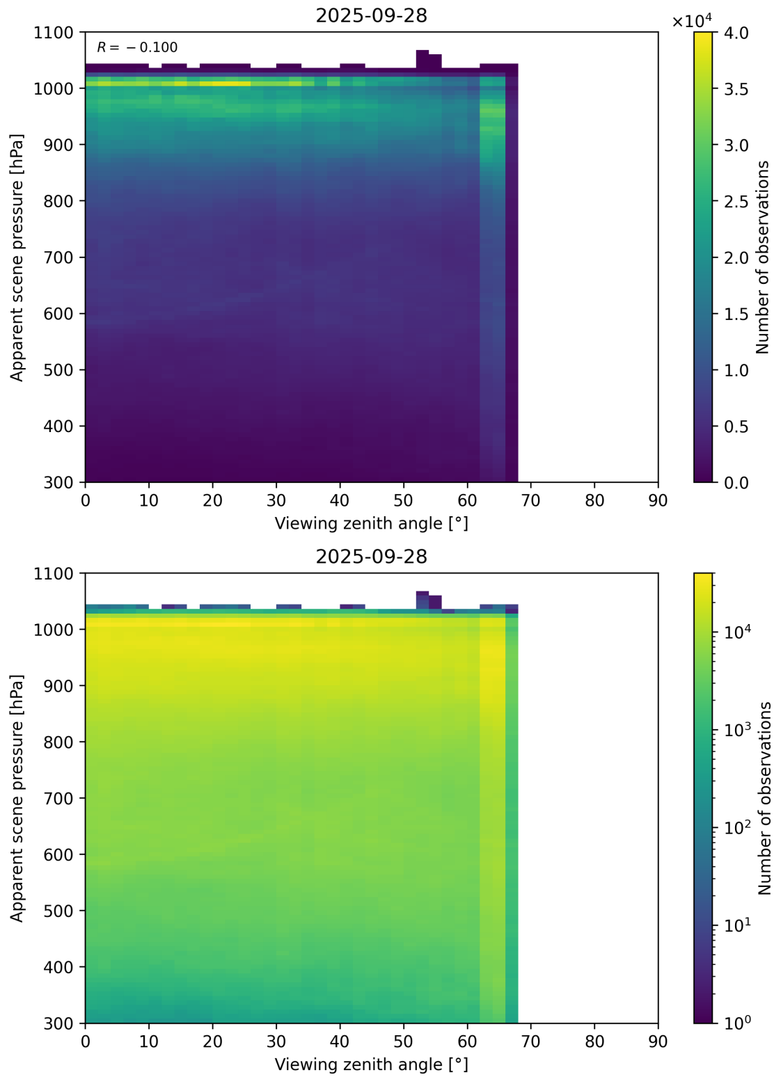
Figure 118: Scatter density plot of “Viewing zenith angle” against “Apparent scene pressure” for 2025-09-27 to 2025-09-29.
