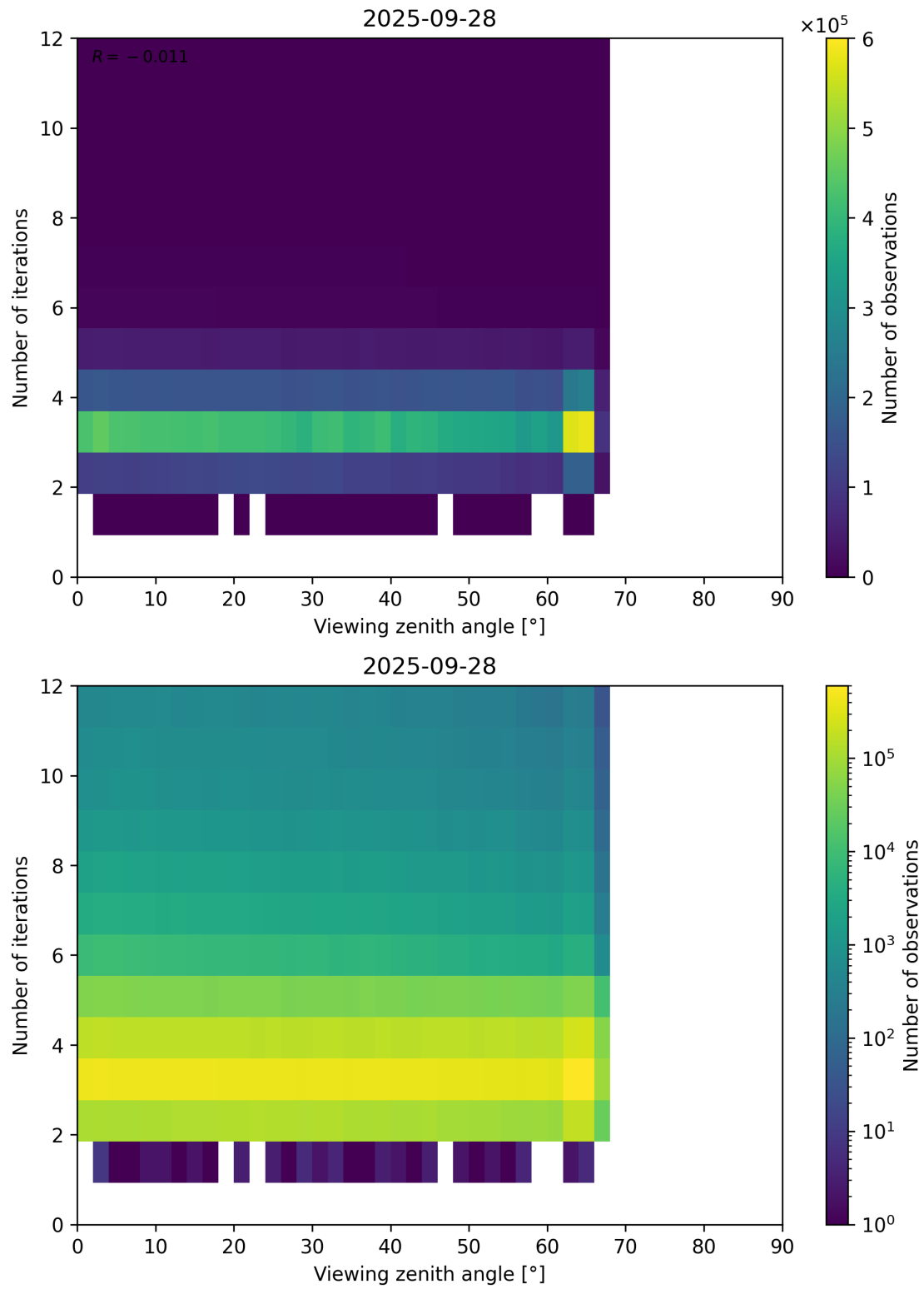
Figure 124: Scatter density plot of “Viewing zenith angle” against “Number of iterations” for 2025-09-27 to 2025-09-29.
