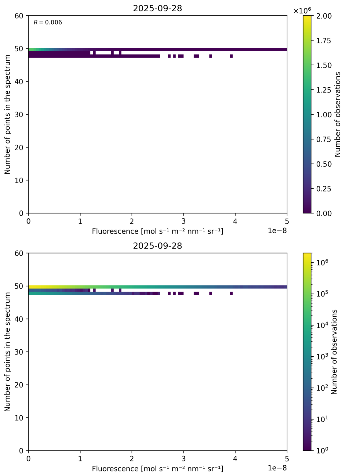
Figure 86: Scatter density plot of “Fluorescence” against “Number of points in the spectrum” for 2025-09-27 to 2025-09-29.
