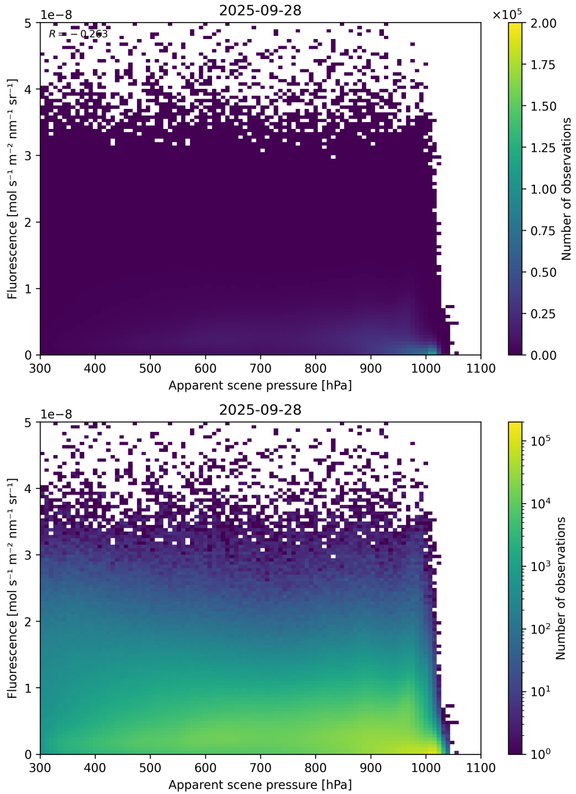
Figure 64: Scatter density plot of “Apparent scene pressure” against “Fluorescence” for 2025-09-27 to 2025-09-29.
