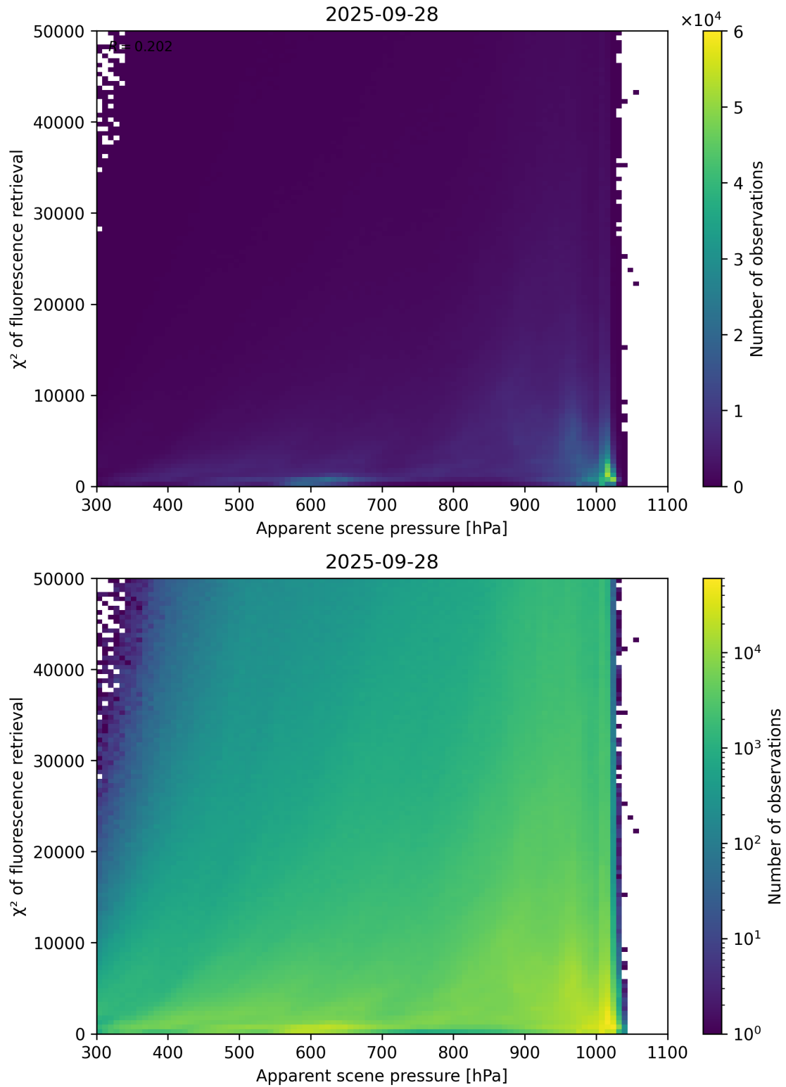
Figure 63: Scatter density plot of “Apparent scene pressure” against “ \chi^2 of fluorescence retrieval” for 2025-09-27 to 2025-09-29.
