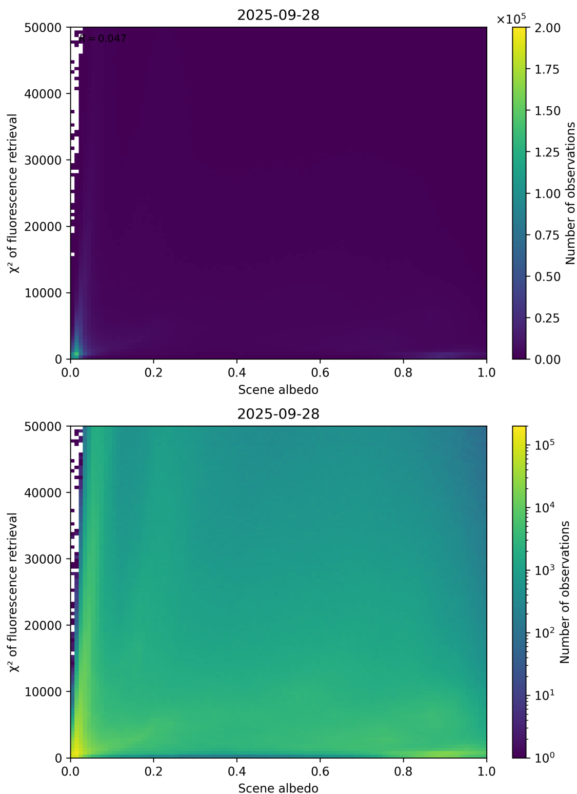
Figure 103: Scatter density plot of “Scene albedo” against “ \chi^2 of fluorescence retrieval” for 2025-09-27 to 2025-09-29.
