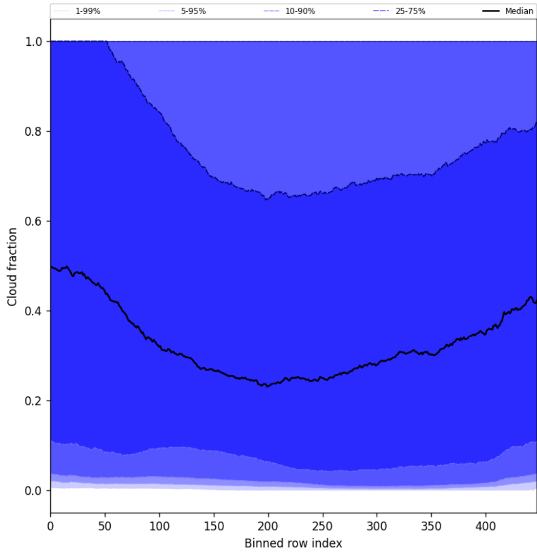
Figure 49: Along track statistics of “Cloud fraction” for 2025-09-27 to 2025-09-29
