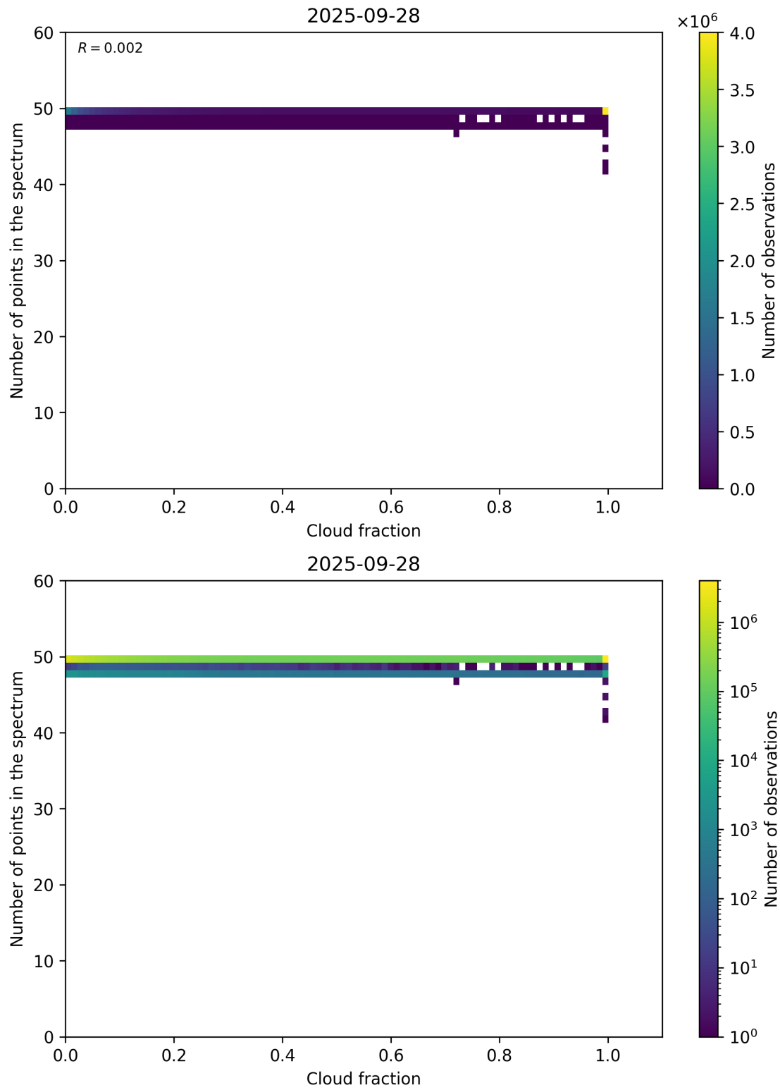
Figure 74: Scatter density plot of “Cloud fraction” against “Number of points in the spectrum” for 2025-09-27 to 2025-09-29.
