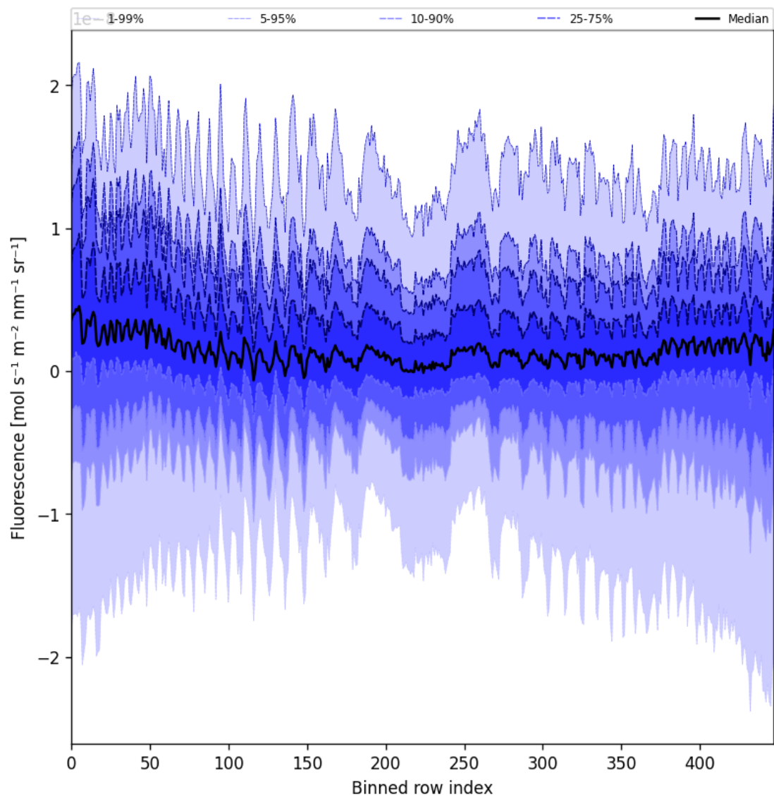
Figure 57: Along track statistics of “Fluorescence” for 2025-09-27 to 2025-09-29
