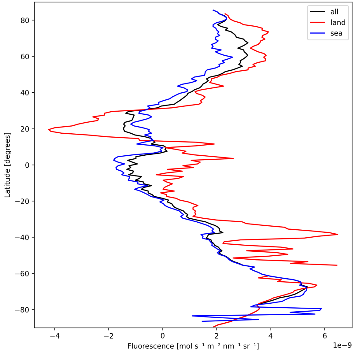
Figure 23: Zonal average of “Fluorescence” for 2025-09-27 to 2025-09-29.
