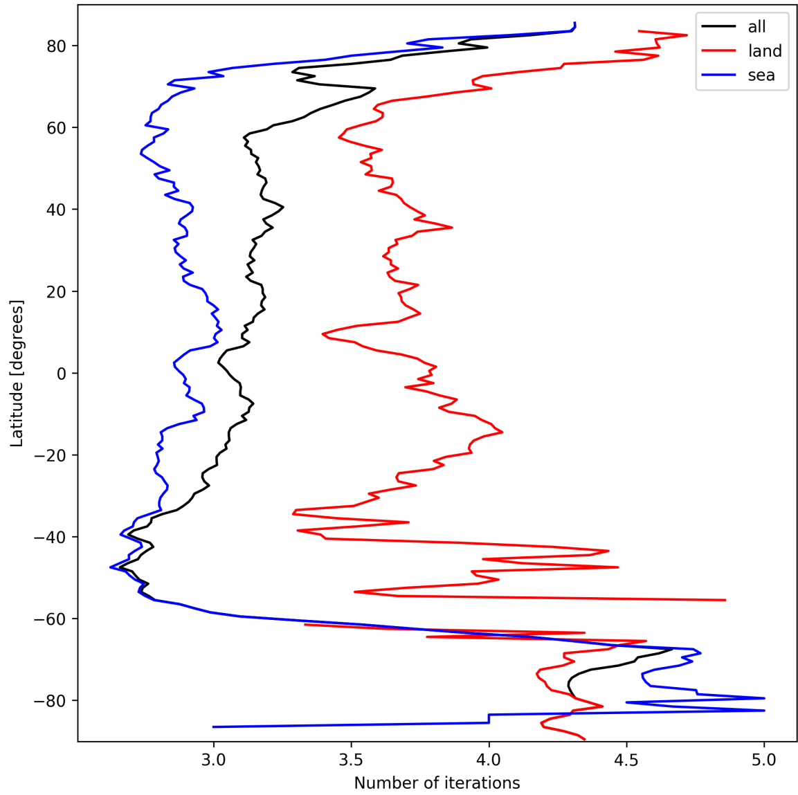
Figure 22: Zonal average of “Number of iterations” for 2025-09-27 to 2025-09-29.
