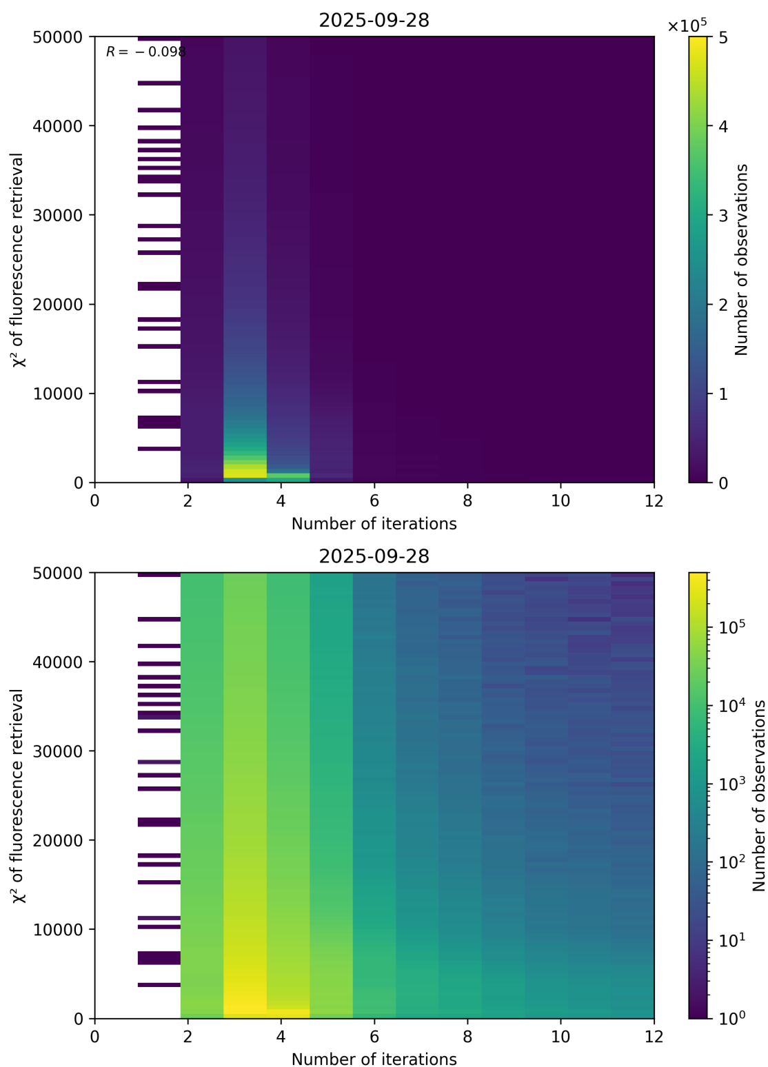
Figure 97: Scatter density plot of “Number of iterations” against “ \chi^2 of fluorescence retrieval” for 2025-09-27 to 2025-09-29.
