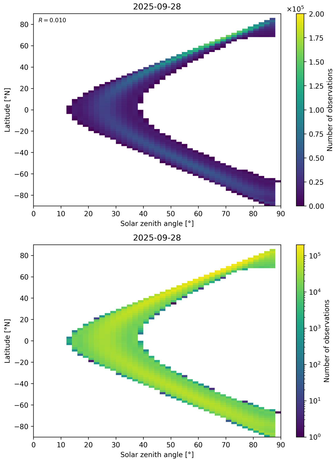
Figure 113: Scatter density plot of “Solar zenith angle” against “Latitude” for 2025-09-27 to 2025-09-29.
