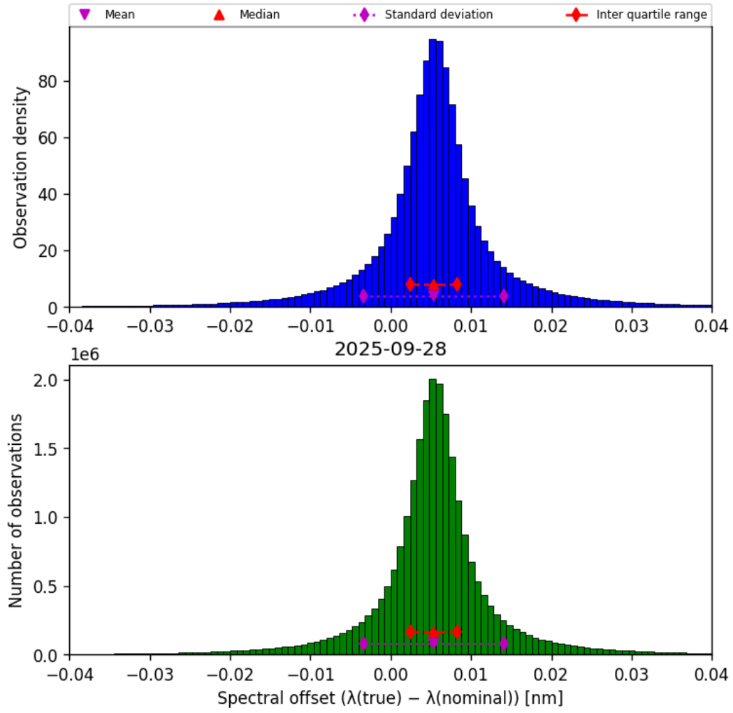
Figure 45: Histogram of “Spectral offset ( \lambda_{\text{true}} - \lambda_{\text{nominal}} )” for 2025-09-27 to 2025-09-29
