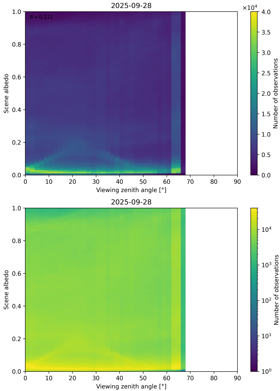
Figure 126: Scatter density plot of “Viewing zenith angle” against “Scene albedo” for 2025-09-27 to 2025-09-29.
