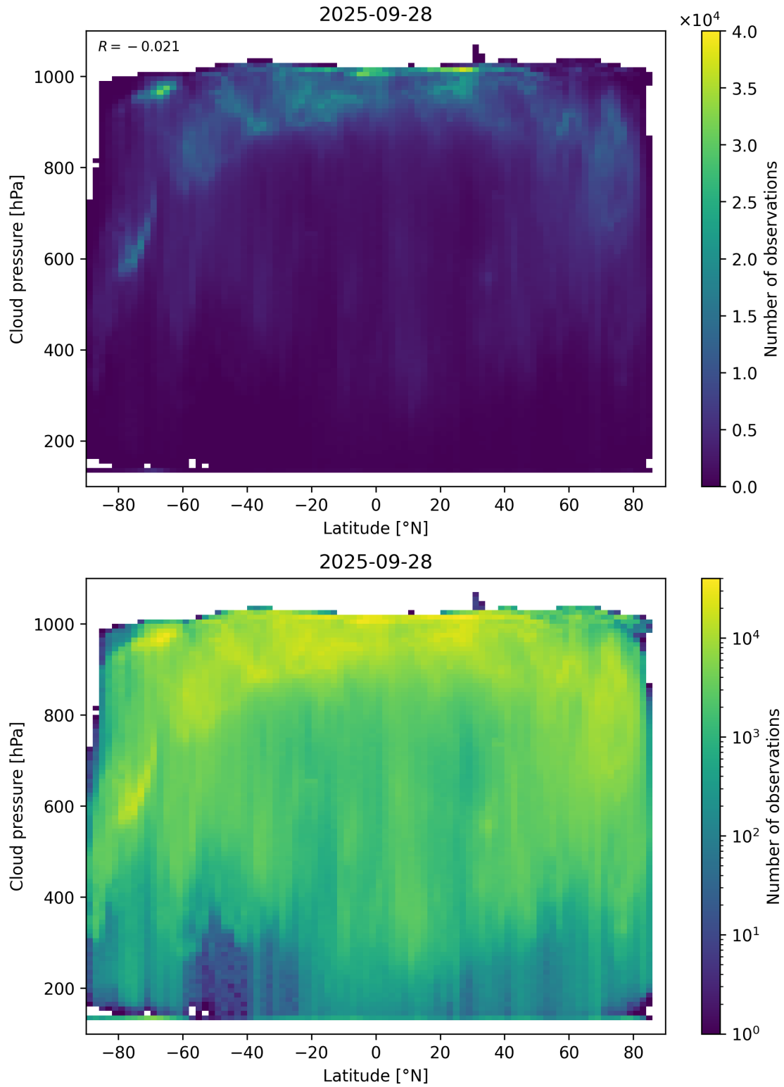
Figure 91: Scatter density plot of “Latitude” against “Cloud pressure” for 2025-09-27 to 2025-09-29.
