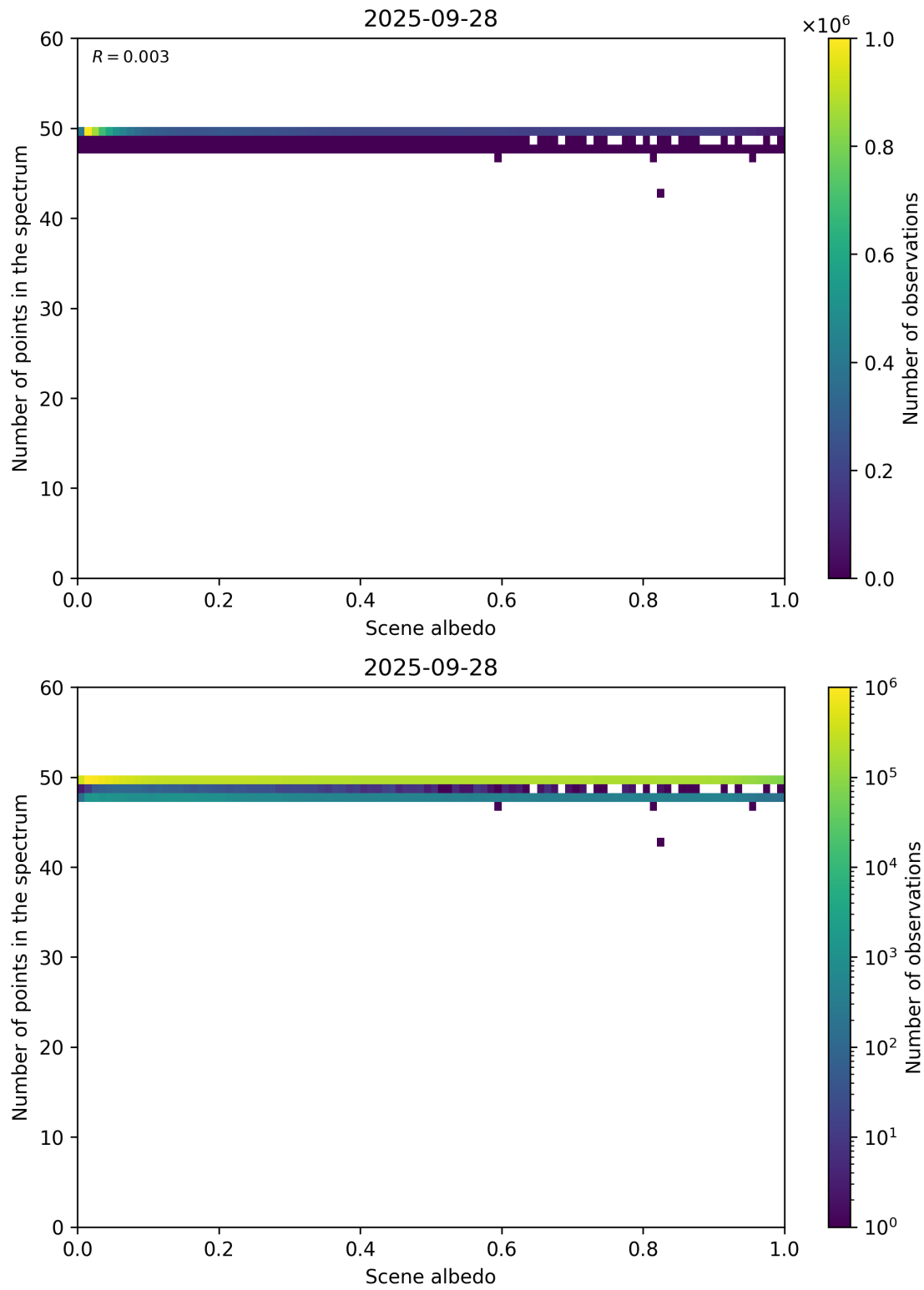
Figure 106: Scatter density plot of “Scene albedo” against “Number of points in the spectrum” for 2025-09-27 to 2025-09-29.
