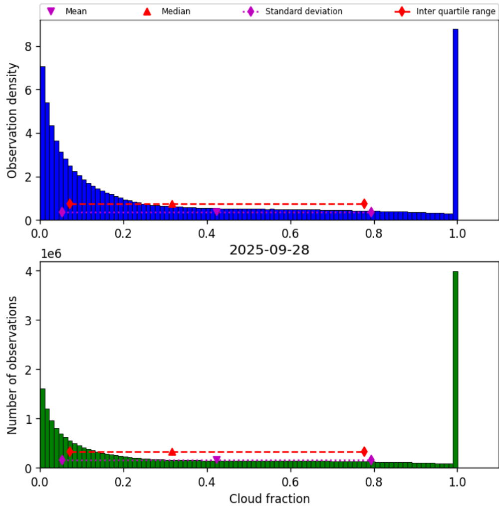
Figure 32: Histogram of “Cloud fraction” for 2025-09-27 to 2025-09-29
