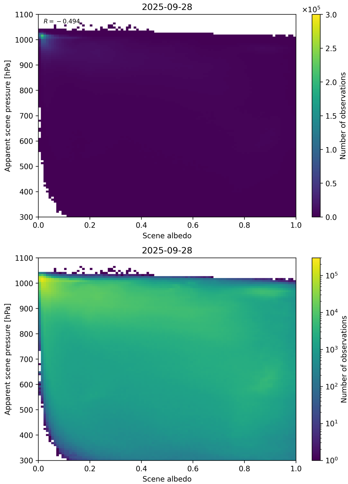
Figure 102: Scatter density plot of “Scene albedo” against “Apparent scene pressure” for 2025-09-27 to 2025-09-29.
