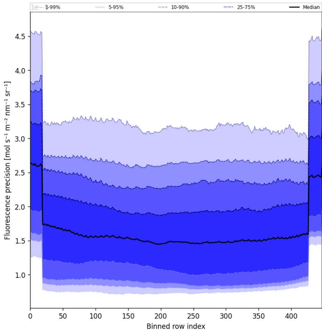
Figure 58: Along track statistics of “Fluorescence precision” for 2025-09-27 to 2025-09-29
