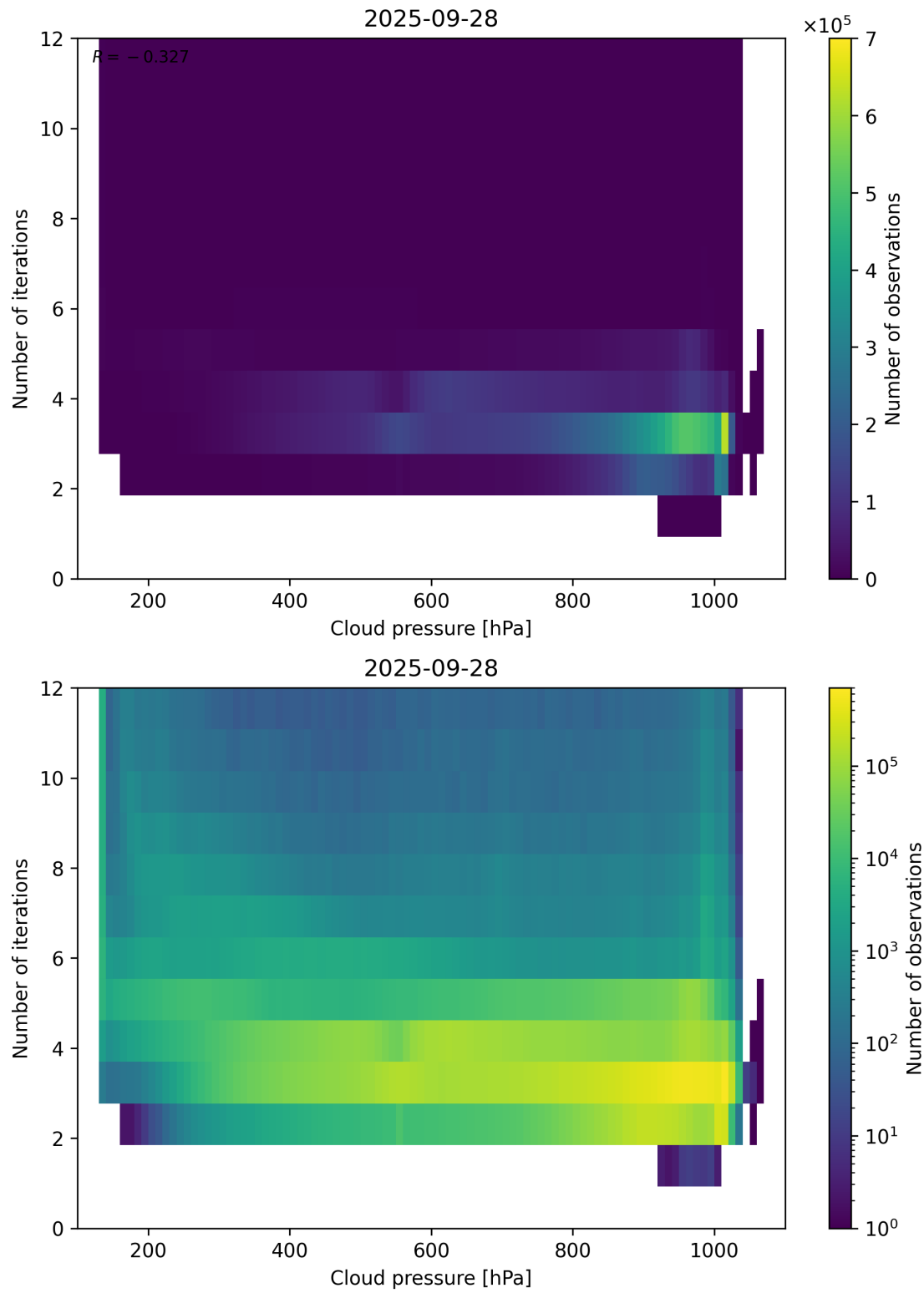
Figure 81: Scatter density plot of “Cloud pressure” against “Number of iterations” for 2025-09-27 to 2025-09-29.
