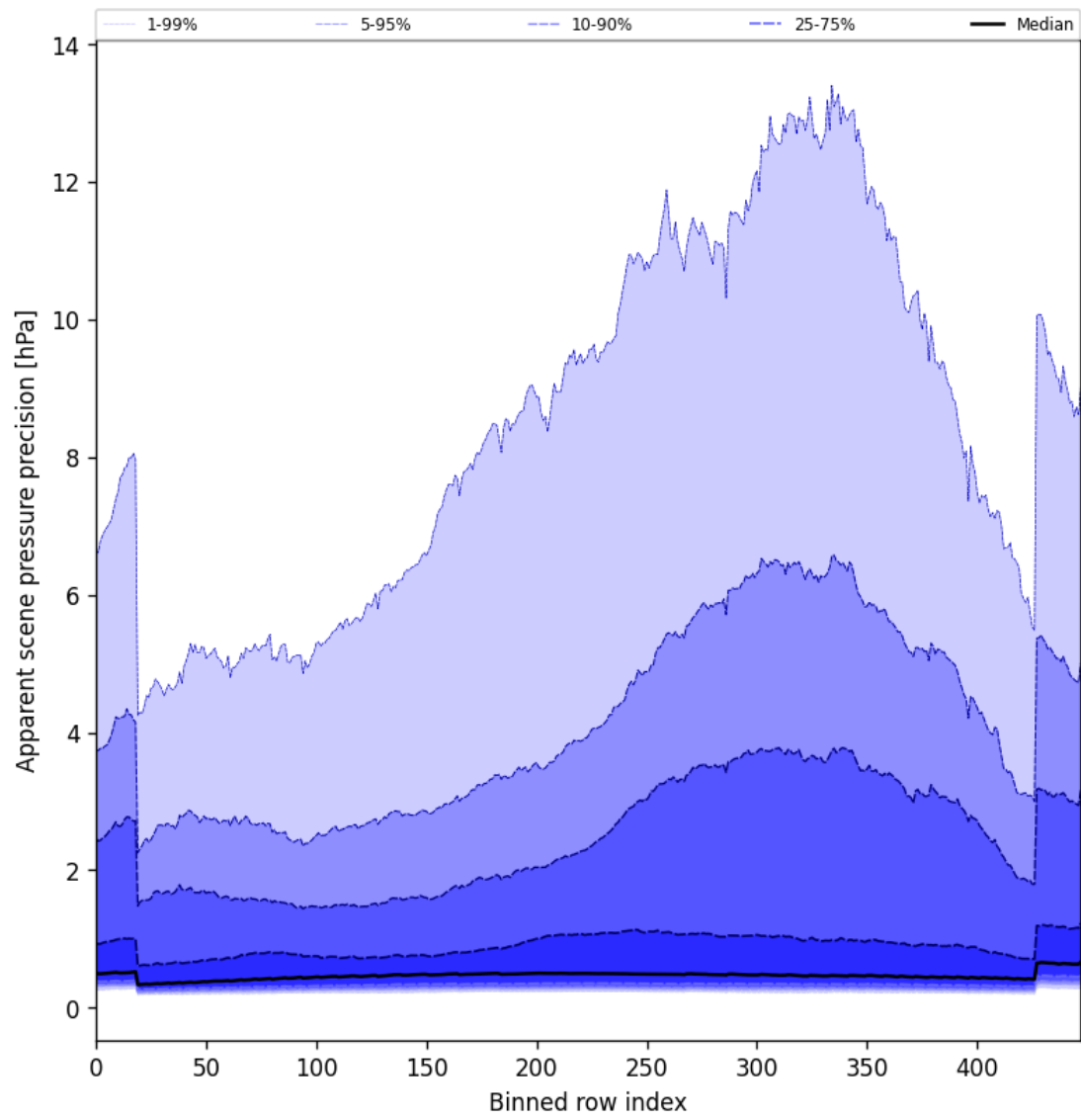
Figure 54: Along track statistics of “Apparent scene pressure precision” for 2025-09-27 to 2025-09-29
