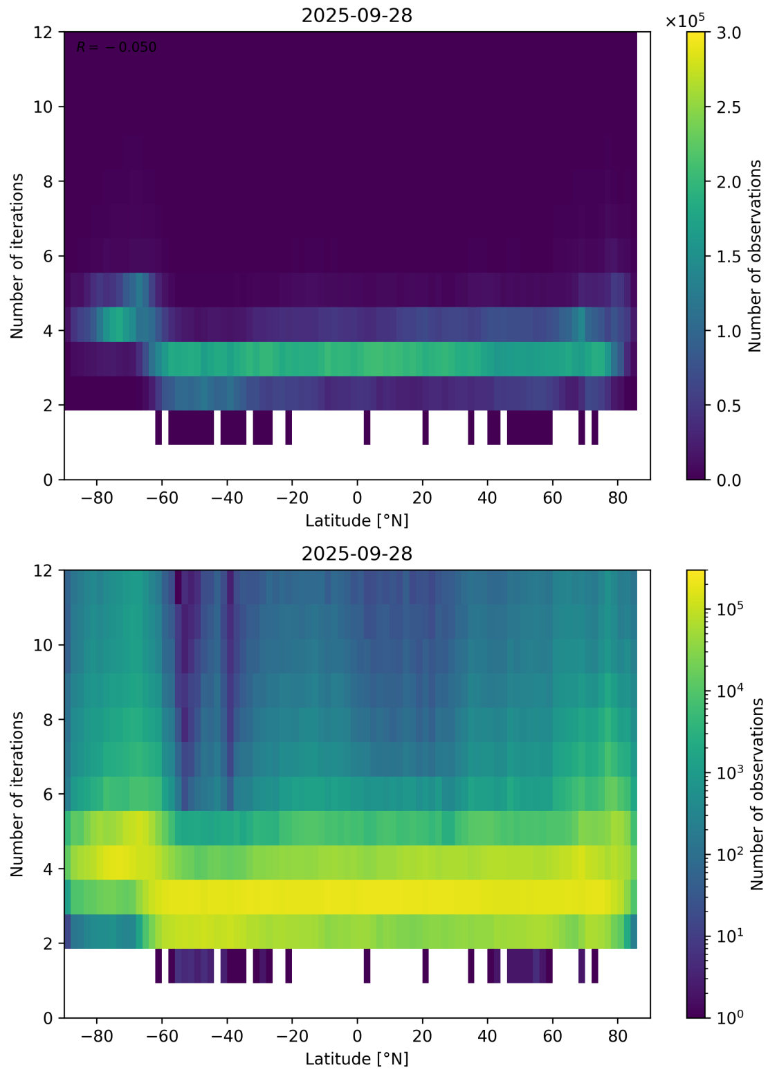
Figure 93: Scatter density plot of “Latitude” against “Number of iterations” for 2025-09-27 to 2025-09-29.
