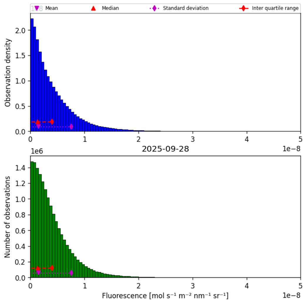
Figure 40: Histogram of “Fluorescence” for 2025-09-27 to 2025-09-29
