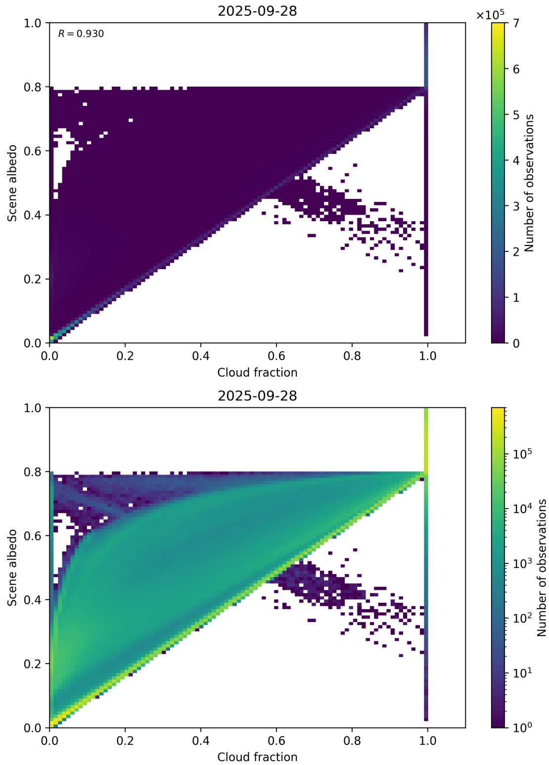
Figure 75: Scatter density plot of “Cloud fraction” against “Scene albedo” for 2025-09-27 to 2025-09-29.
