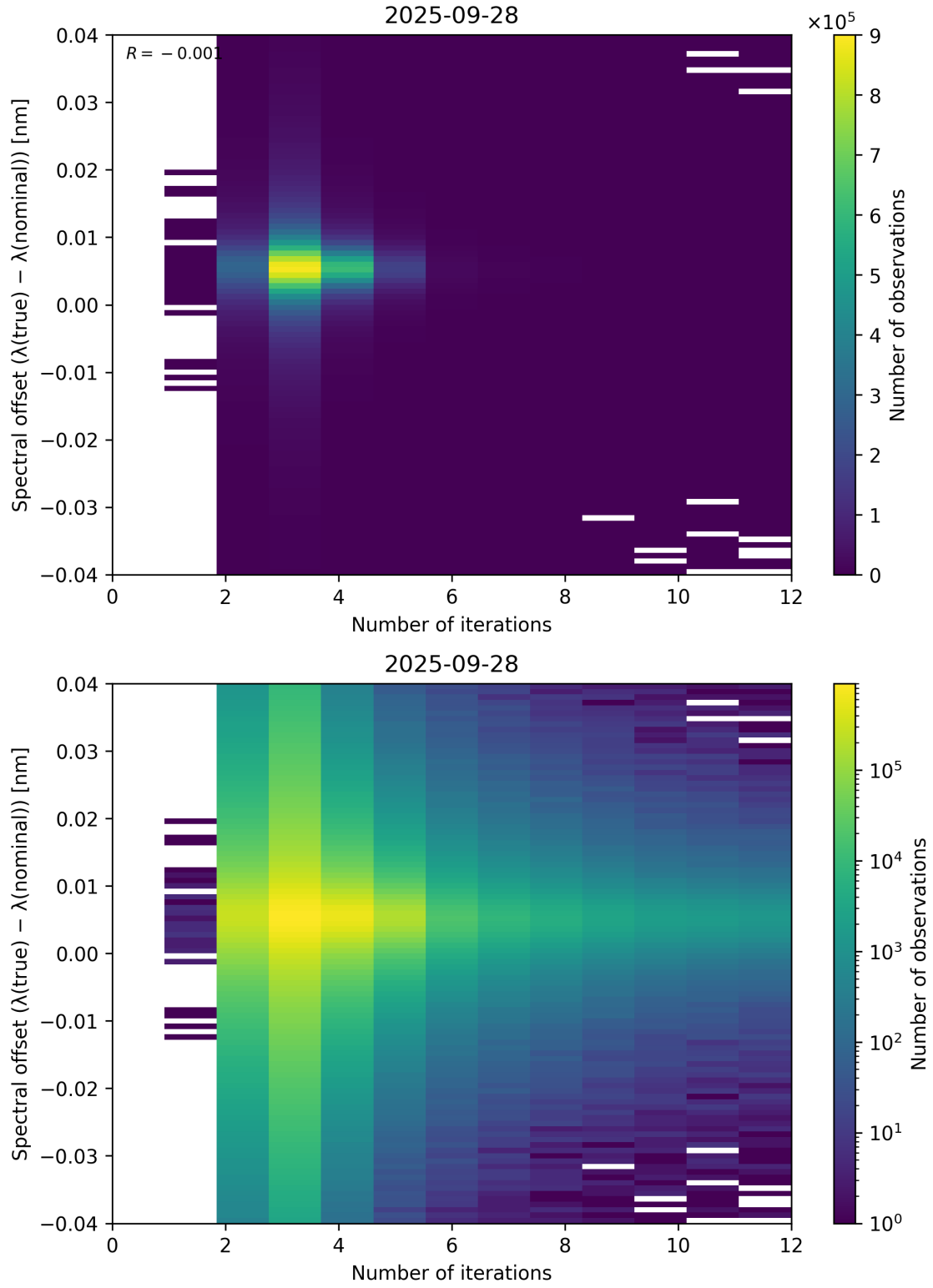
Figure 100: Scatter density plot of “Number of iterations” against “Spectral offset ( \lambda_{\text{true}} - \lambda_{\text{nominal}} )” for 2025-09-27 to 2025-09-29.
