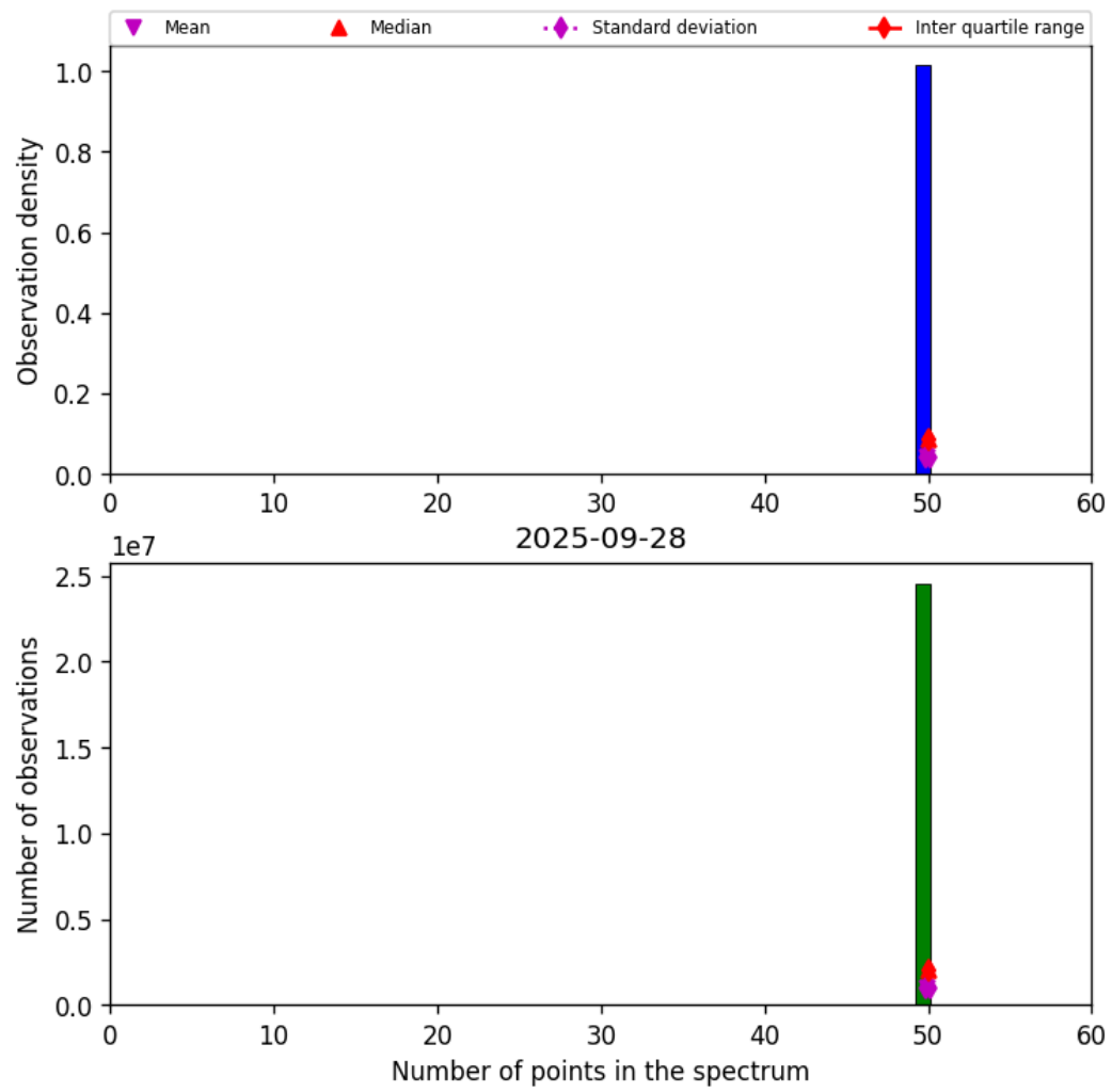
Figure 44: Histogram of “Number of points in the spectrum” for 2025-09-27 to 2025-09-29
