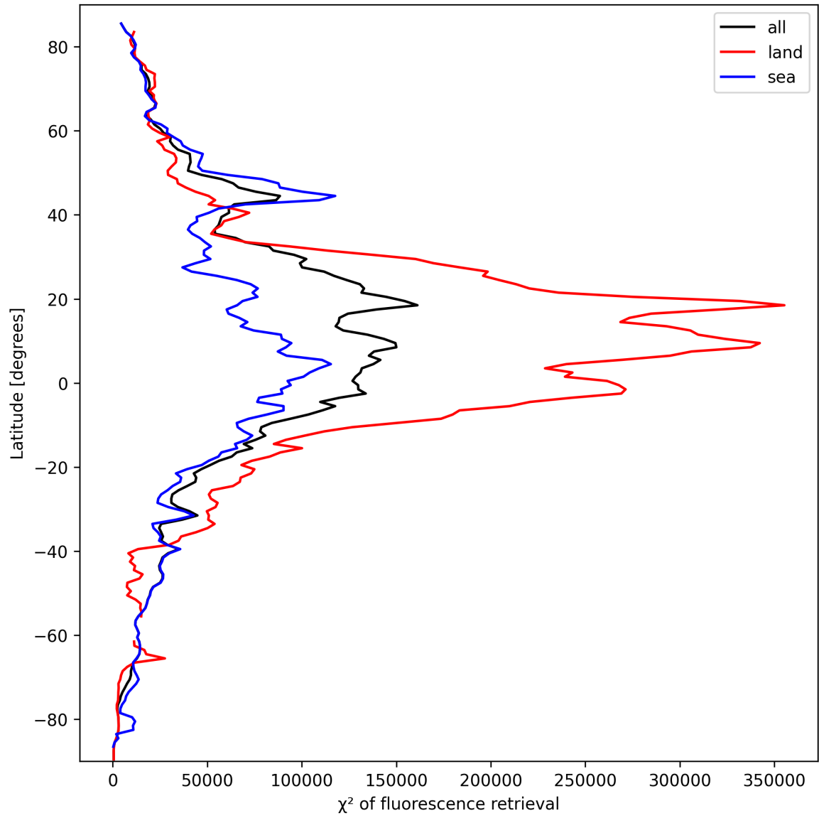
Figure 25: Zonal average of “ \chi^2 of fluorescence retrieval” for 2025-09-27 to 2025-09-29.
