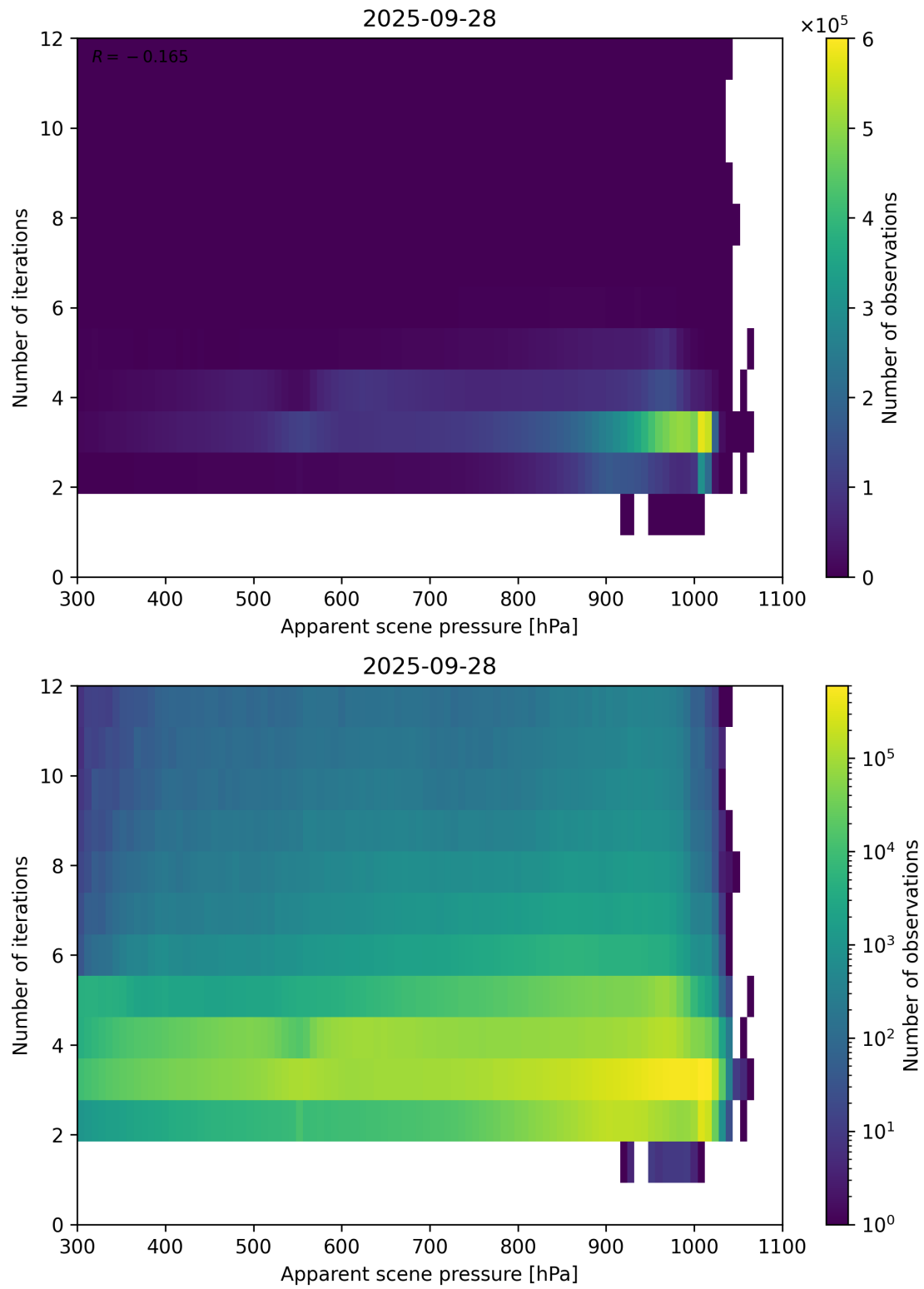
Figure 65: Scatter density plot of “Apparent scene pressure” against “Number of iterations” for 2025-09-27 to 2025-09-29.
