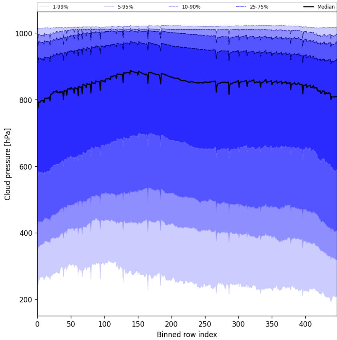
Figure 47: Along track statistics of “Cloud pressure” for 2025-09-27 to 2025-09-29
