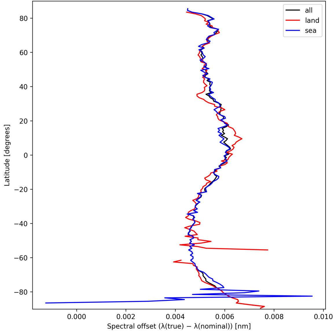
Figure 28: Zonal average of “Spectral offset ( \lambda_{\text{true}} - \lambda_{\text{nominal}} )” for 2025-09-27 to 2025-09-29.
