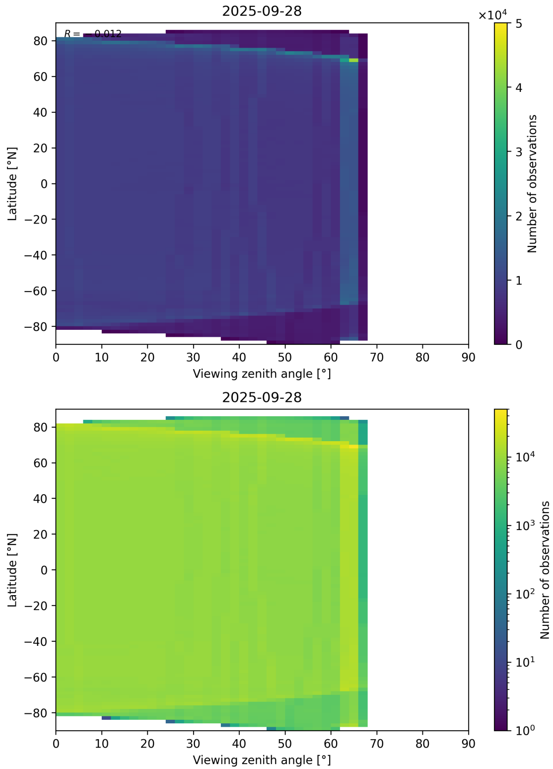
Figure 123: Scatter density plot of “Viewing zenith angle” against “Latitude” for 2025-09-27 to 2025-09-29.
