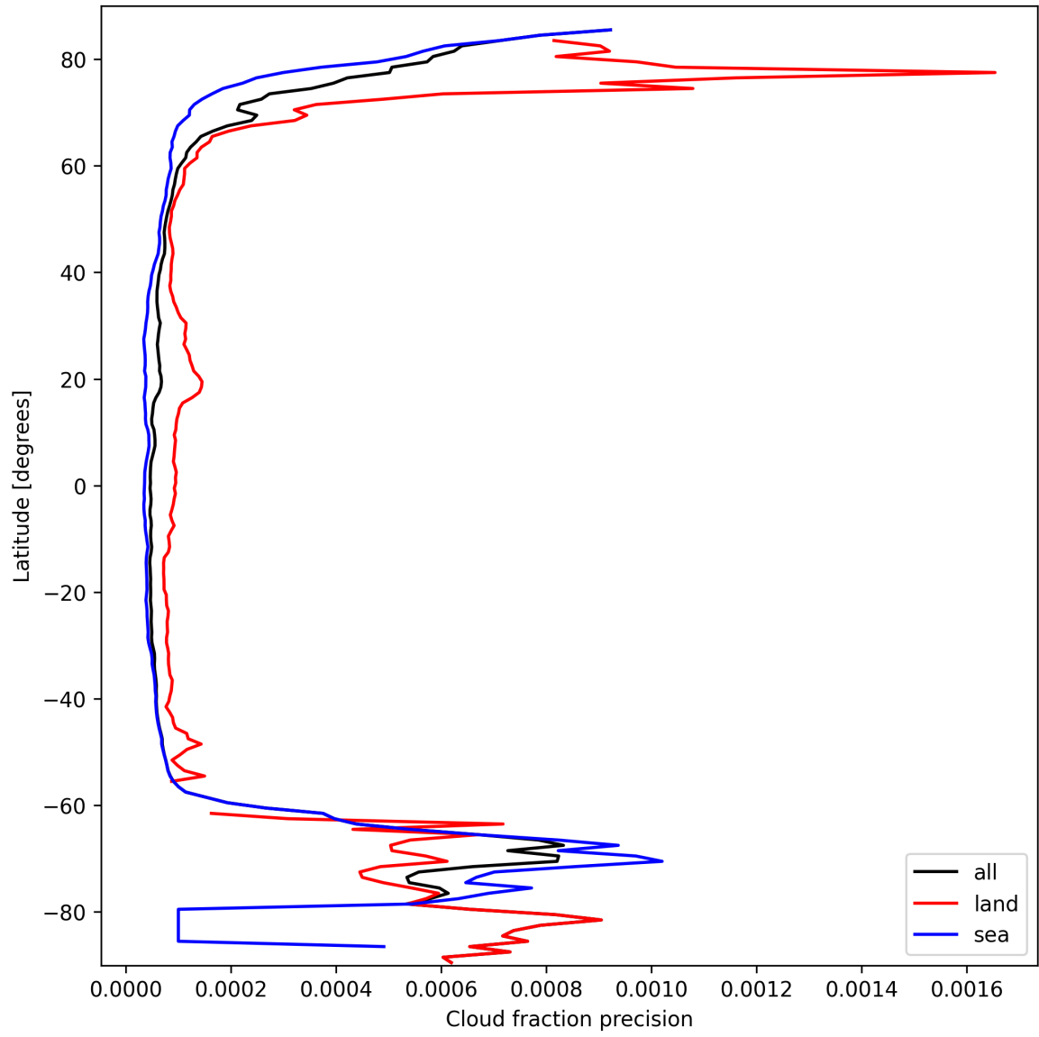
Figure 16: Zonal average of “Cloud fraction precision” for 2025-09-27 to 2025-09-29.
