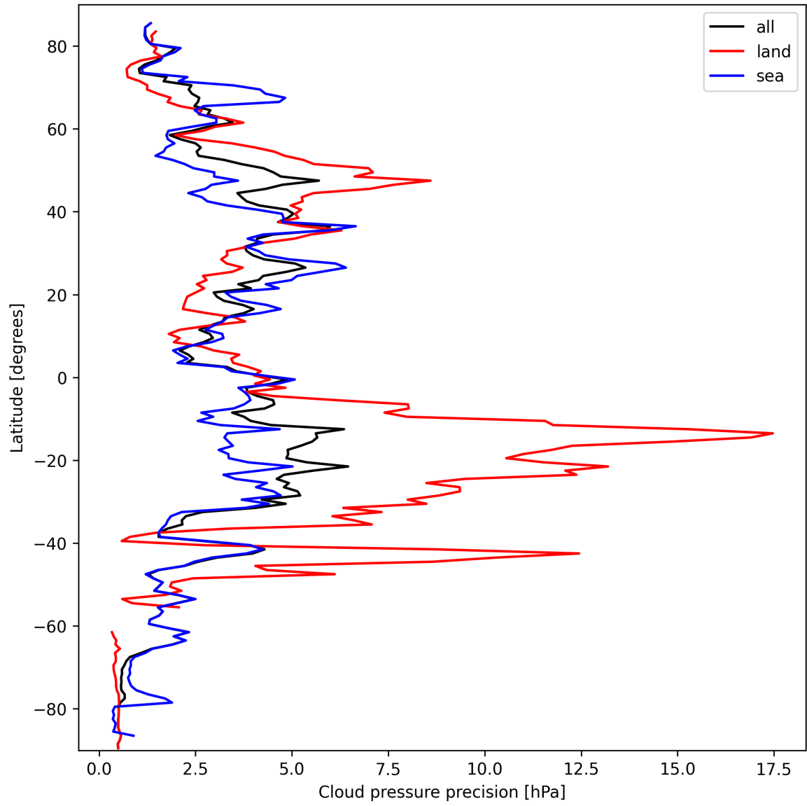
Figure 14: Zonal average of “Cloud pressure precision” for 2025-09-27 to 2025-09-29.
