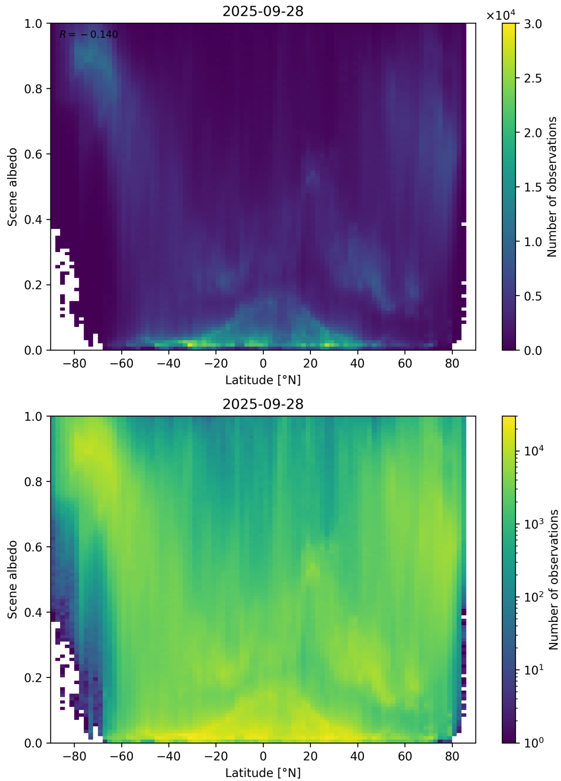
Figure 95: Scatter density plot of “Latitude” against “Scene albedo” for 2025-09-27 to 2025-09-29.
