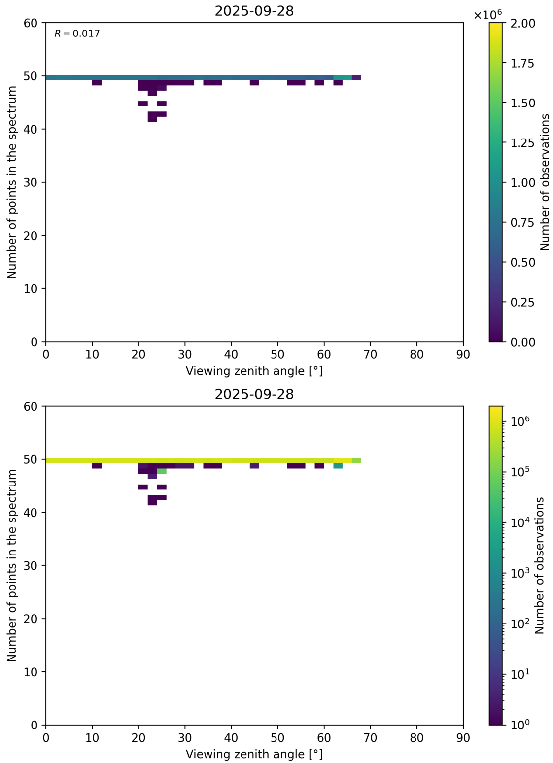
Figure 125: Scatter density plot of “Viewing zenith angle” against “Number of points in the spectrum” for 2025-09-27 to 2025-09-29.
