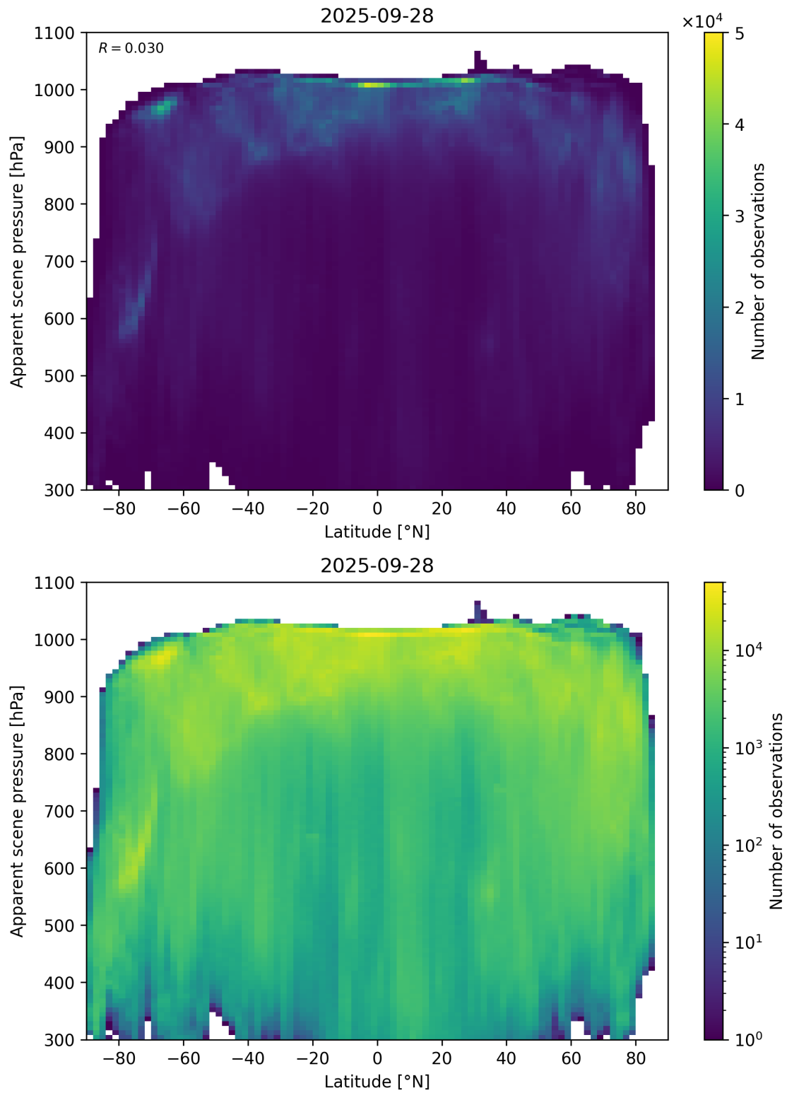
Figure 88: Scatter density plot of “Latitude” against “Apparent scene pressure” for 2025-09-27 to 2025-09-29.
