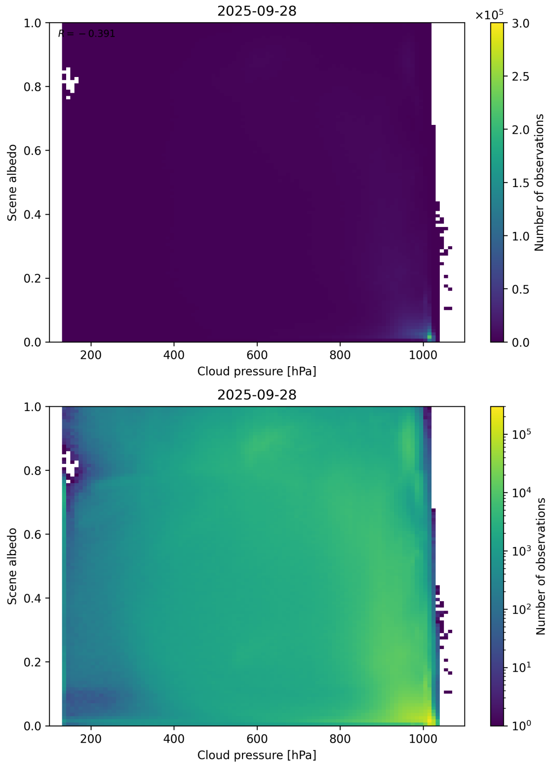
Figure 83: Scatter density plot of “Cloud pressure” against “Scene albedo” for 2025-09-27 to 2025-09-29.
