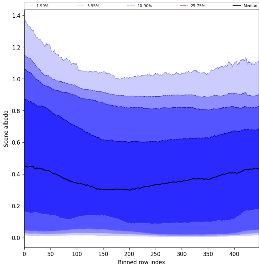
Figure 51: Along track statistics of “Scene albedo” for 2025-09-27 to 2025-09-29
