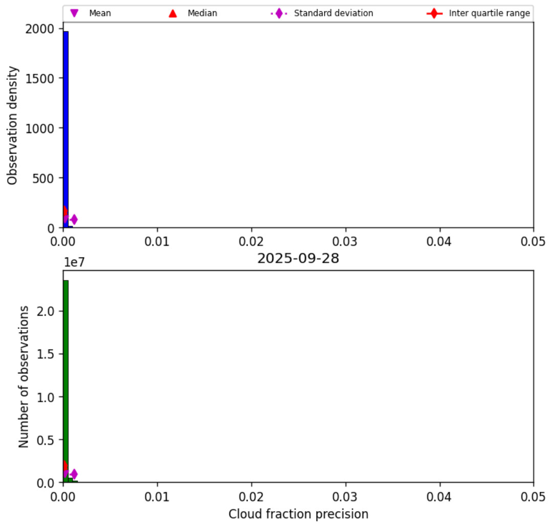
Figure 33: Histogram of “Cloud fraction precision” for 2025-09-27 to 2025-09-29
