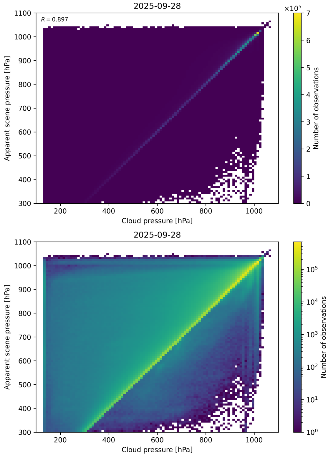
Figure 77: Scatter density plot of “Cloud pressure” against “Apparent scene pressure” for 2025-09-27 to 2025-09-29.
