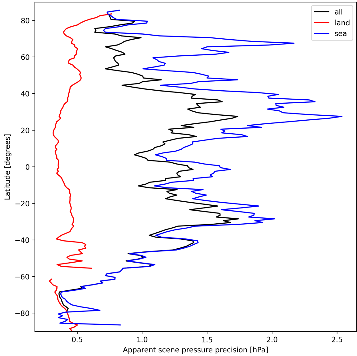
Figure 20: Zonal average of “Apparent scene pressure precision” for 2025-09-27 to 2025-09-29.
