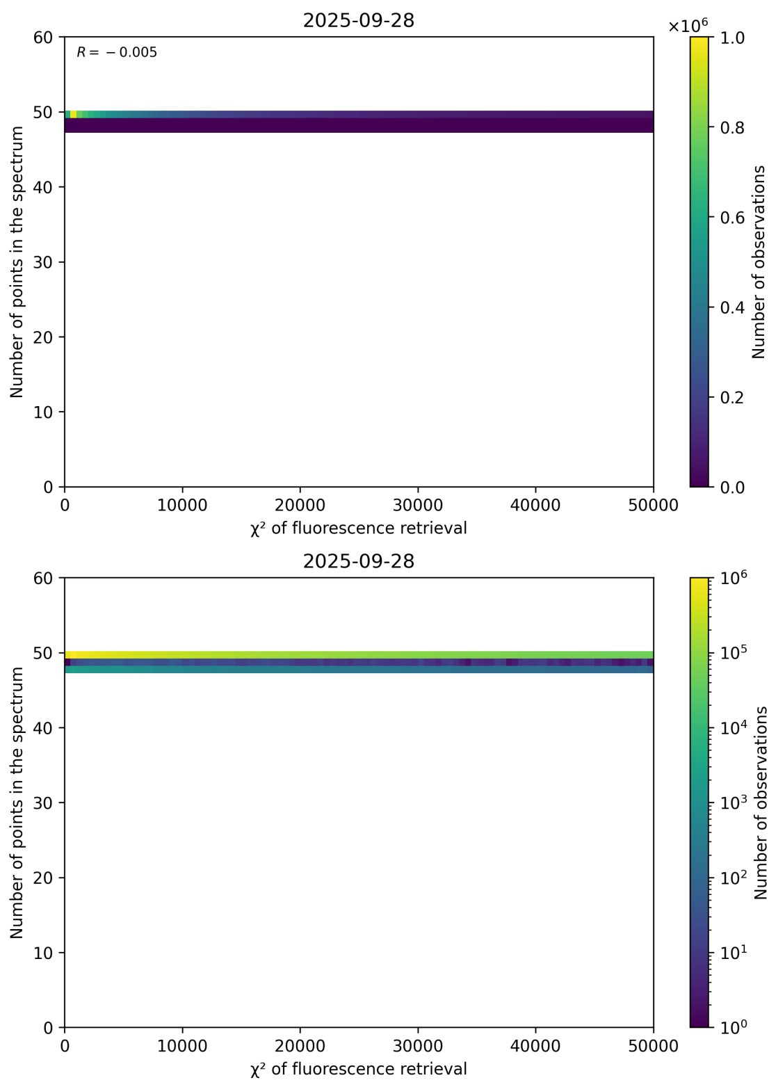
Figure 68: Scatter density plot of " \chi^2 of fluorescence retrieval" against "Number of points in the spectrum" for 2025-09-27 to 2025-09-29.
