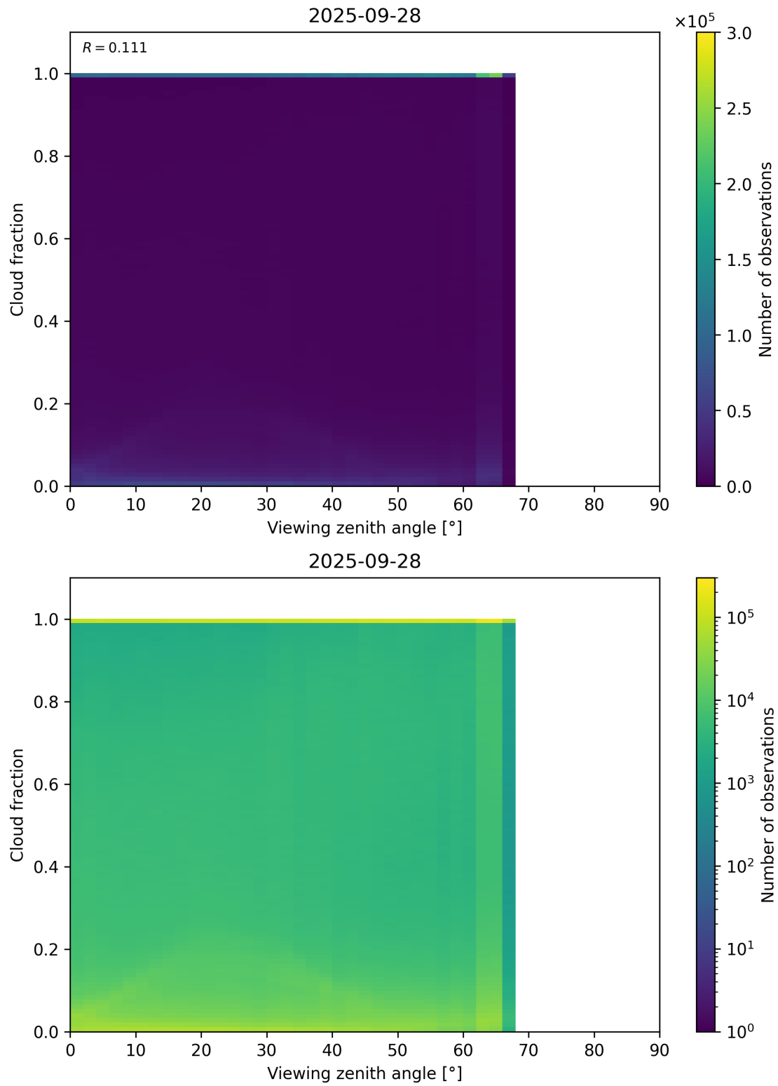
Figure 120: Scatter density plot of “Viewing zenith angle” against “Cloud fraction” for 2025-09-27 to 2025-09-29.
