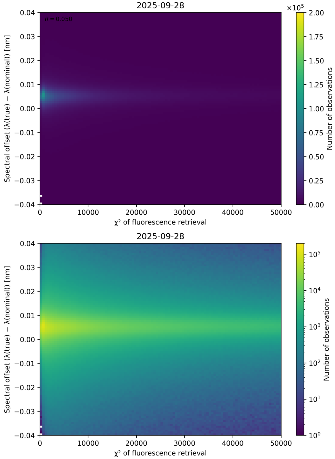
Figure 69: Scatter density plot of “ \chi^2 of fluorescence retrieval” against “Spectral offset ( \lambda_{\text{true}} - \lambda_{\text{nominal}} )” for 2025-09-27 to 2025-09-29.
