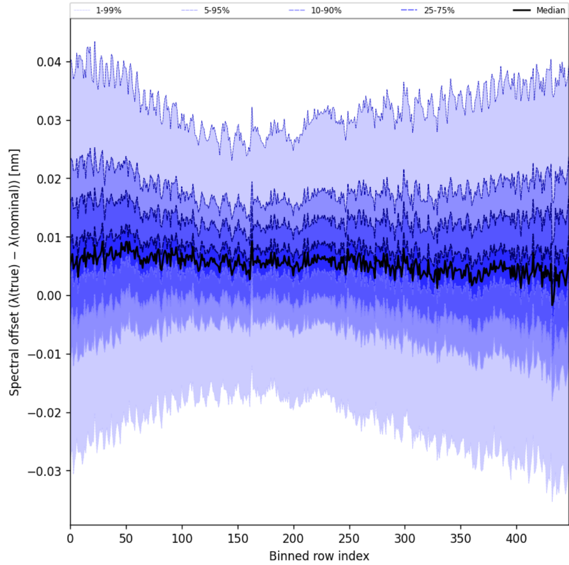
Figure 62: Along track statistics of “Spectral offset ( \lambda_{\text{true}} - \lambda_{\text{nominal}} )” for 2025-09-27 to 2025-09-29
