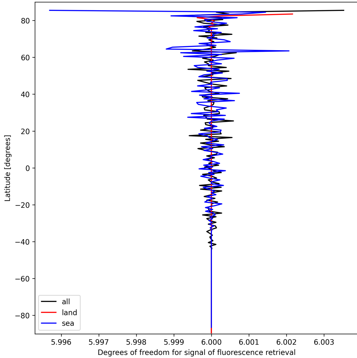
Figure 26: Zonal average of “Degrees of freedom for signal of fluorescence retrieval” for 2025-09-27 to 2025-09-29.
