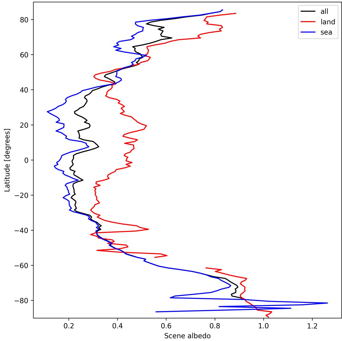
Figure 17: Zonal average of “Scene albedo” for 2025-09-27 to 2025-09-29.
