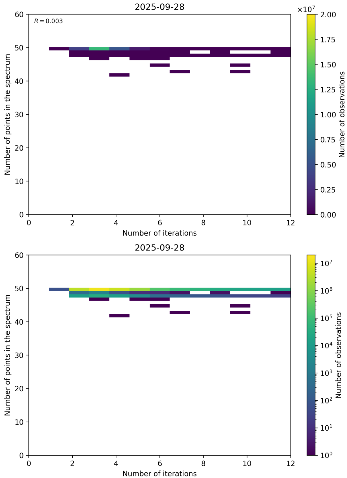
Figure 99: Scatter density plot of “Number of iterations” against “Number of points in the spectrum” for 2025-09-27 to 2025-09-29.
