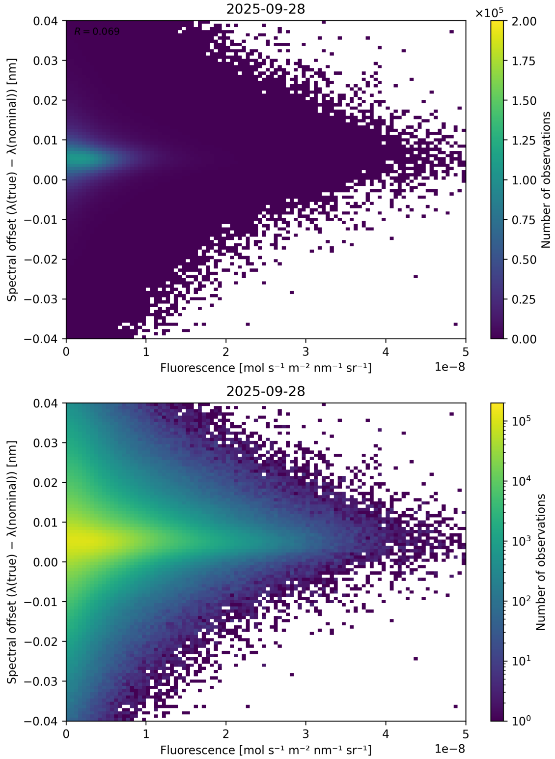
Figure 87: Scatter density plot of “Fluorescence” against “Spectral offset ( \lambda_{\text{true}} - \lambda_{\text{nominal}} )” for 2025-09-27 to 2025-09-29.
