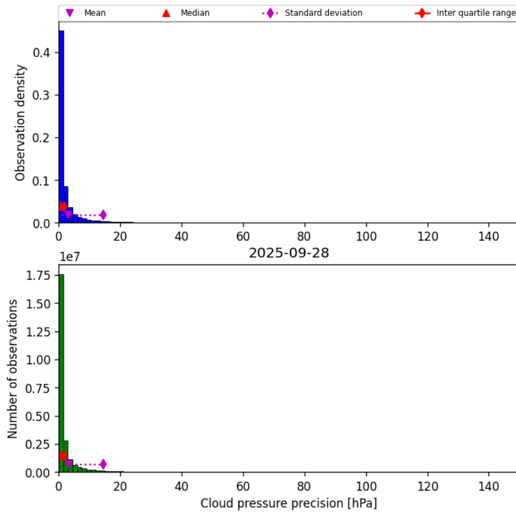
Figure 31: Histogram of “Cloud pressure precision” for 2025-09-27 to 2025-09-29
