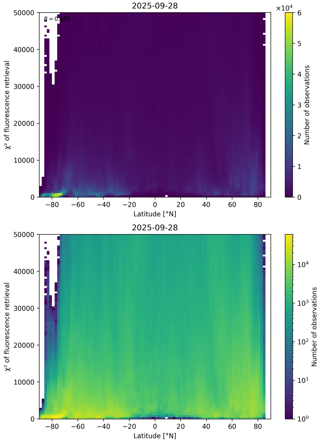
Figure 89: Scatter density plot of “Latitude” against “ \chi^2 of fluorescence retrieval” for 2025-09-27 to 2025-09-29.
