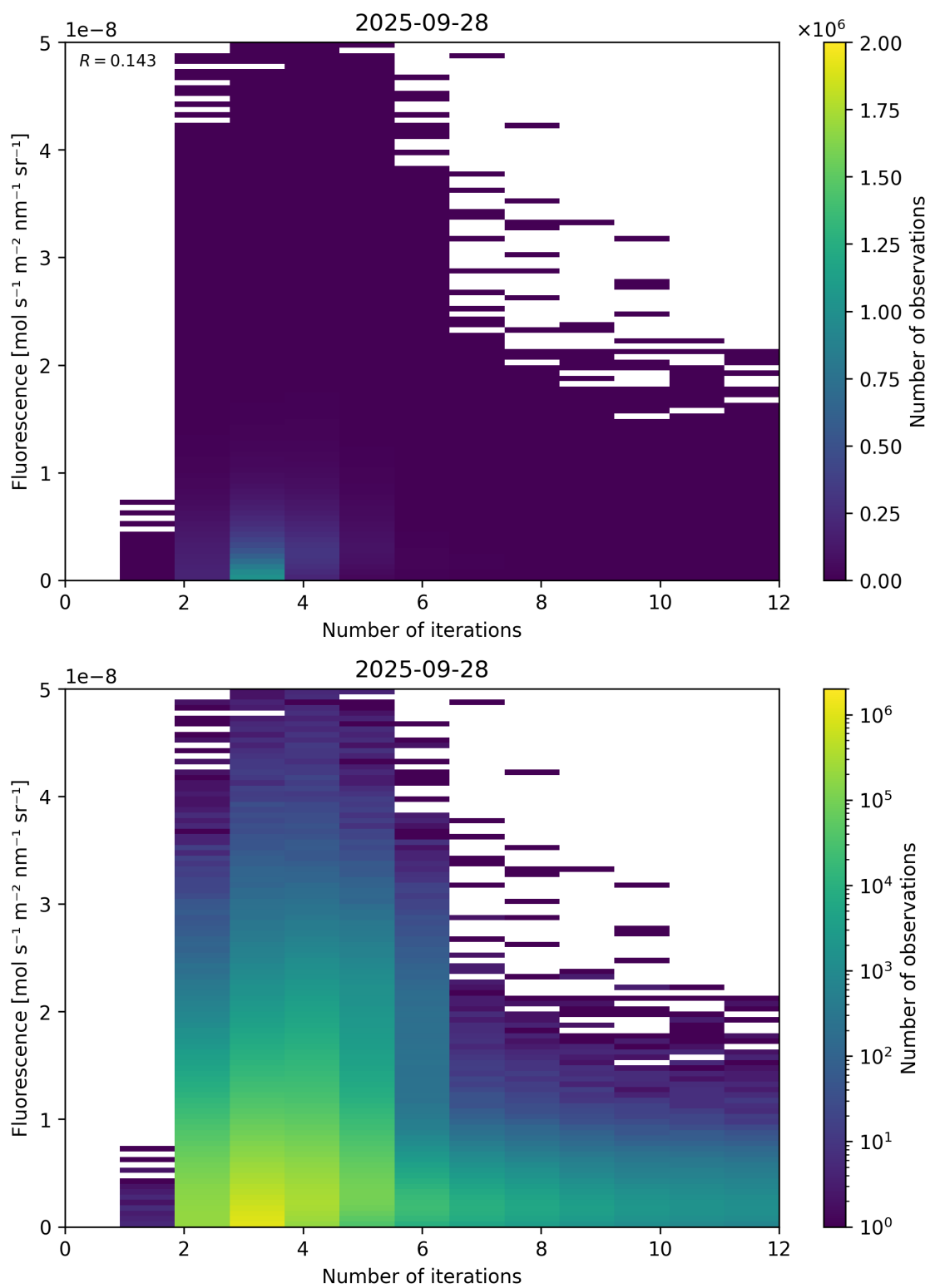
Figure 98: Scatter density plot of “Number of iterations” against “Fluorescence” for 2025-09-27 to 2025-09-29.
