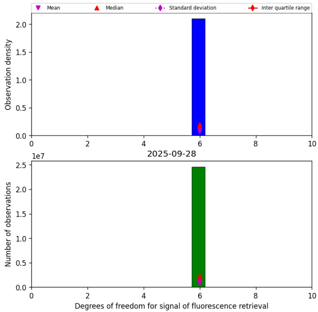
Figure 43: Histogram of “Degrees of freedom for signal of fluorescence retrieval” for 2025-09-27 to 2025-09-29
