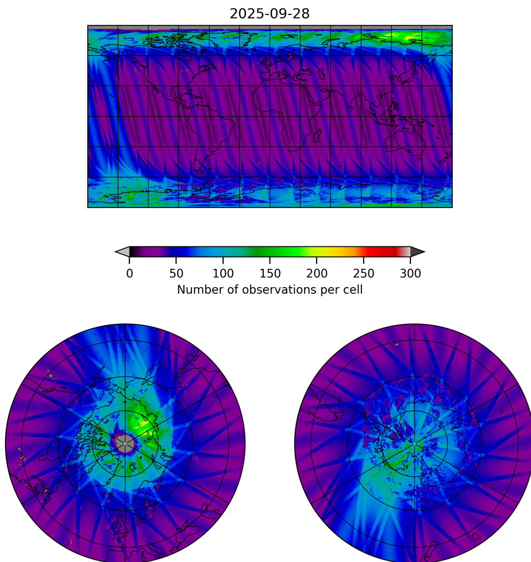
Figure 11: Map of the number of observations for 2025-09-27 to 2025-09-29
