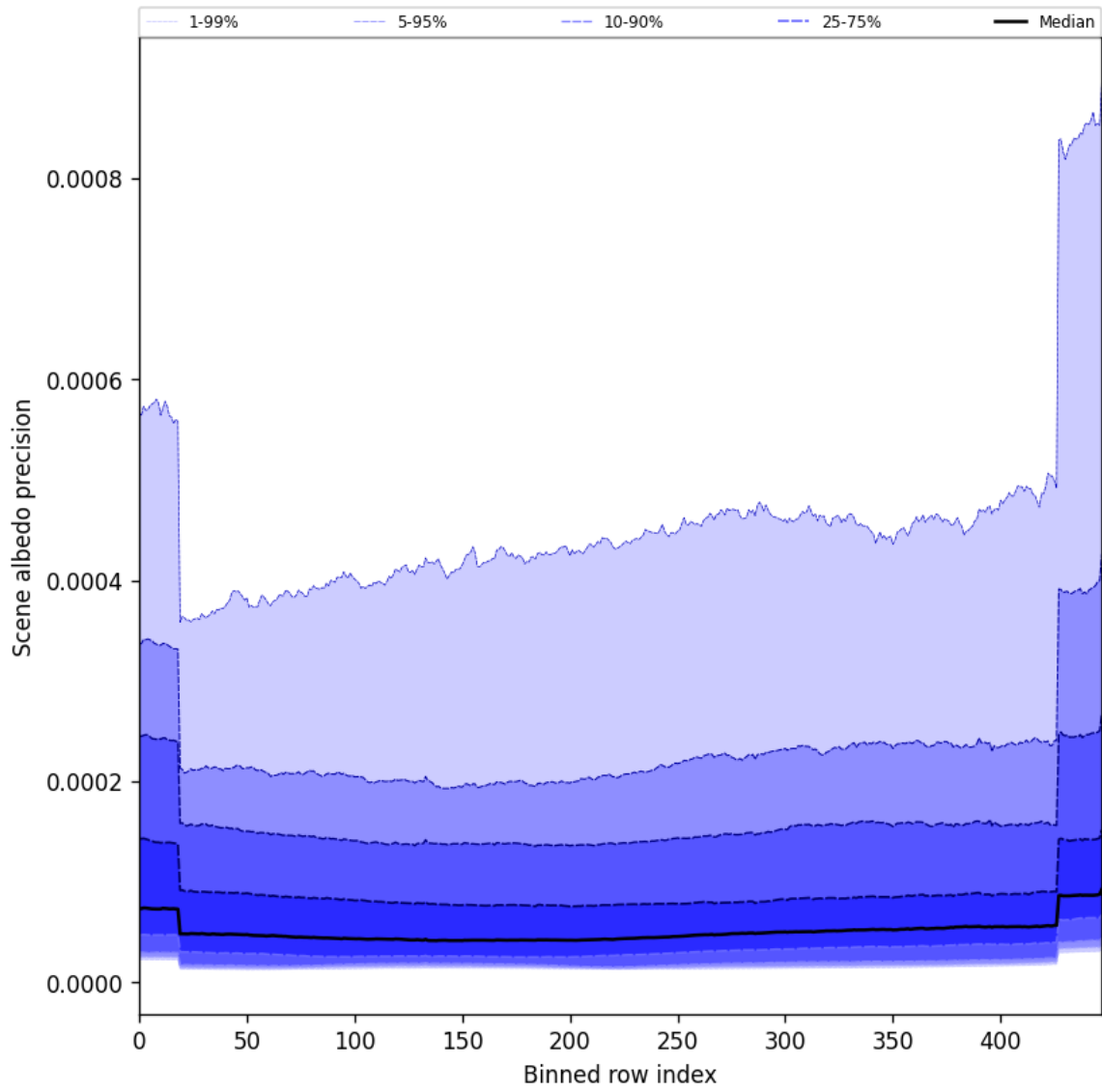
Figure 52: Along track statistics of “Scene albedo precision” for 2025-09-27 to 2025-09-29
