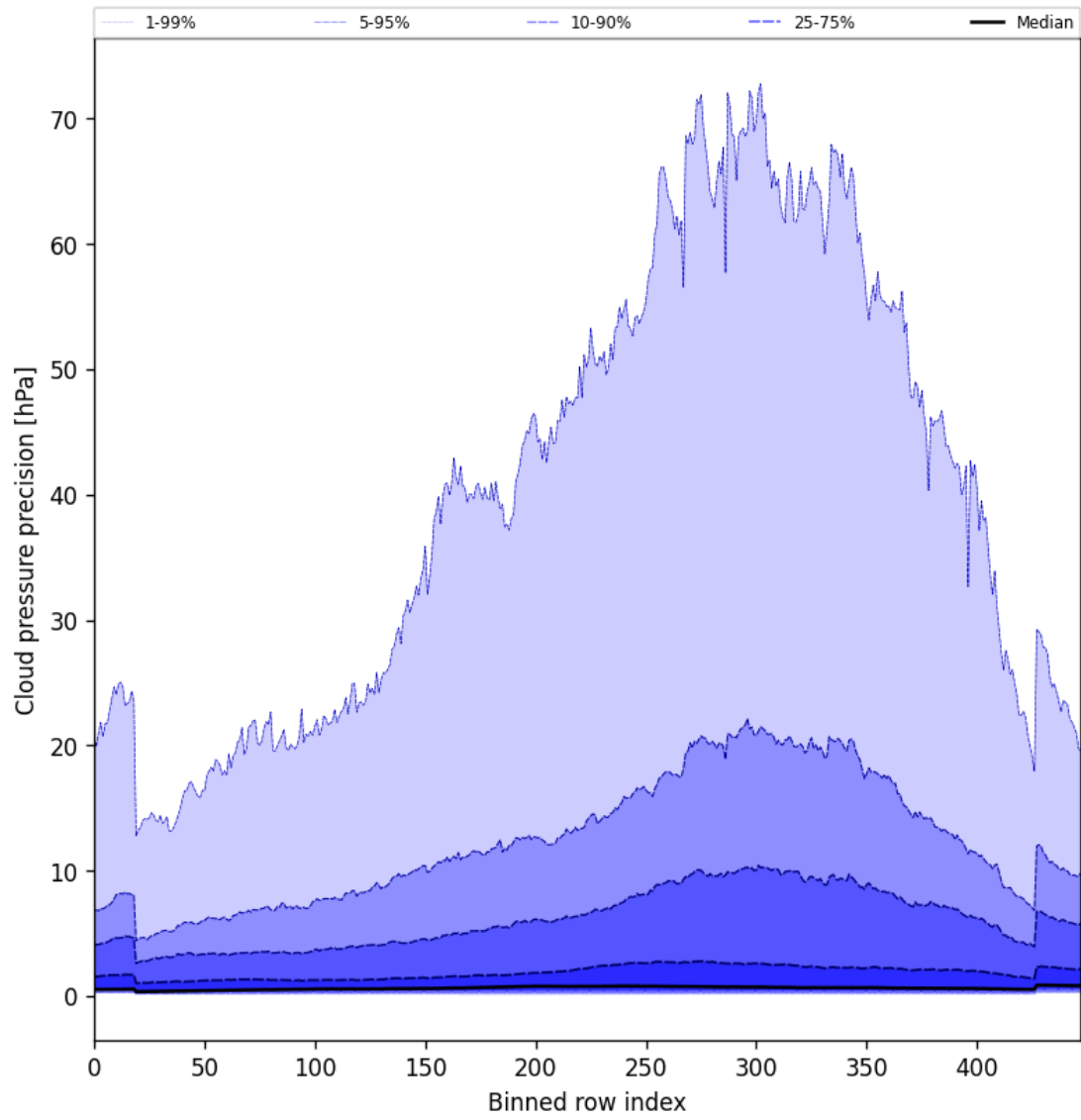
Figure 48: Along track statistics of “Cloud pressure precision” for 2025-09-27 to 2025-09-29
