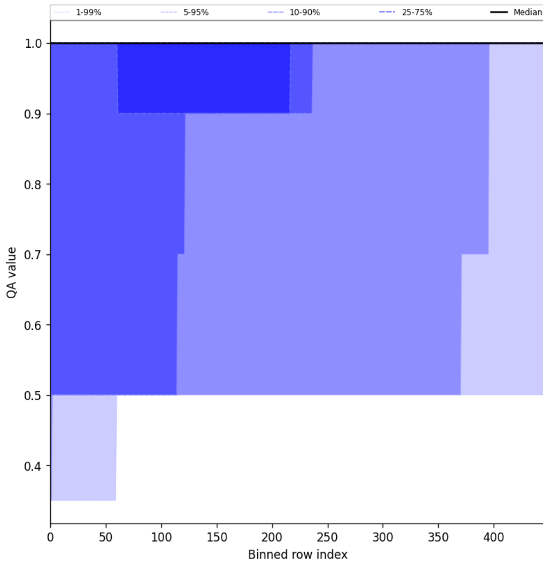
Figure 46: Along track statistics of “QA value” for 2025-09-27 to 2025-09-29
