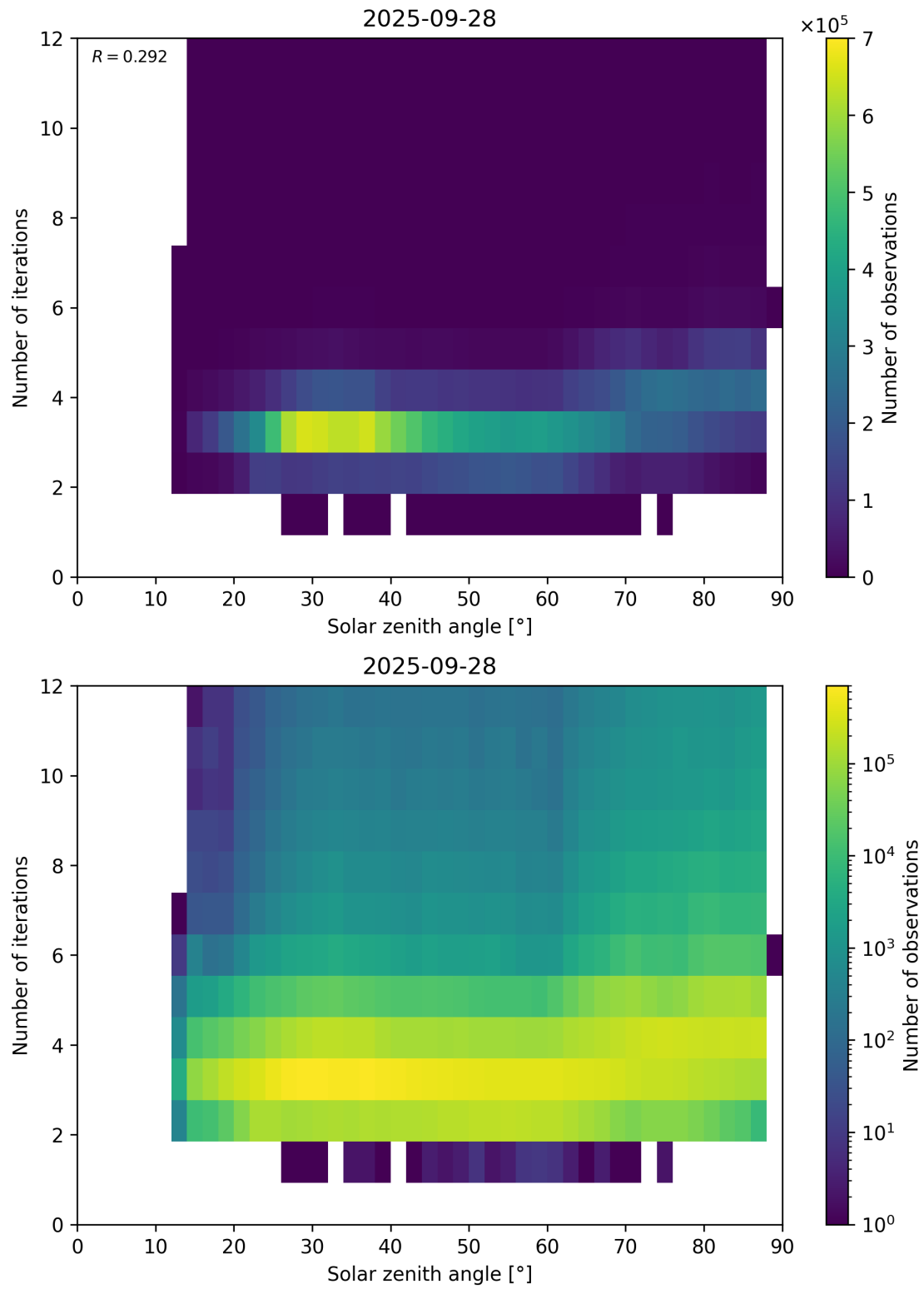
Figure 114: Scatter density plot of “Solar zenith angle” against “Number of iterations” for 2025-09-27 to 2025-09-29.
