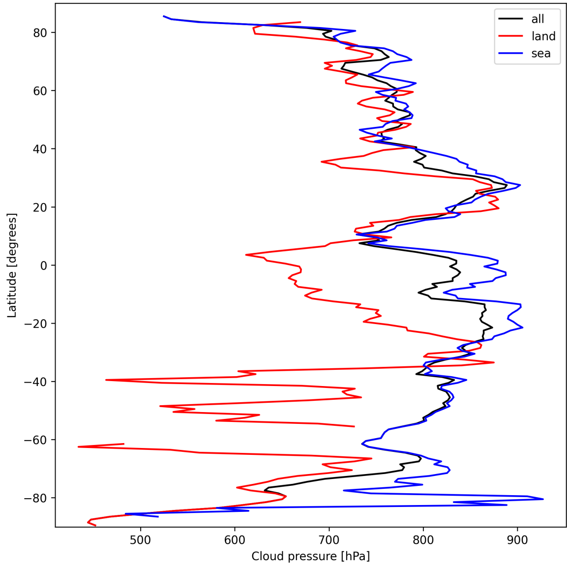
Figure 13: Zonal average of “Cloud pressure” for 2025-09-27 to 2025-09-29.
