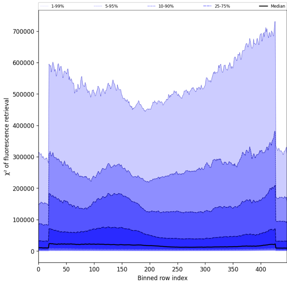
Figure 59: Along track statistics of “ \chi^2 of fluorescence retrieval” for 2025-09-27 to 2025-09-29
