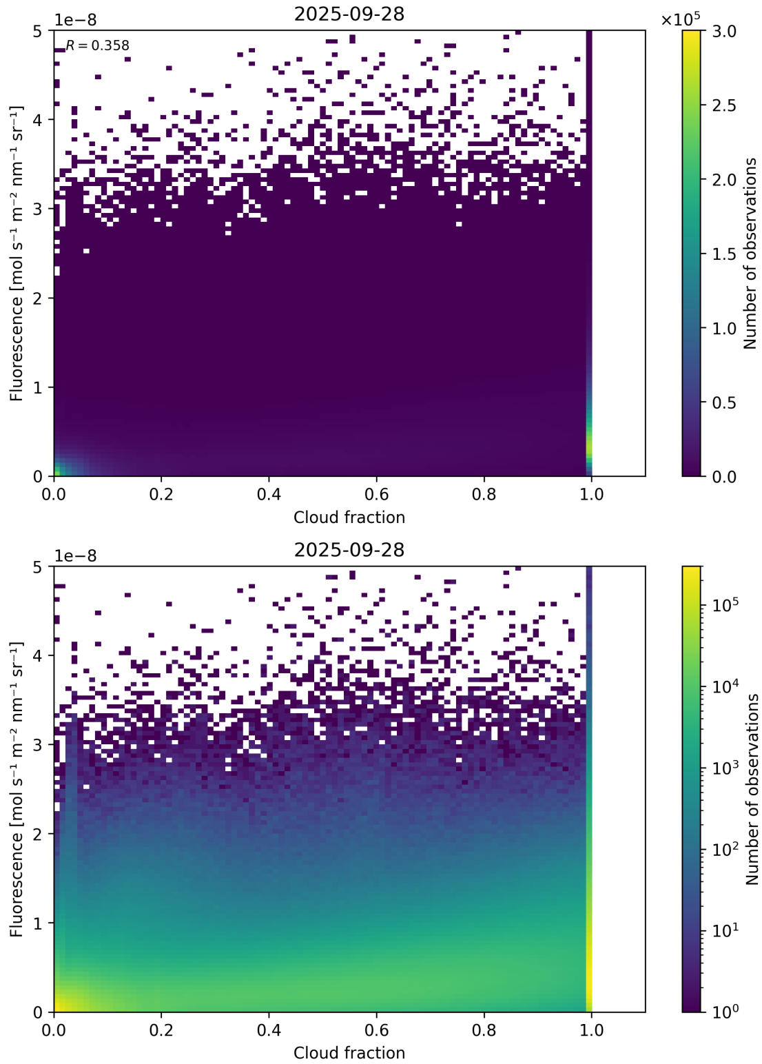
Figure 72: Scatter density plot of “Cloud fraction” against “Fluorescence” for 2025-09-27 to 2025-09-29.
