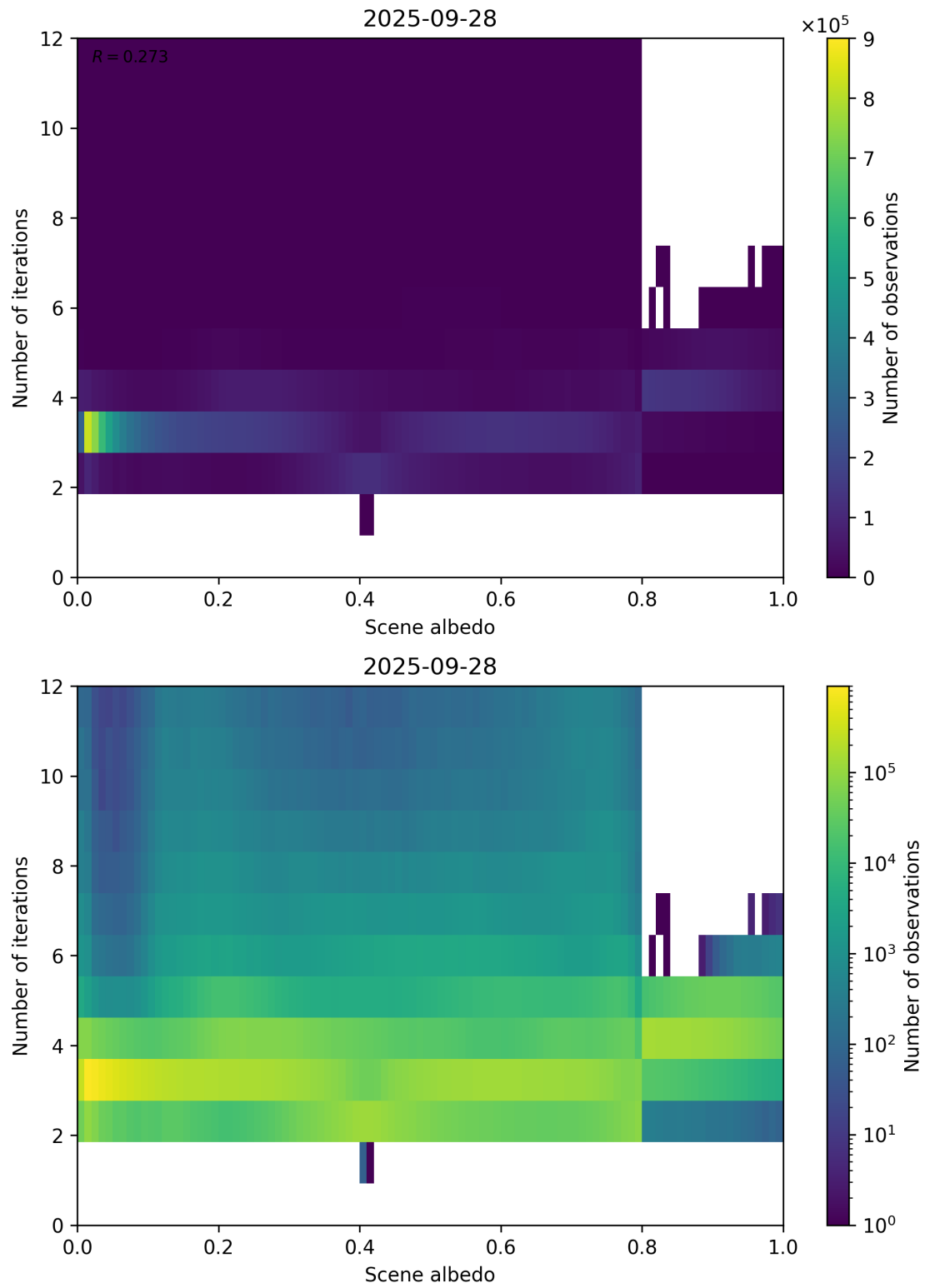
Figure 105: Scatter density plot of “Scene albedo” against “Number of iterations” for 2025-09-27 to 2025-09-29.
