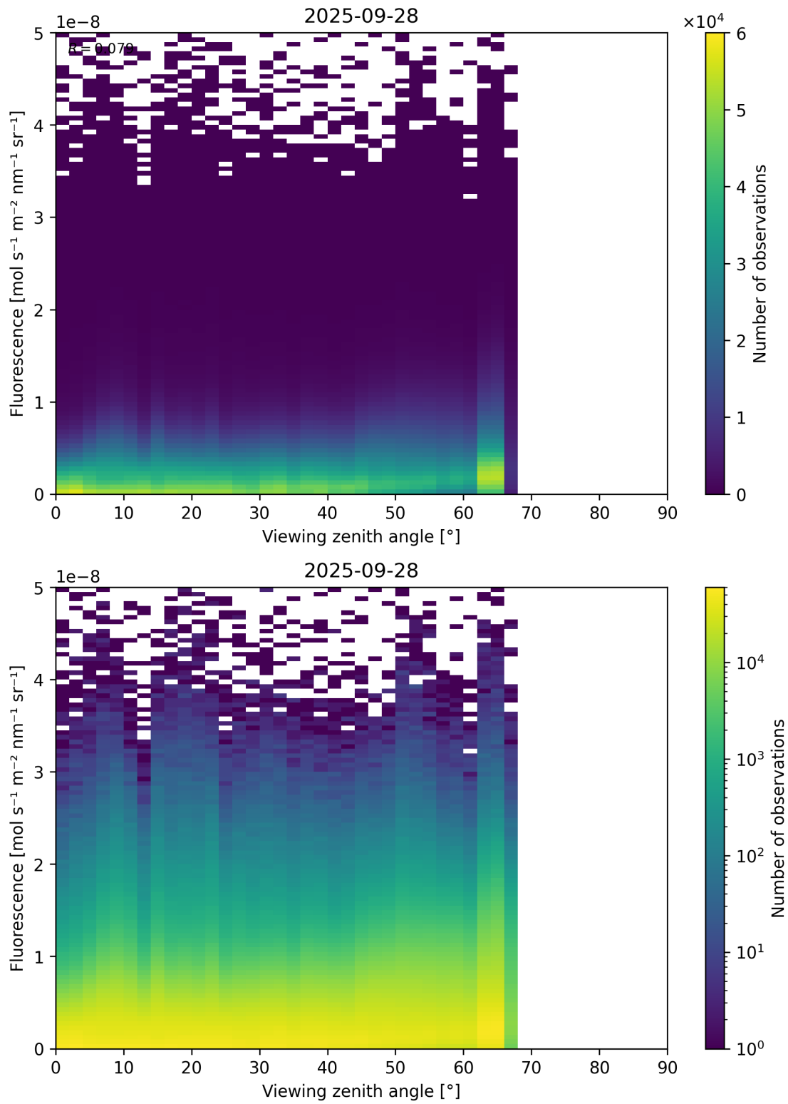
Figure 122: Scatter density plot of “Viewing zenith angle” against “Fluorescence” for 2025-09-27 to 2025-09-29.
