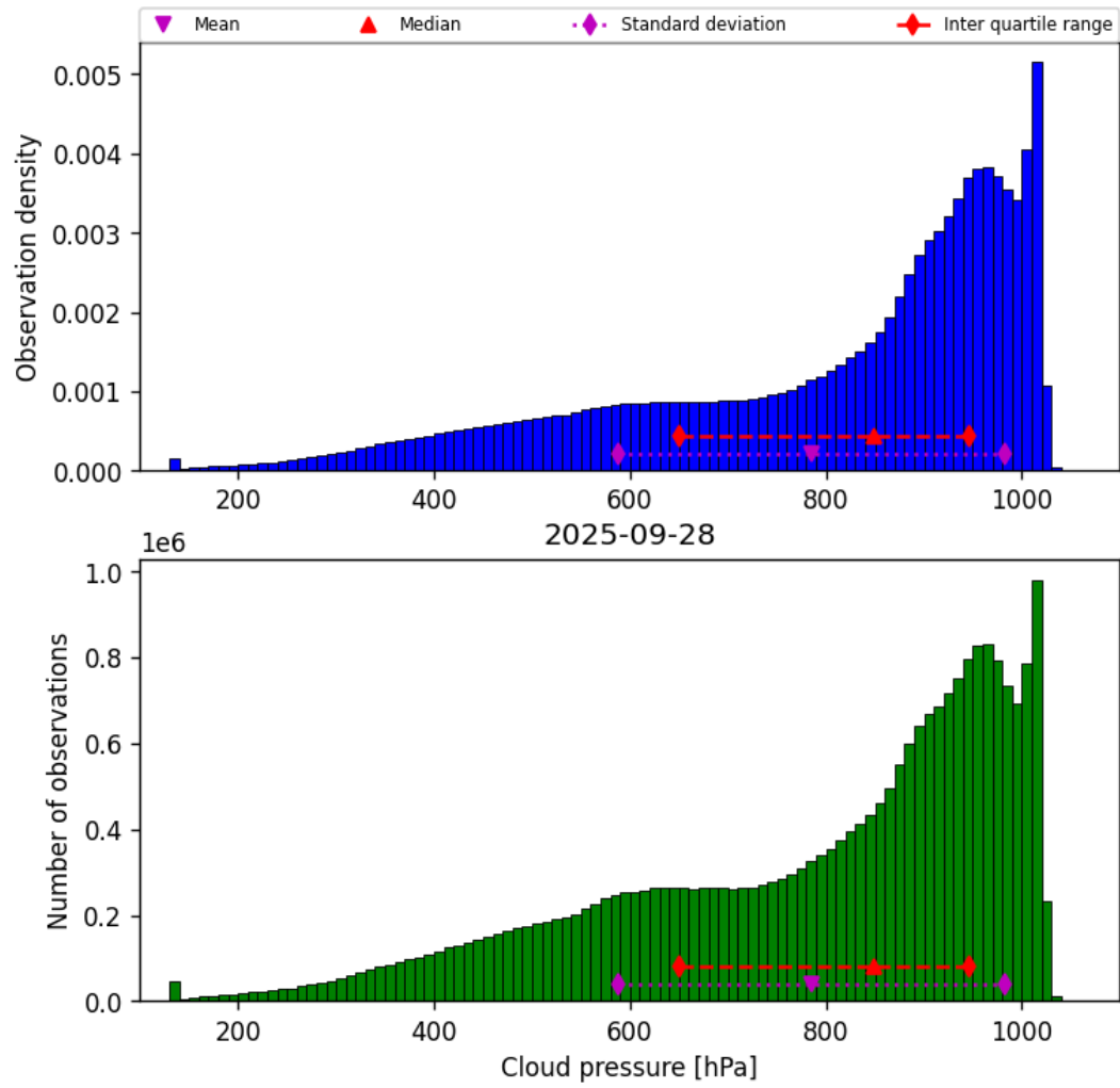
Figure 30: Histogram of “Cloud pressure” for 2025-09-27 to 2025-09-29
