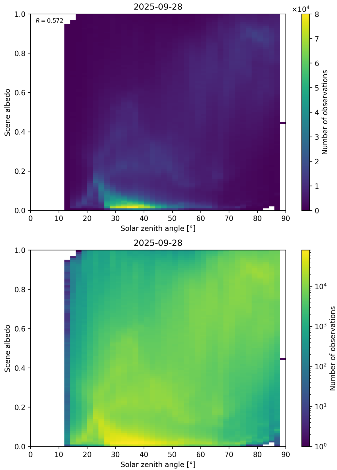
Figure 116: Scatter density plot of “Solar zenith angle” against “Scene albedo” for 2025-09-27 to 2025-09-29.
