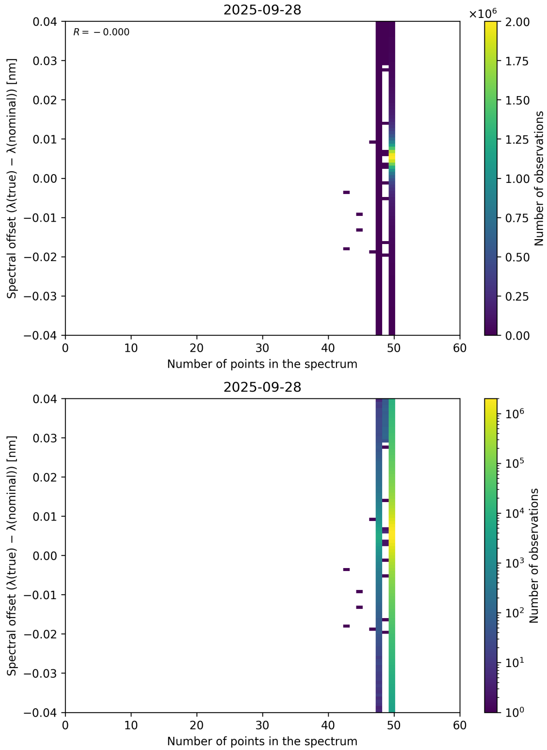
Figure 101: Scatter density plot of “Number of points in the spectrum” against “Spectral offset ( \lambda_{\text{true}} - \lambda_{\text{nominal}} )” for 2025-09-27 to 2025-09-29.
