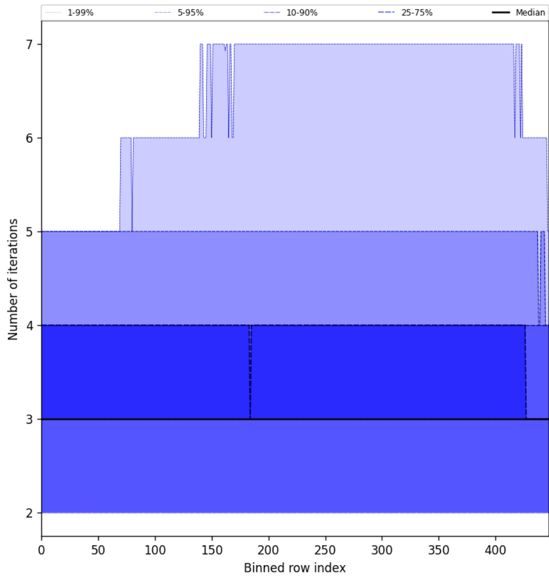
Figure 56: Along track statistics of “Number of iterations” for 2025-09-27 to 2025-09-29
