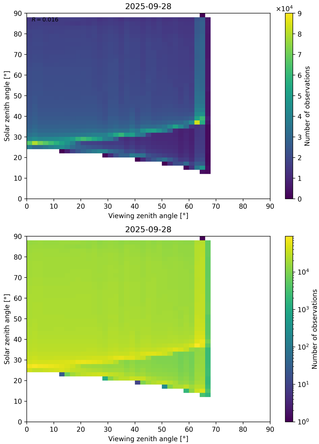
Figure 127: Scatter density plot of “Viewing zenith angle” against “Solar zenith angle” for 2025-09-27 to 2025-09-29.
