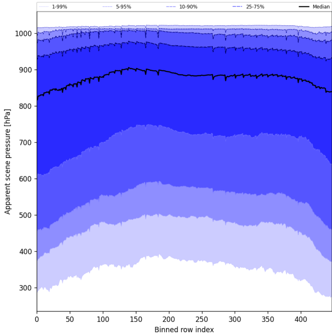
Figure 53: Along track statistics of “Apparent scene pressure” for 2025-09-27 to 2025-09-29
