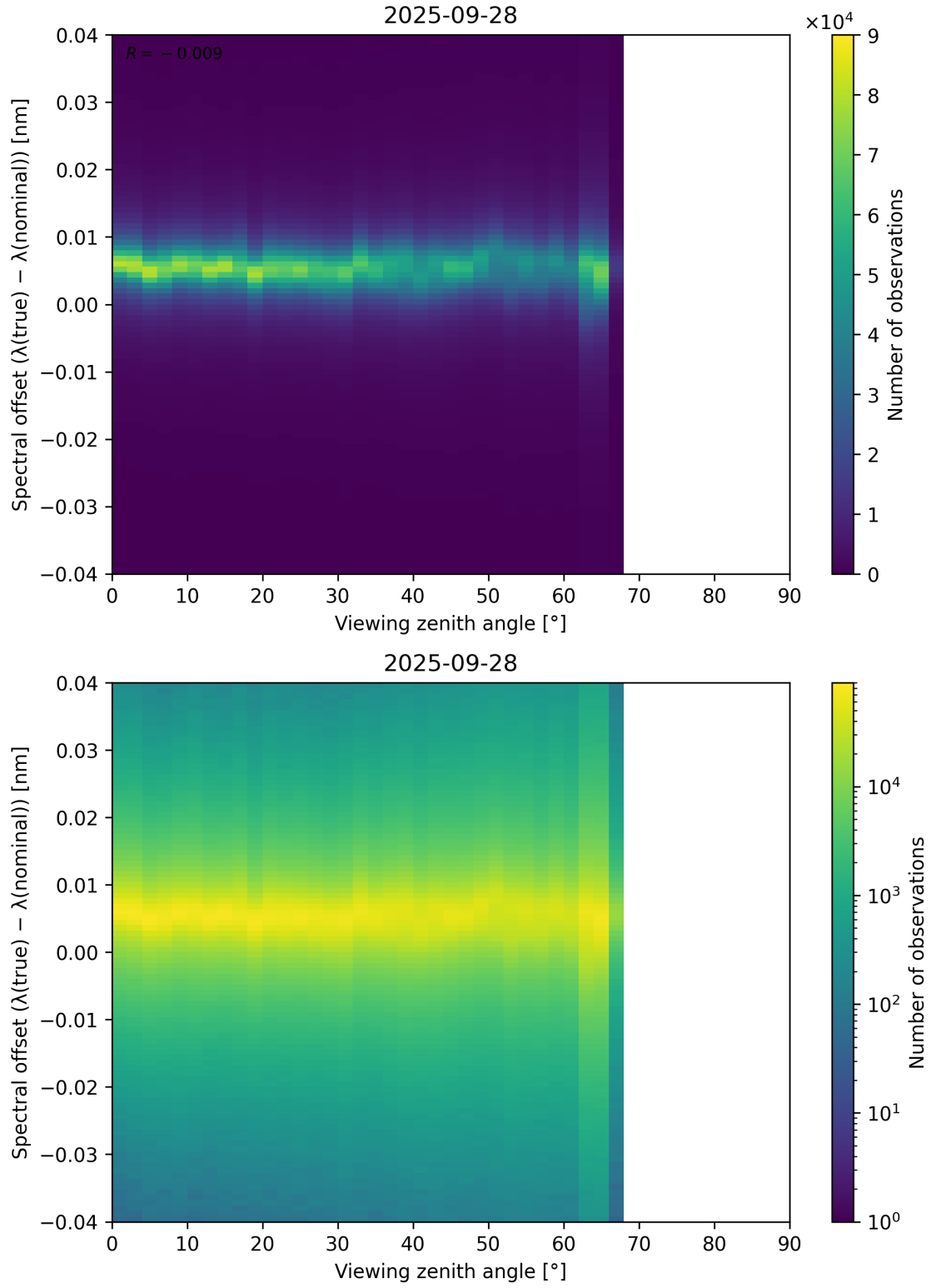
Figure 128: Scatter density plot of “Viewing zenith angle” against “Spectral offset ( \lambda_{\text{true}} - \lambda_{\text{nominal}} )” for 2025-09-27 to 2025-09-29.
