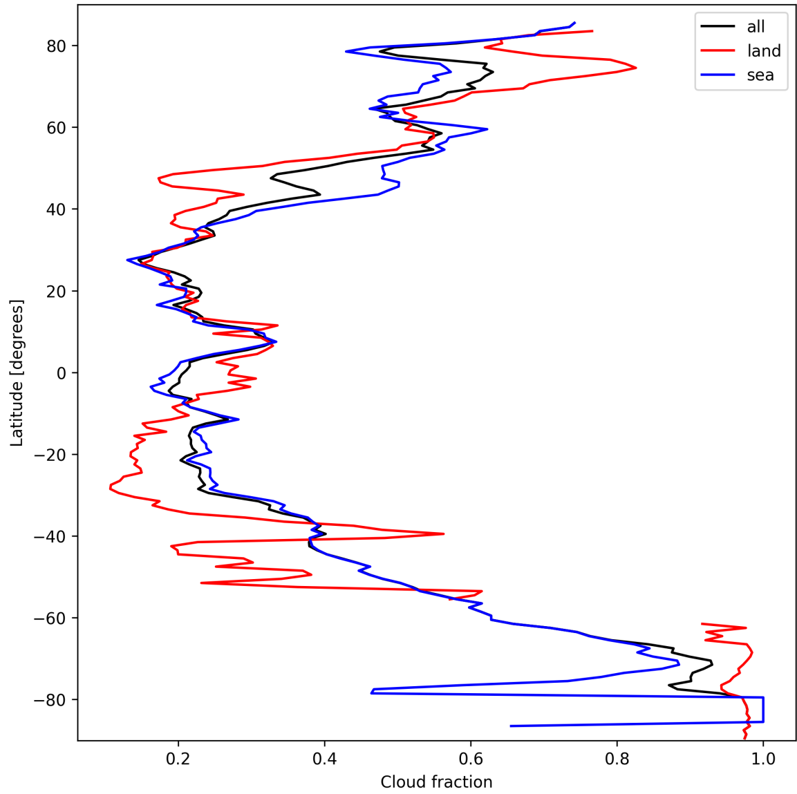
Figure 15: Zonal average of “Cloud fraction” for 2025-09-27 to 2025-09-29.
