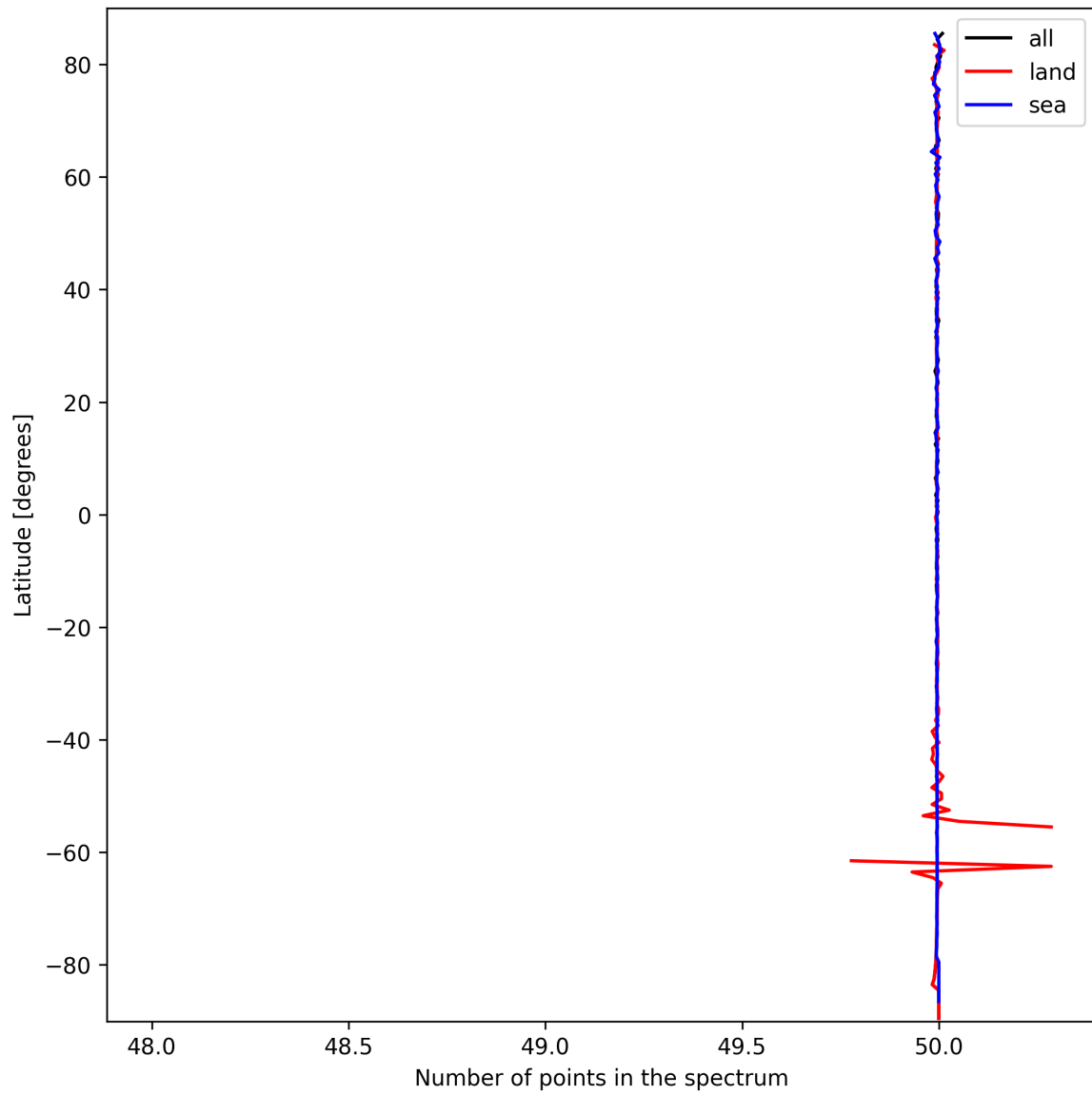
Figure 27: Zonal average of “Number of points in the spectrum” for 2025-09-27 to 2025-09-29.
