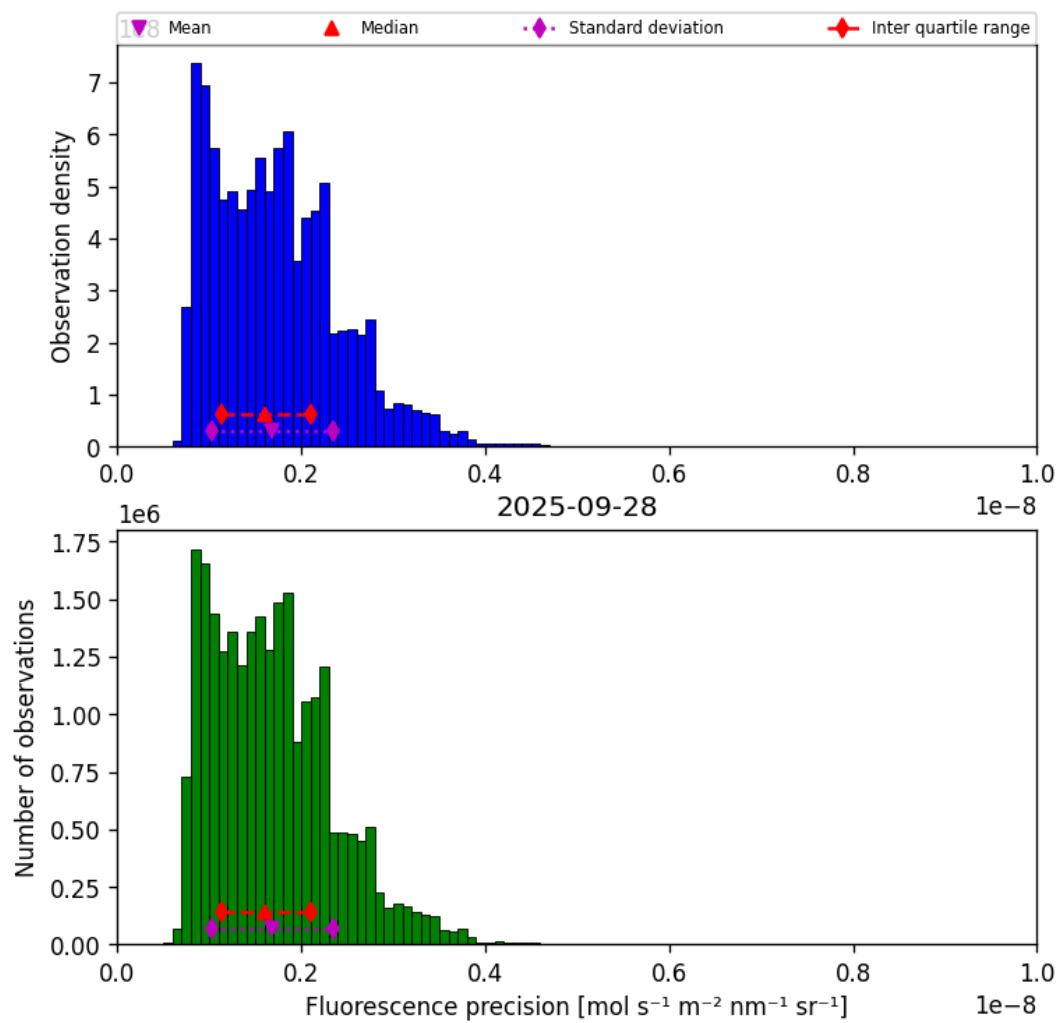
Figure 41: Histogram of “Fluorescence precision” for 2025-09-27 to 2025-09-29
