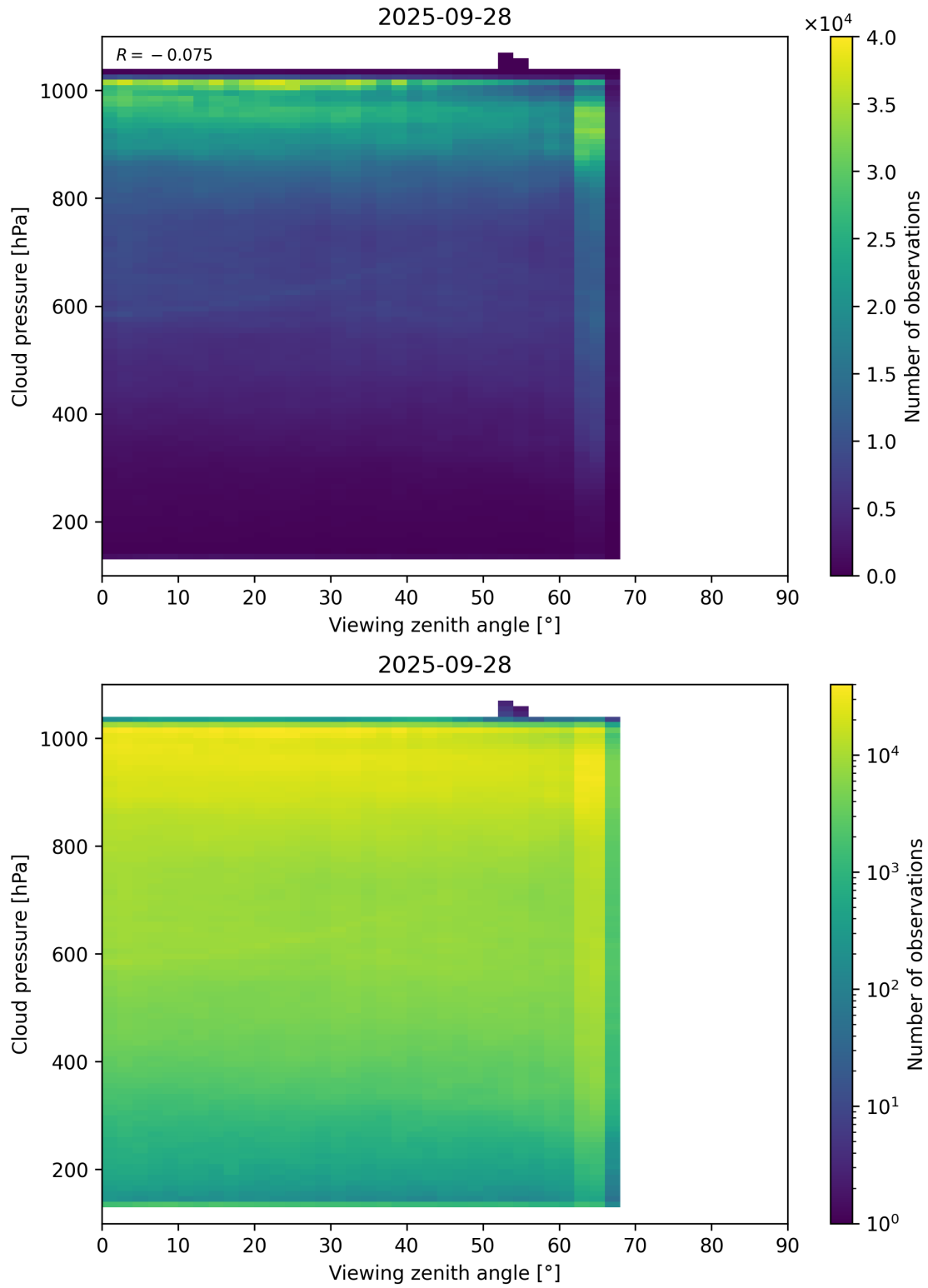
Figure 121: Scatter density plot of “Viewing zenith angle” against “Cloud pressure” for 2025-09-27 to 2025-09-29.
