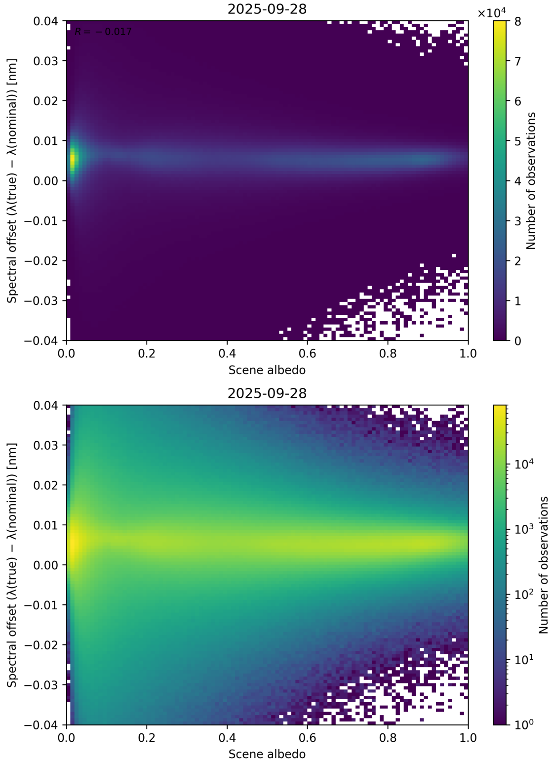
Figure 107: Scatter density plot of “Scene albedo” against “Spectral offset ( \lambda_{\text{true}} - \lambda_{\text{nominal}} )” for 2025-09-27 to 2025-09-29.
