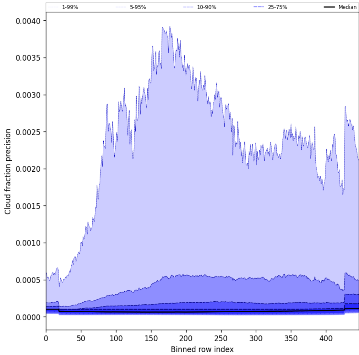
Figure 50: Along track statistics of “Cloud fraction precision” for 2025-09-27 to 2025-09-29
