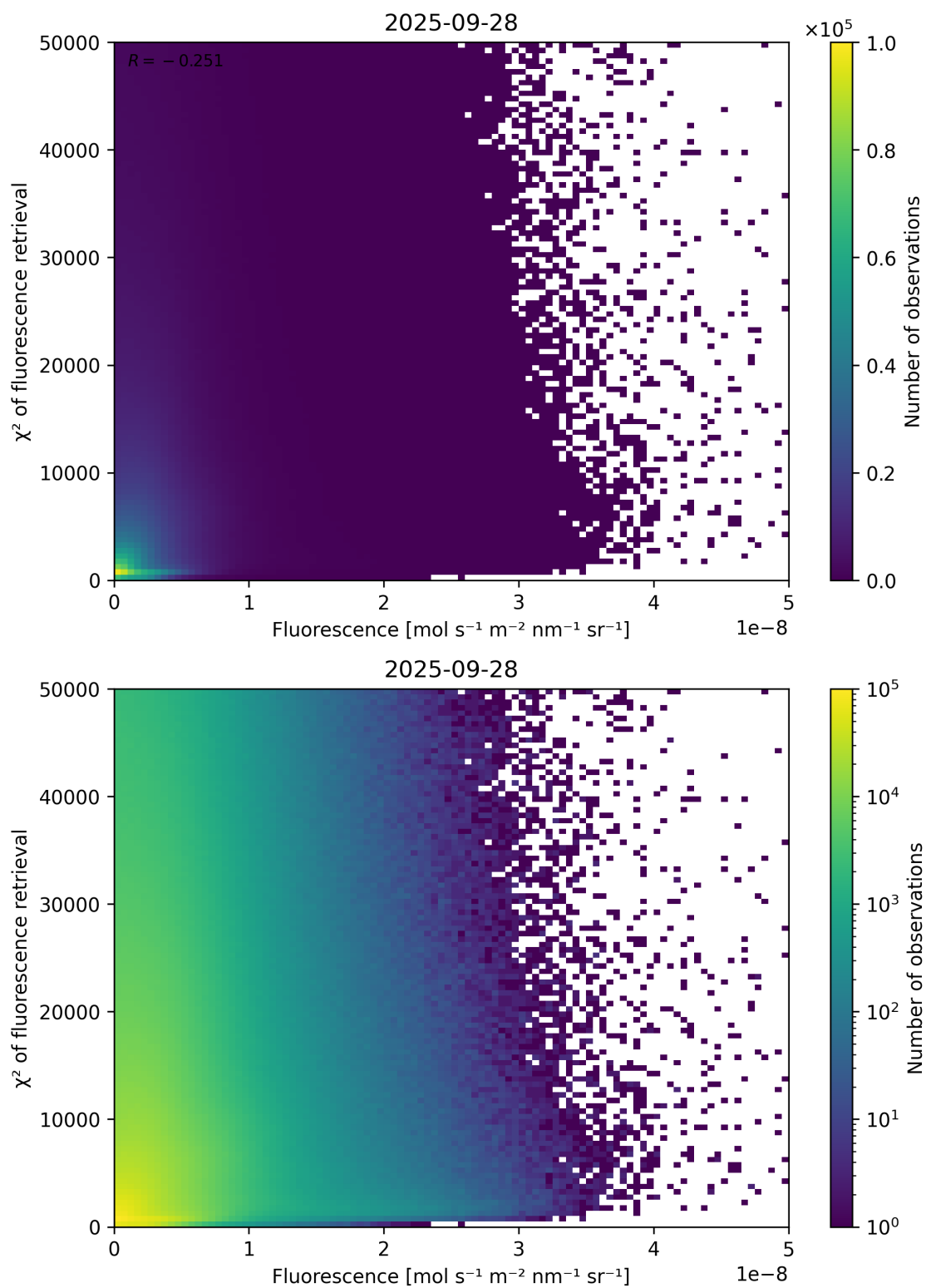
Figure 85: Scatter density plot of “Fluorescence” against “ \chi^2 of fluorescence retrieval” for 2025-09-27 to 2025-09-29.
