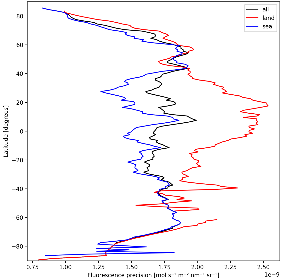
Figure 24: Zonal average of “Fluorescence precision” for 2025-09-27 to 2025-09-29.
