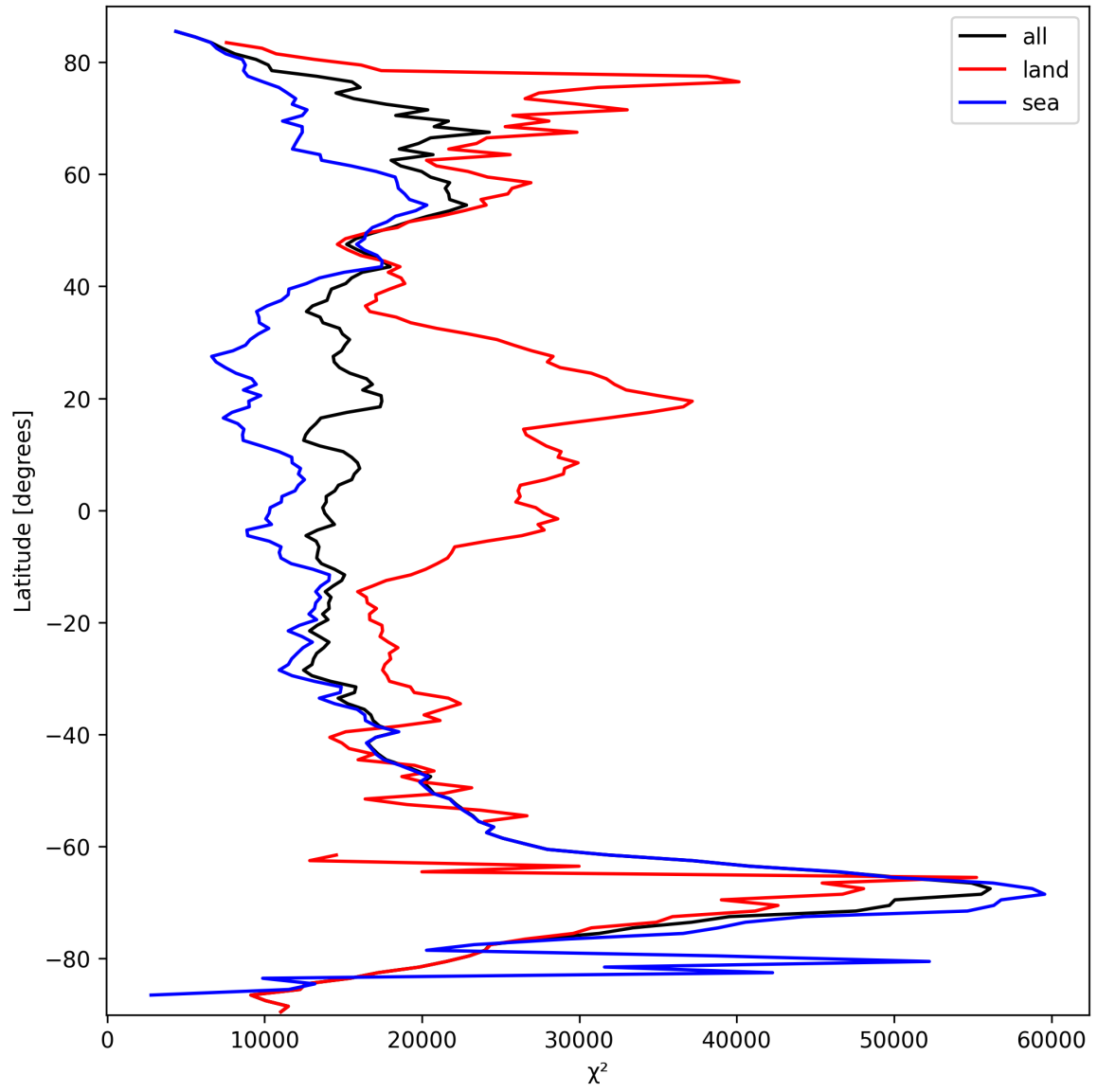
Figure 21: Zonal average of “ \chi^2 ” for 2025-09-27 to 2025-09-29.
