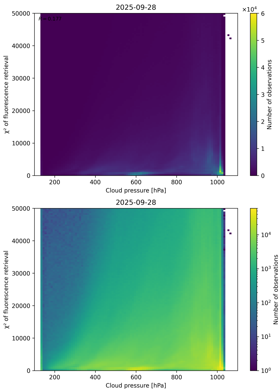
Figure 78: Scatter density plot of “Cloud pressure” against “ \chi^2 of fluorescence retrieval” for 2025-09-27 to 2025-09-29.
