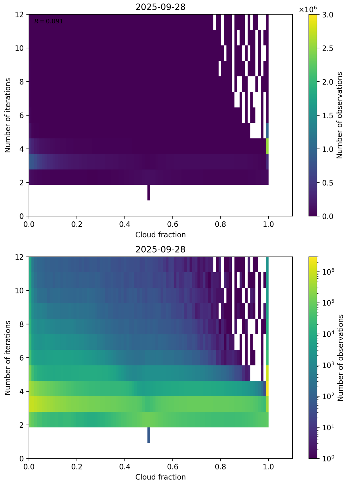
Figure 73: Scatter density plot of “Cloud fraction” against “Number of iterations” for 2025-09-27 to 2025-09-29.
