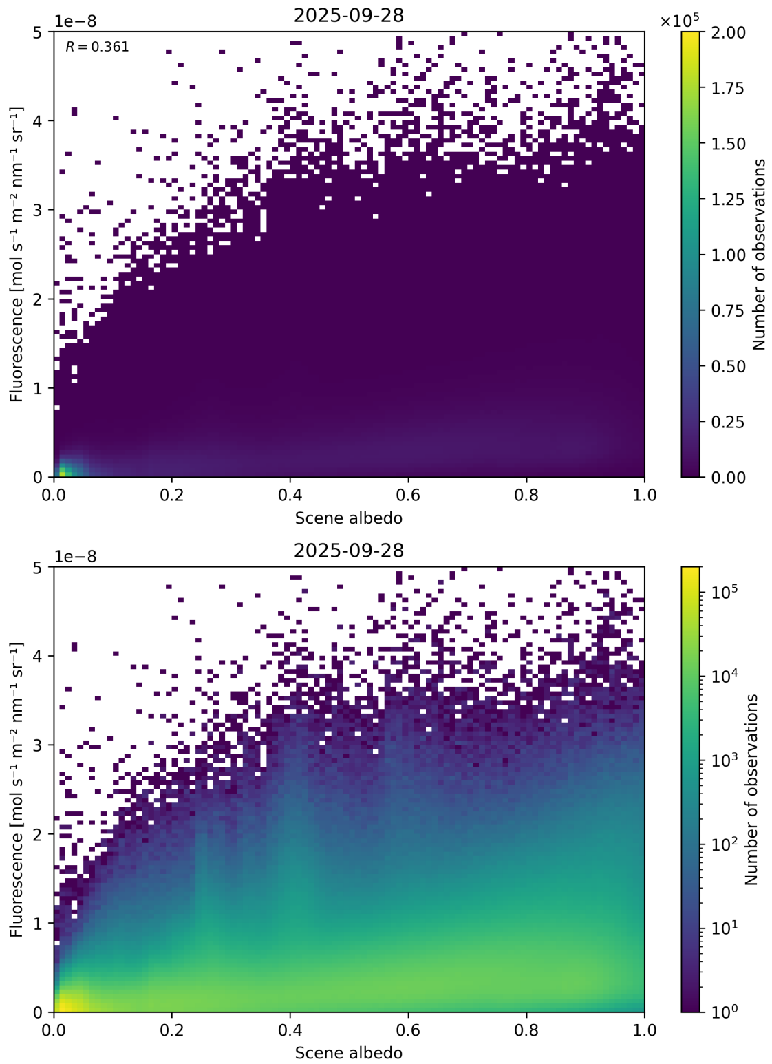
Figure 104: Scatter density plot of “Scene albedo” against “Fluorescence” for 2025-09-27 to 2025-09-29.
