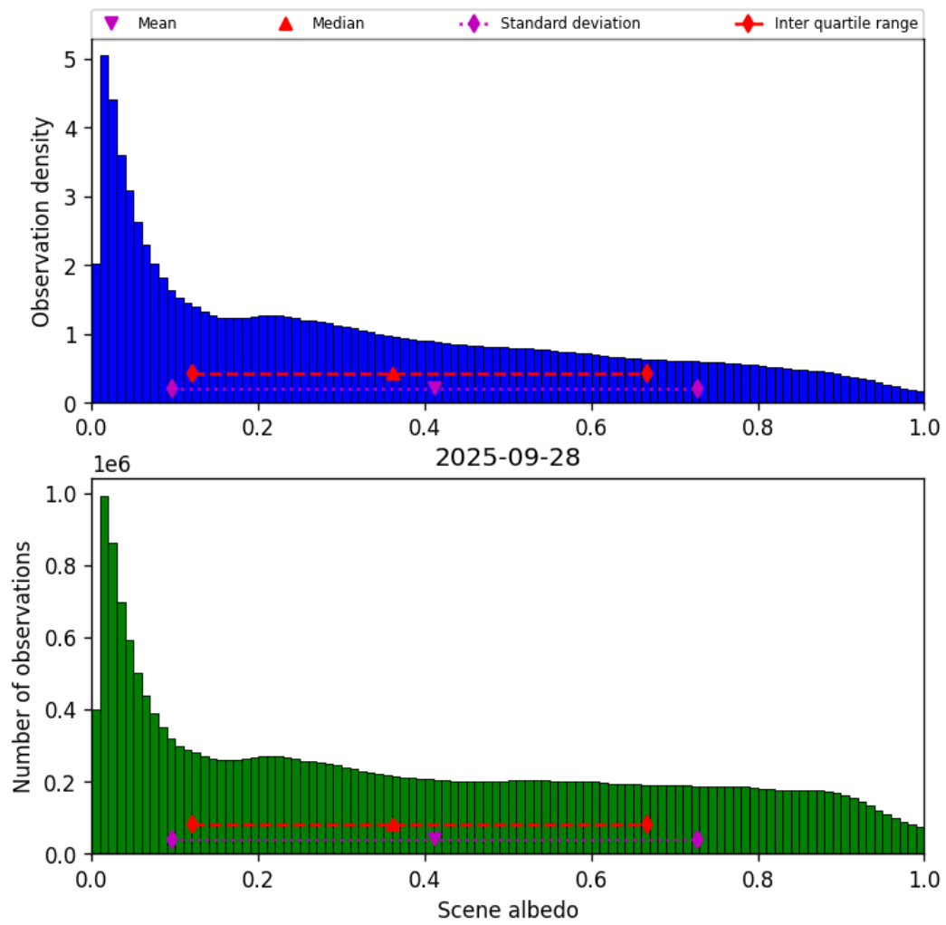
Figure 34: Histogram of “Scene albedo” for 2025-09-27 to 2025-09-29
