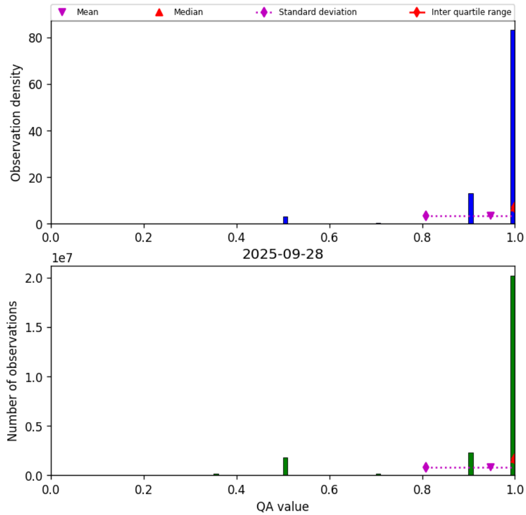
Figure 29: Histogram of “QA value” for 2025-09-27 to 2025-09-29
