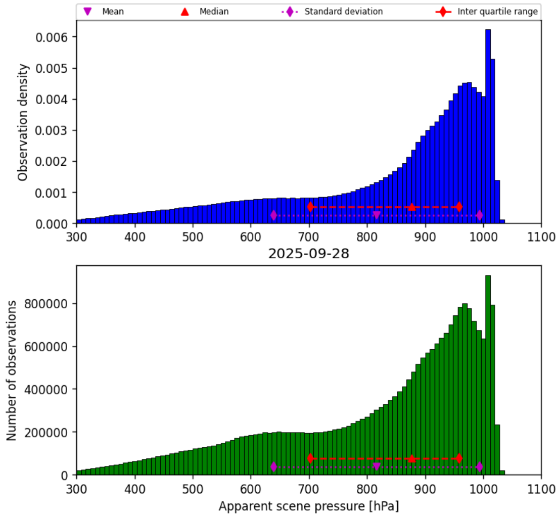
Figure 36: Histogram of “Apparent scene pressure” for 2025-09-27 to 2025-09-29
