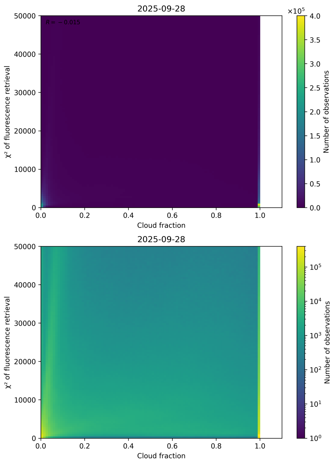
Figure 71: Scatter density plot of “Cloud fraction” against “ \chi^2 of fluorescence retrieval” for 2025-09-27 to 2025-09-29.
