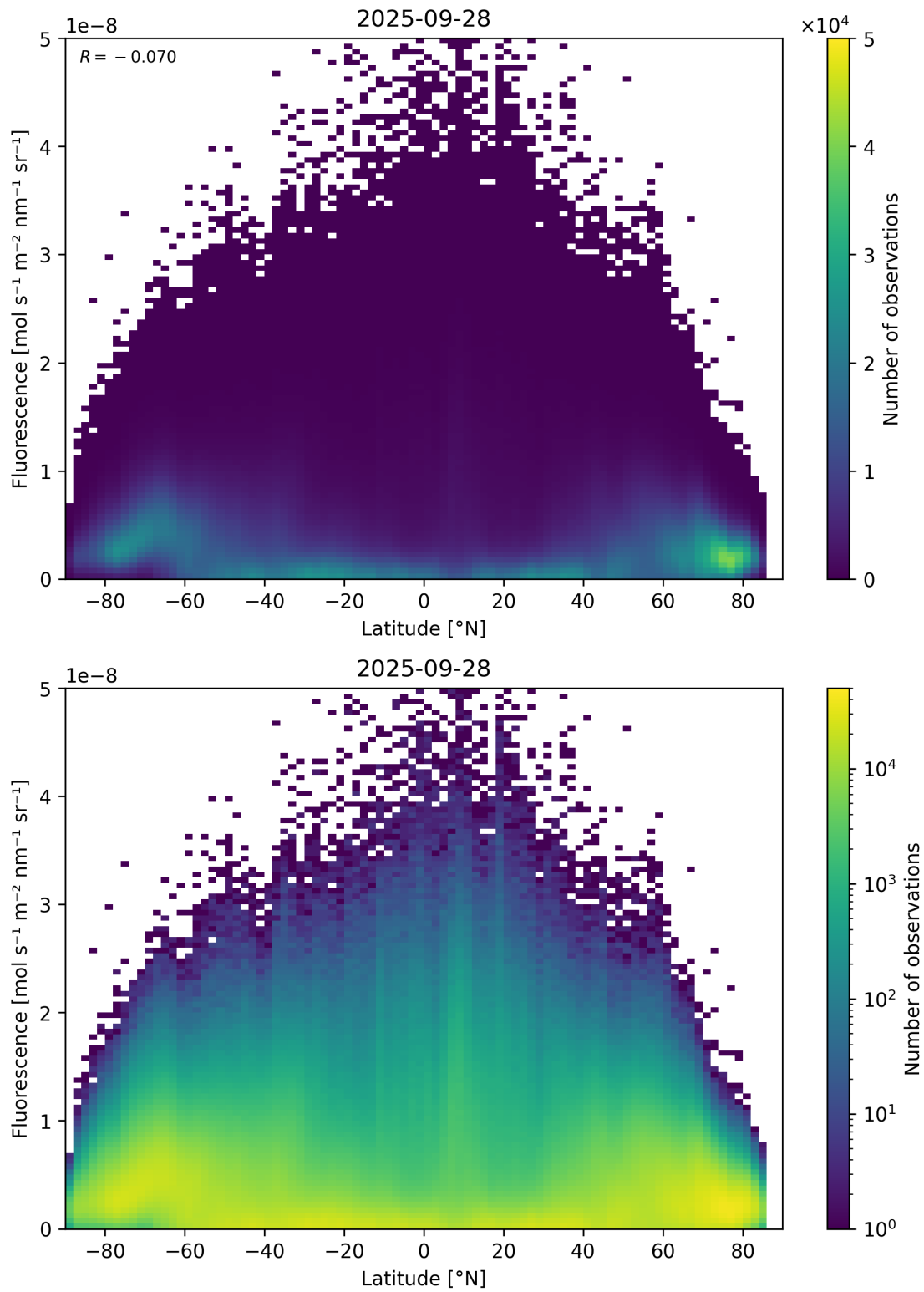
Figure 92: Scatter density plot of “Latitude” against “Fluorescence” for 2025-09-27 to 2025-09-29.
