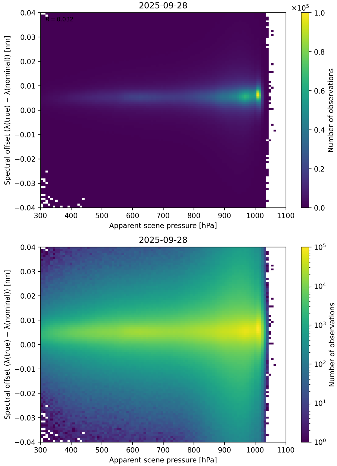
Figure 67: Scatter density plot of “Apparent scene pressure” against “Spectral offset ( \lambda_{\text{true}} - \lambda_{\text{nominal}} )” for 2025-09-27 to 2025-09-29.
