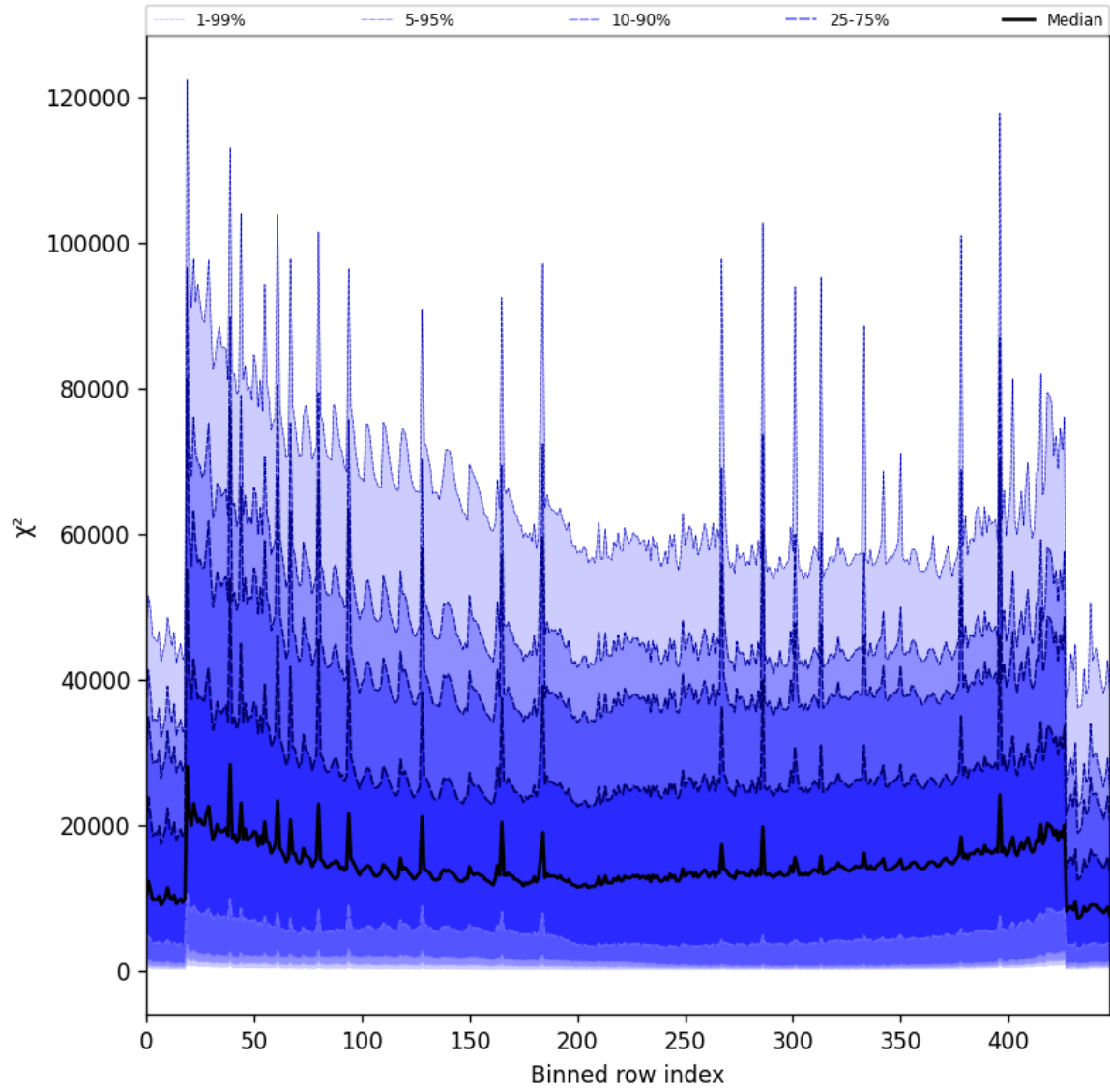
Figure 55: Along track statistics of “ \chi^2 ” for 2025-09-27 to 2025-09-29
