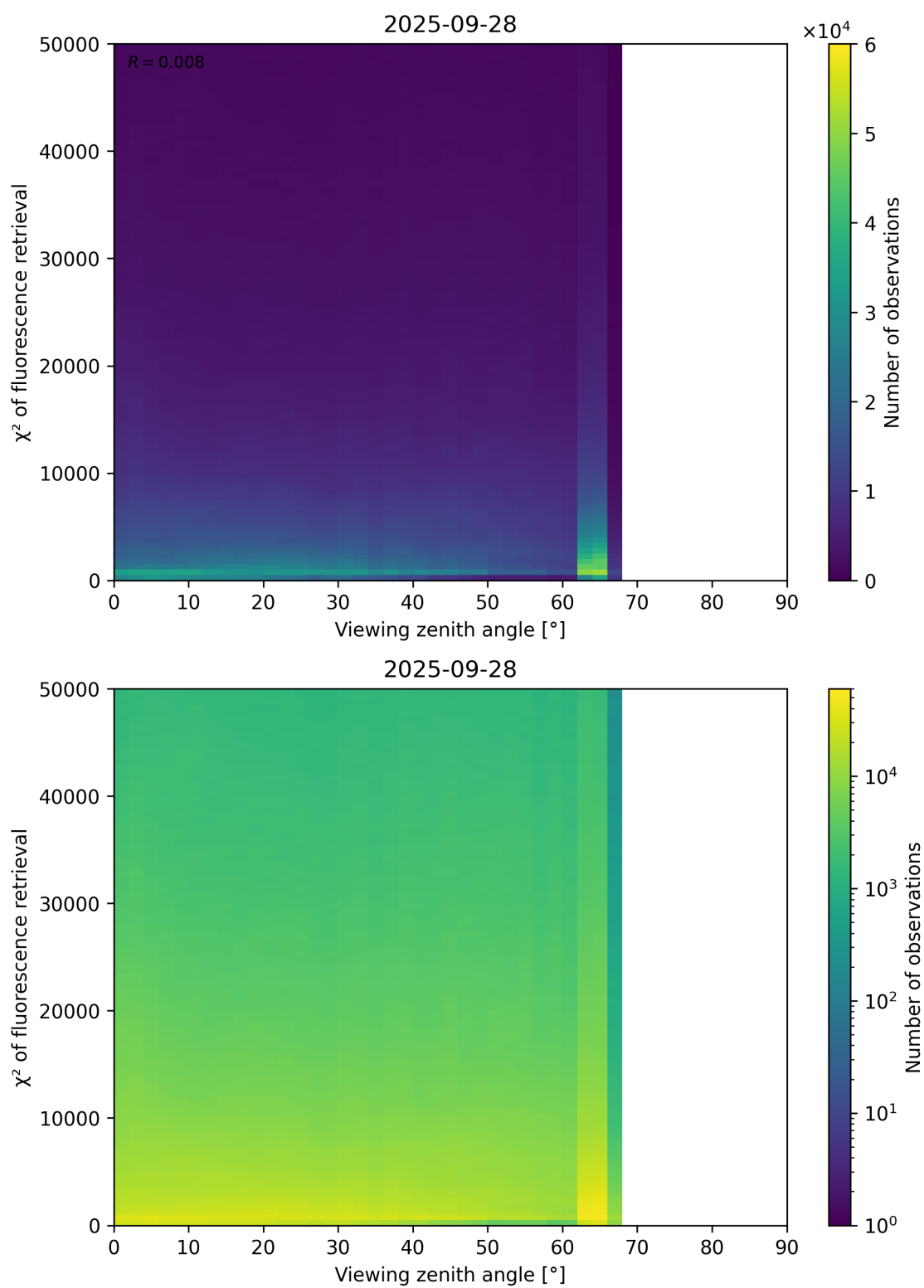
Figure 119: Scatter density plot of “Viewing zenith angle” against “ \chi^2 of fluorescence retrieval” for 2025-09-27 to 2025-09-29.
