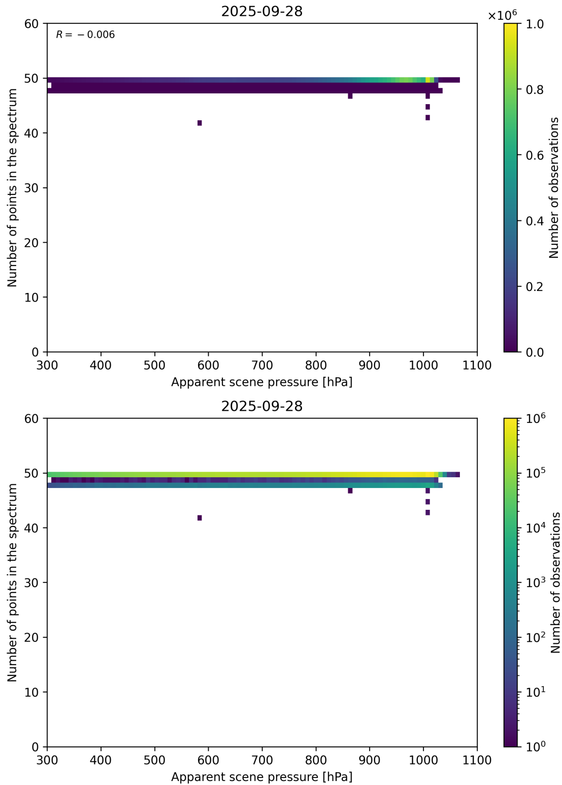
Figure 66: Scatter density plot of “Apparent scene pressure” against “Number of points in the spectrum” for 2025-09-27 to 2025-09-29.
