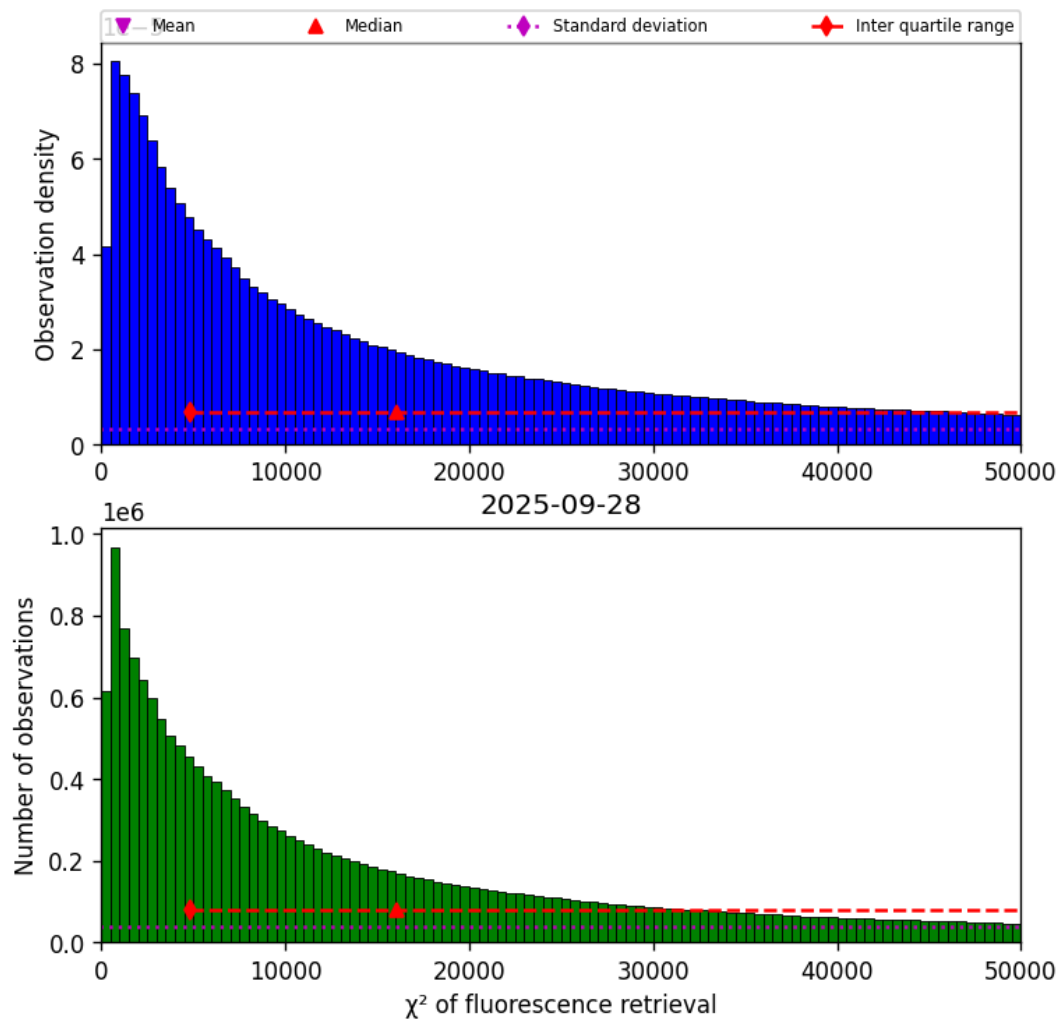
Figure 42: Histogram of “ \chi^2 of fluorescence retrieval” for 2025-09-27 to 2025-09-29
