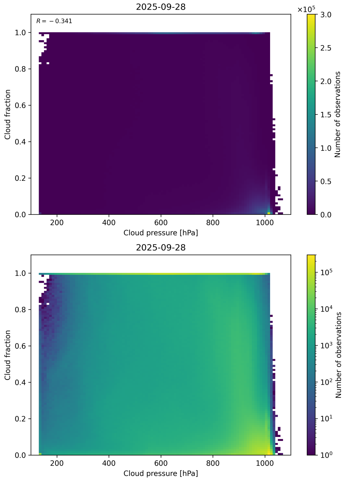
Figure 79: Scatter density plot of “Cloud pressure” against “Cloud fraction” for 2025-09-27 to 2025-09-29.
