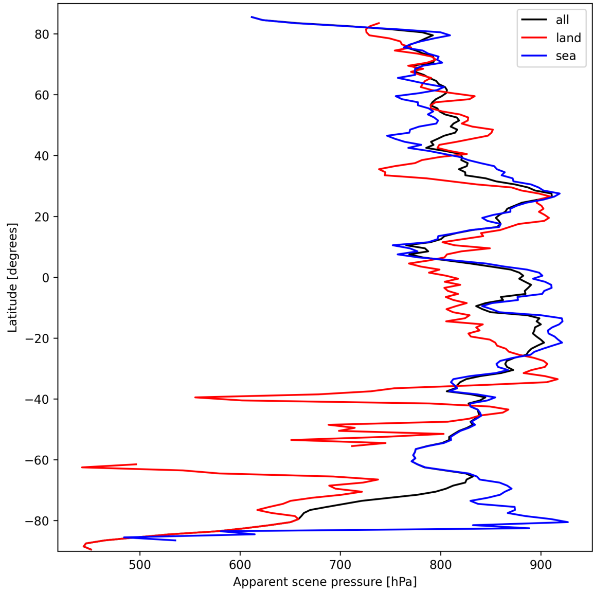
Figure 19: Zonal average of “Apparent scene pressure” for 2025-09-27 to 2025-09-29.
