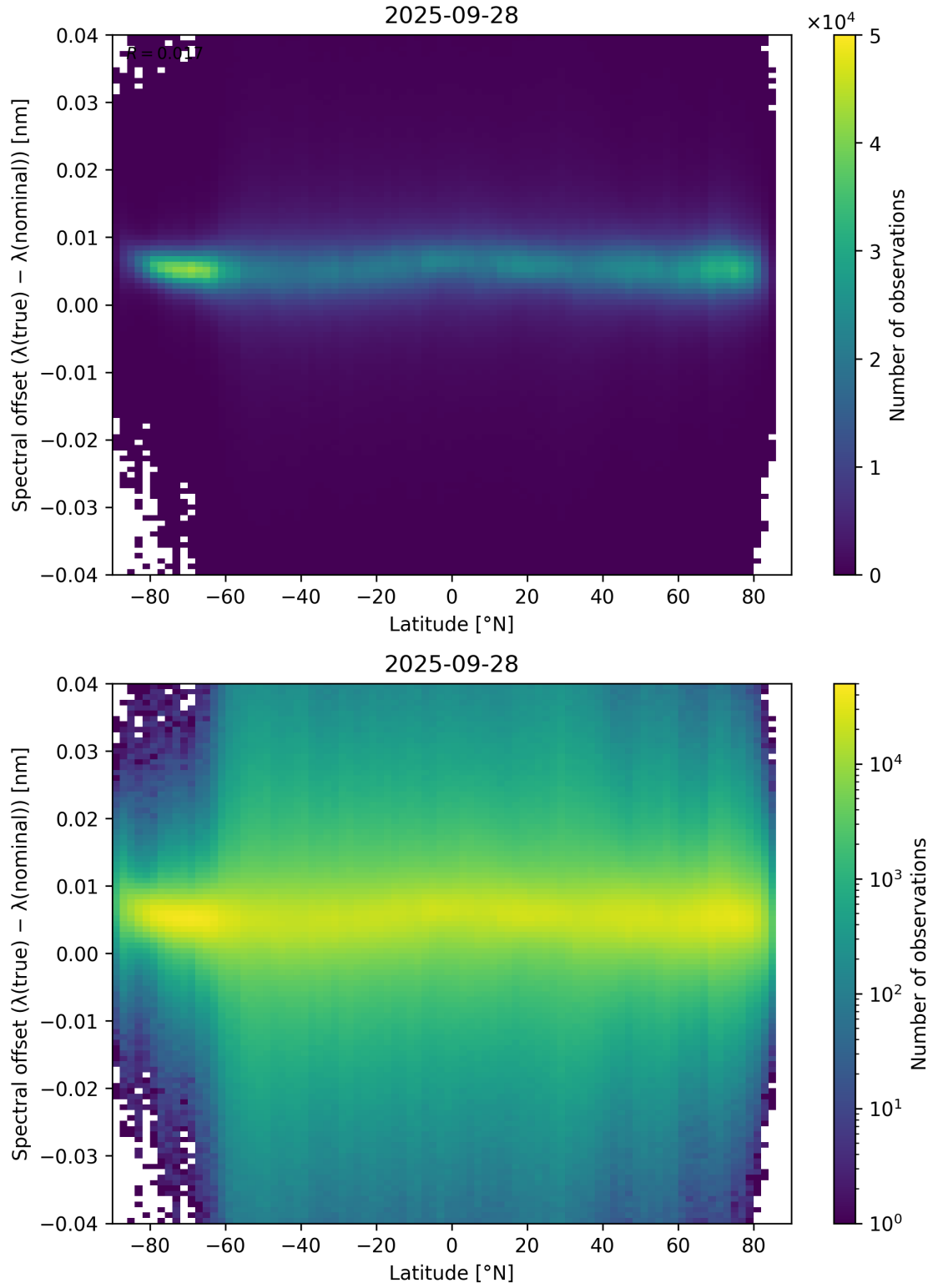
Figure 96: Scatter density plot of “Latitude” against “Spectral offset ( \lambda_{\text{true}} - \lambda_{\text{nominal}} )” for 2025-09-27 to 2025-09-29.
