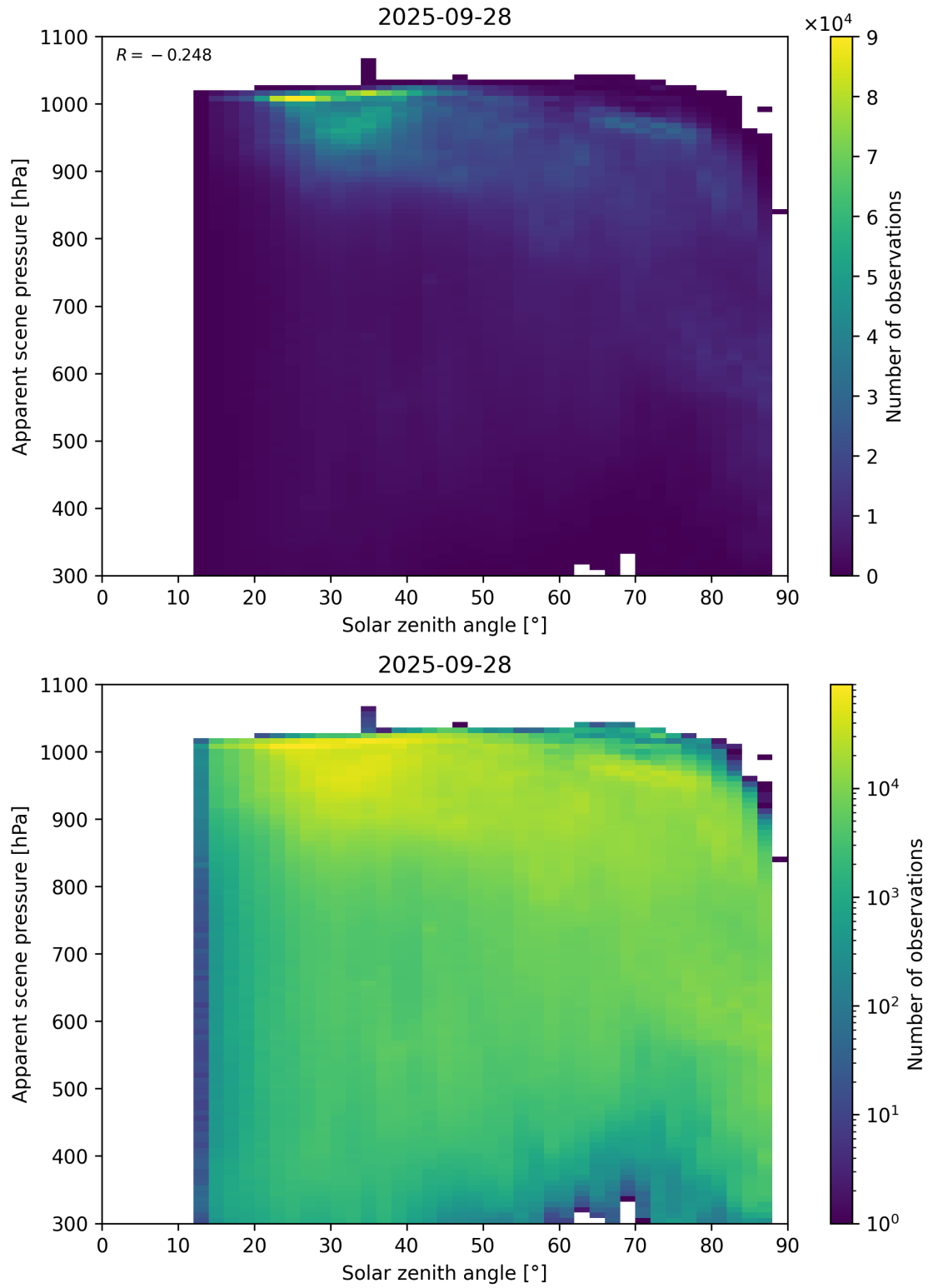
Figure 108: Scatter density plot of “Solar zenith angle” against “Apparent scene pressure” for 2025-09-27 to 2025-09-29.
