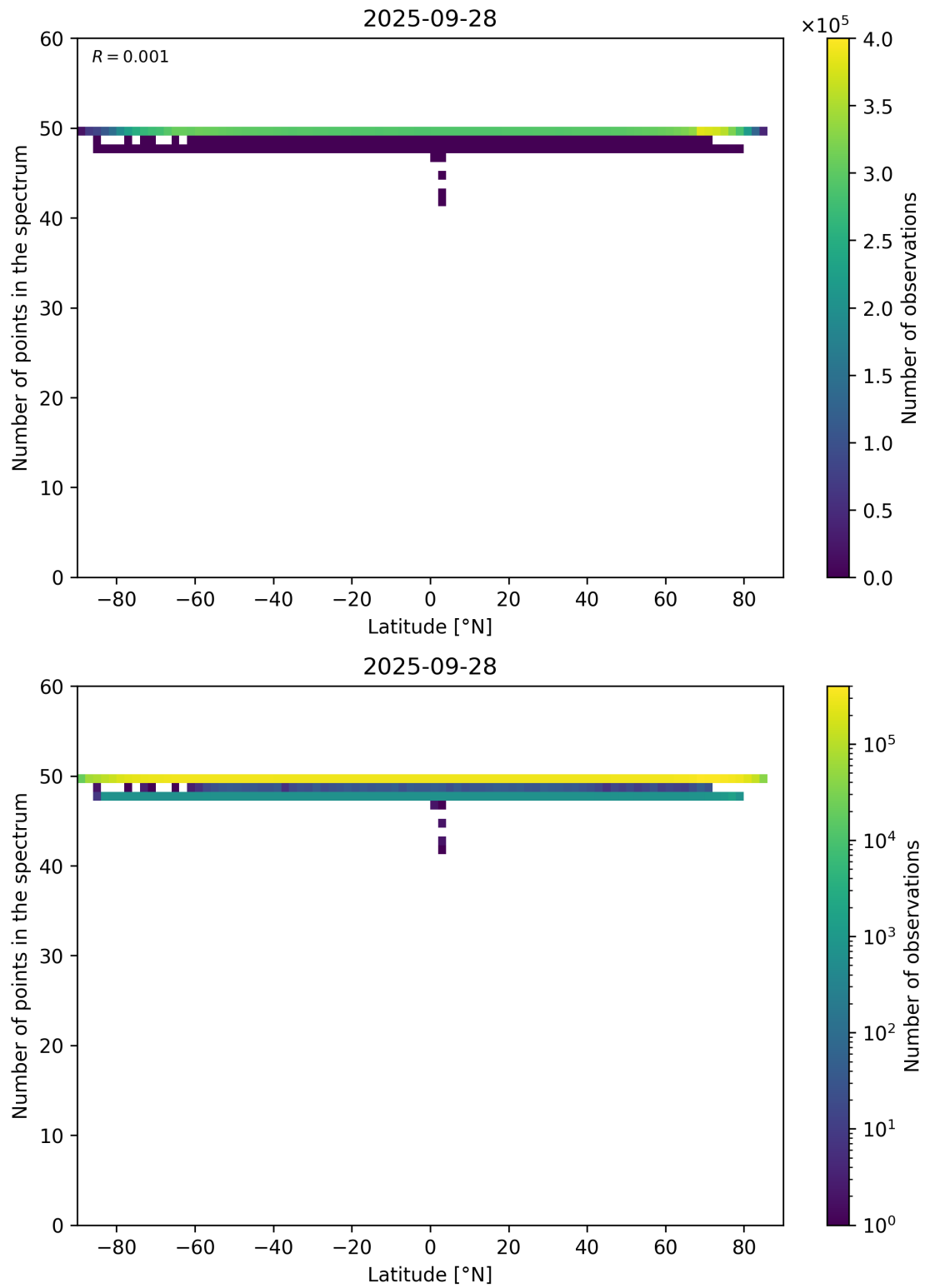
Figure 94: Scatter density plot of “Latitude” against “Number of points in the spectrum” for 2025-09-27 to 2025-09-29.
