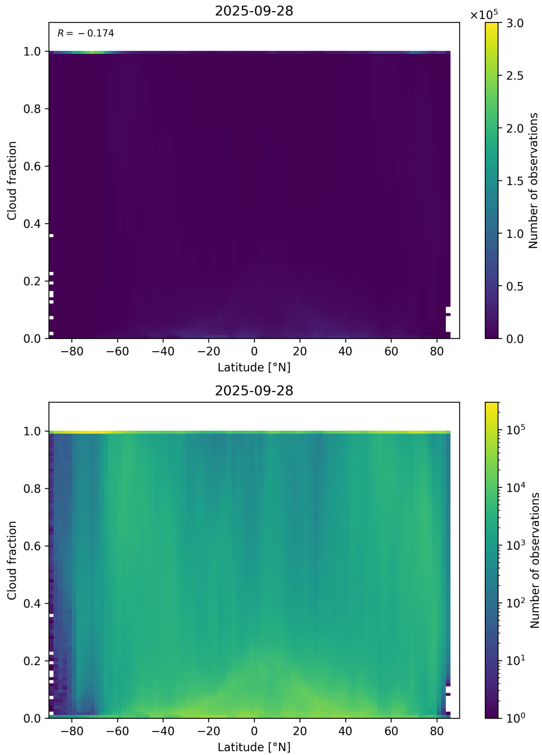
Figure 90: Scatter density plot of “Latitude” against “Cloud fraction” for 2025-09-27 to 2025-09-29.
