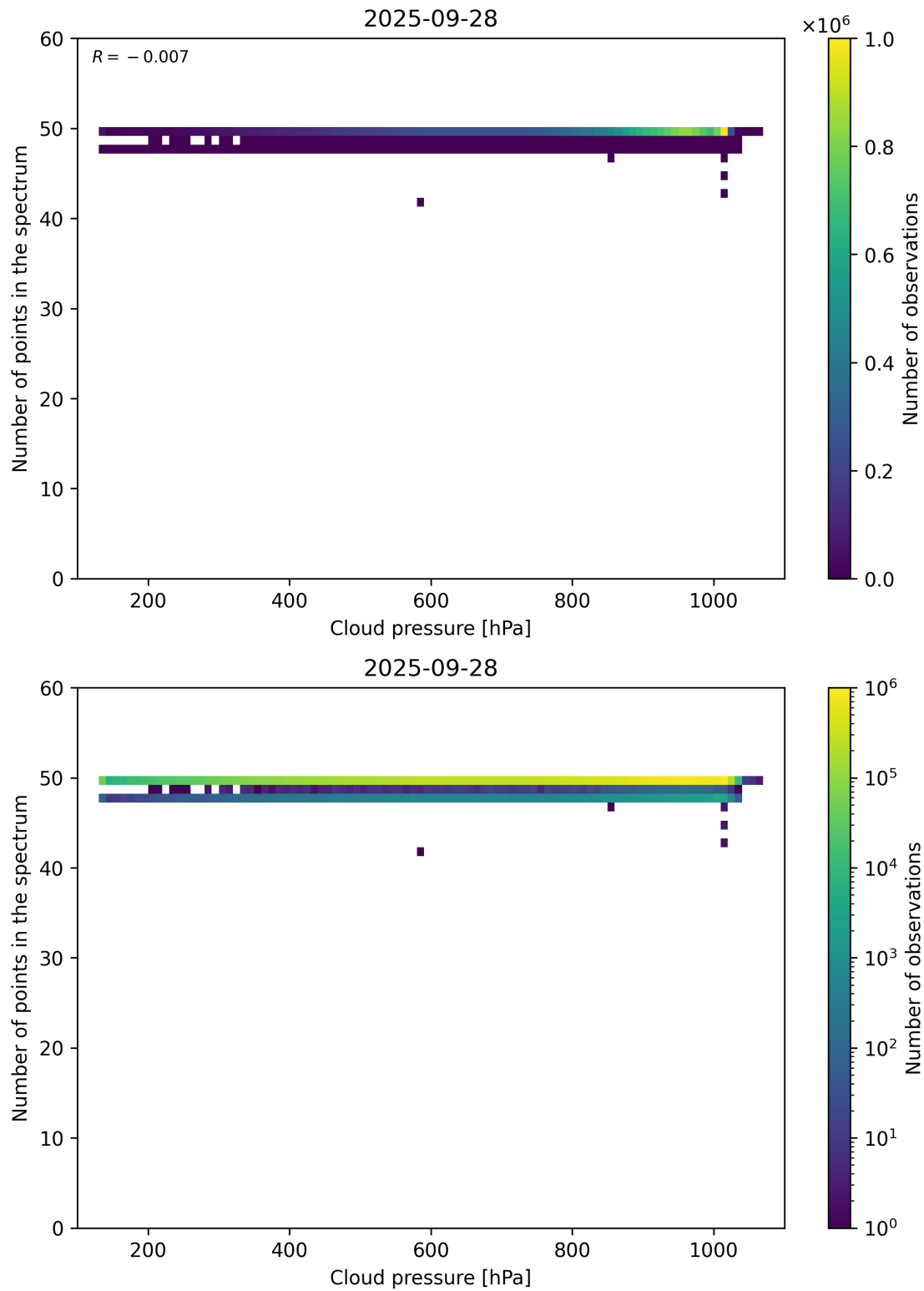
Figure 82: Scatter density plot of “Cloud pressure” against “Number of points in the spectrum” for 2025-09-27 to 2025-09-29.
