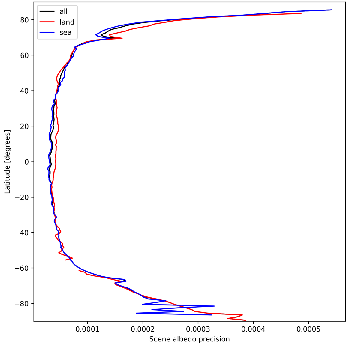
Figure 18: Zonal average of “Scene albedo precision” for 2025-09-27 to 2025-09-29.
