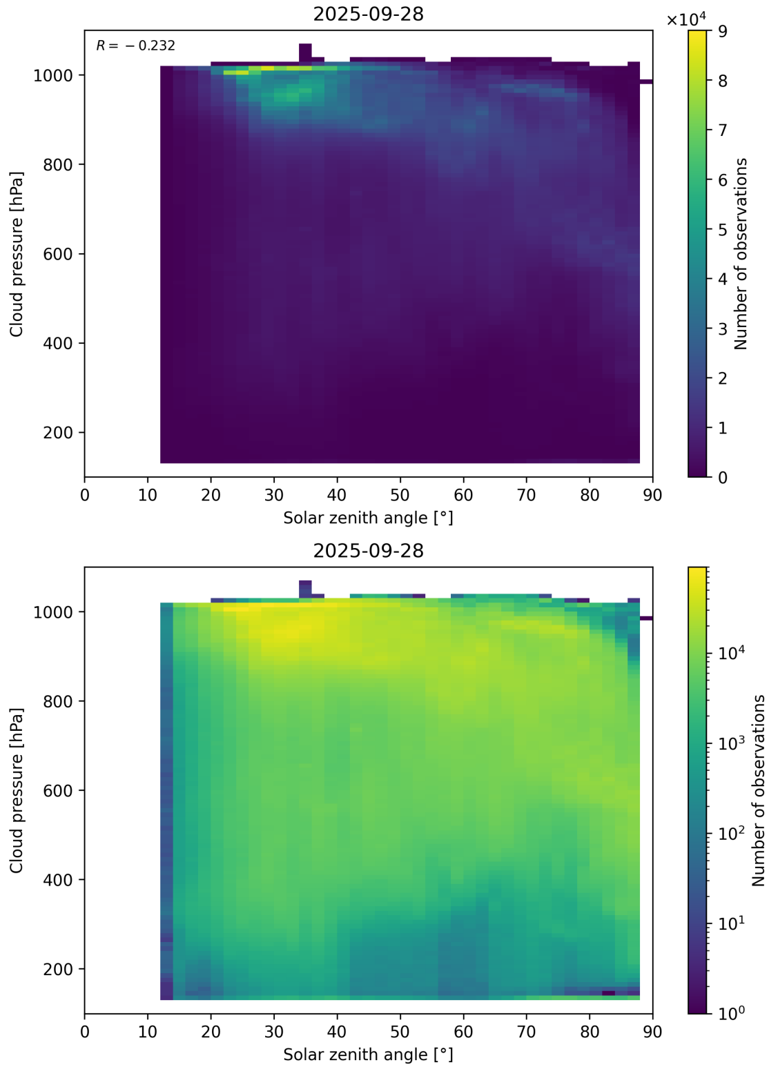
Figure 111: Scatter density plot of “Solar zenith angle” against “Cloud pressure” for 2025-09-27 to 2025-09-29.
