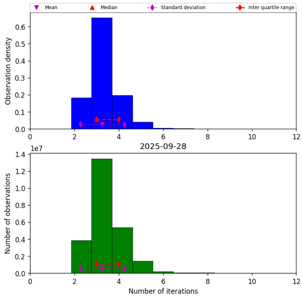
Figure 39: Histogram of “Number of iterations” for 2025-09-27 to 2025-09-29
