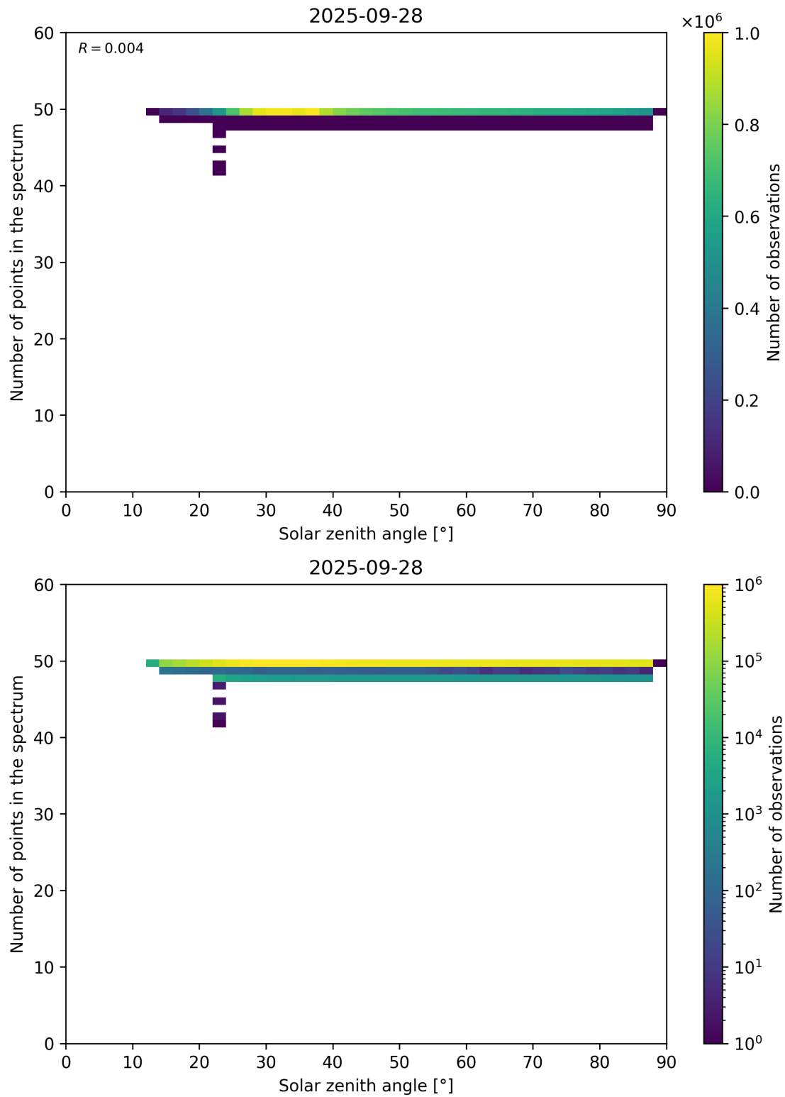
Figure 115: Scatter density plot of “Solar zenith angle” against “Number of points in the spectrum” for 2025-09-27 to 2025-09-29.
