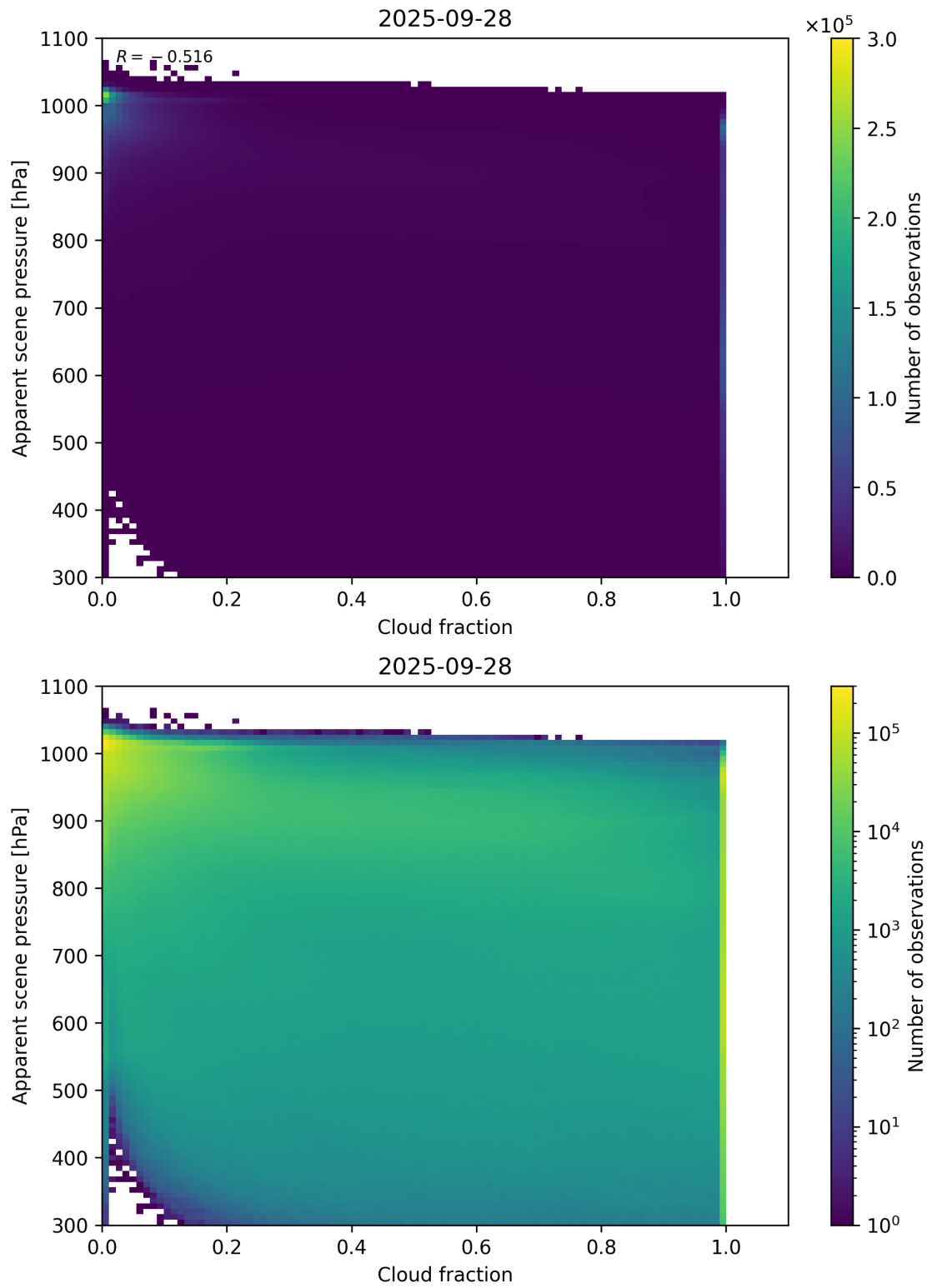
Figure 70: Scatter density plot of “Cloud fraction” against “Apparent scene pressure” for 2025-09-27 to 2025-09-29.
