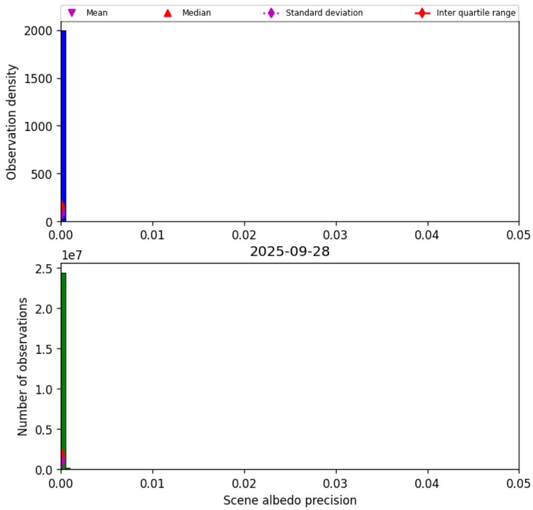
Figure 35: Histogram of “Scene albedo precision” for 2025-09-27 to 2025-09-29
