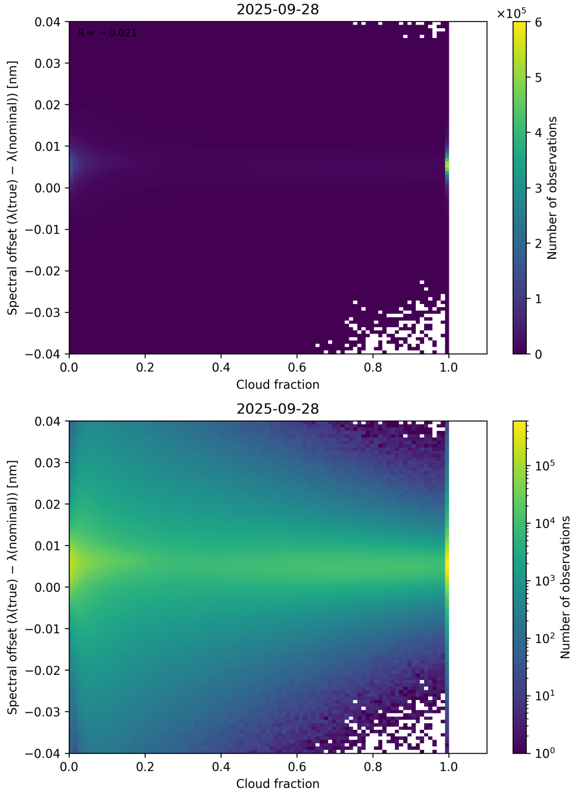
Figure 76: Scatter density plot of “Cloud fraction” against “Spectral offset ( \lambda_{\text{true}} - \lambda_{\text{nominal}} )” for 2025-09-27 to 2025-09-29.
