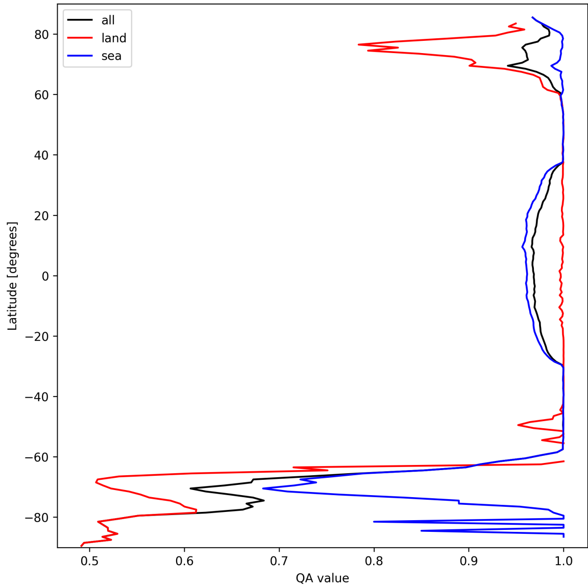
Figure 12: Zonal average of "QA value" for 2025-09-27 to 2025-09-29.
