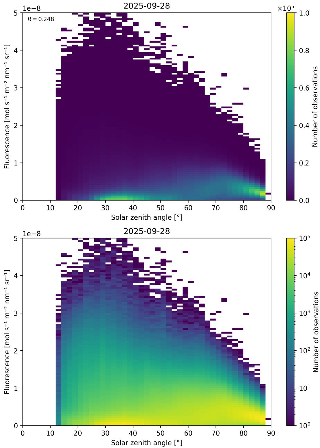
Figure 112: Scatter density plot of “Solar zenith angle” against “Fluorescence” for 2025-09-27 to 2025-09-29.
