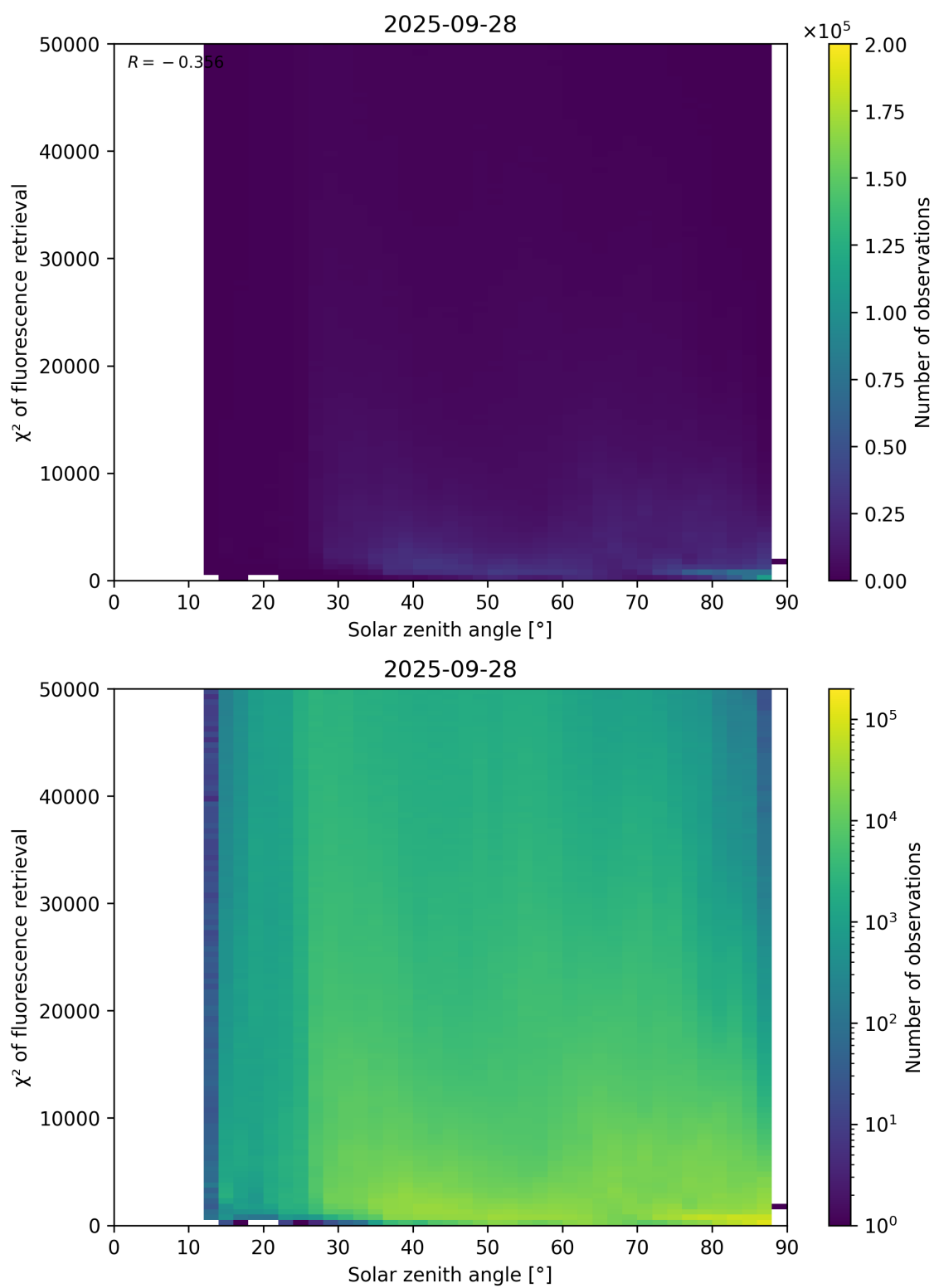
Figure 109: Scatter density plot of “Solar zenith angle” against “ \chi^2 of fluorescence retrieval” for 2025-09-27 to 2025-09-29.
