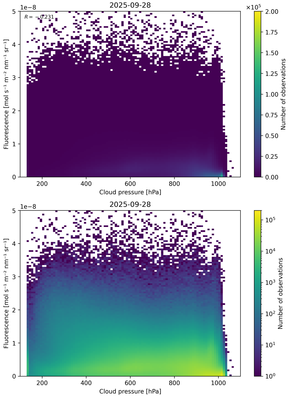
Figure 80: Scatter density plot of “Cloud pressure” against “Fluorescence” for 2025-09-27 to 2025-09-29.
