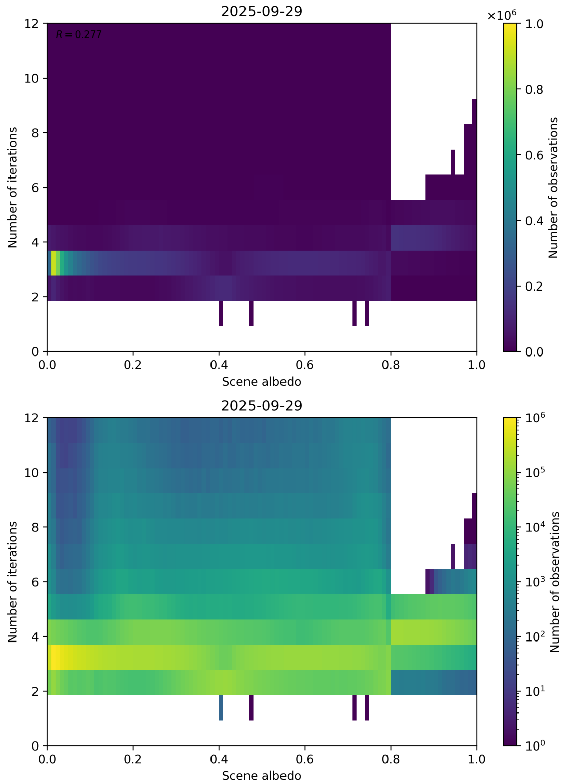
Figure 105: Scatter density plot of “Scene albedo” against “Number of iterations” for 2025-09-28 to 2025-09-30.
