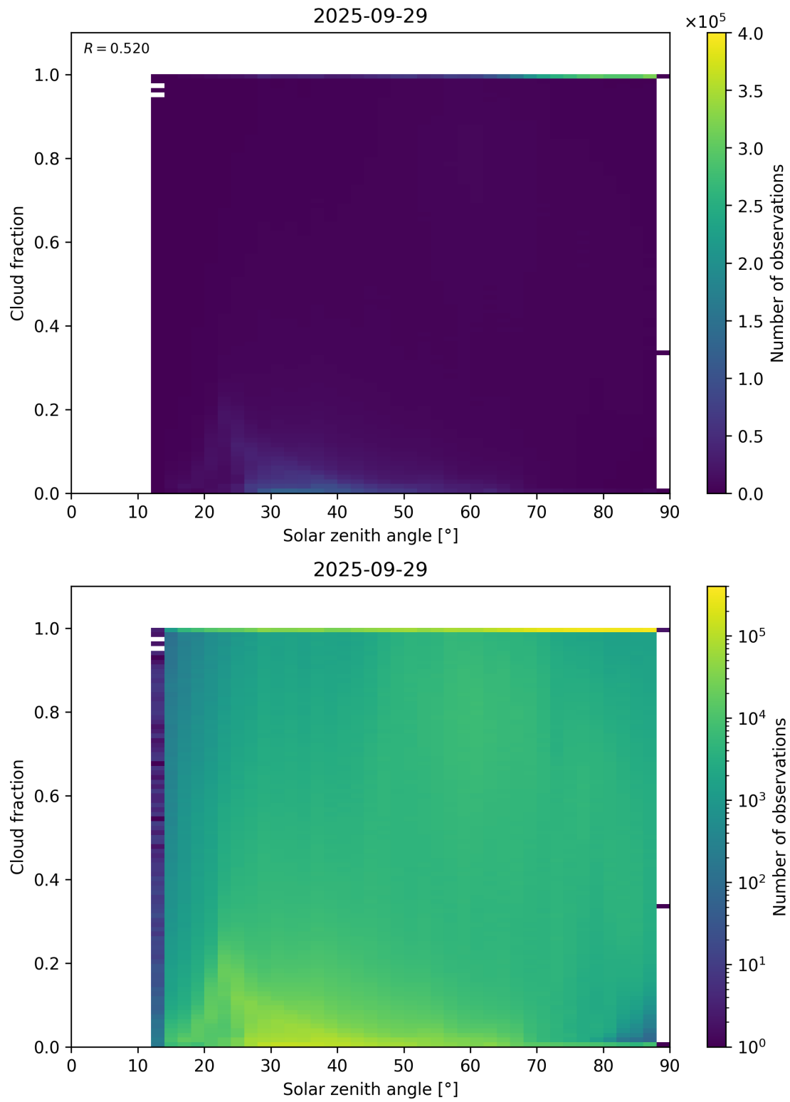
Figure 110: Scatter density plot of “Solar zenith angle” against “Cloud fraction” for 2025-09-28 to 2025-09-30.
