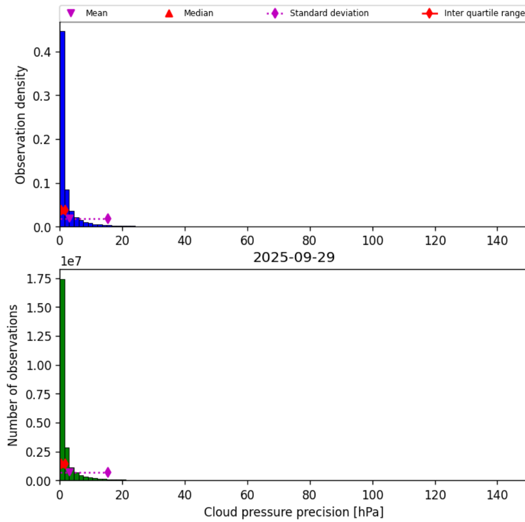
Figure 31: Histogram of “Cloud pressure precision” for 2025-09-28 to 2025-09-30
