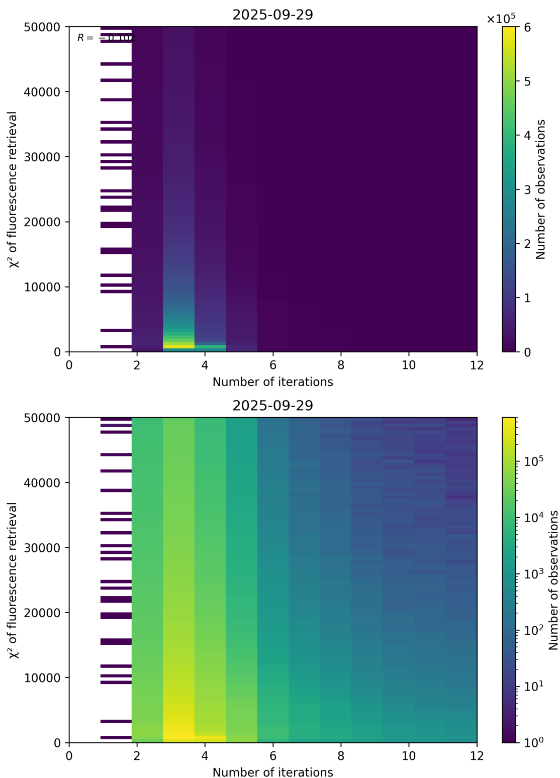
Figure 97: Scatter density plot of “Number of iterations” against “ \chi^2 of fluorescence retrieval” for 2025-09-28 to 2025-09-30.
