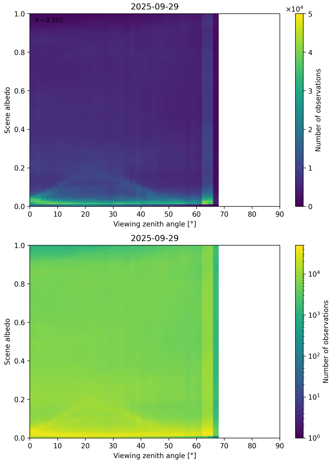
Figure 126: Scatter density plot of “Viewing zenith angle” against “Scene albedo” for 2025-09-28 to 2025-09-30.
