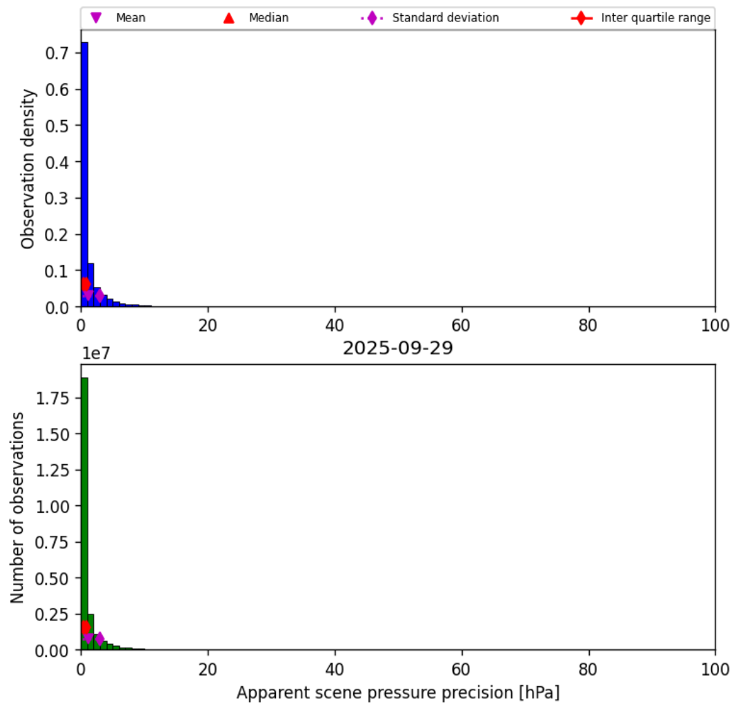
Figure 37: Histogram of “Apparent scene pressure precision” for 2025-09-28 to 2025-09-30
