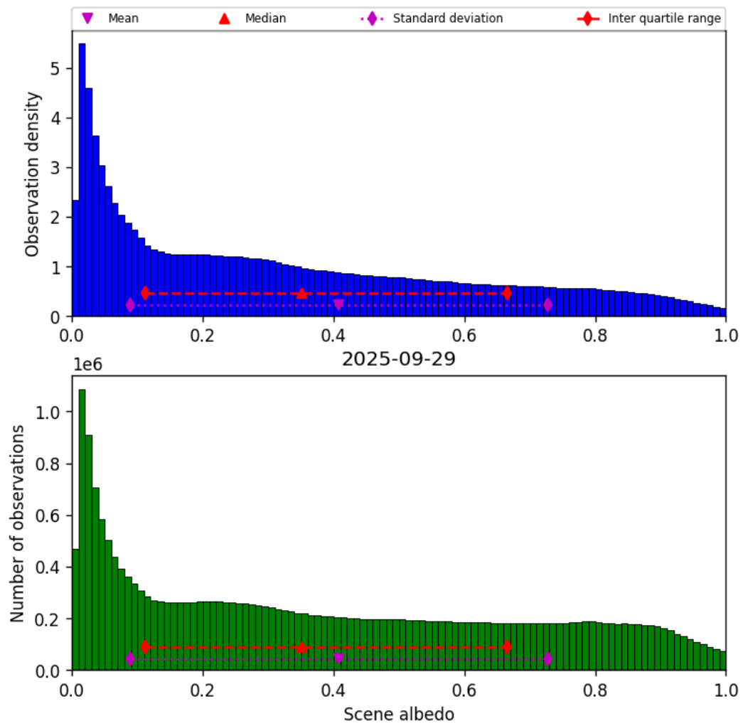
Figure 34: Histogram of “Scene albedo” for 2025-09-28 to 2025-09-30
