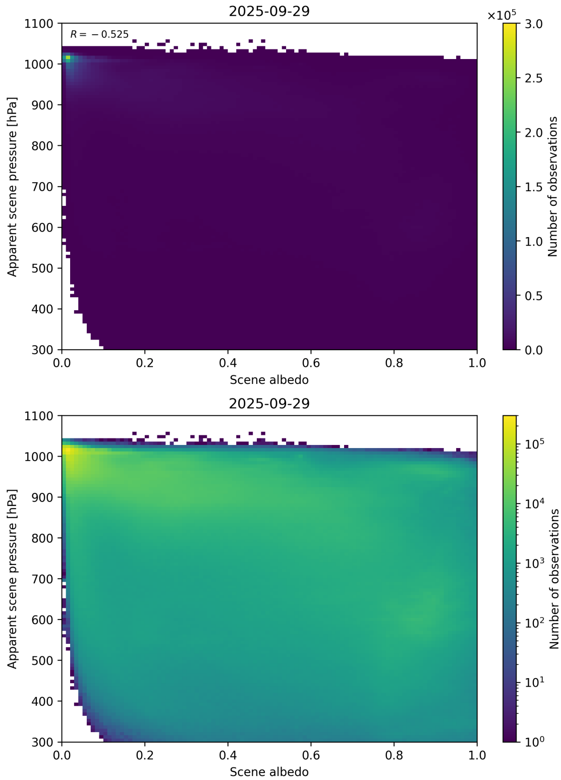
Figure 102: Scatter density plot of “Scene albedo” against “Apparent scene pressure” for 2025-09-28 to 2025-09-30.
