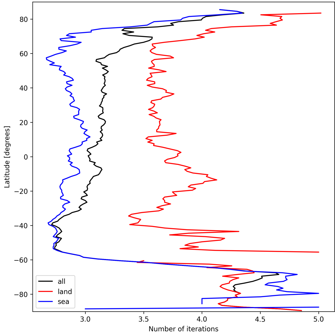
Figure 22: Zonal average of “Number of iterations” for 2025-09-28 to 2025-09-30.
