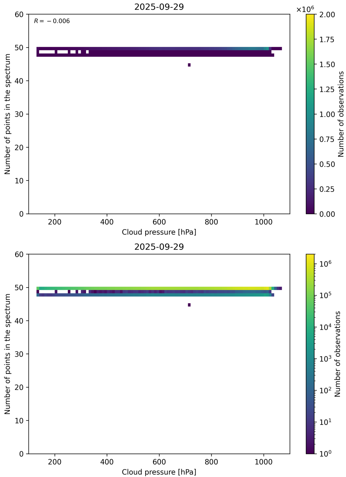
Figure 82: Scatter density plot of “Cloud pressure” against “Number of points in the spectrum” for 2025-09-28 to 2025-09-30.
