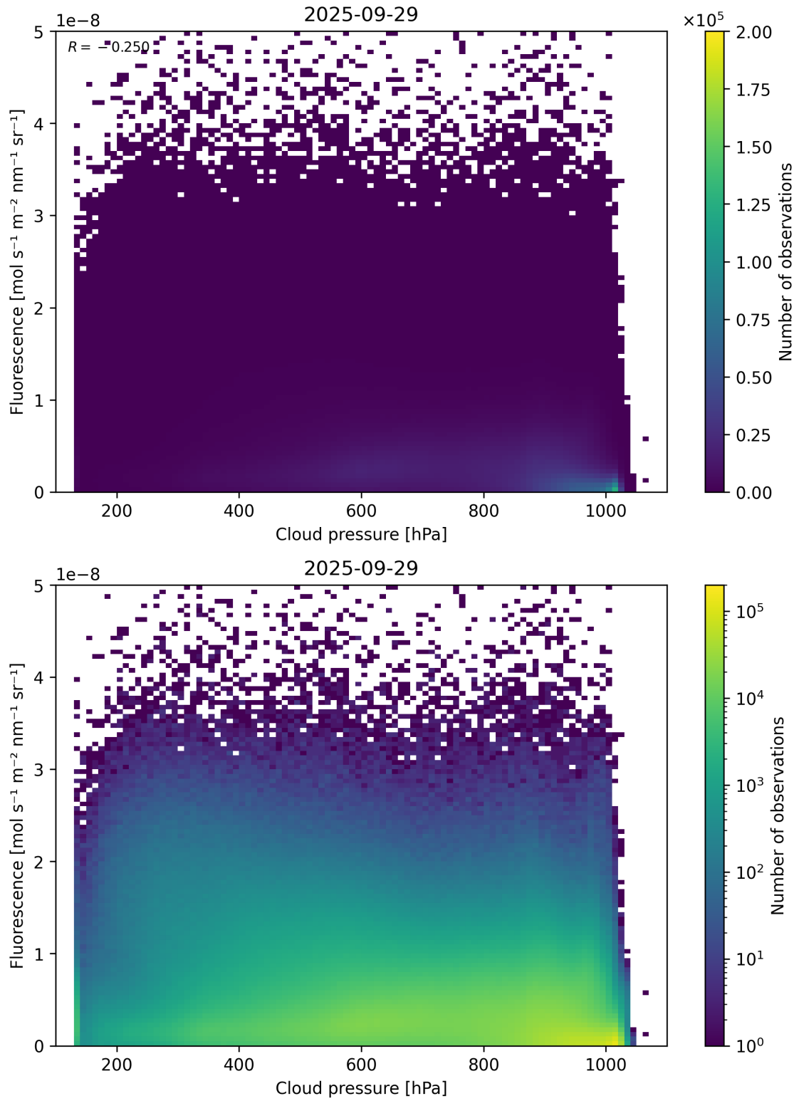
Figure 80: Scatter density plot of “Cloud pressure” against “Fluorescence” for 2025-09-28 to 2025-09-30.
