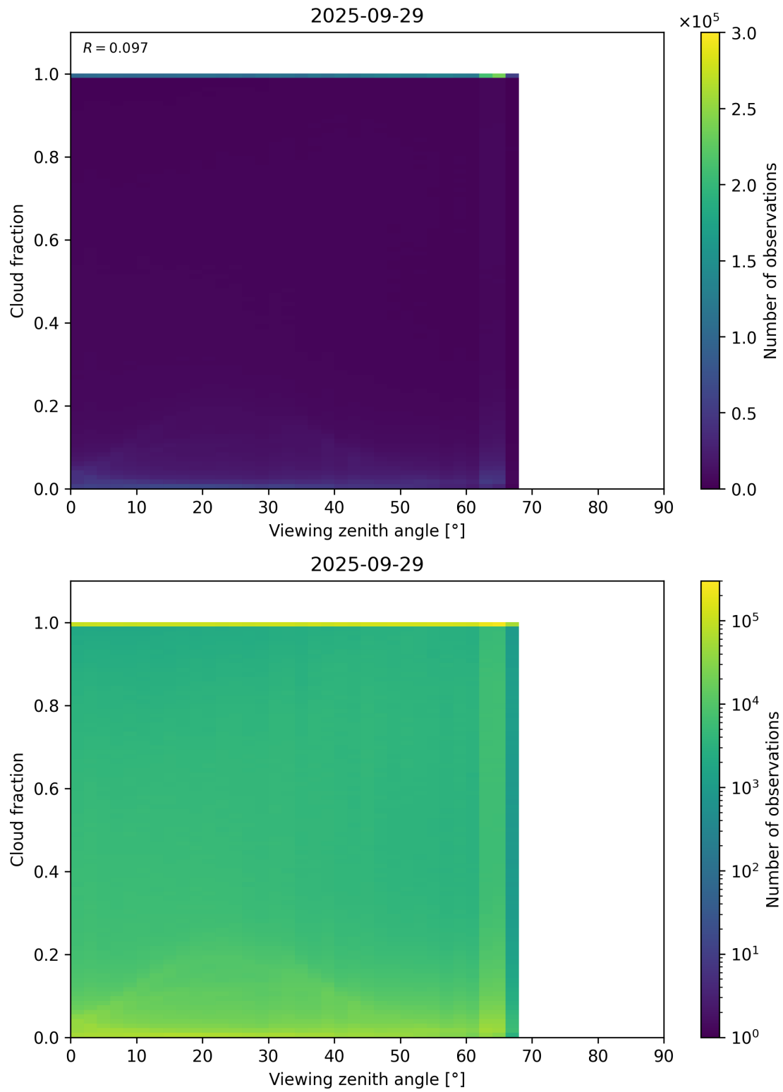
Figure 120: Scatter density plot of “Viewing zenith angle” against “Cloud fraction” for 2025-09-28 to 2025-09-30.
