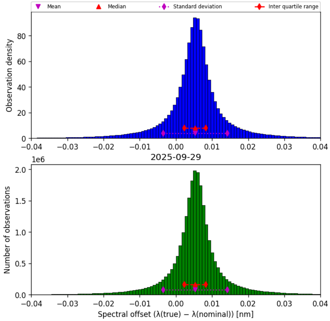
Figure 45: Histogram of “Spectral offset ( \lambda_{\text{true}} - \lambda_{\text{nominal}} )” for 2025-09-28 to 2025-09-30
