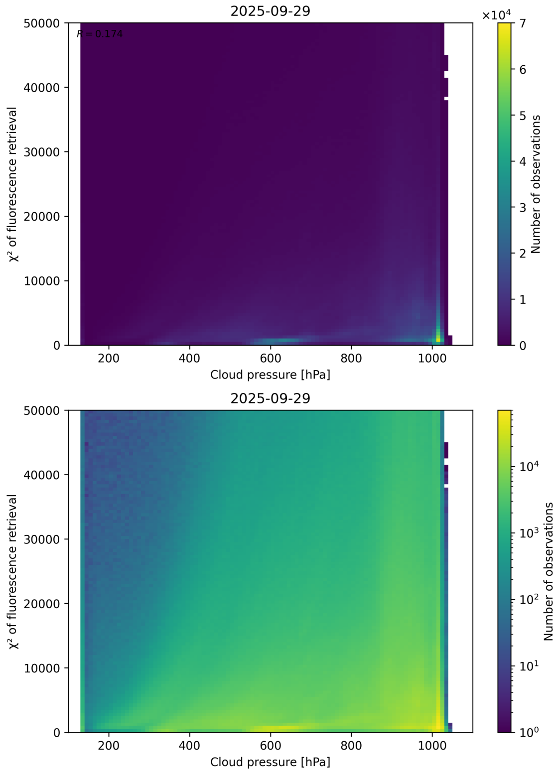
Figure 78: Scatter density plot of “Cloud pressure” against “ \chi^2 of fluorescence retrieval” for 2025-09-28 to 2025-09-30.
