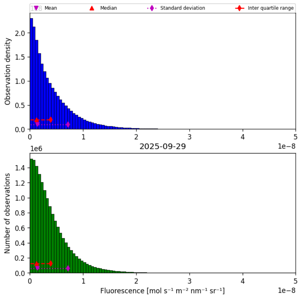
Figure 40: Histogram of “Fluorescence” for 2025-09-28 to 2025-09-30
