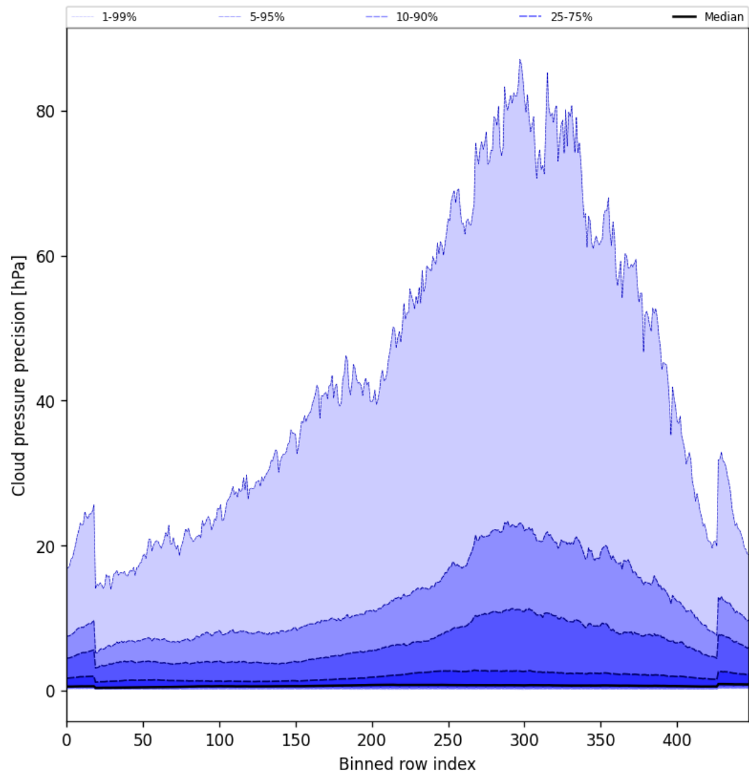
Figure 48: Along track statistics of “Cloud pressure precision” for 2025-09-28 to 2025-09-30
