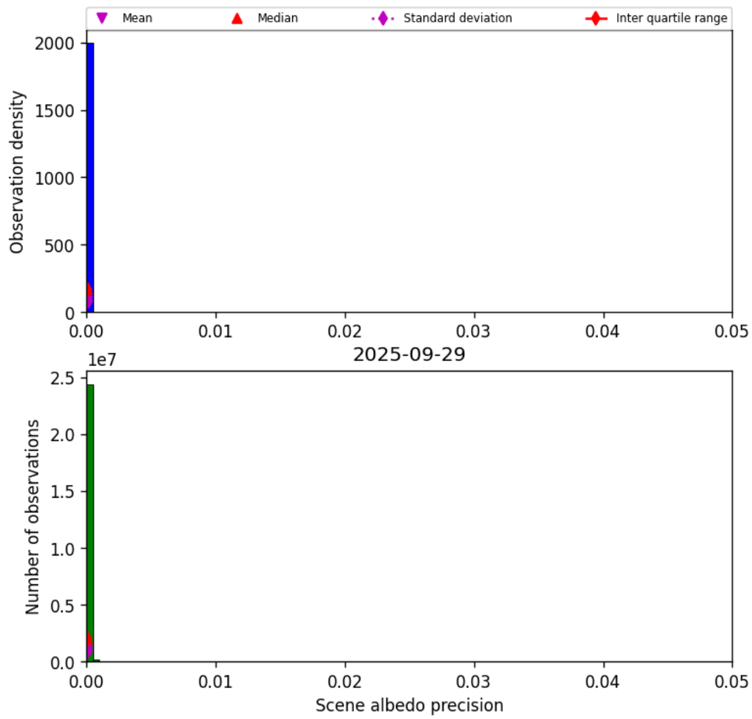
Figure 35: Histogram of “Scene albedo precision” for 2025-09-28 to 2025-09-30
