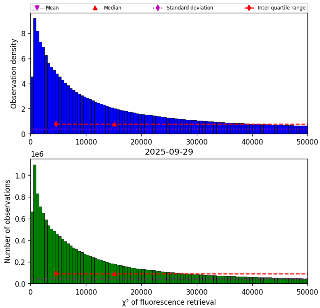
Figure 42: Histogram of “ \chi^2 of fluorescence retrieval” for 2025-09-28 to 2025-09-30
