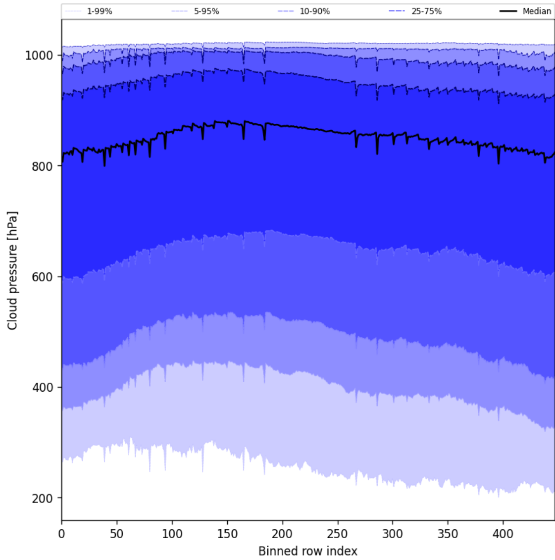
Figure 47: Along track statistics of “Cloud pressure” for 2025-09-28 to 2025-09-30
