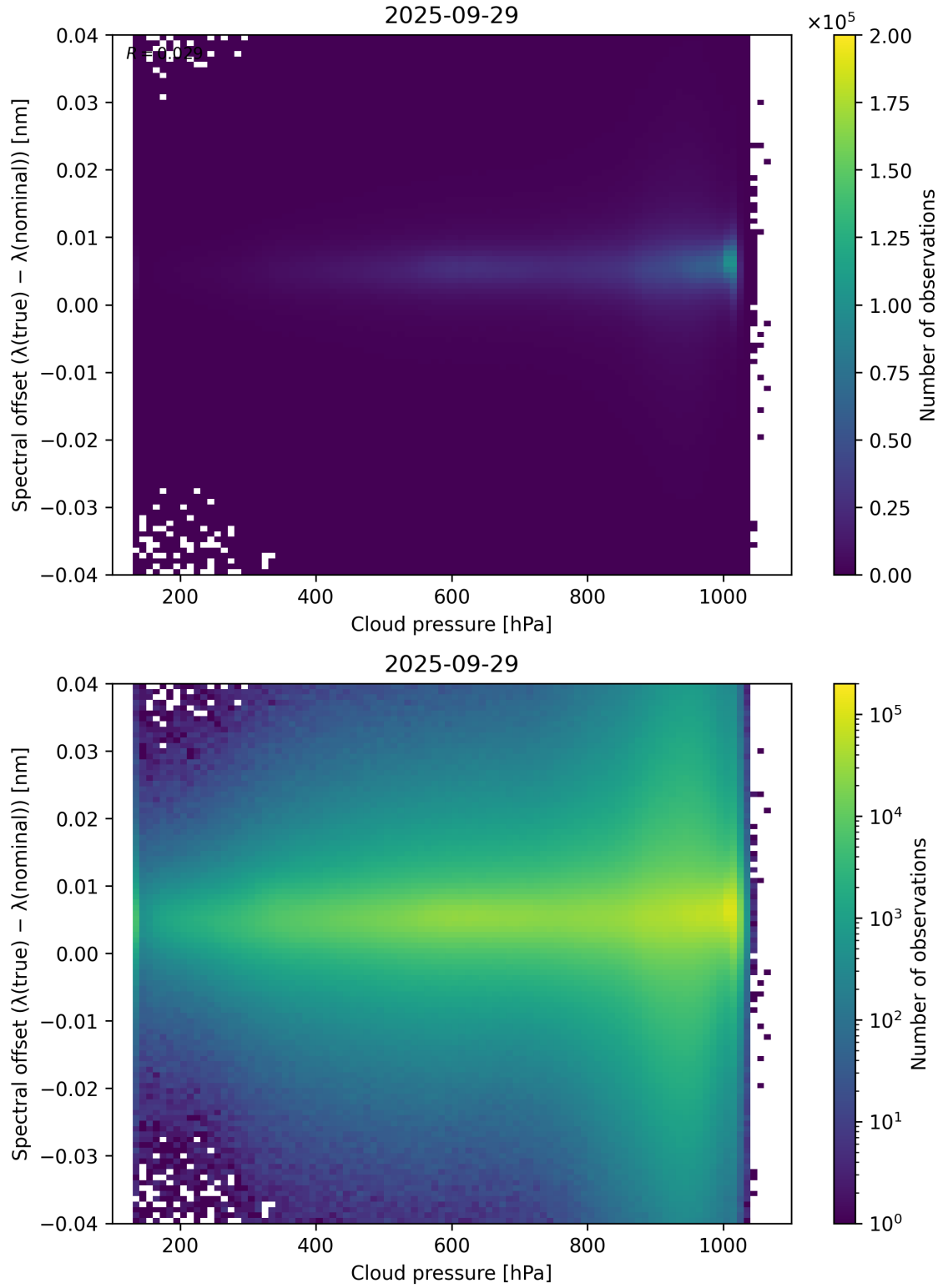
Figure 84: Scatter density plot of “Cloud pressure” against “Spectral offset ( \lambda_{\text{true}} - \lambda_{\text{nominal}} )” for 2025-09-28 to 2025-09-30.
