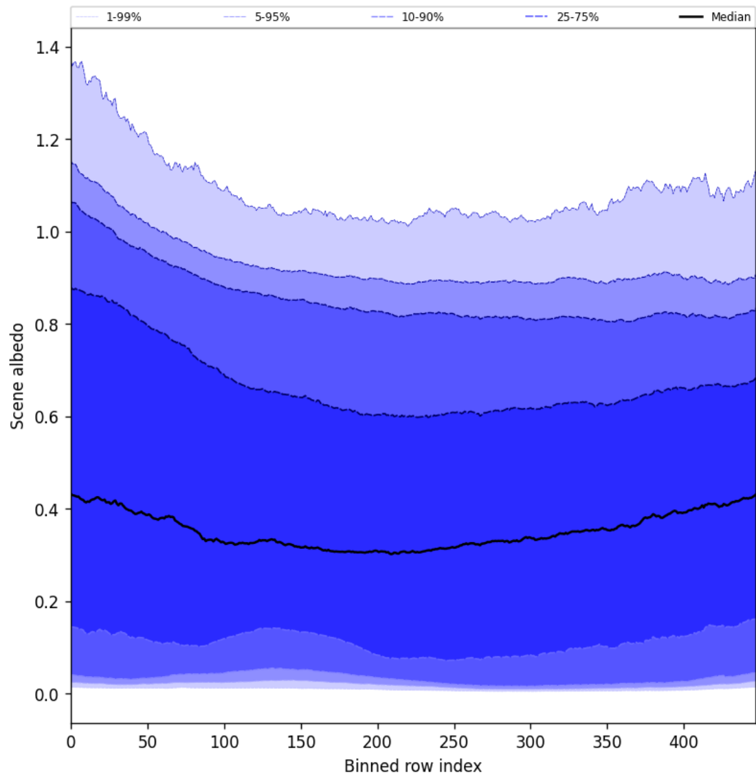
Figure 51: Along track statistics of “Scene albedo” for 2025-09-28 to 2025-09-30
