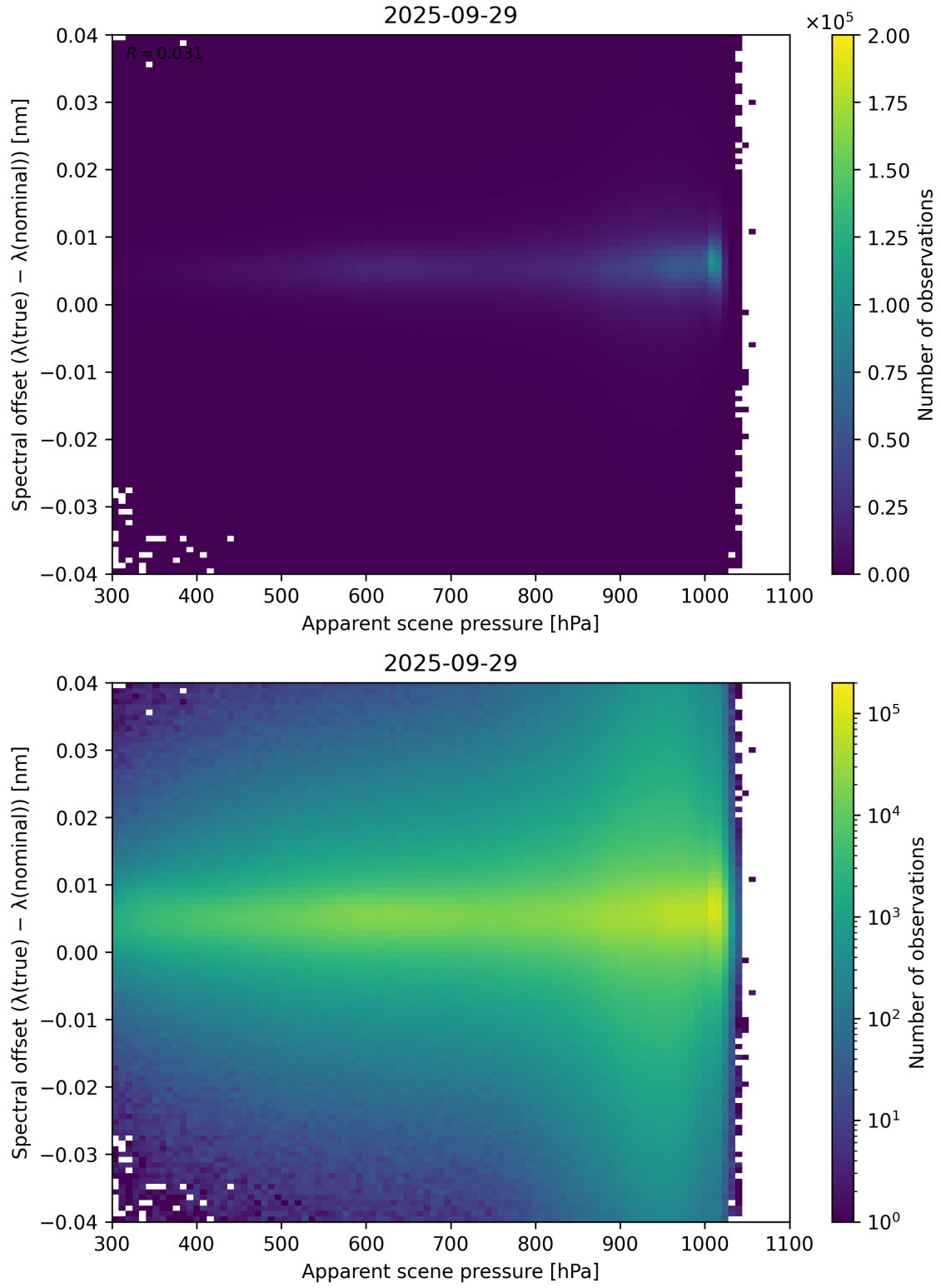
Figure 67: Scatter density plot of “Apparent scene pressure” against “Spectral offset ( \lambda_{\text{true}} - \lambda_{\text{nominal}} )” for 2025-09-28 to 2025-09-30.
