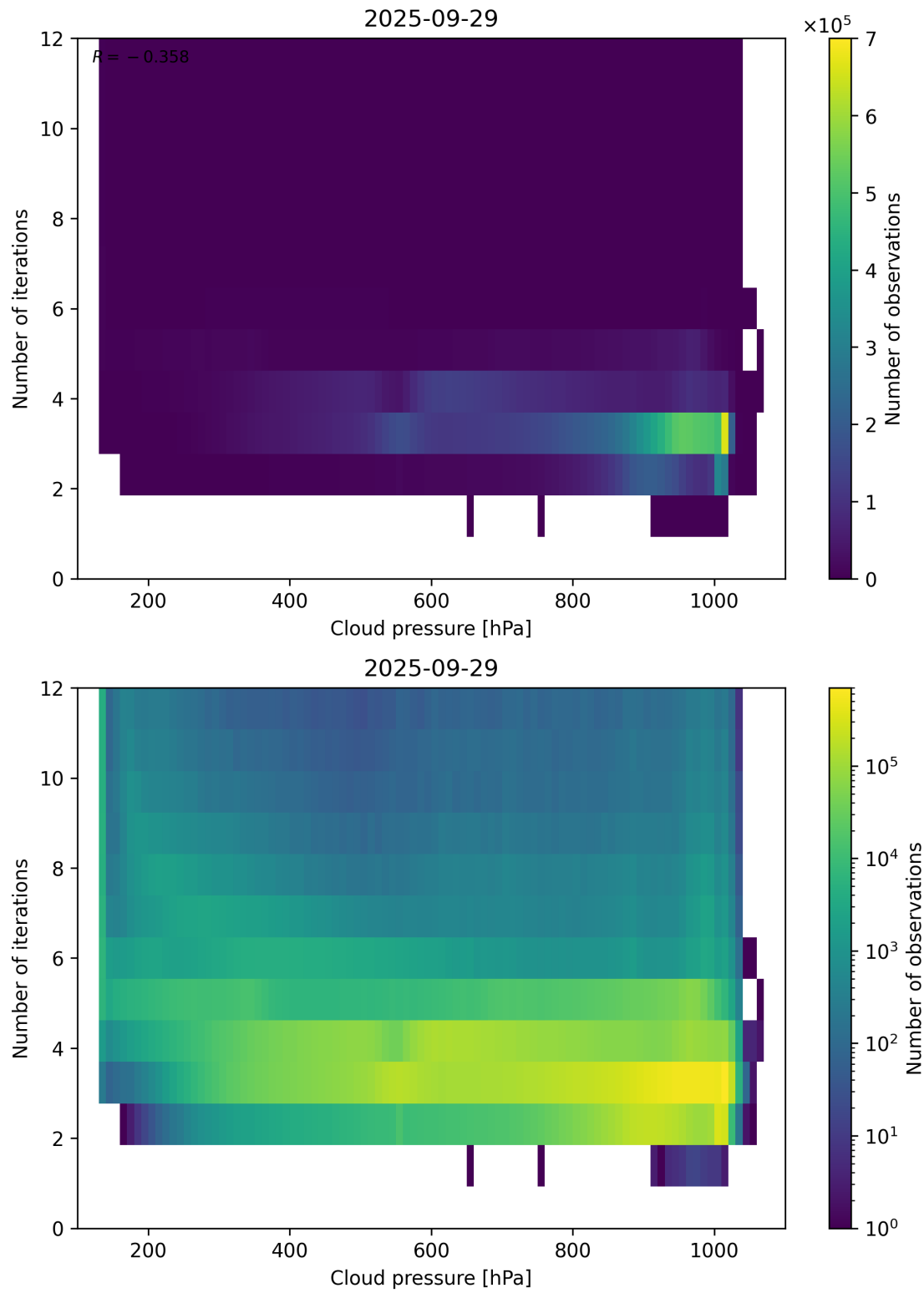
Figure 81: Scatter density plot of “Cloud pressure” against “Number of iterations” for 2025-09-28 to 2025-09-30.
