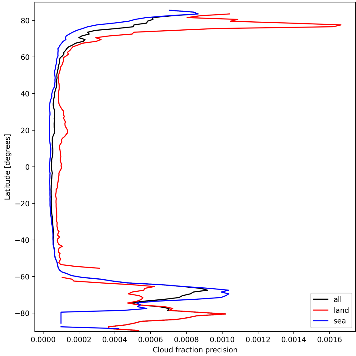
Figure 16: Zonal average of “Cloud fraction precision” for 2025-09-28 to 2025-09-30.
