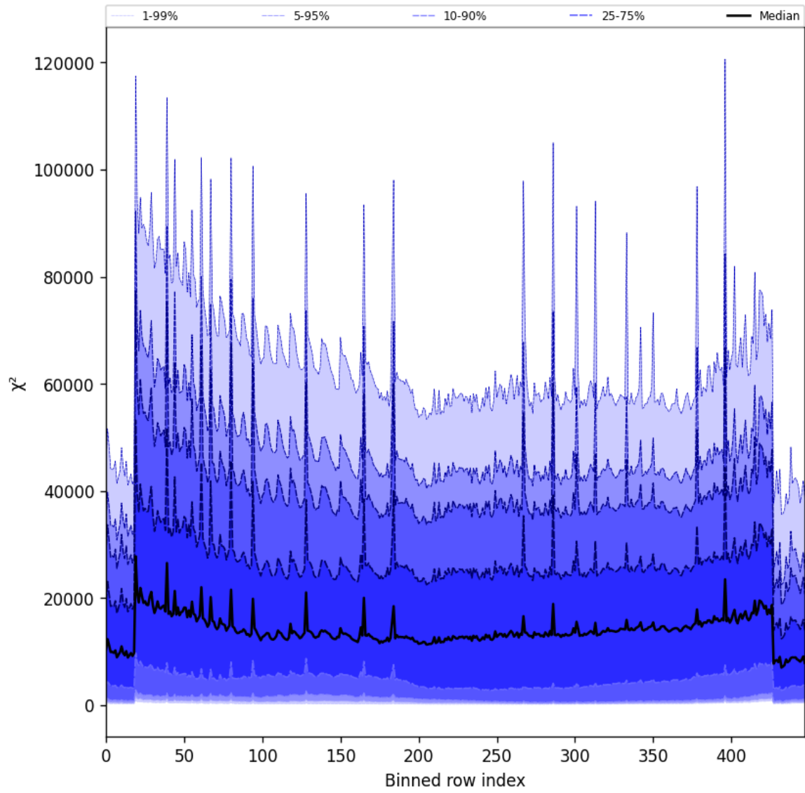
Figure 55: Along track statistics of “ \chi^2 ” for 2025-09-28 to 2025-09-30
