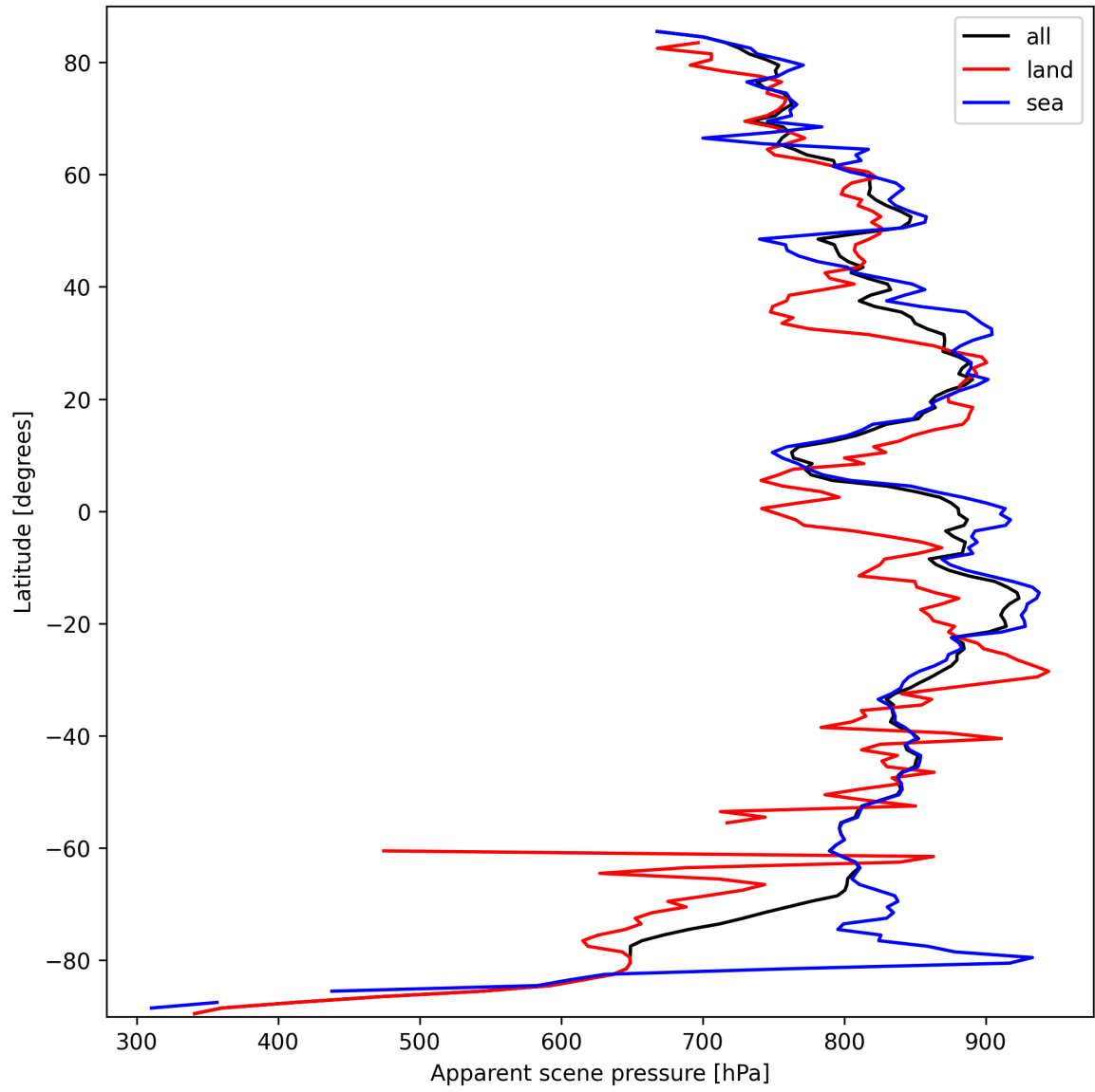
Figure 19: Zonal average of “Apparent scene pressure” for 2025-09-28 to 2025-09-30.
