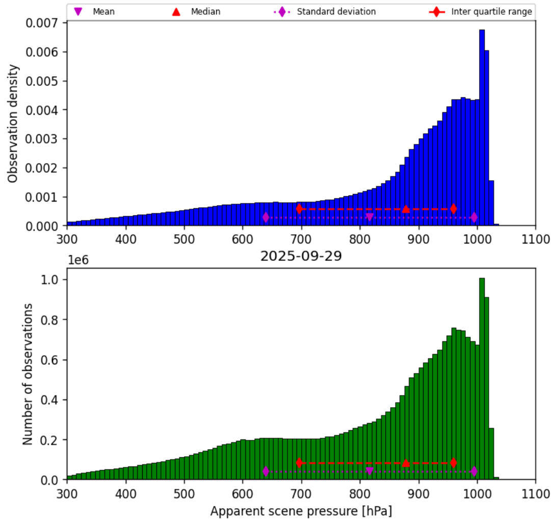
Figure 36: Histogram of “Apparent scene pressure” for 2025-09-28 to 2025-09-30
