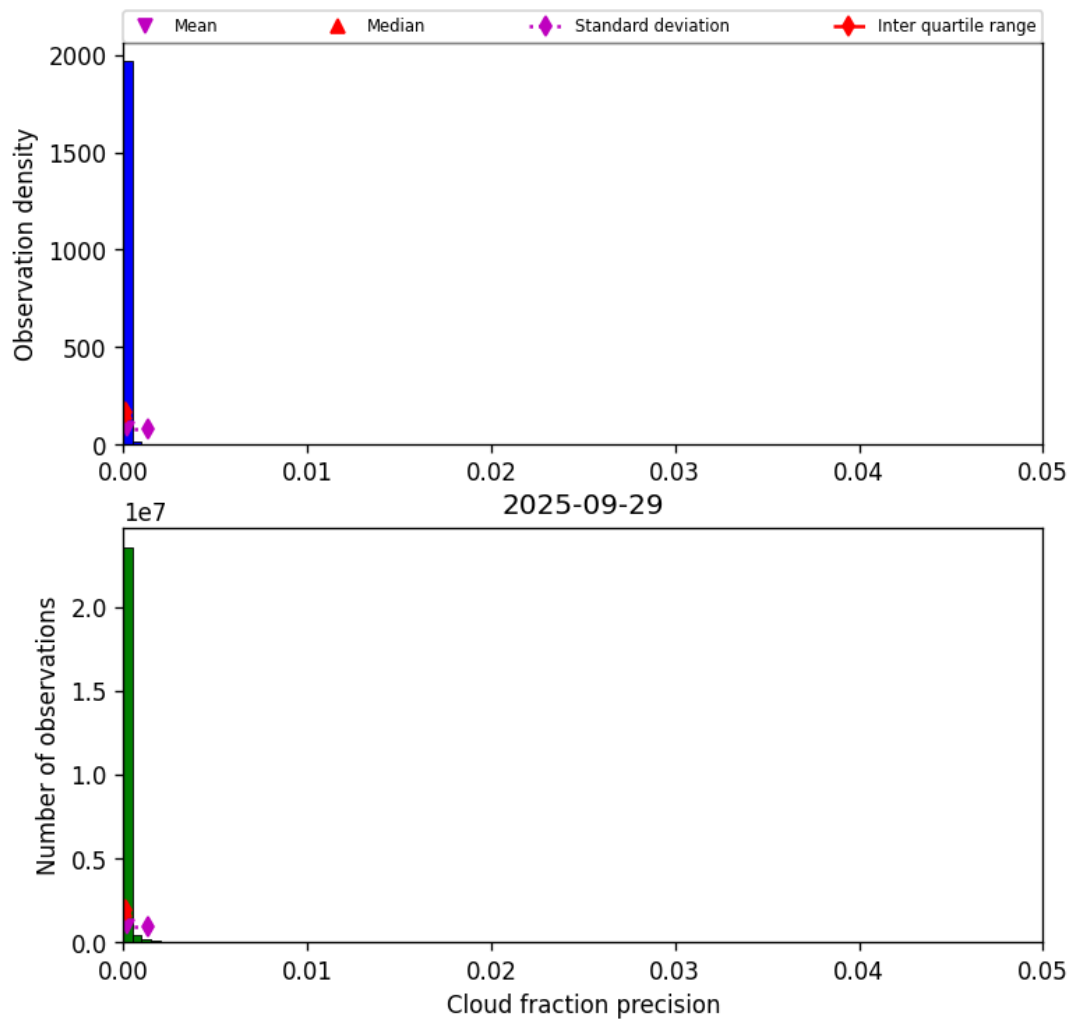
Figure 33: Histogram of “Cloud fraction precision” for 2025-09-28 to 2025-09-30
