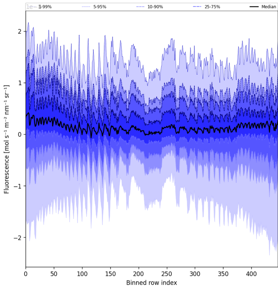
Figure 57: Along track statistics of “Fluorescence” for 2025-09-28 to 2025-09-30
