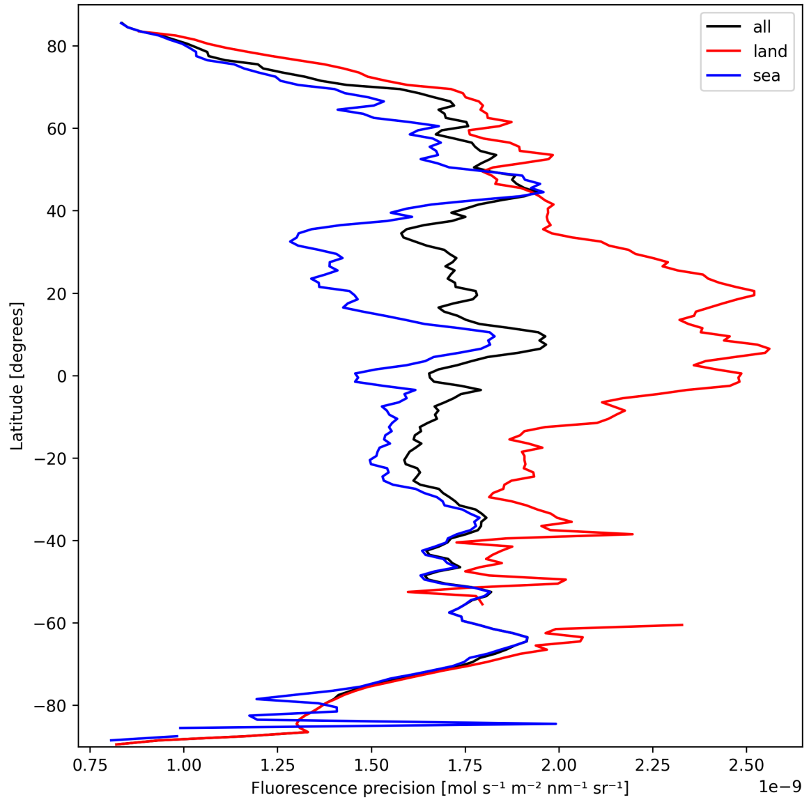
Figure 24: Zonal average of “Fluorescence precision” for 2025-09-28 to 2025-09-30.
