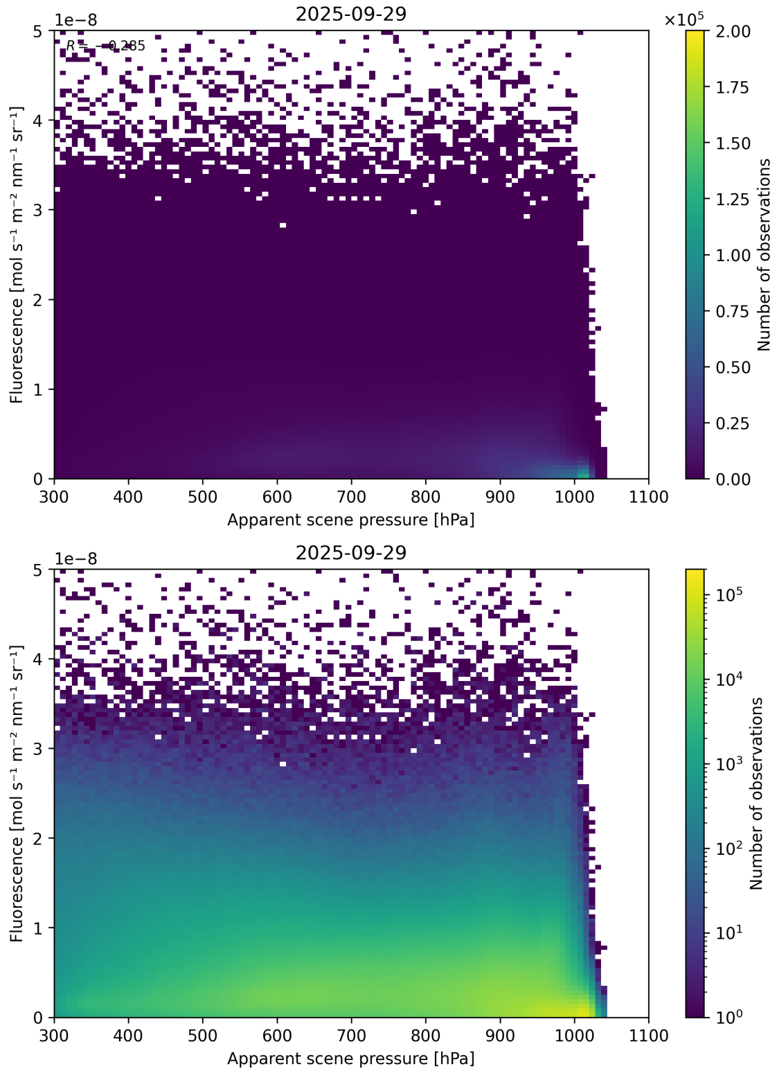
Figure 64: Scatter density plot of “Apparent scene pressure” against “Fluorescence” for 2025-09-28 to 2025-09-30.
