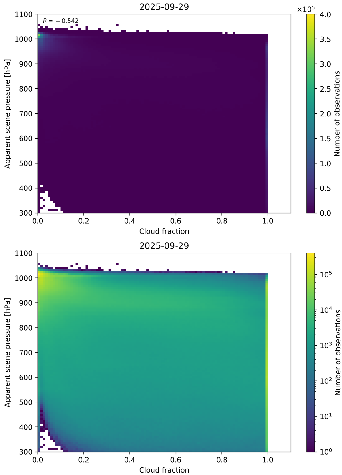
Figure 70: Scatter density plot of “Cloud fraction” against “Apparent scene pressure” for 2025-09-28 to 2025-09-30.
