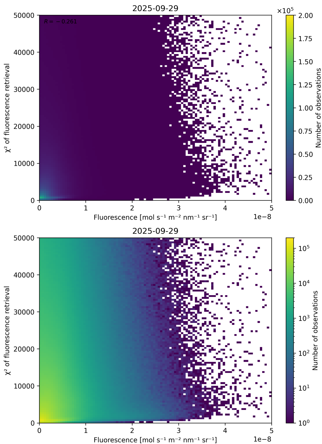
Figure 85: Scatter density plot of “Fluorescence” against “ \chi^2 of fluorescence retrieval” for 2025-09-28 to 2025-09-30.
