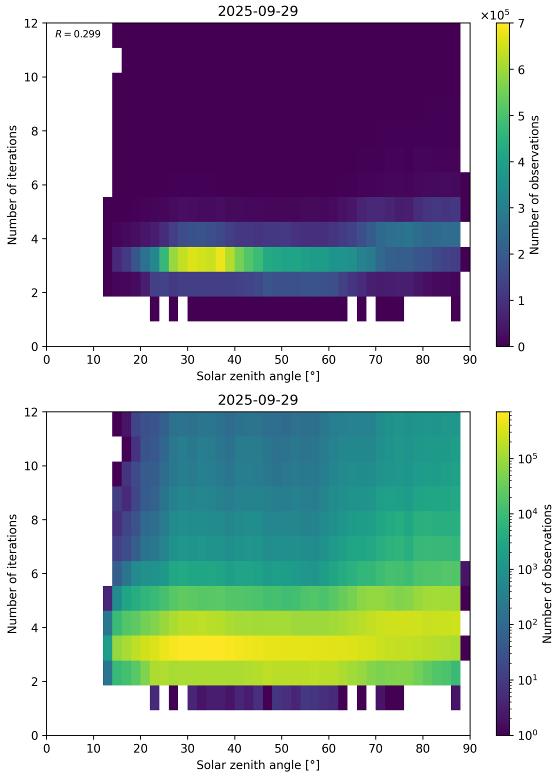
Figure 114: Scatter density plot of “Solar zenith angle” against “Number of iterations” for 2025-09-28 to 2025-09-30.
