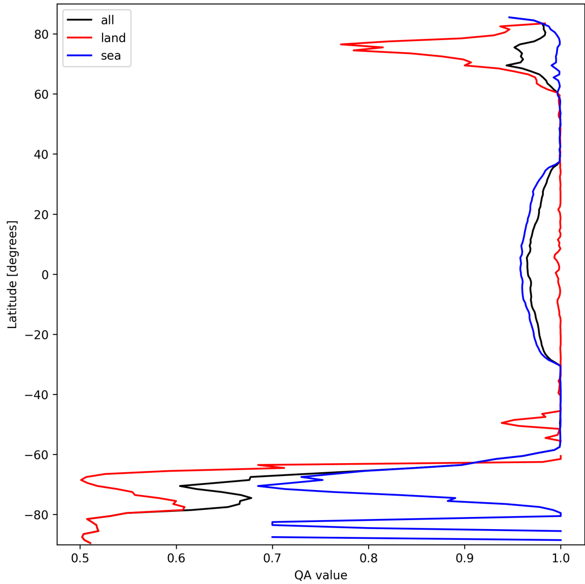
Figure 12: Zonal average of "QA value" for 2025-09-28 to 2025-09-30.
