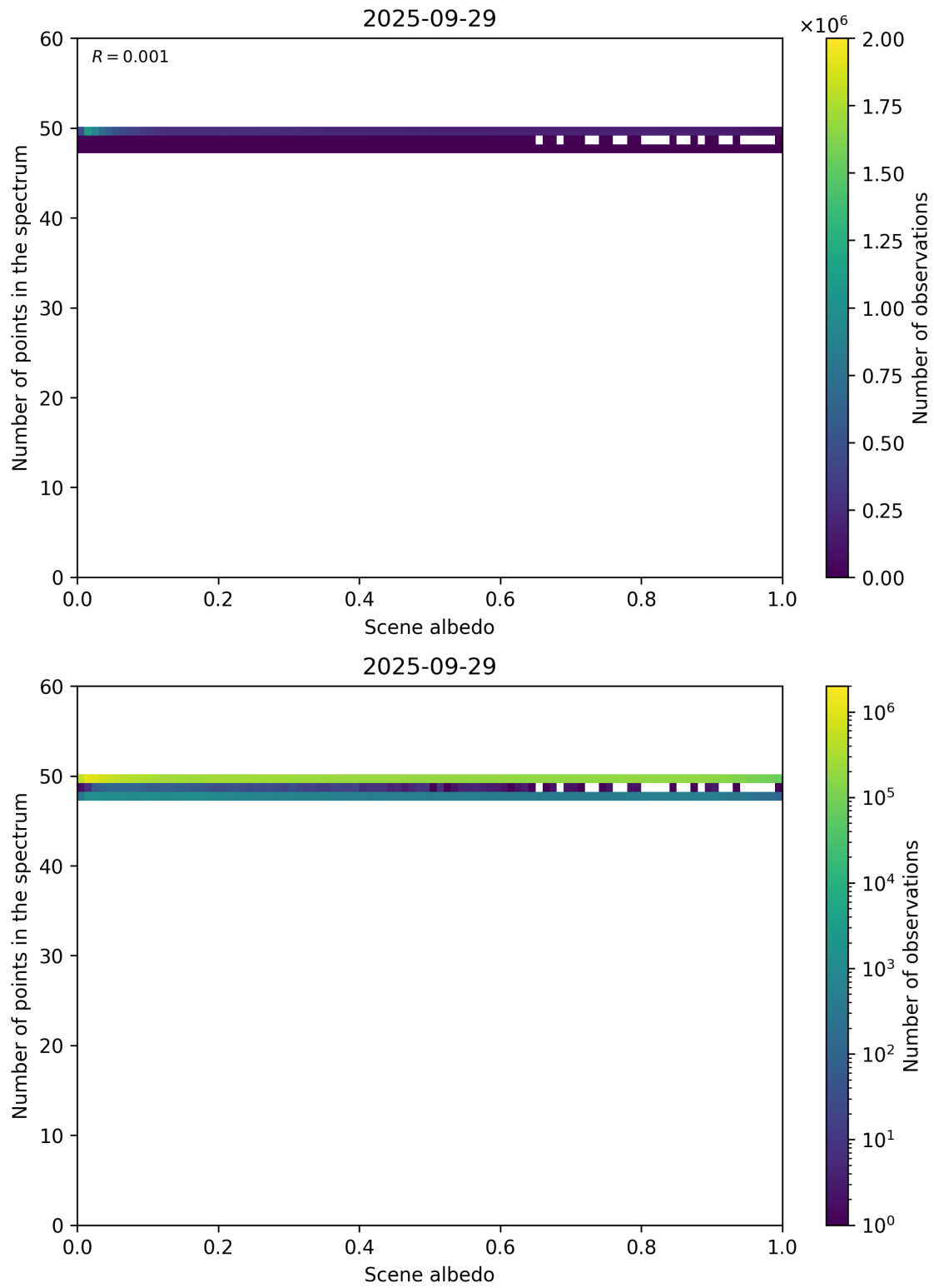
Figure 106: Scatter density plot of “Scene albedo” against “Number of points in the spectrum” for 2025-09-28 to 2025-09-30.
