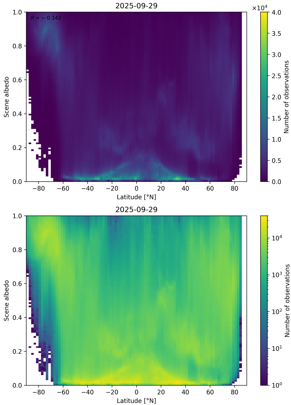
Figure 95: Scatter density plot of “Latitude” against “Scene albedo” for 2025-09-28 to 2025-09-30.
