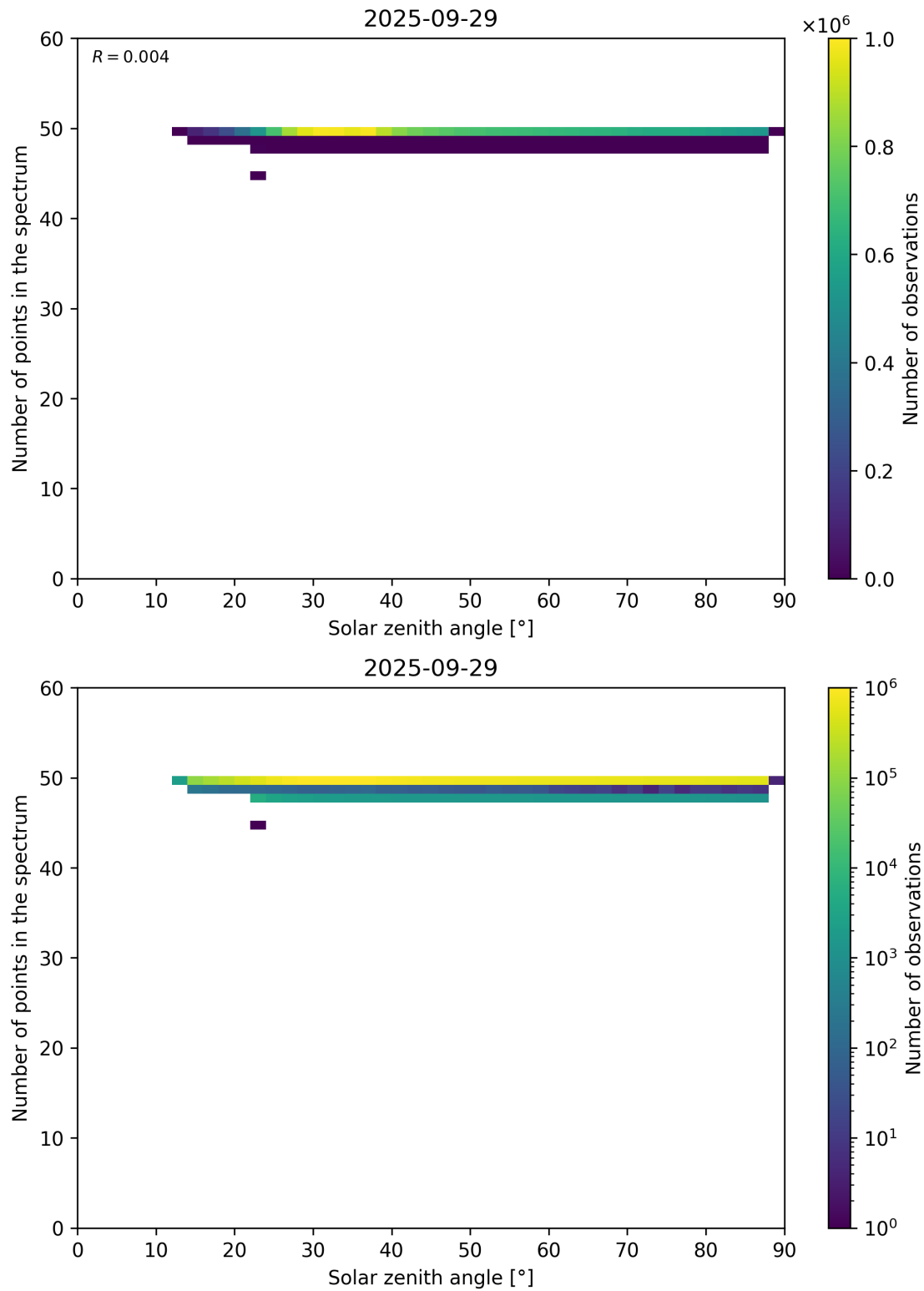
Figure 115: Scatter density plot of “Solar zenith angle” against “Number of points in the spectrum” for 2025-09-28 to 2025-09-30.
