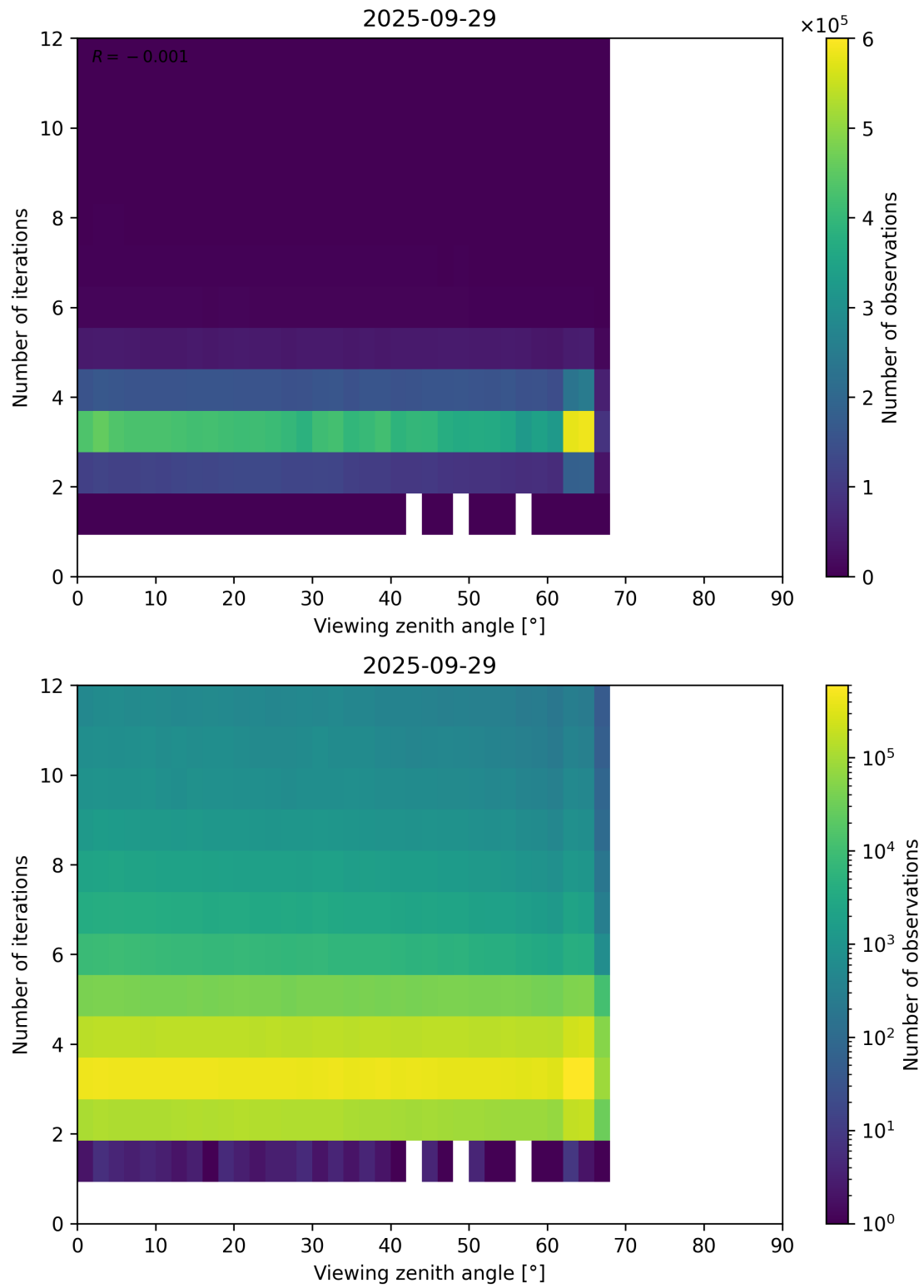
Figure 124: Scatter density plot of “Viewing zenith angle” against “Number of iterations” for 2025-09-28 to 2025-09-30.
