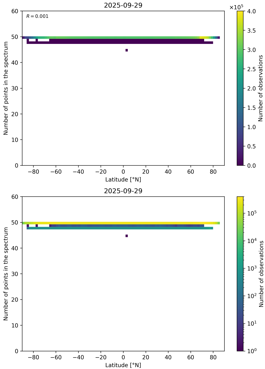
Figure 94: Scatter density plot of “Latitude” against “Number of points in the spectrum” for 2025-09-28 to 2025-09-30.
