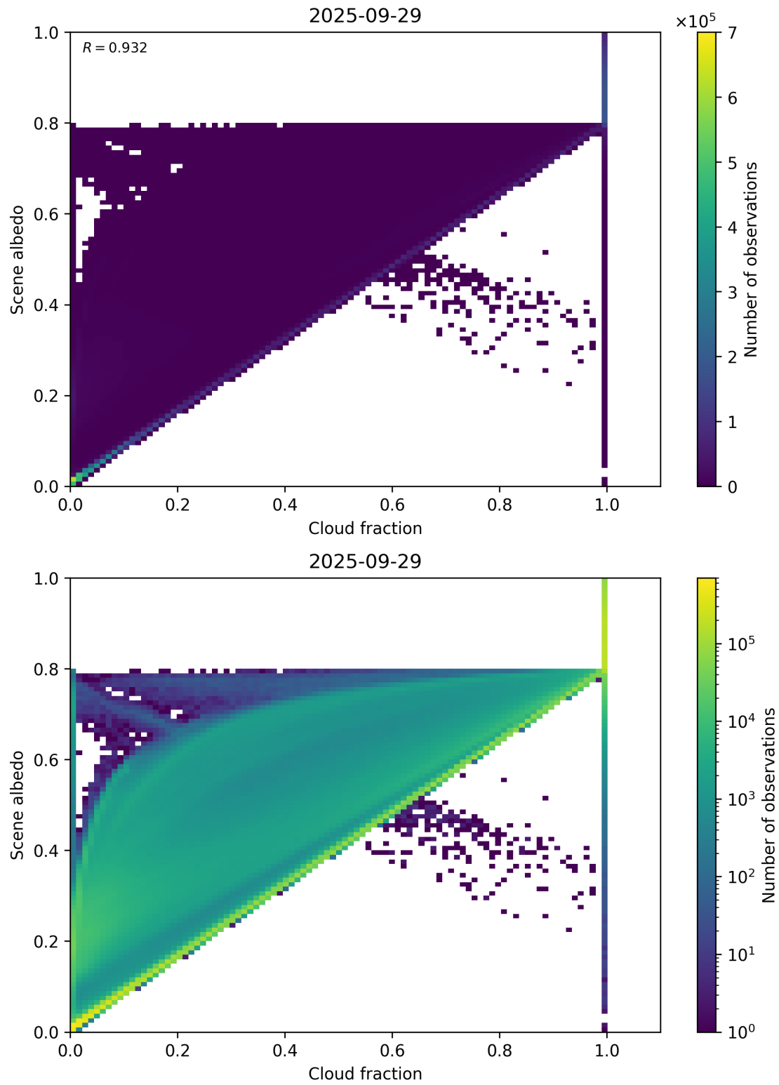
Figure 75: Scatter density plot of “Cloud fraction” against “Scene albedo” for 2025-09-28 to 2025-09-30.
