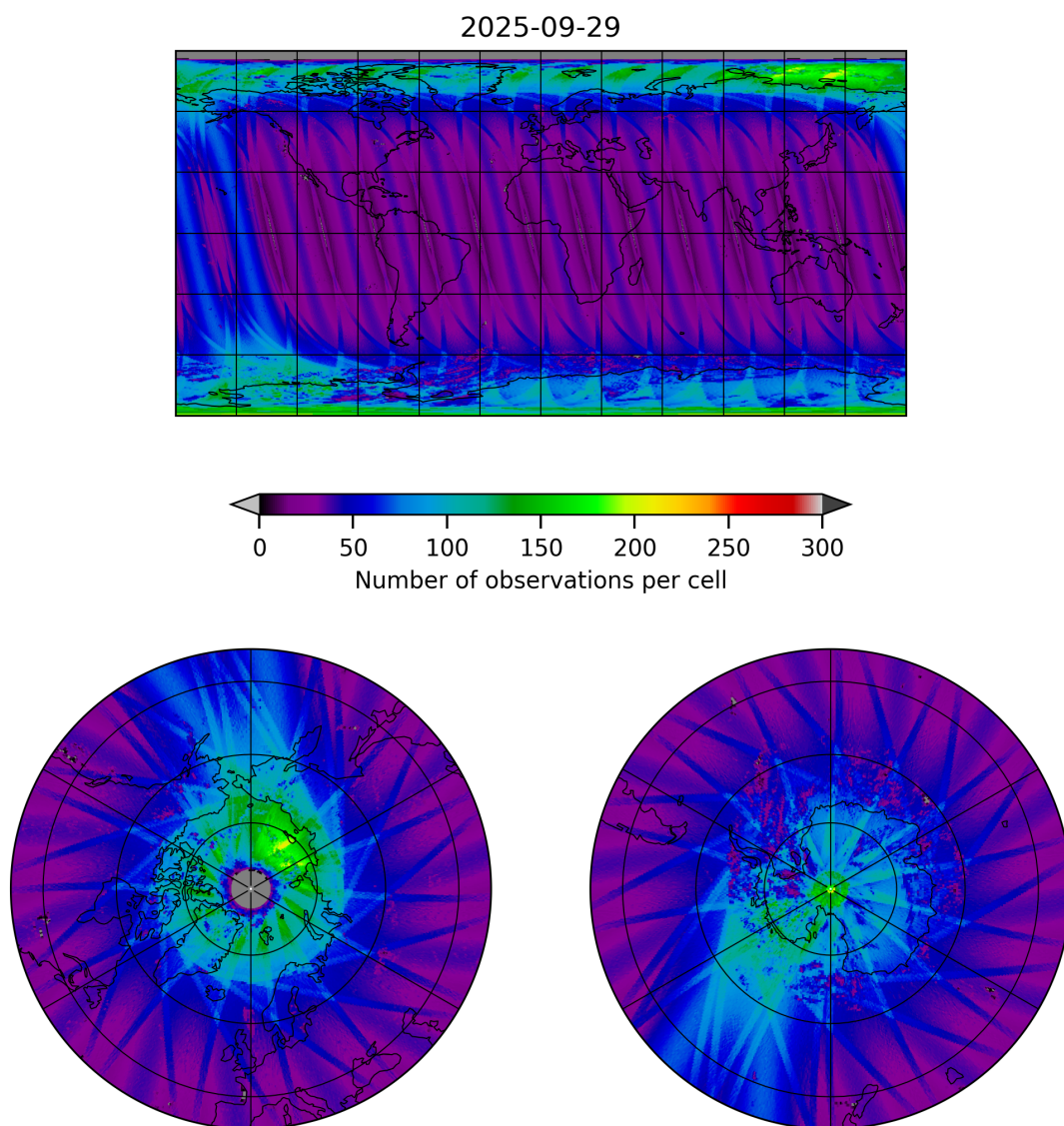
Figure 11: Map of the number of observations for 2025-09-28 to 2025-09-30
