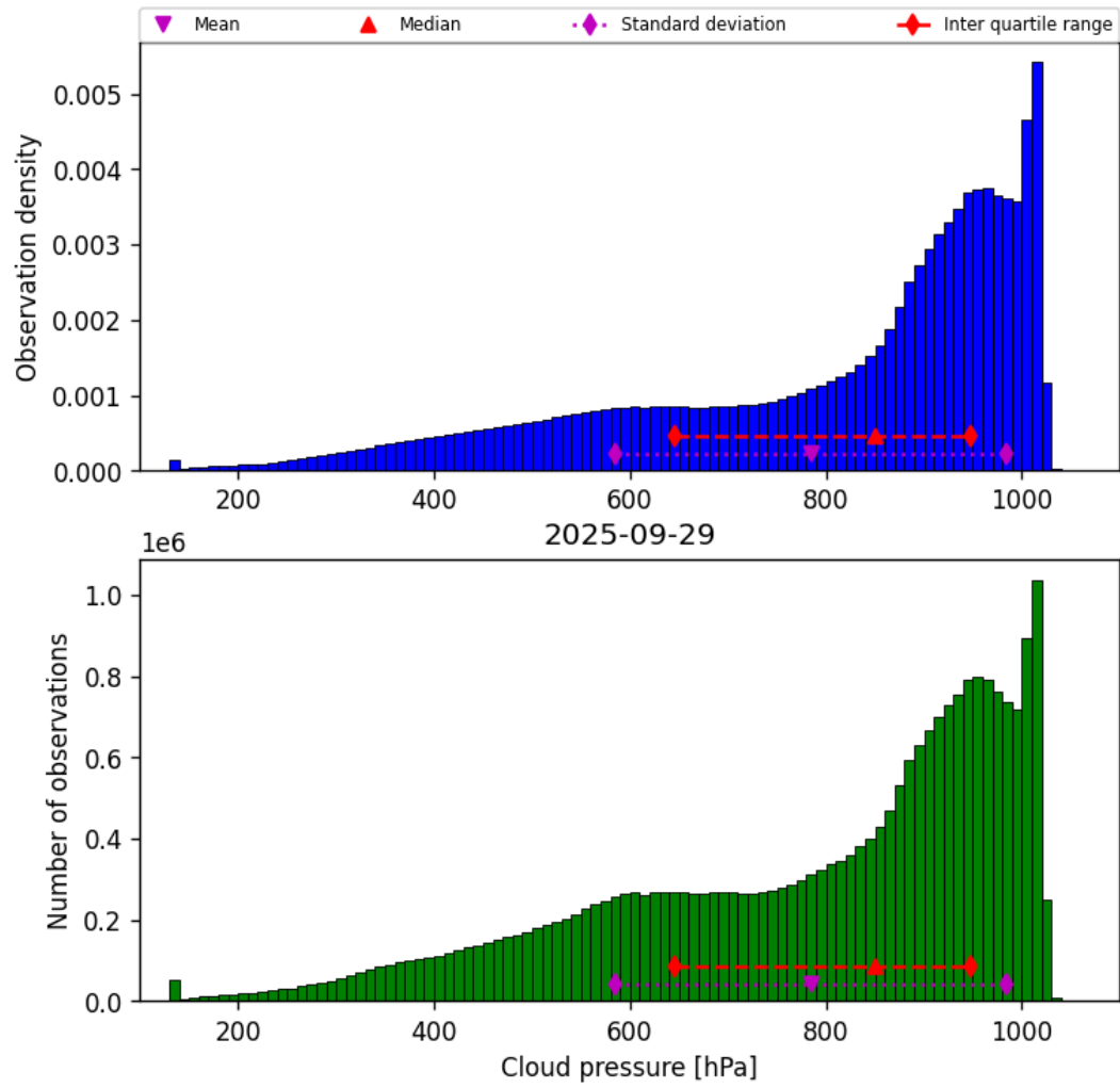
Figure 30: Histogram of “Cloud pressure” for 2025-09-28 to 2025-09-30
