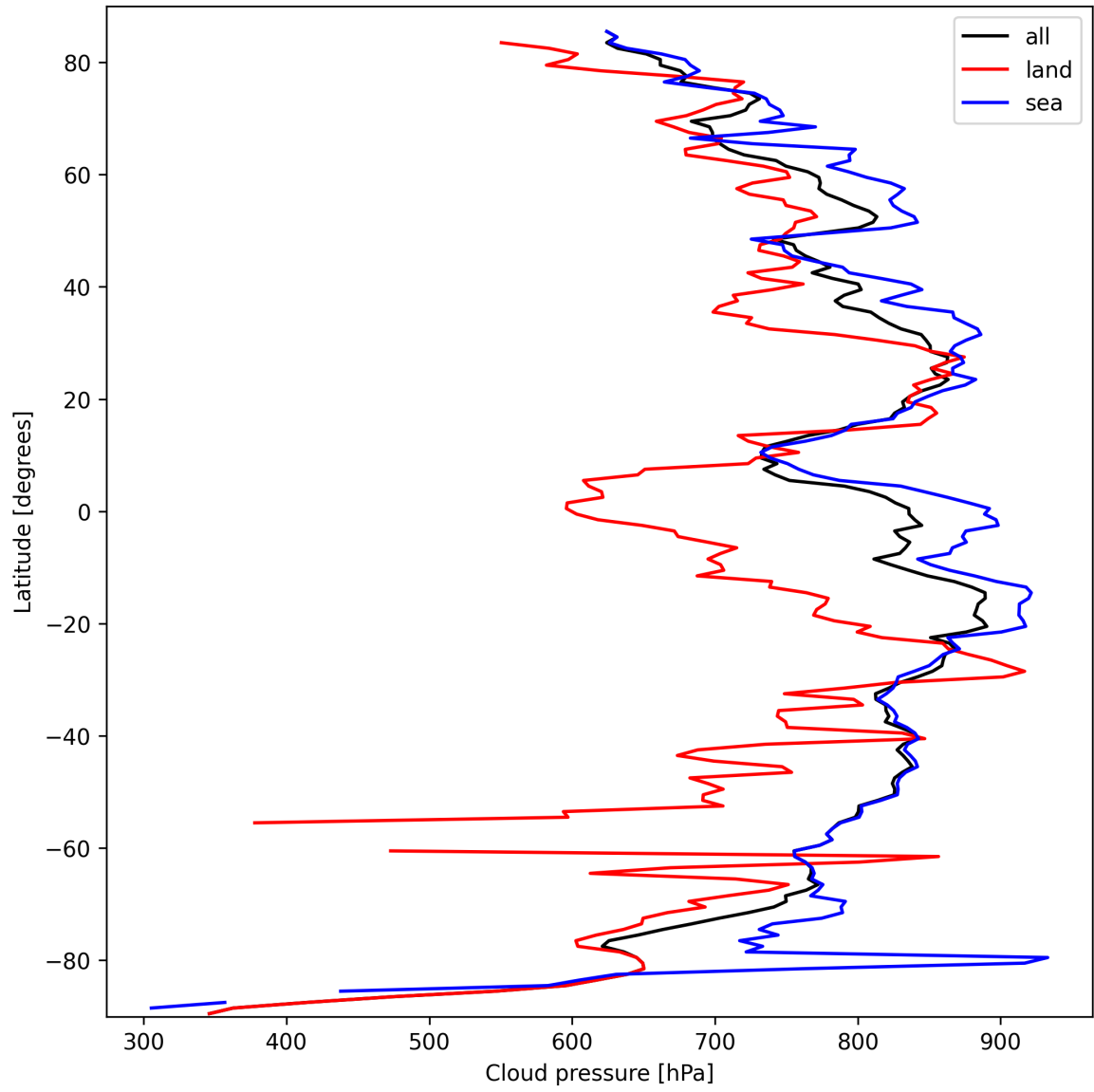
Figure 13: Zonal average of “Cloud pressure” for 2025-09-28 to 2025-09-30.
