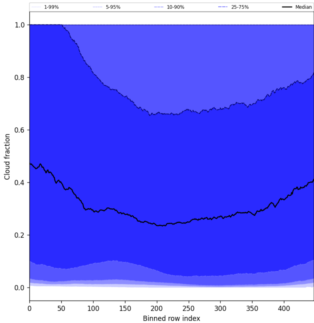
Figure 49: Along track statistics of “Cloud fraction” for 2025-09-28 to 2025-09-30
