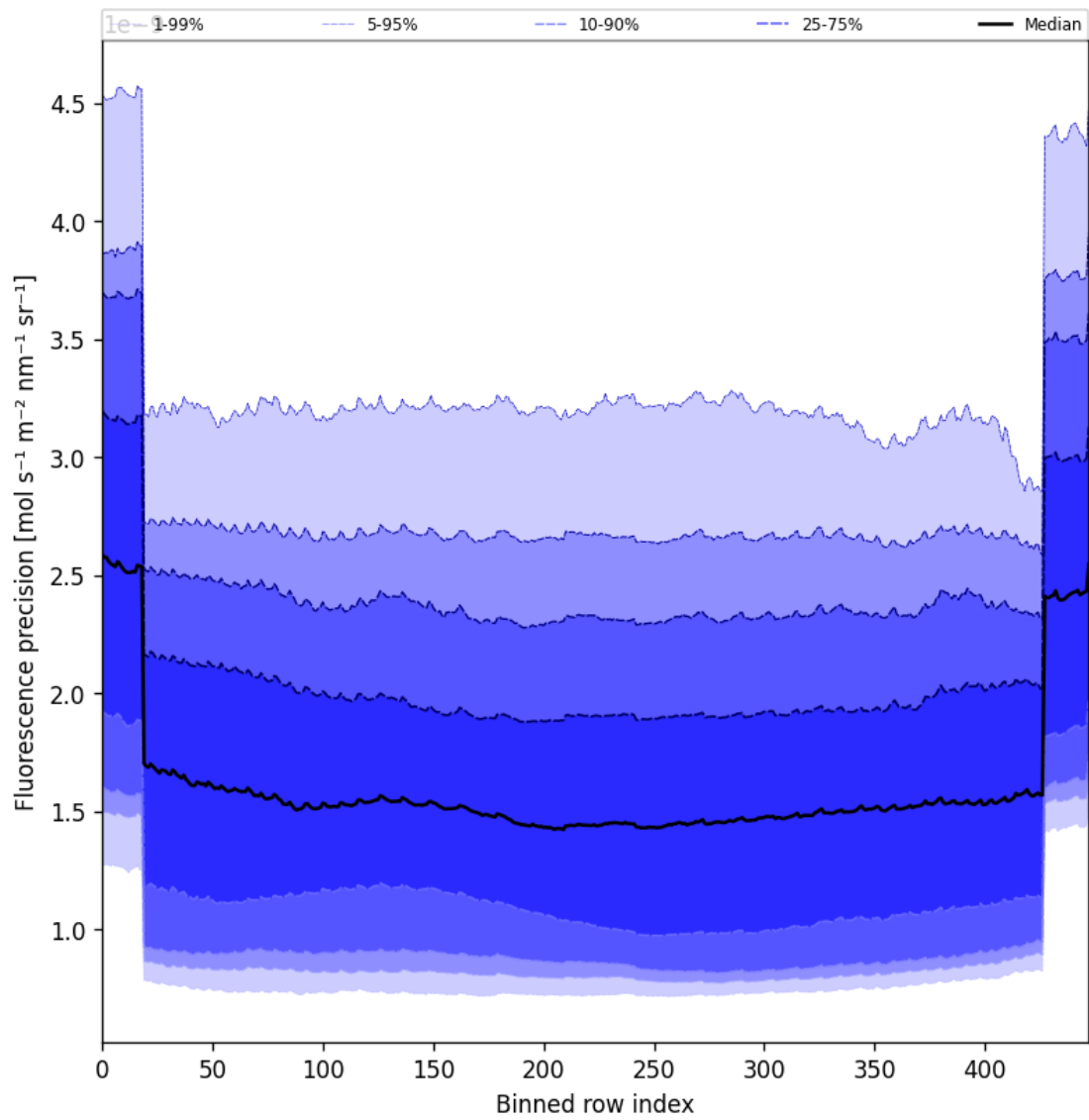
Figure 58: Along track statistics of “Fluorescence precision” for 2025-09-28 to 2025-09-30
