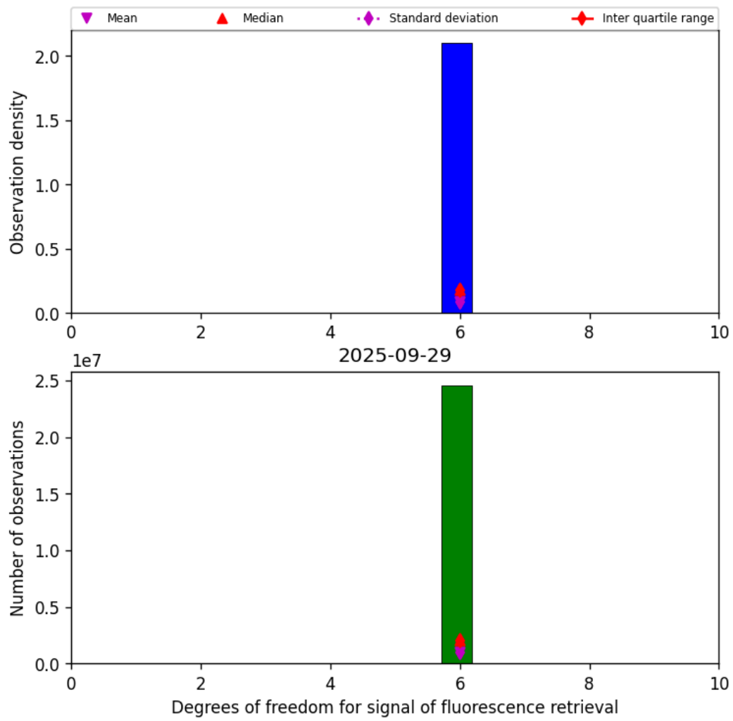
Figure 43: Histogram of "Degrees of freedom for signal of fluorescence retrieval" for 2025-09-28 to 2025-09-30
