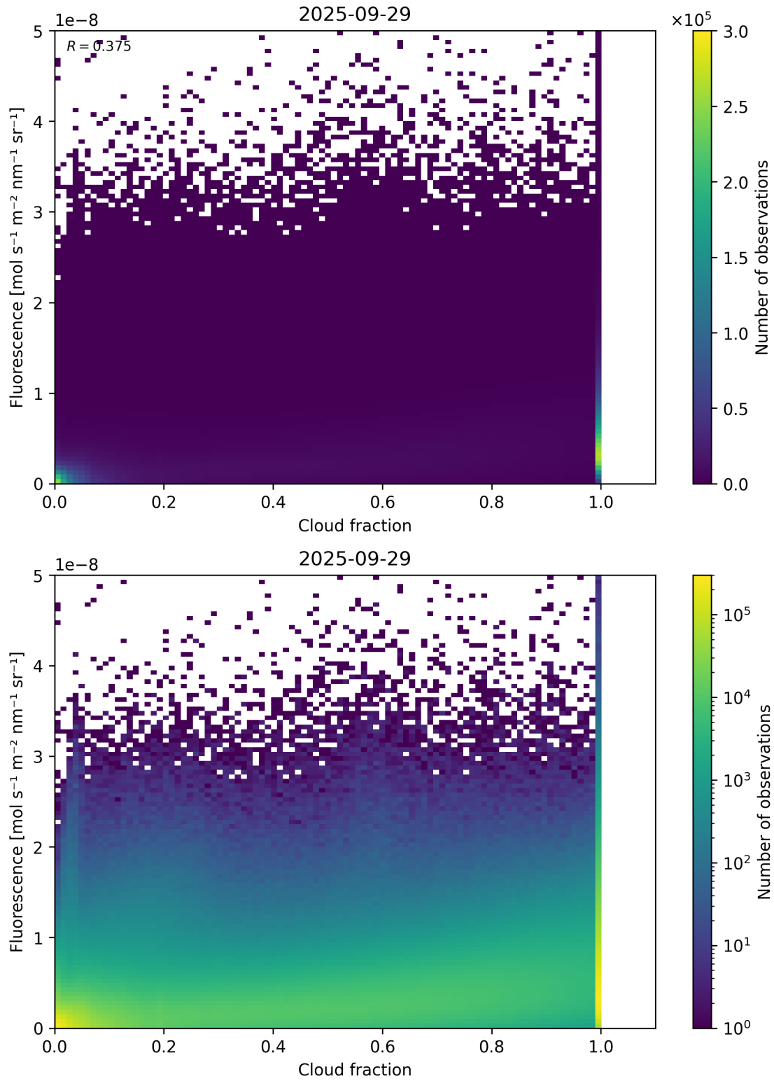
Figure 72: Scatter density plot of “Cloud fraction” against “Fluorescence” for 2025-09-28 to 2025-09-30.
