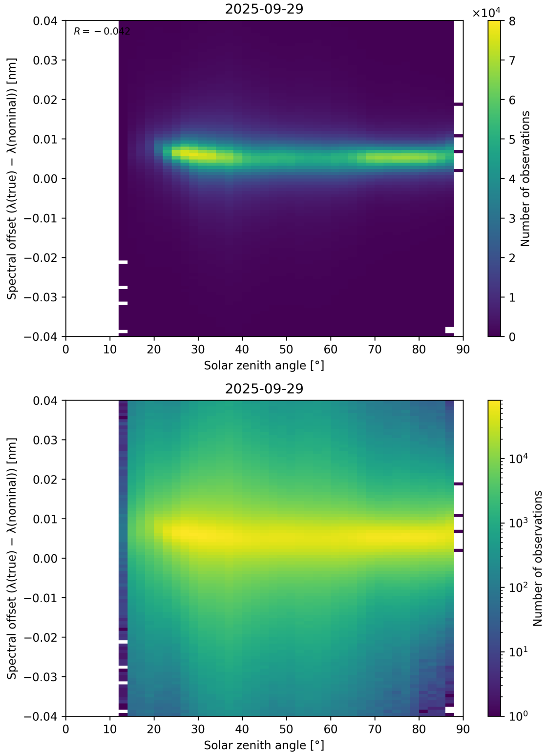
Figure 117: Scatter density plot of “Solar zenith angle” against “Spectral offset ( \lambda_{\text{true}} - \lambda_{\text{nominal}} )” for 2025-09-28 to 2025-09-30.
