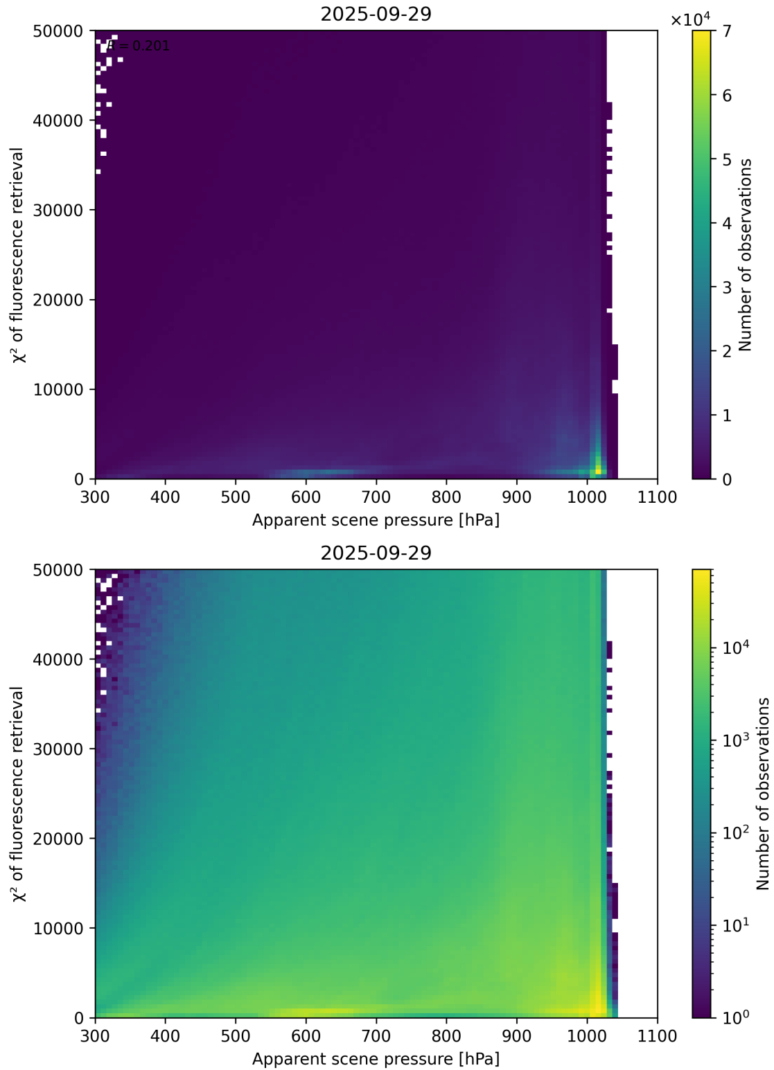
Figure 63: Scatter density plot of “Apparent scene pressure” against “ \chi^2 of fluorescence retrieval” for 2025-09-28 to 2025-09-30.
