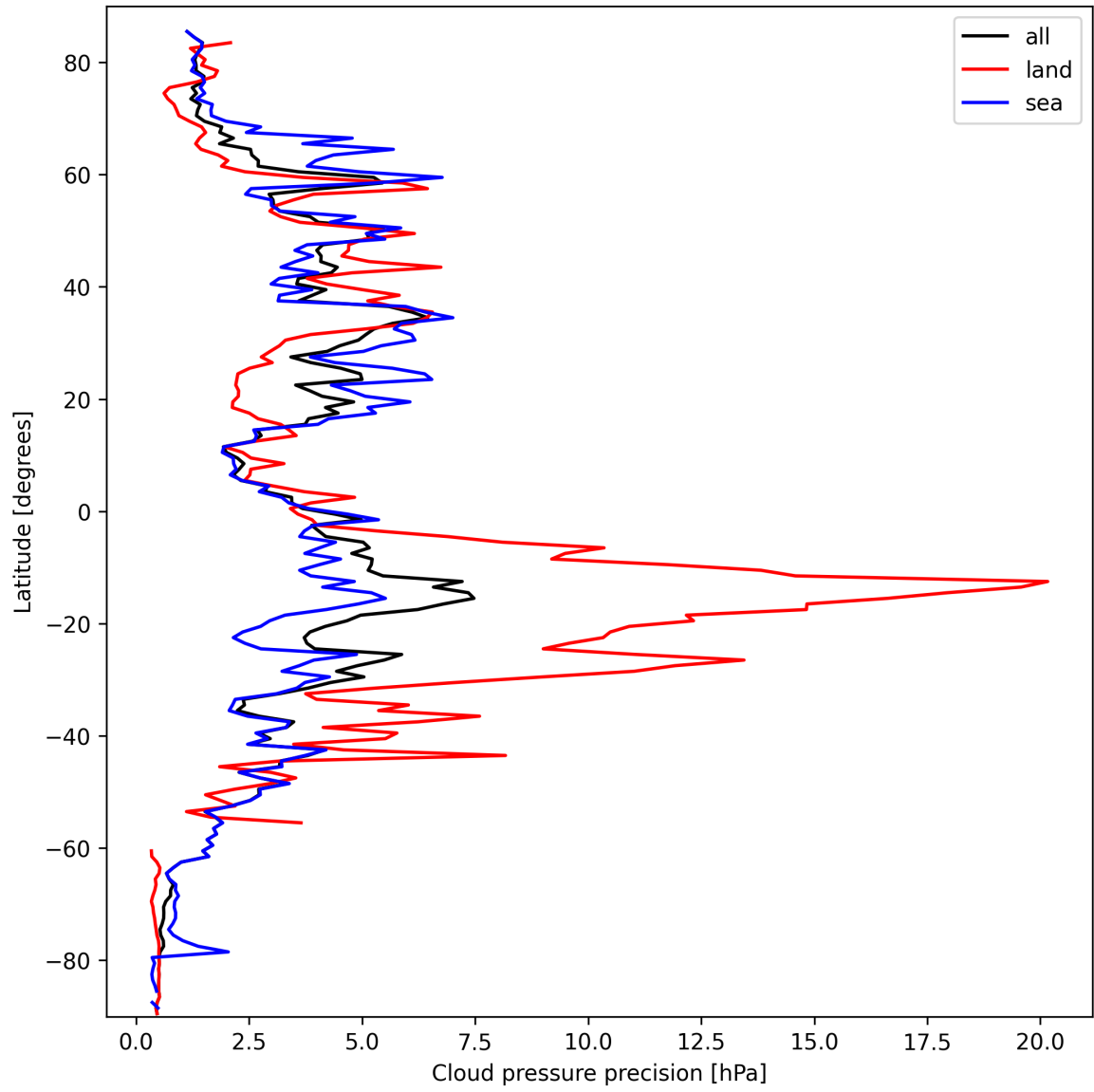
Figure 14: Zonal average of “Cloud pressure precision” for 2025-09-28 to 2025-09-30.
