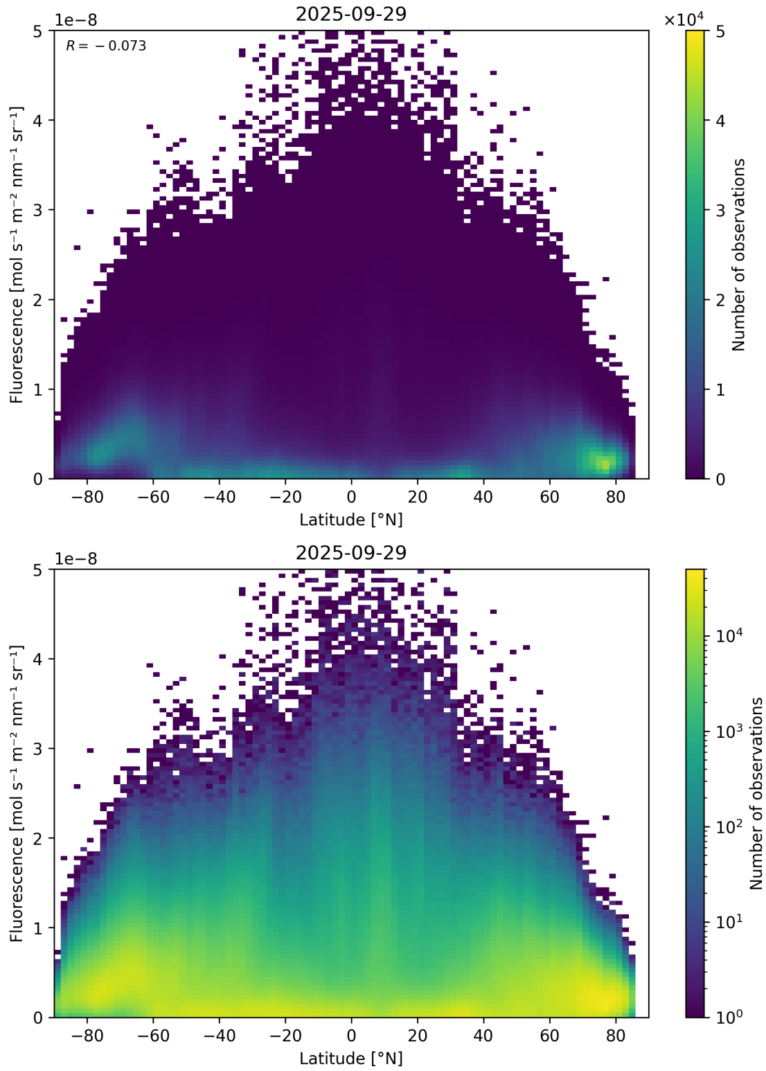
Figure 92: Scatter density plot of “Latitude” against “Fluorescence” for 2025-09-28 to 2025-09-30.
