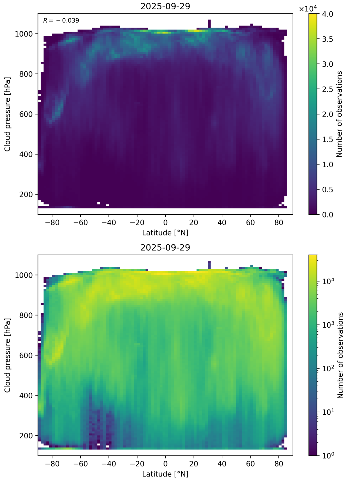
Figure 91: Scatter density plot of “Latitude” against “Cloud pressure” for 2025-09-28 to 2025-09-30.
