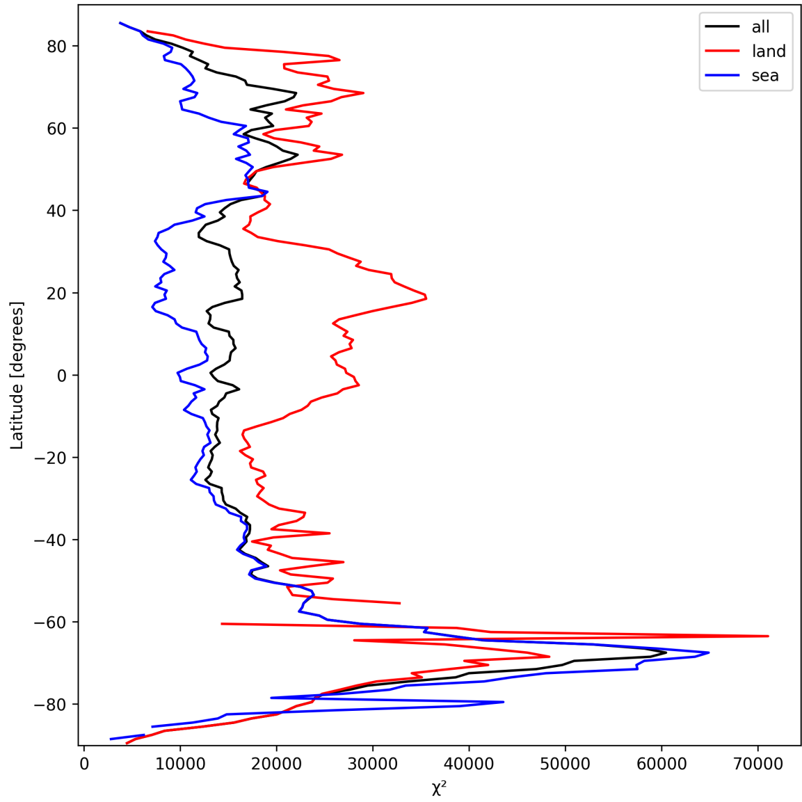
Figure 21: Zonal average of “ \chi^2 ” for 2025-09-28 to 2025-09-30.
