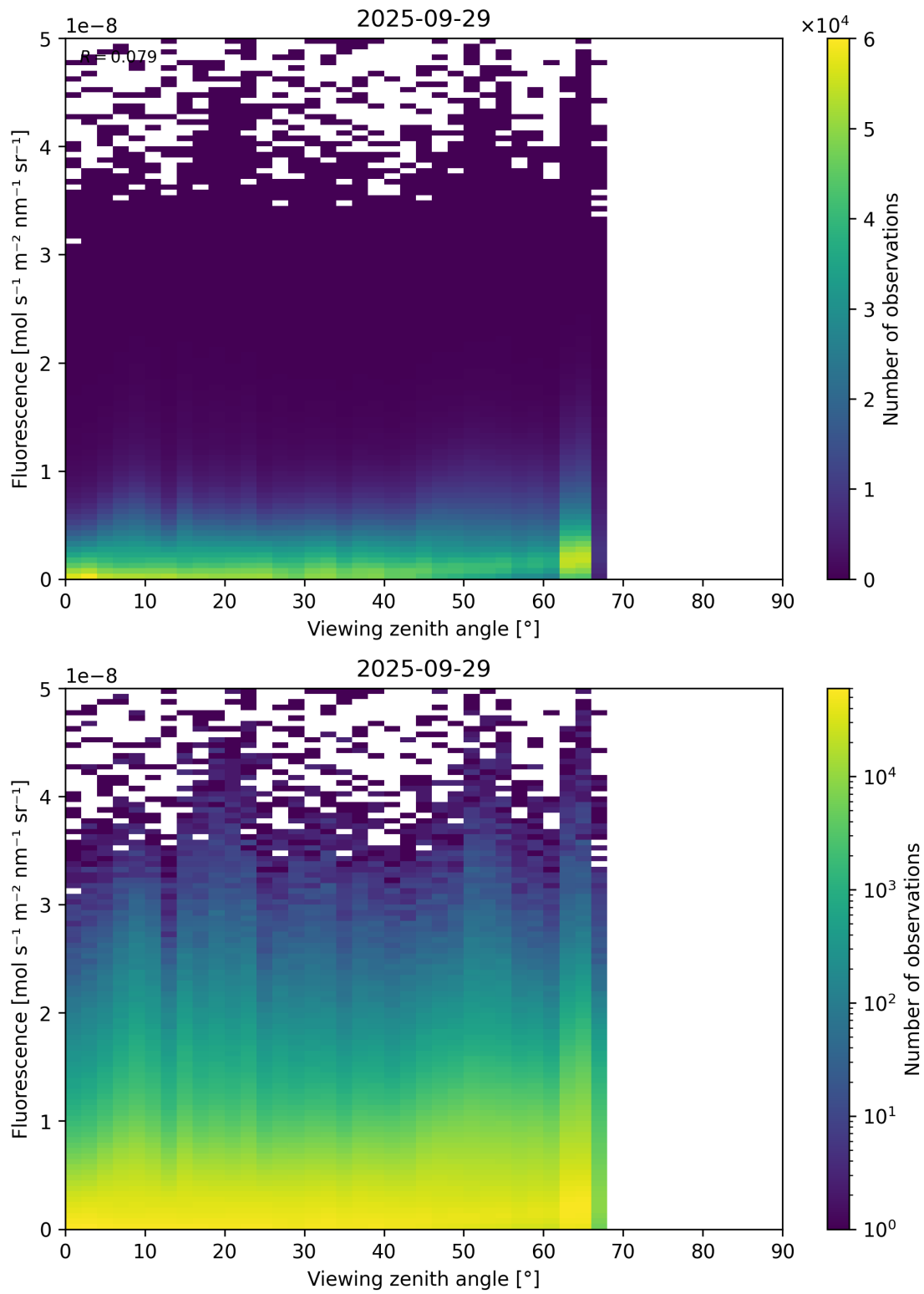
Figure 122: Scatter density plot of “Viewing zenith angle” against “Fluorescence” for 2025-09-28 to 2025-09-30.
