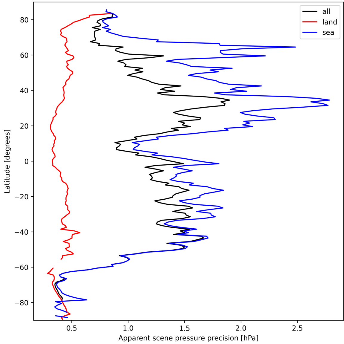
Figure 20: Zonal average of “Apparent scene pressure precision” for 2025-09-28 to 2025-09-30.
