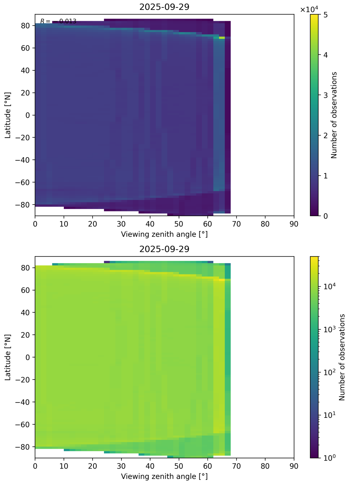
Figure 123: Scatter density plot of “Viewing zenith angle” against “Latitude” for 2025-09-28 to 2025-09-30.
