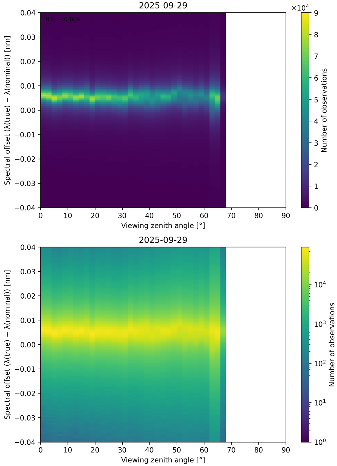
Figure 128: Scatter density plot of “Viewing zenith angle” against “Spectral offset ( \lambda_{\text{true}} - \lambda_{\text{nominal}} )” for 2025-09-28 to 2025-09-30.
