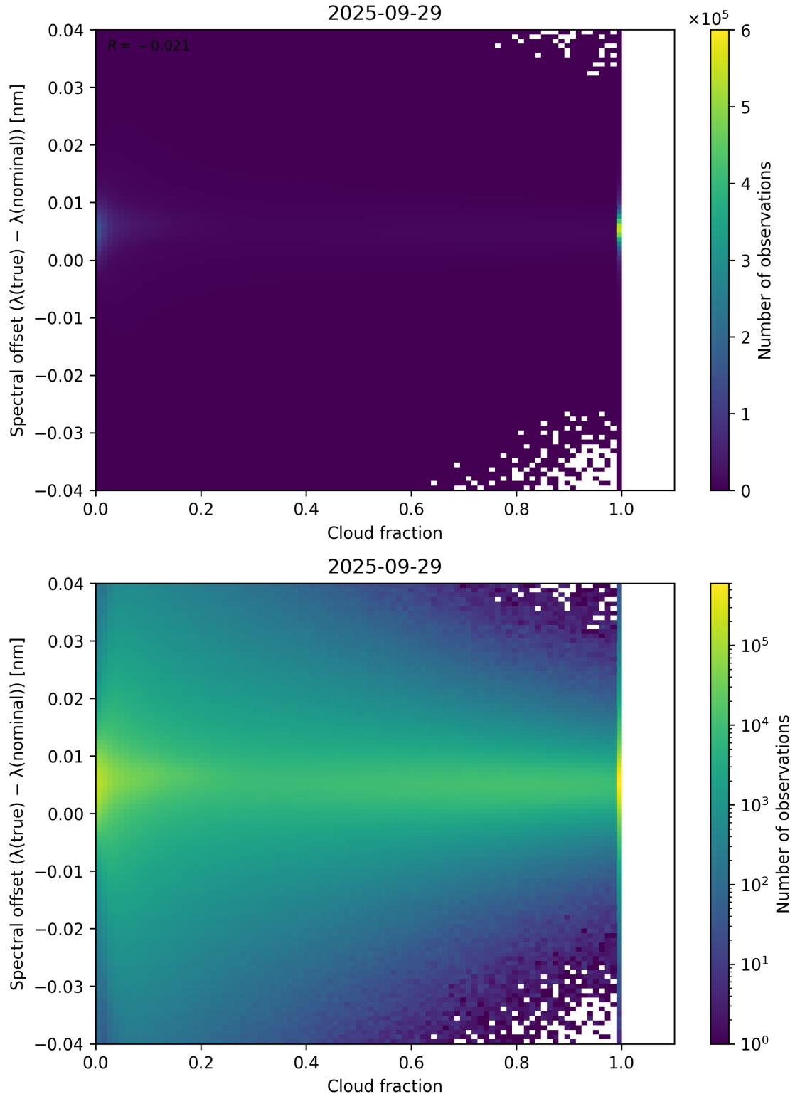
Figure 76: Scatter density plot of “Cloud fraction” against “Spectral offset ( \lambda_{\text{true}} - \lambda_{\text{nominal}} )” for 2025-09-28 to 2025-09-30.
