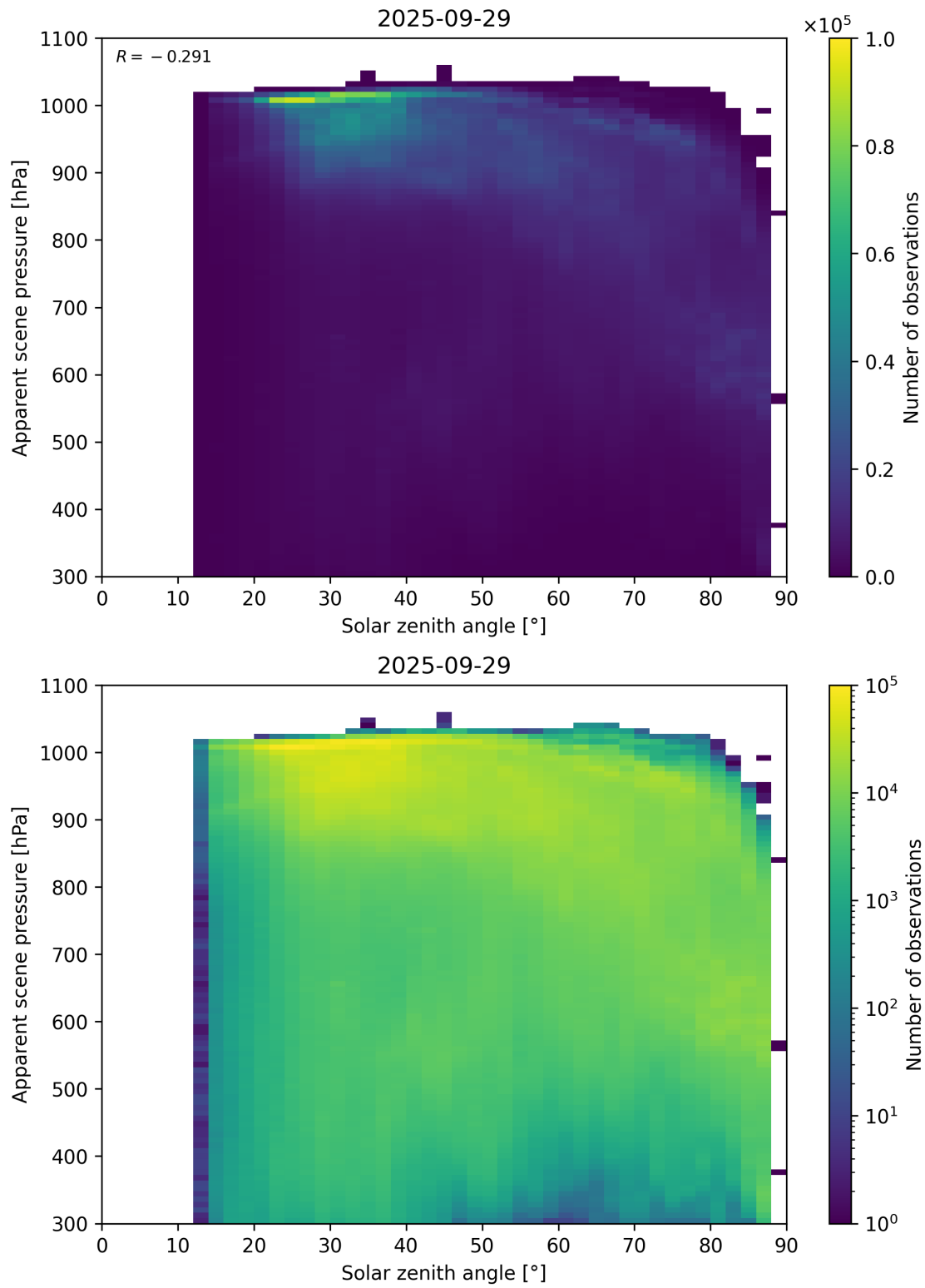
Figure 108: Scatter density plot of “Solar zenith angle” against “Apparent scene pressure” for 2025-09-28 to 2025-09-30.
