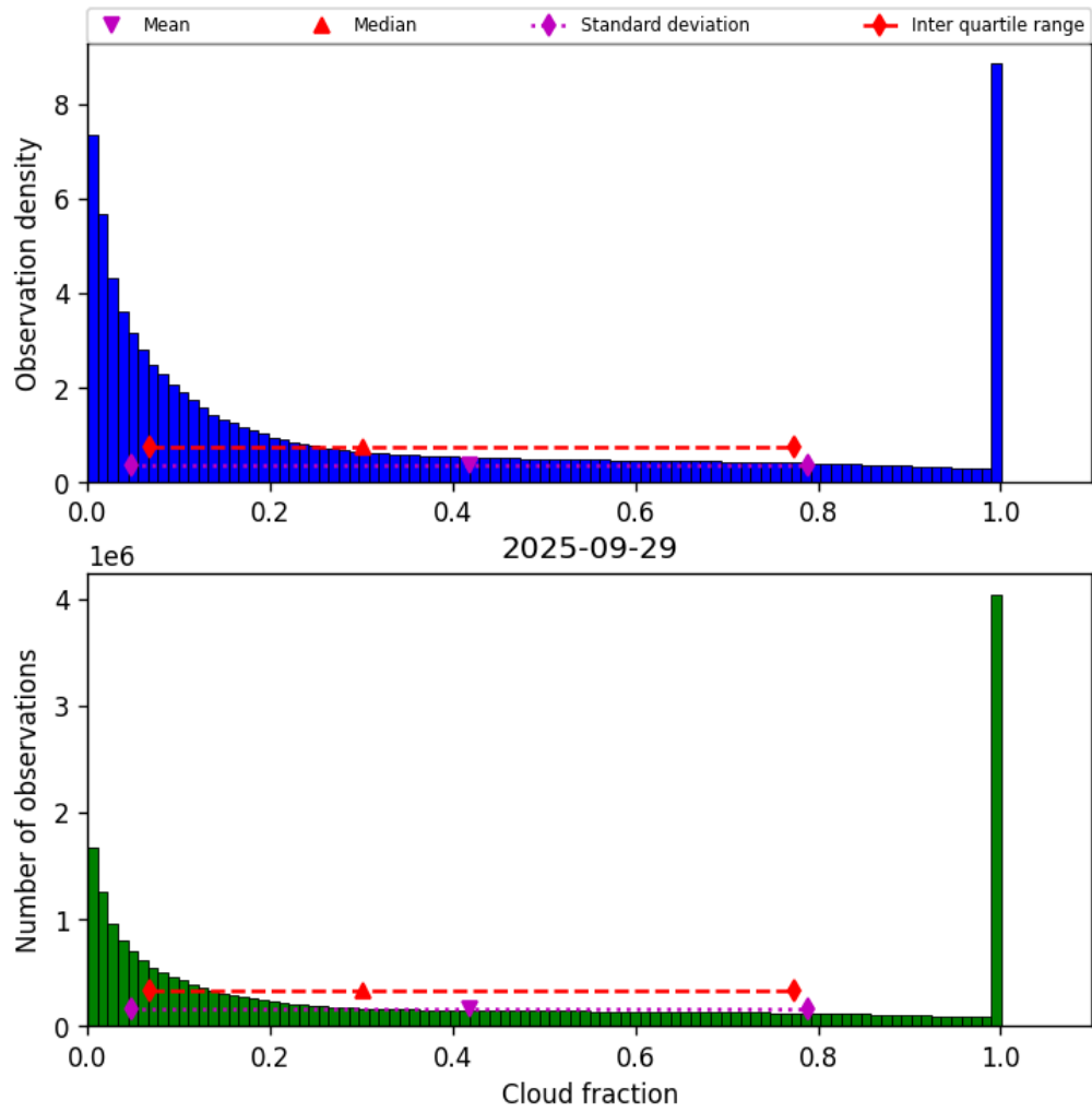
Figure 32: Histogram of “Cloud fraction” for 2025-09-28 to 2025-09-30
