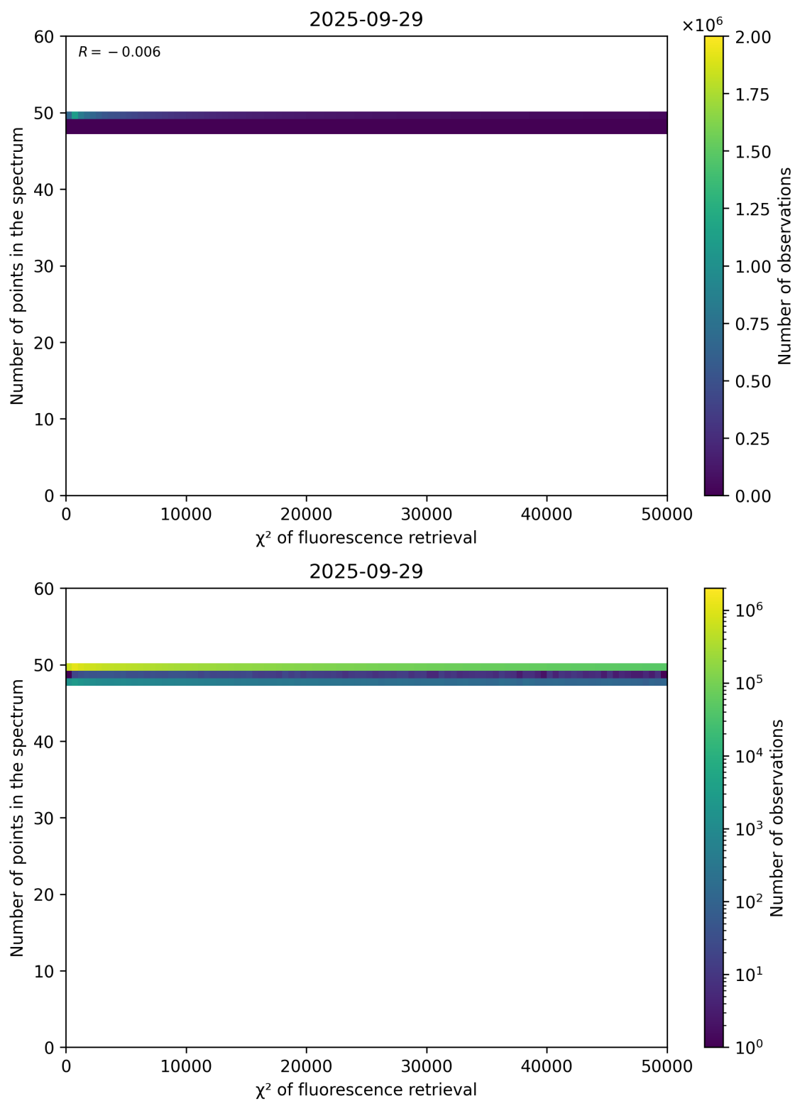
Figure 68: Scatter density plot of “ \chi^2 of fluorescence retrieval” against “Number of points in the spectrum” for 2025-09-28 to 2025-09-30.
