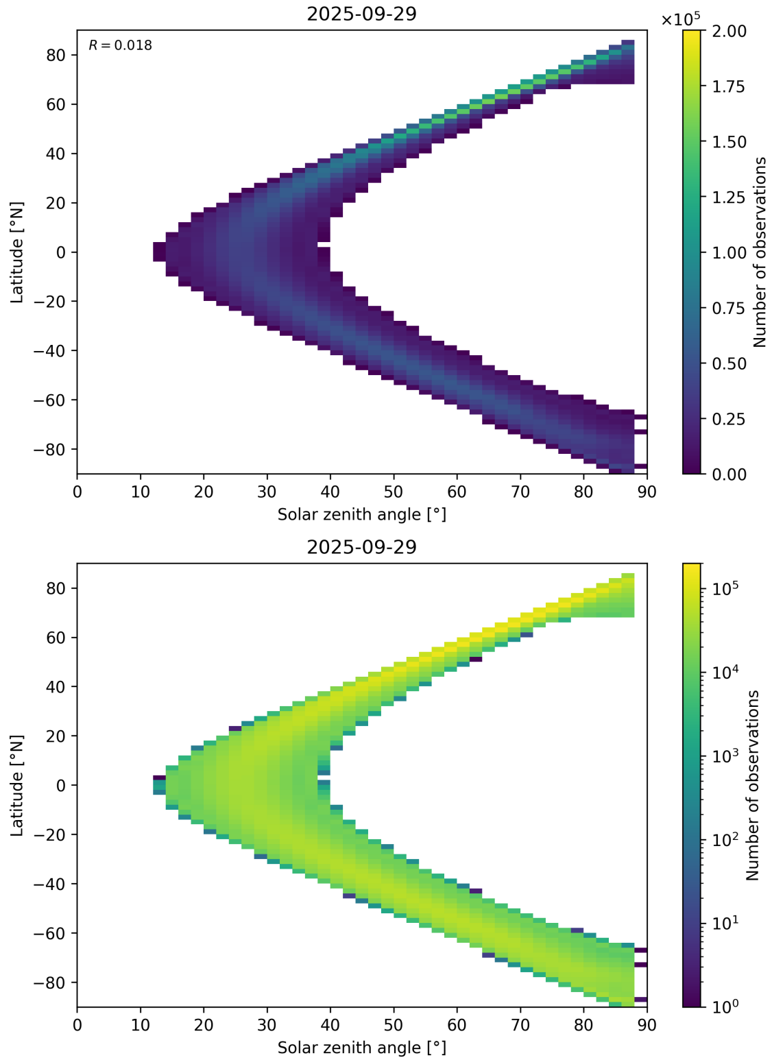
Figure 113: Scatter density plot of “Solar zenith angle” against “Latitude” for 2025-09-28 to 2025-09-30.
