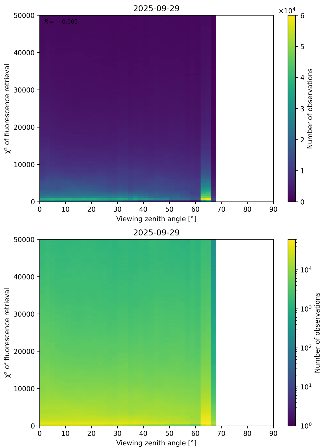
Figure 119: Scatter density plot of “Viewing zenith angle” against “ \chi^2 of fluorescence retrieval” for 2025-09-28 to 2025-09-30.
