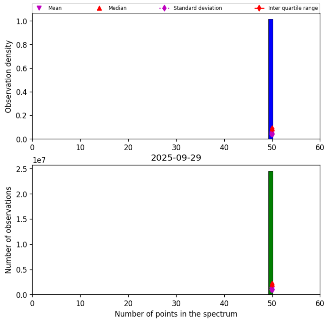
Figure 44: Histogram of “Number of points in the spectrum” for 2025-09-28 to 2025-09-30
