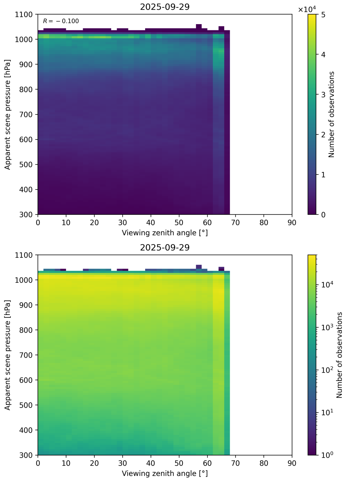
Figure 118: Scatter density plot of “Viewing zenith angle” against “Apparent scene pressure” for 2025-09-28 to 2025-09-30.
