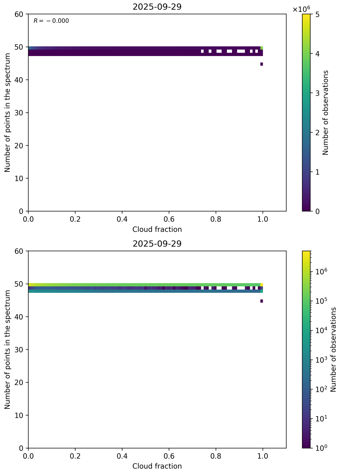
Figure 74: Scatter density plot of “Cloud fraction” against “Number of points in the spectrum” for 2025-09-28 to 2025-09-30.
