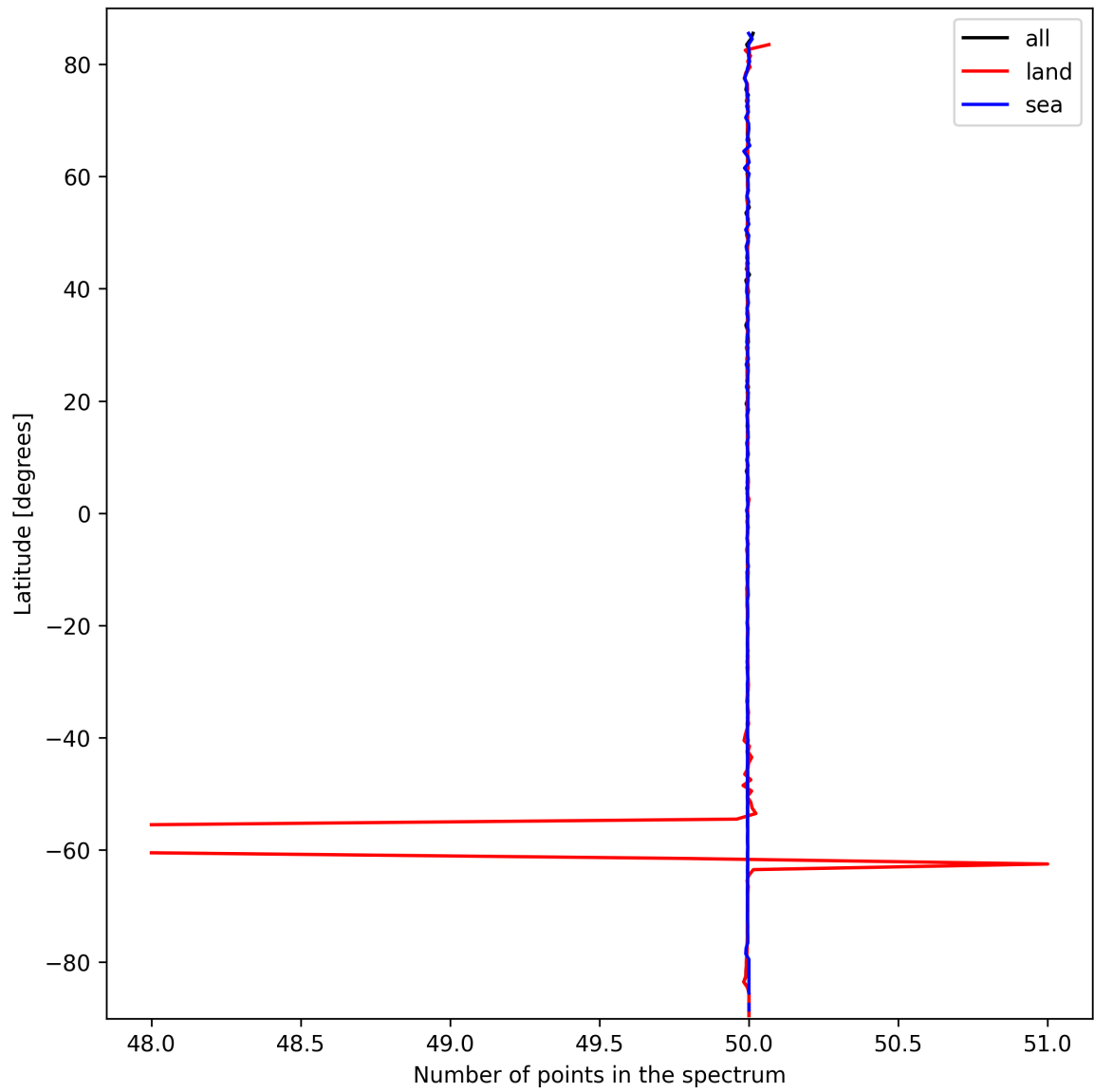
Figure 27: Zonal average of “Number of points in the spectrum” for 2025-09-28 to 2025-09-30.
