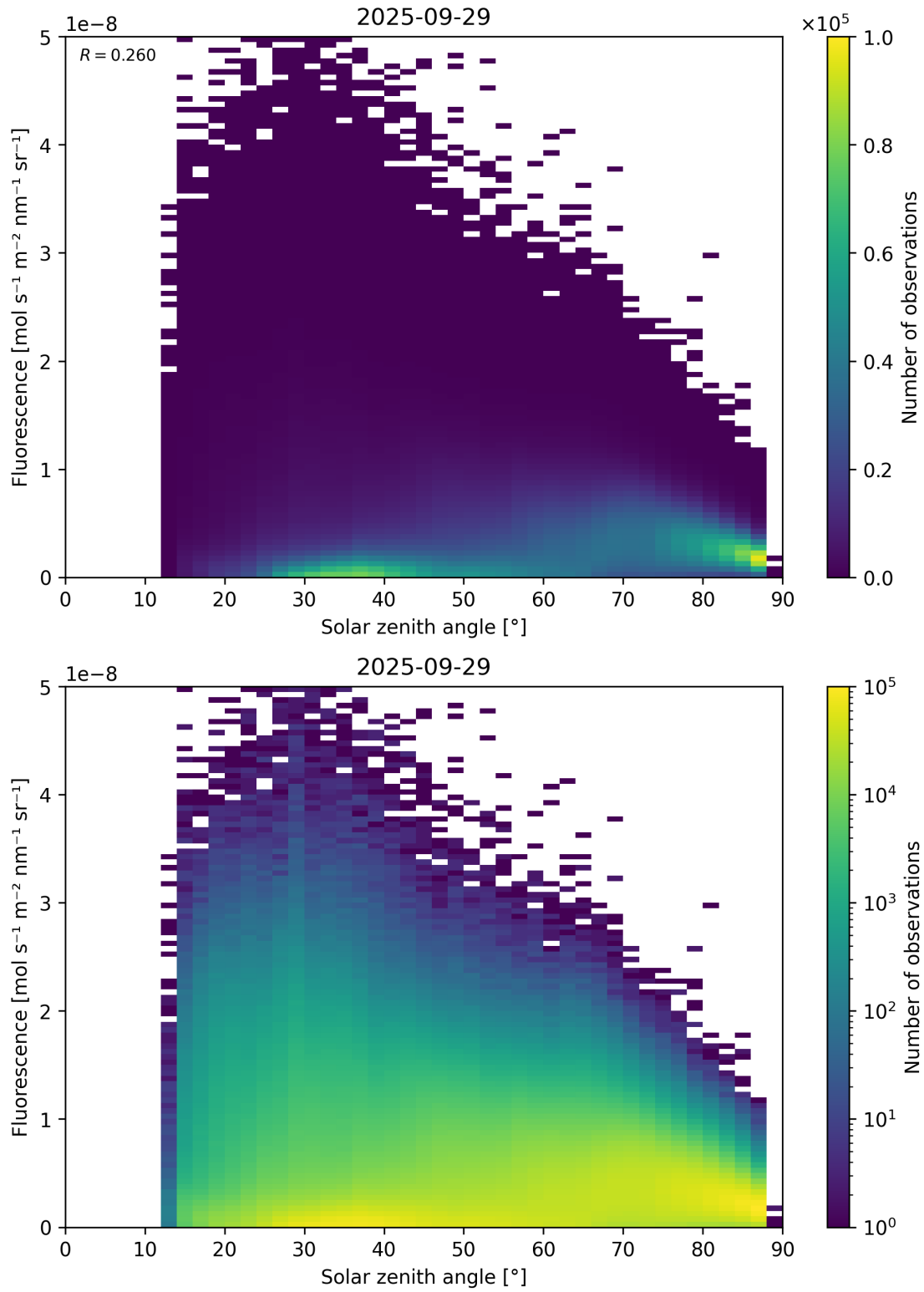
Figure 112: Scatter density plot of “Solar zenith angle” against “Fluorescence” for 2025-09-28 to 2025-09-30.
