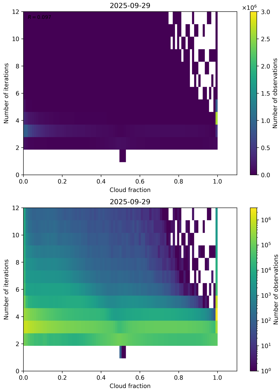
Figure 73: Scatter density plot of “Cloud fraction” against “Number of iterations” for 2025-09-28 to 2025-09-30.
