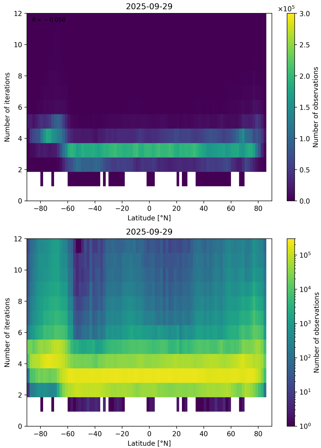
Figure 93: Scatter density plot of “Latitude” against “Number of iterations” for 2025-09-28 to 2025-09-30.
