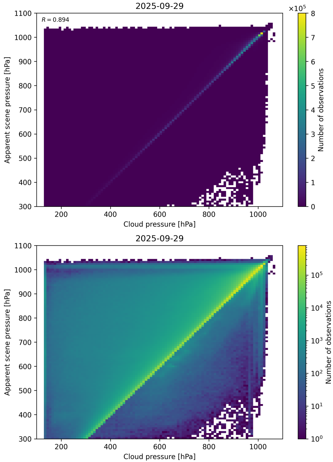
Figure 77: Scatter density plot of “Cloud pressure” against “Apparent scene pressure” for 2025-09-28 to 2025-09-30.
