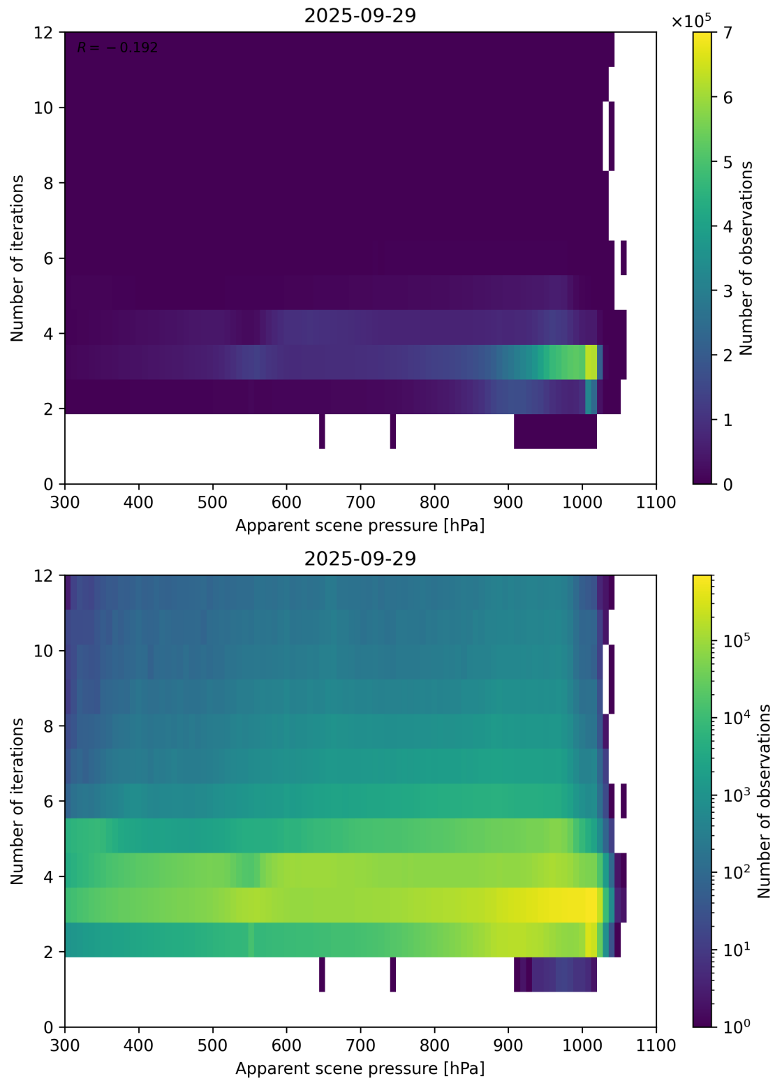
Figure 65: Scatter density plot of “Apparent scene pressure” against “Number of iterations” for 2025-09-28 to 2025-09-30.
