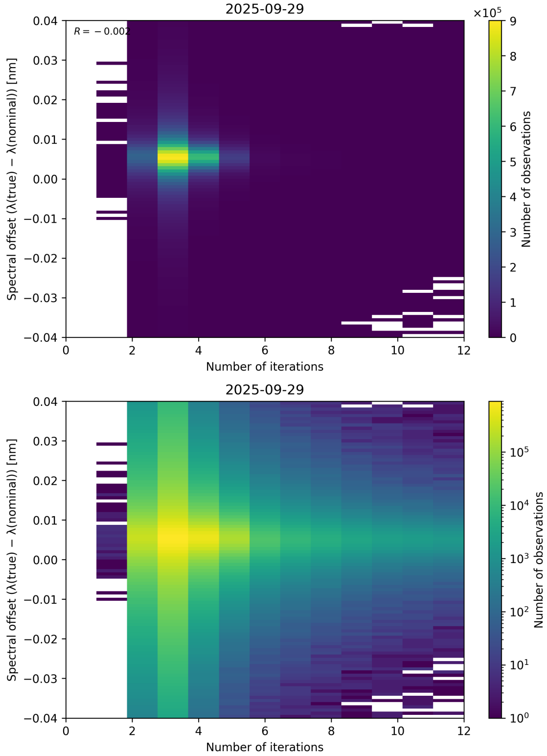
Figure 100: Scatter density plot of “Number of iterations” against “Spectral offset ( \lambda_{\text{true}} - \lambda_{\text{nominal}} )” for 2025-09-28 to 2025-09-30.
