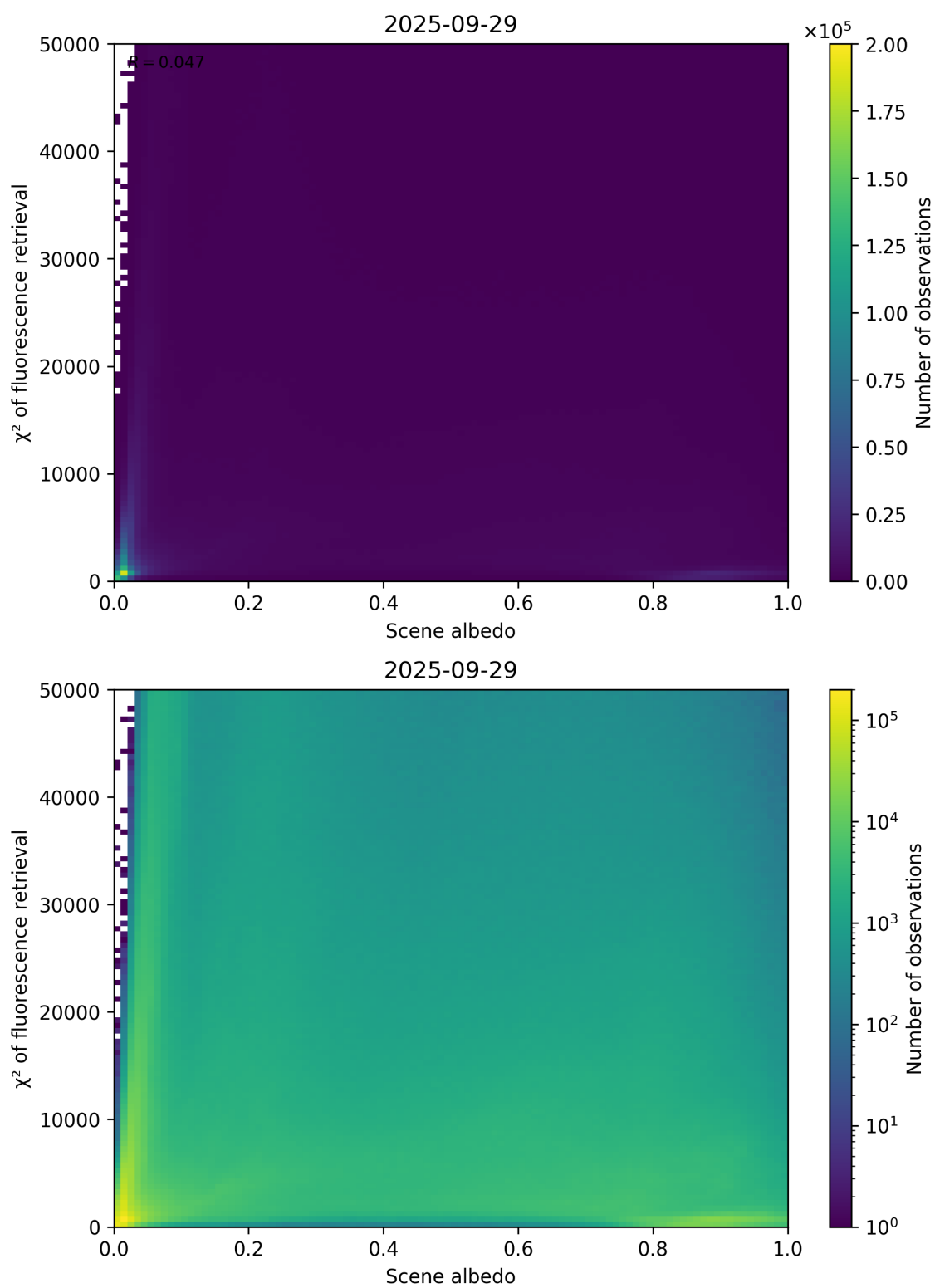
Figure 103: Scatter density plot of “Scene albedo” against “ \chi^2 of fluorescence retrieval” for 2025-09-28 to 2025-09-30.
