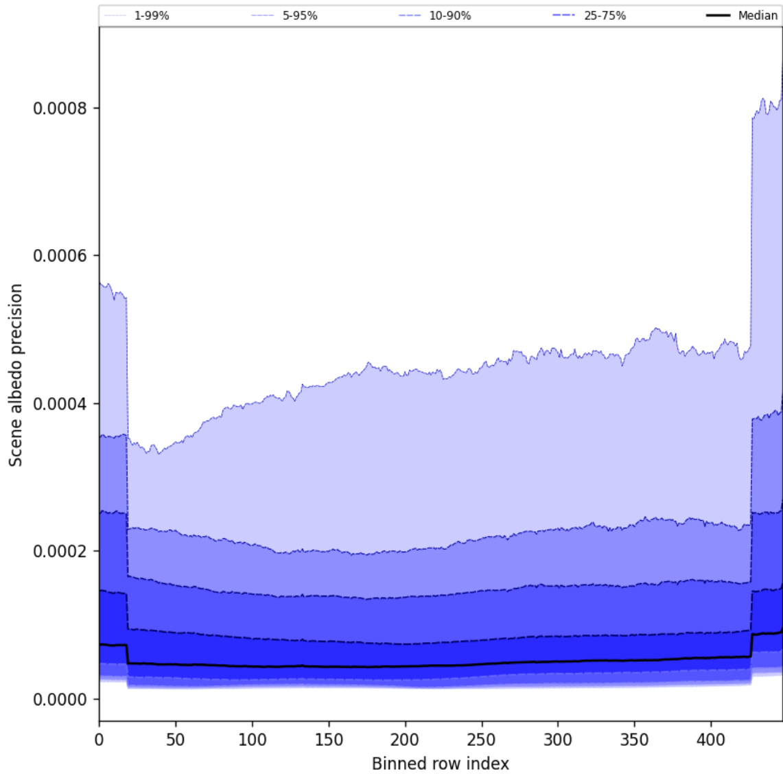
Figure 52: Along track statistics of “Scene albedo precision” for 2025-09-28 to 2025-09-30
