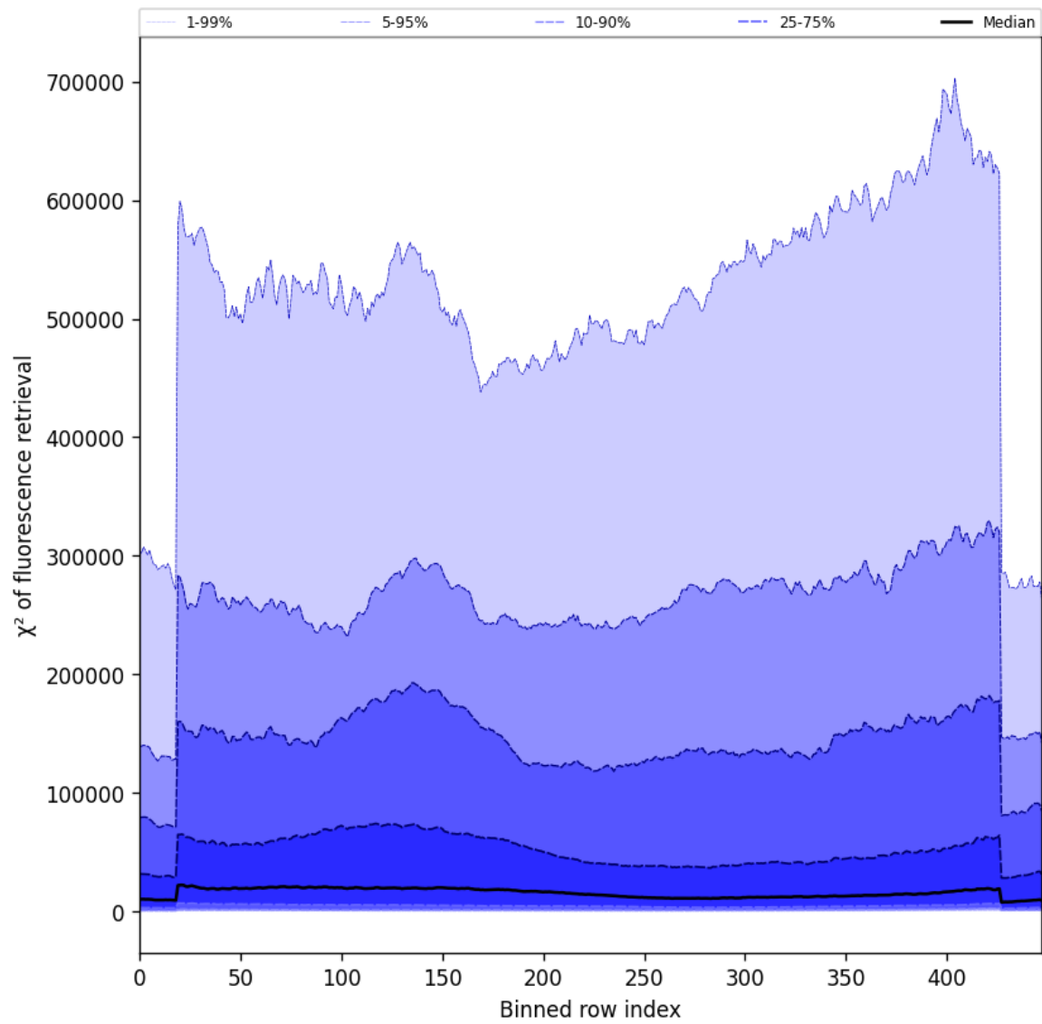
Figure 59: Along track statistics of “ \chi^2 of fluorescence retrieval” for 2025-09-28 to 2025-09-30
