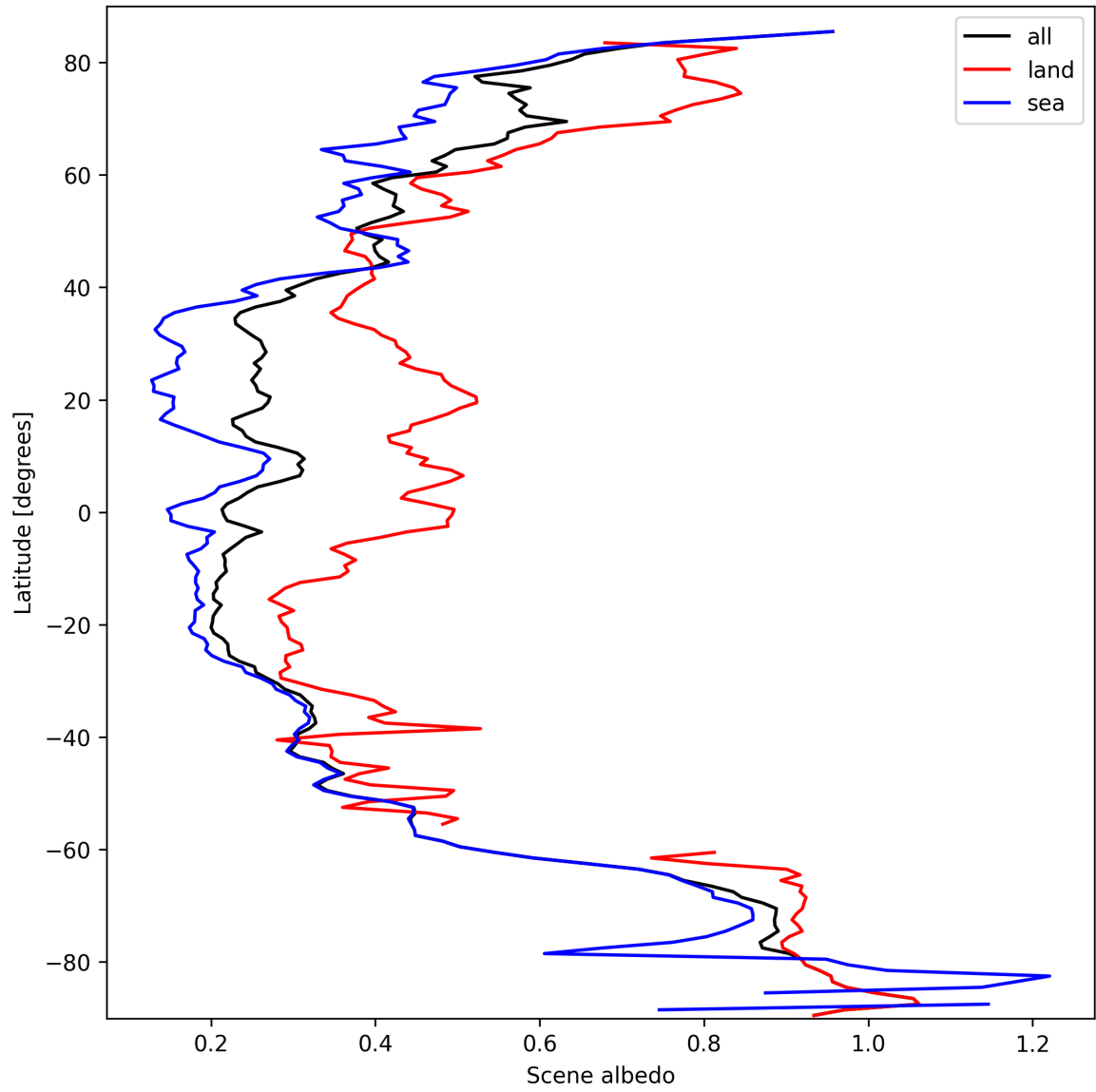
Figure 17: Zonal average of “Scene albedo” for 2025-09-28 to 2025-09-30.
