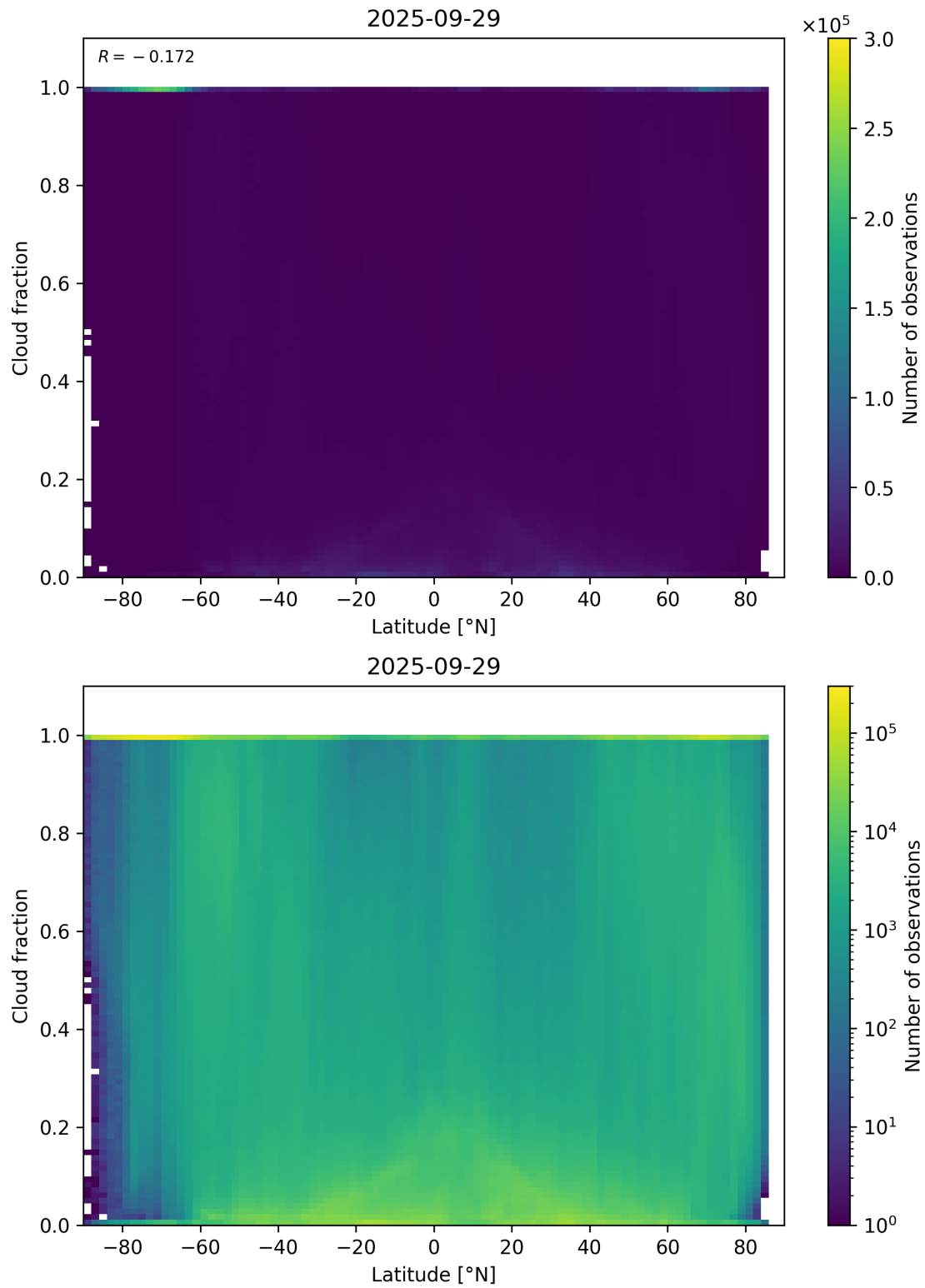
Figure 90: Scatter density plot of “Latitude” against “Cloud fraction” for 2025-09-28 to 2025-09-30.
