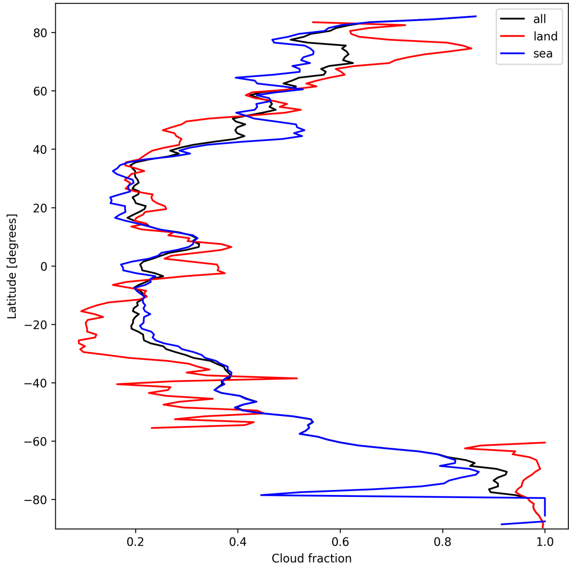
Figure 15: Zonal average of “Cloud fraction” for 2025-09-28 to 2025-09-30.
