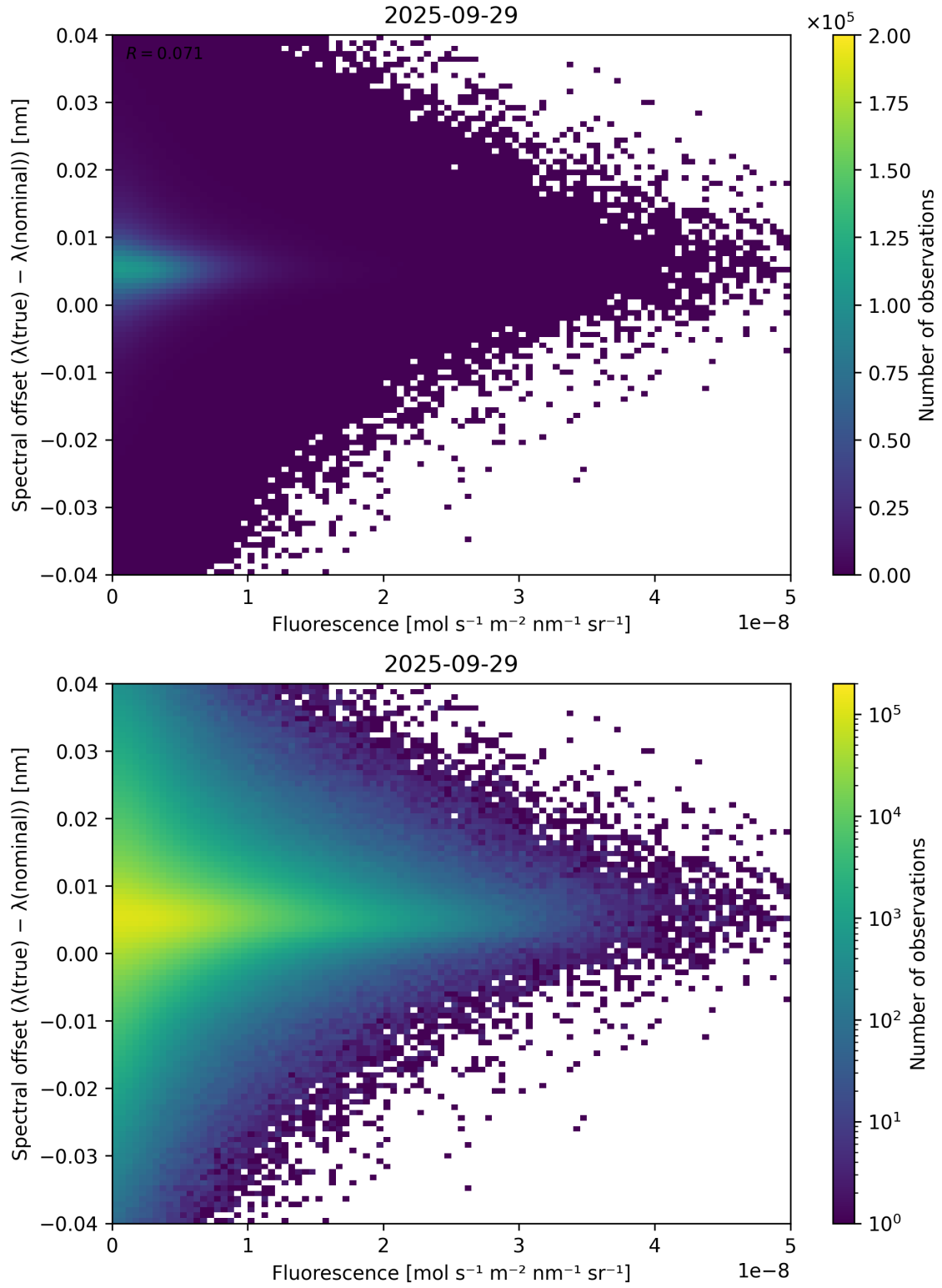
Figure 87: Scatter density plot of “Fluorescence” against “Spectral offset ( \lambda_{\text{true}} - \lambda_{\text{nominal}} )” for 2025-09-28 to 2025-09-30.
