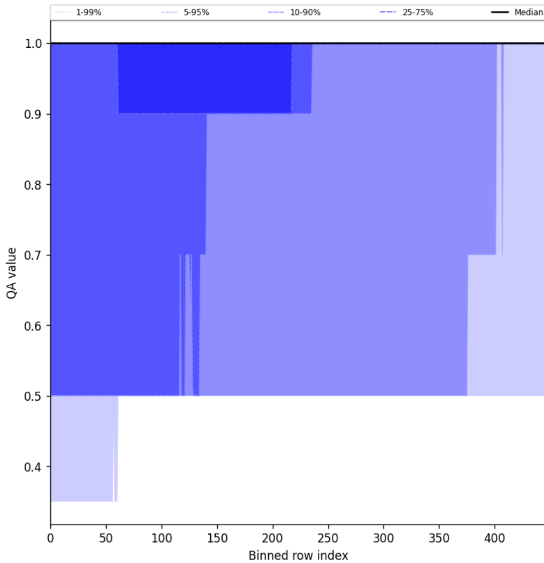
Figure 46: Along track statistics of “QA value” for 2025-09-28 to 2025-09-30
