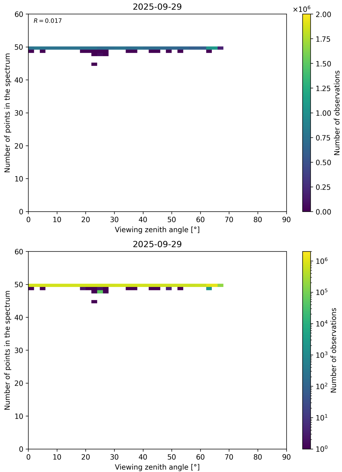
Figure 125: Scatter density plot of “Viewing zenith angle” against “Number of points in the spectrum” for 2025-09-28 to 2025-09-30.
