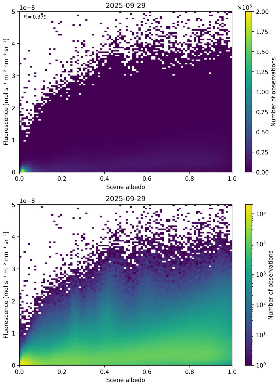
Figure 104: Scatter density plot of “Scene albedo” against “Fluorescence” for 2025-09-28 to 2025-09-30.
