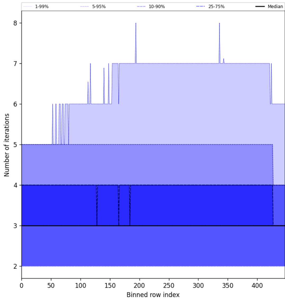
Figure 56: Along track statistics of “Number of iterations” for 2025-09-28 to 2025-09-30
