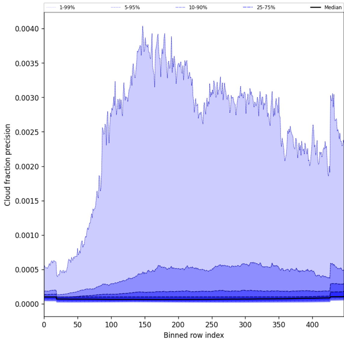
Figure 50: Along track statistics of “Cloud fraction precision” for 2025-09-28 to 2025-09-30
