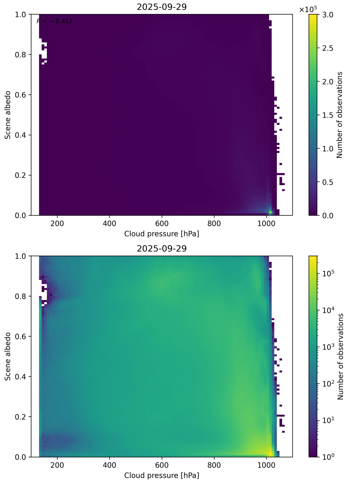
Figure 83: Scatter density plot of “Cloud pressure” against “Scene albedo” for 2025-09-28 to 2025-09-30.
