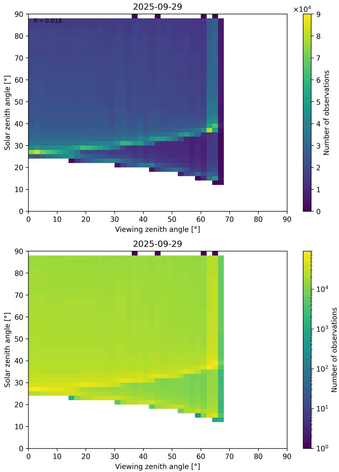
Figure 127: Scatter density plot of “Viewing zenith angle” against “Solar zenith angle” for 2025-09-28 to 2025-09-30.
