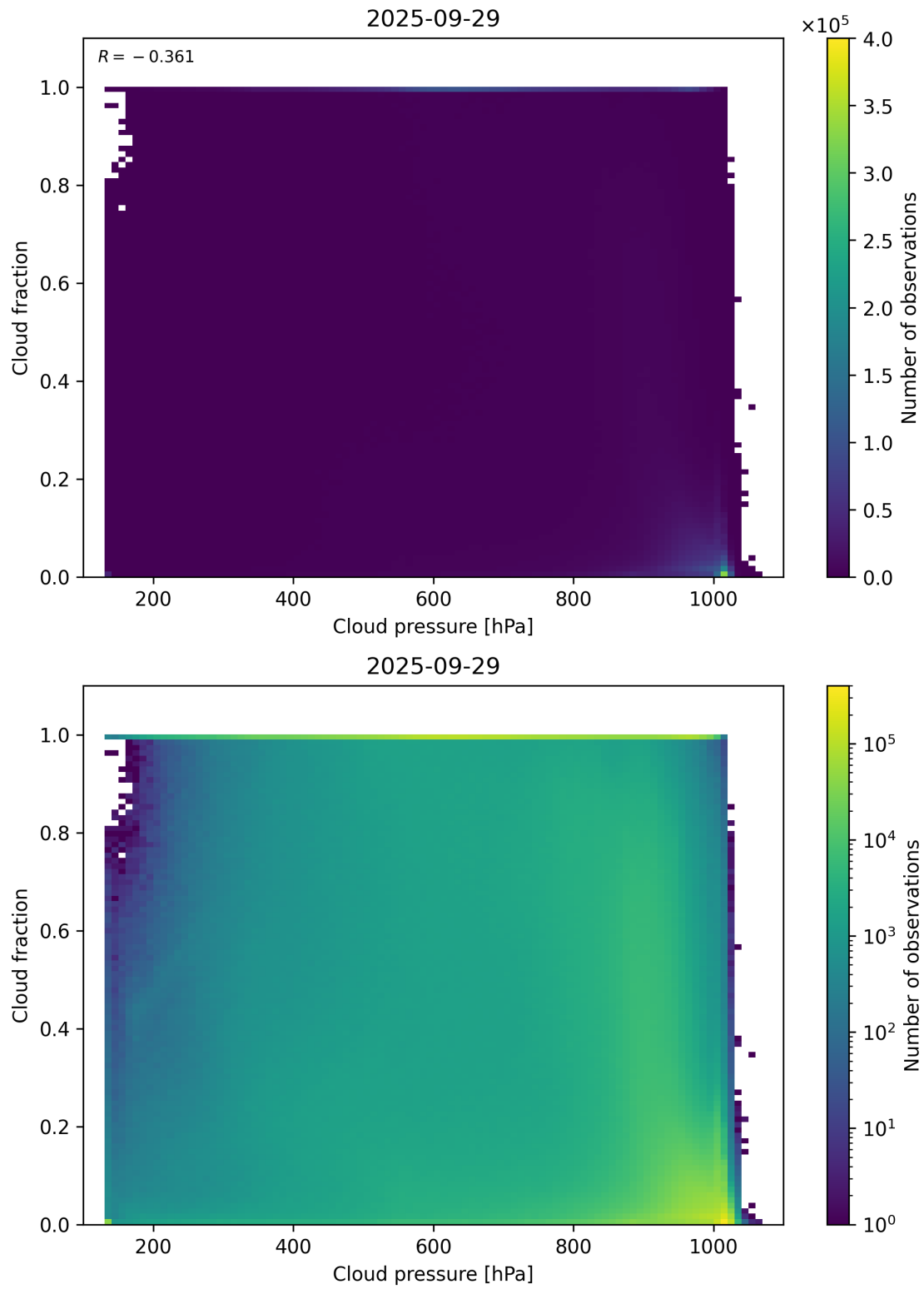
Figure 79: Scatter density plot of “Cloud pressure” against “Cloud fraction” for 2025-09-28 to 2025-09-30.
