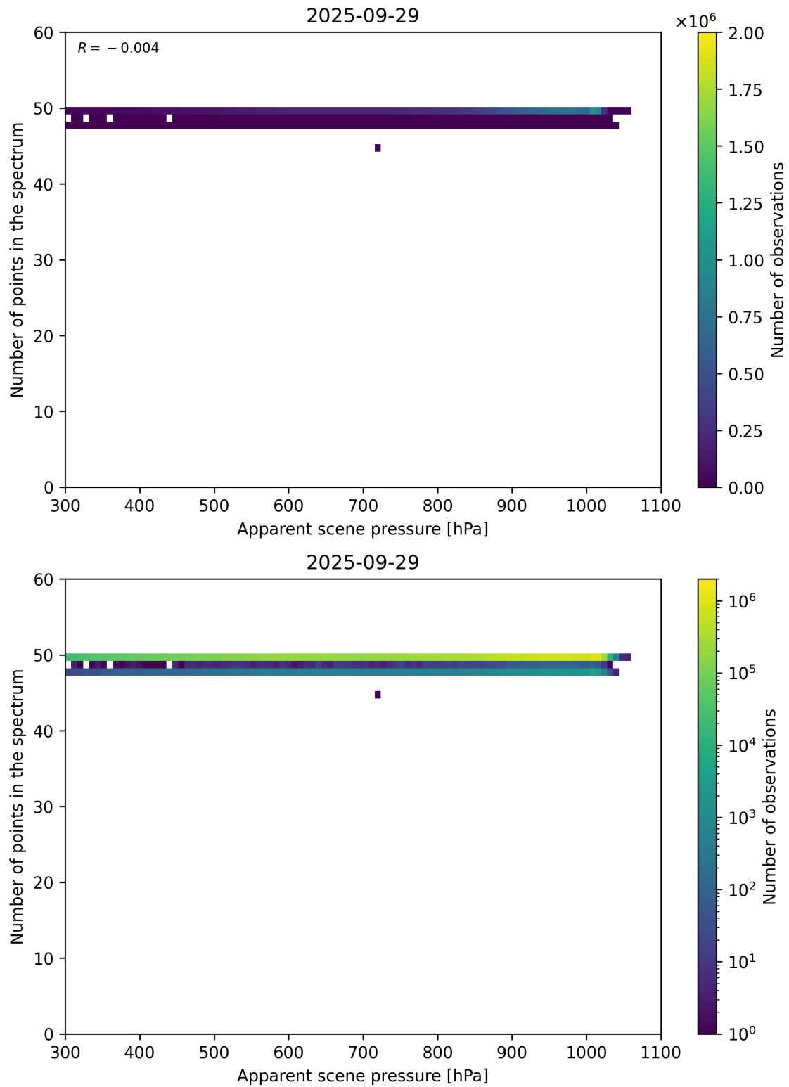
Figure 66: Scatter density plot of “Apparent scene pressure” against “Number of points in the spectrum” for 2025-09-28 to 2025-09-30.
