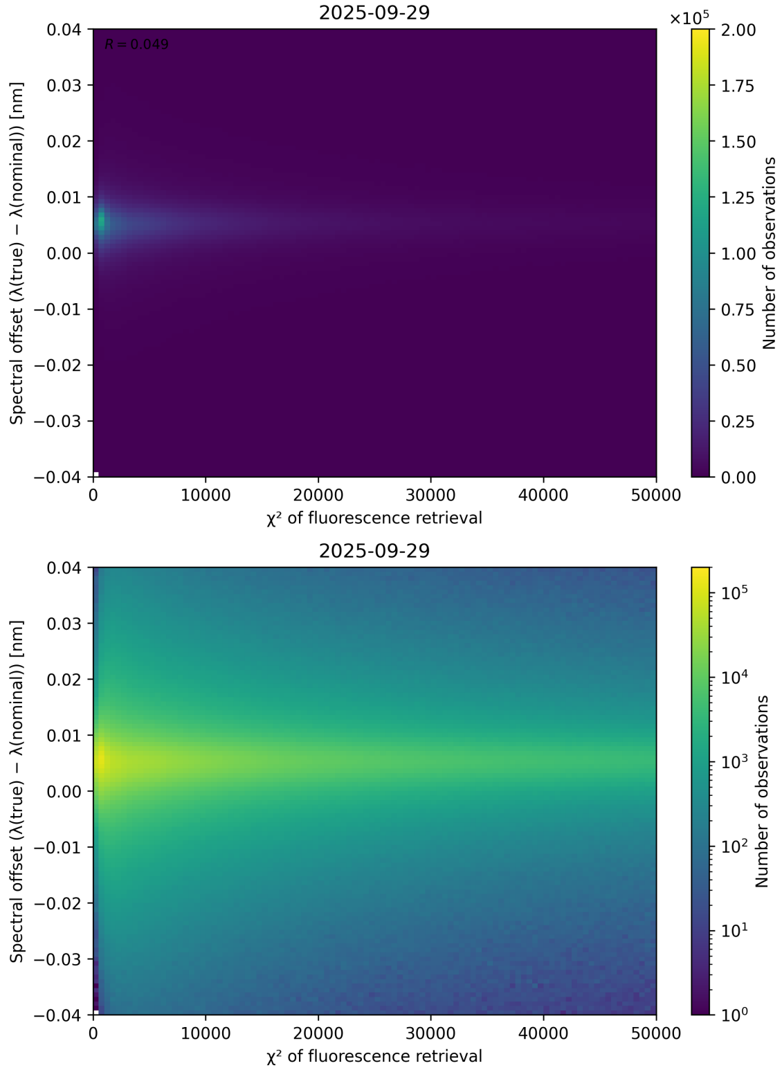
Figure 69: Scatter density plot of “ \chi^2 of fluorescence retrieval” against “Spectral offset ( \lambda_{\text{true}} - \lambda_{\text{nominal}} )” for 2025-09-28 to 2025-09-30.
