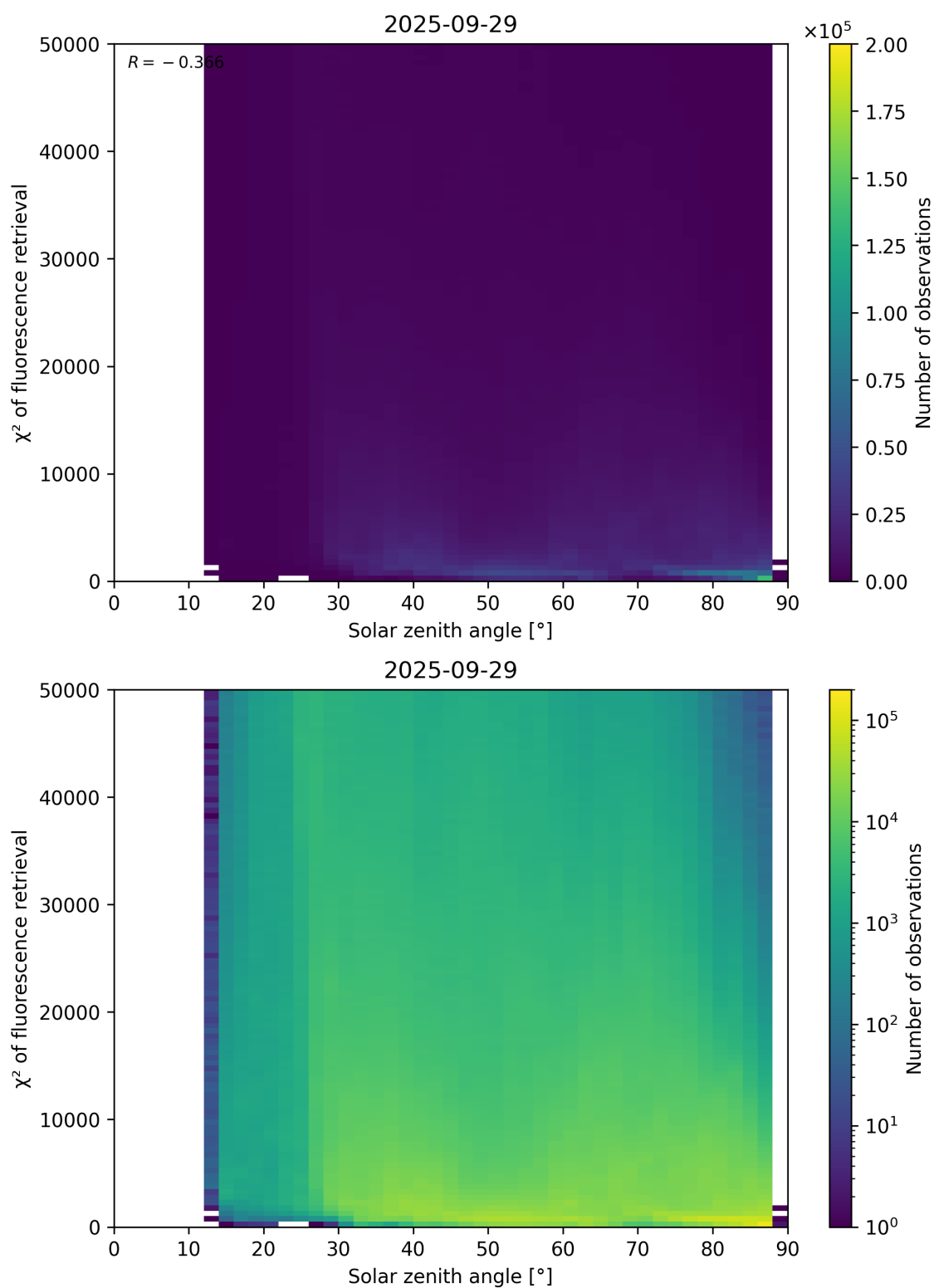
Figure 109: Scatter density plot of “Solar zenith angle” against “ \chi^2 of fluorescence retrieval” for 2025-09-28 to 2025-09-30.
