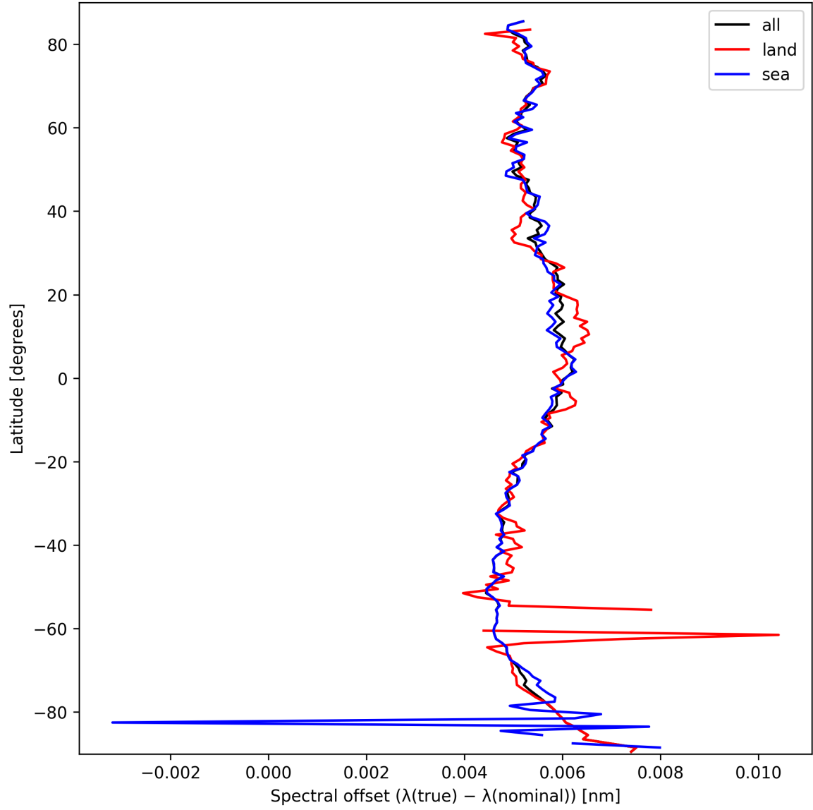
Figure 28: Zonal average of “Spectral offset ( \lambda_{\text{true}} - \lambda_{\text{nominal}} )” for 2025-09-28 to 2025-09-30.
