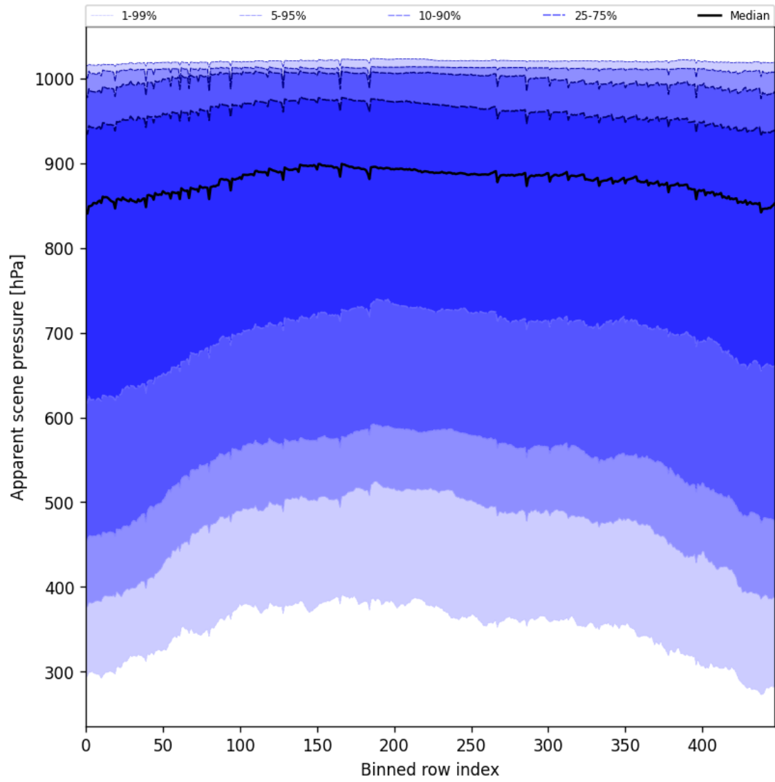
Figure 53: Along track statistics of “Apparent scene pressure” for 2025-09-28 to 2025-09-30
