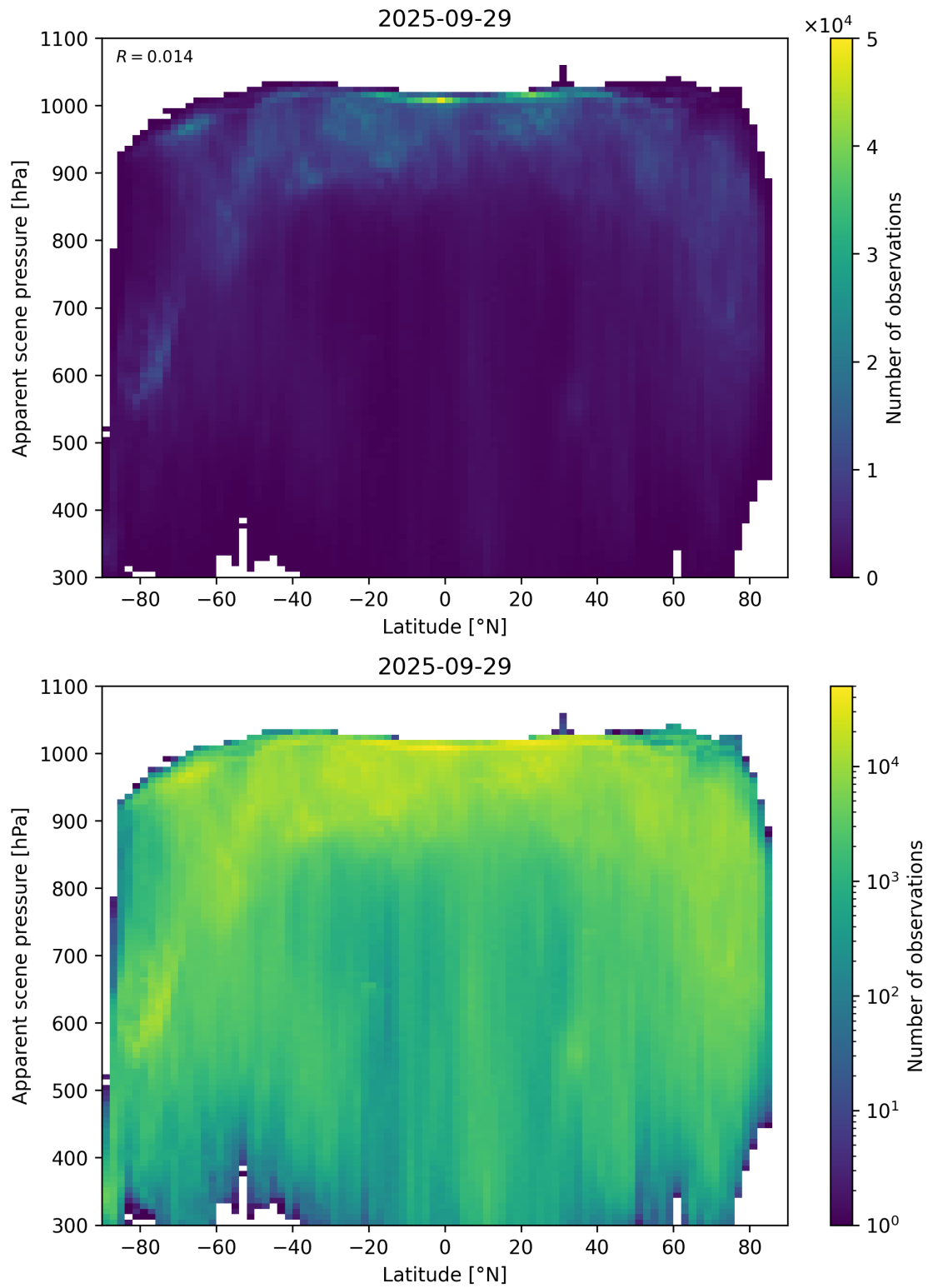
Figure 88: Scatter density plot of “Latitude” against “Apparent scene pressure” for 2025-09-28 to 2025-09-30.
