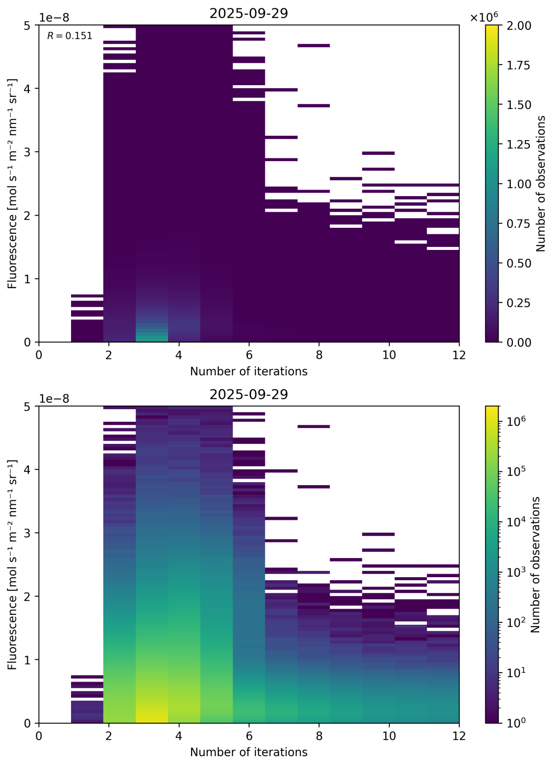
Figure 98: Scatter density plot of “Number of iterations” against “Fluorescence” for 2025-09-28 to 2025-09-30.
