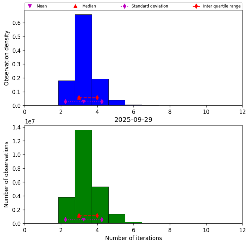
Figure 39: Histogram of “Number of iterations” for 2025-09-28 to 2025-09-30
