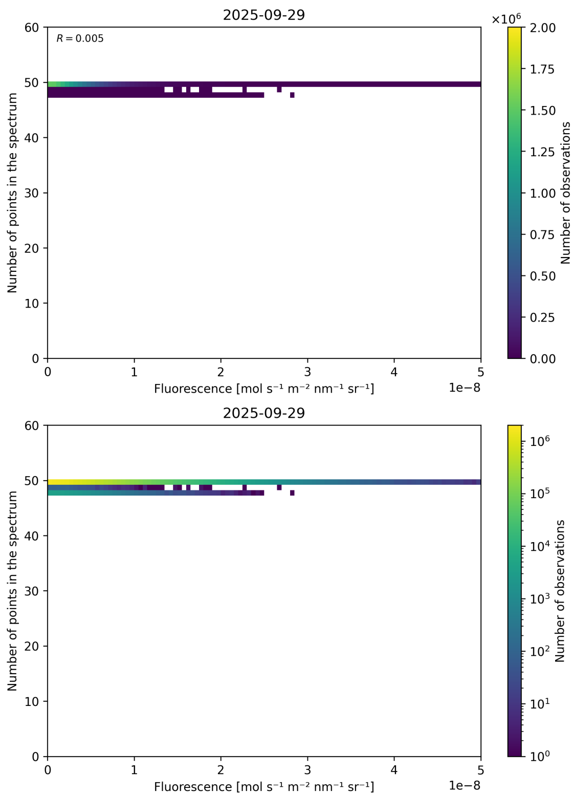
Figure 86: Scatter density plot of “Fluorescence” against “Number of points in the spectrum” for 2025-09-28 to 2025-09-30.
