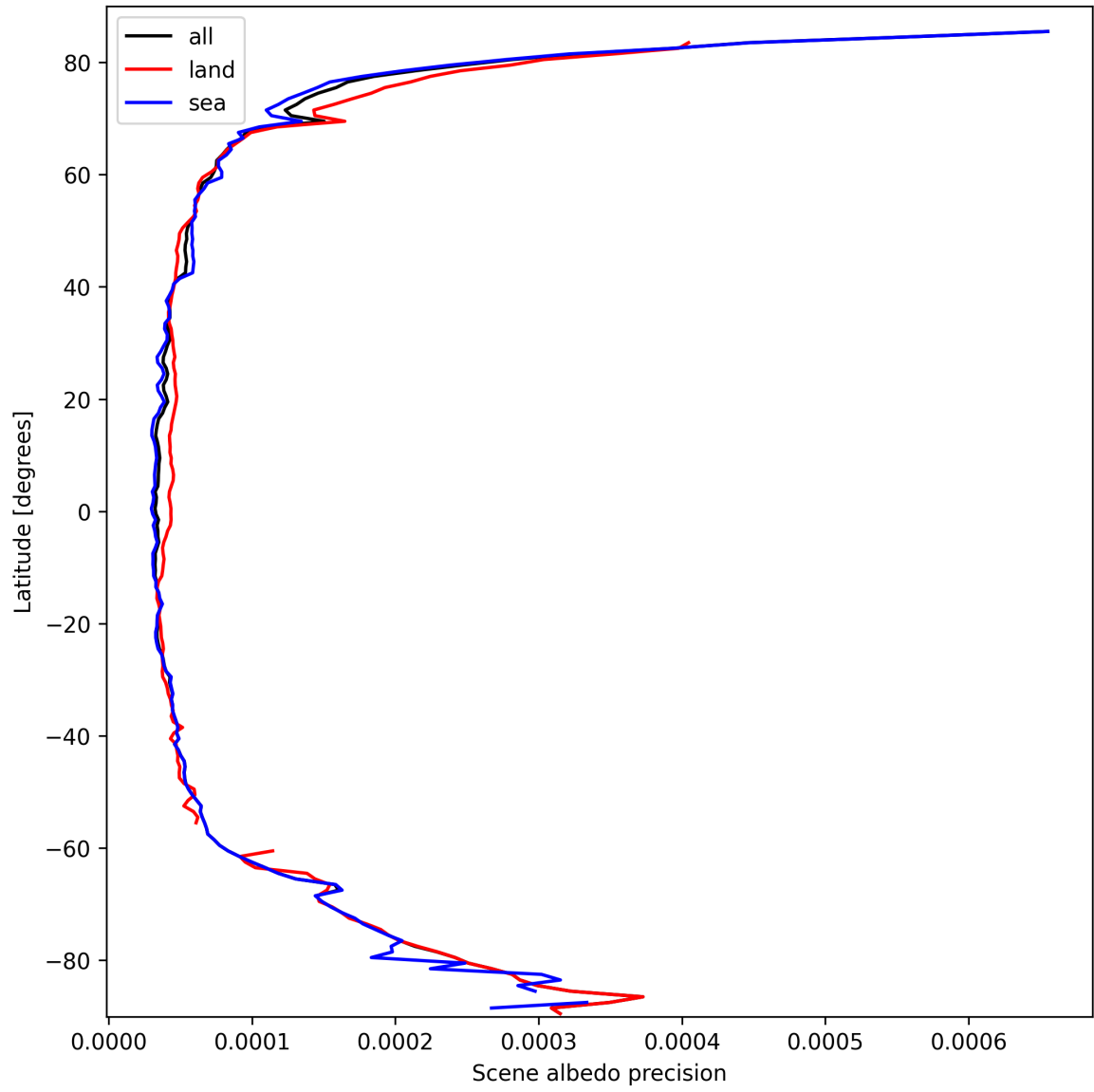
Figure 18: Zonal average of “Scene albedo precision” for 2025-09-28 to 2025-09-30.
