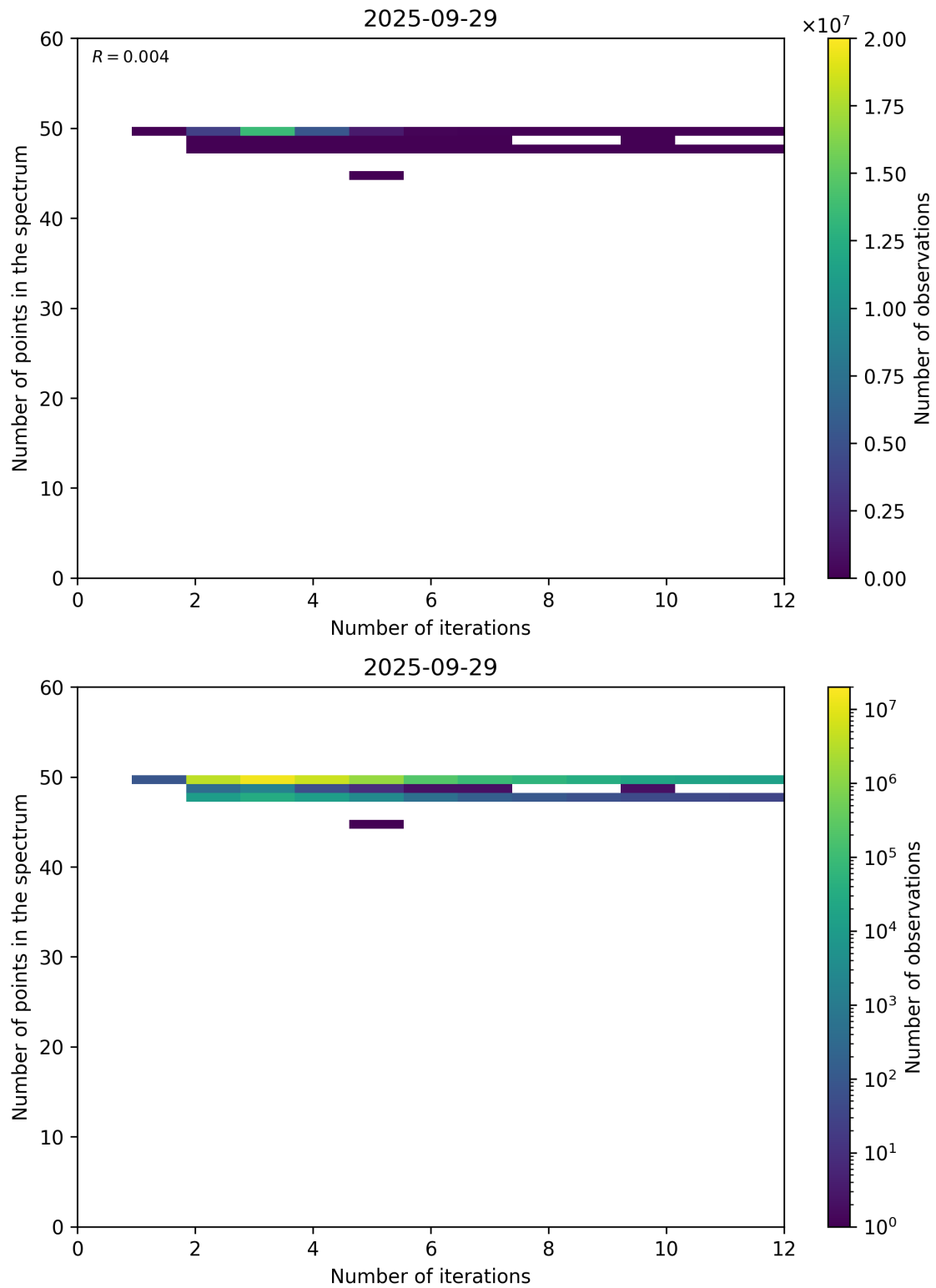
Figure 99: Scatter density plot of “Number of iterations” against “Number of points in the spectrum” for 2025-09-28 to 2025-09-30.
