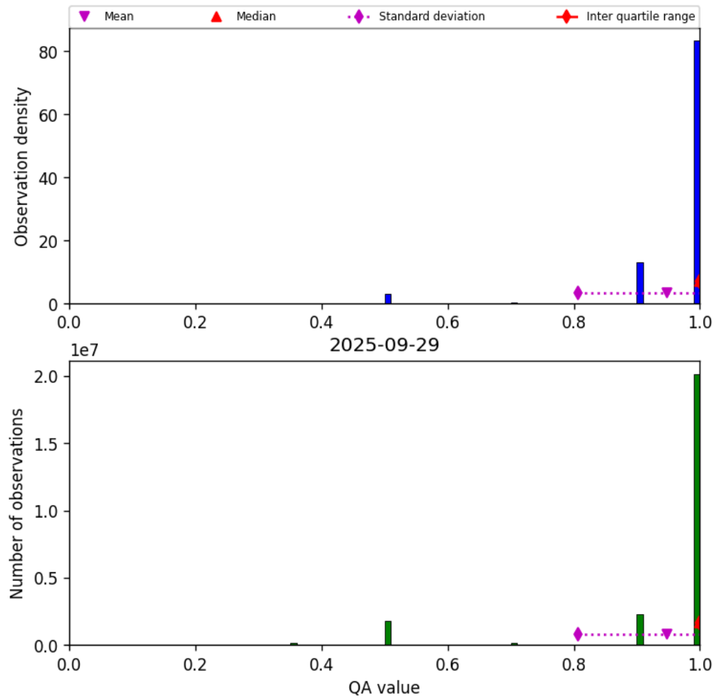
Figure 29: Histogram of “QA value” for 2025-09-28 to 2025-09-30
