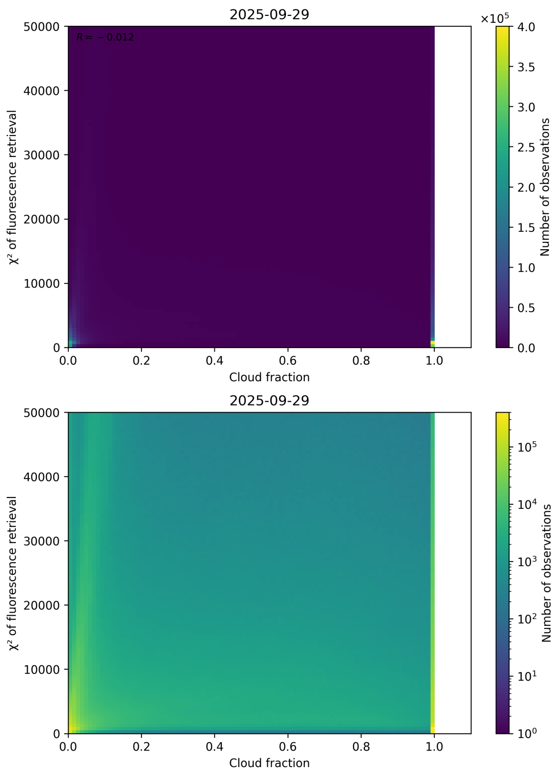
Figure 71: Scatter density plot of “Cloud fraction” against “ \chi^2 of fluorescence retrieval” for 2025-09-28 to 2025-09-30.
