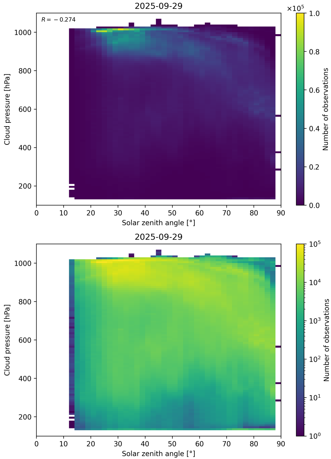
Figure 111: Scatter density plot of “Solar zenith angle” against “Cloud pressure” for 2025-09-28 to 2025-09-30.
