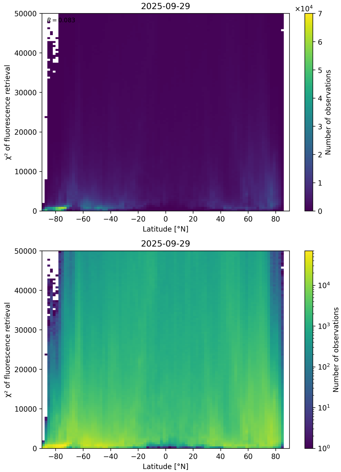
Figure 89: Scatter density plot of “Latitude” against “ \chi^2 of fluorescence retrieval” for 2025-09-28 to 2025-09-30.
