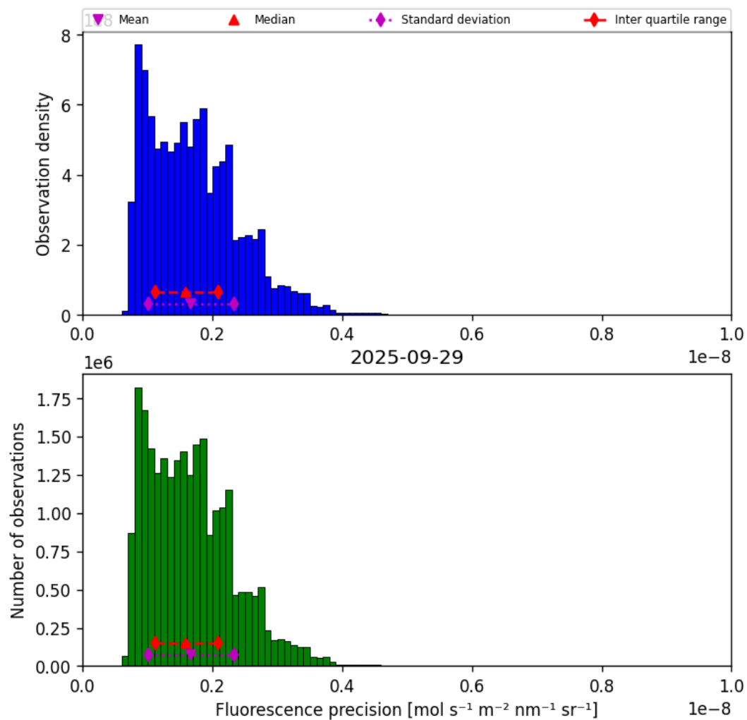
Figure 41: Histogram of “Fluorescence precision” for 2025-09-28 to 2025-09-30
