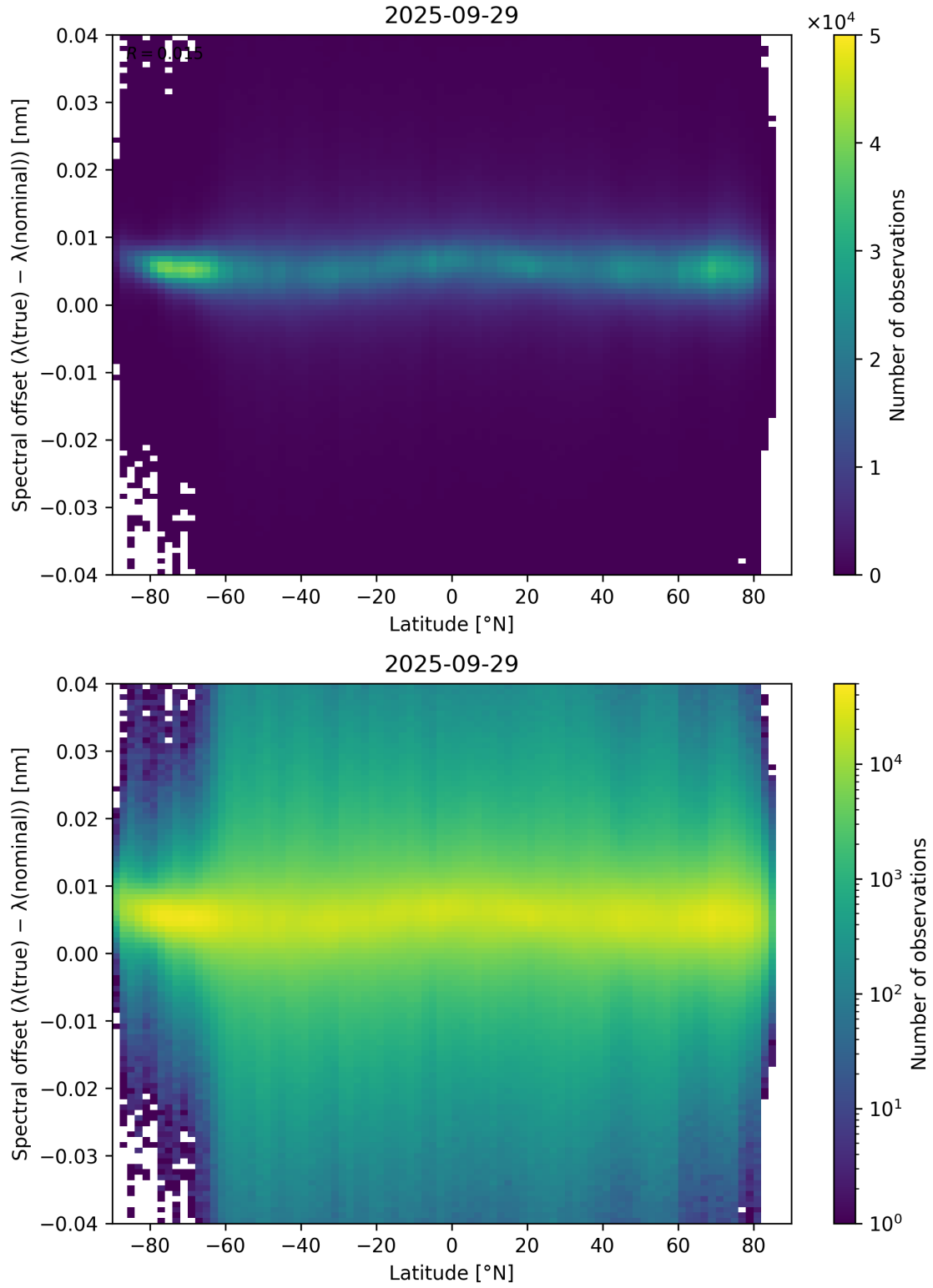
Figure 96: Scatter density plot of “Latitude” against “Spectral offset ( \lambda_{\text{true}} - \lambda_{\text{nominal}} )” for 2025-09-28 to 2025-09-30.
