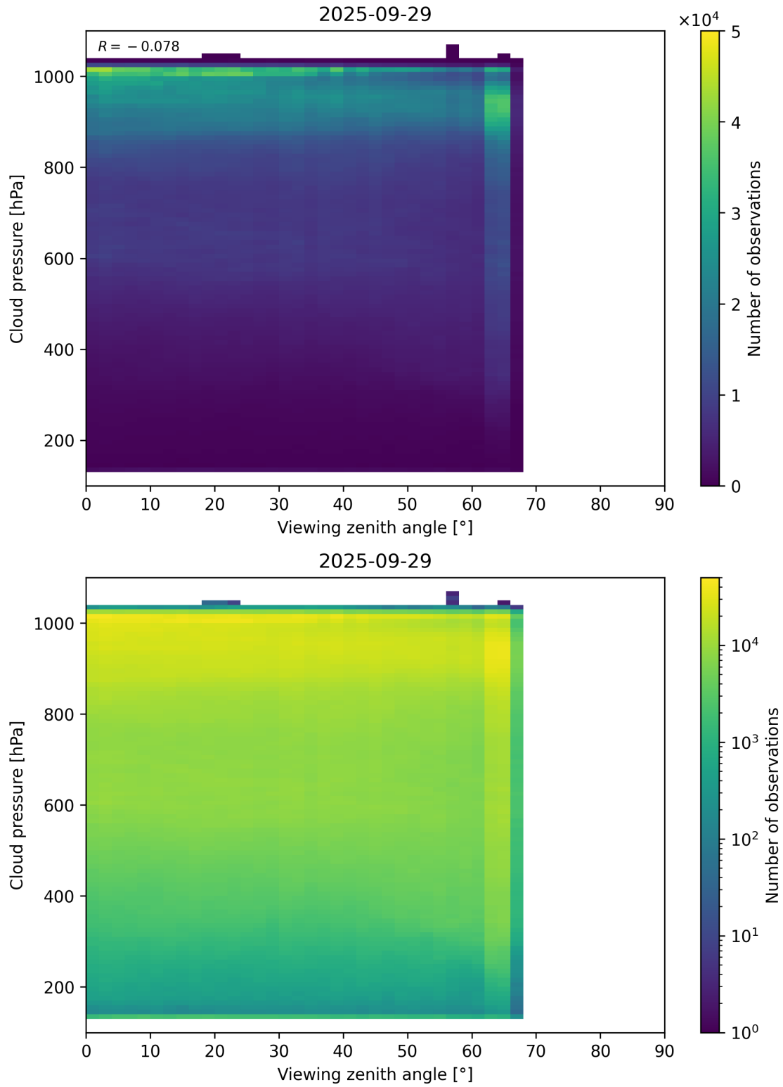
Figure 121: Scatter density plot of “Viewing zenith angle” against “Cloud pressure” for 2025-09-28 to 2025-09-30.
