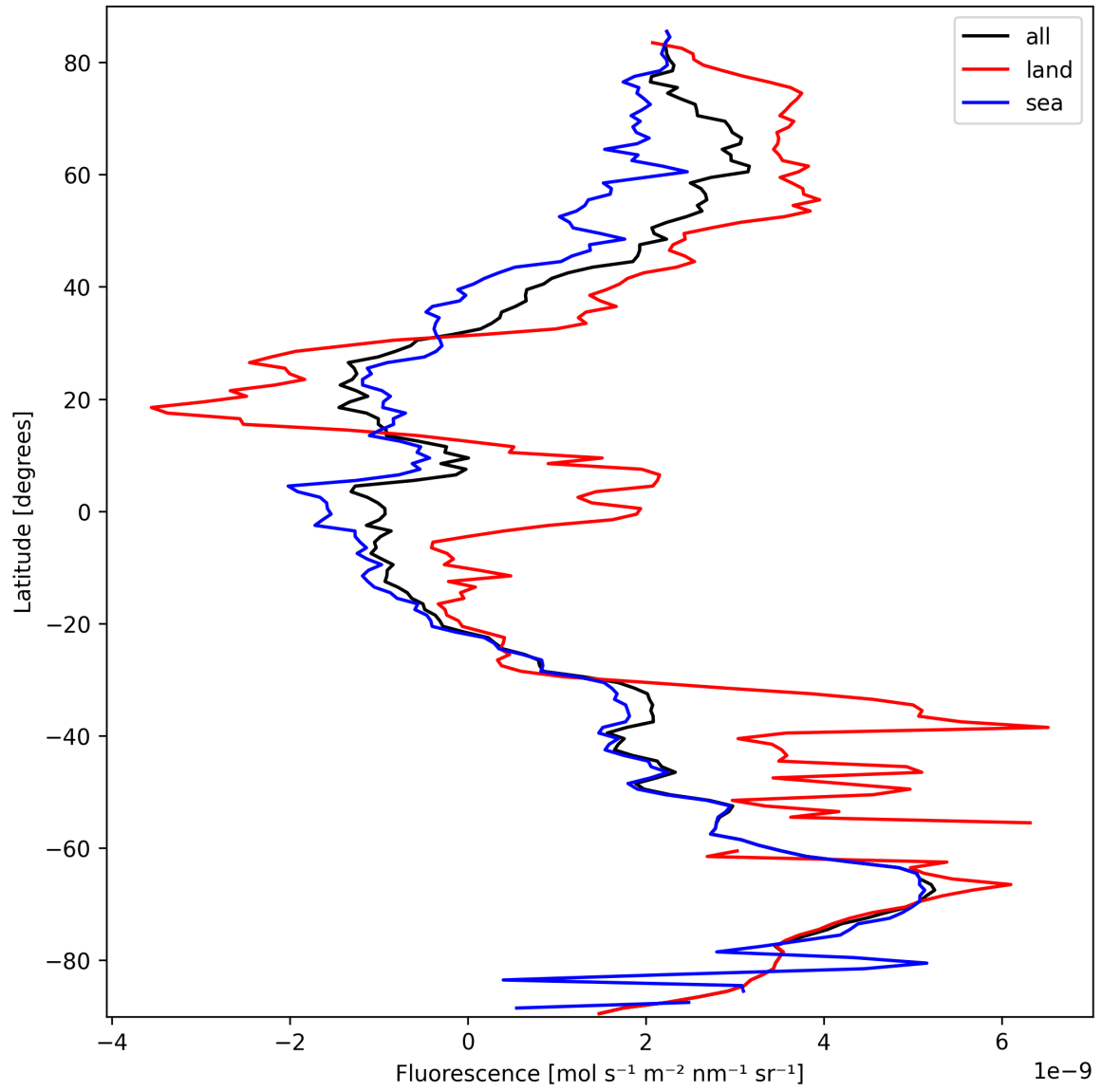
Figure 23: Zonal average of “Fluorescence” for 2025-09-28 to 2025-09-30.
