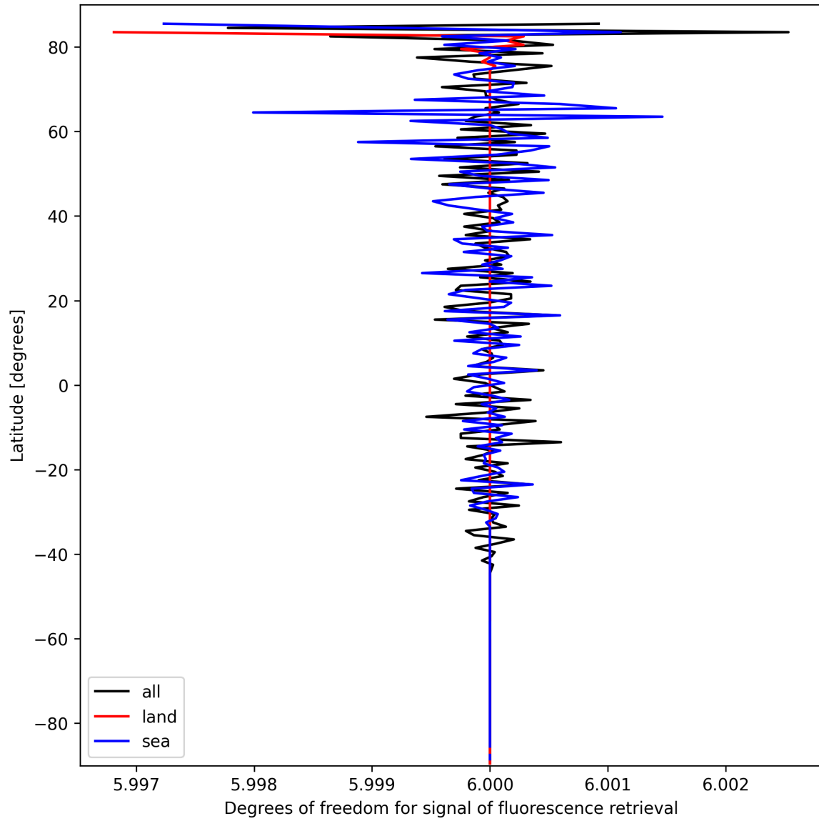
Figure 26: Zonal average of “Degrees of freedom for signal of fluorescence retrieval” for 2025-09-28 to 2025-09-30.
