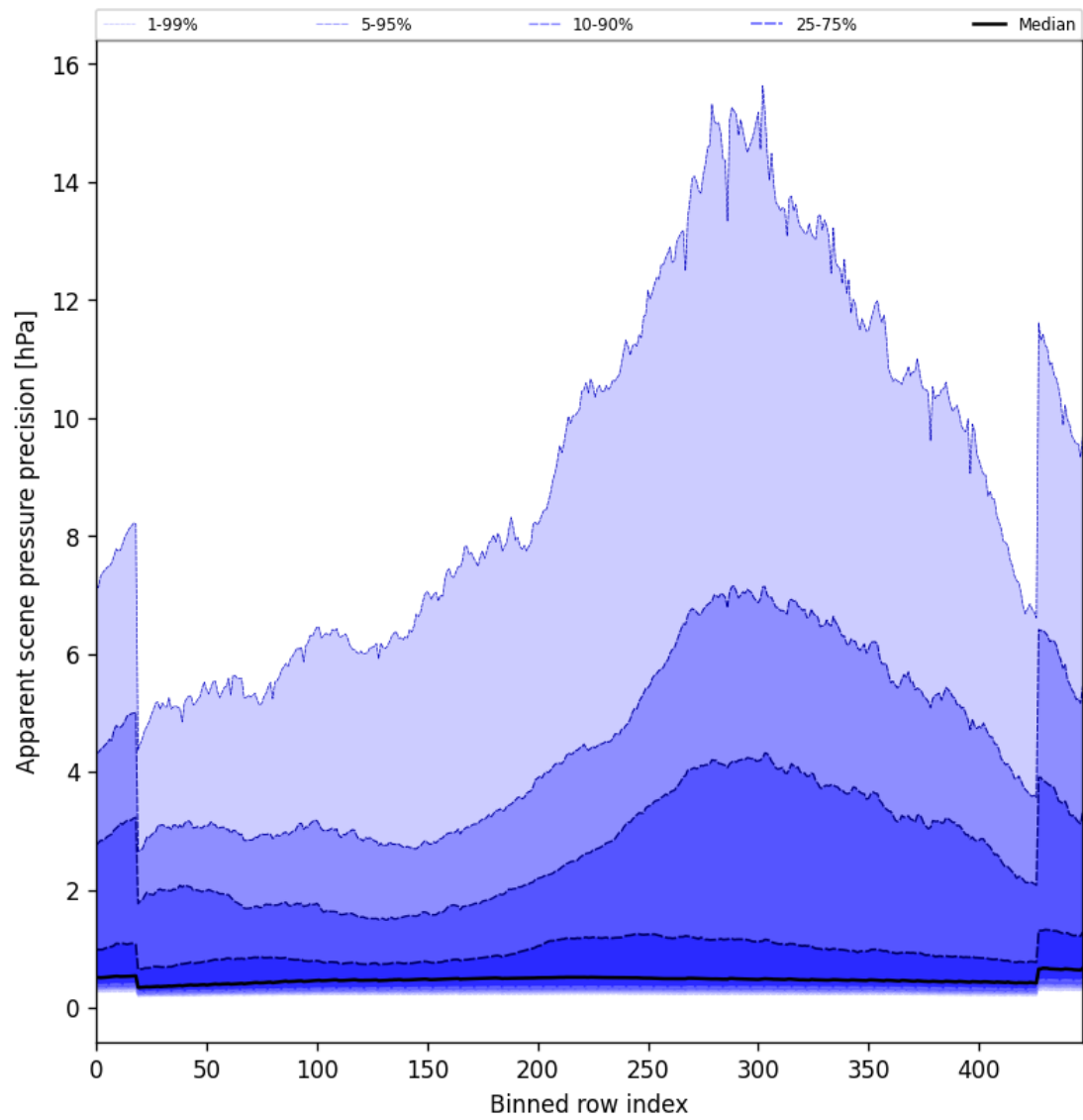
Figure 54: Along track statistics of “Apparent scene pressure precision” for 2025-09-28 to 2025-09-30
