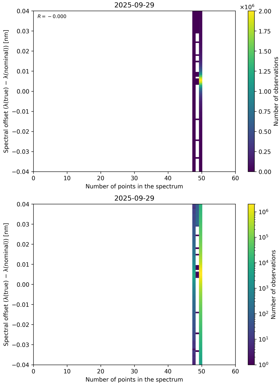
Figure 101: Scatter density plot of “Number of points in the spectrum” against “Spectral offset ( \lambda_{\text{true}} - \lambda_{\text{nominal}} )” for 2025-09-28 to 2025-09-30.
