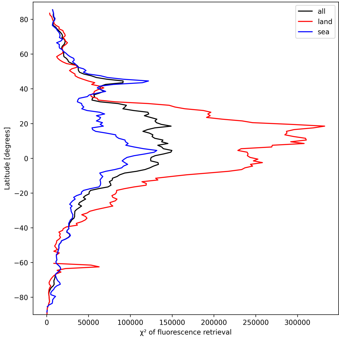
Figure 25: Zonal average of “ \chi^2 of fluorescence retrieval” for 2025-09-28 to 2025-09-30.
