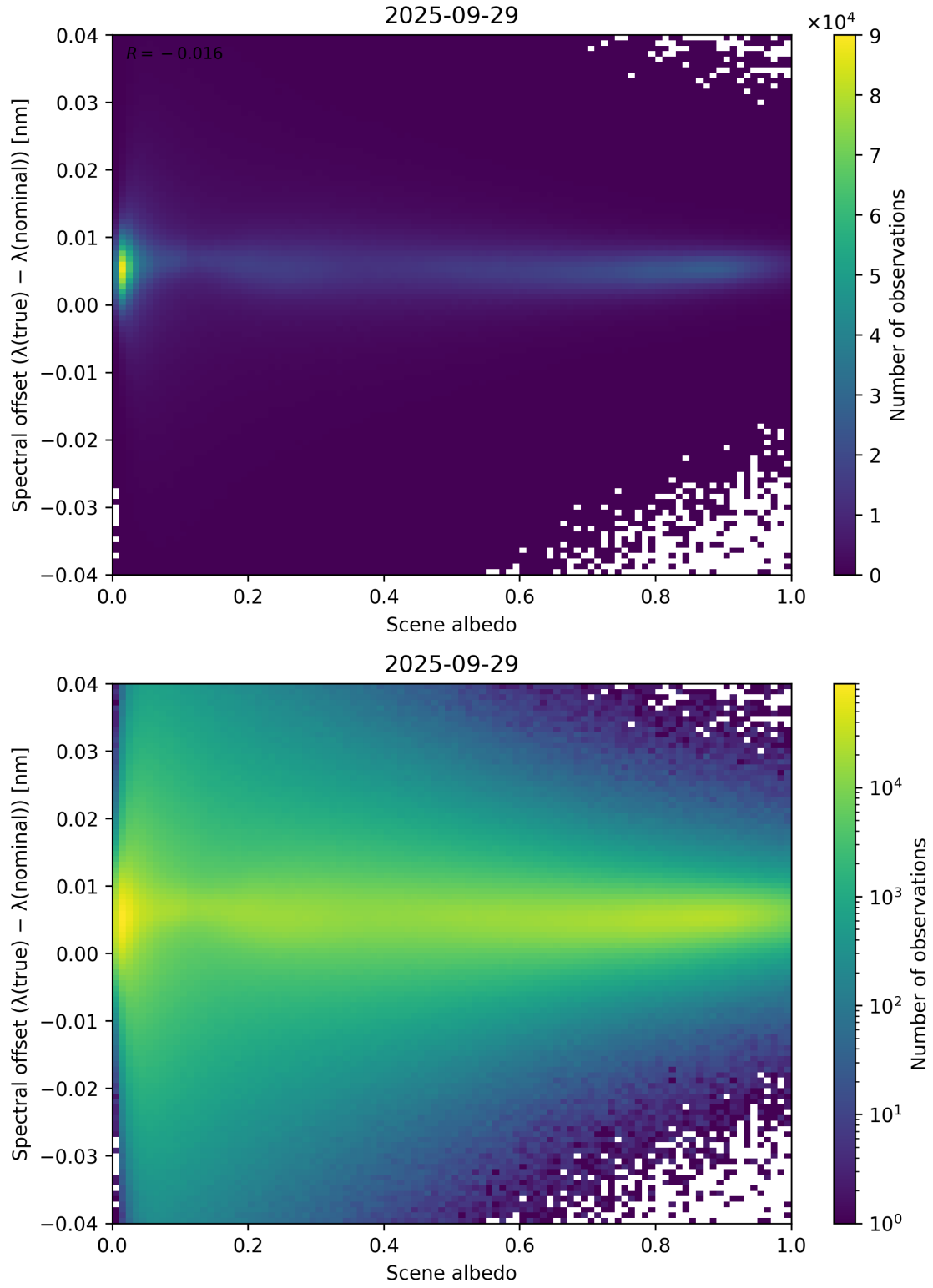
Figure 107: Scatter density plot of “Scene albedo” against “Spectral offset ( \lambda_{\text{true}} - \lambda_{\text{nominal}} )” for 2025-09-28 to 2025-09-30.
