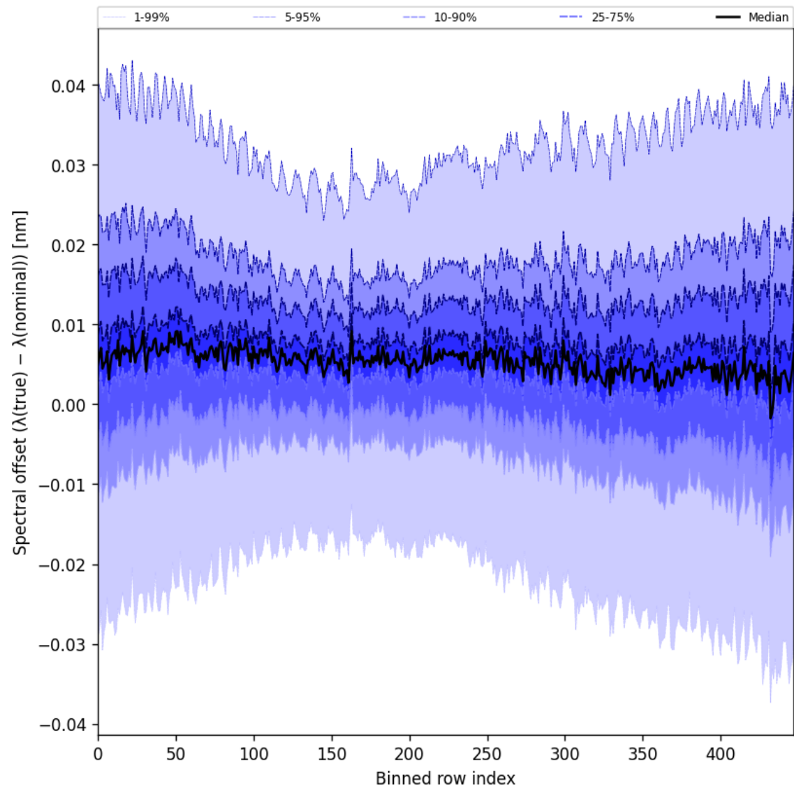
Figure 62: Along track statistics of “Spectral offset ( \lambda_{\text{true}} - \lambda_{\text{nominal}} )” for 2025-09-28 to 2025-09-30
