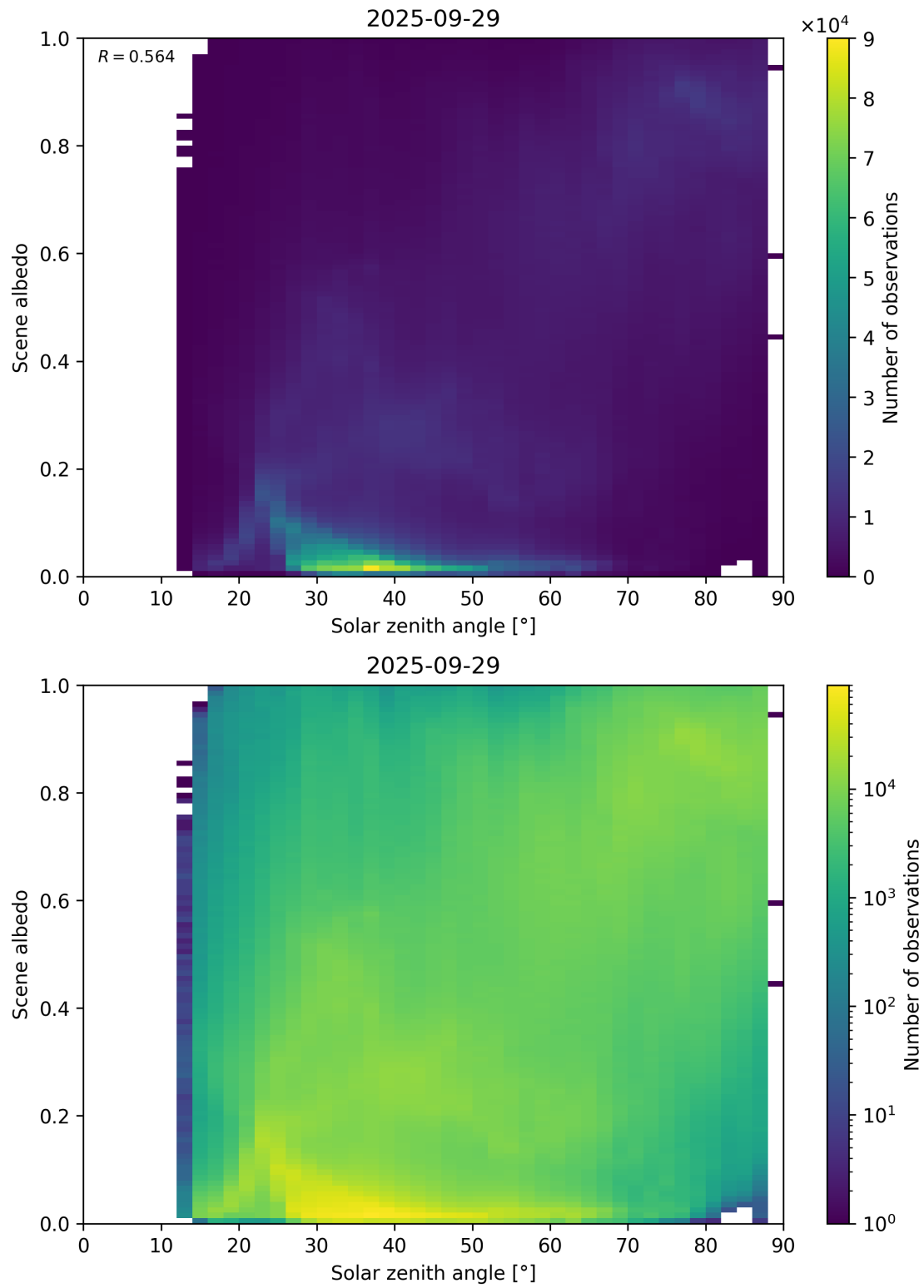
Figure 116: Scatter density plot of “Solar zenith angle” against “Scene albedo” for 2025-09-28 to 2025-09-30.
