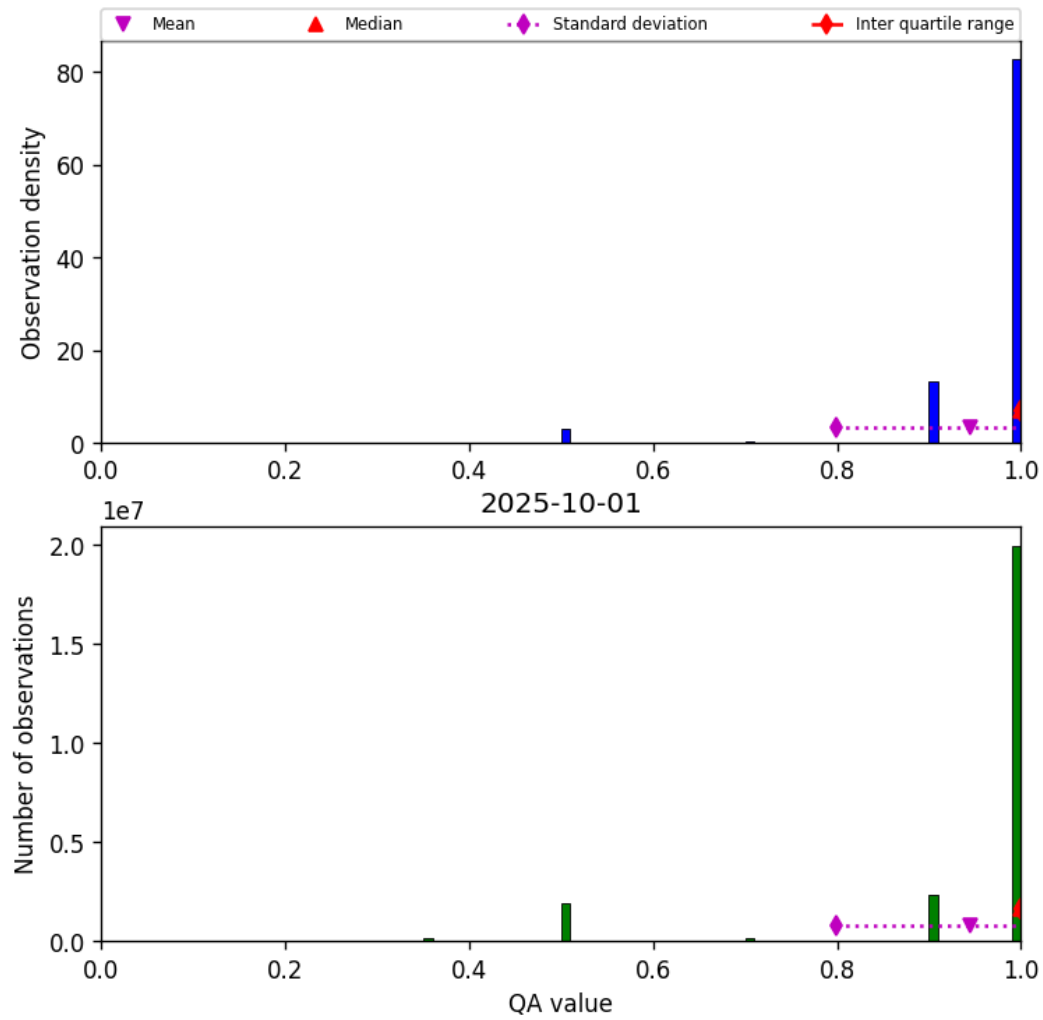
Figure 29: Histogram of “QA value” for 2025-10-01 to 2025-10-02
