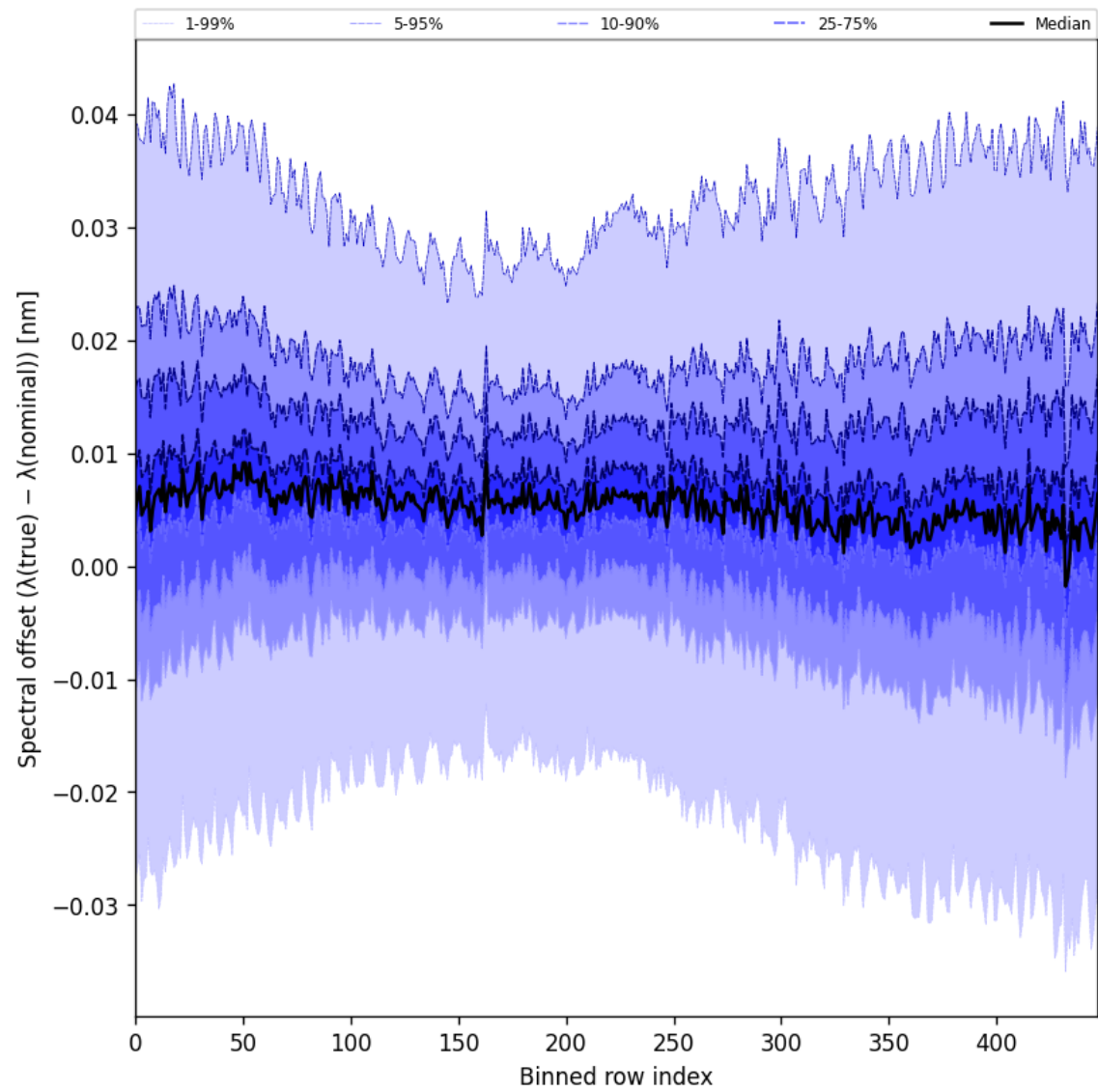
Figure 62: Along track statistics of “Spectral offset ( \lambda_{\text{true}} - \lambda_{\text{nominal}} )” for 2025-10-01 to 2025-10-02
