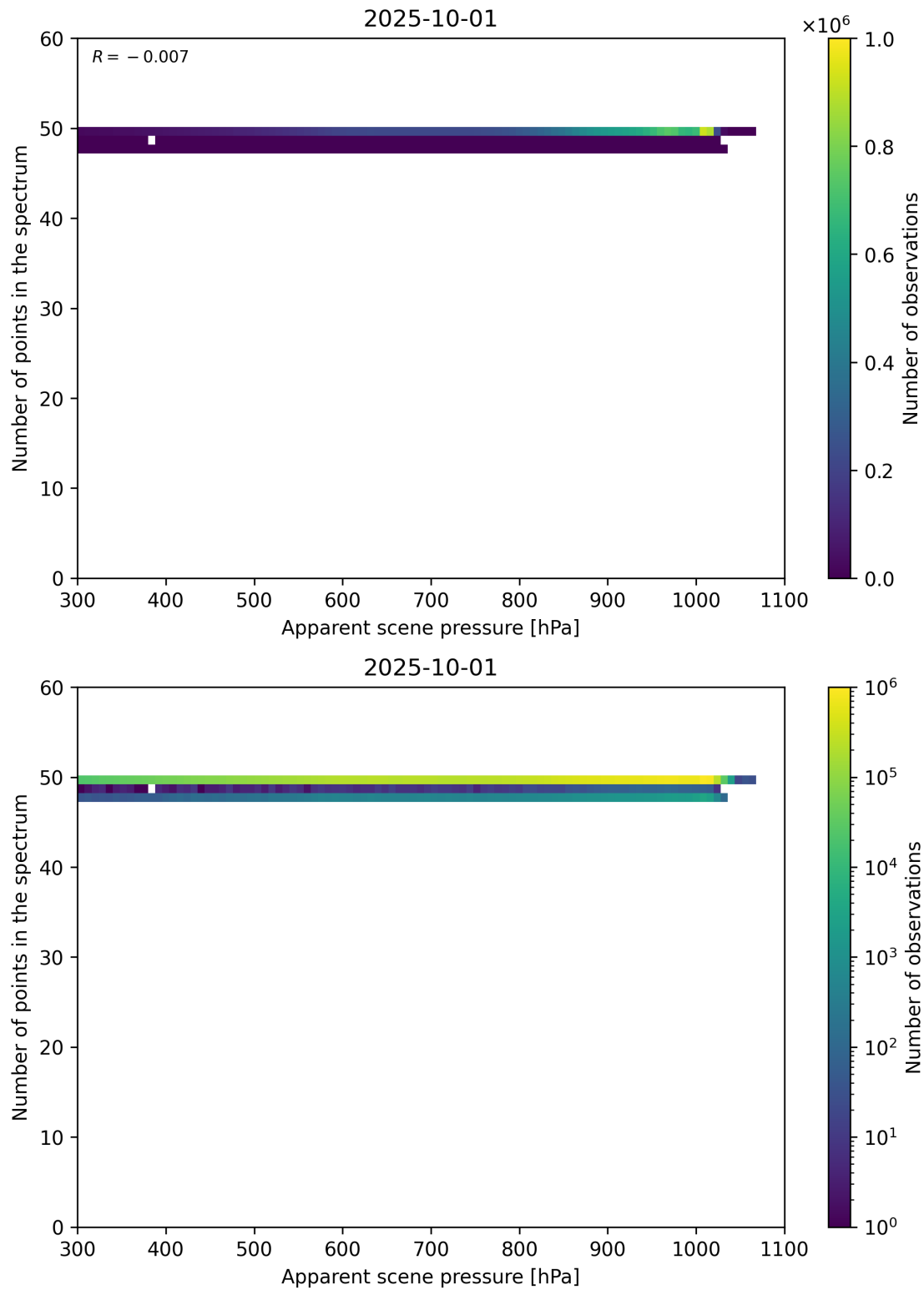
Figure 66: Scatter density plot of “Apparent scene pressure” against “Number of points in the spectrum” for 2025-10-01 to 2025-10-02.
