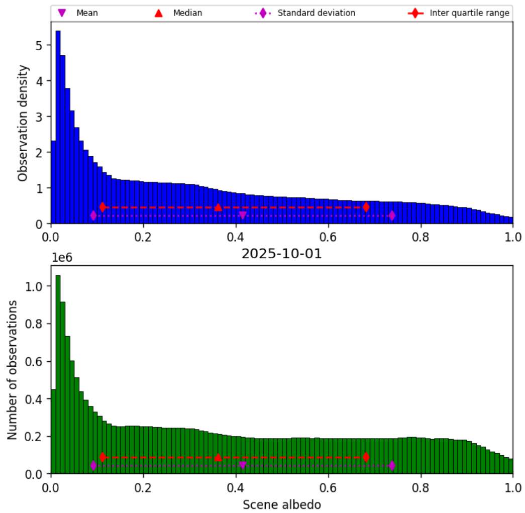
Figure 34: Histogram of “Scene albedo” for 2025-10-01 to 2025-10-02
