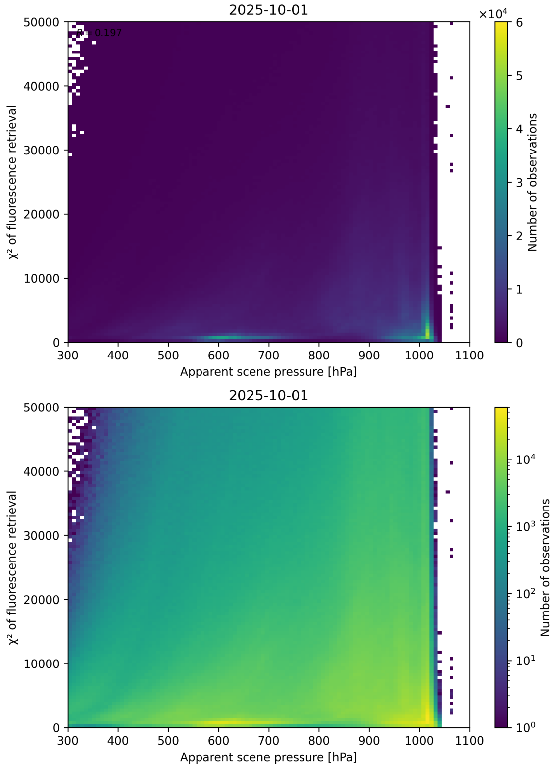
Figure 63: Scatter density plot of “Apparent scene pressure” against “ \chi^2 of fluorescence retrieval” for 2025-10-01 to 2025-10-02.
