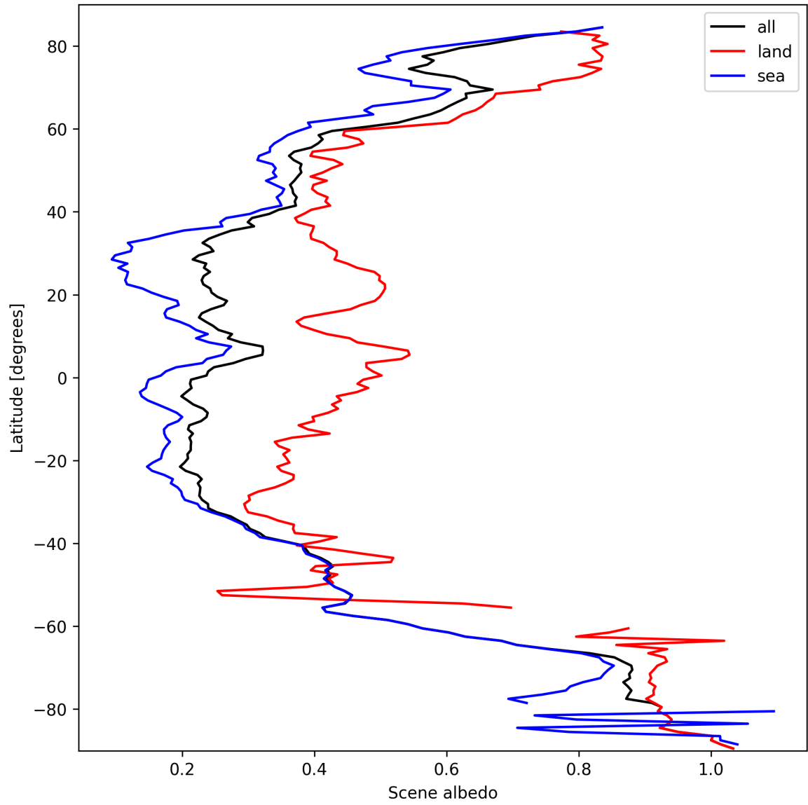
Figure 17: Zonal average of “Scene albedo” for 2025-10-01 to 2025-10-02.
