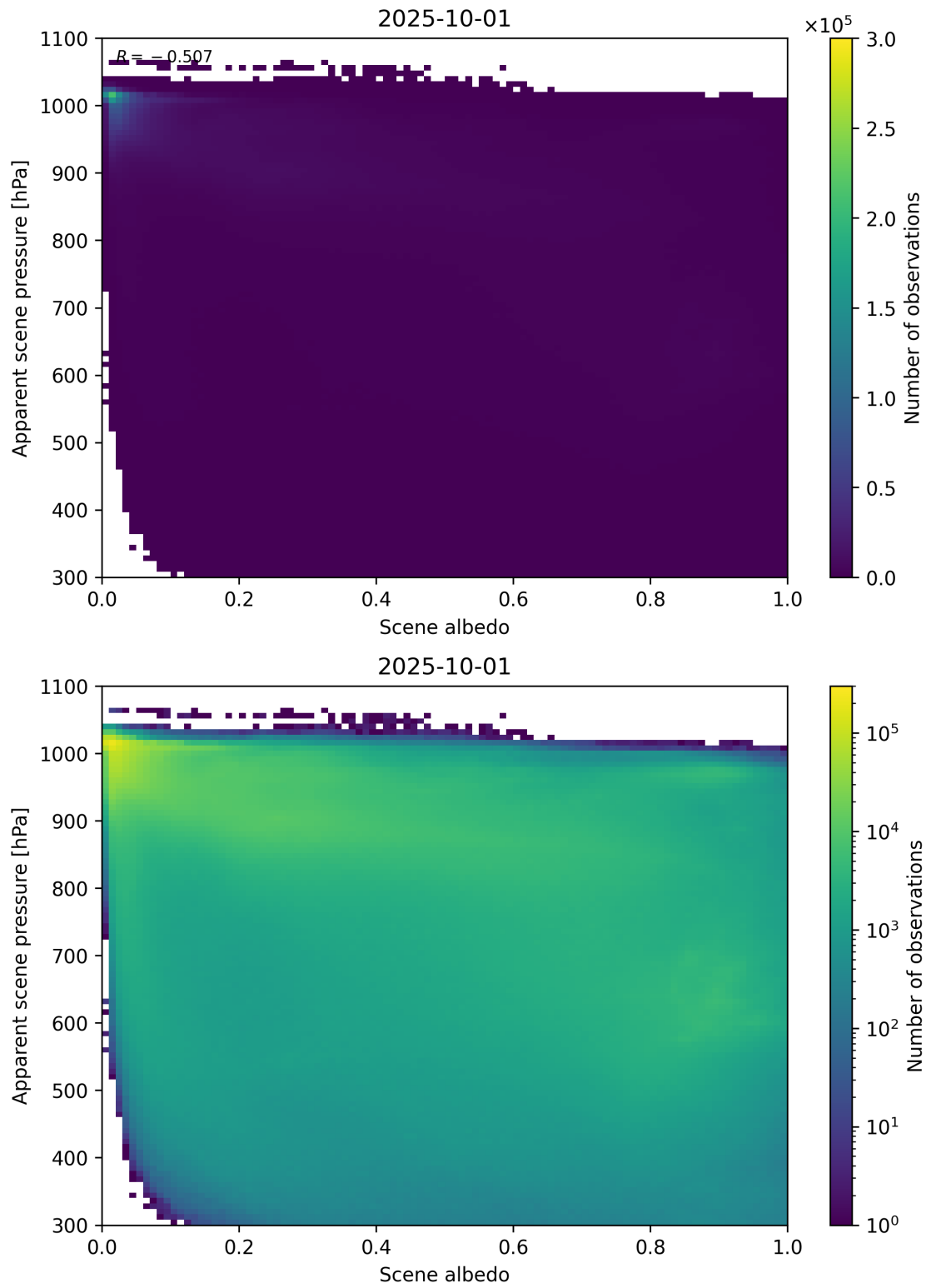
Figure 102: Scatter density plot of “Scene albedo” against “Apparent scene pressure” for 2025-10-01 to 2025-10-02.
