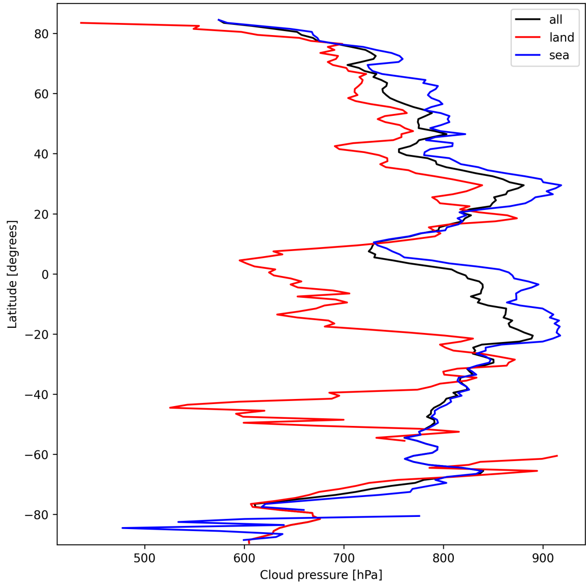
Figure 13: Zonal average of “Cloud pressure” for 2025-10-01 to 2025-10-02.
