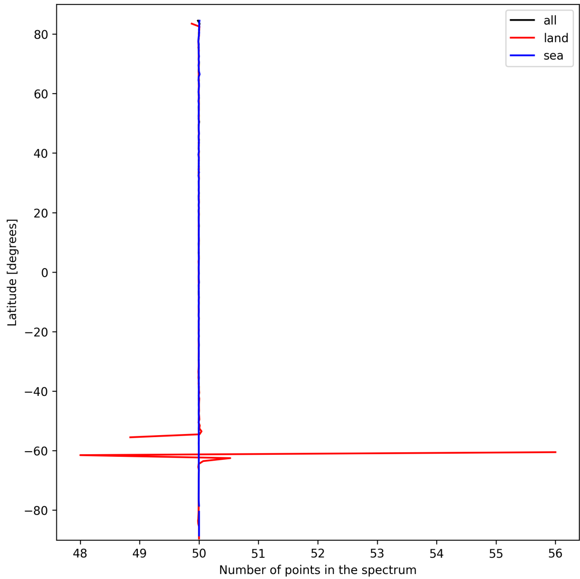
Figure 27: Zonal average of “Number of points in the spectrum” for 2025-10-01 to 2025-10-02.
