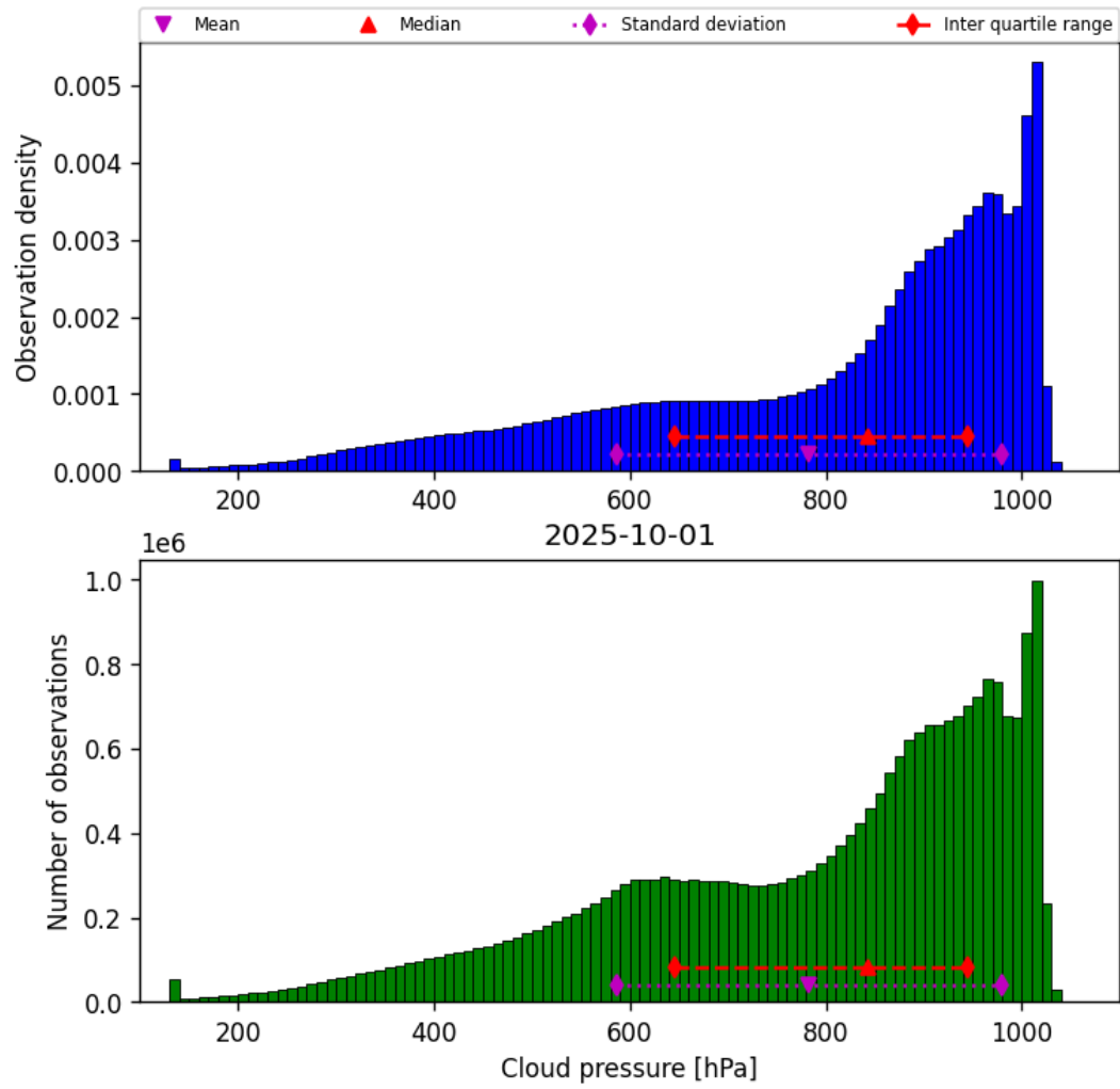
Figure 30: Histogram of “Cloud pressure” for 2025-10-01 to 2025-10-02
