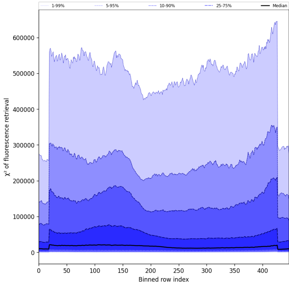
Figure 59: Along track statistics of “ \chi^2 of fluorescence retrieval” for 2025-10-01 to 2025-10-02
