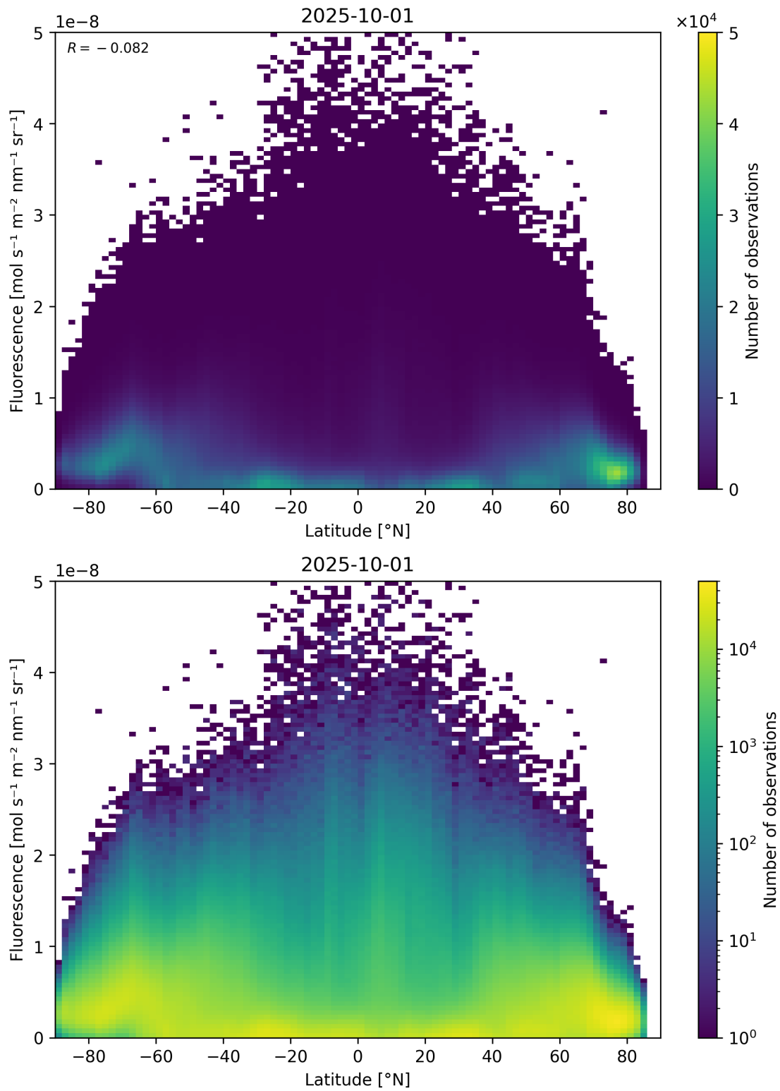
Figure 92: Scatter density plot of “Latitude” against “Fluorescence” for 2025-10-01 to 2025-10-02.
