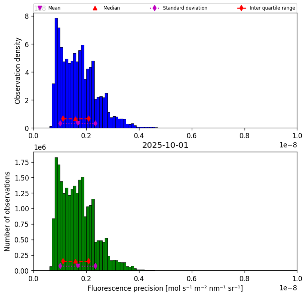
Figure 41: Histogram of “Fluorescence precision” for 2025-10-01 to 2025-10-02
