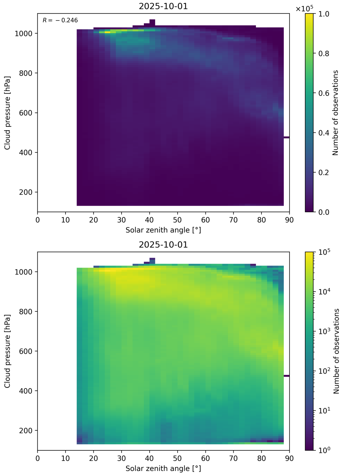
Figure 111: Scatter density plot of “Solar zenith angle” against “Cloud pressure” for 2025-10-01 to 2025-10-02.
