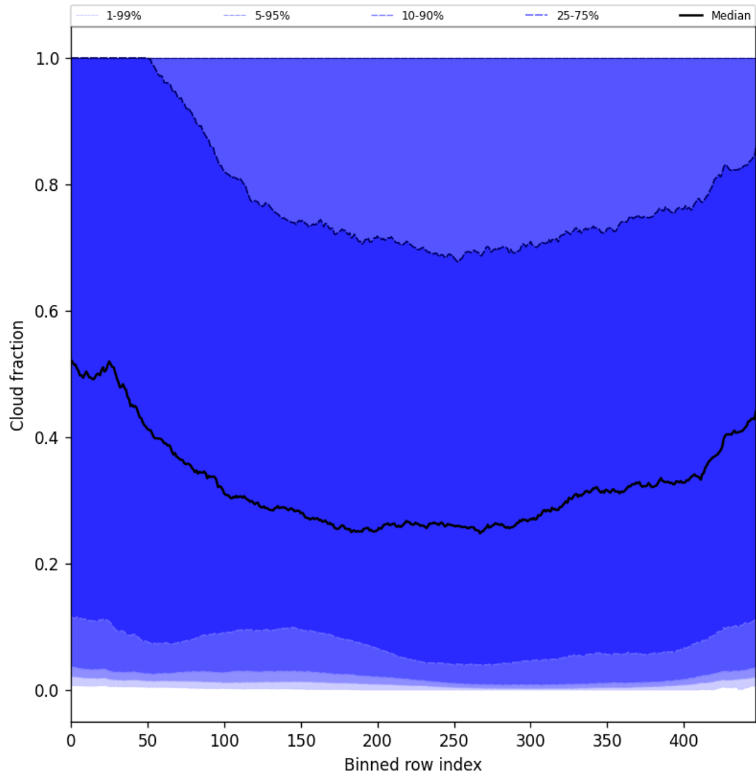
Figure 49: Along track statistics of “Cloud fraction” for 2025-10-01 to 2025-10-02
