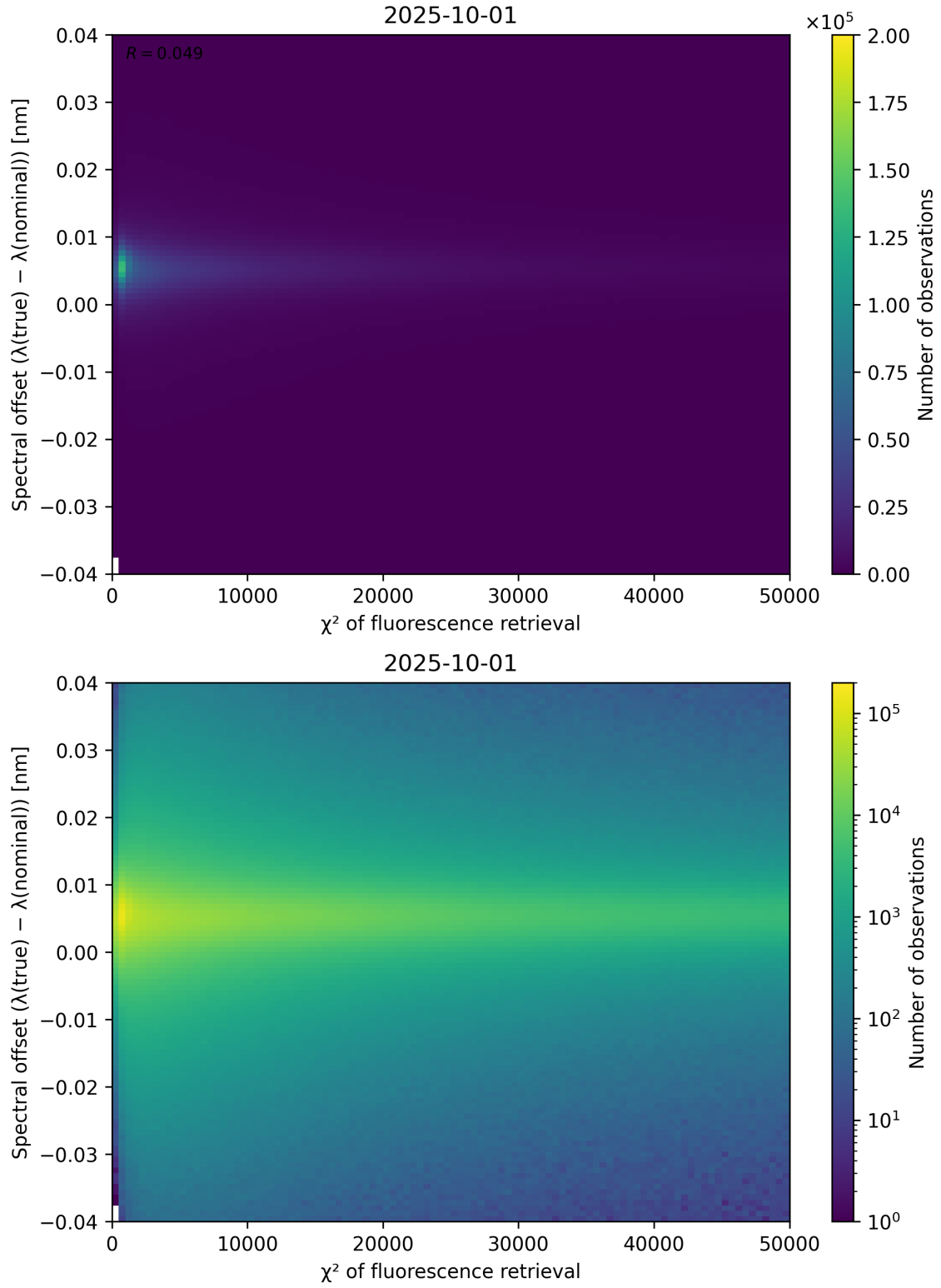
Figure 69: Scatter density plot of “ \chi^2 of fluorescence retrieval” against “Spectral offset ( \lambda_{\text{true}} - \lambda_{\text{nominal}} )” for 2025-10-01 to 2025-10-02.
