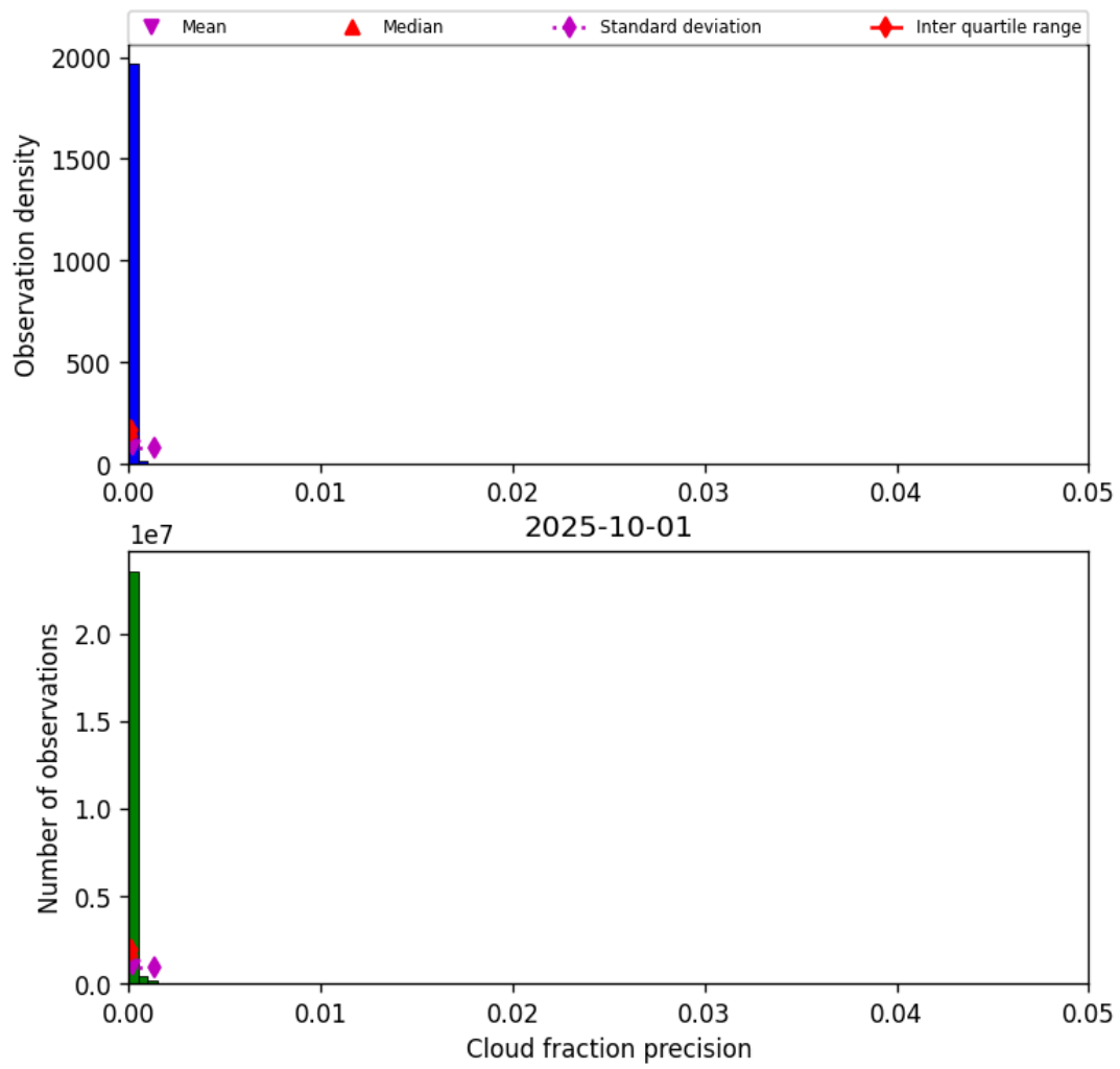
Figure 33: Histogram of “Cloud fraction precision” for 2025-10-01 to 2025-10-02
