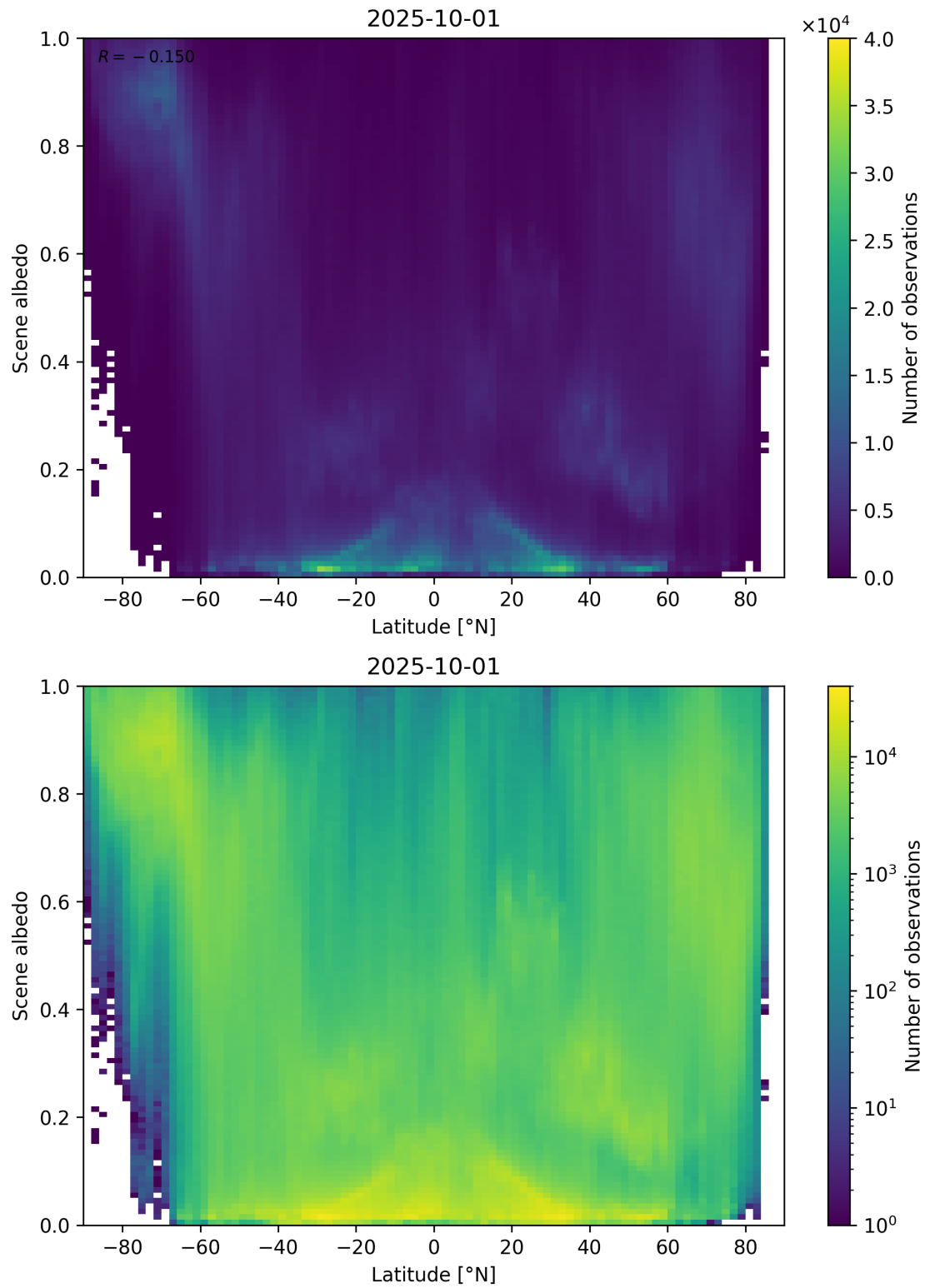
Figure 95: Scatter density plot of “Latitude” against “Scene albedo” for 2025-10-01 to 2025-10-02.
