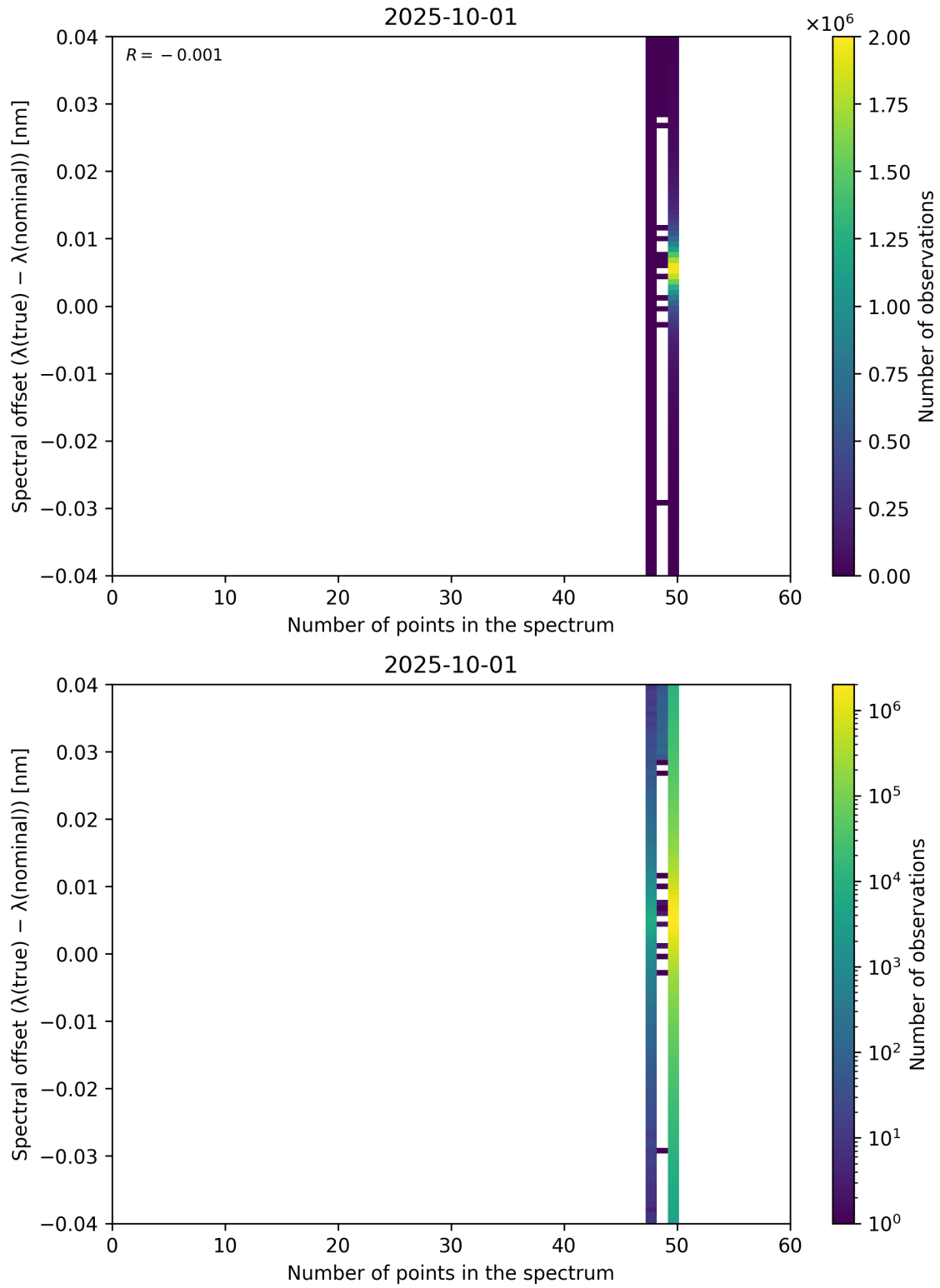
Figure 101: Scatter density plot of “Number of points in the spectrum” against “Spectral offset ( \lambda_{\text{true}} - \lambda_{\text{nominal}} )” for 2025-10-01 to 2025-10-02.
