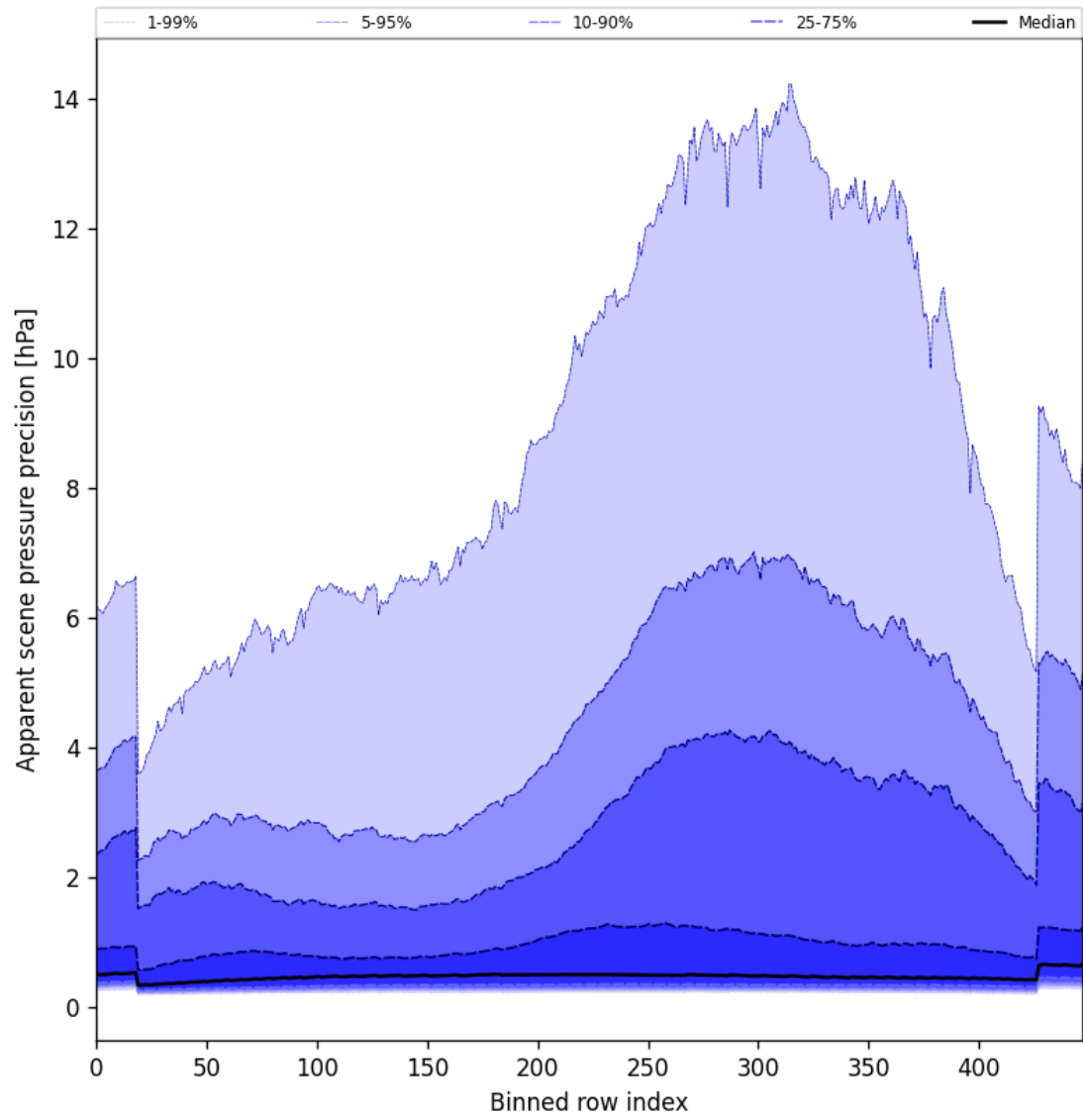
Figure 54: Along track statistics of “Apparent scene pressure precision” for 2025-10-01 to 2025-10-02
