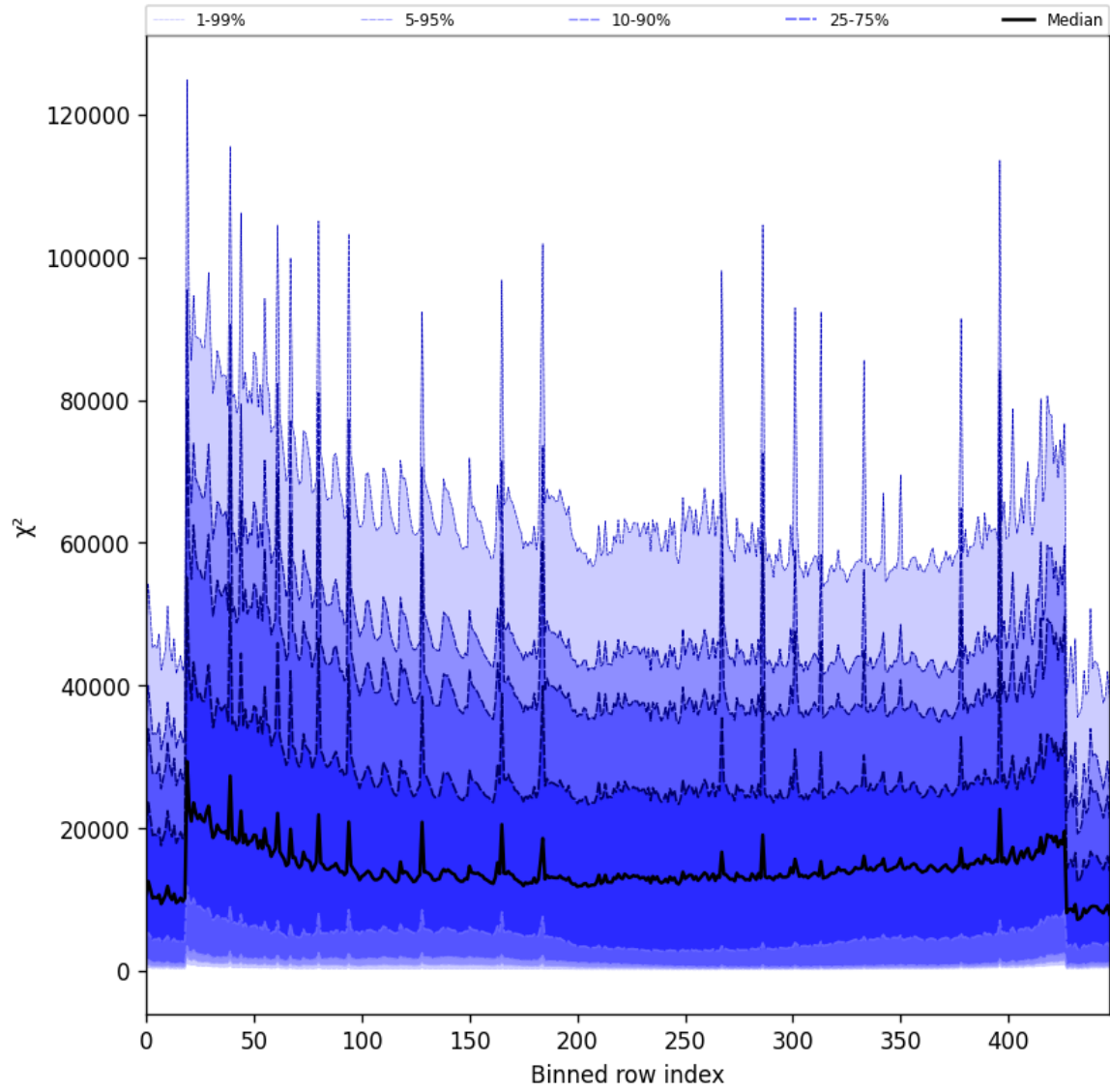
Figure 55: Along track statistics of “ \chi^2 ” for 2025-10-01 to 2025-10-02
