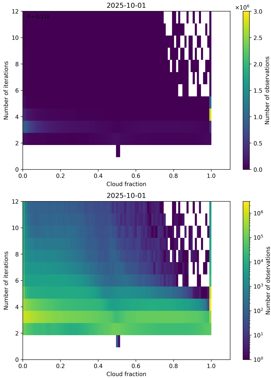
Figure 73: Scatter density plot of “Cloud fraction” against “Number of iterations” for 2025-10-01 to 2025-10-02.
