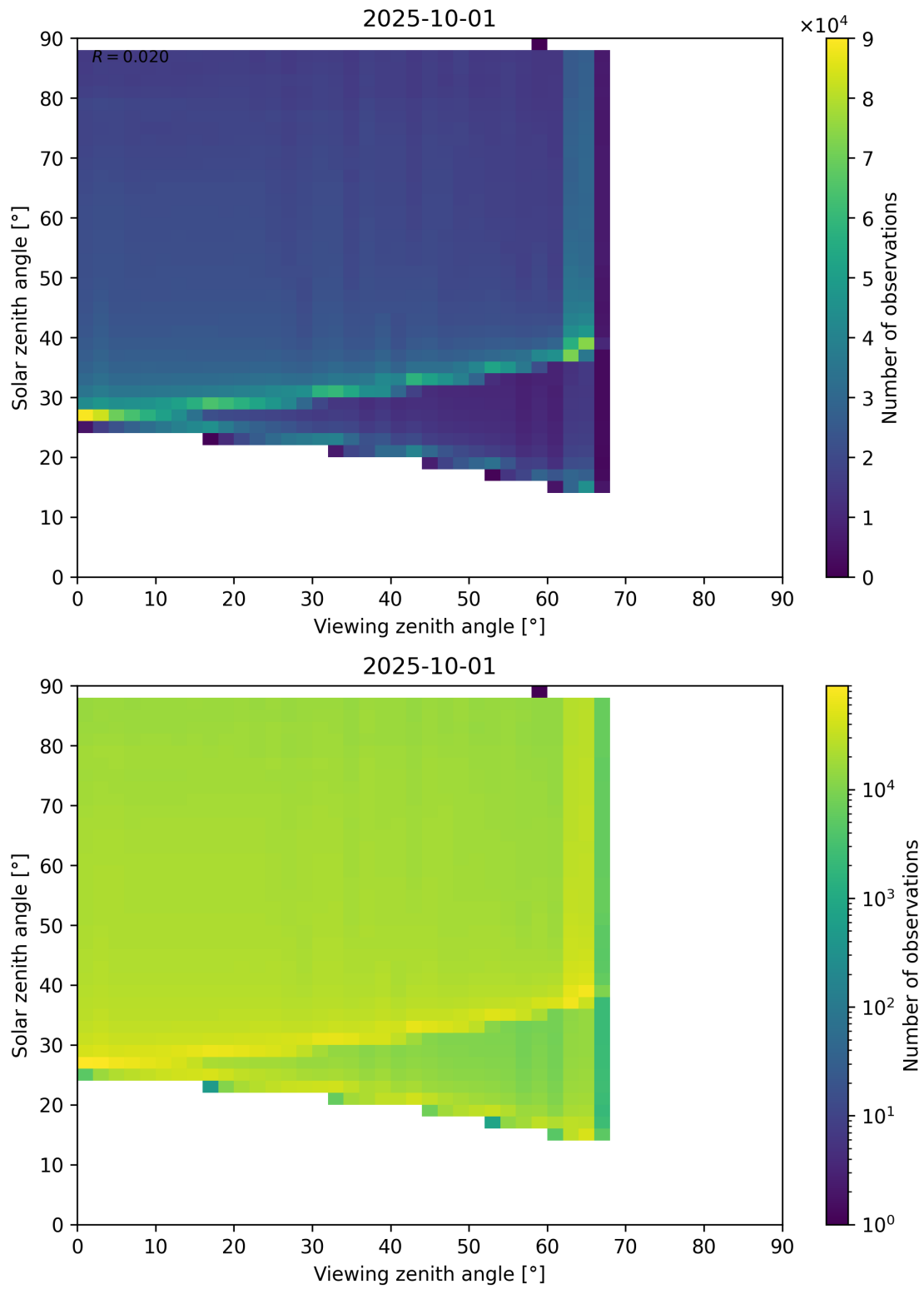
Figure 127: Scatter density plot of “Viewing zenith angle” against “Solar zenith angle” for 2025-10-01 to 2025-10-02.
