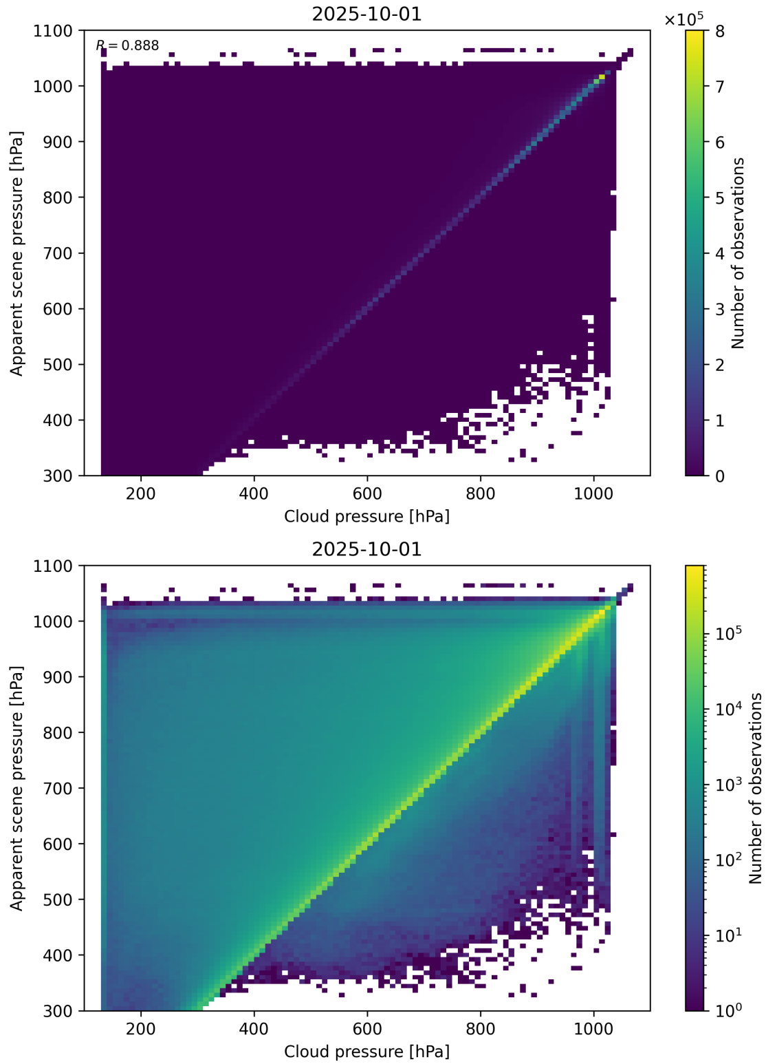
Figure 77: Scatter density plot of “Cloud pressure” against “Apparent scene pressure” for 2025-10-01 to 2025-10-02.
