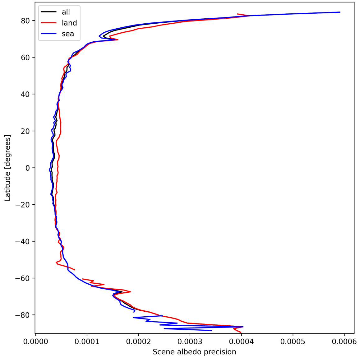
Figure 18: Zonal average of “Scene albedo precision” for 2025-10-01 to 2025-10-02.
