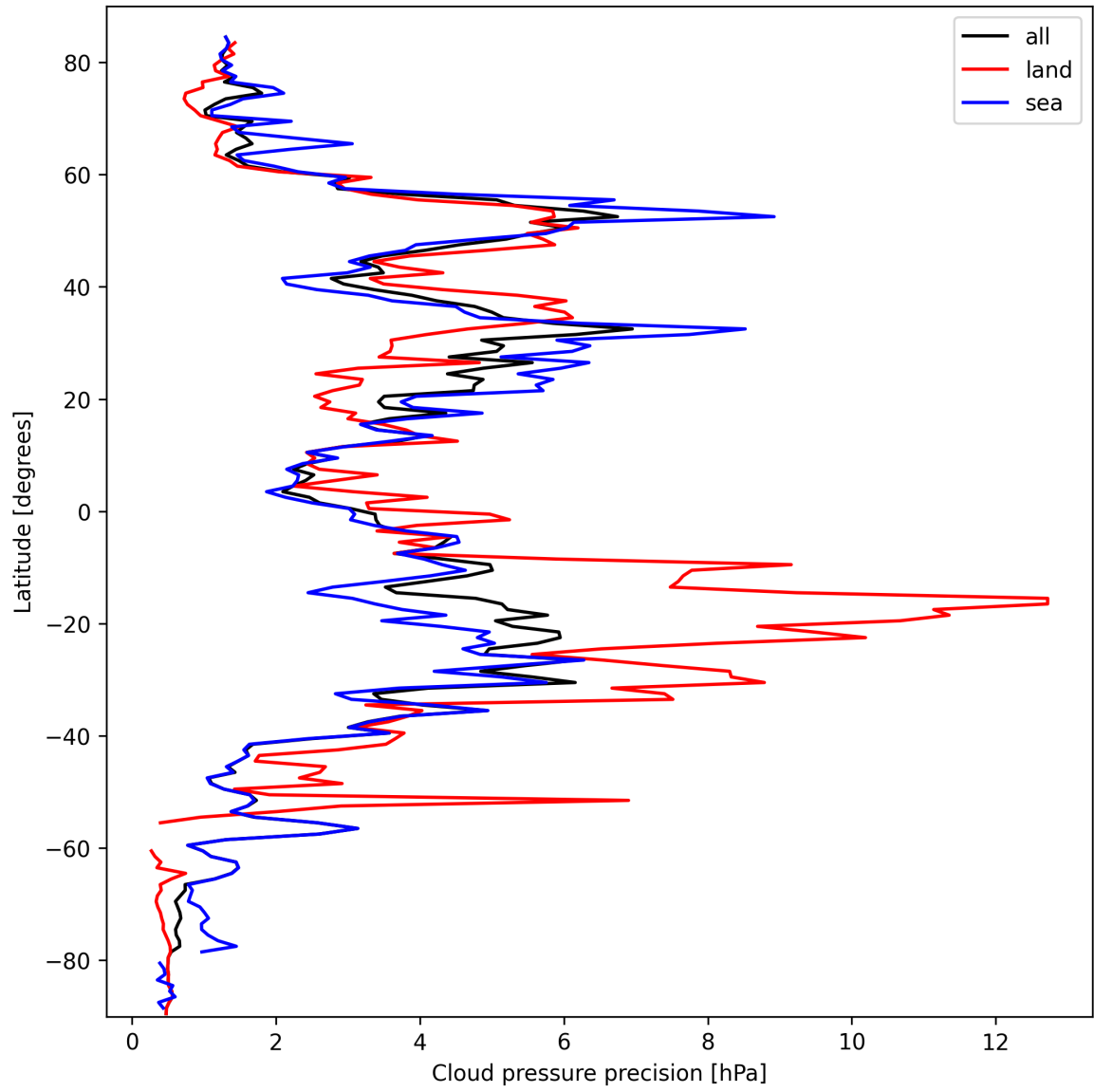
Figure 14: Zonal average of “Cloud pressure precision” for 2025-10-01 to 2025-10-02.
