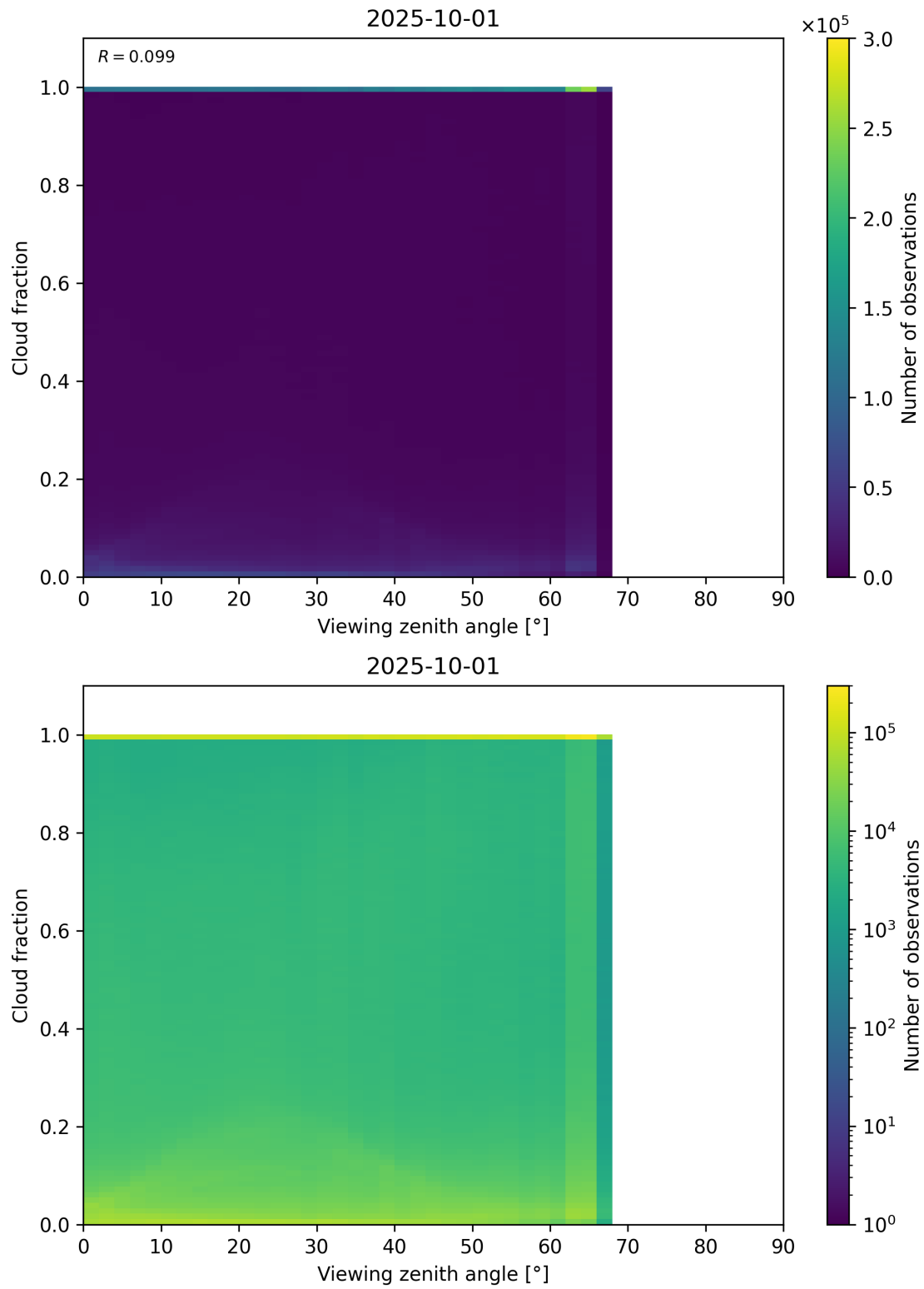
Figure 120: Scatter density plot of “Viewing zenith angle” against “Cloud fraction” for 2025-10-01 to 2025-10-02.
