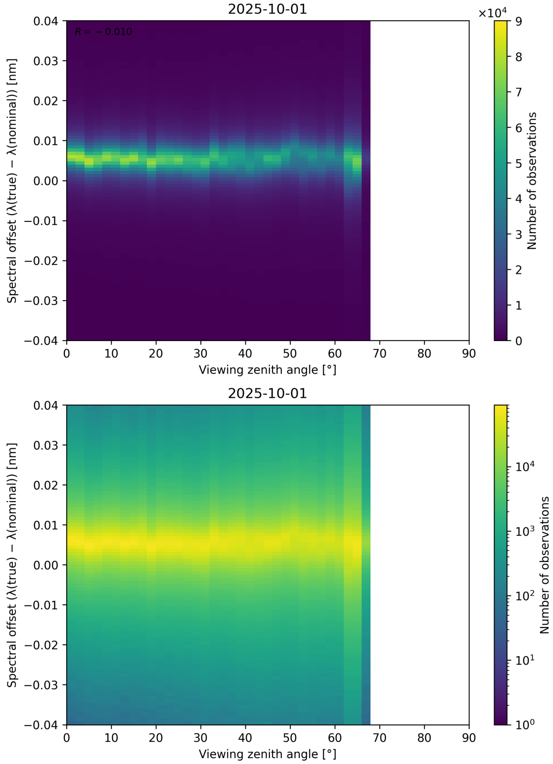
Figure 128: Scatter density plot of “Viewing zenith angle” against “Spectral offset ( \lambda_{\text{true}} - \lambda_{\text{nominal}} )” for 2025-10-01 to 2025-10-02.
