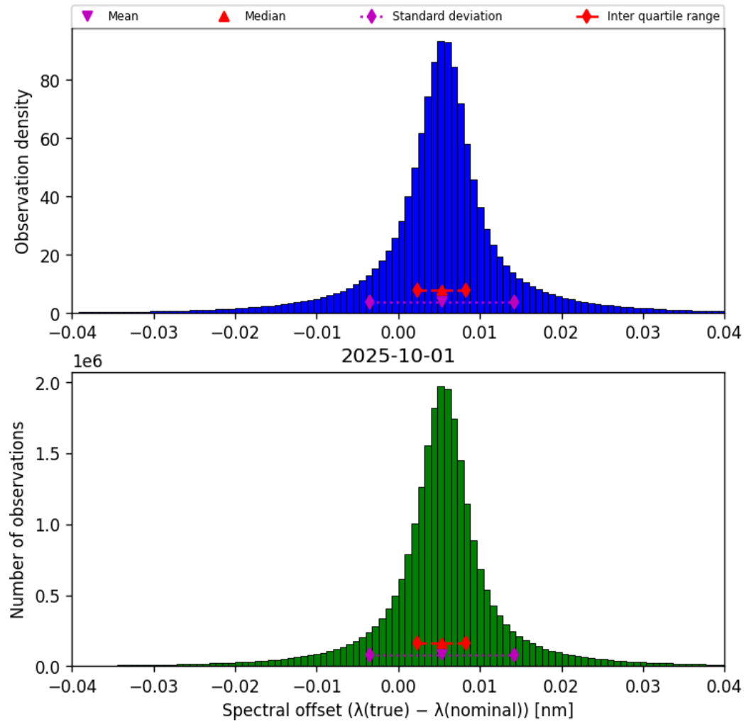
Figure 45: Histogram of “Spectral offset ( \lambda_{\text{true}} - \lambda_{\text{nominal}} )” for 2025-10-01 to 2025-10-02
