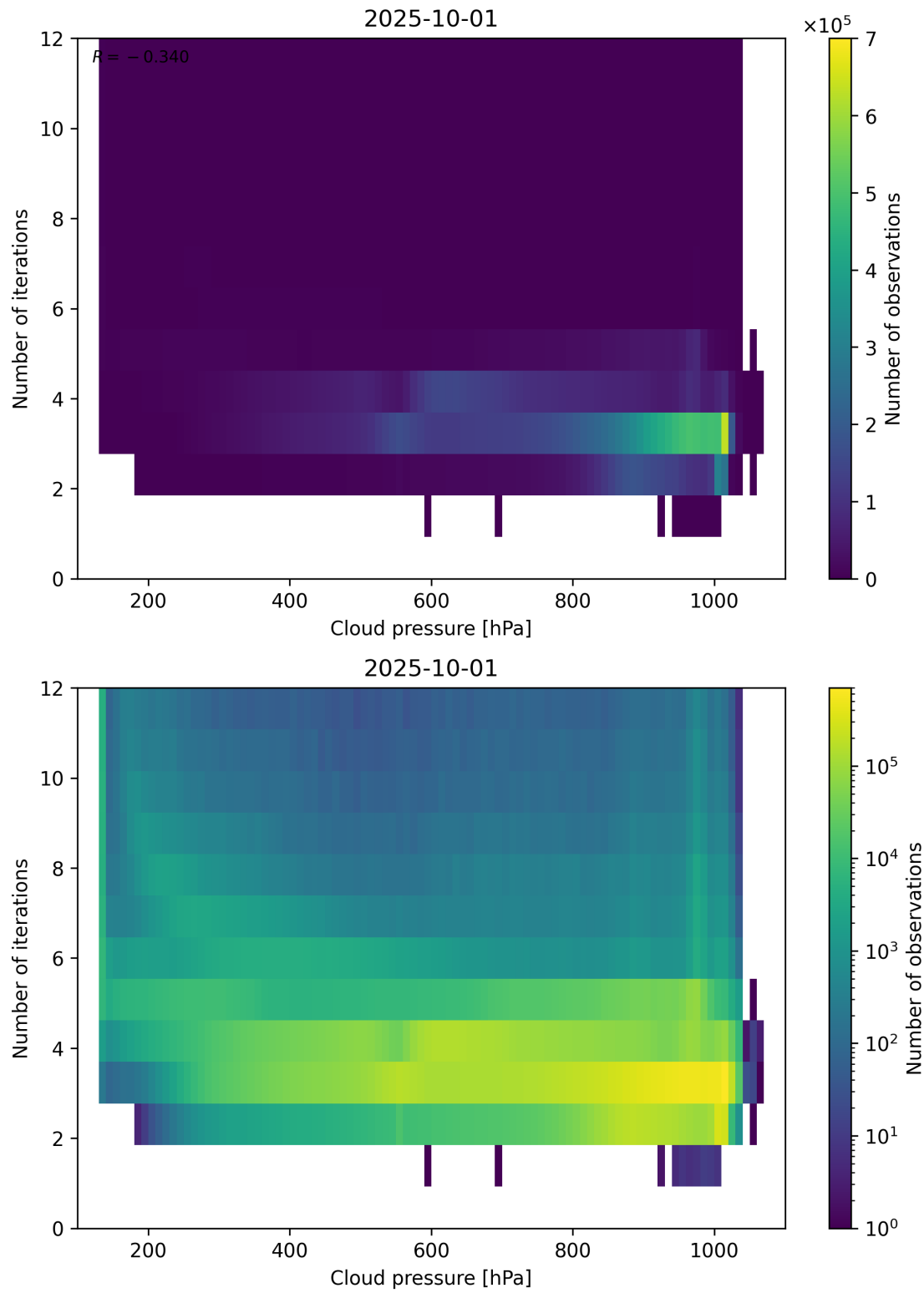
Figure 81: Scatter density plot of “Cloud pressure” against “Number of iterations” for 2025-10-01 to 2025-10-02.
