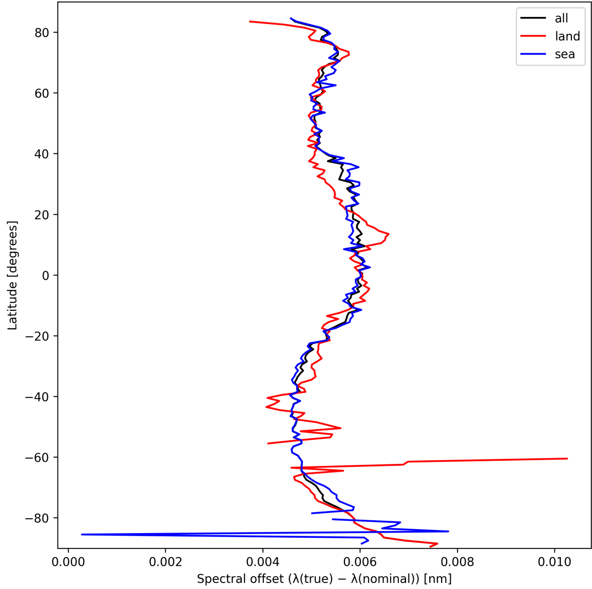
Figure 28: Zonal average of “Spectral offset ( \lambda_{\text{true}} - \lambda_{\text{nominal}} )” for 2025-10-01 to 2025-10-02.
