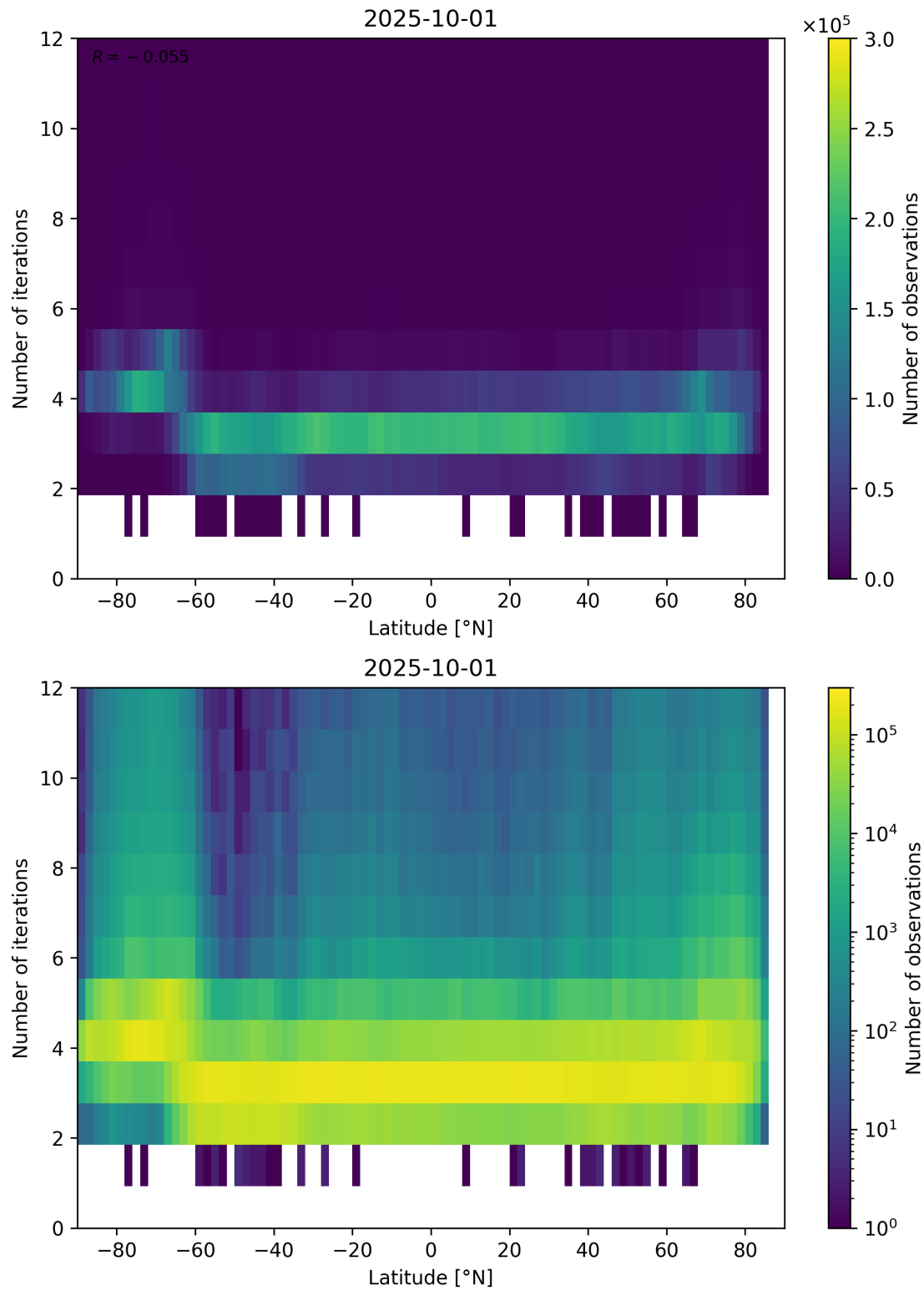
Figure 93: Scatter density plot of “Latitude” against “Number of iterations” for 2025-10-01 to 2025-10-02.
