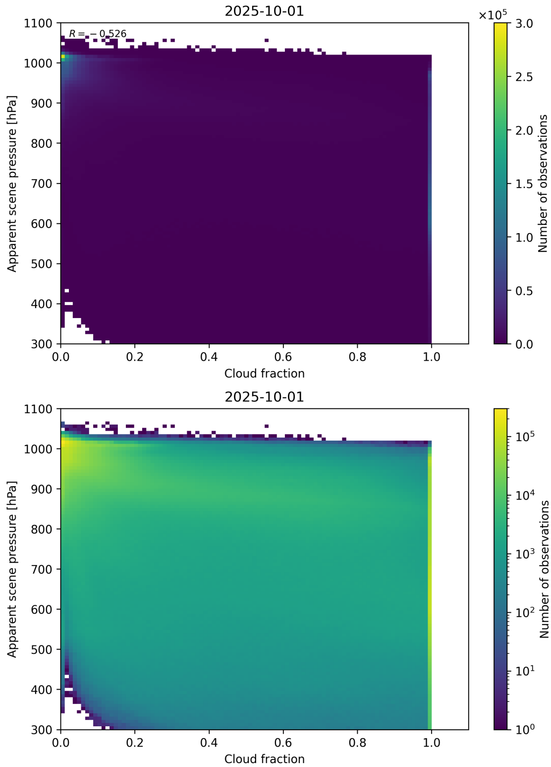
Figure 70: Scatter density plot of “Cloud fraction” against “Apparent scene pressure” for 2025-10-01 to 2025-10-02.
