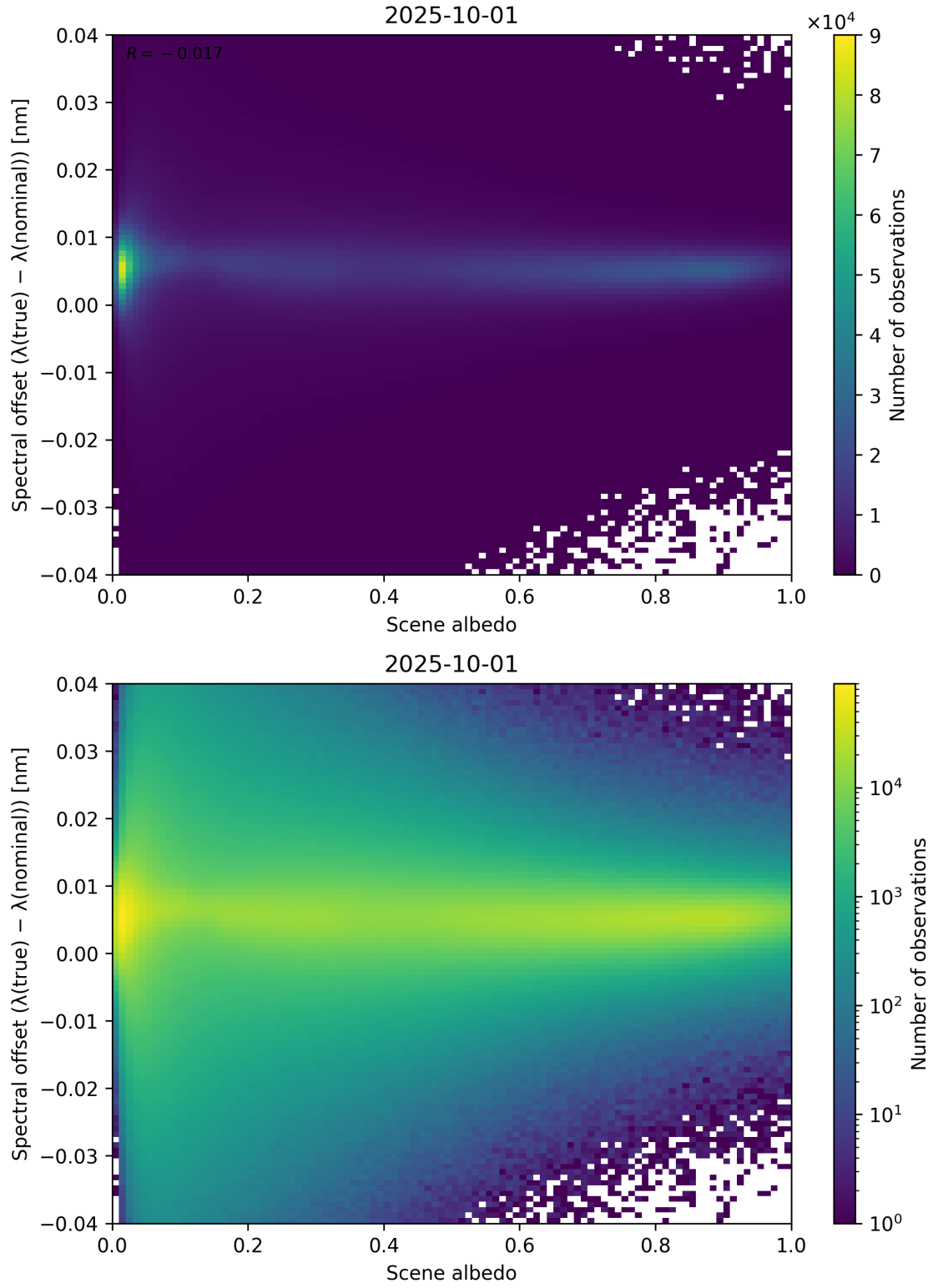
Figure 107: Scatter density plot of “Scene albedo” against “Spectral offset ( \lambda_{\text{true}} - \lambda_{\text{nominal}} )” for 2025-10-01 to 2025-10-02.
