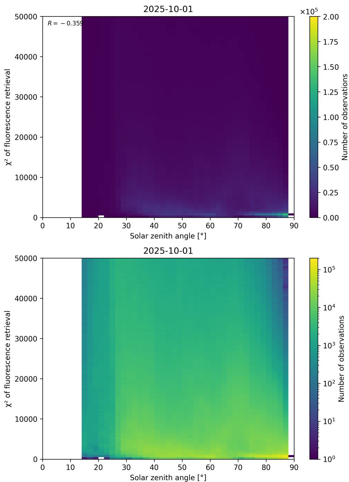
Figure 109: Scatter density plot of “Solar zenith angle” against “ \chi^2 of fluorescence retrieval” for 2025-10-01 to 2025-10-02.
