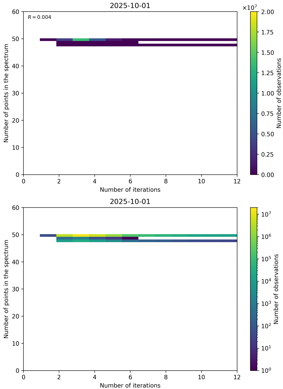
Figure 99: Scatter density plot of “Number of iterations” against “Number of points in the spectrum” for 2025-10-01 to 2025-10-02.
