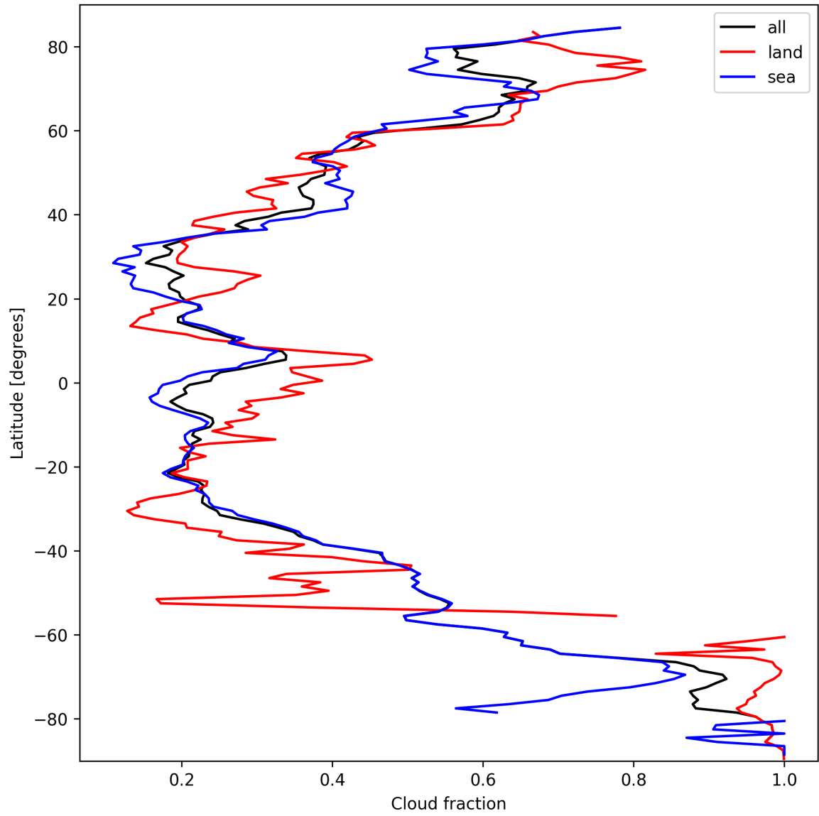
Figure 15: Zonal average of “Cloud fraction” for 2025-10-01 to 2025-10-02.
