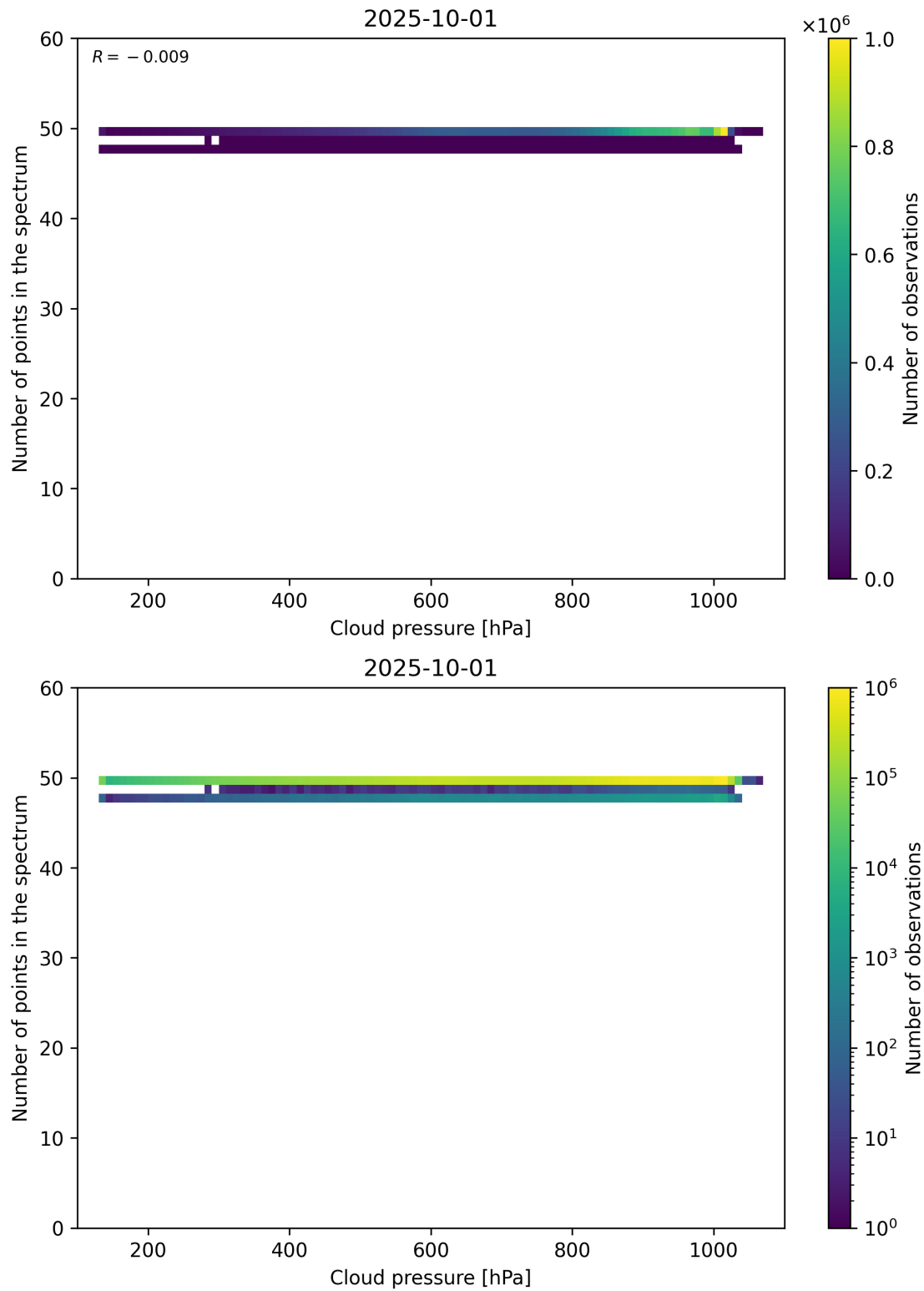
Figure 82: Scatter density plot of “Cloud pressure” against “Number of points in the spectrum” for 2025-10-01 to 2025-10-02.
