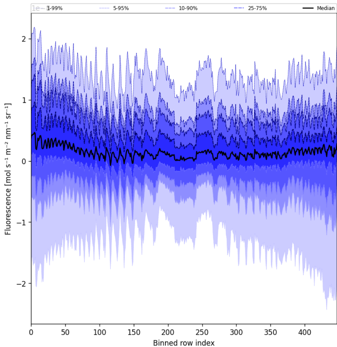
Figure 57: Along track statistics of “Fluorescence” for 2025-10-01 to 2025-10-02
