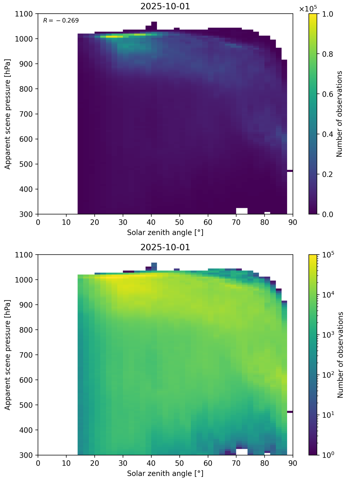
Figure 108: Scatter density plot of “Solar zenith angle” against “Apparent scene pressure” for 2025-10-01 to 2025-10-02.
