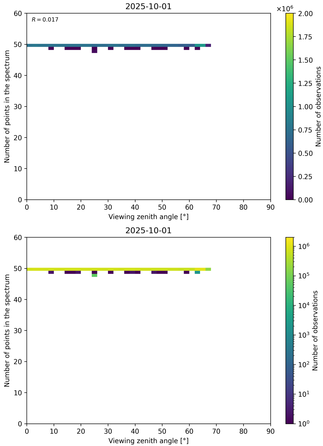
Figure 125: Scatter density plot of “Viewing zenith angle” against “Number of points in the spectrum” for 2025-10-01 to 2025-10-02.
