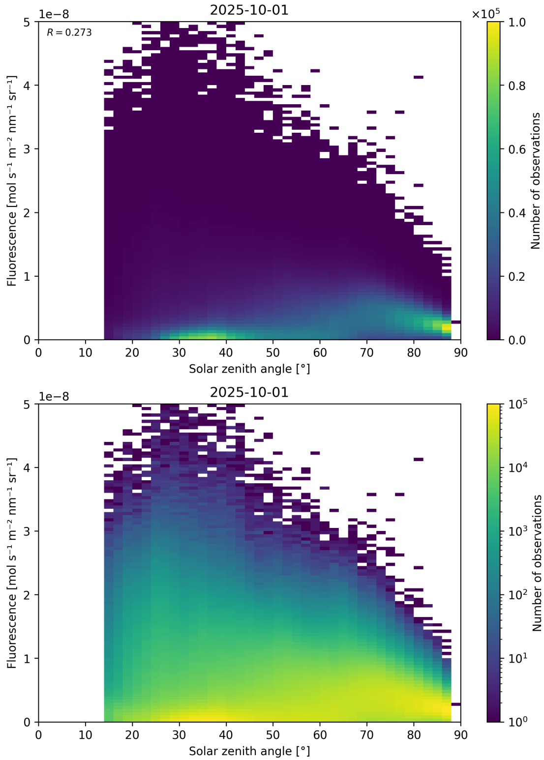
Figure 112: Scatter density plot of “Solar zenith angle” against “Fluorescence” for 2025-10-01 to 2025-10-02.
