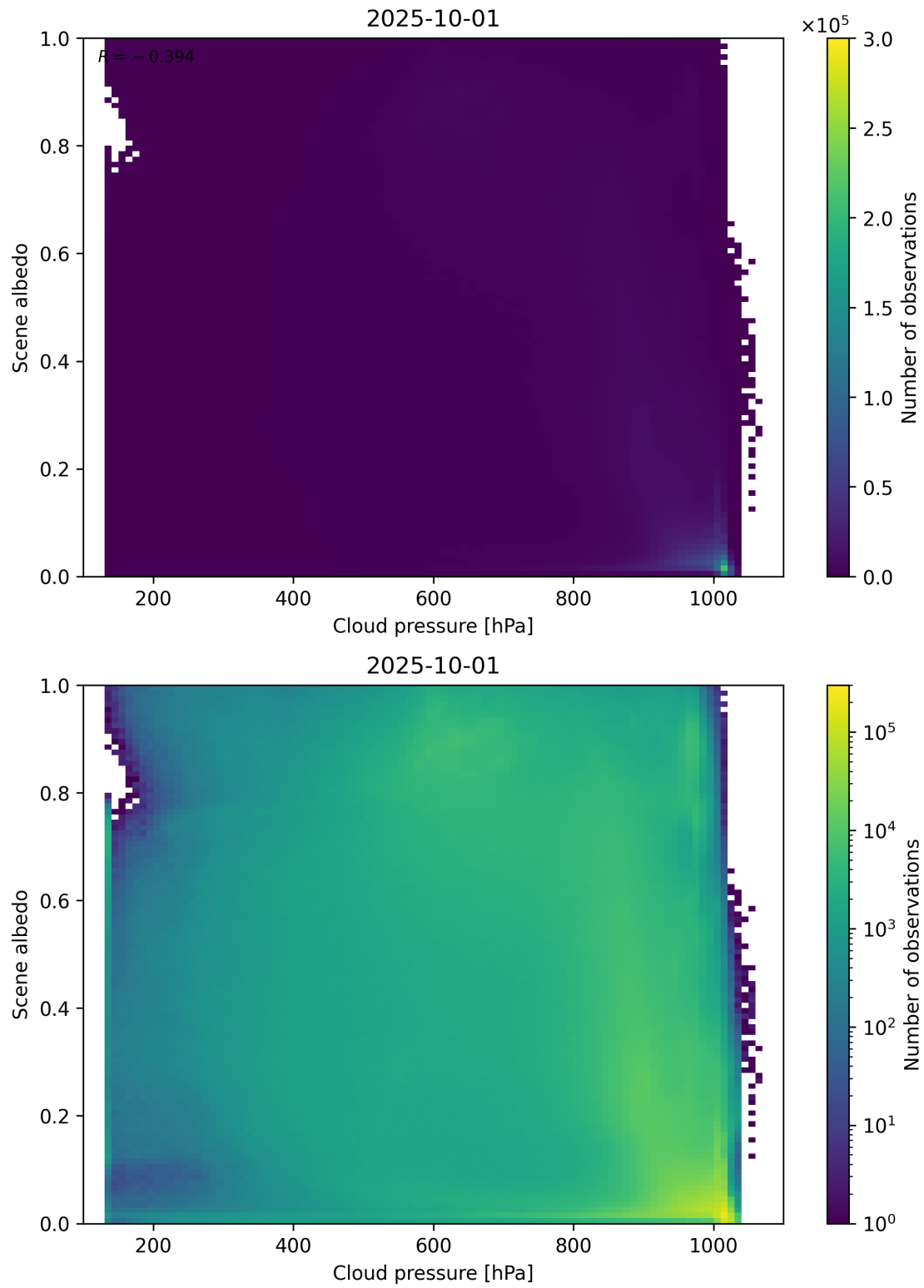
Figure 83: Scatter density plot of “Cloud pressure” against “Scene albedo” for 2025-10-01 to 2025-10-02.
