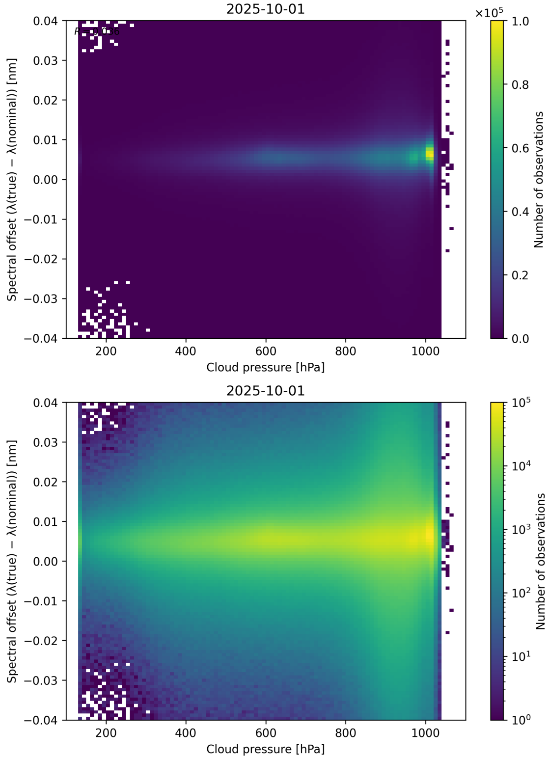
Figure 84: Scatter density plot of “Cloud pressure” against “Spectral offset ( \lambda_{\text{true}} - \lambda_{\text{nominal}} )” for 2025-10-01 to 2025-10-02.
