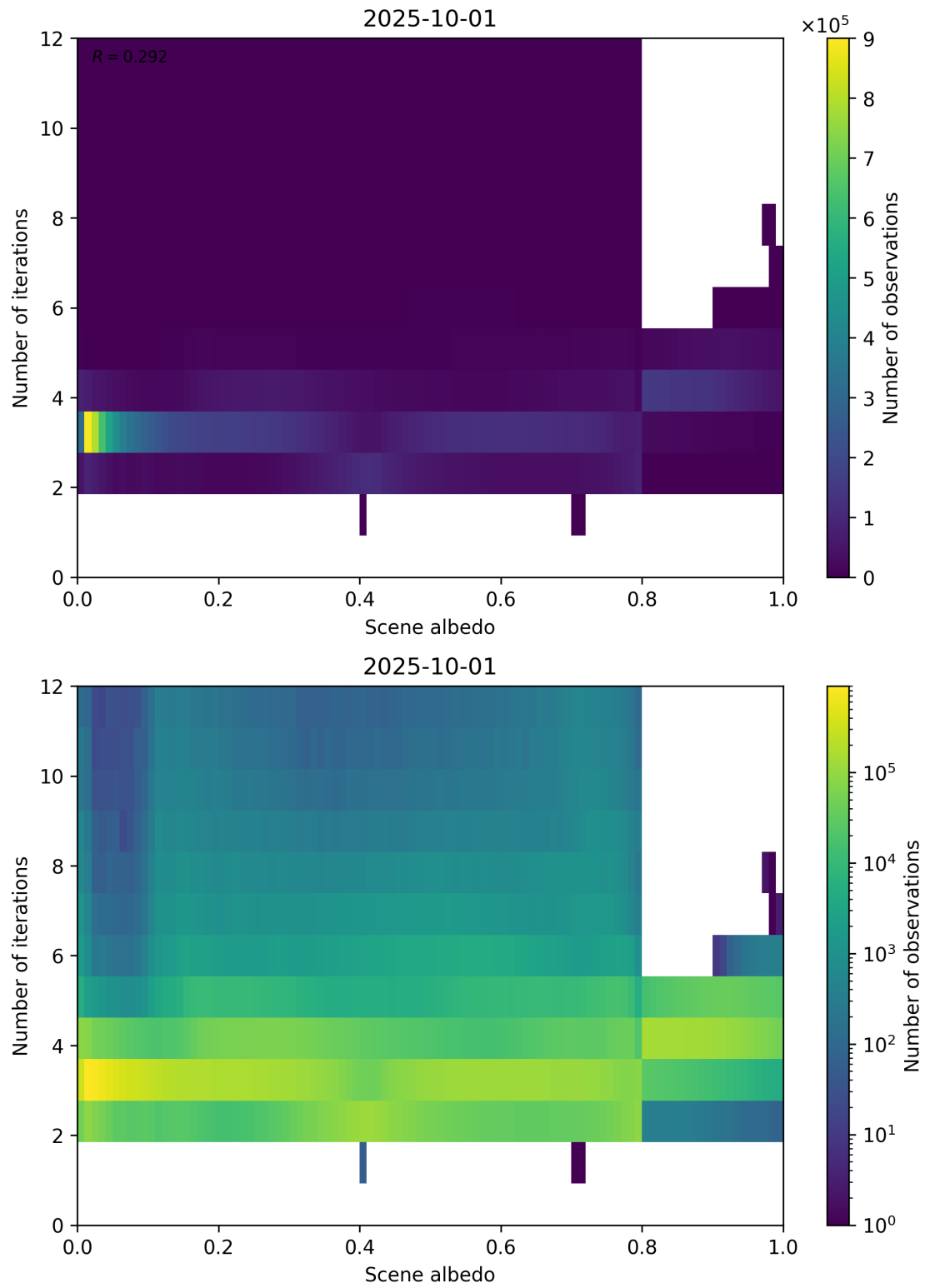
Figure 105: Scatter density plot of “Scene albedo” against “Number of iterations” for 2025-10-01 to 2025-10-02.
