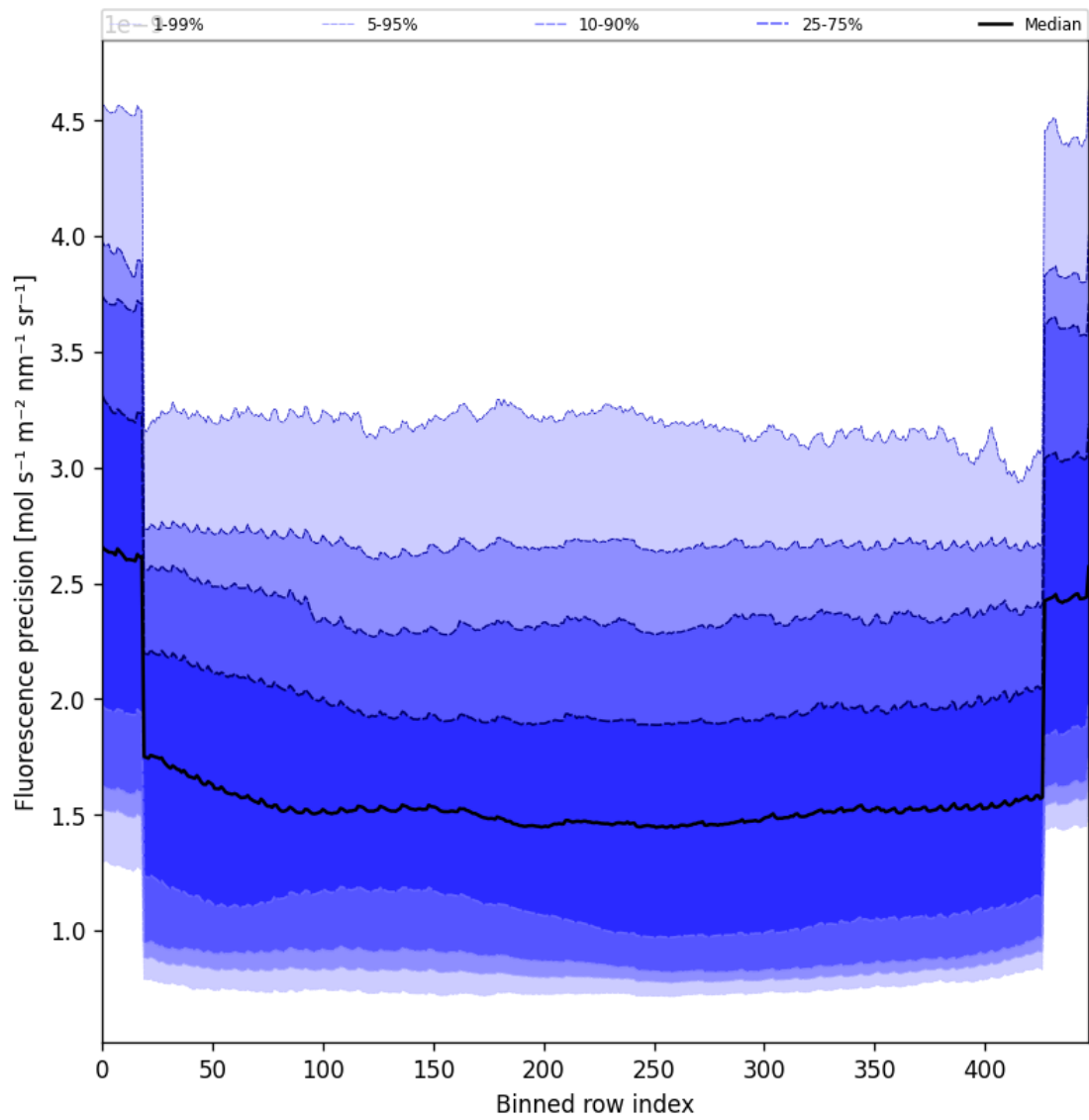
Figure 58: Along track statistics of “Fluorescence precision” for 2025-10-01 to 2025-10-02
