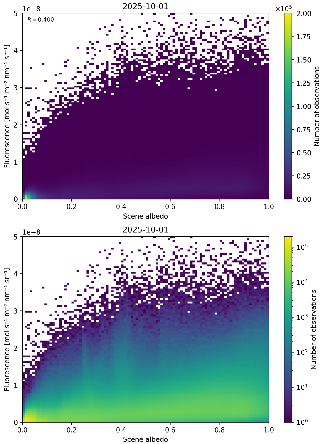
Figure 104: Scatter density plot of "Scene albedo" against "Fluorescence" for 2025-10-01 to 2025-10-02.
