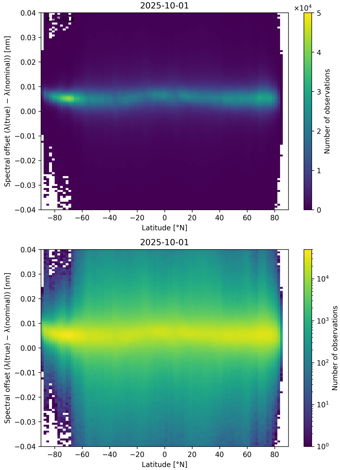
Figure 96: Scatter density plot of “Latitude” against “Spectral offset ( \lambda_{\text{true}} - \lambda_{\text{nominal}} )” for 2025-10-01 to 2025-10-02.
