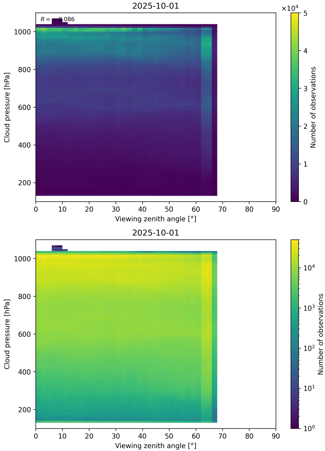
Figure 121: Scatter density plot of “Viewing zenith angle” against “Cloud pressure” for 2025-10-01 to 2025-10-02.
