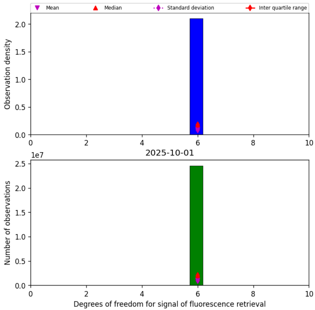
Figure 43: Histogram of "Degrees of freedom for signal of fluorescence retrieval" for 2025-10-01 to 2025-10-02
