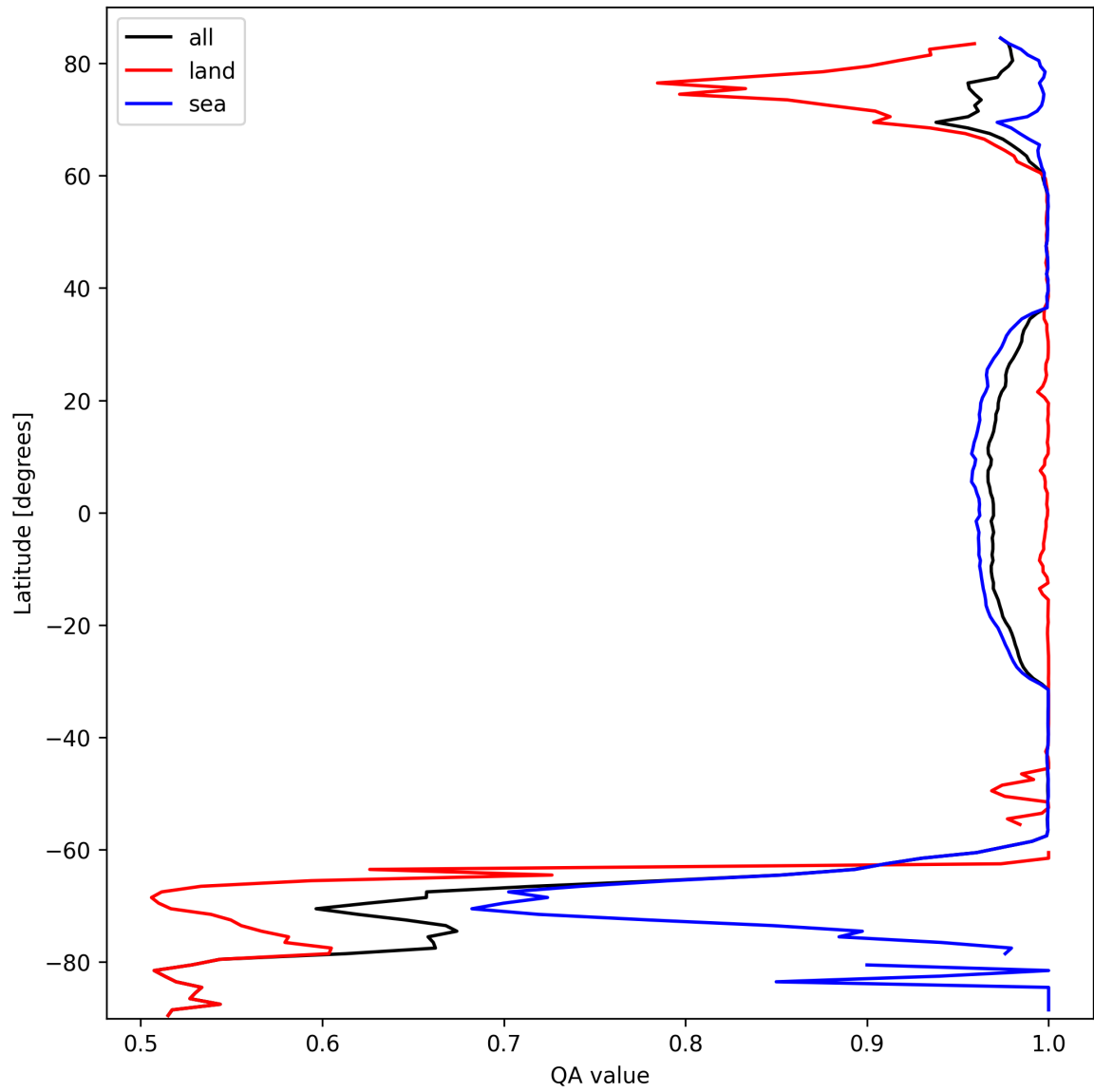
Figure 12: Zonal average of "QA value" for 2025-10-01 to 2025-10-02.
