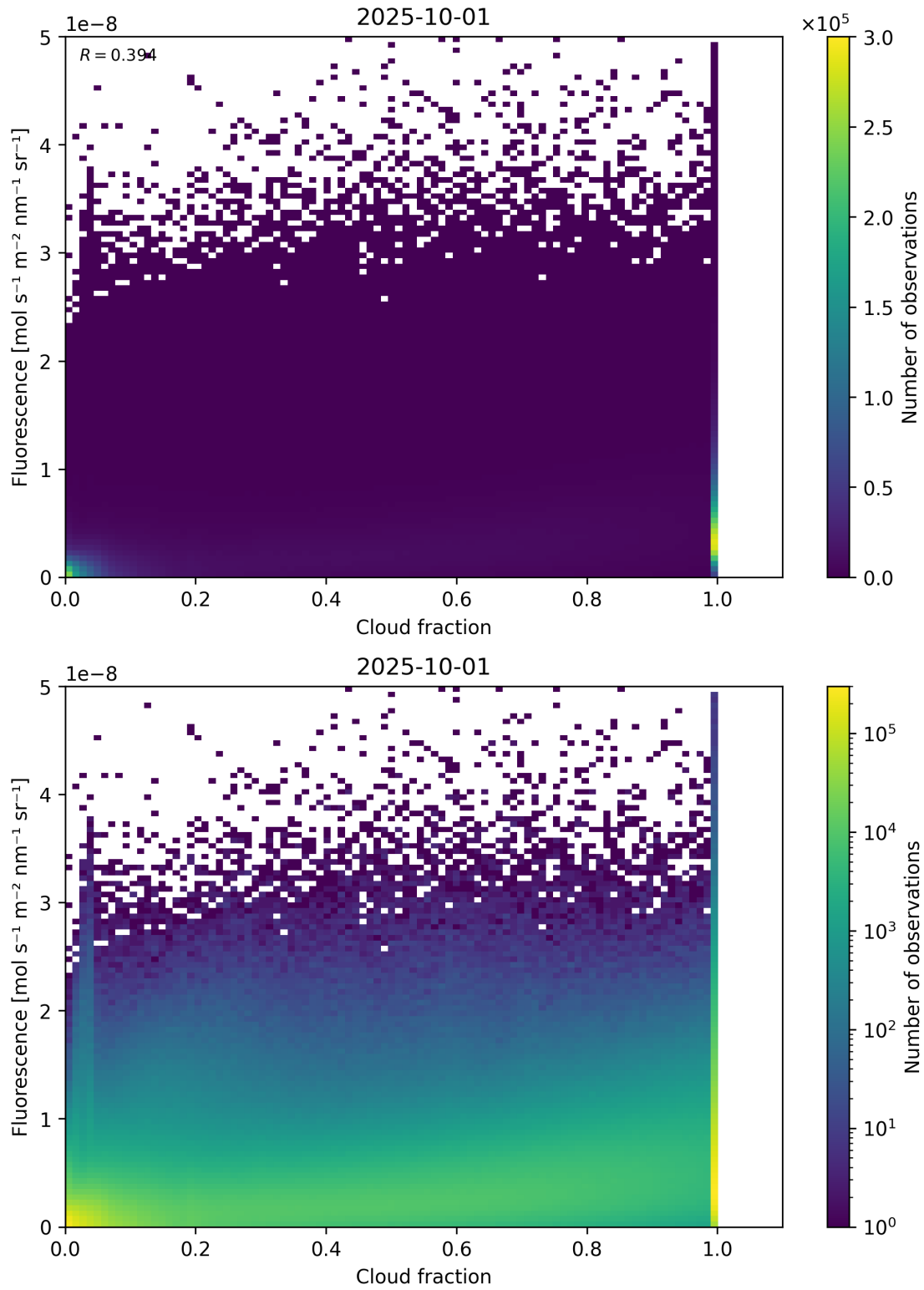
Figure 72: Scatter density plot of “Cloud fraction” against “Fluorescence” for 2025-10-01 to 2025-10-02.
