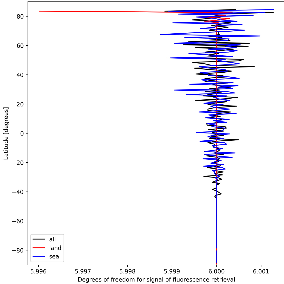
Figure 26: Zonal average of “Degrees of freedom for signal of fluorescence retrieval” for 2025-10-01 to 2025-10-02.
