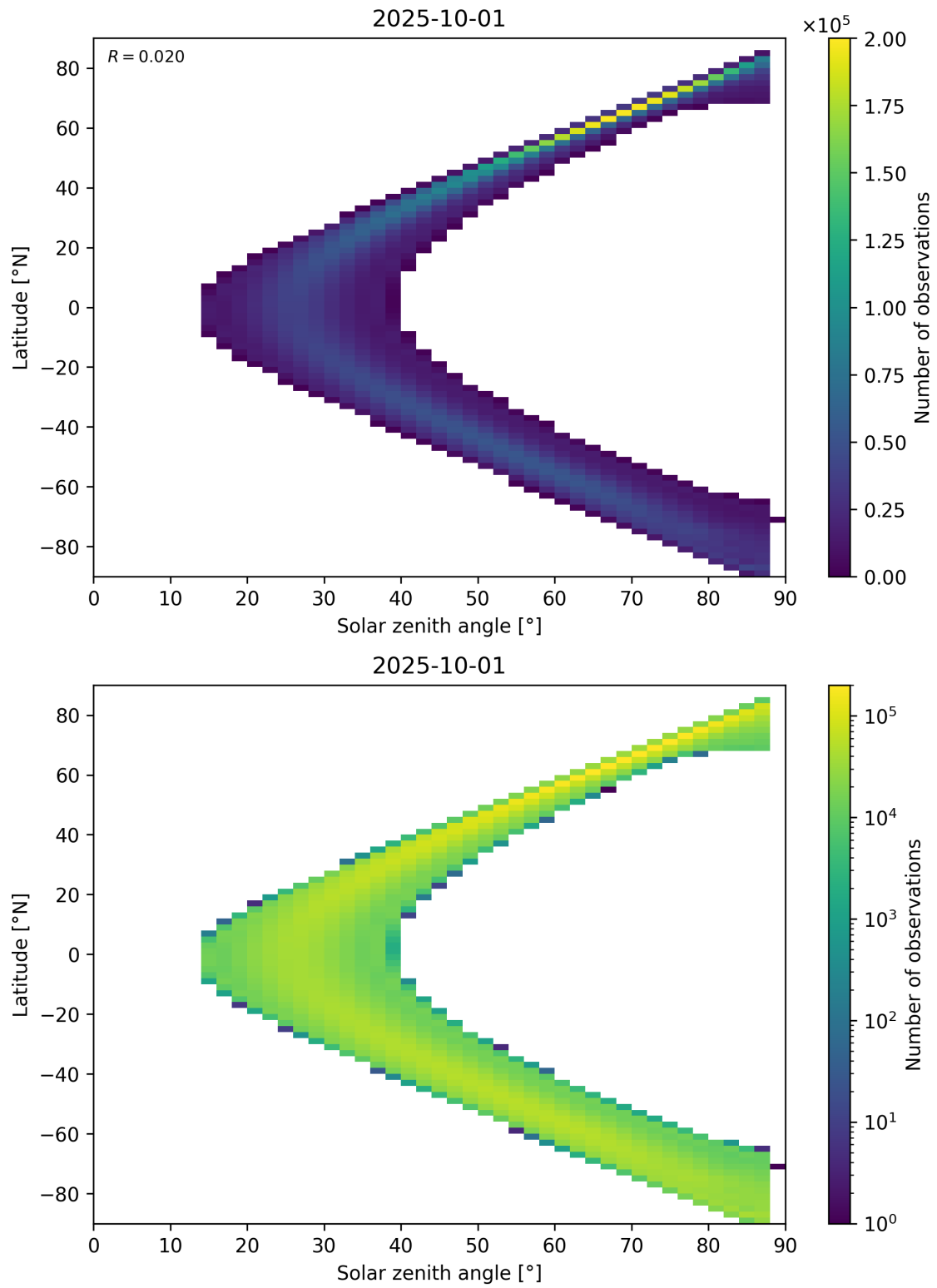
Figure 113: Scatter density plot of “Solar zenith angle” against “Latitude” for 2025-10-01 to 2025-10-02.
