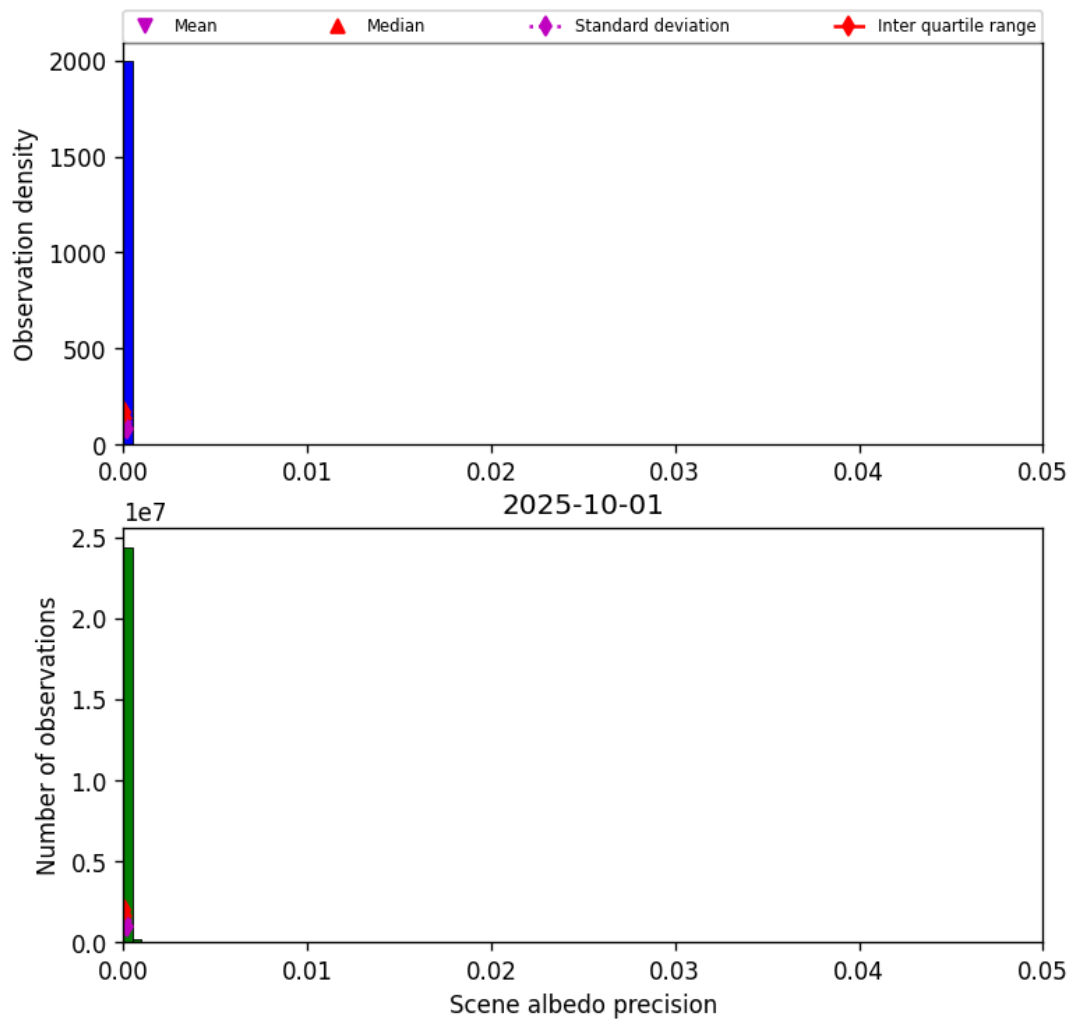
Figure 35: Histogram of “Scene albedo precision” for 2025-10-01 to 2025-10-02
