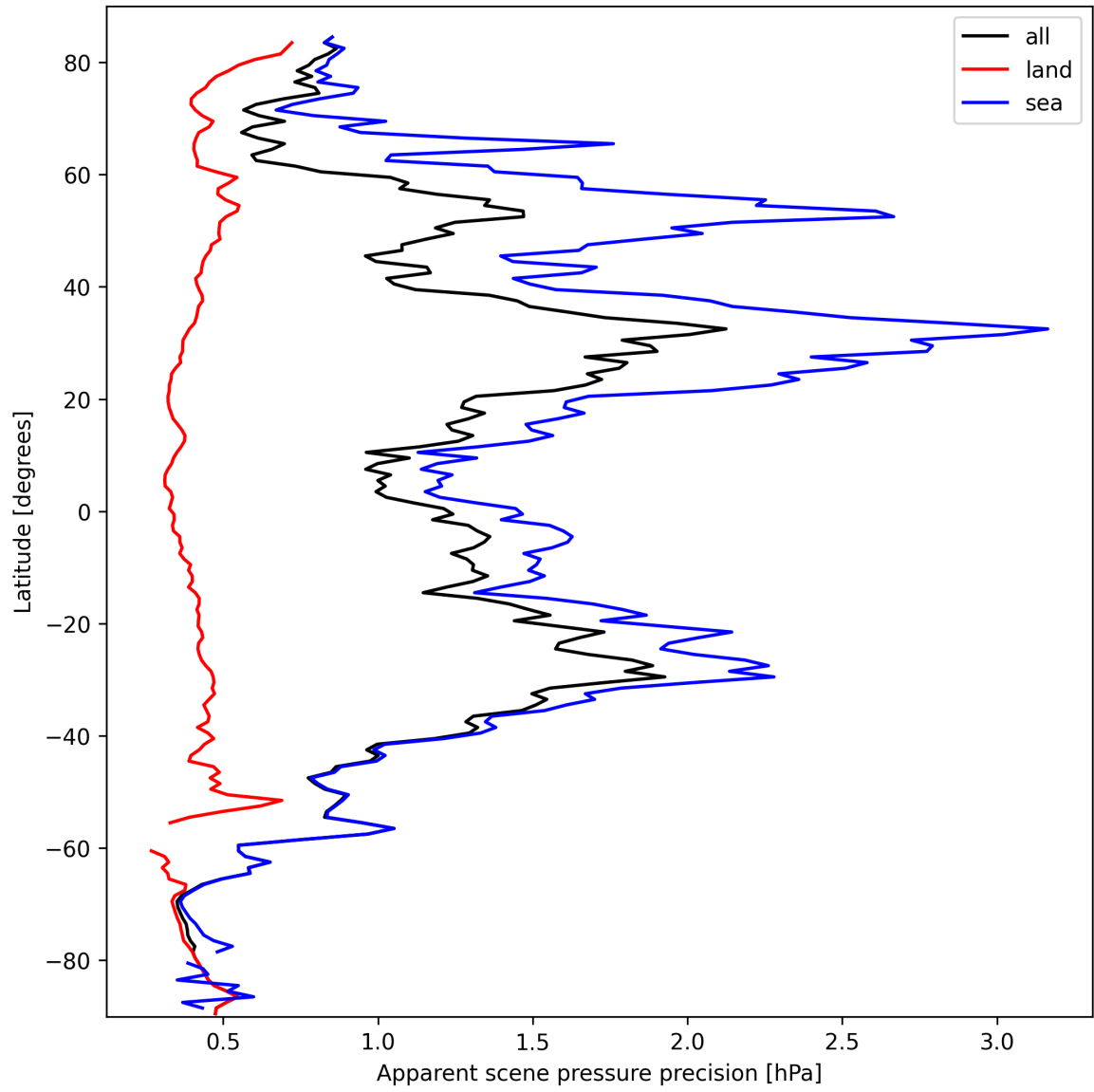
Figure 20: Zonal average of “Apparent scene pressure precision” for 2025-10-01 to 2025-10-02.
