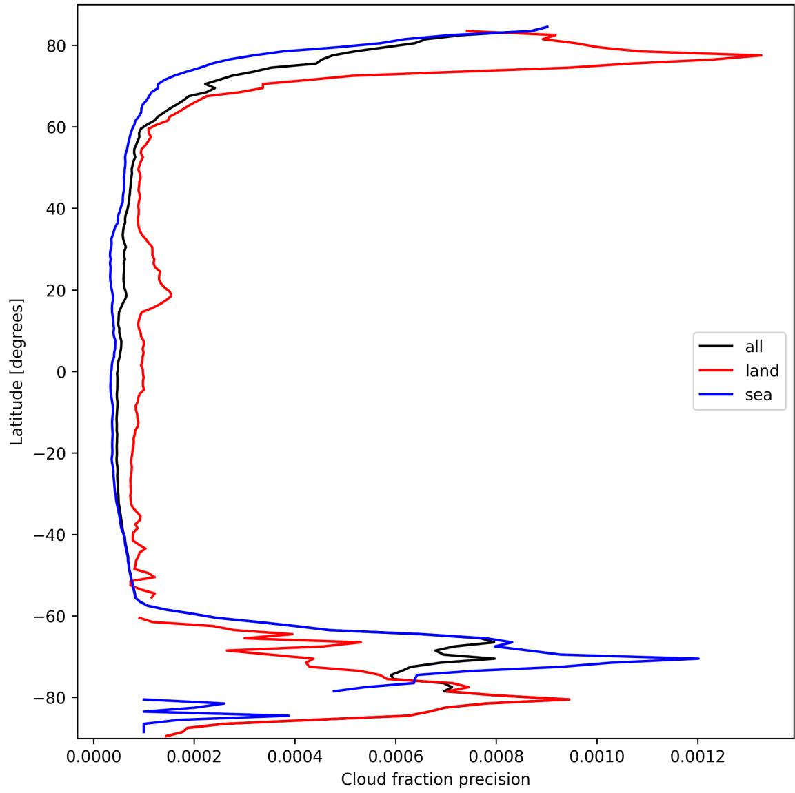
Figure 16: Zonal average of “Cloud fraction precision” for 2025-10-01 to 2025-10-02.
