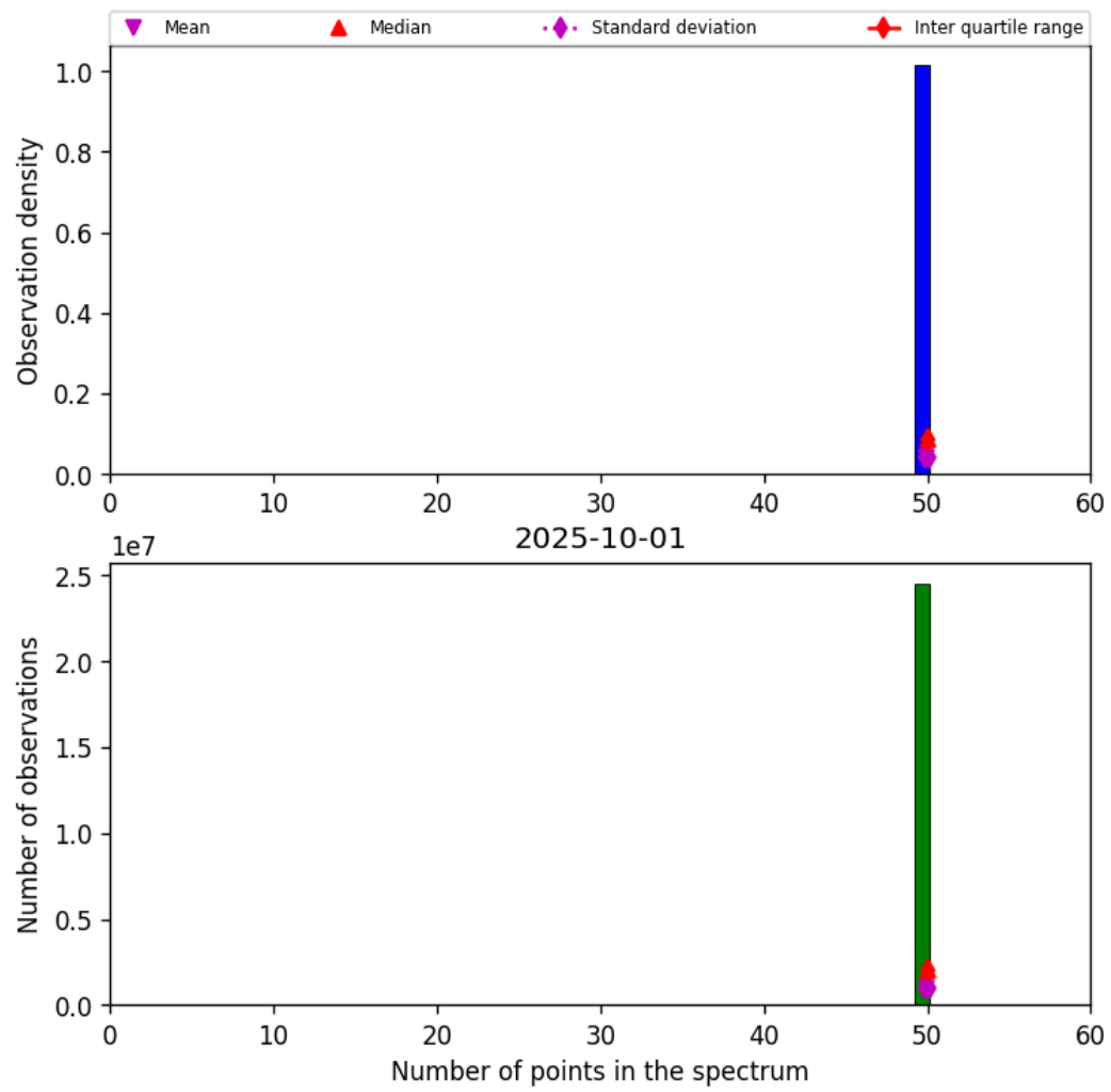
Figure 44: Histogram of “Number of points in the spectrum” for 2025-10-01 to 2025-10-02
