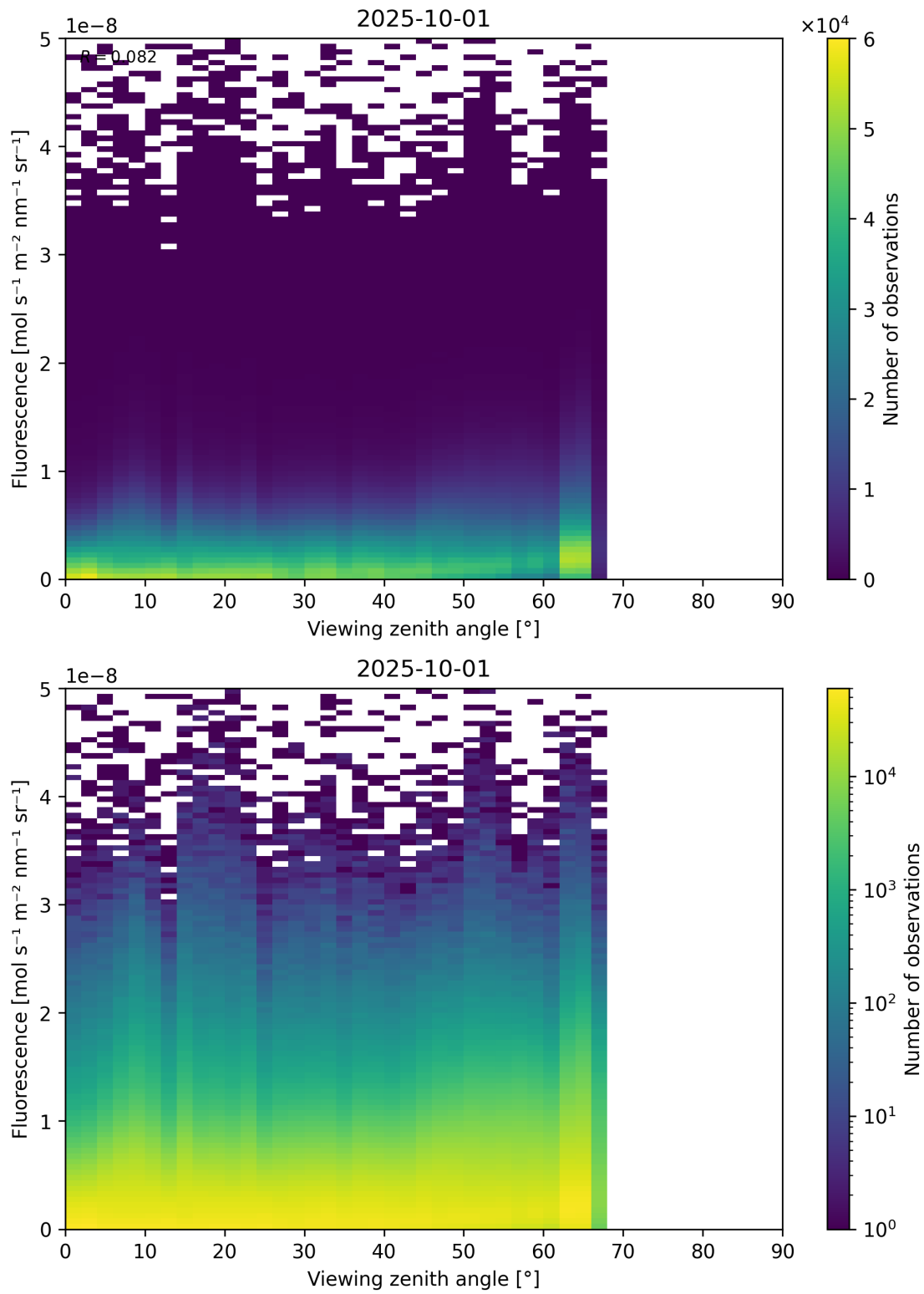
Figure 122: Scatter density plot of “Viewing zenith angle” against “Fluorescence” for 2025-10-01 to 2025-10-02.
