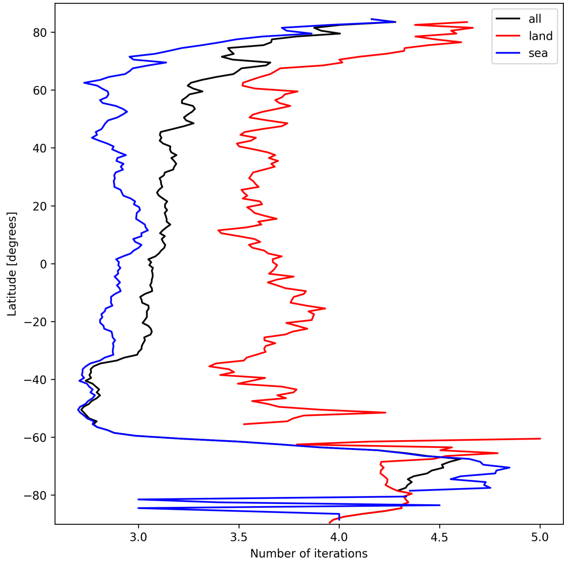
Figure 22: Zonal average of “Number of iterations” for 2025-10-01 to 2025-10-02.
