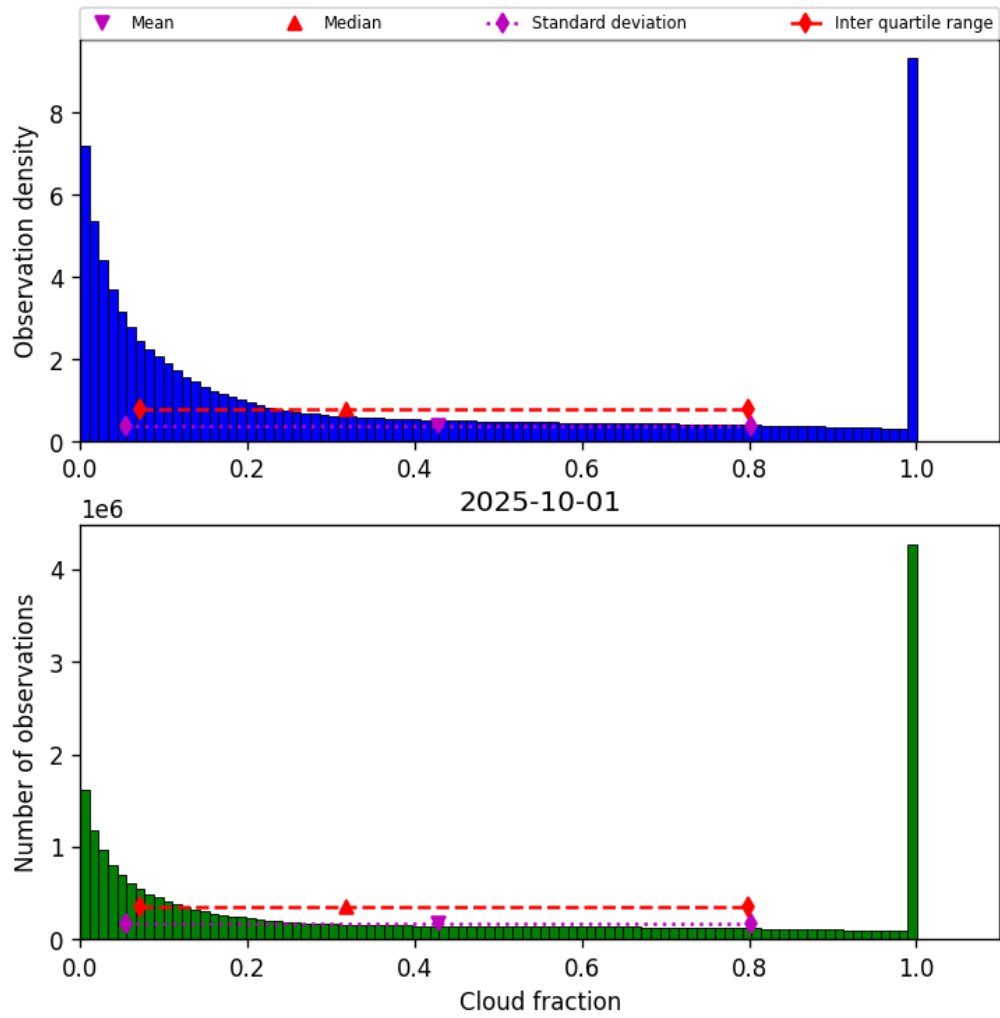
Figure 32: Histogram of “Cloud fraction” for 2025-10-01 to 2025-10-02
