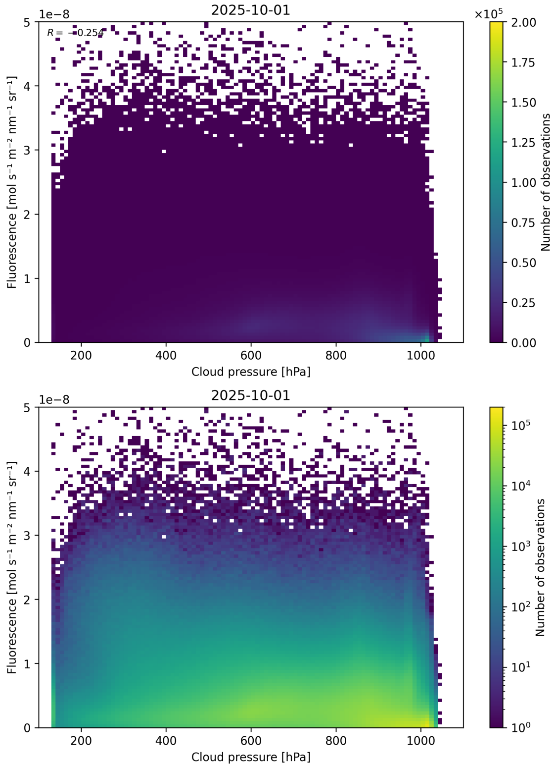
Figure 80: Scatter density plot of “Cloud pressure” against “Fluorescence” for 2025-10-01 to 2025-10-02.
