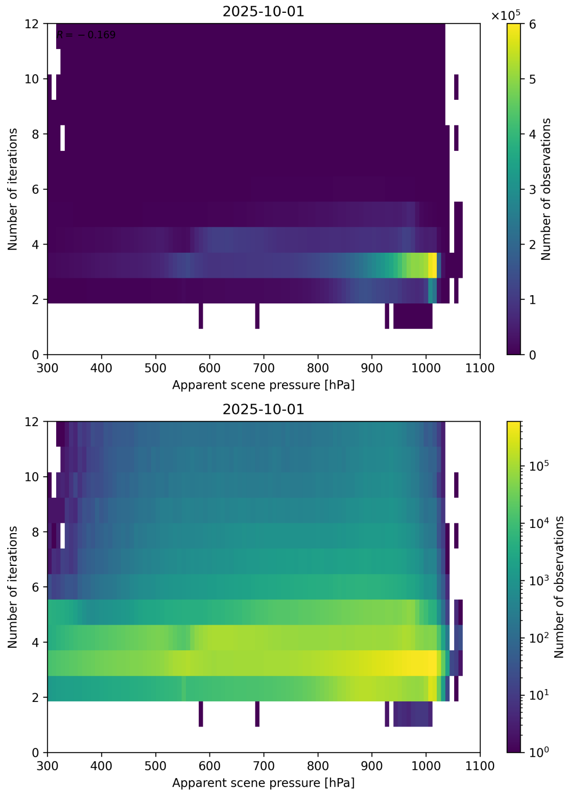
Figure 65: Scatter density plot of “Apparent scene pressure” against “Number of iterations” for 2025-10-01 to 2025-10-02.
