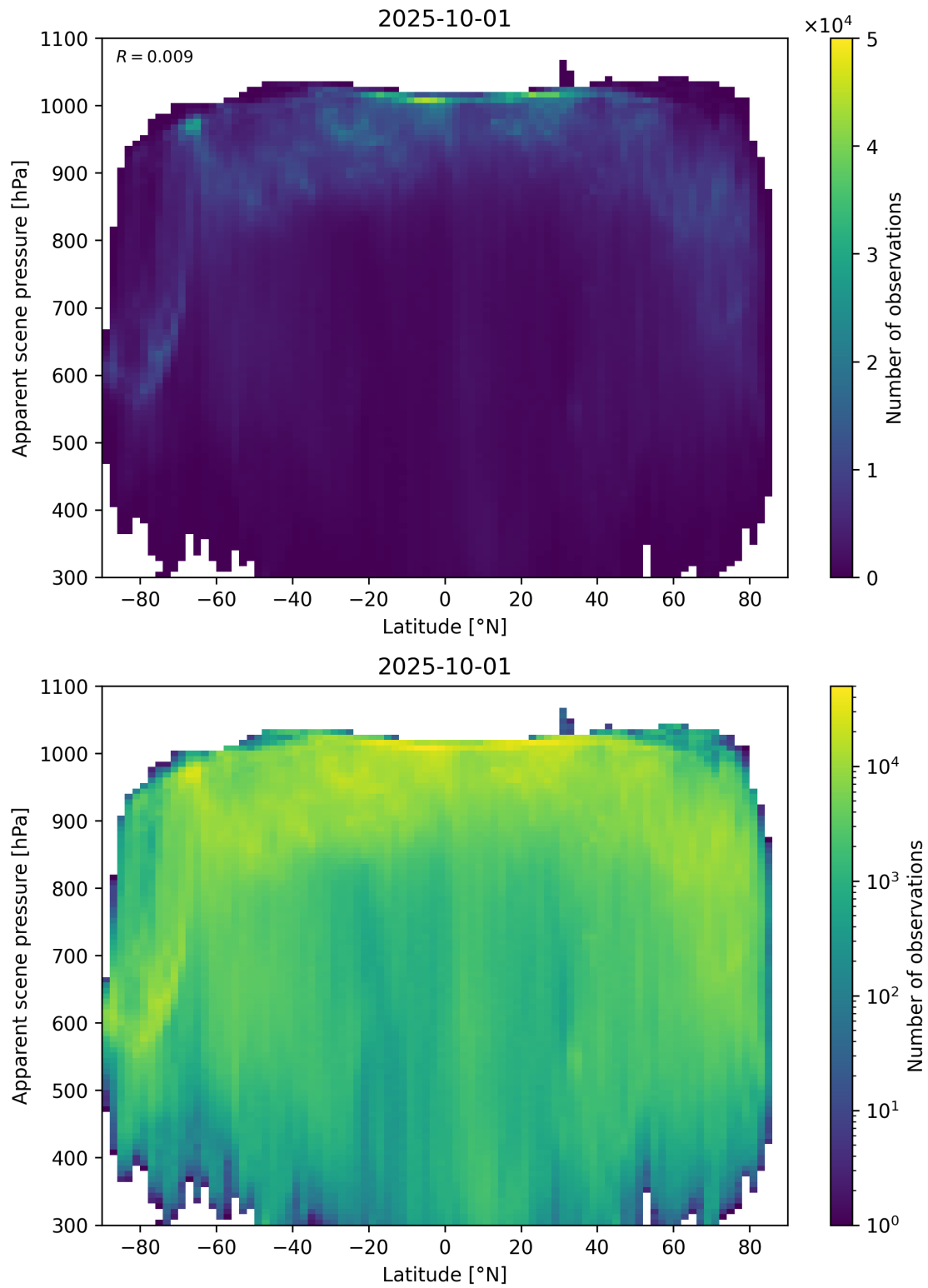
Figure 88: Scatter density plot of “Latitude” against “Apparent scene pressure” for 2025-10-01 to 2025-10-02.
