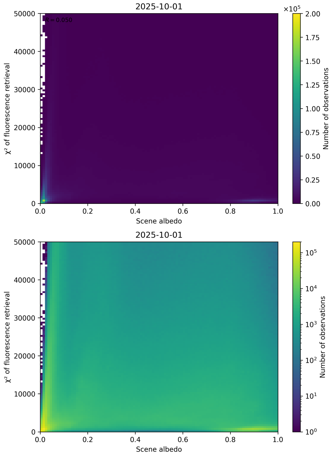
Figure 103: Scatter density plot of “Scene albedo” against “ \chi^2 of fluorescence retrieval” for 2025-10-01 to 2025-10-02.
