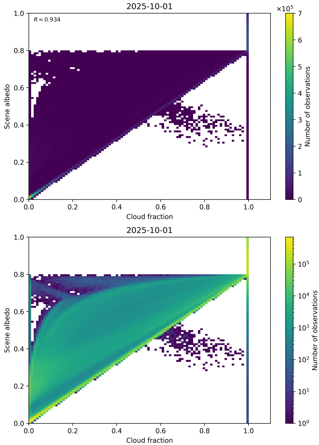
Figure 75: Scatter density plot of “Cloud fraction” against “Scene albedo” for 2025-10-01 to 2025-10-02.
