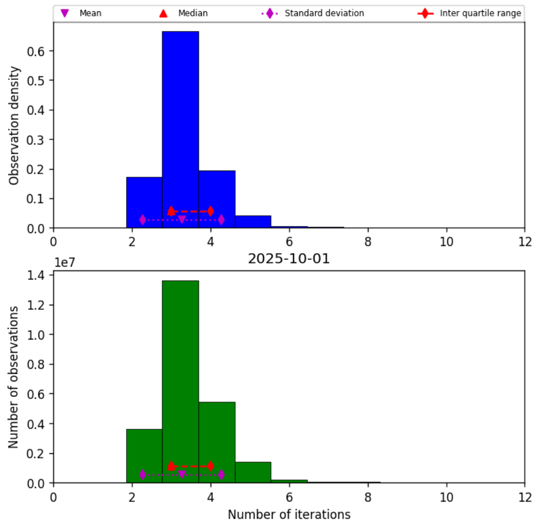
Figure 39: Histogram of “Number of iterations” for 2025-10-01 to 2025-10-02
