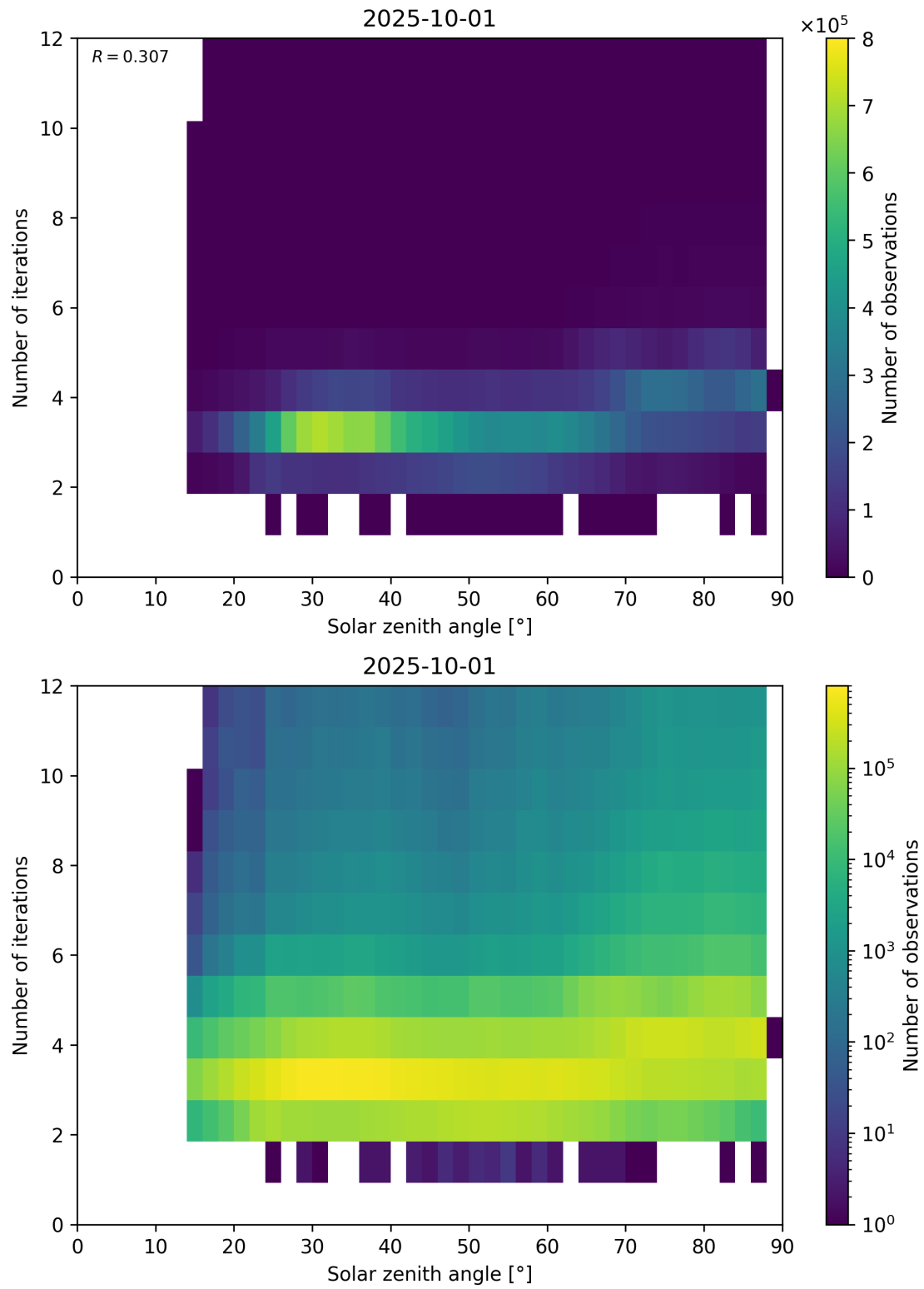
Figure 114: Scatter density plot of “Solar zenith angle” against “Number of iterations” for 2025-10-01 to 2025-10-02.
