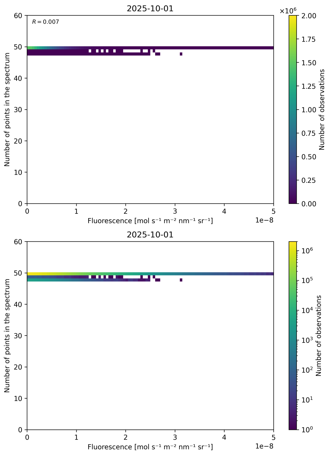
Figure 86: Scatter density plot of “Fluorescence” against “Number of points in the spectrum” for 2025-10-01 to 2025-10-02.
