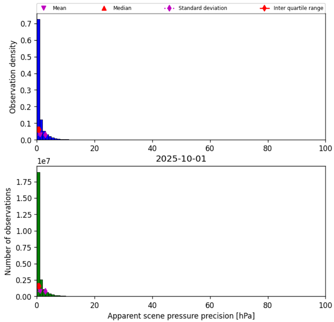
Figure 37: Histogram of “Apparent scene pressure precision” for 2025-10-01 to 2025-10-02
