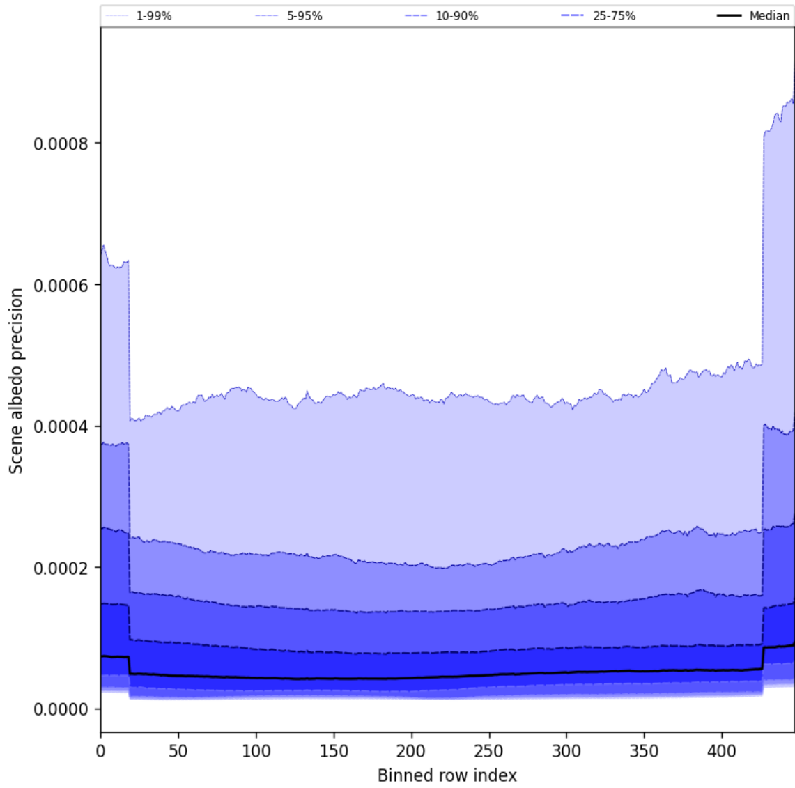
Figure 52: Along track statistics of “Scene albedo precision” for 2025-10-01 to 2025-10-02
