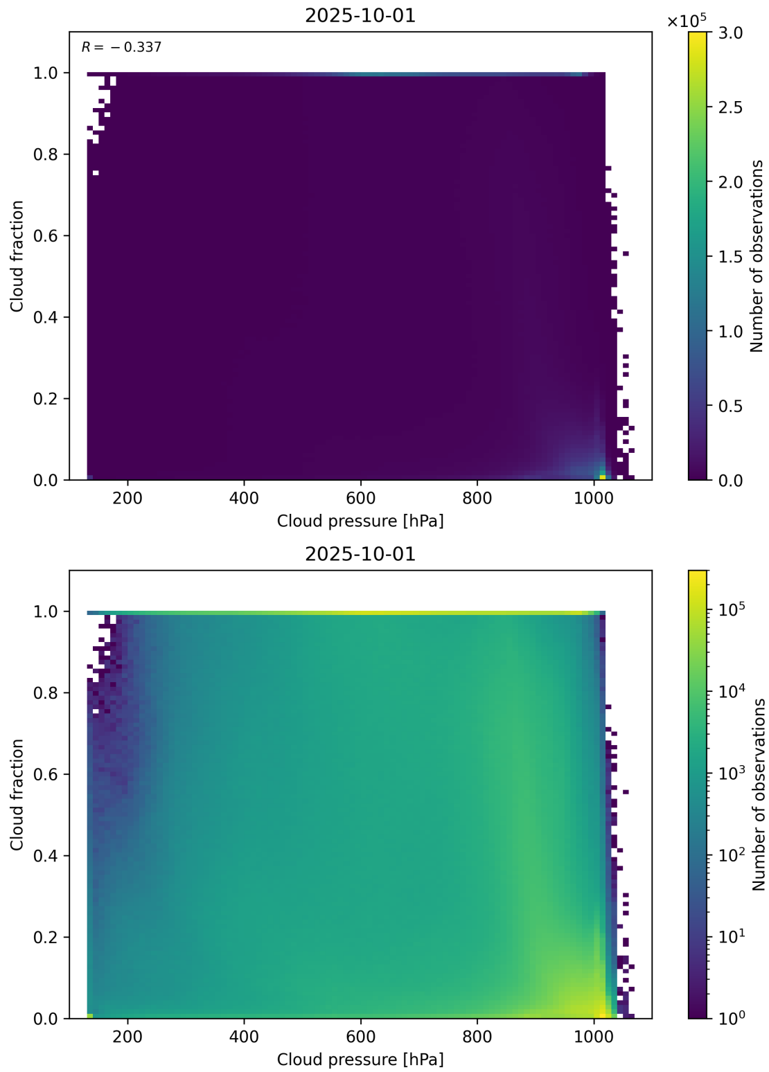
Figure 79: Scatter density plot of “Cloud pressure” against “Cloud fraction” for 2025-10-01 to 2025-10-02.
