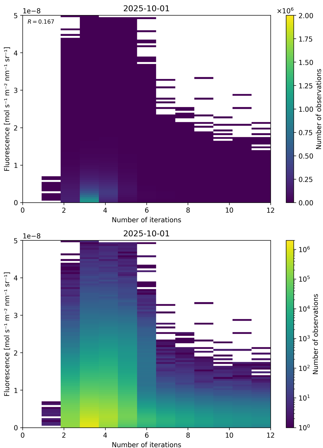
Figure 98: Scatter density plot of “Number of iterations” against “Fluorescence” for 2025-10-01 to 2025-10-02.
