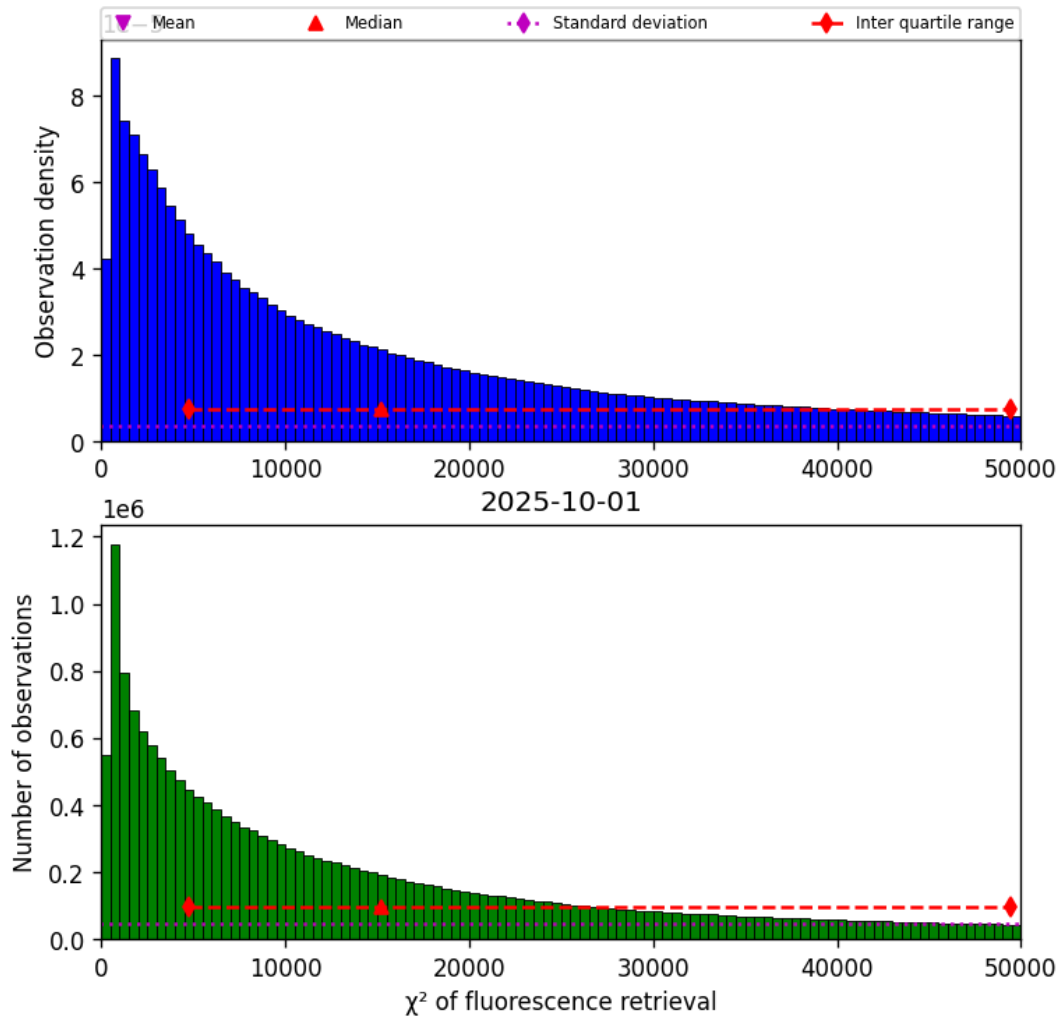
Figure 42: Histogram of “ \chi^2 of fluorescence retrieval” for 2025-10-01 to 2025-10-02
