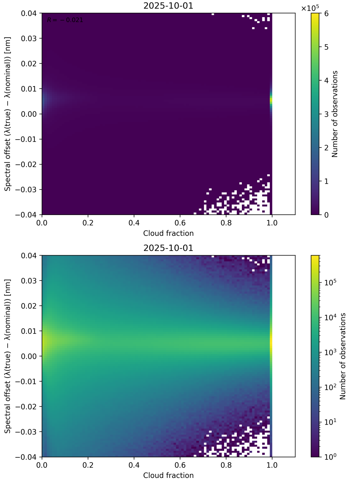
Figure 76: Scatter density plot of “Cloud fraction” against “Spectral offset ( \lambda_{\text{true}} - \lambda_{\text{nominal}} )” for 2025-10-01 to 2025-10-02.
