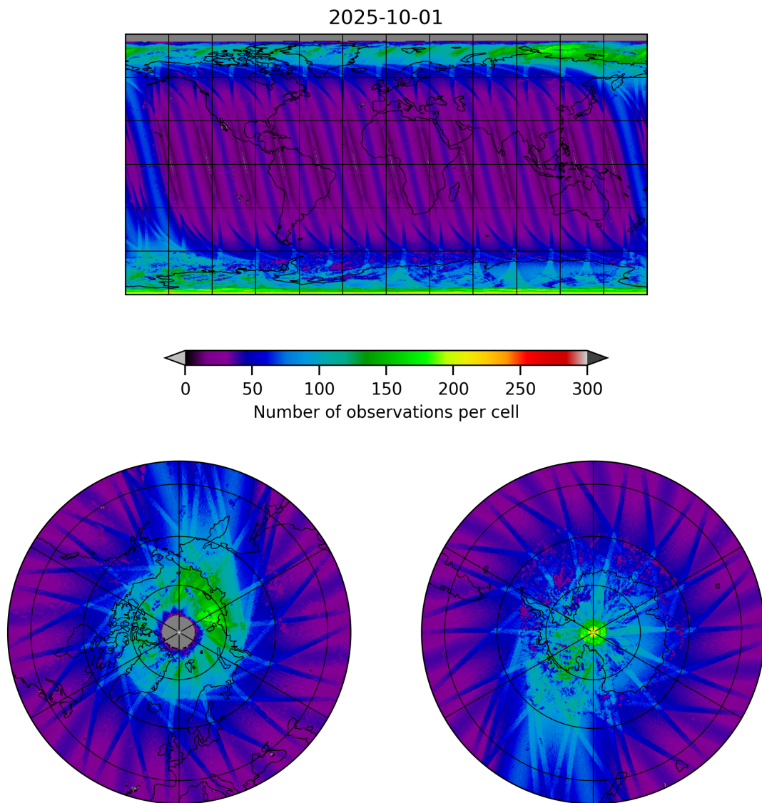
Figure 11: Map of the number of observations for 2025-10-01 to 2025-10-02
