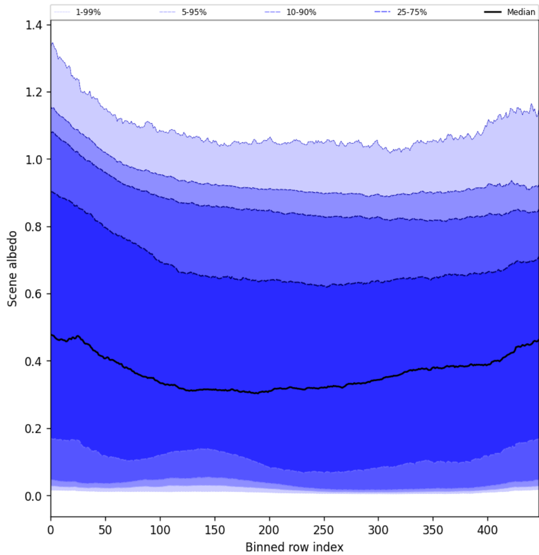
Figure 51: Along track statistics of “Scene albedo” for 2025-10-01 to 2025-10-02
