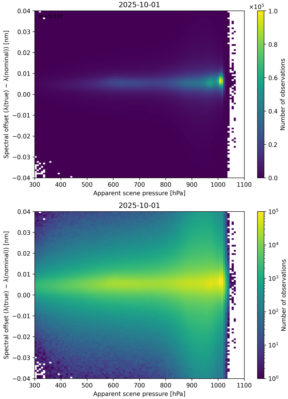
Figure 67: Scatter density plot of “Apparent scene pressure” against “Spectral offset ( \lambda_{\text{true}} - \lambda_{\text{nominal}} )” for 2025-10-01 to 2025-10-02.
