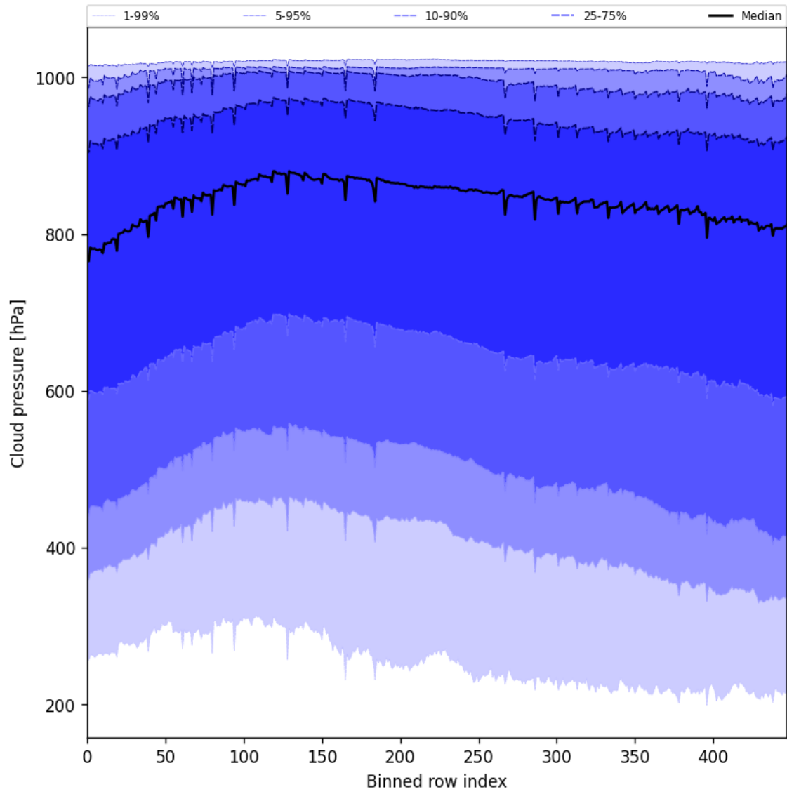
Figure 47: Along track statistics of “Cloud pressure” for 2025-10-01 to 2025-10-02
