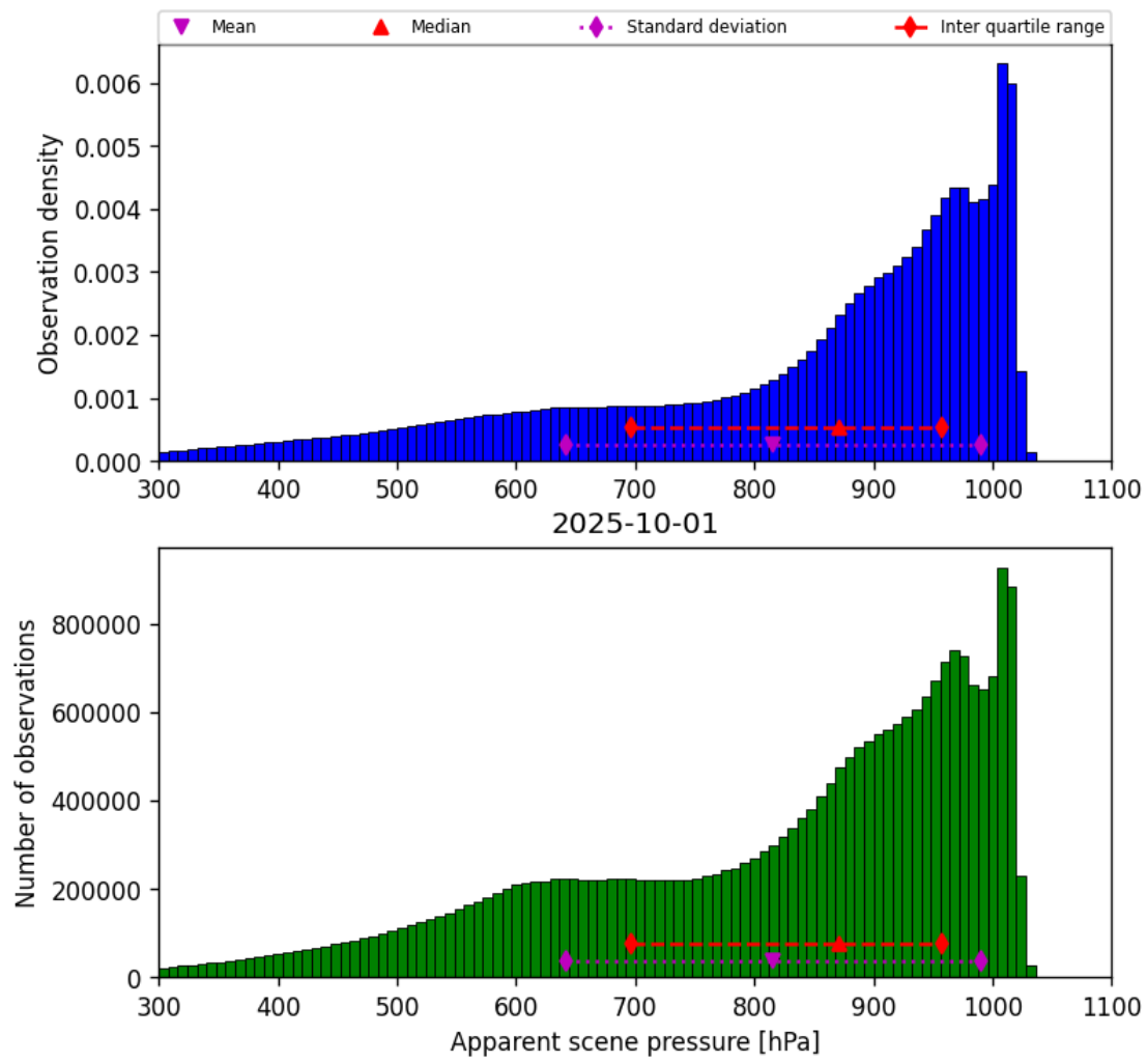
Figure 36: Histogram of “Apparent scene pressure” for 2025-10-01 to 2025-10-02
