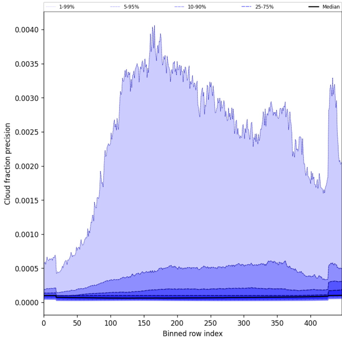
Figure 50: Along track statistics of “Cloud fraction precision” for 2025-10-01 to 2025-10-02
