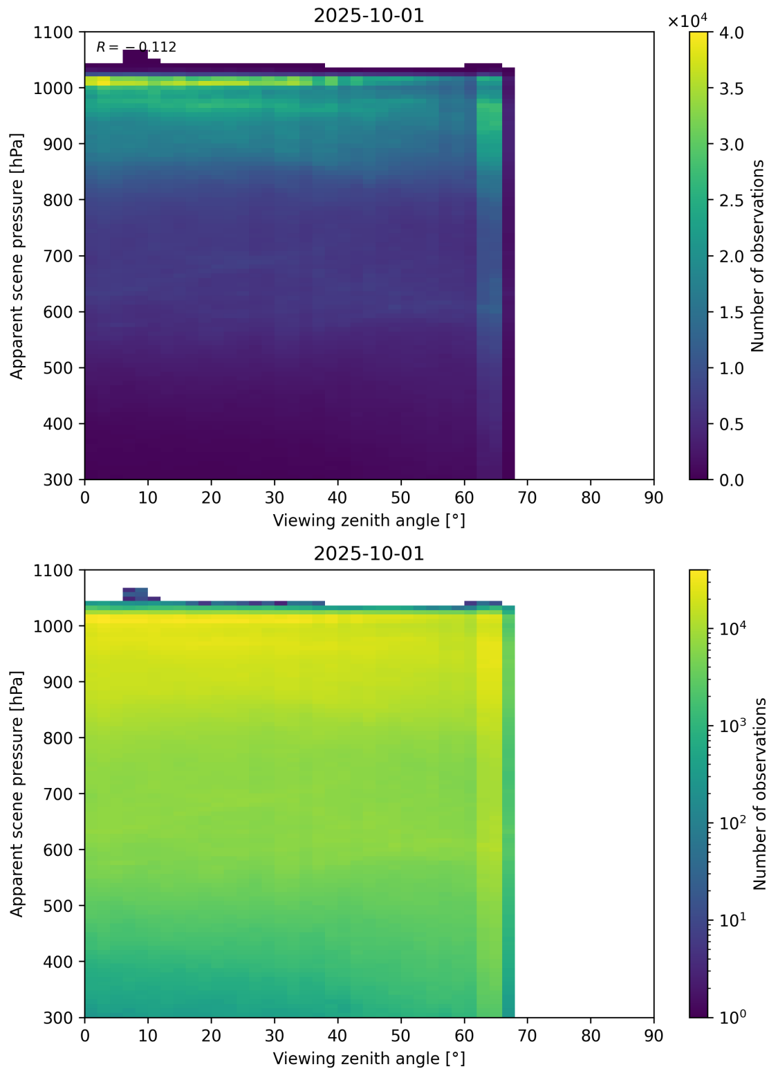
Figure 118: Scatter density plot of “Viewing zenith angle” against “Apparent scene pressure” for 2025-10-01 to 2025-10-02.
