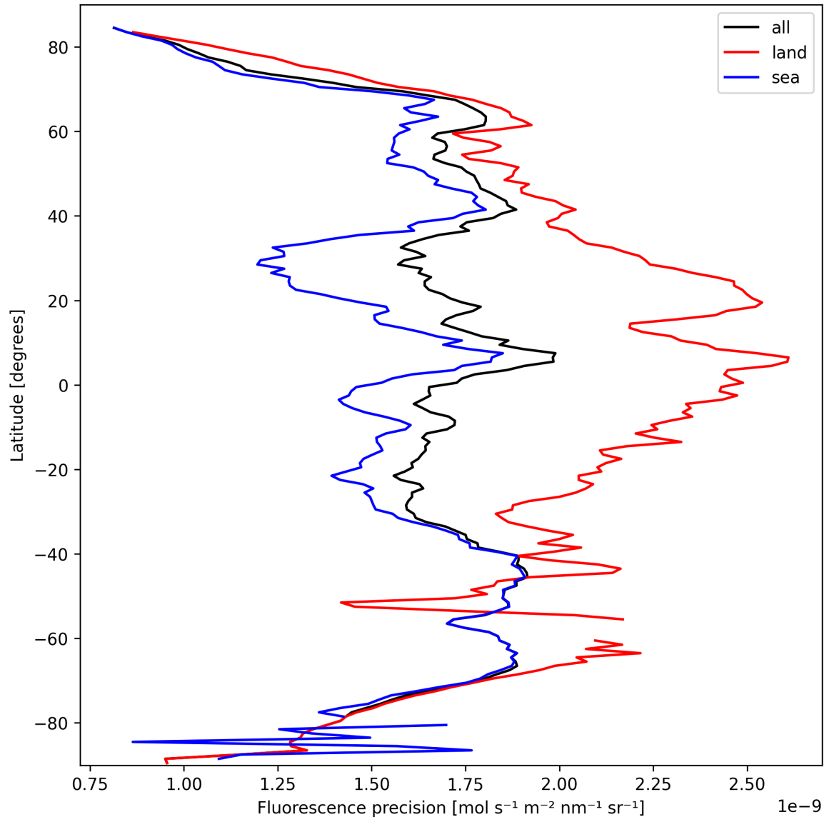
Figure 24: Zonal average of “Fluorescence precision” for 2025-10-01 to 2025-10-02.
