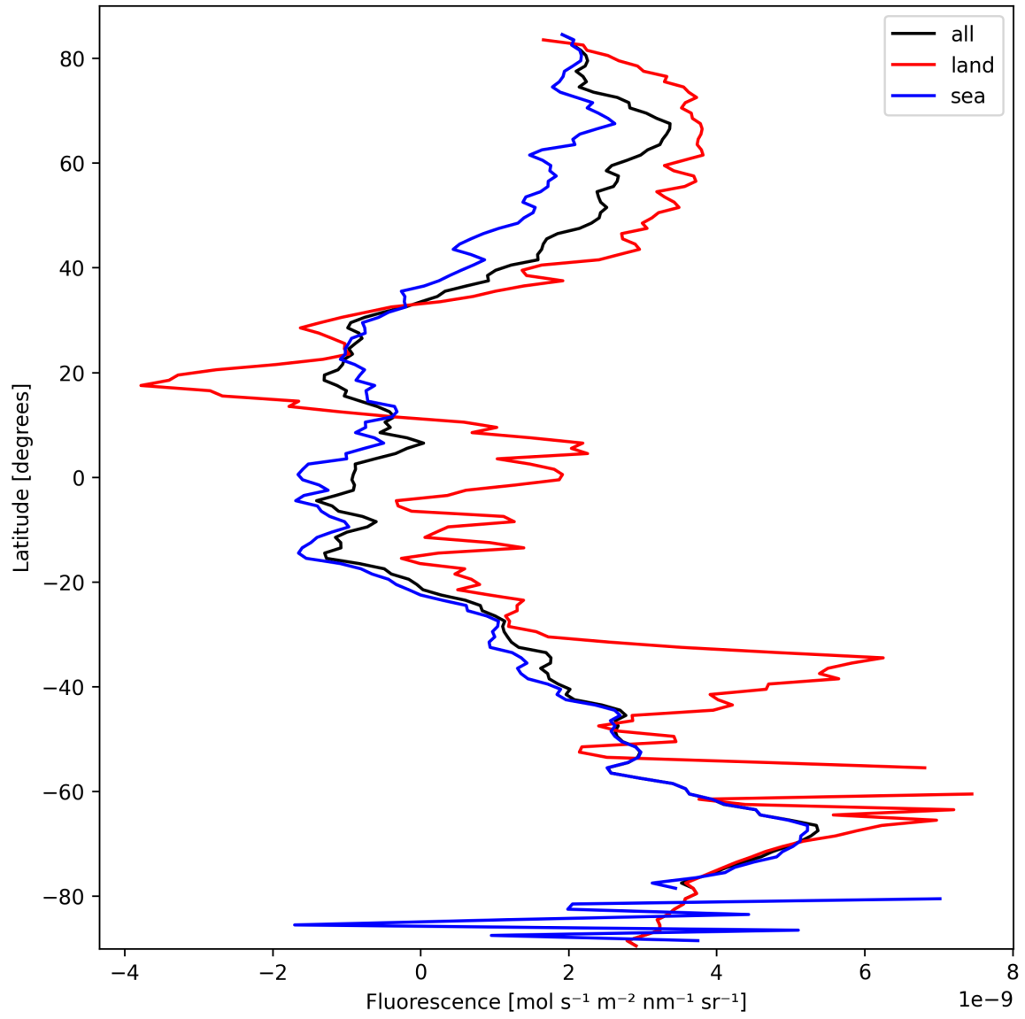
Figure 23: Zonal average of “Fluorescence” for 2025-10-01 to 2025-10-02.
