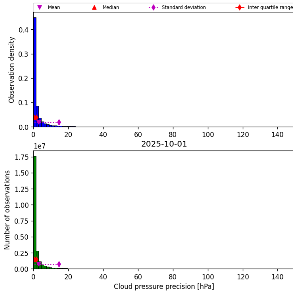
Figure 31: Histogram of “Cloud pressure precision” for 2025-10-01 to 2025-10-02
