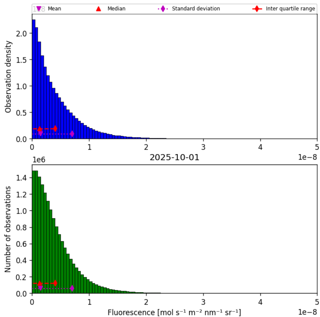
Figure 40: Histogram of “Fluorescence” for 2025-10-01 to 2025-10-02
