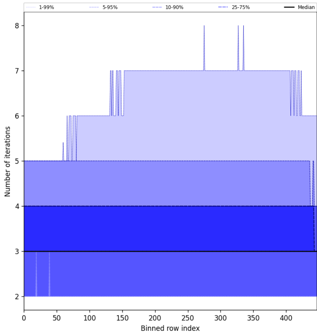
Figure 56: Along track statistics of “Number of iterations” for 2025-10-01 to 2025-10-02
