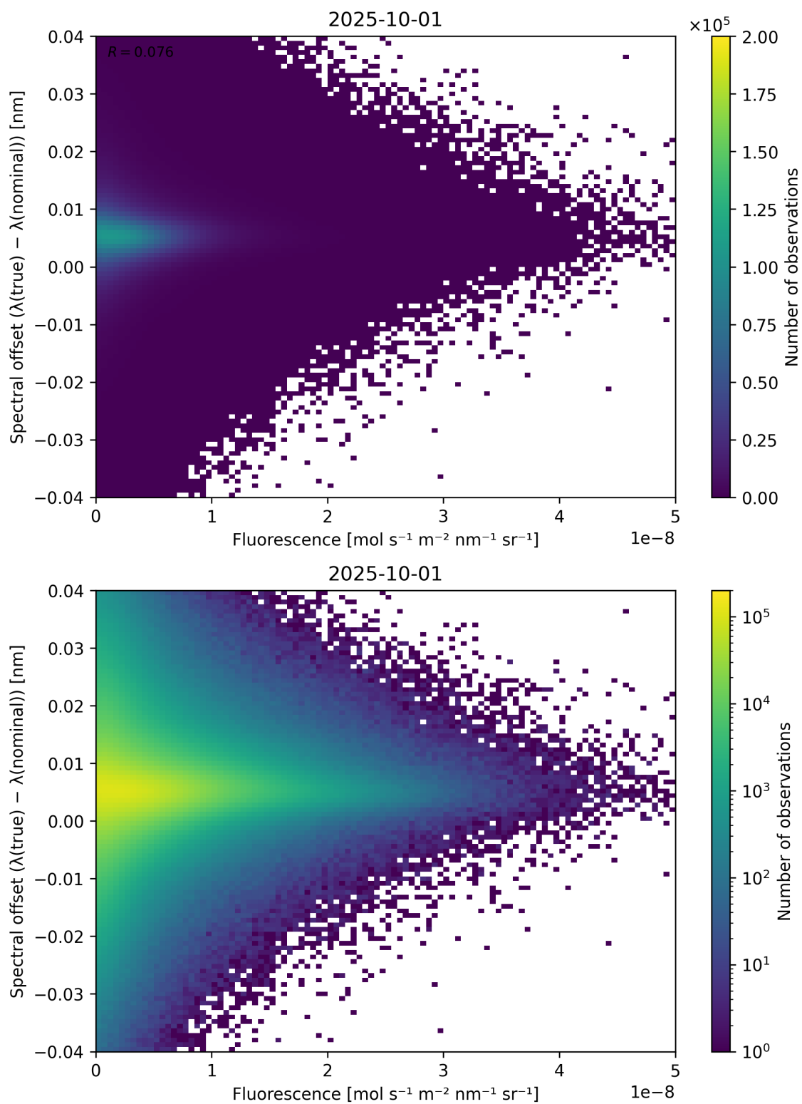
Figure 87: Scatter density plot of “Fluorescence” against “Spectral offset ( \lambda_{\text{true}} - \lambda_{\text{nominal}} )” for 2025-10-01 to 2025-10-02.
