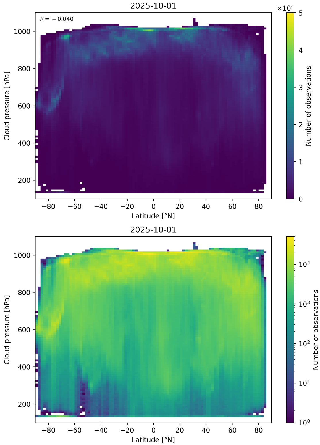
Figure 91: Scatter density plot of “Latitude” against “Cloud pressure” for 2025-10-01 to 2025-10-02.
