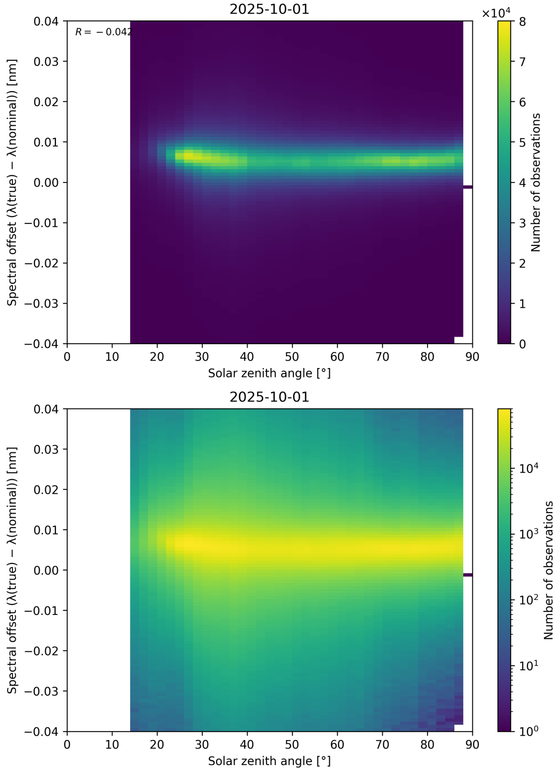
Figure 117: Scatter density plot of “Solar zenith angle” against “Spectral offset ( \lambda_{\text{true}} - \lambda_{\text{nominal}} )” for 2025-10-01 to 2025-10-02.
