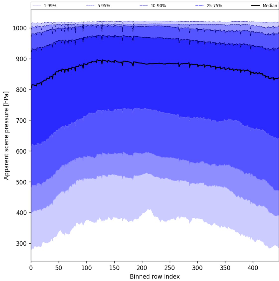
Figure 53: Along track statistics of “Apparent scene pressure” for 2025-10-01 to 2025-10-02
