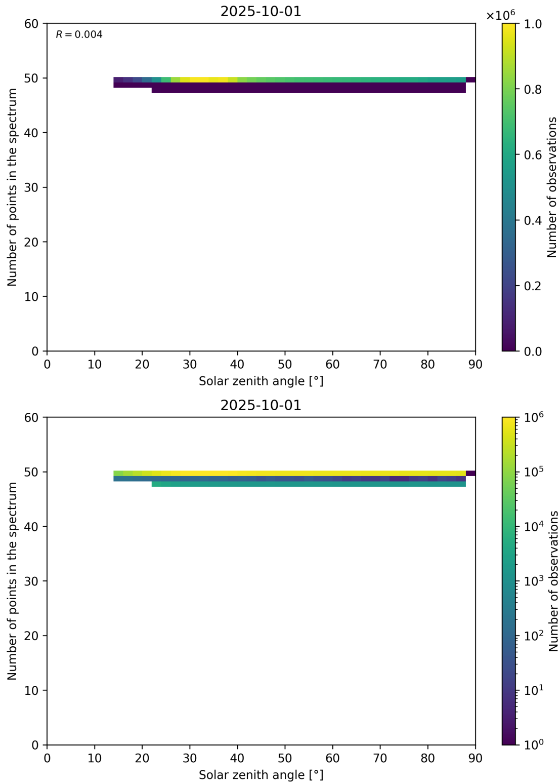
Figure 115: Scatter density plot of “Solar zenith angle” against “Number of points in the spectrum” for 2025-10-01 to 2025-10-02.
