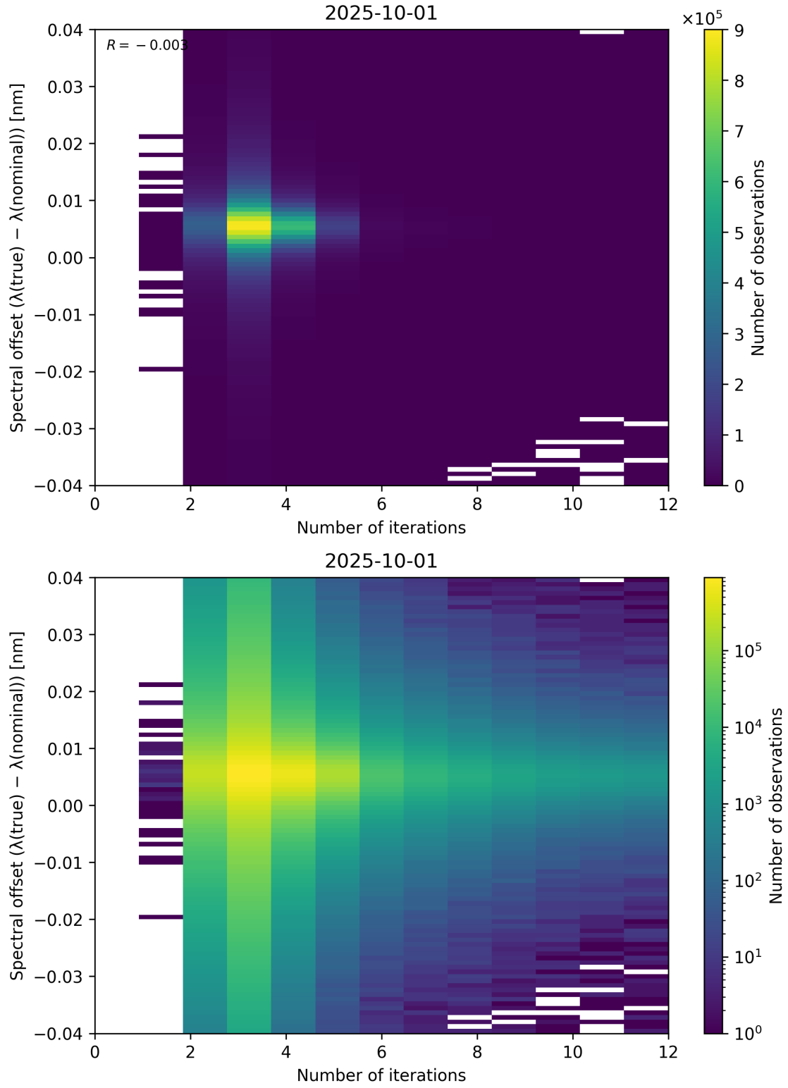
Figure 100: Scatter density plot of “Number of iterations” against “Spectral offset ( \lambda_{\text{true}} - \lambda_{\text{nominal}} )” for 2025-10-01 to 2025-10-02.
