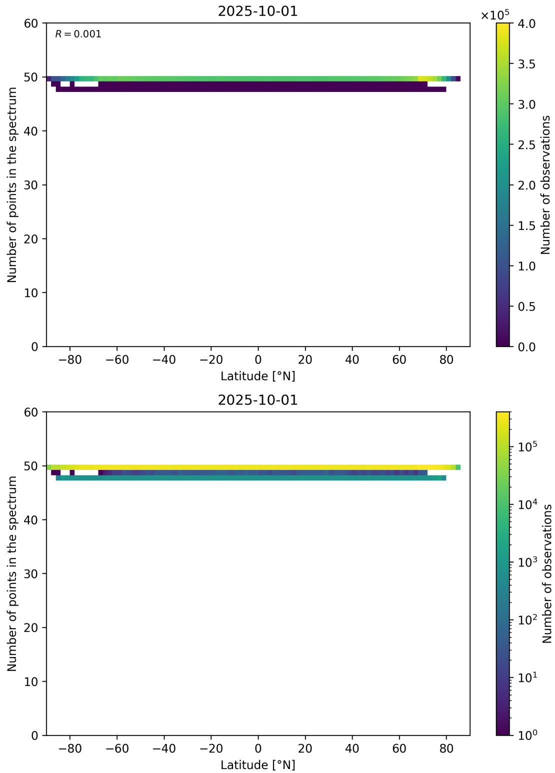
Figure 94: Scatter density plot of “Latitude” against “Number of points in the spectrum” for 2025-10-01 to 2025-10-02.
