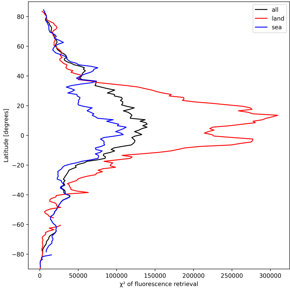
Figure 25: Zonal average of “ \chi^2 of fluorescence retrieval” for 2025-10-01 to 2025-10-02.
