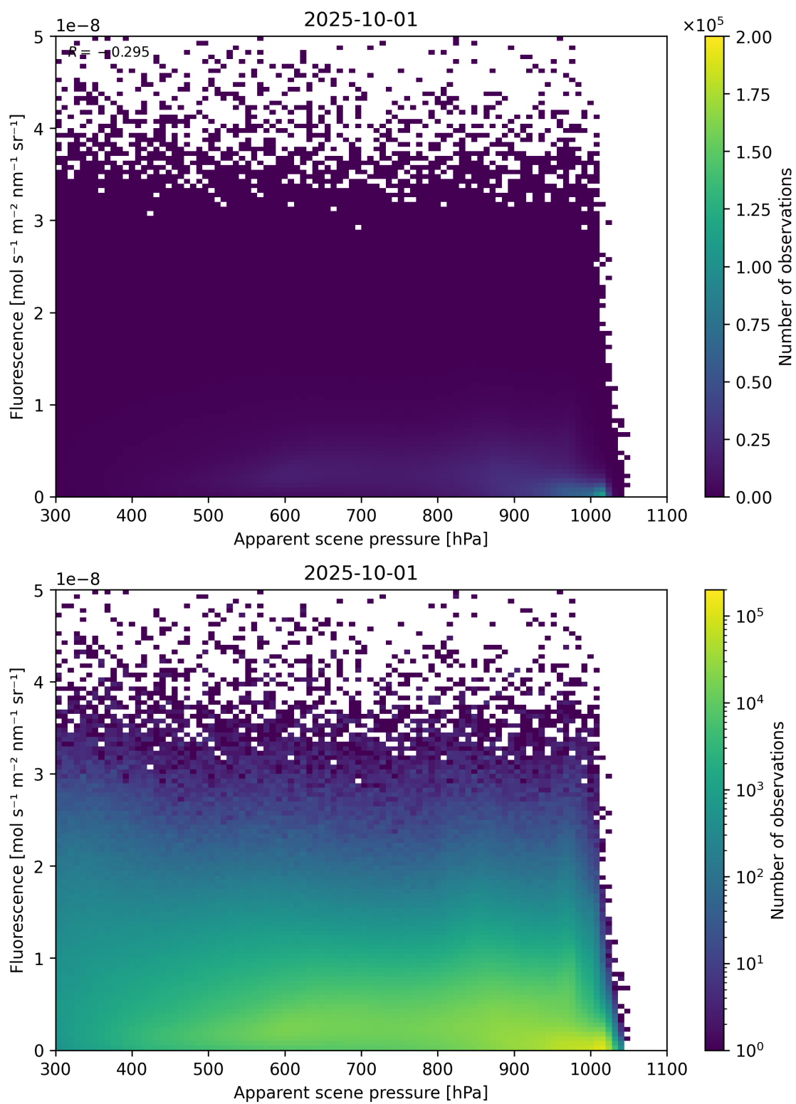
Figure 64: Scatter density plot of “Apparent scene pressure” against “Fluorescence” for 2025-10-01 to 2025-10-02.
