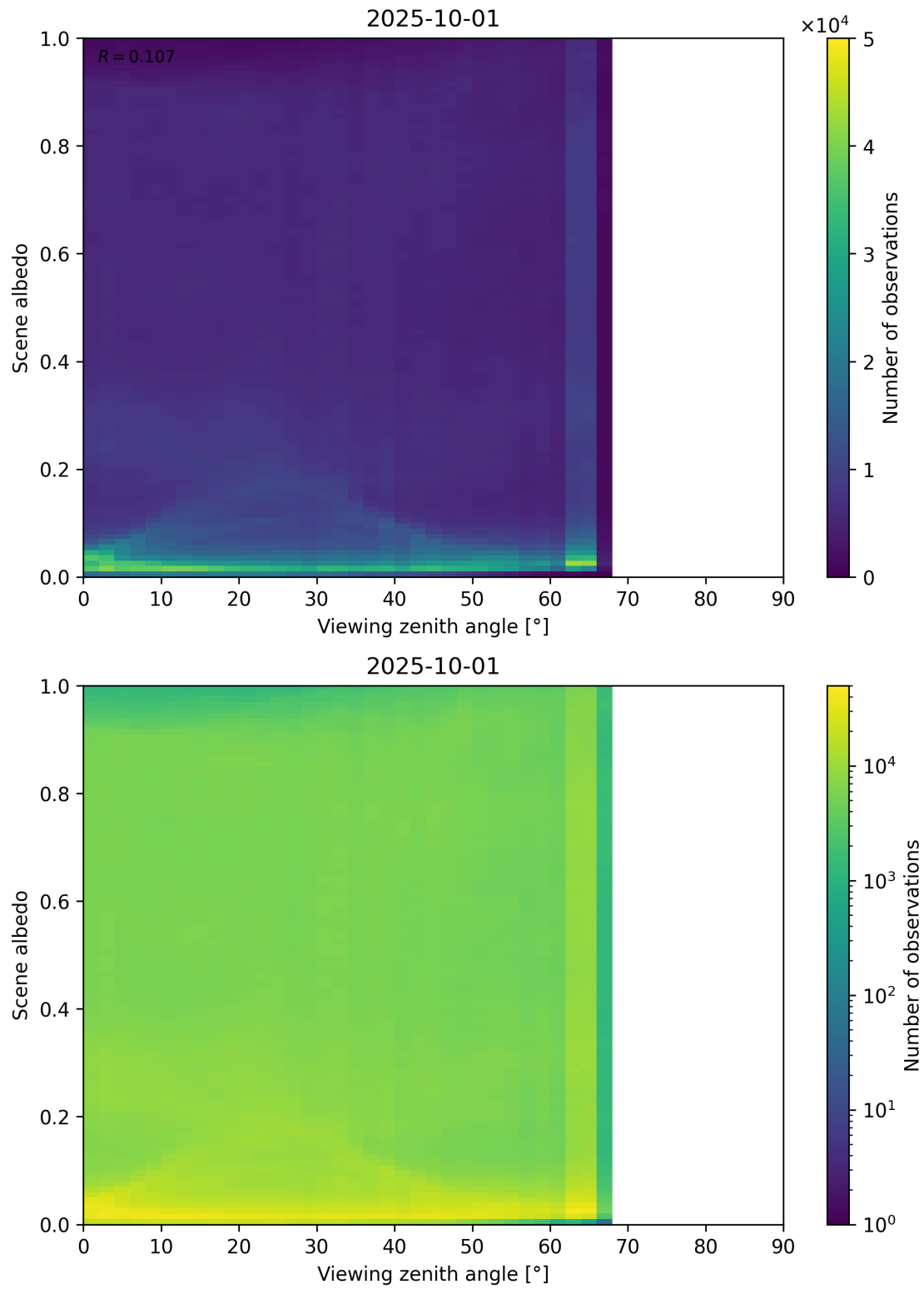
Figure 126: Scatter density plot of “Viewing zenith angle” against “Scene albedo” for 2025-10-01 to 2025-10-02.
