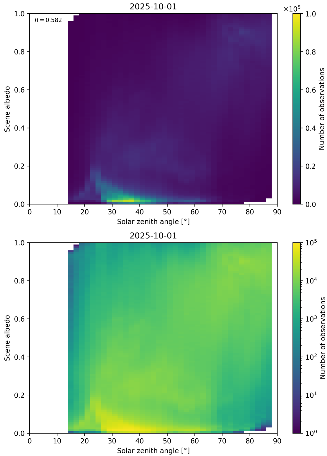
Figure 116: Scatter density plot of “Solar zenith angle” against “Scene albedo” for 2025-10-01 to 2025-10-02.
