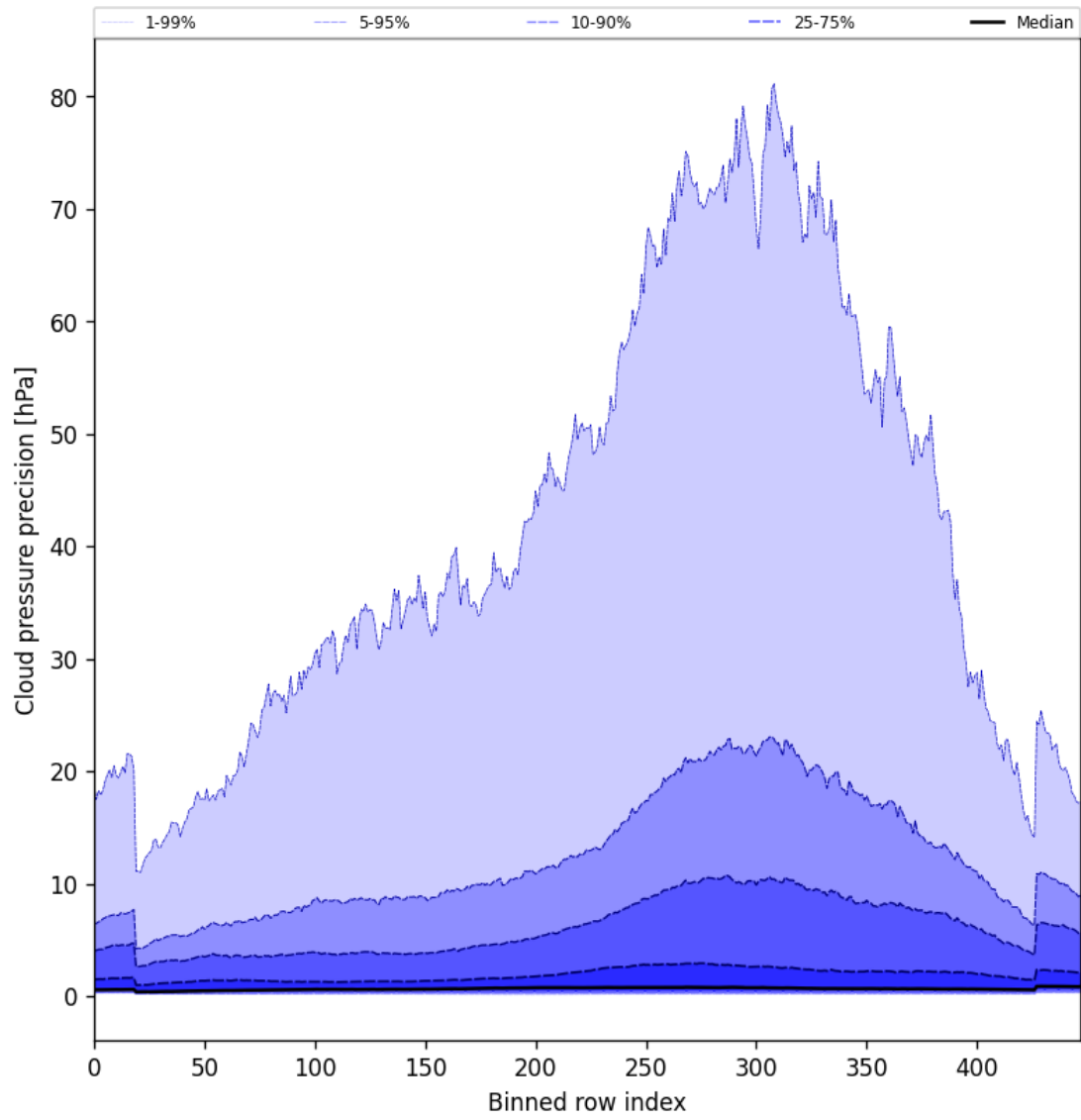
Figure 48: Along track statistics of “Cloud pressure precision” for 2025-10-01 to 2025-10-02
