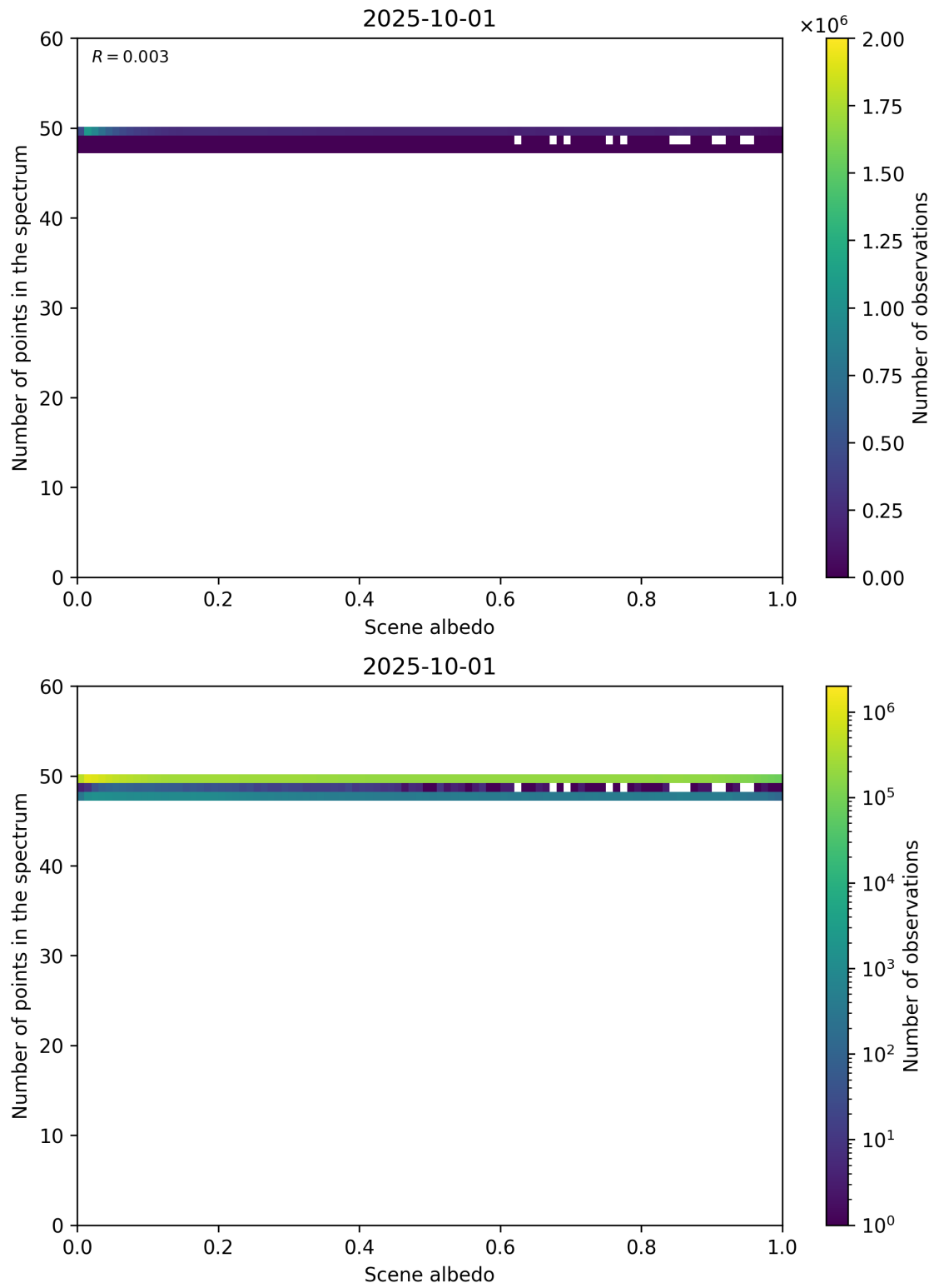
Figure 106: Scatter density plot of “Scene albedo” against “Number of points in the spectrum” for 2025-10-01 to 2025-10-02.
