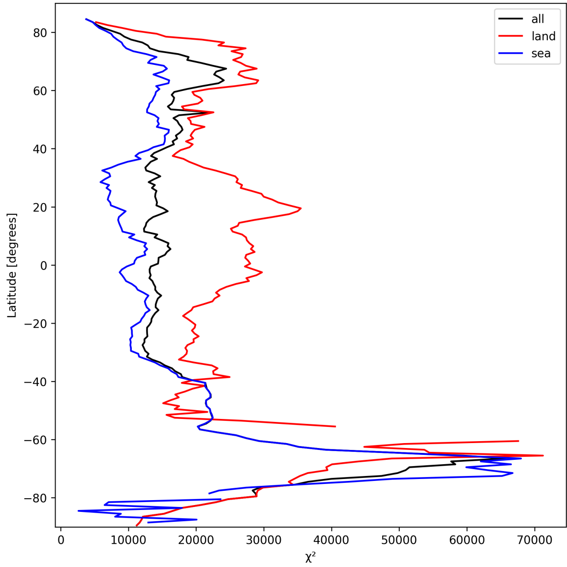
Figure 21: Zonal average of “ \chi^2 ” for 2025-10-01 to 2025-10-02.
