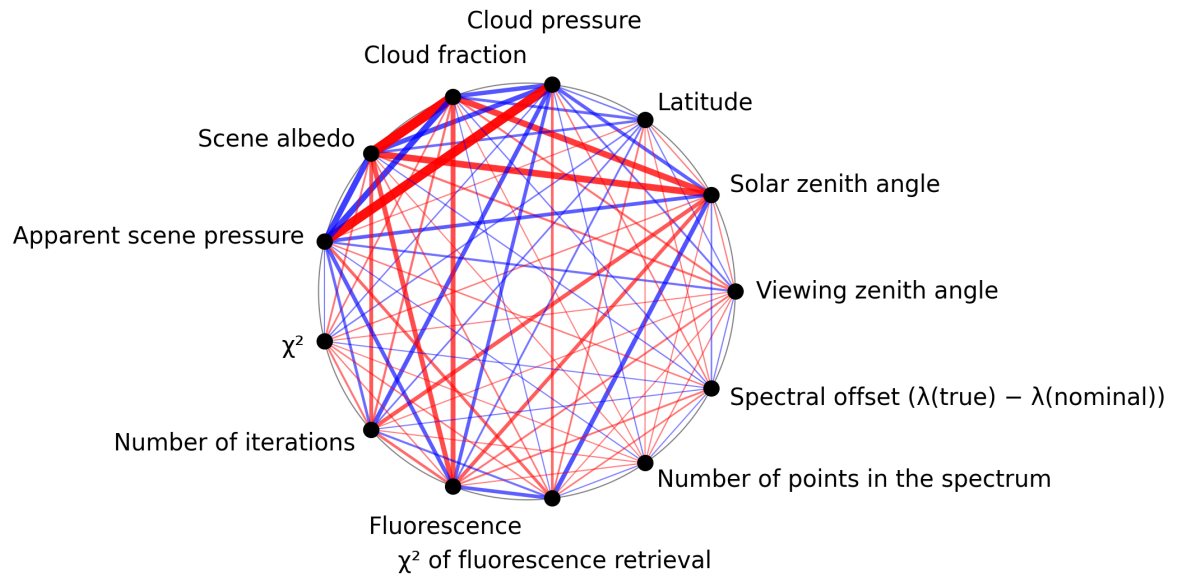
Figure 1: Map of correlation graph for 2025-10-01 to 2025-10-02.
