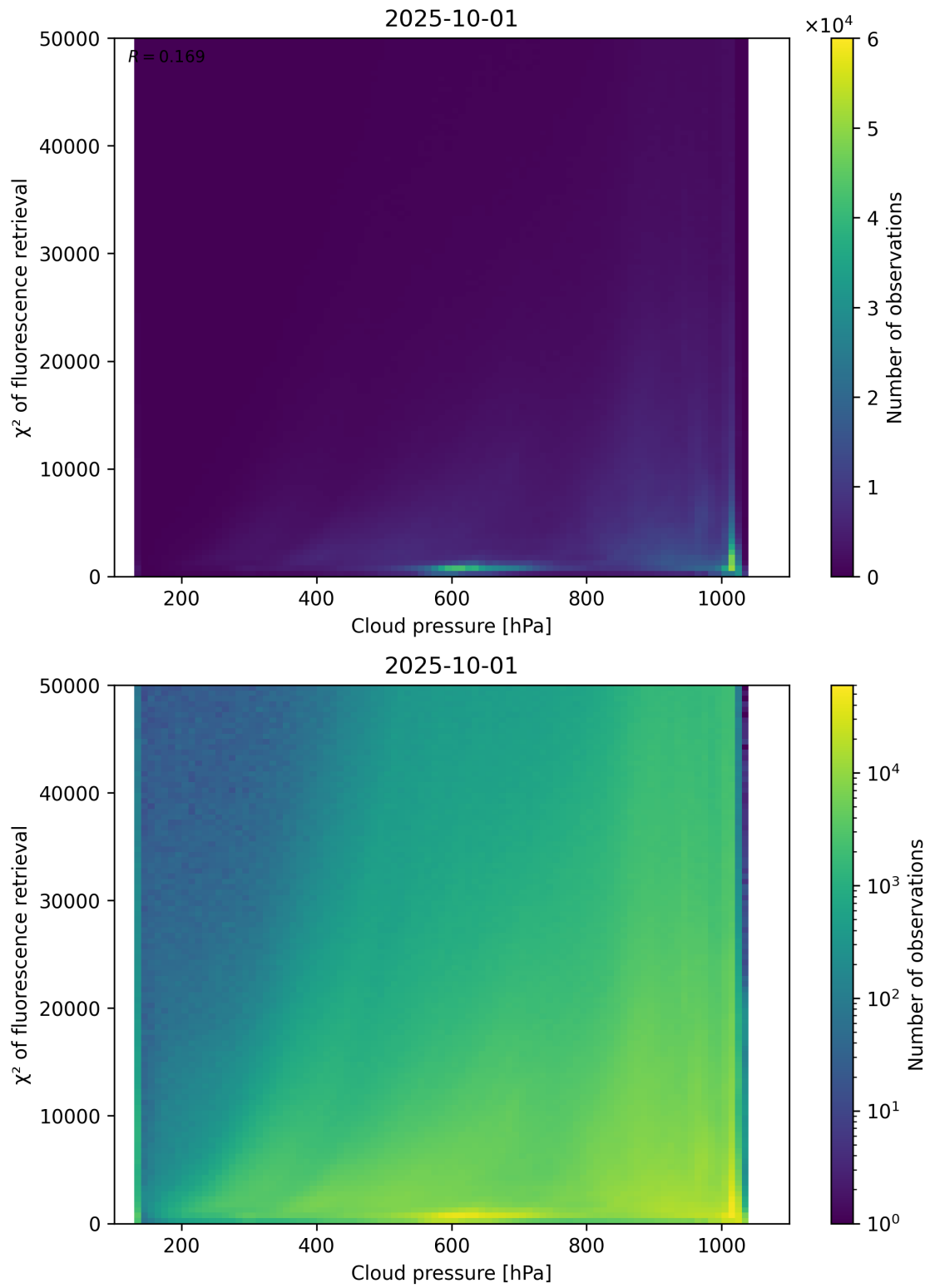
Figure 78: Scatter density plot of “Cloud pressure” against “ \chi^2 of fluorescence retrieval” for 2025-10-01 to 2025-10-02.
