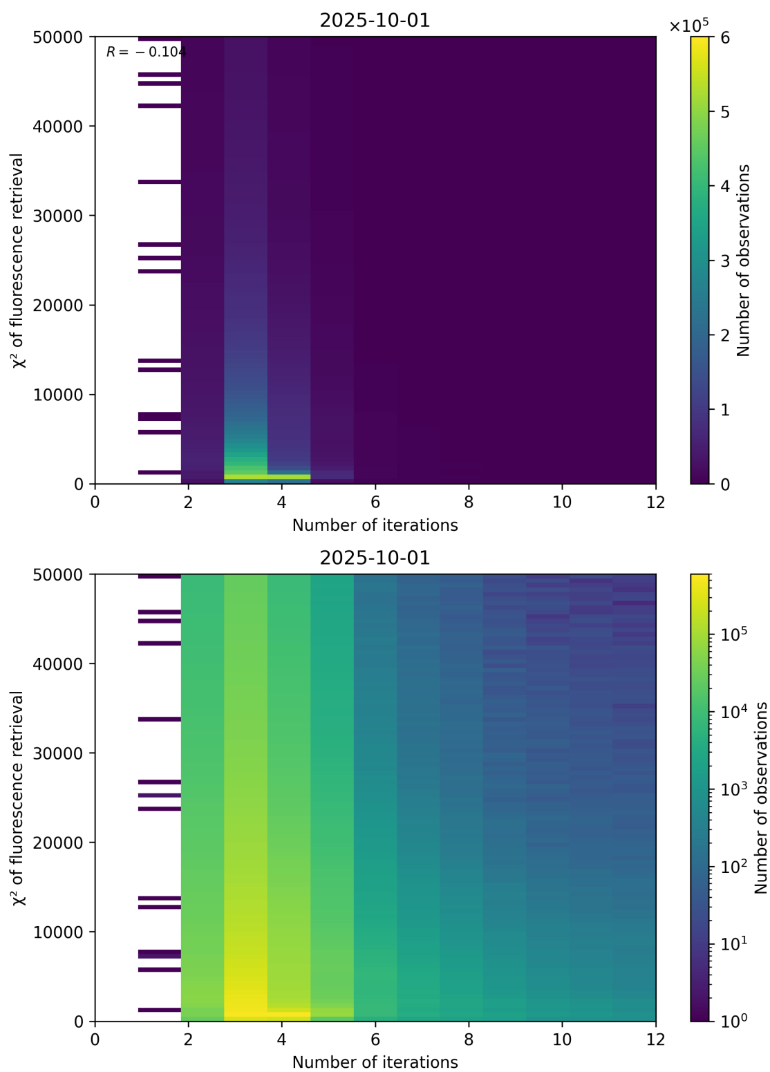
Figure 97: Scatter density plot of “Number of iterations” against “ \chi^2 of fluorescence retrieval” for 2025-10-01 to 2025-10-02.
