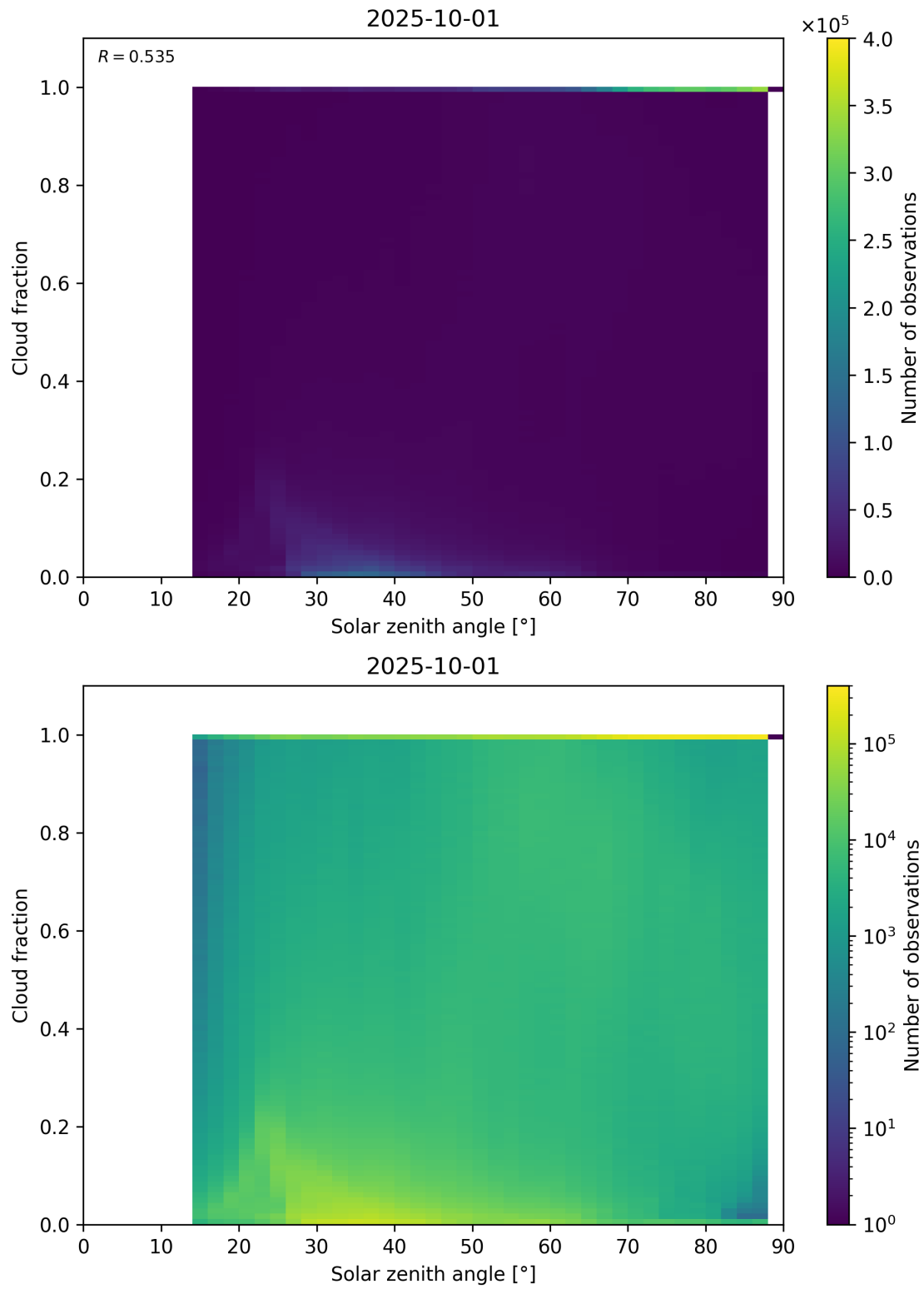
Figure 110: Scatter density plot of “Solar zenith angle” against “Cloud fraction” for 2025-10-01 to 2025-10-02.
