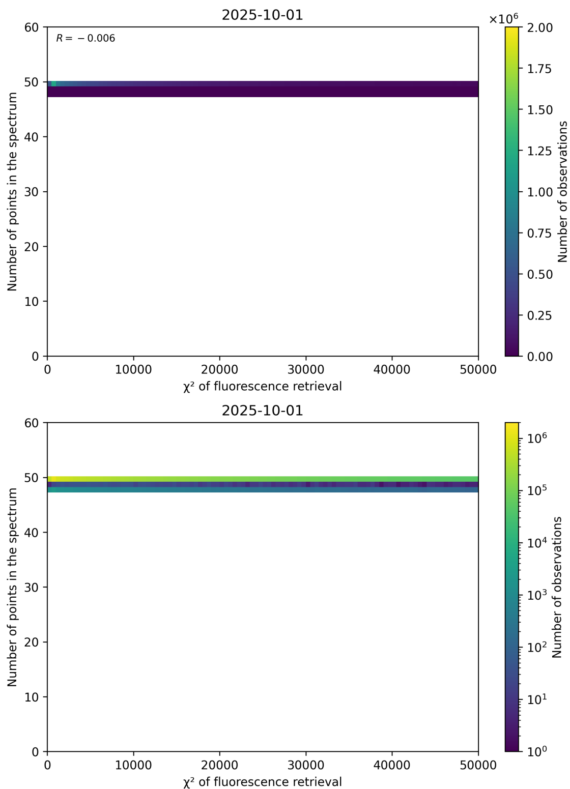
Figure 68: Scatter density plot of “ \chi^2 of fluorescence retrieval” against “Number of points in the spectrum” for 2025-10-01 to 2025-10-02.
