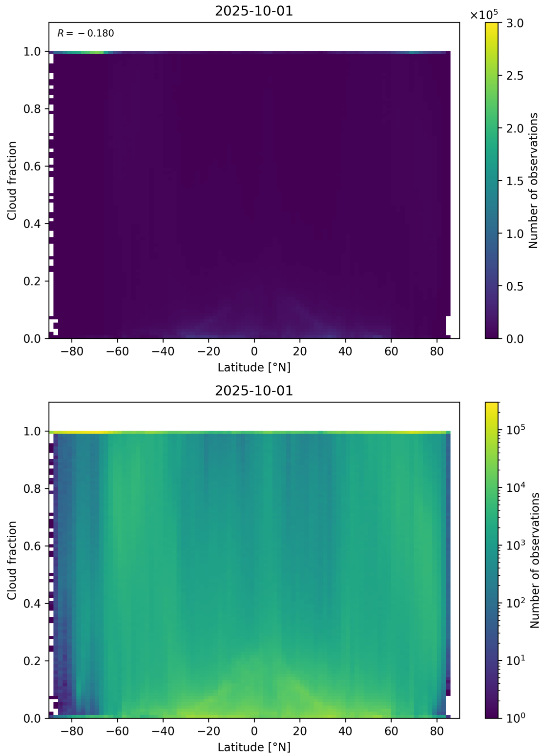
Figure 90: Scatter density plot of “Latitude” against “Cloud fraction” for 2025-10-01 to 2025-10-02.
