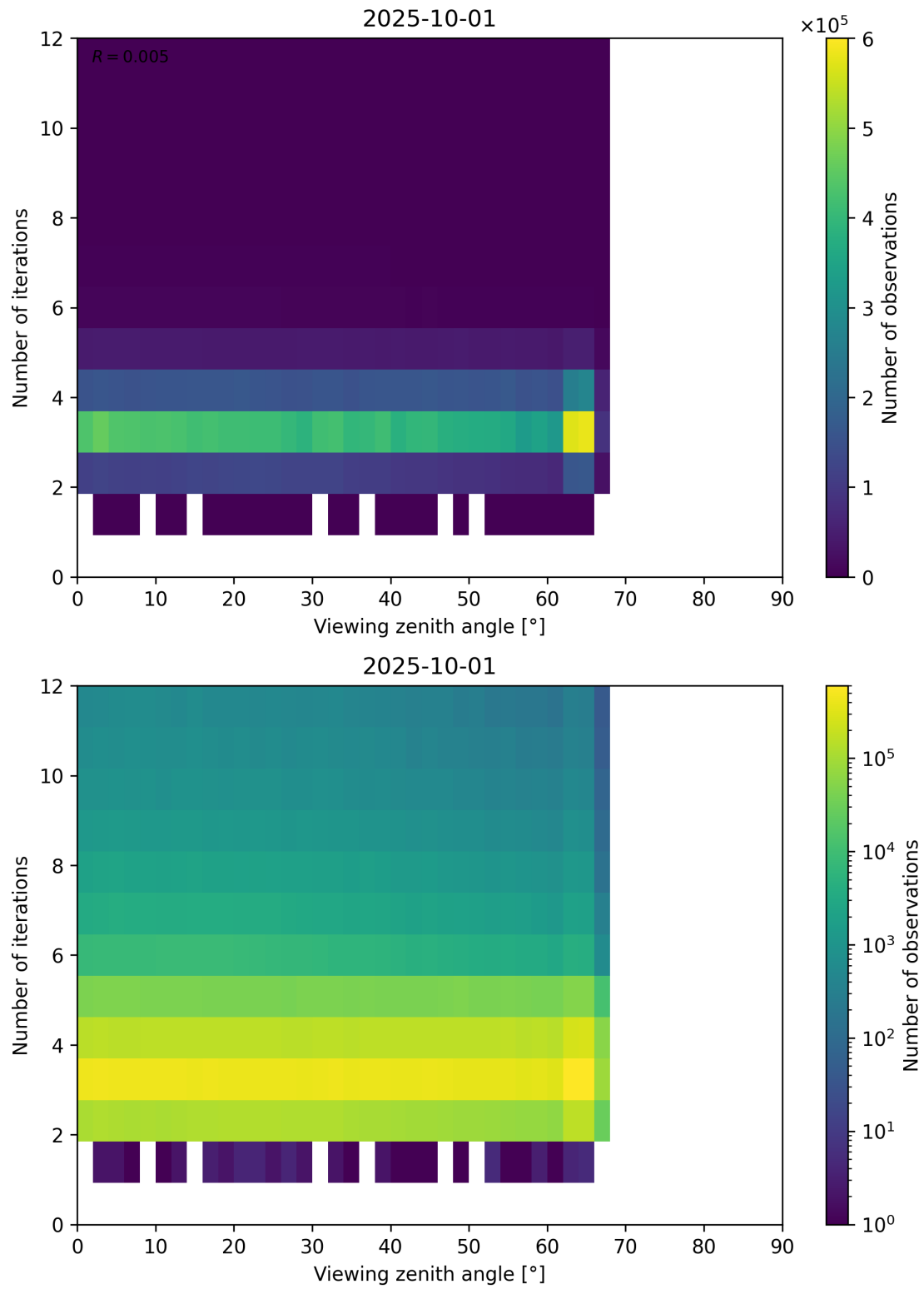
Figure 124: Scatter density plot of “Viewing zenith angle” against “Number of iterations” for 2025-10-01 to 2025-10-02.
