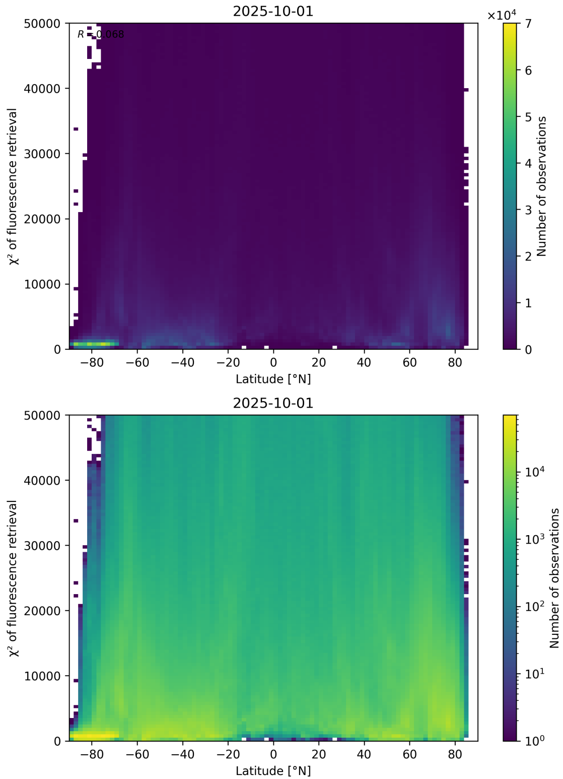
Figure 89: Scatter density plot of “Latitude” against “ \chi^2 of fluorescence retrieval” for 2025-10-01 to 2025-10-02.
