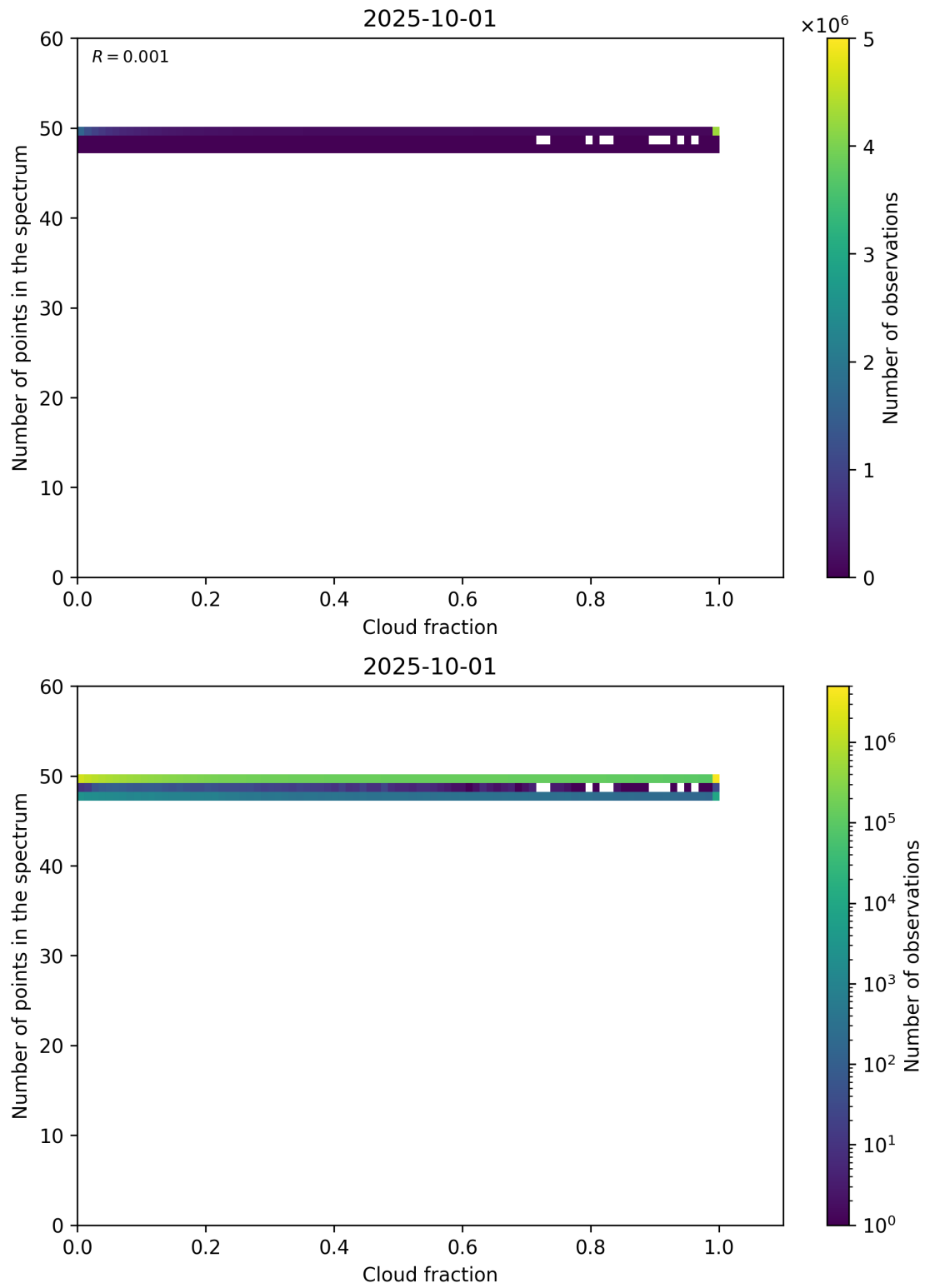
Figure 74: Scatter density plot of “Cloud fraction” against “Number of points in the spectrum” for 2025-10-01 to 2025-10-02.
