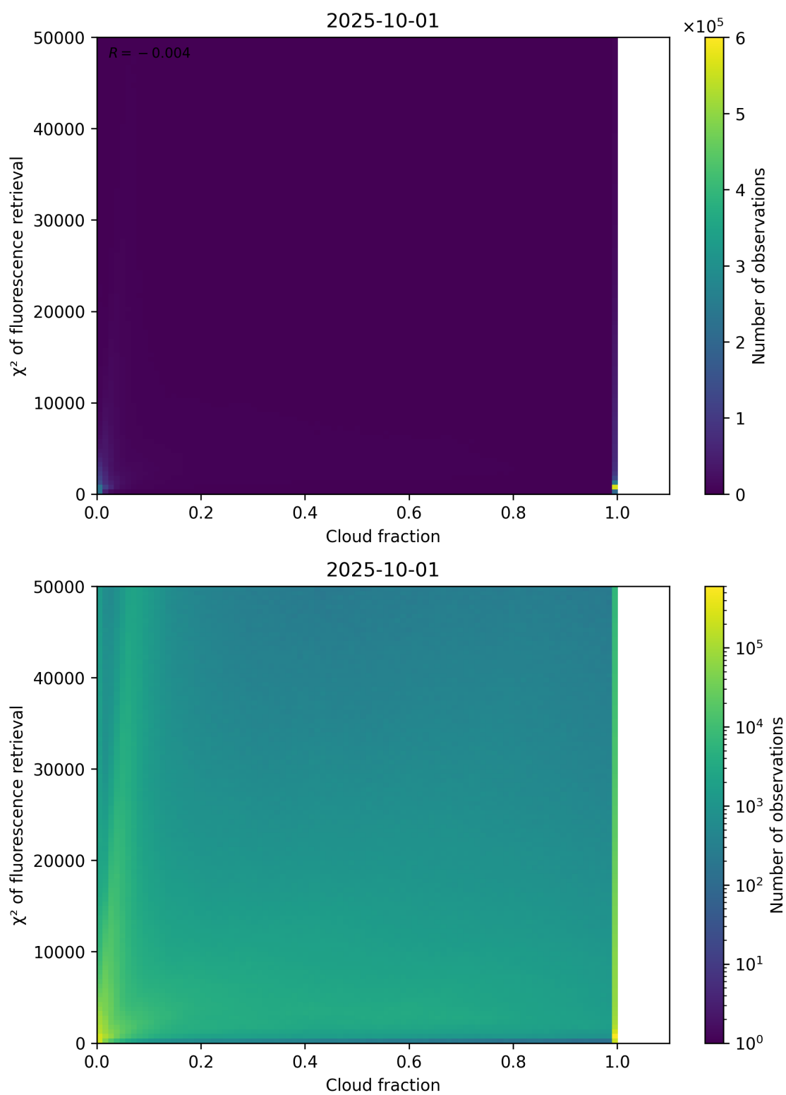
Figure 71: Scatter density plot of “Cloud fraction” against “ \chi^2 of fluorescence retrieval” for 2025-10-01 to 2025-10-02.
