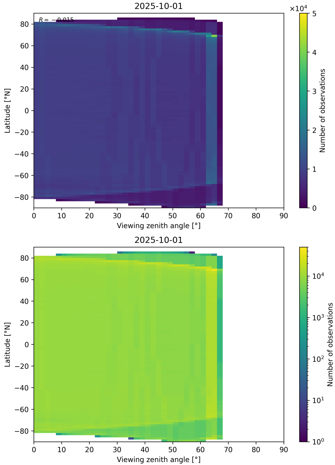
Figure 123: Scatter density plot of “Viewing zenith angle” against “Latitude” for 2025-10-01 to 2025-10-02.
