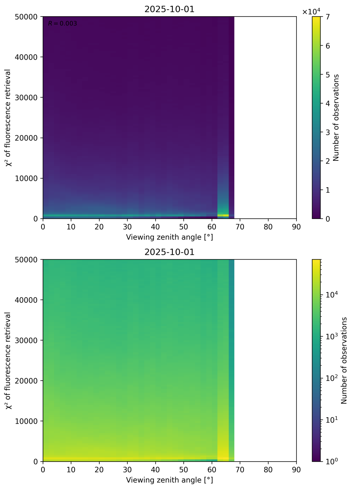
Figure 119: Scatter density plot of “Viewing zenith angle” against “ \chi^2 of fluorescence retrieval” for 2025-10-01 to 2025-10-02.
