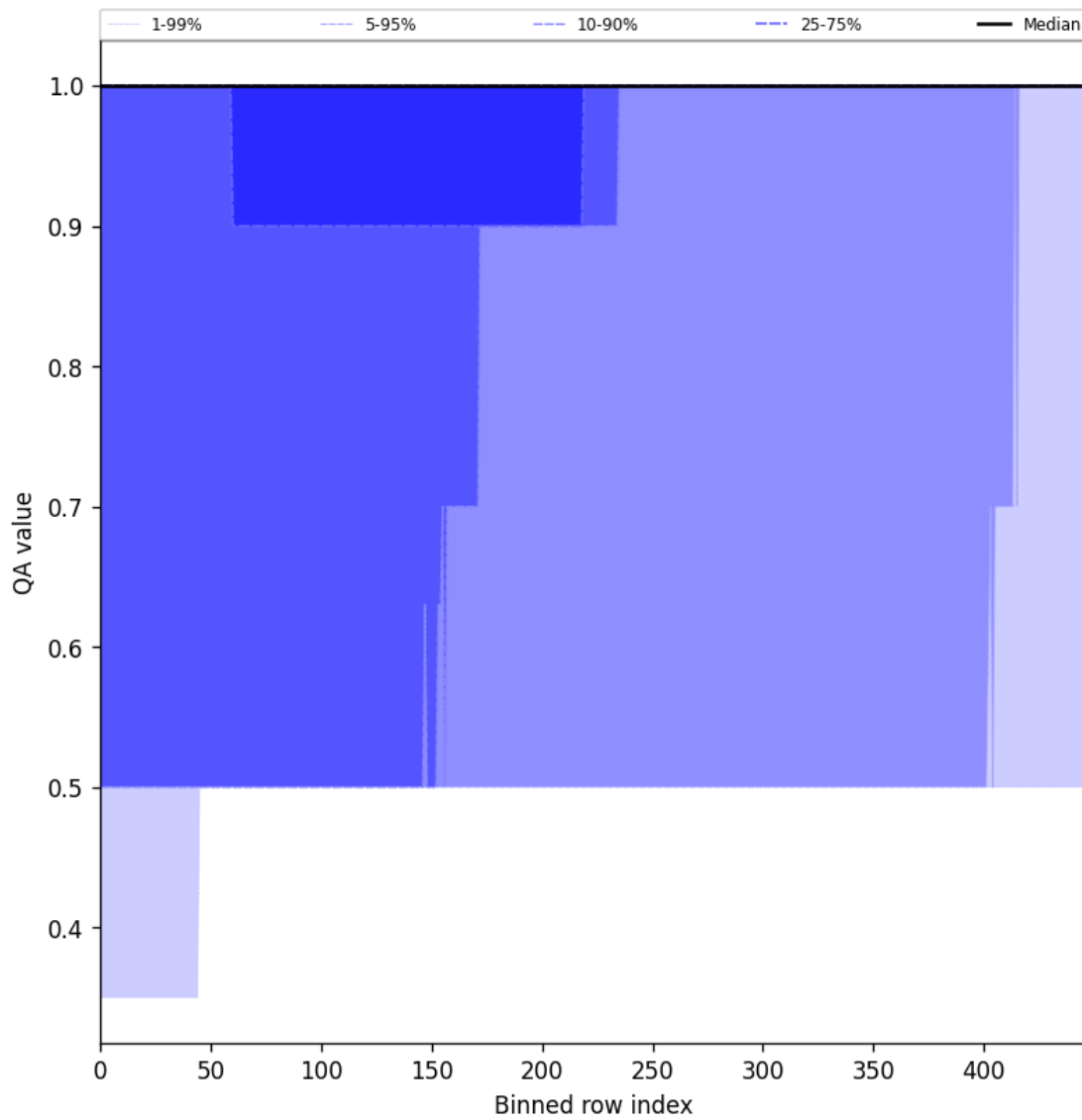
Figure 46: Along track statistics of “QA value” for 2025-10-01 to 2025-10-02
