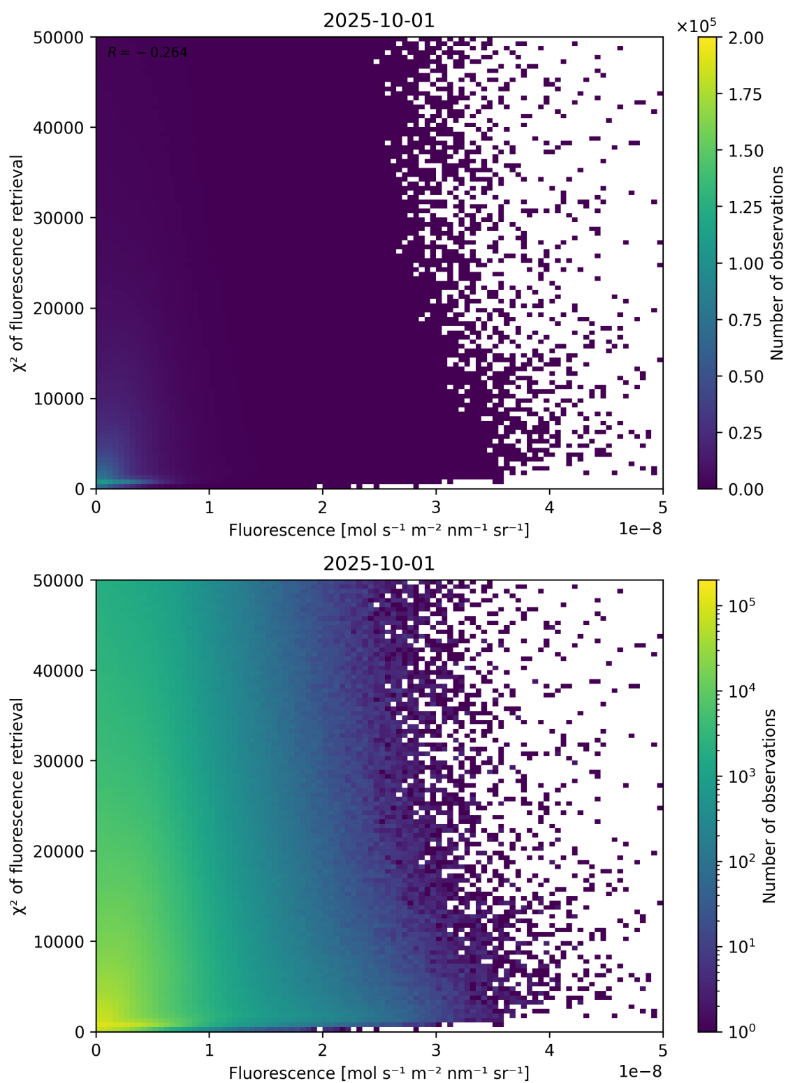
Figure 85: Scatter density plot of “Fluorescence” against “ \chi^2 of fluorescence retrieval” for 2025-10-01 to 2025-10-02.
