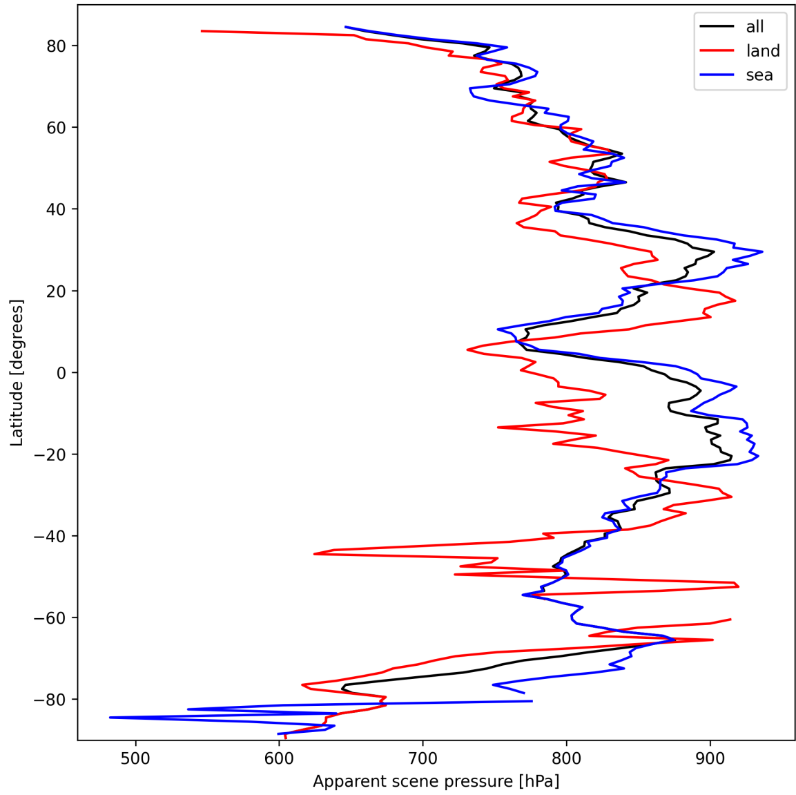
Figure 19: Zonal average of “Apparent scene pressure” for 2025-10-01 to 2025-10-02.
