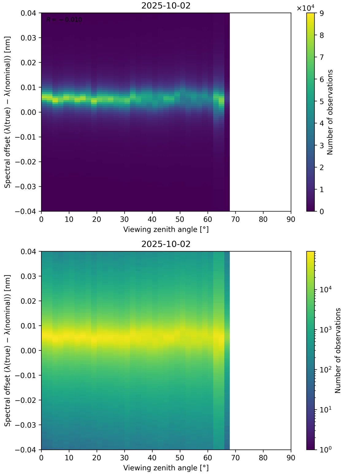
Figure 128: Scatter density plot of “Viewing zenith angle” against “Spectral offset ( \lambda_{\text{true}} - \lambda_{\text{nominal}} )” for 2025-10-01 to 2025-10-03.
