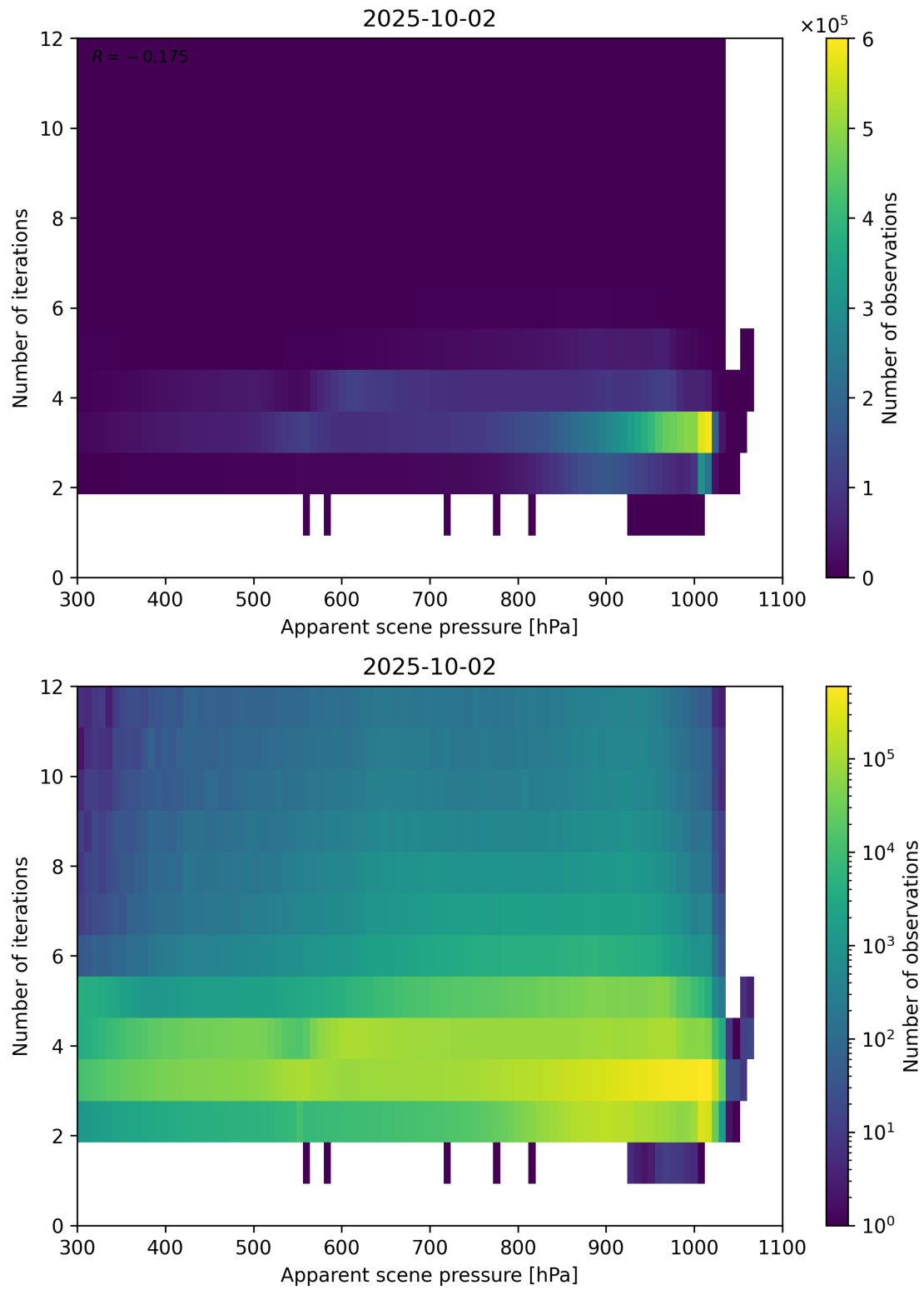
Figure 65: Scatter density plot of “Apparent scene pressure” against “Number of iterations” for 2025-10-01 to 2025-10-03.
