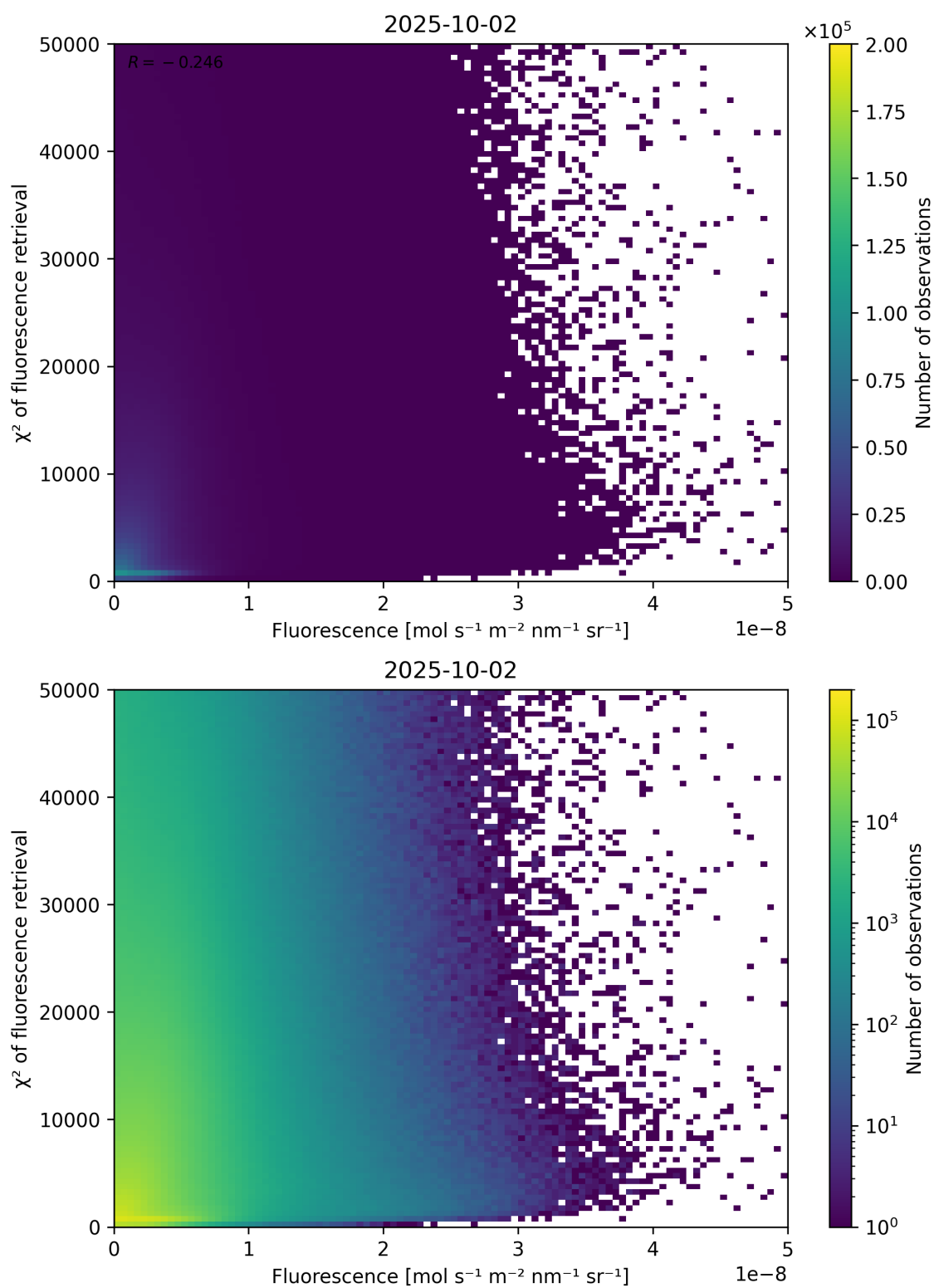
Figure 85: Scatter density plot of “Fluorescence” against “ \chi^2 of fluorescence retrieval” for 2025-10-01 to 2025-10-03.
