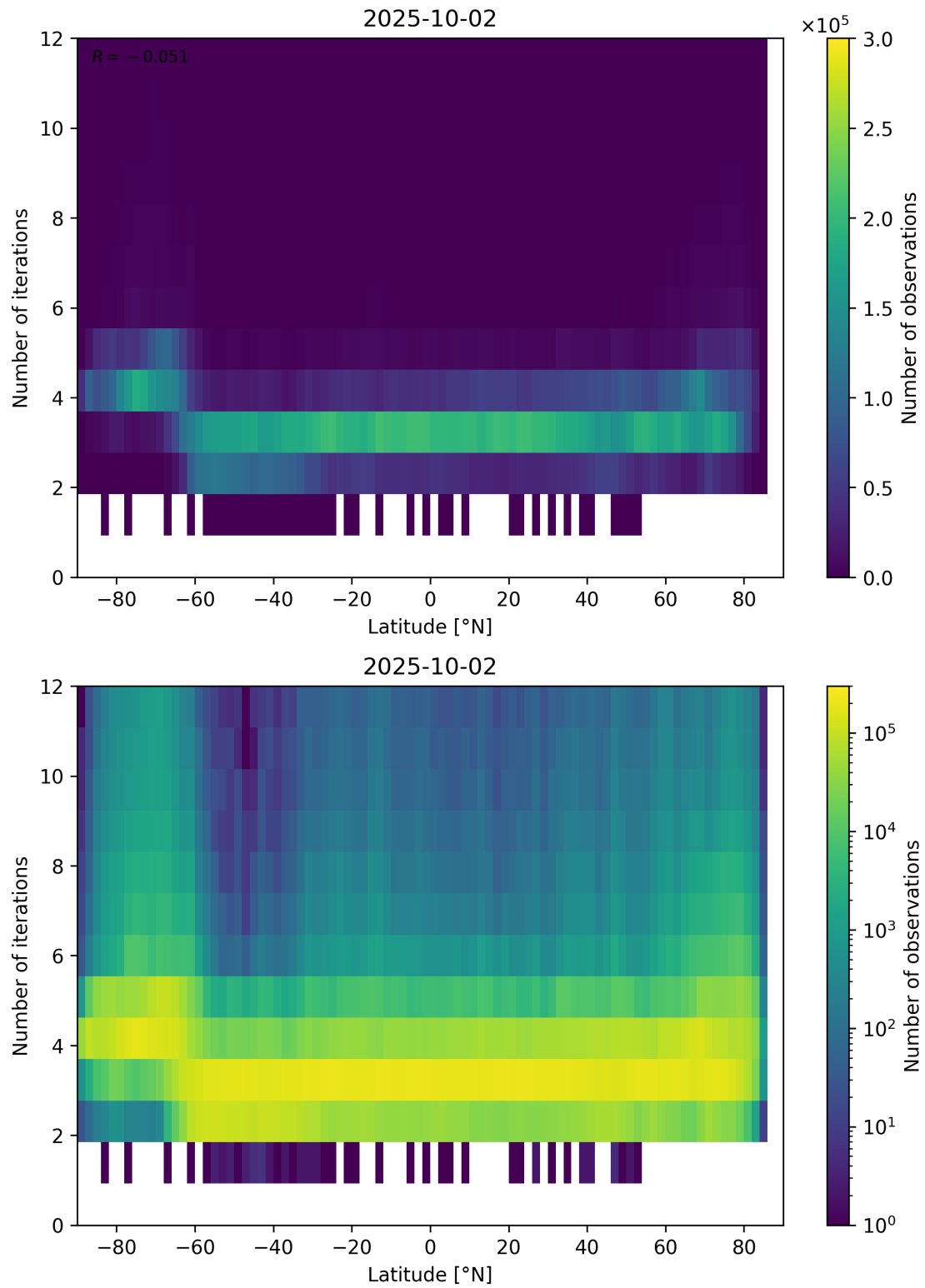
Figure 93: Scatter density plot of “Latitude” against “Number of iterations” for 2025-10-01 to 2025-10-03.
