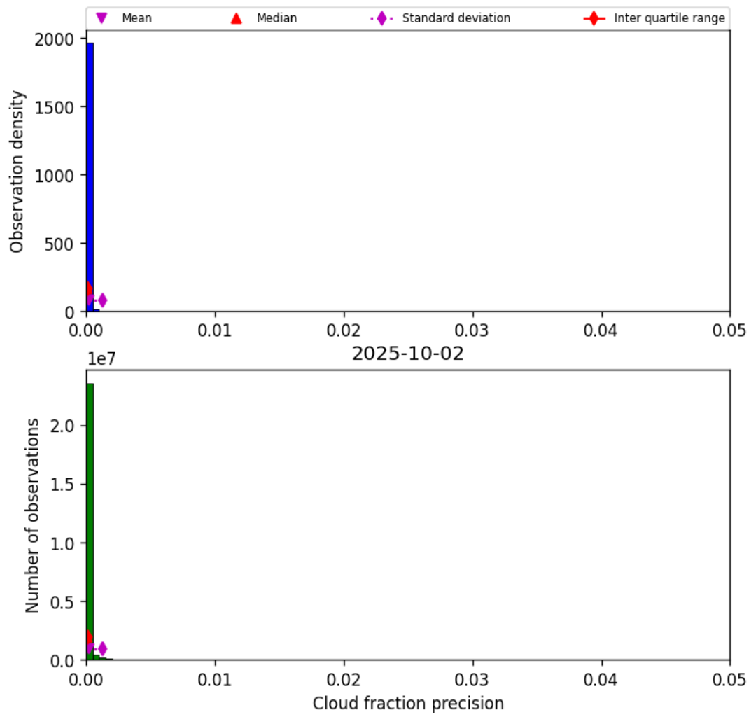
Figure 33: Histogram of “Cloud fraction precision” for 2025-10-01 to 2025-10-03
