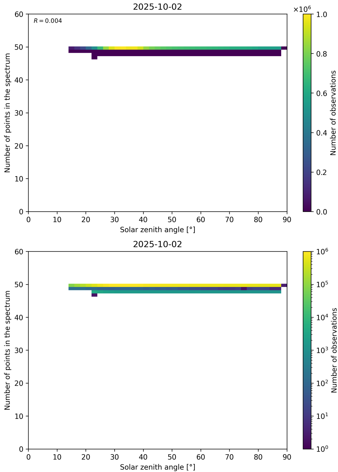
Figure 115: Scatter density plot of “Solar zenith angle” against “Number of points in the spectrum” for 2025-10-01 to 2025-10-03.
