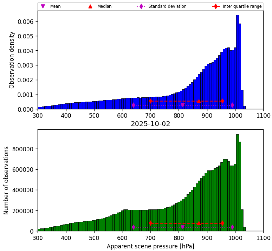
Figure 36: Histogram of “Apparent scene pressure” for 2025-10-01 to 2025-10-03
