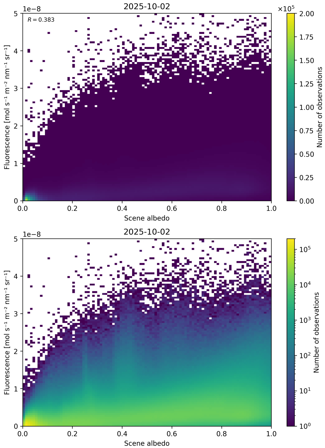
Figure 104: Scatter density plot of “Scene albedo” against “Fluorescence” for 2025-10-01 to 2025-10-03.
