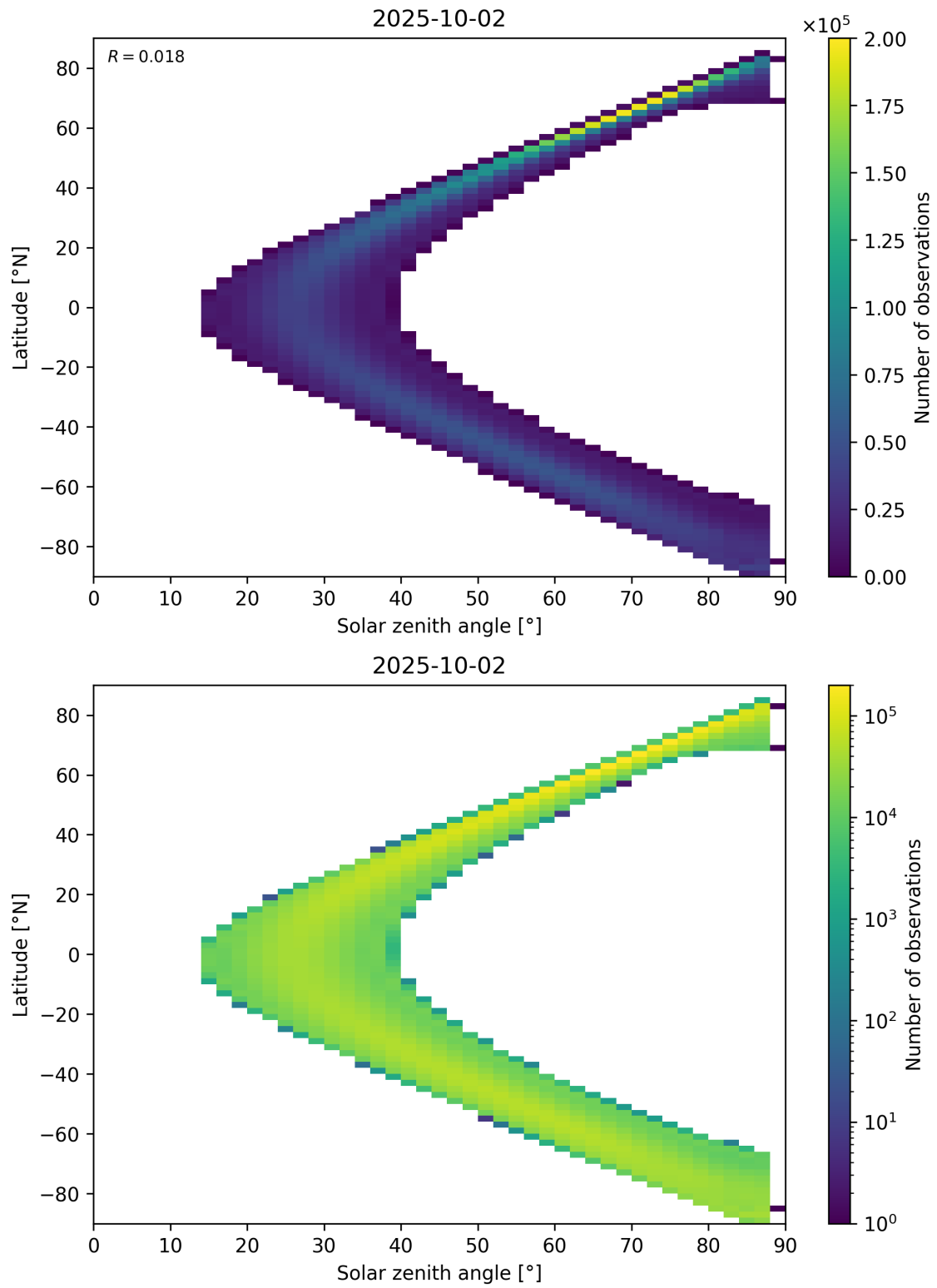
Figure 113: Scatter density plot of “Solar zenith angle” against “Latitude” for 2025-10-01 to 2025-10-03.
