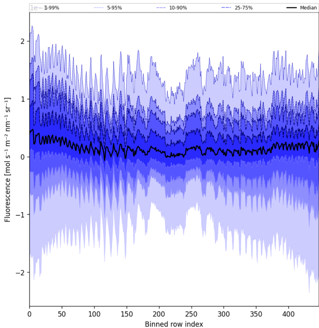
Figure 57: Along track statistics of “Fluorescence” for 2025-10-01 to 2025-10-03
