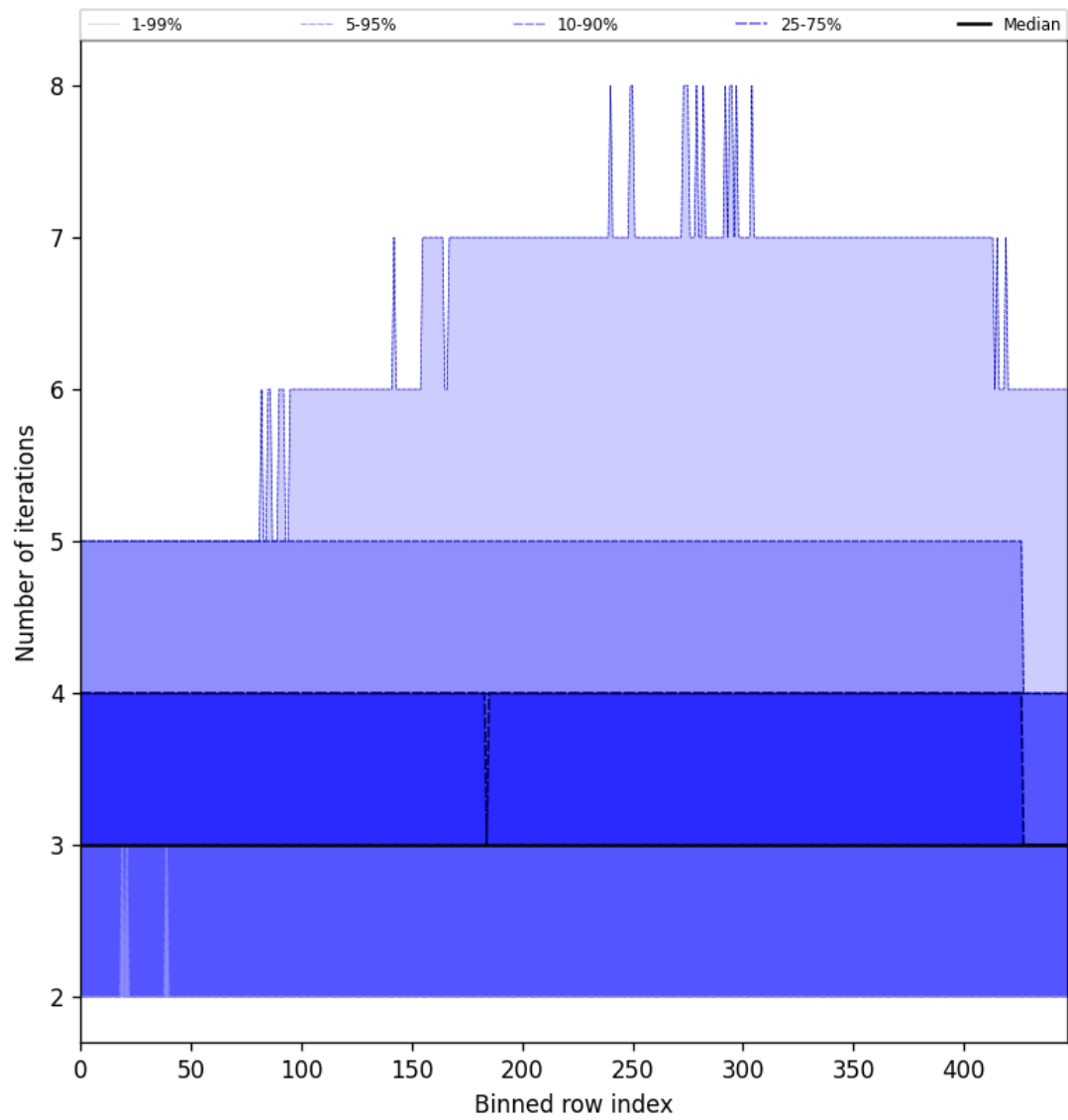
Figure 56: Along track statistics of “Number of iterations” for 2025-10-01 to 2025-10-03
