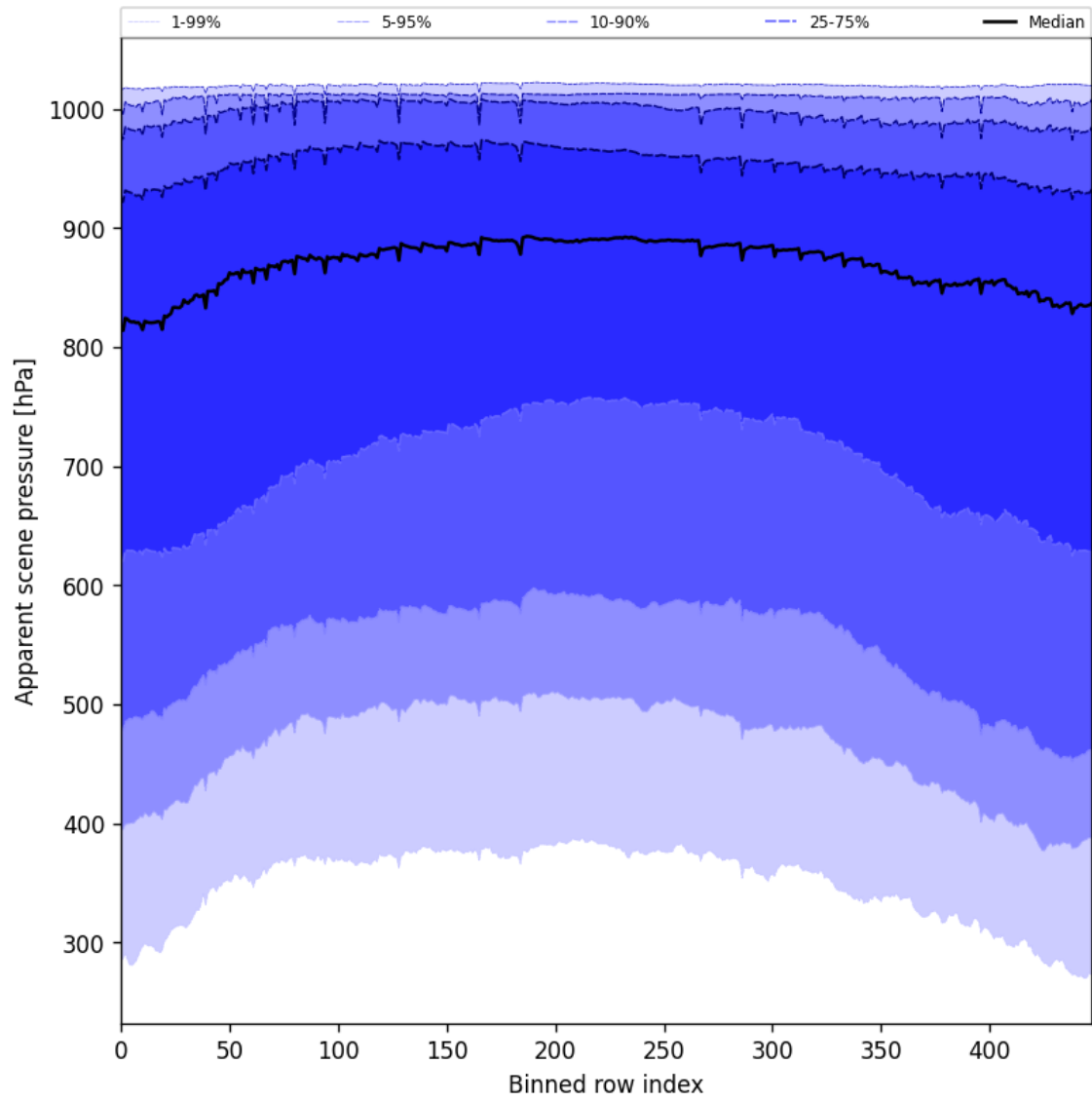
Figure 53: Along track statistics of “Apparent scene pressure” for 2025-10-01 to 2025-10-03
