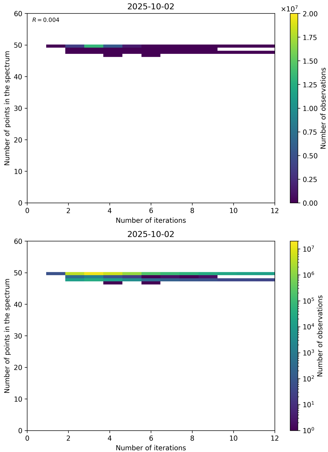
Figure 99: Scatter density plot of “Number of iterations” against “Number of points in the spectrum” for 2025-10-01 to 2025-10-03.
