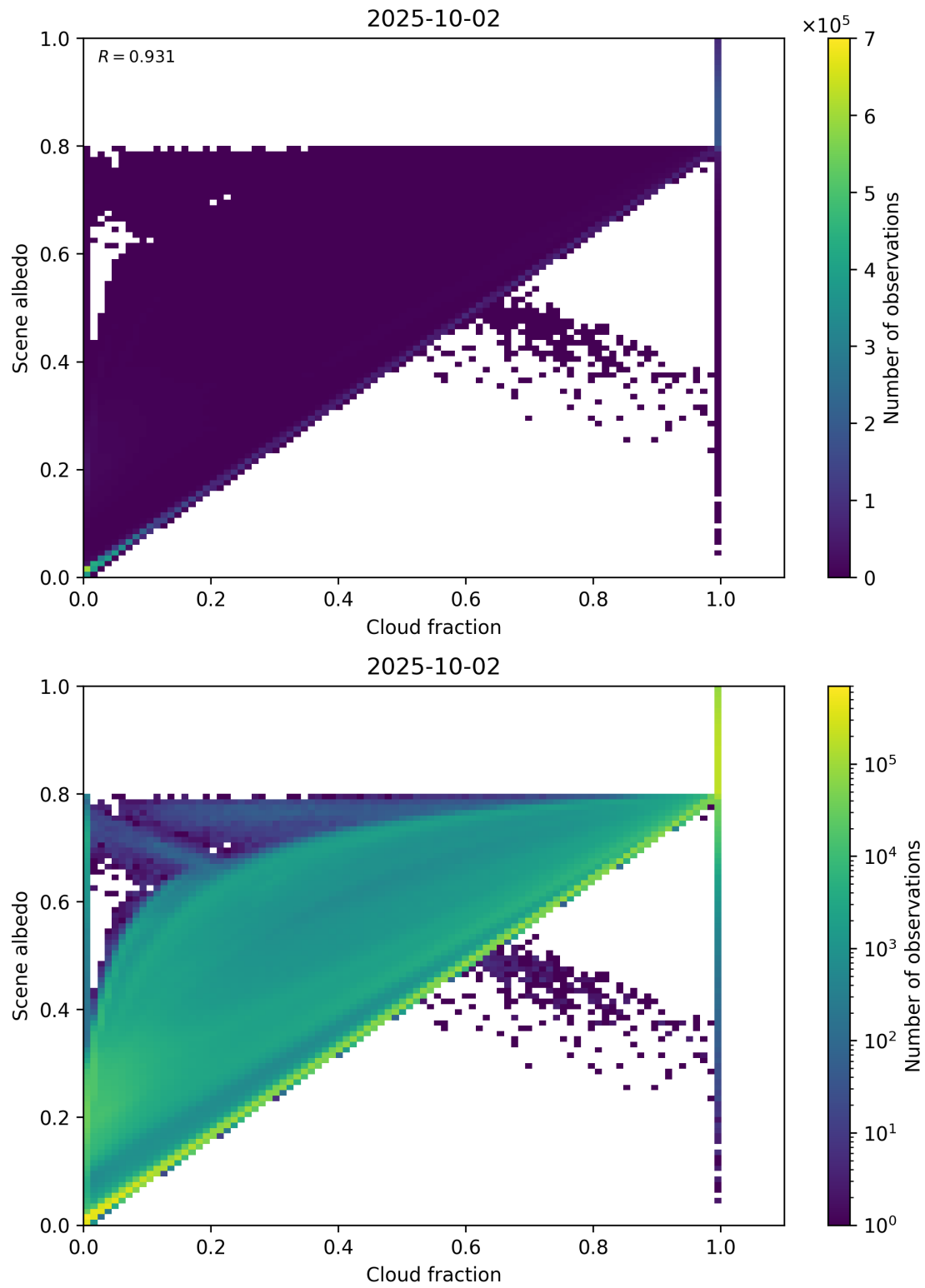
Figure 75: Scatter density plot of “Cloud fraction” against “Scene albedo” for 2025-10-01 to 2025-10-03.
