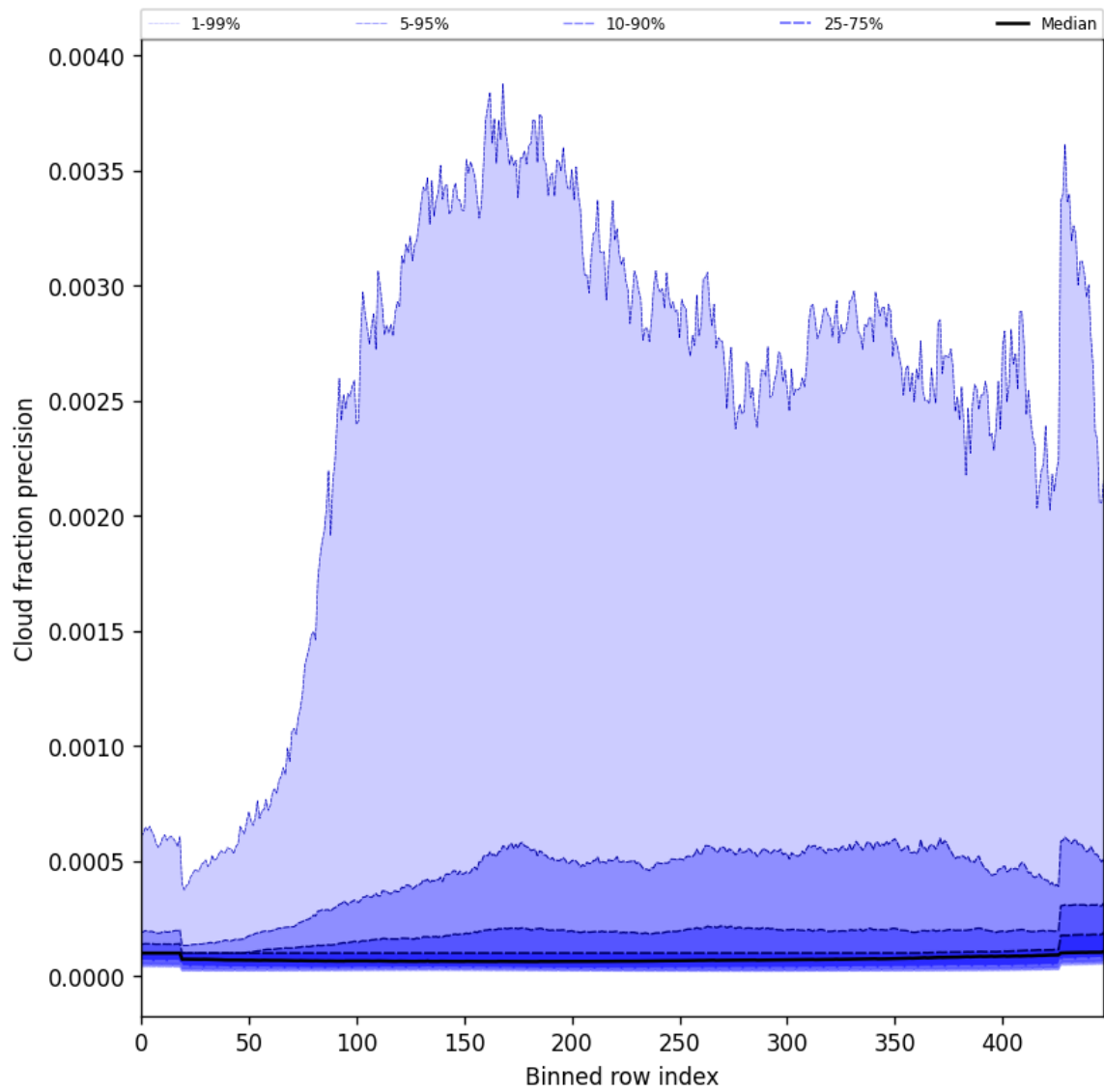
Figure 50: Along track statistics of “Cloud fraction precision” for 2025-10-01 to 2025-10-03
