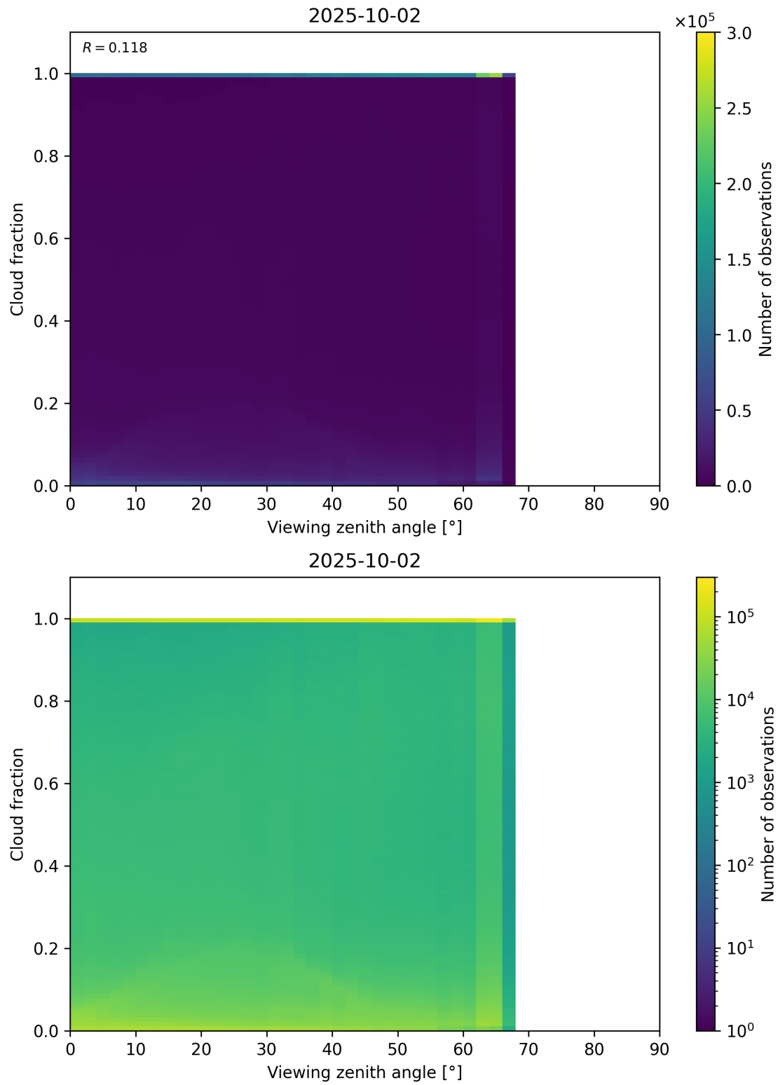
Figure 120: Scatter density plot of “Viewing zenith angle” against “Cloud fraction” for 2025-10-01 to 2025-10-03.
