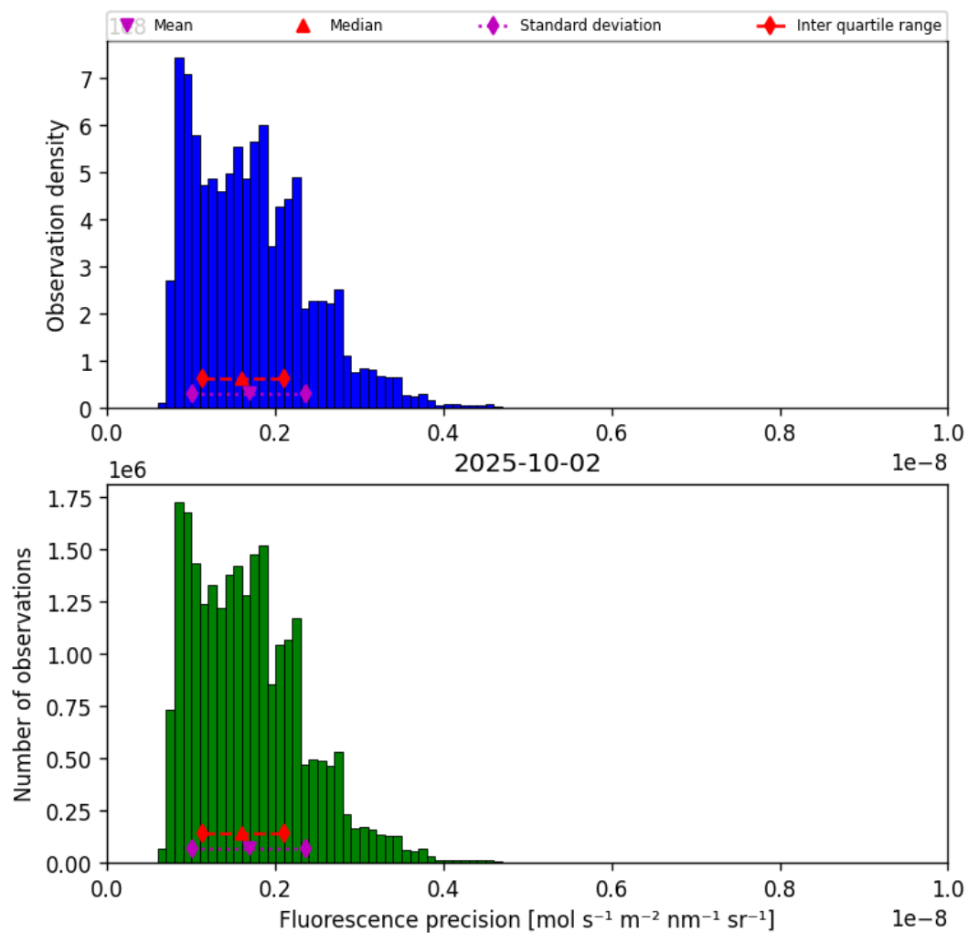
Figure 41: Histogram of “Fluorescence precision” for 2025-10-01 to 2025-10-03
