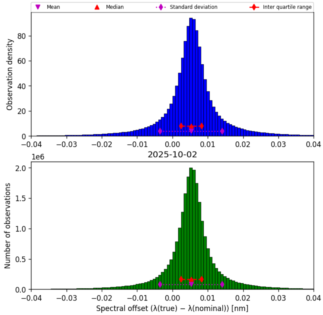
Figure 45: Histogram of “Spectral offset ( \lambda_{\text{true}} - \lambda_{\text{nominal}} )” for 2025-10-01 to 2025-10-03
