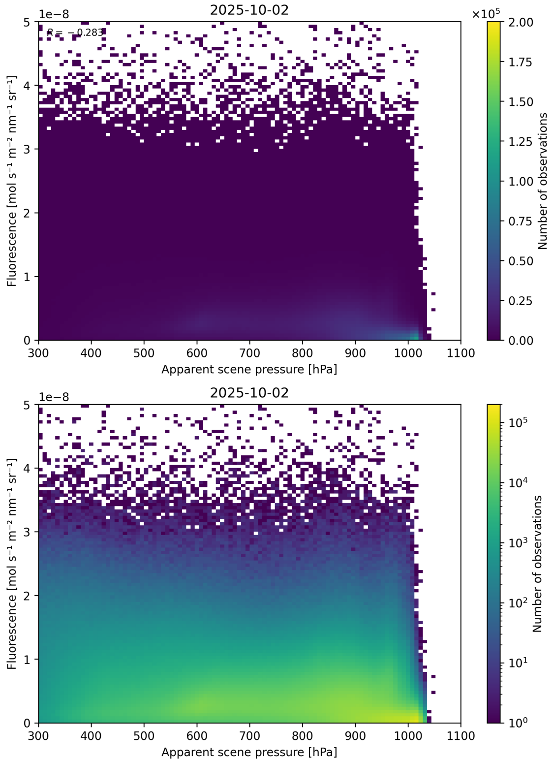
Figure 64: Scatter density plot of “Apparent scene pressure” against “Fluorescence” for 2025-10-01 to 2025-10-03.
