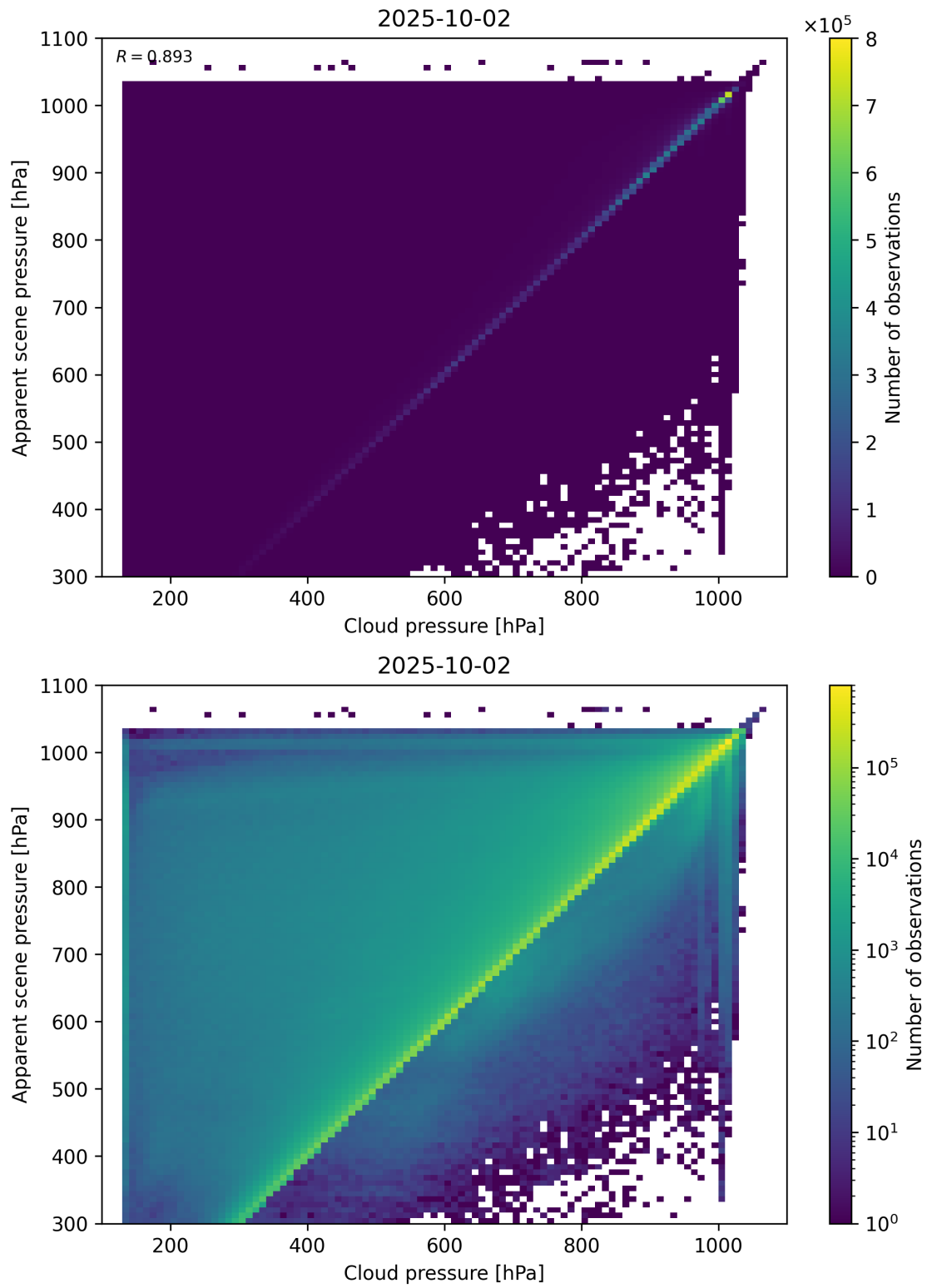
Figure 77: Scatter density plot of “Cloud pressure” against “Apparent scene pressure” for 2025-10-01 to 2025-10-03.
