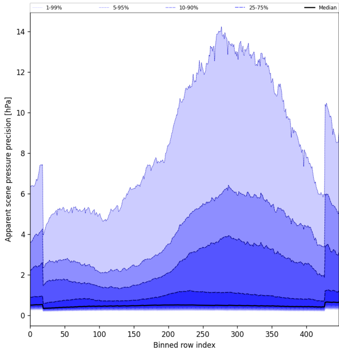
Figure 54: Along track statistics of “Apparent scene pressure precision” for 2025-10-01 to 2025-10-03
