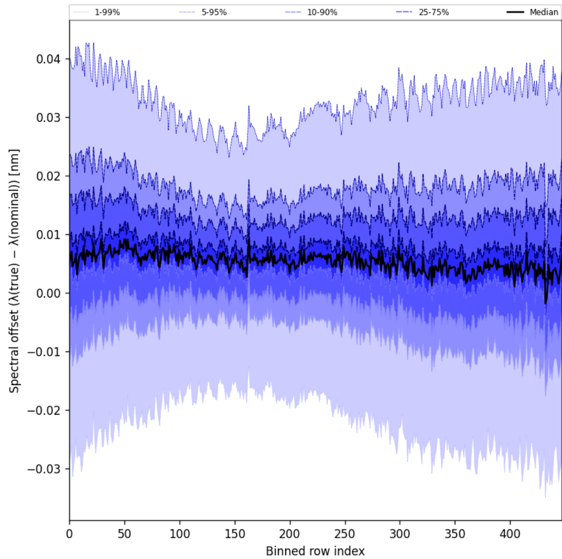
Figure 62: Along track statistics of “Spectral offset ( \lambda_{\text{true}} - \lambda_{\text{nominal}} )” for 2025-10-01 to 2025-10-03
