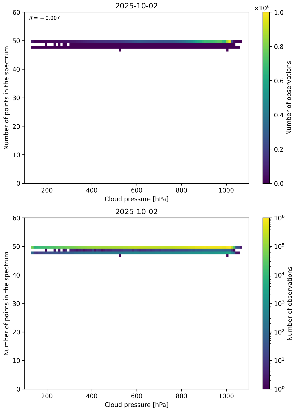
Figure 82: Scatter density plot of “Cloud pressure” against “Number of points in the spectrum” for 2025-10-01 to 2025-10-03.
