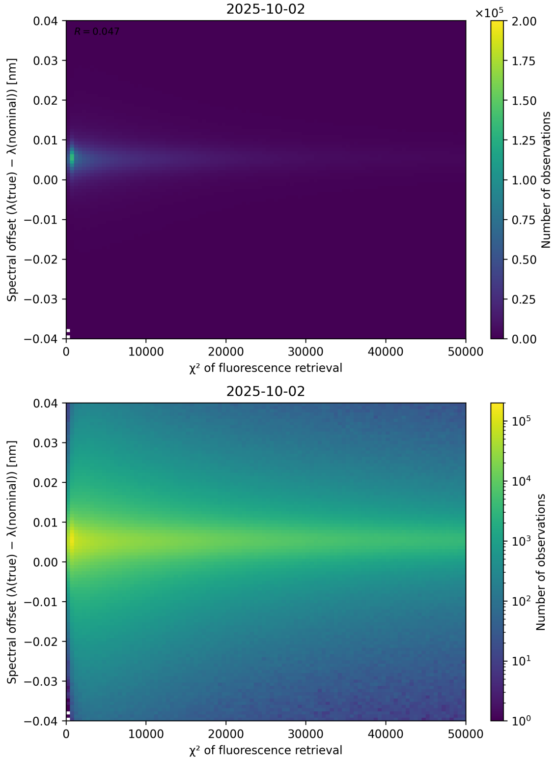
Figure 69: Scatter density plot of “ \chi^2 of fluorescence retrieval” against “Spectral offset ( \lambda_{\text{true}} - \lambda_{\text{nominal}} )” for 2025-10-01 to 2025-10-03.
