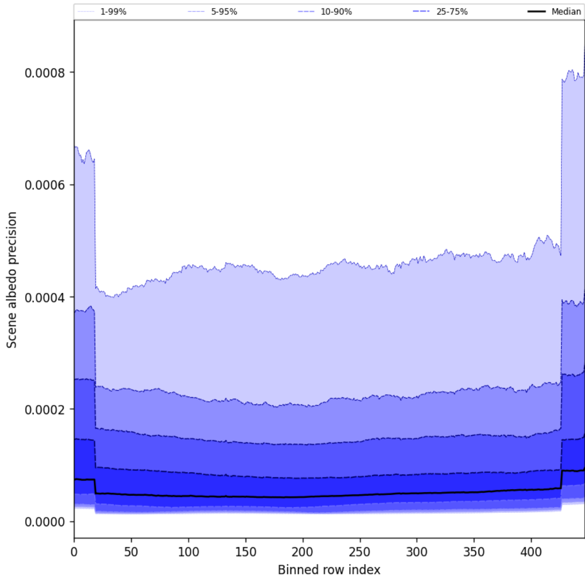
Figure 52: Along track statistics of “Scene albedo precision” for 2025-10-01 to 2025-10-03
