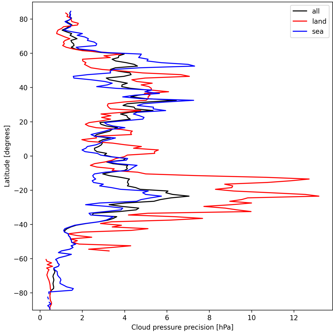
Figure 14: Zonal average of “Cloud pressure precision” for 2025-10-01 to 2025-10-03.
