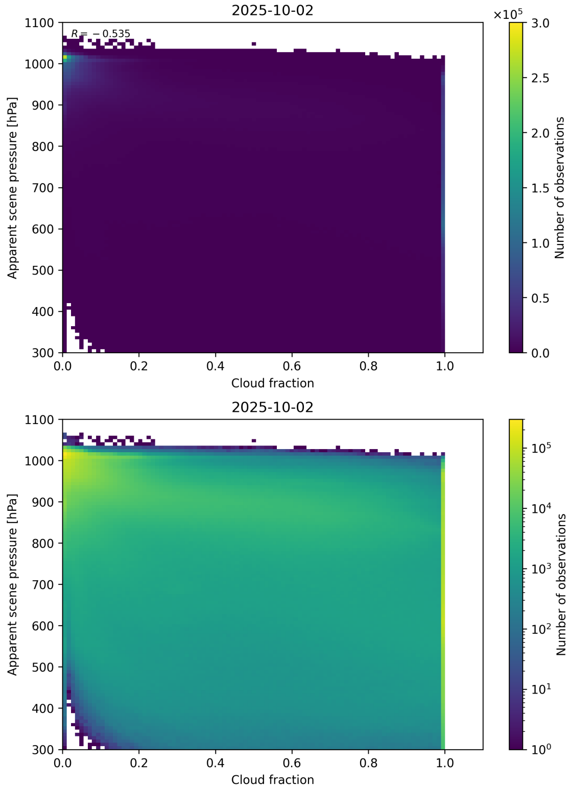
Figure 70: Scatter density plot of “Cloud fraction” against “Apparent scene pressure” for 2025-10-01 to 2025-10-03.
