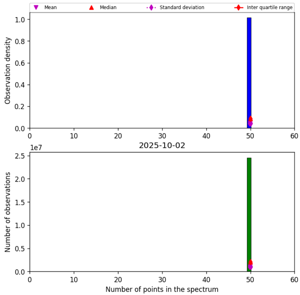
Figure 44: Histogram of "Number of points in the spectrum" for 2025-10-01 to 2025-10-03
