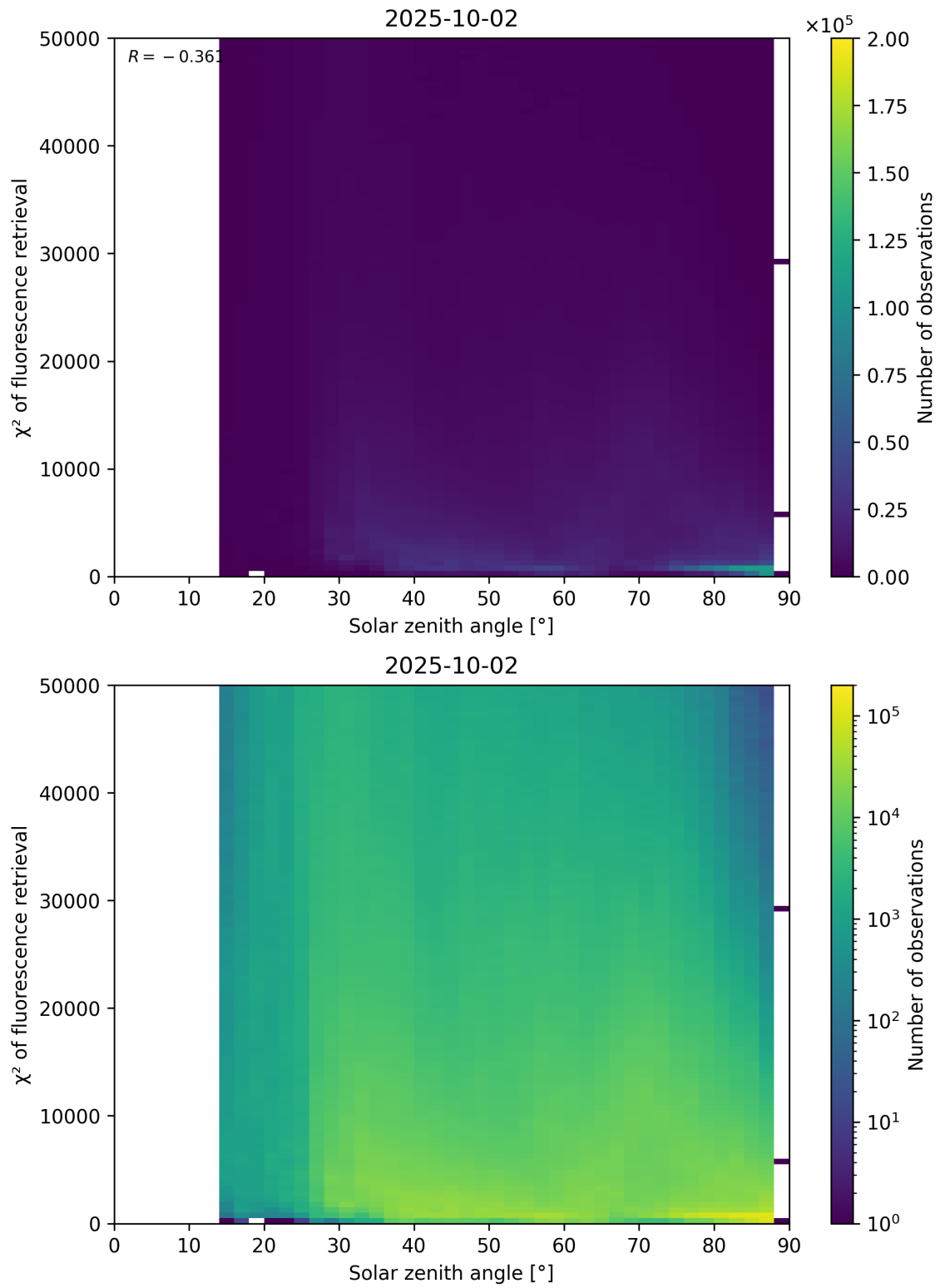
Figure 109: Scatter density plot of “Solar zenith angle” against “ \chi^2 of fluorescence retrieval” for 2025-10-01 to 2025-10-03.
