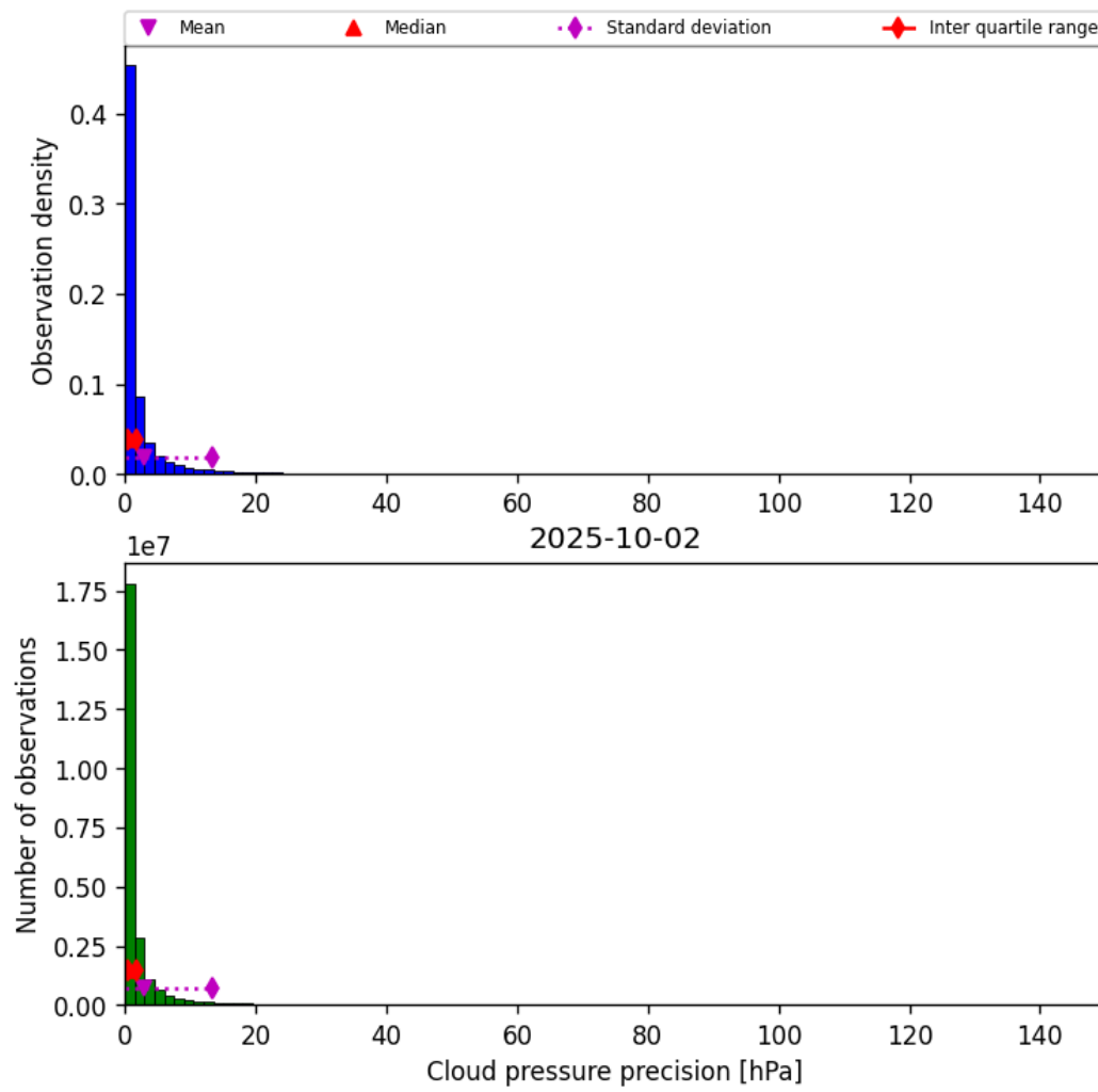
Figure 31: Histogram of “Cloud pressure precision” for 2025-10-01 to 2025-10-03
