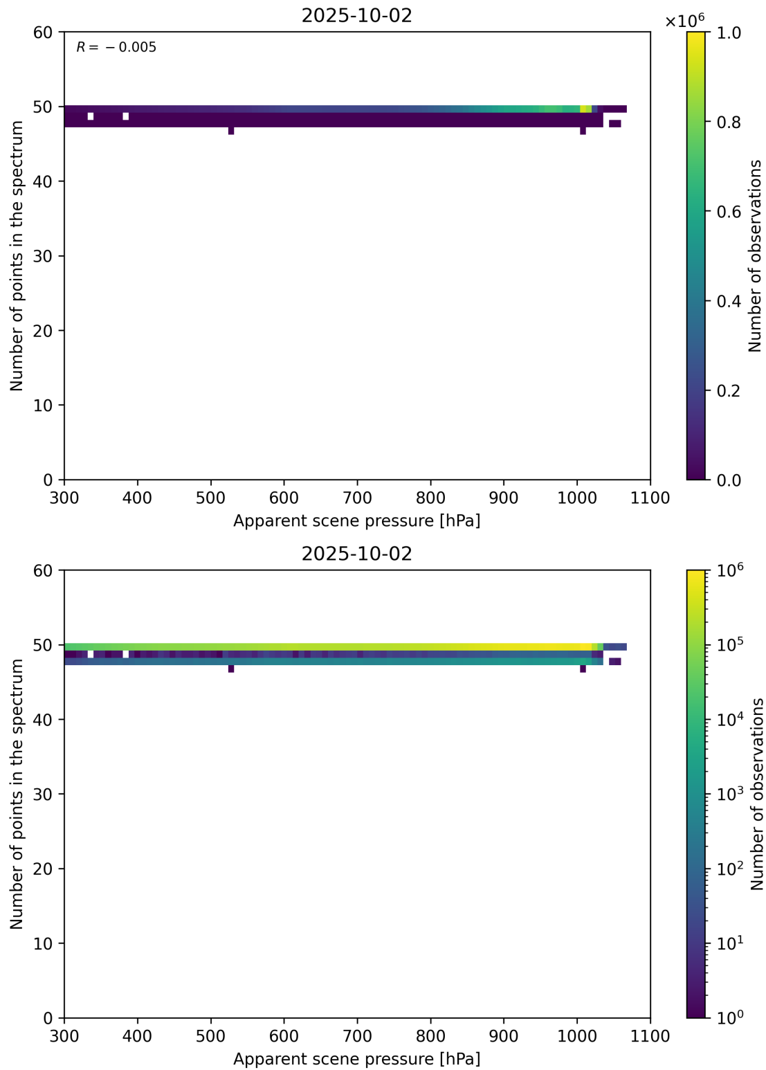
Figure 66: Scatter density plot of “Apparent scene pressure” against “Number of points in the spectrum” for 2025-10-01 to 2025-10-03.
