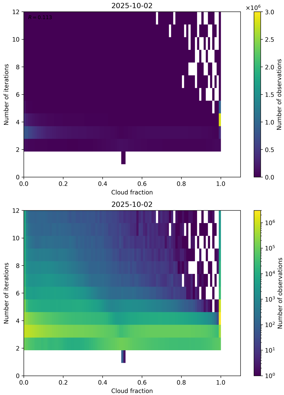
Figure 73: Scatter density plot of “Cloud fraction” against “Number of iterations” for 2025-10-01 to 2025-10-03.
