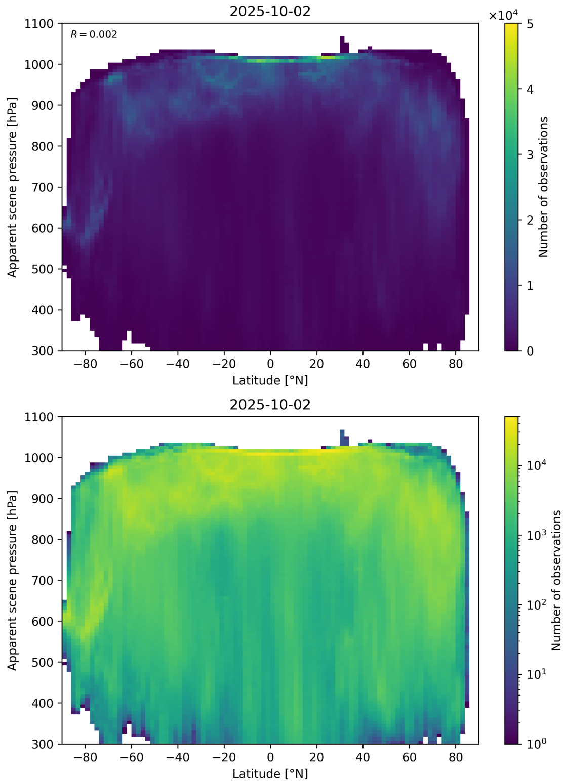
Figure 88: Scatter density plot of “Latitude” against “Apparent scene pressure” for 2025-10-01 to 2025-10-03.
