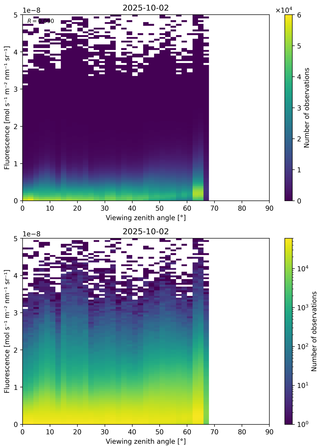
Figure 122: Scatter density plot of “Viewing zenith angle” against “Fluorescence” for 2025-10-01 to 2025-10-03.
