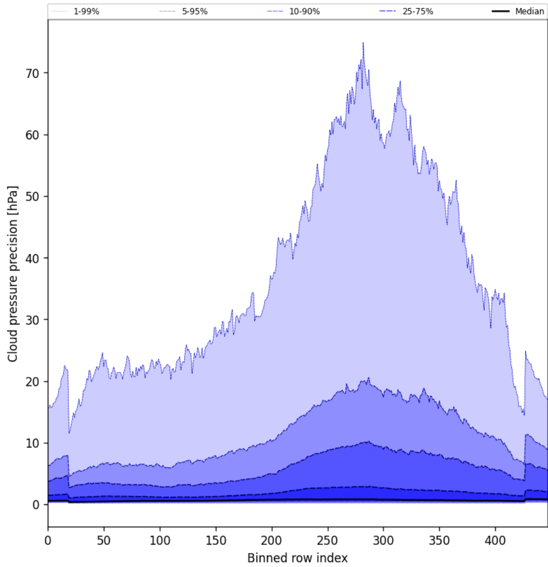
Figure 48: Along track statistics of “Cloud pressure precision” for 2025-10-01 to 2025-10-03
