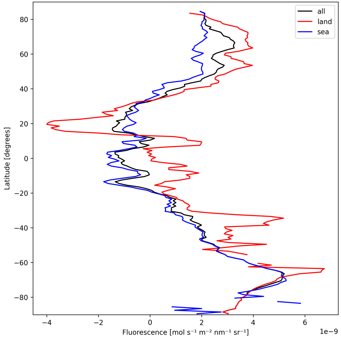
Figure 23: Zonal average of “Fluorescence” for 2025-10-01 to 2025-10-03.
