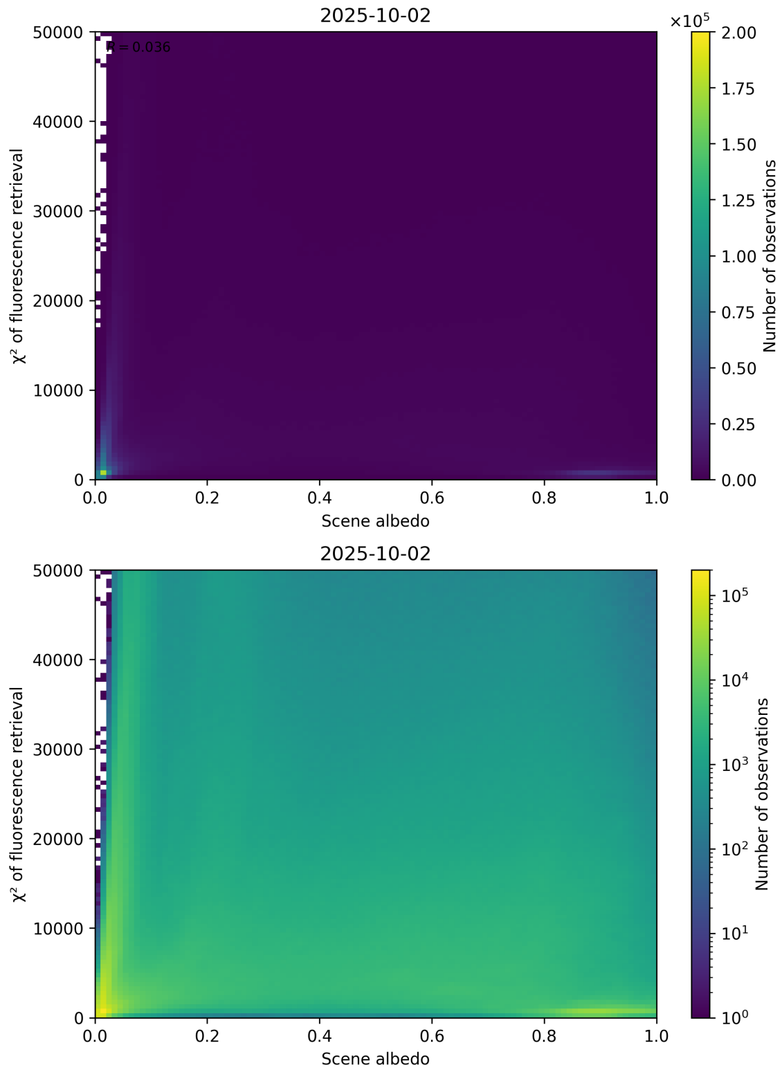
Figure 103: Scatter density plot of “Scene albedo” against “ \chi^2 of fluorescence retrieval” for 2025-10-01 to 2025-10-03.
