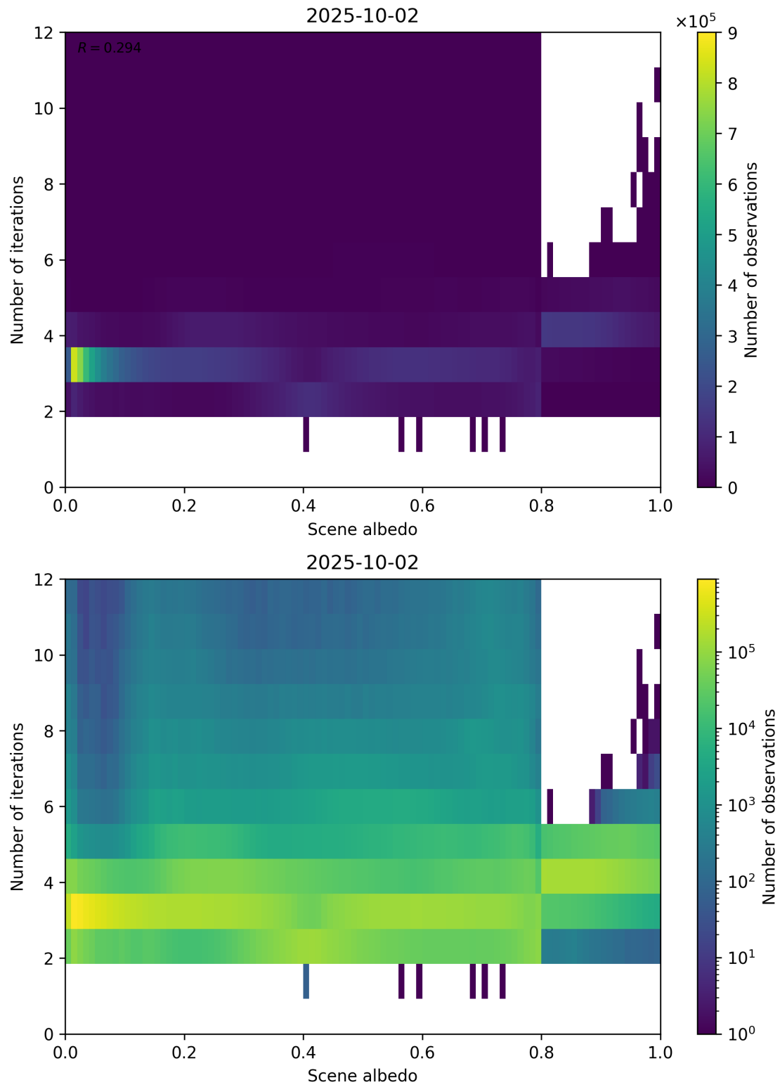
Figure 105: Scatter density plot of “Scene albedo” against “Number of iterations” for 2025-10-01 to 2025-10-03.
