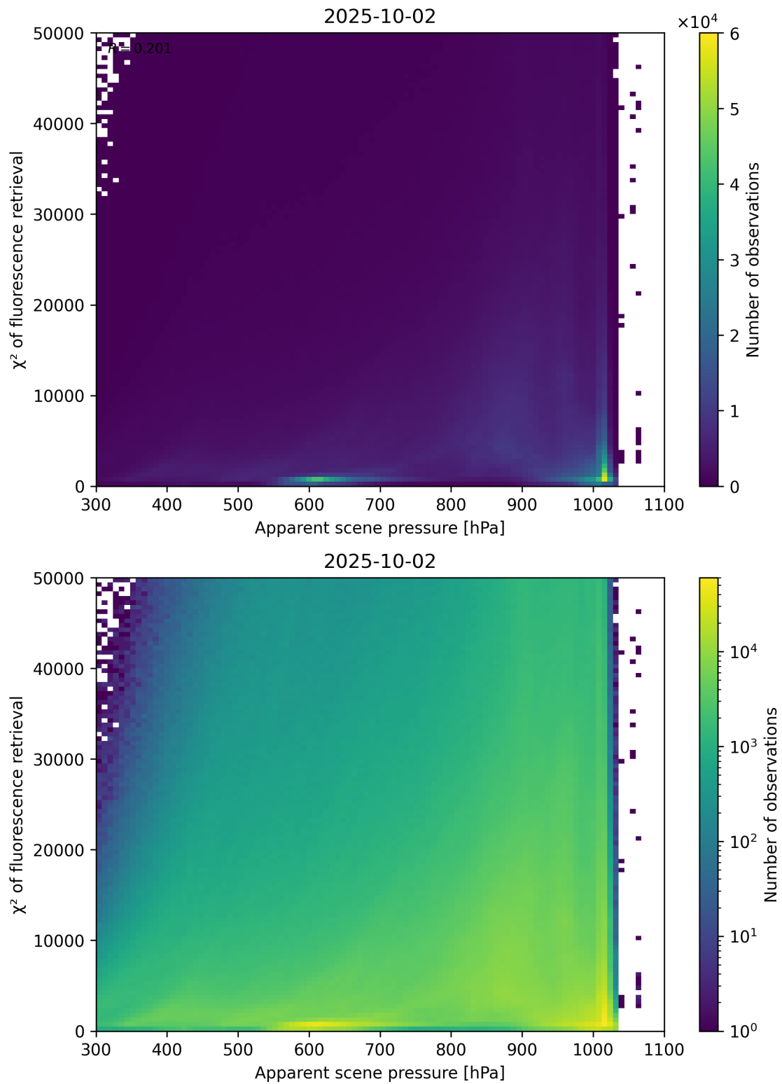
Figure 63: Scatter density plot of “Apparent scene pressure” against “ \chi^2 of fluorescence retrieval” for 2025-10-01 to 2025-10-03.
