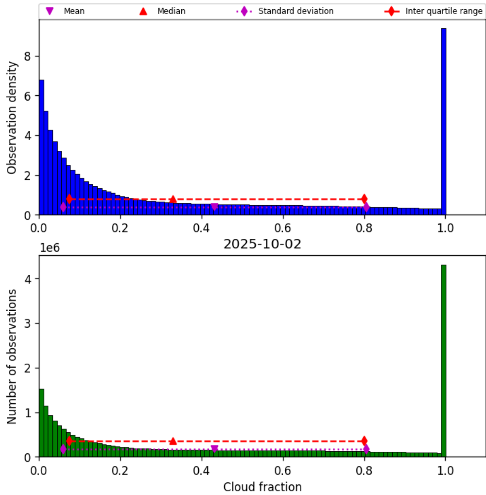
Figure 32: Histogram of “Cloud fraction” for 2025-10-01 to 2025-10-03
