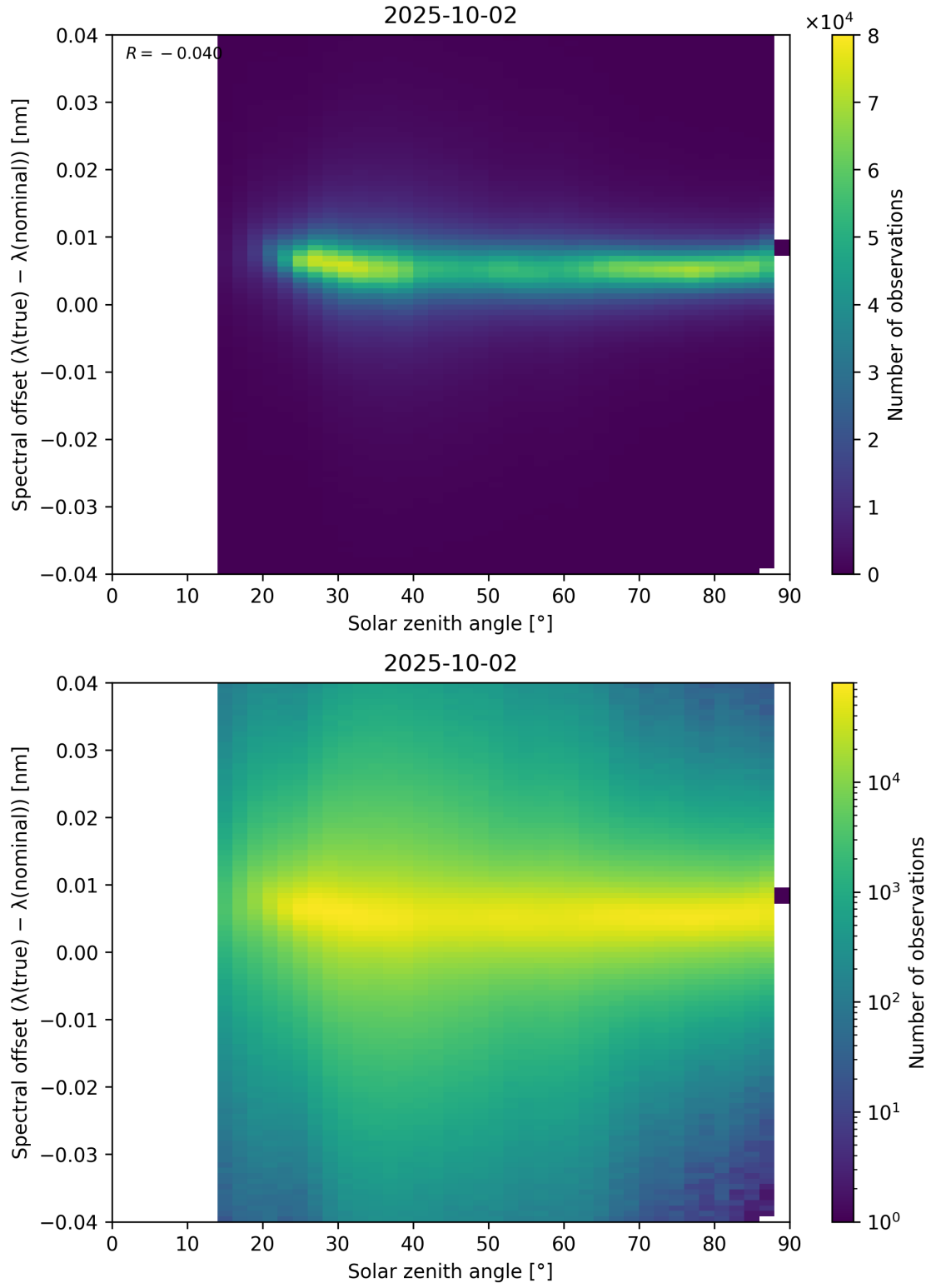
Figure 117: Scatter density plot of “Solar zenith angle” against “Spectral offset ( \lambda_{\text{true}} - \lambda_{\text{nominal}} )” for 2025-10-01 to 2025-10-03.
