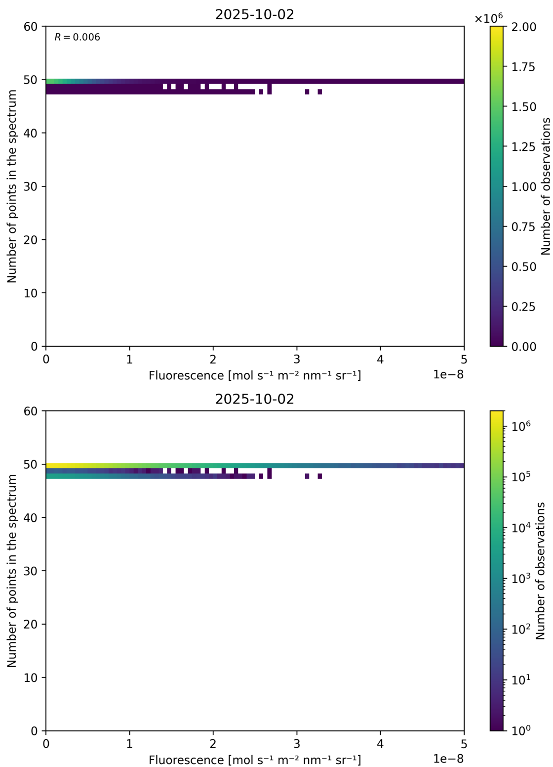
Figure 86: Scatter density plot of “Fluorescence” against “Number of points in the spectrum” for 2025-10-01 to 2025-10-03.
