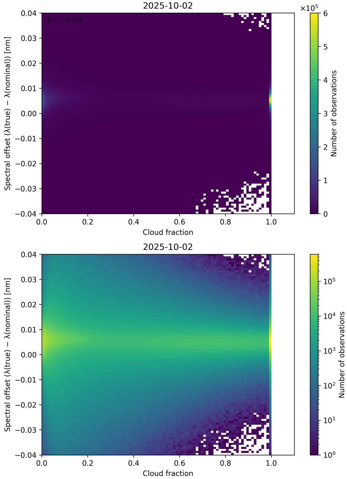
Figure 76: Scatter density plot of “Cloud fraction” against “Spectral offset ( \lambda_{\text{true}} - \lambda_{\text{nominal}} )” for 2025-10-01 to 2025-10-03.
