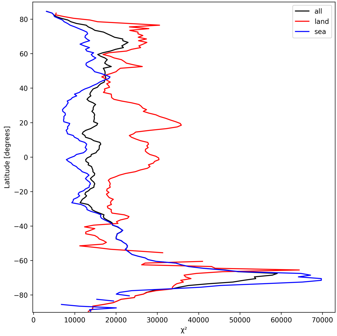
Figure 21: Zonal average of “ \chi^2 ” for 2025-10-01 to 2025-10-03.
