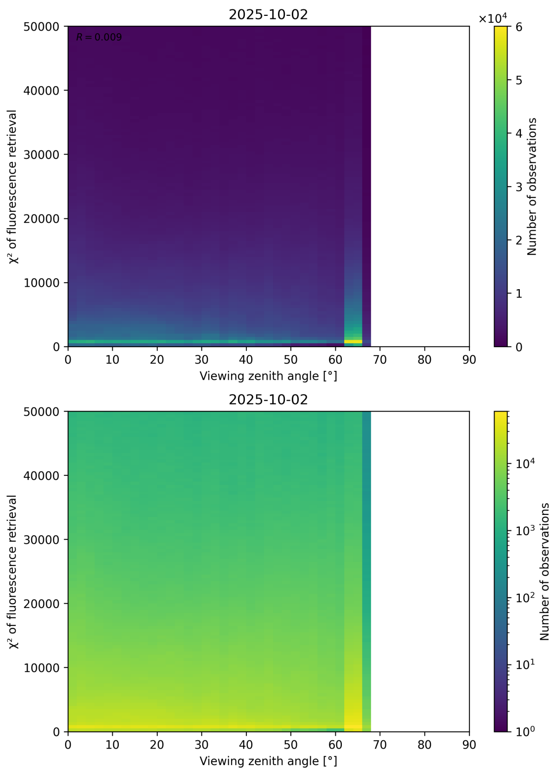
Figure 119: Scatter density plot of “Viewing zenith angle” against “ \chi^2 of fluorescence retrieval” for 2025-10-01 to 2025-10-03.
