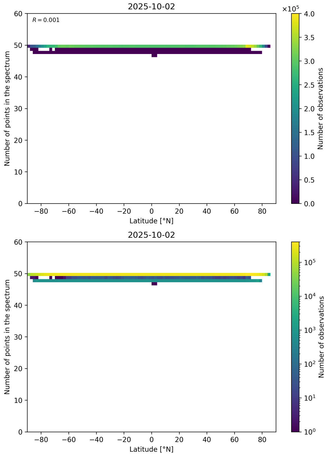
Figure 94: Scatter density plot of “Latitude” against “Number of points in the spectrum” for 2025-10-01 to 2025-10-03.
