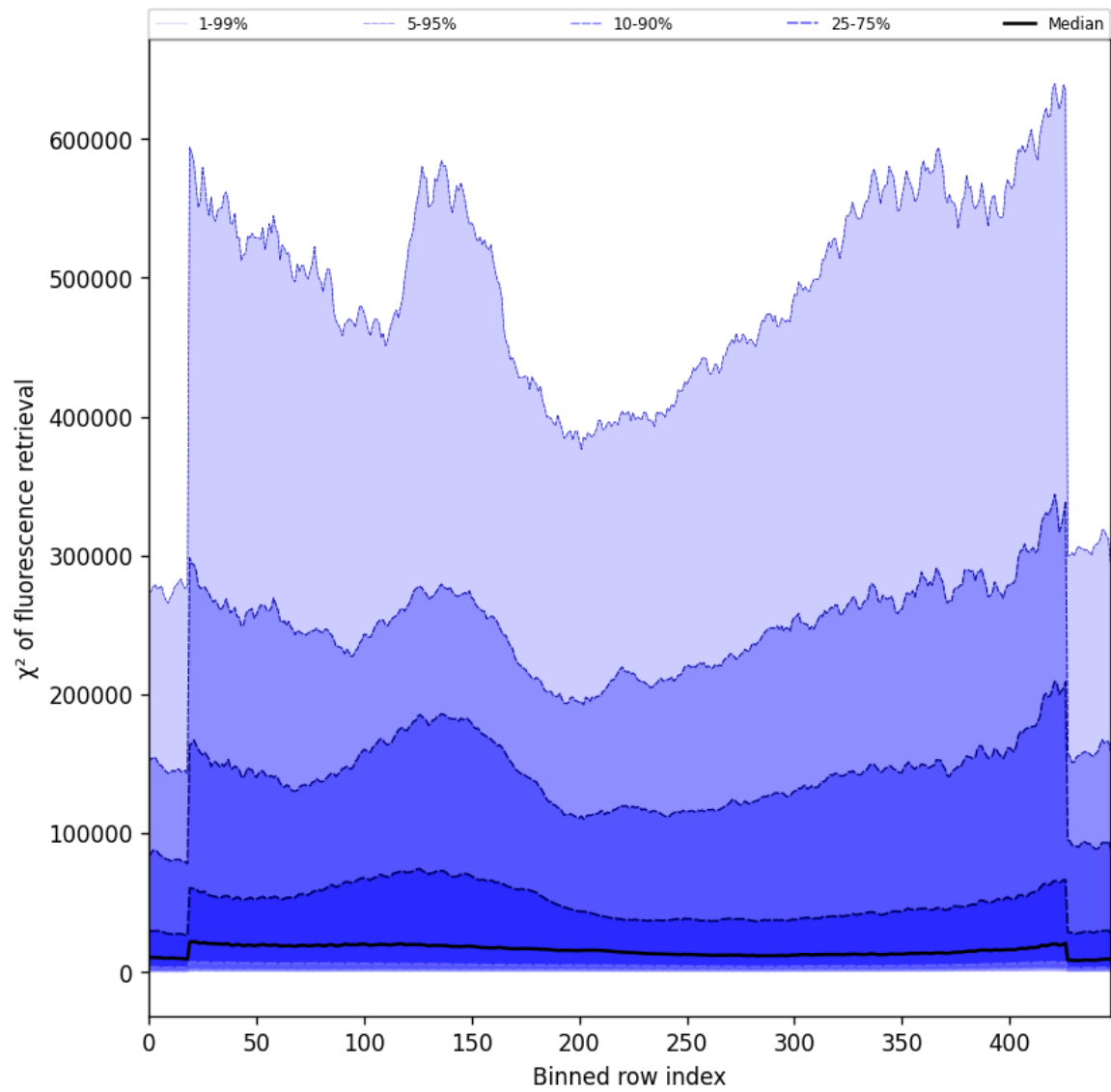
Figure 59: Along track statistics of “ \chi^2 of fluorescence retrieval” for 2025-10-01 to 2025-10-03
