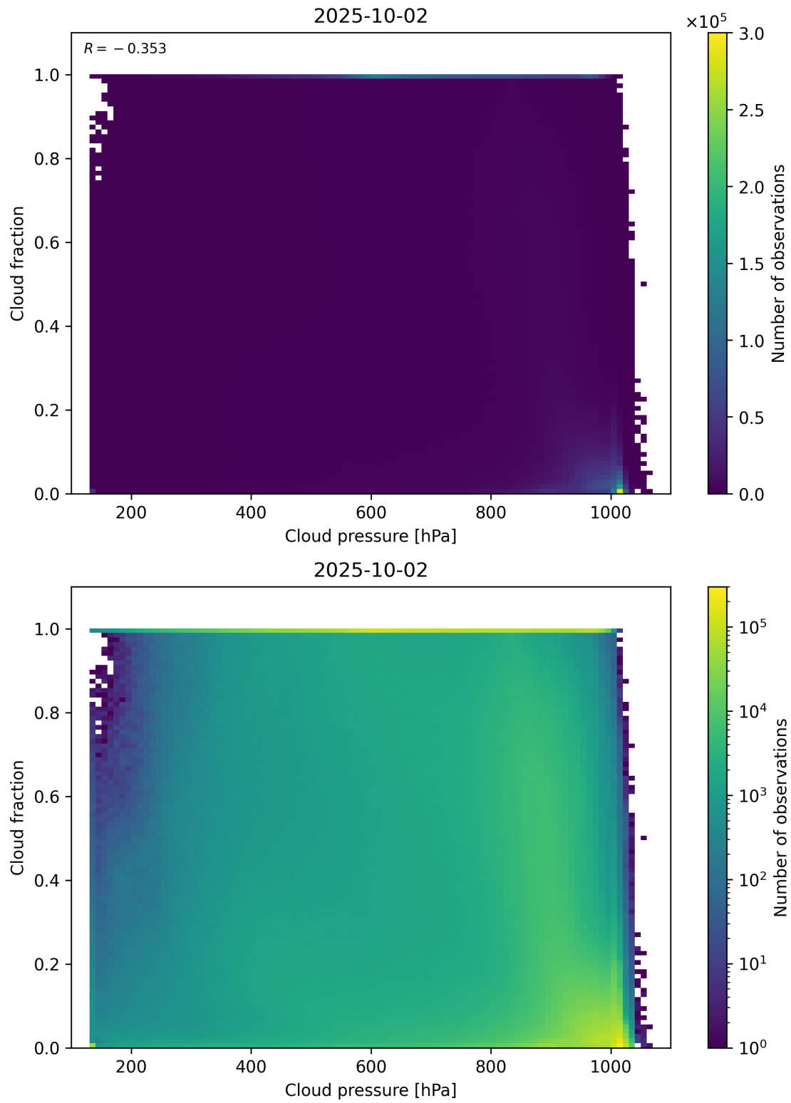
Figure 79: Scatter density plot of “Cloud pressure” against “Cloud fraction” for 2025-10-01 to 2025-10-03.
