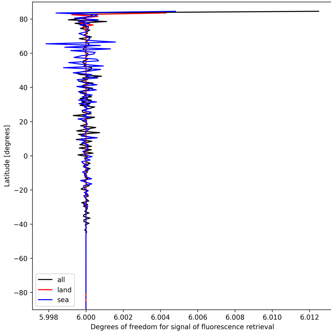
Figure 26: Zonal average of “Degrees of freedom for signal of fluorescence retrieval” for 2025-10-01 to 2025-10-03.
