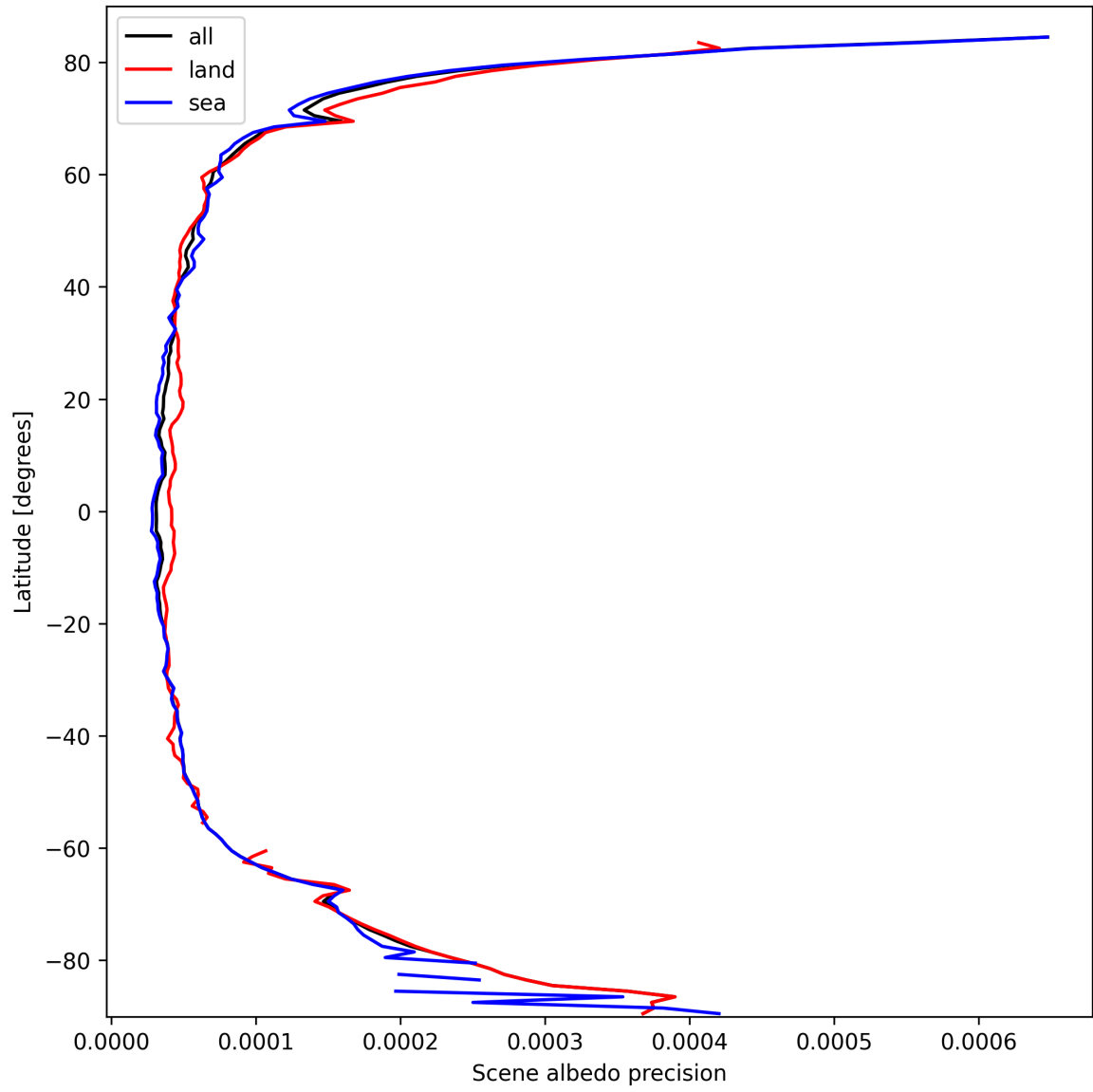
Figure 18: Zonal average of “Scene albedo precision” for 2025-10-01 to 2025-10-03.
