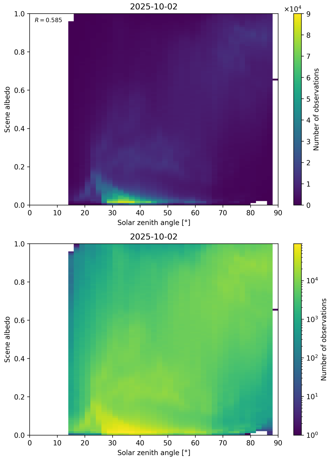
Figure 116: Scatter density plot of “Solar zenith angle” against “Scene albedo” for 2025-10-01 to 2025-10-03.
