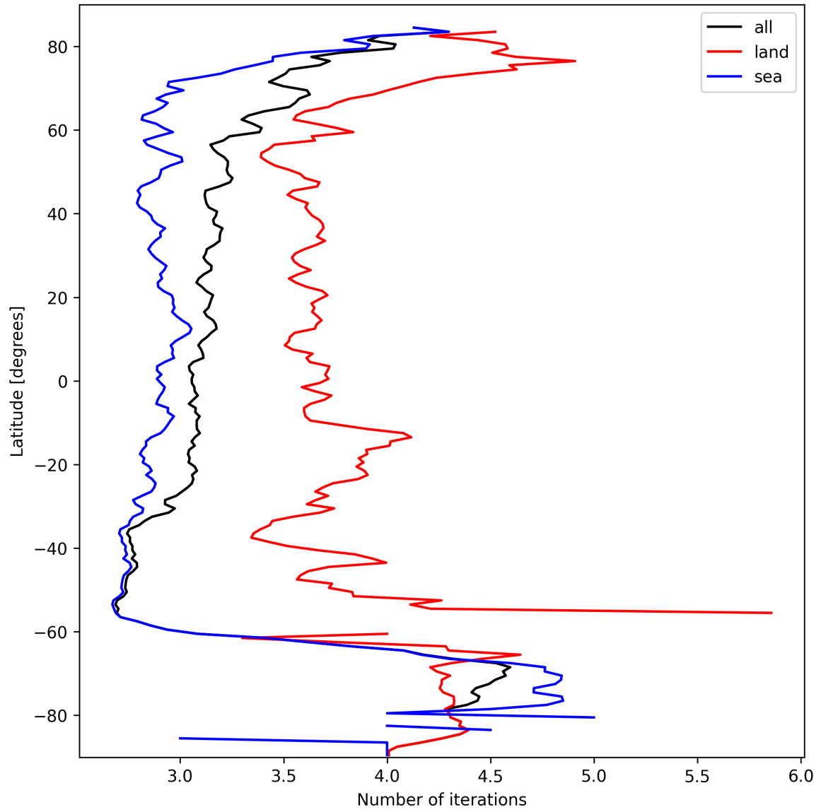
Figure 22: Zonal average of “Number of iterations” for 2025-10-01 to 2025-10-03.
