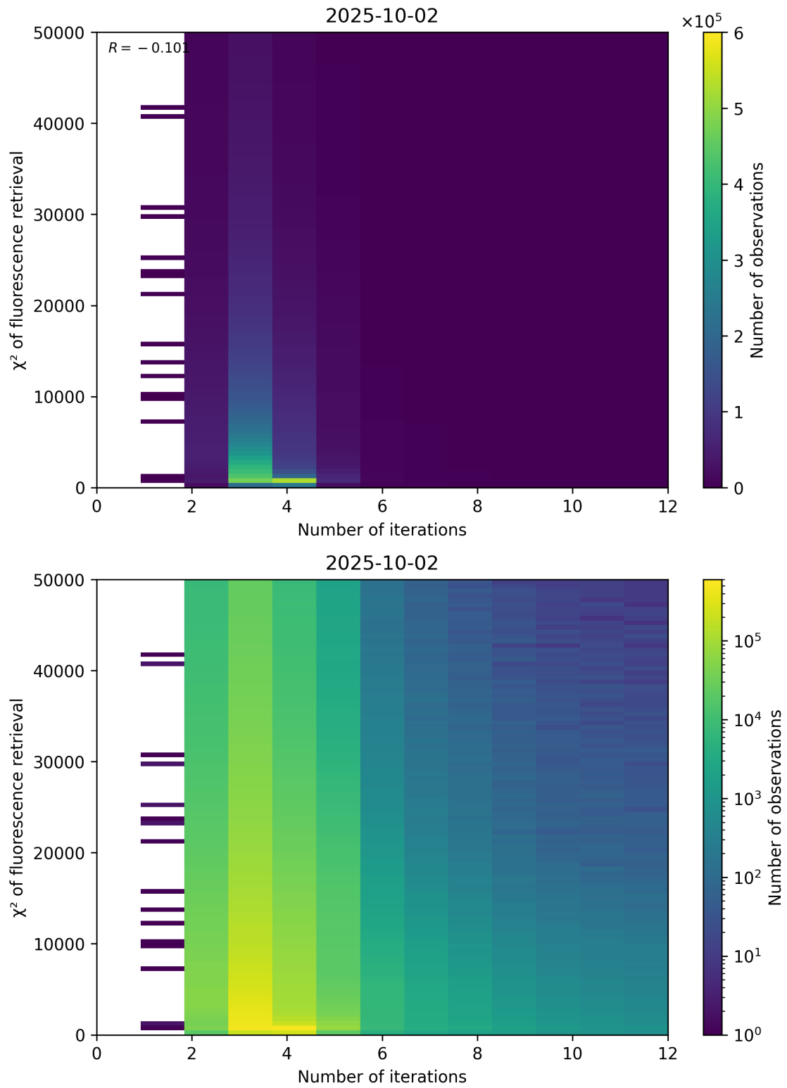
Figure 97: Scatter density plot of “Number of iterations” against “ \chi^2 of fluorescence retrieval” for 2025-10-01 to 2025-10-03.
