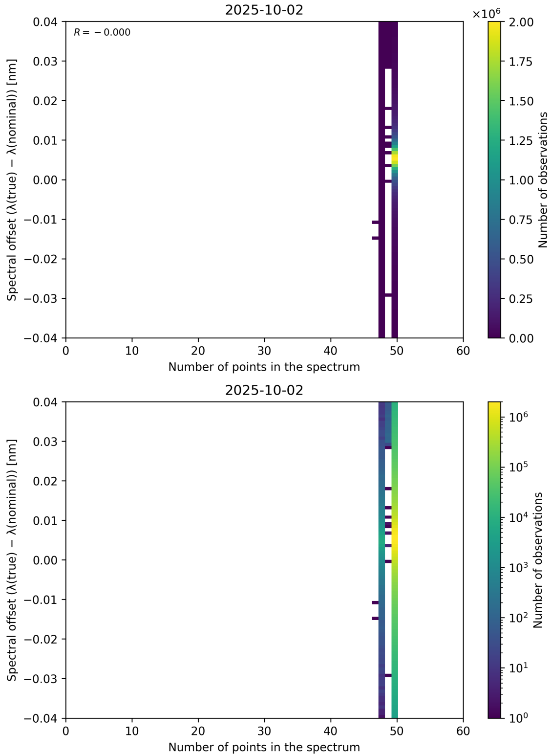
Figure 101: Scatter density plot of “Number of points in the spectrum” against “Spectral offset ( \lambda_{\text{true}} - \lambda_{\text{nominal}} )” for 2025-10-01 to 2025-10-03.
