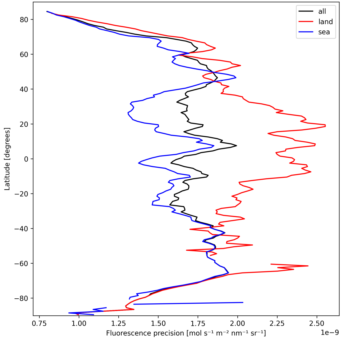
Figure 24: Zonal average of “Fluorescence precision” for 2025-10-01 to 2025-10-03.
