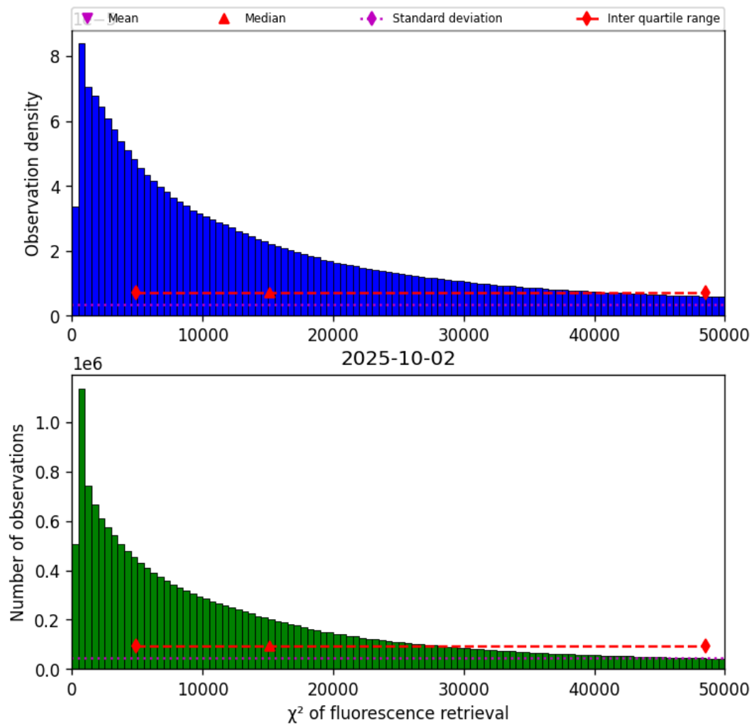
Figure 42: Histogram of “ \chi^2 of fluorescence retrieval” for 2025-10-01 to 2025-10-03
