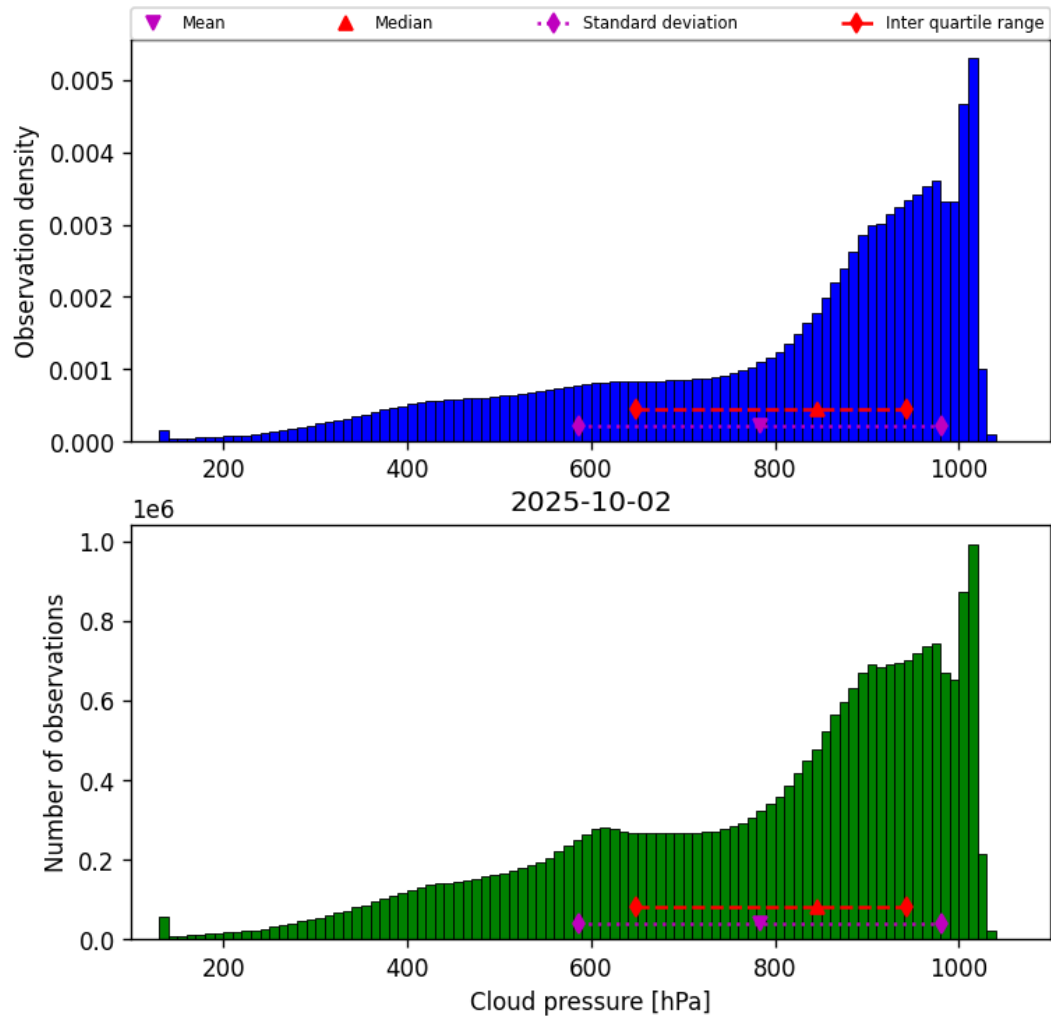
Figure 30: Histogram of “Cloud pressure” for 2025-10-01 to 2025-10-03
