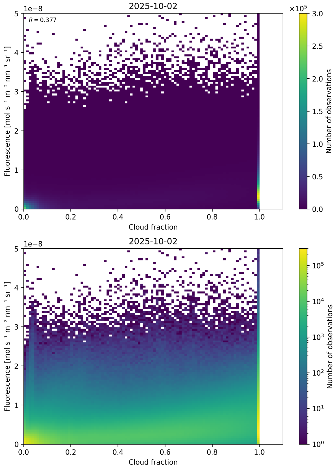
Figure 72: Scatter density plot of “Cloud fraction” against “Fluorescence” for 2025-10-01 to 2025-10-03.
