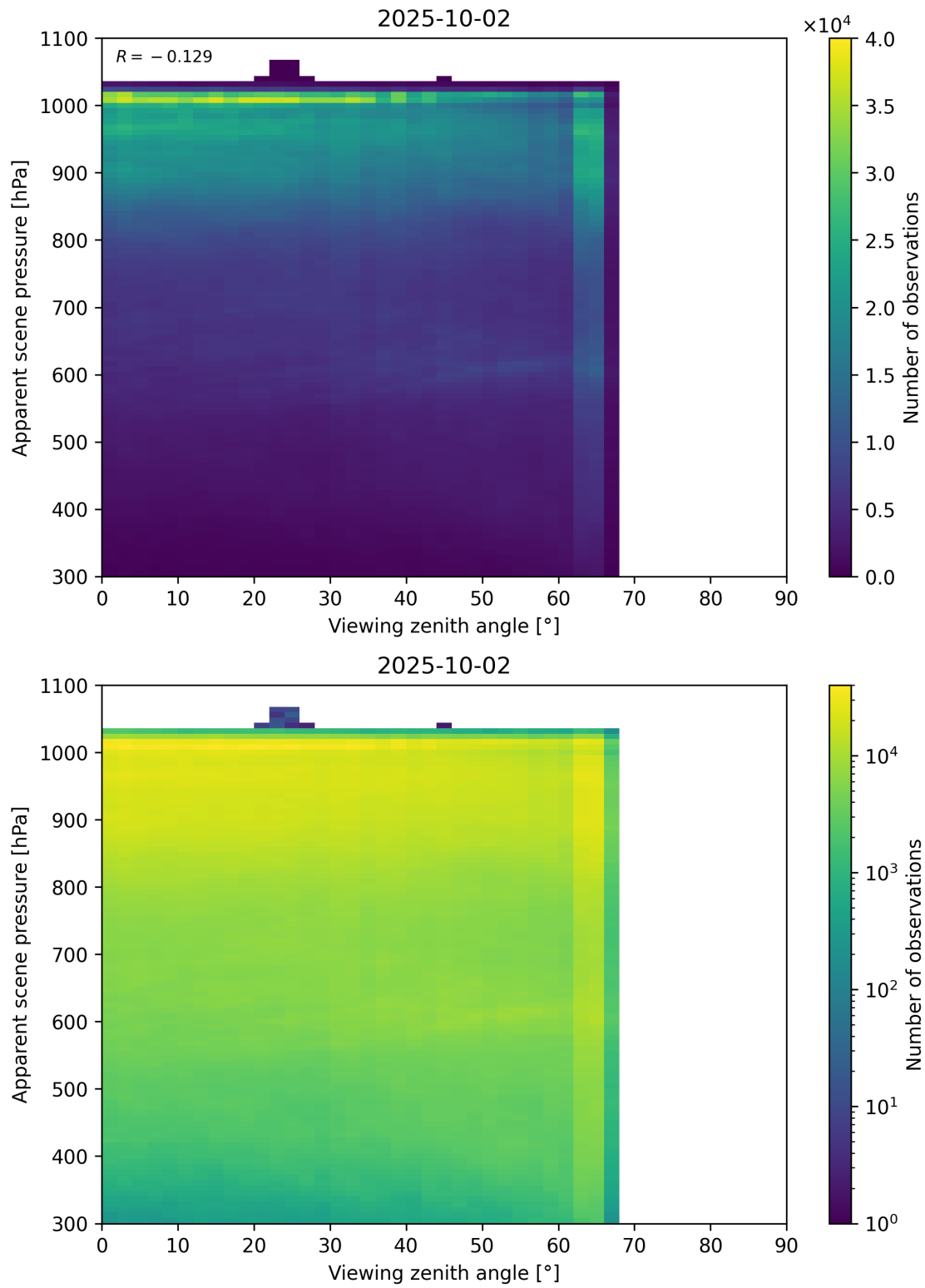
Figure 118: Scatter density plot of “Viewing zenith angle” against “Apparent scene pressure” for 2025-10-01 to 2025-10-03.
