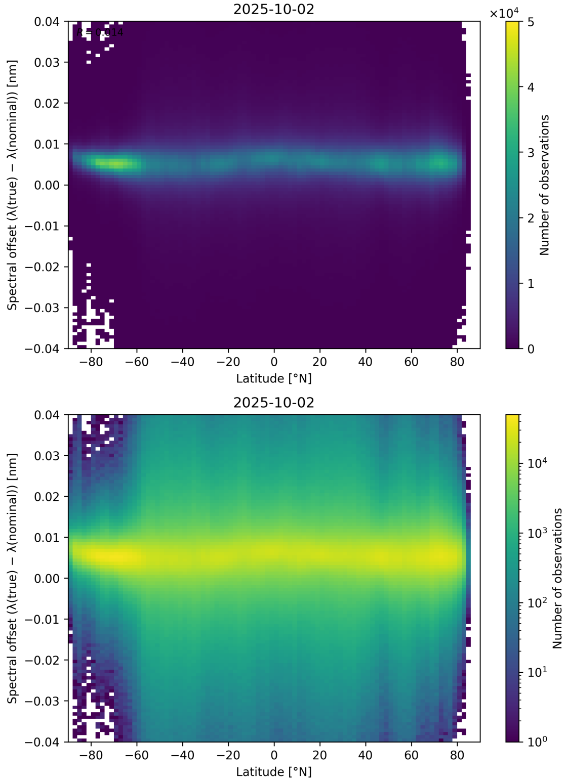
Figure 96: Scatter density plot of “Latitude” against “Spectral offset ( \lambda_{\text{true}} - \lambda_{\text{nominal}} )” for 2025-10-01 to 2025-10-03.
