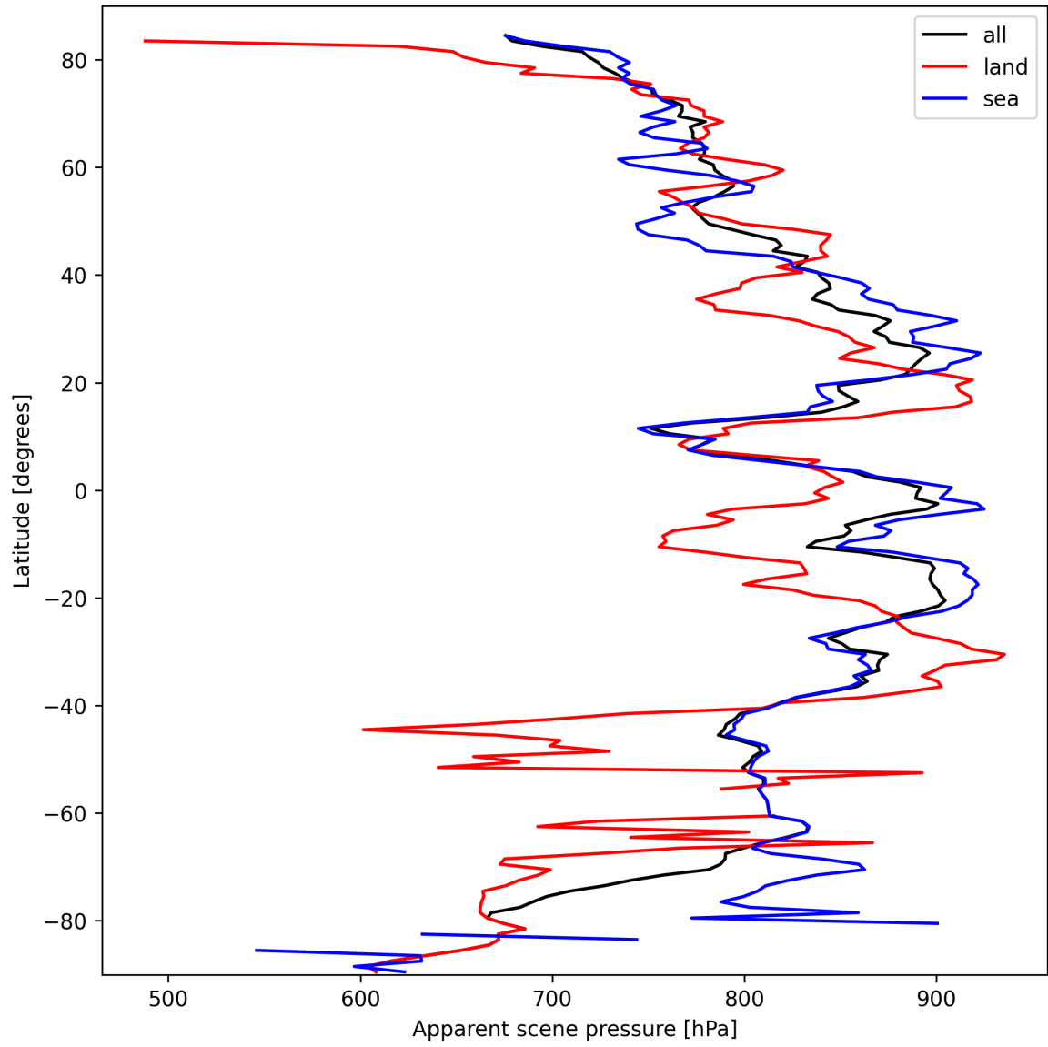
Figure 19: Zonal average of “Apparent scene pressure” for 2025-10-01 to 2025-10-03.
