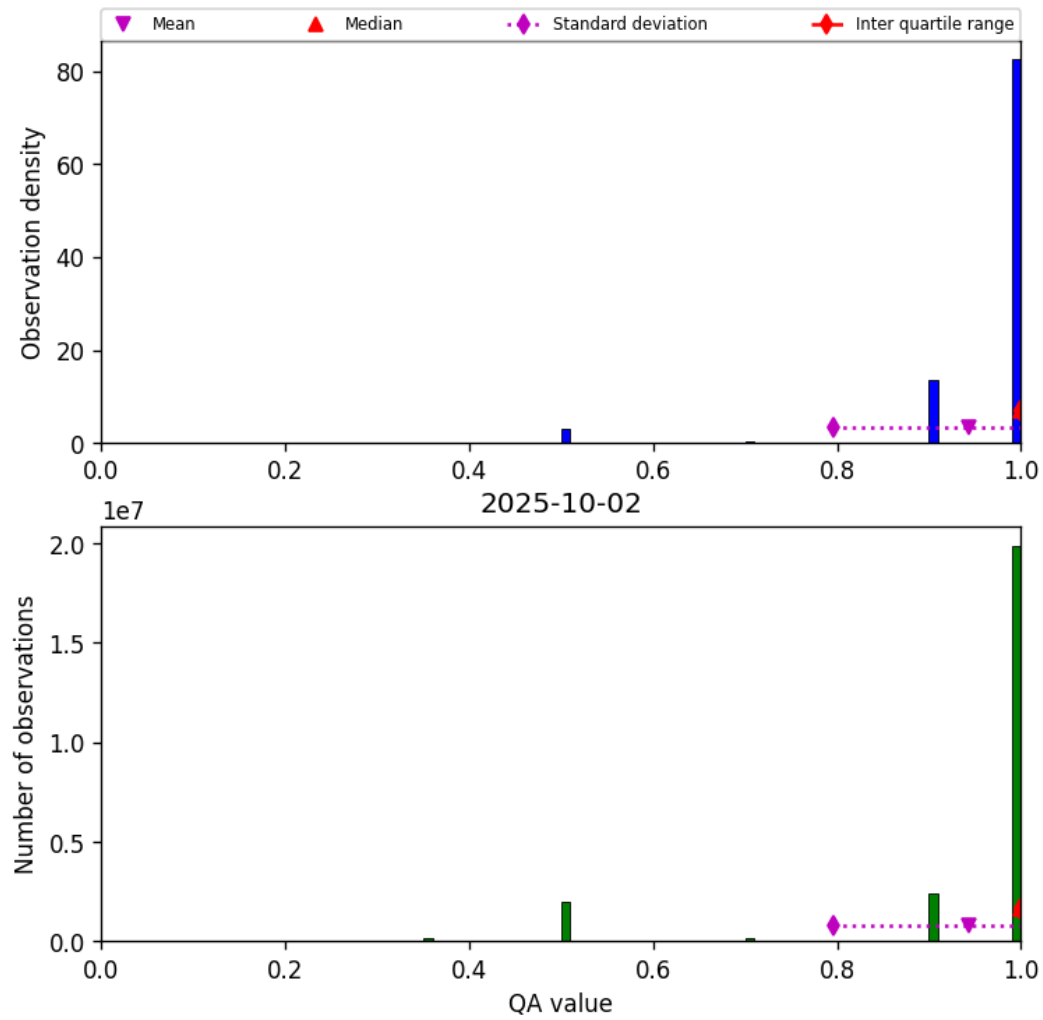
Figure 29: Histogram of "QA value" for 2025-10-01 to 2025-10-03
