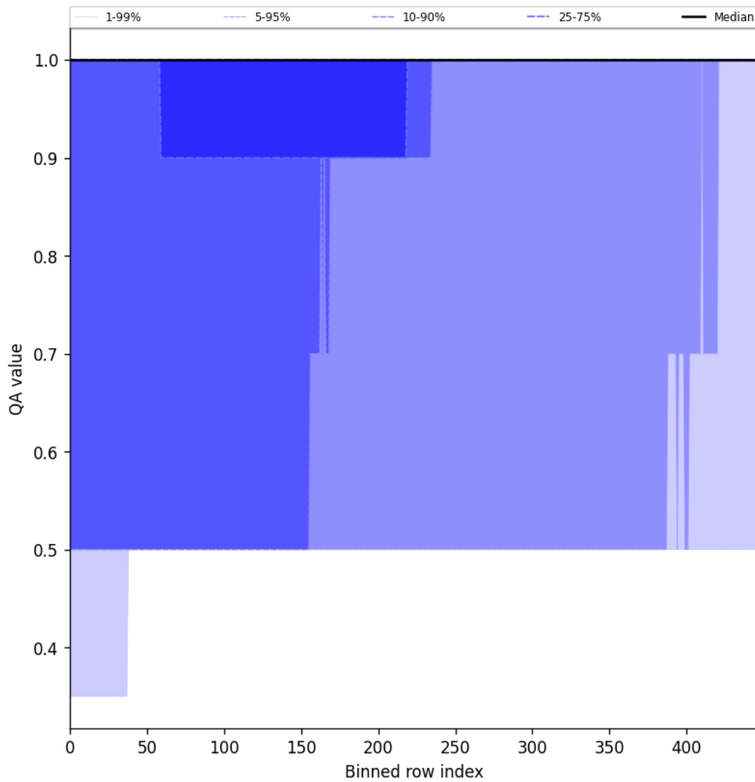
Figure 46: Along track statistics of “QA value” for 2025-10-01 to 2025-10-03
