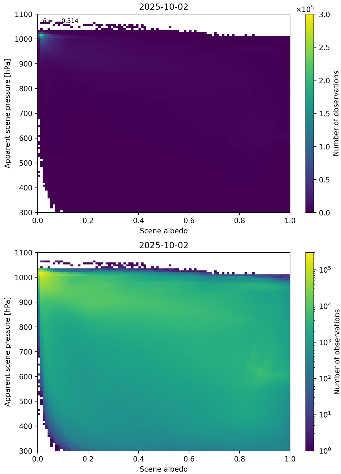
Figure 102: Scatter density plot of “Scene albedo” against “Apparent scene pressure” for 2025-10-01 to 2025-10-03.
