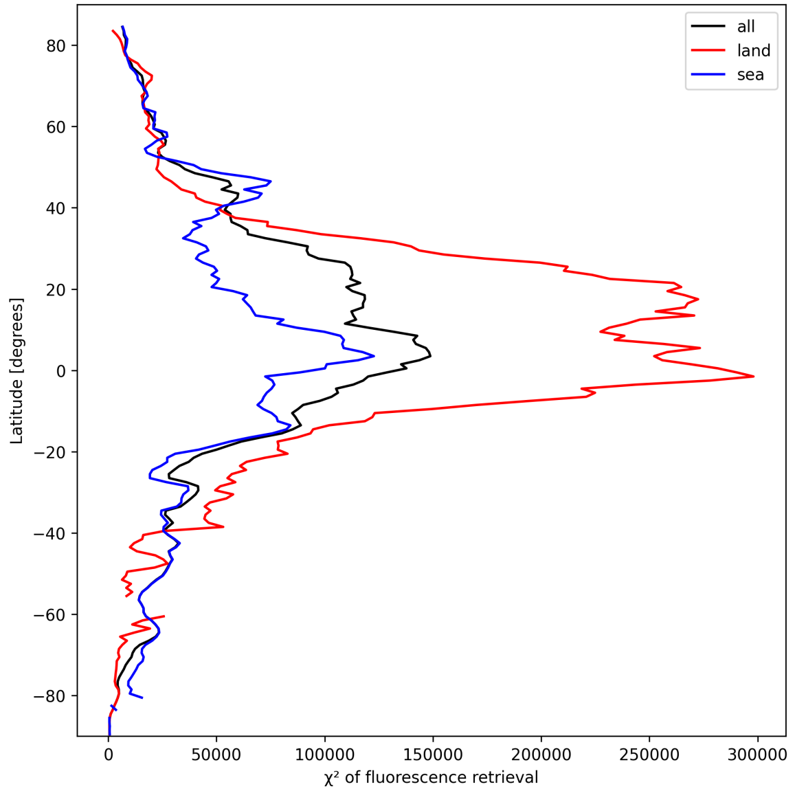
Figure 25: Zonal average of “ \chi^2 of fluorescence retrieval” for 2025-10-01 to 2025-10-03.
