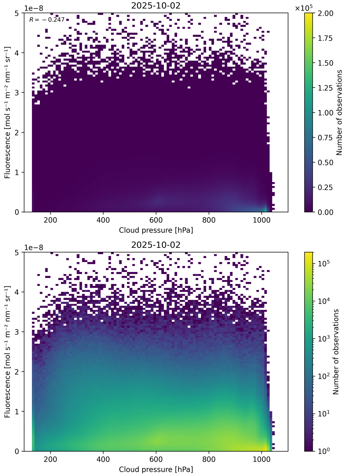
Figure 80: Scatter density plot of “Cloud pressure” against “Fluorescence” for 2025-10-01 to 2025-10-03.
