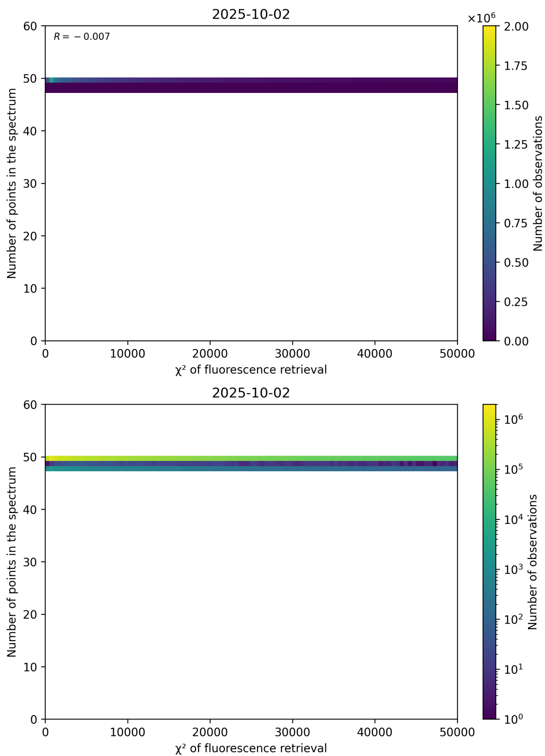
Figure 68: Scatter density plot of “ \chi^2 of fluorescence retrieval” against “Number of points in the spectrum” for 2025-10-01 to 2025-10-03.
