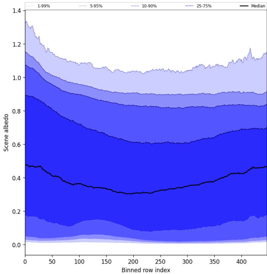
Figure 51: Along track statistics of “Scene albedo” for 2025-10-01 to 2025-10-03
