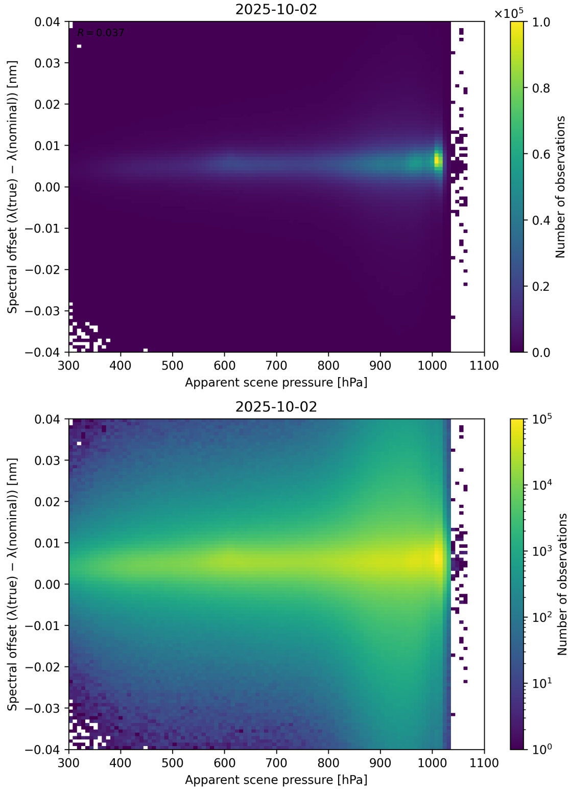
Figure 67: Scatter density plot of “Apparent scene pressure” against “Spectral offset ( \lambda_{\text{true}} - \lambda_{\text{nominal}} )” for 2025-10-01 to 2025-10-03.
