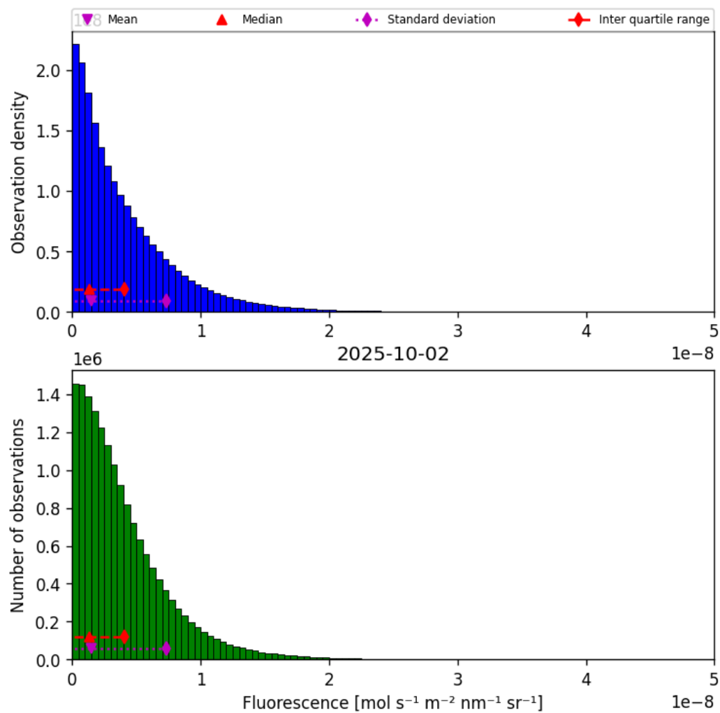
Figure 40: Histogram of “Fluorescence” for 2025-10-01 to 2025-10-03
