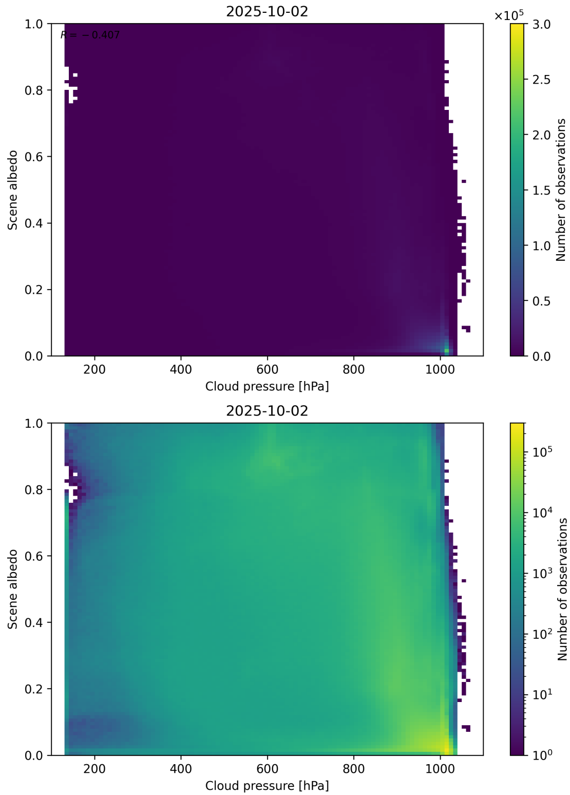
Figure 83: Scatter density plot of “Cloud pressure” against “Scene albedo” for 2025-10-01 to 2025-10-03.
