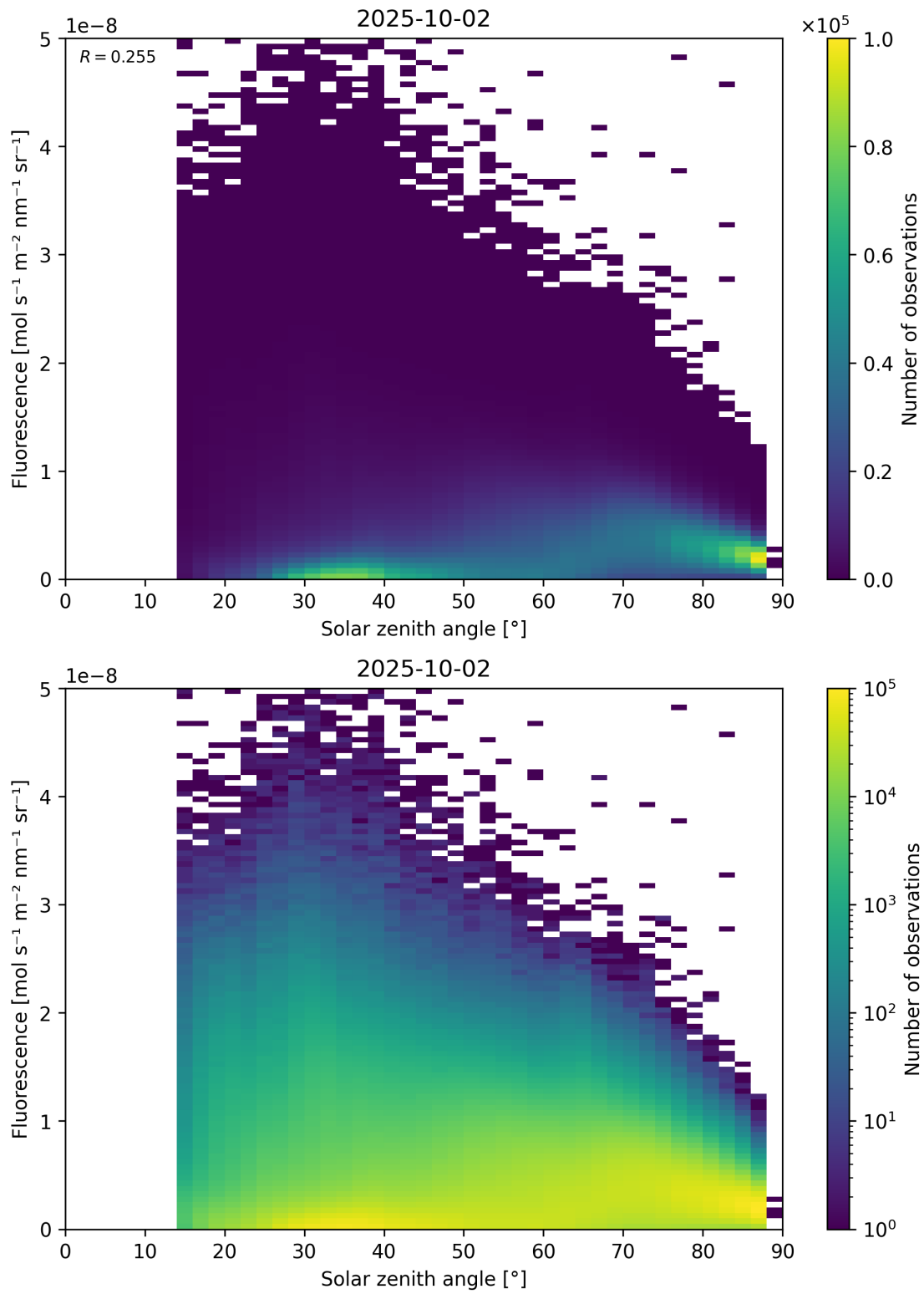
Figure 112: Scatter density plot of “Solar zenith angle” against “Fluorescence” for 2025-10-01 to 2025-10-03.
