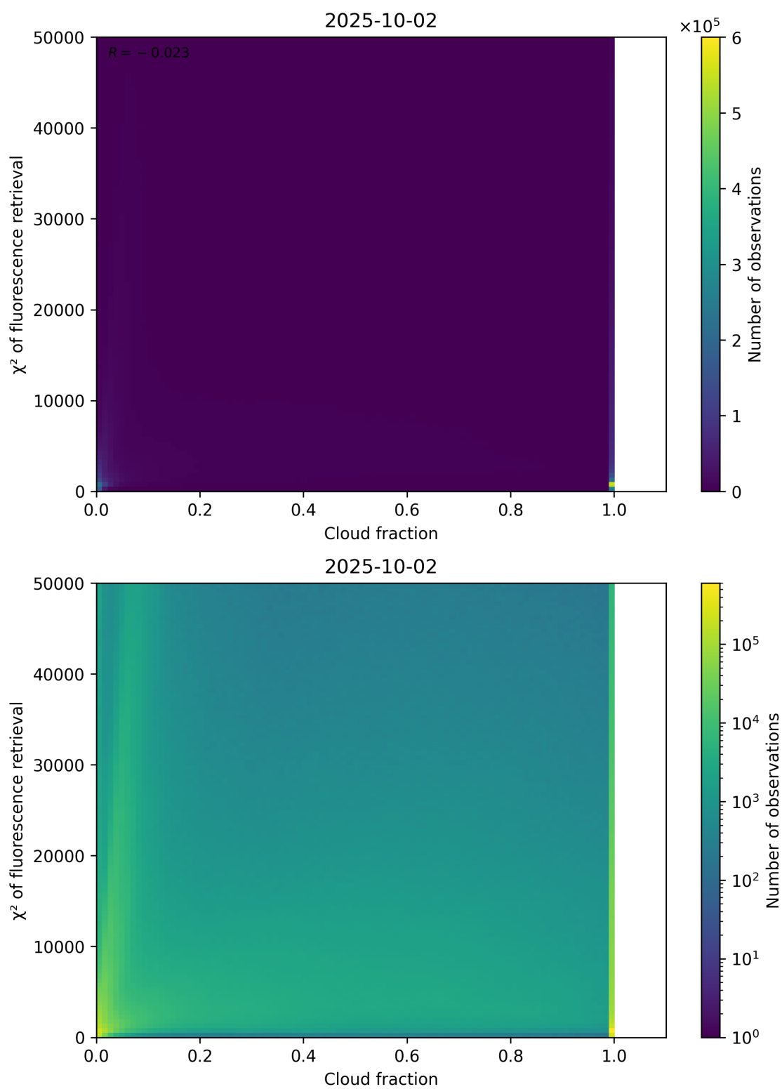
Figure 71: Scatter density plot of “Cloud fraction” against “ \chi^2 of fluorescence retrieval” for 2025-10-01 to 2025-10-03.
