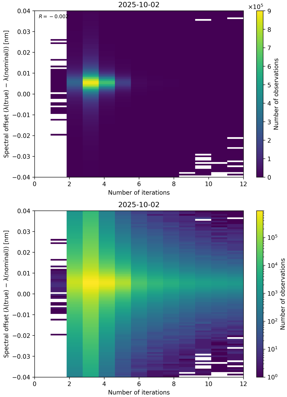
Figure 100: Scatter density plot of “Number of iterations” against “Spectral offset ( \lambda_{\text{true}} - \lambda_{\text{nominal}} )” for 2025-10-01 to 2025-10-03.
