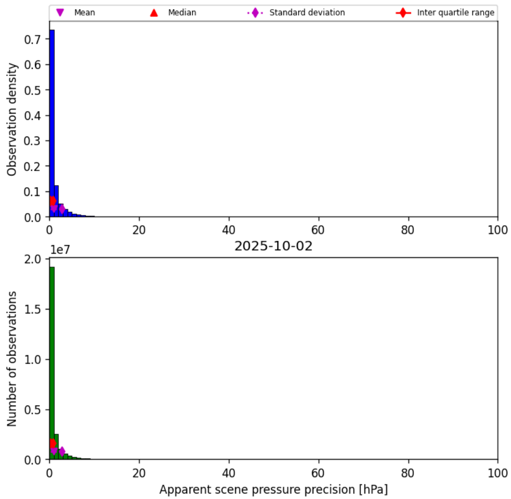
Figure 37: Histogram of “Apparent scene pressure precision” for 2025-10-01 to 2025-10-03
