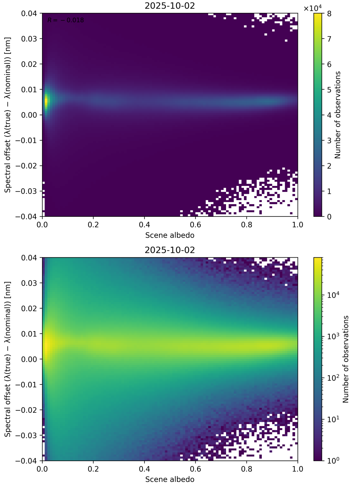
Figure 107: Scatter density plot of “Scene albedo” against “Spectral offset ( \lambda_{\text{true}} - \lambda_{\text{nominal}} )” for 2025-10-01 to 2025-10-03.
