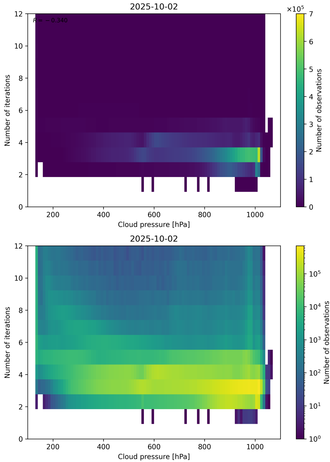
Figure 81: Scatter density plot of “Cloud pressure” against “Number of iterations” for 2025-10-01 to 2025-10-03.
