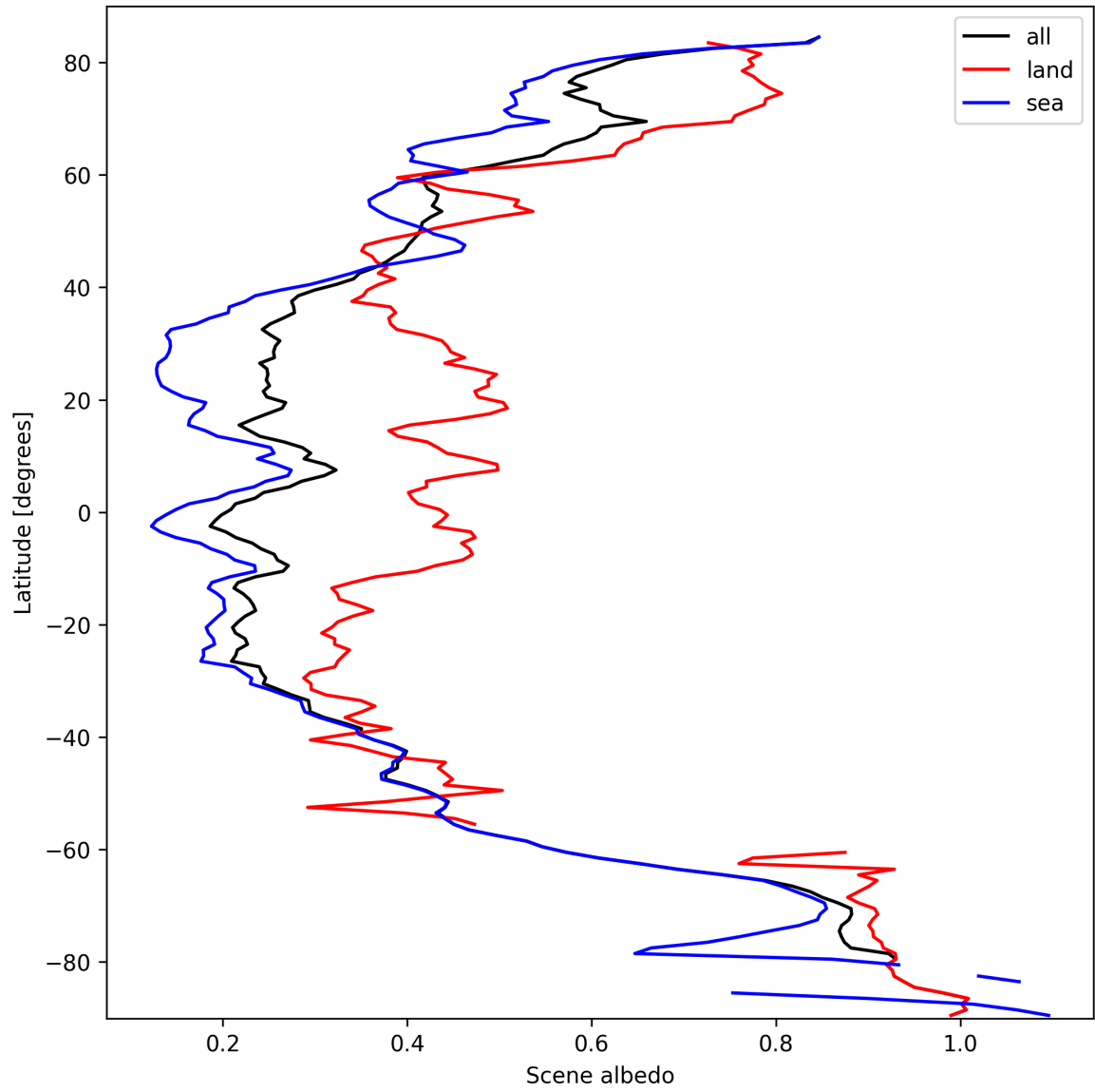
Figure 17: Zonal average of “Scene albedo” for 2025-10-01 to 2025-10-03.
