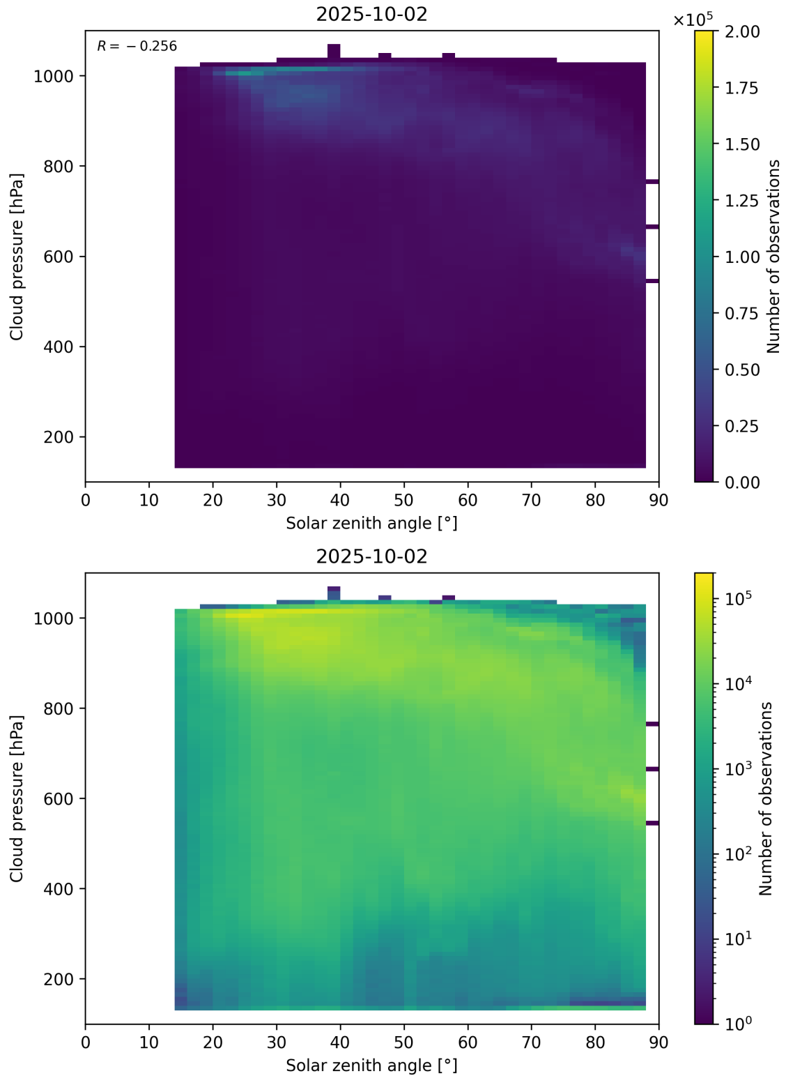
Figure 111: Scatter density plot of “Solar zenith angle” against “Cloud pressure” for 2025-10-01 to 2025-10-03.
