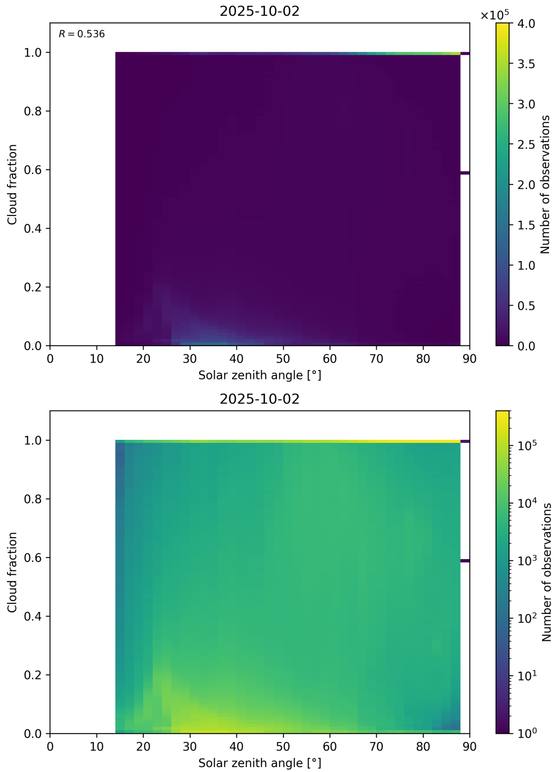
Figure 110: Scatter density plot of “Solar zenith angle” against “Cloud fraction” for 2025-10-01 to 2025-10-03.
