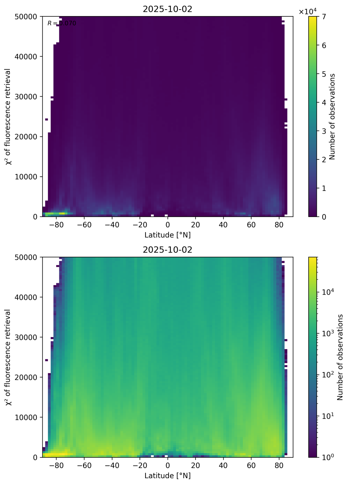
Figure 89: Scatter density plot of “Latitude” against “ \chi^2 of fluorescence retrieval” for 2025-10-01 to 2025-10-03.
