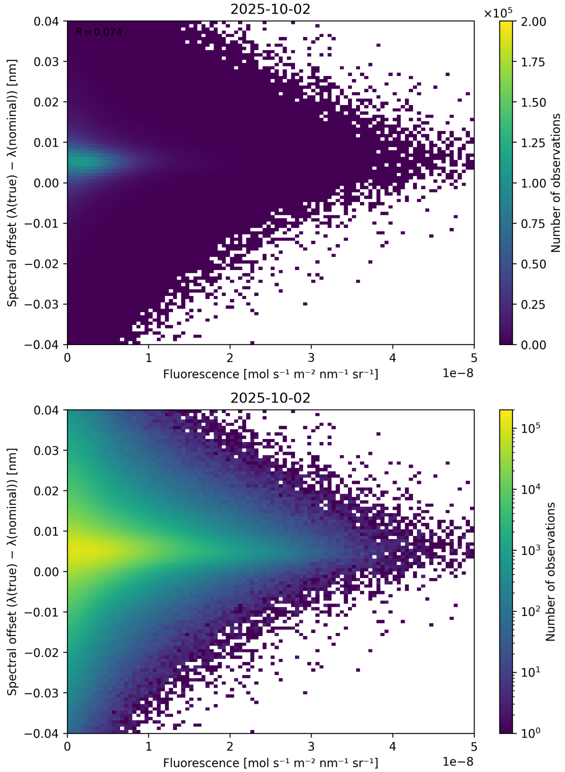
Figure 87: Scatter density plot of “Fluorescence” against “Spectral offset ( \lambda_{\text{true}} - \lambda_{\text{nominal}} )” for 2025-10-01 to 2025-10-03.
