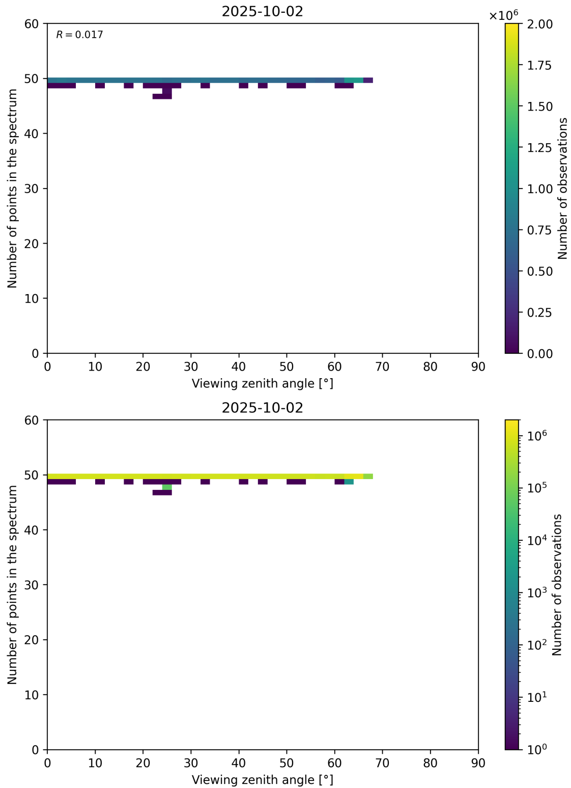
Figure 125: Scatter density plot of “Viewing zenith angle” against “Number of points in the spectrum” for 2025-10-01 to 2025-10-03.
