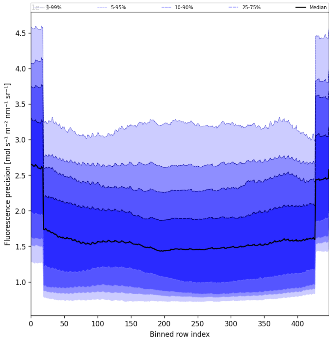
Figure 58: Along track statistics of “Fluorescence precision” for 2025-10-01 to 2025-10-03
