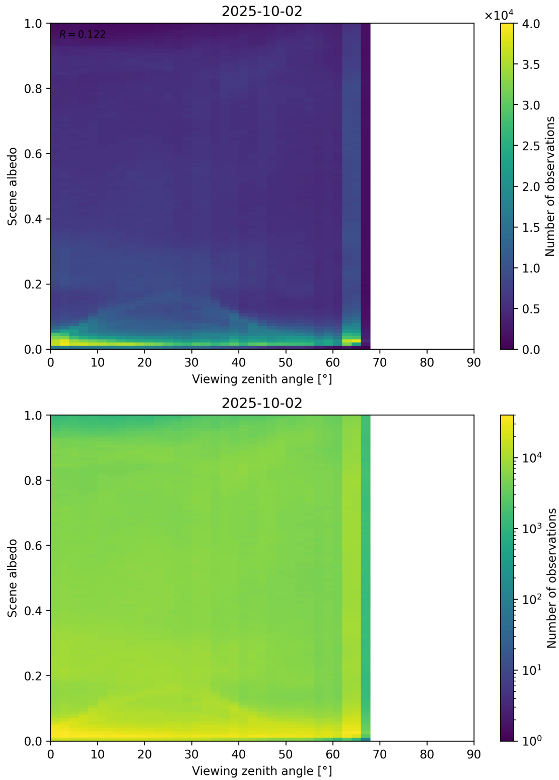
Figure 126: Scatter density plot of “Viewing zenith angle” against “Scene albedo” for 2025-10-01 to 2025-10-03.
