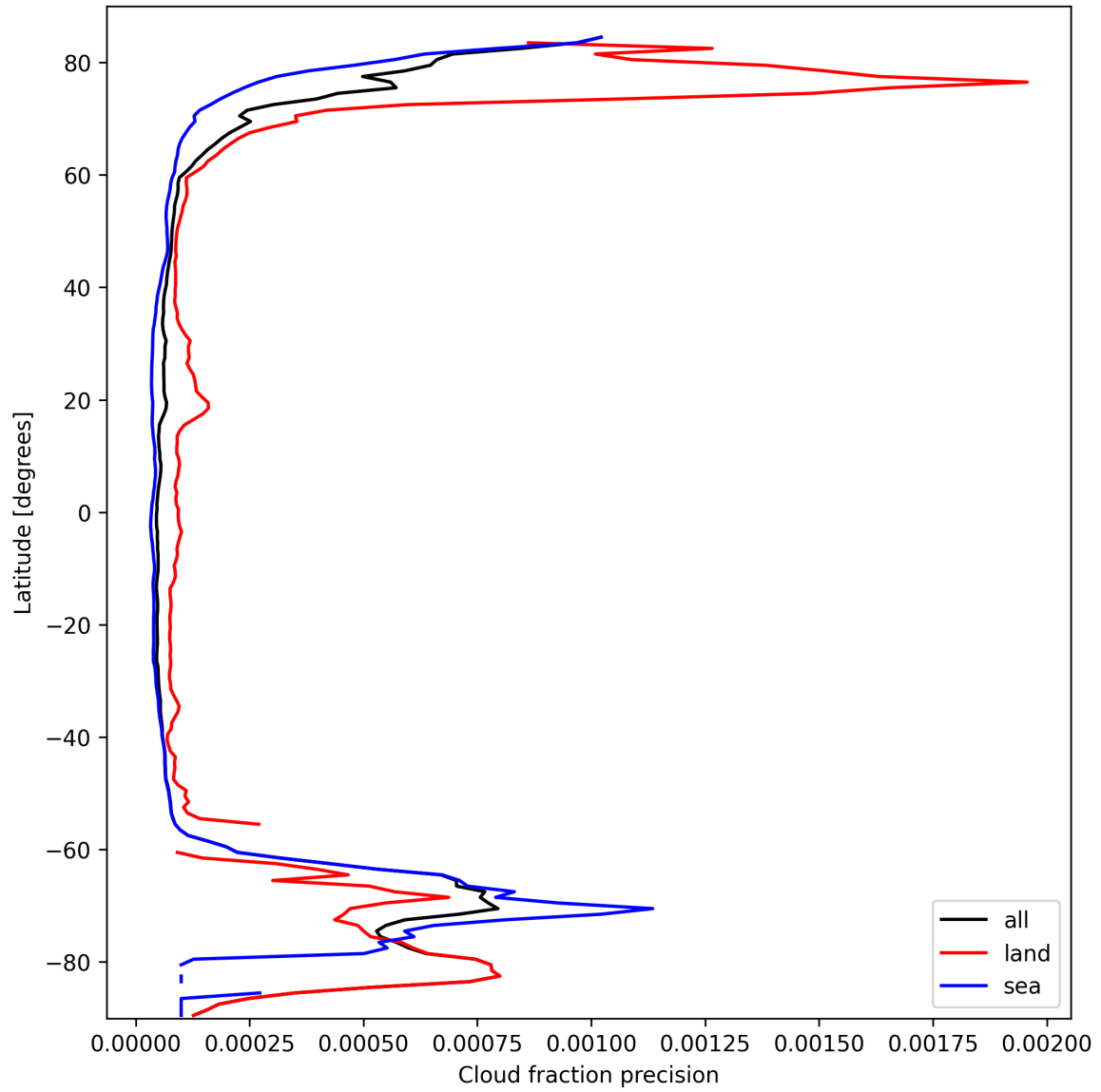
Figure 16: Zonal average of “Cloud fraction precision” for 2025-10-01 to 2025-10-03.
