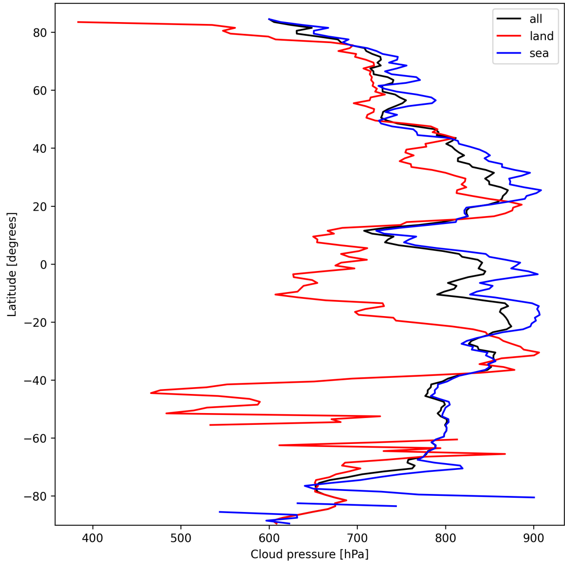
Figure 13: Zonal average of “Cloud pressure” for 2025-10-01 to 2025-10-03.
