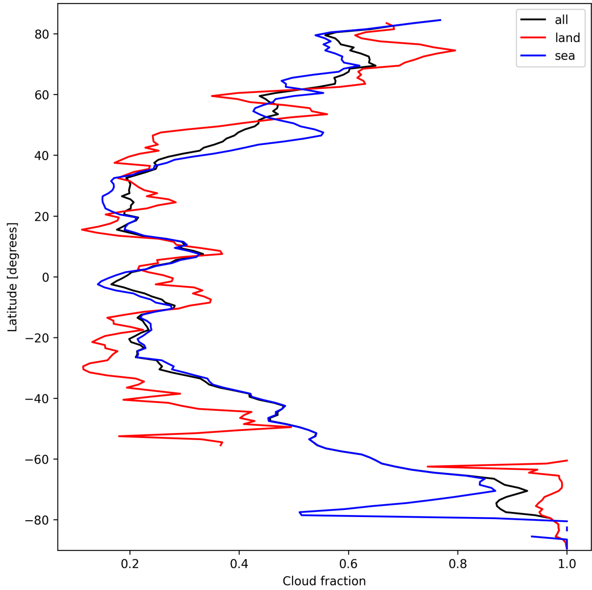
Figure 15: Zonal average of “Cloud fraction” for 2025-10-01 to 2025-10-03.
