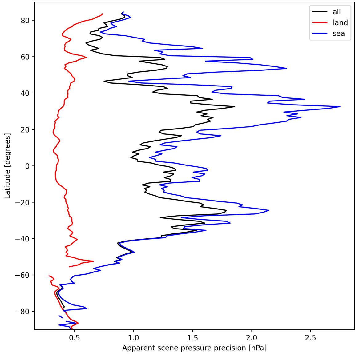
Figure 20: Zonal average of “Apparent scene pressure precision” for 2025-10-01 to 2025-10-03.
