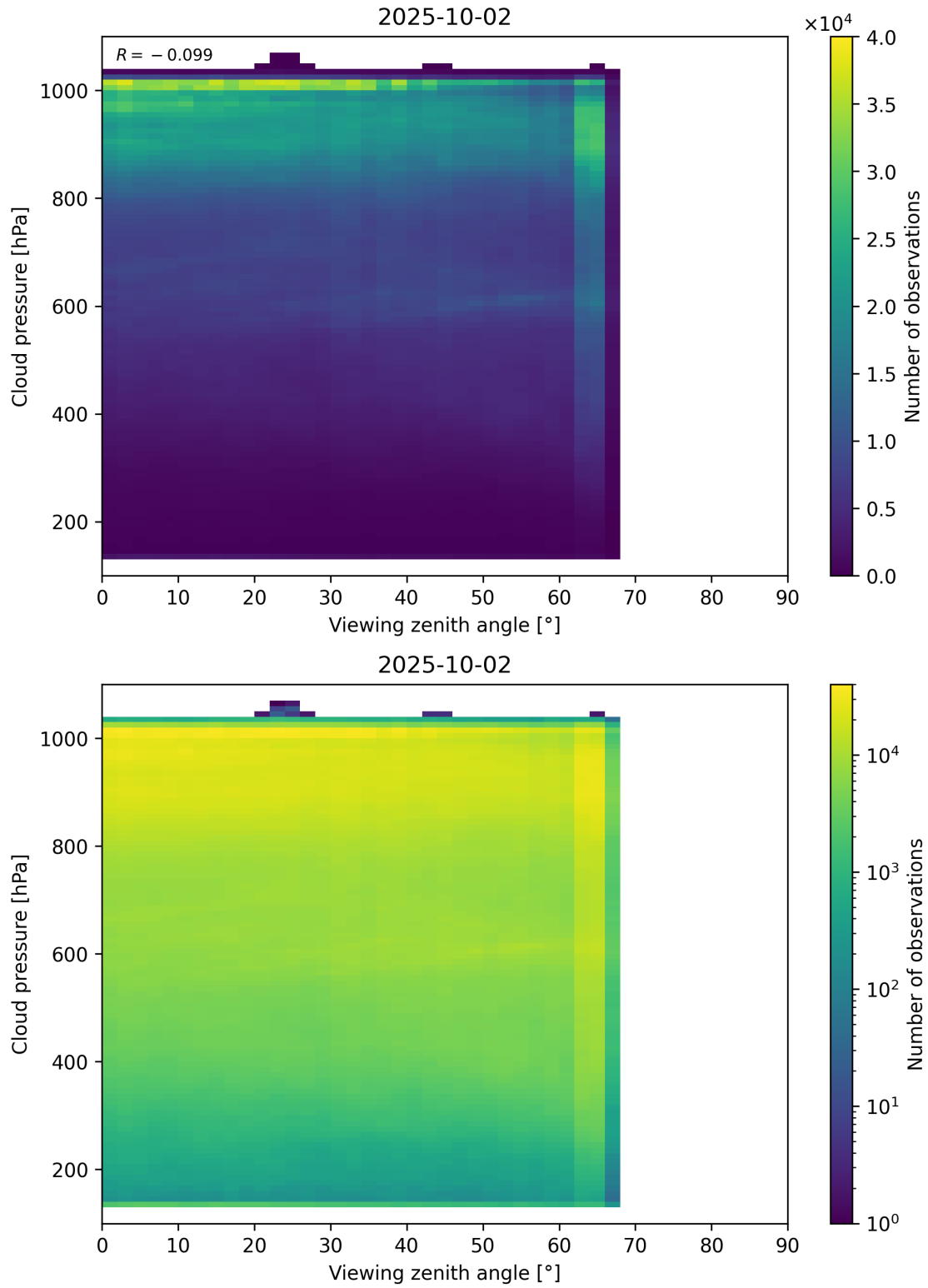
Figure 121: Scatter density plot of “Viewing zenith angle” against “Cloud pressure” for 2025-10-01 to 2025-10-03.
