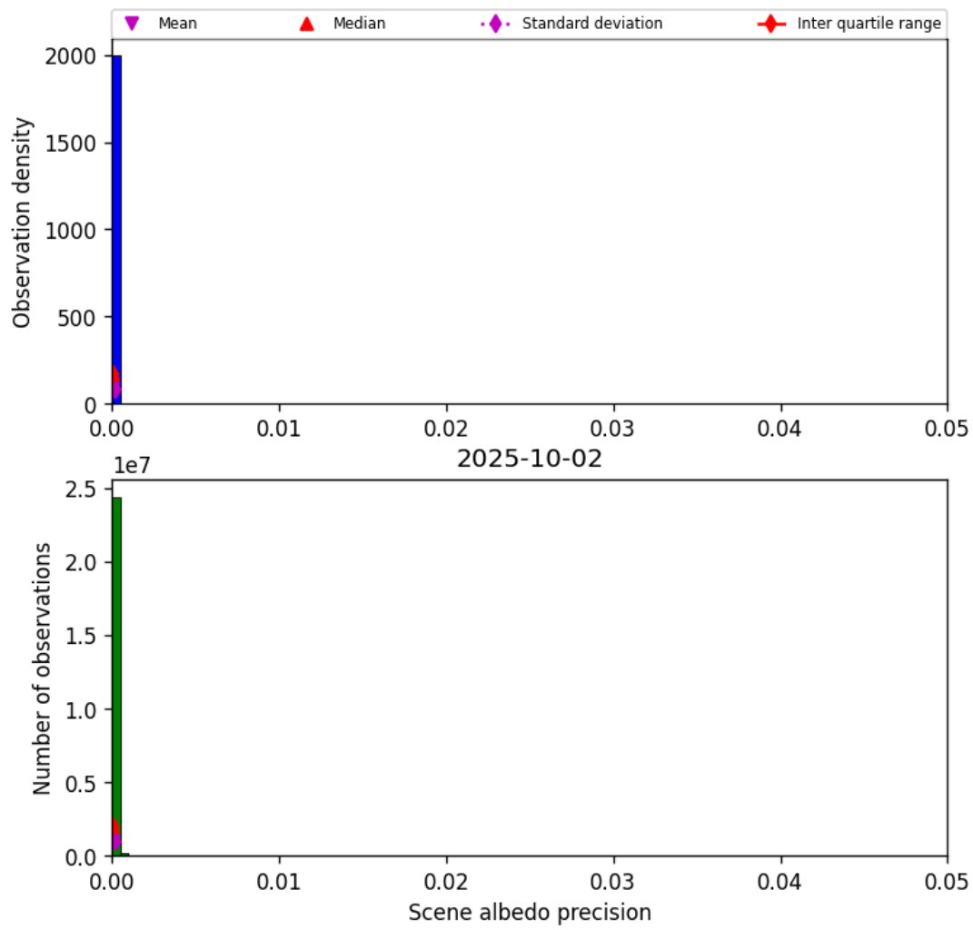
Figure 35: Histogram of “Scene albedo precision” for 2025-10-01 to 2025-10-03
