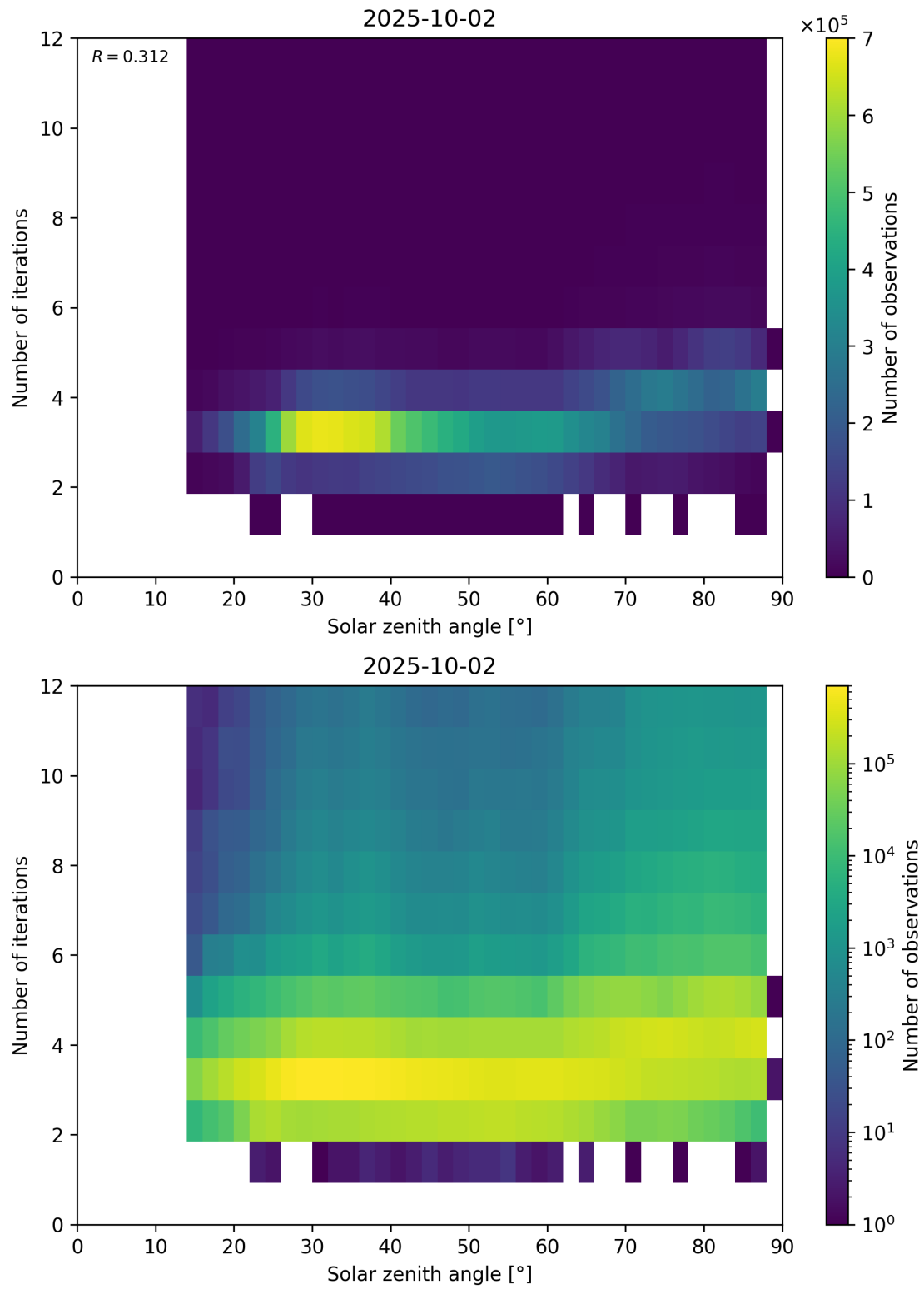
Figure 114: Scatter density plot of “Solar zenith angle” against “Number of iterations” for 2025-10-01 to 2025-10-03.
