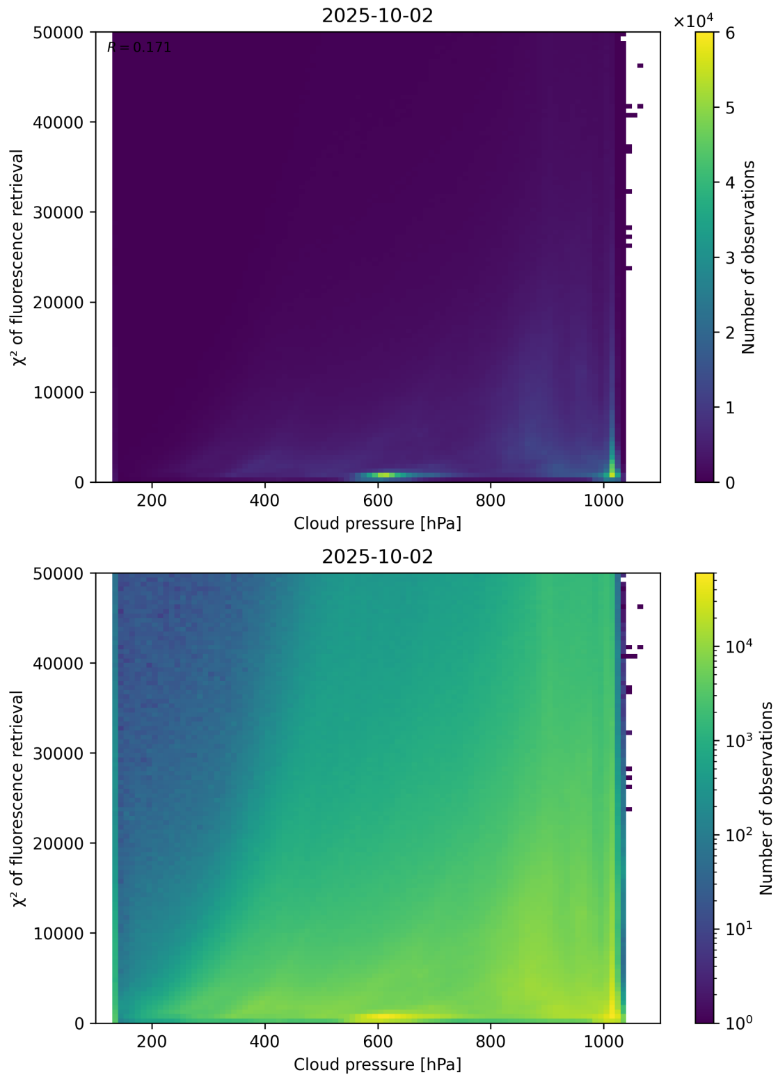
Figure 78: Scatter density plot of “Cloud pressure” against “ \chi^2 of fluorescence retrieval” for 2025-10-01 to 2025-10-03.
