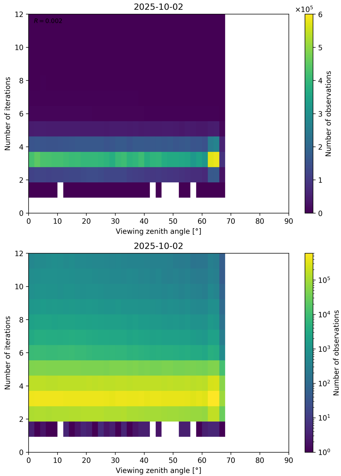
Figure 124: Scatter density plot of “Viewing zenith angle” against “Number of iterations” for 2025-10-01 to 2025-10-03.
