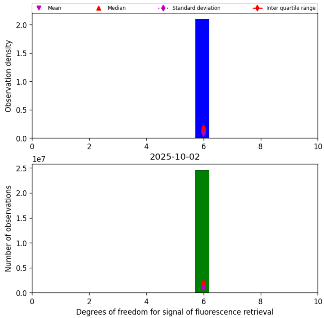
Figure 43: Histogram of “Degrees of freedom for signal of fluorescence retrieval” for 2025-10-01 to 2025-10-03
