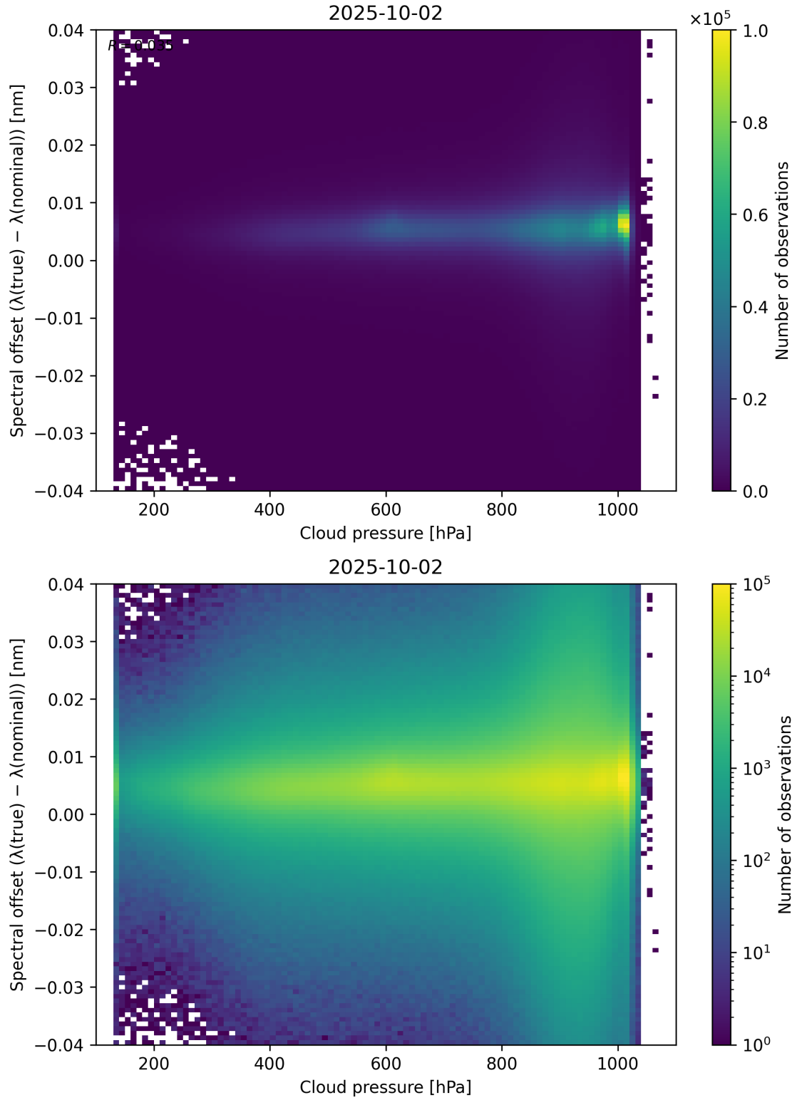
Figure 84: Scatter density plot of “Cloud pressure” against “Spectral offset ( \lambda_{\text{true}} - \lambda_{\text{nominal}} )” for 2025-10-01 to 2025-10-03.
