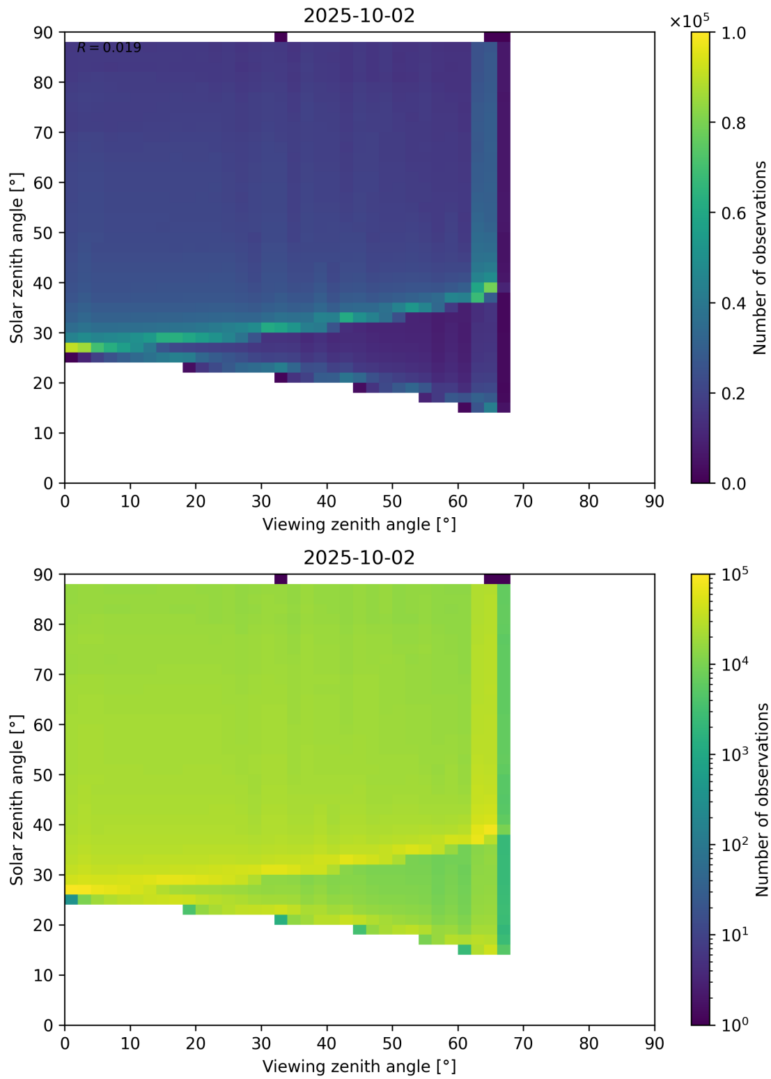
Figure 127: Scatter density plot of “Viewing zenith angle” against “Solar zenith angle” for 2025-10-01 to 2025-10-03.
