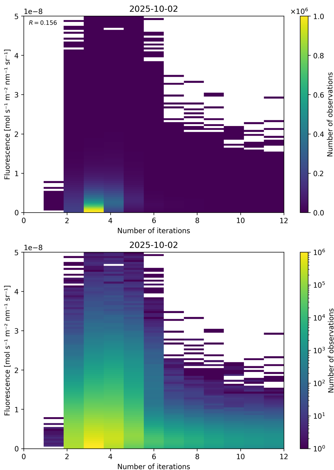
Figure 98: Scatter density plot of “Number of iterations” against “Fluorescence” for 2025-10-01 to 2025-10-03.
