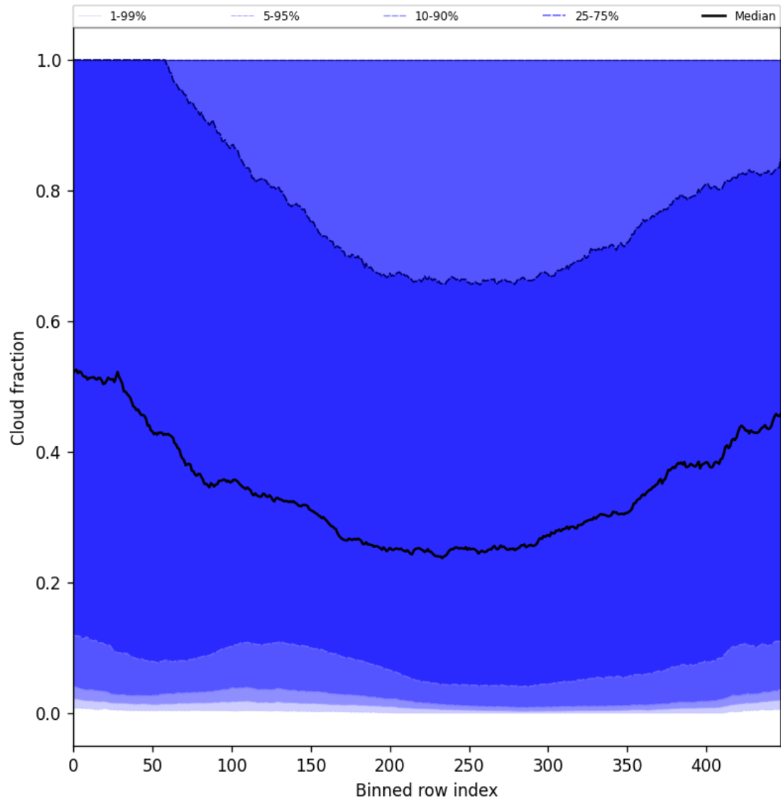
Figure 49: Along track statistics of “Cloud fraction” for 2025-10-01 to 2025-10-03
