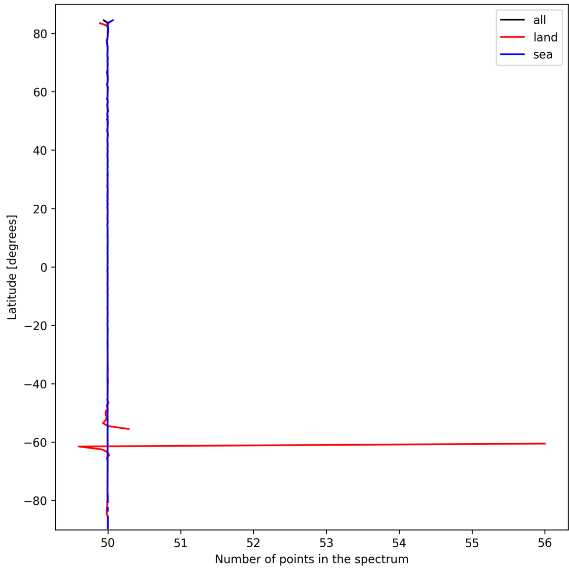
Figure 27: Zonal average of “Number of points in the spectrum” for 2025-10-01 to 2025-10-03.
