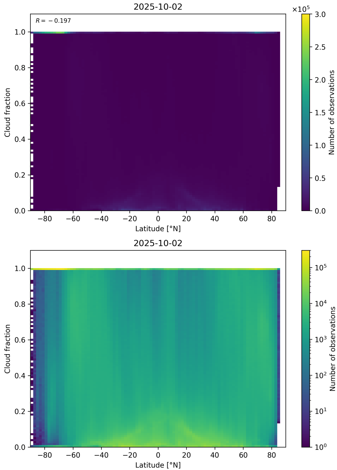
Figure 90: Scatter density plot of “Latitude” against “Cloud fraction” for 2025-10-01 to 2025-10-03.
