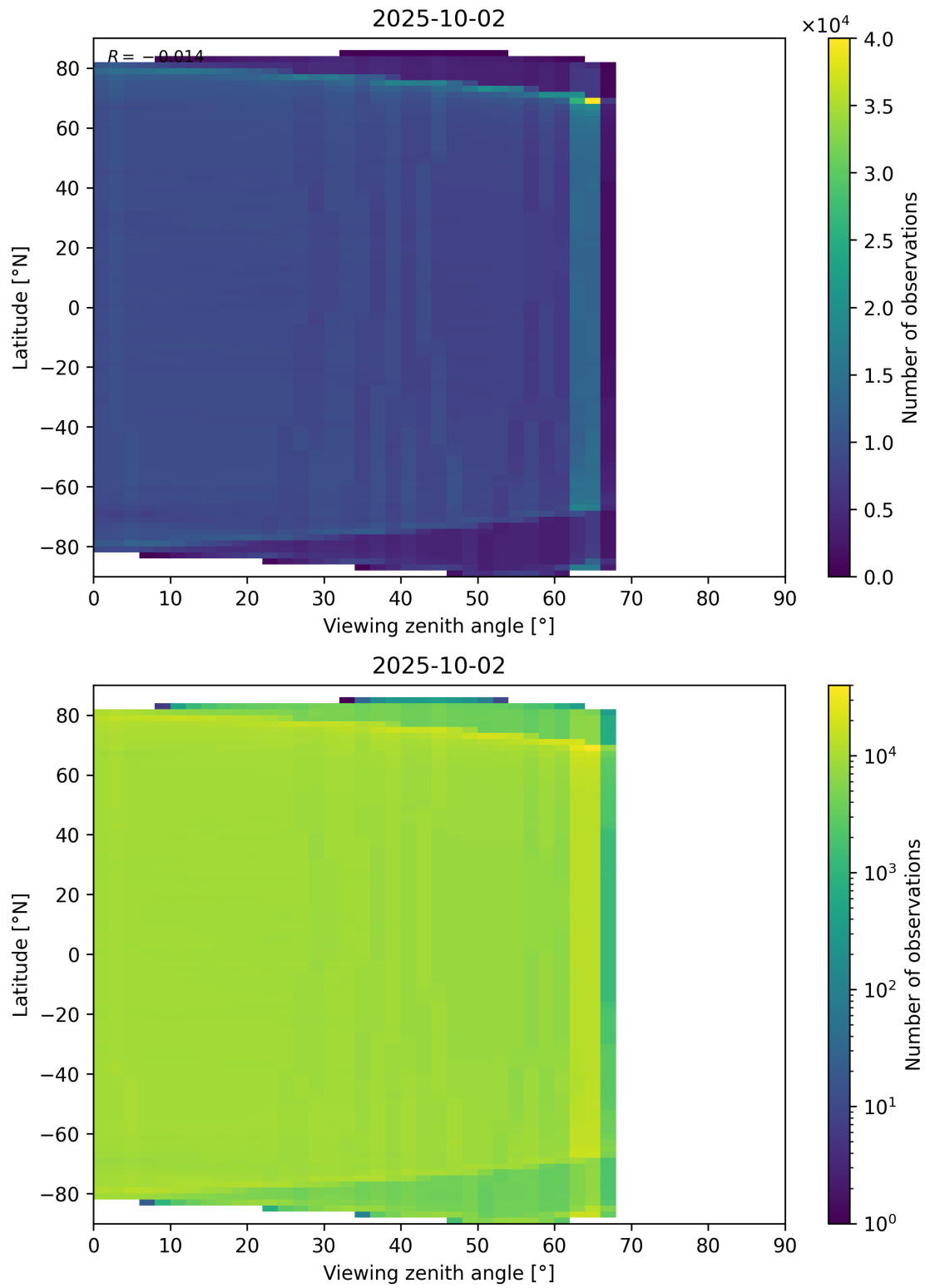
Figure 123: Scatter density plot of “Viewing zenith angle” against “Latitude” for 2025-10-01 to 2025-10-03.
