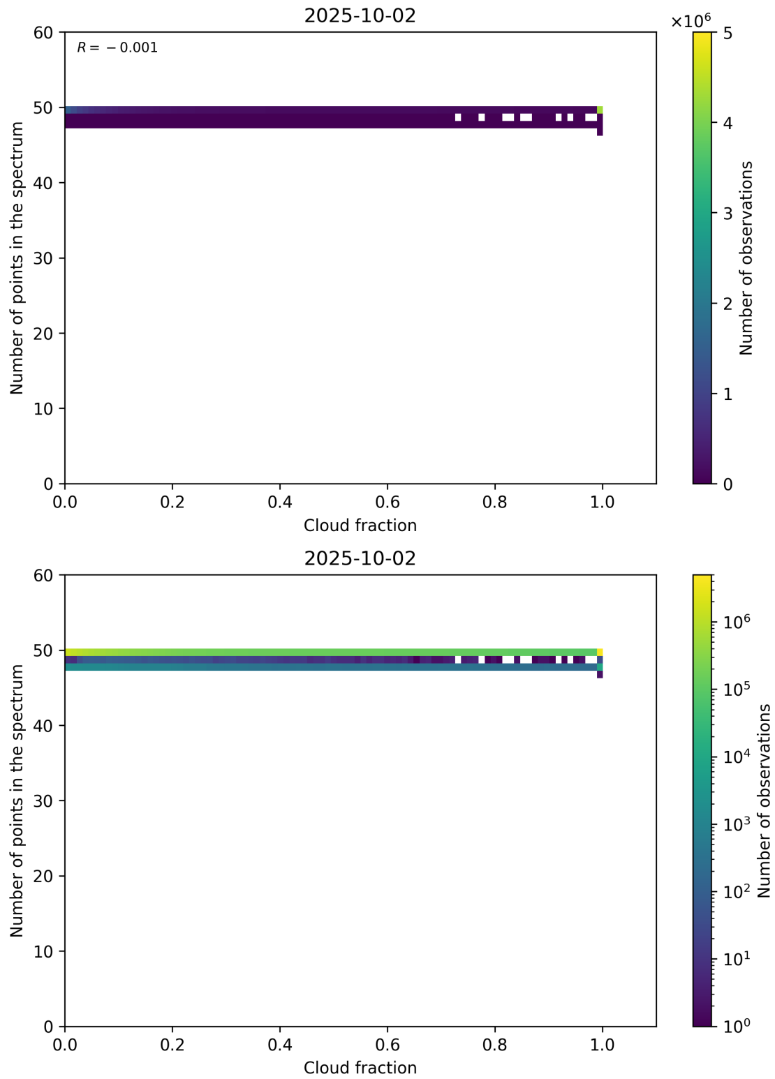
Figure 74: Scatter density plot of “Cloud fraction” against “Number of points in the spectrum” for 2025-10-01 to 2025-10-03.
