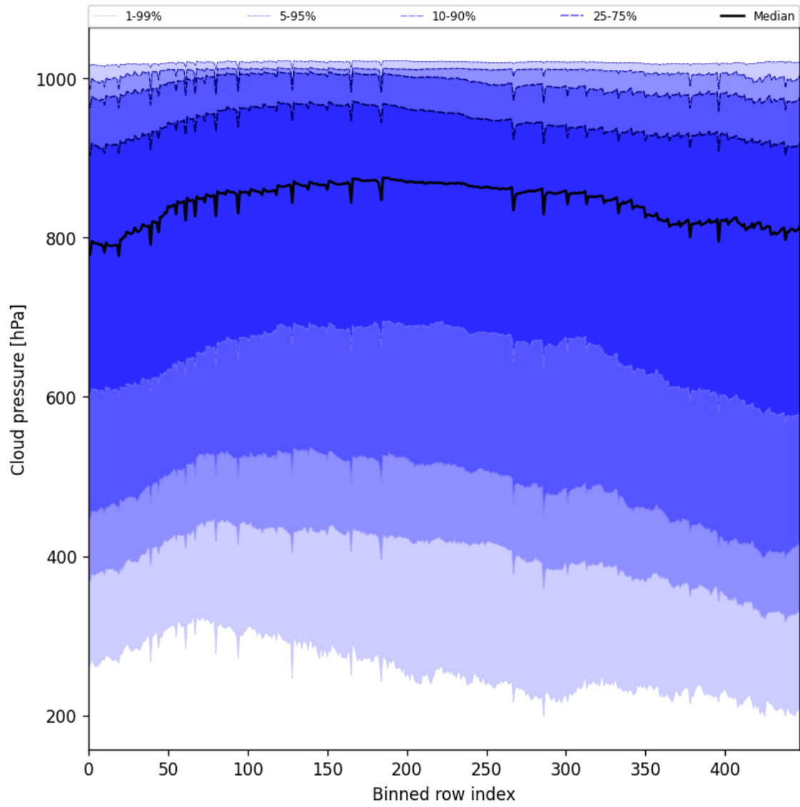
Figure 47: Along track statistics of “Cloud pressure” for 2025-10-01 to 2025-10-03
