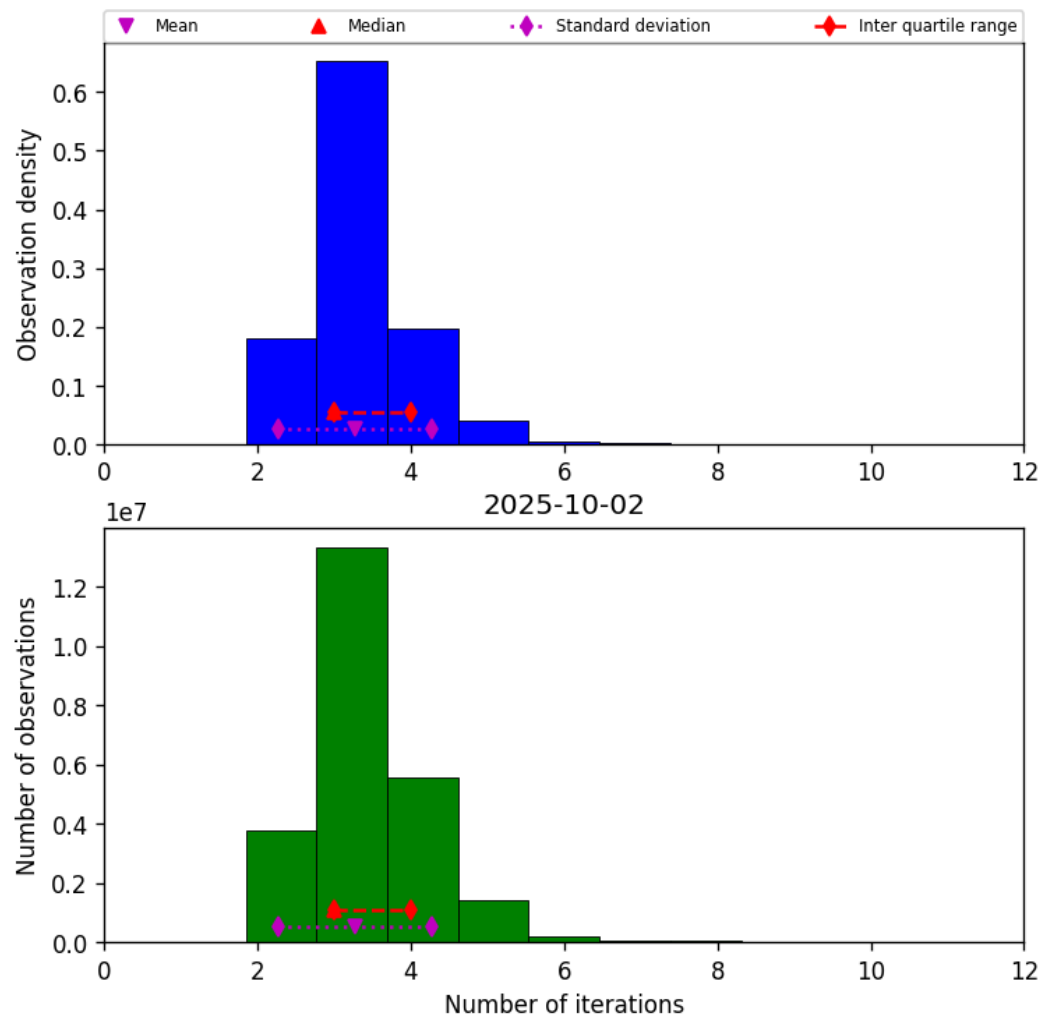
Figure 39: Histogram of “Number of iterations” for 2025-10-01 to 2025-10-03
