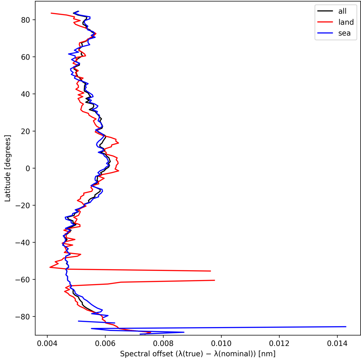
Figure 28: Zonal average of “Spectral offset ( \lambda_{\text{true}} - \lambda_{\text{nominal}} )” for 2025-10-01 to 2025-10-03.
