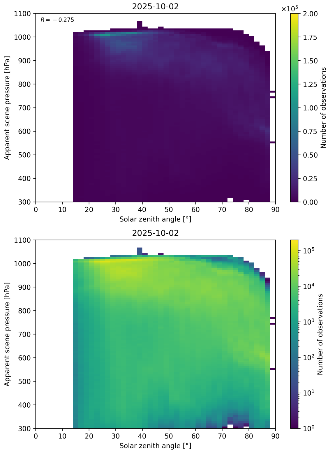
Figure 108: Scatter density plot of “Solar zenith angle” against “Apparent scene pressure” for 2025-10-01 to 2025-10-03.
