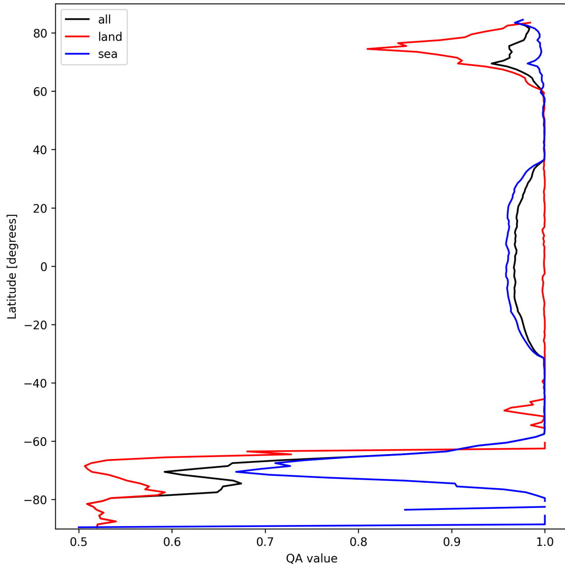
Figure 12: Zonal average of “QA value” for 2025-10-01 to 2025-10-03.
