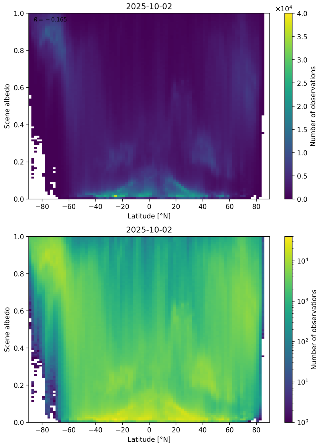
Figure 95: Scatter density plot of “Latitude” against “Scene albedo” for 2025-10-01 to 2025-10-03.
