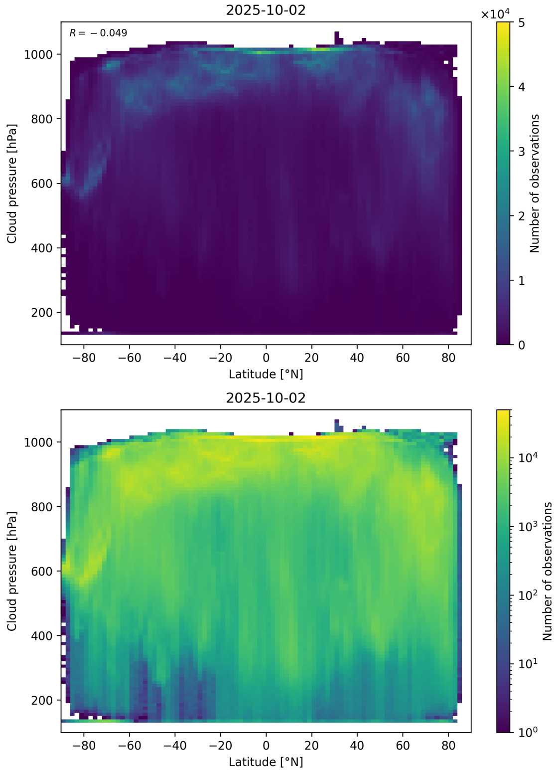
Figure 91: Scatter density plot of “Latitude” against “Cloud pressure” for 2025-10-01 to 2025-10-03.
