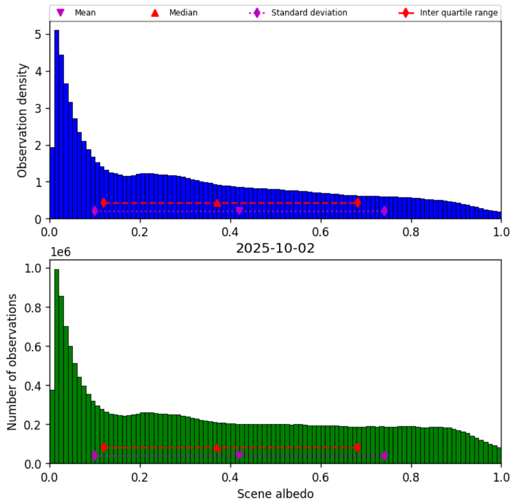
Figure 34: Histogram of “Scene albedo” for 2025-10-01 to 2025-10-03
