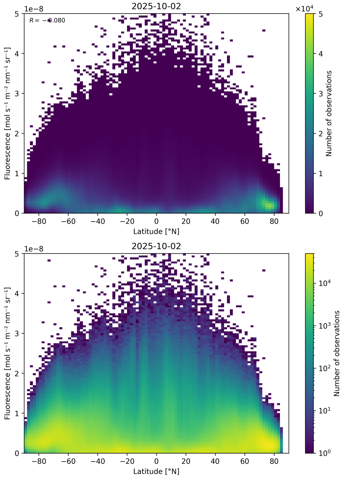
Figure 92: Scatter density plot of “Latitude” against “Fluorescence” for 2025-10-01 to 2025-10-03.
