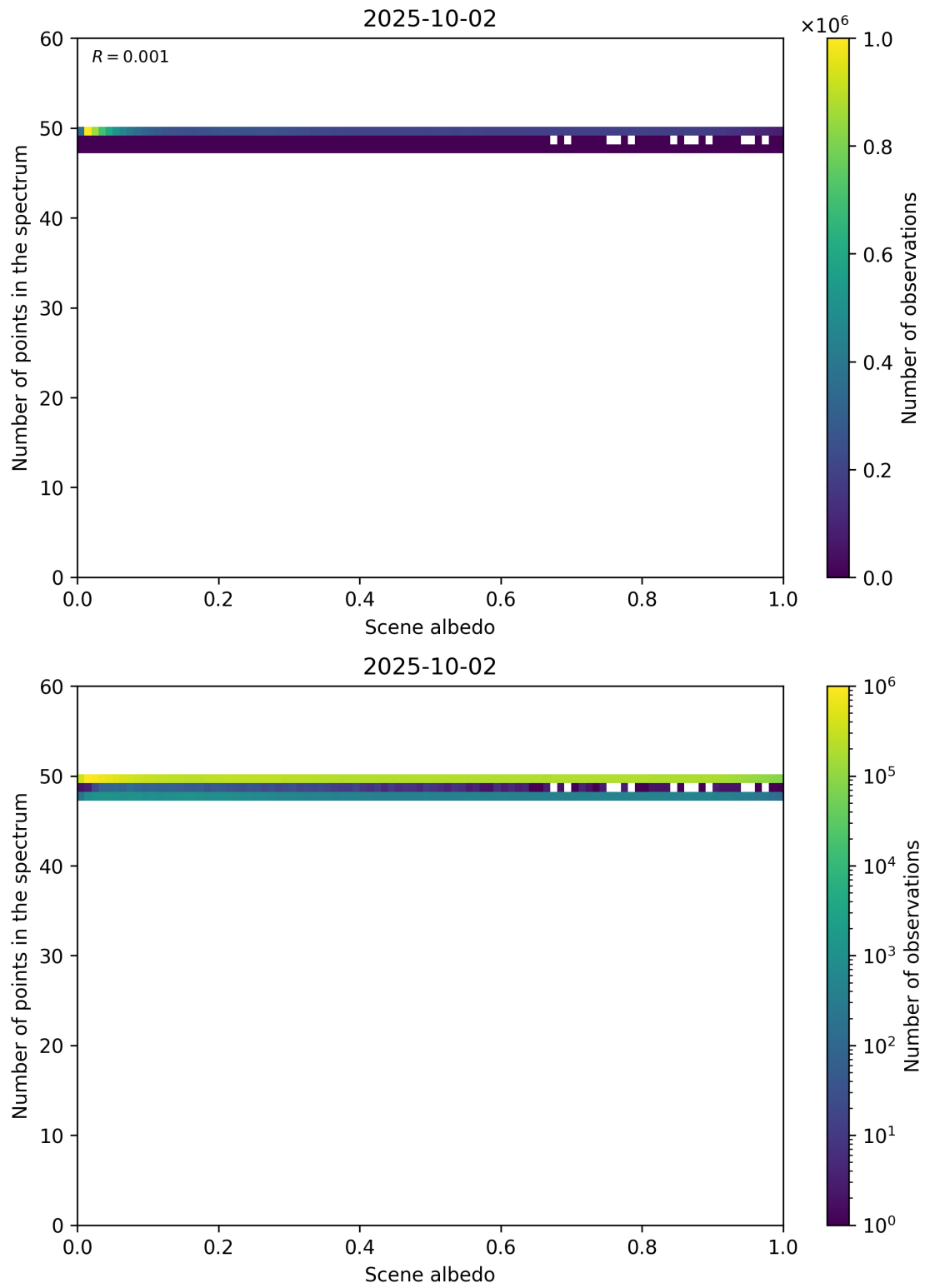
Figure 106: Scatter density plot of “Scene albedo” against “Number of points in the spectrum” for 2025-10-01 to 2025-10-03.
