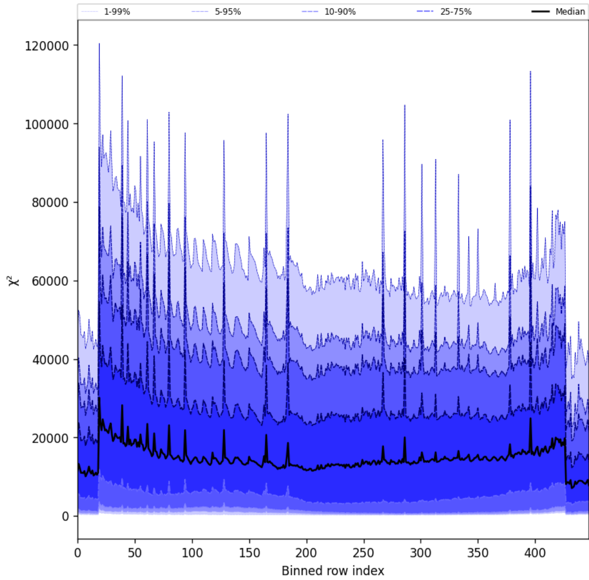
Figure 55: Along track statistics of “ \chi^2 ” for 2025-10-01 to 2025-10-03
