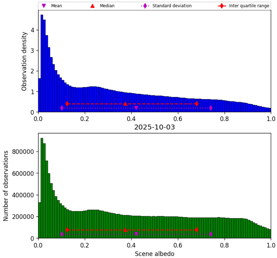
Figure 34: Histogram of “Scene albedo” for 2025-10-02 to 2025-10-04
