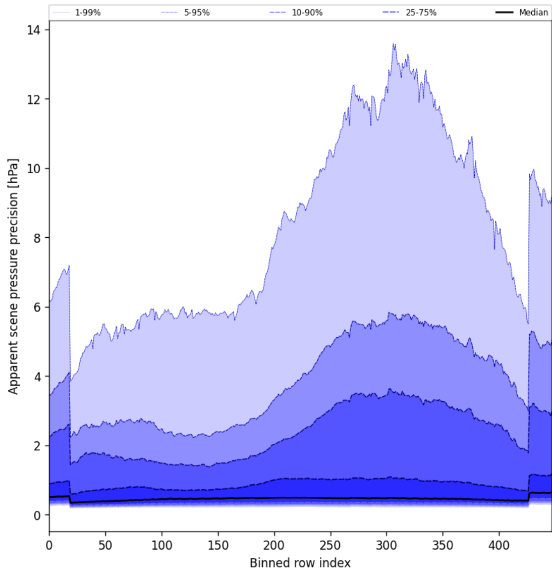
Figure 54: Along track statistics of “Apparent scene pressure precision” for 2025-10-02 to 2025-10-04
