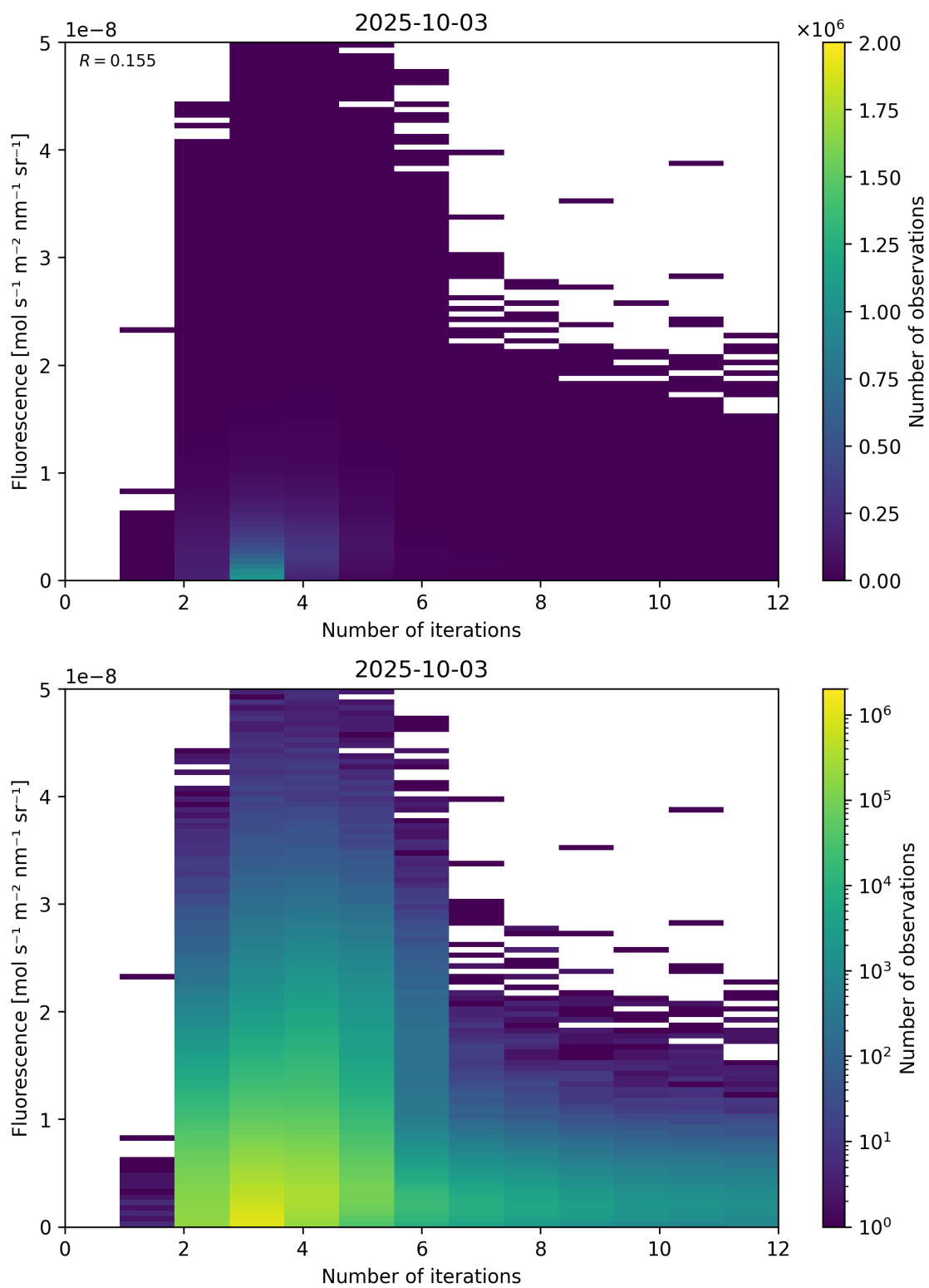
Figure 98: Scatter density plot of “Number of iterations” against “Fluorescence” for 2025-10-02 to 2025-10-04.
