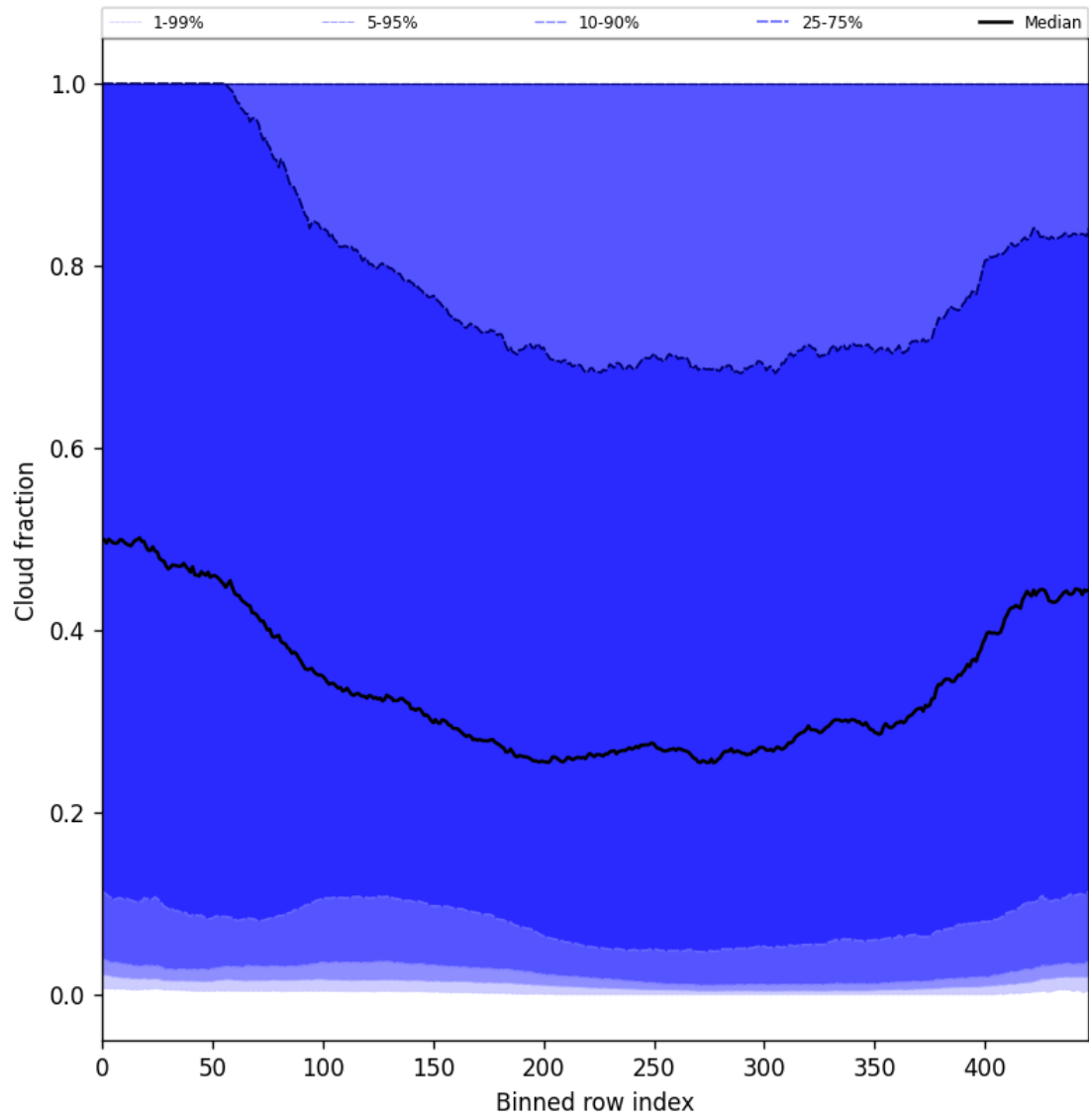
Figure 49: Along track statistics of “Cloud fraction” for 2025-10-02 to 2025-10-04
