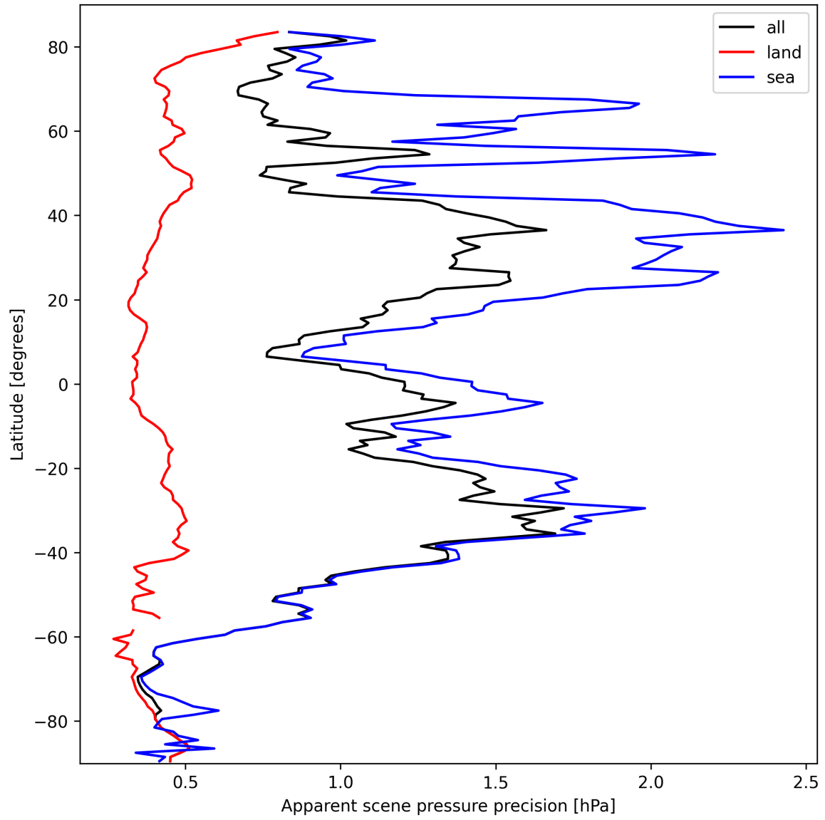
Figure 20: Zonal average of “Apparent scene pressure precision” for 2025-10-02 to 2025-10-04.
