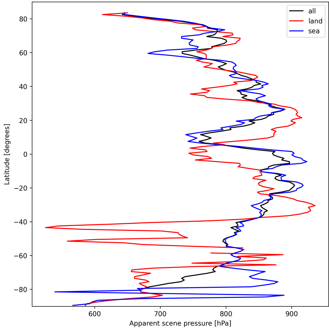
Figure 19: Zonal average of “Apparent scene pressure” for 2025-10-02 to 2025-10-04.
