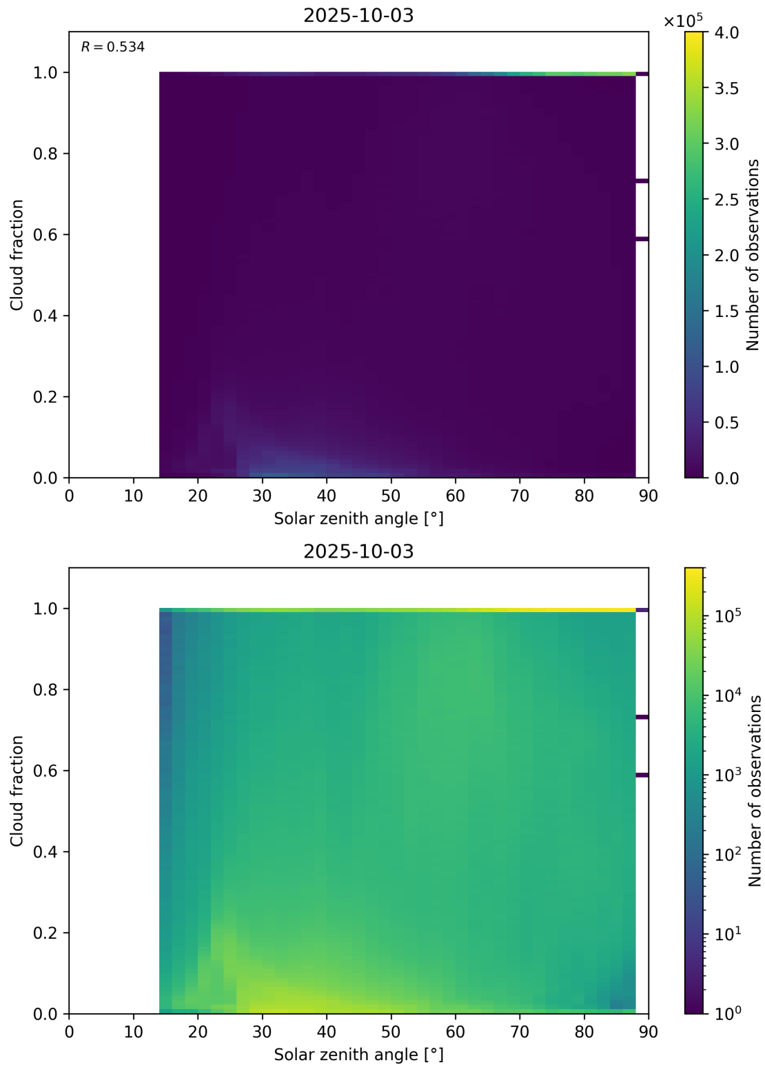
Figure 110: Scatter density plot of “Solar zenith angle” against “Cloud fraction” for 2025-10-02 to 2025-10-04.
