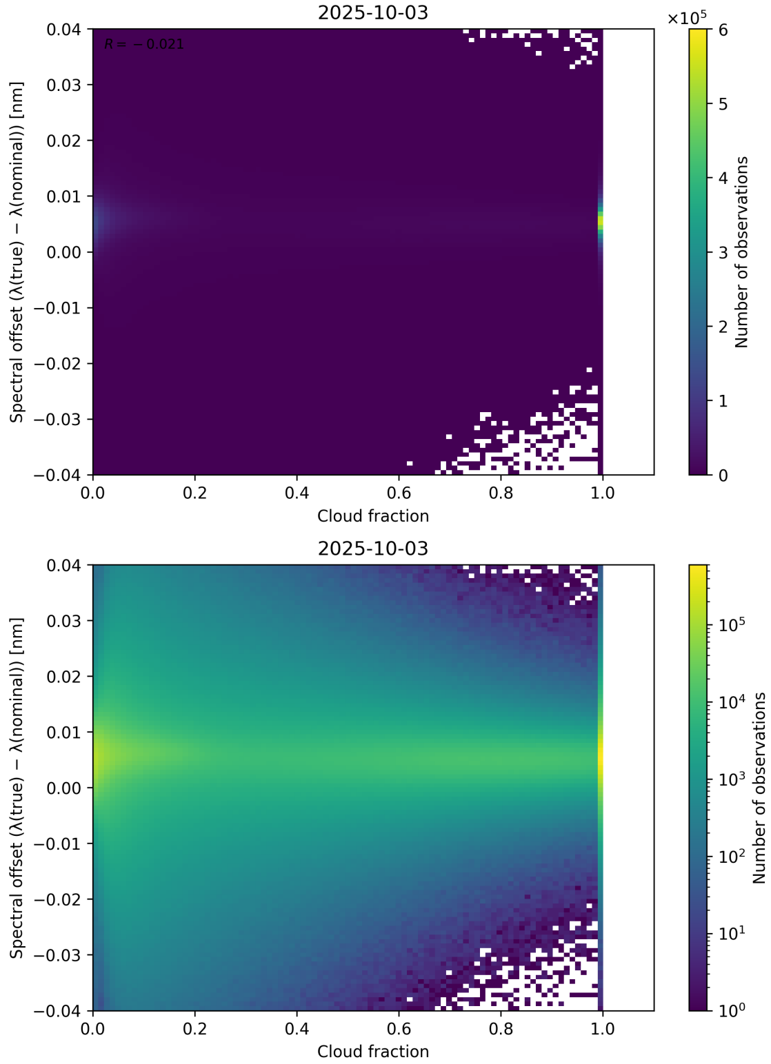
Figure 76: Scatter density plot of “Cloud fraction” against “Spectral offset ( \lambda_{\text{true}} - \lambda_{\text{nominal}} )” for 2025-10-02 to 2025-10-04.
