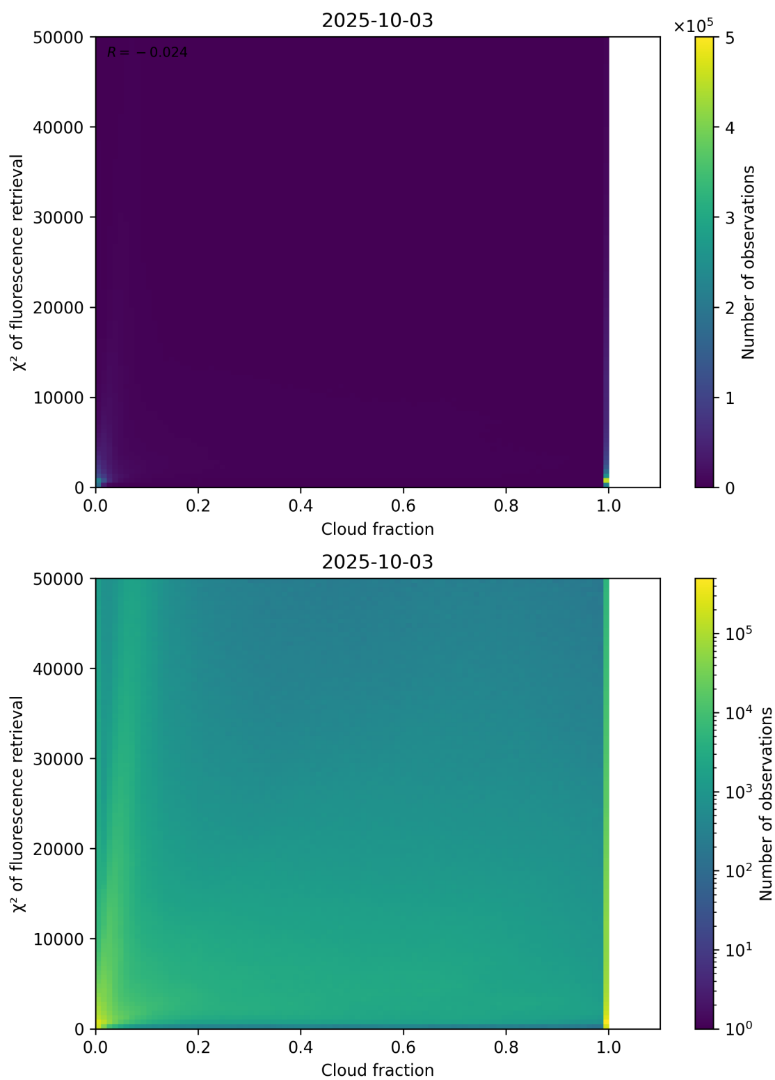
Figure 71: Scatter density plot of “Cloud fraction” against “ \chi^2 of fluorescence retrieval” for 2025-10-02 to 2025-10-04.
