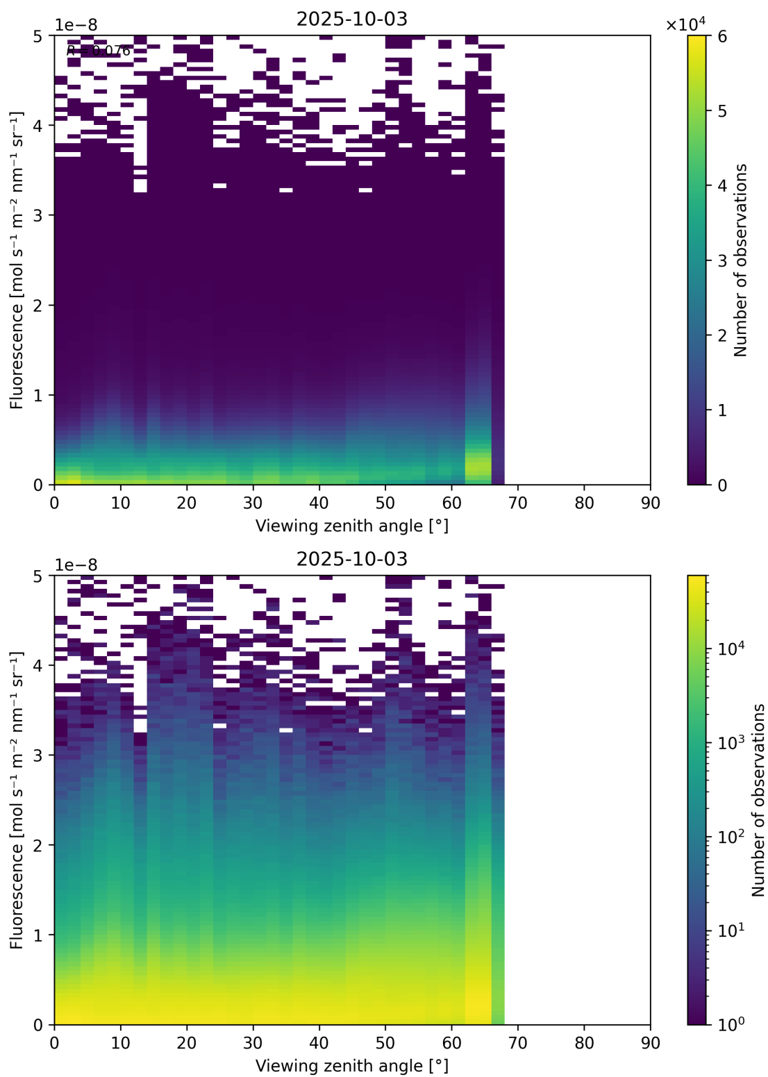
Figure 122: Scatter density plot of "Viewing zenith angle" against "Fluorescence" for 2025-10-02 to 2025-10-04.
