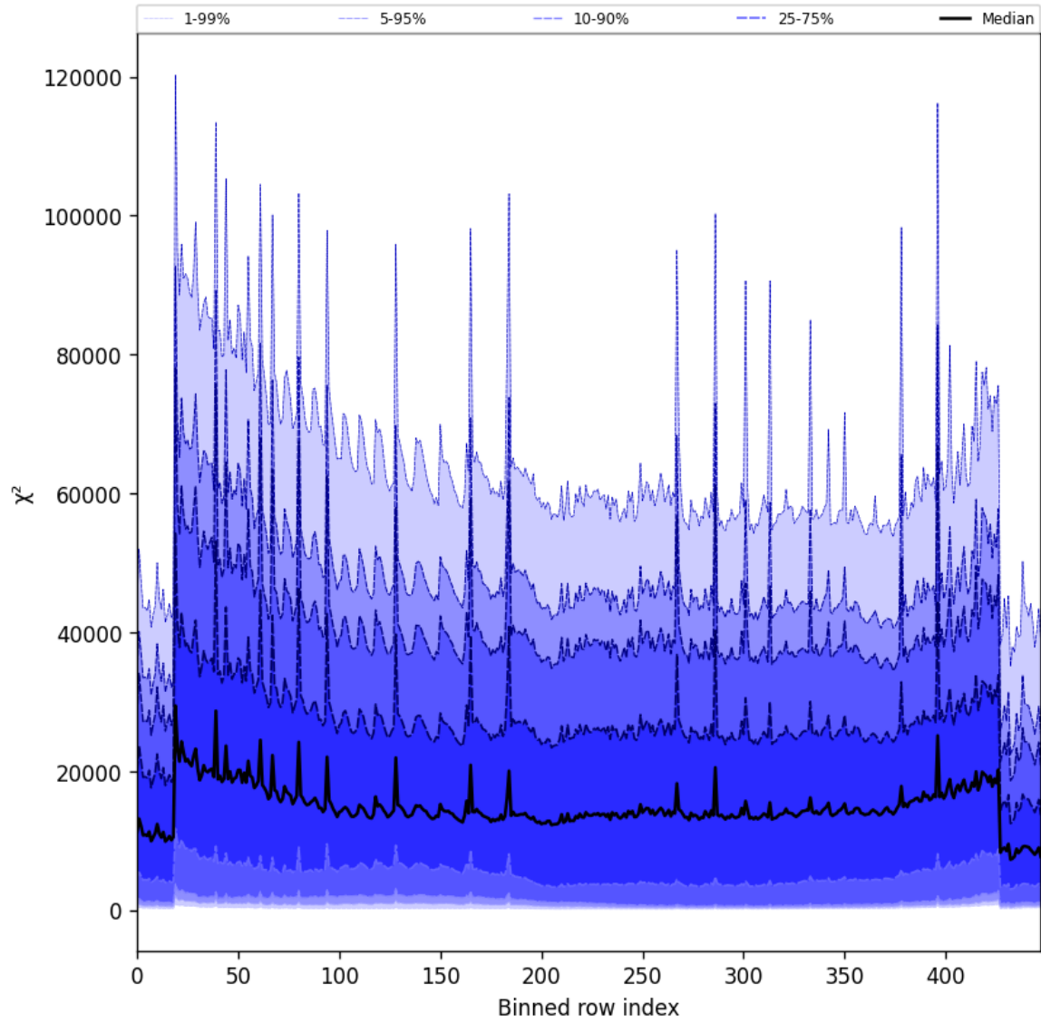
Figure 55: Along track statistics of “ \chi^2 ” for 2025-10-02 to 2025-10-04
