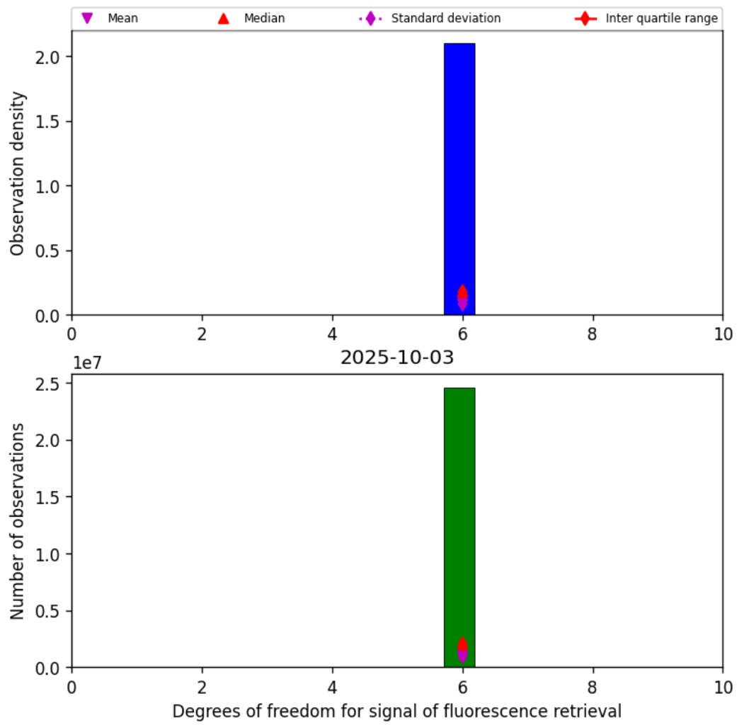
Figure 43: Histogram of "Degrees of freedom for signal of fluorescence retrieval" for 2025-10-02 to 2025-10-04
