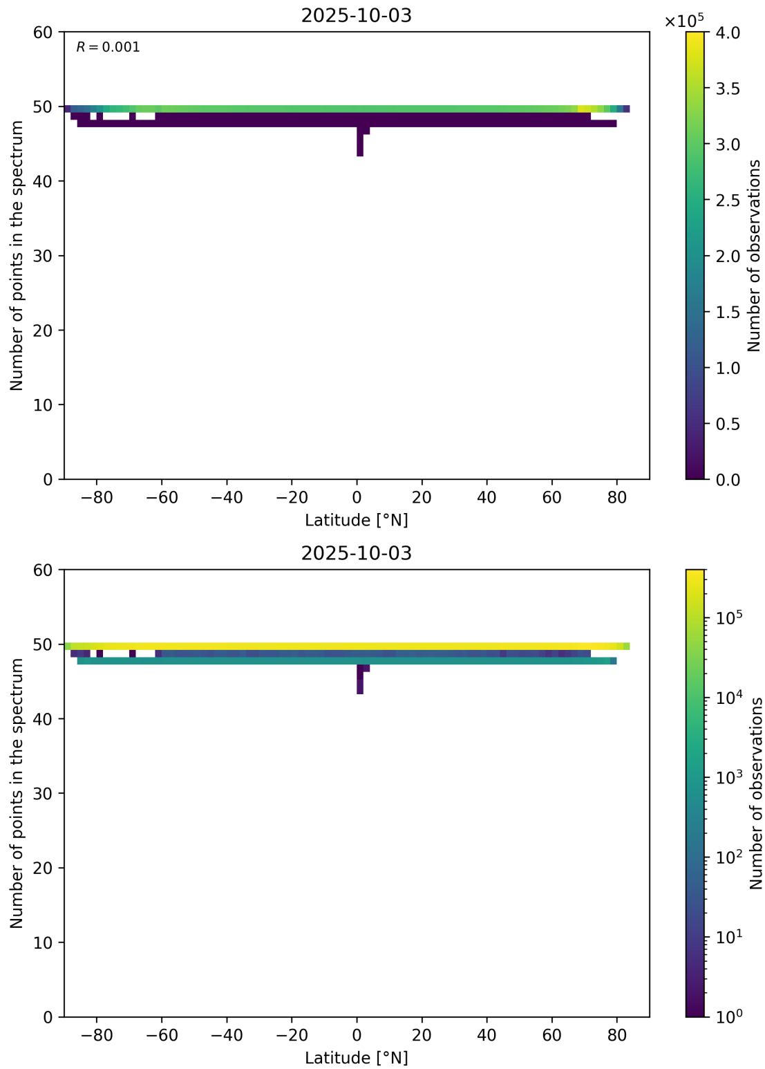
Figure 94: Scatter density plot of “Latitude” against “Number of points in the spectrum” for 2025-10-02 to 2025-10-04.
