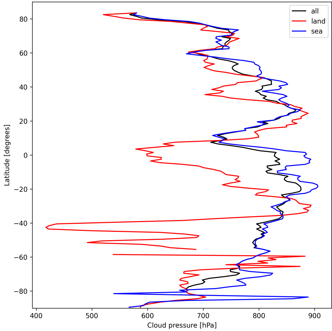
Figure 13: Zonal average of “Cloud pressure” for 2025-10-02 to 2025-10-04.
