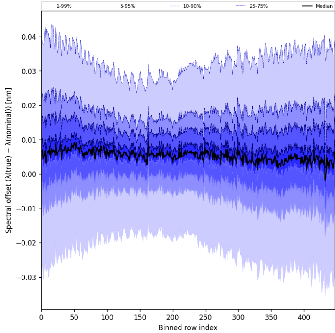
Figure 62: Along track statistics of “Spectral offset ( \lambda_{\text{true}} - \lambda_{\text{nominal}} )” for 2025-10-02 to 2025-10-04
