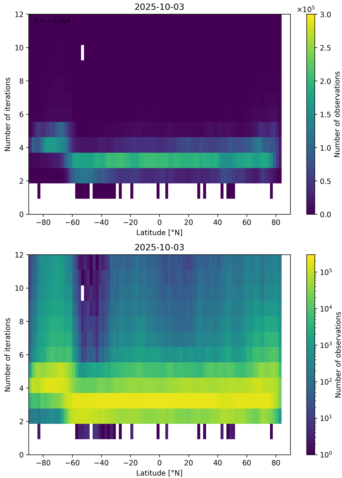
Figure 93: Scatter density plot of “Latitude” against “Number of iterations” for 2025-10-02 to 2025-10-04.
