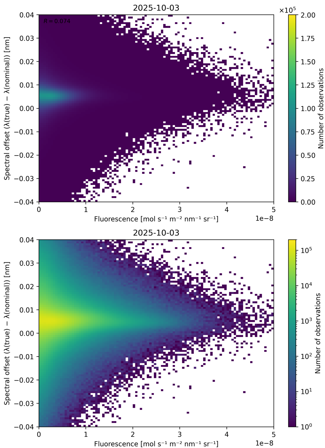
Figure 87: Scatter density plot of “Fluorescence” against “Spectral offset ( \lambda_{\text{true}} - \lambda_{\text{nominal}} )” for 2025-10-02 to 2025-10-04.
