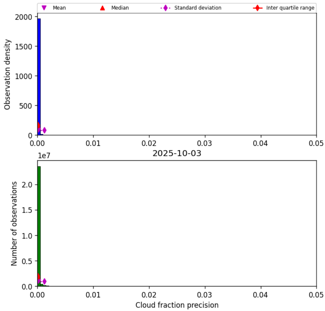
Figure 33: Histogram of “Cloud fraction precision” for 2025-10-02 to 2025-10-04
