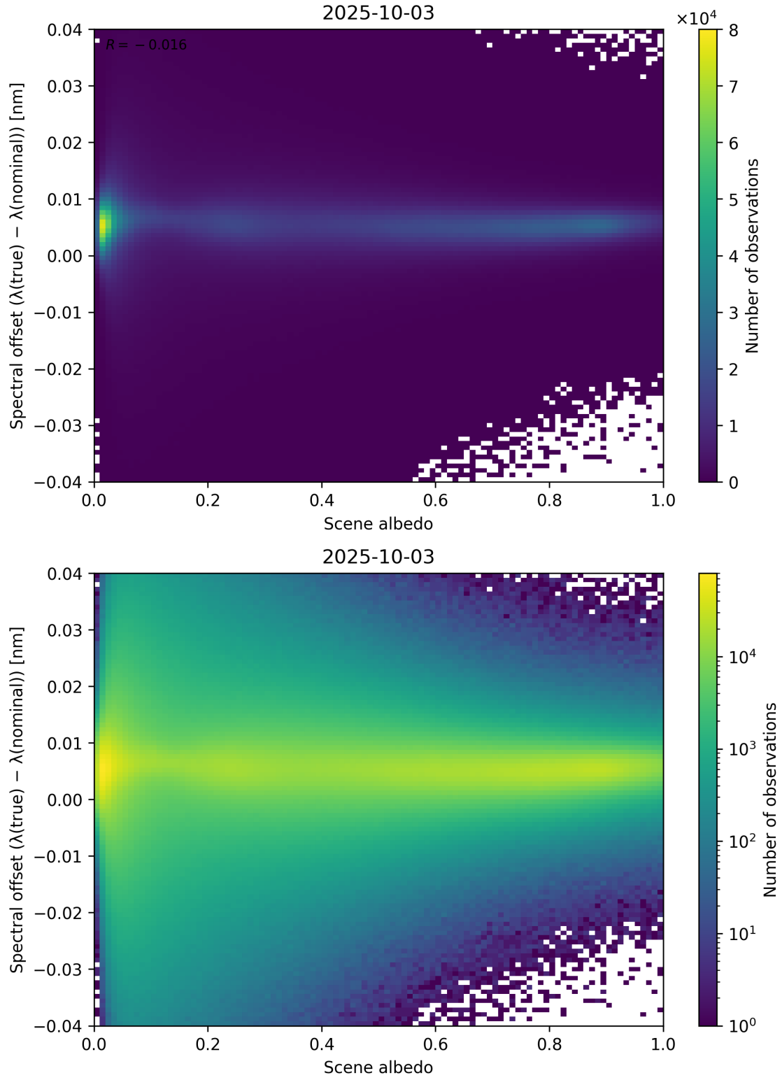
Figure 107: Scatter density plot of “Scene albedo” against “Spectral offset ( \lambda_{\text{true}} - \lambda_{\text{nominal}} )” for 2025-10-02 to 2025-10-04.
