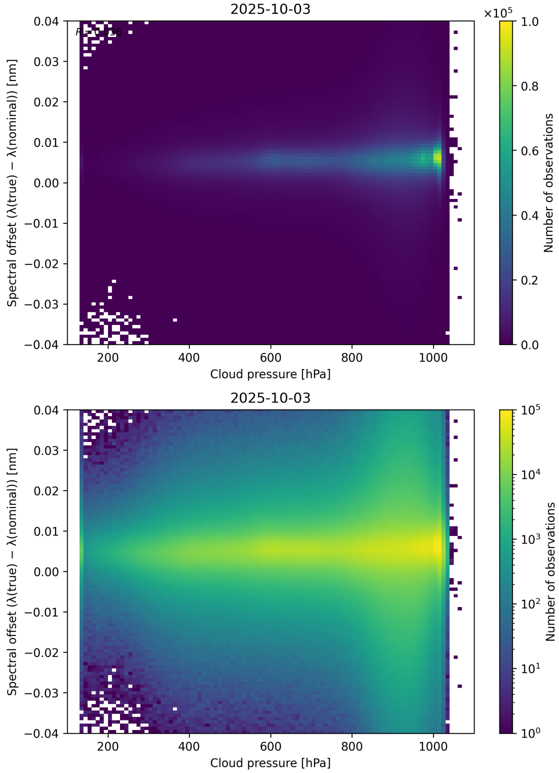
Figure 84: Scatter density plot of “Cloud pressure” against “Spectral offset ( \lambda_{\text{true}} - \lambda_{\text{nominal}} )” for 2025-10-02 to 2025-10-04.
