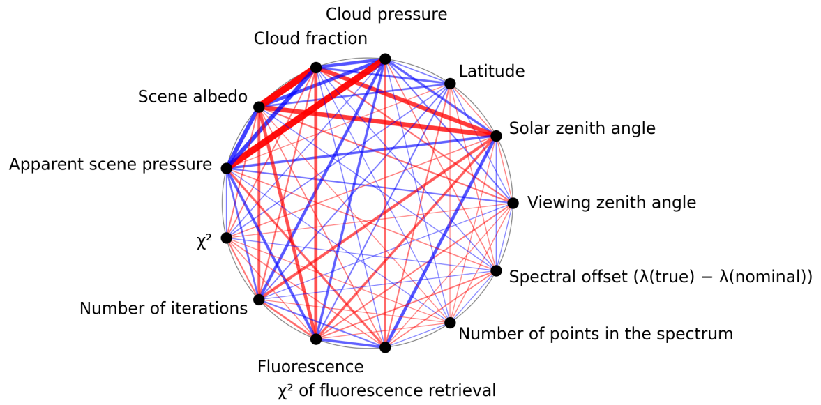
Figure 1: Map of correlation graph for 2025-10-02 to 2025-10-04.
