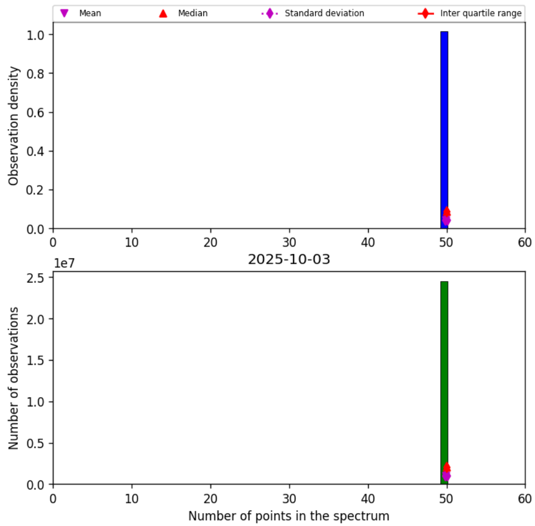
Figure 44: Histogram of “Number of points in the spectrum” for 2025-10-02 to 2025-10-04
