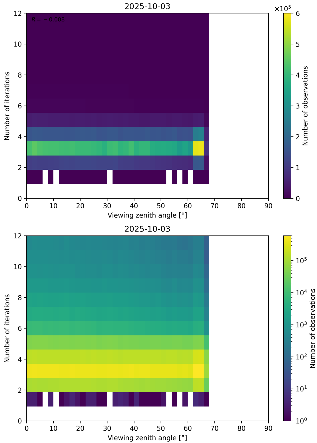
Figure 124: Scatter density plot of “Viewing zenith angle” against “Number of iterations” for 2025-10-02 to 2025-10-04.
