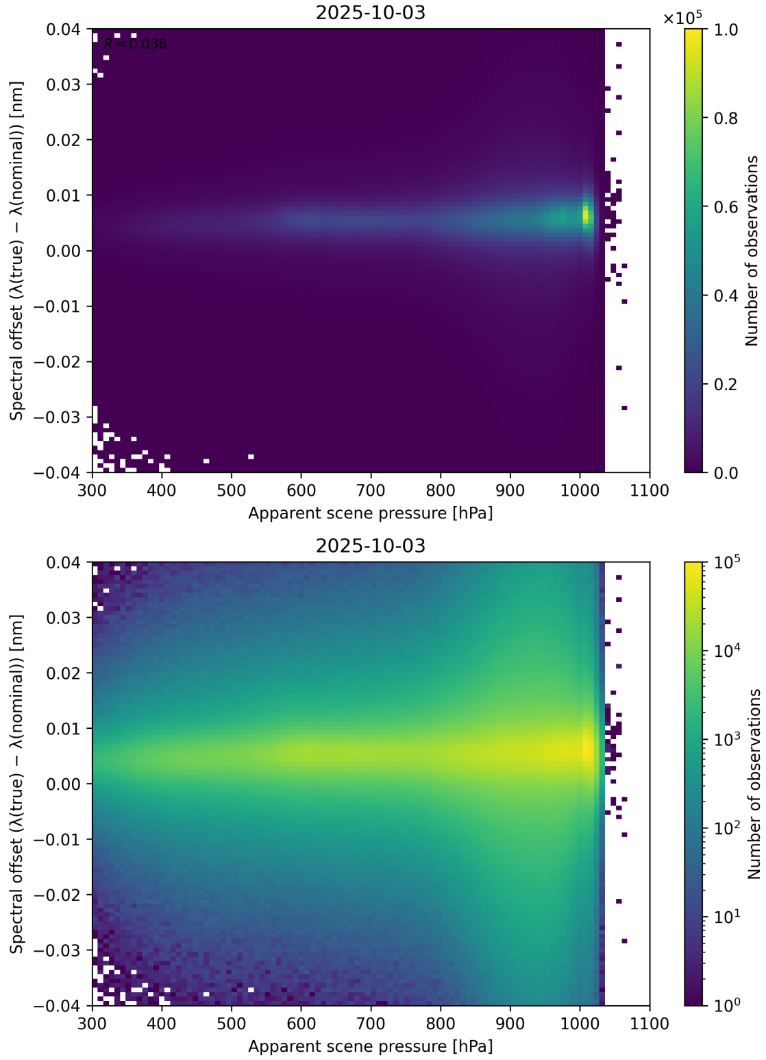
Figure 67: Scatter density plot of “Apparent scene pressure” against “Spectral offset ( \lambda_{\text{true}} - \lambda_{\text{nominal}} )” for 2025-10-02 to 2025-10-04.
