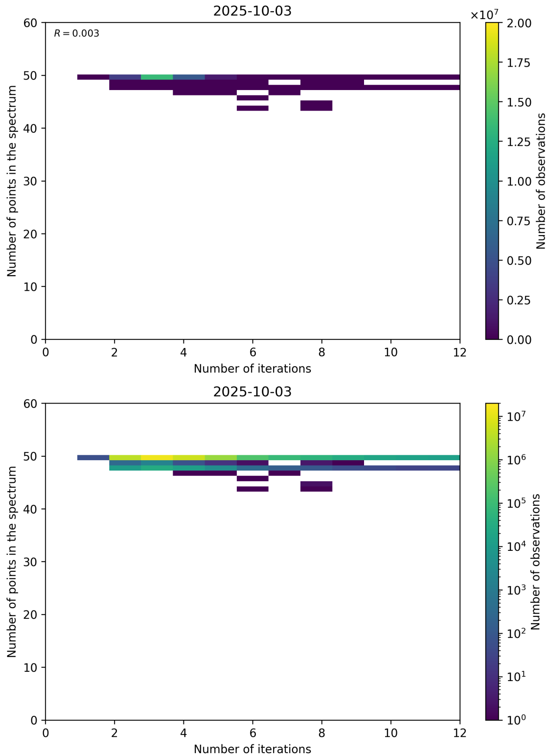
Figure 99: Scatter density plot of “Number of iterations” against “Number of points in the spectrum” for 2025-10-02 to 2025-10-04.
