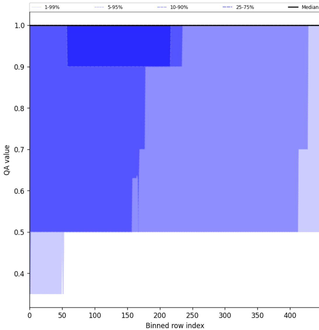
Figure 46: Along track statistics of “QA value” for 2025-10-02 to 2025-10-04
