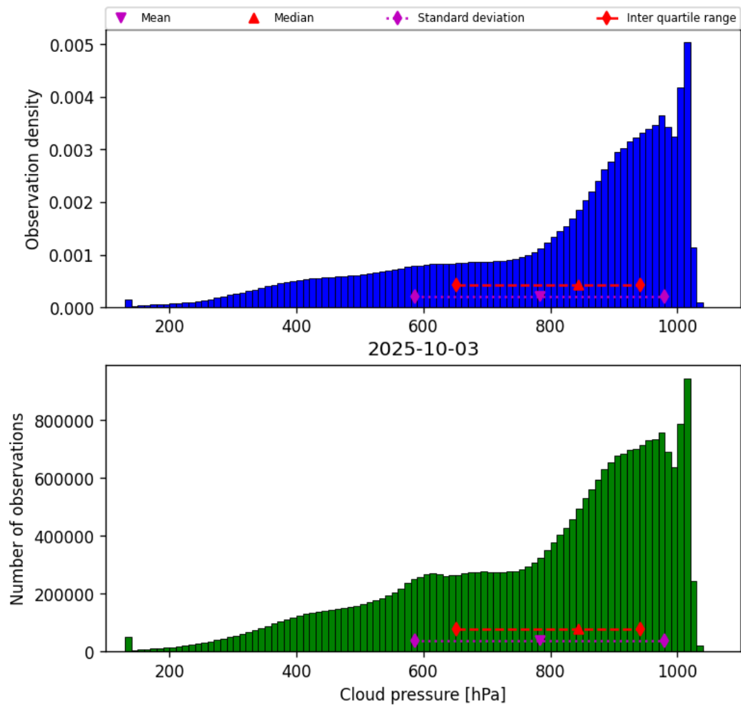
Figure 30: Histogram of “Cloud pressure” for 2025-10-02 to 2025-10-04
