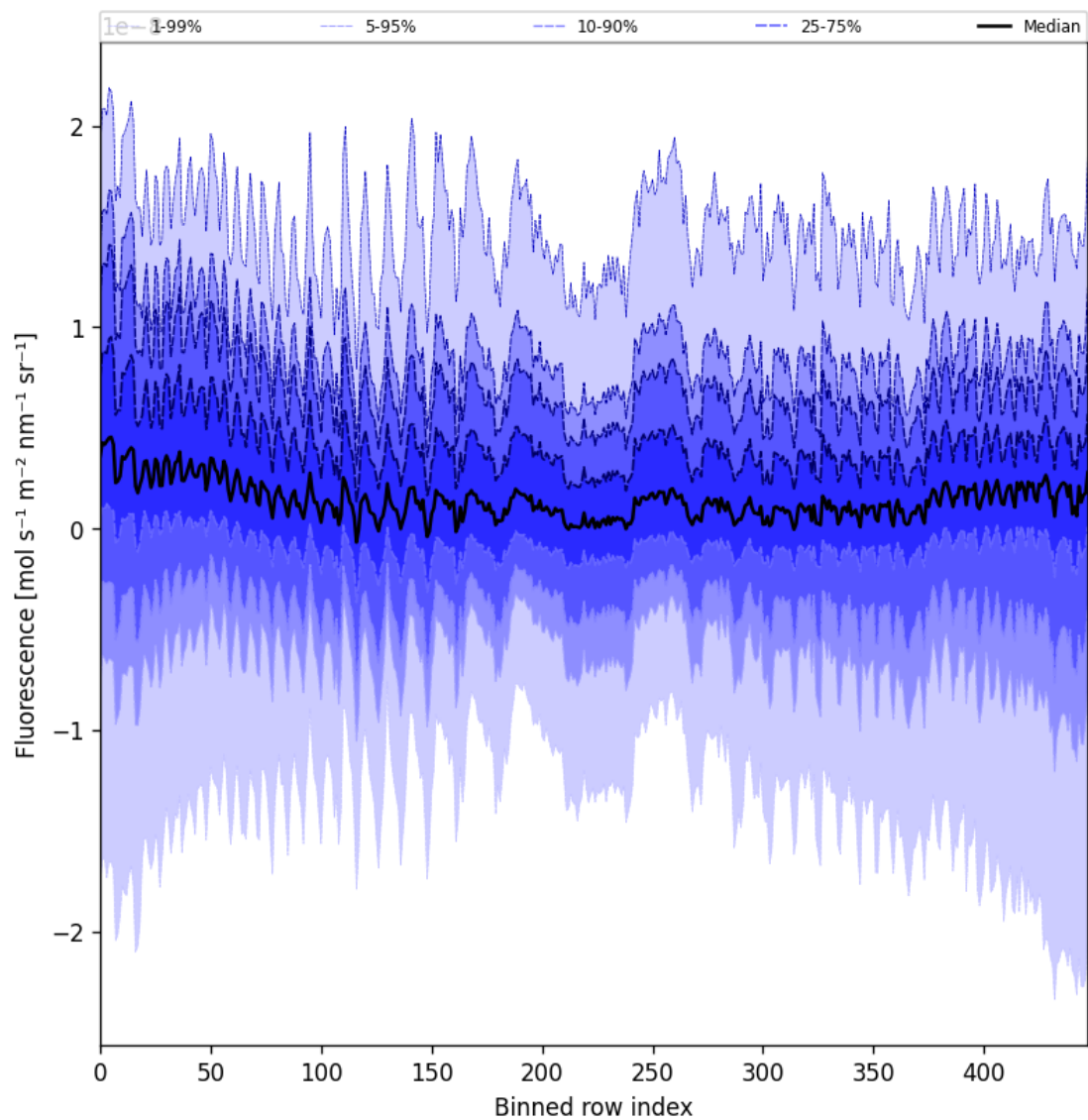
Figure 57: Along track statistics of "Fluorescence" for 2025-10-02 to 2025-10-04
