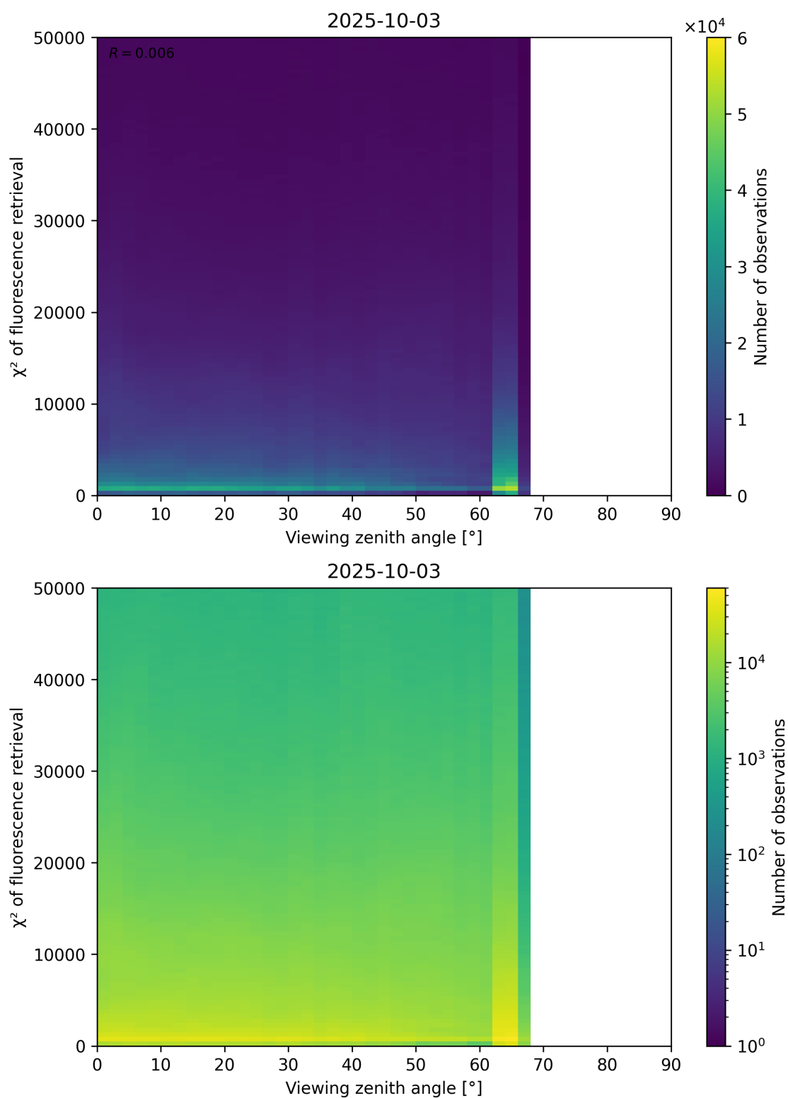
Figure 119: Scatter density plot of “Viewing zenith angle” against “ \chi^2 of fluorescence retrieval” for 2025-10-02 to 2025-10-04.
