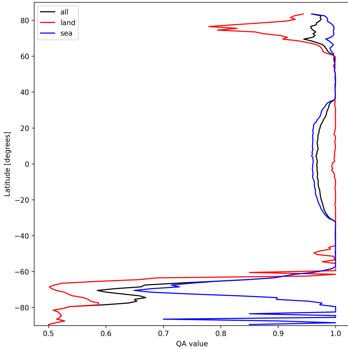
Figure 12: Zonal average of “QA value” for 2025-10-02 to 2025-10-04.
