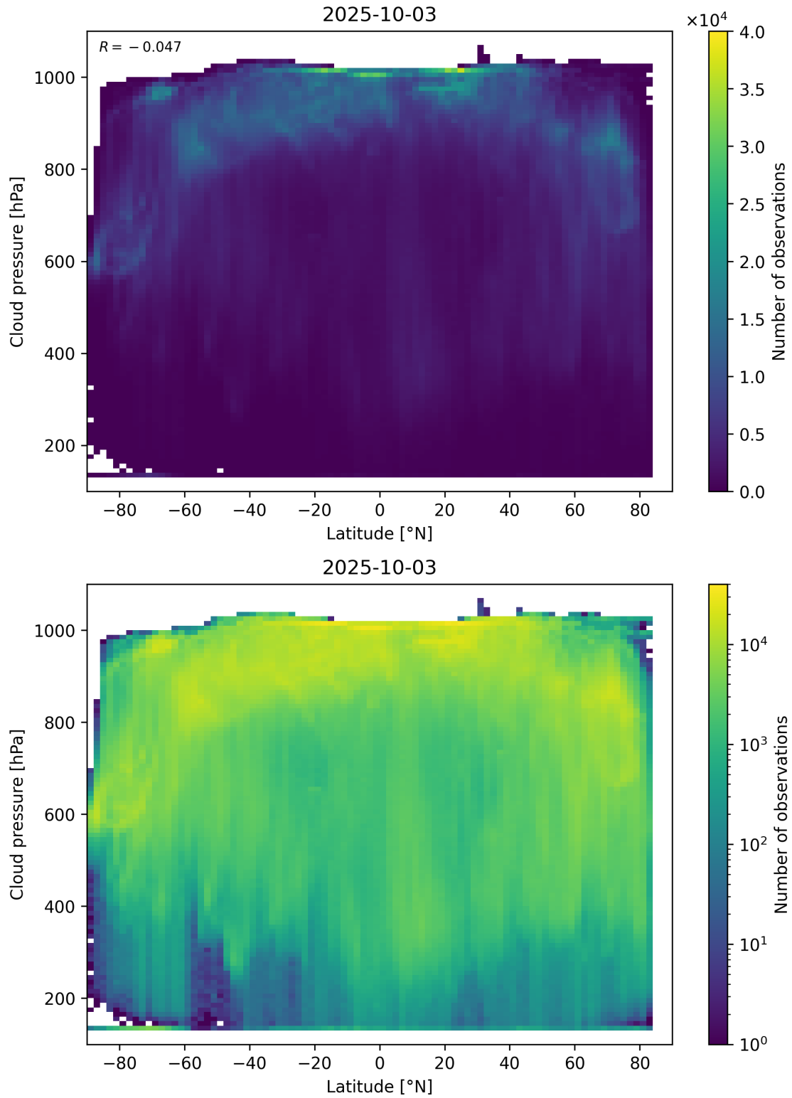
Figure 91: Scatter density plot of “Latitude” against “Cloud pressure” for 2025-10-02 to 2025-10-04.
