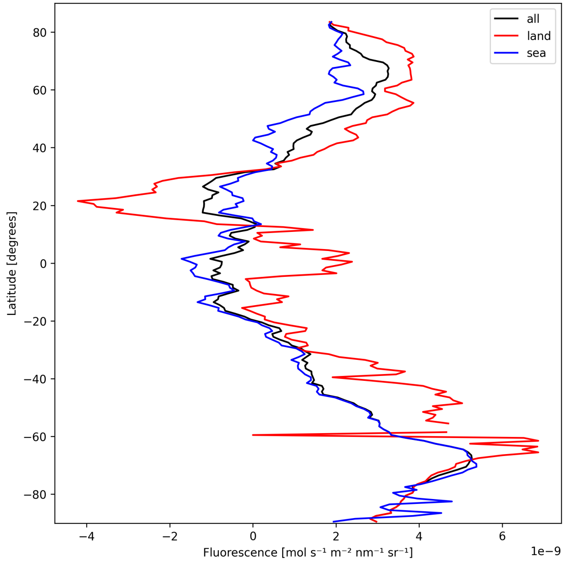
Figure 23: Zonal average of “Fluorescence” for 2025-10-02 to 2025-10-04.
