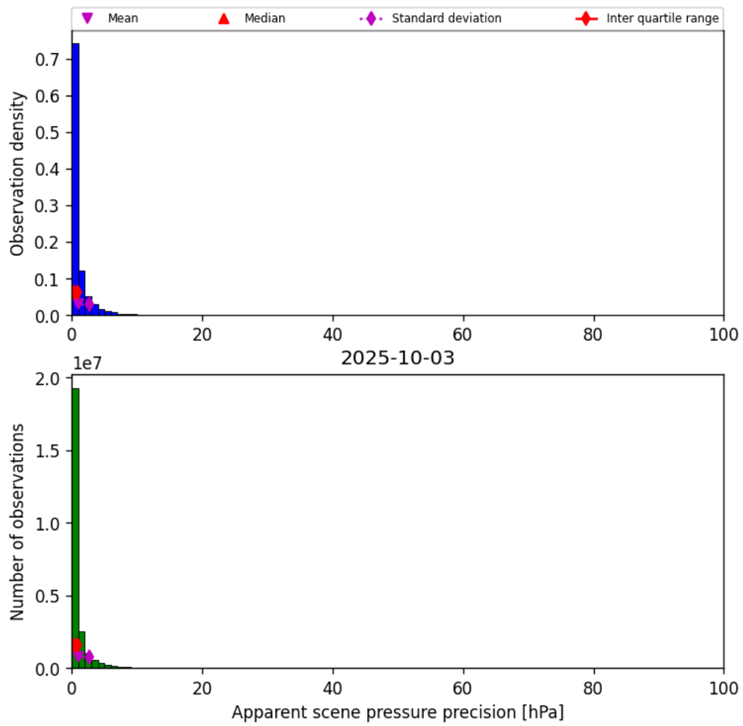
Figure 37: Histogram of “Apparent scene pressure precision” for 2025-10-02 to 2025-10-04
