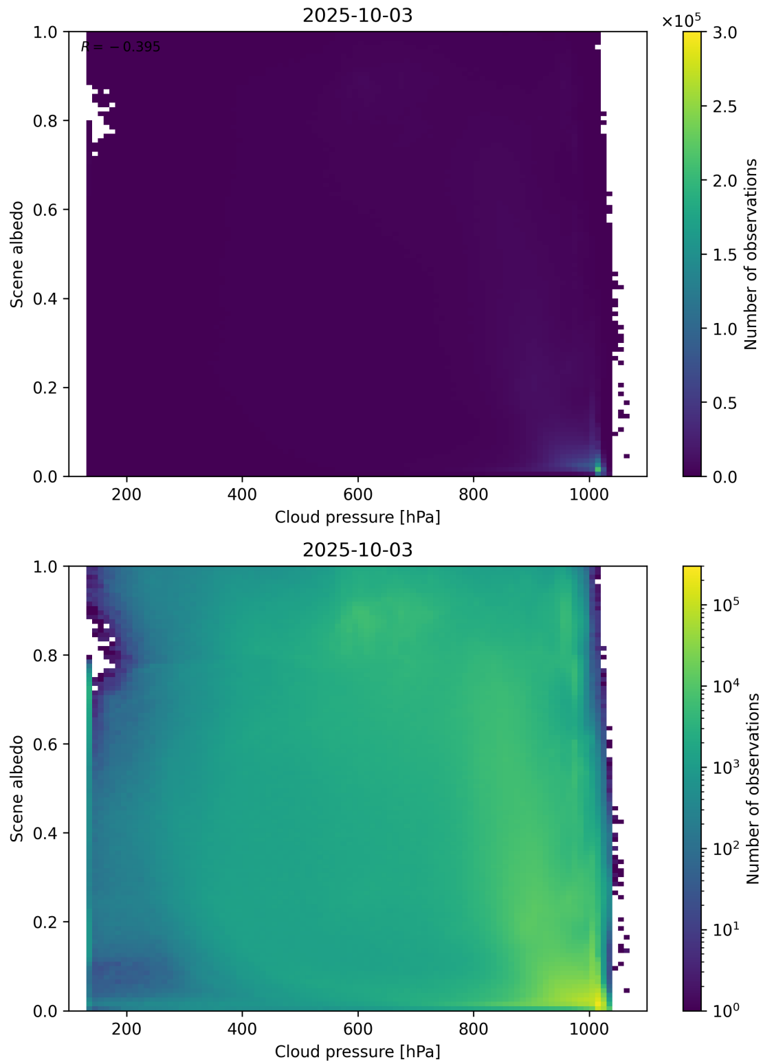
Figure 83: Scatter density plot of “Cloud pressure” against “Scene albedo” for 2025-10-02 to 2025-10-04.
