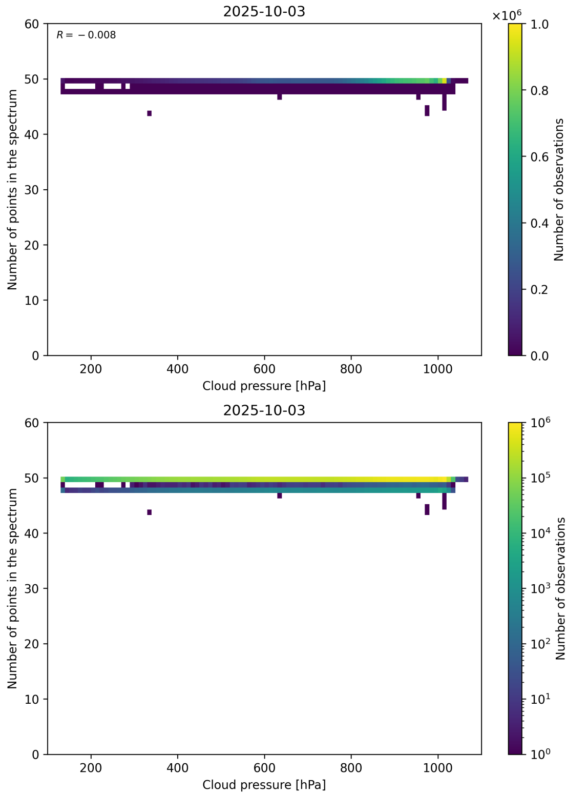
Figure 82: Scatter density plot of “Cloud pressure” against “Number of points in the spectrum” for 2025-10-02 to 2025-10-04.
