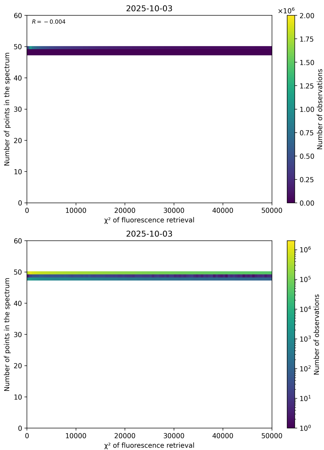
Figure 68: Scatter density plot of " \chi^2 of fluorescence retrieval" against "Number of points in the spectrum" for 2025-10-02 to 2025-10-04.
