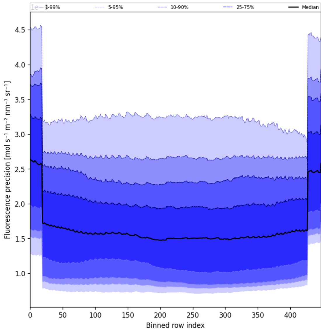
Figure 58: Along track statistics of “Fluorescence precision” for 2025-10-02 to 2025-10-04
