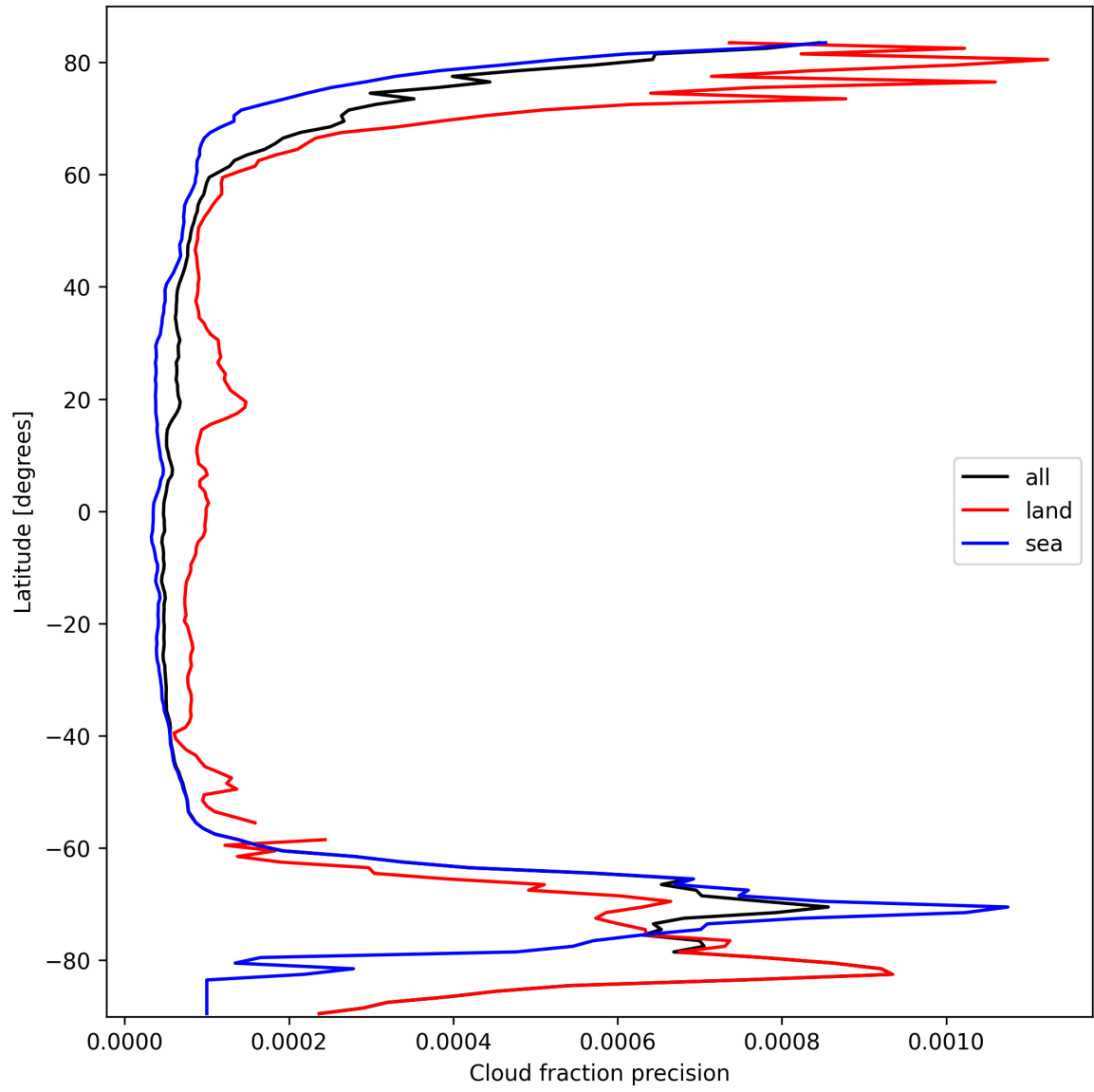
Figure 16: Zonal average of “Cloud fraction precision” for 2025-10-02 to 2025-10-04.
