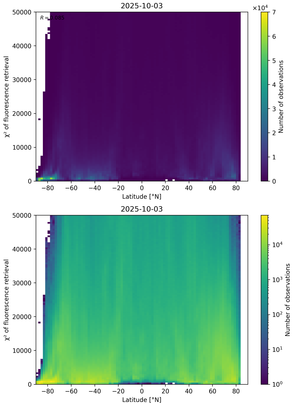
Figure 89: Scatter density plot of “Latitude” against “ \chi^2 of fluorescence retrieval” for 2025-10-02 to 2025-10-04.
