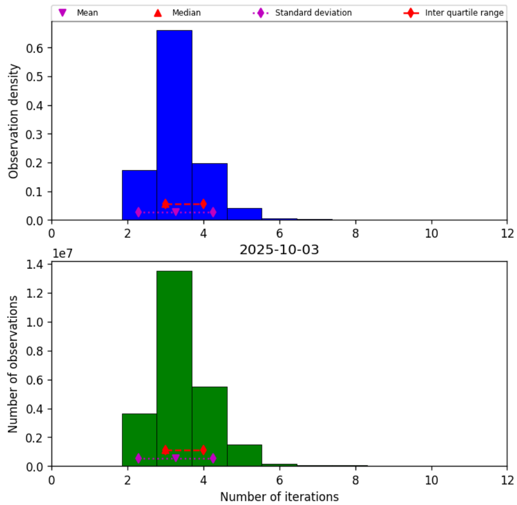
Figure 39: Histogram of “Number of iterations” for 2025-10-02 to 2025-10-04
