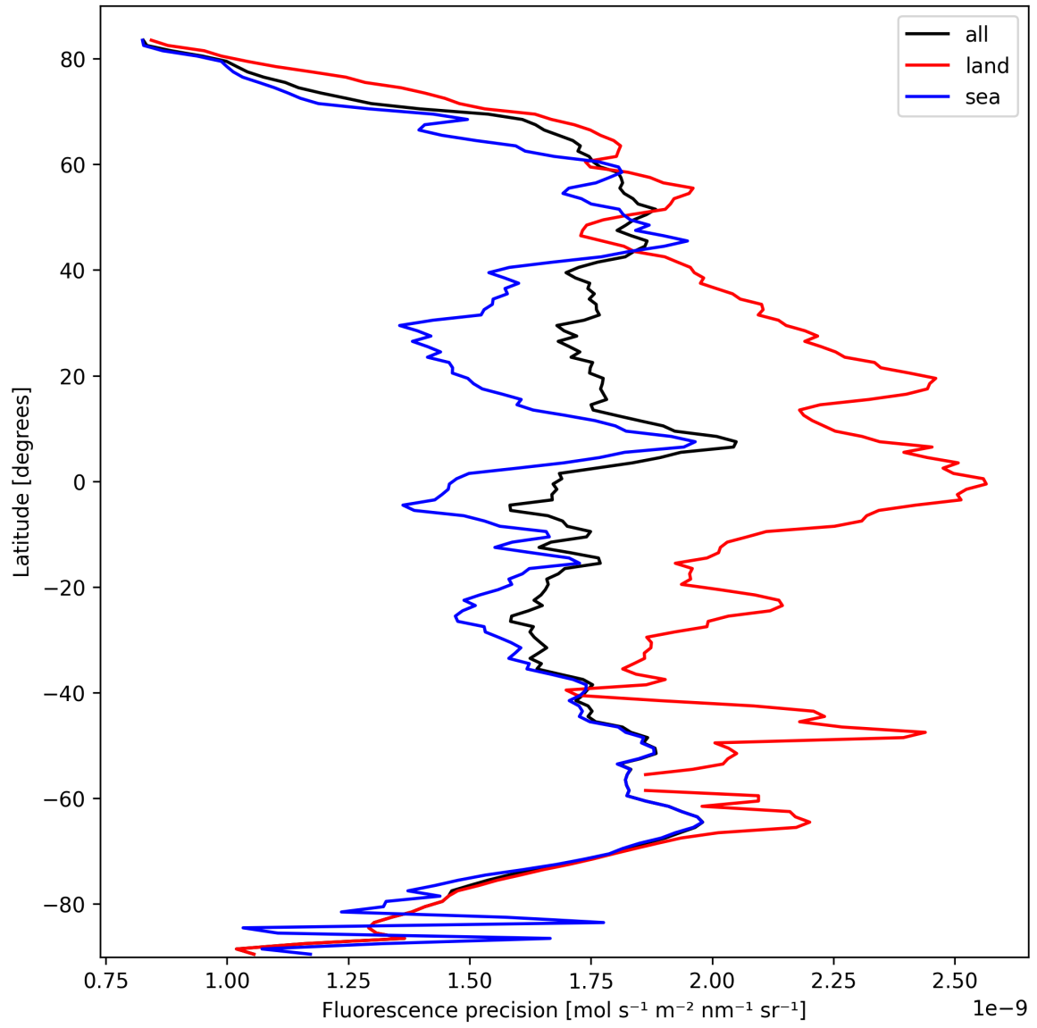
Figure 24: Zonal average of “Fluorescence precision” for 2025-10-02 to 2025-10-04.
