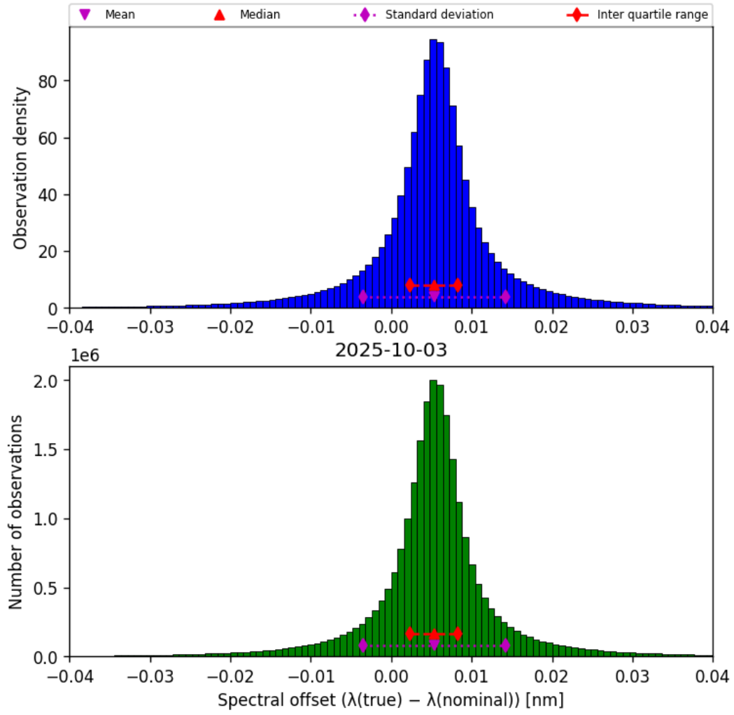
Figure 45: Histogram of “Spectral offset ( \lambda_{\text{true}} - \lambda_{\text{nominal}} )” for 2025-10-02 to 2025-10-04
