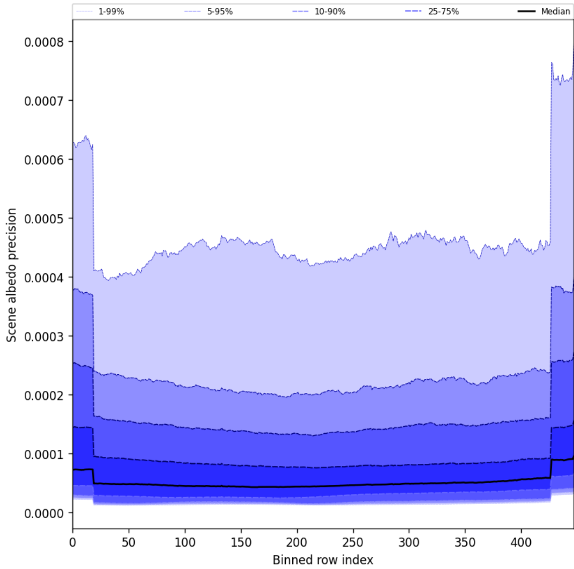
Figure 52: Along track statistics of “Scene albedo precision” for 2025-10-02 to 2025-10-04
