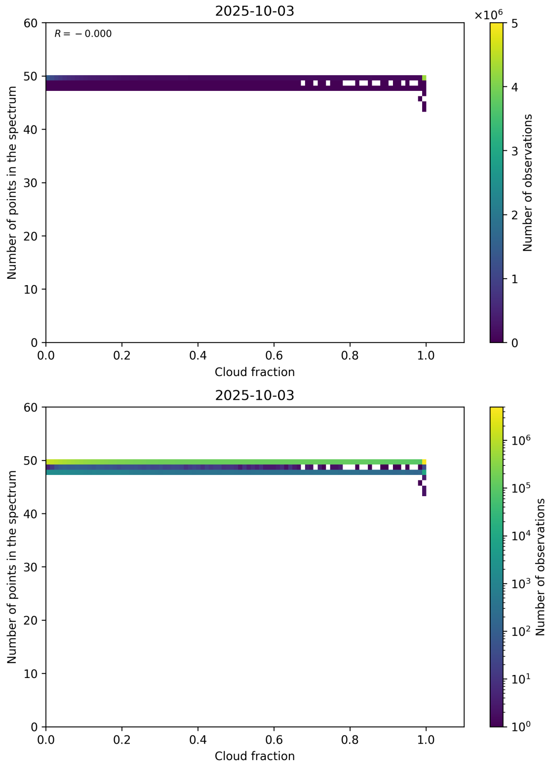
Figure 74: Scatter density plot of “Cloud fraction” against “Number of points in the spectrum” for 2025-10-02 to 2025-10-04.
