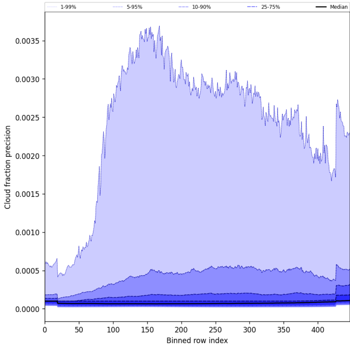
Figure 50: Along track statistics of “Cloud fraction precision” for 2025-10-02 to 2025-10-04
