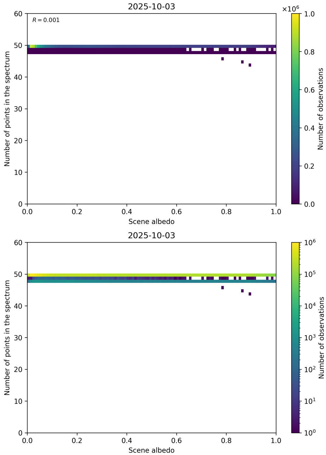
Figure 106: Scatter density plot of “Scene albedo” against “Number of points in the spectrum” for 2025-10-02 to 2025-10-04.
