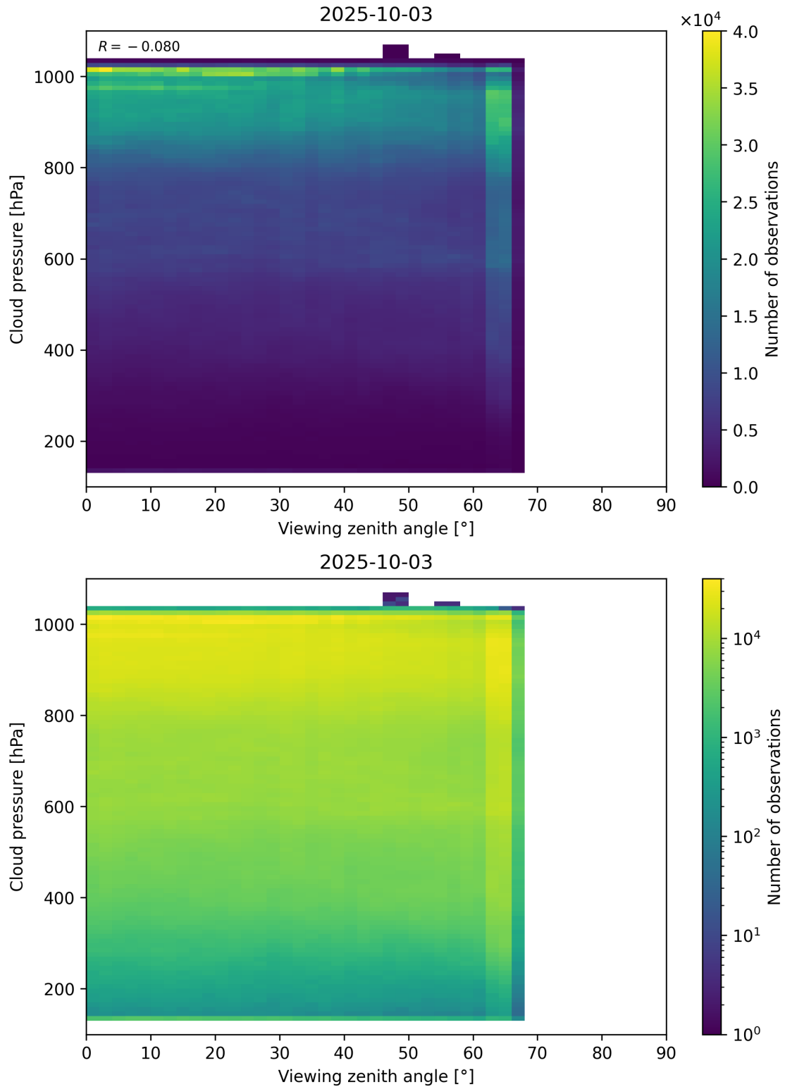
Figure 121: Scatter density plot of “Viewing zenith angle” against “Cloud pressure” for 2025-10-02 to 2025-10-04.
