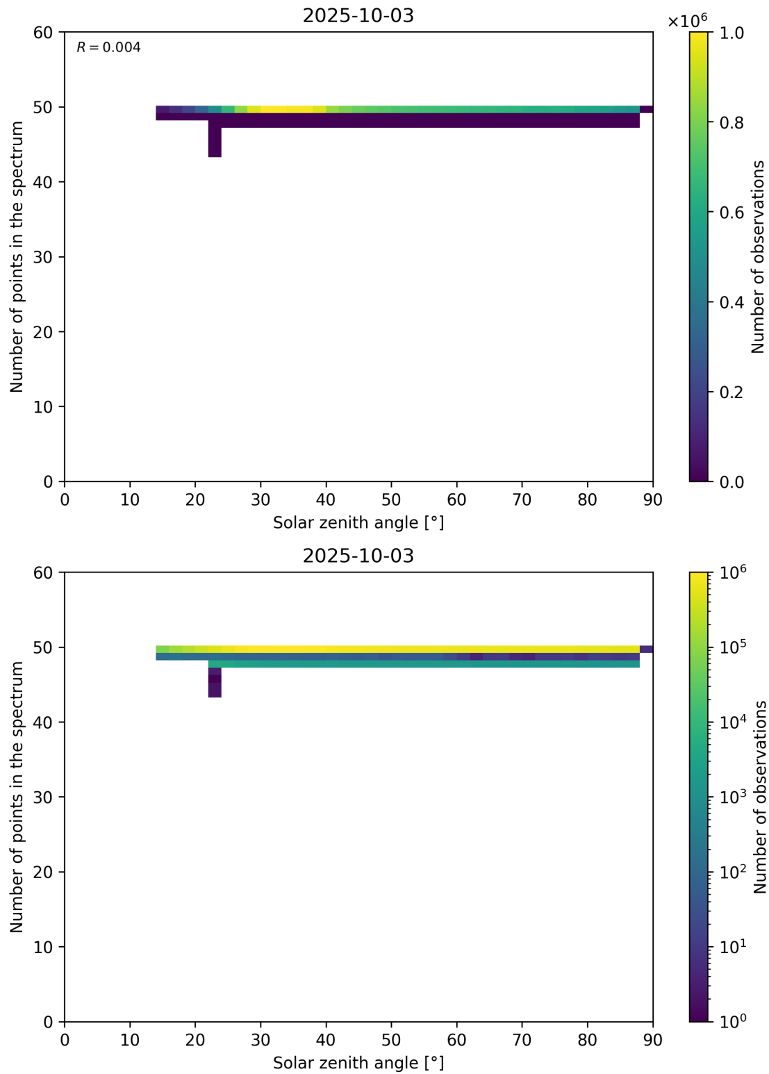
Figure 115: Scatter density plot of “Solar zenith angle” against “Number of points in the spectrum” for 2025-10-02 to 2025-10-04.
