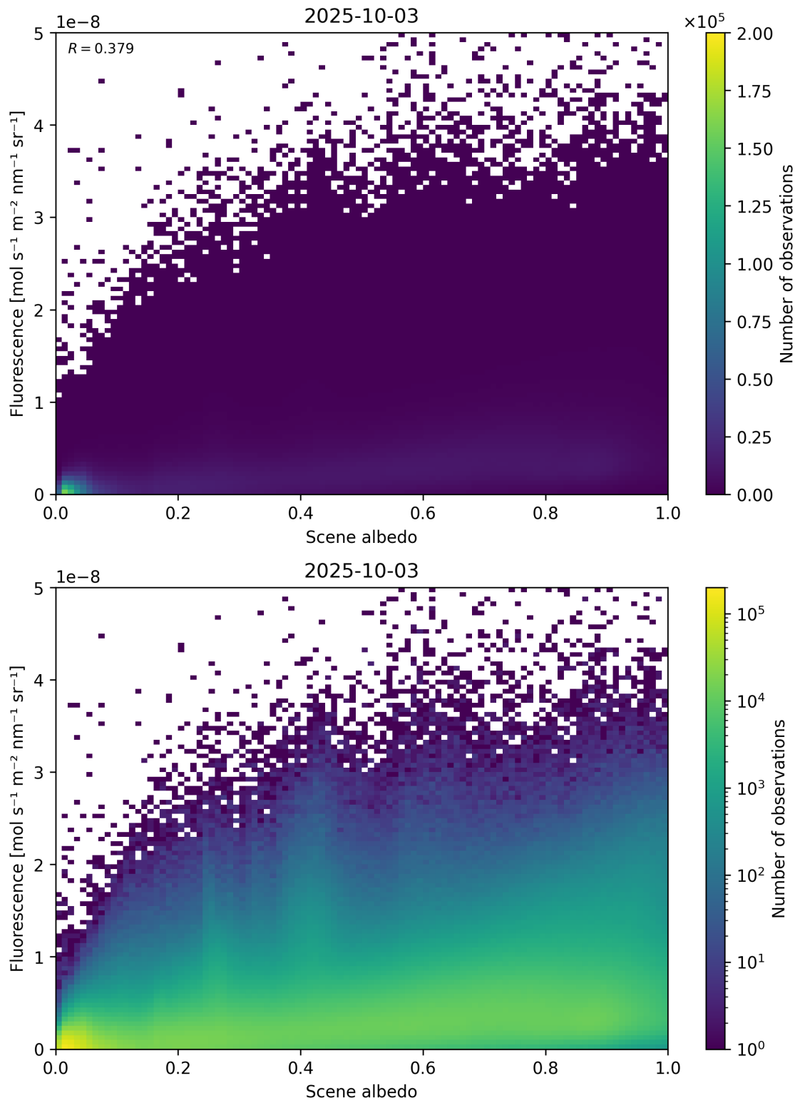
Figure 104: Scatter density plot of “Scene albedo” against “Fluorescence” for 2025-10-02 to 2025-10-04.
