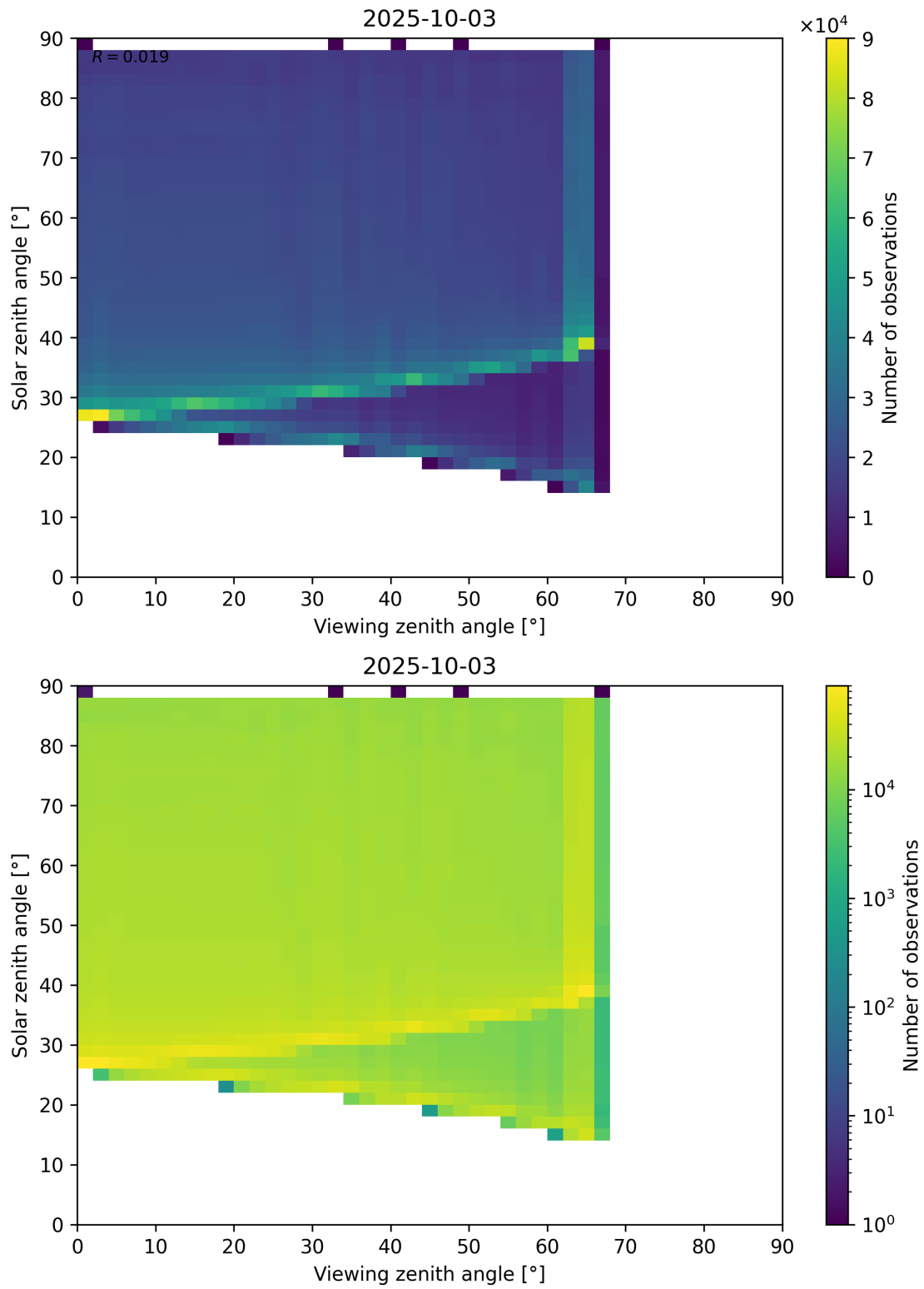
Figure 127: Scatter density plot of “Viewing zenith angle” against “Solar zenith angle” for 2025-10-02 to 2025-10-04.
