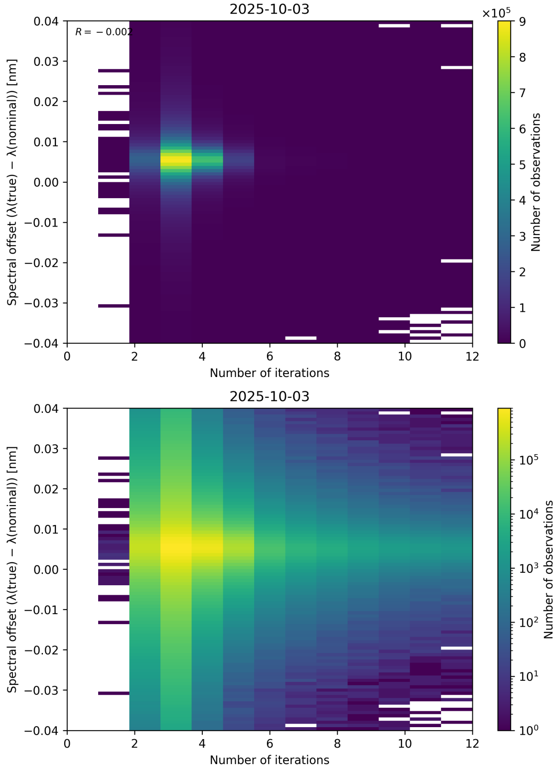
Figure 100: Scatter density plot of “Number of iterations” against “Spectral offset ( \lambda_{\text{true}} - \lambda_{\text{nominal}} )” for 2025-10-02 to 2025-10-04.
