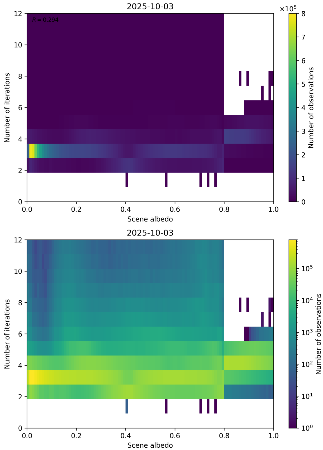
Figure 105: Scatter density plot of “Scene albedo” against “Number of iterations” for 2025-10-02 to 2025-10-04.
