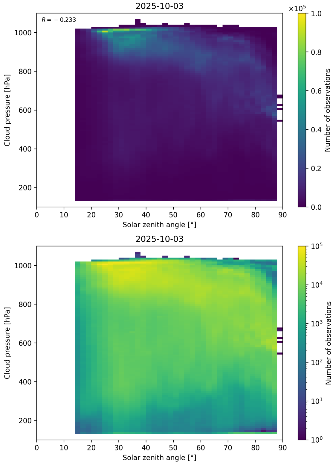
Figure 111: Scatter density plot of “Solar zenith angle” against “Cloud pressure” for 2025-10-02 to 2025-10-04.
