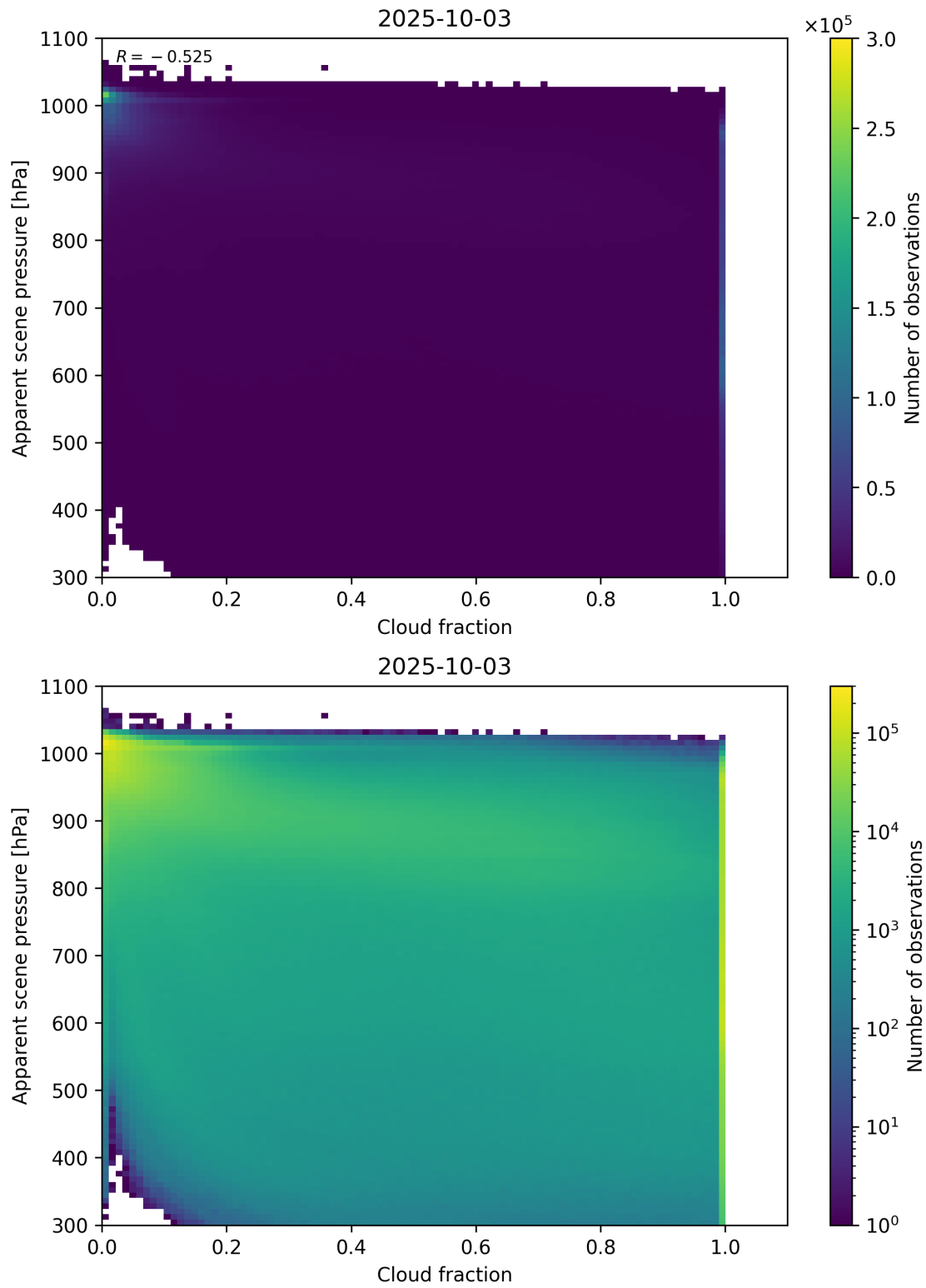
Figure 70: Scatter density plot of “Cloud fraction” against “Apparent scene pressure” for 2025-10-02 to 2025-10-04.
