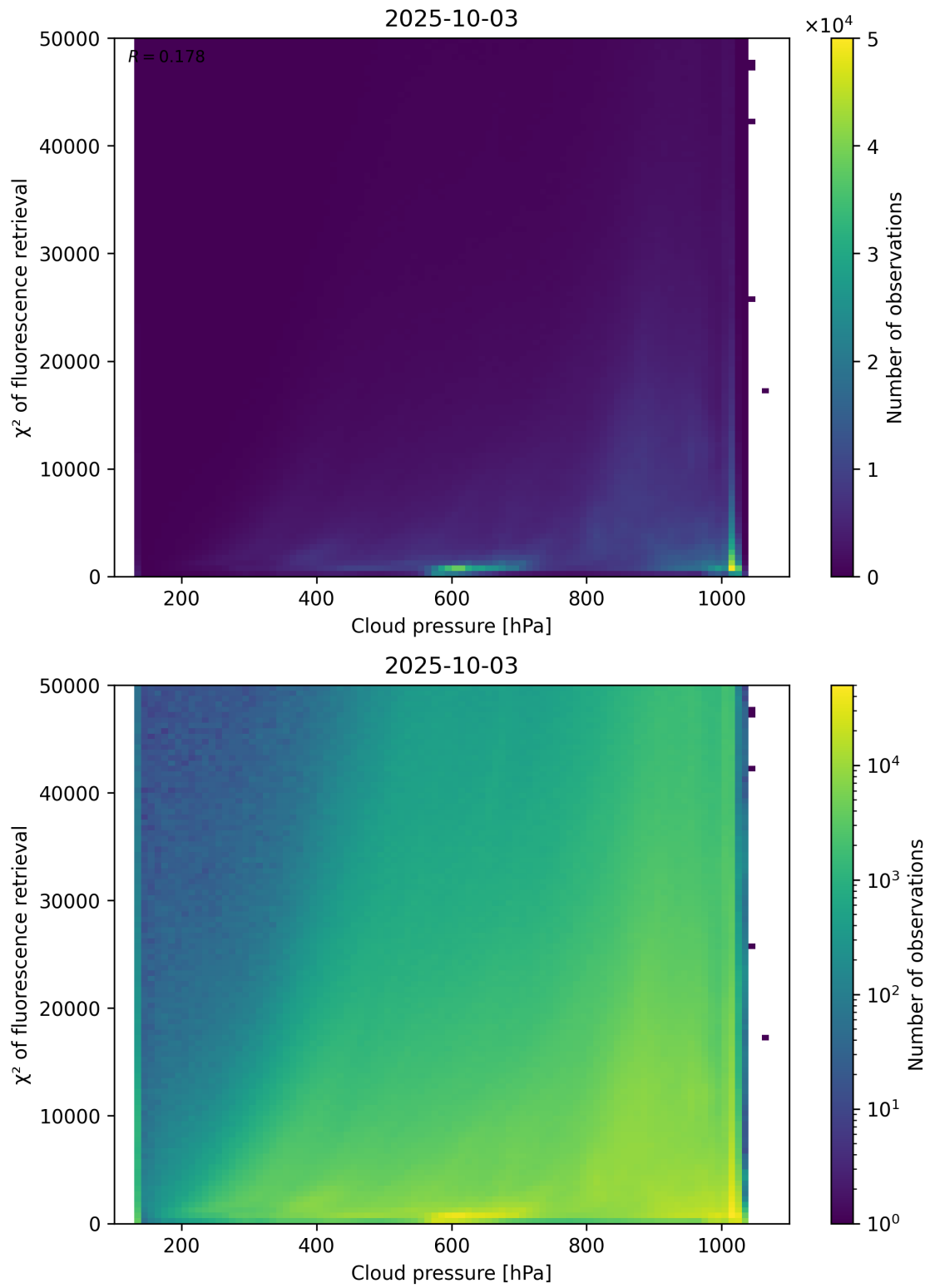
Figure 78: Scatter density plot of “Cloud pressure” against “ \chi^2 of fluorescence retrieval” for 2025-10-02 to 2025-10-04.
