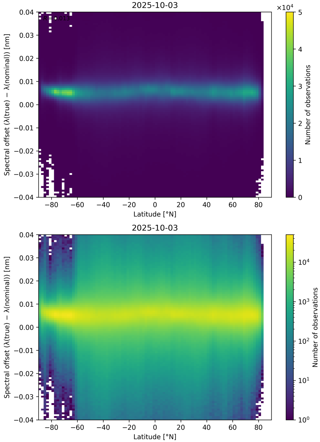
Figure 96: Scatter density plot of “Latitude” against “Spectral offset ( \lambda_{\text{true}} - \lambda_{\text{nominal}} )” for 2025-10-02 to 2025-10-04.
