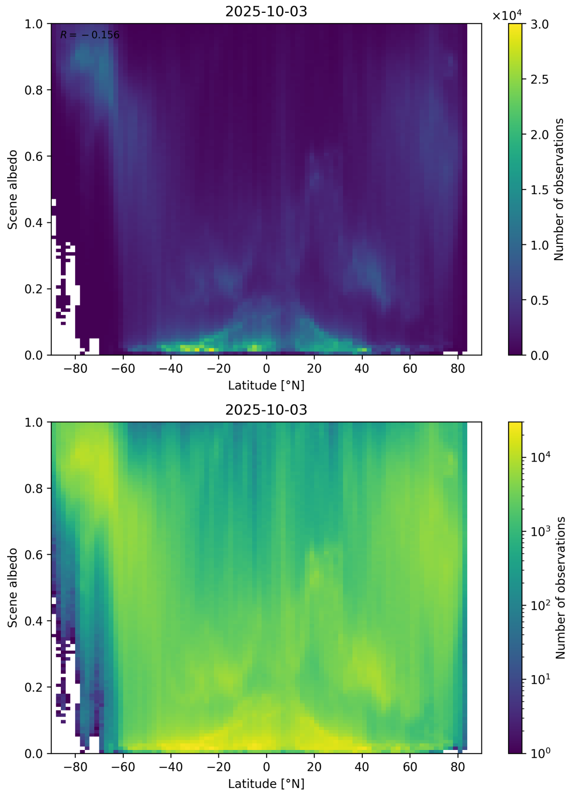
Figure 95: Scatter density plot of “Latitude” against “Scene albedo” for 2025-10-02 to 2025-10-04.
