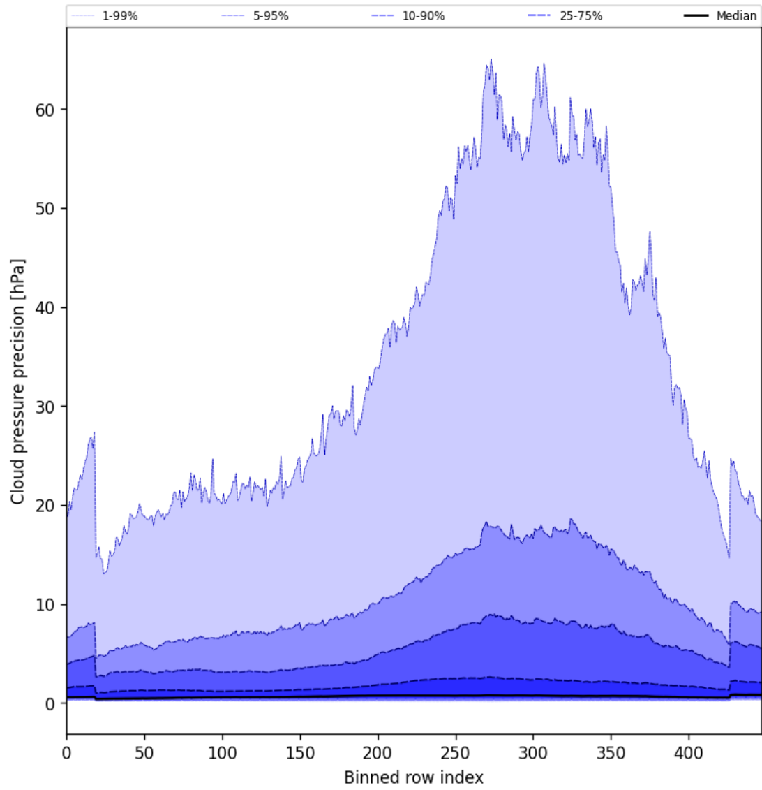
Figure 48: Along track statistics of “Cloud pressure precision” for 2025-10-02 to 2025-10-04
