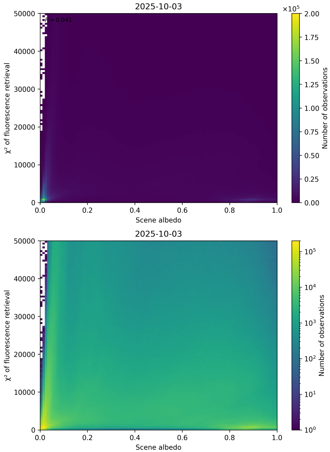
Figure 103: Scatter density plot of “Scene albedo” against “ \chi^2 of fluorescence retrieval” for 2025-10-02 to 2025-10-04.
