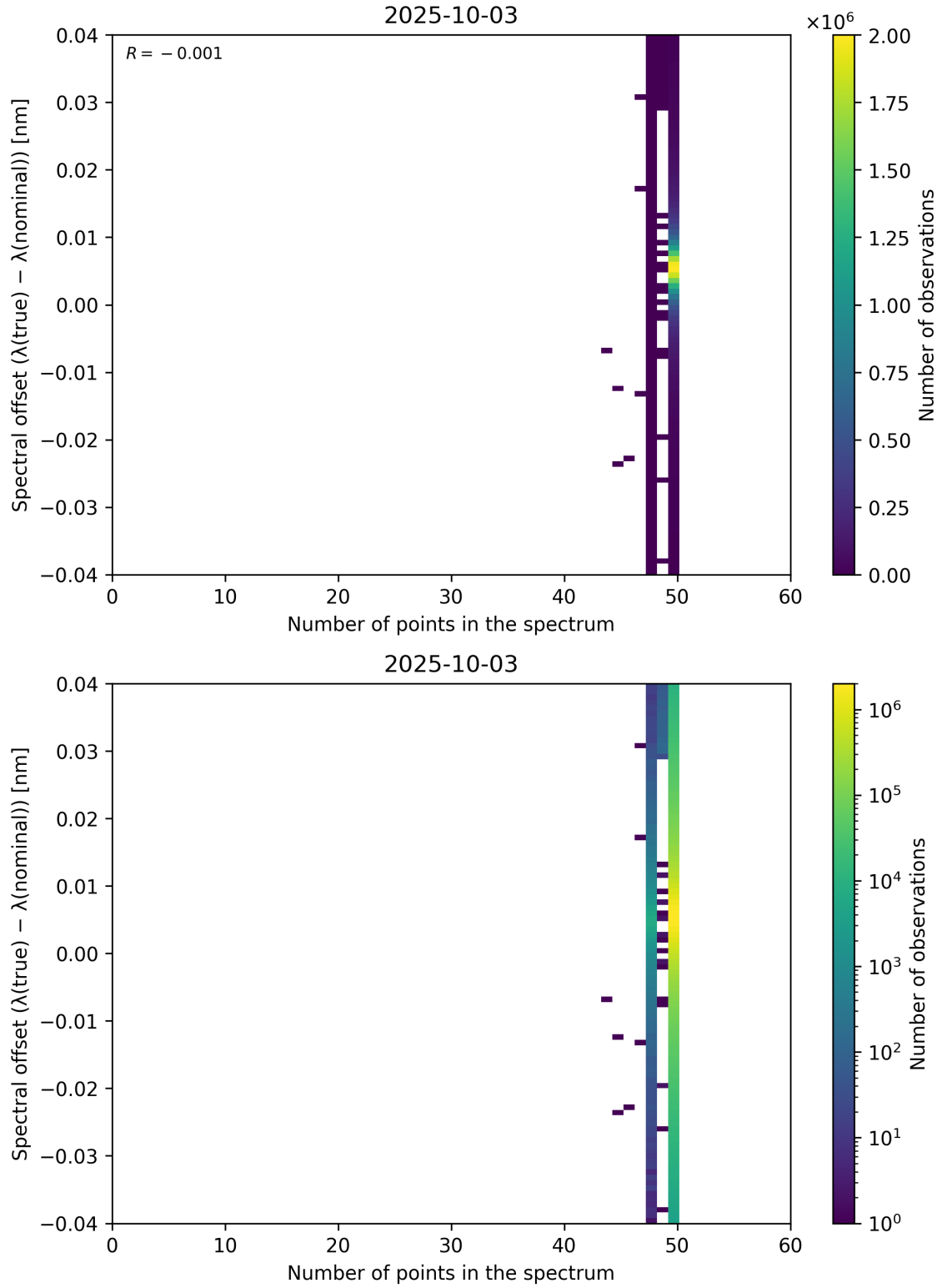
Figure 101: Scatter density plot of “Number of points in the spectrum” against “Spectral offset ( \lambda_{\text{true}} - \lambda_{\text{nominal}} )” for 2025-10-02 to 2025-10-04.
