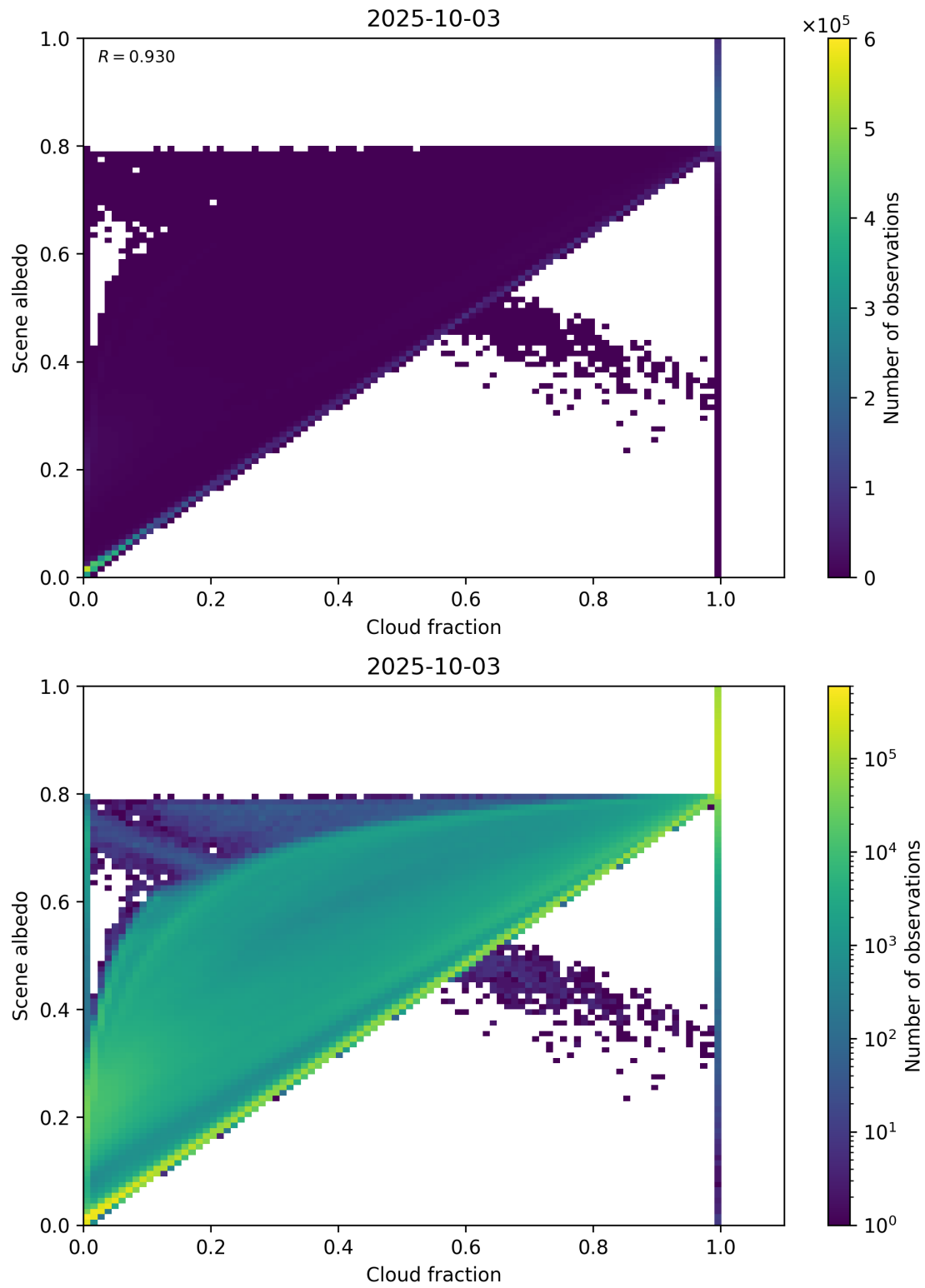
Figure 75: Scatter density plot of “Cloud fraction” against “Scene albedo” for 2025-10-02 to 2025-10-04.
