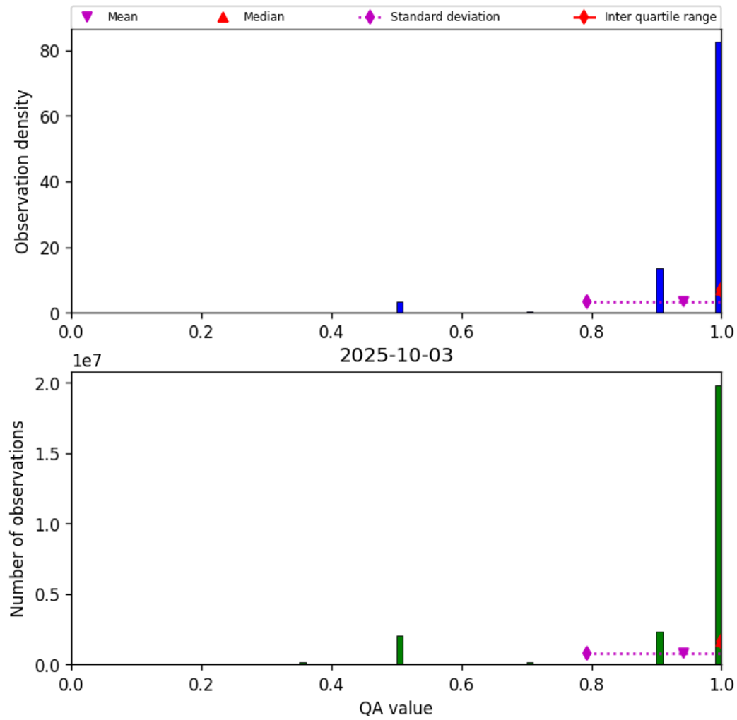
Figure 29: Histogram of “QA value” for 2025-10-02 to 2025-10-04
