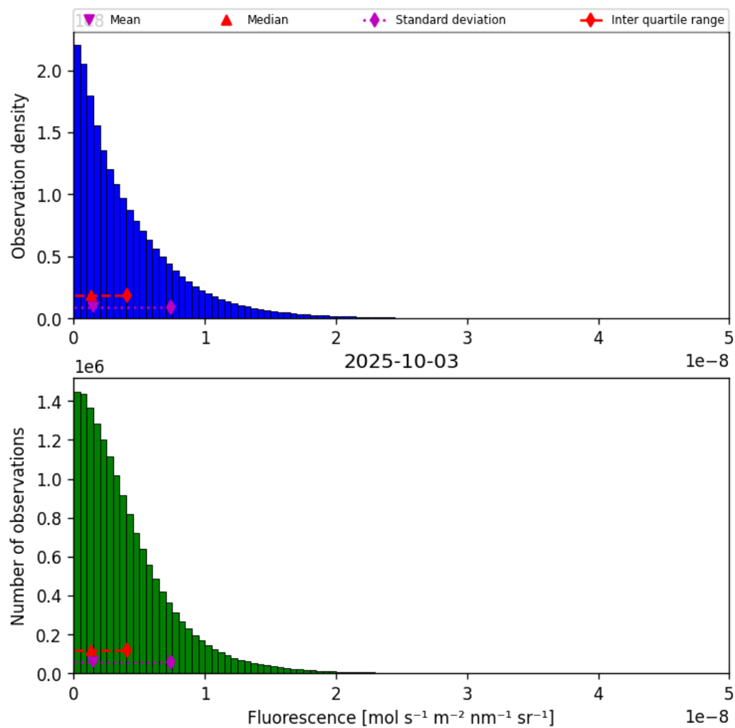
Figure 40: Histogram of “Fluorescence” for 2025-10-02 to 2025-10-04
