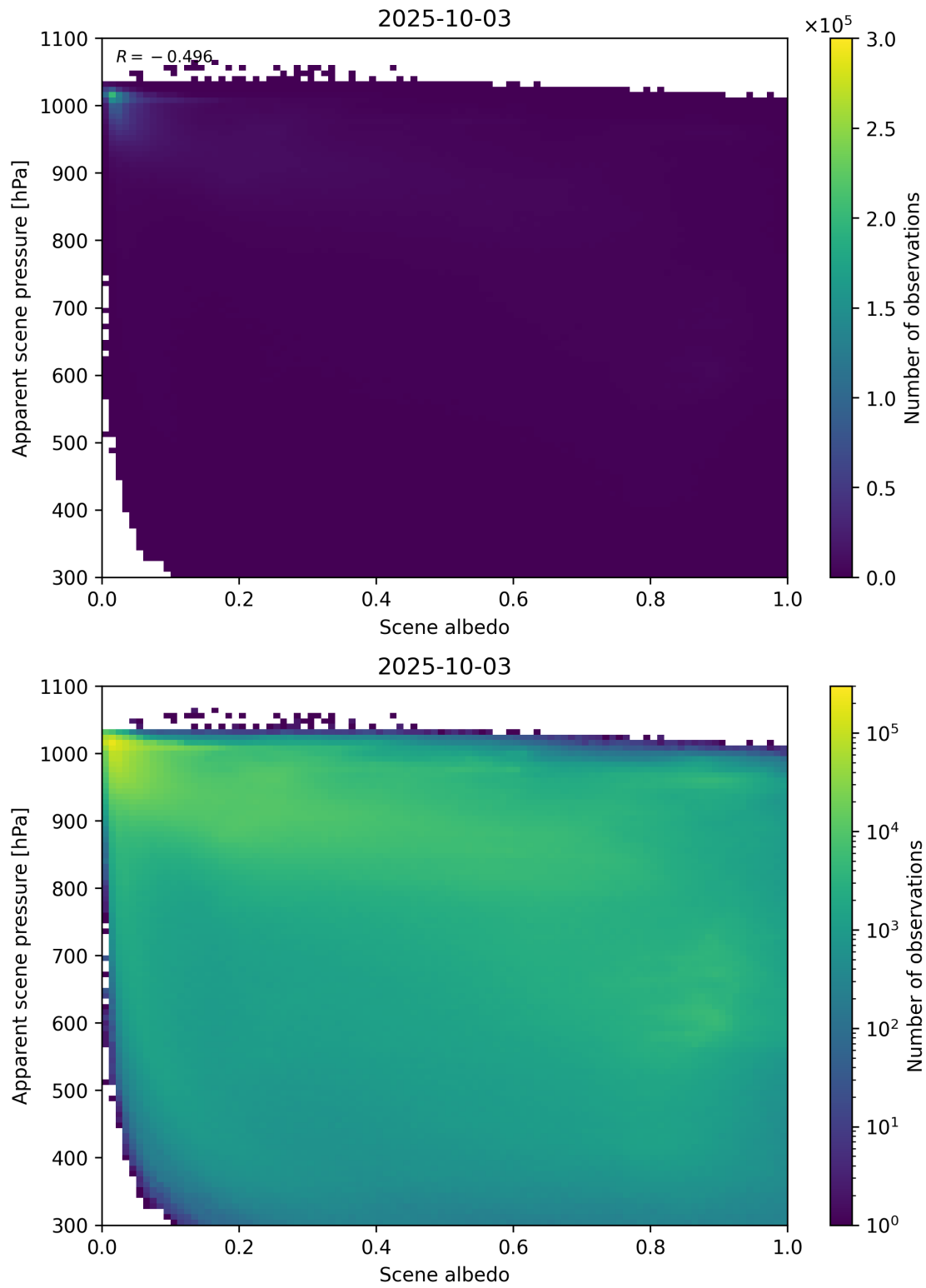
Figure 102: Scatter density plot of “Scene albedo” against “Apparent scene pressure” for 2025-10-02 to 2025-10-04.
