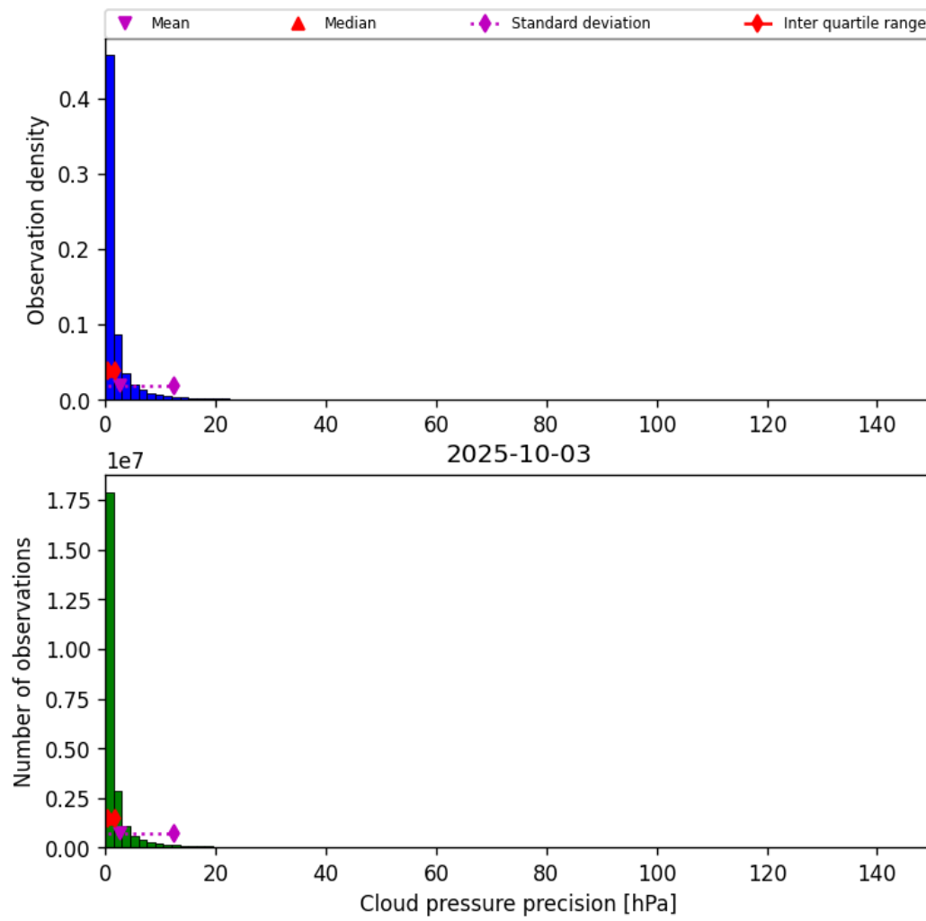
Figure 31: Histogram of “Cloud pressure precision” for 2025-10-02 to 2025-10-04
