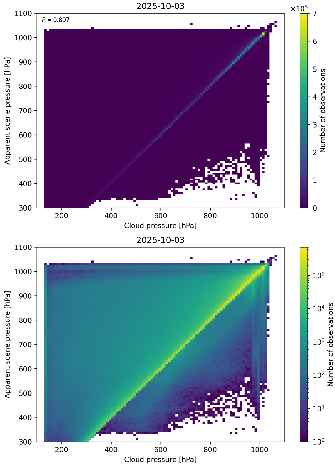
Figure 77: Scatter density plot of “Cloud pressure” against “Apparent scene pressure” for 2025-10-02 to 2025-10-04.
