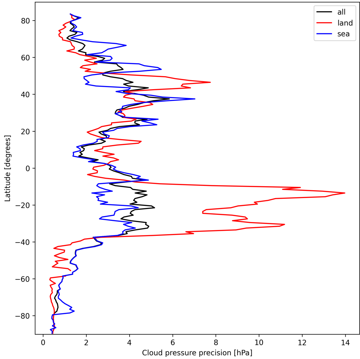
Figure 14: Zonal average of “Cloud pressure precision” for 2025-10-02 to 2025-10-04.
