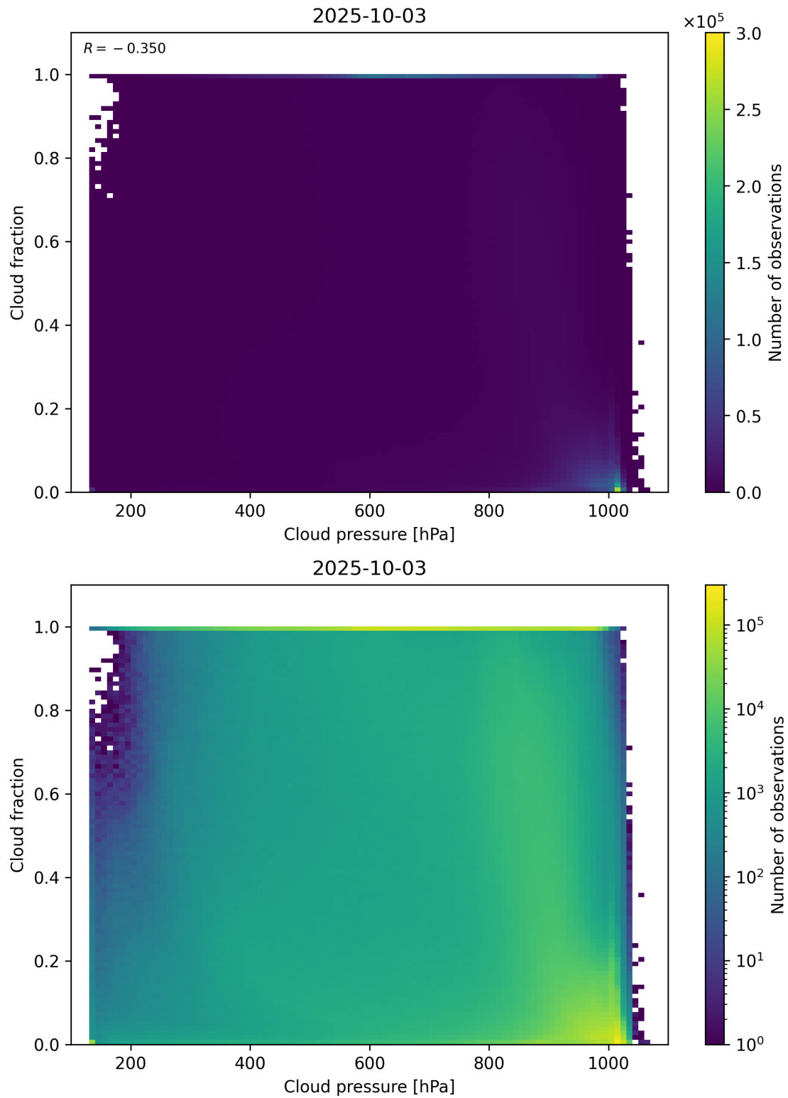
Figure 79: Scatter density plot of “Cloud pressure” against “Cloud fraction” for 2025-10-02 to 2025-10-04.
