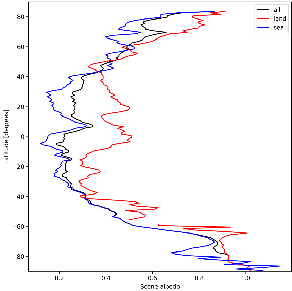
Figure 17: Zonal average of “Scene albedo” for 2025-10-02 to 2025-10-04.
