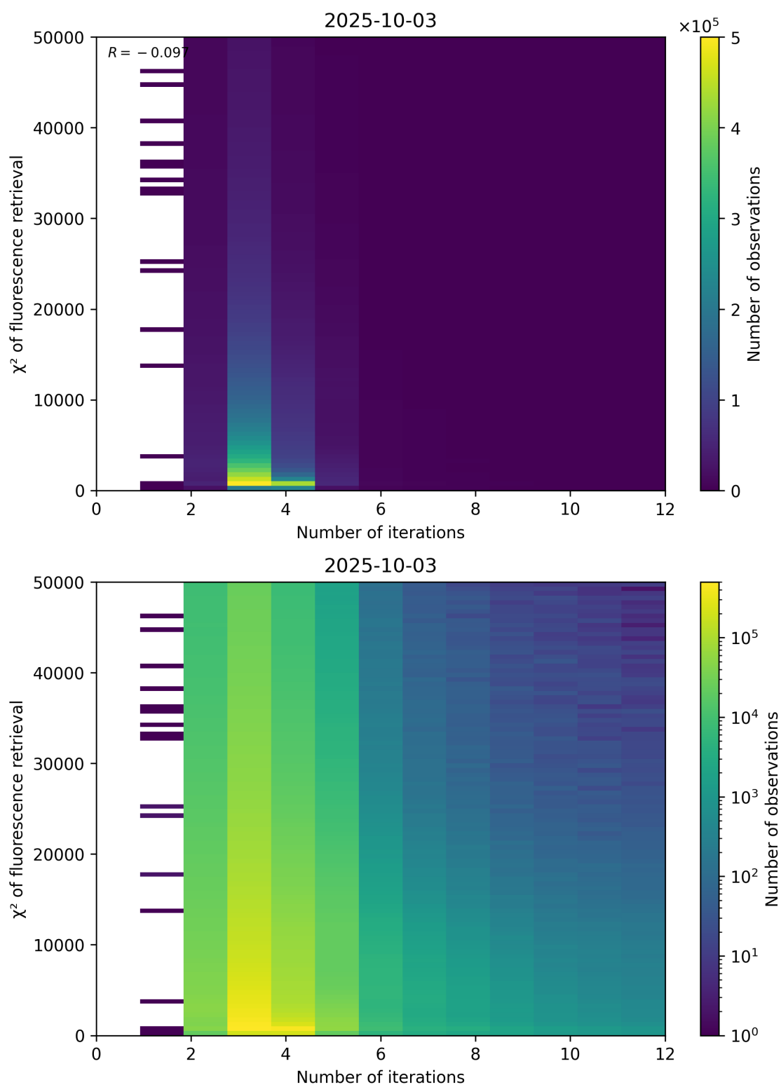
Figure 97: Scatter density plot of “Number of iterations” against “ \chi^2 of fluorescence retrieval” for 2025-10-02 to 2025-10-04.
