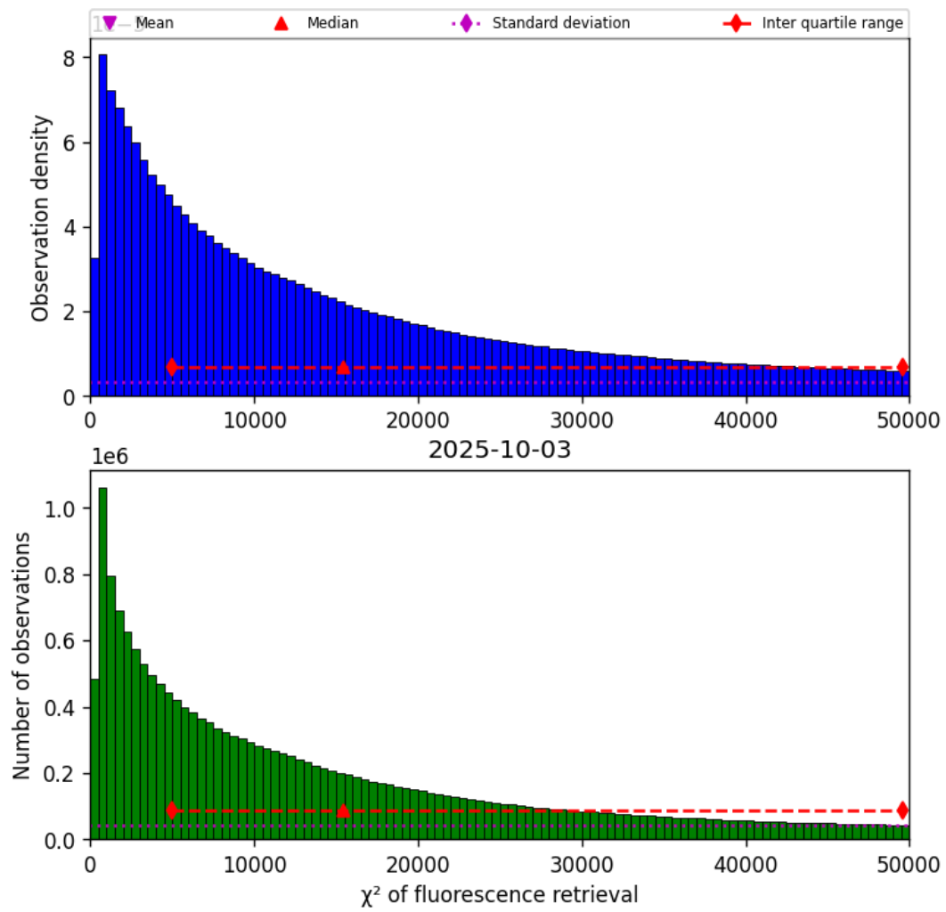
Figure 42: Histogram of “ \chi^2 of fluorescence retrieval” for 2025-10-02 to 2025-10-04
