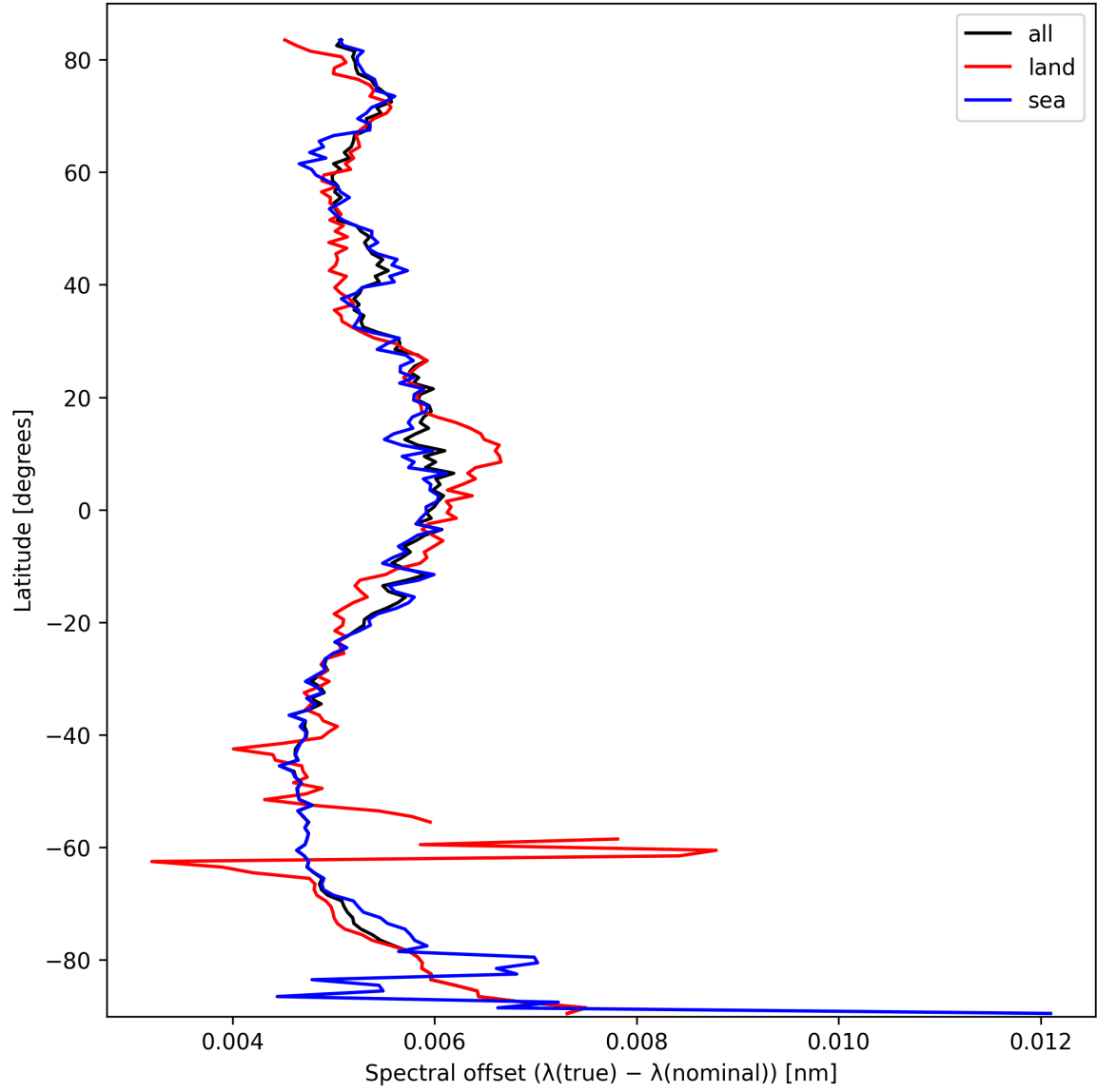
Figure 28: Zonal average of “Spectral offset ( \lambda_{\text{true}} - \lambda_{\text{nominal}} )” for 2025-10-02 to 2025-10-04.
