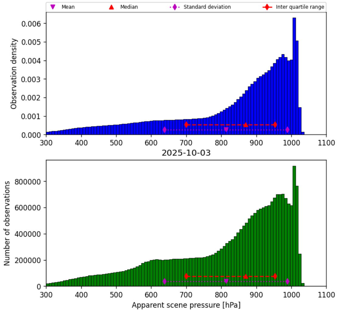
Figure 36: Histogram of “Apparent scene pressure” for 2025-10-02 to 2025-10-04
