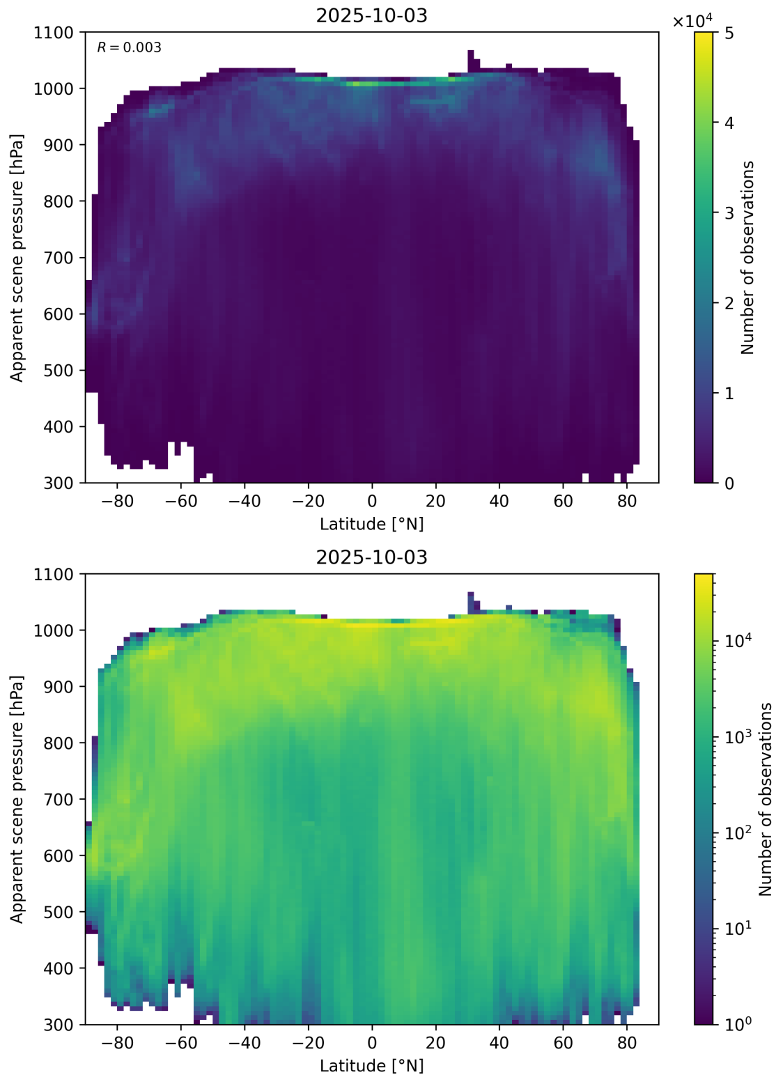
Figure 88: Scatter density plot of “Latitude” against “Apparent scene pressure” for 2025-10-02 to 2025-10-04.
