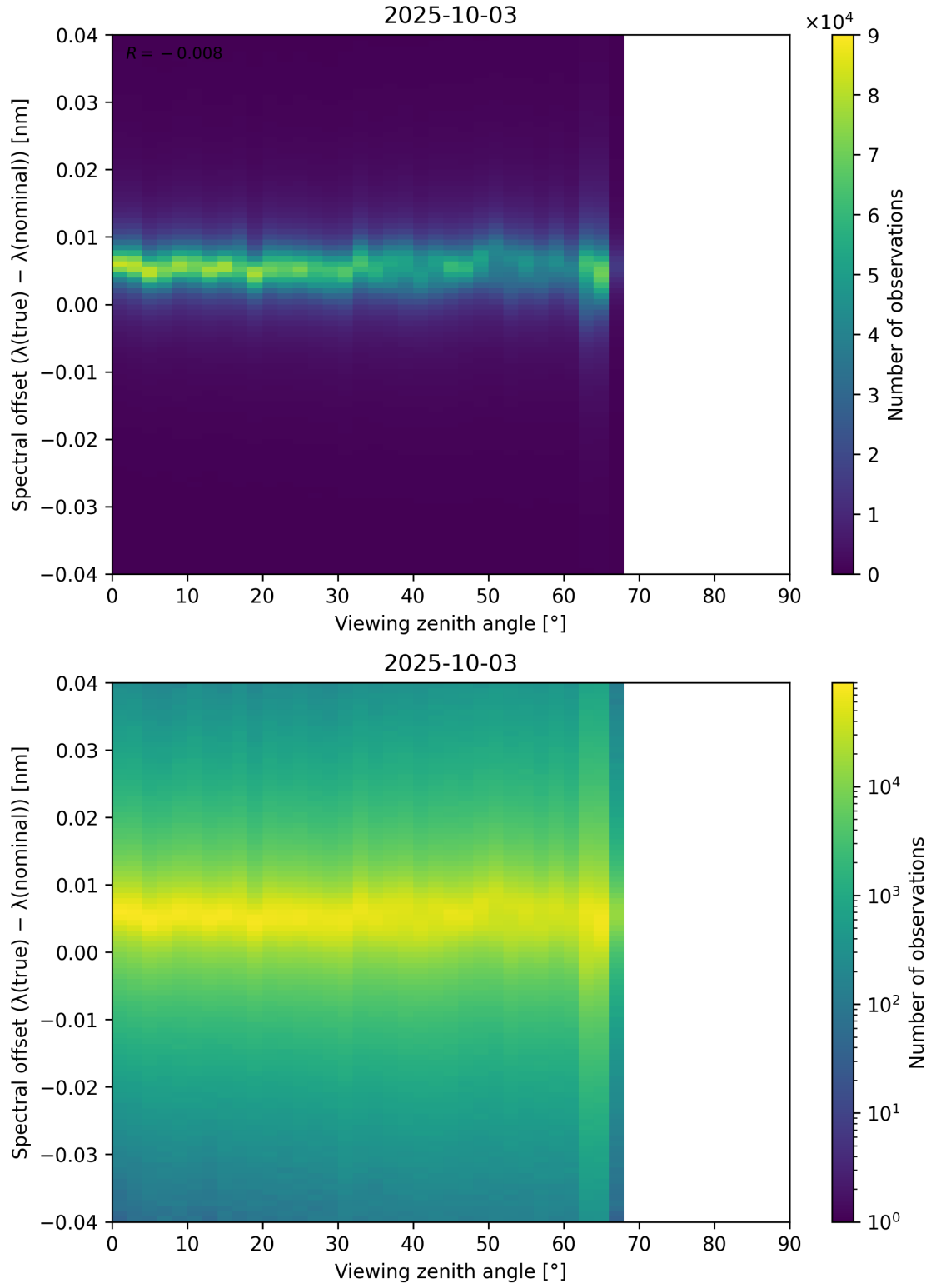
Figure 128: Scatter density plot of “Viewing zenith angle” against “Spectral offset ( \lambda_{\text{true}} - \lambda_{\text{nominal}} )” for 2025-10-02 to 2025-10-04.
