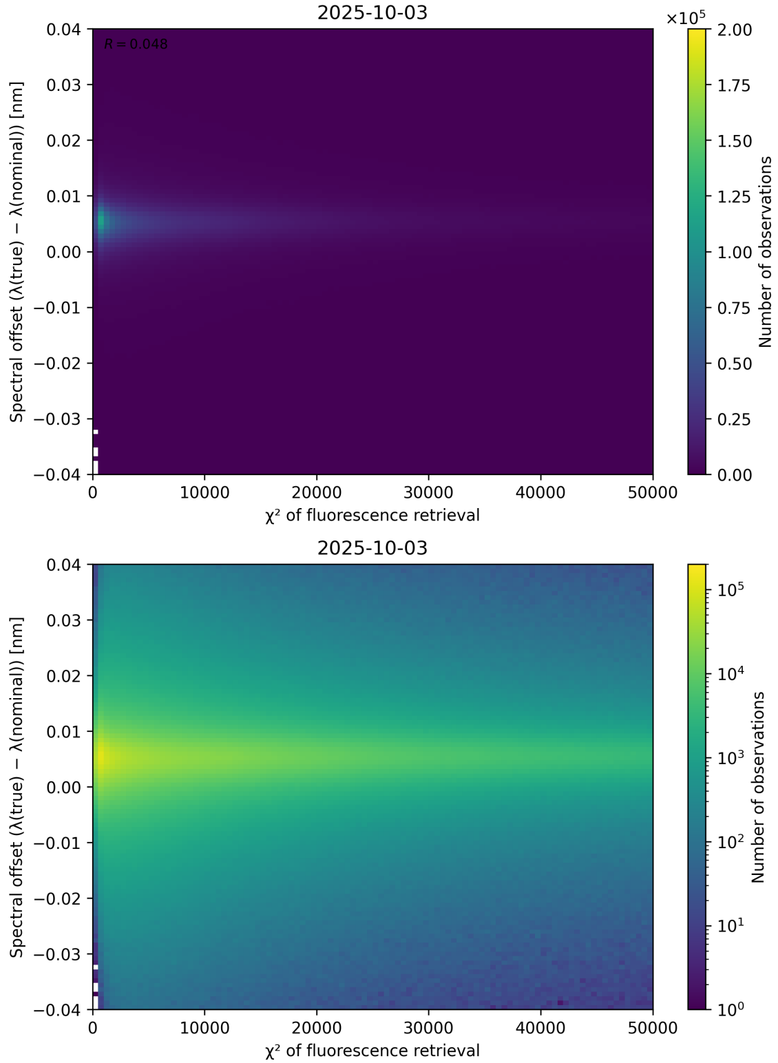
Figure 69: Scatter density plot of “ \chi^2 of fluorescence retrieval” against “Spectral offset ( \lambda_{\text{true}} - \lambda_{\text{nominal}} )” for 2025-10-02 to 2025-10-04.
