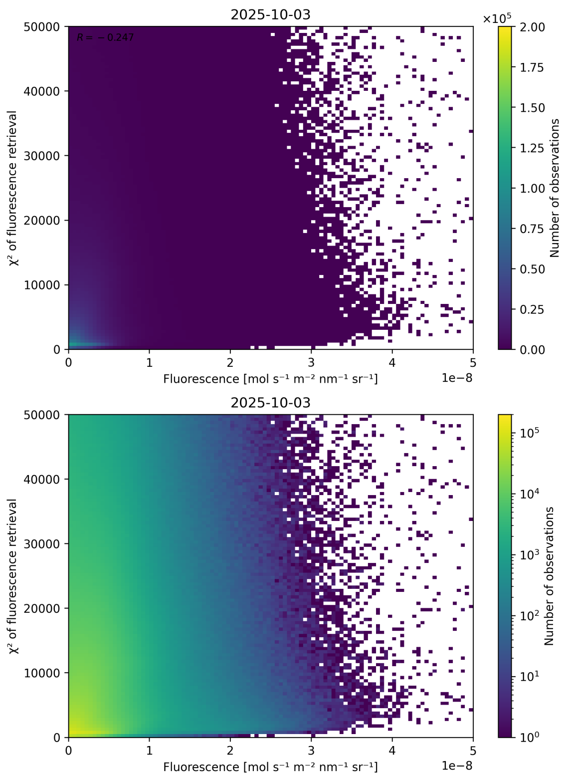
Figure 85: Scatter density plot of “Fluorescence” against “ \chi^2 of fluorescence retrieval” for 2025-10-02 to 2025-10-04.
