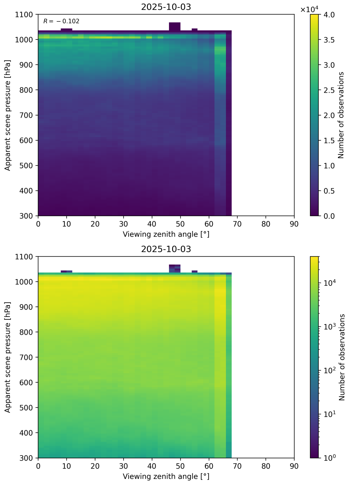
Figure 118: Scatter density plot of “Viewing zenith angle” against “Apparent scene pressure” for 2025-10-02 to 2025-10-04.
