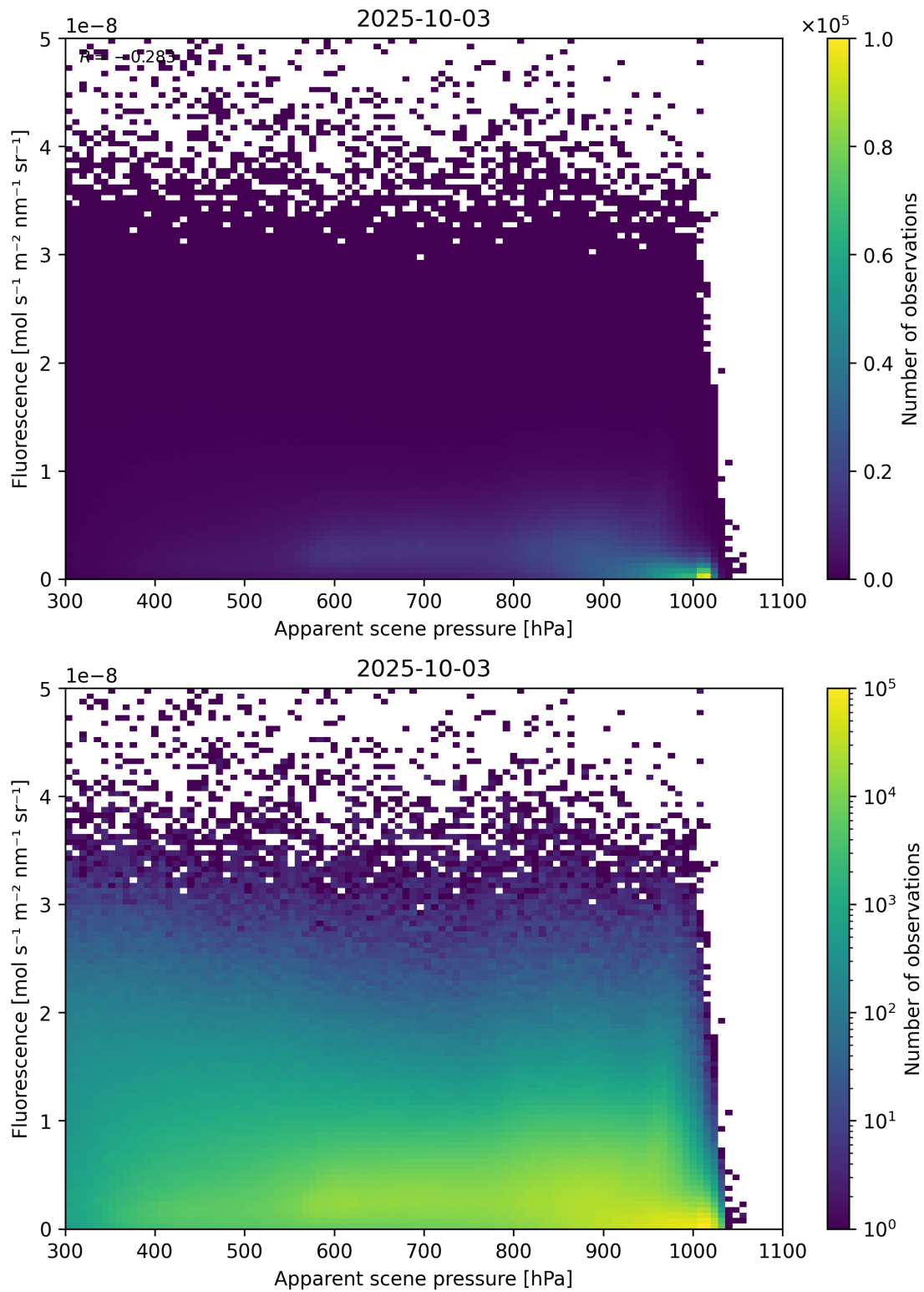
Figure 64: Scatter density plot of “Apparent scene pressure” against “Fluorescence” for 2025-10-02 to 2025-10-04.
