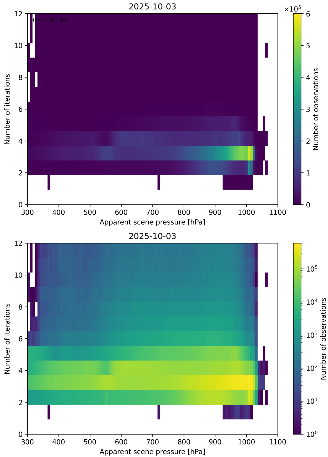
Figure 65: Scatter density plot of “Apparent scene pressure” against “Number of iterations” for 2025-10-02 to 2025-10-04.
