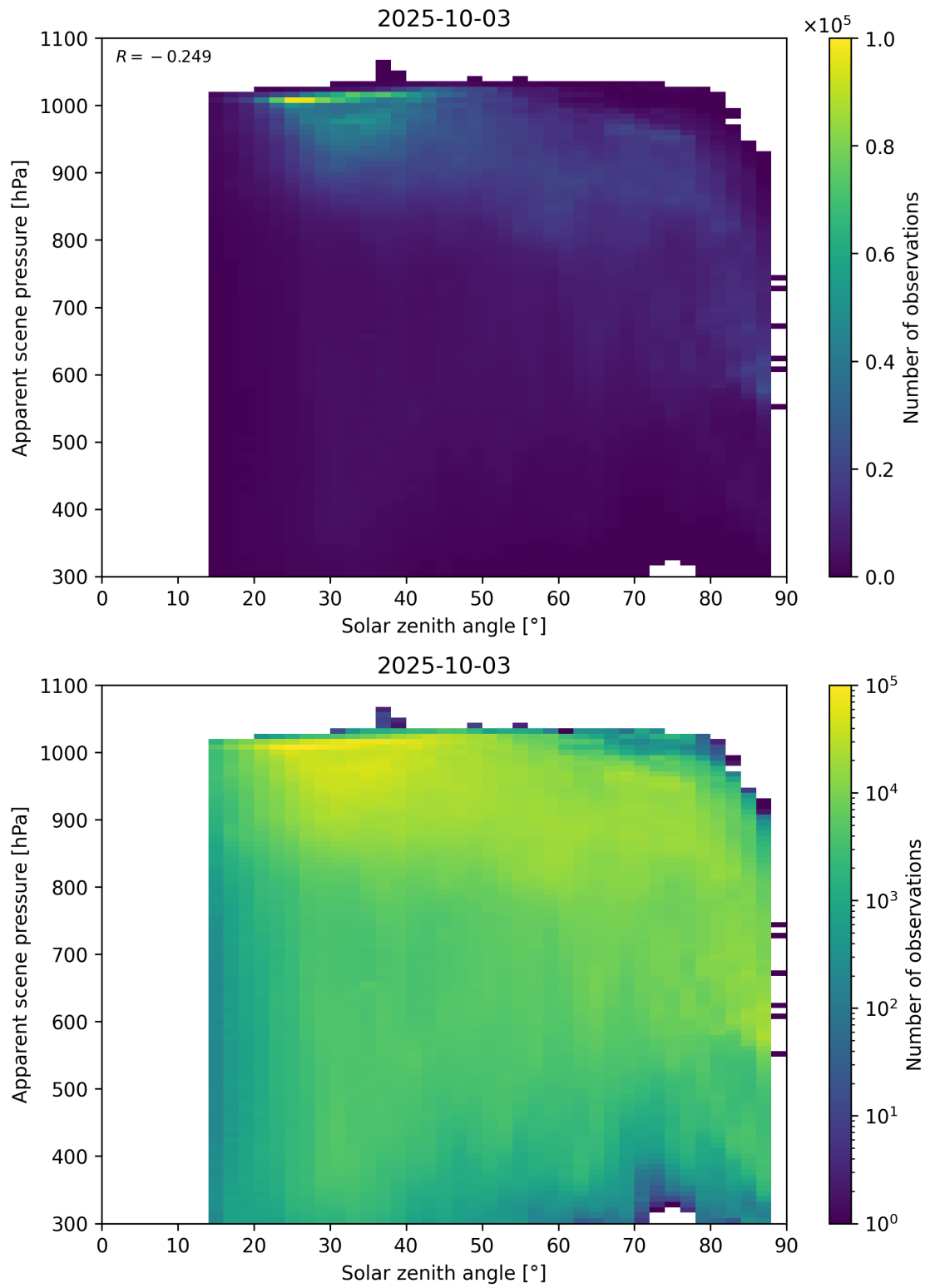
Figure 108: Scatter density plot of “Solar zenith angle” against “Apparent scene pressure” for 2025-10-02 to 2025-10-04.
