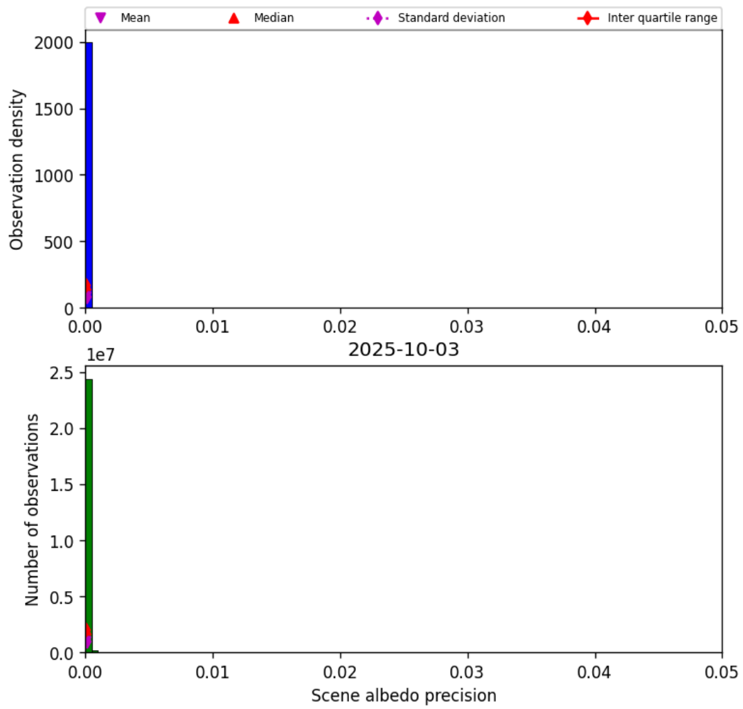
Figure 35: Histogram of “Scene albedo precision” for 2025-10-02 to 2025-10-04
