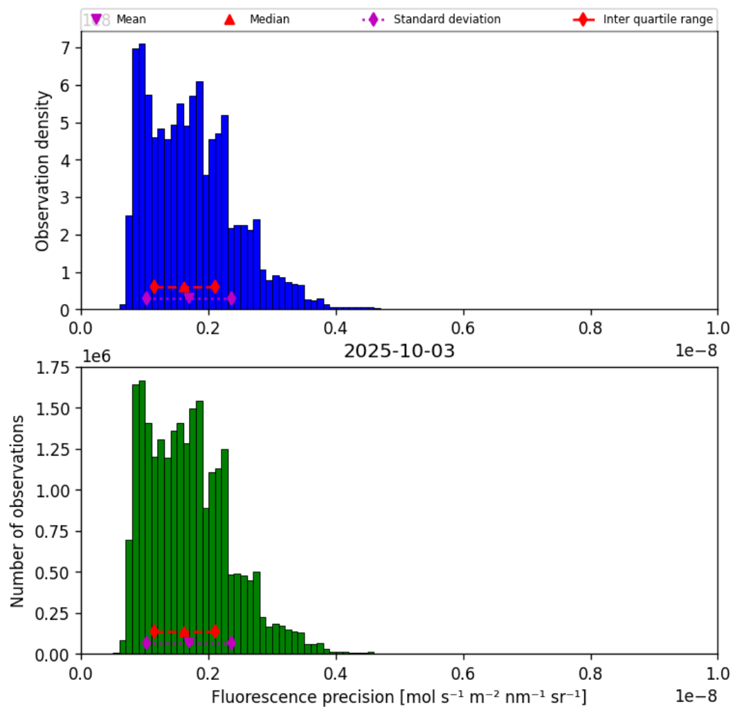
Figure 41: Histogram of “Fluorescence precision” for 2025-10-02 to 2025-10-04
