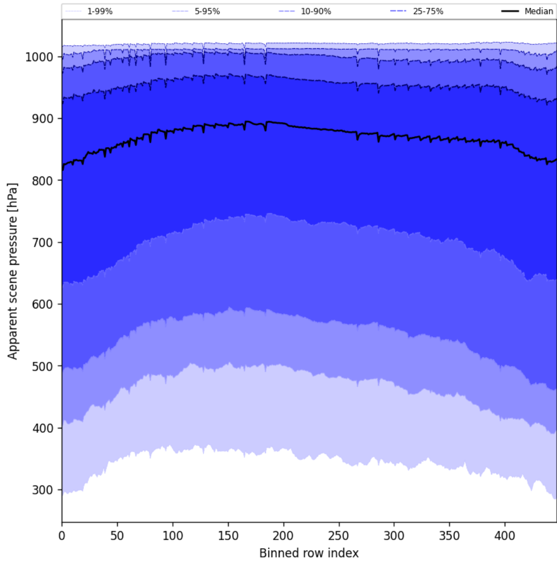
Figure 53: Along track statistics of “Apparent scene pressure” for 2025-10-02 to 2025-10-04
