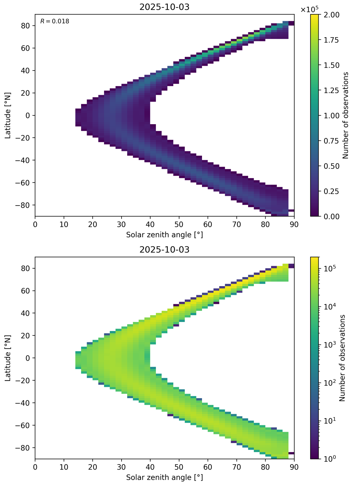
Figure 113: Scatter density plot of “Solar zenith angle” against “Latitude” for 2025-10-02 to 2025-10-04.
