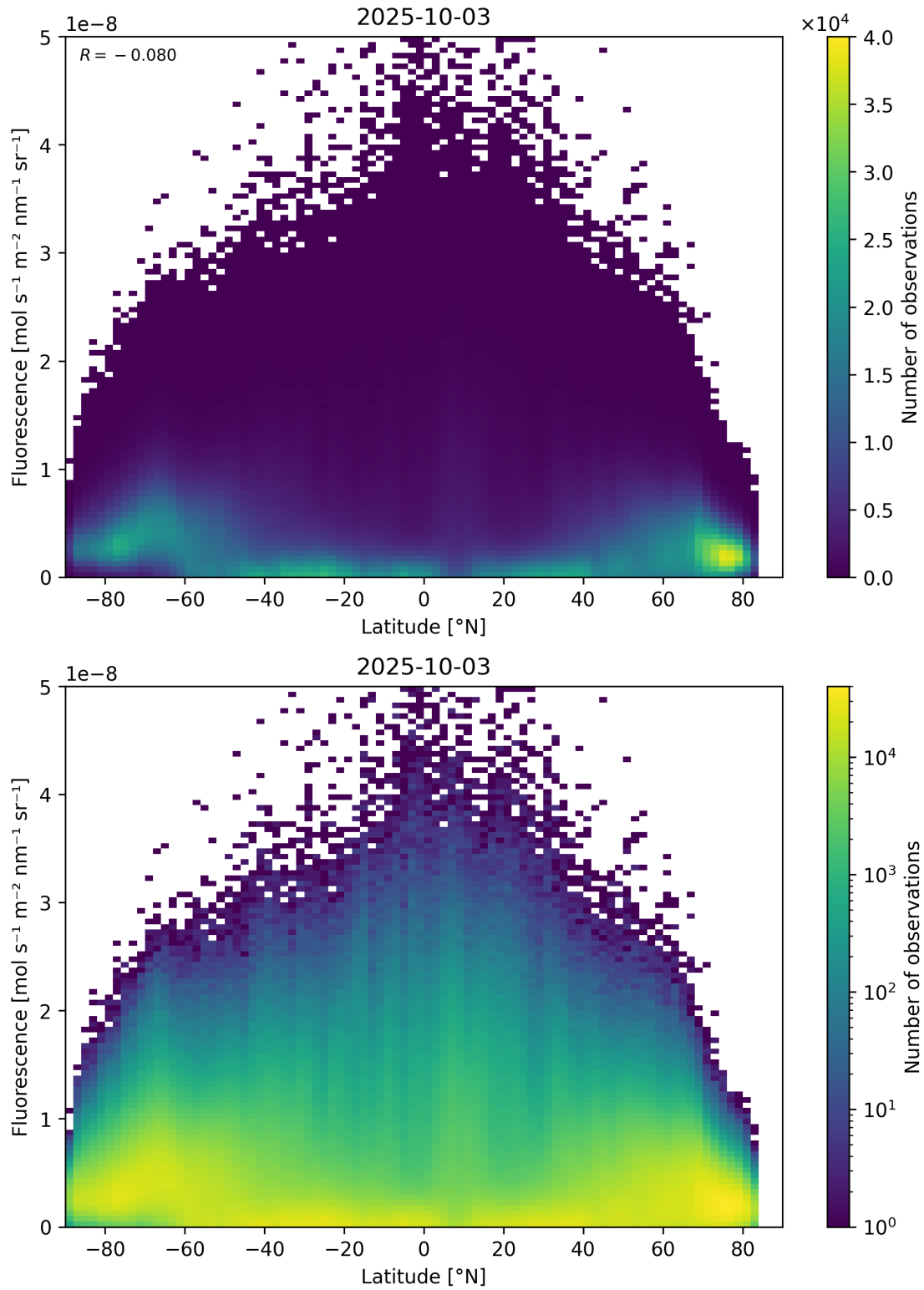
Figure 92: Scatter density plot of “Latitude” against “Fluorescence” for 2025-10-02 to 2025-10-04.
