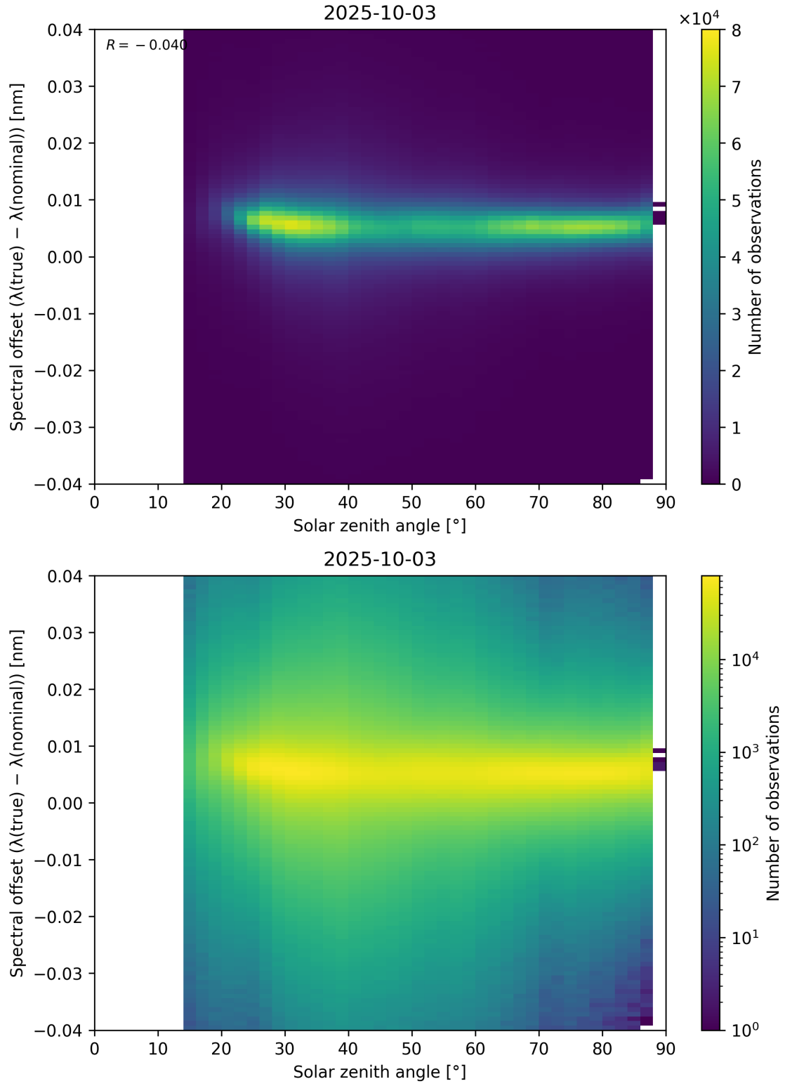
Figure 117: Scatter density plot of “Solar zenith angle” against “Spectral offset ( \lambda_{\text{true}} - \lambda_{\text{nominal}} )” for 2025-10-02 to 2025-10-04.
