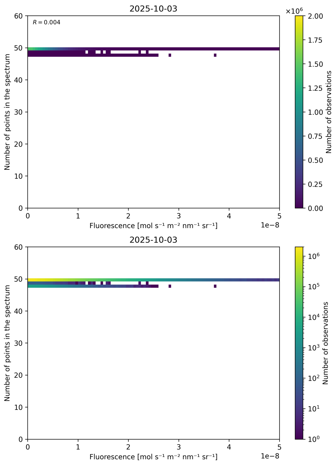
Figure 86: Scatter density plot of “Fluorescence” against “Number of points in the spectrum” for 2025-10-02 to 2025-10-04.
