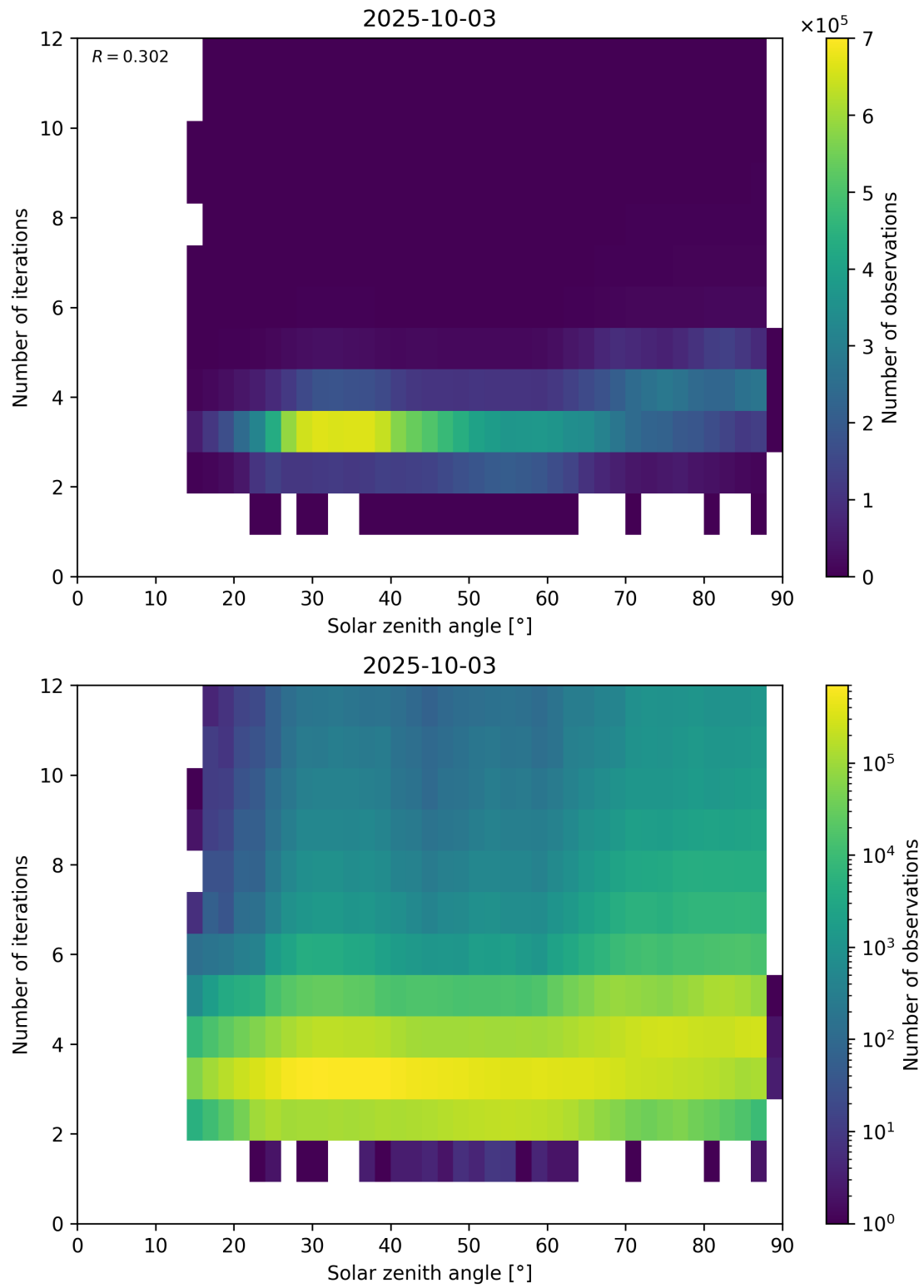
Figure 114: Scatter density plot of “Solar zenith angle” against “Number of iterations” for 2025-10-02 to 2025-10-04.
