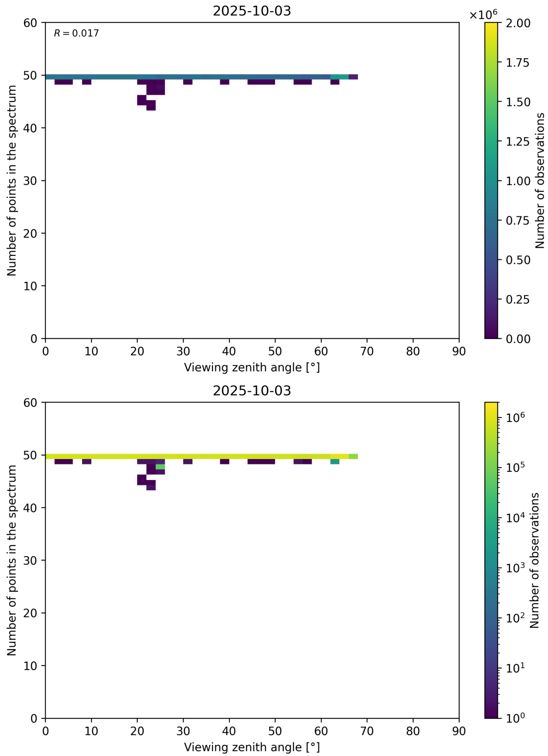
Figure 125: Scatter density plot of “Viewing zenith angle” against “Number of points in the spectrum” for 2025-10-02 to 2025-10-04.
