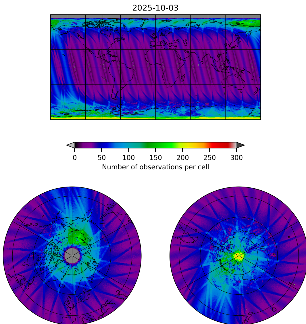
Figure 11: Map of the number of observations for 2025-10-02 to 2025-10-04
