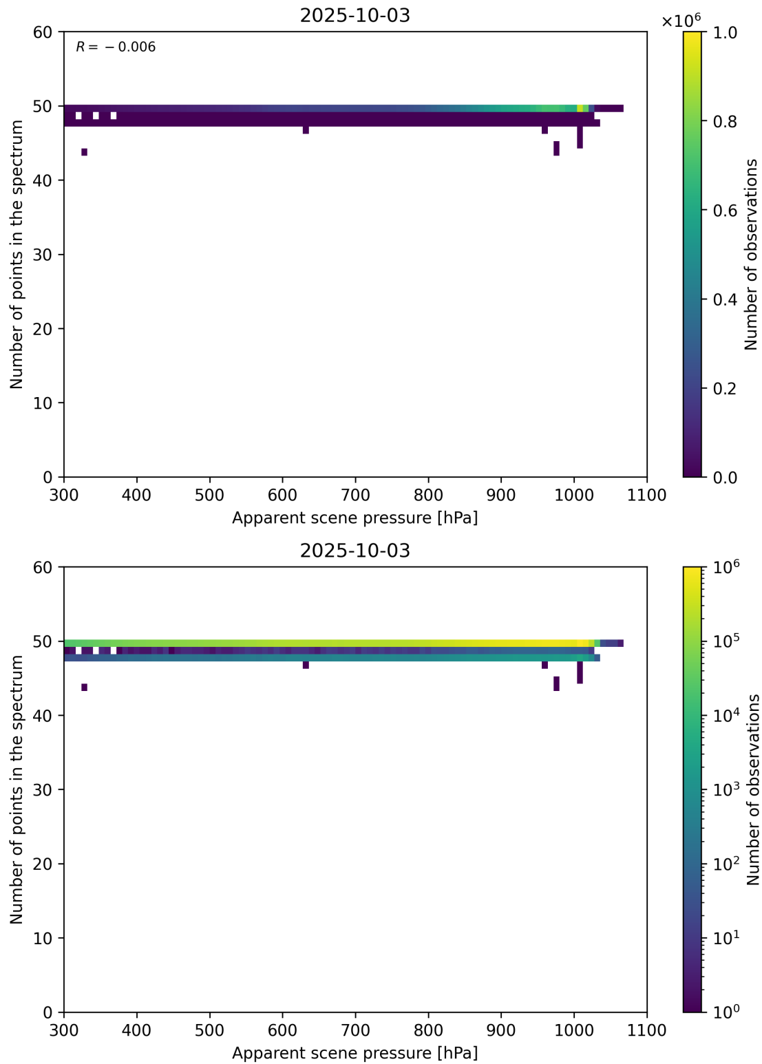
Figure 66: Scatter density plot of “Apparent scene pressure” against “Number of points in the spectrum” for 2025-10-02 to 2025-10-04.
