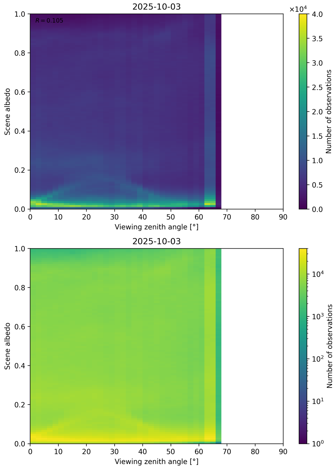
Figure 126: Scatter density plot of “Viewing zenith angle” against “Scene albedo” for 2025-10-02 to 2025-10-04.
