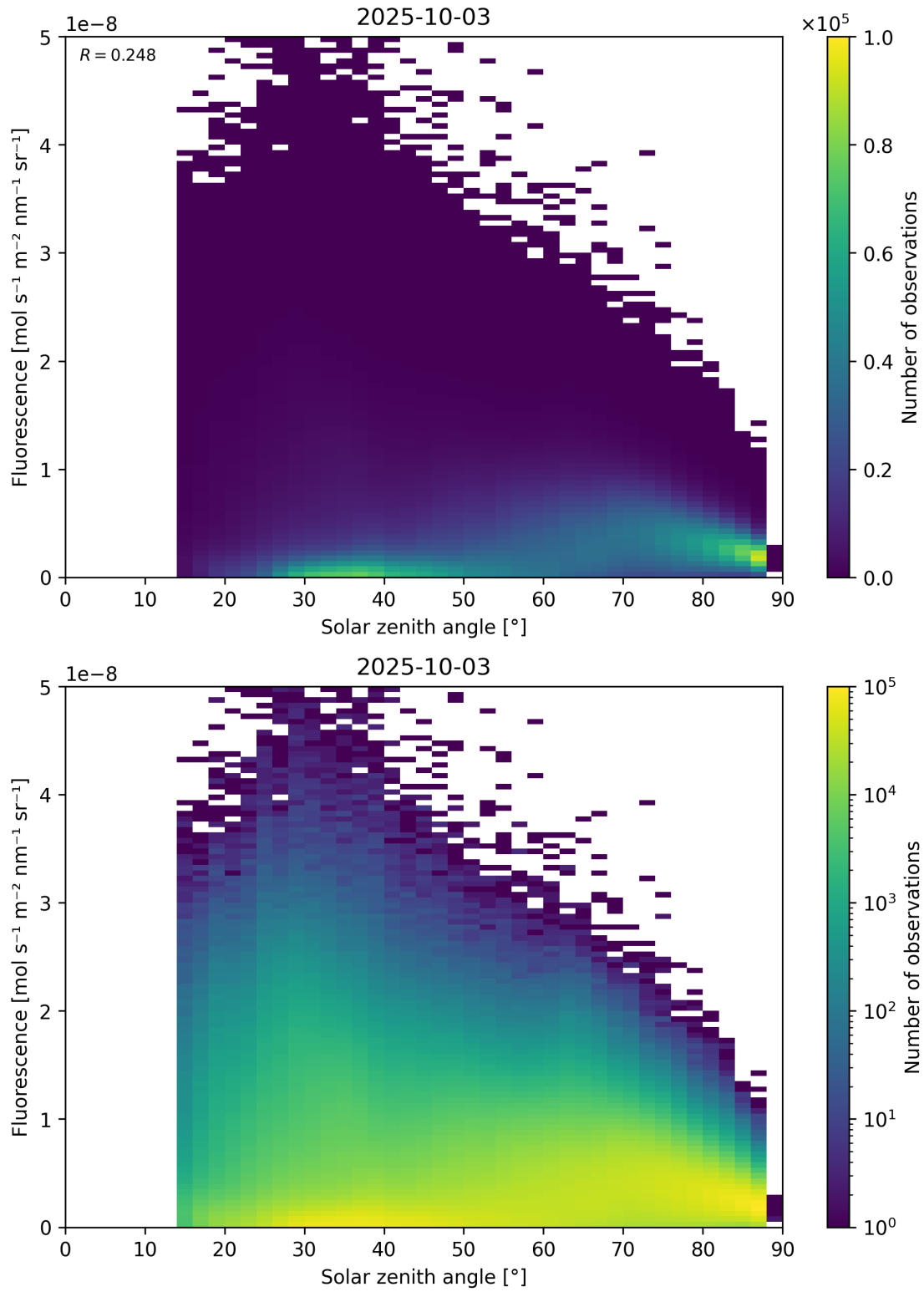
Figure 112: Scatter density plot of “Solar zenith angle” against “Fluorescence” for 2025-10-02 to 2025-10-04.
