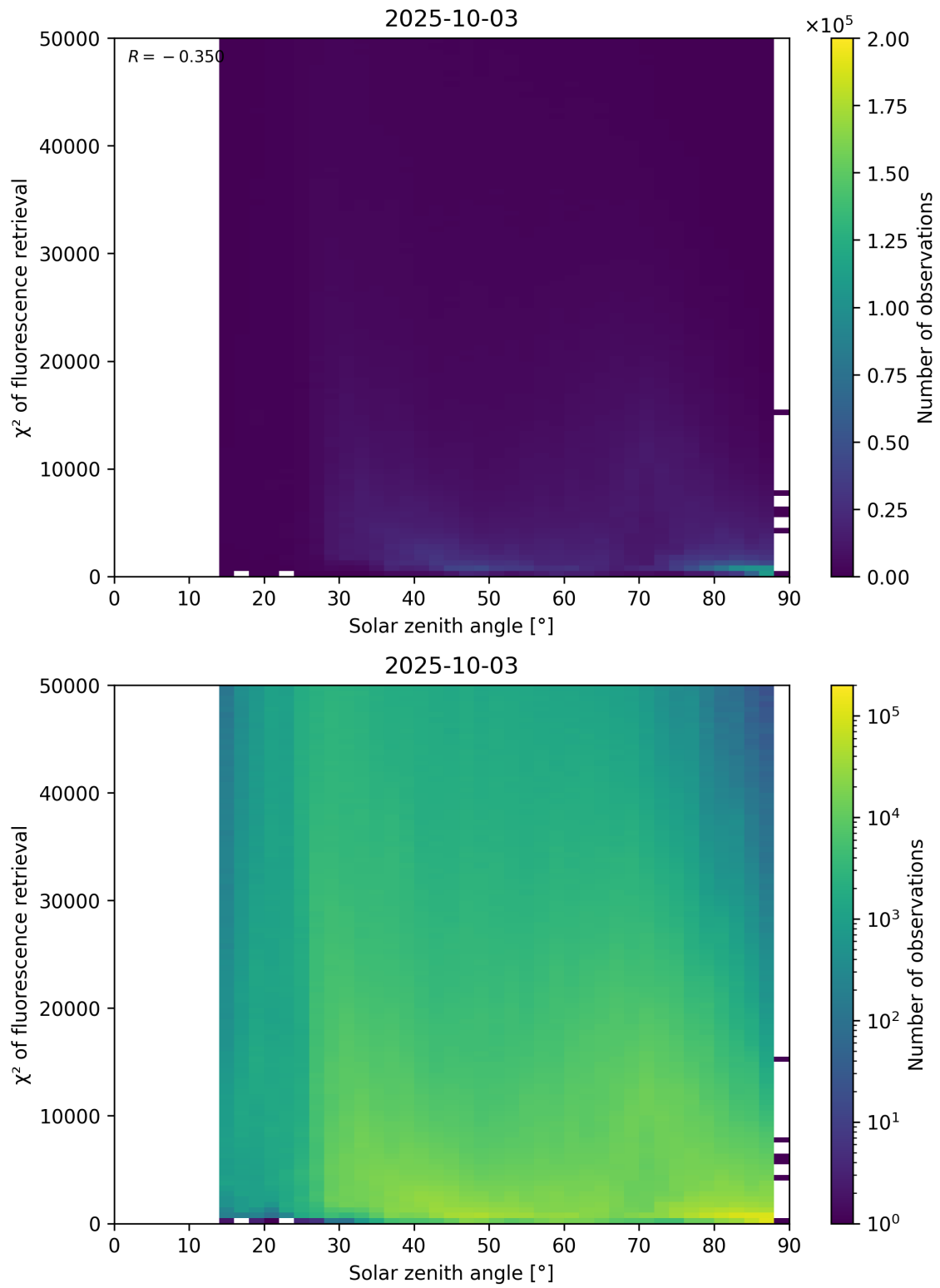
Figure 109: Scatter density plot of “Solar zenith angle” against “ \chi^2 of fluorescence retrieval” for 2025-10-02 to 2025-10-04.
