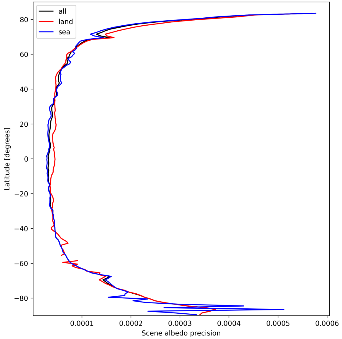
Figure 18: Zonal average of “Scene albedo precision” for 2025-10-02 to 2025-10-04.
