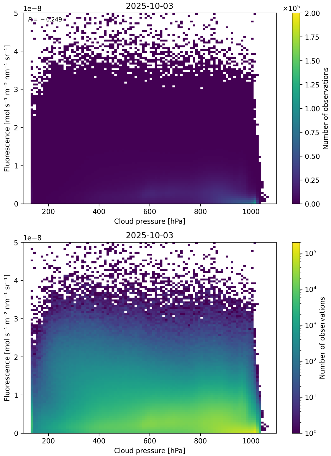
Figure 80: Scatter density plot of “Cloud pressure” against “Fluorescence” for 2025-10-02 to 2025-10-04.
