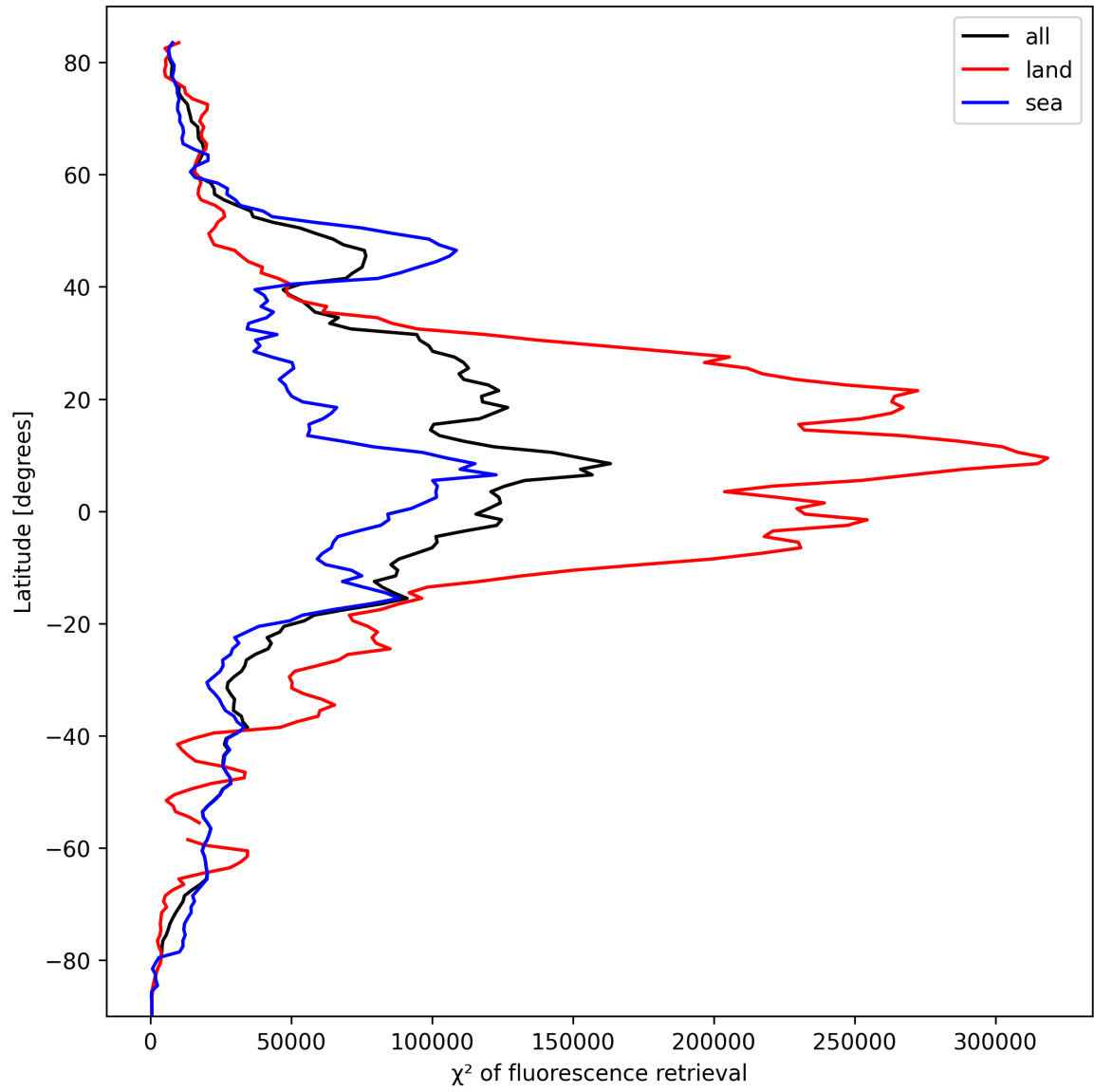
Figure 25: Zonal average of “ \chi^2 of fluorescence retrieval” for 2025-10-02 to 2025-10-04.
