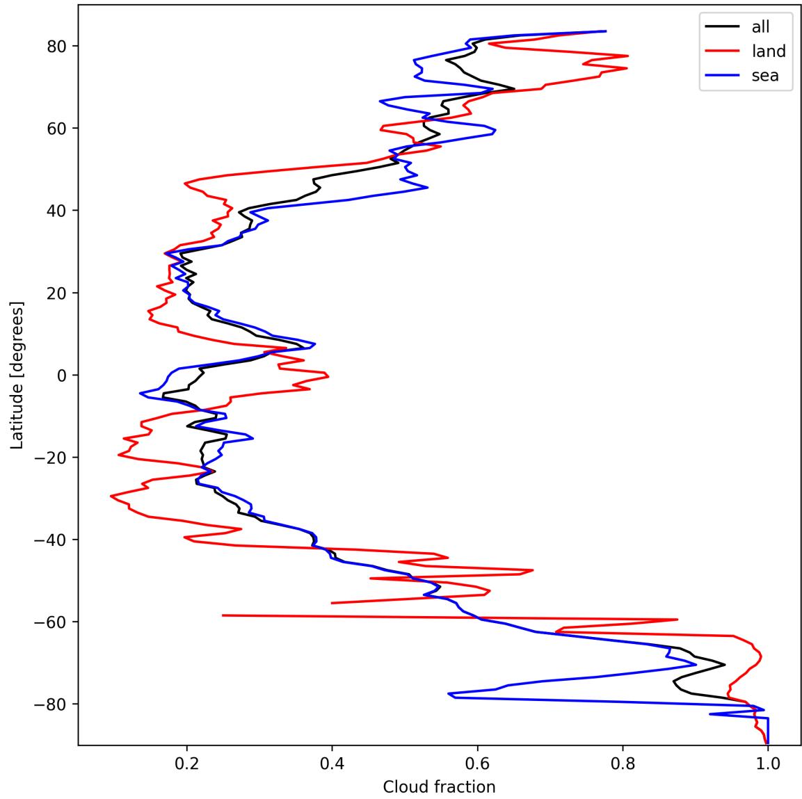
Figure 15: Zonal average of “Cloud fraction” for 2025-10-02 to 2025-10-04.
