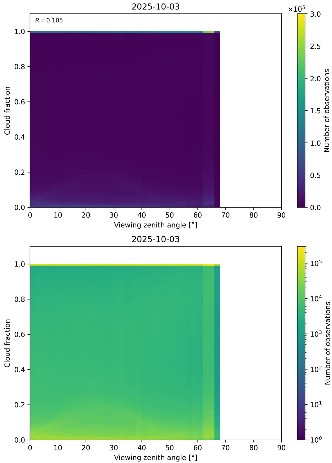
Figure 120: Scatter density plot of “Viewing zenith angle” against “Cloud fraction” for 2025-10-02 to 2025-10-04.
