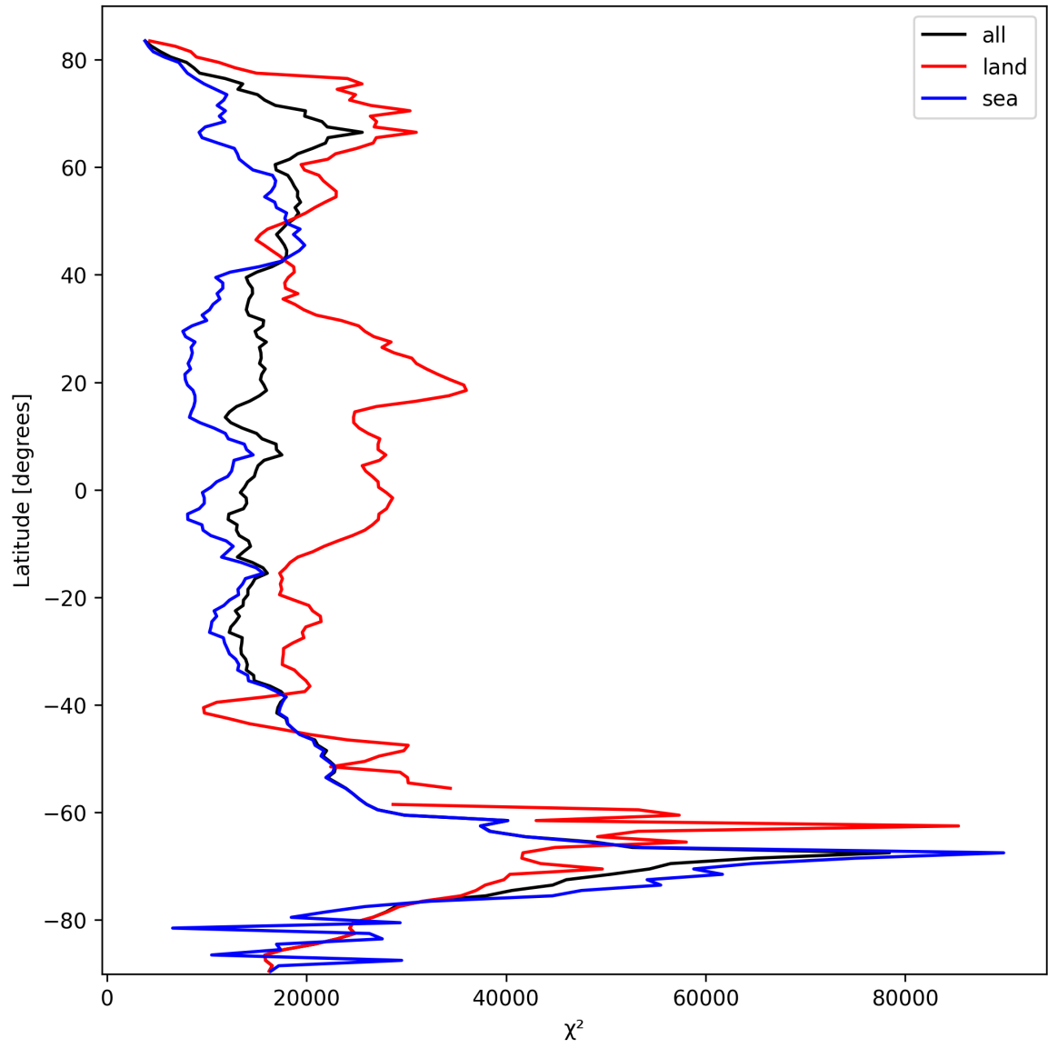
Figure 21: Zonal average of “ \chi^2 ” for 2025-10-02 to 2025-10-04.
