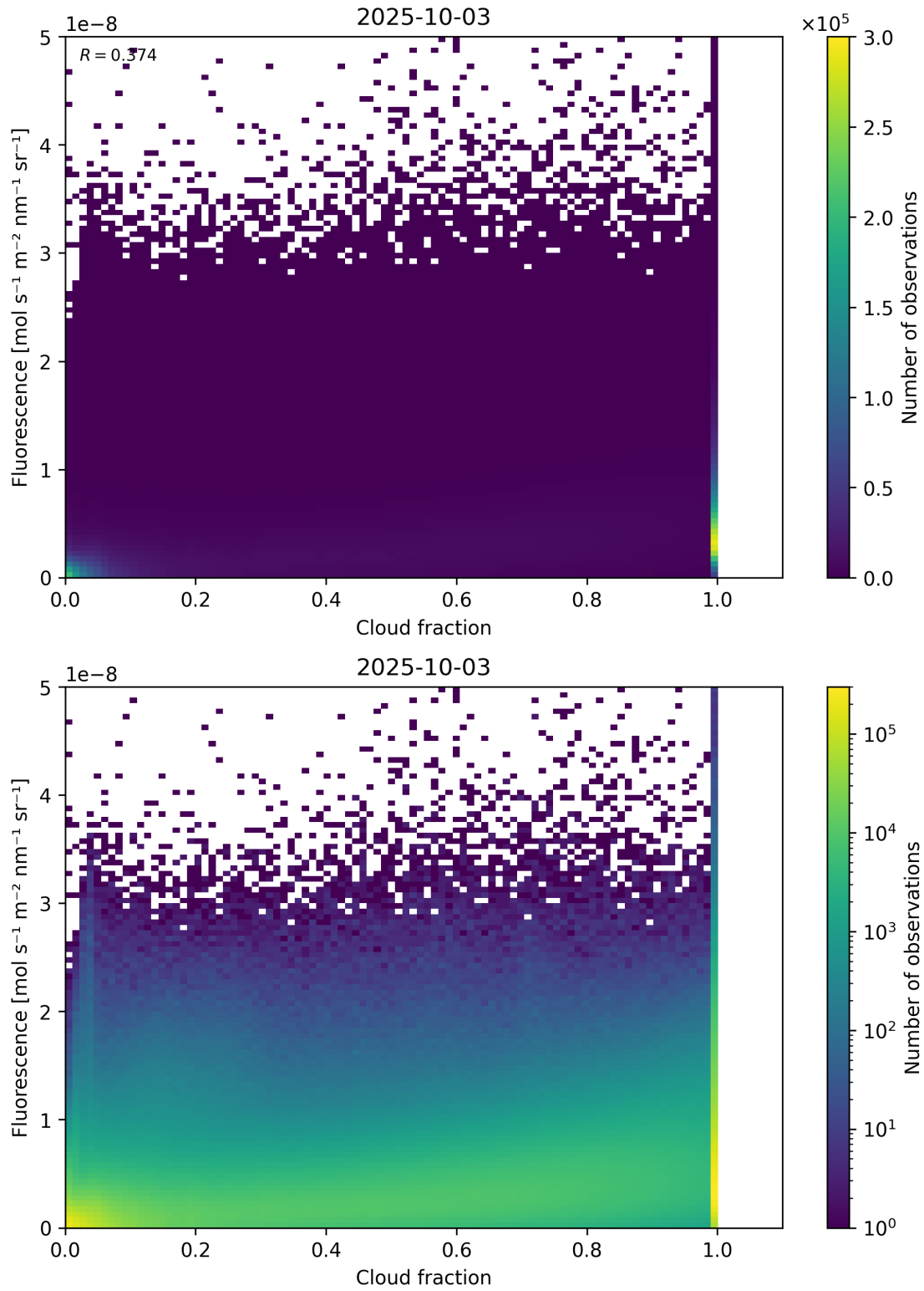
Figure 72: Scatter density plot of “Cloud fraction” against “Fluorescence” for 2025-10-02 to 2025-10-04.
