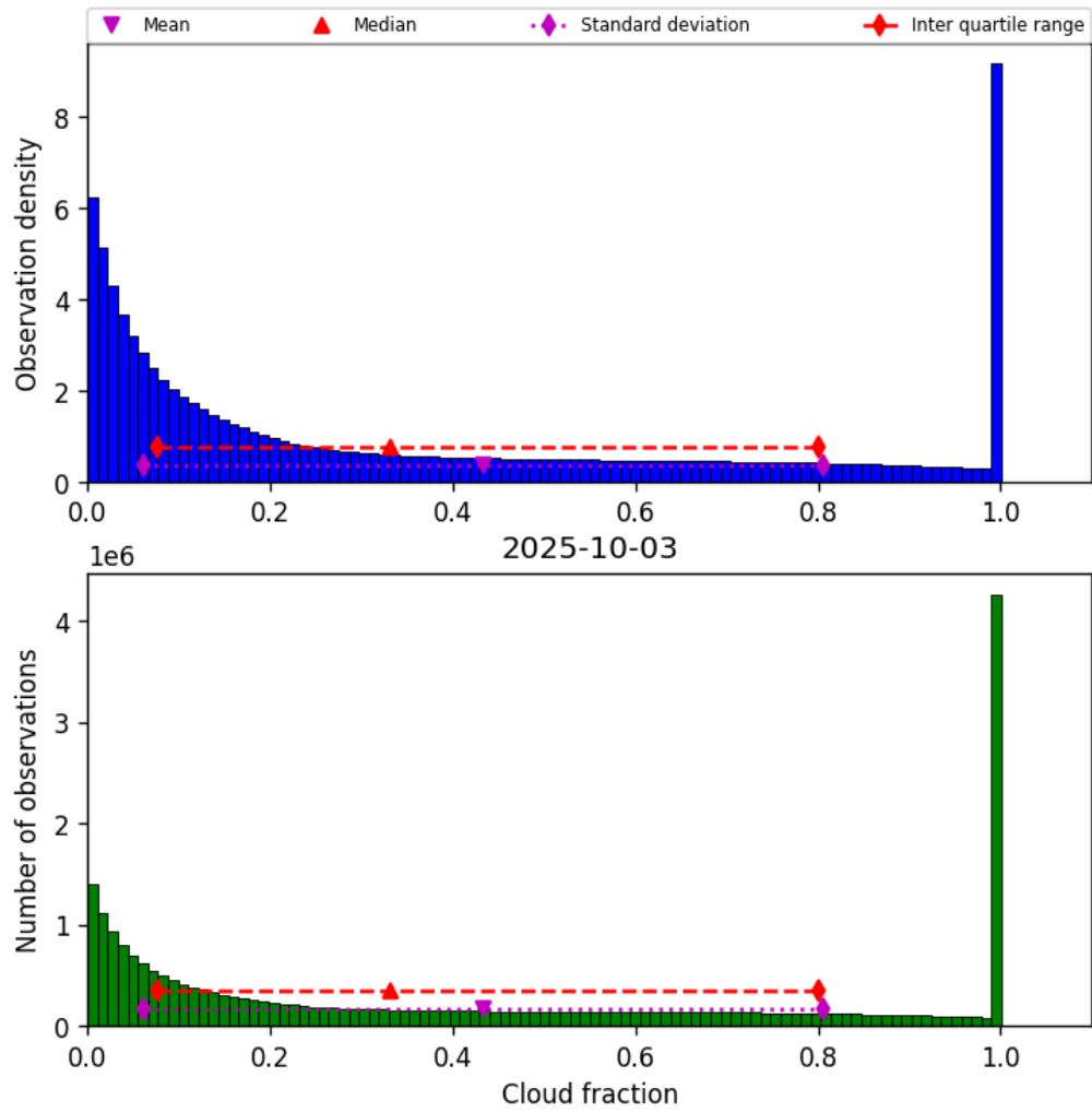
Figure 32: Histogram of “Cloud fraction” for 2025-10-02 to 2025-10-04
