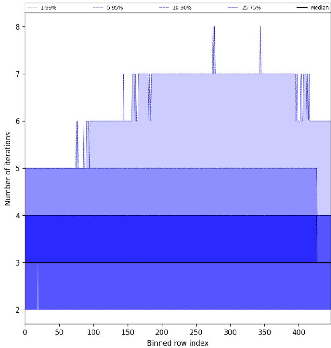
Figure 56: Along track statistics of “Number of iterations” for 2025-10-02 to 2025-10-04
