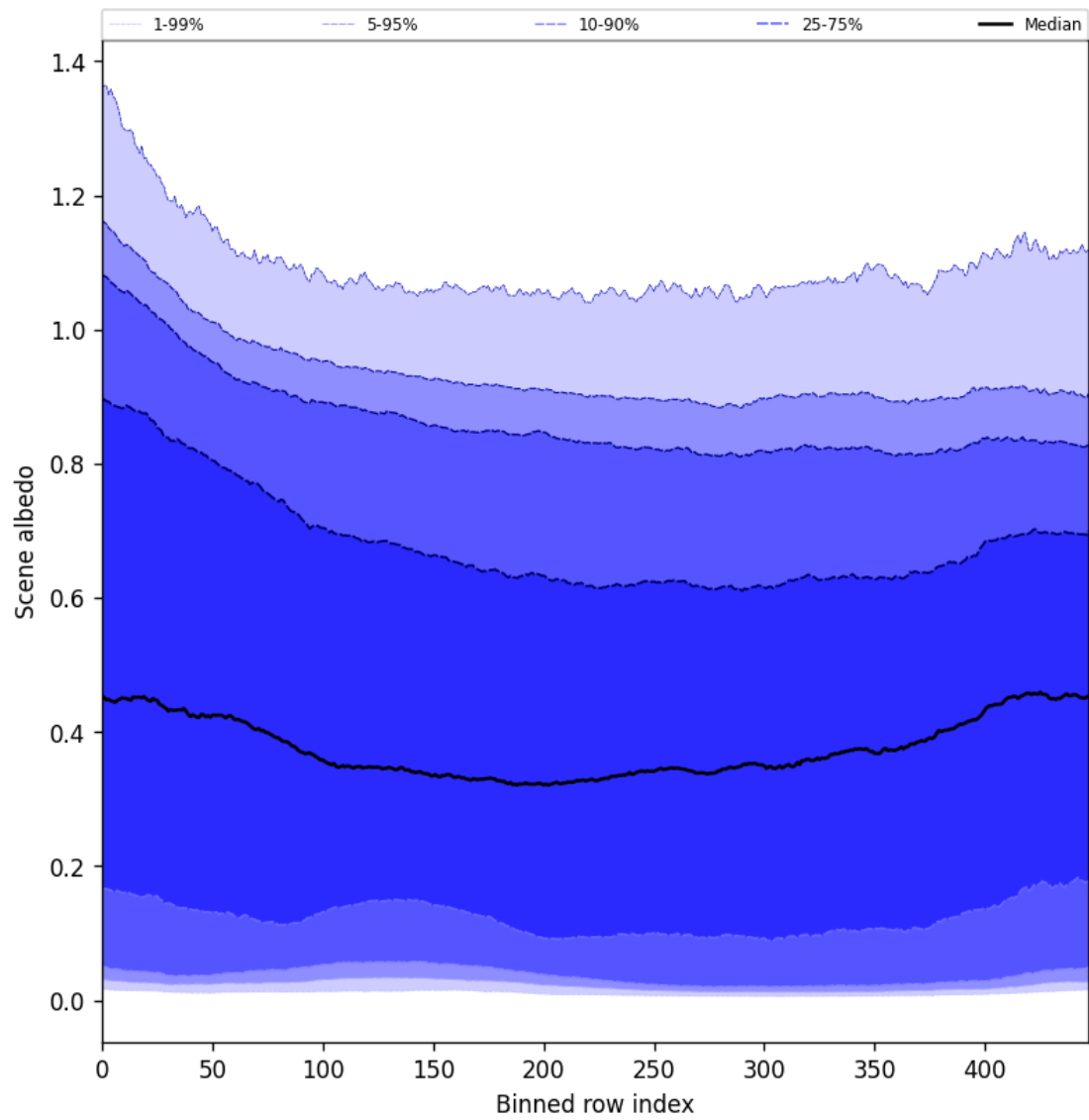
Figure 51: Along track statistics of “Scene albedo” for 2025-10-02 to 2025-10-04
