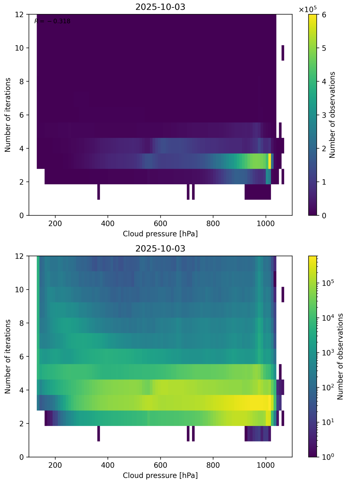
Figure 81: Scatter density plot of “Cloud pressure” against “Number of iterations” for 2025-10-02 to 2025-10-04.
