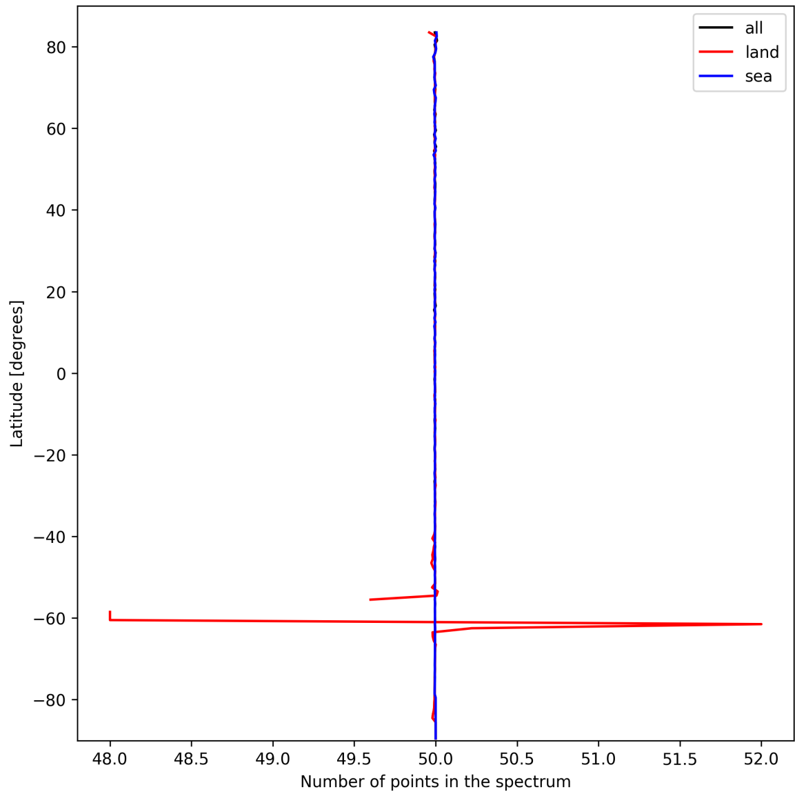
Figure 27: Zonal average of “Number of points in the spectrum” for 2025-10-02 to 2025-10-04.
