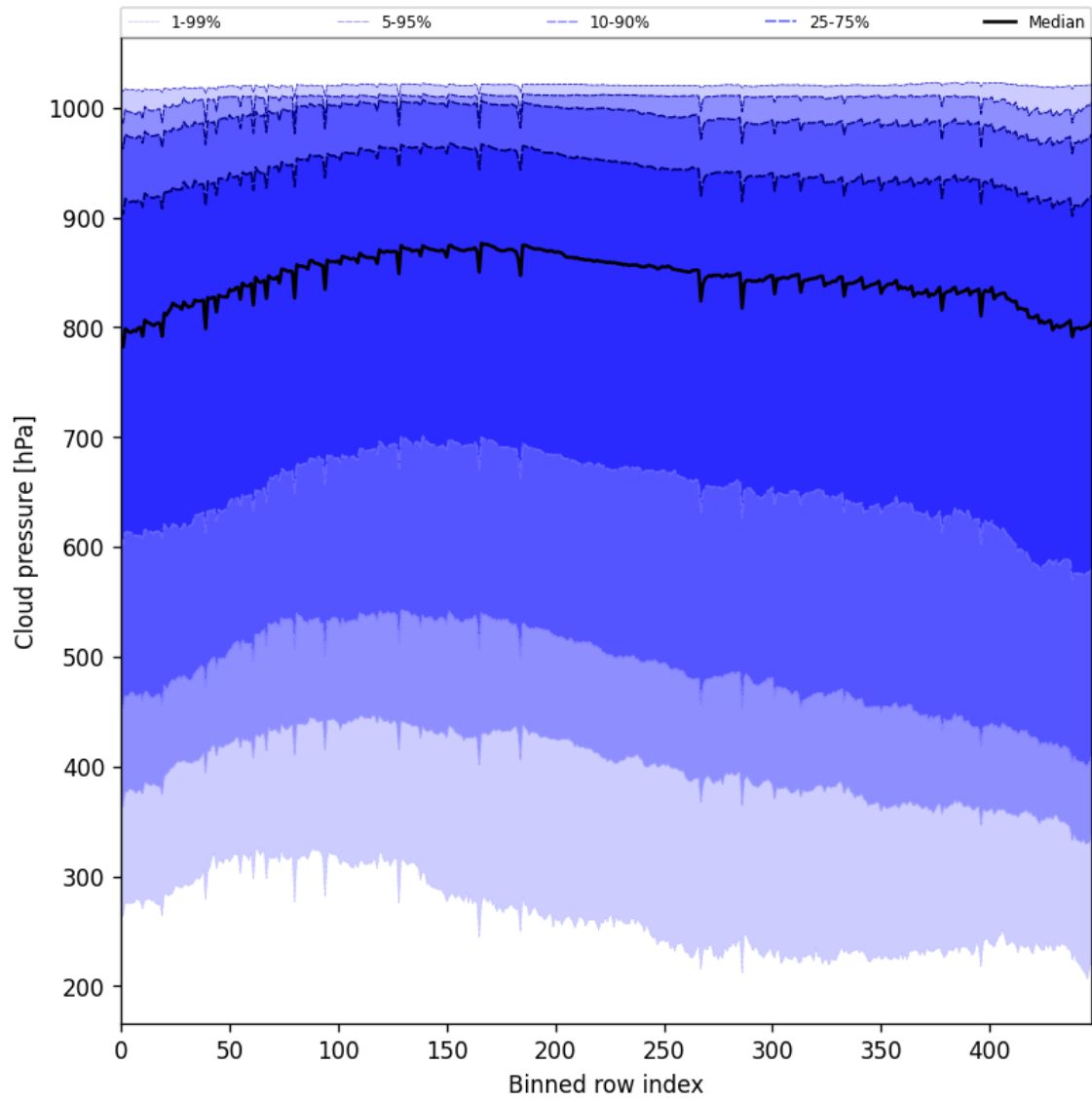
Figure 47: Along track statistics of “Cloud pressure” for 2025-10-02 to 2025-10-04
