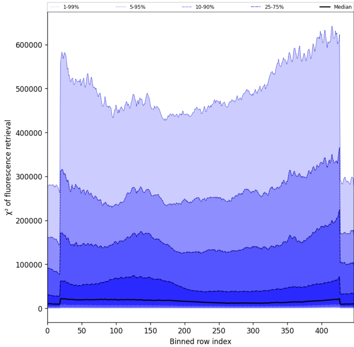
Figure 59: Along track statistics of “ \chi^2 of fluorescence retrieval” for 2025-10-02 to 2025-10-04
