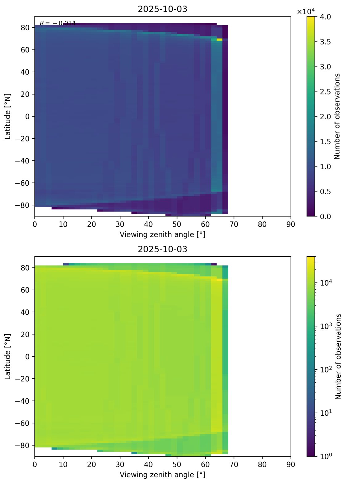
Figure 123: Scatter density plot of “Viewing zenith angle” against “Latitude” for 2025-10-02 to 2025-10-04.
