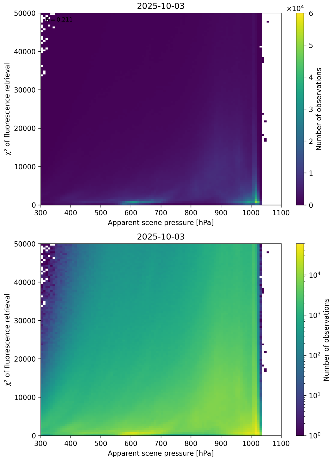
Figure 63: Scatter density plot of “Apparent scene pressure” against “ \chi^2 of fluorescence retrieval” for 2025-10-02 to 2025-10-04.
