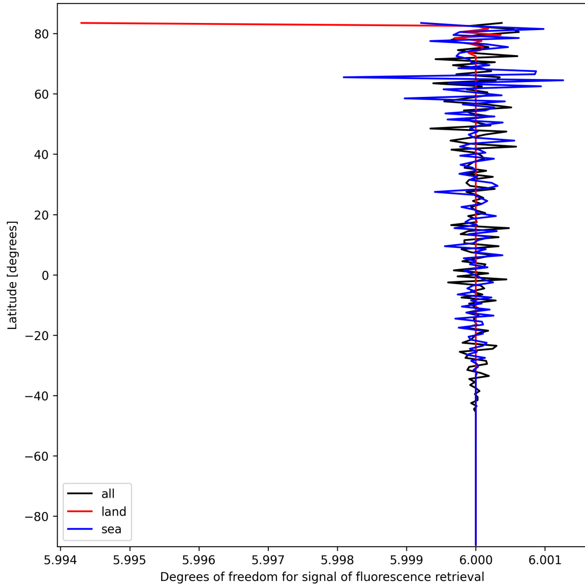
Figure 26: Zonal average of “Degrees of freedom for signal of fluorescence retrieval” for 2025-10-02 to 2025-10-04.
