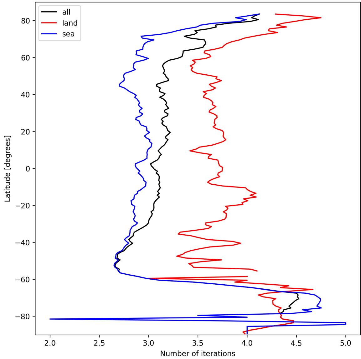
Figure 22: Zonal average of “Number of iterations” for 2025-10-02 to 2025-10-04.
