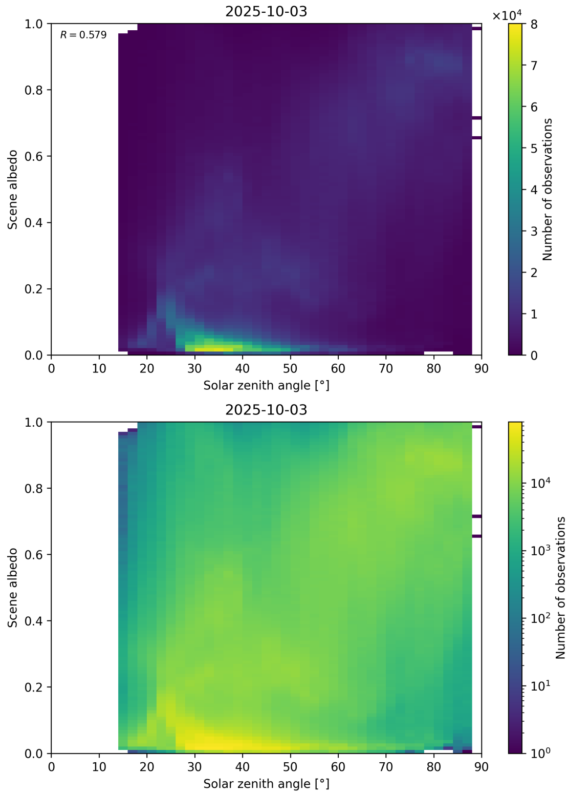
Figure 116: Scatter density plot of “Solar zenith angle” against “Scene albedo” for 2025-10-02 to 2025-10-04.
