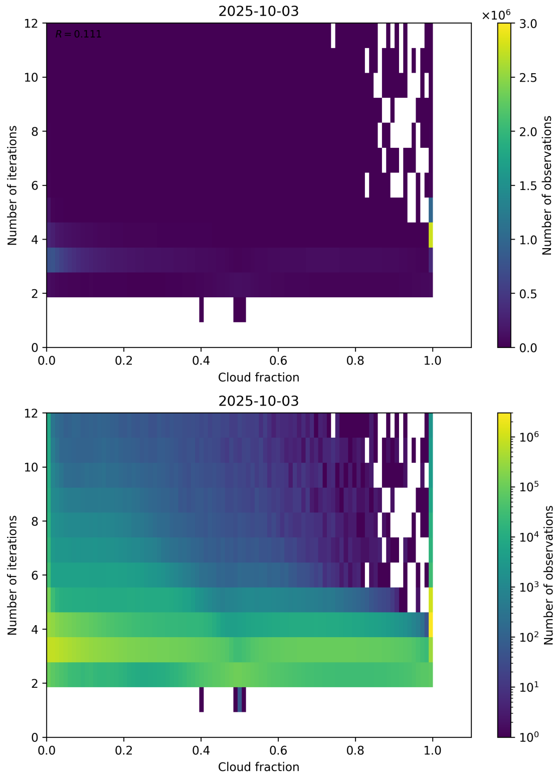
Figure 73: Scatter density plot of “Cloud fraction” against “Number of iterations” for 2025-10-02 to 2025-10-04.
