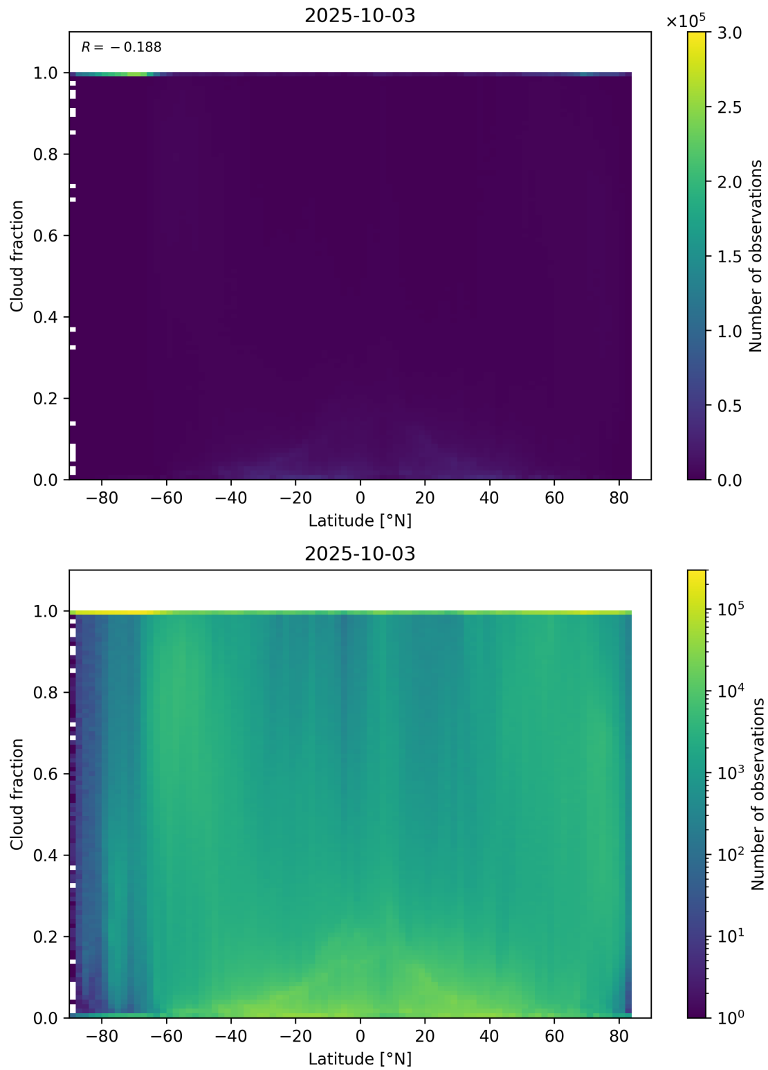
Figure 90: Scatter density plot of “Latitude” against “Cloud fraction” for 2025-10-02 to 2025-10-04.
