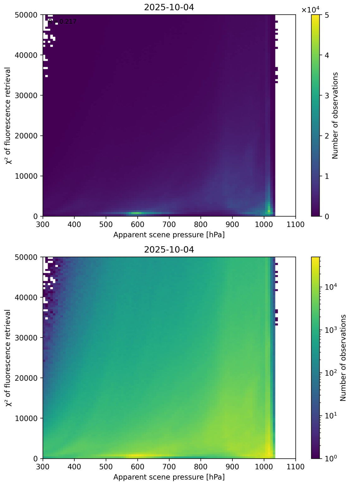
Figure 63: Scatter density plot of “Apparent scene pressure” against “ \chi^2 of fluorescence retrieval” for 2025-10-03 to 2025-10-05.
