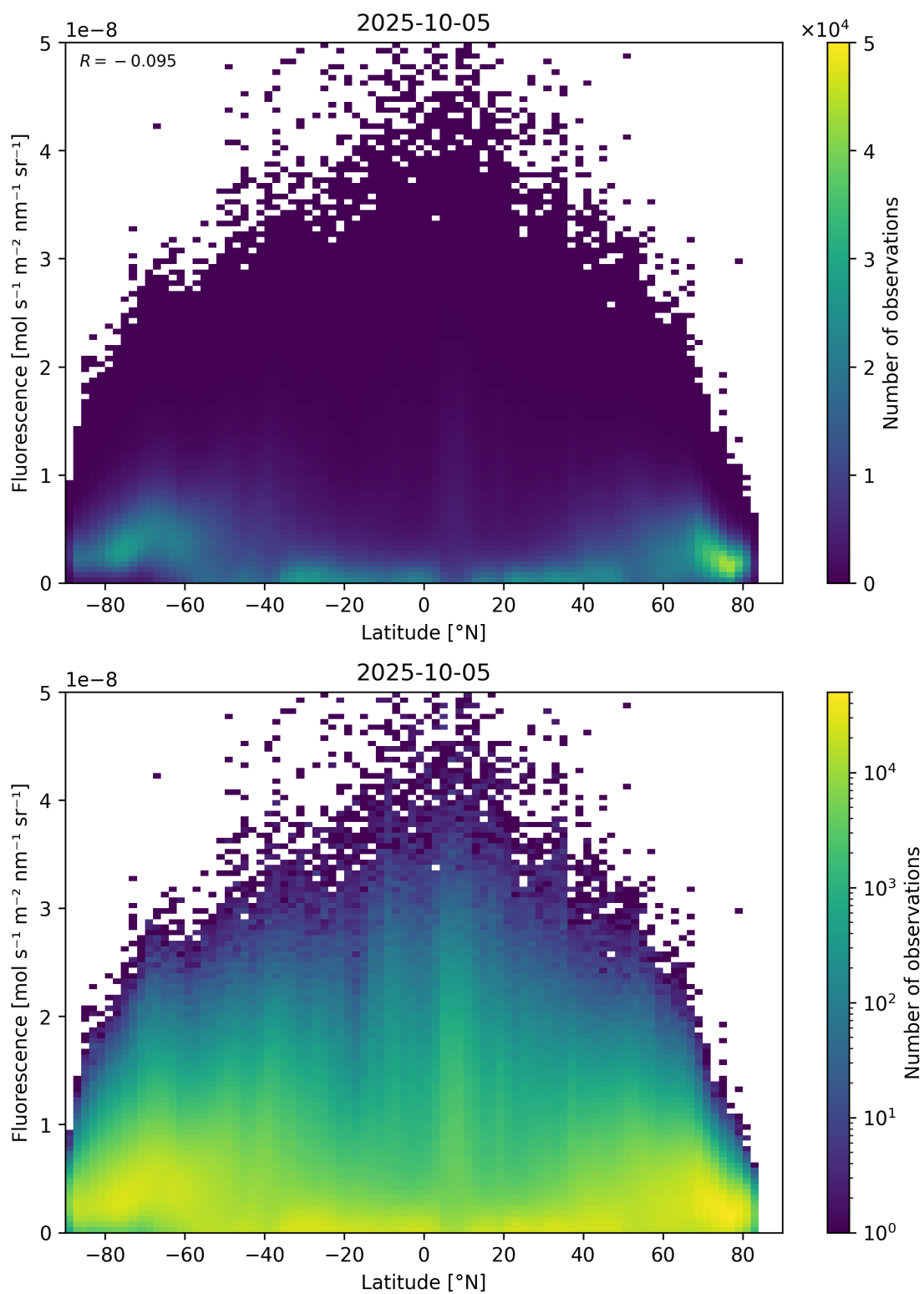
Figure 92: Scatter density plot of “Latitude” against “Fluorescence” for 2025-10-04 to 2025-10-06.
