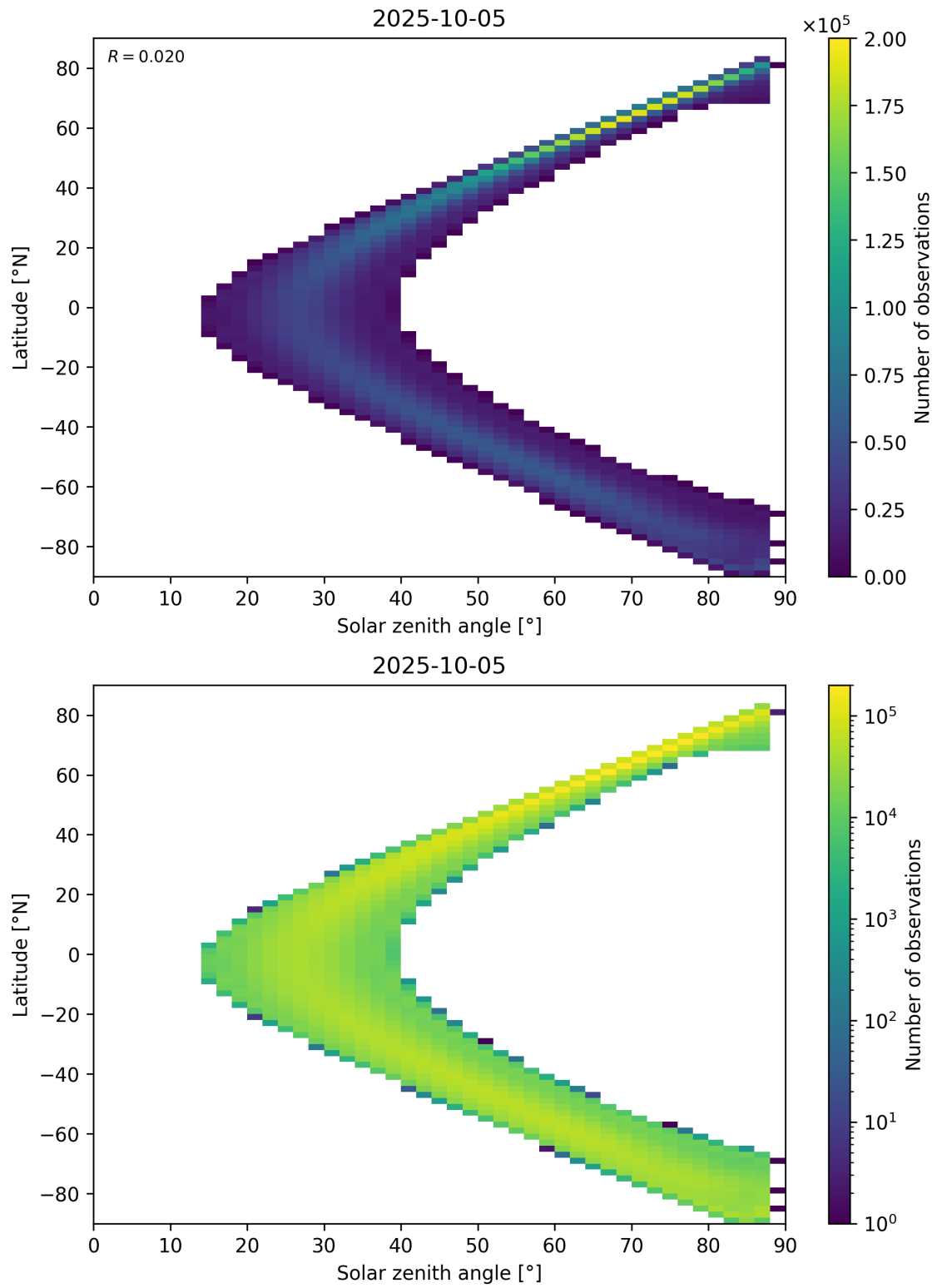
Figure 113: Scatter density plot of “Solar zenith angle” against “Latitude” for 2025-10-04 to 2025-10-06.
