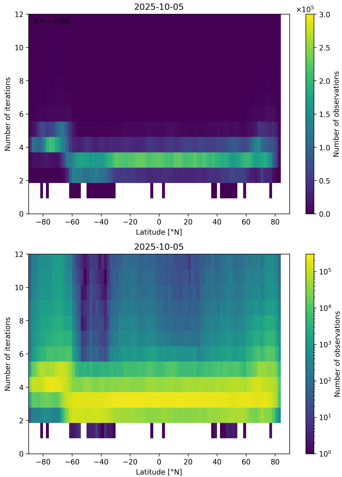
Figure 93: Scatter density plot of “Latitude” against “Number of iterations” for 2025-10-04 to 2025-10-06.
