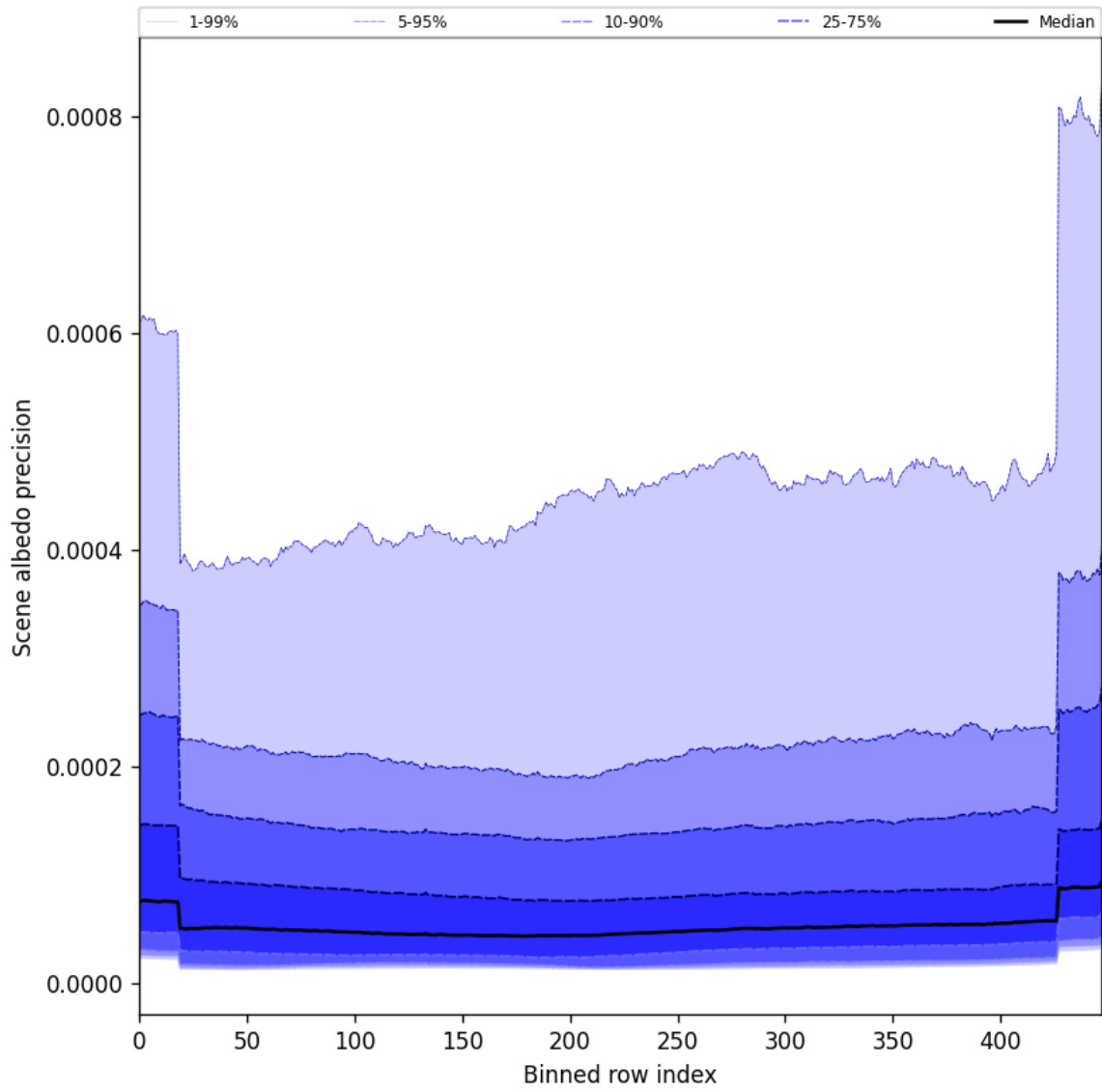
Figure 52: Along track statistics of “Scene albedo precision” for 2025-10-04 to 2025-10-06
