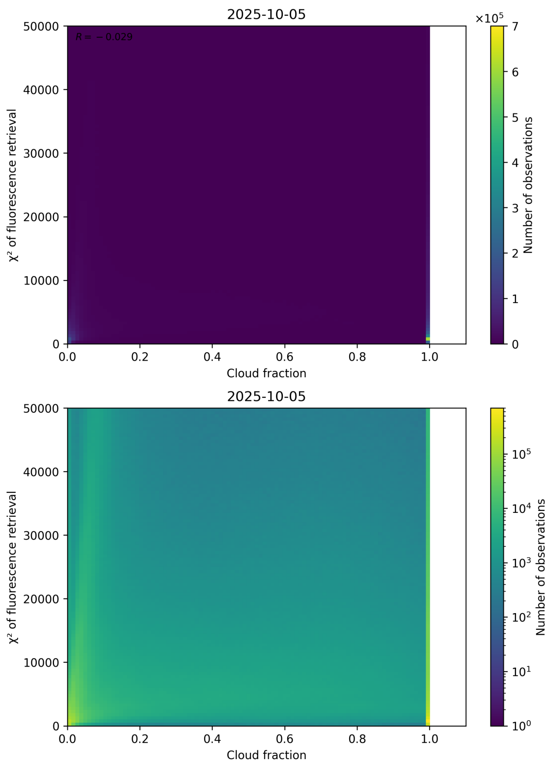
Figure 71: Scatter density plot of “Cloud fraction” against “ \chi^2 of fluorescence retrieval” for 2025-10-04 to 2025-10-06.
