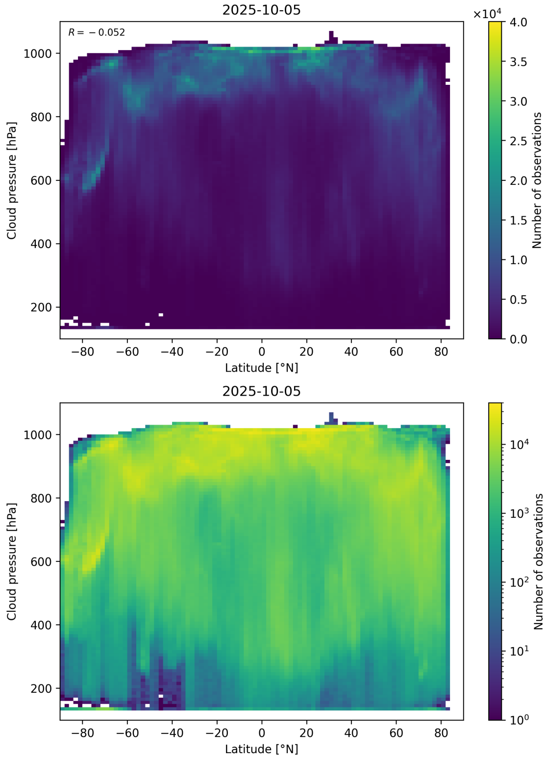
Figure 91: Scatter density plot of “Latitude” against “Cloud pressure” for 2025-10-04 to 2025-10-06.
