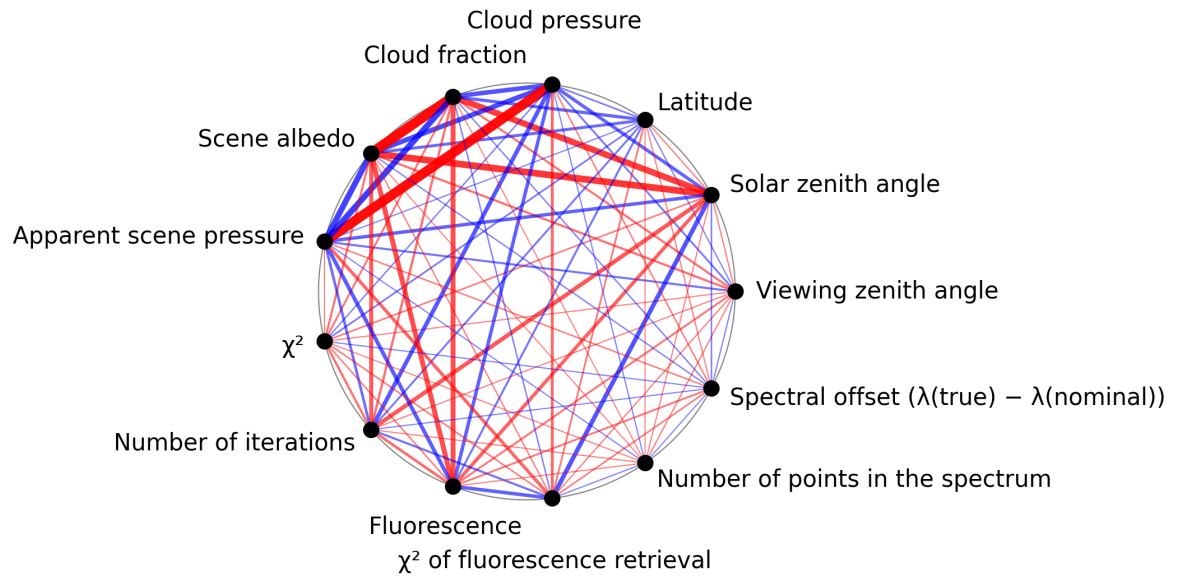
Figure 1: Map of correlation graph for 2025-10-04 to 2025-10-06.
