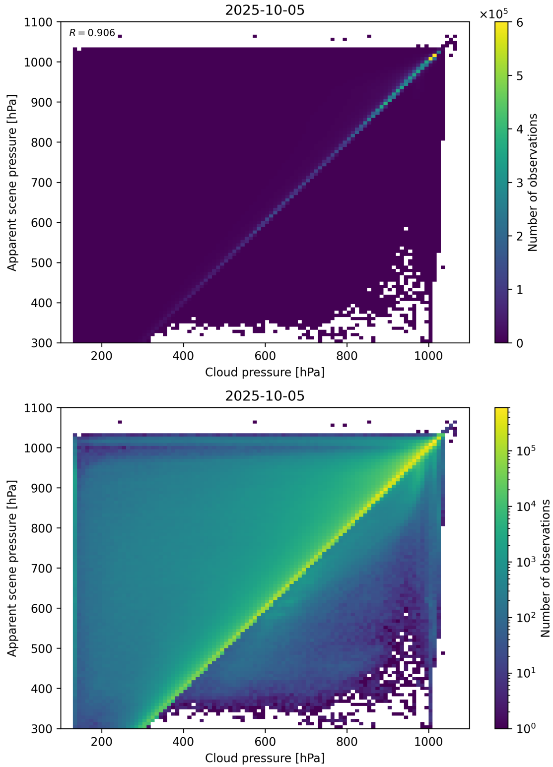
Figure 77: Scatter density plot of “Cloud pressure” against “Apparent scene pressure” for 2025-10-04 to 2025-10-06.
