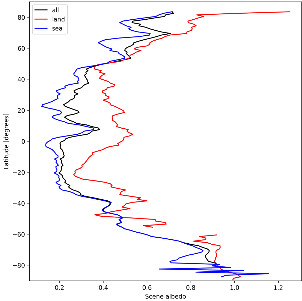
Figure 17: Zonal average of “Scene albedo” for 2025-10-04 to 2025-10-06.
