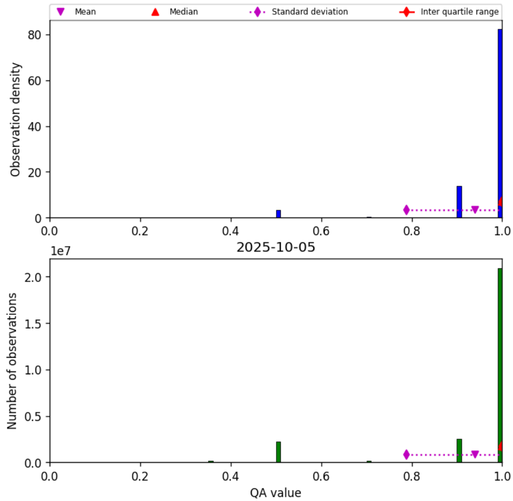
Figure 29: Histogram of “QA value” for 2025-10-04 to 2025-10-06
