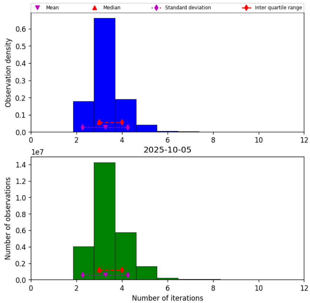
Figure 39: Histogram of “Number of iterations” for 2025-10-04 to 2025-10-06
