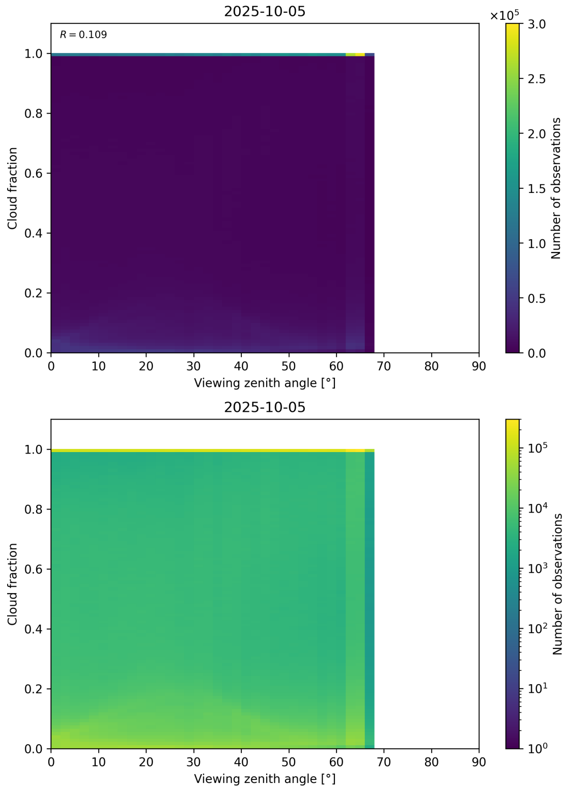
Figure 120: Scatter density plot of “Viewing zenith angle” against “Cloud fraction” for 2025-10-04 to 2025-10-06.
