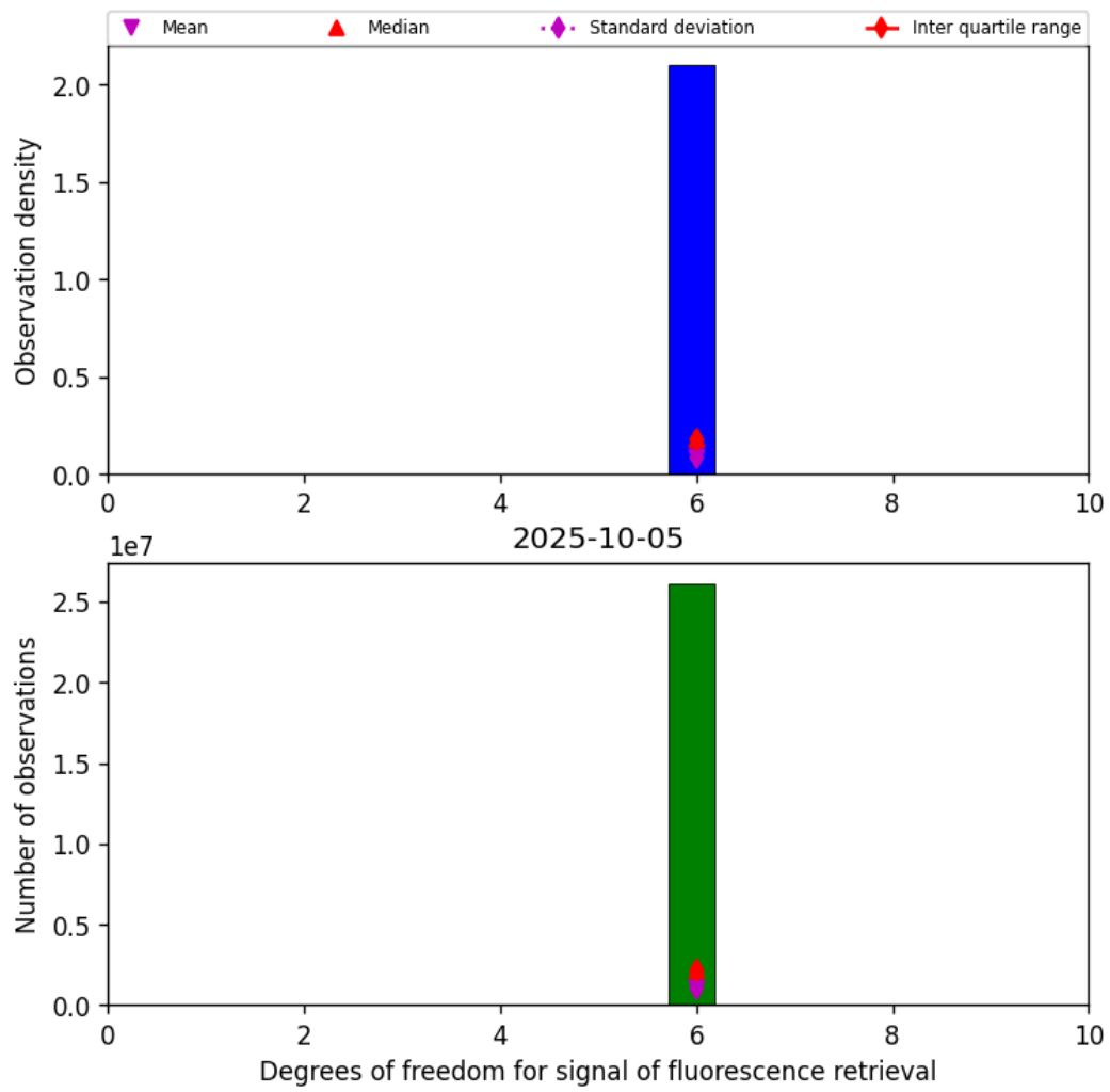
Figure 43: Histogram of "Degrees of freedom for signal of fluorescence retrieval" for 2025-10-04 to 2025-10-06
