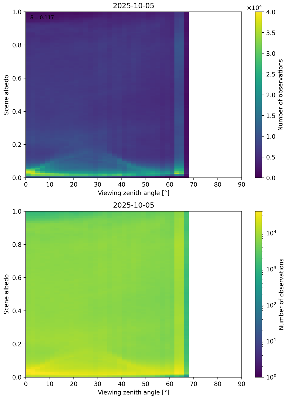
Figure 126: Scatter density plot of “Viewing zenith angle” against “Scene albedo” for 2025-10-04 to 2025-10-06.
