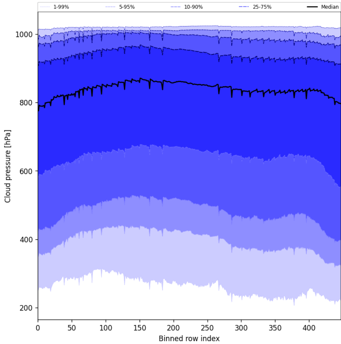
Figure 47: Along track statistics of “Cloud pressure” for 2025-10-04 to 2025-10-06
