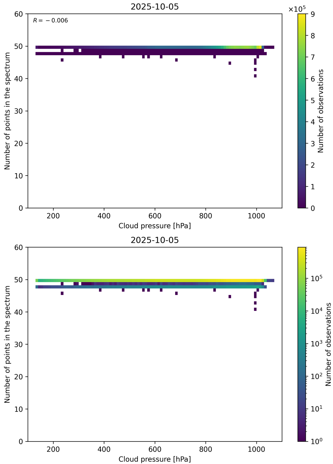
Figure 82: Scatter density plot of “Cloud pressure” against “Number of points in the spectrum” for 2025-10-04 to 2025-10-06.
