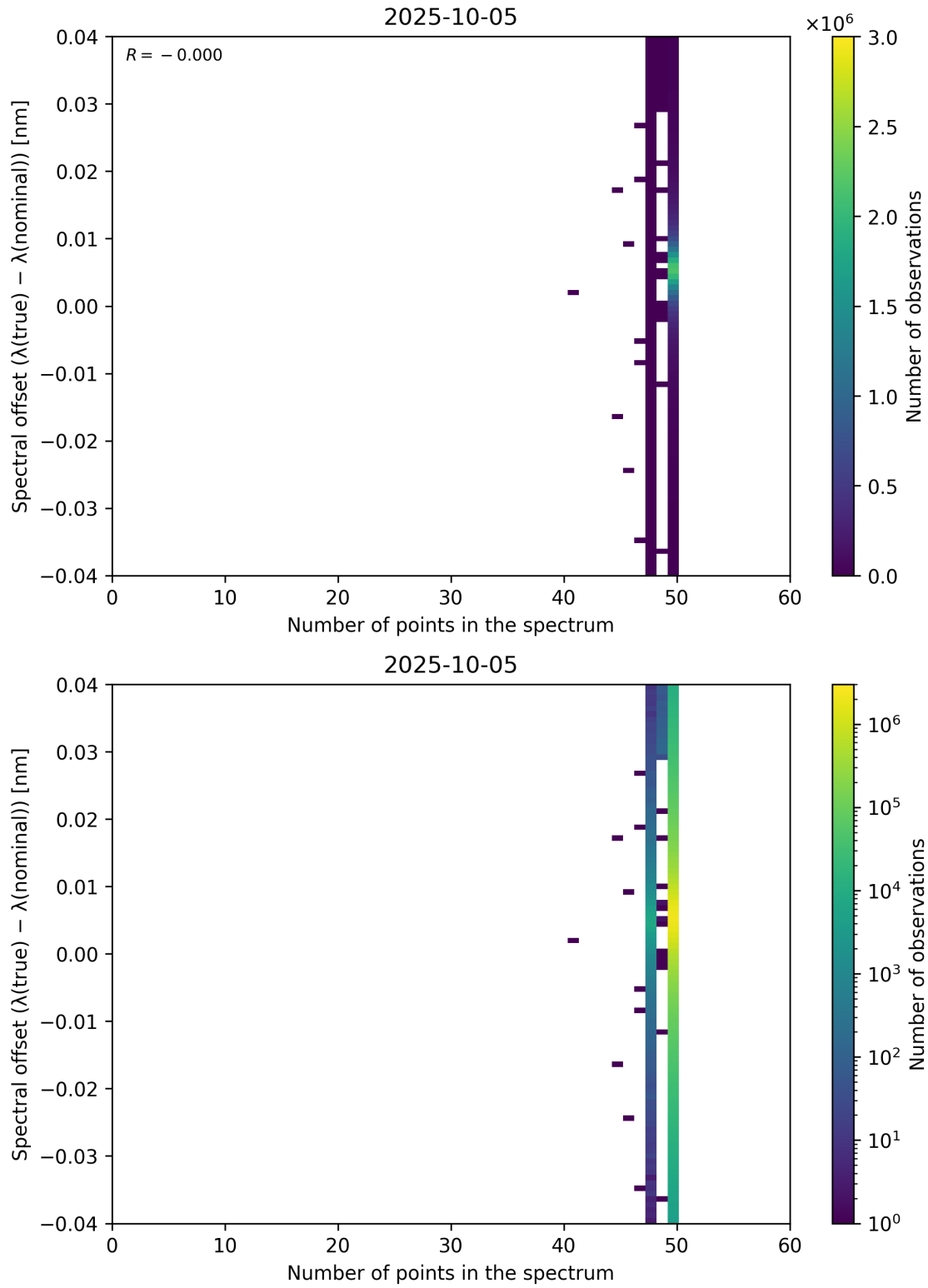
Figure 101: Scatter density plot of “Number of points in the spectrum” against “Spectral offset ( \lambda_{\text{true}} - \lambda_{\text{nominal}} )” for 2025-10-04 to 2025-10-06.
