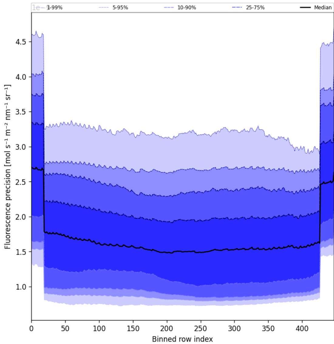
Figure 58: Along track statistics of “Fluorescence precision” for 2025-10-04 to 2025-10-06
