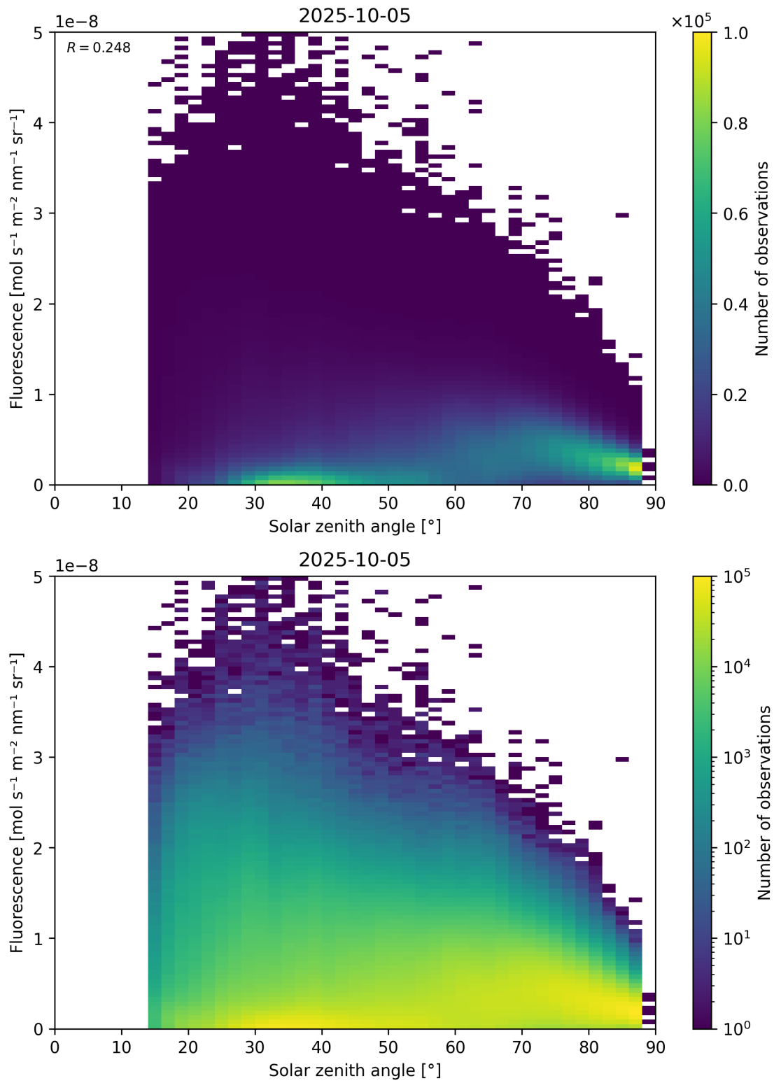
Figure 112: Scatter density plot of “Solar zenith angle” against “Fluorescence” for 2025-10-04 to 2025-10-06.
