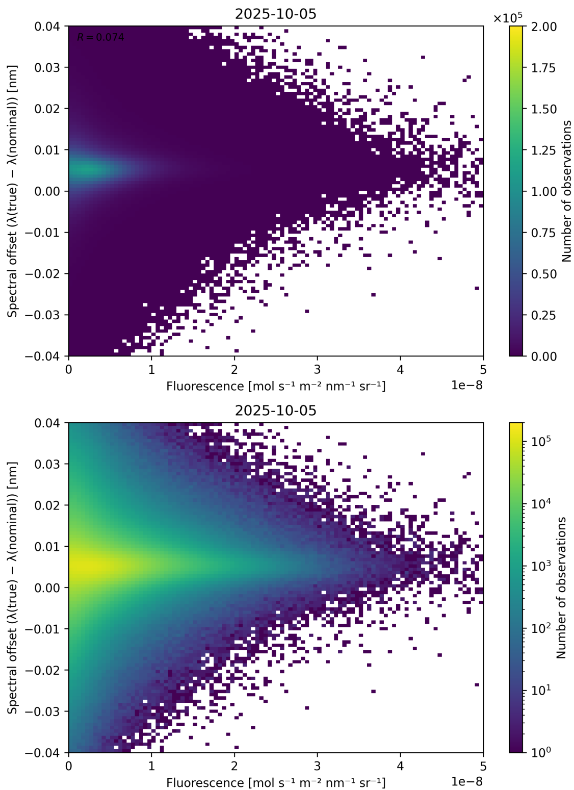
Figure 87: Scatter density plot of “Fluorescence” against “Spectral offset ( \lambda_{\text{true}} - \lambda_{\text{nominal}} )” for 2025-10-04 to 2025-10-06.
