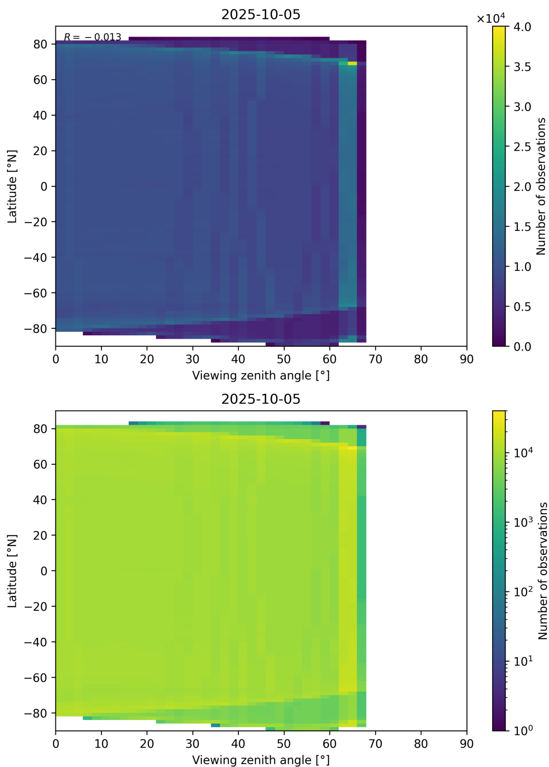
Figure 123: Scatter density plot of “Viewing zenith angle” against “Latitude” for 2025-10-04 to 2025-10-06.
