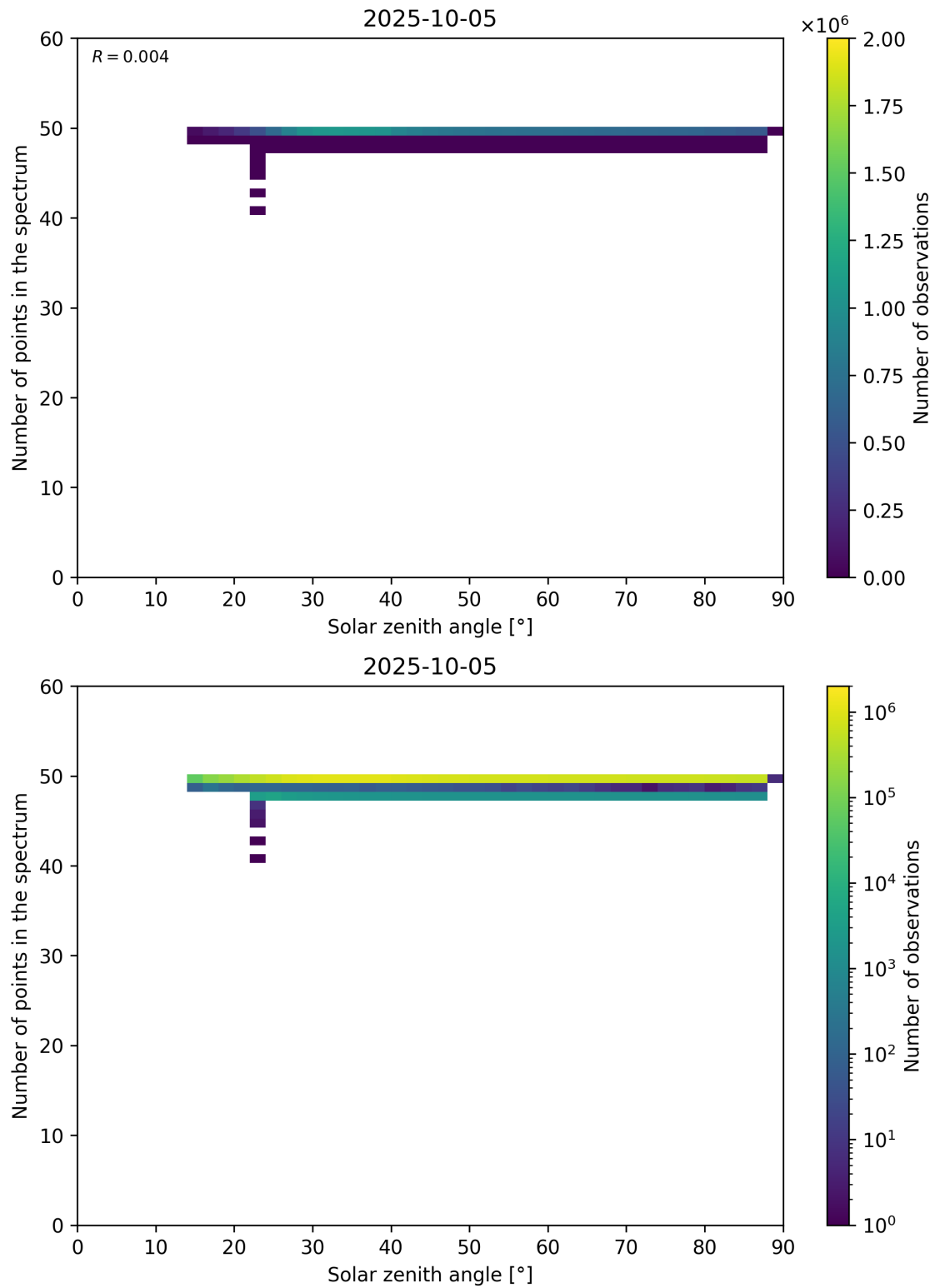
Figure 115: Scatter density plot of “Solar zenith angle” against “Number of points in the spectrum” for 2025-10-04 to 2025-10-06.
