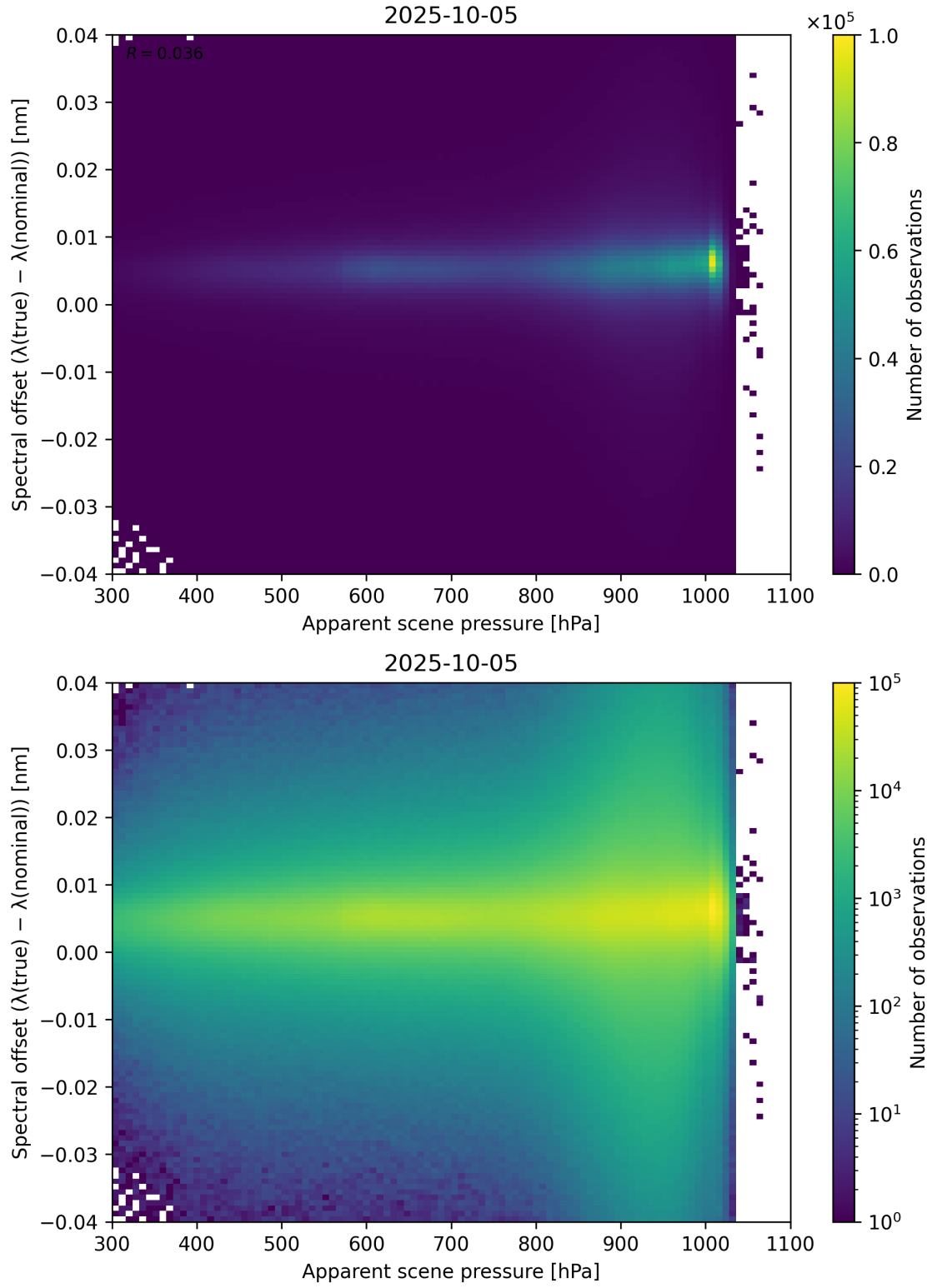
Figure 67: Scatter density plot of “Apparent scene pressure” against “Spectral offset ( \lambda_{\text{true}} - \lambda_{\text{nominal}} )” for 2025-10-04 to 2025-10-06.
