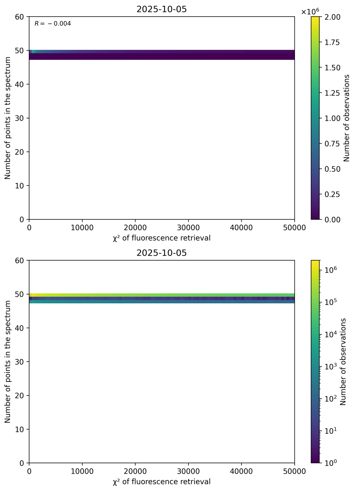
Figure 68: Scatter density plot of " \chi^2 of fluorescence retrieval" against "Number of points in the spectrum" for 2025-10-04 to 2025-10-06.
