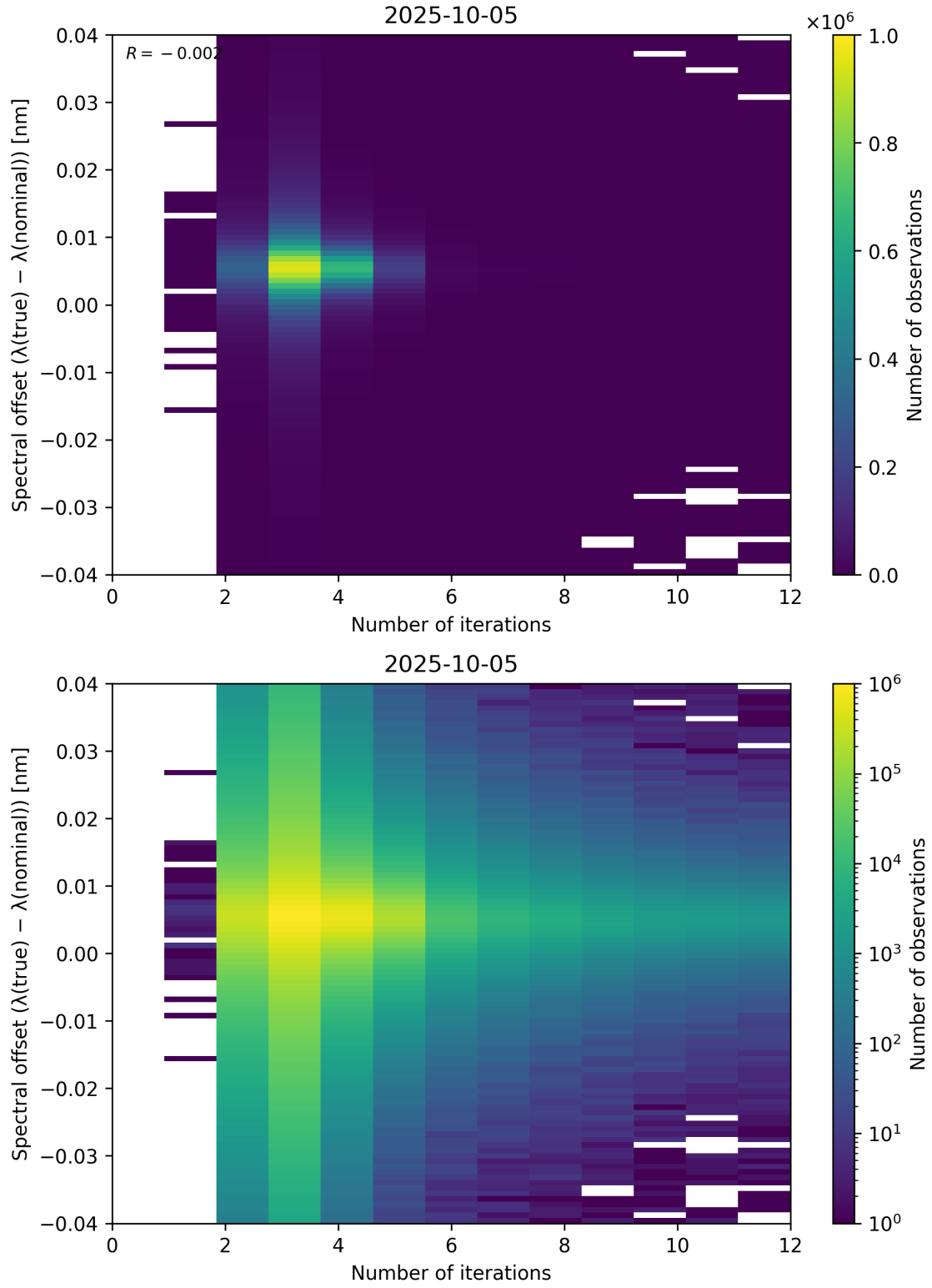
Figure 100: Scatter density plot of “Number of iterations” against “Spectral offset ( \lambda_{\text{true}} - \lambda_{\text{nominal}} )” for 2025-10-04 to 2025-10-06.
