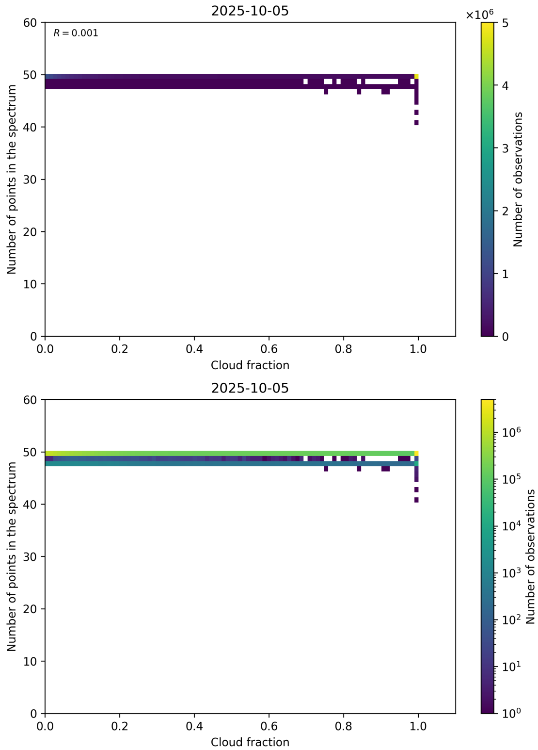
Figure 74: Scatter density plot of “Cloud fraction” against “Number of points in the spectrum” for 2025-10-04 to 2025-10-06.
