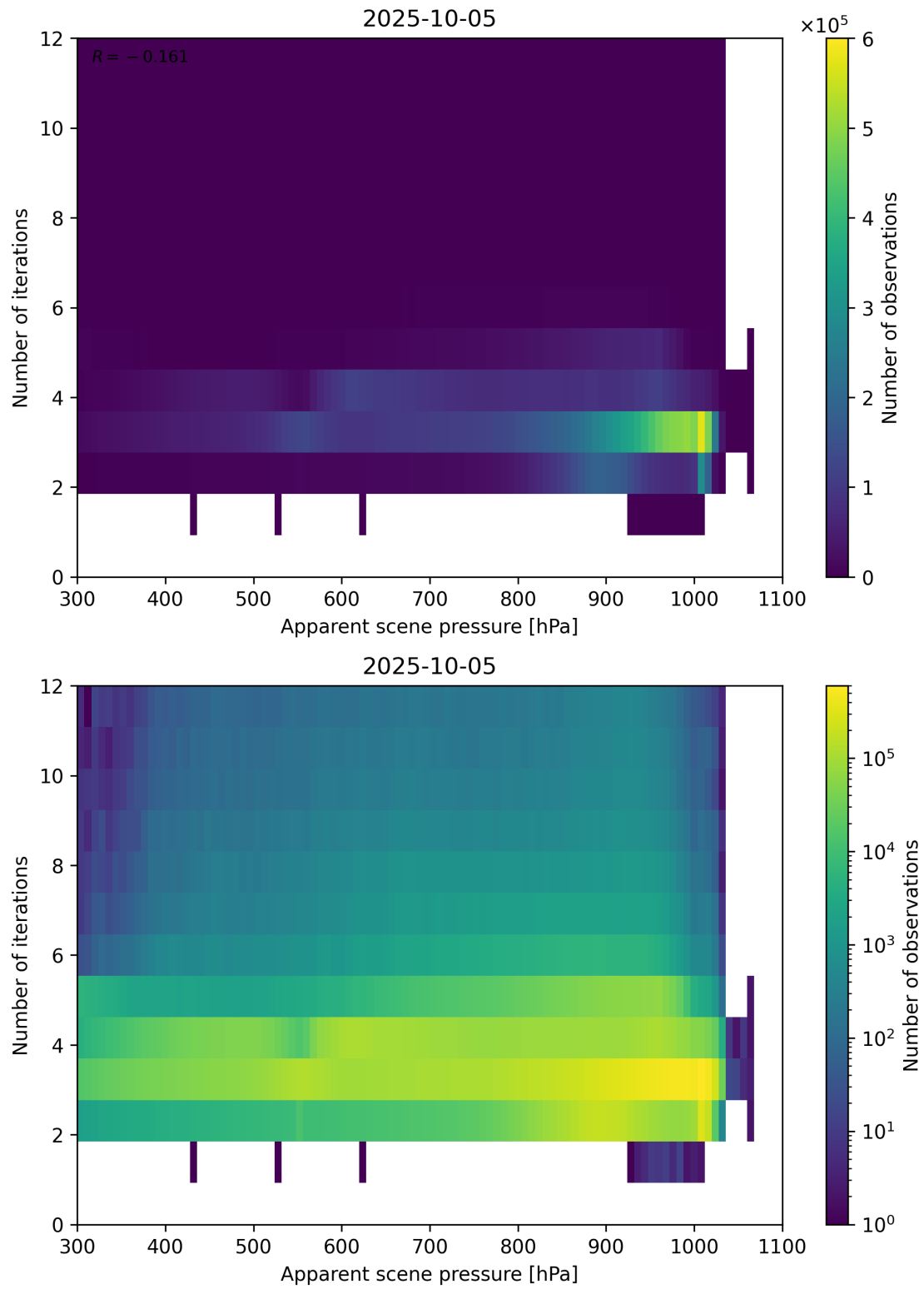
Figure 65: Scatter density plot of “Apparent scene pressure” against “Number of iterations” for 2025-10-04 to 2025-10-06.
