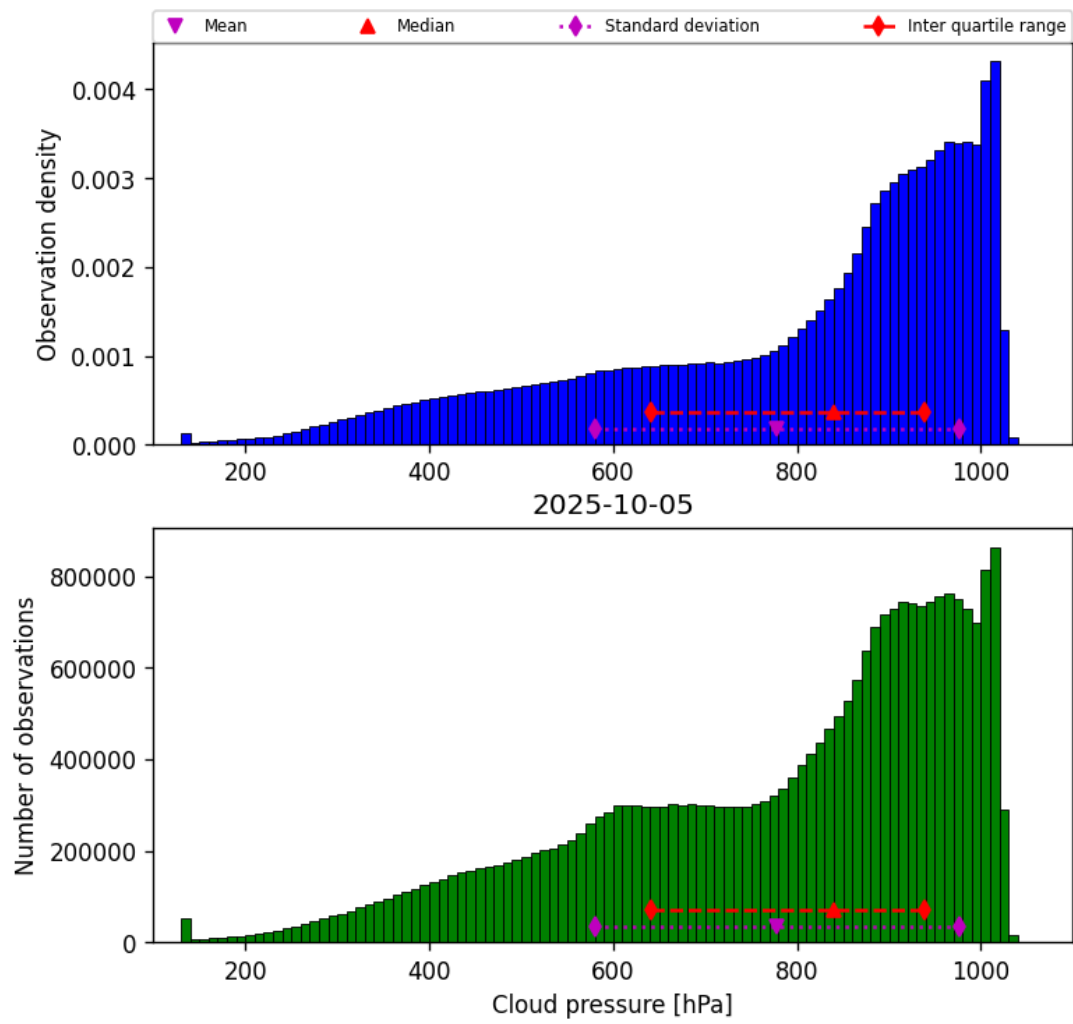
Figure 30: Histogram of “Cloud pressure” for 2025-10-04 to 2025-10-06
