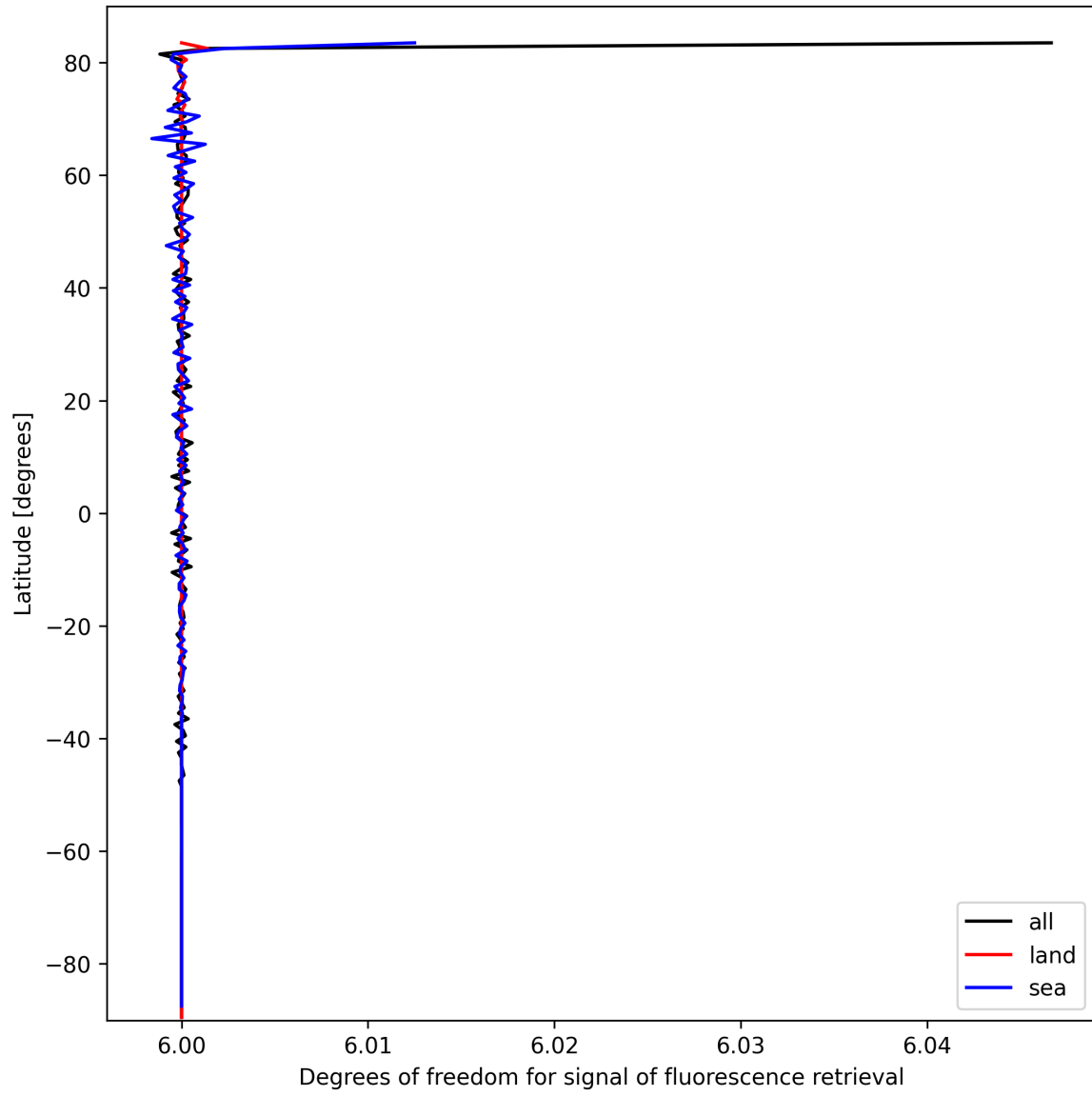
Figure 26: Zonal average of “Degrees of freedom for signal of fluorescence retrieval” for 2025-10-04 to 2025-10-06.
