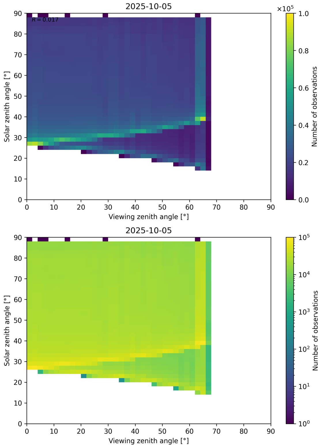
Figure 127: Scatter density plot of “Viewing zenith angle” against “Solar zenith angle” for 2025-10-04 to 2025-10-06.
