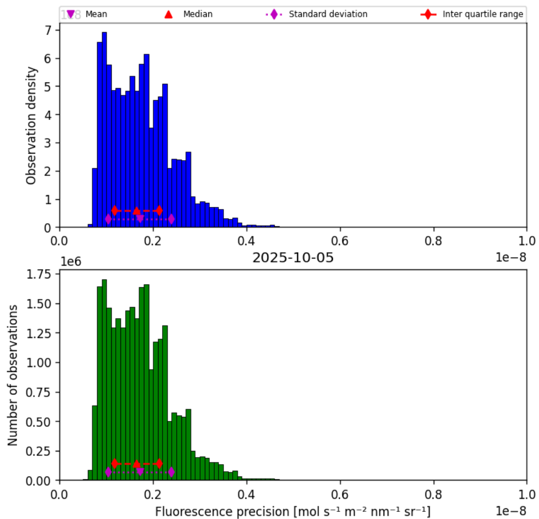
Figure 41: Histogram of “Fluorescence precision” for 2025-10-04 to 2025-10-06
