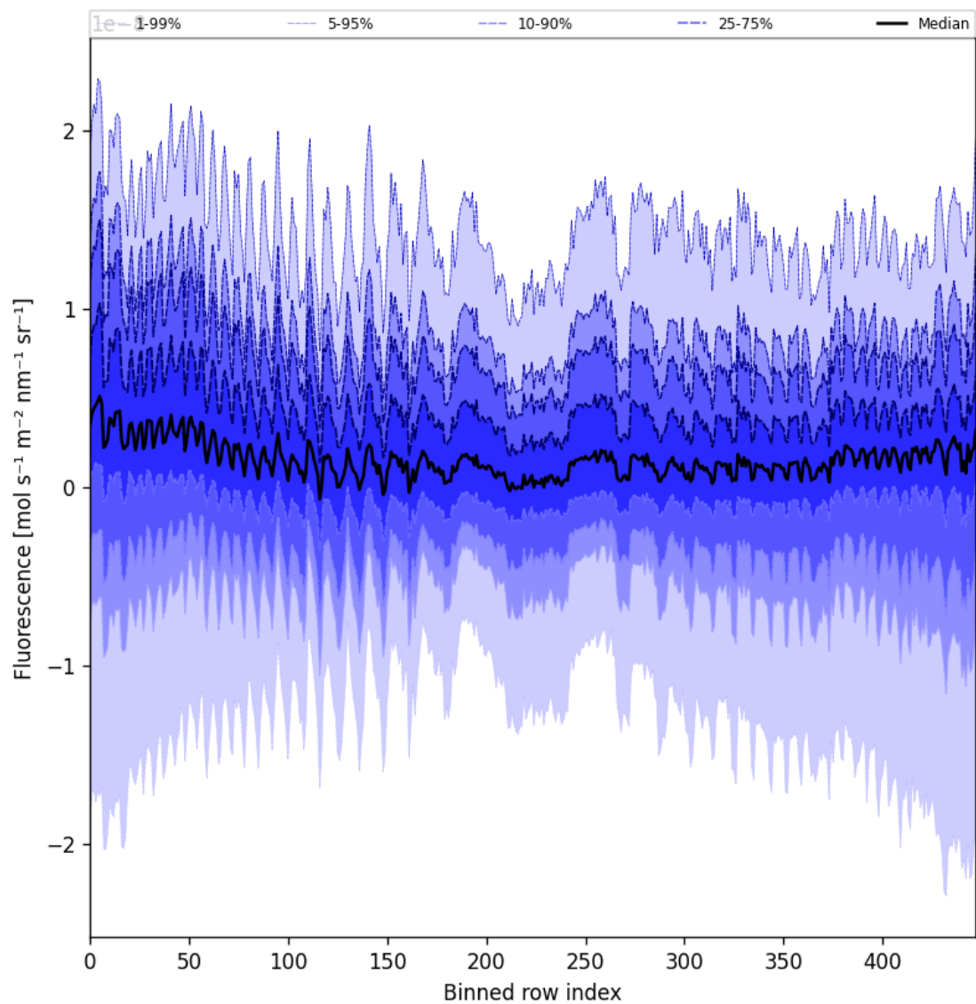
Figure 57: Along track statistics of “Fluorescence” for 2025-10-04 to 2025-10-06
