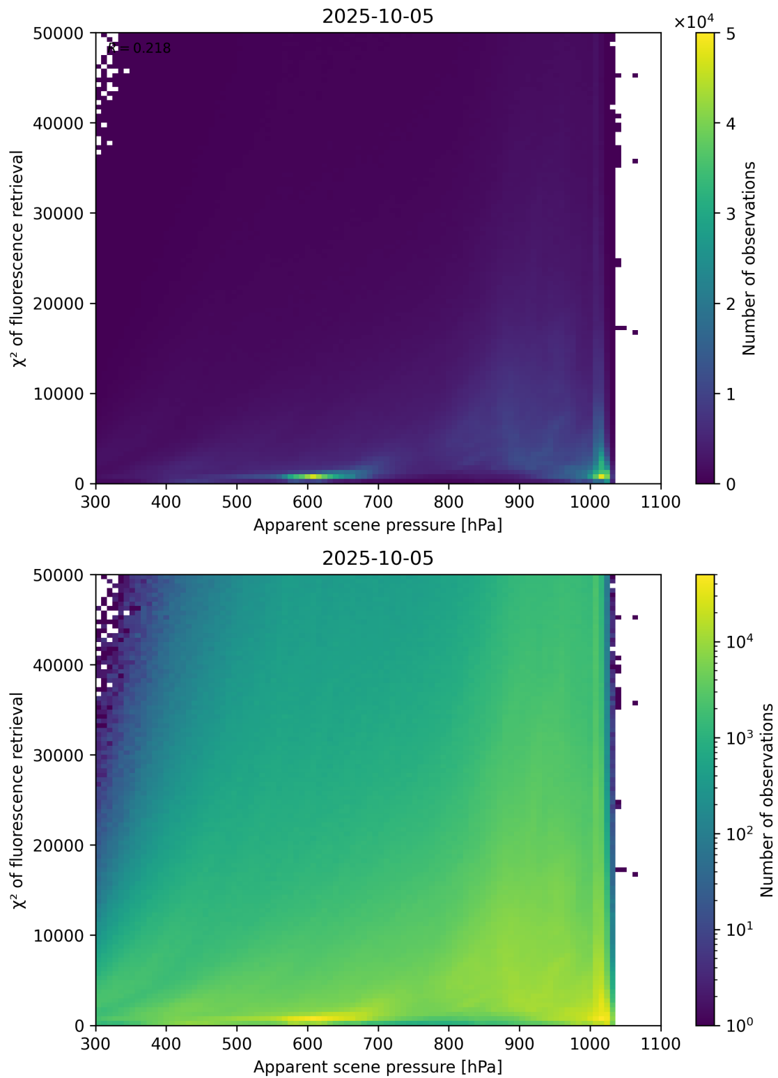
Figure 63: Scatter density plot of “Apparent scene pressure” against “ \chi^2 of fluorescence retrieval” for 2025-10-04 to 2025-10-06.
