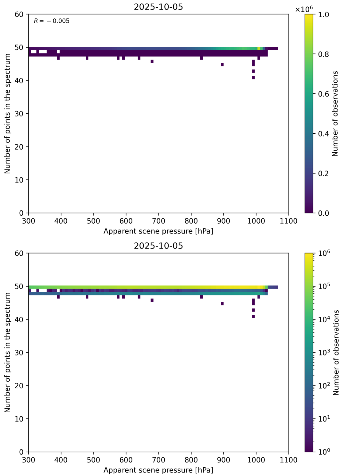
Figure 66: Scatter density plot of “Apparent scene pressure” against “Number of points in the spectrum” for 2025-10-04 to 2025-10-06.
