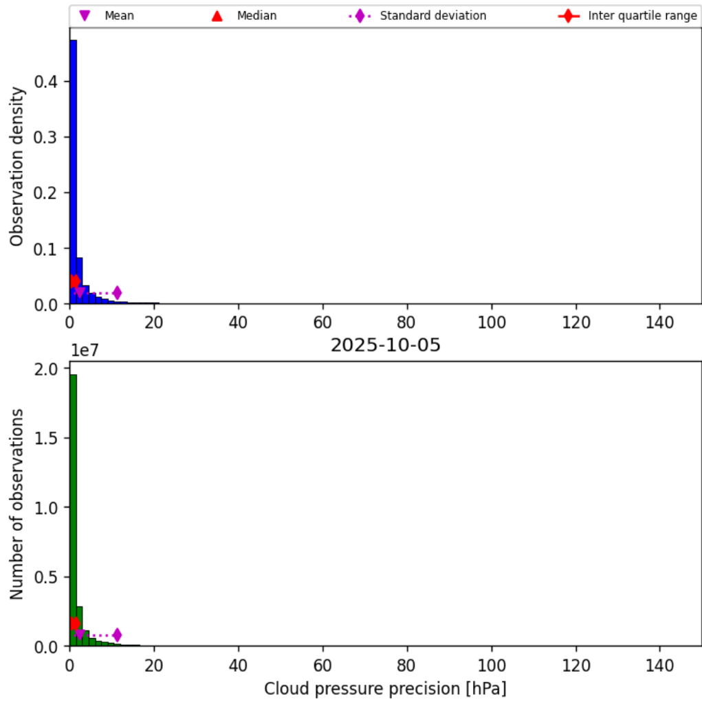
Figure 31: Histogram of “Cloud pressure precision” for 2025-10-04 to 2025-10-06
