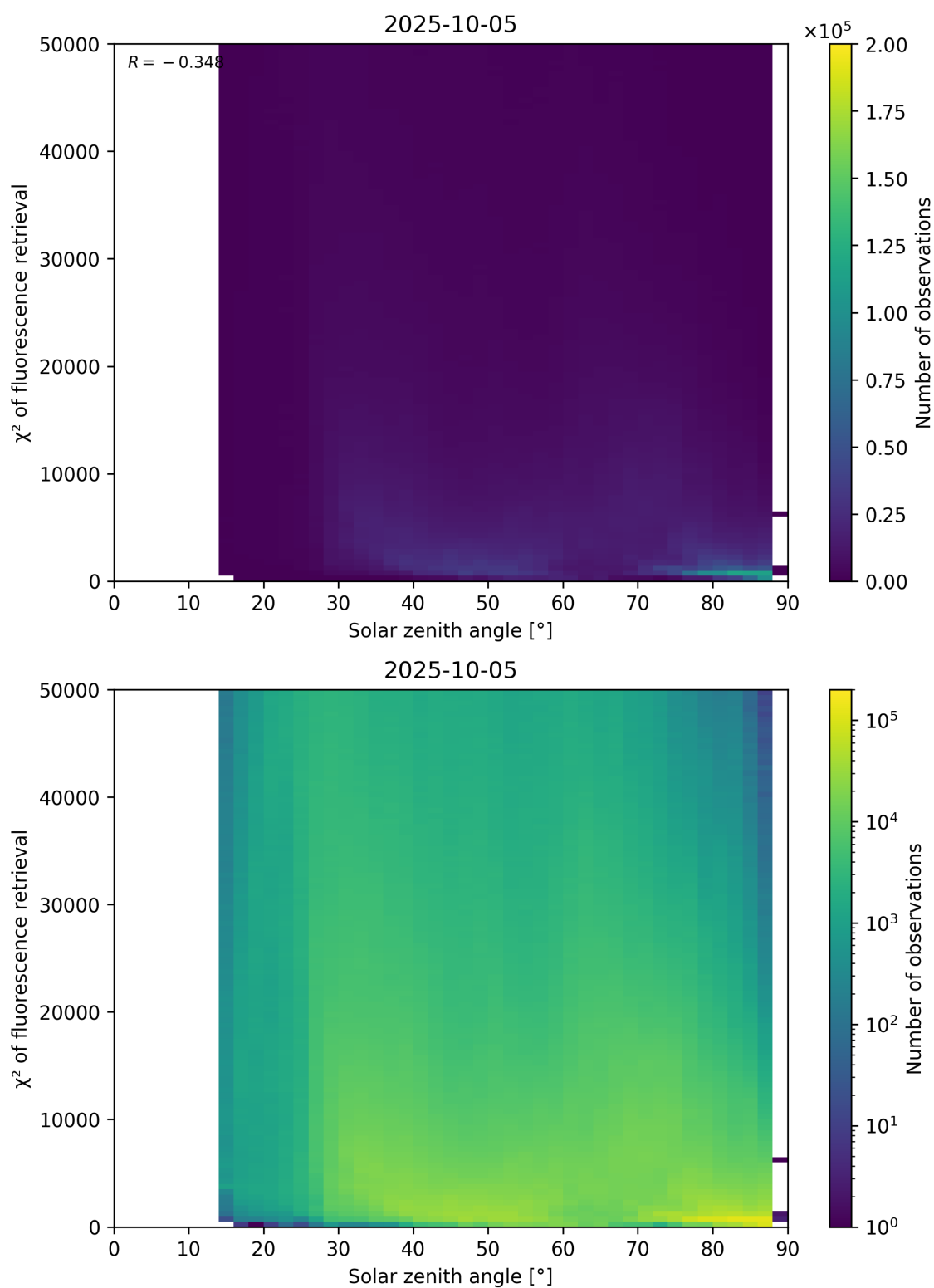
Figure 109: Scatter density plot of “Solar zenith angle” against “ \chi^2 of fluorescence retrieval” for 2025-10-04 to 2025-10-06.
