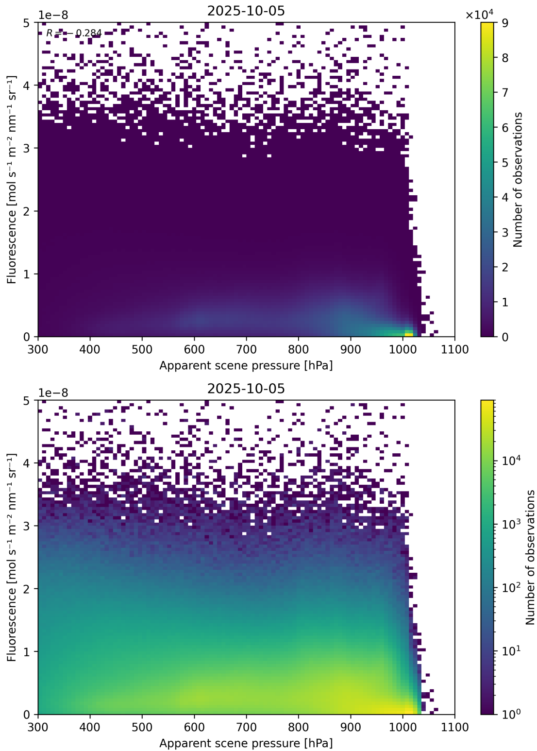
Figure 64: Scatter density plot of “Apparent scene pressure” against “Fluorescence” for 2025-10-04 to 2025-10-06.
