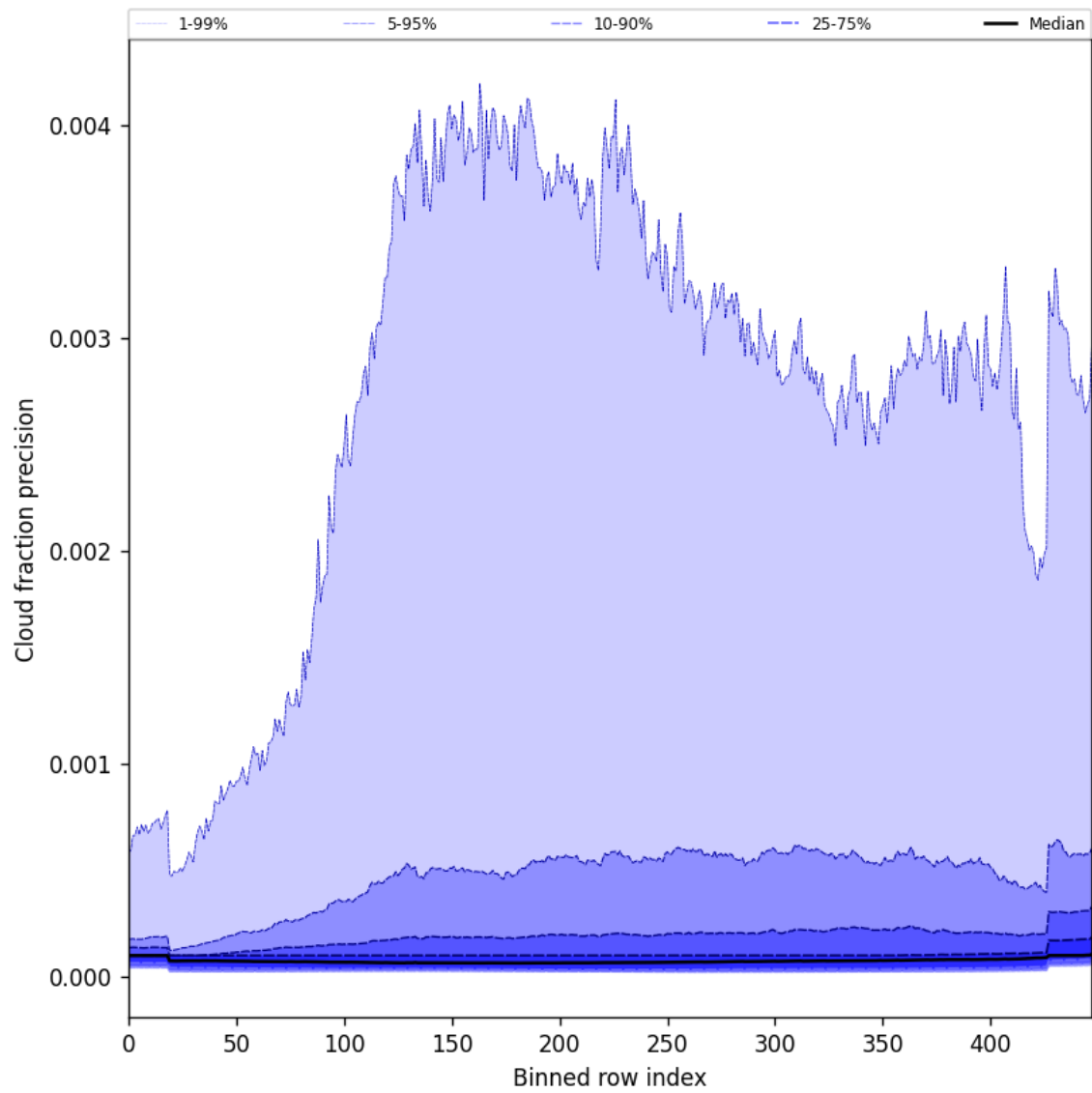
Figure 50: Along track statistics of “Cloud fraction precision” for 2025-10-04 to 2025-10-06
