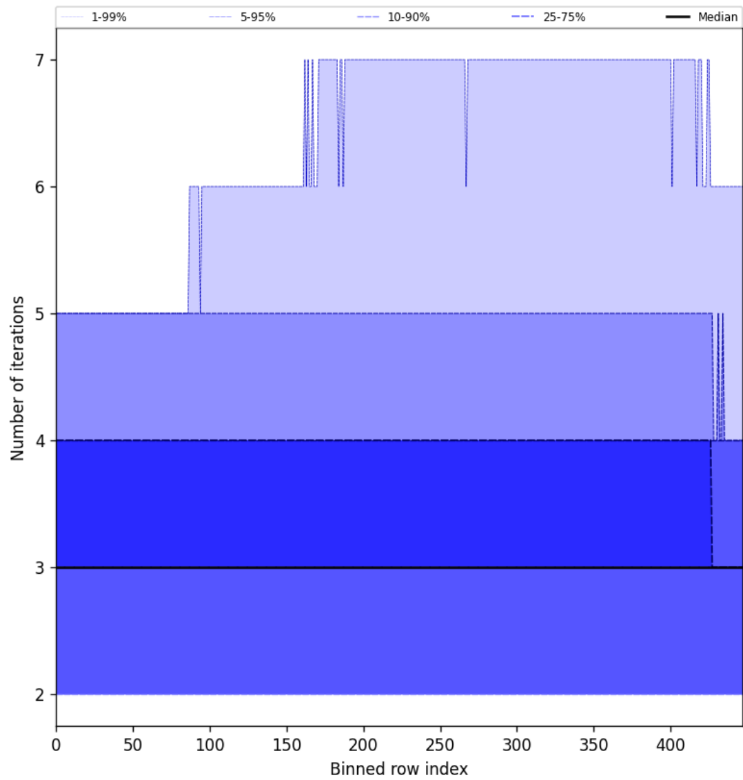
Figure 56: Along track statistics of “Number of iterations” for 2025-10-04 to 2025-10-06
