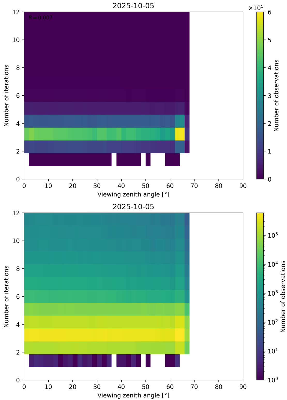
Figure 124: Scatter density plot of “Viewing zenith angle” against “Number of iterations” for 2025-10-04 to 2025-10-06.
