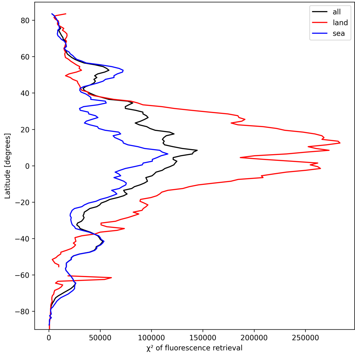
Figure 25: Zonal average of “ \chi^2 of fluorescence retrieval” for 2025-10-04 to 2025-10-06.
