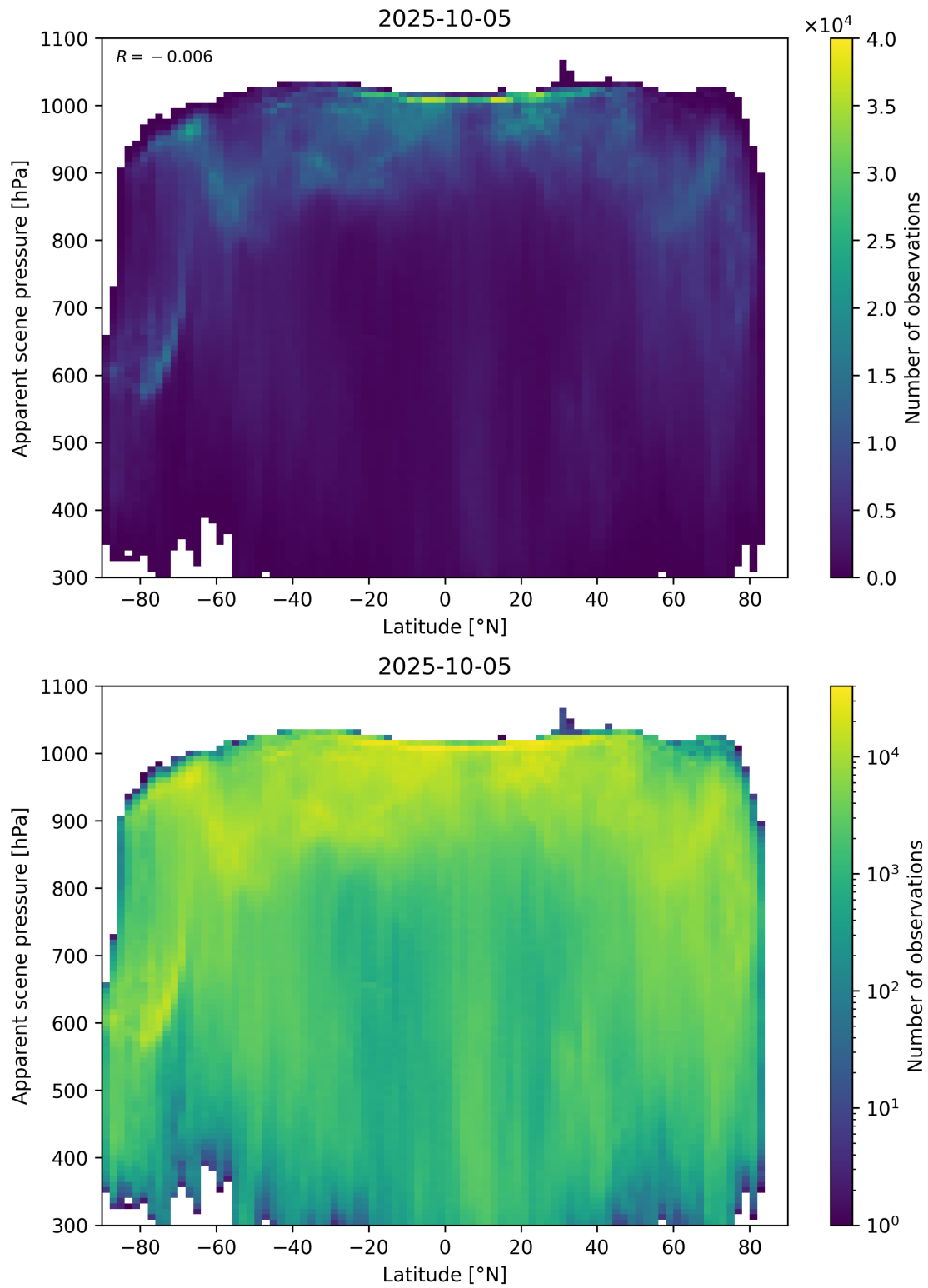
Figure 88: Scatter density plot of “Latitude” against “Apparent scene pressure” for 2025-10-04 to 2025-10-06.
