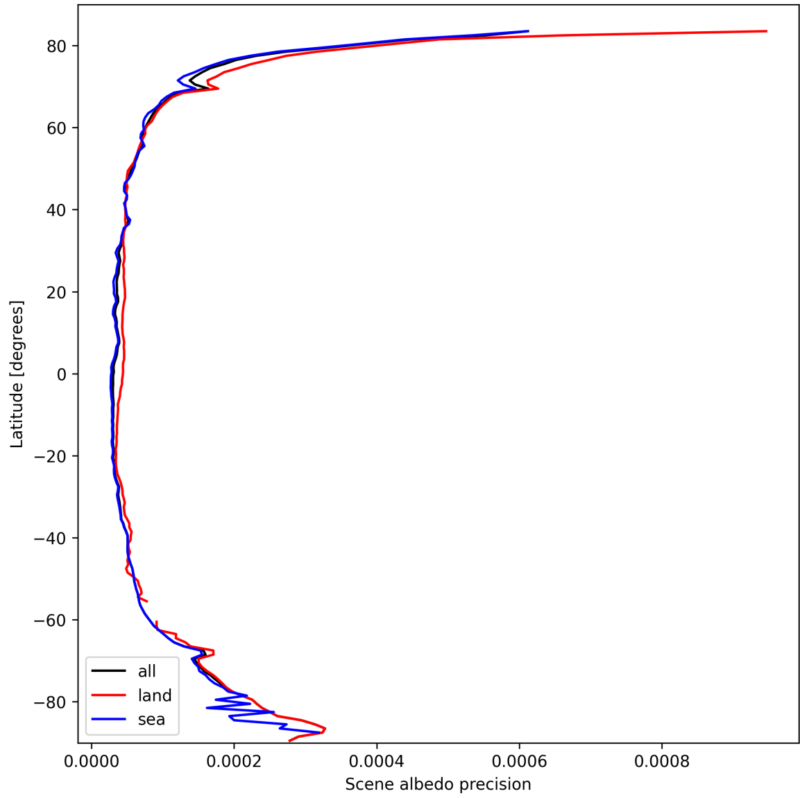
Figure 18: Zonal average of “Scene albedo precision” for 2025-10-04 to 2025-10-06.
