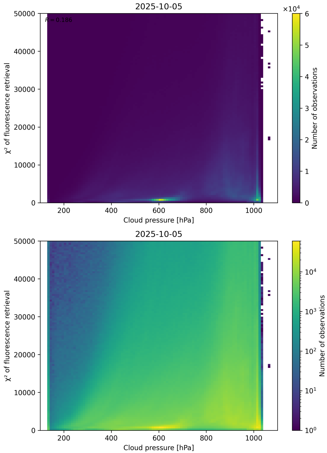
Figure 78: Scatter density plot of “Cloud pressure” against “ \chi^2 of fluorescence retrieval” for 2025-10-04 to 2025-10-06.
