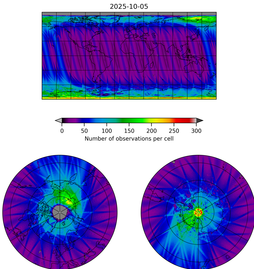
Figure 11: Map of the number of observations for 2025-10-04 to 2025-10-06
