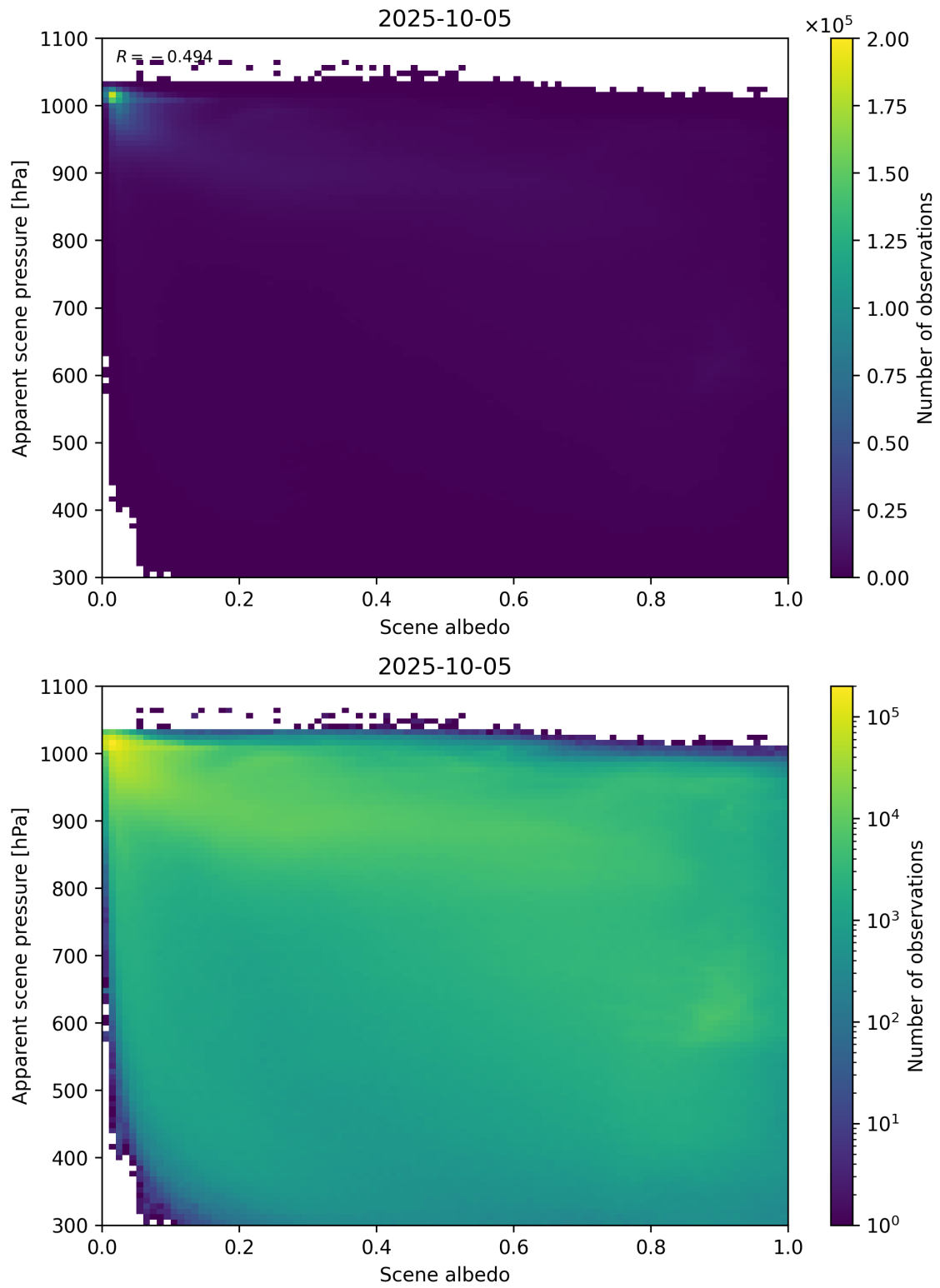
Figure 102: Scatter density plot of “Scene albedo” against “Apparent scene pressure” for 2025-10-04 to 2025-10-06.
