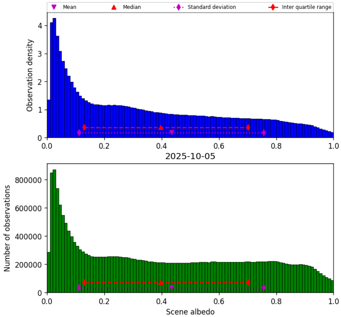
Figure 34: Histogram of “Scene albedo” for 2025-10-04 to 2025-10-06
