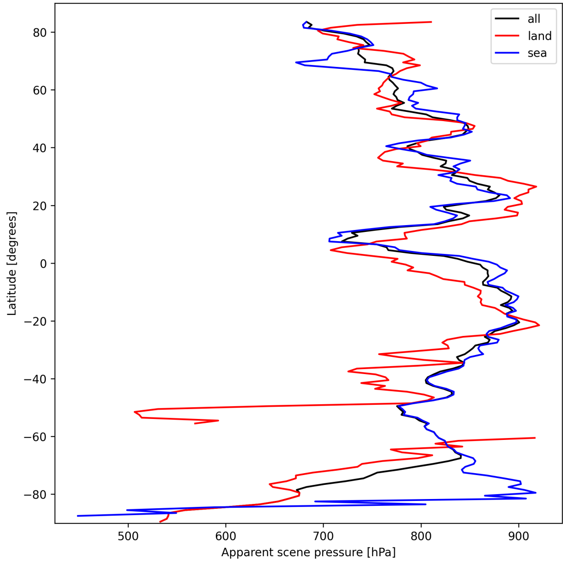
Figure 19: Zonal average of “Apparent scene pressure” for 2025-10-04 to 2025-10-06.
