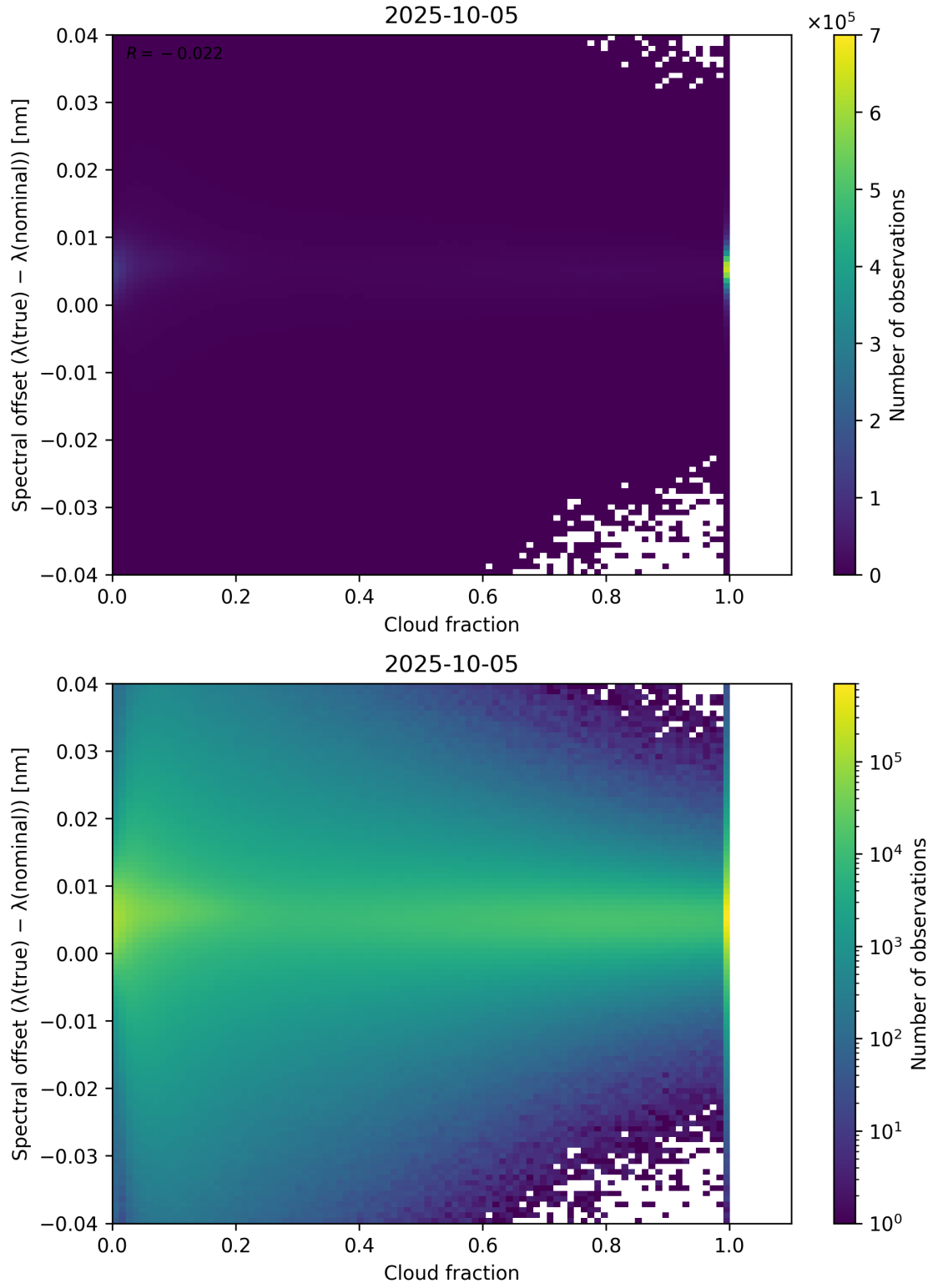
Figure 76: Scatter density plot of “Cloud fraction” against “Spectral offset ( \lambda_{\text{true}} - \lambda_{\text{nominal}} )” for 2025-10-04 to 2025-10-06.
