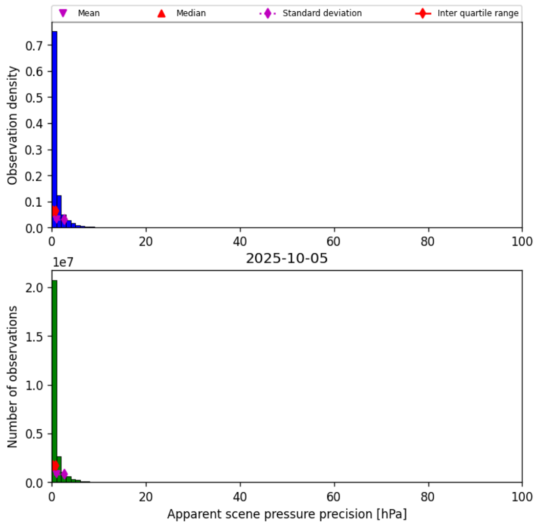
Figure 37: Histogram of “Apparent scene pressure precision” for 2025-10-04 to 2025-10-06
