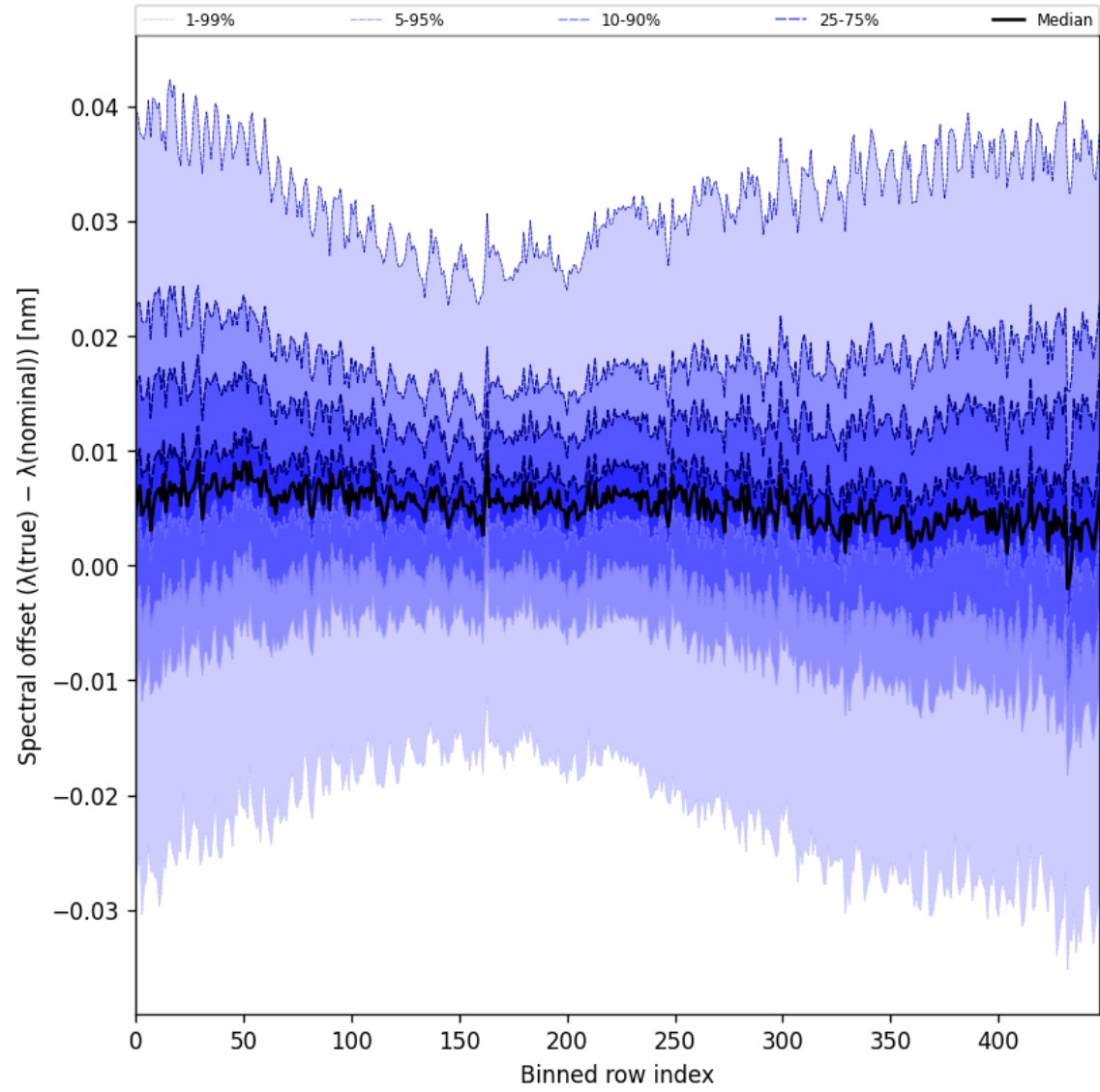
Figure 62: Along track statistics of “Spectral offset ( \lambda_{\text{true}} - \lambda_{\text{nominal}} )” for 2025-10-04 to 2025-10-06
