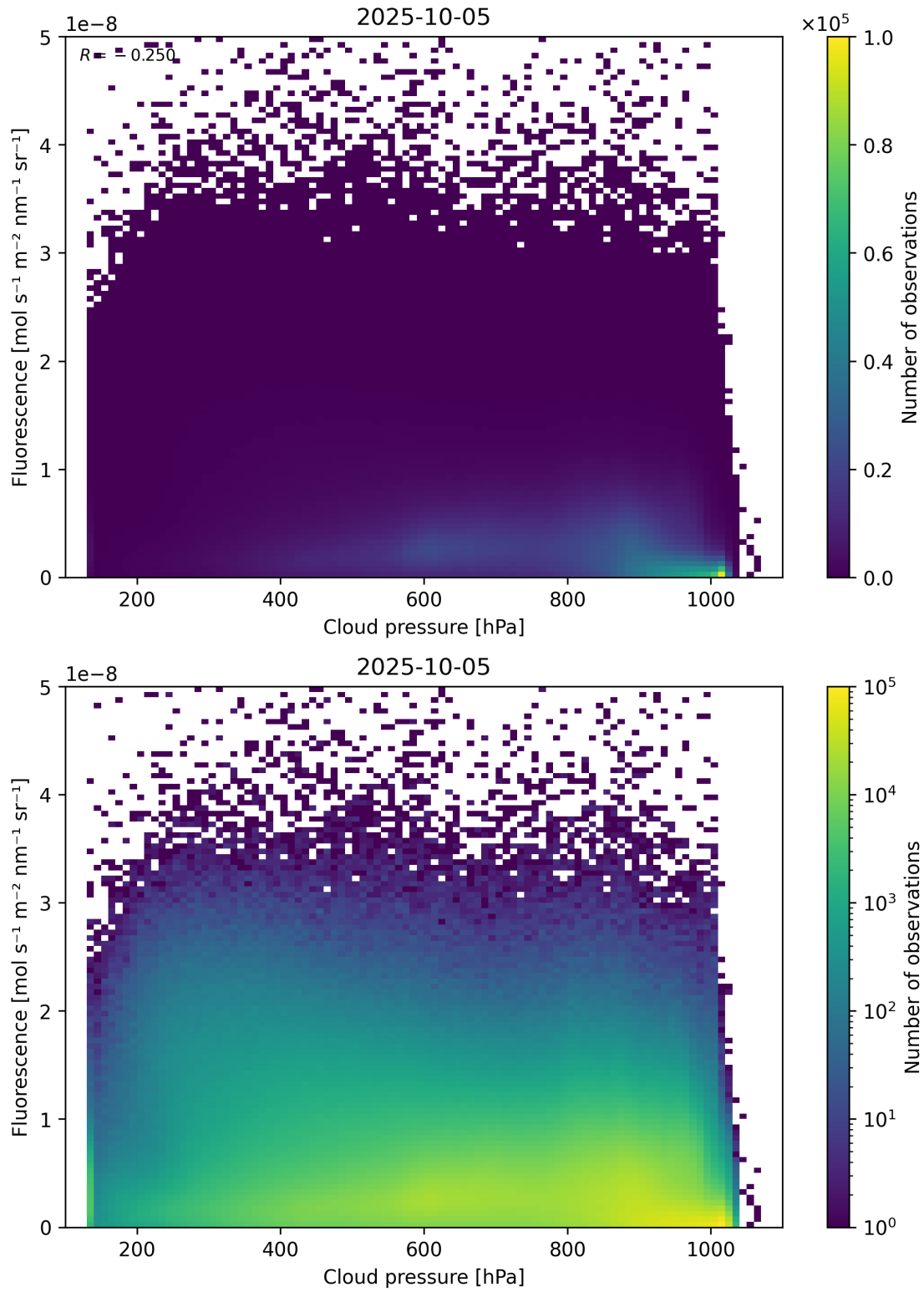
Figure 80: Scatter density plot of “Cloud pressure” against “Fluorescence” for 2025-10-04 to 2025-10-06.
