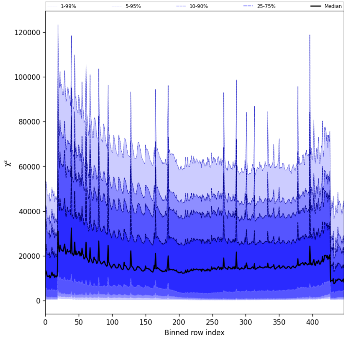
Figure 55: Along track statistics of “ \chi^2 ” for 2025-10-04 to 2025-10-06
