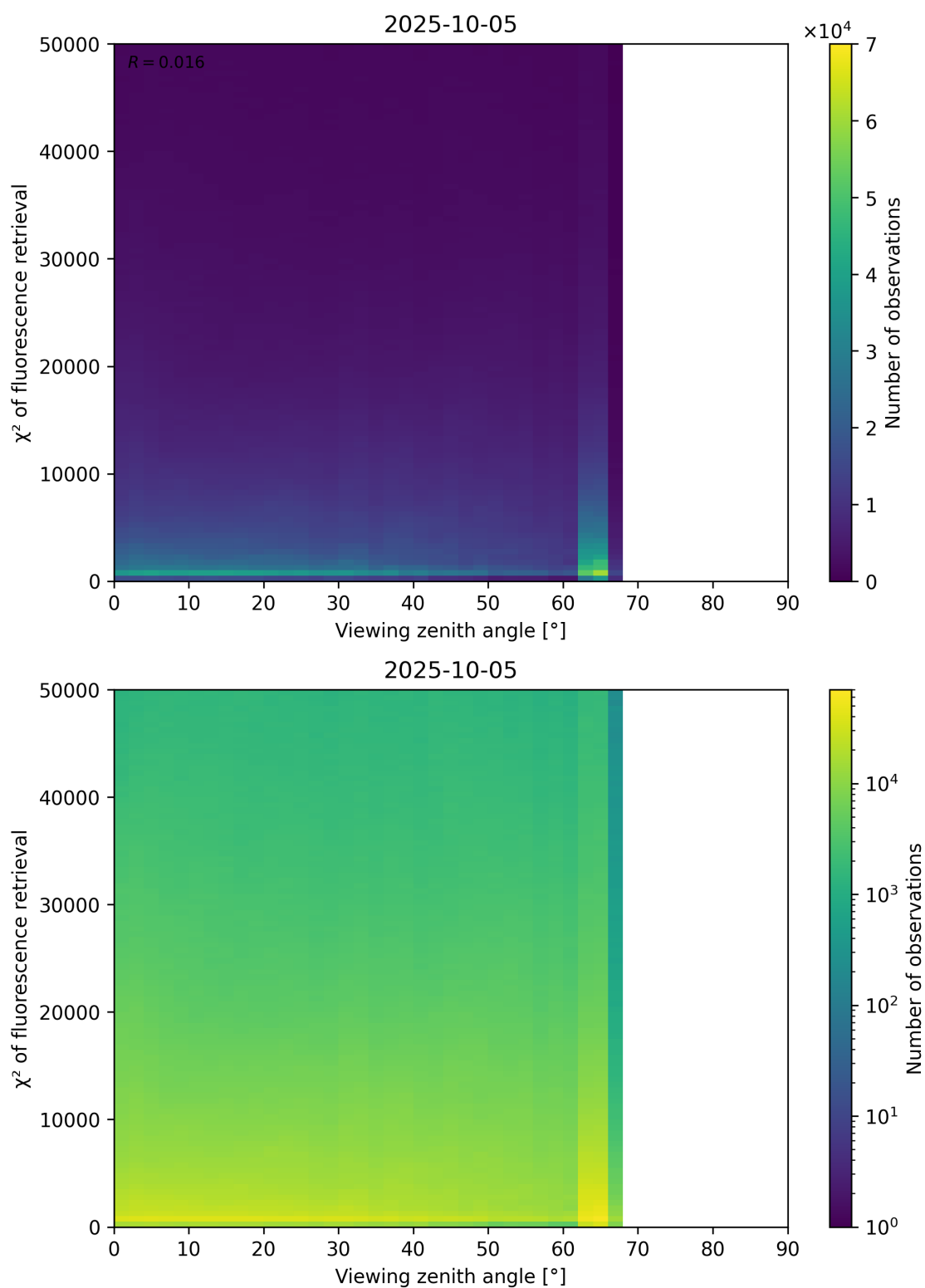
Figure 119: Scatter density plot of “Viewing zenith angle” against “ \chi^2 of fluorescence retrieval” for 2025-10-04 to 2025-10-06.
