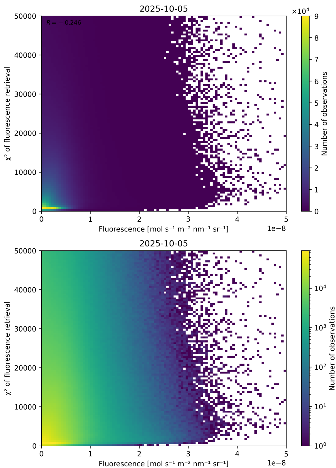
Figure 85: Scatter density plot of “Fluorescence” against “ \chi^2 of fluorescence retrieval” for 2025-10-04 to 2025-10-06.
