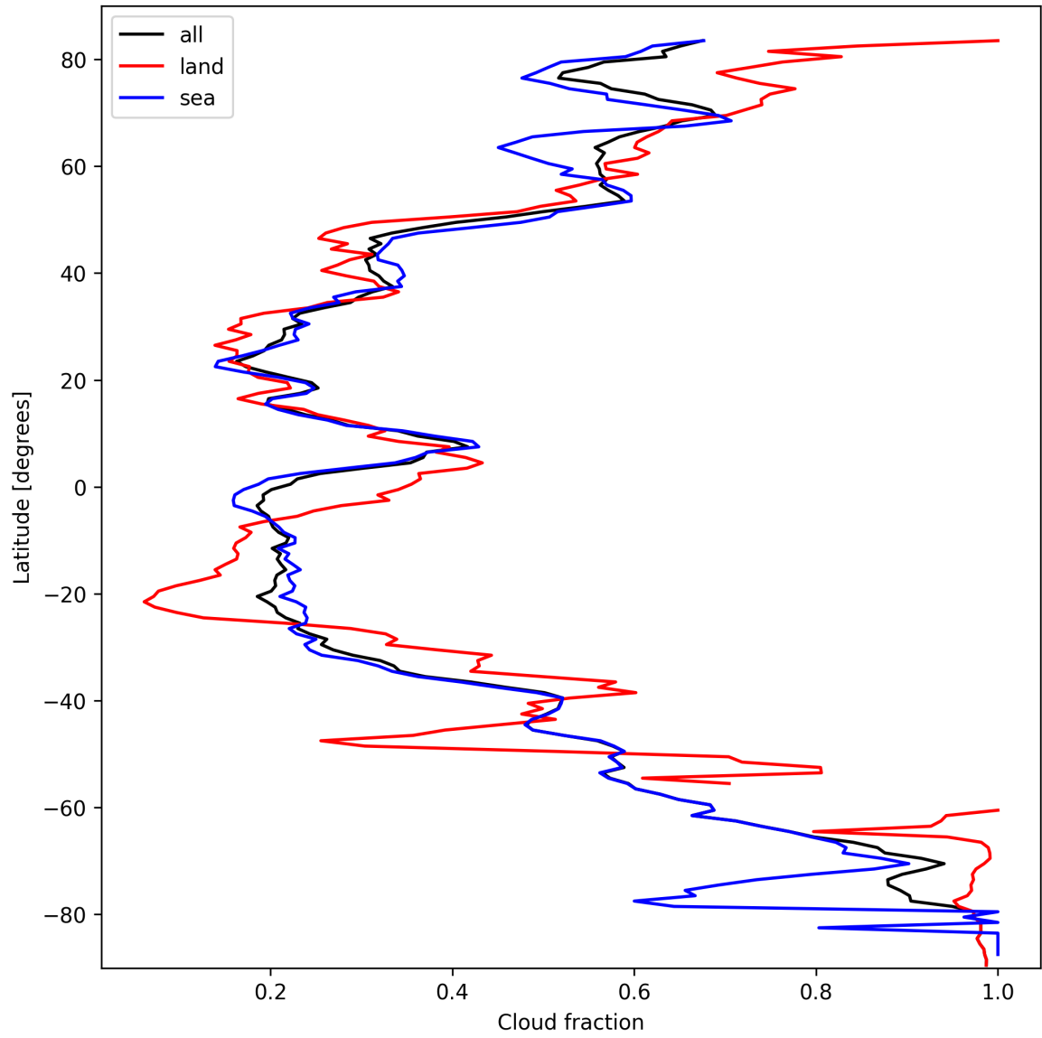
Figure 15: Zonal average of “Cloud fraction” for 2025-10-04 to 2025-10-06.
