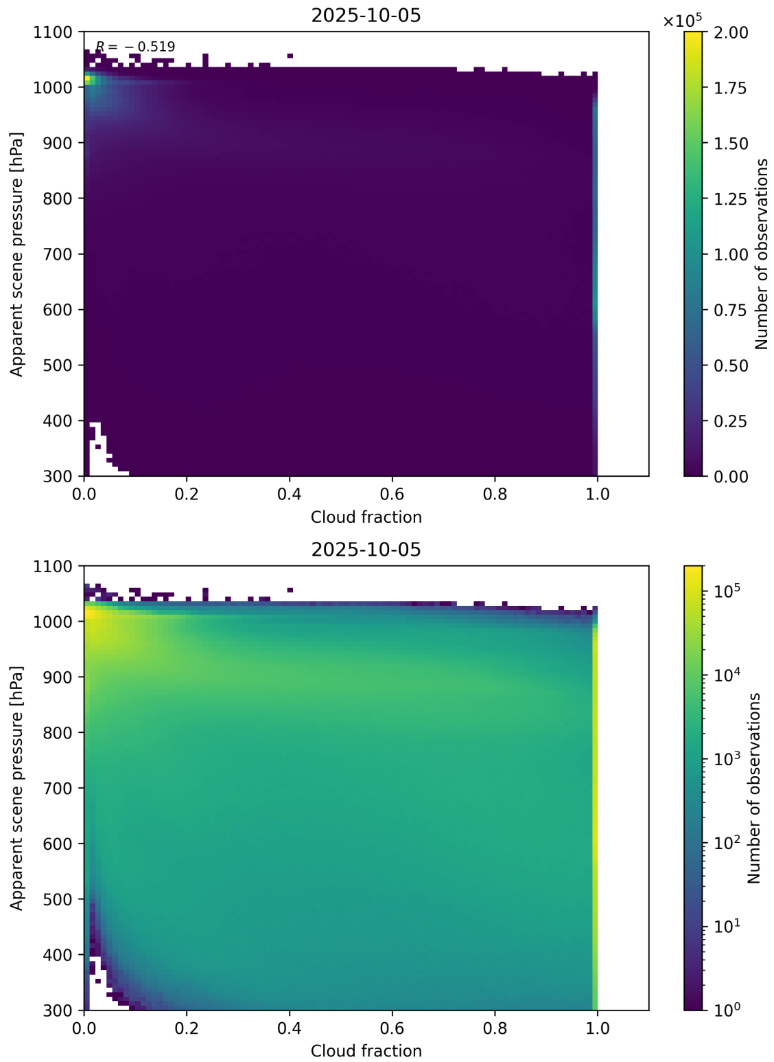
Figure 70: Scatter density plot of “Cloud fraction” against “Apparent scene pressure” for 2025-10-04 to 2025-10-06.
