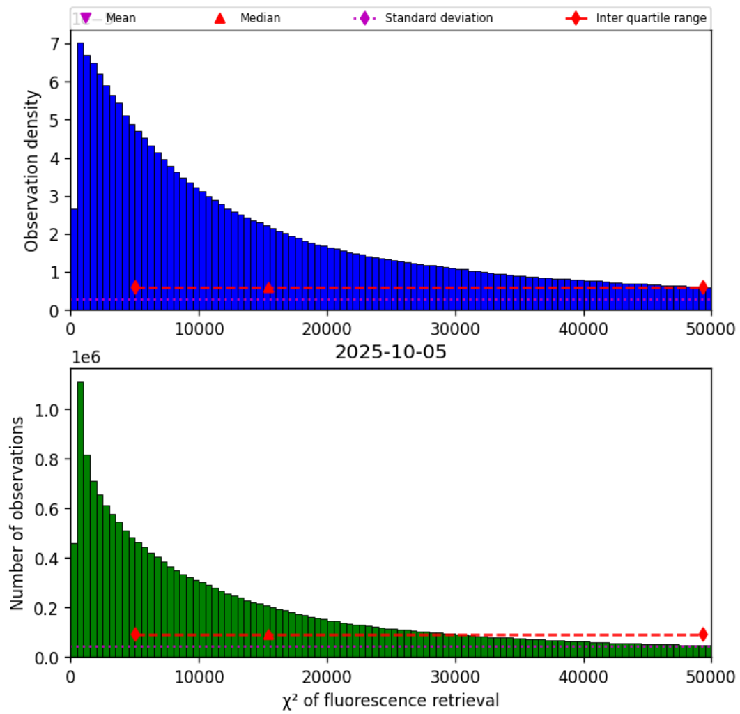
Figure 42: Histogram of “ \chi^2 of fluorescence retrieval” for 2025-10-04 to 2025-10-06
