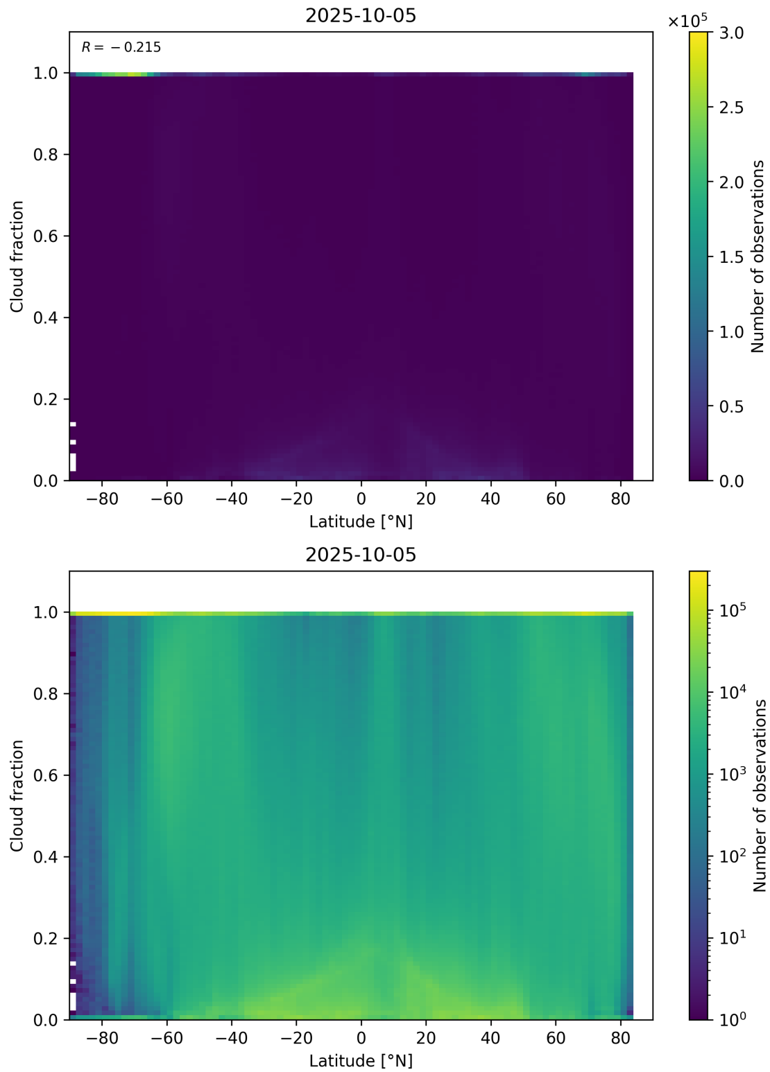
Figure 90: Scatter density plot of “Latitude” against “Cloud fraction” for 2025-10-04 to 2025-10-06.
