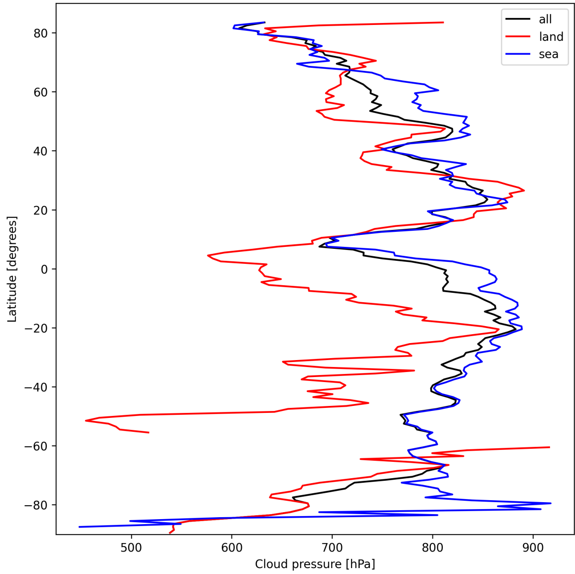
Figure 13: Zonal average of “Cloud pressure” for 2025-10-04 to 2025-10-06.
