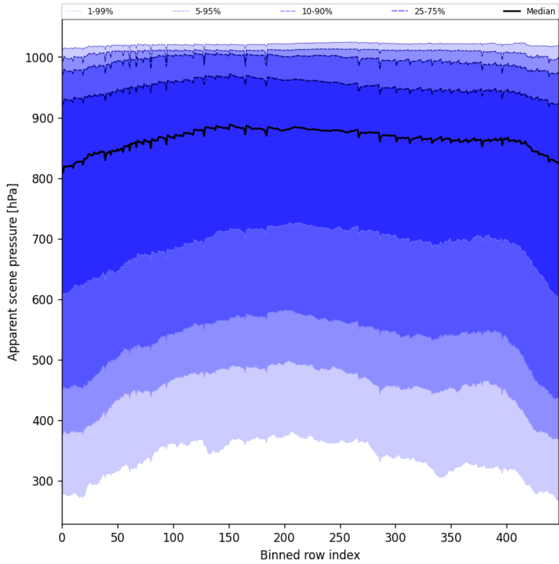
Figure 53: Along track statistics of “Apparent scene pressure” for 2025-10-04 to 2025-10-06
