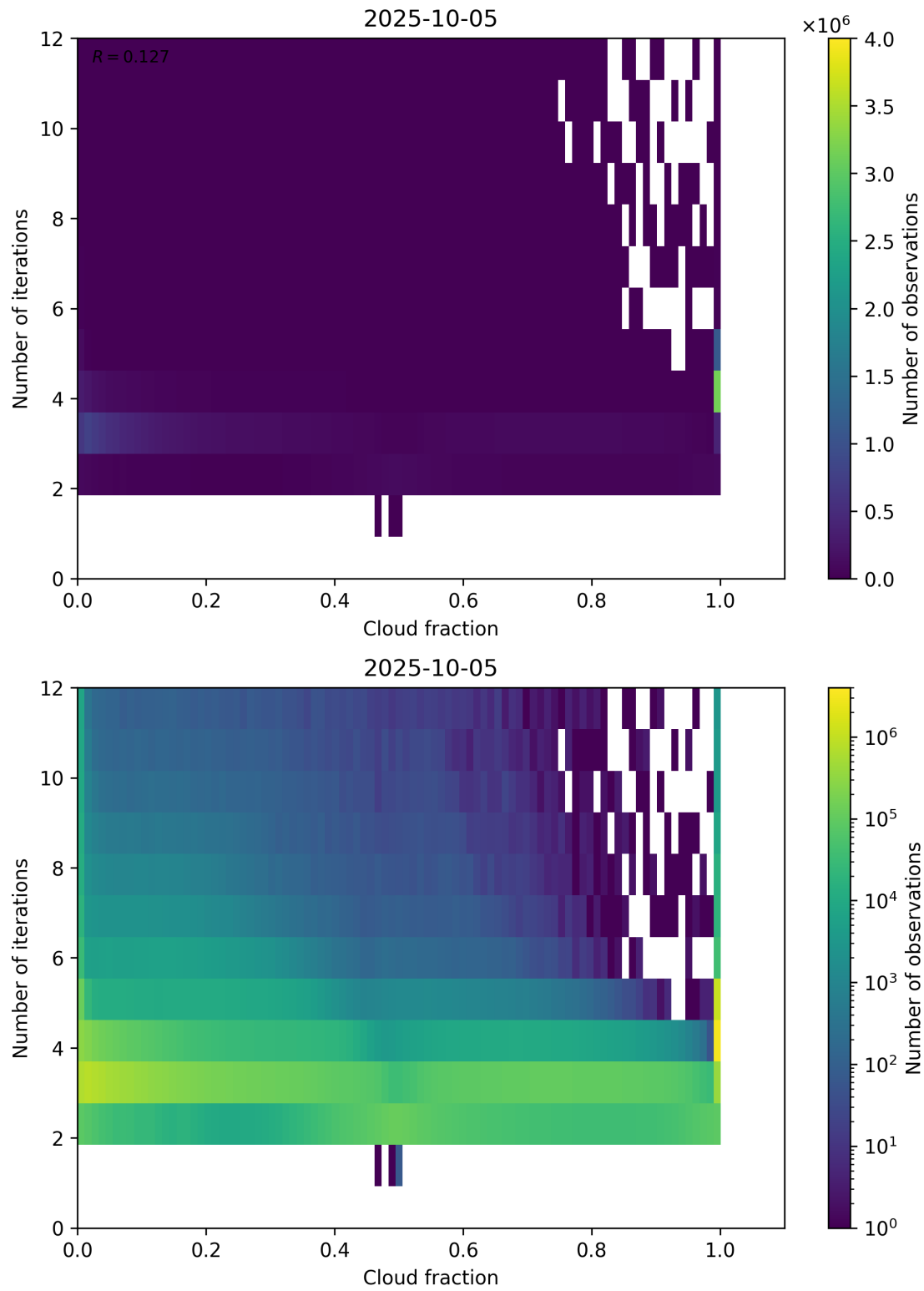
Figure 73: Scatter density plot of “Cloud fraction” against “Number of iterations” for 2025-10-04 to 2025-10-06.
