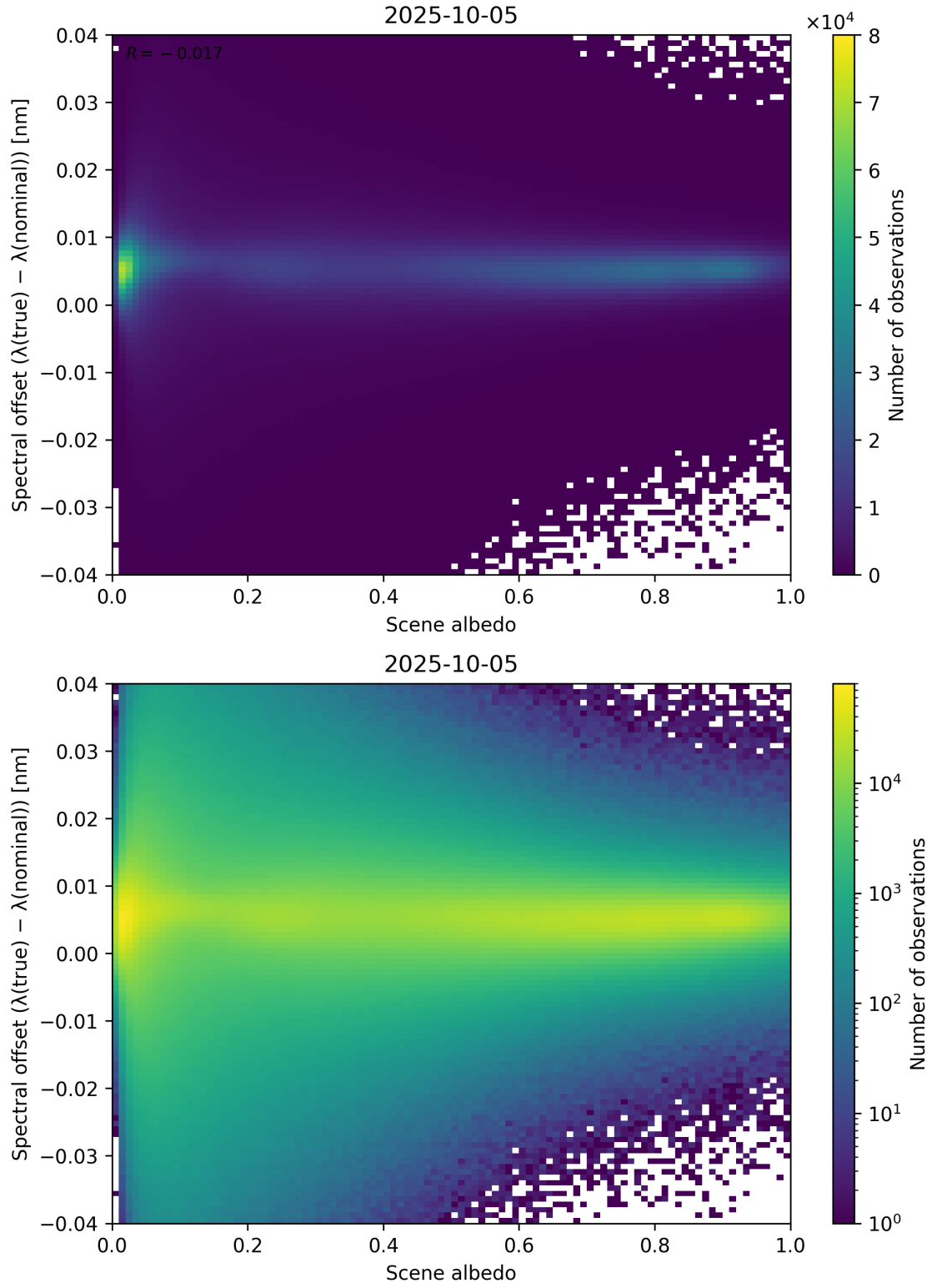
Figure 107: Scatter density plot of “Scene albedo” against “Spectral offset ( \lambda_{\text{true}} - \lambda_{\text{nominal}} )” for 2025-10-04 to 2025-10-06.
