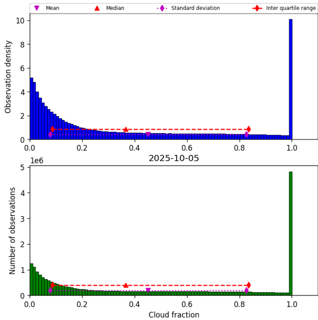
Figure 32: Histogram of “Cloud fraction” for 2025-10-04 to 2025-10-06
