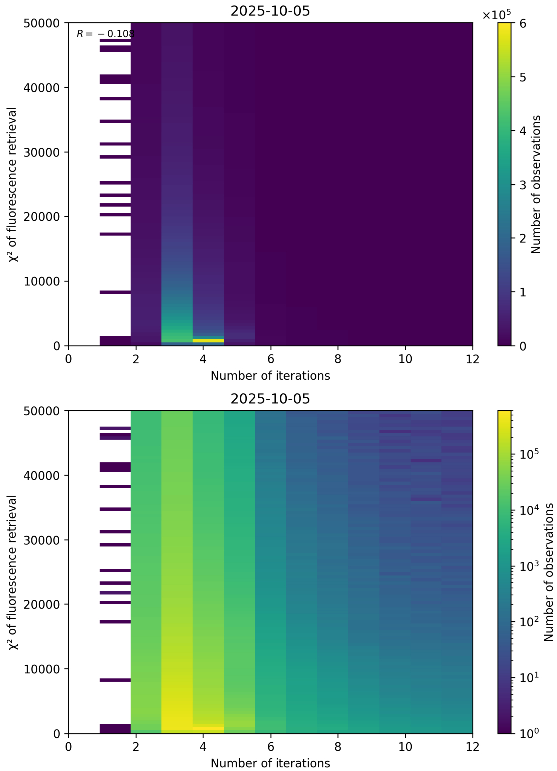
Figure 97: Scatter density plot of “Number of iterations” against “ \chi^2 of fluorescence retrieval” for 2025-10-04 to 2025-10-06.
