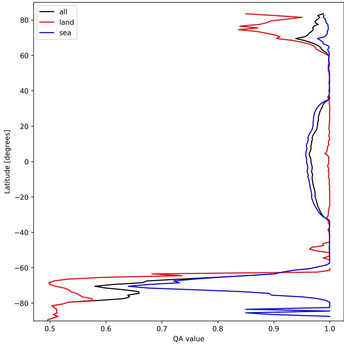
Figure 12: Zonal average of “QA value” for 2025-10-04 to 2025-10-06.
