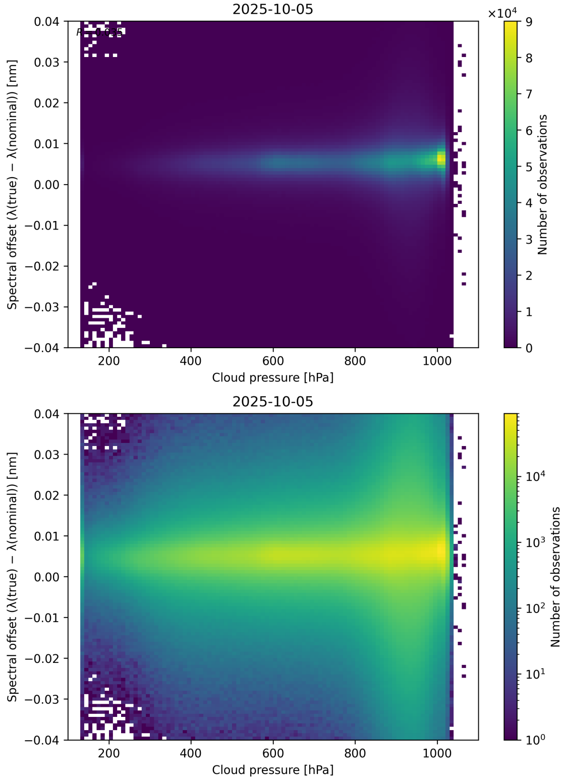
Figure 84: Scatter density plot of “Cloud pressure” against “Spectral offset ( \lambda_{\text{true}} - \lambda_{\text{nominal}} )” for 2025-10-04 to 2025-10-06.
