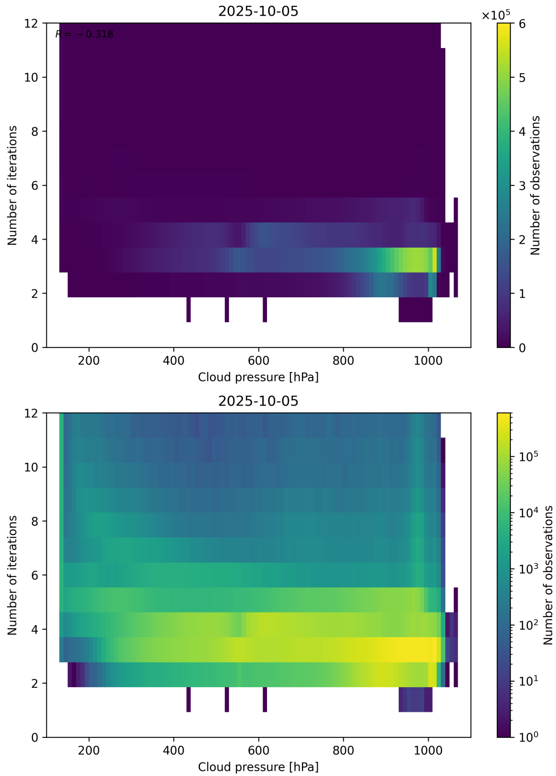
Figure 81: Scatter density plot of “Cloud pressure” against “Number of iterations” for 2025-10-04 to 2025-10-06.
