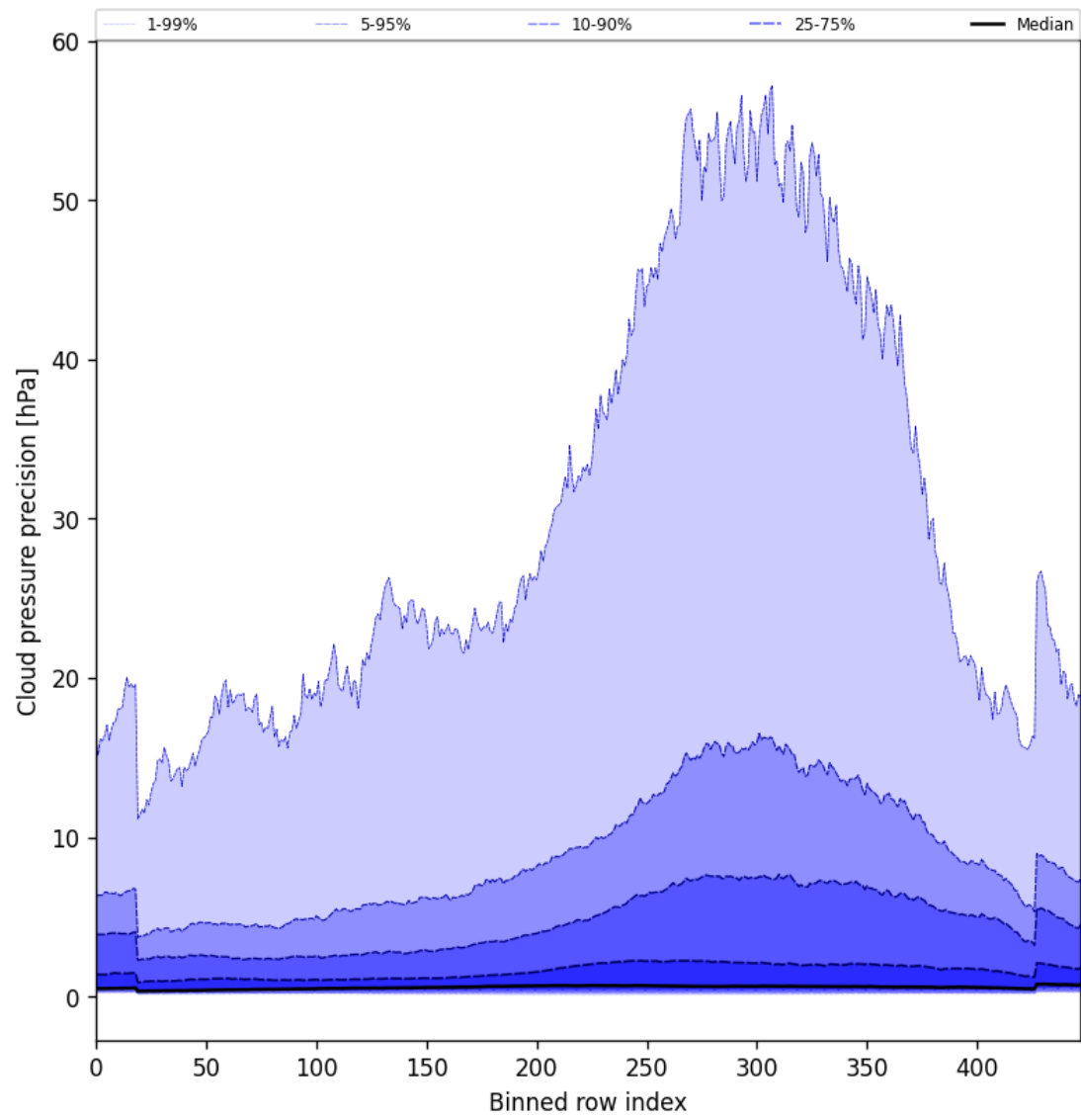
Figure 48: Along track statistics of “Cloud pressure precision” for 2025-10-04 to 2025-10-06
