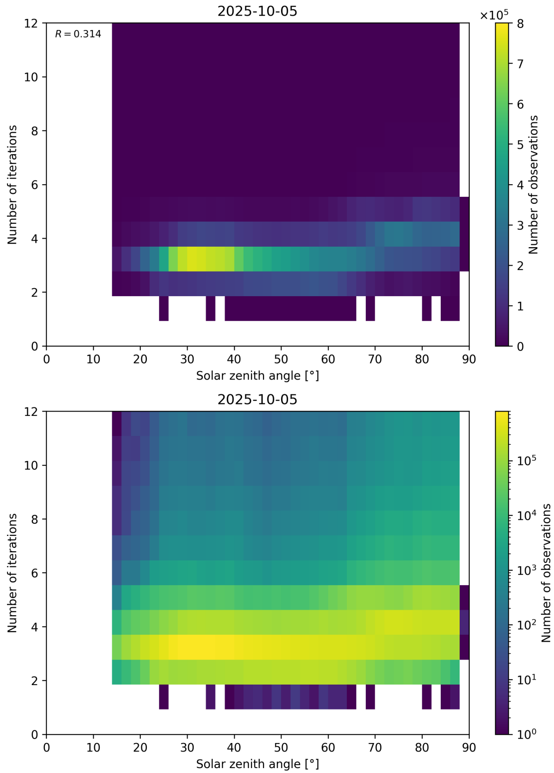
Figure 114: Scatter density plot of “Solar zenith angle” against “Number of iterations” for 2025-10-04 to 2025-10-06.
