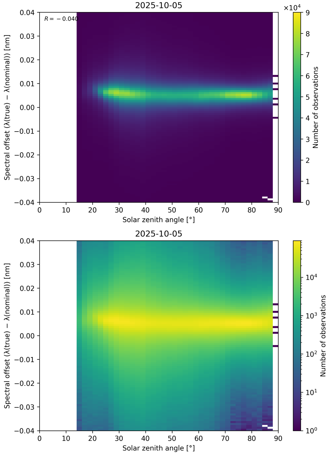
Figure 117: Scatter density plot of “Solar zenith angle” against “Spectral offset ( \lambda_{\text{true}} - \lambda_{\text{nominal}} )” for 2025-10-04 to 2025-10-06.
