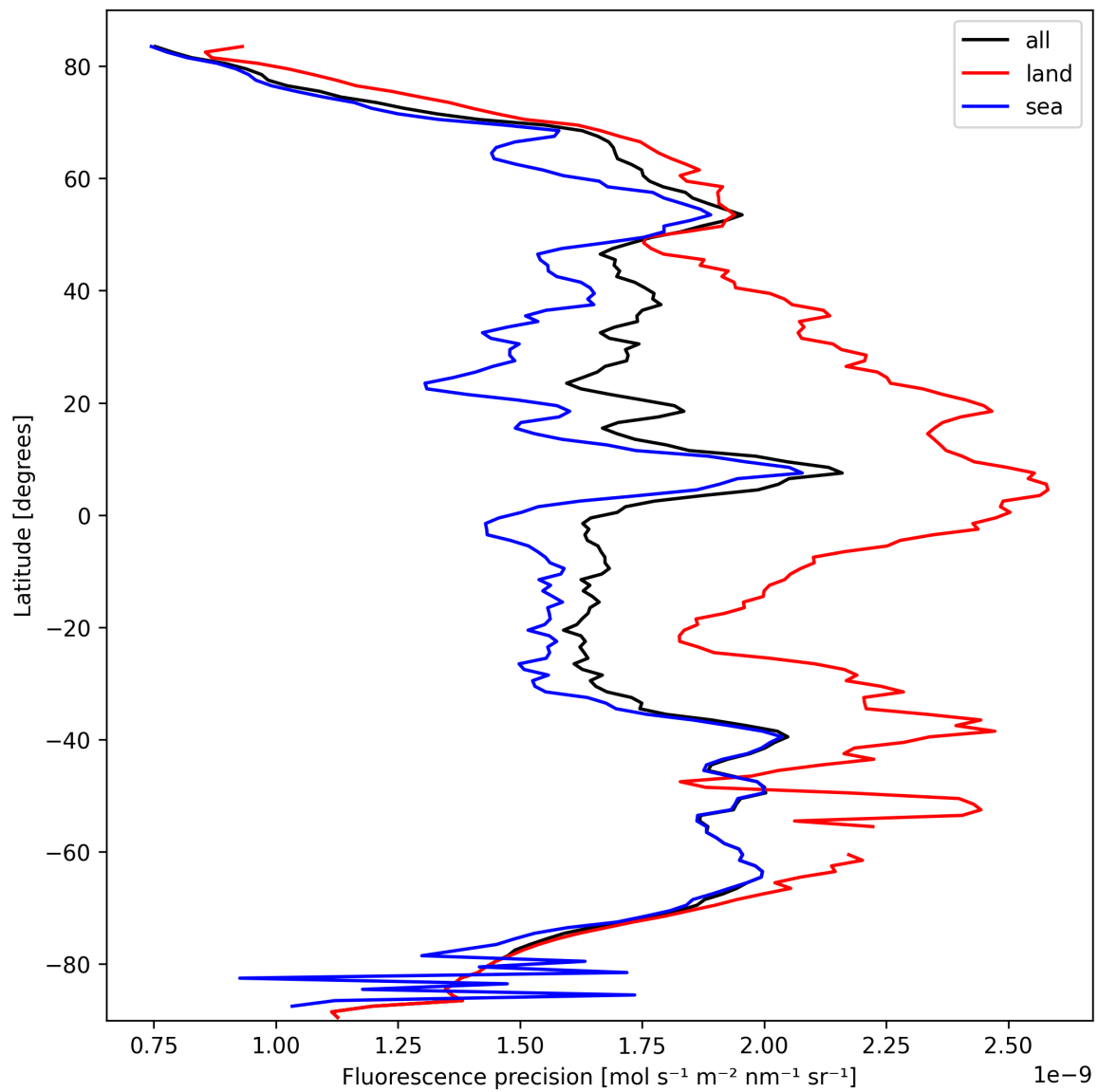
Figure 24: Zonal average of “Fluorescence precision” for 2025-10-04 to 2025-10-06.
