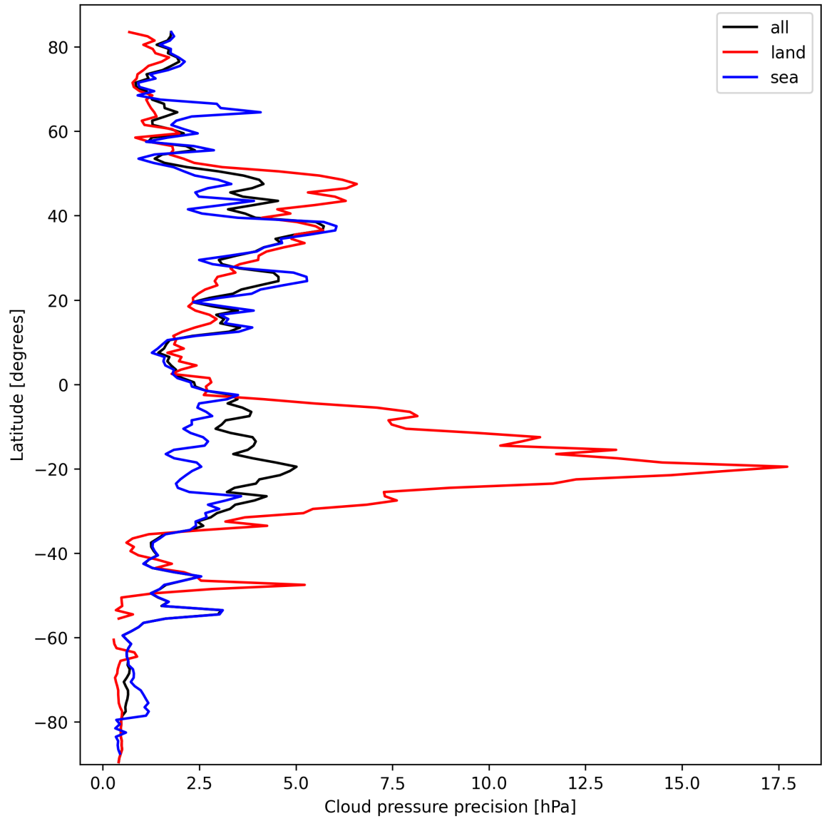
Figure 14: Zonal average of “Cloud pressure precision” for 2025-10-04 to 2025-10-06.
