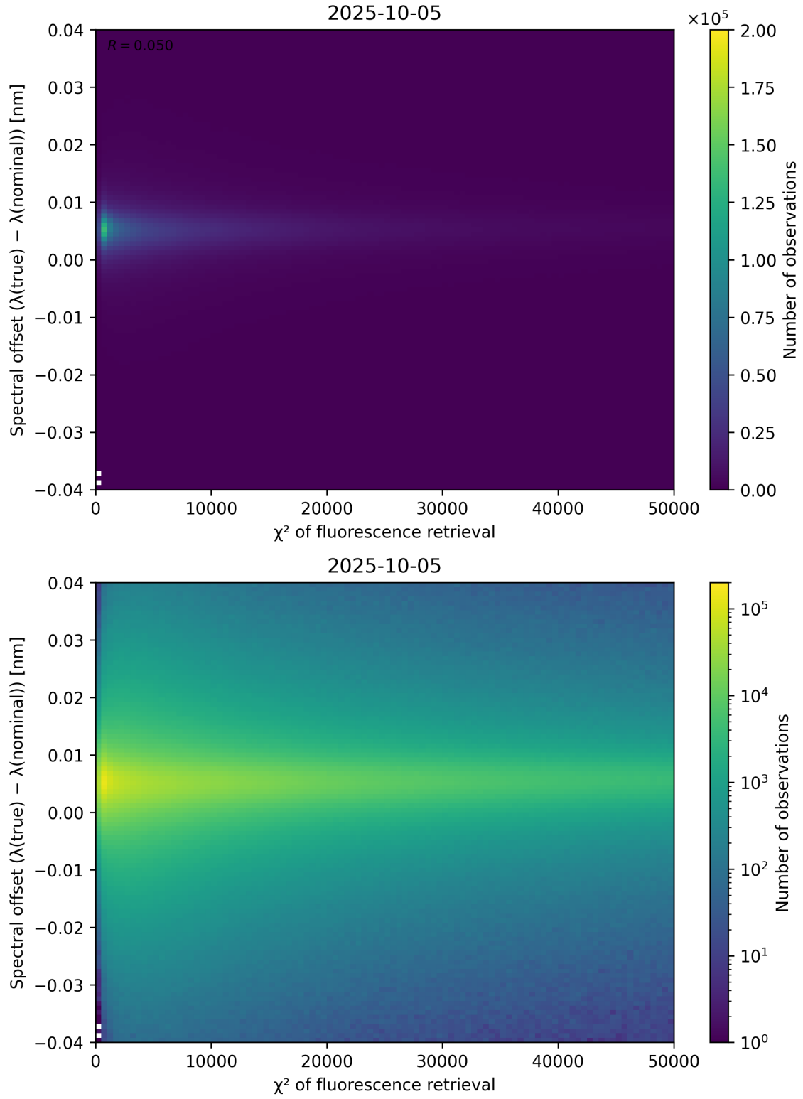
Figure 69: Scatter density plot of “ \chi^2 of fluorescence retrieval” against “Spectral offset ( \lambda_{\text{true}} - \lambda_{\text{nominal}} )” for 2025-10-04 to 2025-10-06.
