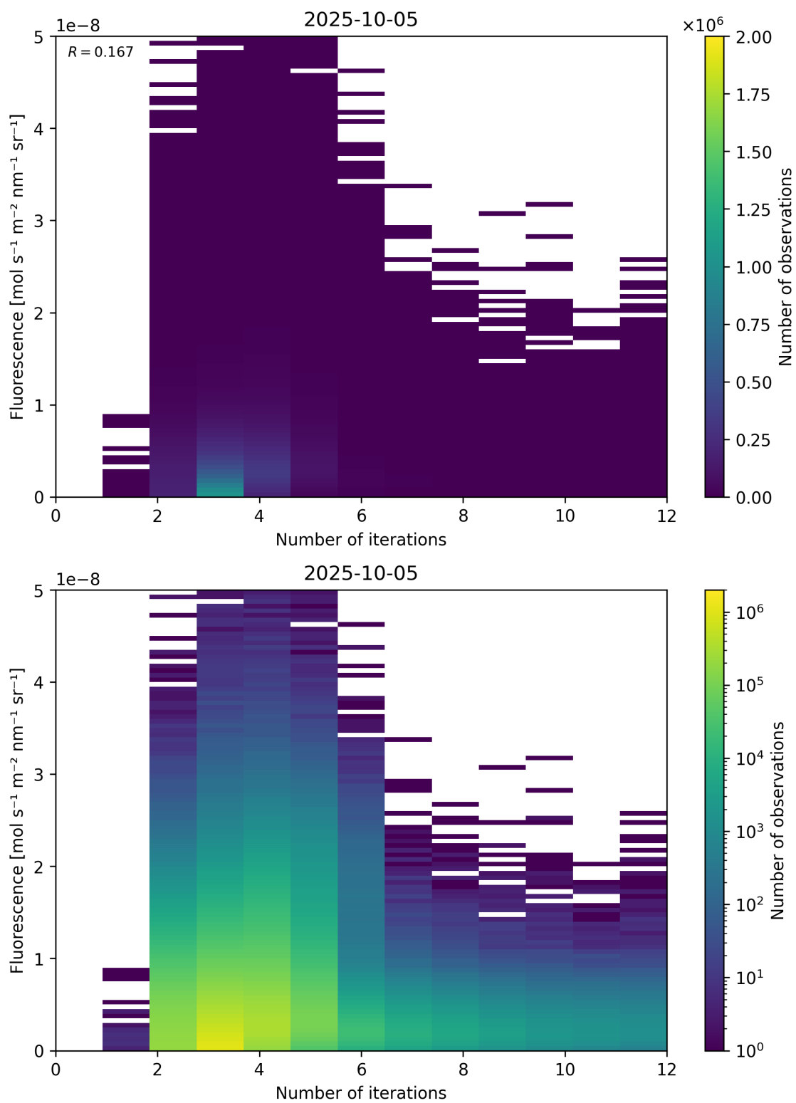
Figure 98: Scatter density plot of “Number of iterations” against “Fluorescence” for 2025-10-04 to 2025-10-06.
