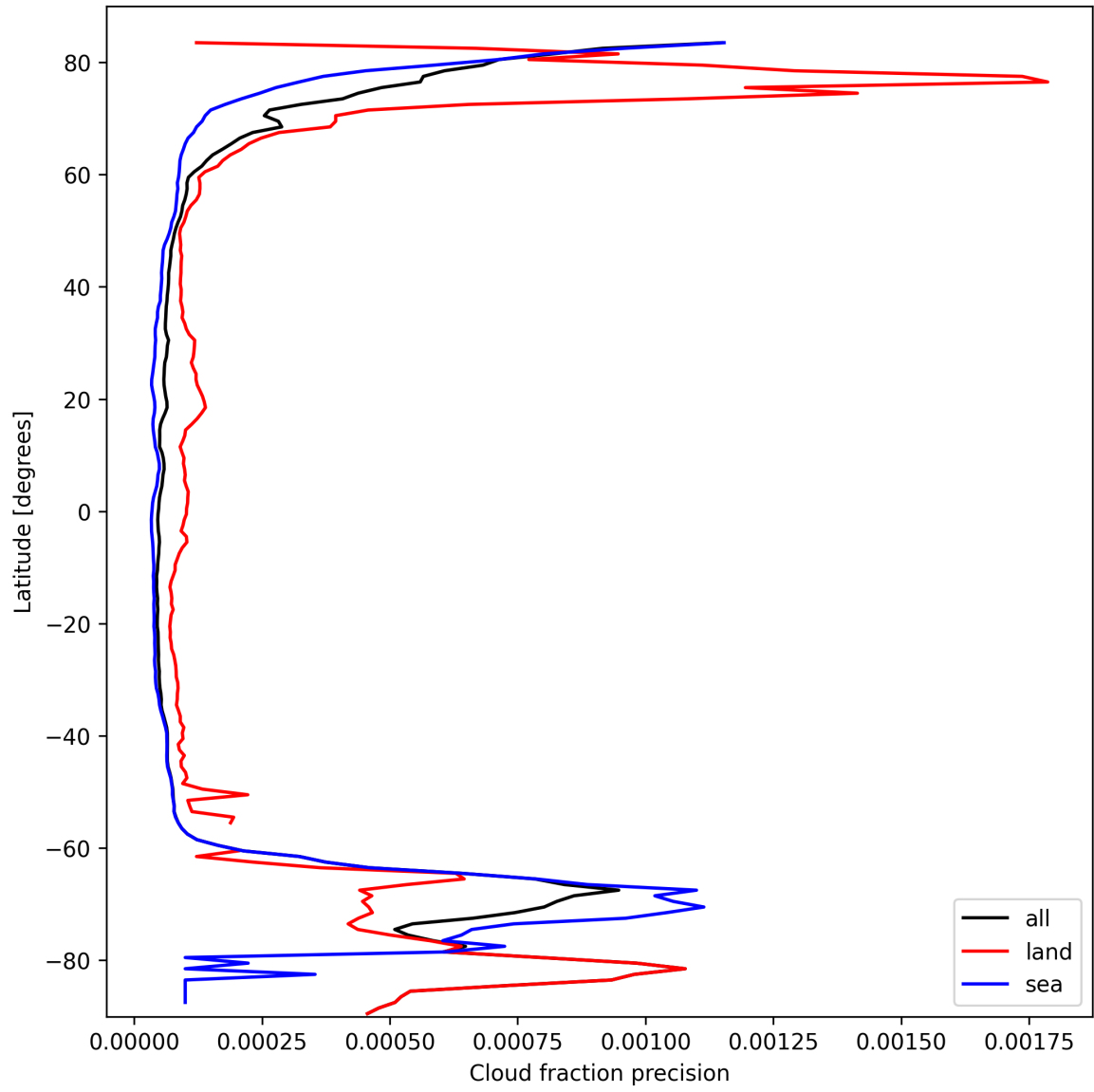
Figure 16: Zonal average of “Cloud fraction precision” for 2025-10-04 to 2025-10-06.
