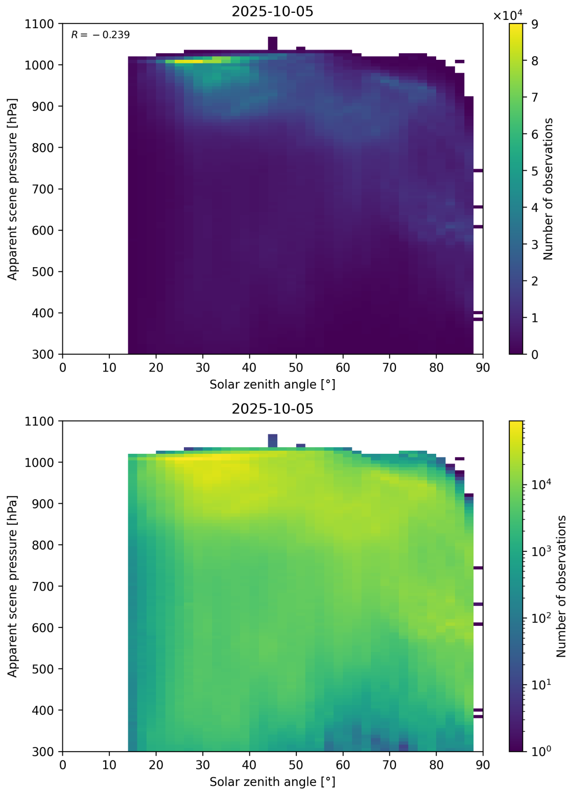
Figure 108: Scatter density plot of “Solar zenith angle” against “Apparent scene pressure” for 2025-10-04 to 2025-10-06.
