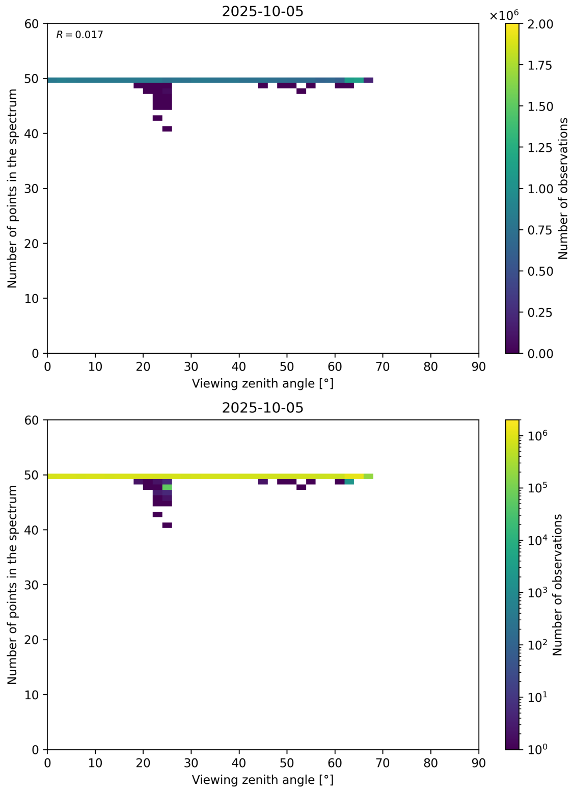
Figure 125: Scatter density plot of “Viewing zenith angle” against “Number of points in the spectrum” for 2025-10-04 to 2025-10-06.
