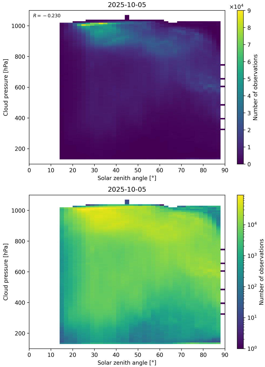
Figure 111: Scatter density plot of “Solar zenith angle” against “Cloud pressure” for 2025-10-04 to 2025-10-06.
