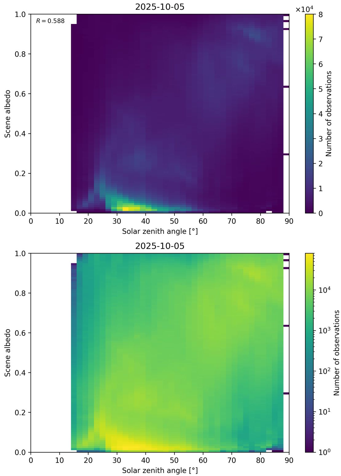
Figure 116: Scatter density plot of “Solar zenith angle” against “Scene albedo” for 2025-10-04 to 2025-10-06.
