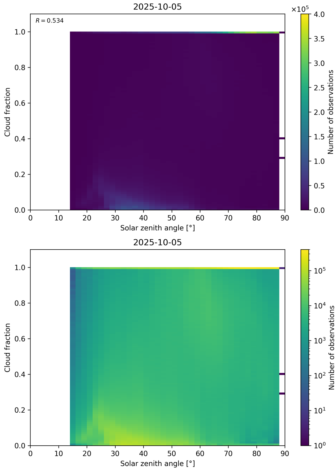
Figure 110: Scatter density plot of “Solar zenith angle” against “Cloud fraction” for 2025-10-04 to 2025-10-06.
