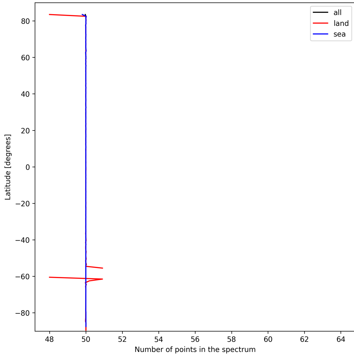
Figure 27: Zonal average of “Number of points in the spectrum” for 2025-10-04 to 2025-10-06.
