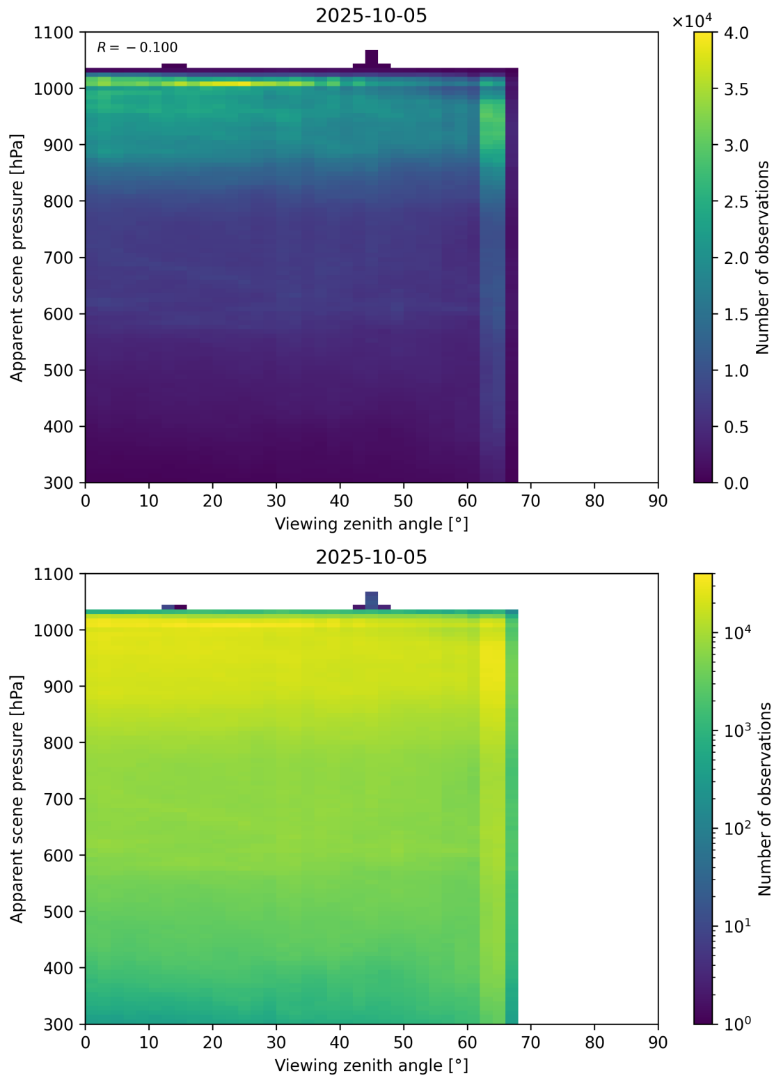
Figure 118: Scatter density plot of “Viewing zenith angle” against “Apparent scene pressure” for 2025-10-04 to 2025-10-06.
