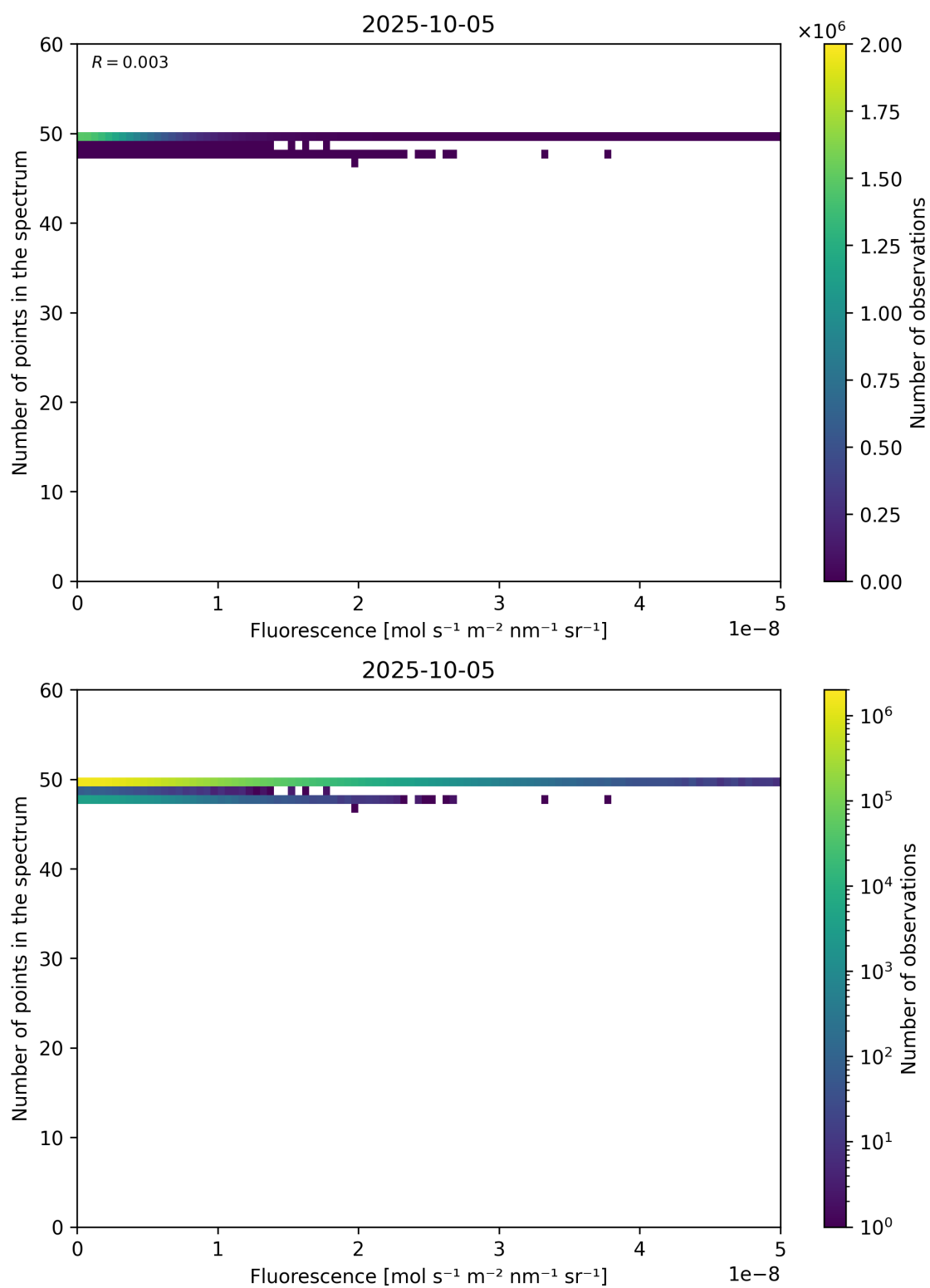
Figure 86: Scatter density plot of “Fluorescence” against “Number of points in the spectrum” for 2025-10-04 to 2025-10-06.
