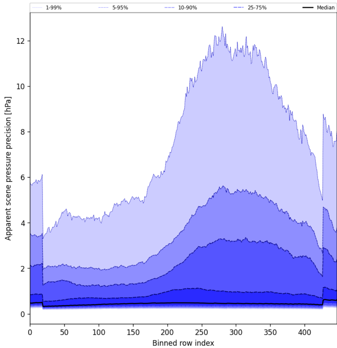
Figure 54: Along track statistics of “Apparent scene pressure precision” for 2025-10-04 to 2025-10-06
