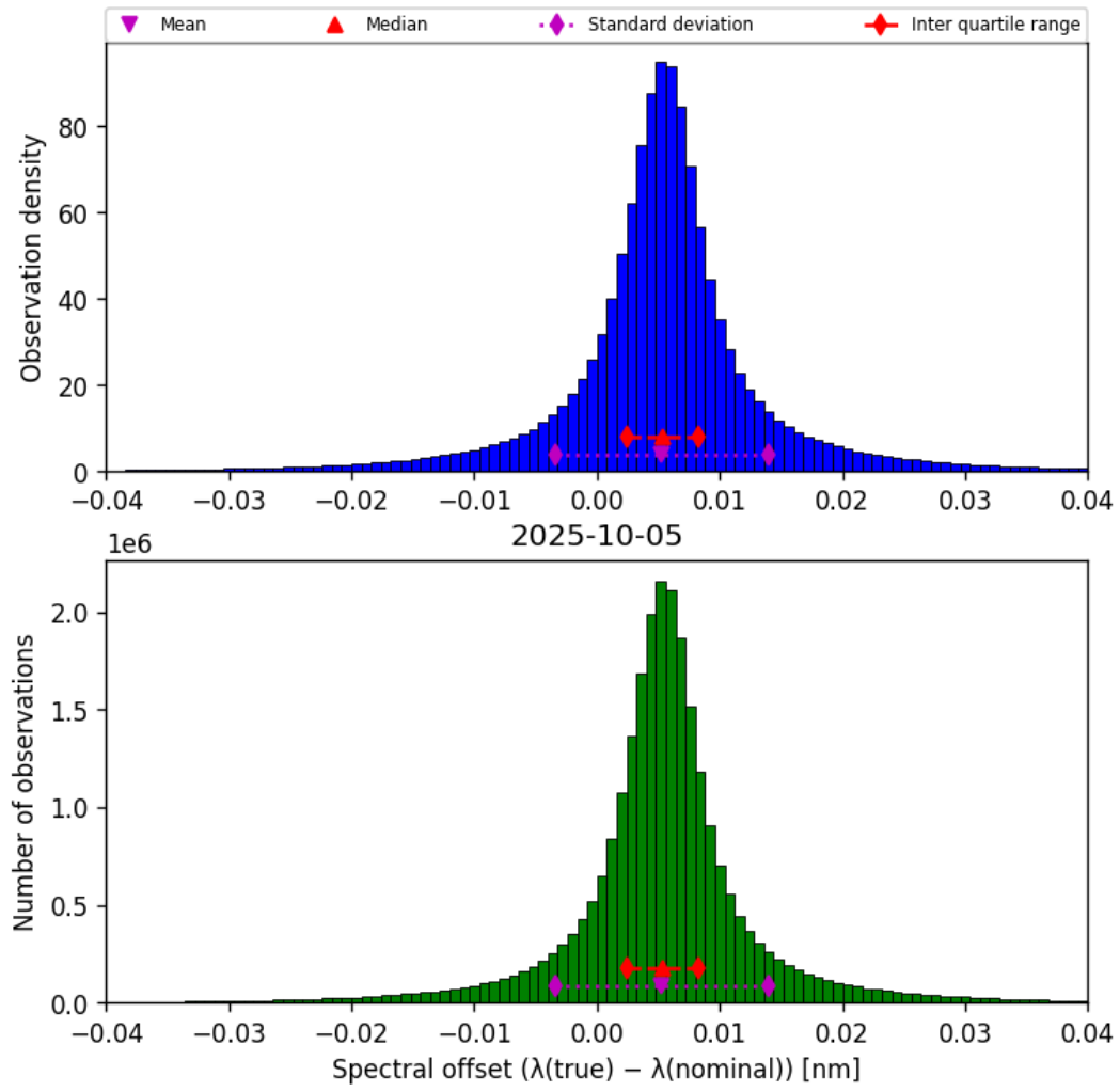
Figure 45: Histogram of “Spectral offset ( \lambda_{\text{true}} - \lambda_{\text{nominal}} )” for 2025-10-04 to 2025-10-06
