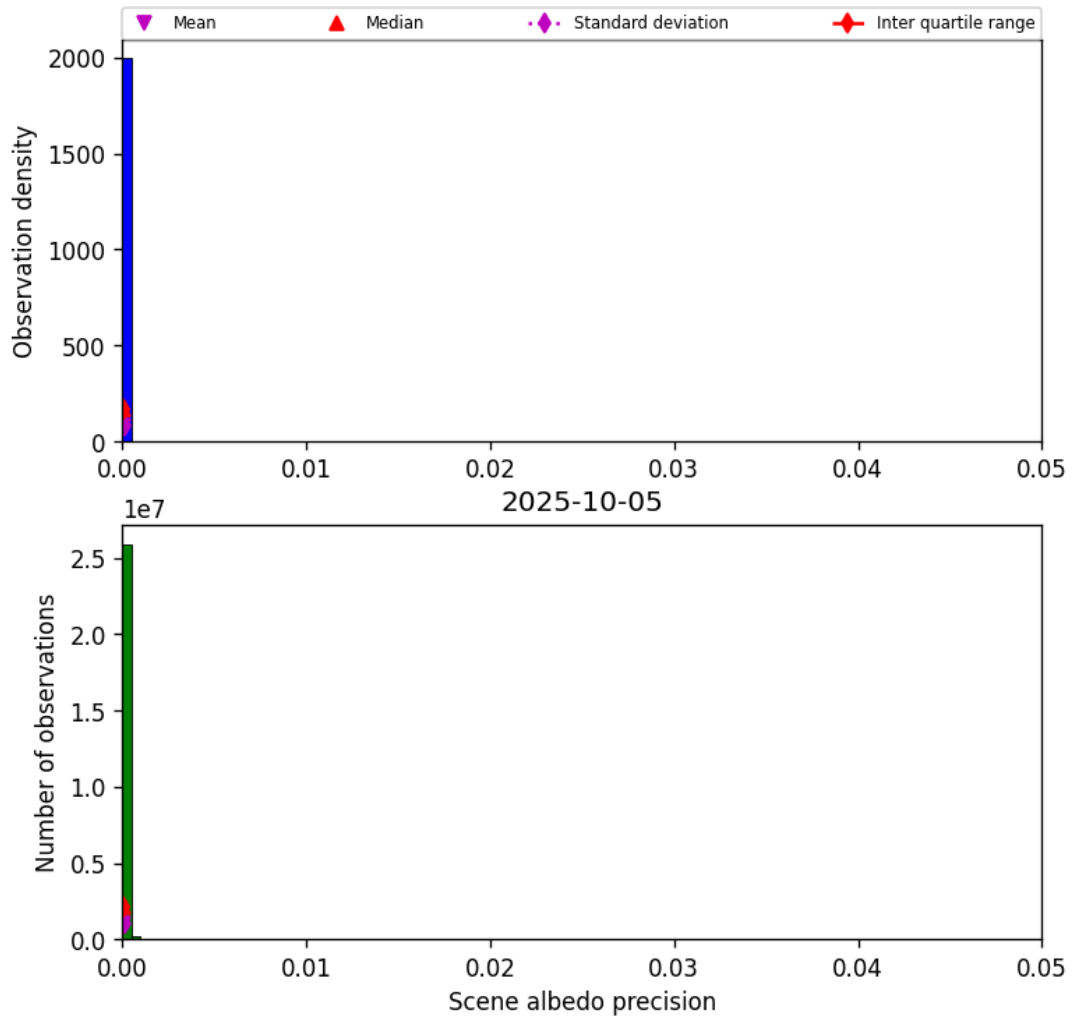
Figure 35: Histogram of “Scene albedo precision” for 2025-10-04 to 2025-10-06
