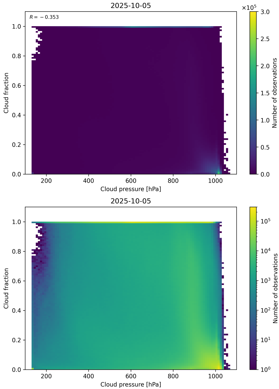
Figure 79: Scatter density plot of “Cloud pressure” against “Cloud fraction” for 2025-10-04 to 2025-10-06.
