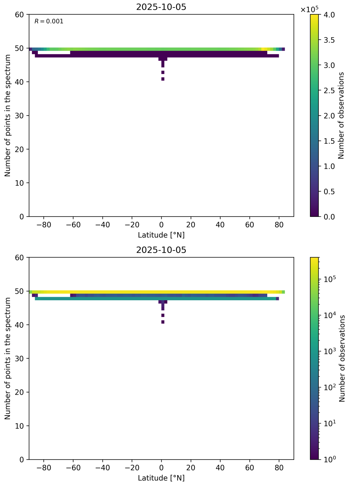
Figure 94: Scatter density plot of “Latitude” against “Number of points in the spectrum” for 2025-10-04 to 2025-10-06.
