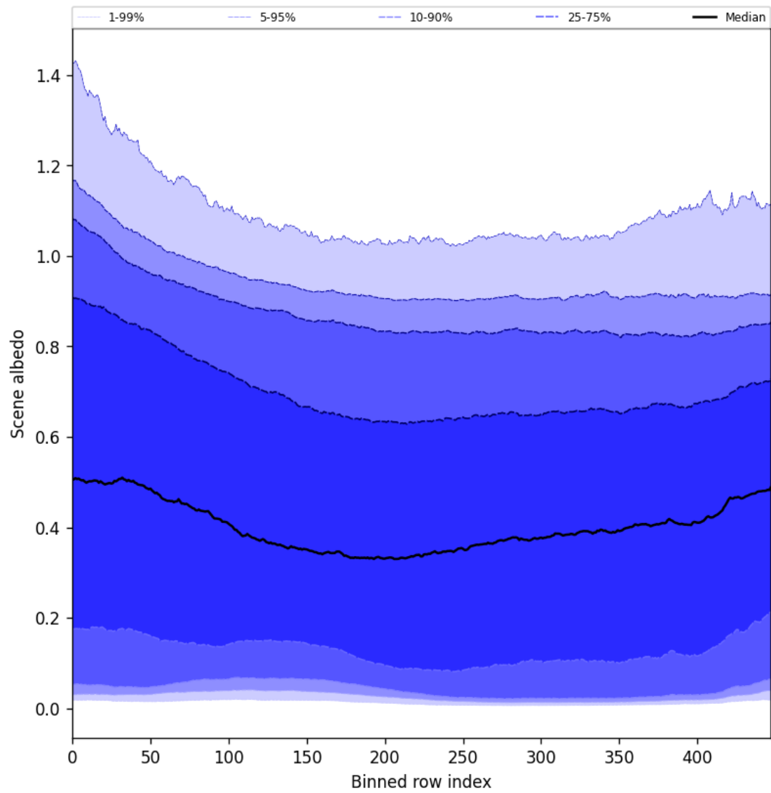
Figure 51: Along track statistics of “Scene albedo” for 2025-10-04 to 2025-10-06
