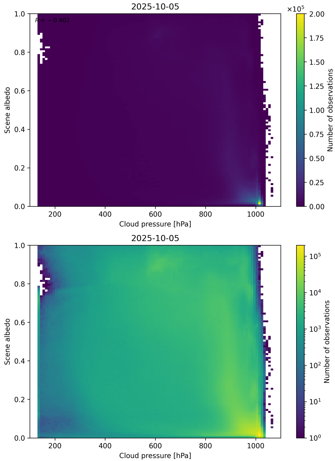
Figure 83: Scatter density plot of “Cloud pressure” against “Scene albedo” for 2025-10-04 to 2025-10-06.
