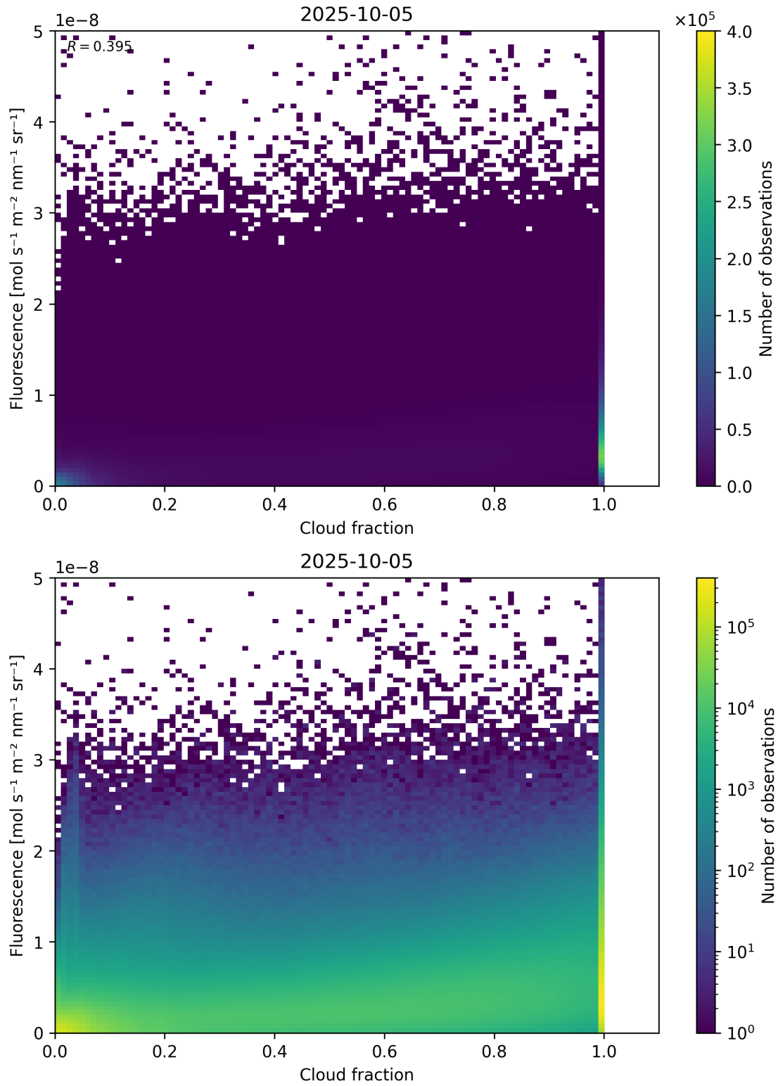
Figure 72: Scatter density plot of “Cloud fraction” against “Fluorescence” for 2025-10-04 to 2025-10-06.
