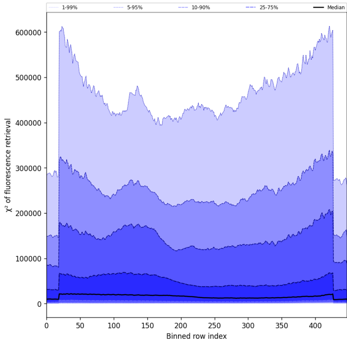
Figure 59: Along track statistics of “ \chi^2 of fluorescence retrieval” for 2025-10-04 to 2025-10-06
