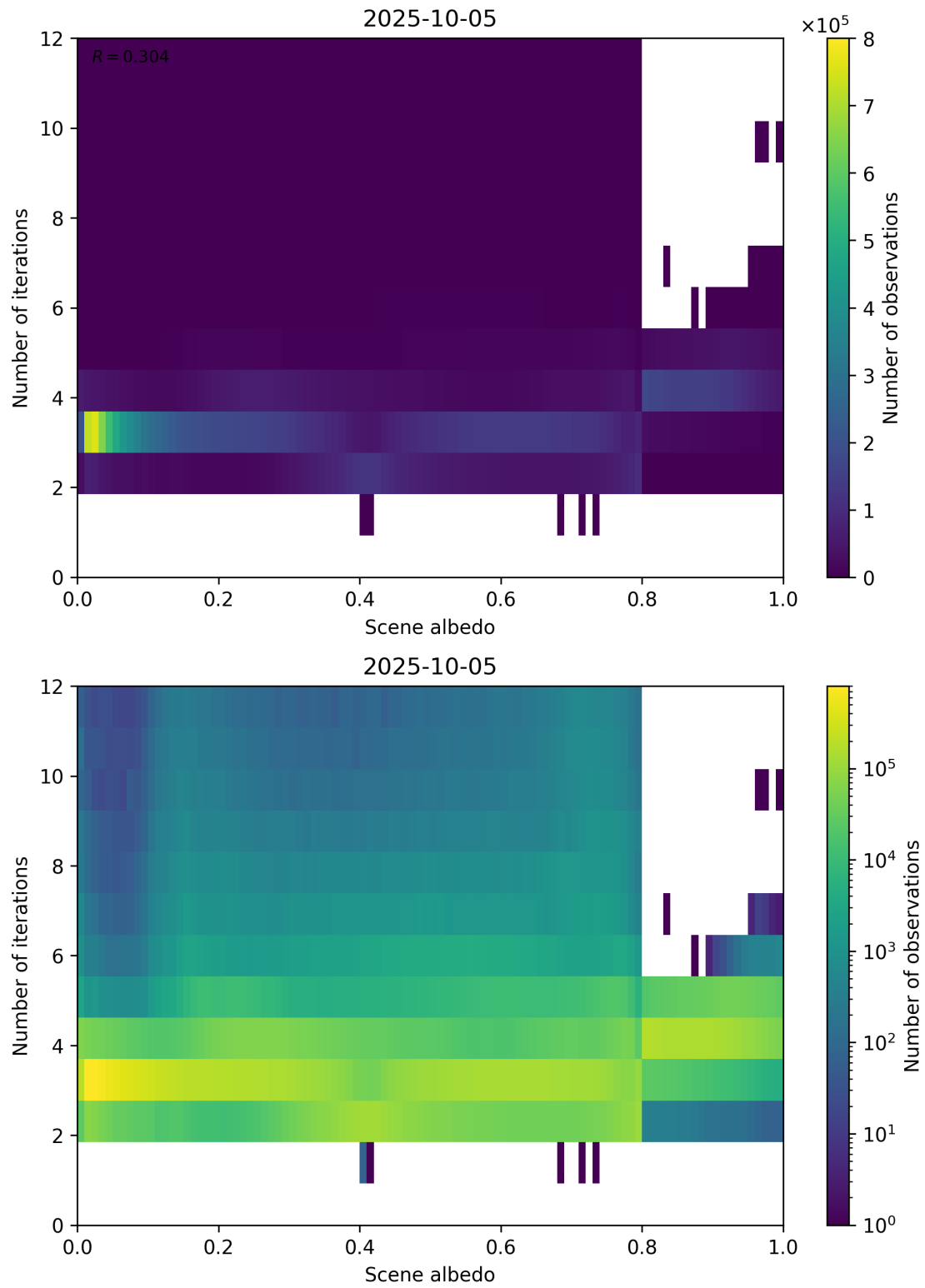
Figure 105: Scatter density plot of “Scene albedo” against “Number of iterations” for 2025-10-04 to 2025-10-06.
