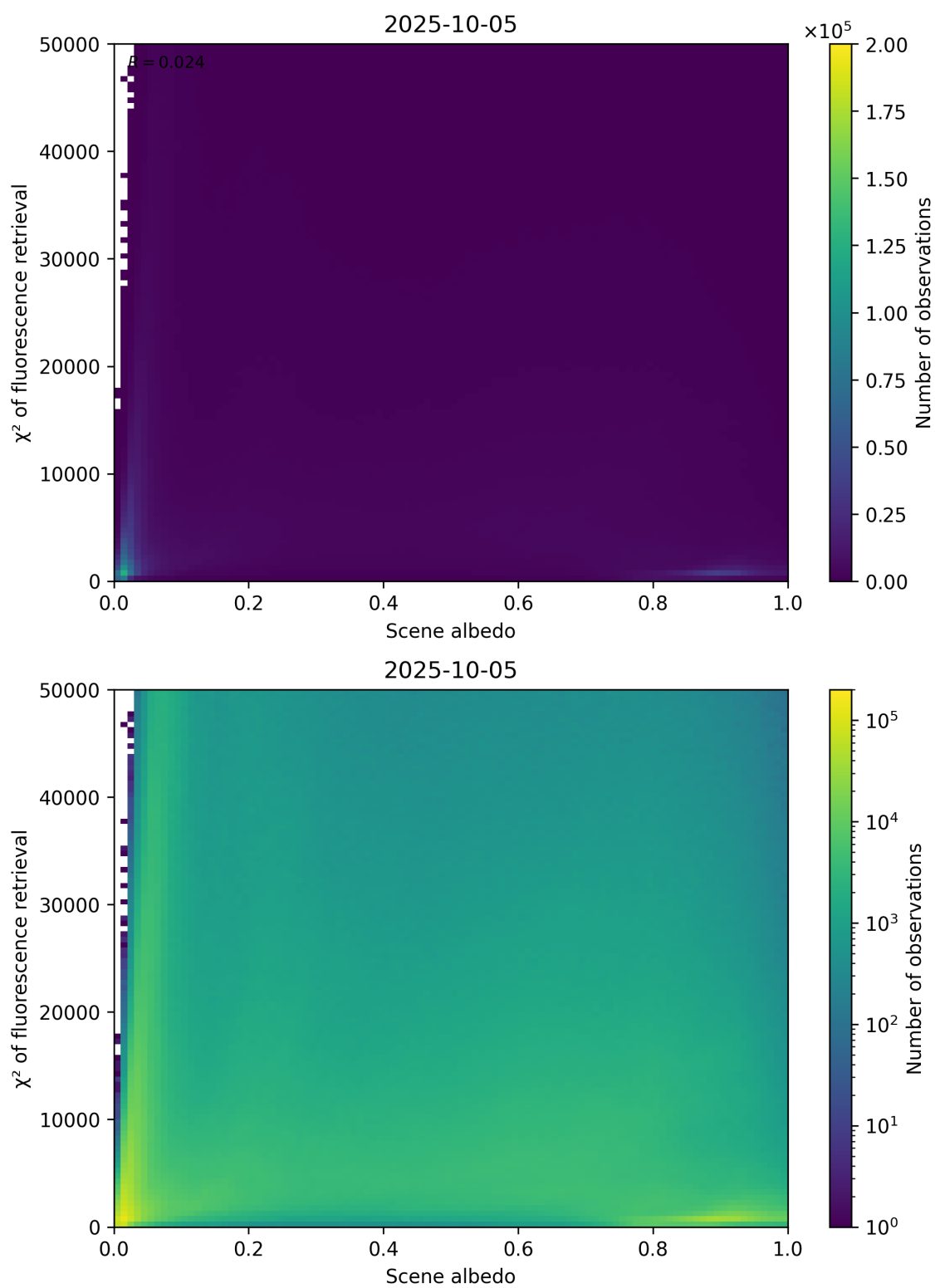
Figure 103: Scatter density plot of “Scene albedo” against “ \chi^2 of fluorescence retrieval” for 2025-10-04 to 2025-10-06.
