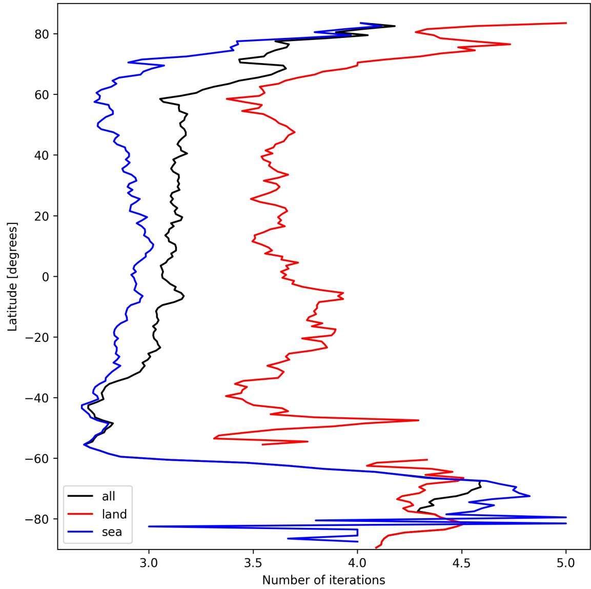
Figure 22: Zonal average of “Number of iterations” for 2025-10-04 to 2025-10-06.
