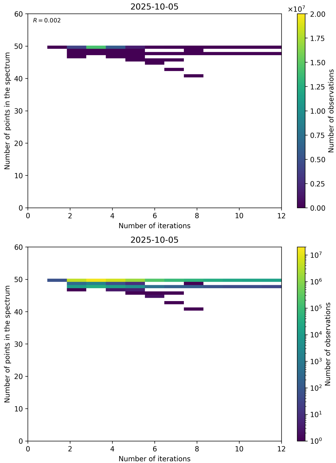
Figure 99: Scatter density plot of “Number of iterations” against “Number of points in the spectrum” for 2025-10-04 to 2025-10-06.
