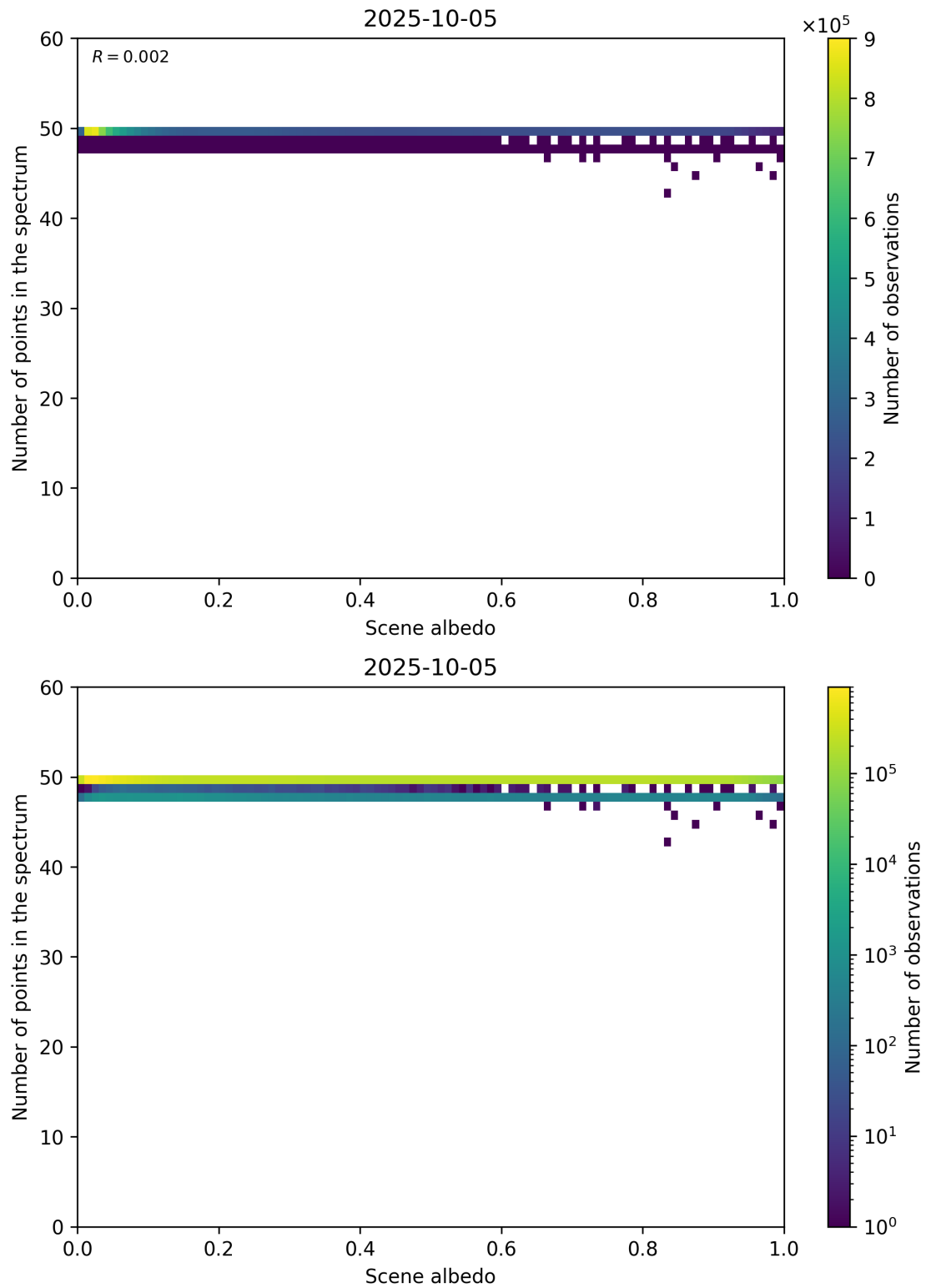
Figure 106: Scatter density plot of “Scene albedo” against “Number of points in the spectrum” for 2025-10-04 to 2025-10-06.
