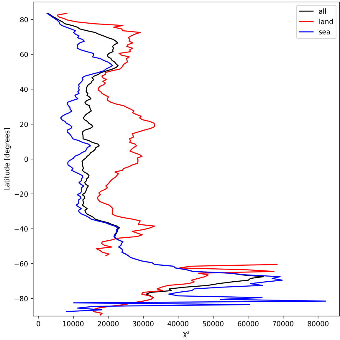
Figure 21: Zonal average of “ \chi^2 ” for 2025-10-04 to 2025-10-06.
