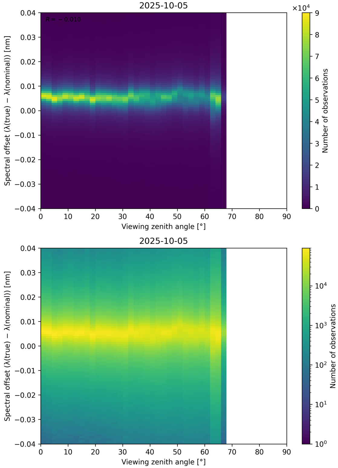
Figure 128: Scatter density plot of “Viewing zenith angle” against “Spectral offset ( \lambda_{\text{true}} - \lambda_{\text{nominal}} )” for 2025-10-04 to 2025-10-06.
