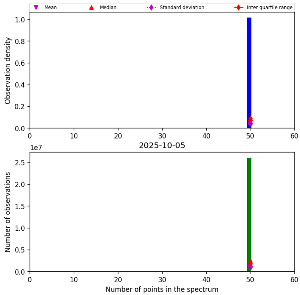
Figure 44: Histogram of “Number of points in the spectrum” for 2025-10-04 to 2025-10-06
