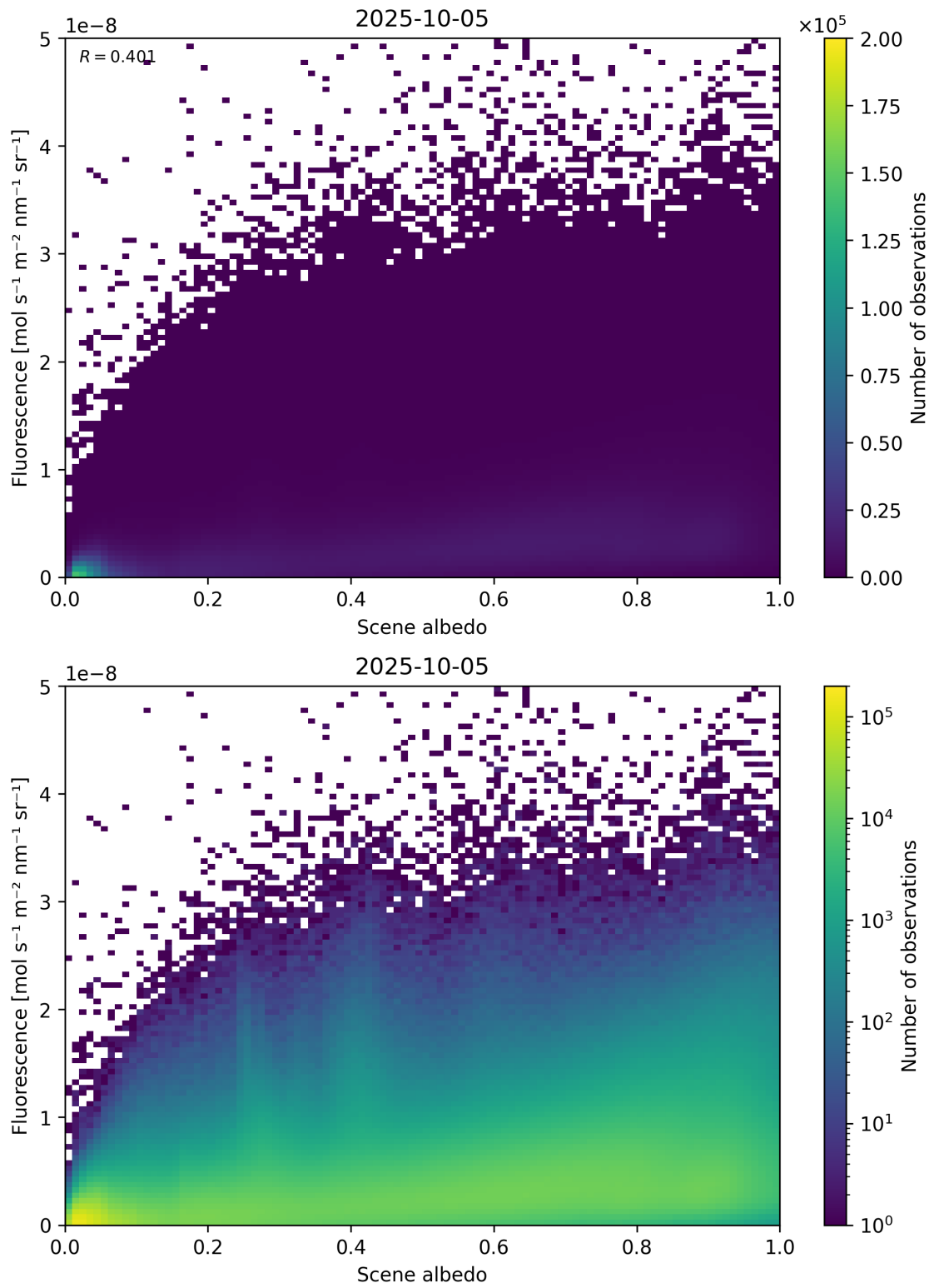
Figure 104: Scatter density plot of “Scene albedo” against “Fluorescence” for 2025-10-04 to 2025-10-06.
