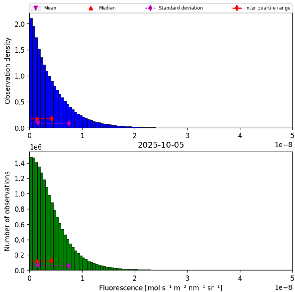
Figure 40: Histogram of “Fluorescence” for 2025-10-04 to 2025-10-06
