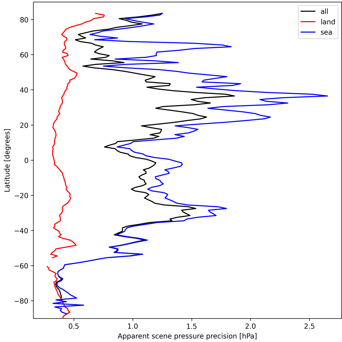
Figure 20: Zonal average of “Apparent scene pressure precision” for 2025-10-04 to 2025-10-06.
