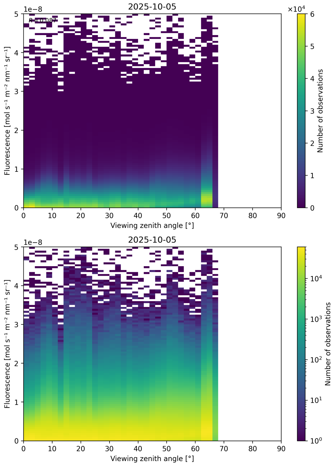
Figure 122: Scatter density plot of “Viewing zenith angle” against “Fluorescence” for 2025-10-04 to 2025-10-06.
