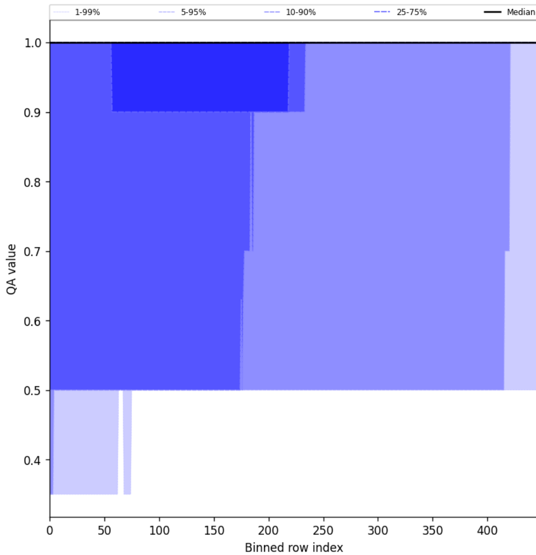
Figure 46: Along track statistics of “QA value” for 2025-10-04 to 2025-10-06
