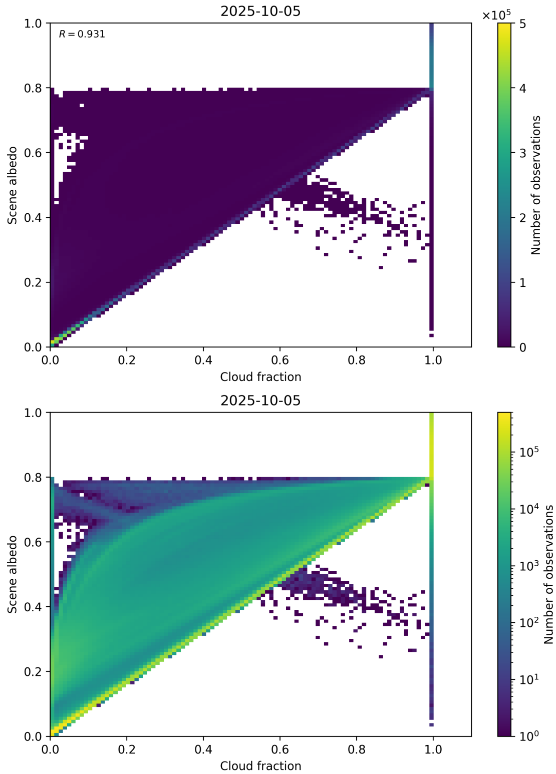
Figure 75: Scatter density plot of “Cloud fraction” against “Scene albedo” for 2025-10-04 to 2025-10-06.
