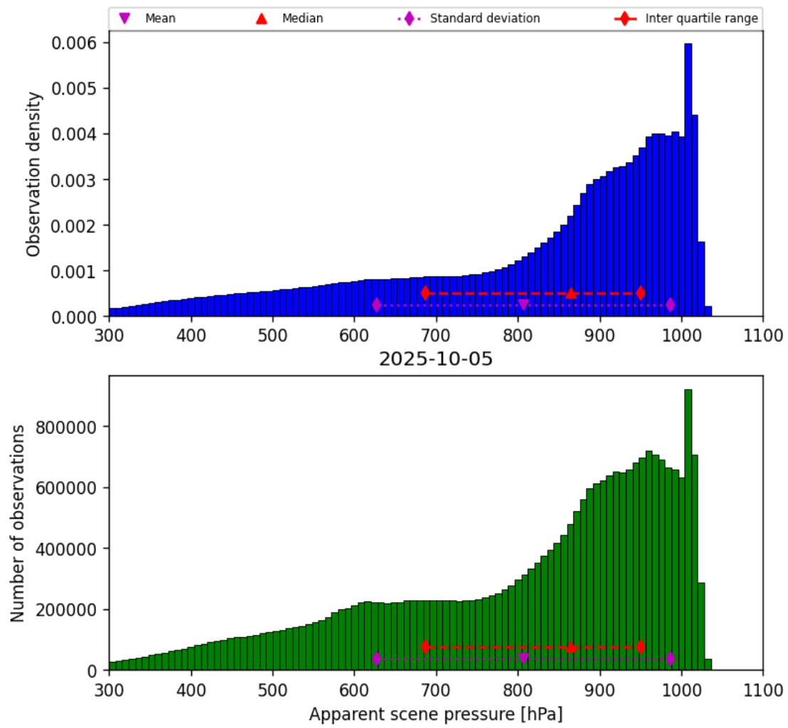
Figure 36: Histogram of “Apparent scene pressure” for 2025-10-04 to 2025-10-06
