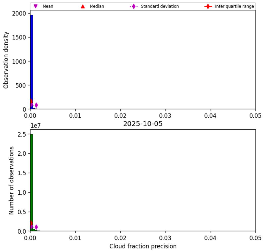
Figure 33: Histogram of “Cloud fraction precision” for 2025-10-04 to 2025-10-06
