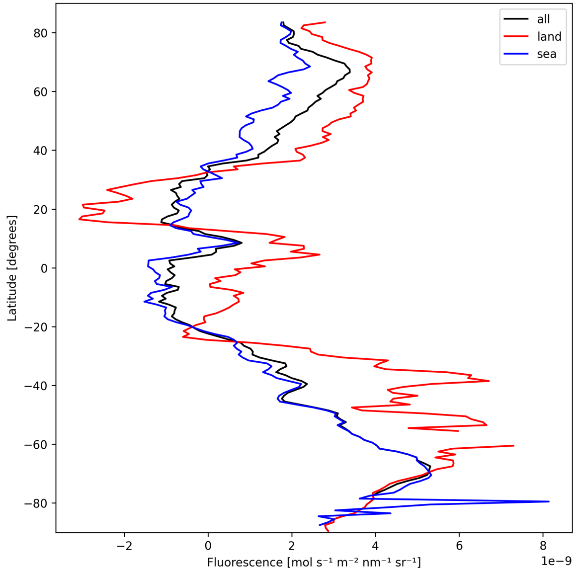
Figure 23: Zonal average of “Fluorescence” for 2025-10-04 to 2025-10-06.
