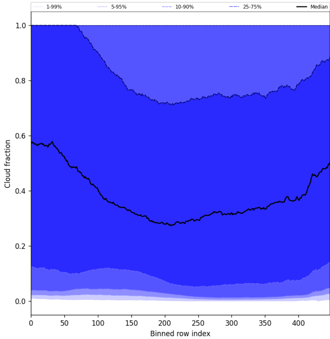
Figure 49: Along track statistics of “Cloud fraction” for 2025-10-04 to 2025-10-06
