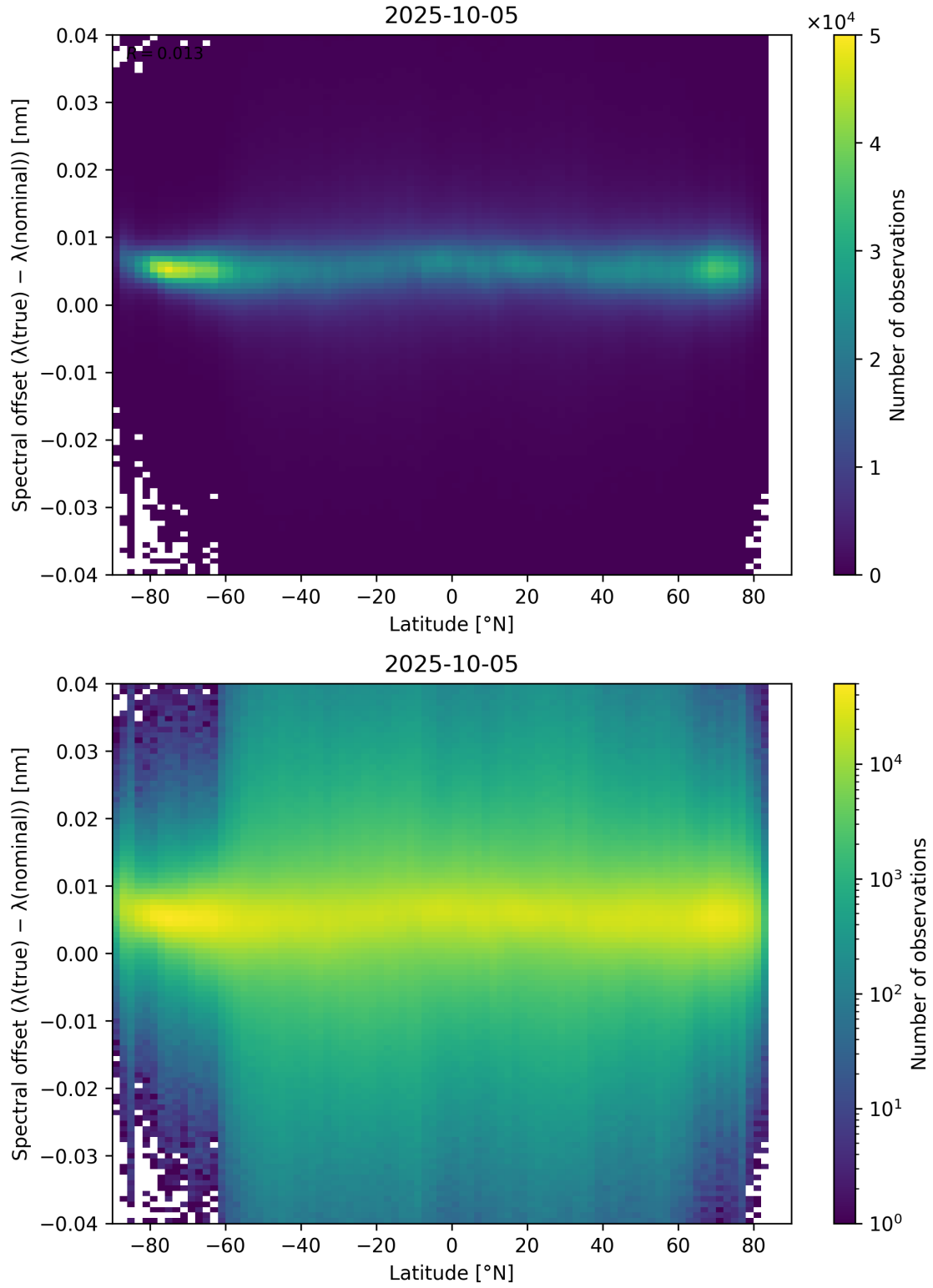
Figure 96: Scatter density plot of “Latitude” against “Spectral offset ( \lambda_{\text{true}} - \lambda_{\text{nominal}} )” for 2025-10-04 to 2025-10-06.
