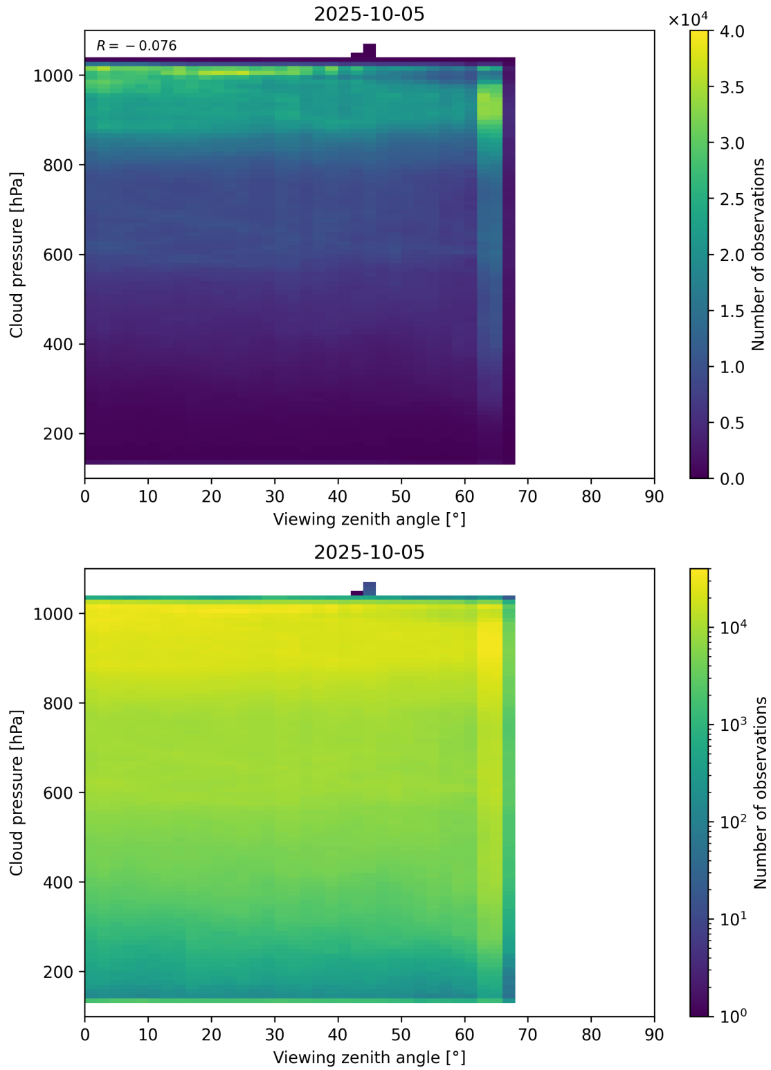
Figure 121: Scatter density plot of “Viewing zenith angle” against “Cloud pressure” for 2025-10-04 to 2025-10-06.
