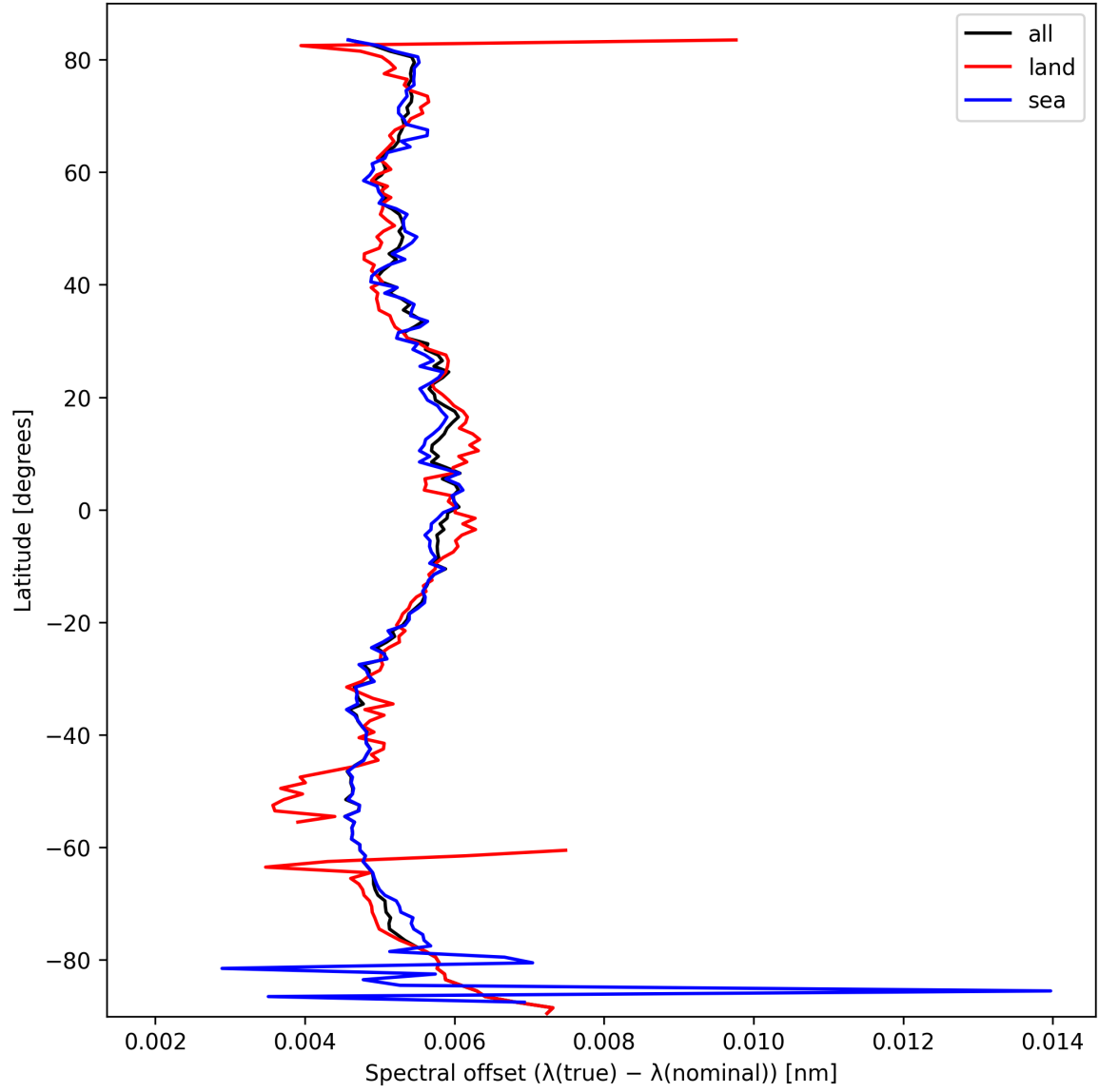
Figure 28: Zonal average of “Spectral offset ( \lambda_{\text{true}} - \lambda_{\text{nominal}} )” for 2025-10-04 to 2025-10-06.
