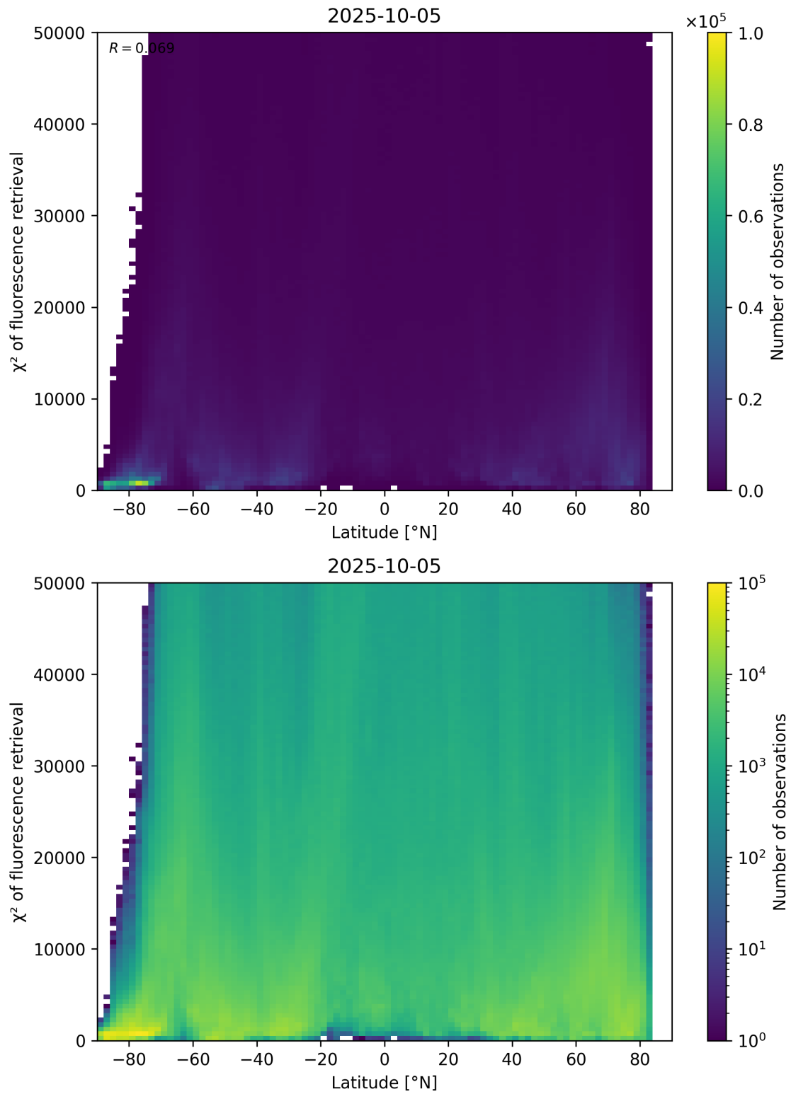
Figure 89: Scatter density plot of “Latitude” against “ \chi^2 of fluorescence retrieval” for 2025-10-04 to 2025-10-06.
