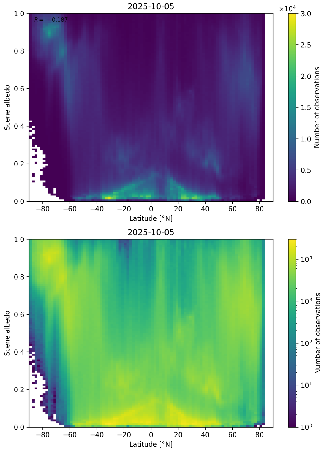
Figure 95: Scatter density plot of “Latitude” against “Scene albedo” for 2025-10-04 to 2025-10-06.
