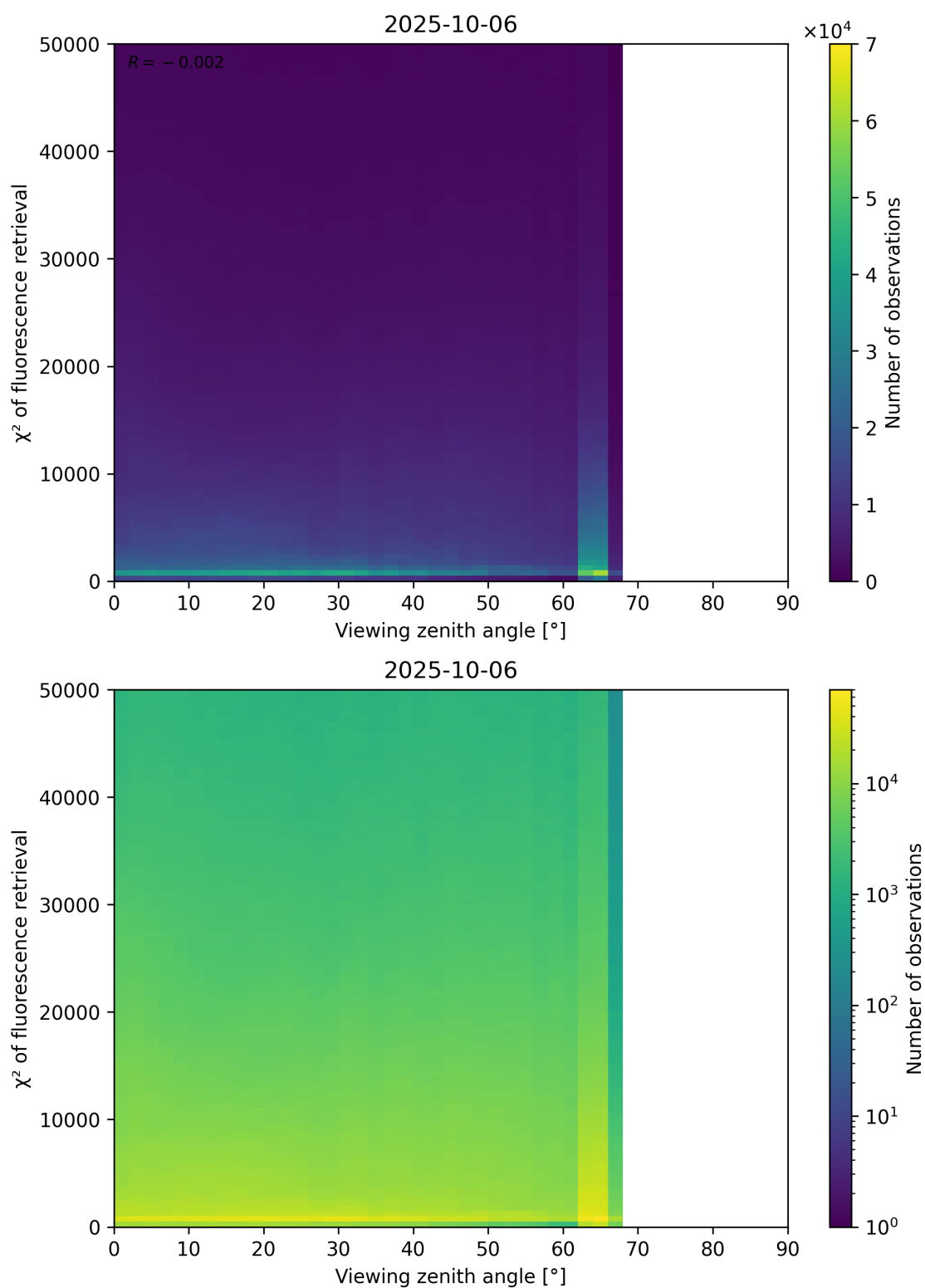
Figure 119: Scatter density plot of “Viewing zenith angle” against “ \chi^2 of fluorescence retrieval” for 2025-10-06 to 2025-10-07.
