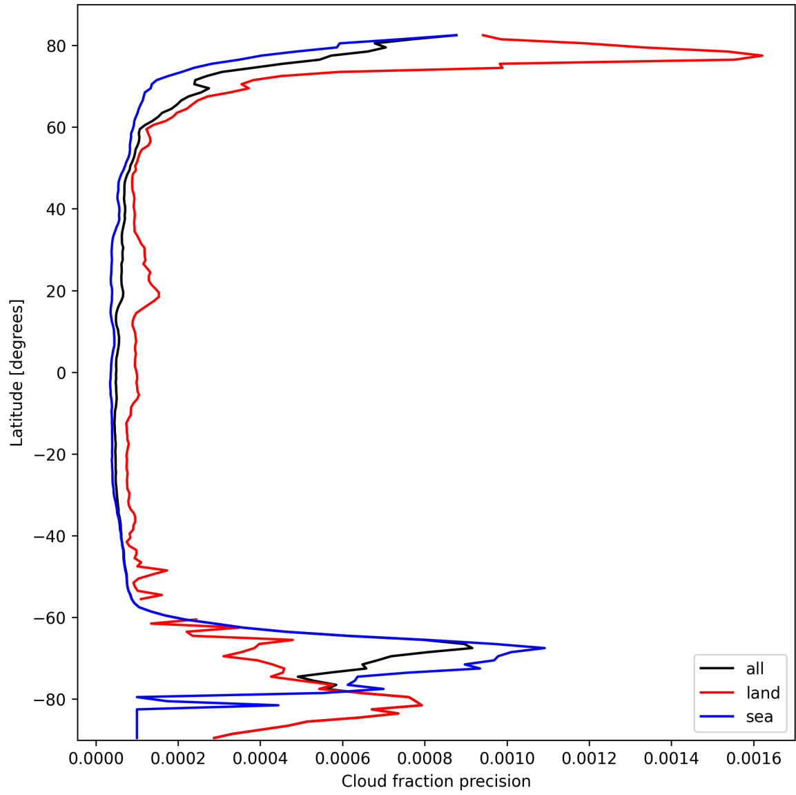
Figure 16: Zonal average of “Cloud fraction precision” for 2025-10-06 to 2025-10-07.
