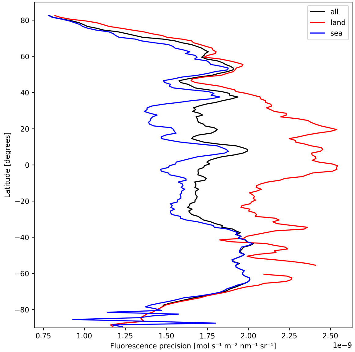
Figure 24: Zonal average of “Fluorescence precision” for 2025-10-06 to 2025-10-07.
