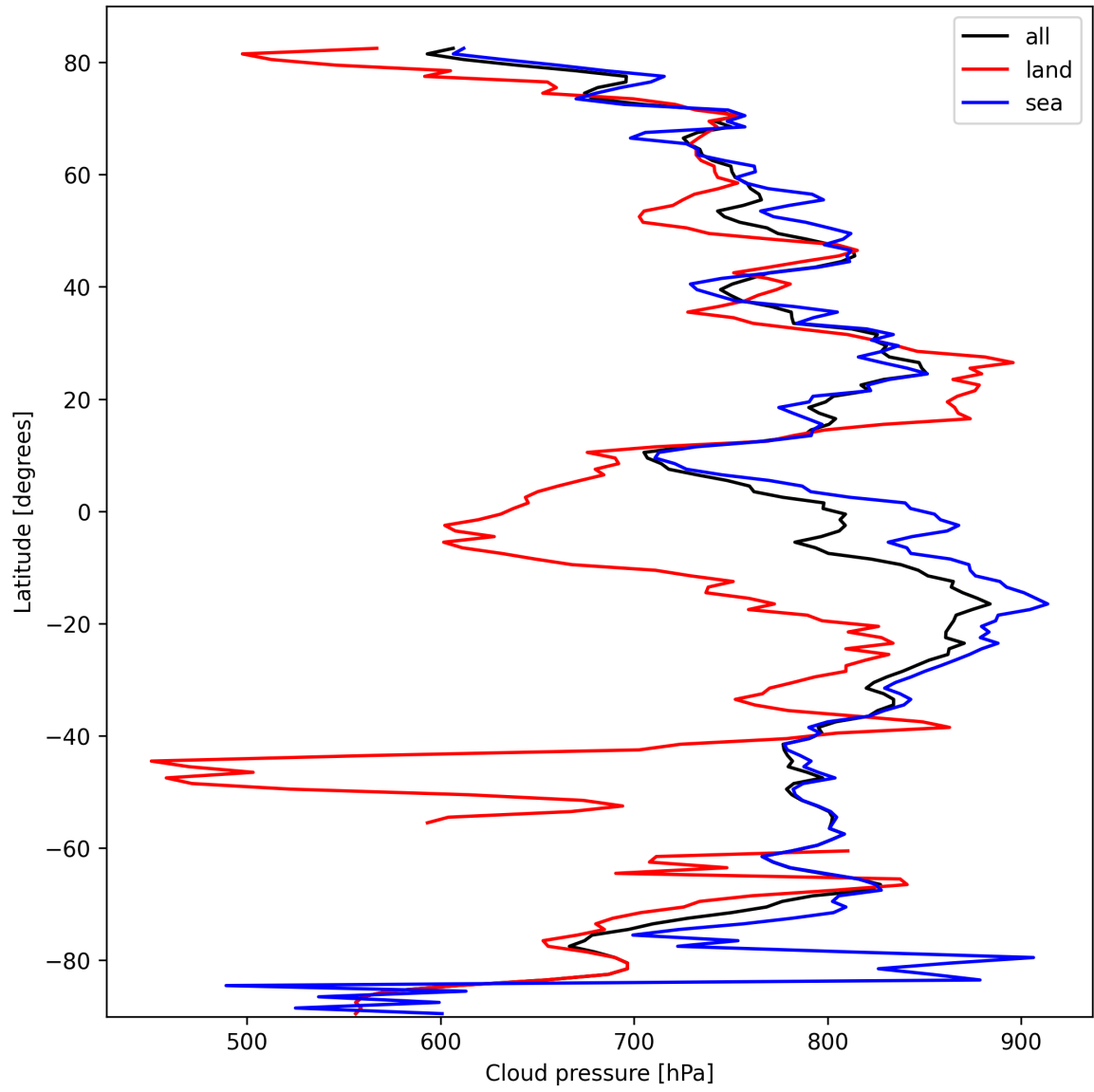
Figure 13: Zonal average of “Cloud pressure” for 2025-10-06 to 2025-10-07.
