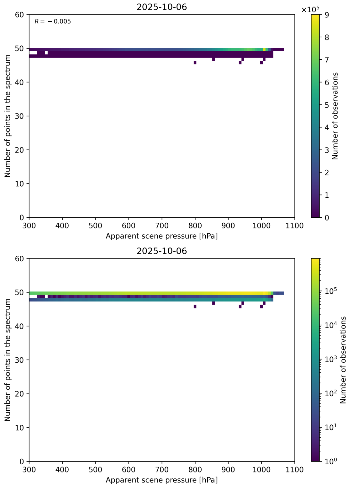
Figure 66: Scatter density plot of “Apparent scene pressure” against “Number of points in the spectrum” for 2025-10-06 to 2025-10-07.
