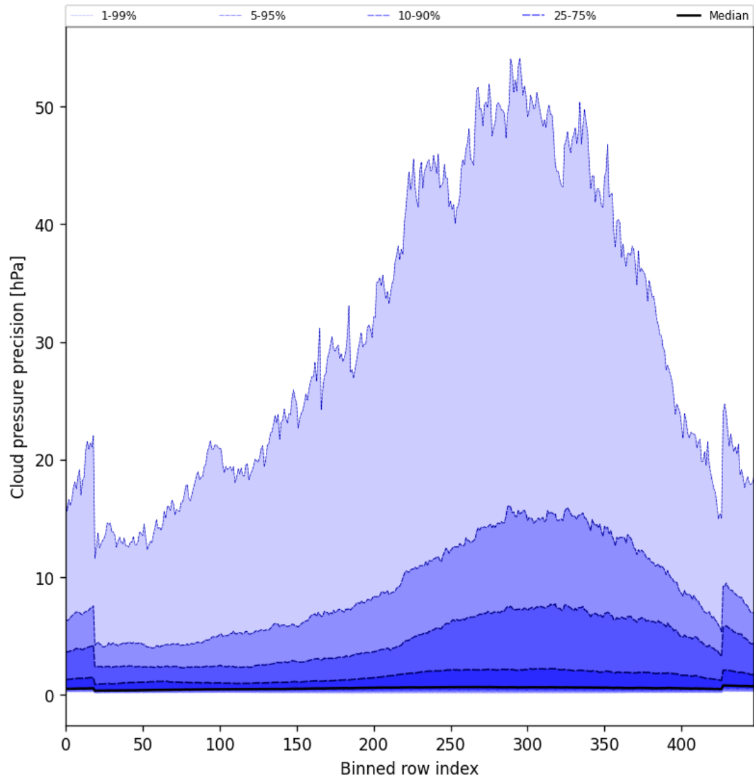
Figure 48: Along track statistics of “Cloud pressure precision” for 2025-10-06 to 2025-10-07
