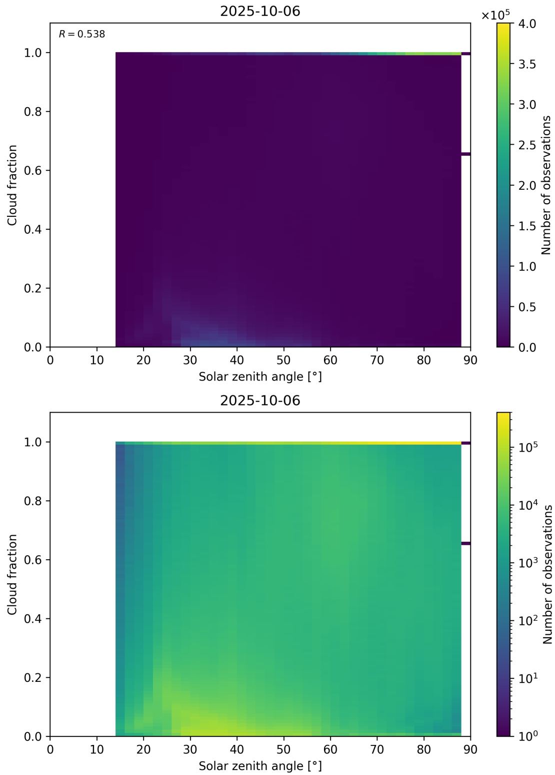
Figure 110: Scatter density plot of “Solar zenith angle” against “Cloud fraction” for 2025-10-06 to 2025-10-07.
