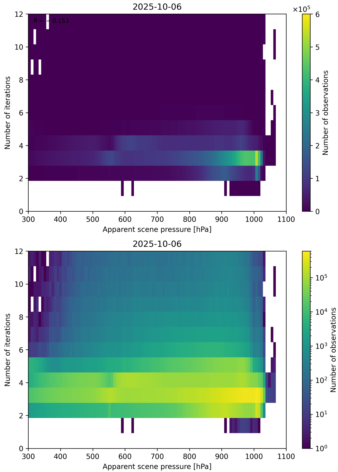
Figure 65: Scatter density plot of “Apparent scene pressure” against “Number of iterations” for 2025-10-06 to 2025-10-07.
