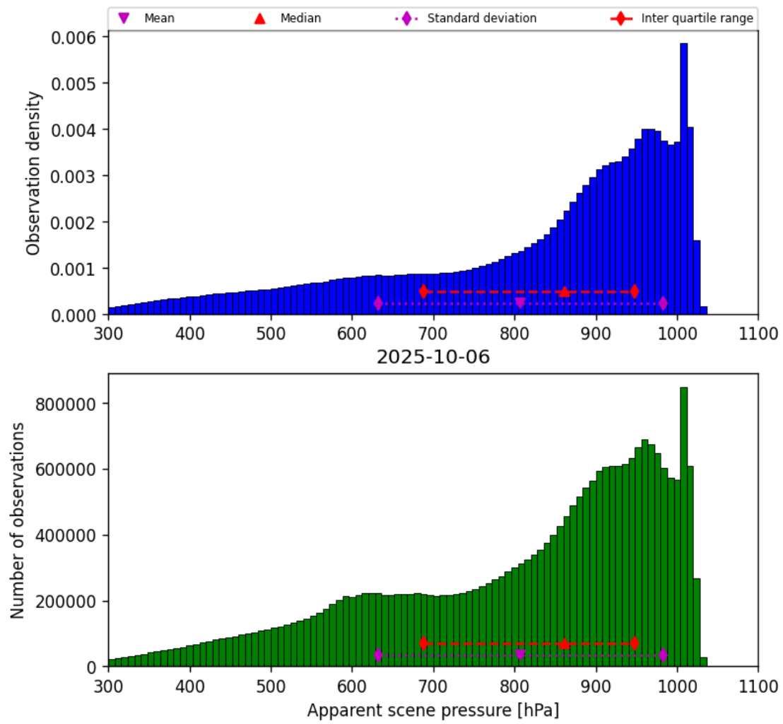
Figure 36: Histogram of “Apparent scene pressure” for 2025-10-06 to 2025-10-07
