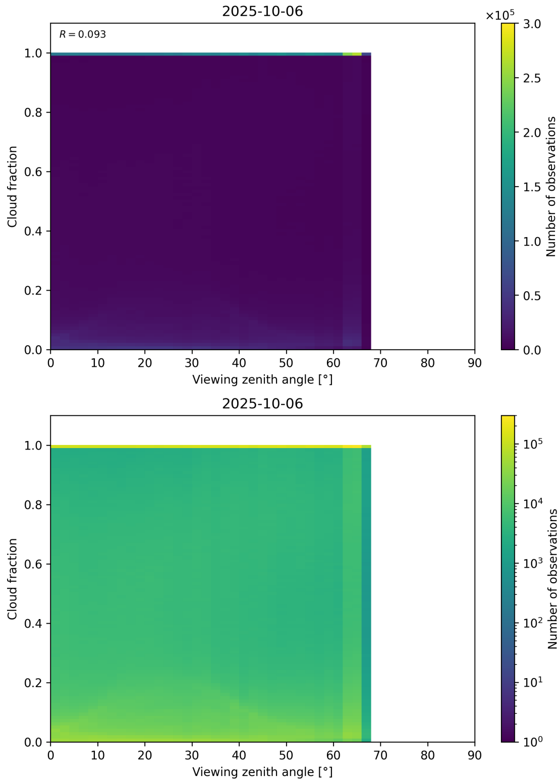
Figure 120: Scatter density plot of “Viewing zenith angle” against “Cloud fraction” for 2025-10-06 to 2025-10-07.
