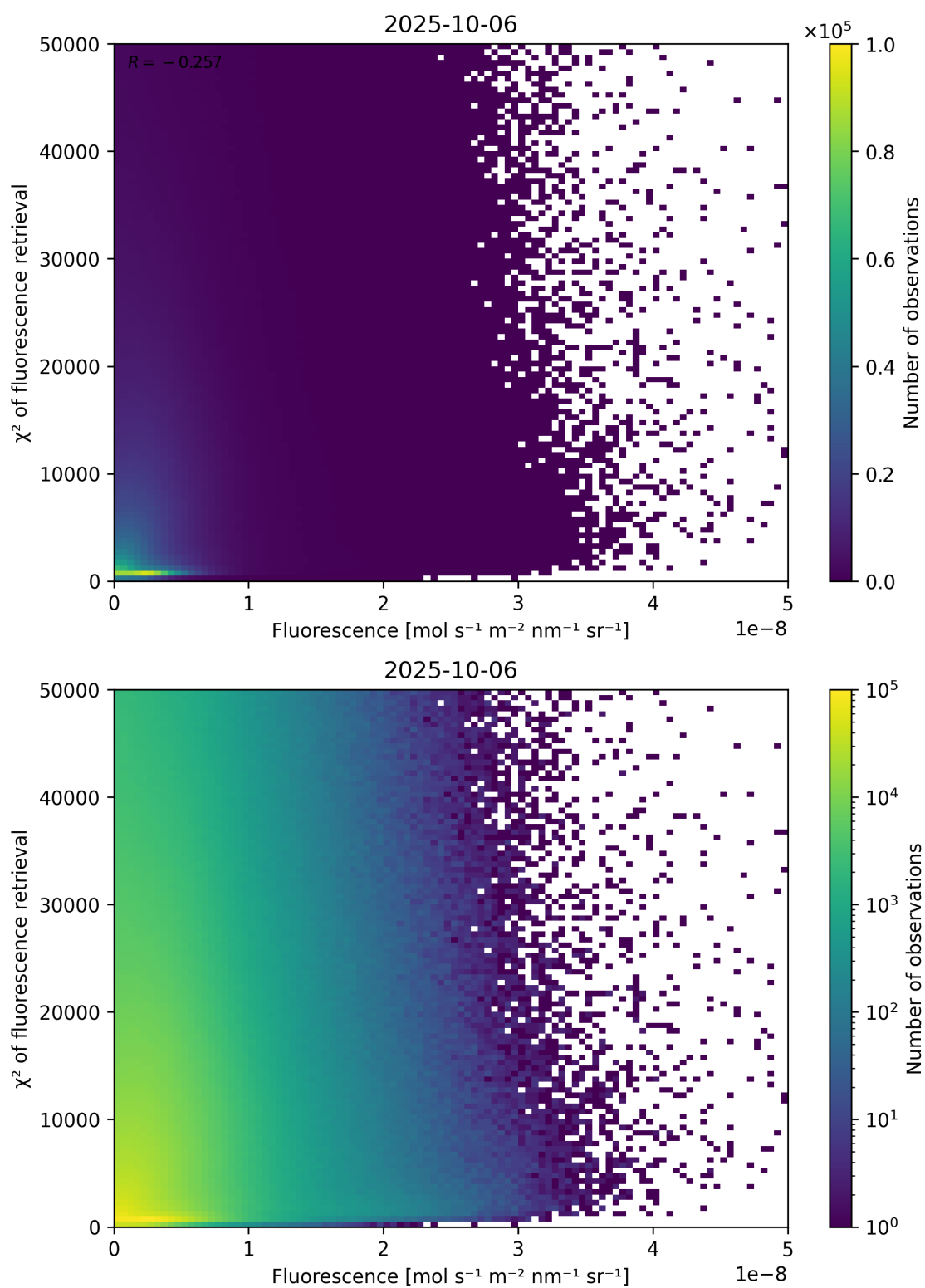
Figure 85: Scatter density plot of “Fluorescence” against “ \chi^2 of fluorescence retrieval” for 2025-10-06 to 2025-10-07.
