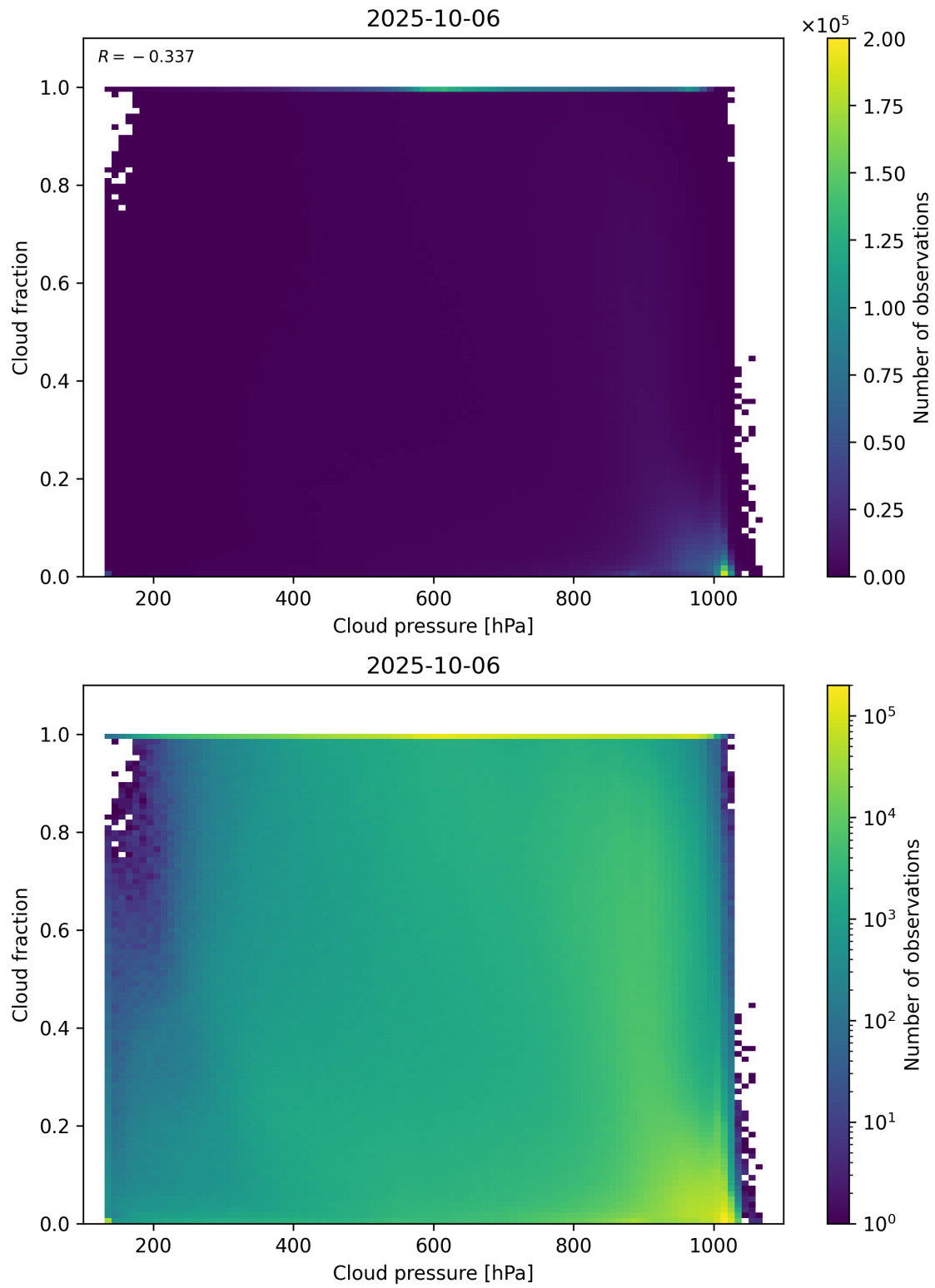
Figure 79: Scatter density plot of “Cloud pressure” against “Cloud fraction” for 2025-10-06 to 2025-10-07.
