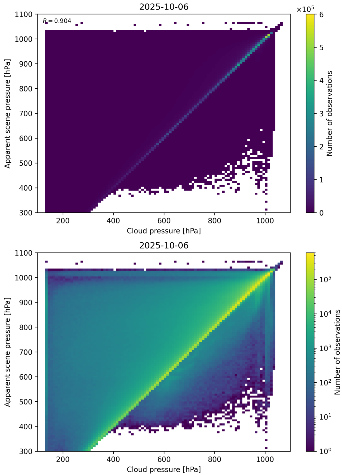
Figure 77: Scatter density plot of “Cloud pressure” against “Apparent scene pressure” for 2025-10-06 to 2025-10-07.
