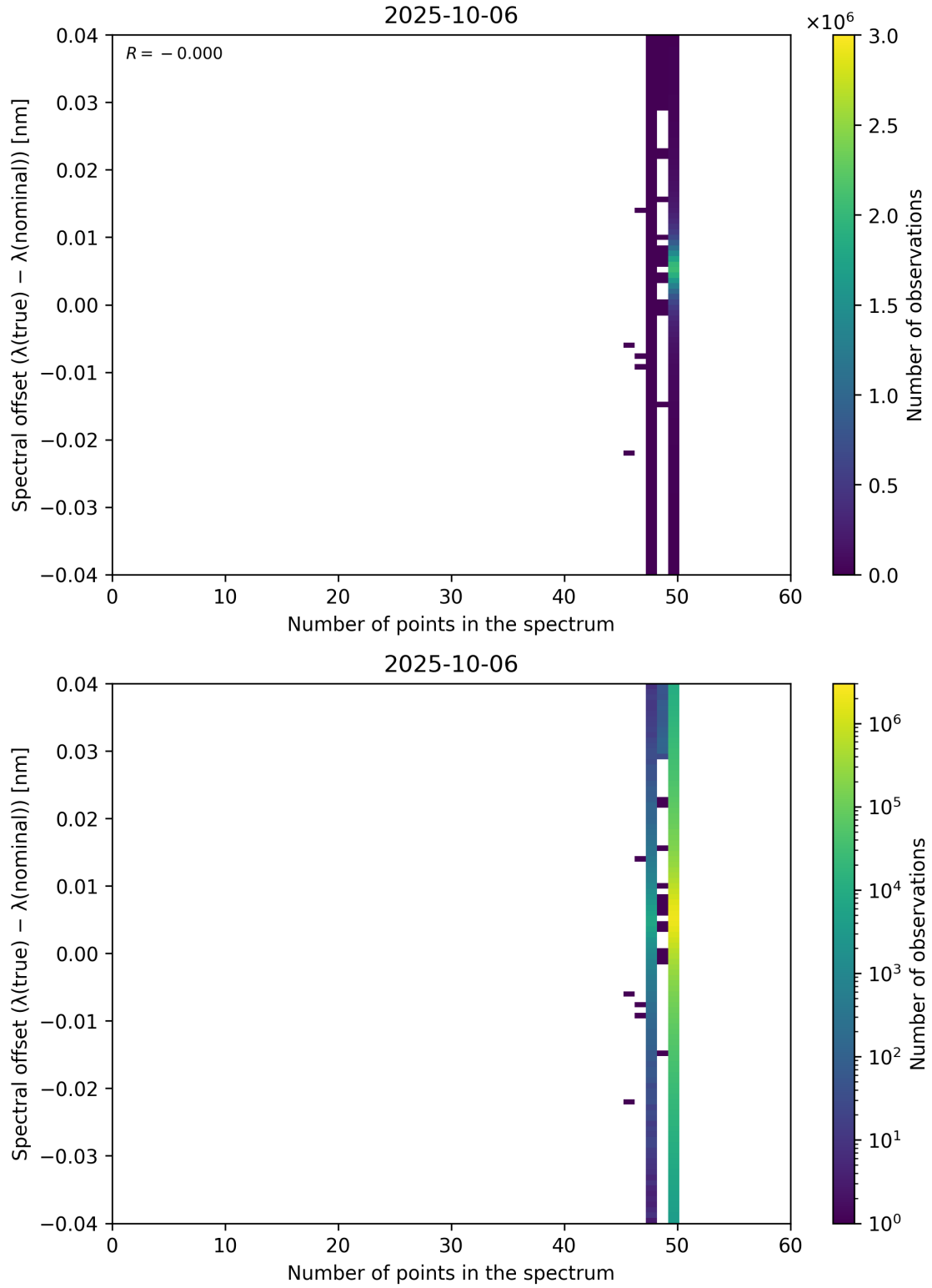
Figure 101: Scatter density plot of “Number of points in the spectrum” against “Spectral offset ( \lambda_{\text{true}} - \lambda_{\text{nominal}} )” for 2025-10-06 to 2025-10-07.
