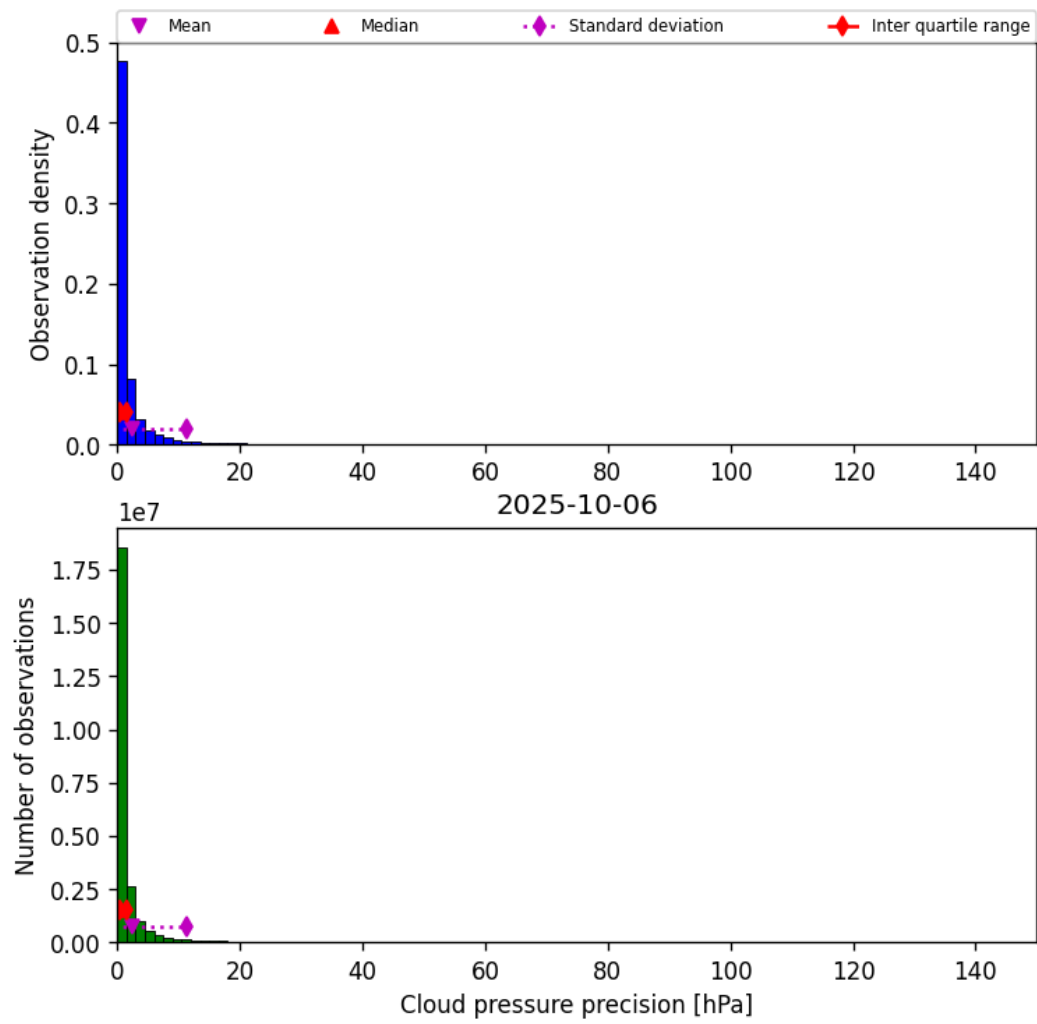
Figure 31: Histogram of “Cloud pressure precision” for 2025-10-06 to 2025-10-07
