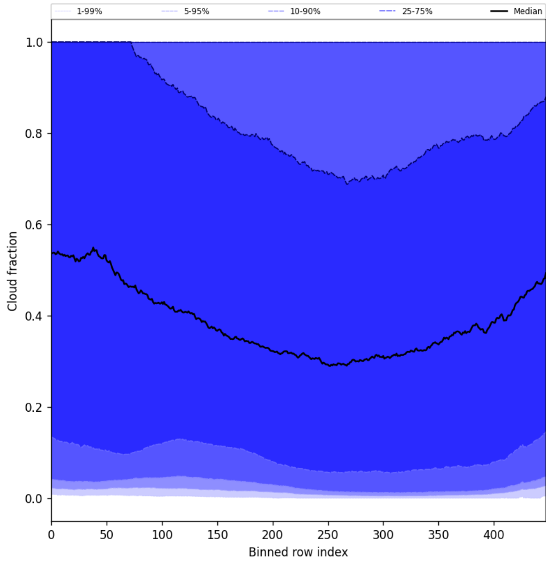
Figure 49: Along track statistics of “Cloud fraction” for 2025-10-06 to 2025-10-07
