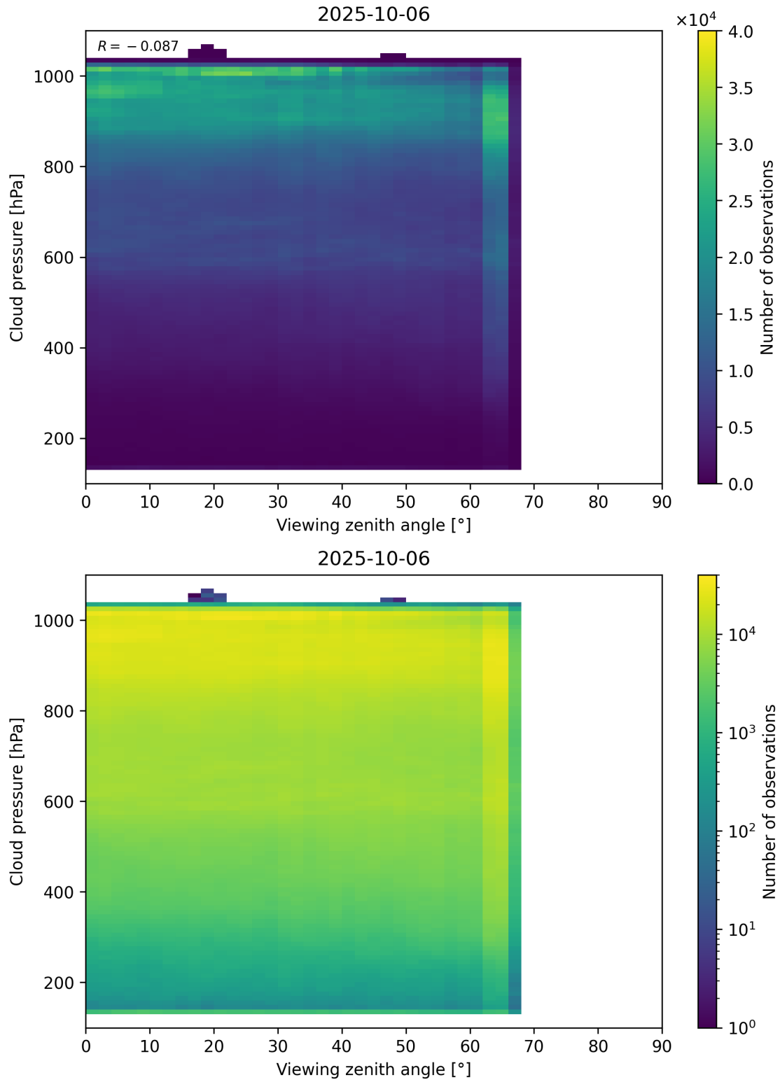
Figure 121: Scatter density plot of “Viewing zenith angle” against “Cloud pressure” for 2025-10-06 to 2025-10-07.
