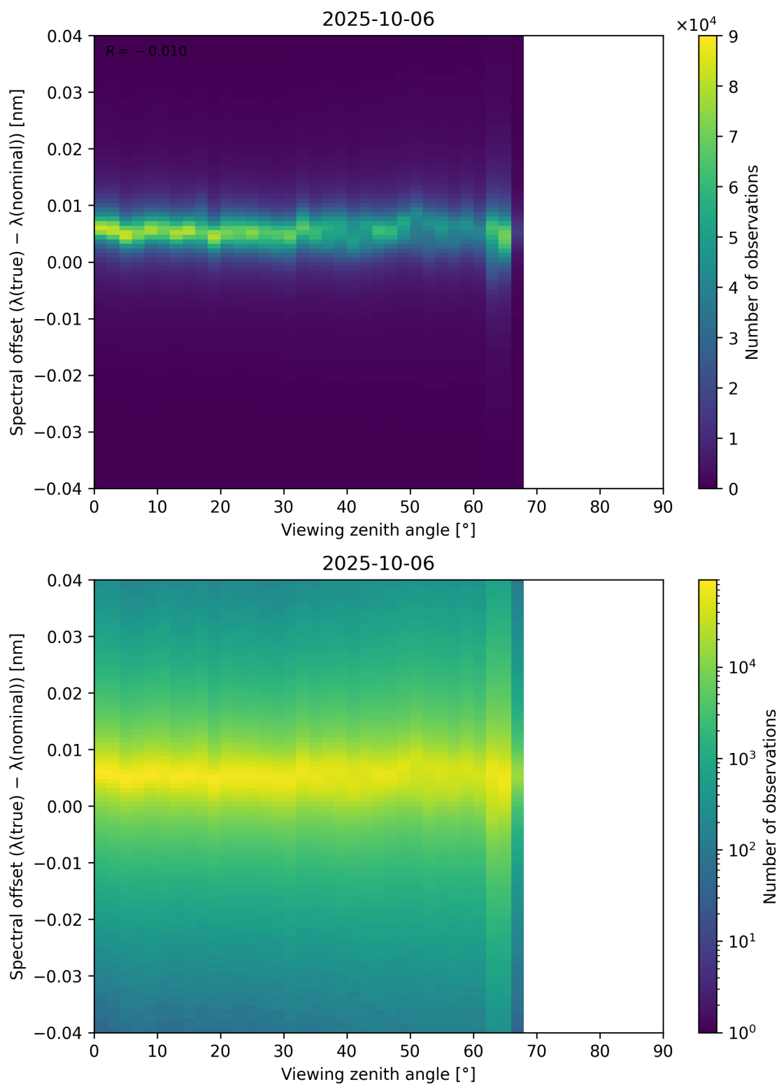
Figure 128: Scatter density plot of “Viewing zenith angle” against “Spectral offset ( \lambda_{\text{true}} - \lambda_{\text{nominal}} )” for 2025-10-06 to 2025-10-07.
