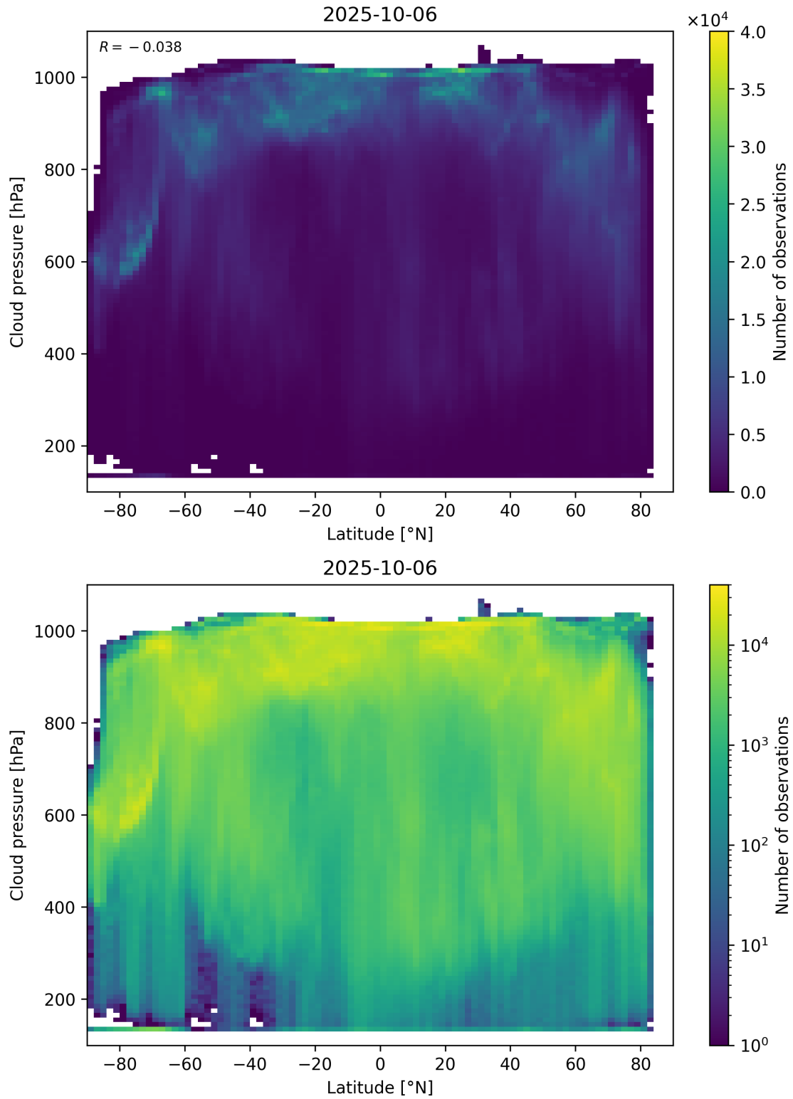
Figure 91: Scatter density plot of “Latitude” against “Cloud pressure” for 2025-10-06 to 2025-10-07.
