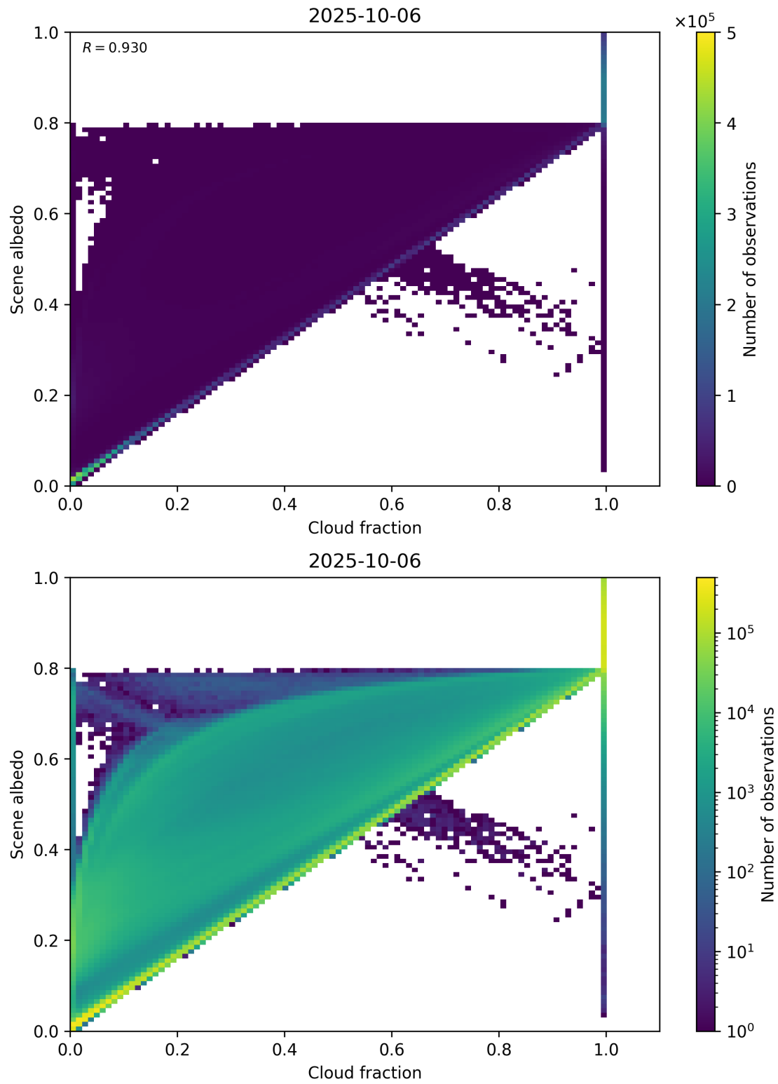
Figure 75: Scatter density plot of “Cloud fraction” against “Scene albedo” for 2025-10-06 to 2025-10-07.
