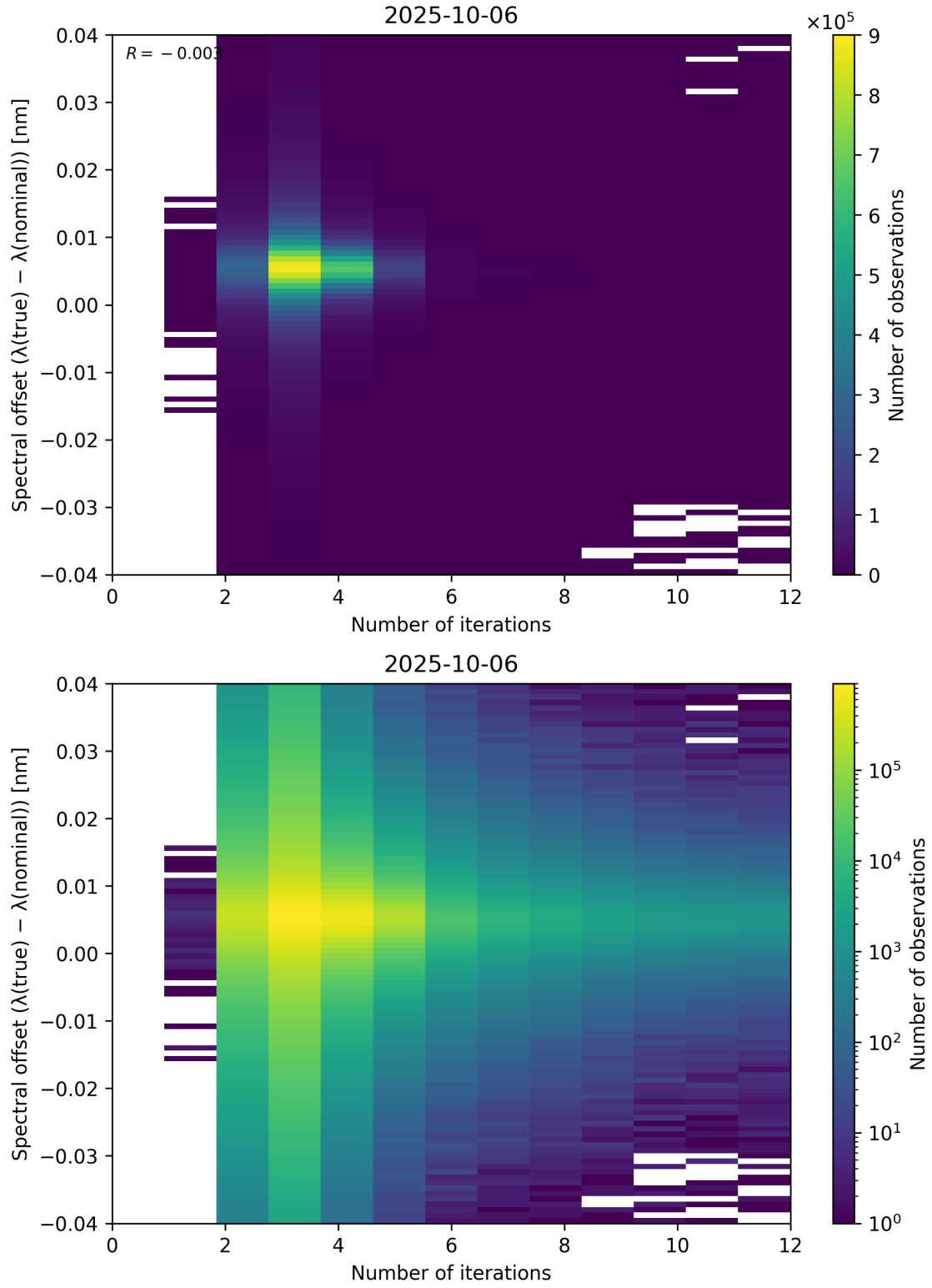
Figure 100: Scatter density plot of “Number of iterations” against “Spectral offset ( \lambda_{\text{true}} - \lambda_{\text{nominal}} )” for 2025-10-06 to 2025-10-07.
