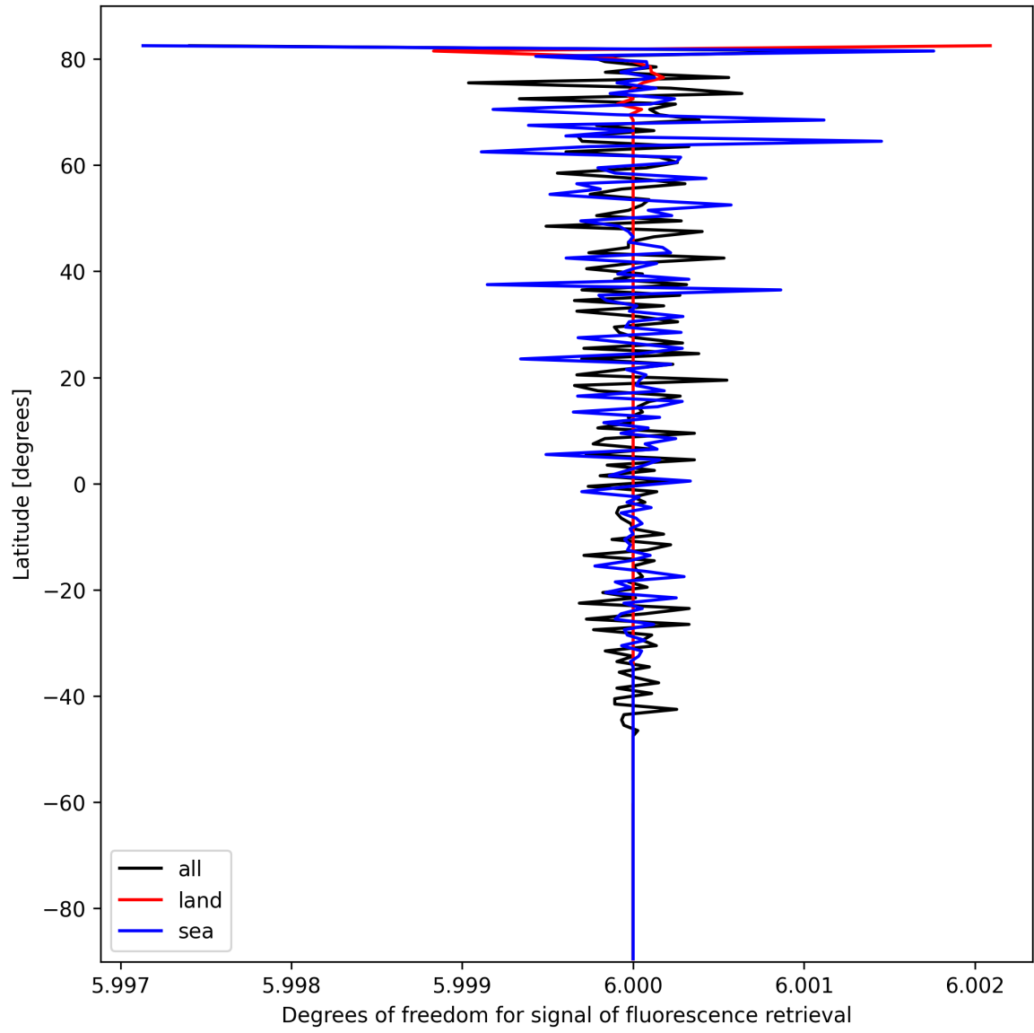
Figure 26: Zonal average of “Degrees of freedom for signal of fluorescence retrieval” for 2025-10-06 to 2025-10-07.
