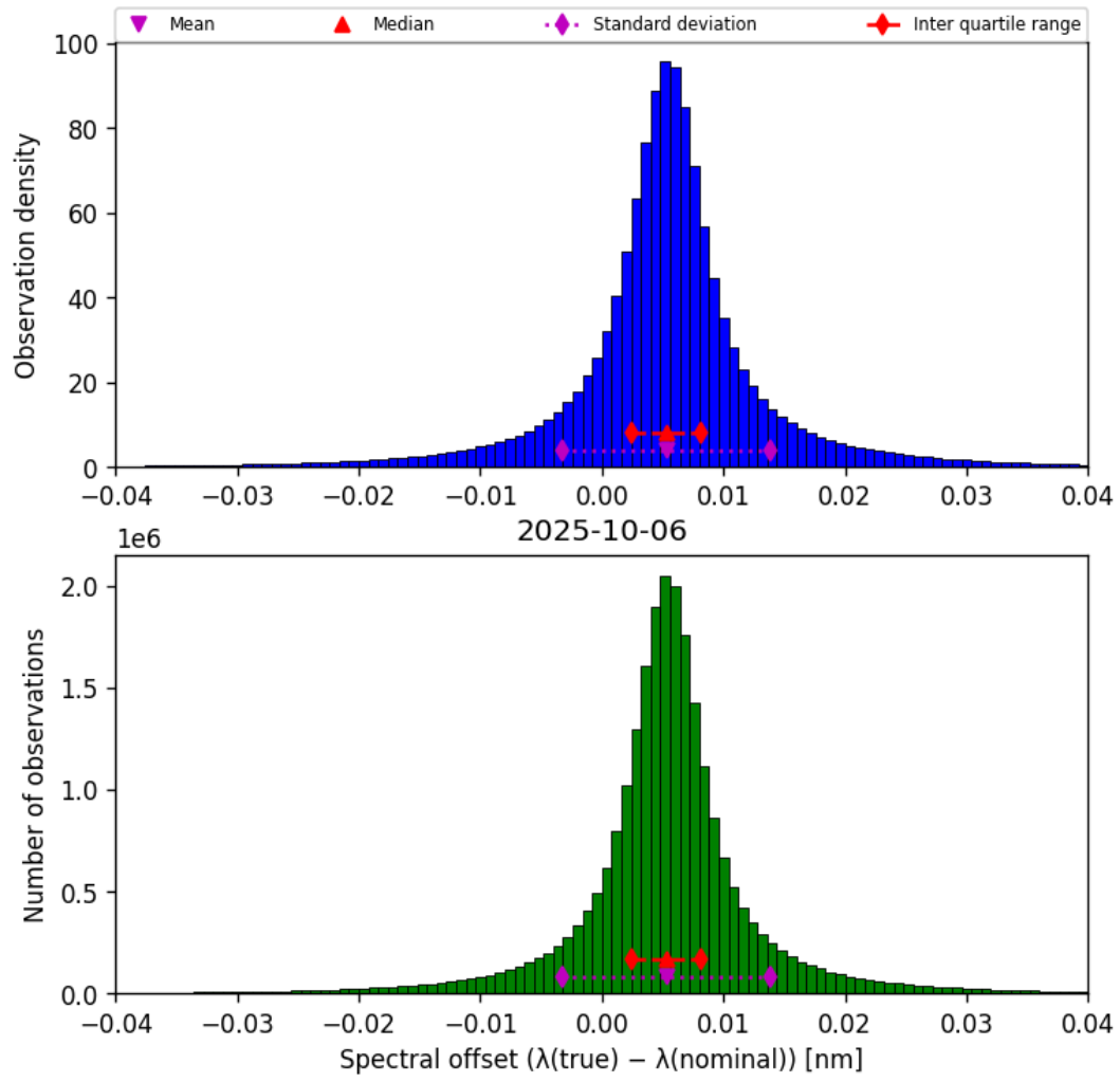
Figure 45: Histogram of “Spectral offset ( \lambda_{\text{true}} - \lambda_{\text{nominal}} )” for 2025-10-06 to 2025-10-07
