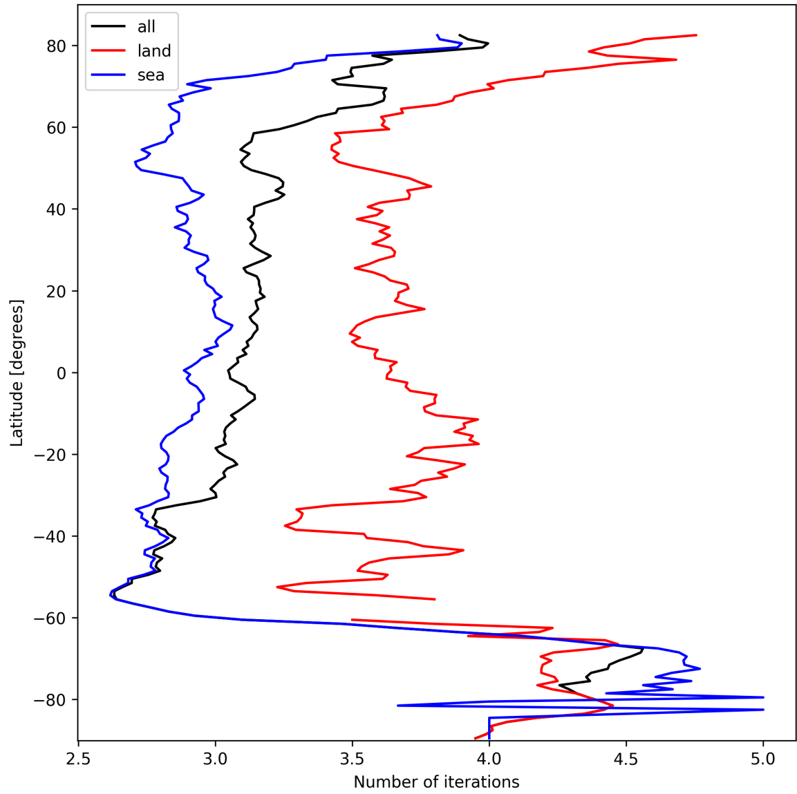
Figure 22: Zonal average of “Number of iterations” for 2025-10-06 to 2025-10-07.
