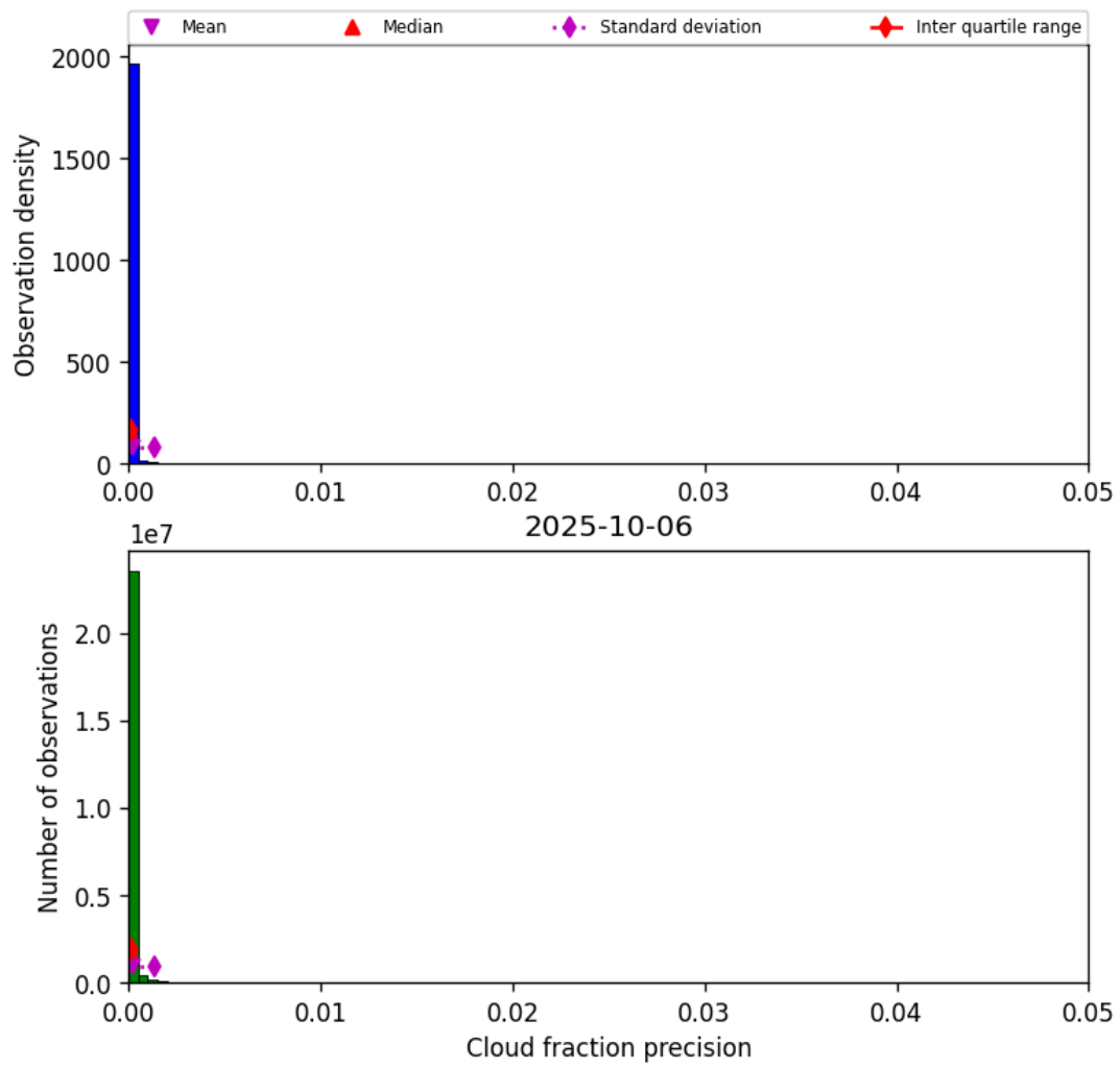
Figure 33: Histogram of “Cloud fraction precision” for 2025-10-06 to 2025-10-07
