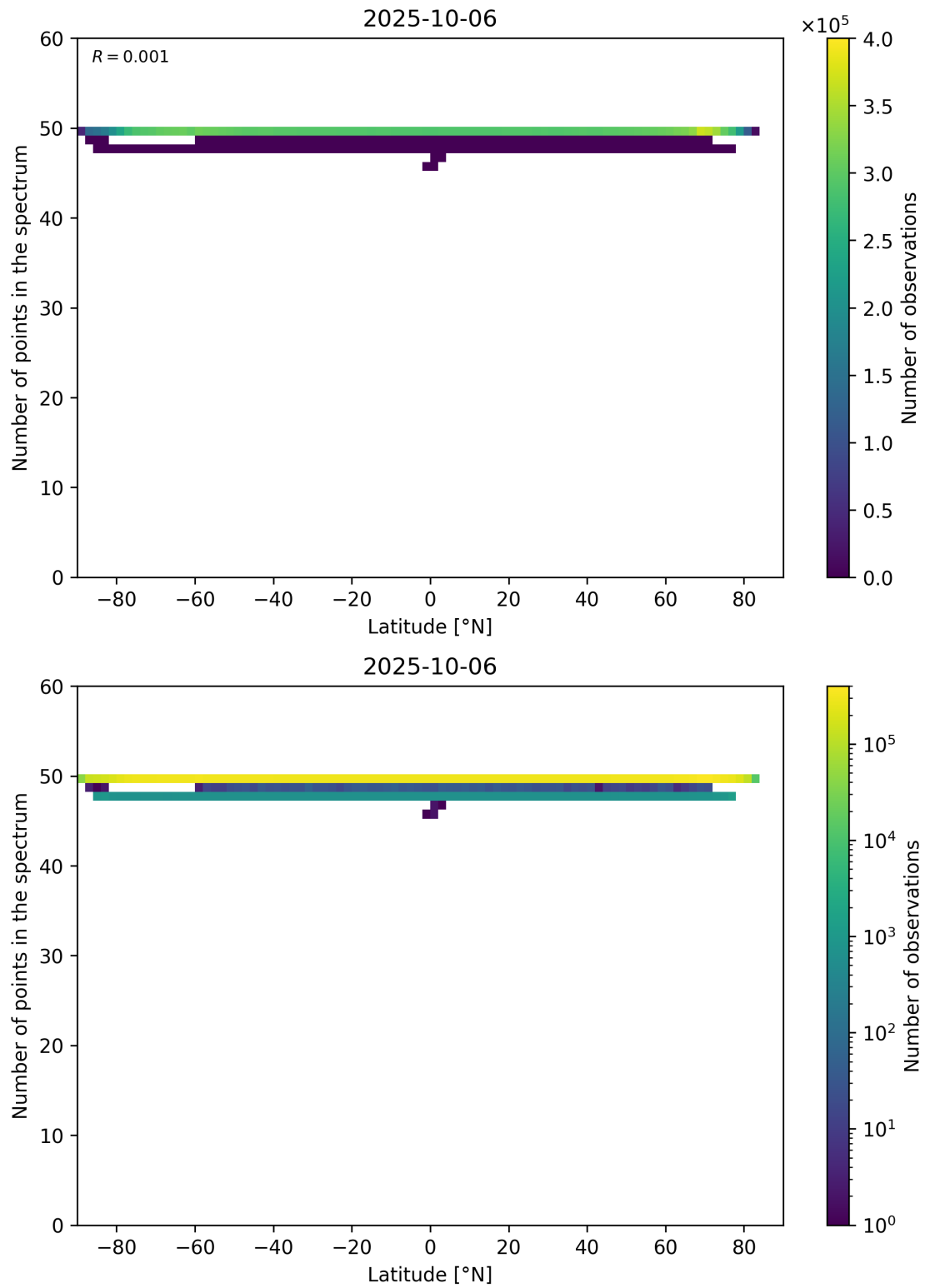
Figure 94: Scatter density plot of “Latitude” against “Number of points in the spectrum” for 2025-10-06 to 2025-10-07.
