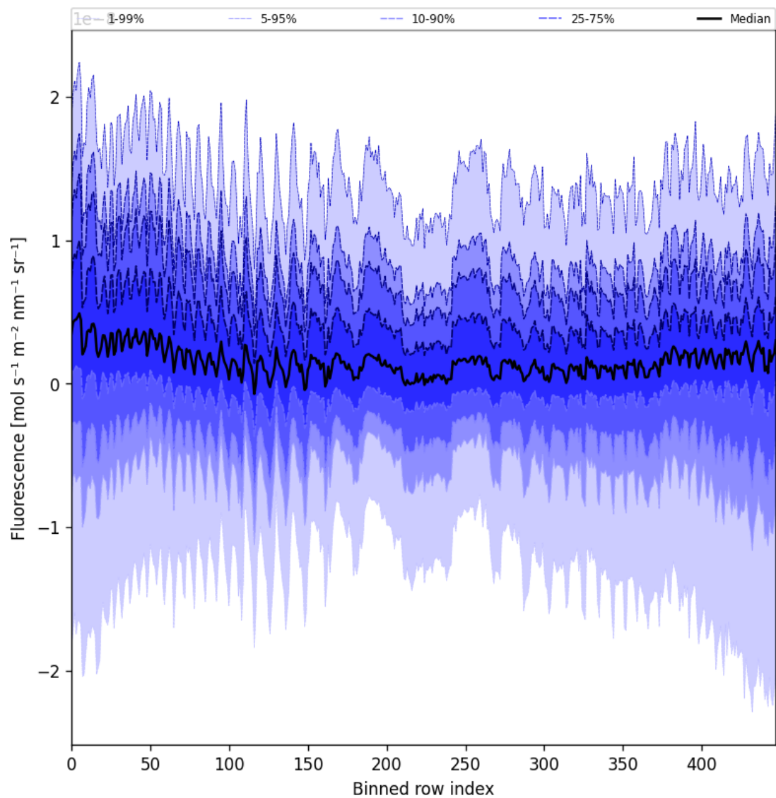
Figure 57: Along track statistics of “Fluorescence” for 2025-10-06 to 2025-10-07
