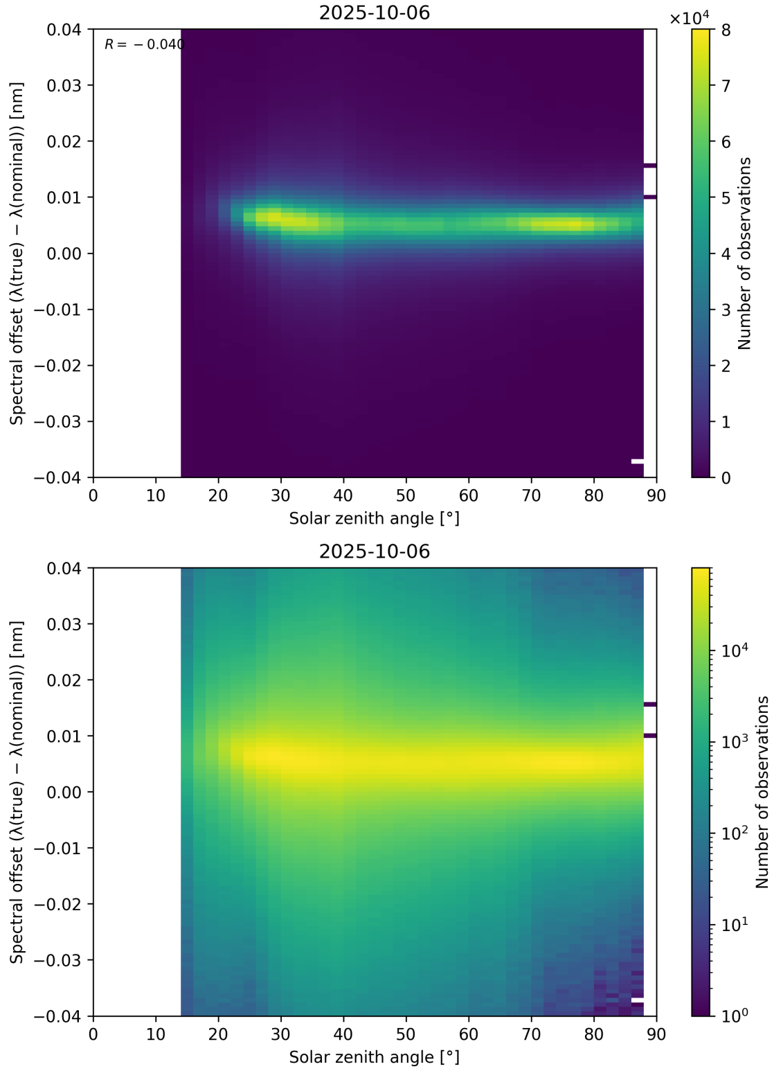
Figure 117: Scatter density plot of “Solar zenith angle” against “Spectral offset ( \lambda_{\text{true}} - \lambda_{\text{nominal}} )” for 2025-10-06 to 2025-10-07.
