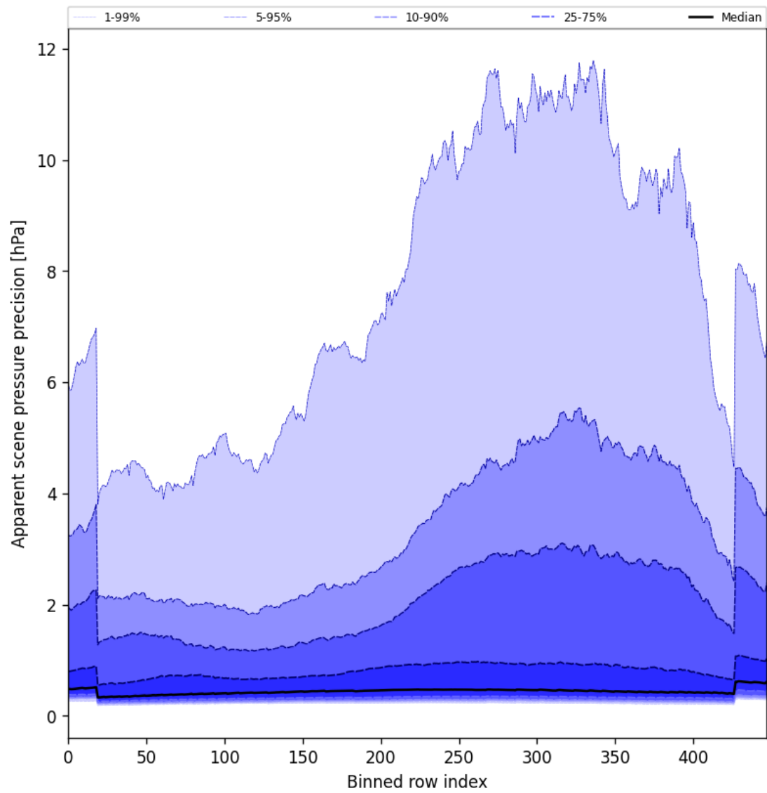
Figure 54: Along track statistics of “Apparent scene pressure precision” for 2025-10-06 to 2025-10-07
