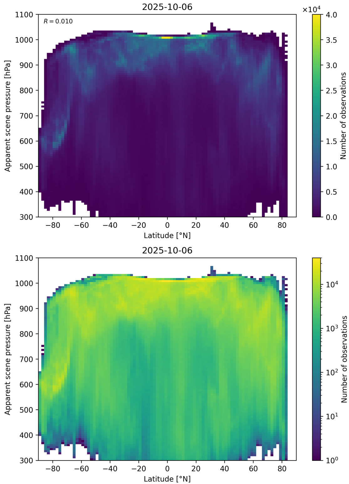
Figure 88: Scatter density plot of “Latitude” against “Apparent scene pressure” for 2025-10-06 to 2025-10-07.
