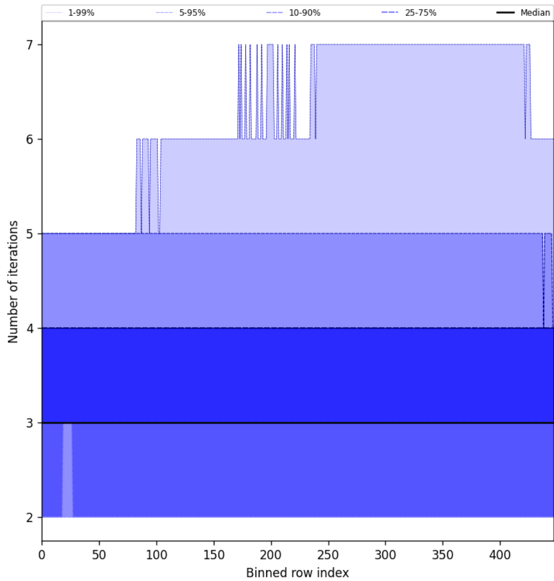
Figure 56: Along track statistics of “Number of iterations” for 2025-10-06 to 2025-10-07
