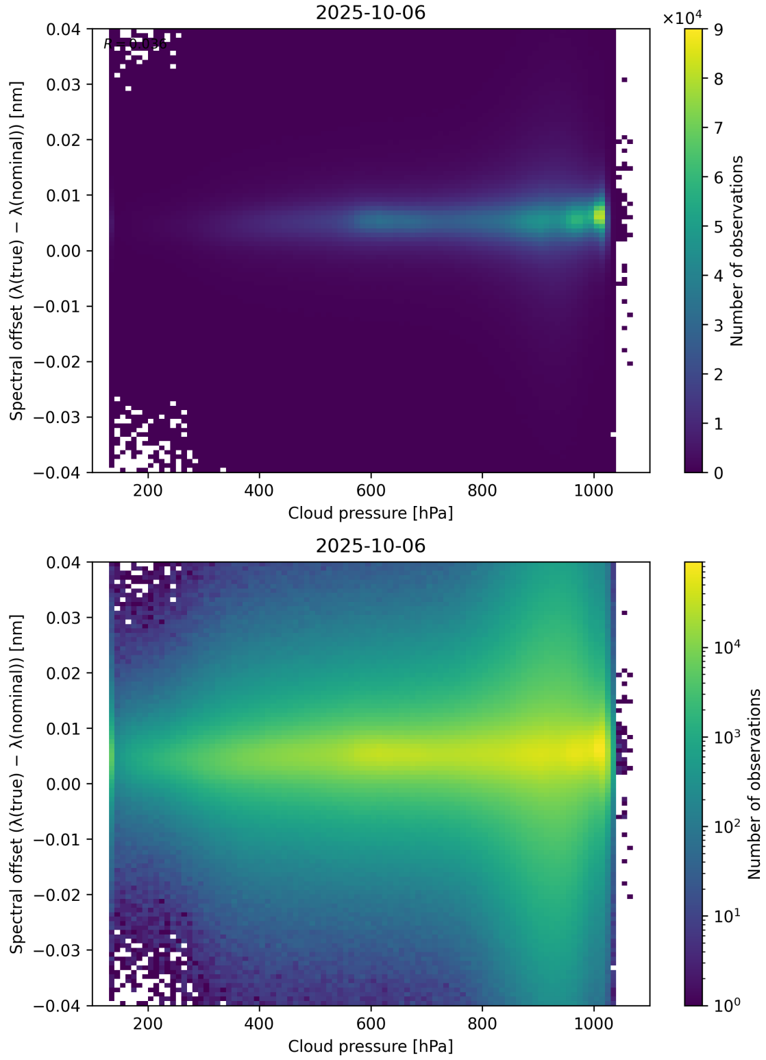
Figure 84: Scatter density plot of “Cloud pressure” against “Spectral offset ( \lambda_{\text{true}} - \lambda_{\text{nominal}} )” for 2025-10-06 to 2025-10-07.
