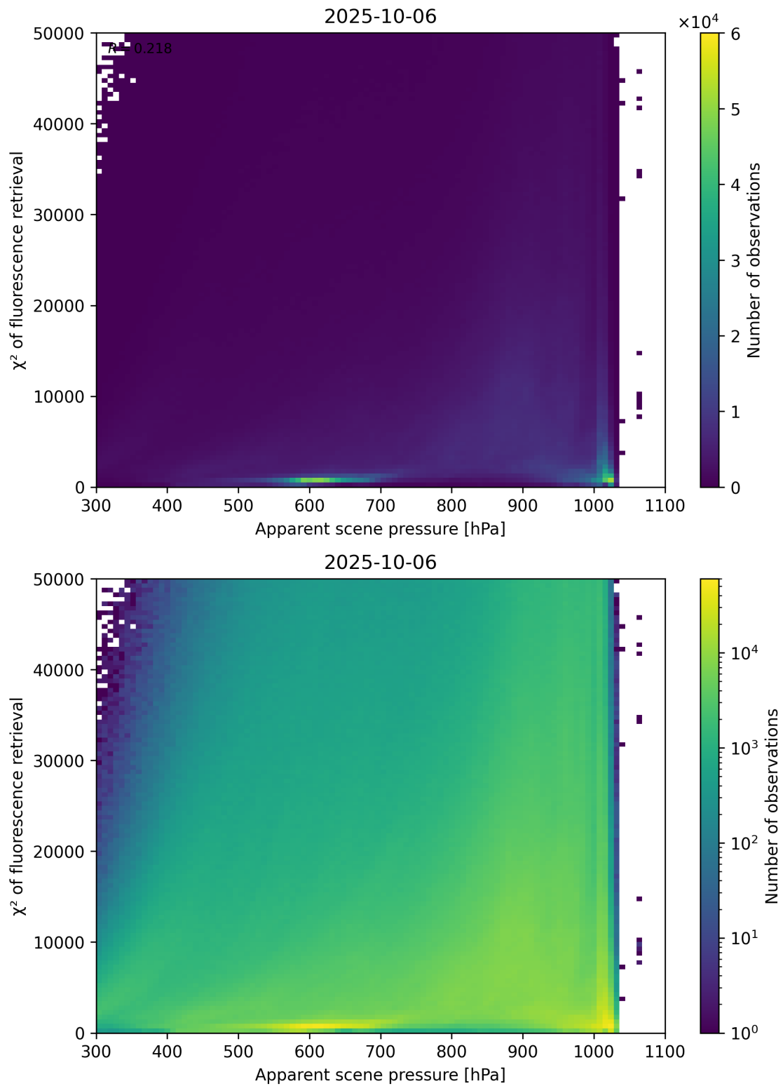
Figure 63: Scatter density plot of “Apparent scene pressure” against “ \chi^2 of fluorescence retrieval” for 2025-10-06 to 2025-10-07.
