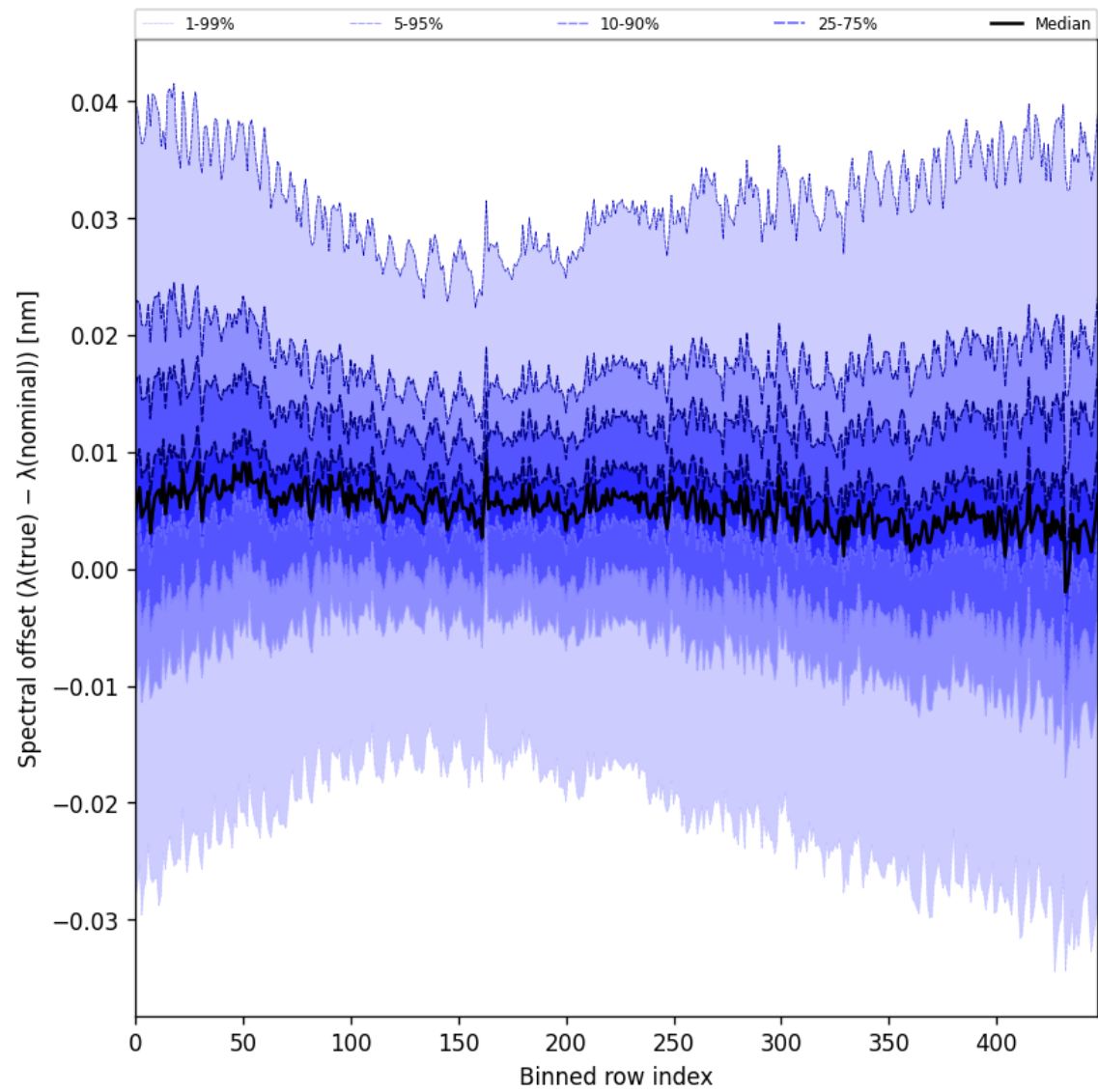
Figure 62: Along track statistics of “Spectral offset ( \lambda_{\text{true}} - \lambda_{\text{nominal}} )” for 2025-10-06 to 2025-10-07
