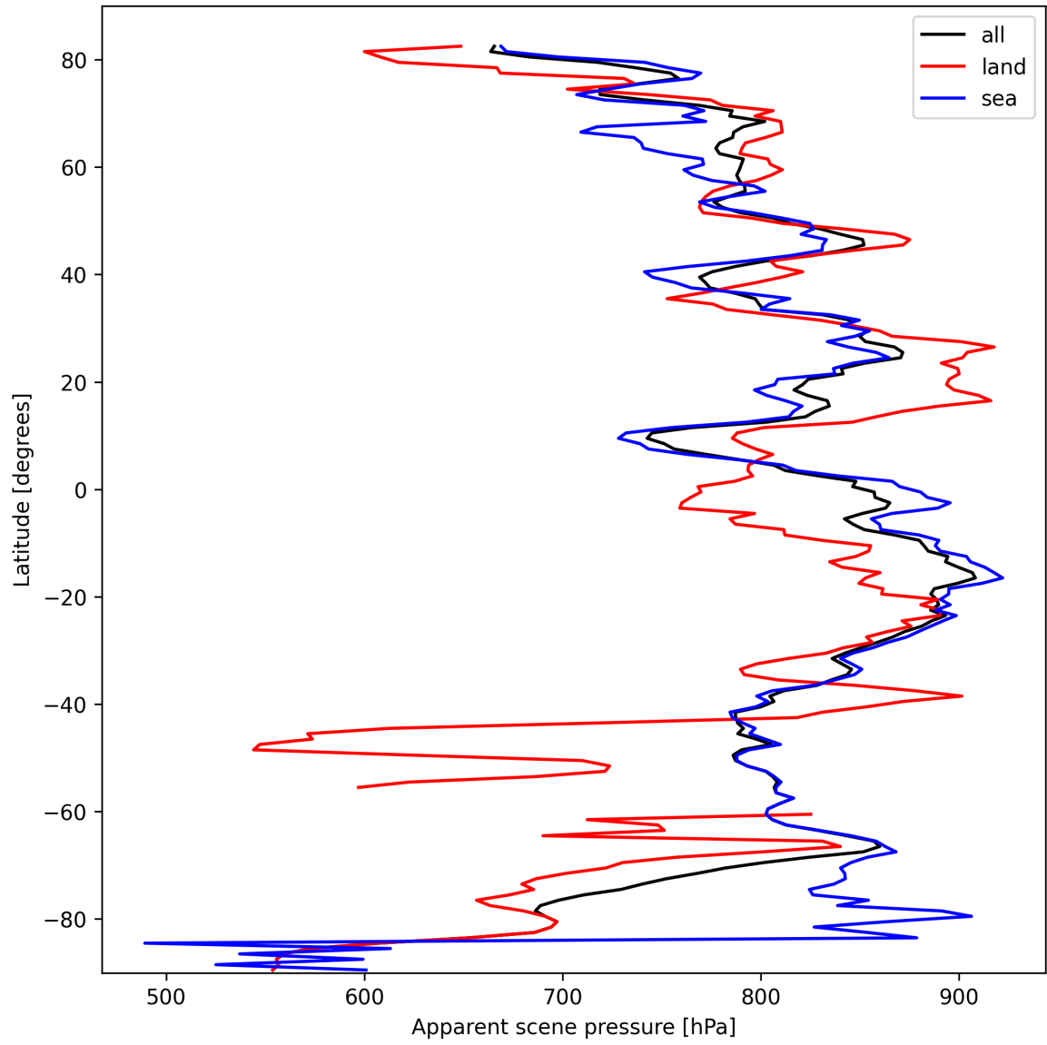
Figure 19: Zonal average of “Apparent scene pressure” for 2025-10-06 to 2025-10-07.
