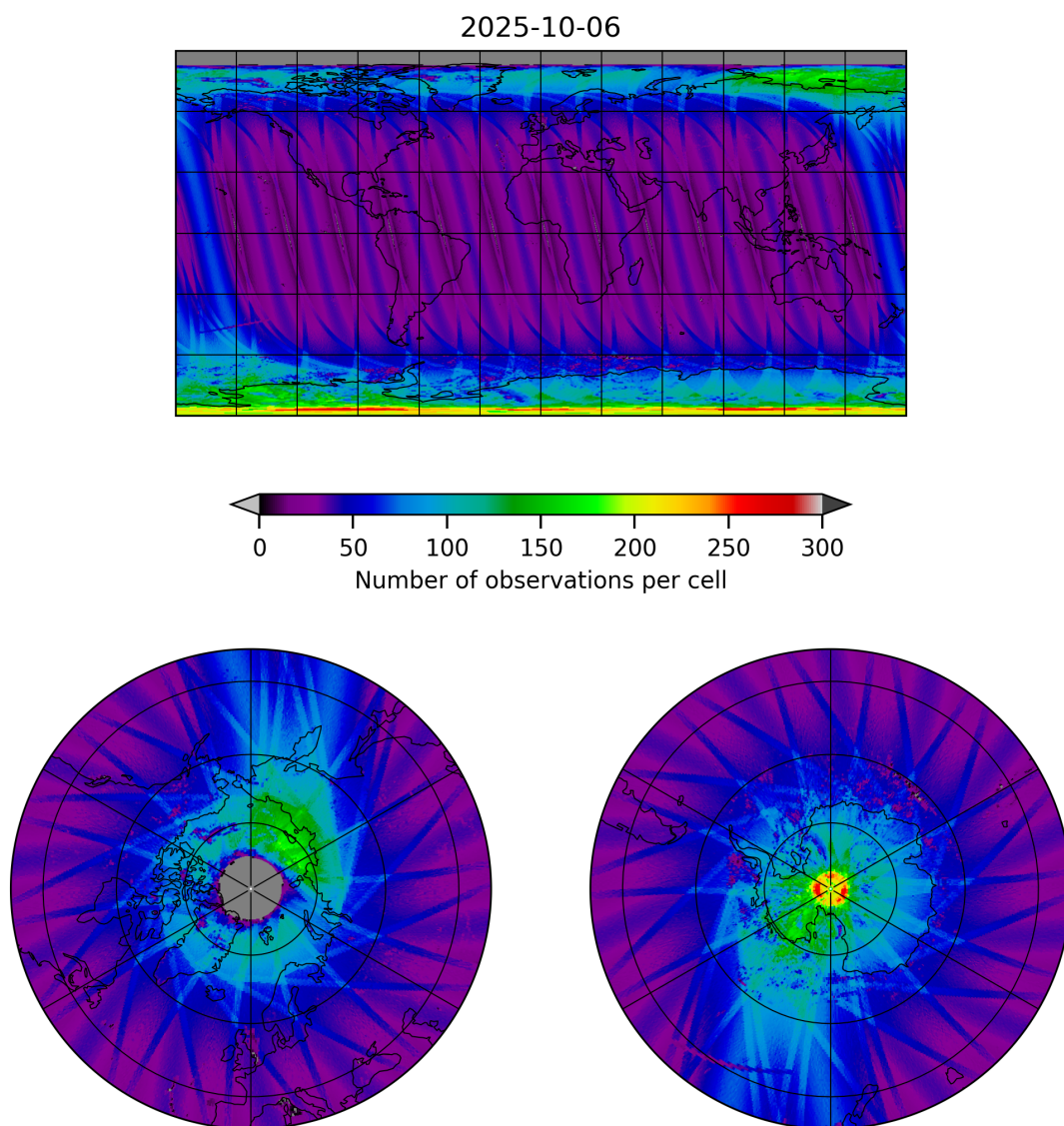
Figure 11: Map of the number of observations for 2025-10-06 to 2025-10-07
