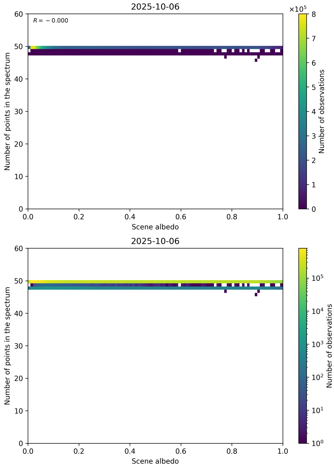
Figure 106: Scatter density plot of “Scene albedo” against “Number of points in the spectrum” for 2025-10-06 to 2025-10-07.
