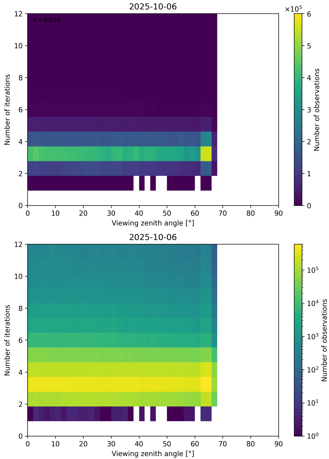
Figure 124: Scatter density plot of “Viewing zenith angle” against “Number of iterations” for 2025-10-06 to 2025-10-07.
