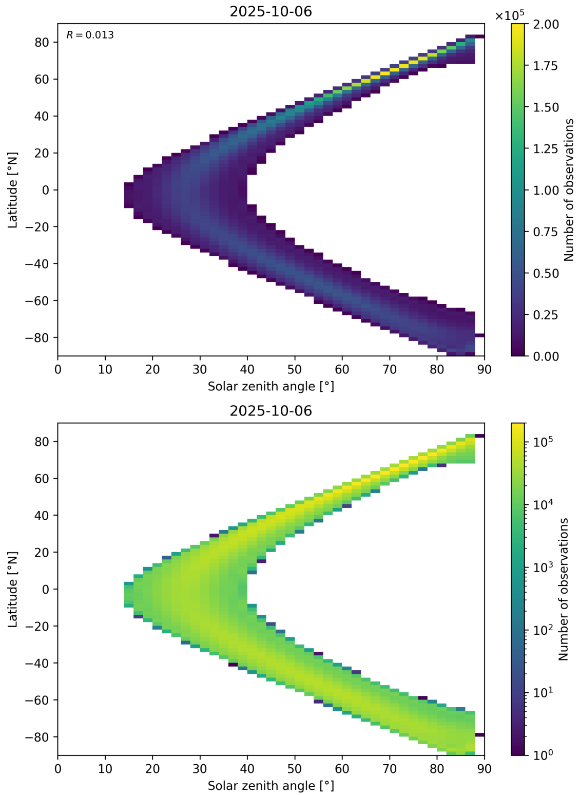
Figure 113: Scatter density plot of “Solar zenith angle” against “Latitude” for 2025-10-06 to 2025-10-07.
