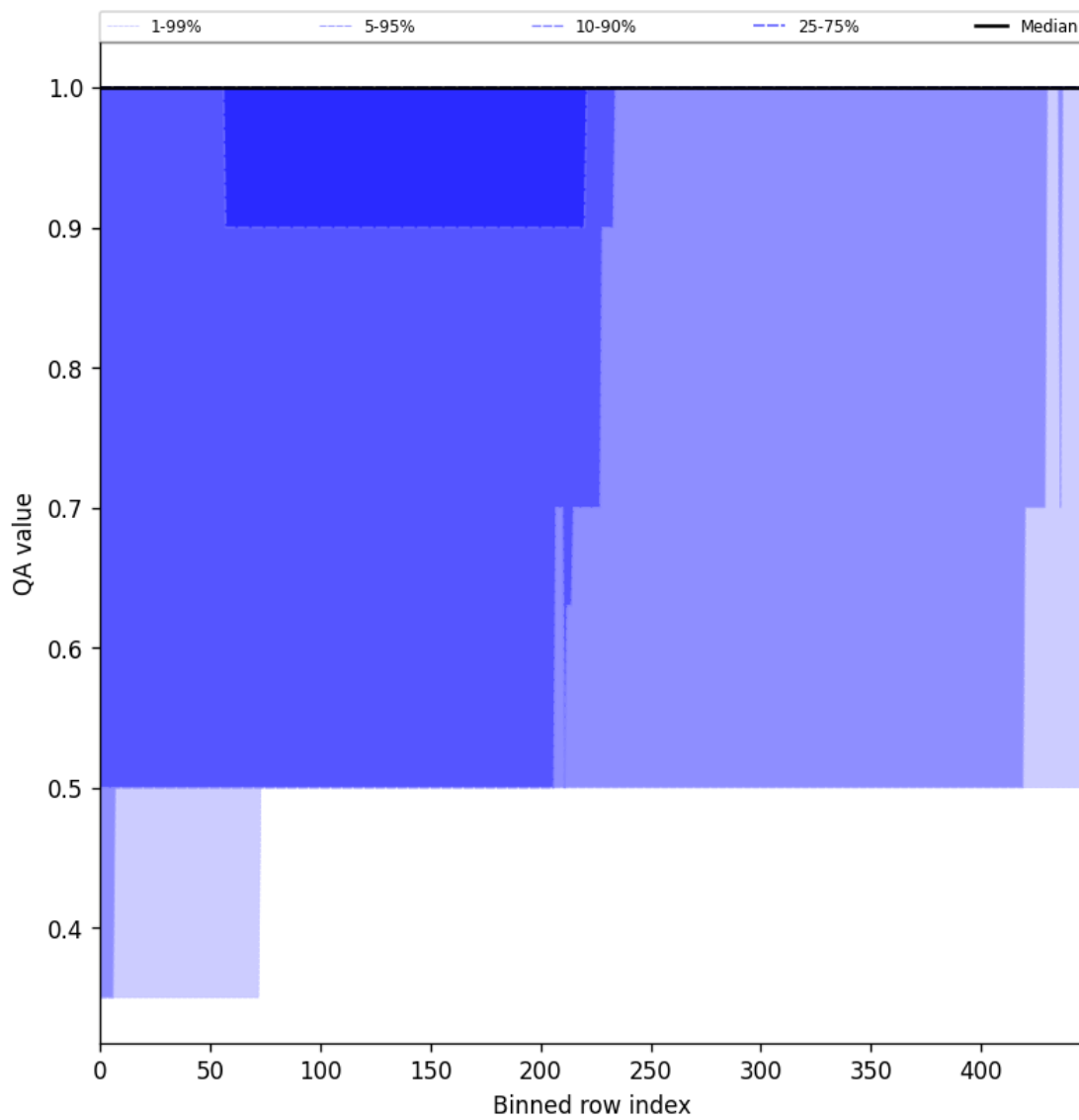
Figure 46: Along track statistics of “QA value” for 2025-10-06 to 2025-10-07
