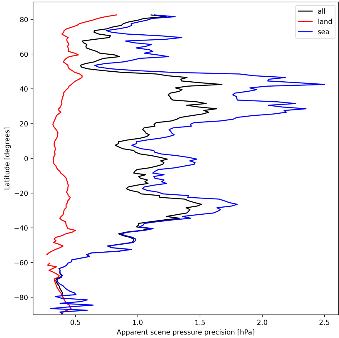
Figure 20: Zonal average of “Apparent scene pressure precision” for 2025-10-06 to 2025-10-07.
