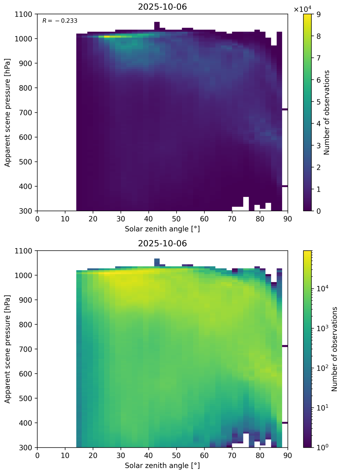
Figure 108: Scatter density plot of “Solar zenith angle” against “Apparent scene pressure” for 2025-10-06 to 2025-10-07.
