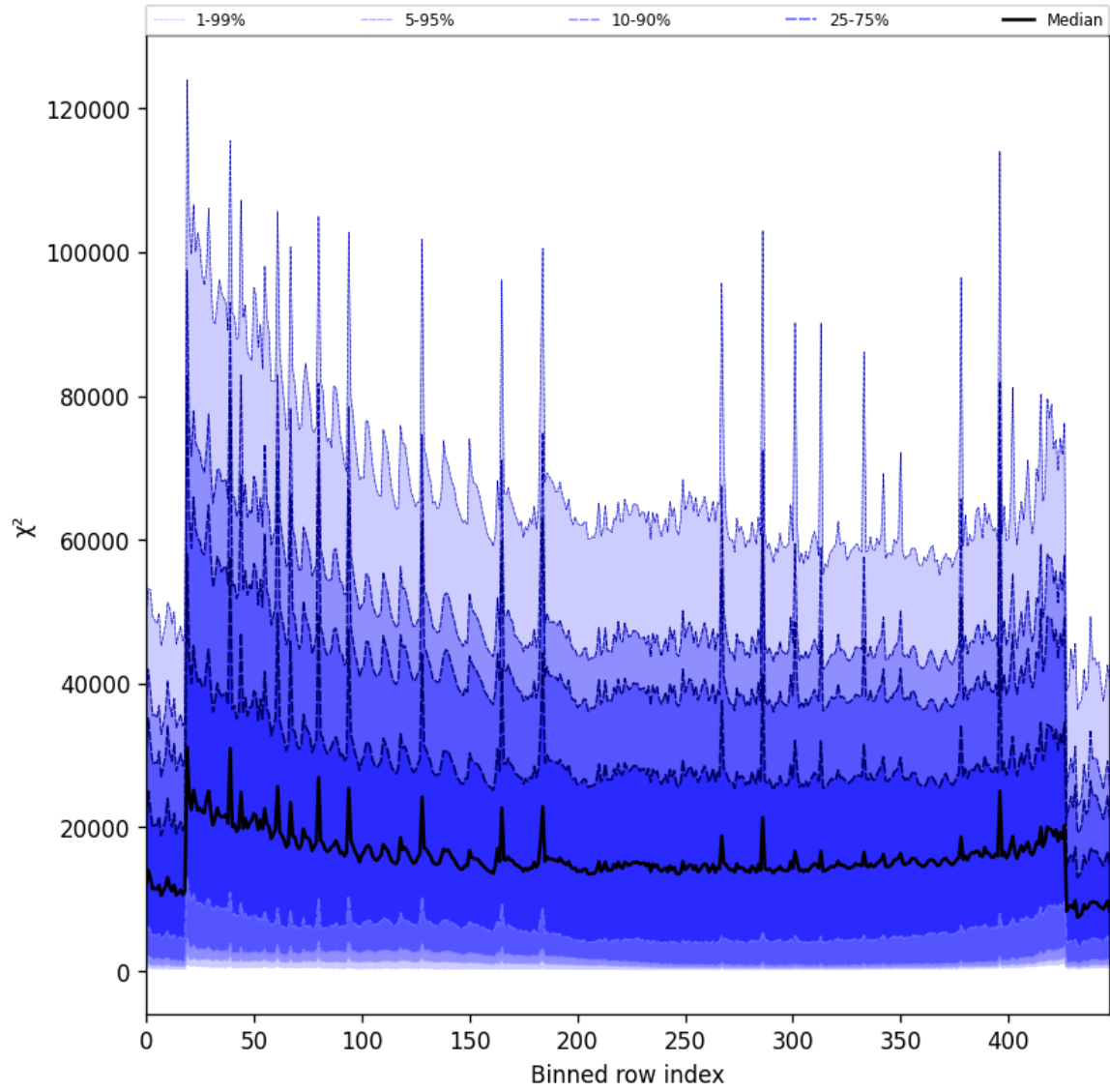
Figure 55: Along track statistics of “ \chi^2 ” for 2025-10-06 to 2025-10-07
