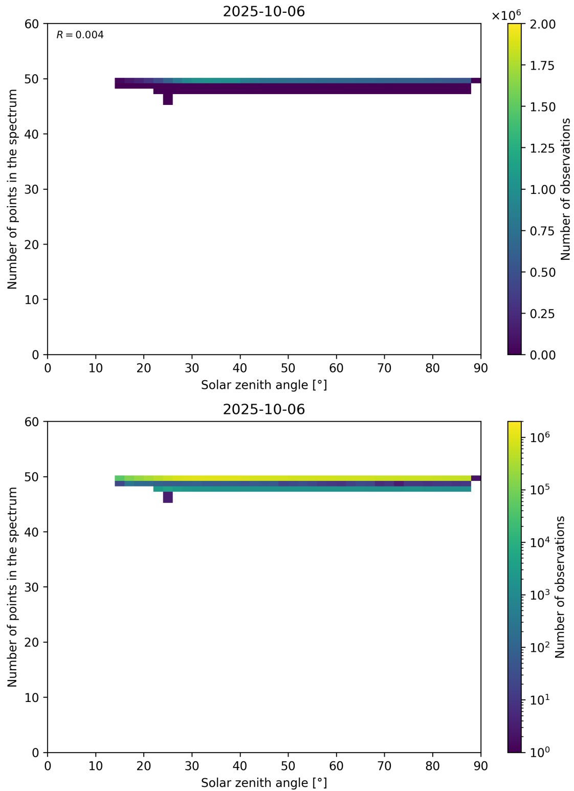
Figure 115: Scatter density plot of “Solar zenith angle” against “Number of points in the spectrum” for 2025-10-06 to 2025-10-07.
