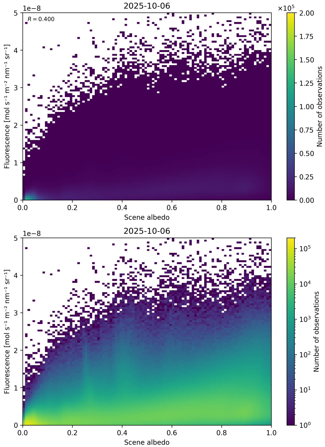
Figure 104: Scatter density plot of “Scene albedo” against “Fluorescence” for 2025-10-06 to 2025-10-07.
