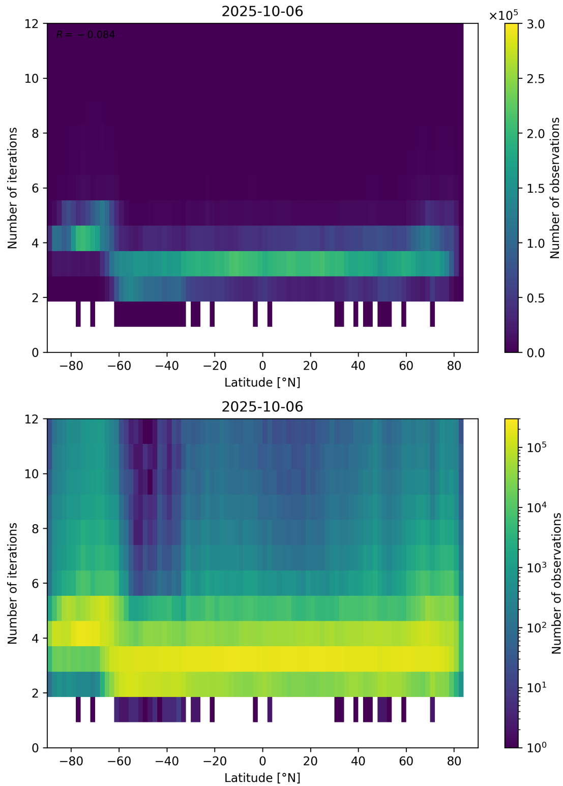
Figure 93: Scatter density plot of “Latitude” against “Number of iterations” for 2025-10-06 to 2025-10-07.
