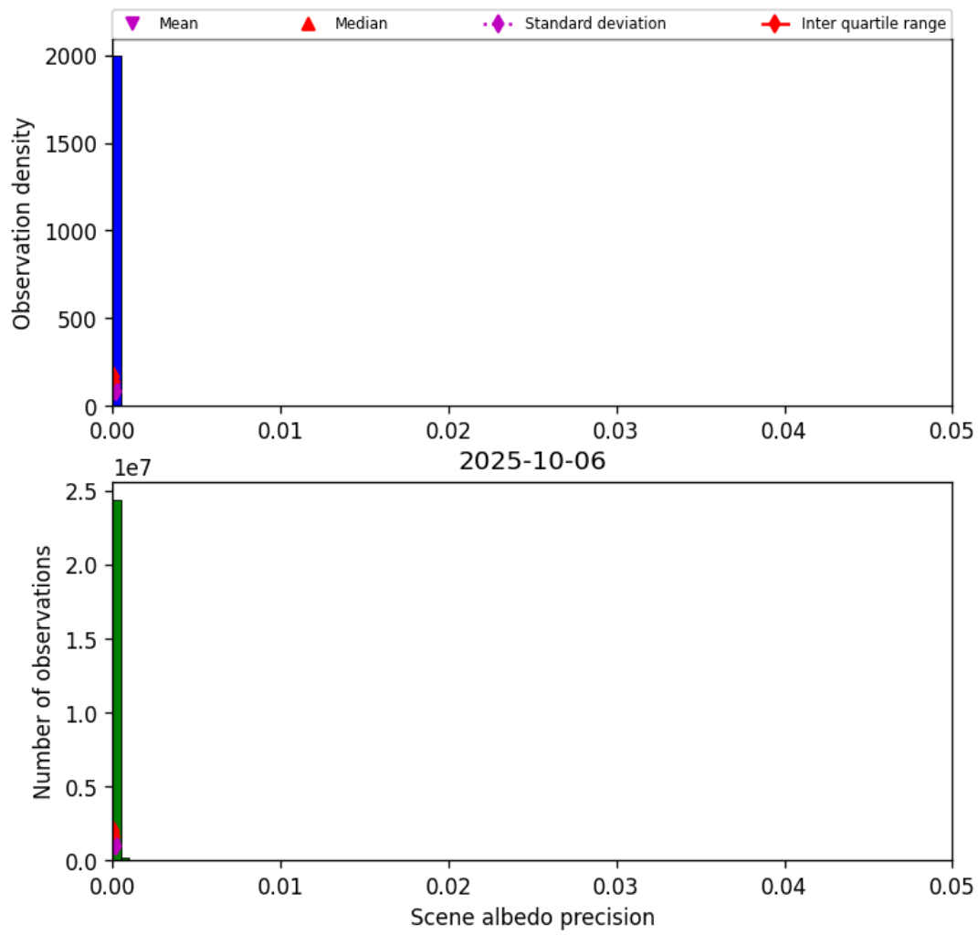
Figure 35: Histogram of “Scene albedo precision” for 2025-10-06 to 2025-10-07
