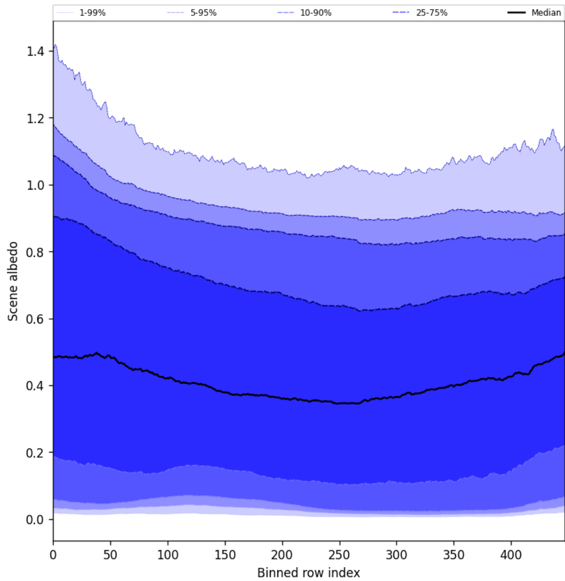
Figure 51: Along track statistics of “Scene albedo” for 2025-10-06 to 2025-10-07
