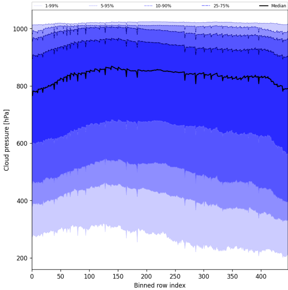
Figure 47: Along track statistics of “Cloud pressure” for 2025-10-06 to 2025-10-07
