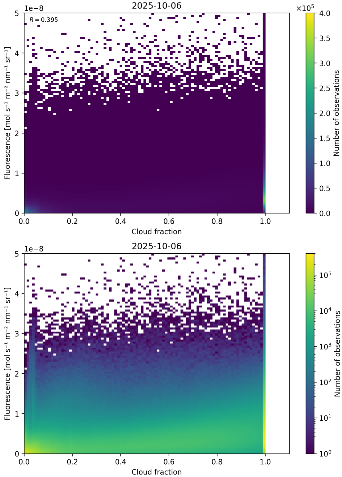
Figure 72: Scatter density plot of “Cloud fraction” against “Fluorescence” for 2025-10-06 to 2025-10-07.
