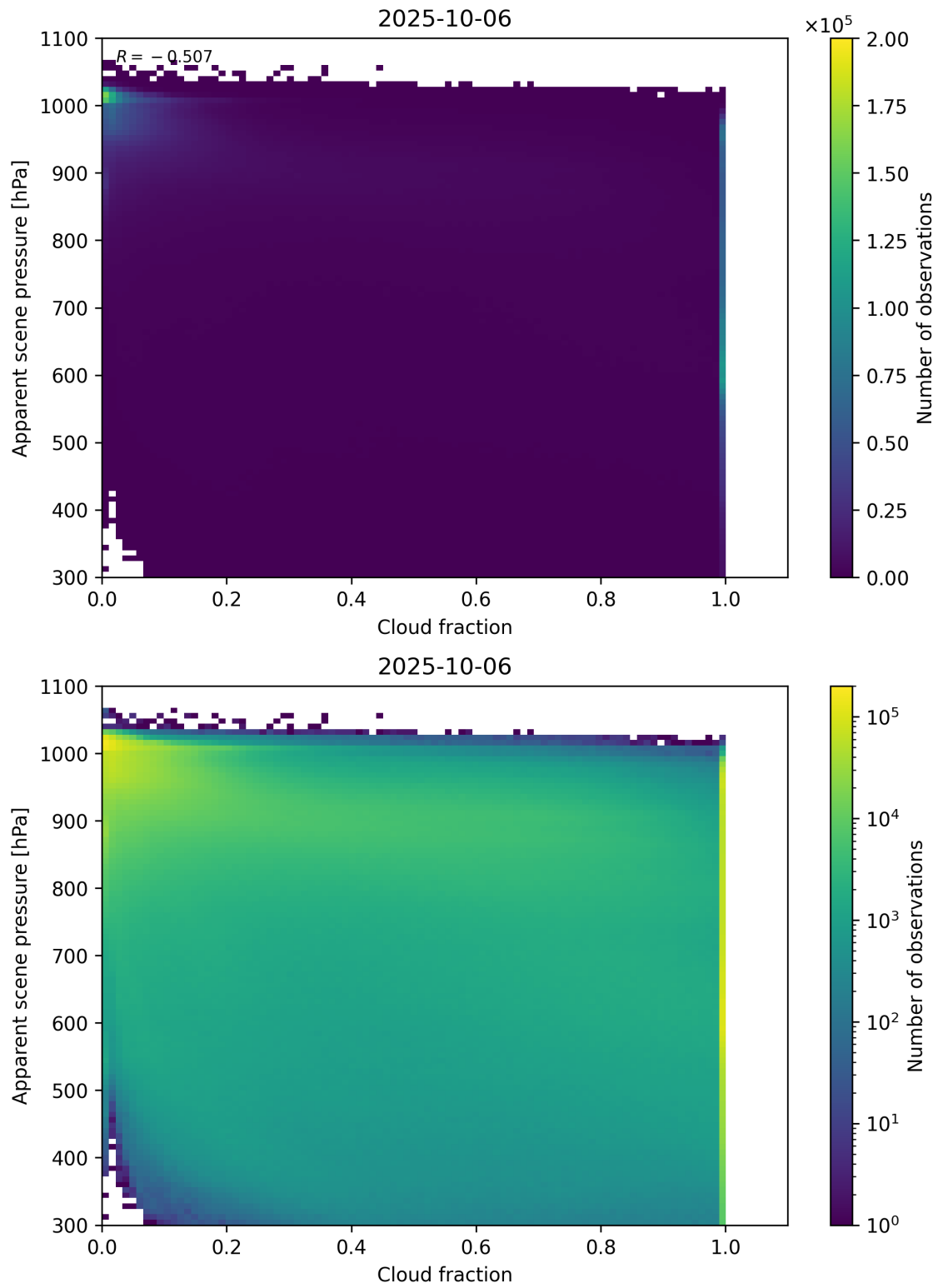
Figure 70: Scatter density plot of “Cloud fraction” against “Apparent scene pressure” for 2025-10-06 to 2025-10-07.
