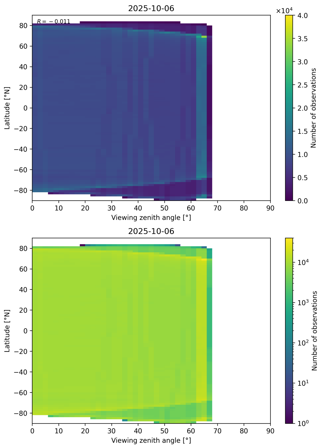
Figure 123: Scatter density plot of “Viewing zenith angle” against “Latitude” for 2025-10-06 to 2025-10-07.
