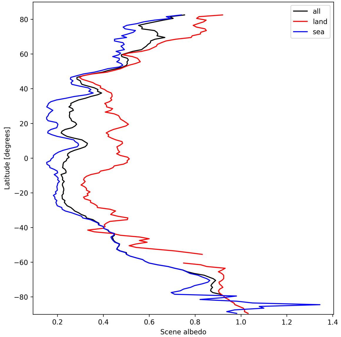
Figure 17: Zonal average of “Scene albedo” for 2025-10-06 to 2025-10-07.
