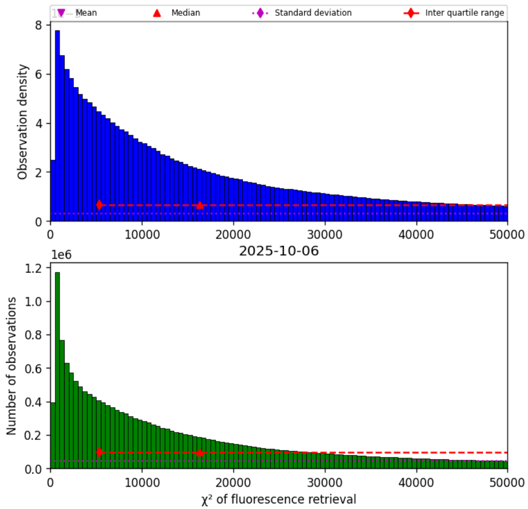
Figure 42: Histogram of “ \chi^2 of fluorescence retrieval” for 2025-10-06 to 2025-10-07
