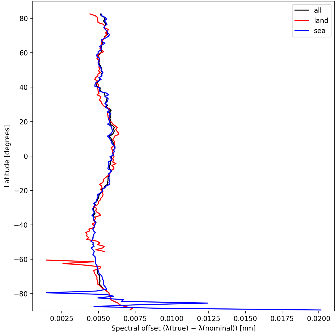
Figure 28: Zonal average of “Spectral offset ( \lambda_{\text{true}} - \lambda_{\text{nominal}} )” for 2025-10-06 to 2025-10-07.
