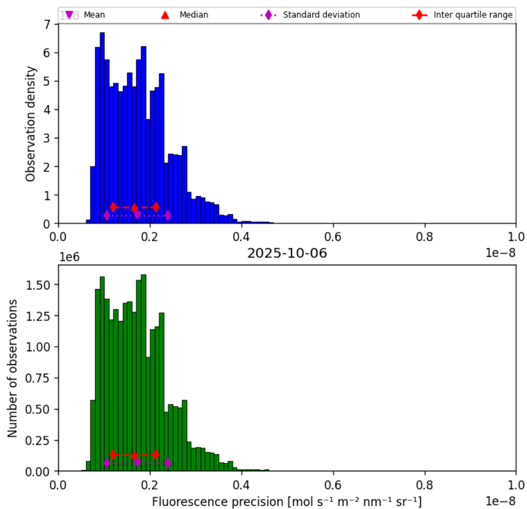
Figure 41: Histogram of “Fluorescence precision” for 2025-10-06 to 2025-10-07
