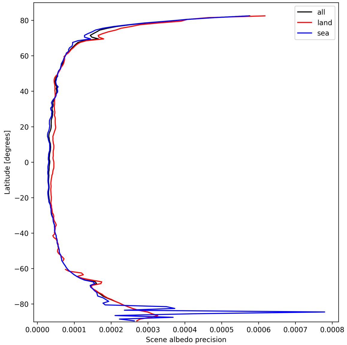
Figure 18: Zonal average of “Scene albedo precision” for 2025-10-06 to 2025-10-07.
