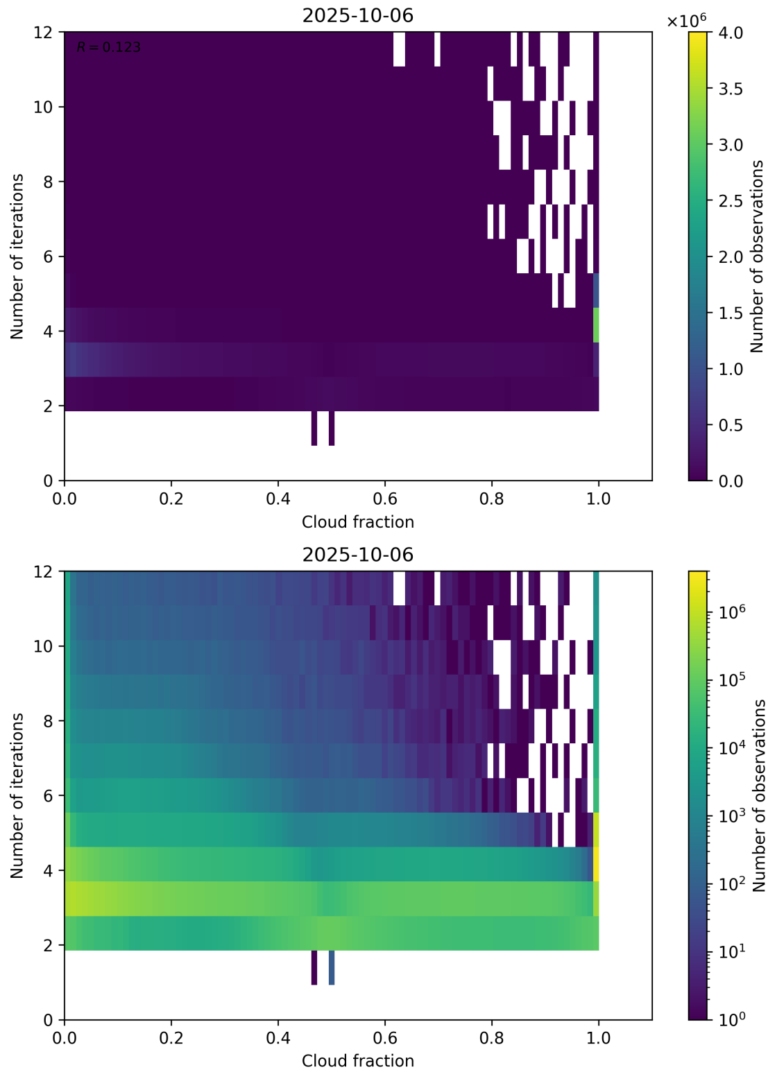
Figure 73: Scatter density plot of “Cloud fraction” against “Number of iterations” for 2025-10-06 to 2025-10-07.
