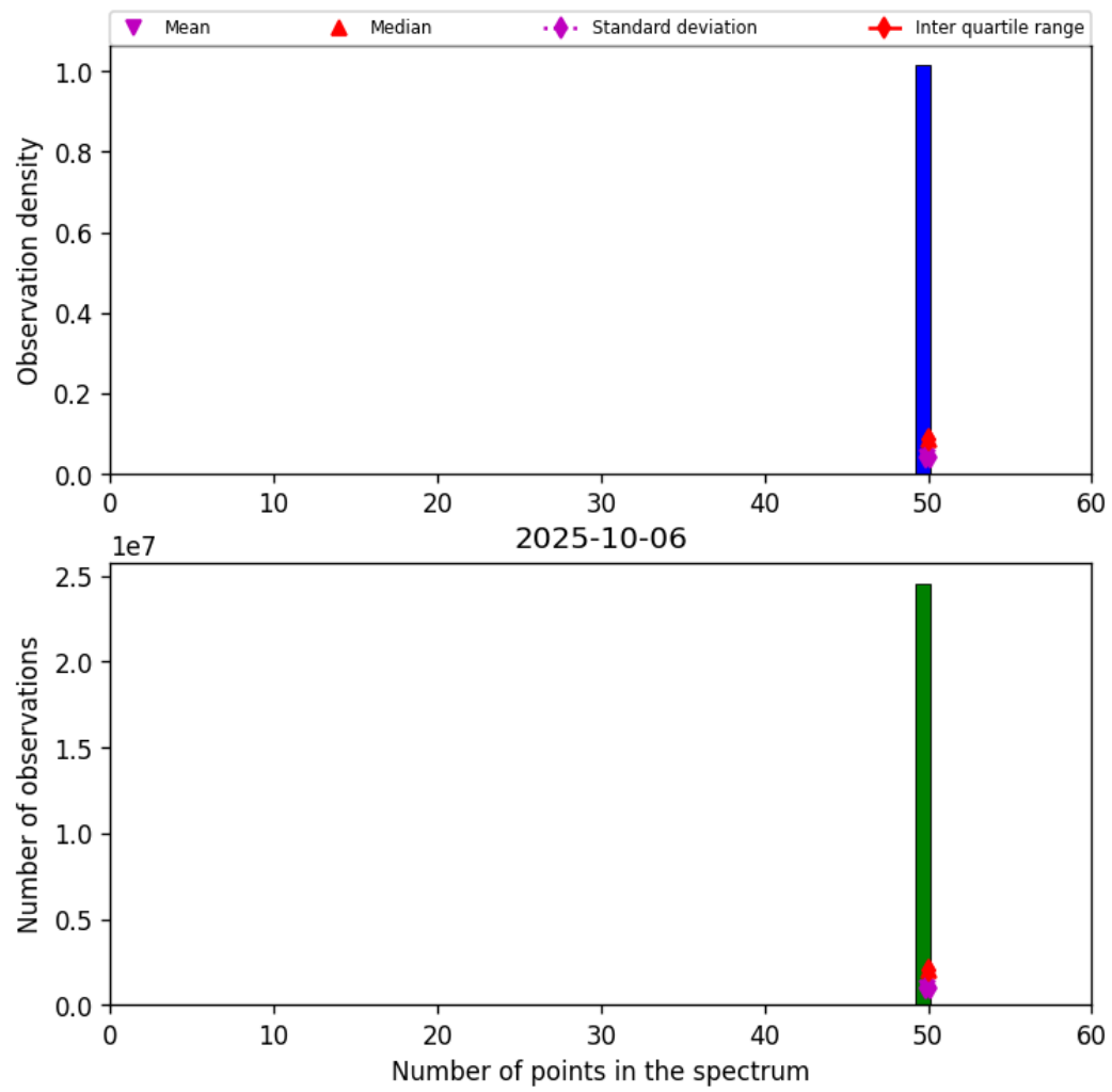
Figure 44: Histogram of “Number of points in the spectrum” for 2025-10-06 to 2025-10-07
