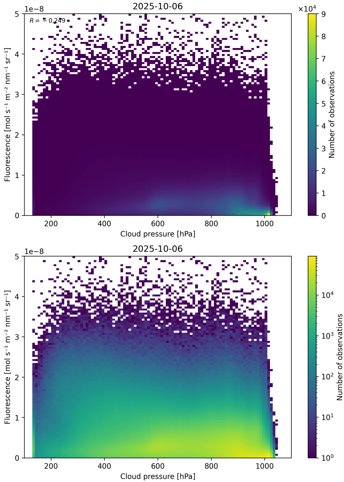
Figure 80: Scatter density plot of “Cloud pressure” against “Fluorescence” for 2025-10-06 to 2025-10-07.
