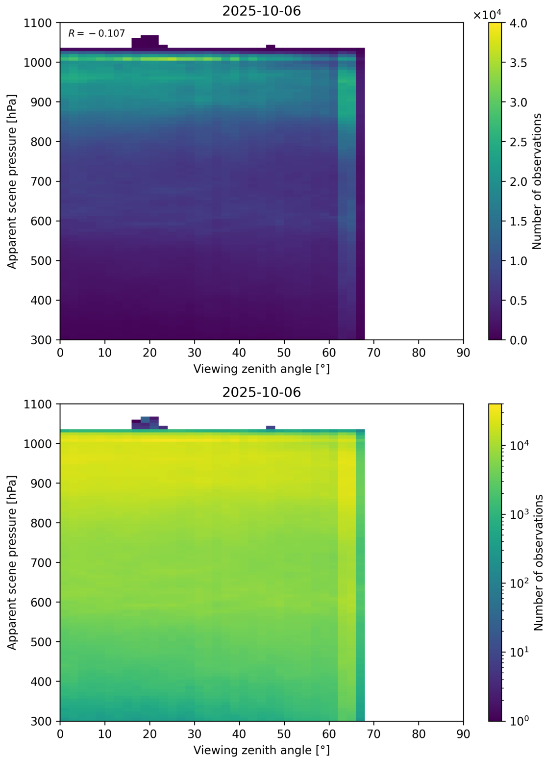
Figure 118: Scatter density plot of “Viewing zenith angle” against “Apparent scene pressure” for 2025-10-06 to 2025-10-07.
