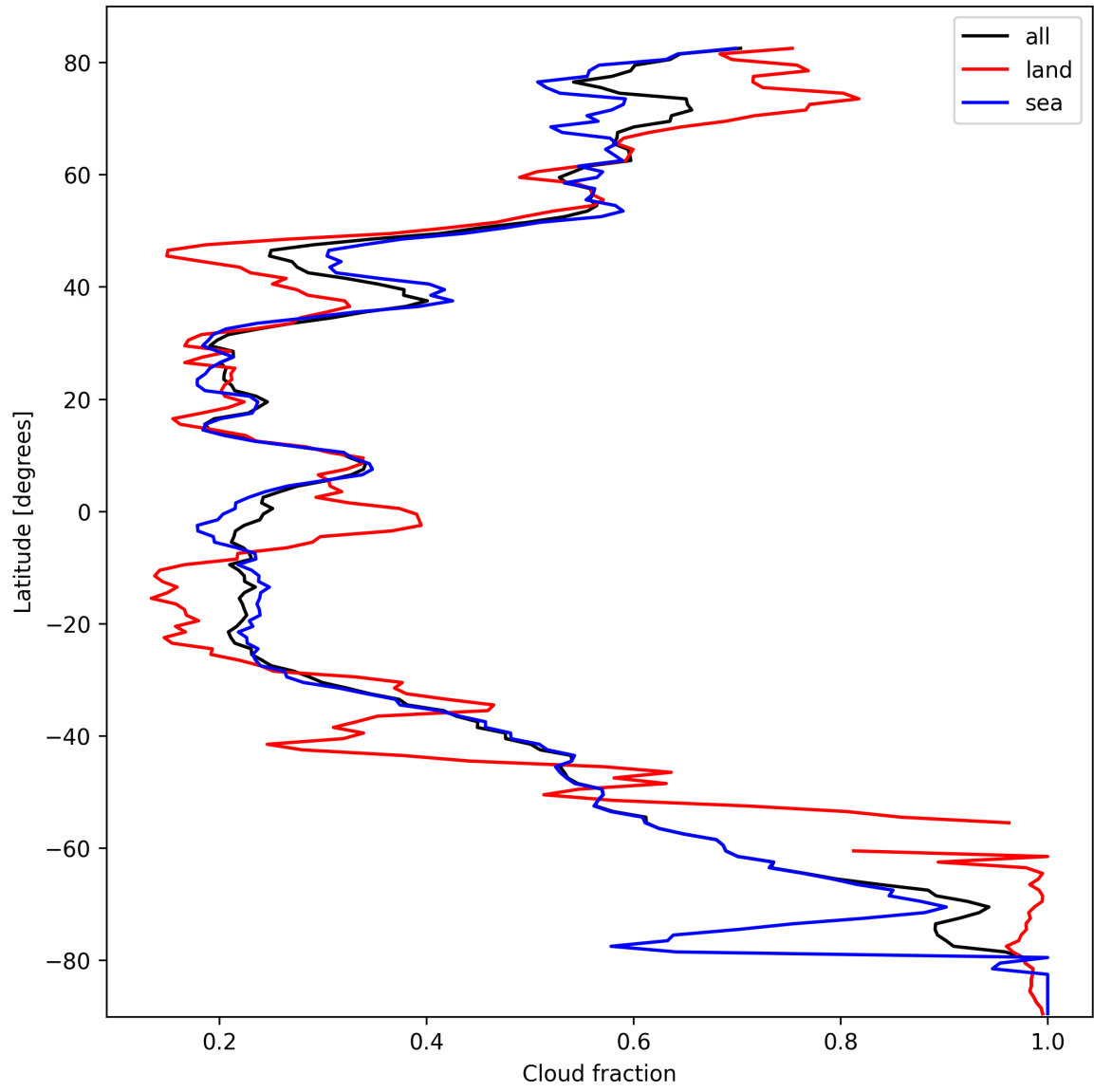
Figure 15: Zonal average of “Cloud fraction” for 2025-10-06 to 2025-10-07.
