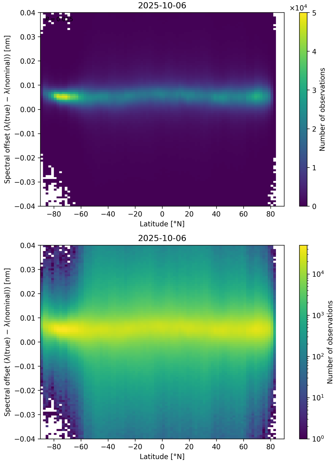
Figure 96: Scatter density plot of “Latitude” against “Spectral offset ( \lambda_{\text{true}} - \lambda_{\text{nominal}} )” for 2025-10-06 to 2025-10-07.
