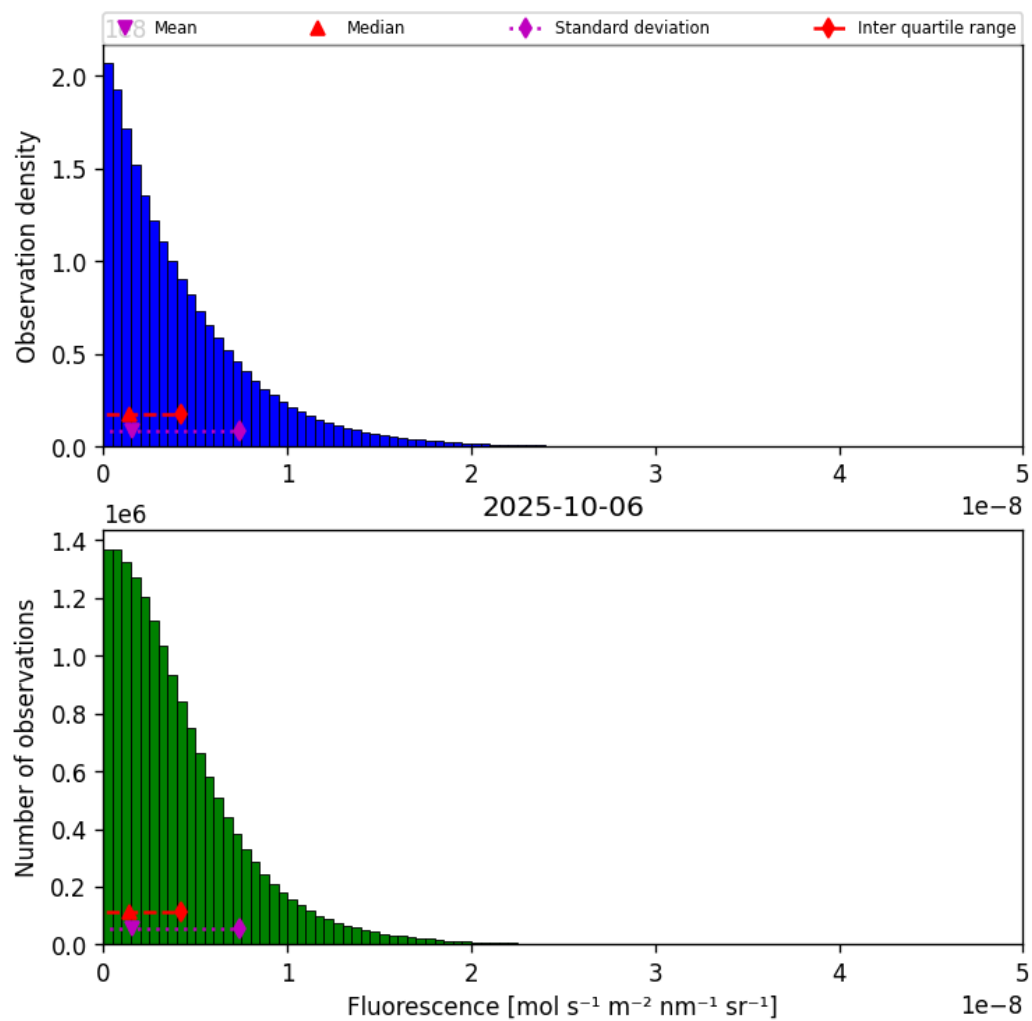
Figure 40: Histogram of “Fluorescence” for 2025-10-06 to 2025-10-07
