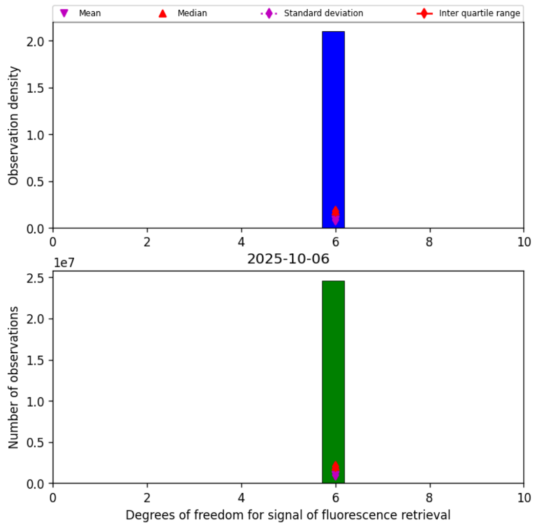
Figure 43: Histogram of "Degrees of freedom for signal of fluorescence retrieval" for 2025-10-06 to 2025-10-07
