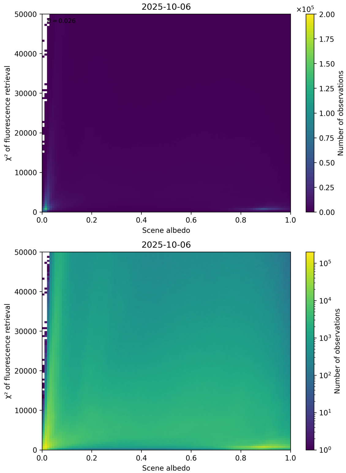
Figure 103: Scatter density plot of “Scene albedo” against “ \chi^2 of fluorescence retrieval” for 2025-10-06 to 2025-10-07.
