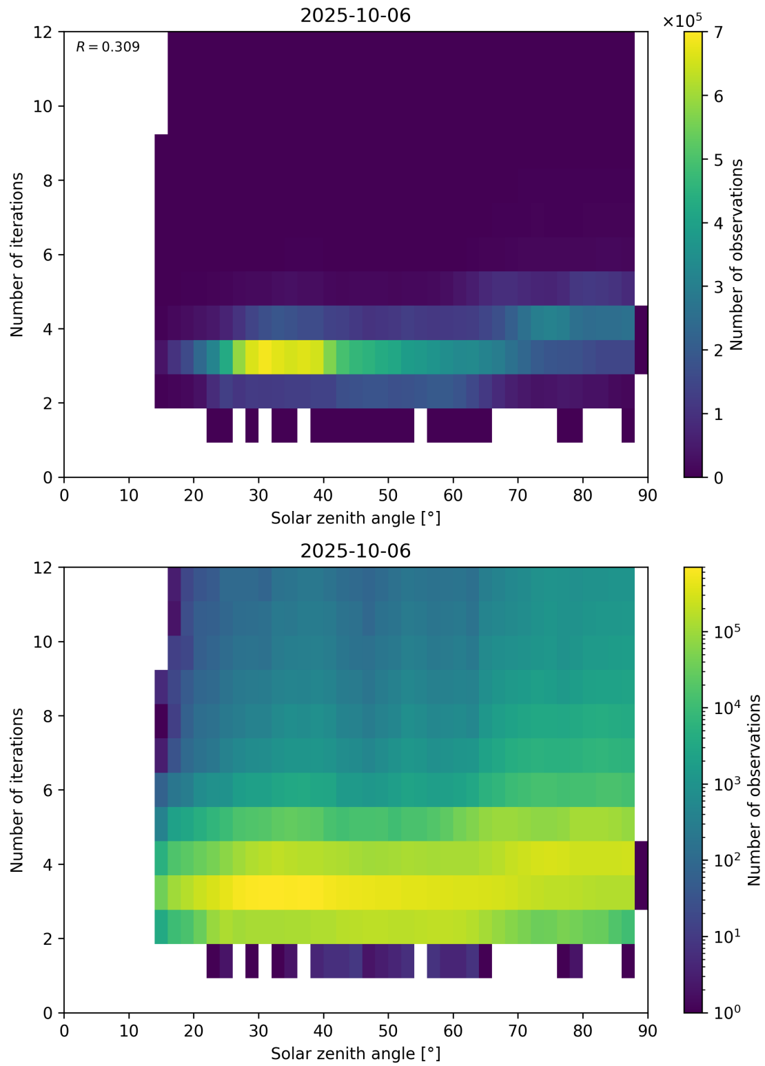
Figure 114: Scatter density plot of “Solar zenith angle” against “Number of iterations” for 2025-10-06 to 2025-10-07.
