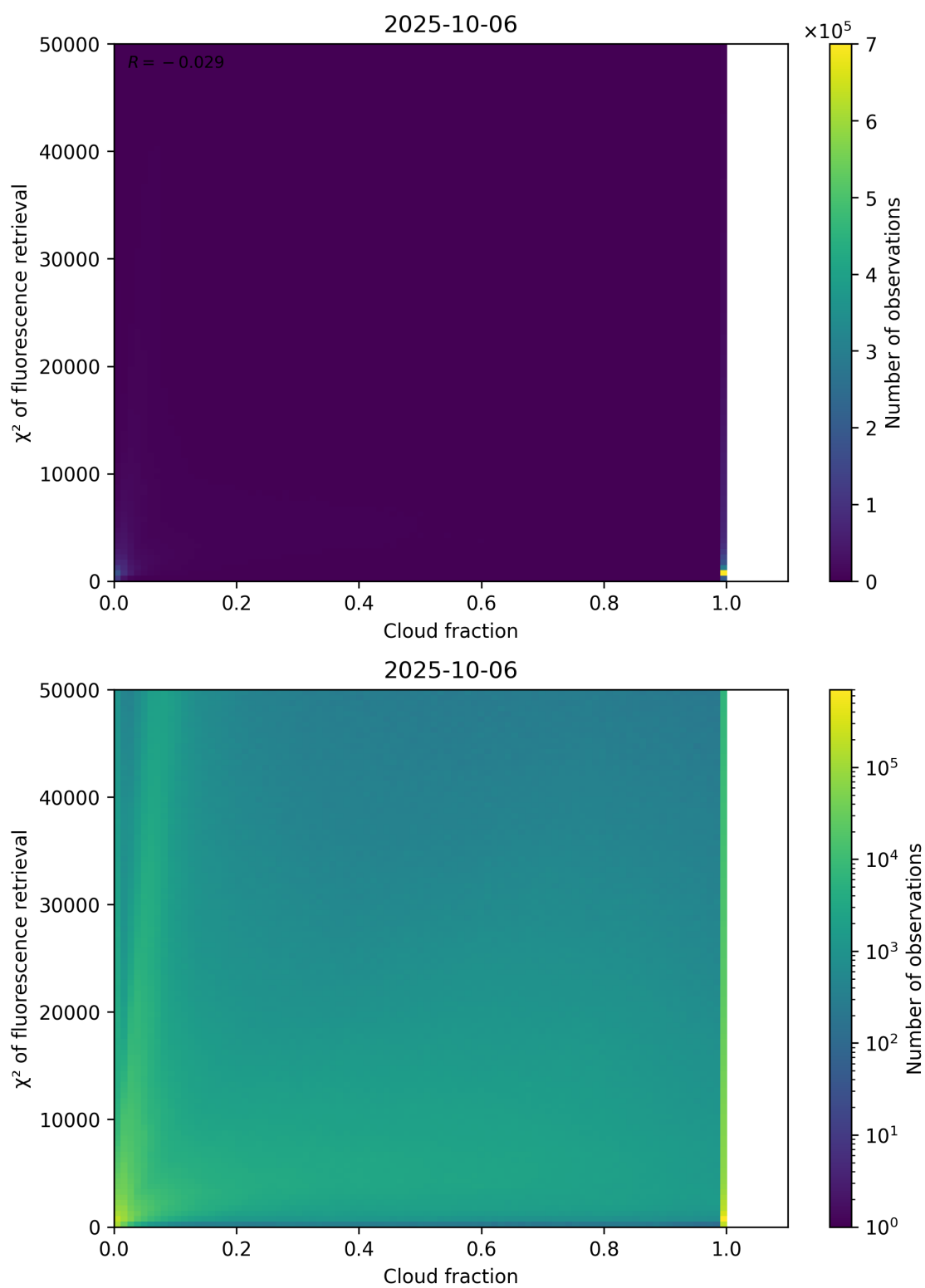
Figure 71: Scatter density plot of “Cloud fraction” against “ \chi^2 of fluorescence retrieval” for 2025-10-06 to 2025-10-07.
