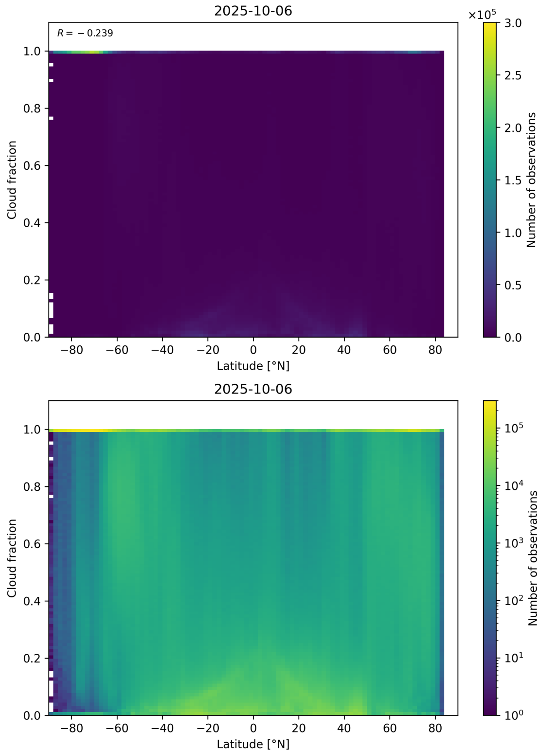
Figure 90: Scatter density plot of “Latitude” against “Cloud fraction” for 2025-10-06 to 2025-10-07.
