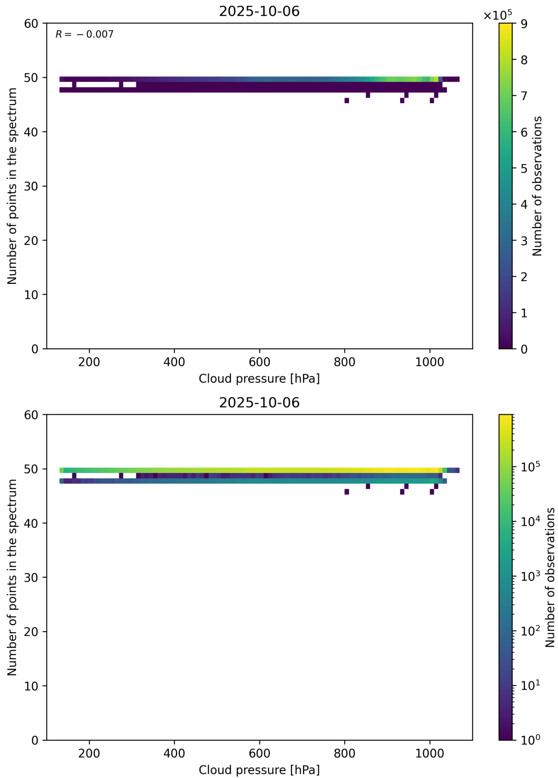
Figure 82: Scatter density plot of “Cloud pressure” against “Number of points in the spectrum” for 2025-10-06 to 2025-10-07.
