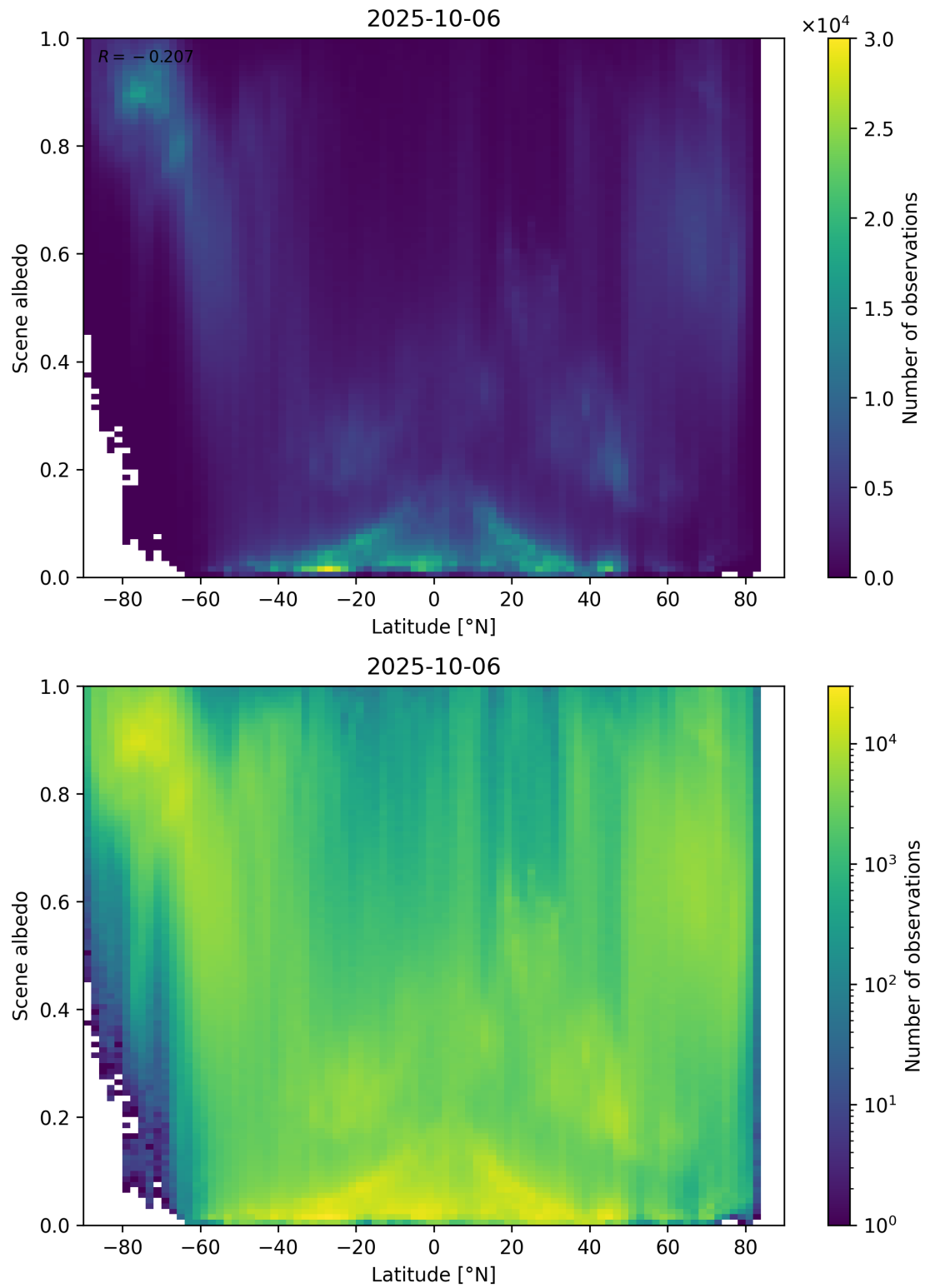
Figure 95: Scatter density plot of “Latitude” against “Scene albedo” for 2025-10-06 to 2025-10-07.
