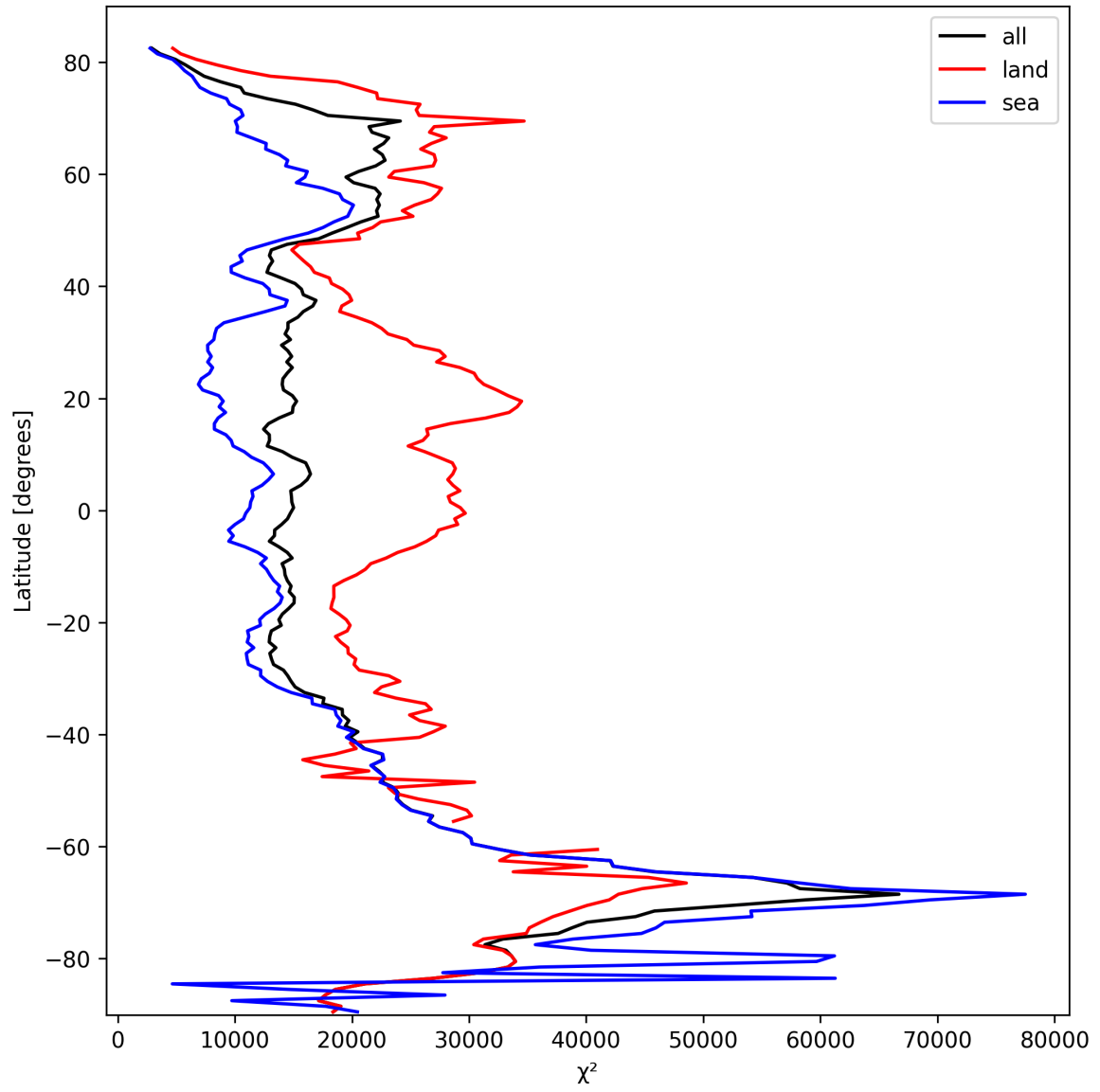
Figure 21: Zonal average of “ \chi^2 ” for 2025-10-06 to 2025-10-07.
