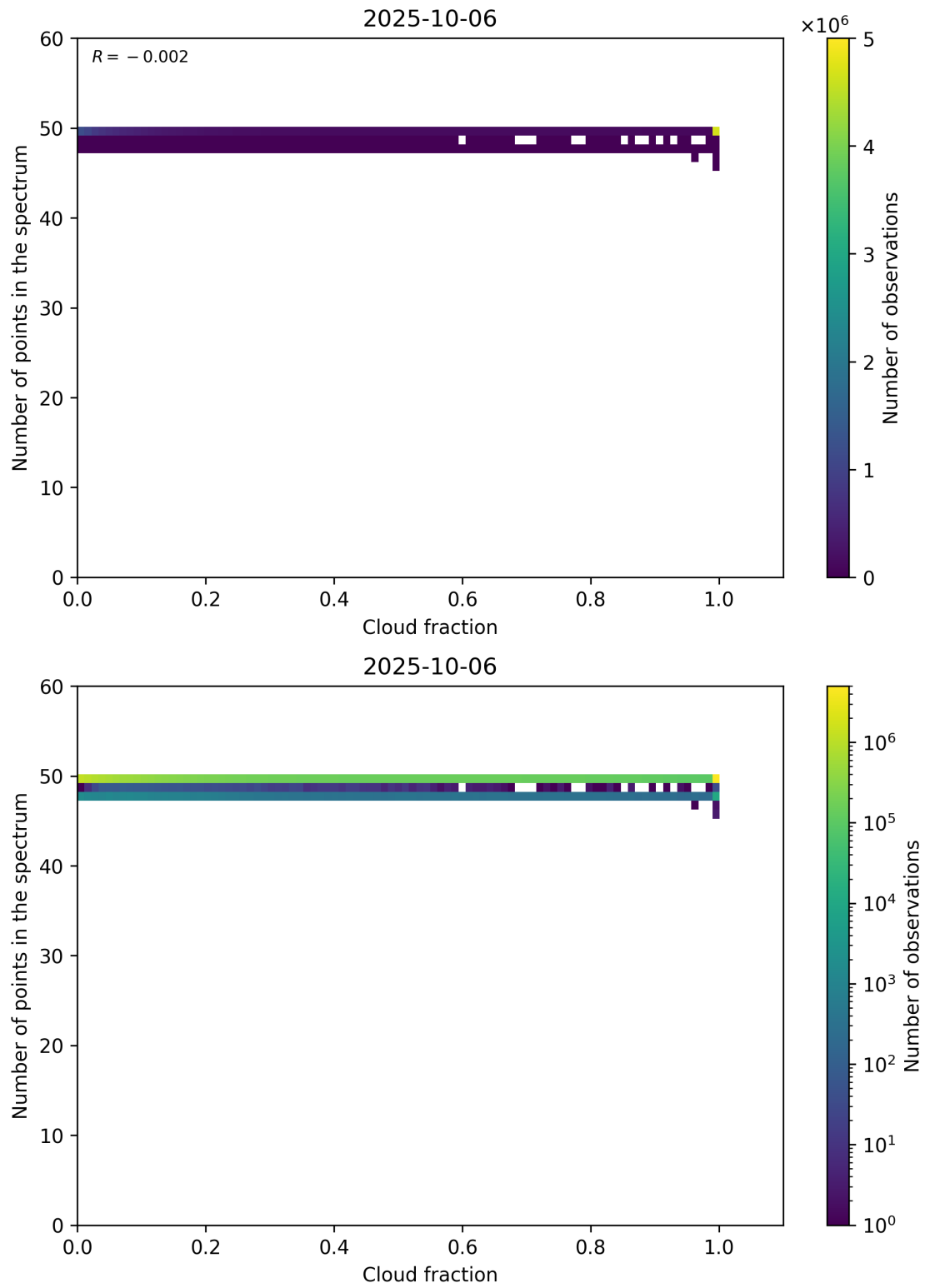
Figure 74: Scatter density plot of “Cloud fraction” against “Number of points in the spectrum” for 2025-10-06 to 2025-10-07.
