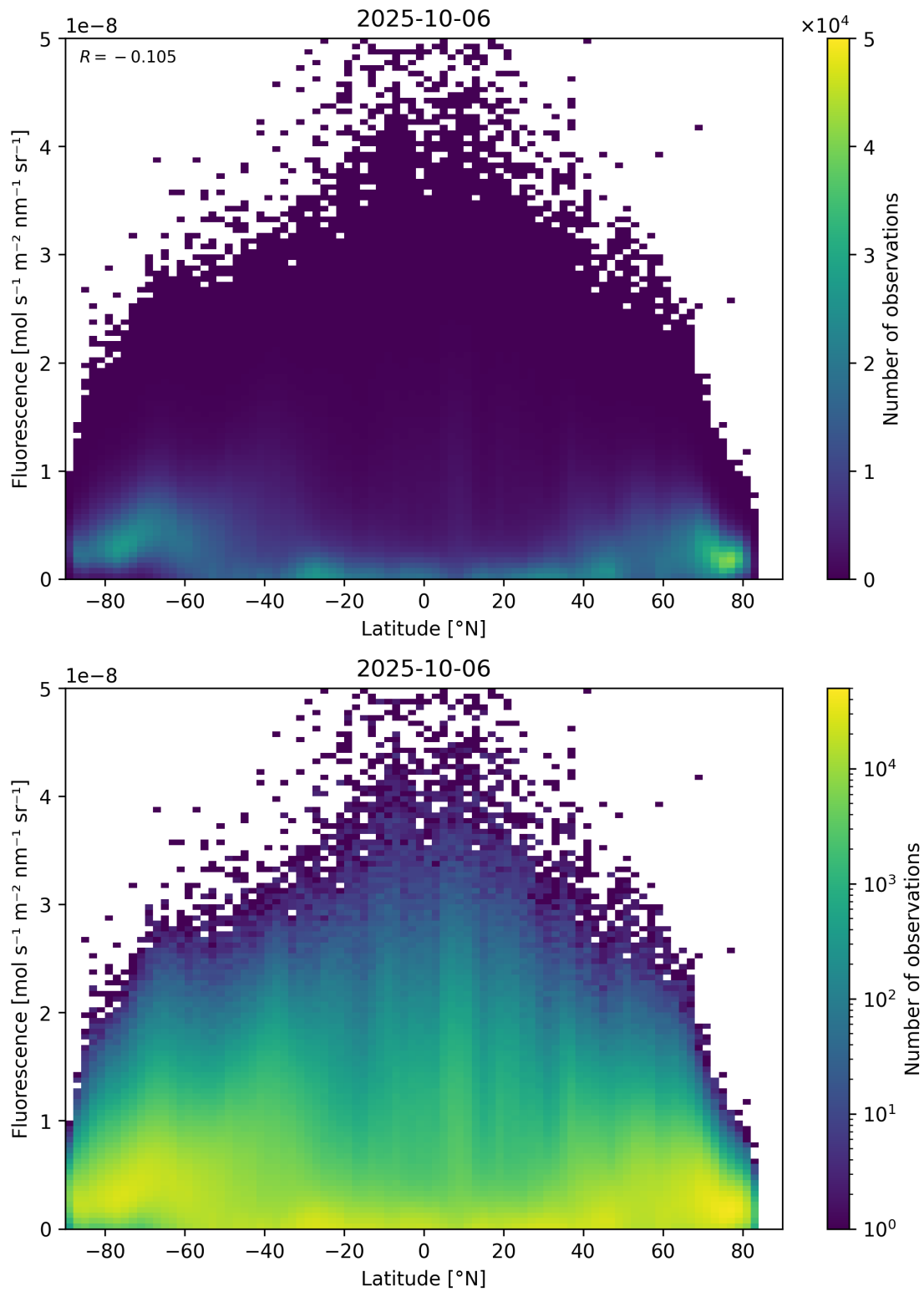
Figure 92: Scatter density plot of “Latitude” against “Fluorescence” for 2025-10-06 to 2025-10-07.
