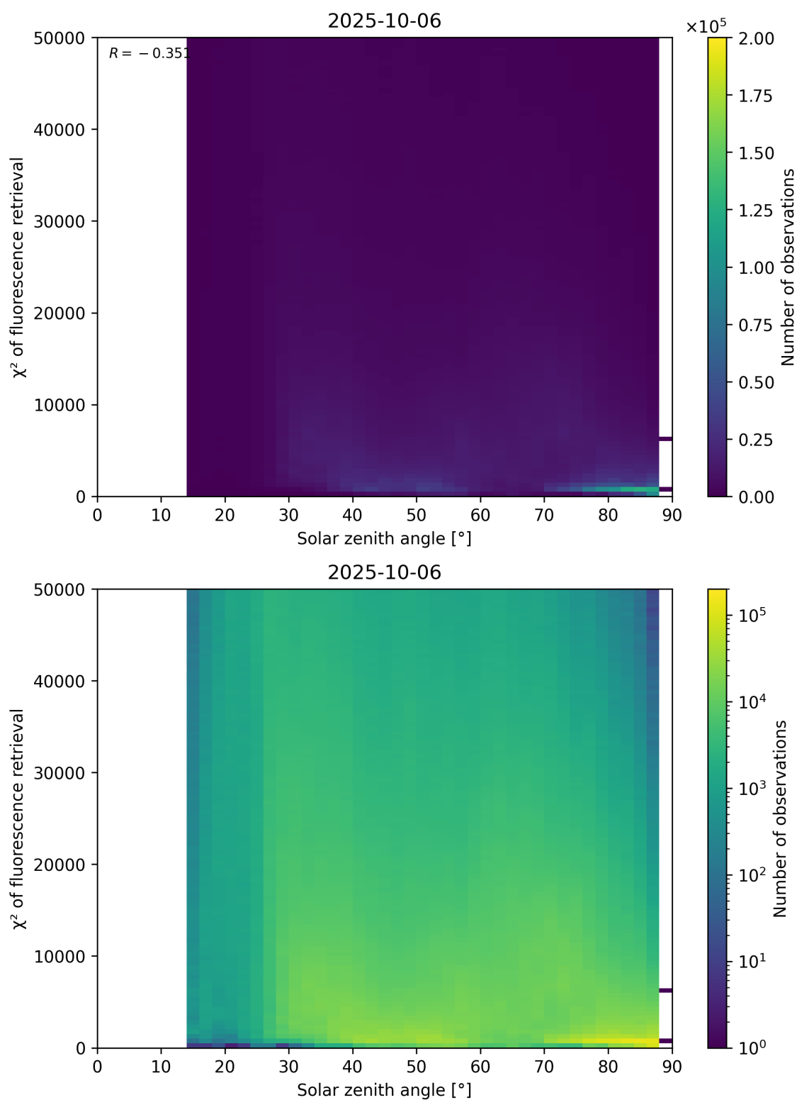
Figure 109: Scatter density plot of “Solar zenith angle” against “ \chi^2 of fluorescence retrieval” for 2025-10-06 to 2025-10-07.
