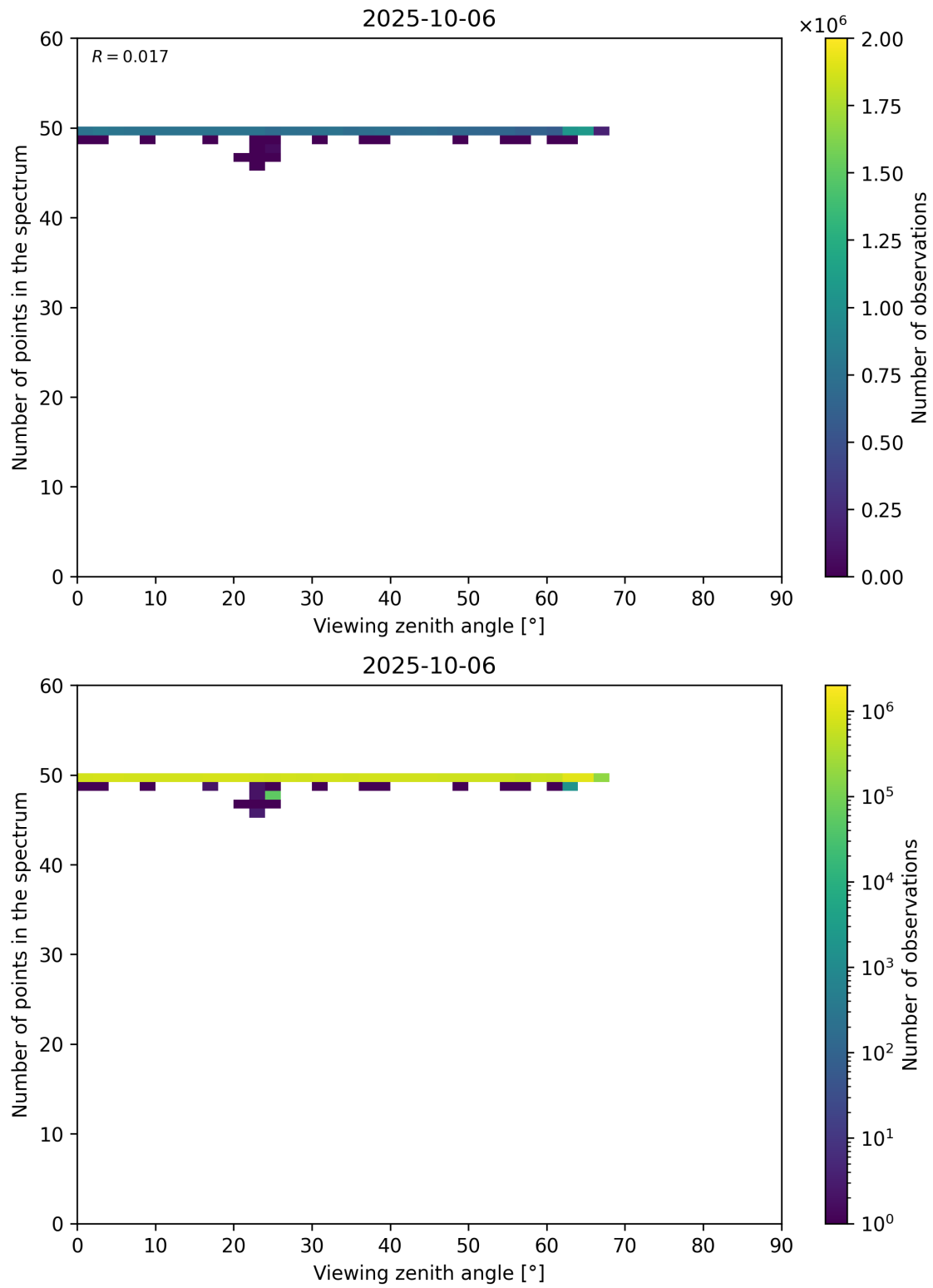
Figure 125: Scatter density plot of “Viewing zenith angle” against “Number of points in the spectrum” for 2025-10-06 to 2025-10-07.
