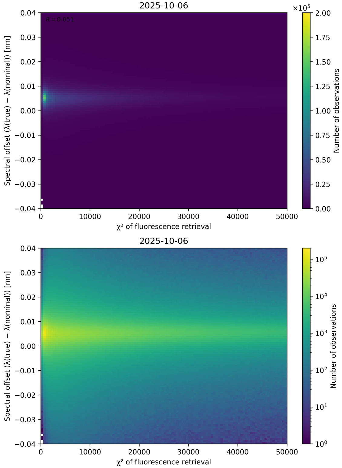
Figure 69: Scatter density plot of “ \chi^2 of fluorescence retrieval” against “Spectral offset ( \lambda_{\text{true}} - \lambda_{\text{nominal}} )” for 2025-10-06 to 2025-10-07.
