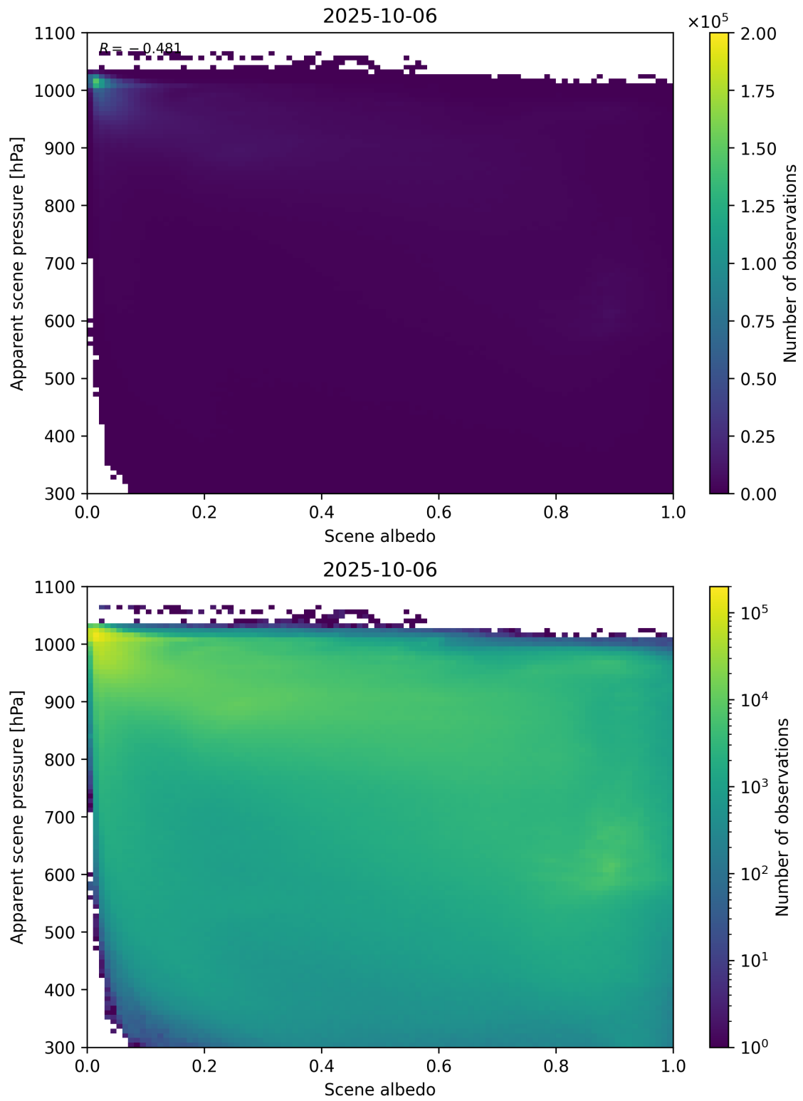
Figure 102: Scatter density plot of “Scene albedo” against “Apparent scene pressure” for 2025-10-06 to 2025-10-07.
