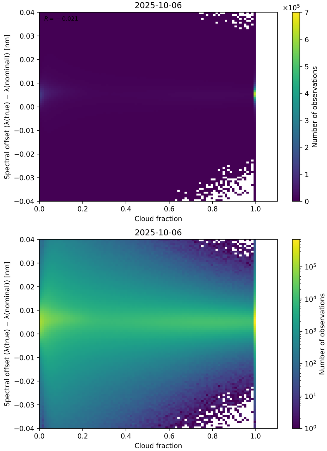
Figure 76: Scatter density plot of “Cloud fraction” against “Spectral offset ( \lambda_{\text{true}} - \lambda_{\text{nominal}} )” for 2025-10-06 to 2025-10-07.
