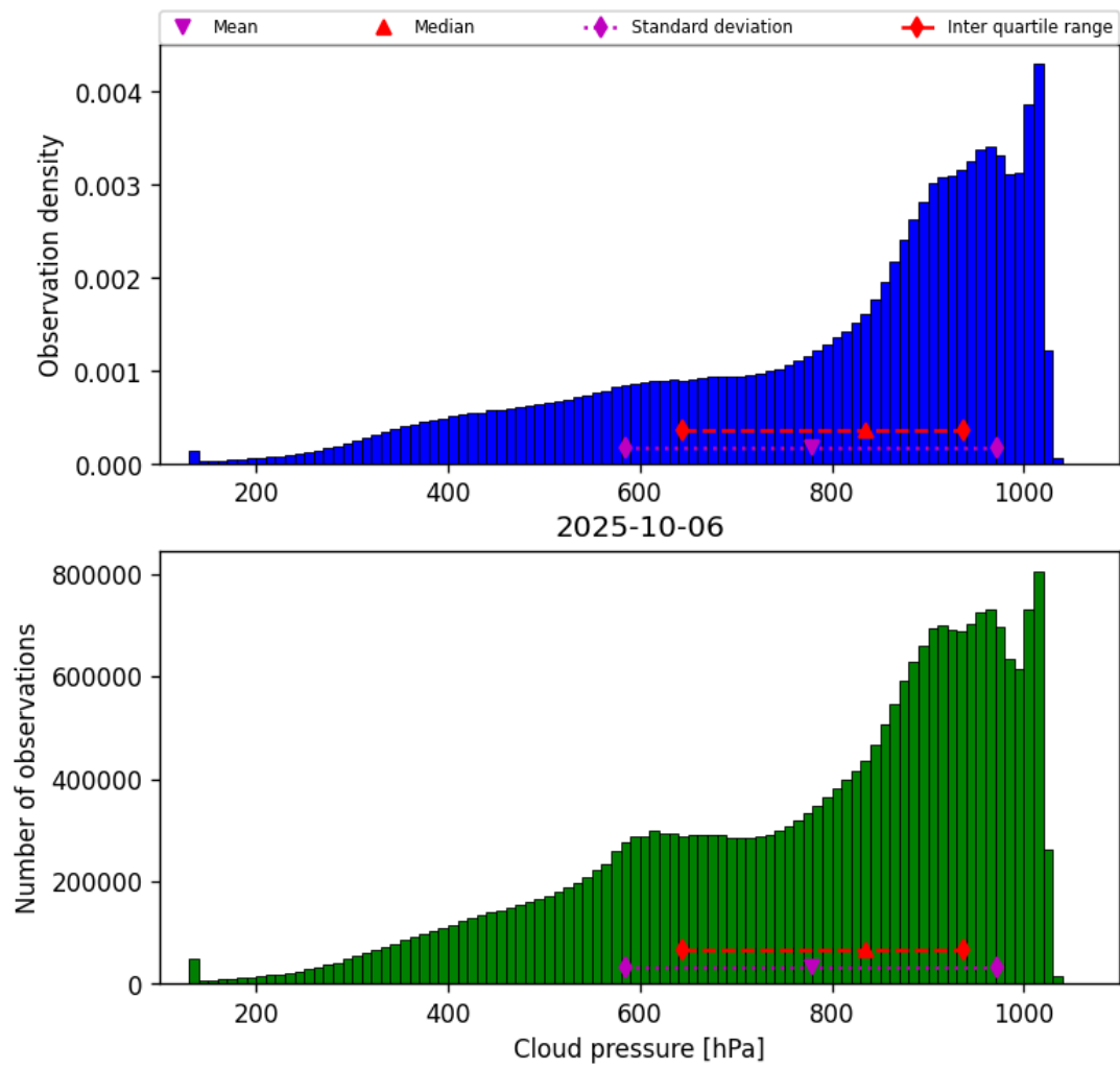
Figure 30: Histogram of “Cloud pressure” for 2025-10-06 to 2025-10-07
