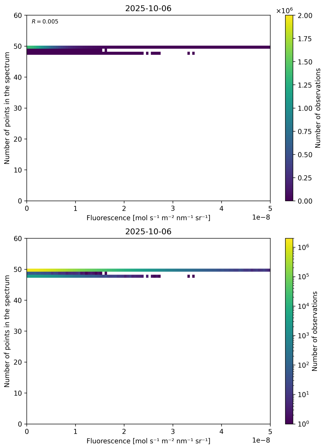
Figure 86: Scatter density plot of “Fluorescence” against “Number of points in the spectrum” for 2025-10-06 to 2025-10-07.
