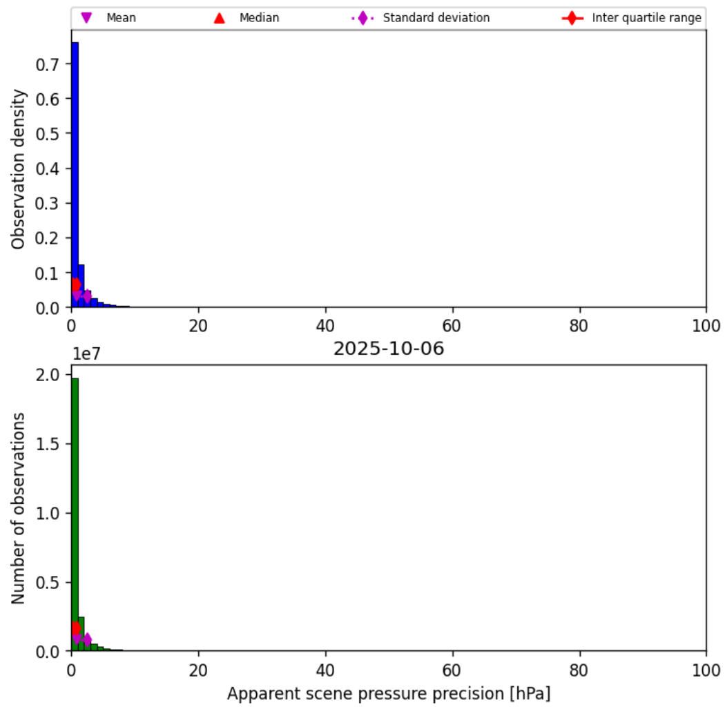
Figure 37: Histogram of “Apparent scene pressure precision” for 2025-10-06 to 2025-10-07
