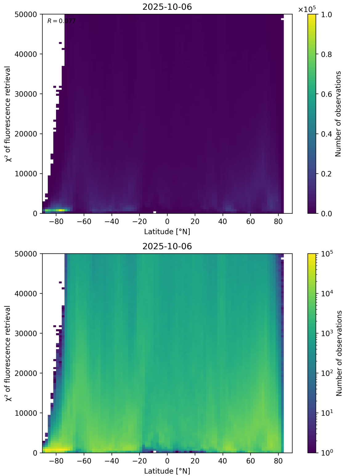
Figure 89: Scatter density plot of “Latitude” against “ \chi^2 of fluorescence retrieval” for 2025-10-06 to 2025-10-07.
