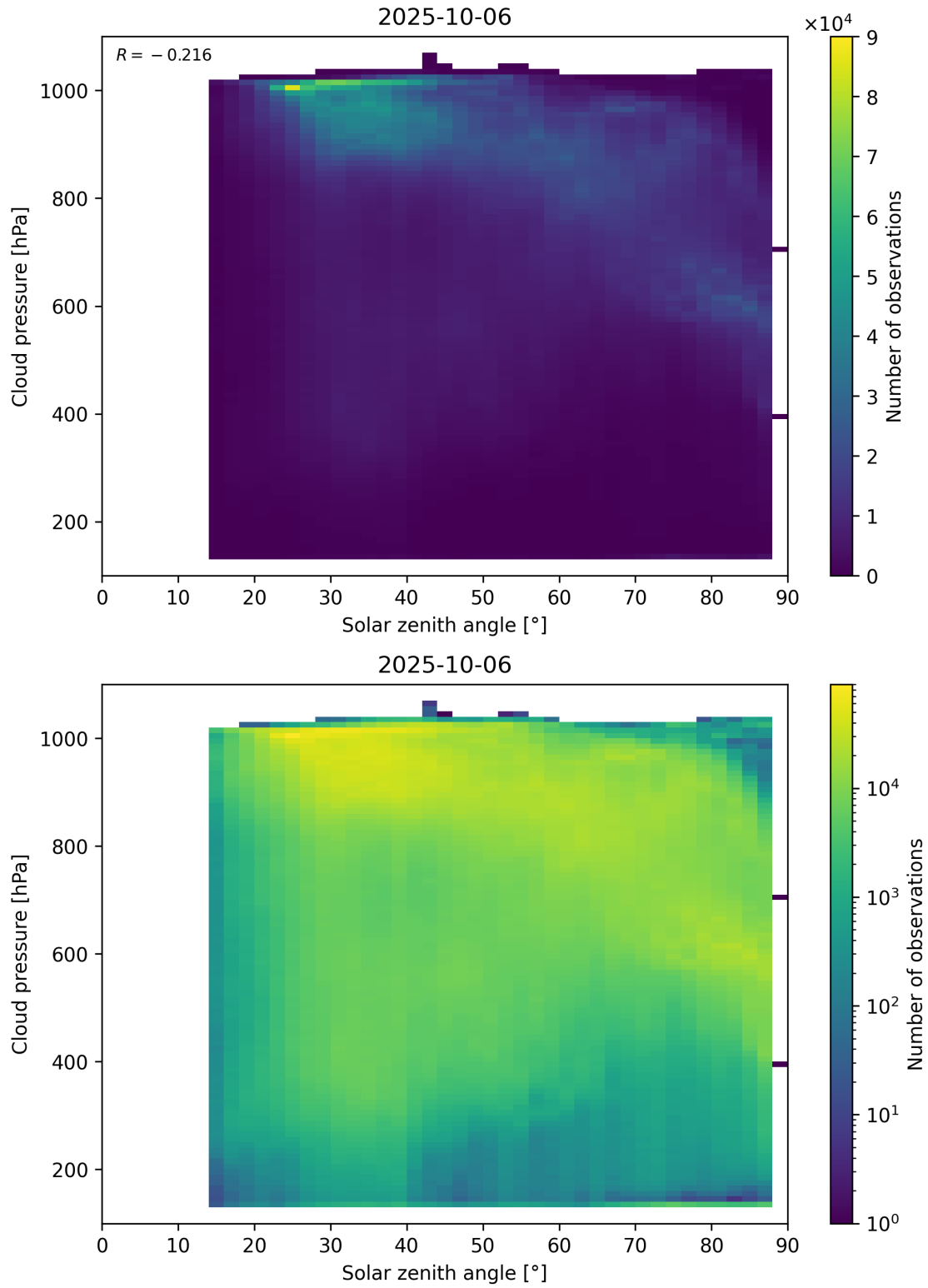
Figure 111: Scatter density plot of “Solar zenith angle” against “Cloud pressure” for 2025-10-06 to 2025-10-07.
