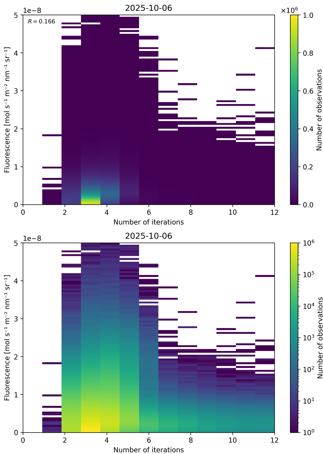
Figure 98: Scatter density plot of “Number of iterations” against “Fluorescence” for 2025-10-06 to 2025-10-07.
