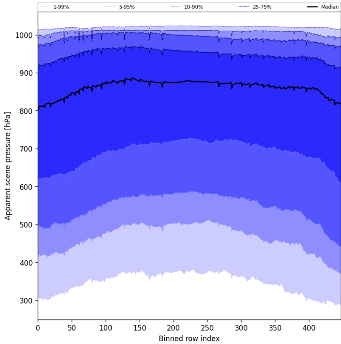
Figure 53: Along track statistics of “Apparent scene pressure” for 2025-10-06 to 2025-10-07
