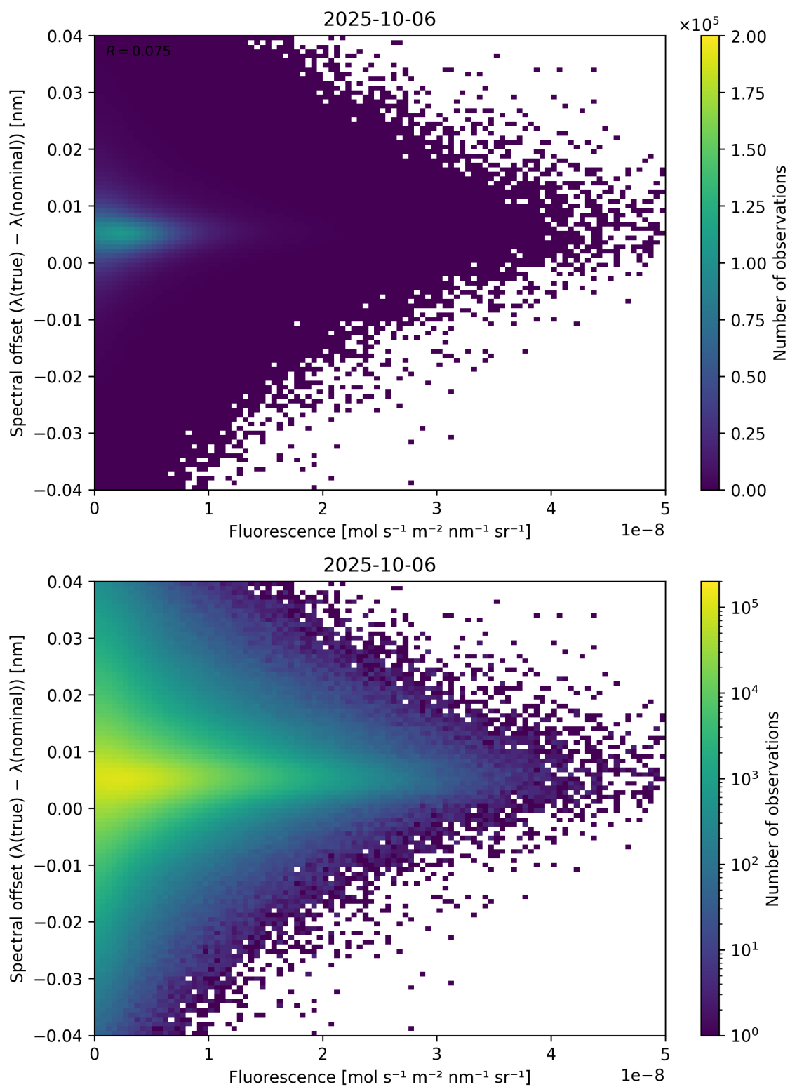
Figure 87: Scatter density plot of “Fluorescence” against “Spectral offset ( \lambda_{\text{true}} - \lambda_{\text{nominal}} )” for 2025-10-06 to 2025-10-07.
