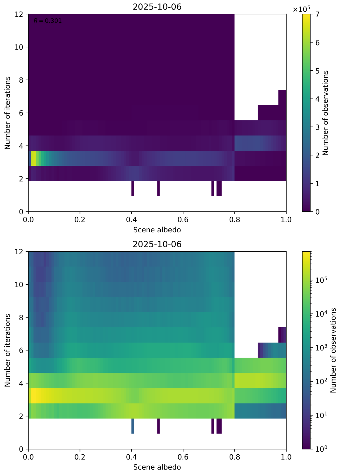
Figure 105: Scatter density plot of “Scene albedo” against “Number of iterations” for 2025-10-06 to 2025-10-07.
