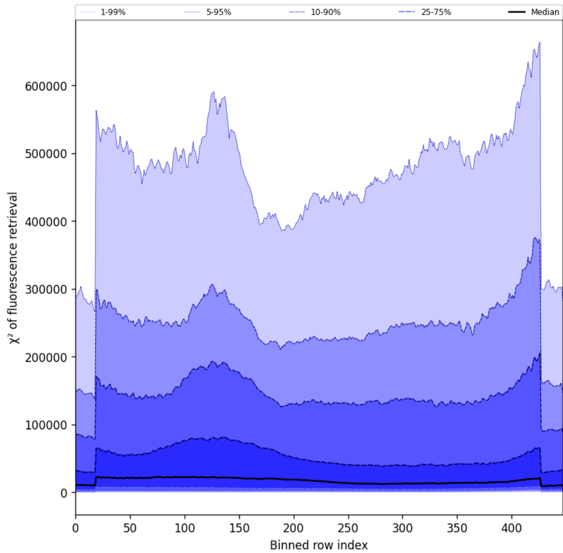
Figure 59: Along track statistics of “ \chi^2 of fluorescence retrieval” for 2025-10-06 to 2025-10-07
