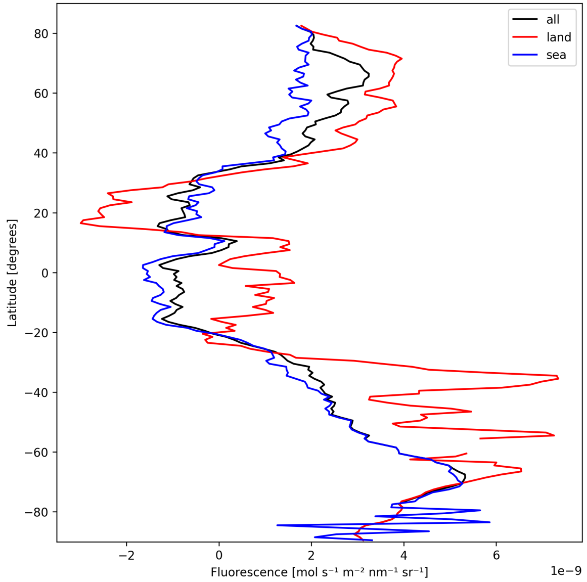
Figure 23: Zonal average of “Fluorescence” for 2025-10-06 to 2025-10-07.
