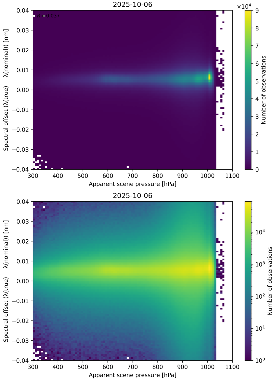
Figure 67: Scatter density plot of “Apparent scene pressure” against “Spectral offset ( \lambda_{\text{true}} - \lambda_{\text{nominal}} )” for 2025-10-06 to 2025-10-07.
