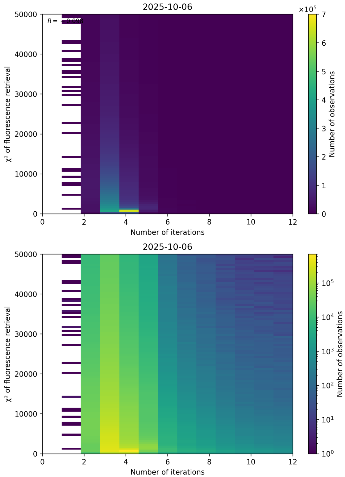
Figure 97: Scatter density plot of “Number of iterations” against “ \chi^2 of fluorescence retrieval” for 2025-10-06 to 2025-10-07.
