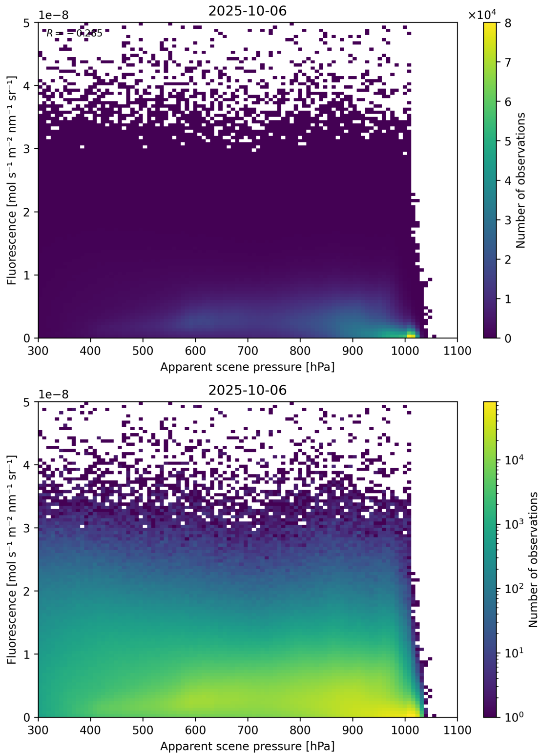
Figure 64: Scatter density plot of “Apparent scene pressure” against “Fluorescence” for 2025-10-06 to 2025-10-07.
