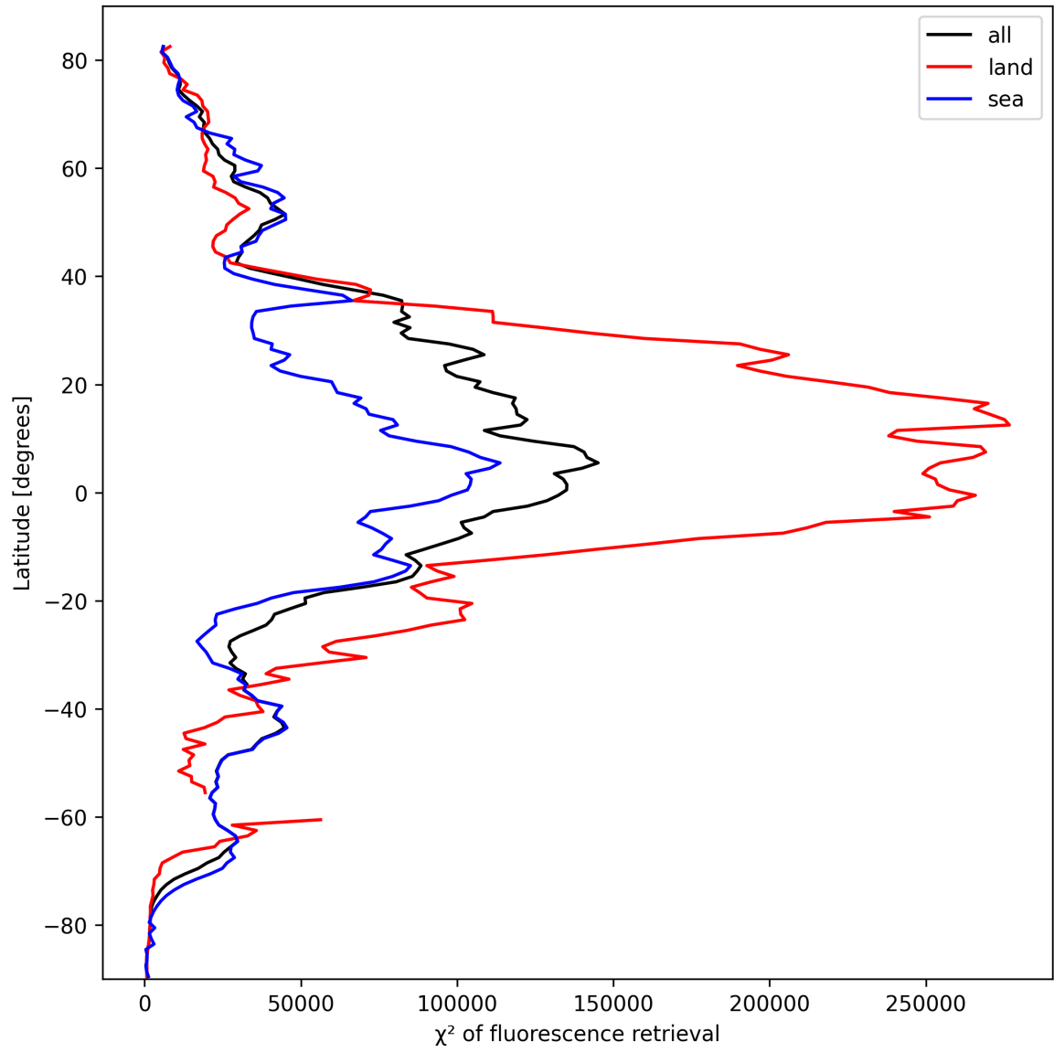
Figure 25: Zonal average of “ \chi^2 of fluorescence retrieval” for 2025-10-06 to 2025-10-07.
