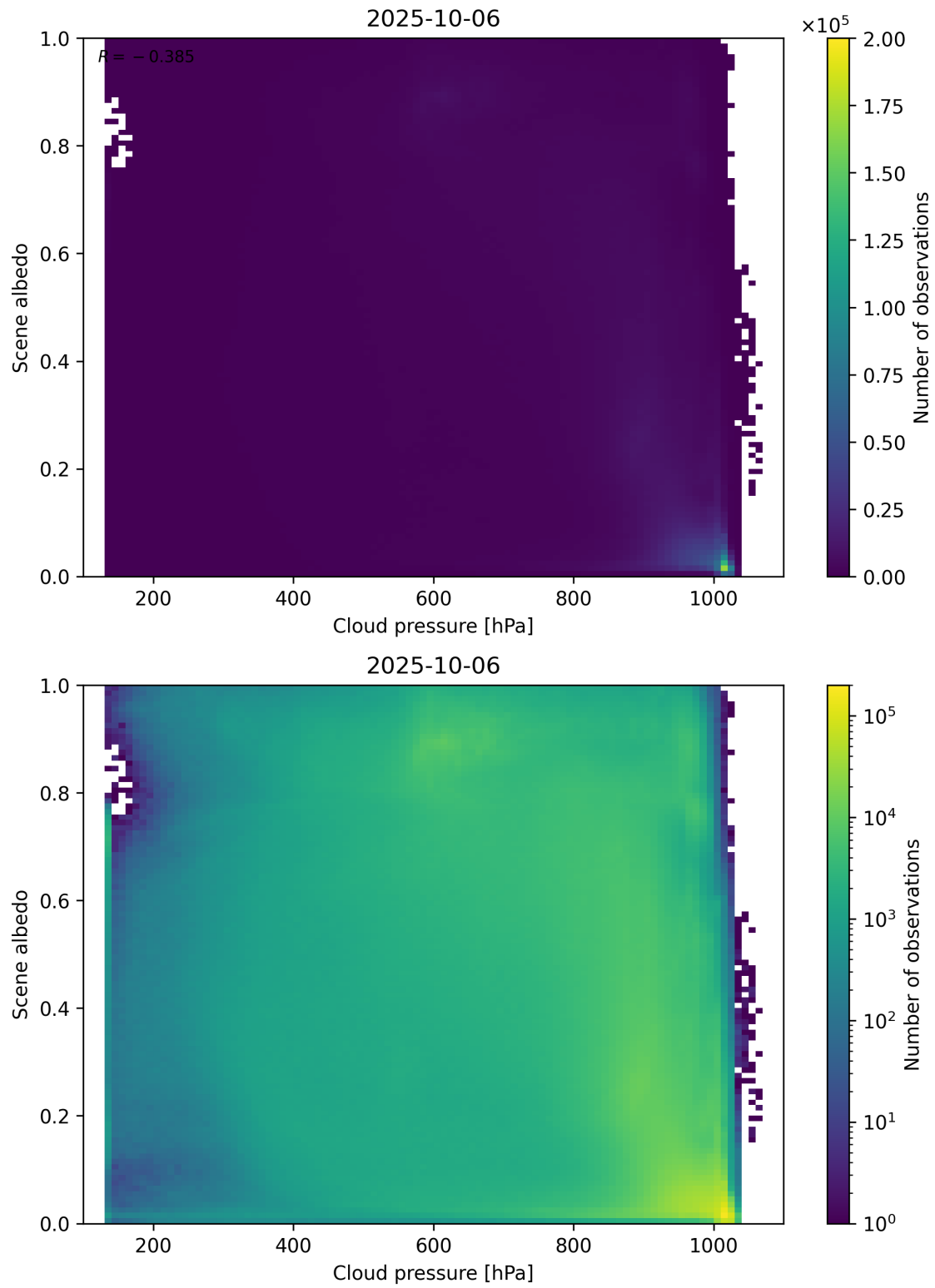
Figure 83: Scatter density plot of “Cloud pressure” against “Scene albedo” for 2025-10-06 to 2025-10-07.
