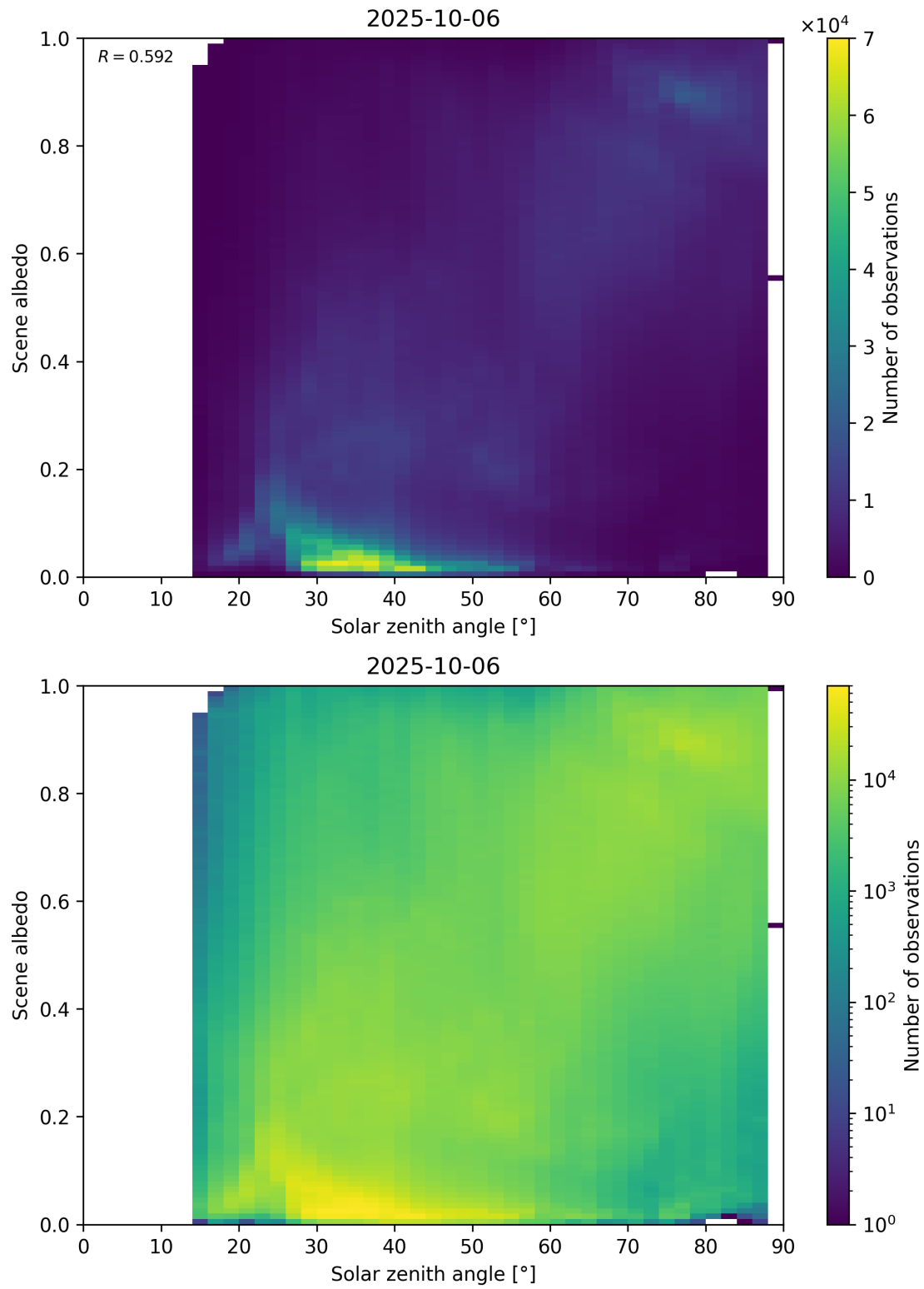
Figure 116: Scatter density plot of “Solar zenith angle” against “Scene albedo” for 2025-10-06 to 2025-10-07.
