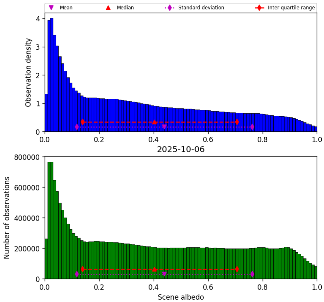
Figure 34: Histogram of “Scene albedo” for 2025-10-06 to 2025-10-07
