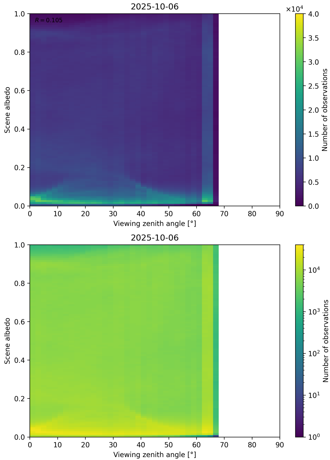
Figure 126: Scatter density plot of “Viewing zenith angle” against “Scene albedo” for 2025-10-06 to 2025-10-07.
