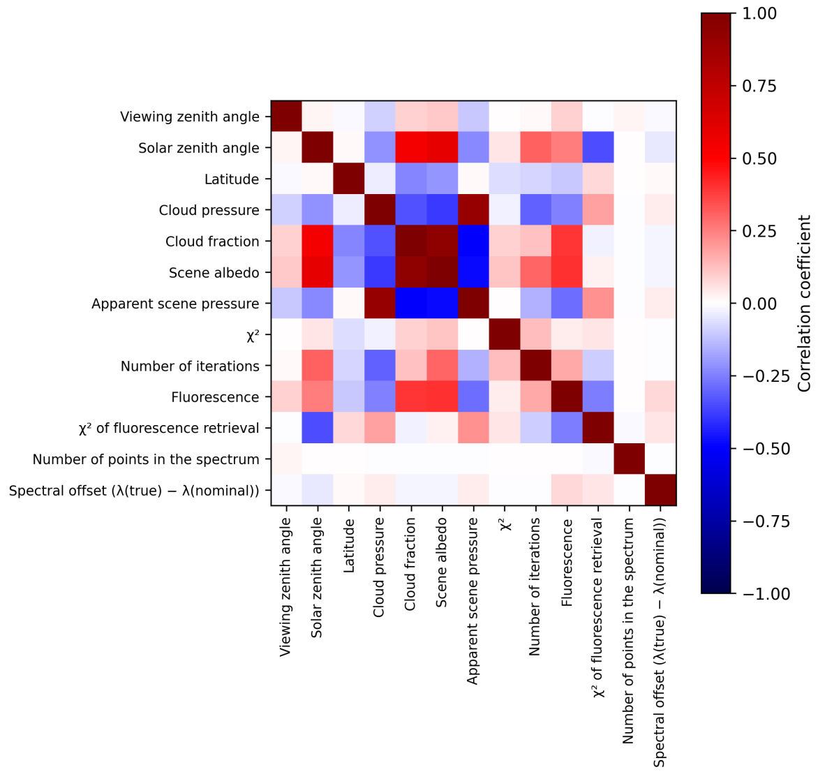
Figure 2: Map of correlation matrix for 2025-10-06 to 2025-10-07.
