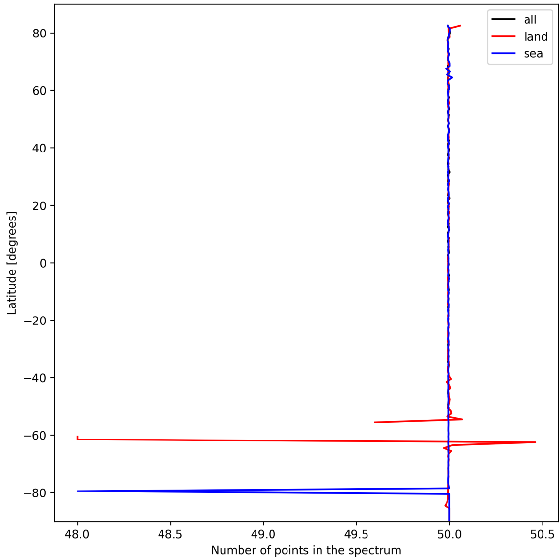
Figure 27: Zonal average of “Number of points in the spectrum” for 2025-10-06 to 2025-10-07.
