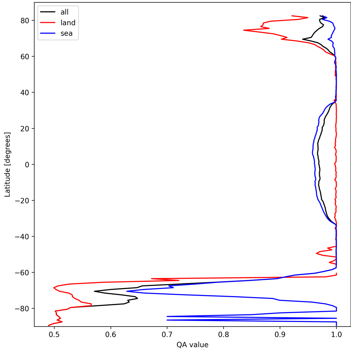
Figure 12: Zonal average of “QA value” for 2025-10-06 to 2025-10-07.
