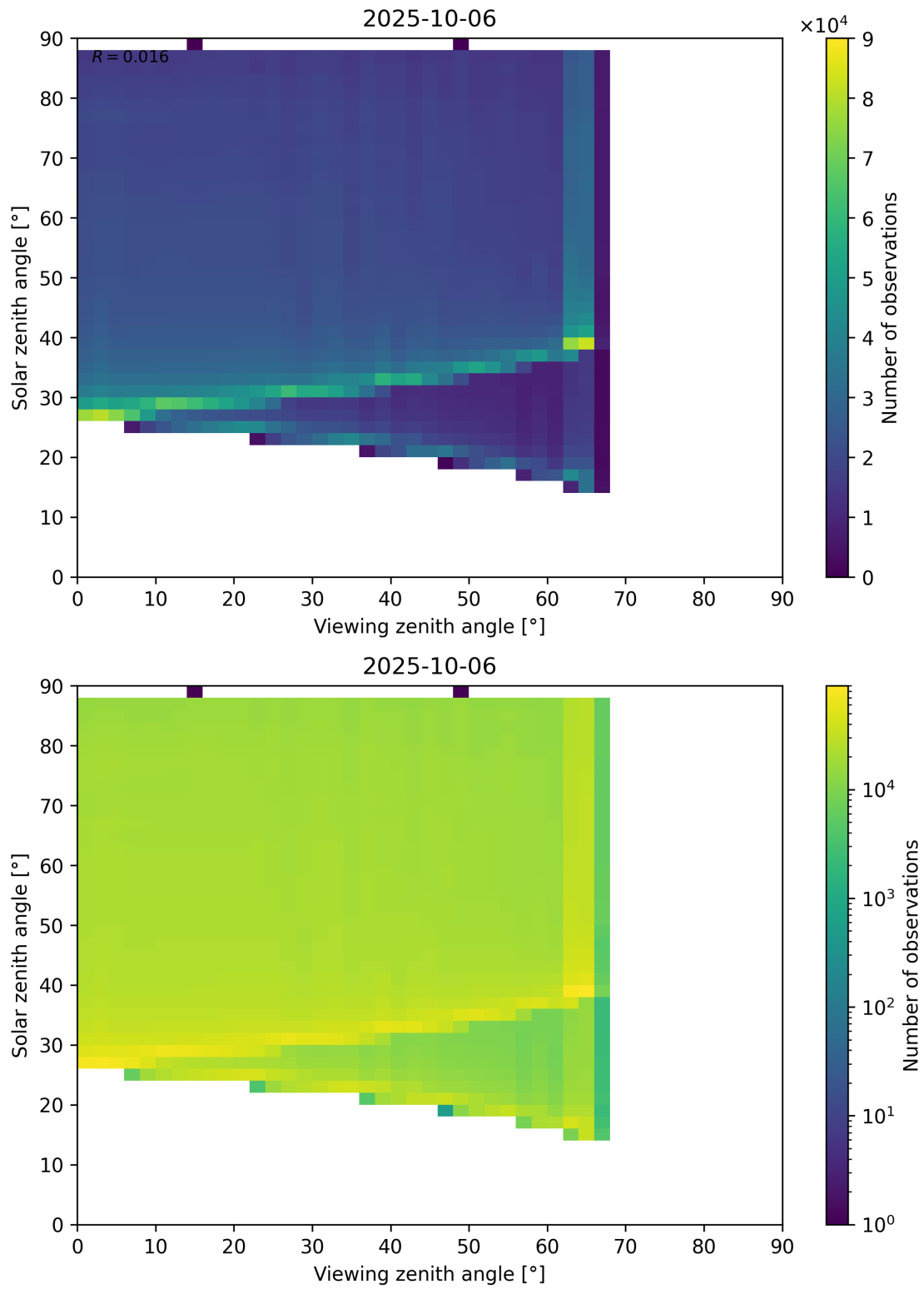
Figure 127: Scatter density plot of “Viewing zenith angle” against “Solar zenith angle” for 2025-10-06 to 2025-10-07.
