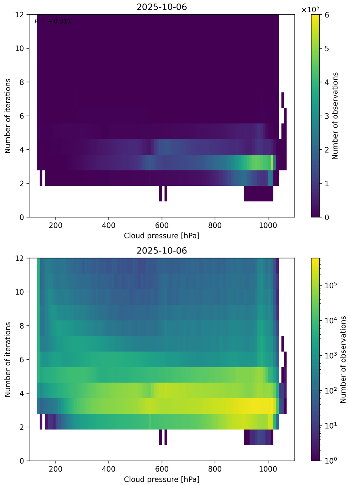
Figure 81: Scatter density plot of “Cloud pressure” against “Number of iterations” for 2025-10-06 to 2025-10-07.
