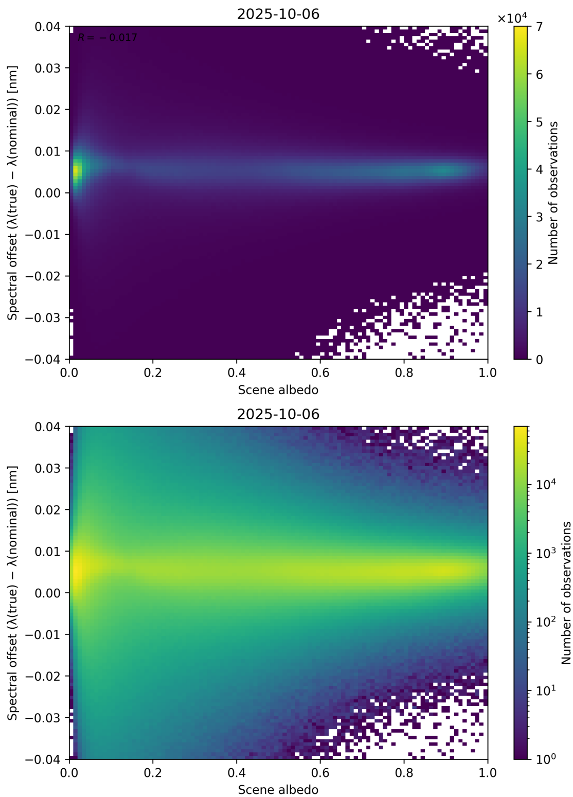
Figure 107: Scatter density plot of “Scene albedo” against “Spectral offset ( \lambda_{\text{true}} - \lambda_{\text{nominal}} )” for 2025-10-06 to 2025-10-07.
