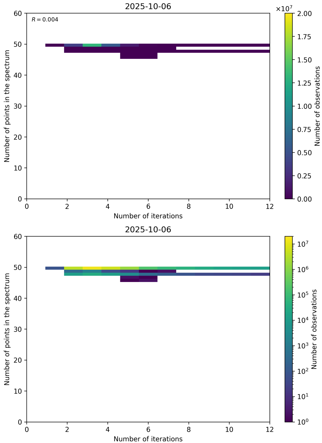
Figure 99: Scatter density plot of “Number of iterations” against “Number of points in the spectrum” for 2025-10-06 to 2025-10-07.
