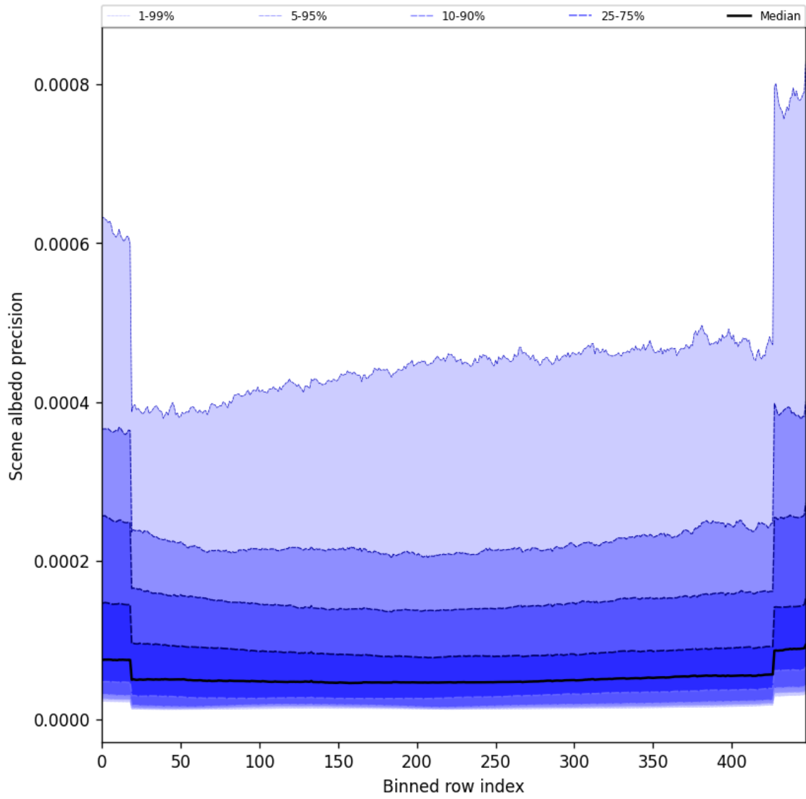
Figure 52: Along track statistics of “Scene albedo precision” for 2025-10-06 to 2025-10-07
