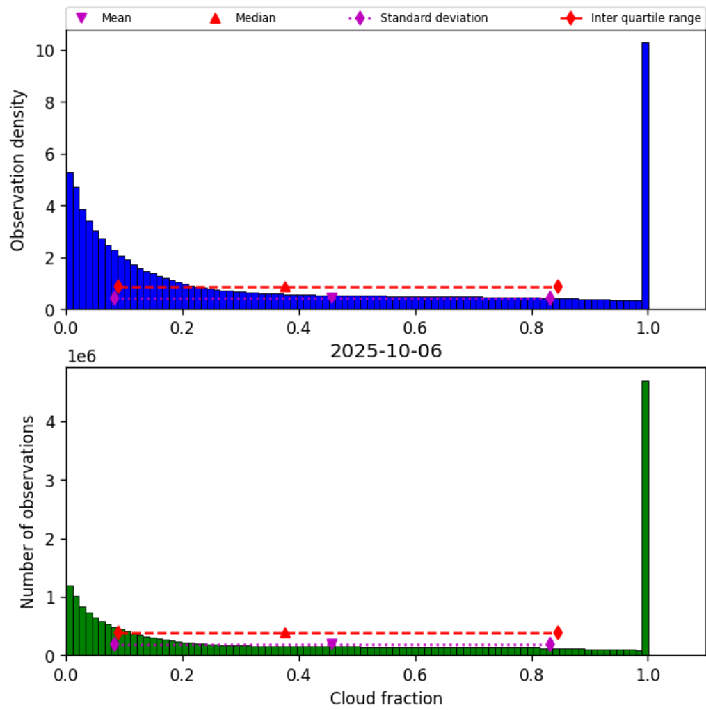
Figure 32: Histogram of “Cloud fraction” for 2025-10-06 to 2025-10-07
