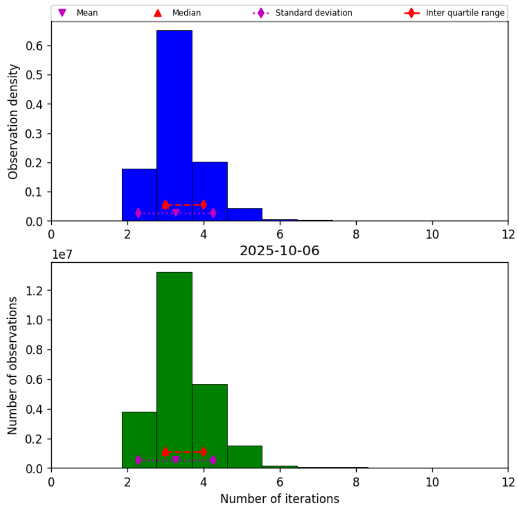
Figure 39: Histogram of “Number of iterations” for 2025-10-06 to 2025-10-07
