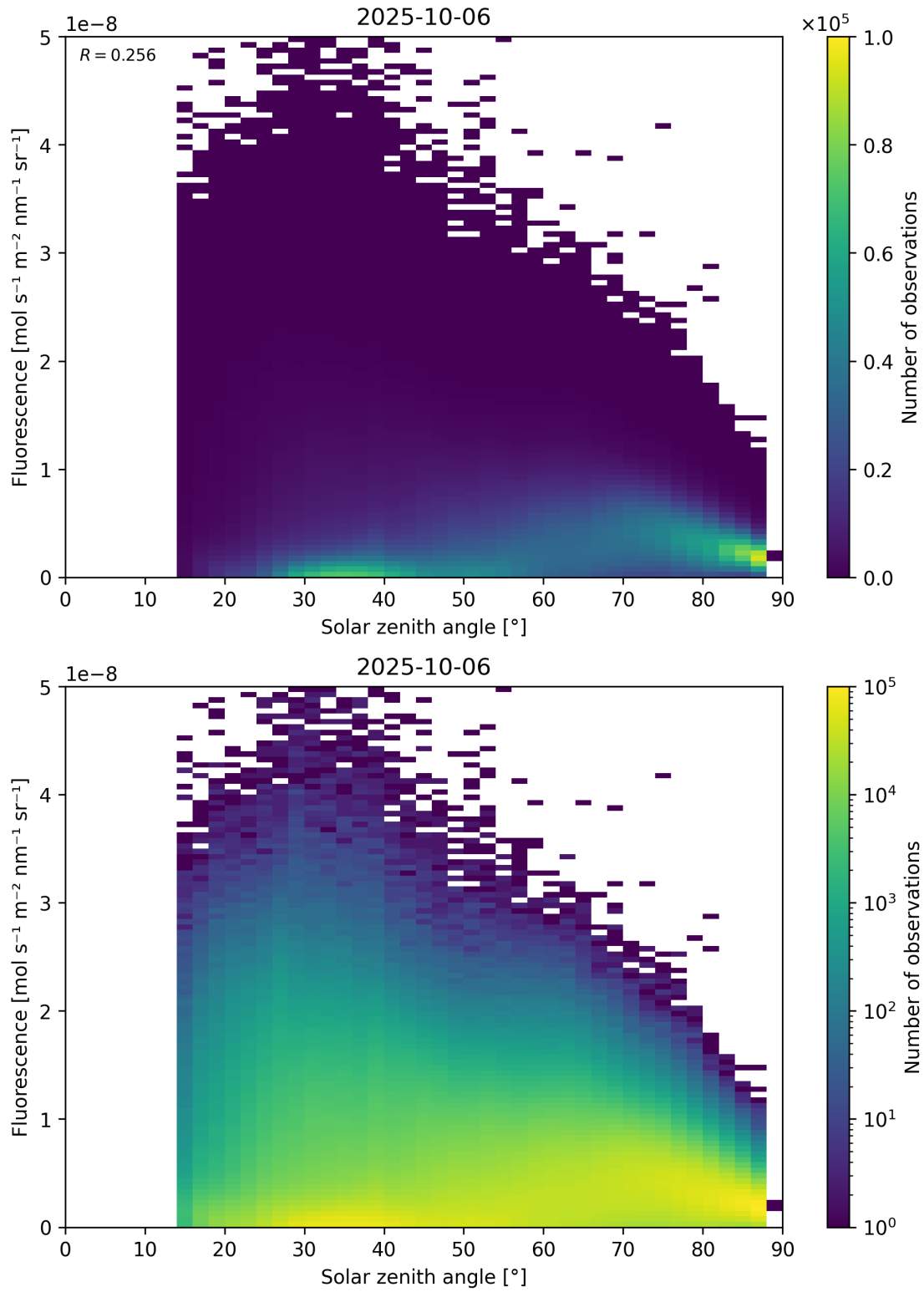
Figure 112: Scatter density plot of “Solar zenith angle” against “Fluorescence” for 2025-10-06 to 2025-10-07.
