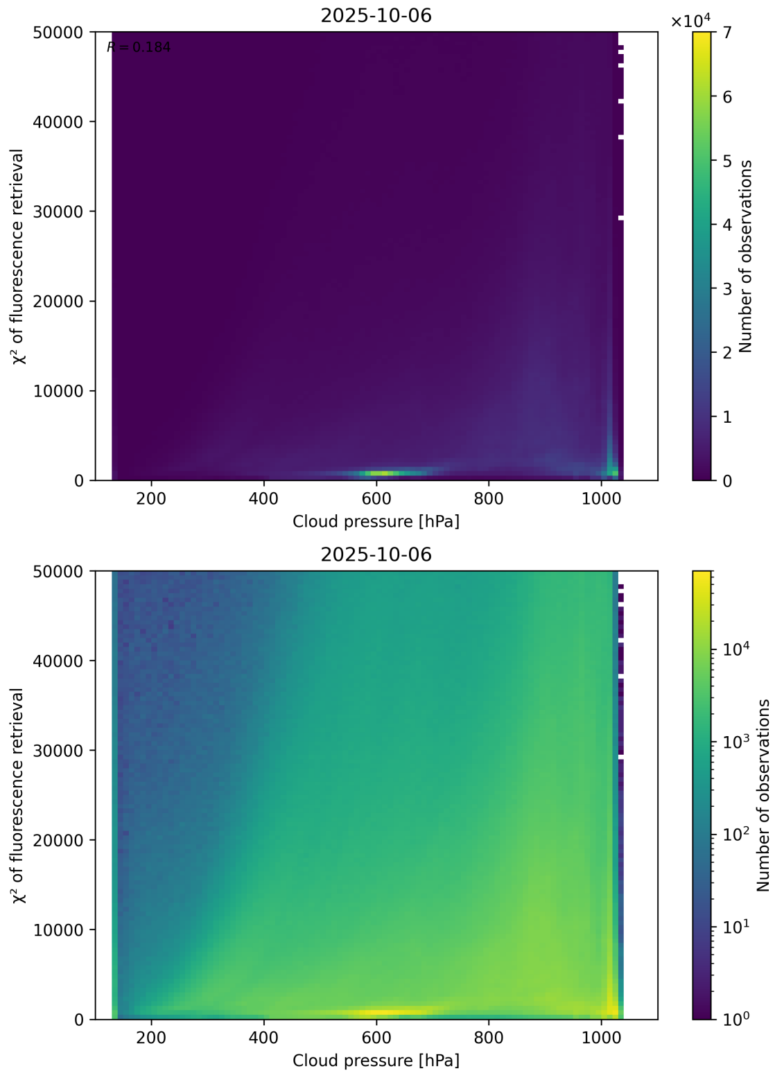
Figure 78: Scatter density plot of “Cloud pressure” against “ \chi^2 of fluorescence retrieval” for 2025-10-06 to 2025-10-07.
