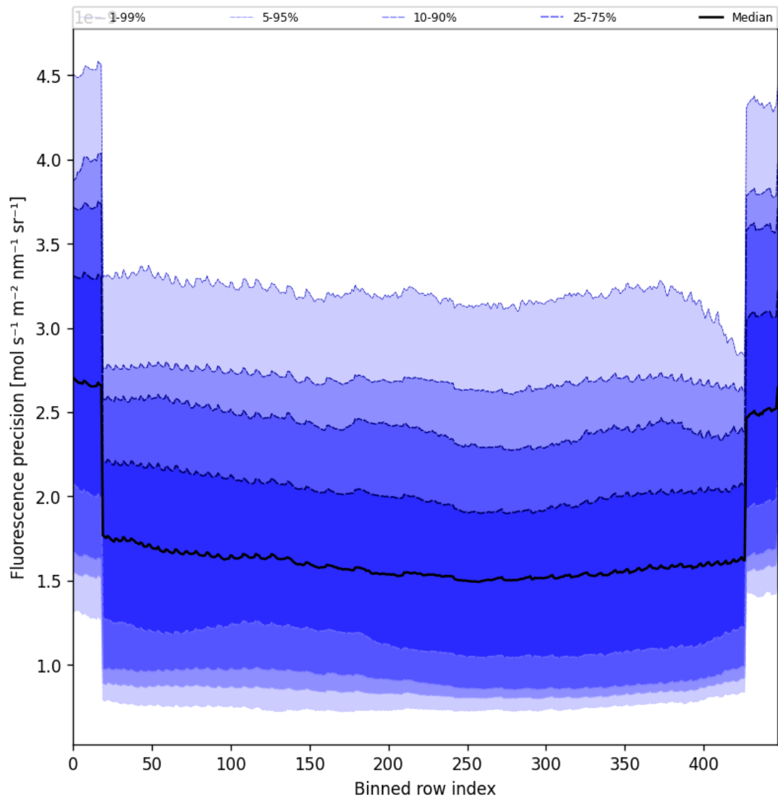
Figure 58: Along track statistics of “Fluorescence precision” for 2025-10-06 to 2025-10-07
