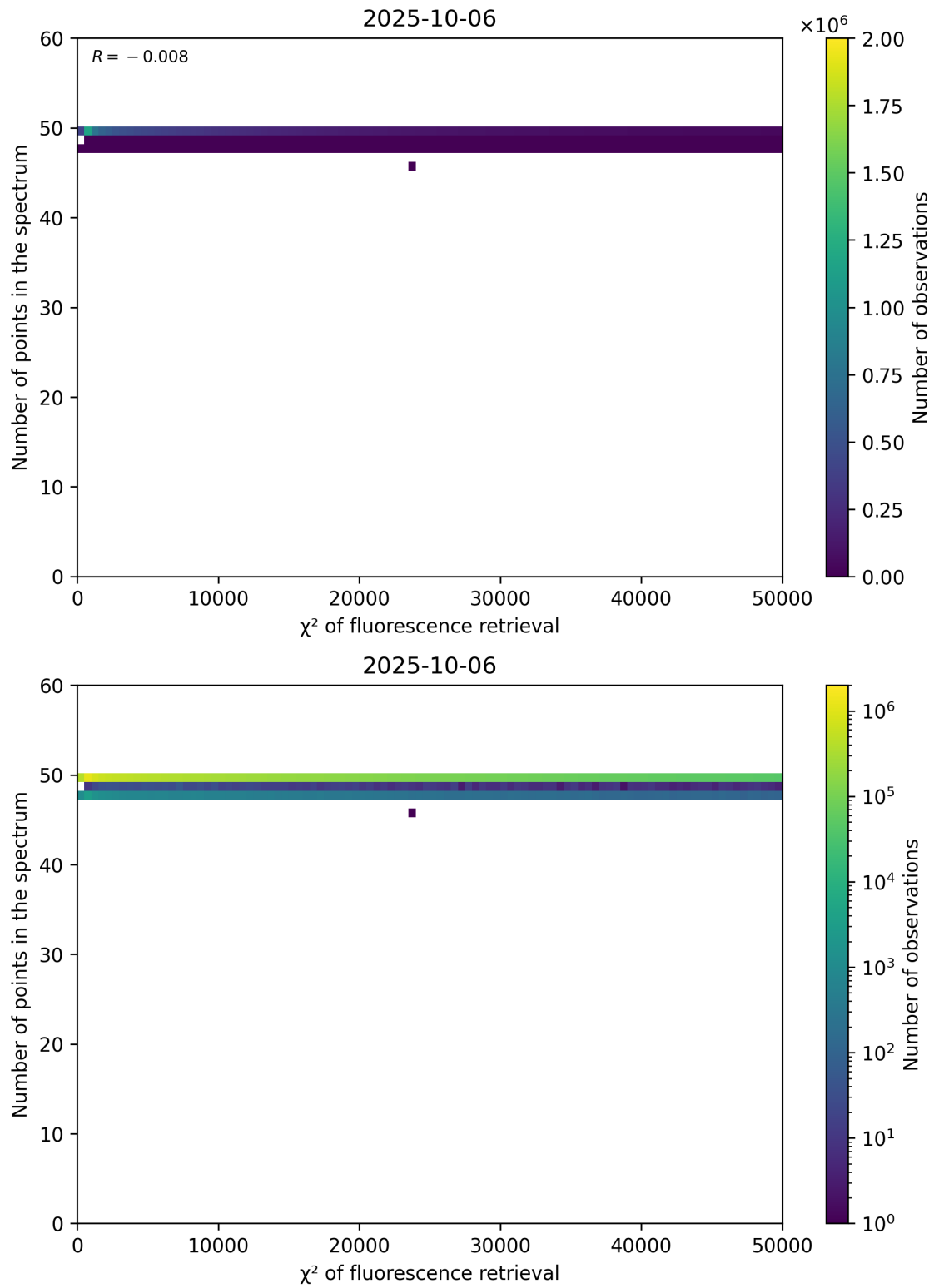
Figure 68: Scatter density plot of “ \chi^2 of fluorescence retrieval” against “Number of points in the spectrum” for 2025-10-06 to 2025-10-07.
