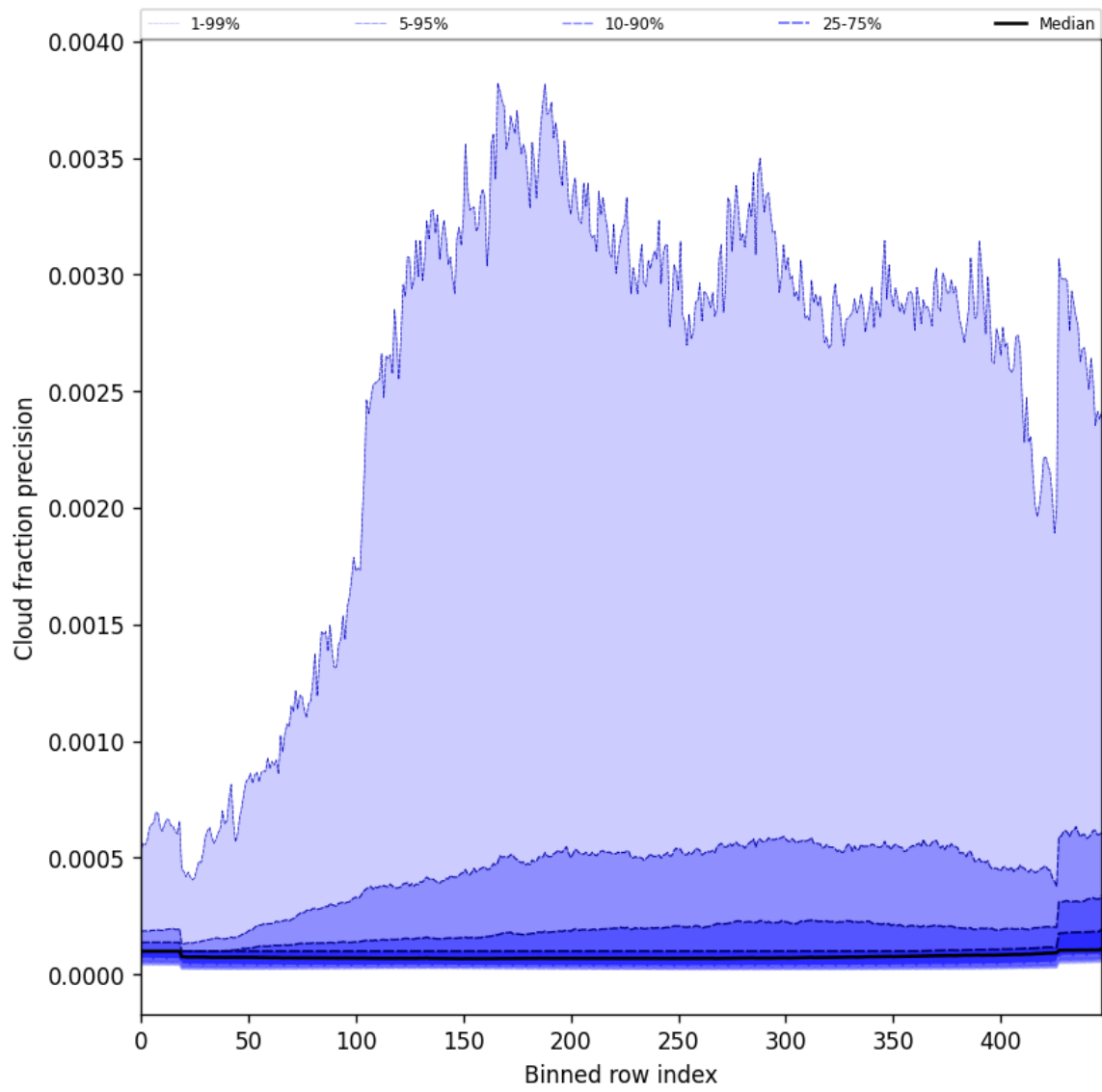
Figure 50: Along track statistics of “Cloud fraction precision” for 2025-10-06 to 2025-10-07
