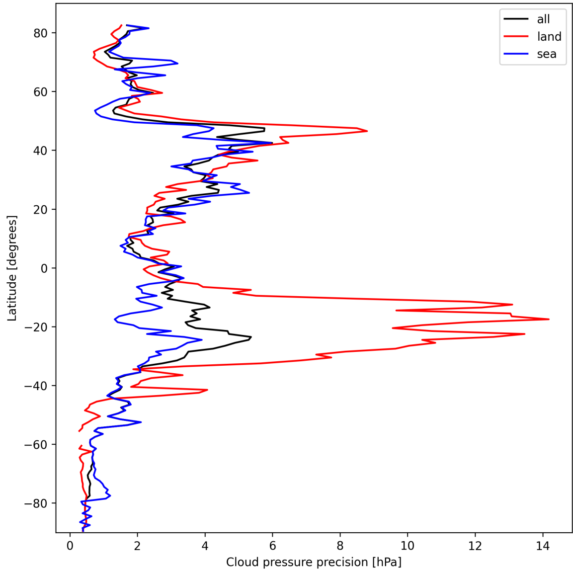
Figure 14: Zonal average of “Cloud pressure precision” for 2025-10-06 to 2025-10-07.
