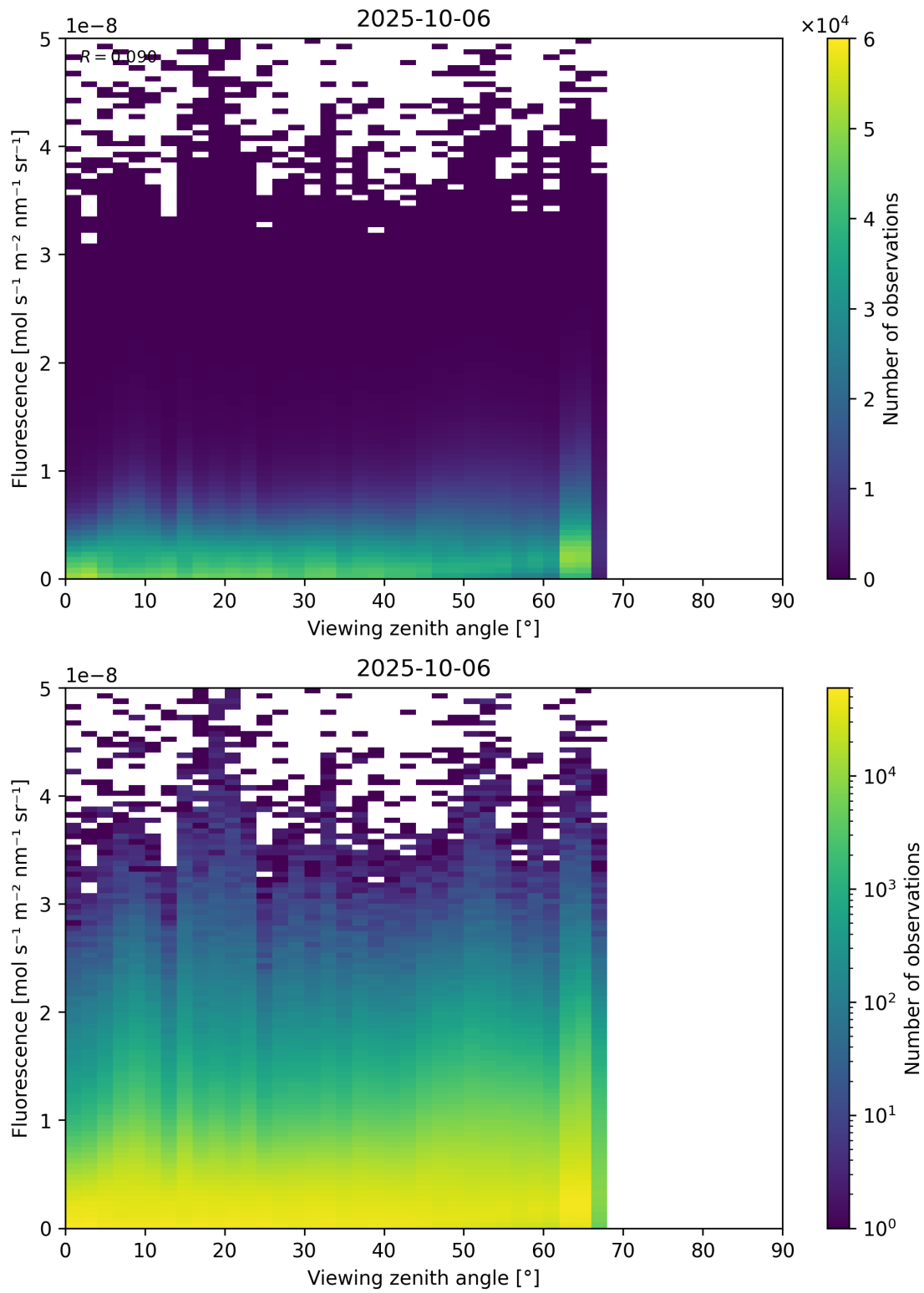
Figure 122: Scatter density plot of “Viewing zenith angle” against “Fluorescence” for 2025-10-06 to 2025-10-07.
