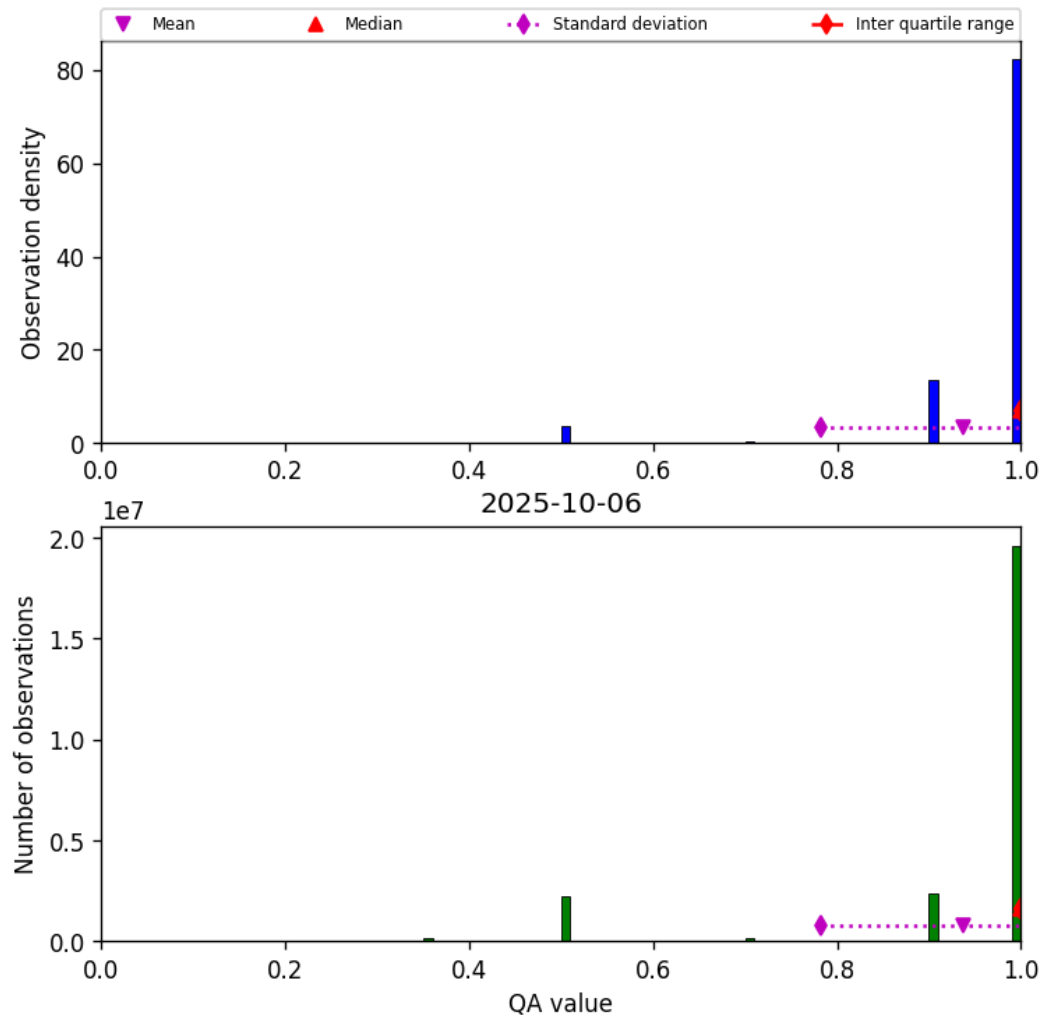
Figure 29: Histogram of “QA value” for 2025-10-06 to 2025-10-07
