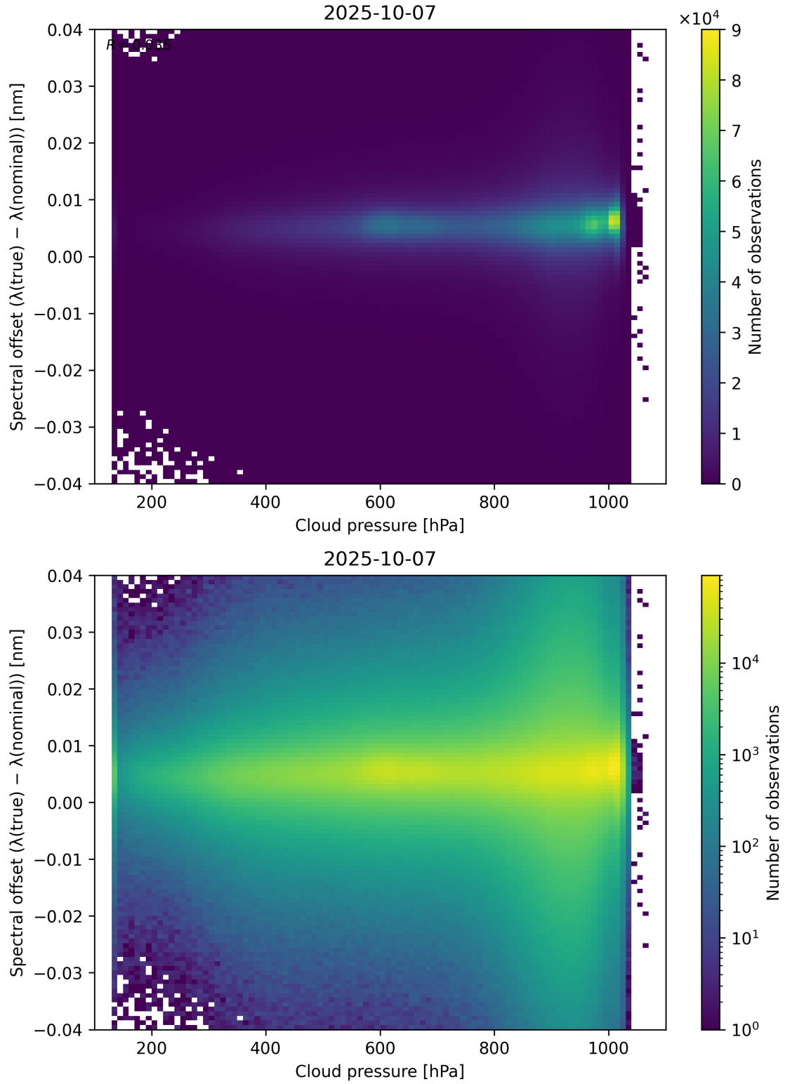
Figure 84: Scatter density plot of “Cloud pressure” against “Spectral offset ( \lambda_{\text{true}} - \lambda_{\text{nominal}} )” for 2025-10-06 to 2025-10-08.
