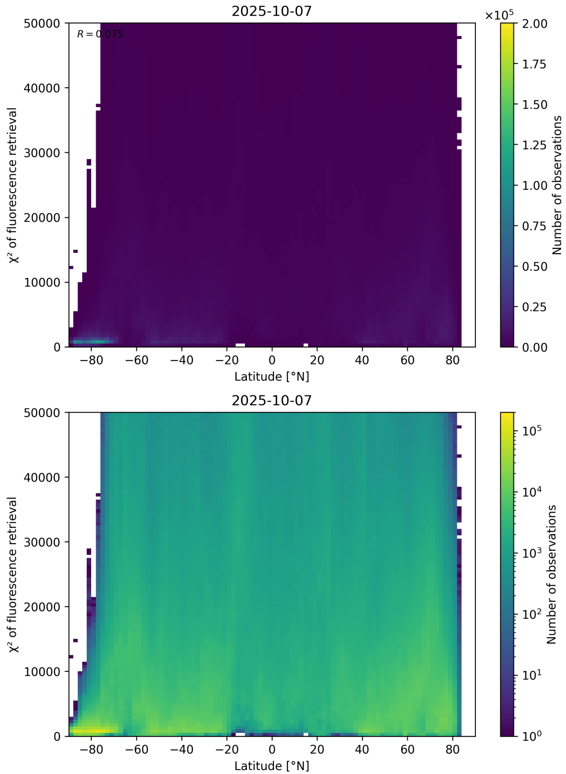
Figure 89: Scatter density plot of “Latitude” against “ \chi^2 of fluorescence retrieval” for 2025-10-06 to 2025-10-08.
