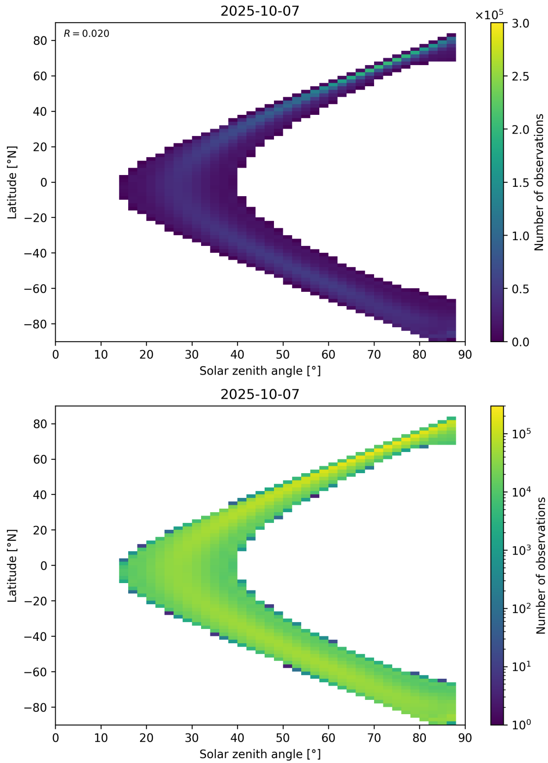
Figure 113: Scatter density plot of “Solar zenith angle” against “Latitude” for 2025-10-06 to 2025-10-08.
