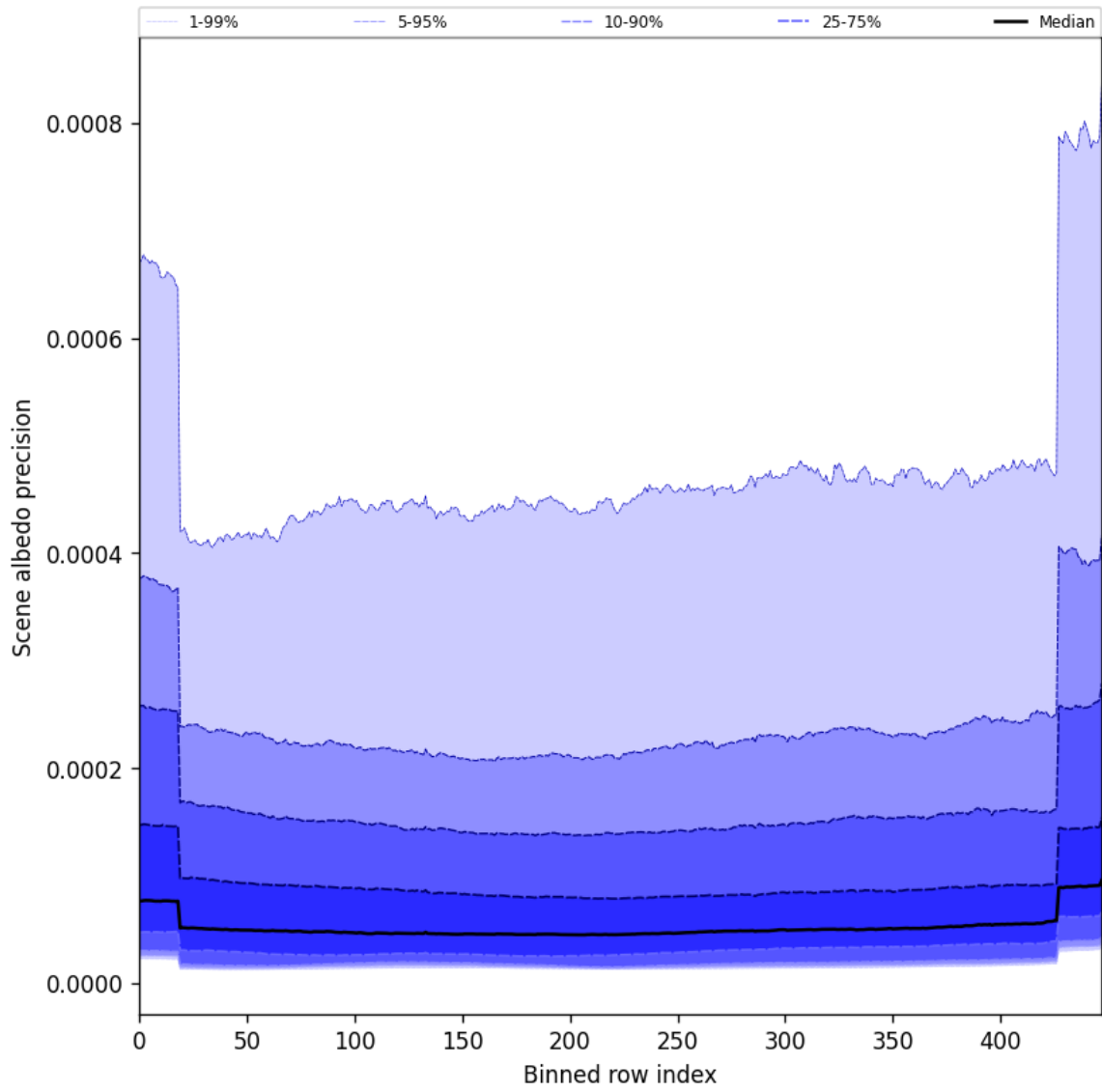
Figure 52: Along track statistics of “Scene albedo precision” for 2025-10-06 to 2025-10-08
