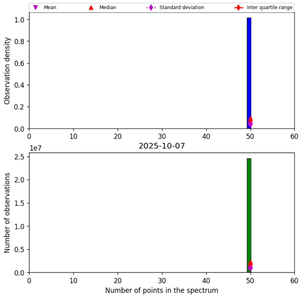
Figure 44: Histogram of “Number of points in the spectrum” for 2025-10-06 to 2025-10-08
