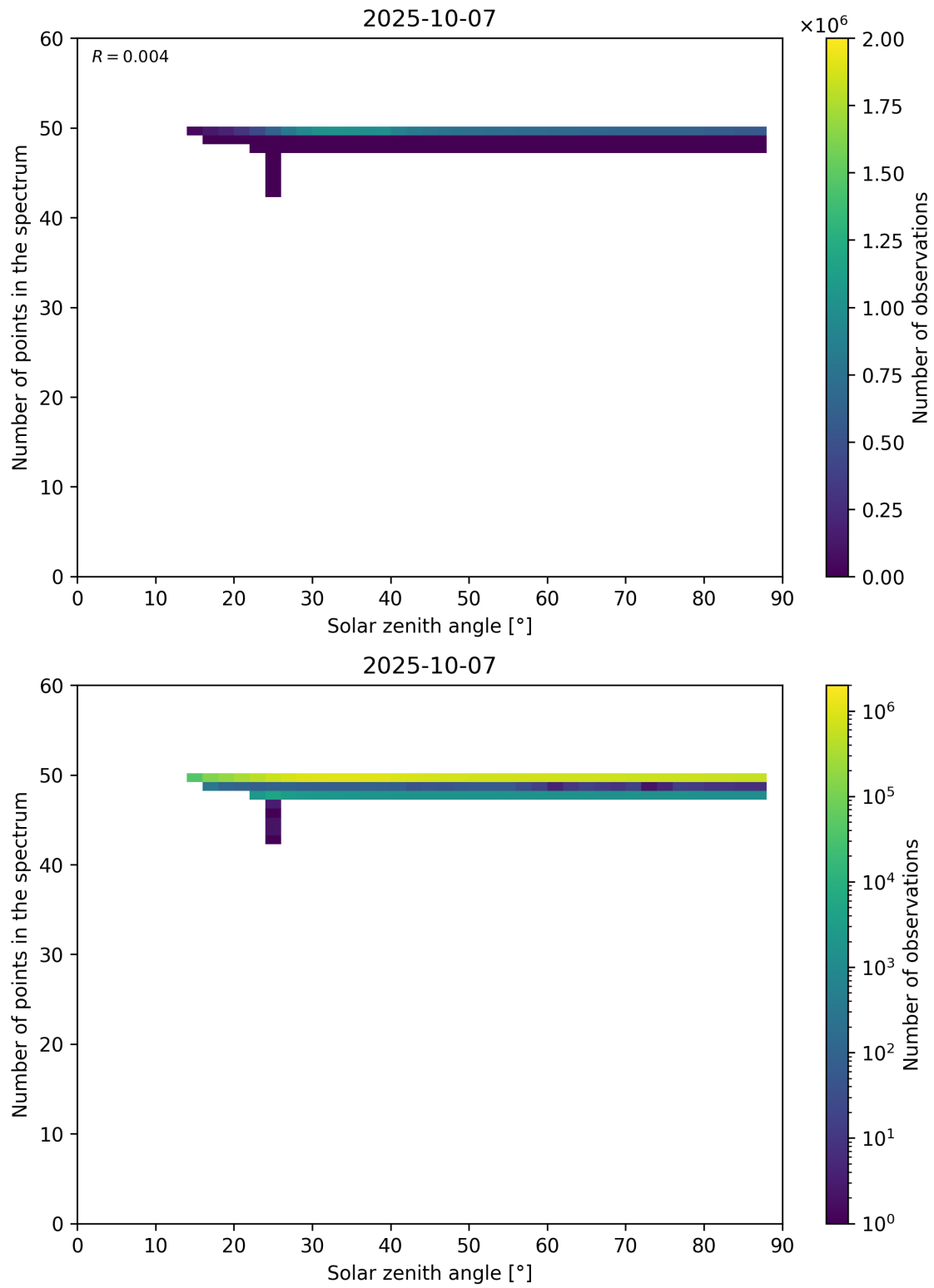
Figure 115: Scatter density plot of “Solar zenith angle” against “Number of points in the spectrum” for 2025-10-06 to 2025-10-08.
