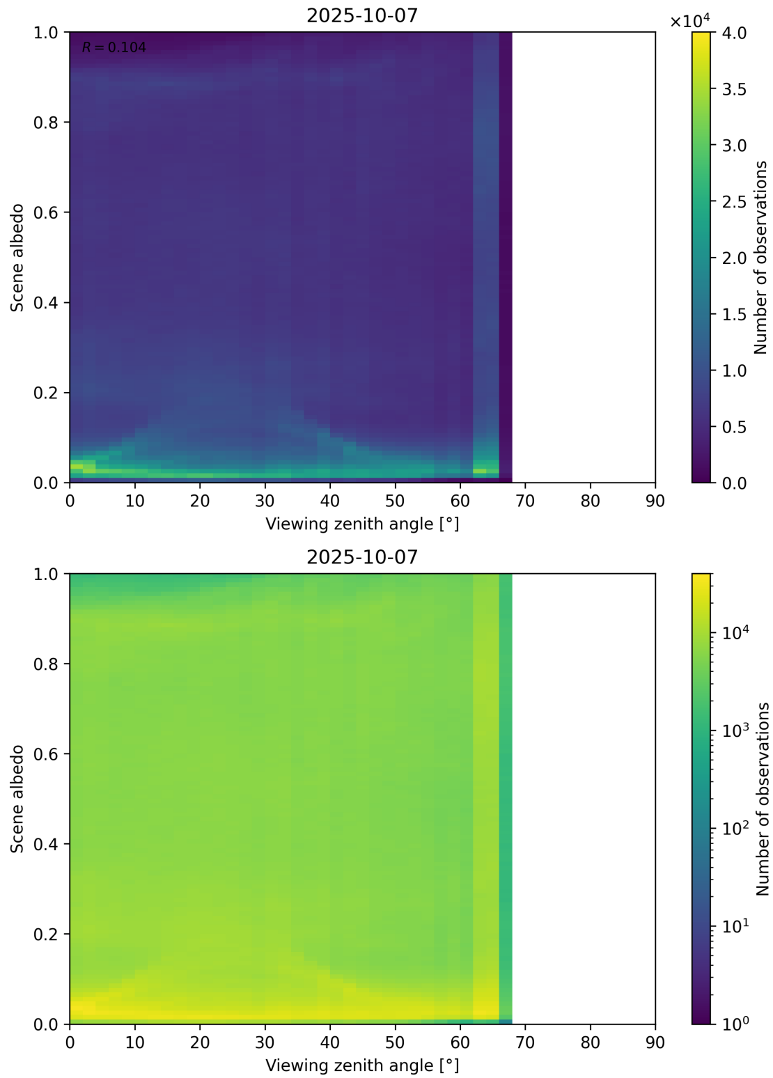
Figure 126: Scatter density plot of “Viewing zenith angle” against “Scene albedo” for 2025-10-06 to 2025-10-08.
