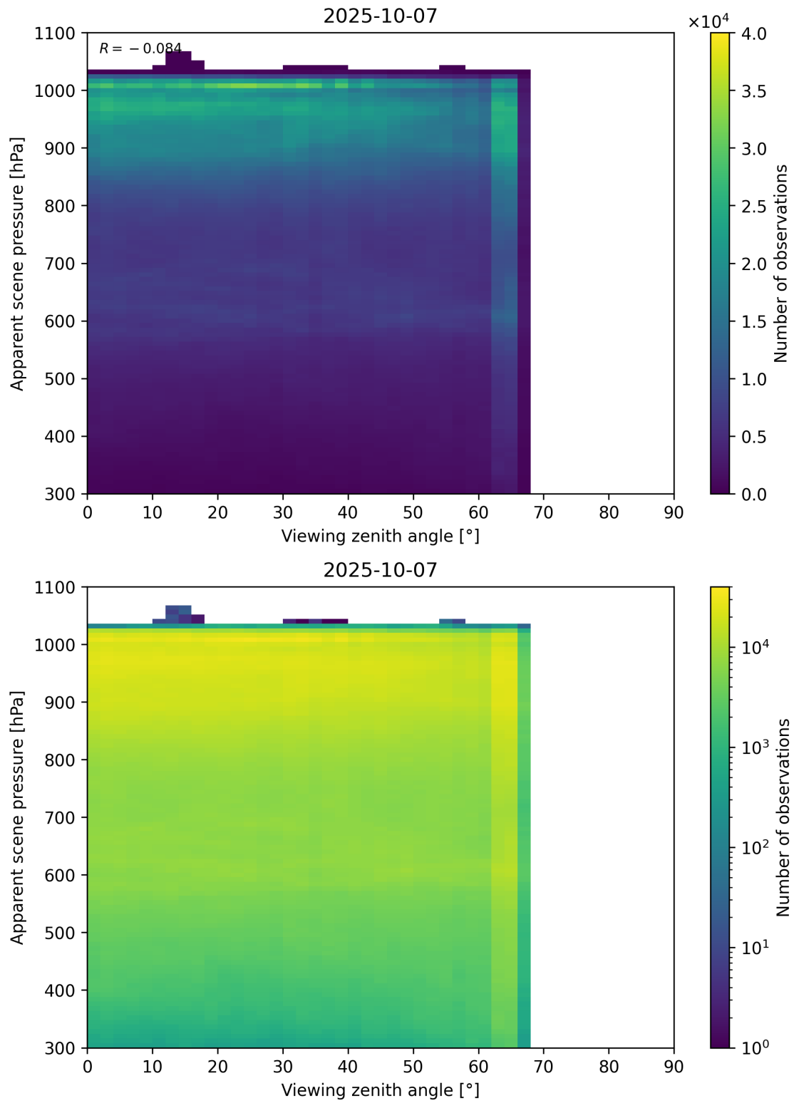
Figure 118: Scatter density plot of “Viewing zenith angle” against “Apparent scene pressure” for 2025-10-06 to 2025-10-08.
