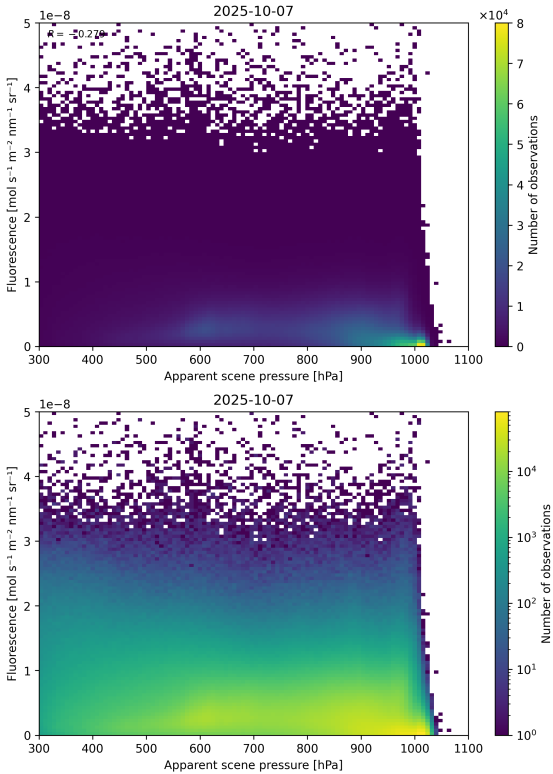
Figure 64: Scatter density plot of “Apparent scene pressure” against “Fluorescence” for 2025-10-06 to 2025-10-08.
