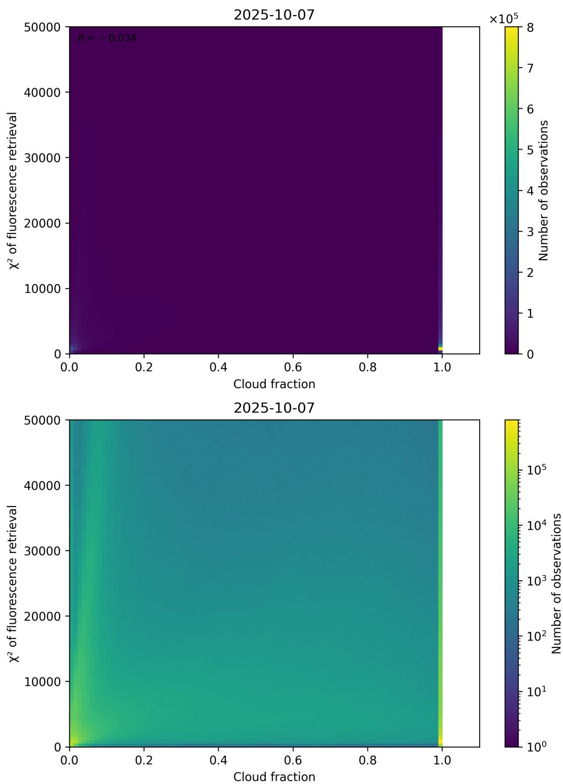
Figure 71: Scatter density plot of “Cloud fraction” against “ \chi^2 of fluorescence retrieval” for 2025-10-06 to 2025-10-08.
