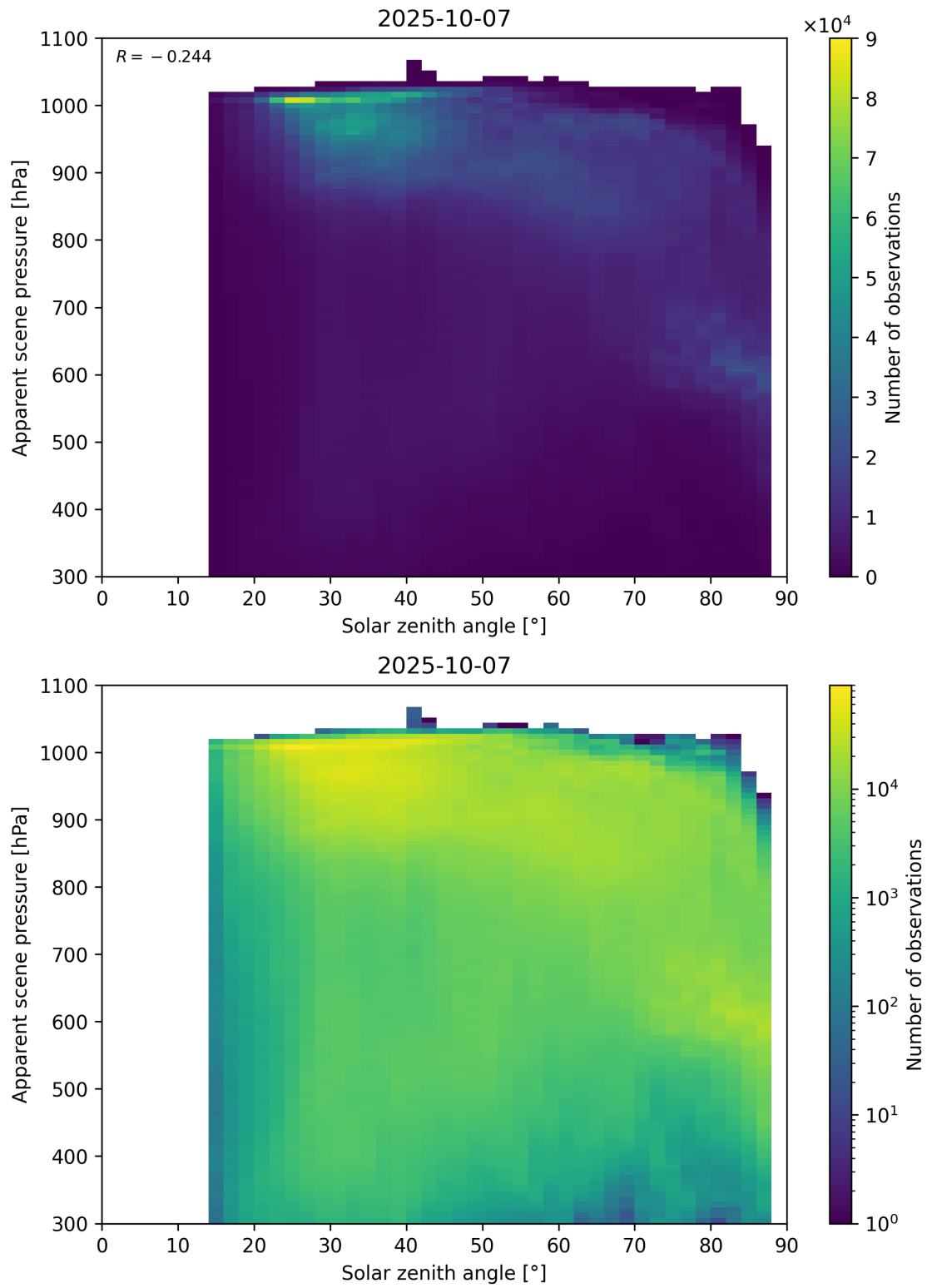
Figure 108: Scatter density plot of “Solar zenith angle” against “Apparent scene pressure” for 2025-10-06 to 2025-10-08.
