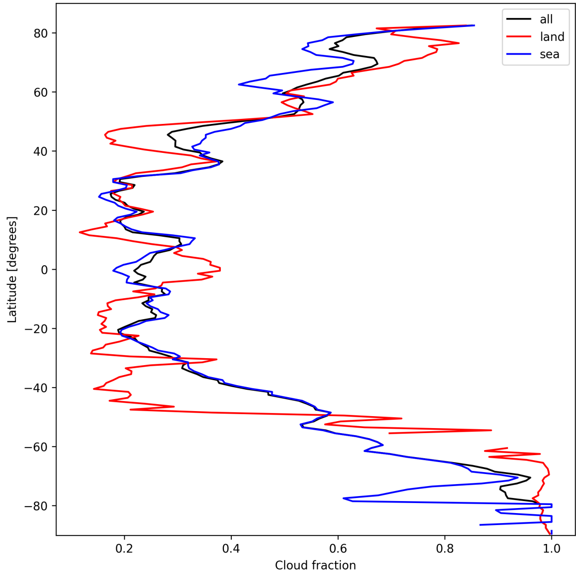
Figure 15: Zonal average of “Cloud fraction” for 2025-10-06 to 2025-10-08.
