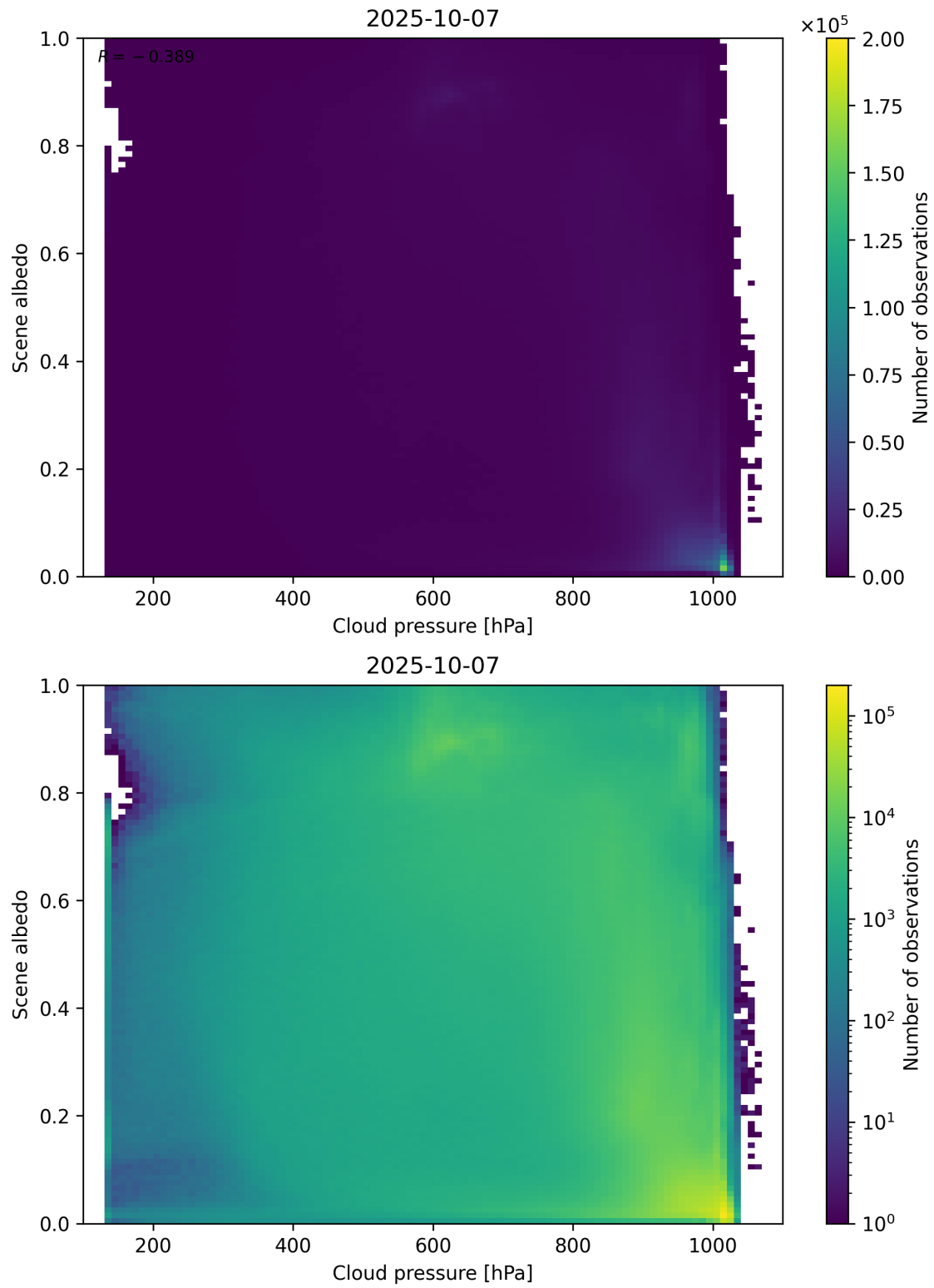
Figure 83: Scatter density plot of “Cloud pressure” against “Scene albedo” for 2025-10-06 to 2025-10-08.
