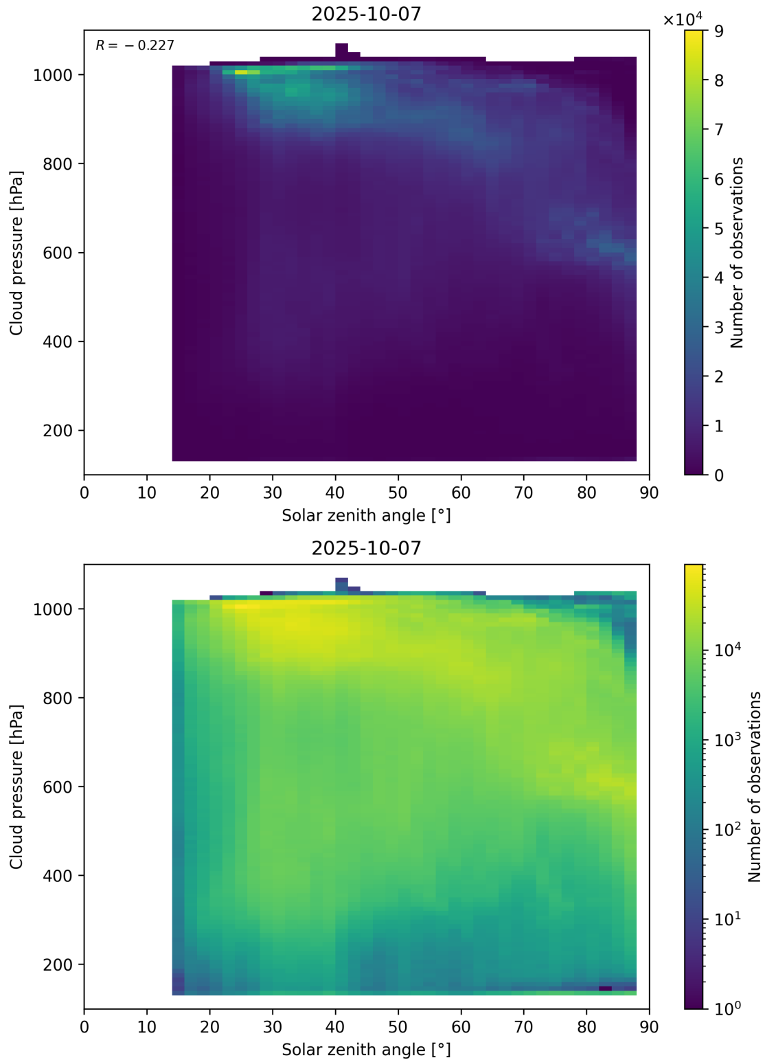
Figure 111: Scatter density plot of “Solar zenith angle” against “Cloud pressure” for 2025-10-06 to 2025-10-08.
