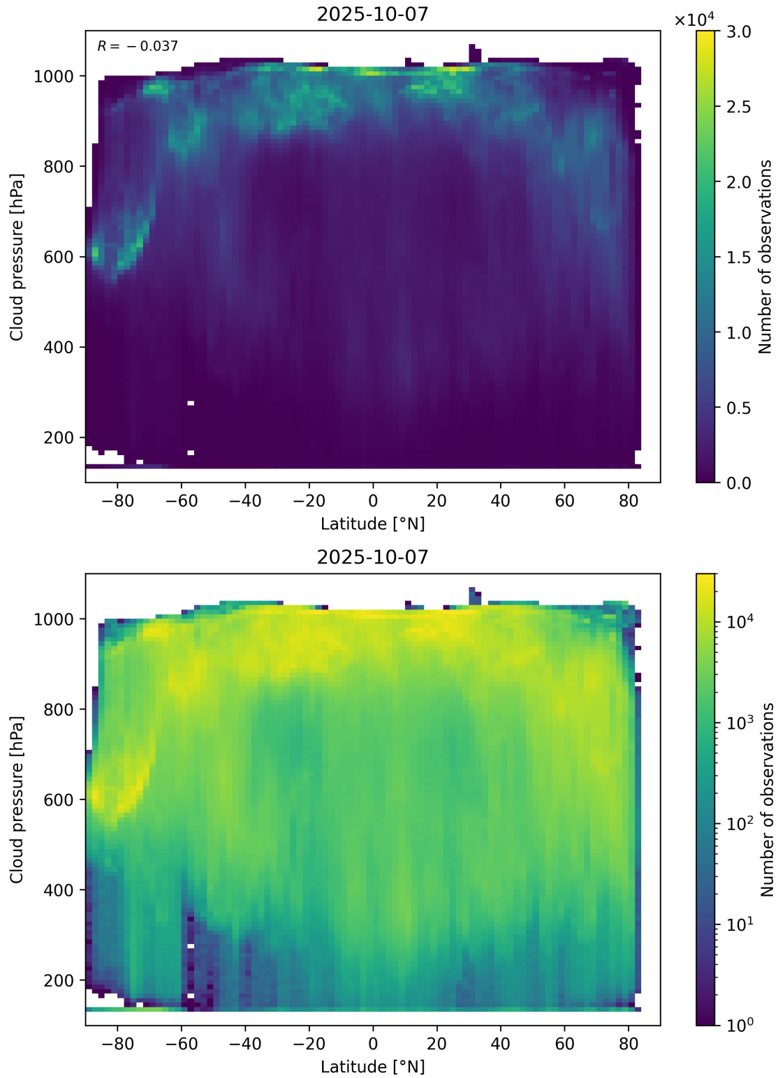
Figure 91: Scatter density plot of “Latitude” against “Cloud pressure” for 2025-10-06 to 2025-10-08.
