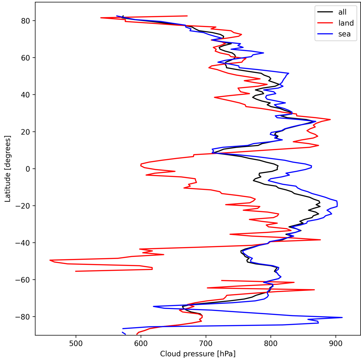
Figure 13: Zonal average of “Cloud pressure” for 2025-10-06 to 2025-10-08.
