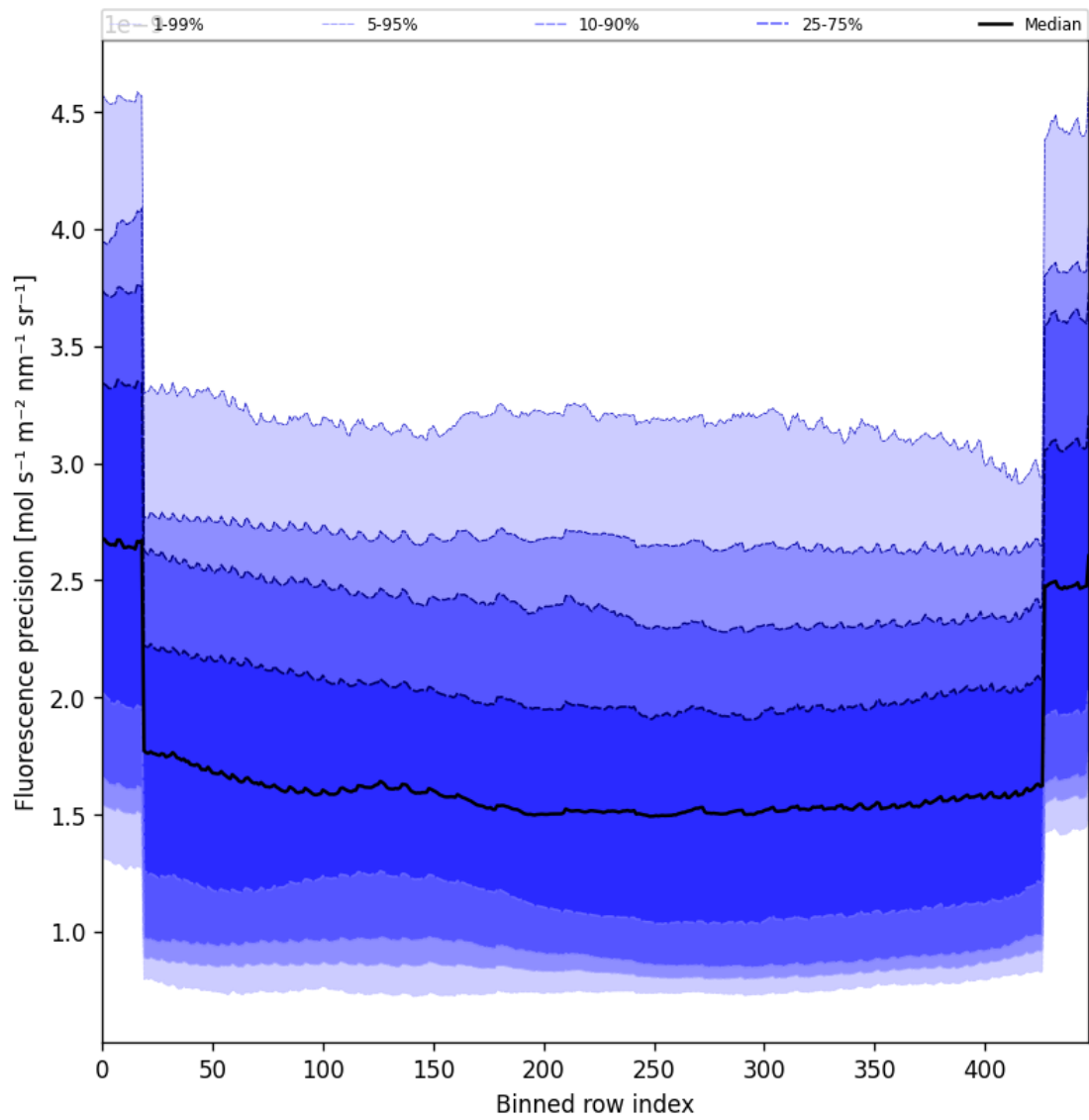
Figure 58: Along track statistics of “Fluorescence precision” for 2025-10-06 to 2025-10-08
