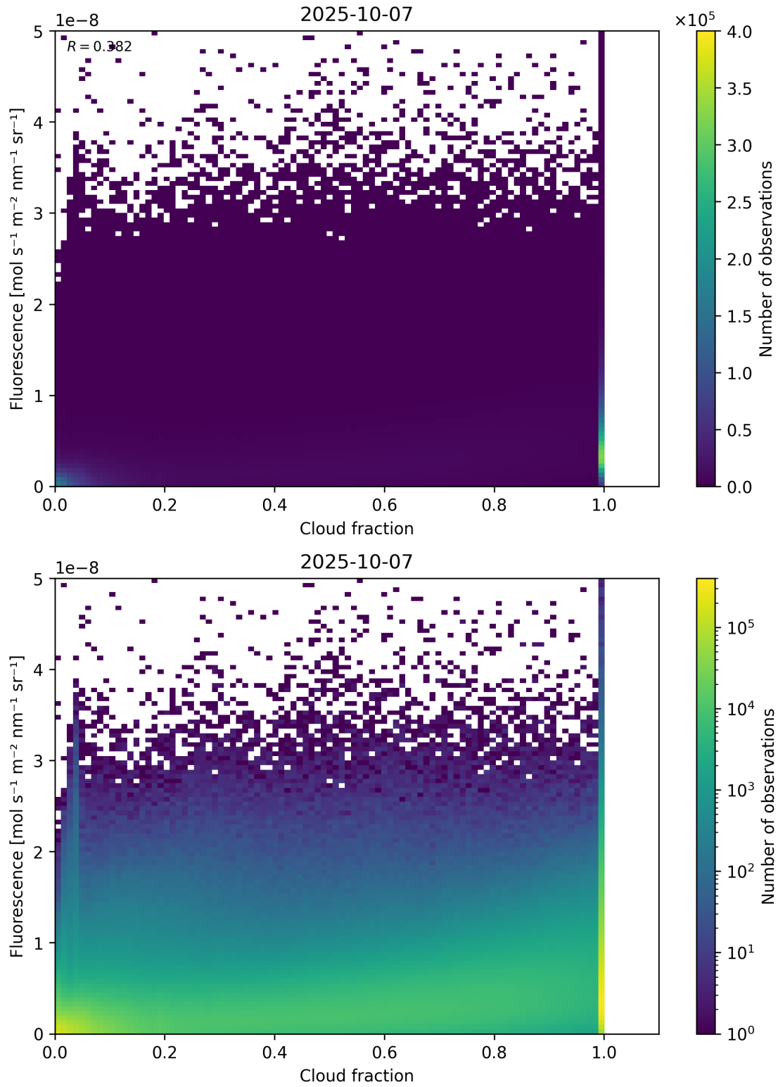
Figure 72: Scatter density plot of “Cloud fraction” against “Fluorescence” for 2025-10-06 to 2025-10-08.
