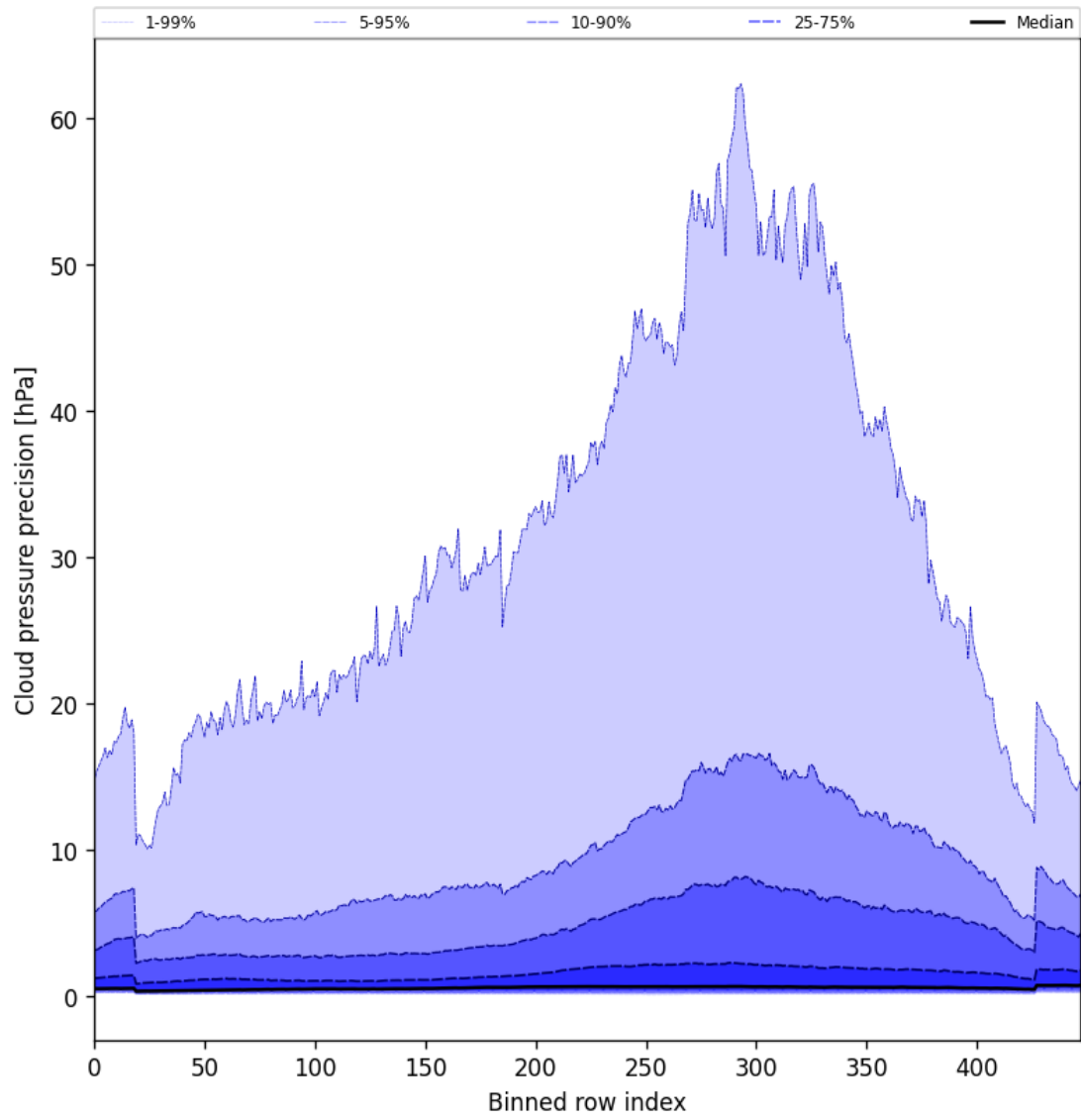
Figure 48: Along track statistics of “Cloud pressure precision” for 2025-10-06 to 2025-10-08
