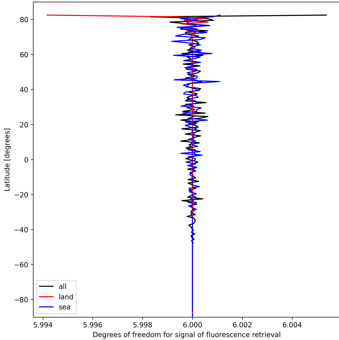
Figure 26: Zonal average of “Degrees of freedom for signal of fluorescence retrieval” for 2025-10-06 to 2025-10-08.
