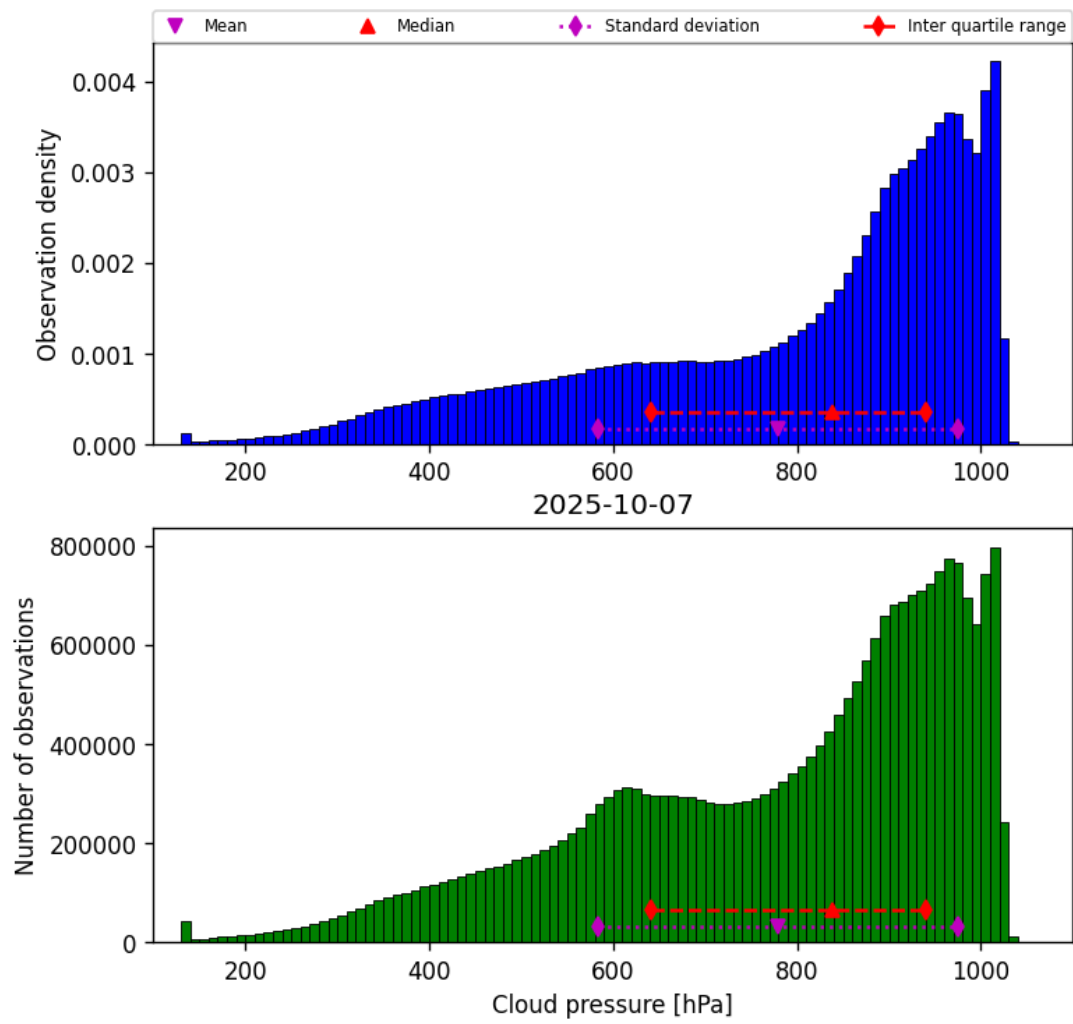
Figure 30: Histogram of “Cloud pressure” for 2025-10-06 to 2025-10-08
