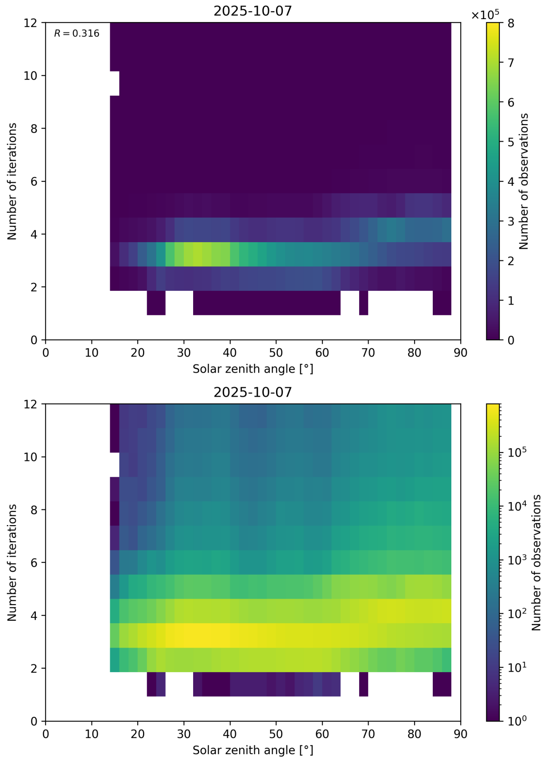
Figure 114: Scatter density plot of “Solar zenith angle” against “Number of iterations” for 2025-10-06 to 2025-10-08.
