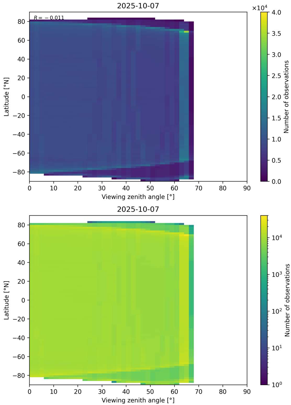
Figure 123: Scatter density plot of “Viewing zenith angle” against “Latitude” for 2025-10-06 to 2025-10-08.
