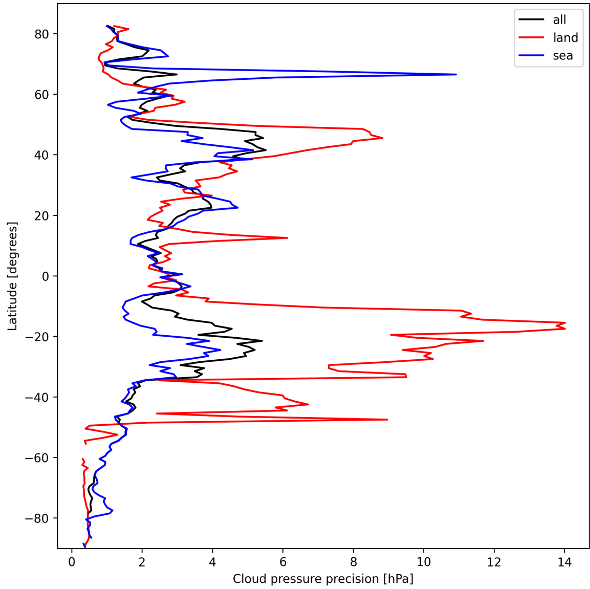
Figure 14: Zonal average of "Cloud pressure precision" for 2025-10-06 to 2025-10-08.
