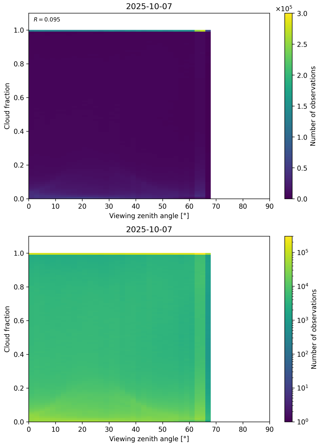
Figure 120: Scatter density plot of “Viewing zenith angle” against “Cloud fraction” for 2025-10-06 to 2025-10-08.
