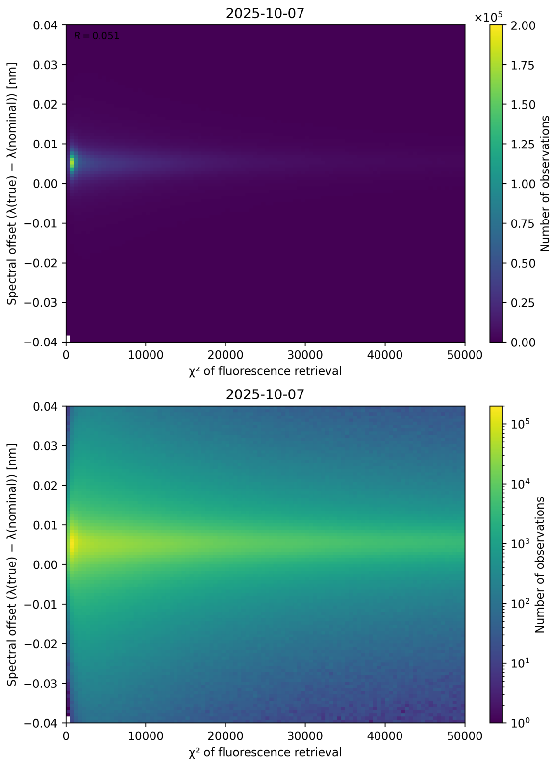
Figure 69: Scatter density plot of “ \chi^2 of fluorescence retrieval” against “Spectral offset ( \lambda_{\text{true}} - \lambda_{\text{nominal}} )” for 2025-10-06 to 2025-10-08.
