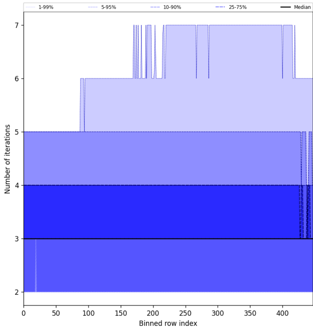
Figure 56: Along track statistics of “Number of iterations” for 2025-10-06 to 2025-10-08
