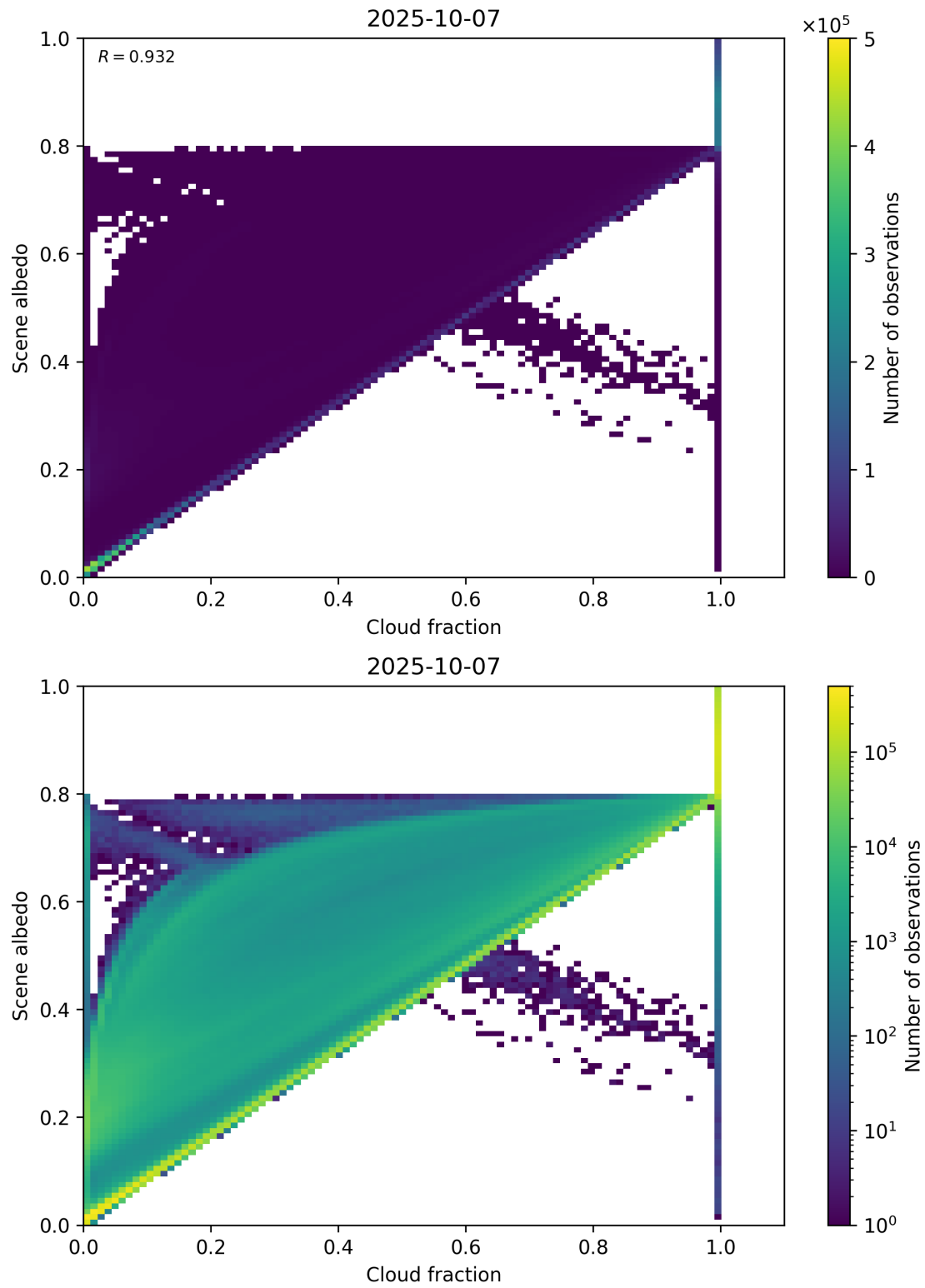
Figure 75: Scatter density plot of “Cloud fraction” against “Scene albedo” for 2025-10-06 to 2025-10-08.
