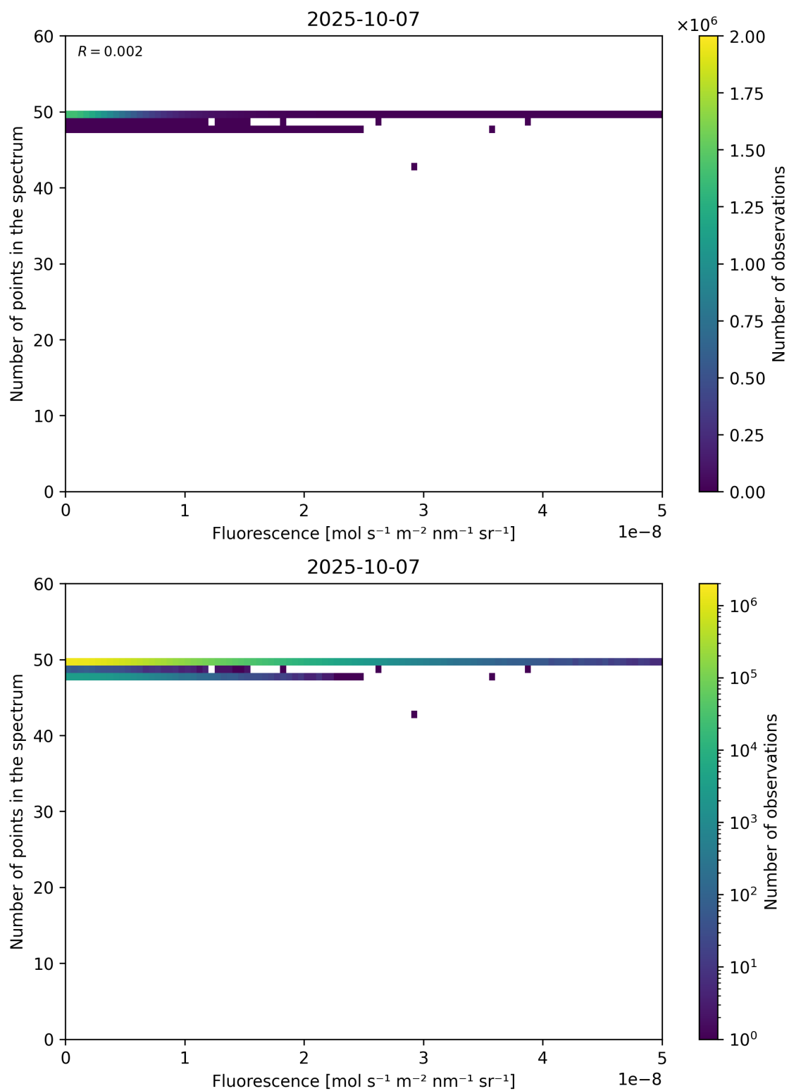
Figure 86: Scatter density plot of “Fluorescence” against “Number of points in the spectrum” for 2025-10-06 to 2025-10-08.
