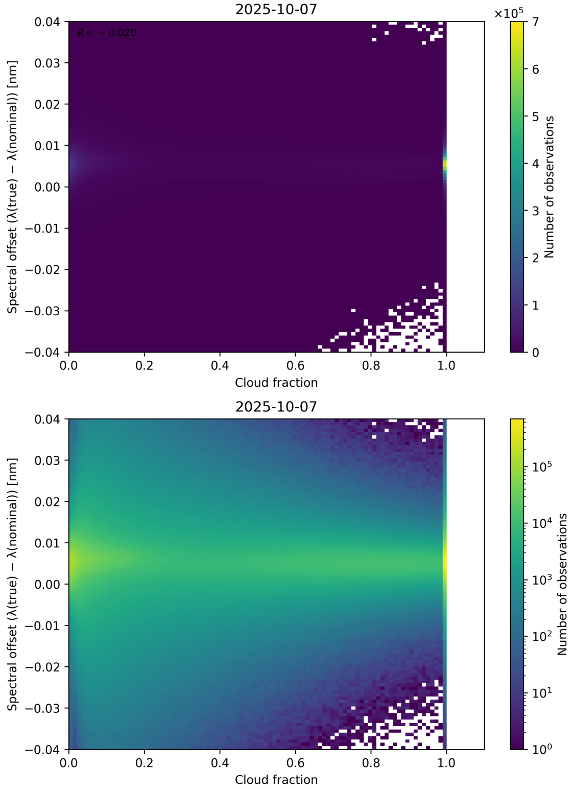
Figure 76: Scatter density plot of “Cloud fraction” against “Spectral offset ( \lambda_{\text{true}} - \lambda_{\text{nominal}} )” for 2025-10-06 to 2025-10-08.
