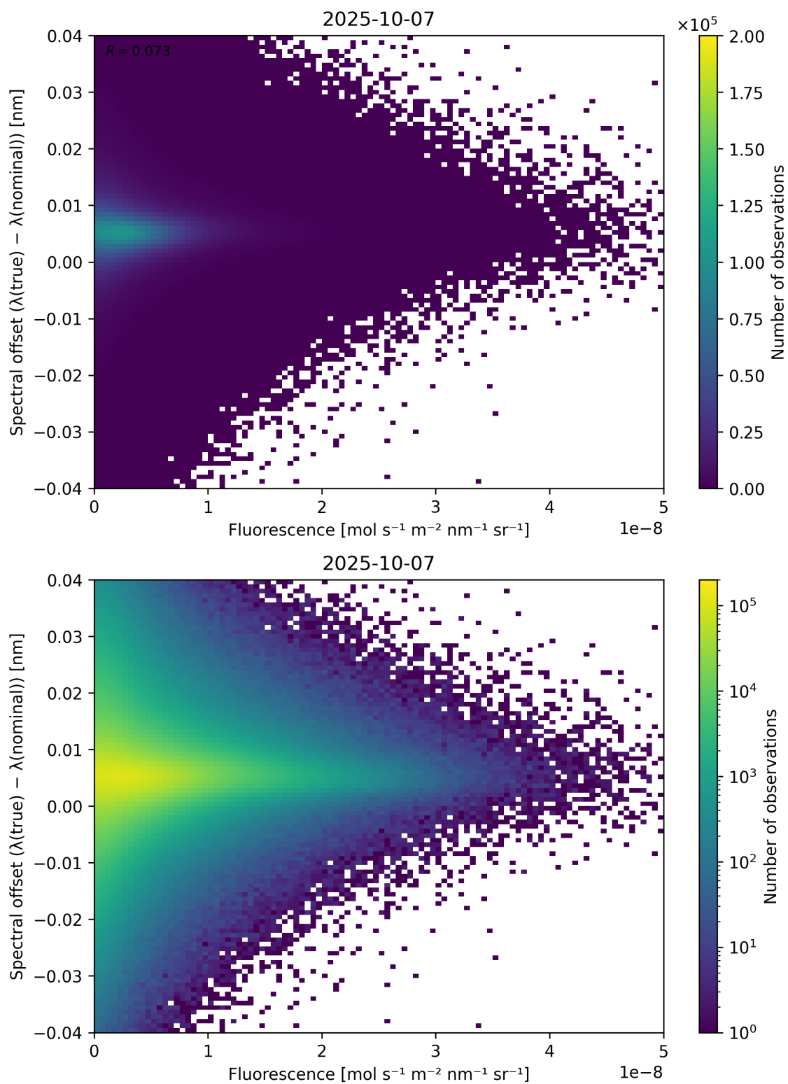
Figure 87: Scatter density plot of “Fluorescence” against “Spectral offset ( \lambda_{\text{true}} - \lambda_{\text{nominal}} )” for 2025-10-06 to 2025-10-08.
