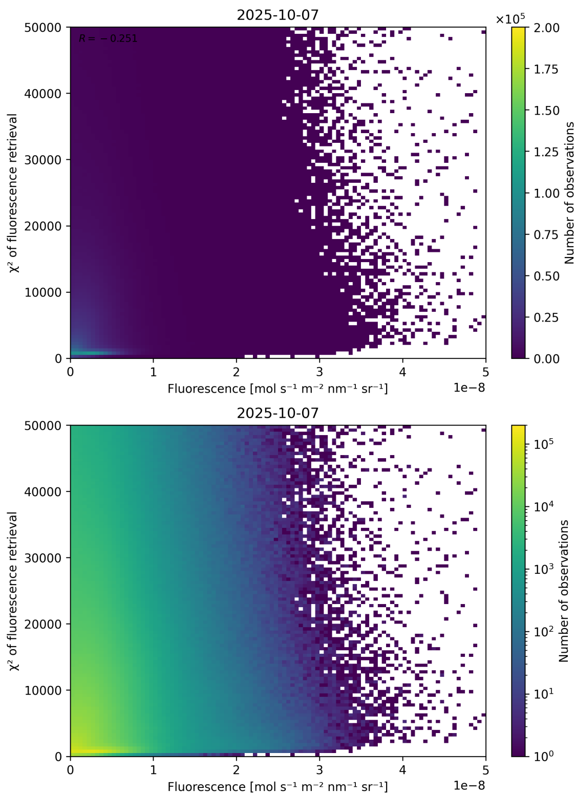
Figure 85: Scatter density plot of “Fluorescence” against “ \chi^2 of fluorescence retrieval” for 2025-10-06 to 2025-10-08.
