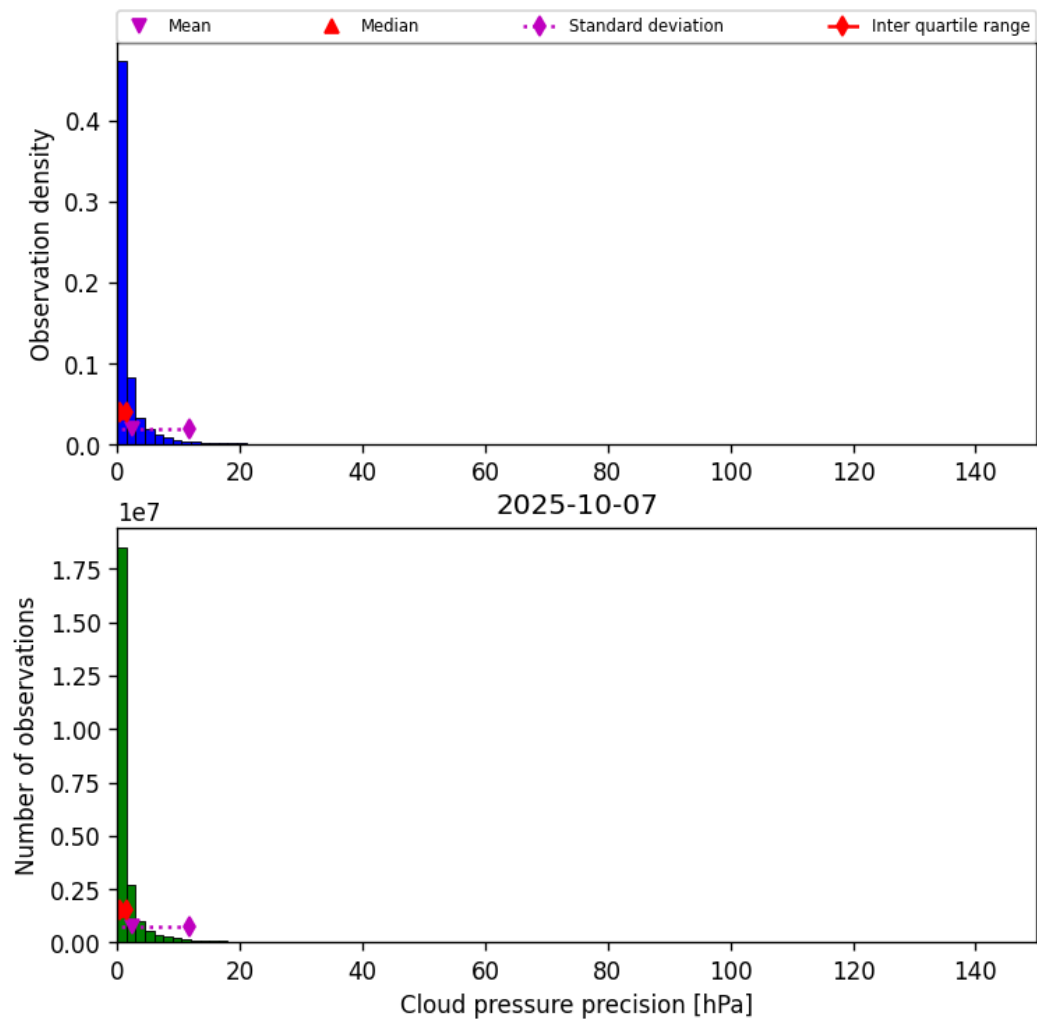
Figure 31: Histogram of “Cloud pressure precision” for 2025-10-06 to 2025-10-08
