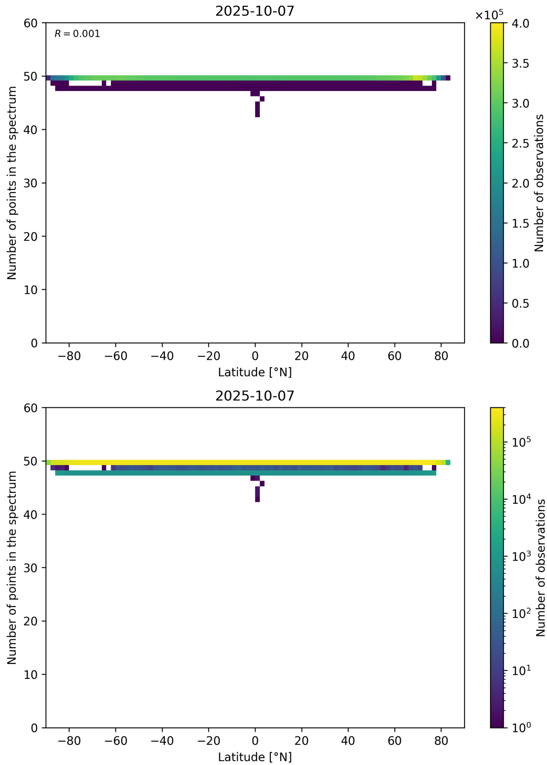
Figure 94: Scatter density plot of “Latitude” against “Number of points in the spectrum” for 2025-10-06 to 2025-10-08.
