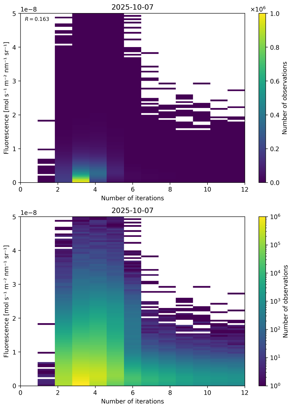
Figure 98: Scatter density plot of “Number of iterations” against “Fluorescence” for 2025-10-06 to 2025-10-08.
