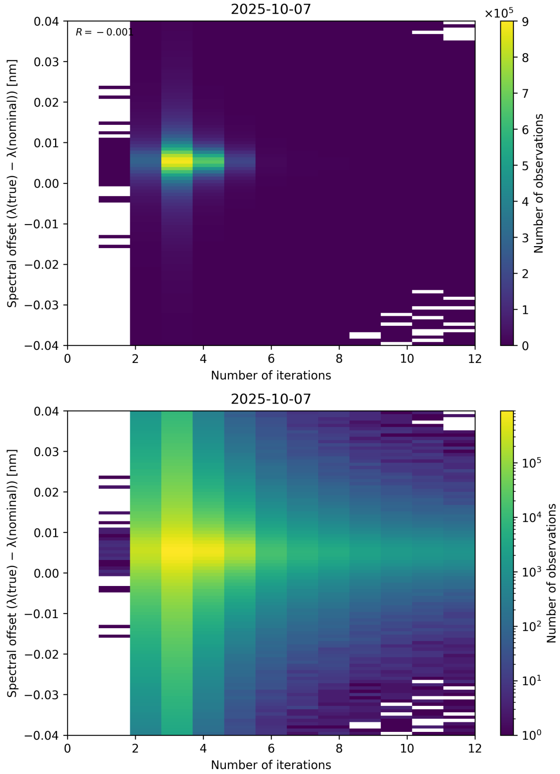
Figure 100: Scatter density plot of “Number of iterations” against “Spectral offset ( \lambda_{\text{true}} - \lambda_{\text{nominal}} )” for 2025-10-06 to 2025-10-08.
