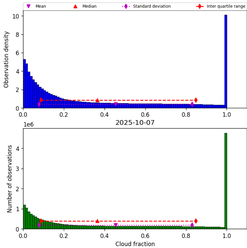
Figure 32: Histogram of “Cloud fraction” for 2025-10-06 to 2025-10-08
