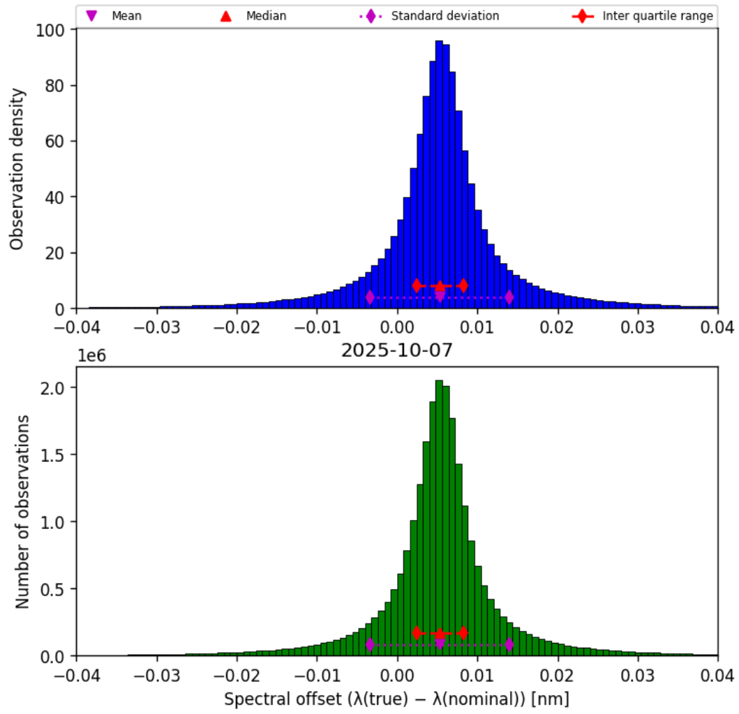
Figure 45: Histogram of “Spectral offset ( \lambda_{\text{true}} - \lambda_{\text{nominal}} )” for 2025-10-06 to 2025-10-08
