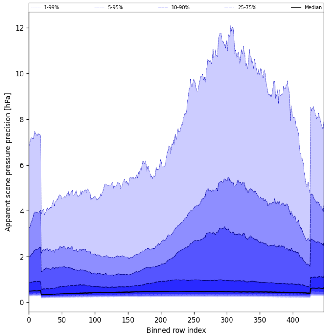
Figure 54: Along track statistics of “Apparent scene pressure precision” for 2025-10-06 to 2025-10-08
