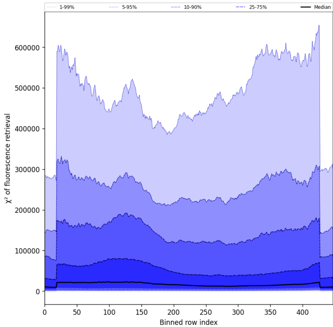
Figure 59: Along track statistics of “ \chi^2 of fluorescence retrieval” for 2025-10-06 to 2025-10-08
