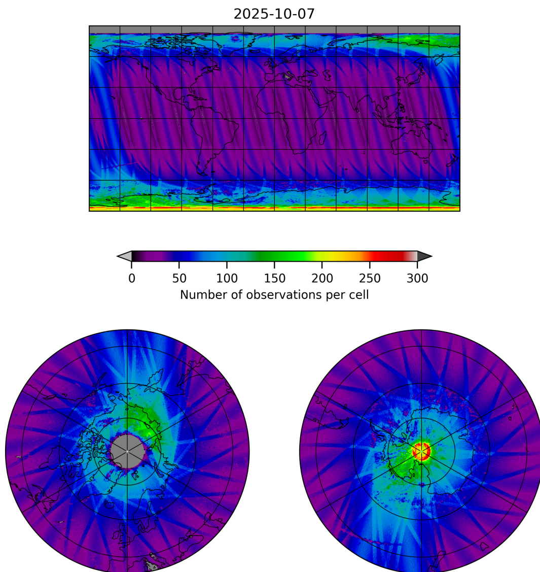
Figure 11: Map of the number of observations for 2025-10-06 to 2025-10-08
