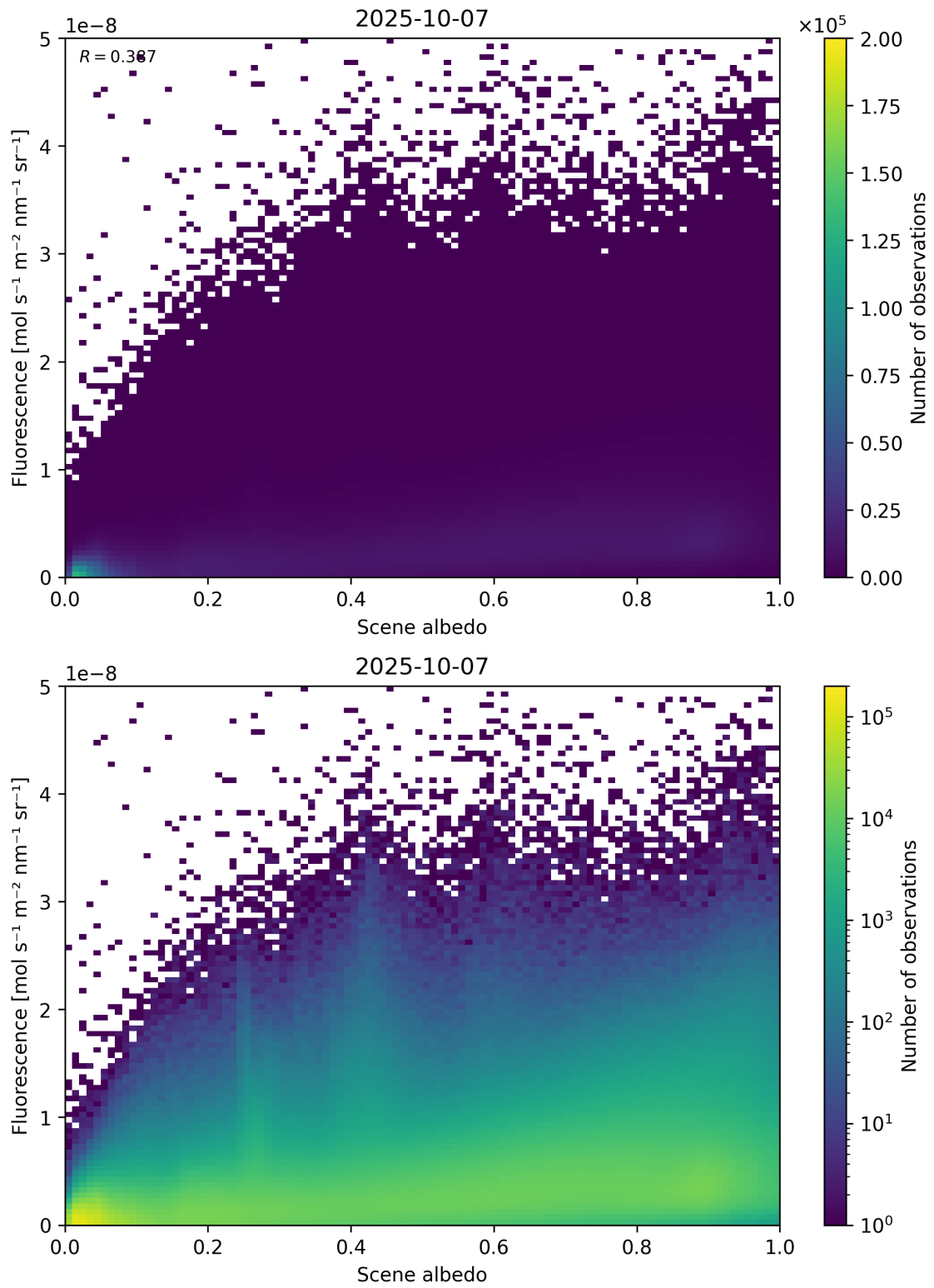
Figure 104: Scatter density plot of “Scene albedo” against “Fluorescence” for 2025-10-06 to 2025-10-08.
