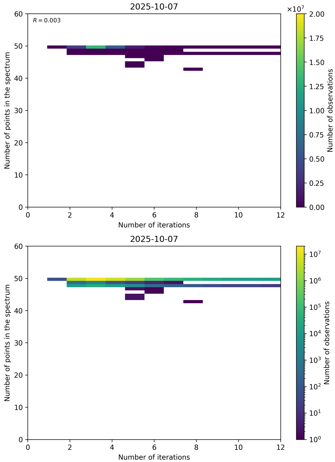
Figure 99: Scatter density plot of “Number of iterations” against “Number of points in the spectrum” for 2025-10-06 to 2025-10-08.
