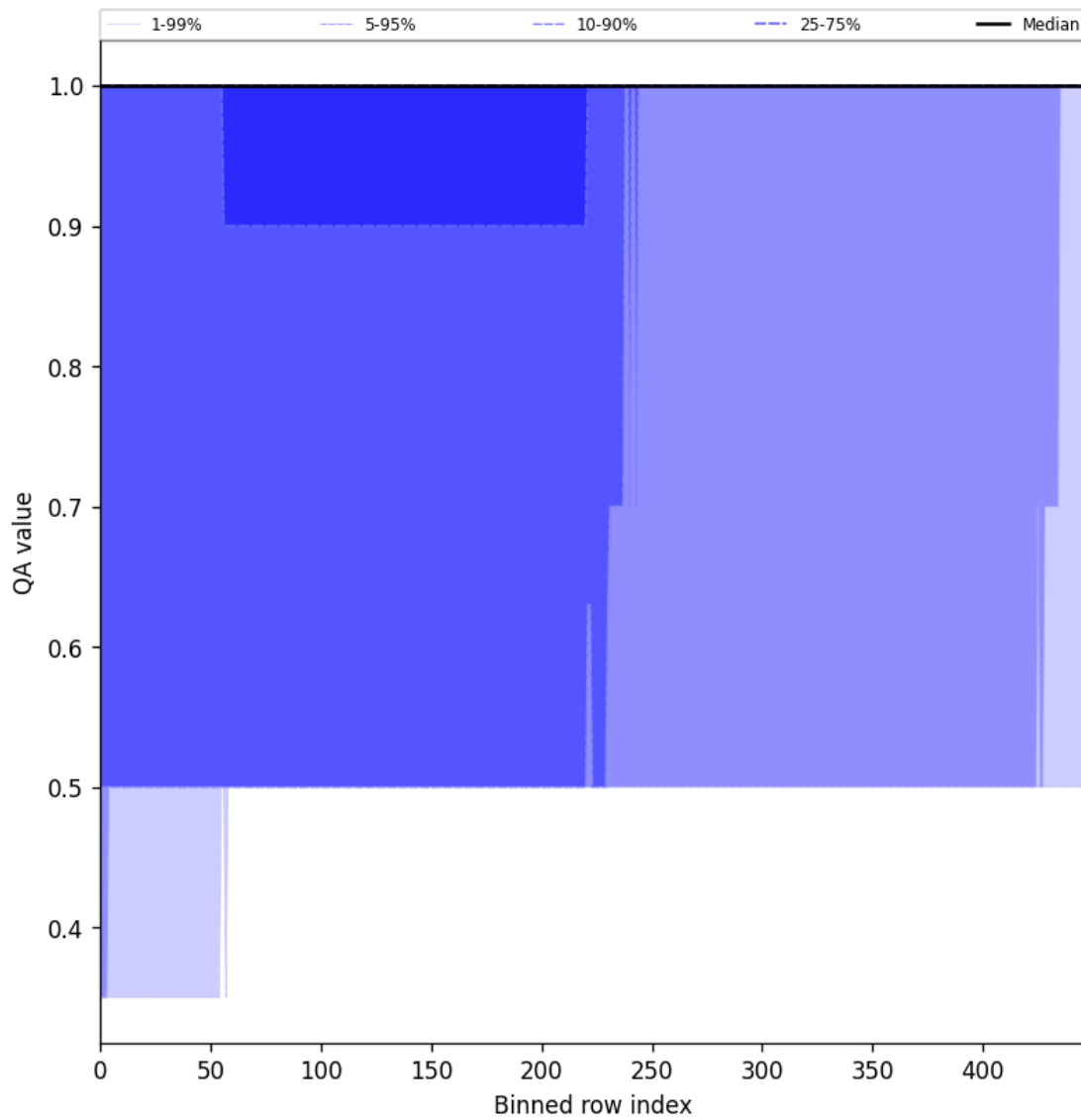
Figure 46: Along track statistics of “QA value” for 2025-10-06 to 2025-10-08
