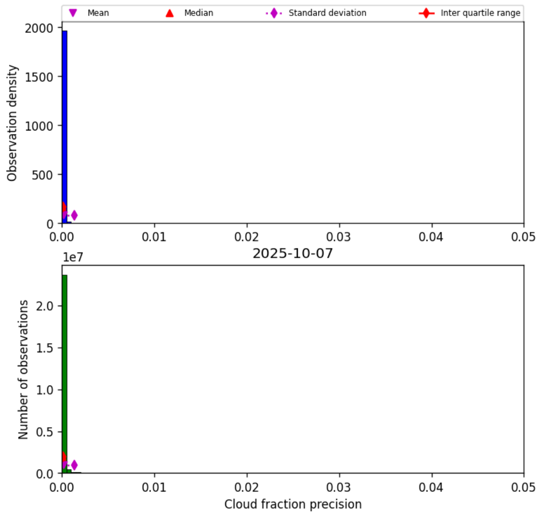
Figure 33: Histogram of “Cloud fraction precision” for 2025-10-06 to 2025-10-08
