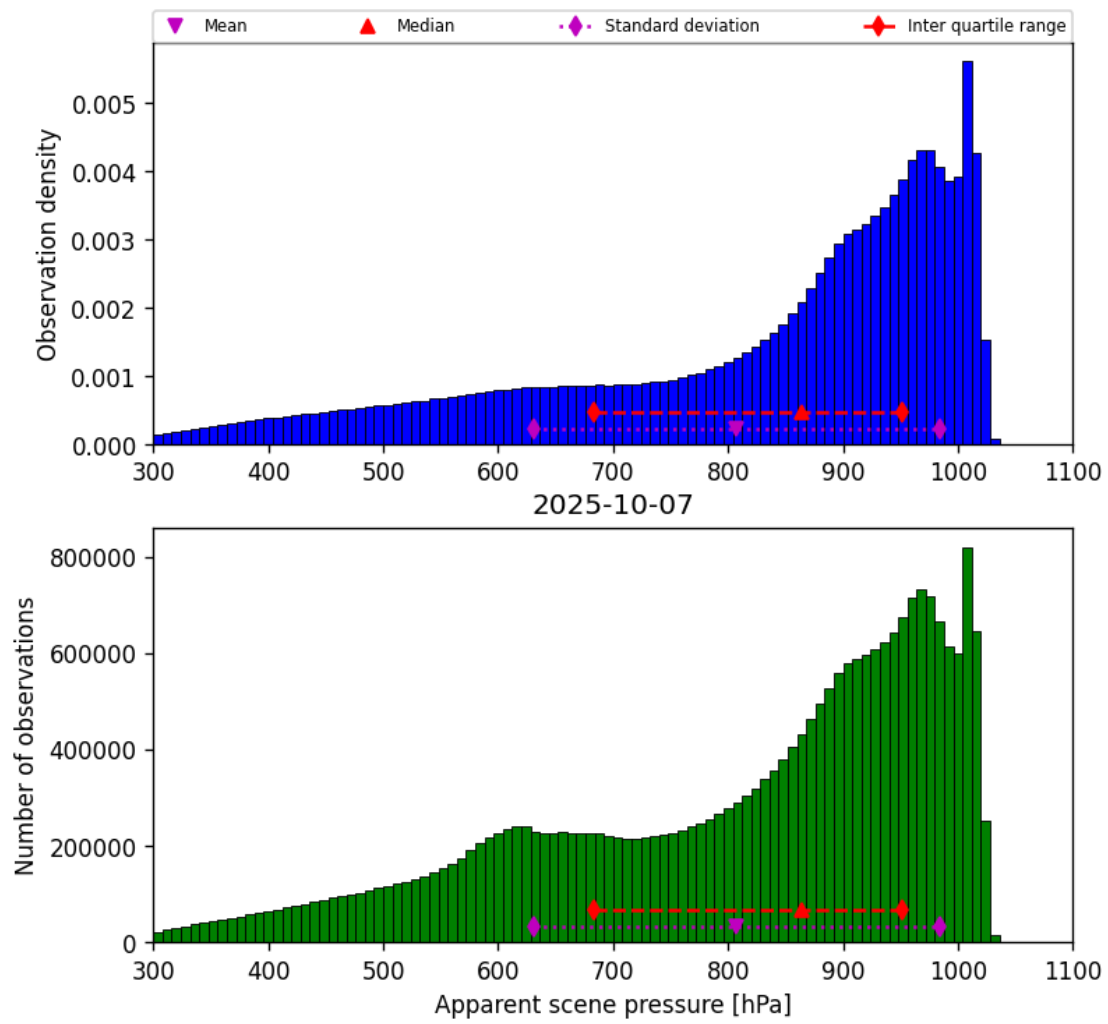
Figure 36: Histogram of “Apparent scene pressure” for 2025-10-06 to 2025-10-08
