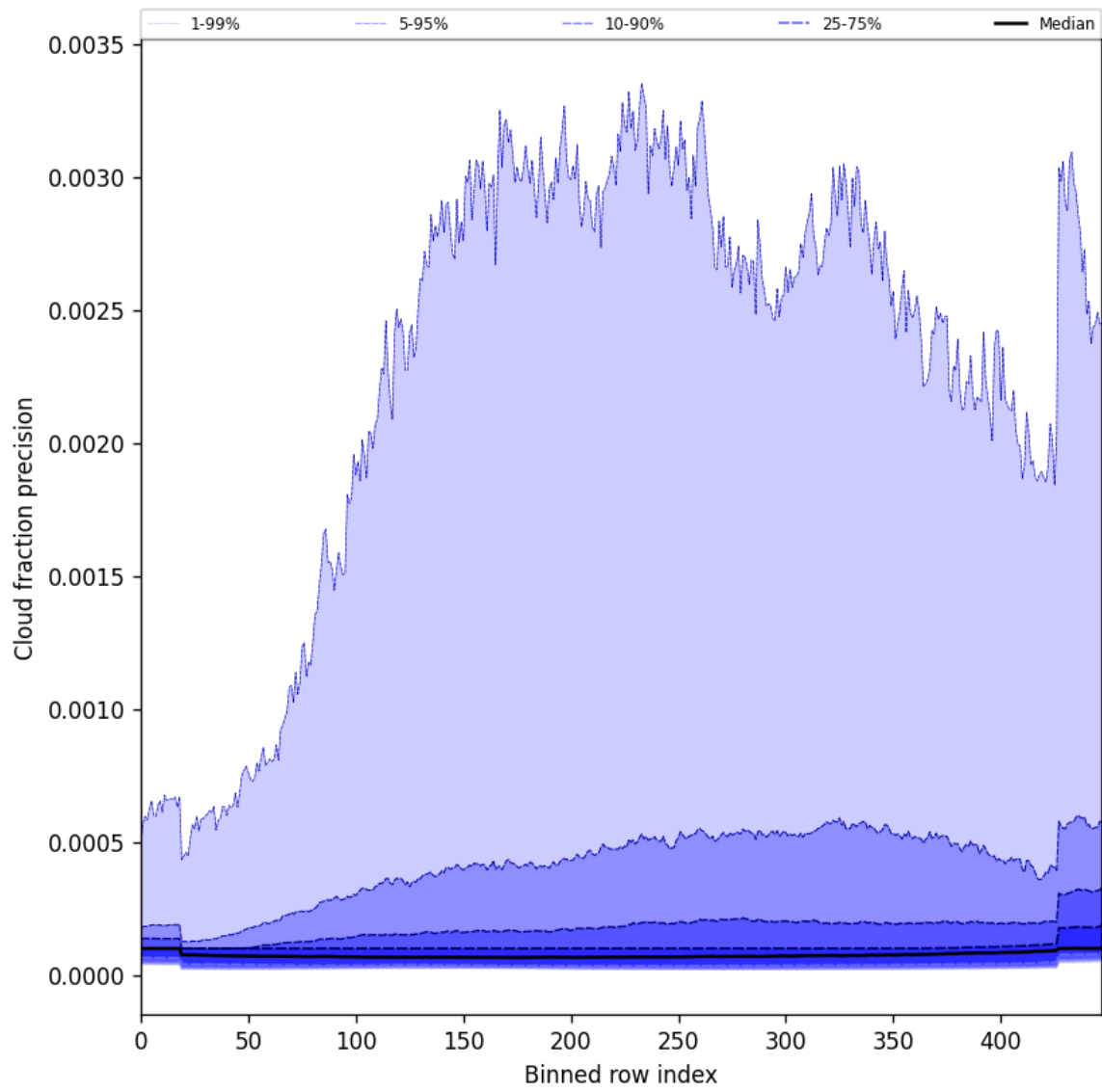
Figure 50: Along track statistics of “Cloud fraction precision” for 2025-10-06 to 2025-10-08
