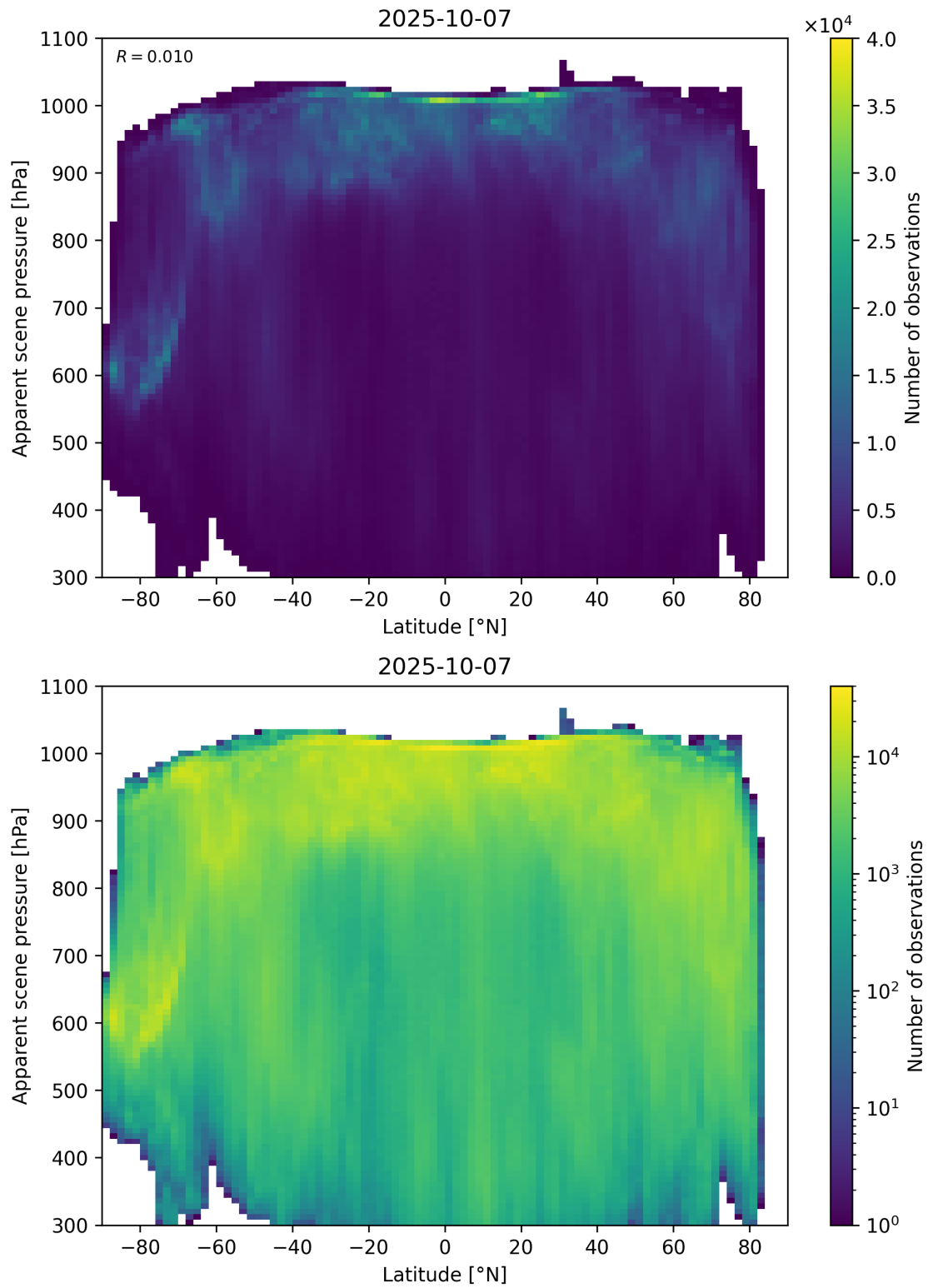
Figure 88: Scatter density plot of “Latitude” against “Apparent scene pressure” for 2025-10-06 to 2025-10-08.
