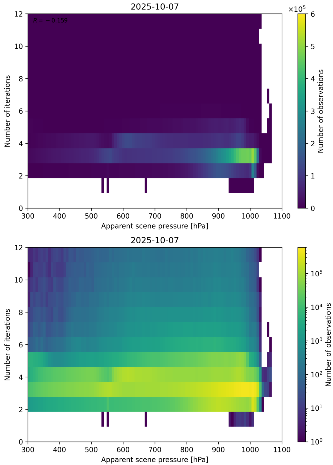
Figure 65: Scatter density plot of “Apparent scene pressure” against “Number of iterations” for 2025-10-06 to 2025-10-08.
