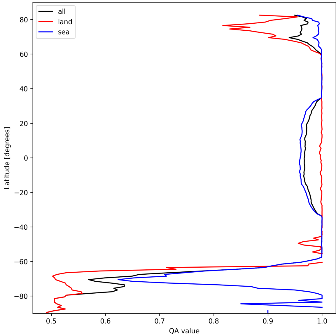
Figure 12: Zonal average of “QA value” for 2025-10-06 to 2025-10-08.
