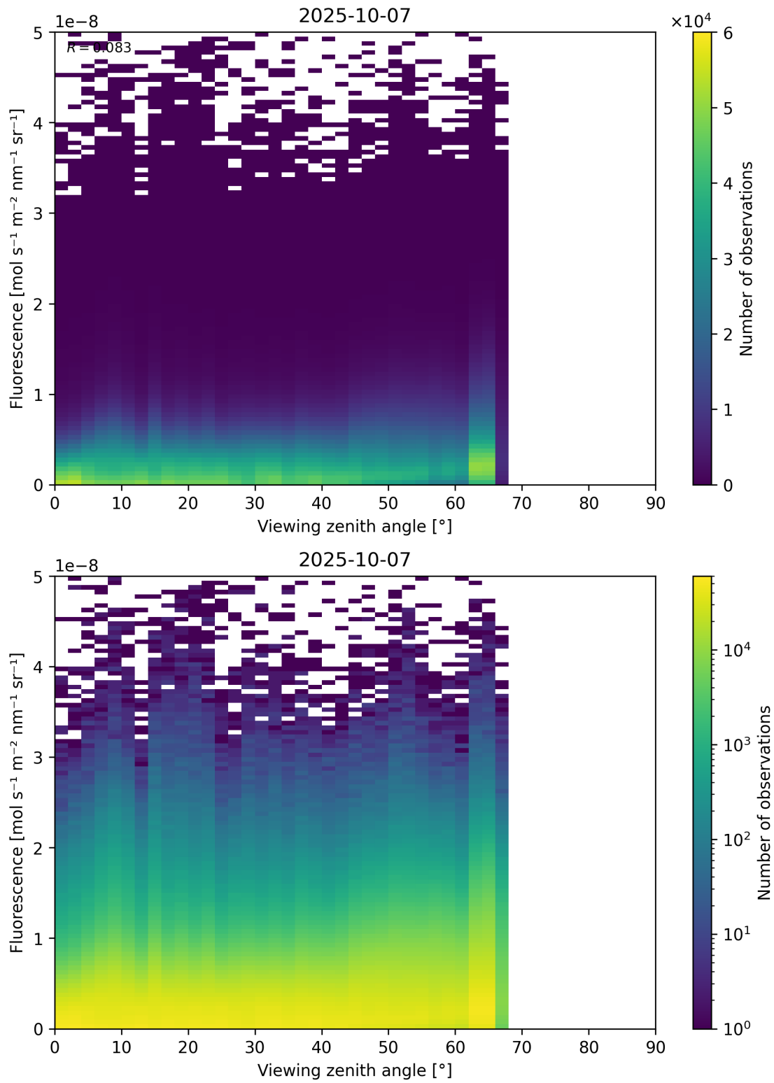
Figure 122: Scatter density plot of “Viewing zenith angle” against “Fluorescence” for 2025-10-06 to 2025-10-08.
