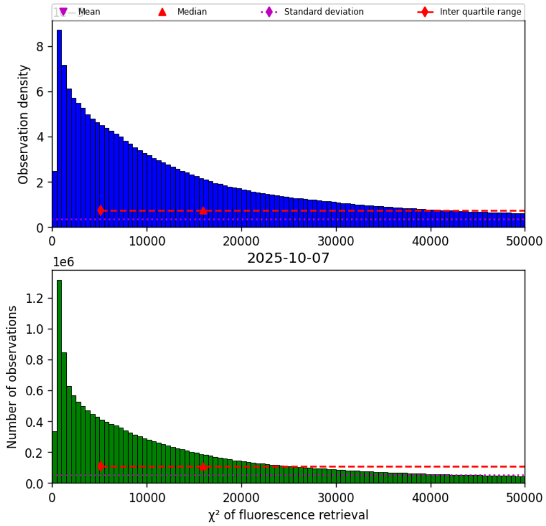
Figure 42: Histogram of “ \chi^2 of fluorescence retrieval” for 2025-10-06 to 2025-10-08
