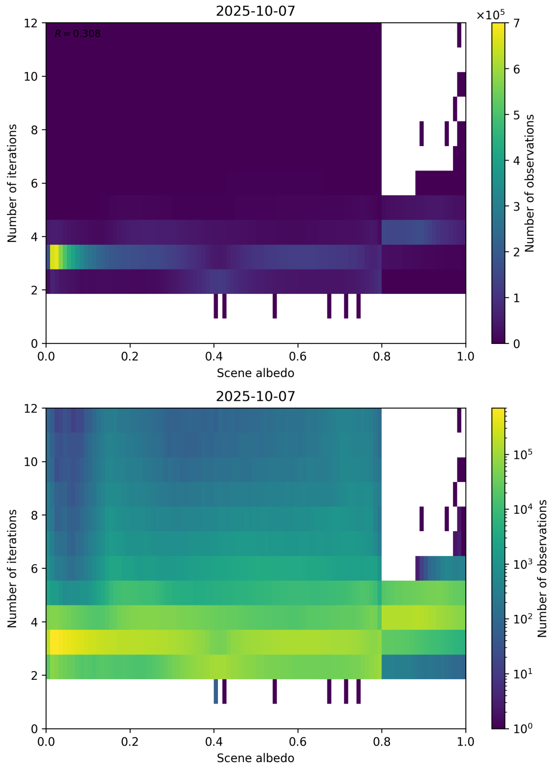
Figure 105: Scatter density plot of “Scene albedo” against “Number of iterations” for 2025-10-06 to 2025-10-08.
