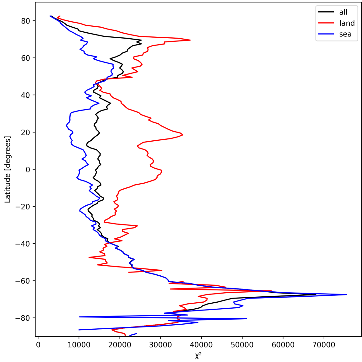
Figure 21: Zonal average of “ \chi^2 ” for 2025-10-06 to 2025-10-08.
