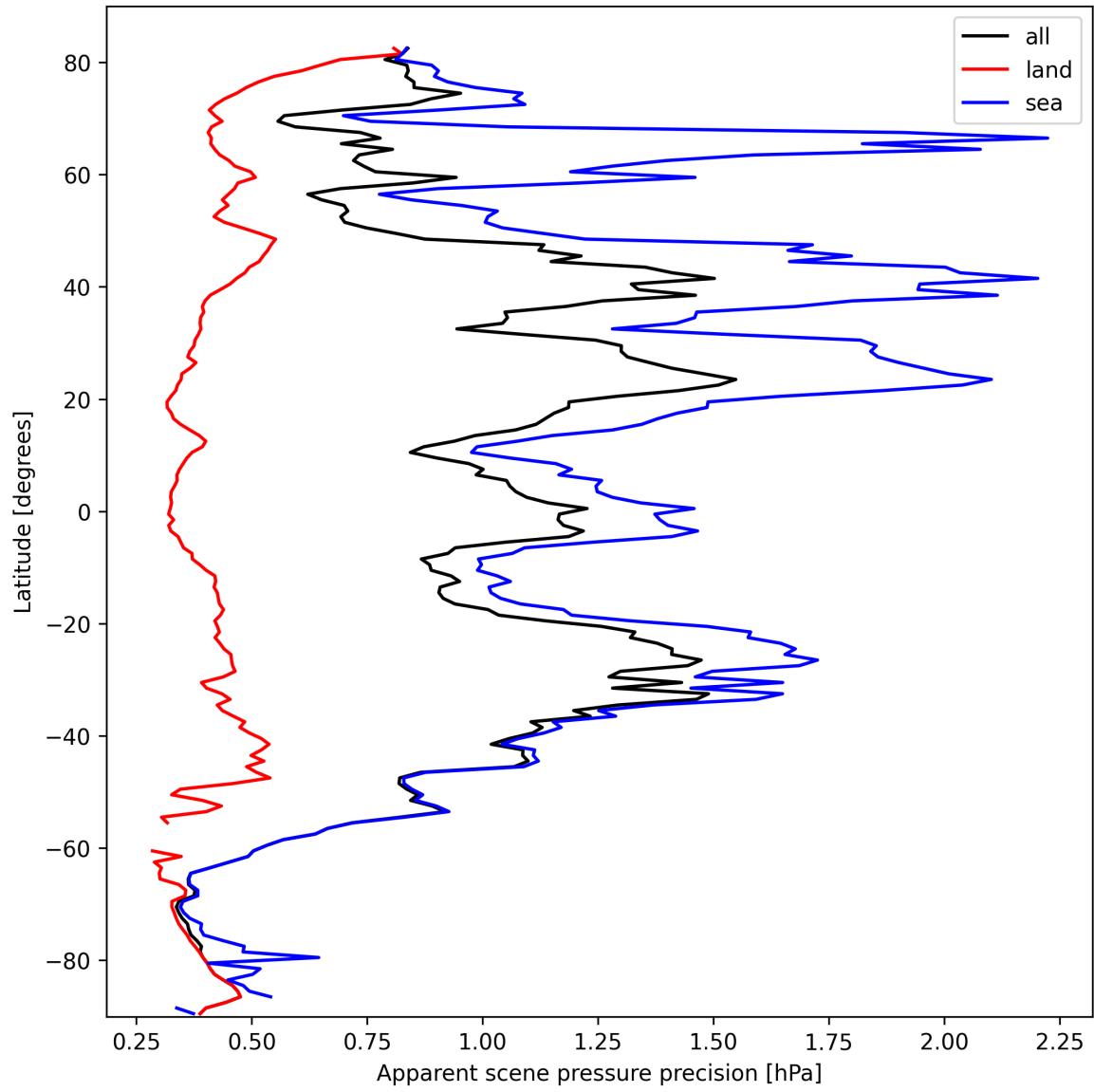
Figure 20: Zonal average of “Apparent scene pressure precision” for 2025-10-06 to 2025-10-08.
