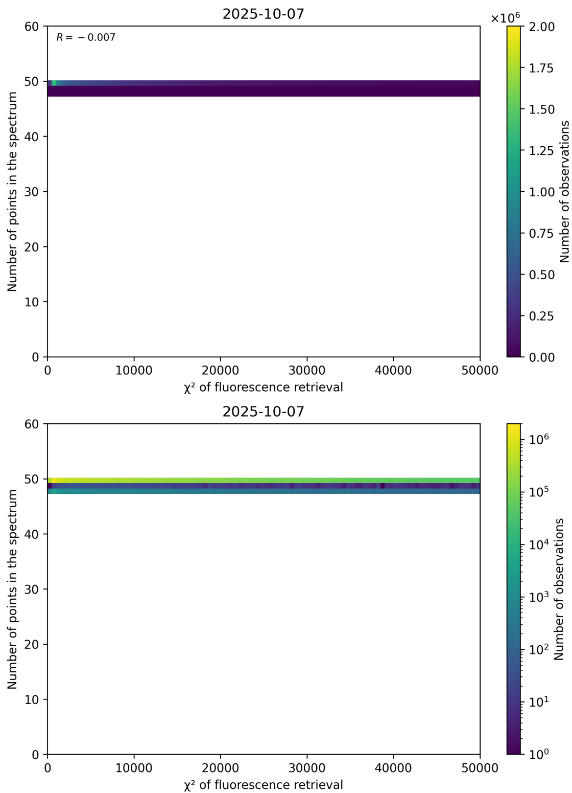
Figure 68: Scatter density plot of “ \chi^2 of fluorescence retrieval” against “Number of points in the spectrum” for 2025-10-06 to 2025-10-08.
