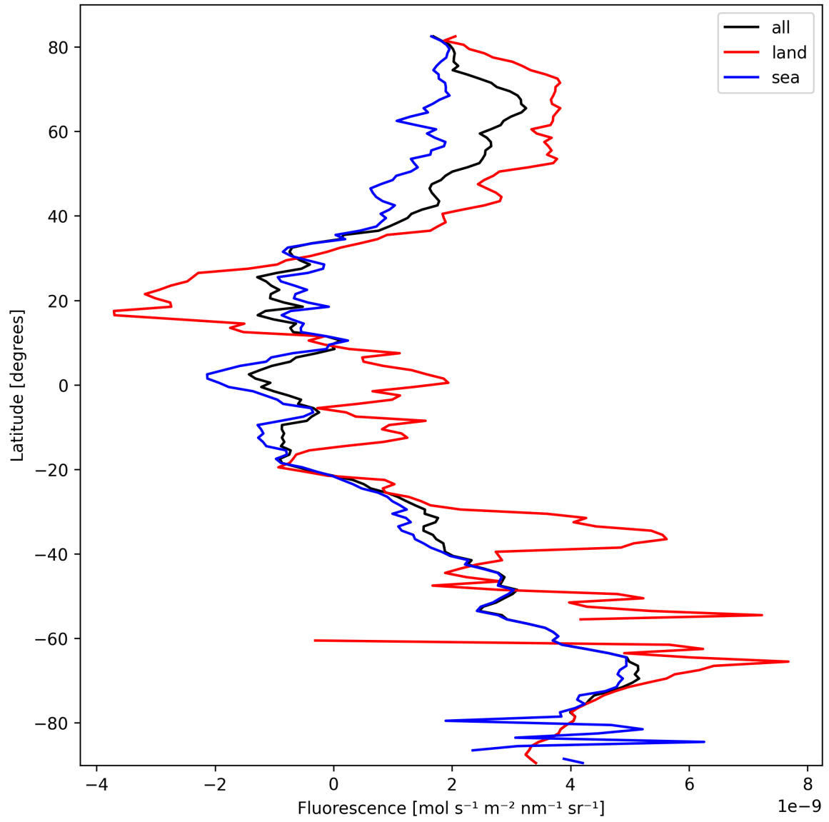
Figure 23: Zonal average of “Fluorescence” for 2025-10-06 to 2025-10-08.
