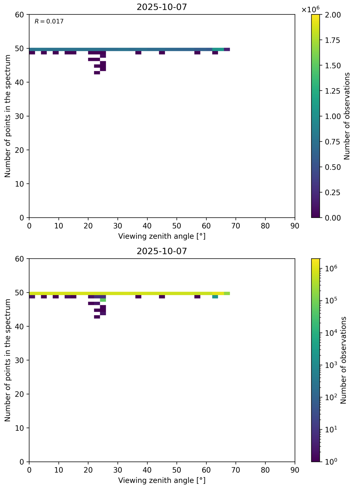
Figure 125: Scatter density plot of “Viewing zenith angle” against “Number of points in the spectrum” for 2025-10-06 to 2025-10-08.
