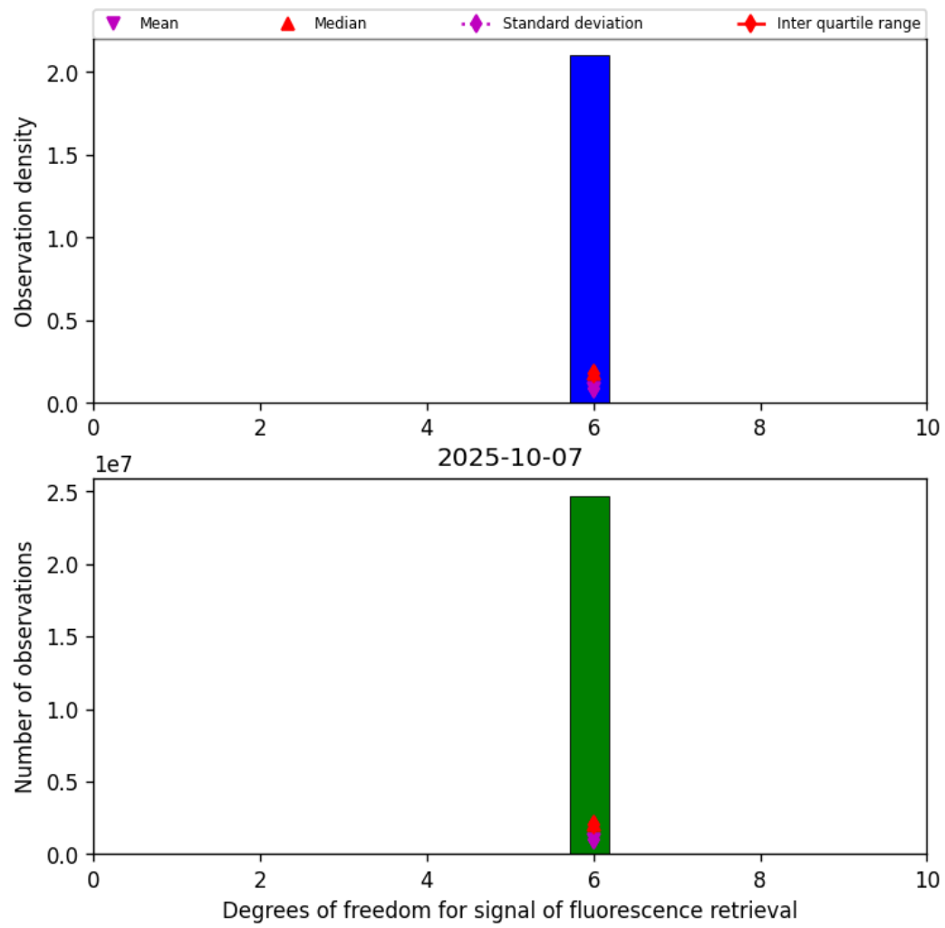
Figure 43: Histogram of “Degrees of freedom for signal of fluorescence retrieval” for 2025-10-06 to 2025-10-08
