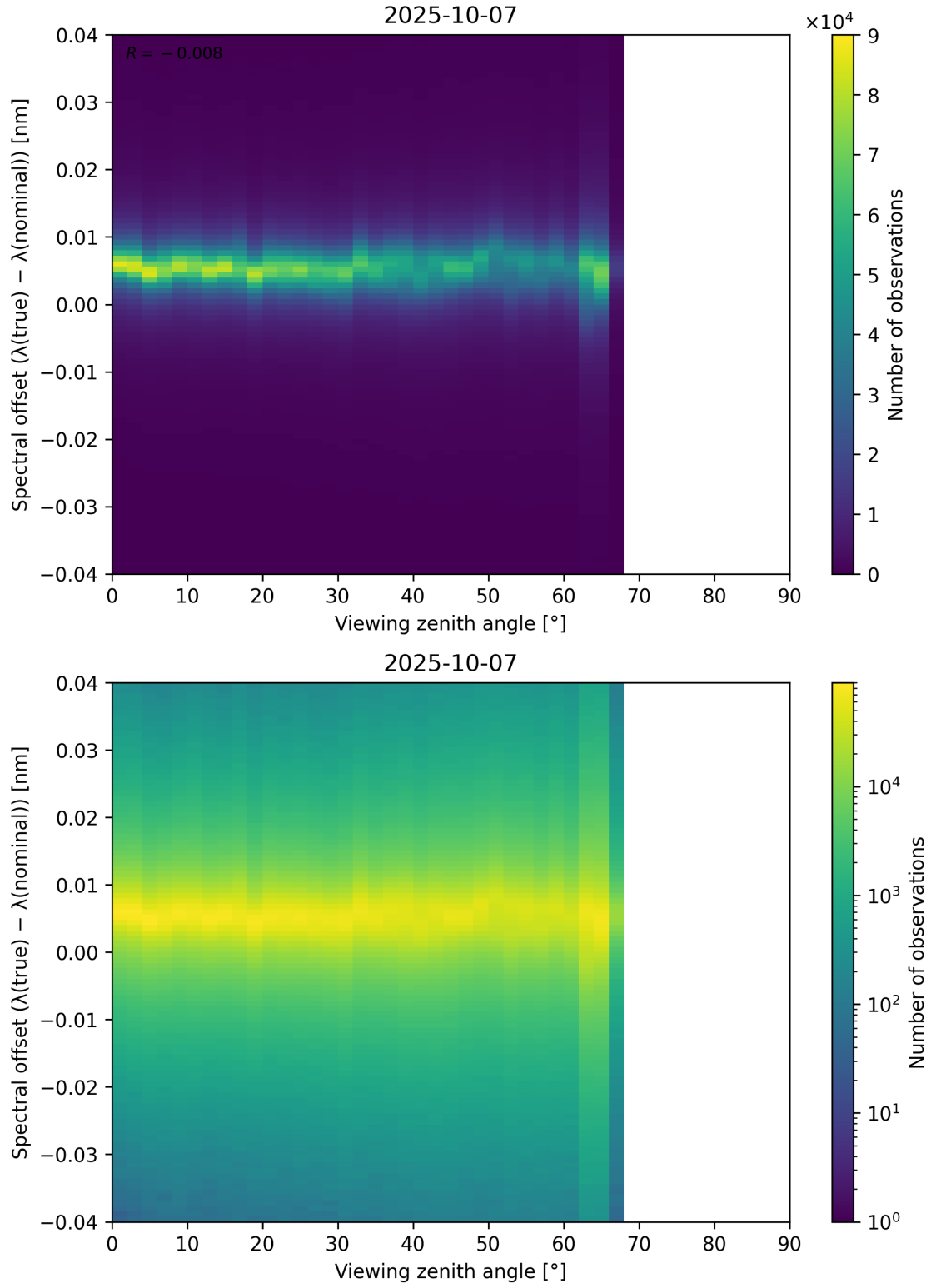
Figure 128: Scatter density plot of “Viewing zenith angle” against “Spectral offset ( \lambda_{\text{true}} - \lambda_{\text{nominal}} )” for 2025-10-06 to 2025-10-08.
