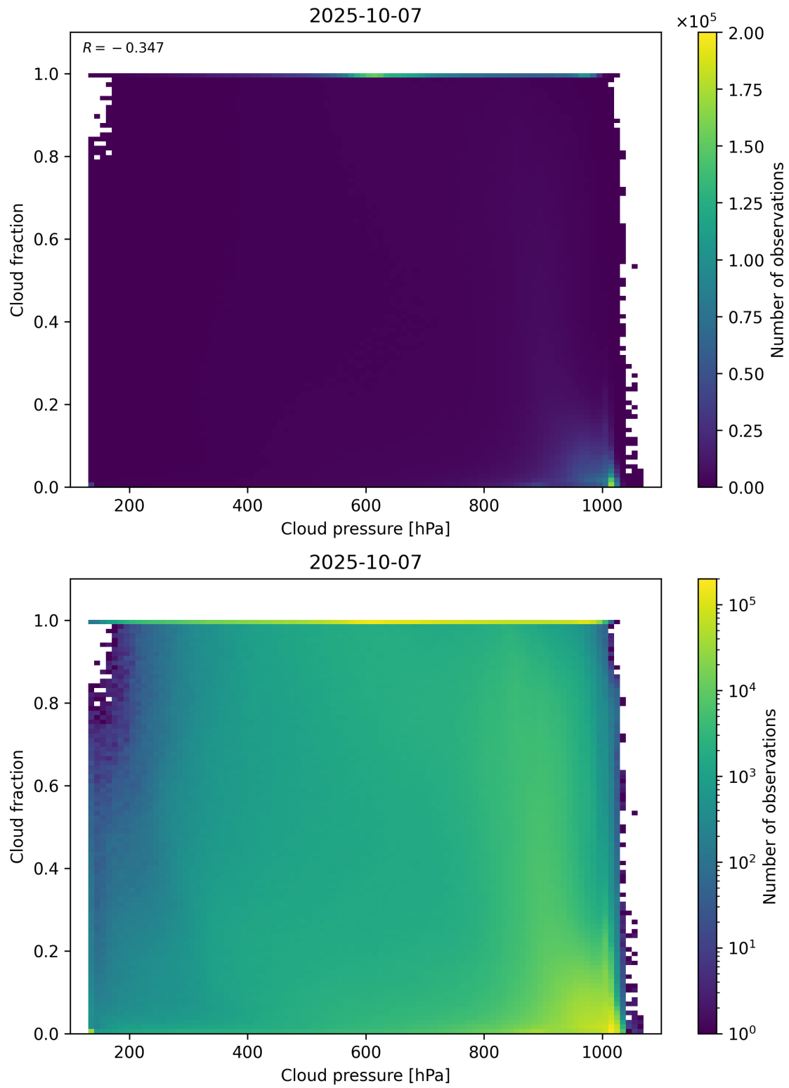
Figure 79: Scatter density plot of “Cloud pressure” against “Cloud fraction” for 2025-10-06 to 2025-10-08.
