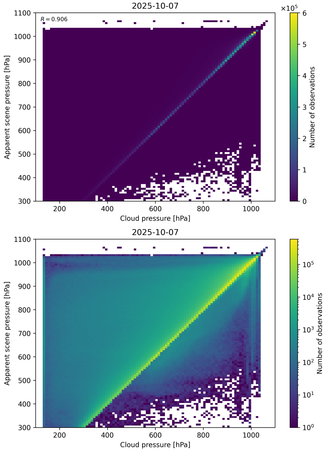
Figure 77: Scatter density plot of “Cloud pressure” against “Apparent scene pressure” for 2025-10-06 to 2025-10-08.
