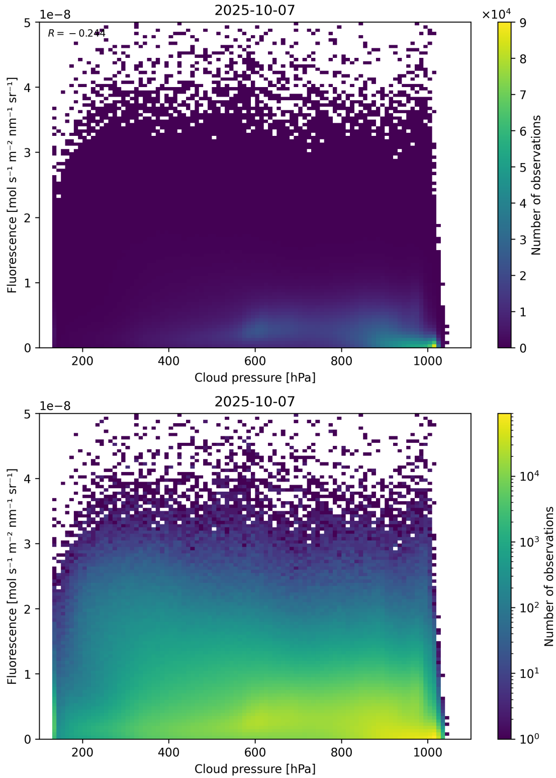
Figure 80: Scatter density plot of “Cloud pressure” against “Fluorescence” for 2025-10-06 to 2025-10-08.
