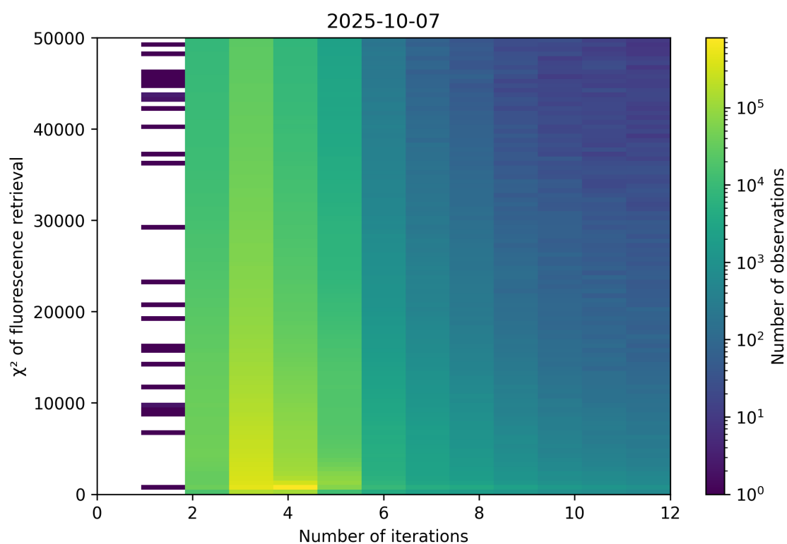
Figure 97: Scatter density plot of “Number of iterations” against “ \chi^2 of fluorescence retrieval” for 2025-10-06 to 2025-10-08.
