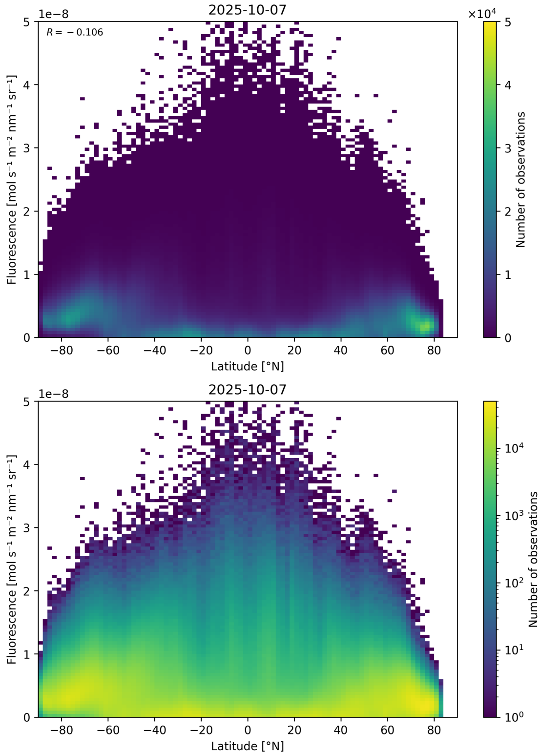
Figure 92: Scatter density plot of “Latitude” against “Fluorescence” for 2025-10-06 to 2025-10-08.
