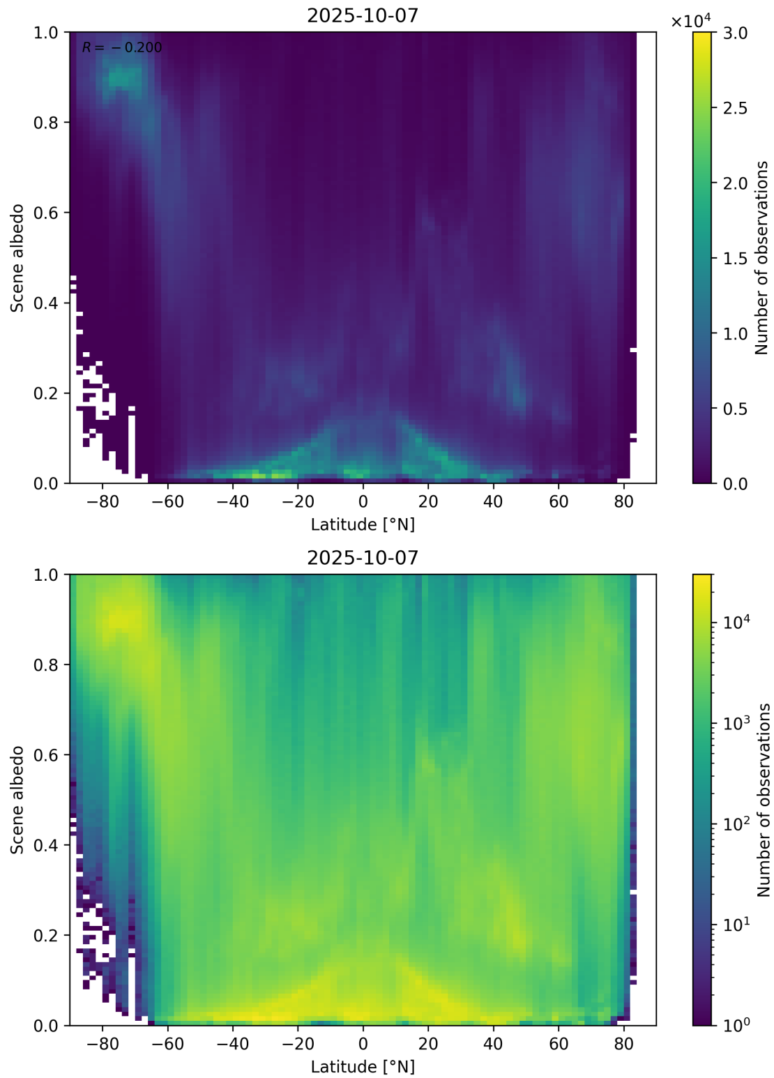
Figure 95: Scatter density plot of “Latitude” against “Scene albedo” for 2025-10-06 to 2025-10-08.
