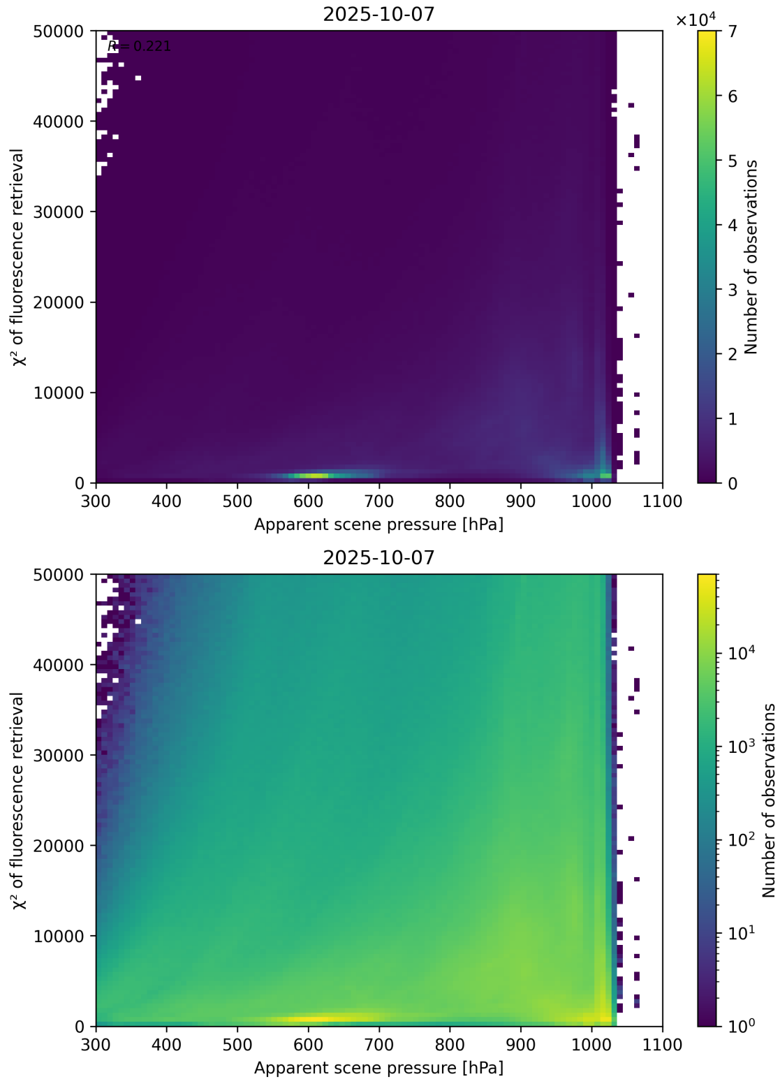
Figure 63: Scatter density plot of “Apparent scene pressure” against “ \chi^2 of fluorescence retrieval” for 2025-10-06 to 2025-10-08.
