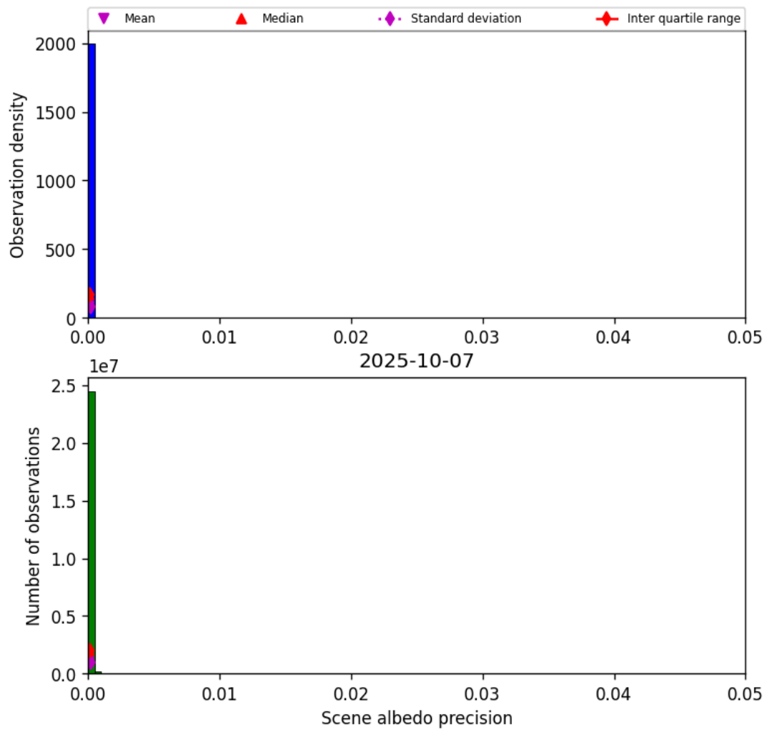
Figure 35: Histogram of “Scene albedo precision” for 2025-10-06 to 2025-10-08
