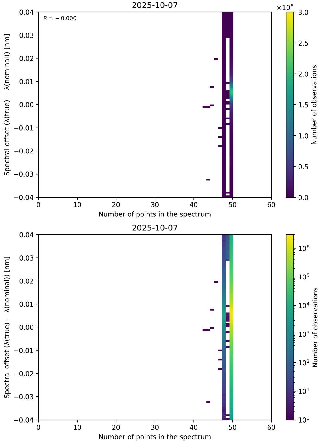
Figure 101: Scatter density plot of “Number of points in the spectrum” against “Spectral offset ( \lambda_{\text{true}} - \lambda_{\text{nominal}} )” for 2025-10-06 to 2025-10-08.
