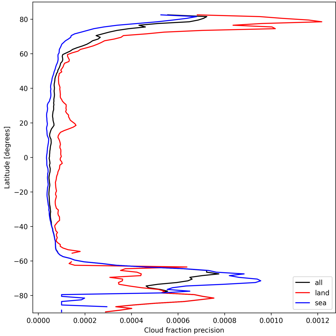
Figure 16: Zonal average of “Cloud fraction precision” for 2025-10-06 to 2025-10-08.
