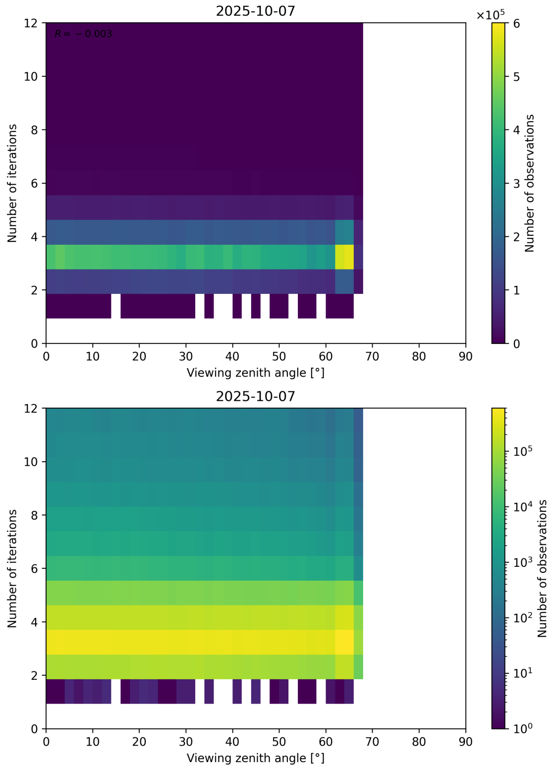
Figure 124: Scatter density plot of “Viewing zenith angle” against “Number of iterations” for 2025-10-06 to 2025-10-08.
