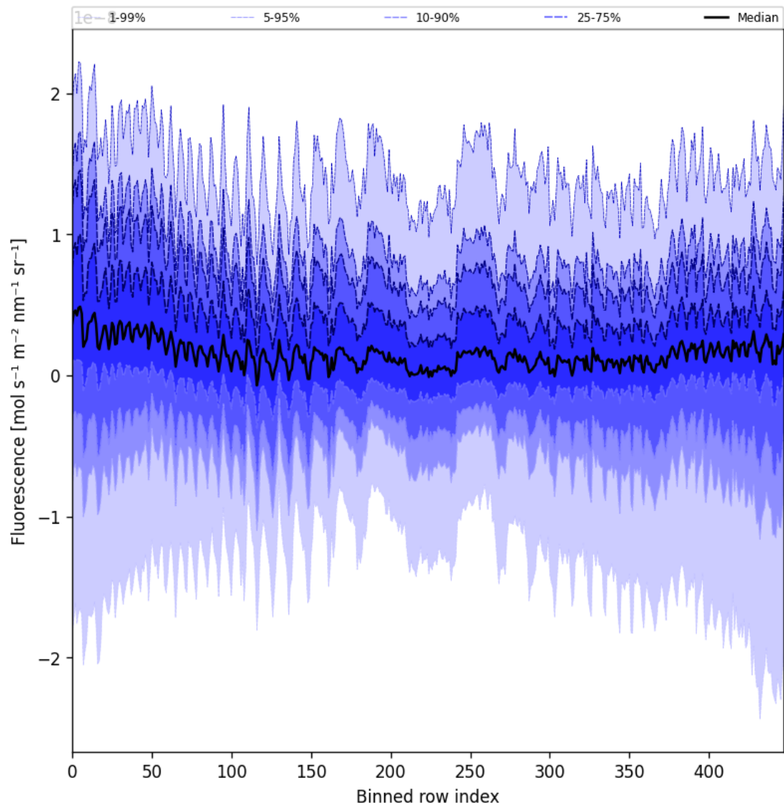
Figure 57: Along track statistics of “Fluorescence” for 2025-10-06 to 2025-10-08
