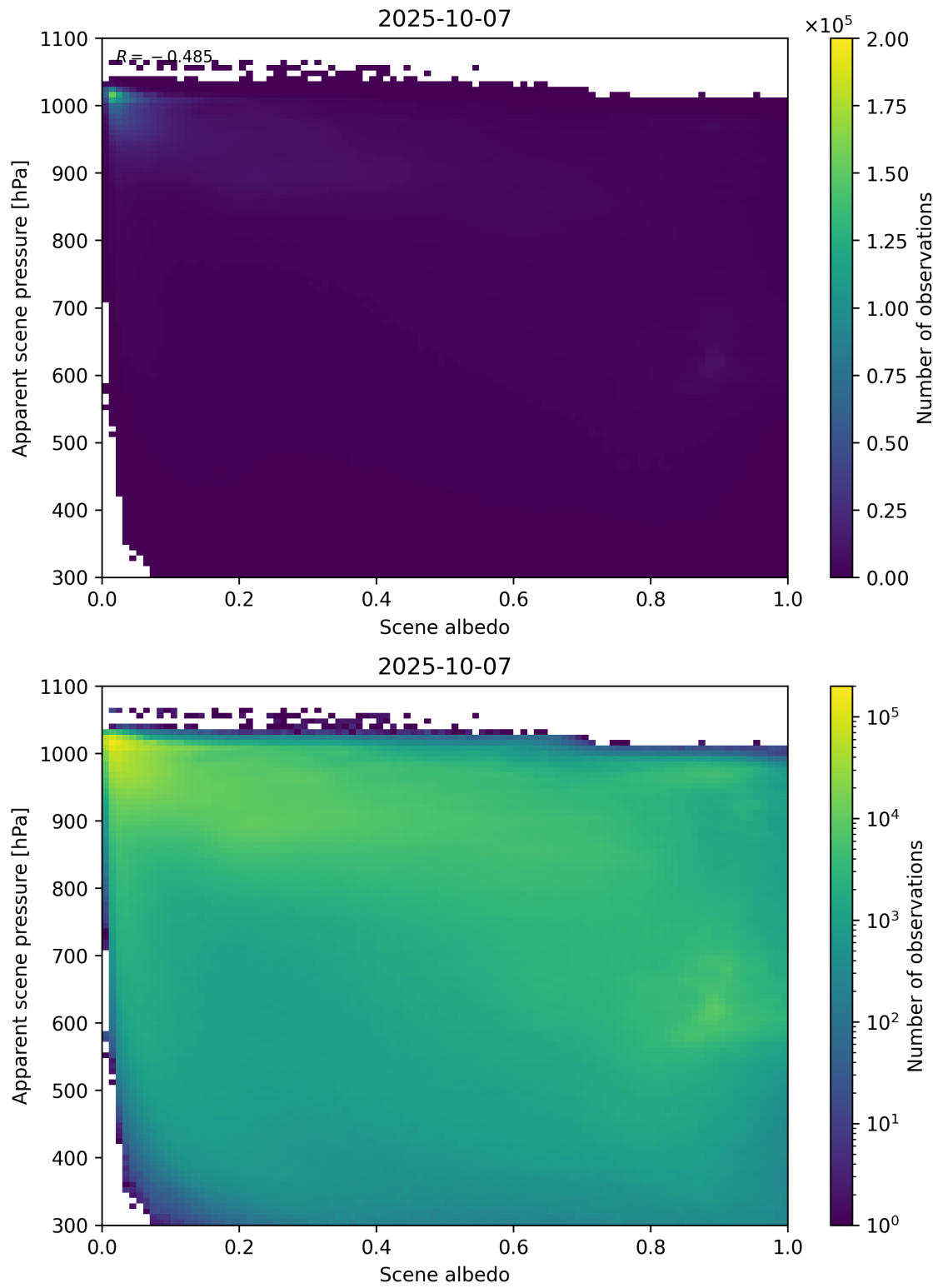
Figure 102: Scatter density plot of “Scene albedo” against “Apparent scene pressure” for 2025-10-06 to 2025-10-08.
