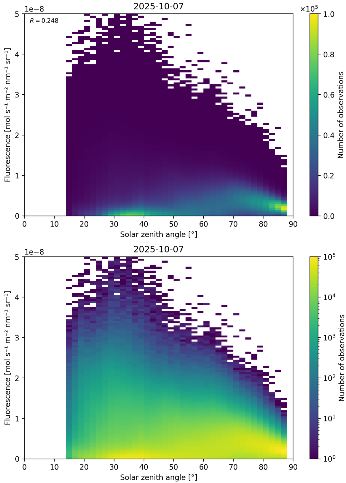
Figure 112: Scatter density plot of “Solar zenith angle” against “Fluorescence” for 2025-10-06 to 2025-10-08.
