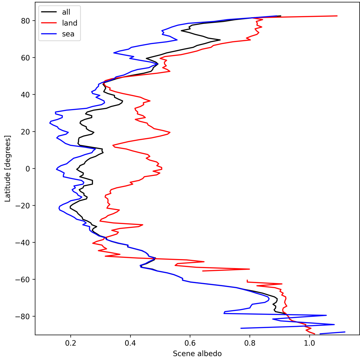
Figure 17: Zonal average of “Scene albedo” for 2025-10-06 to 2025-10-08.
