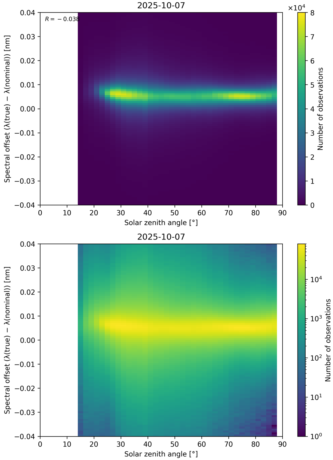
Figure 117: Scatter density plot of “Solar zenith angle” against “Spectral offset ( \lambda_{\text{true}} - \lambda_{\text{nominal}} )” for 2025-10-06 to 2025-10-08.
