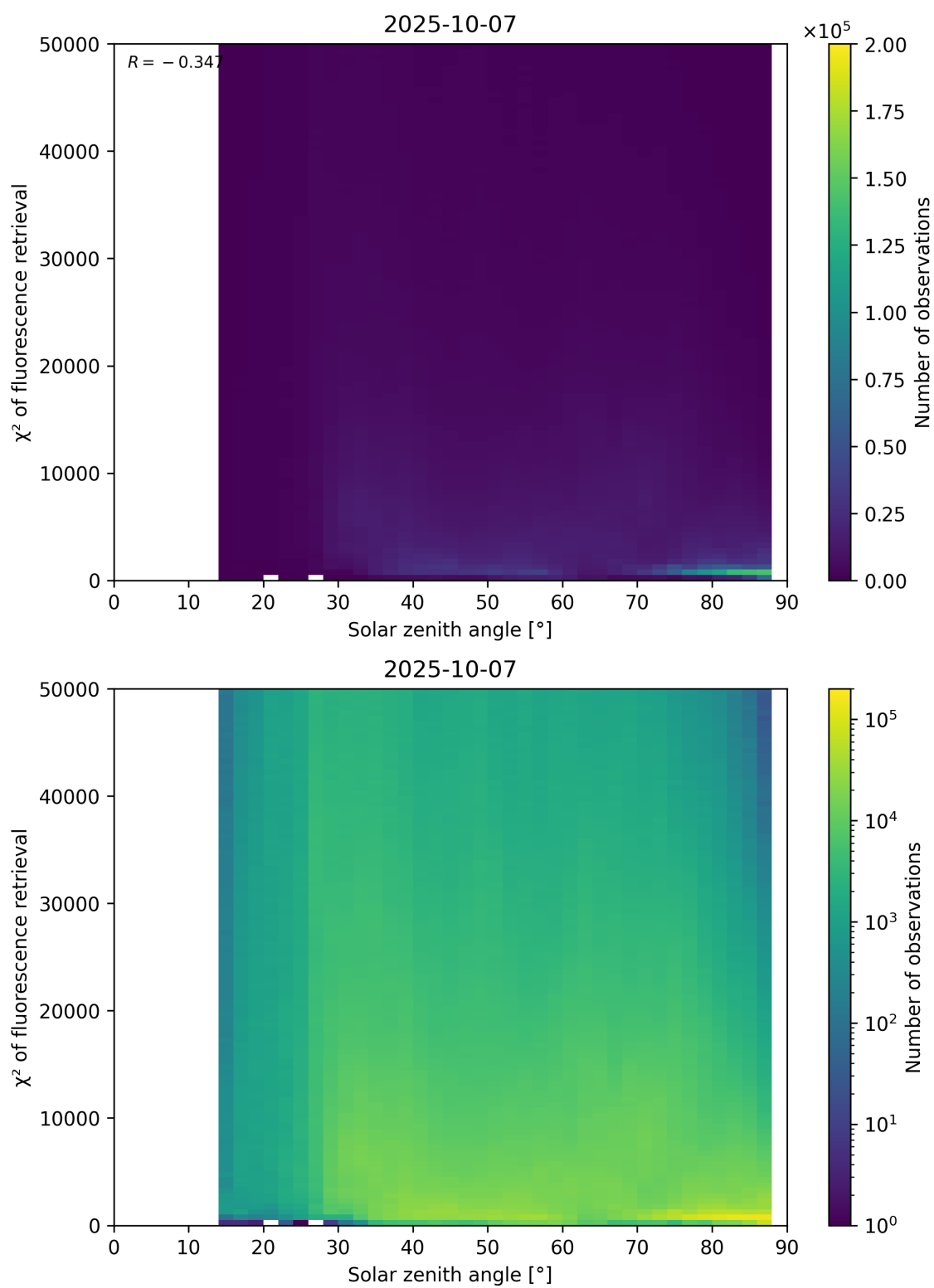
Figure 109: Scatter density plot of “Solar zenith angle” against “ \chi^2 of fluorescence retrieval” for 2025-10-06 to 2025-10-08.
