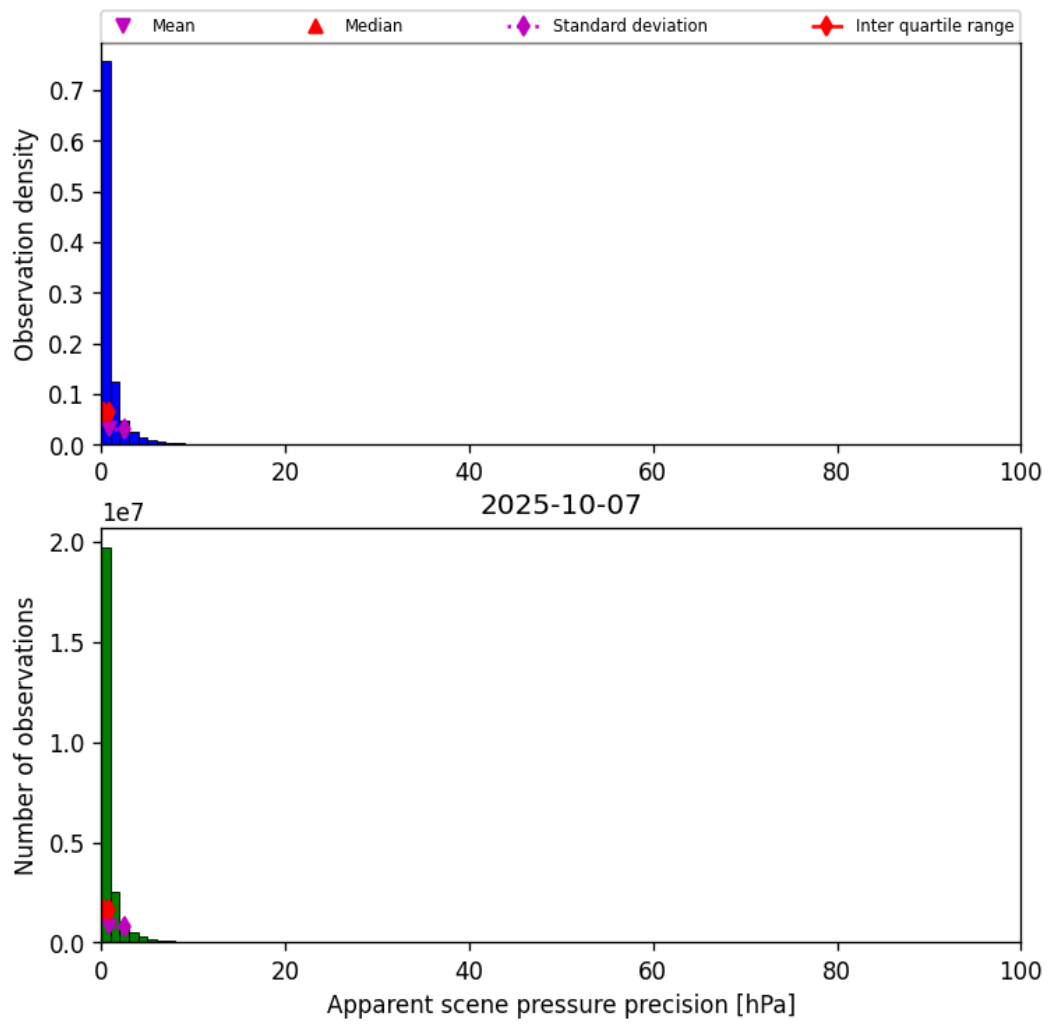
Figure 37: Histogram of “Apparent scene pressure precision” for 2025-10-06 to 2025-10-08
