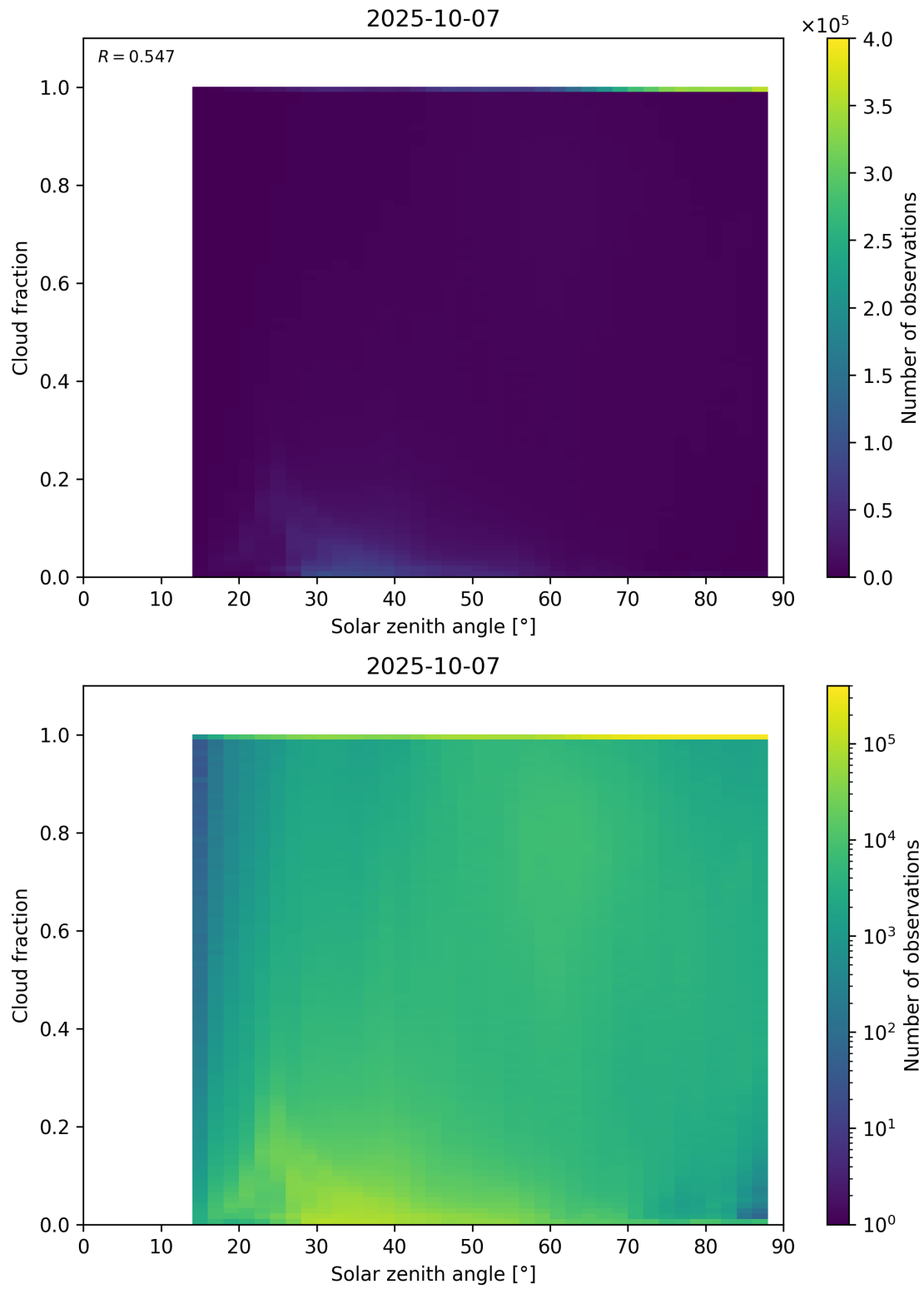
Figure 110: Scatter density plot of “Solar zenith angle” against “Cloud fraction” for 2025-10-06 to 2025-10-08.
