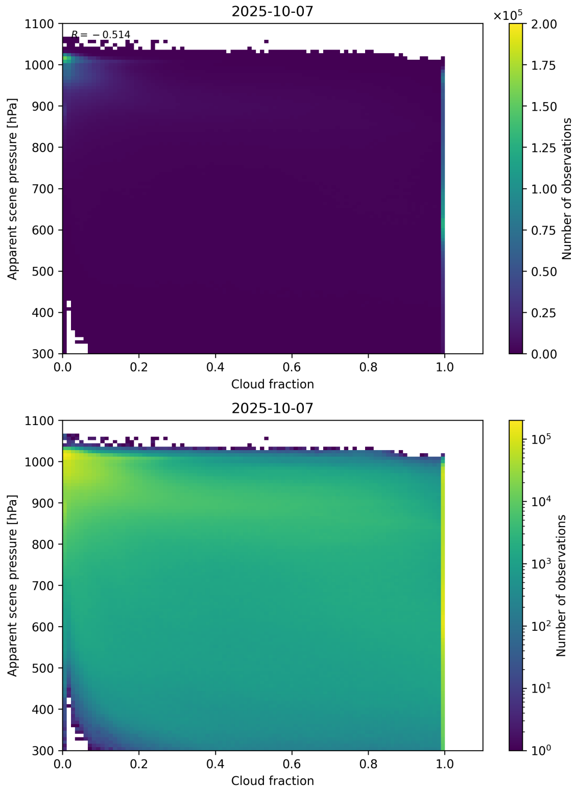
Figure 70: Scatter density plot of “Cloud fraction” against “Apparent scene pressure” for 2025-10-06 to 2025-10-08.
