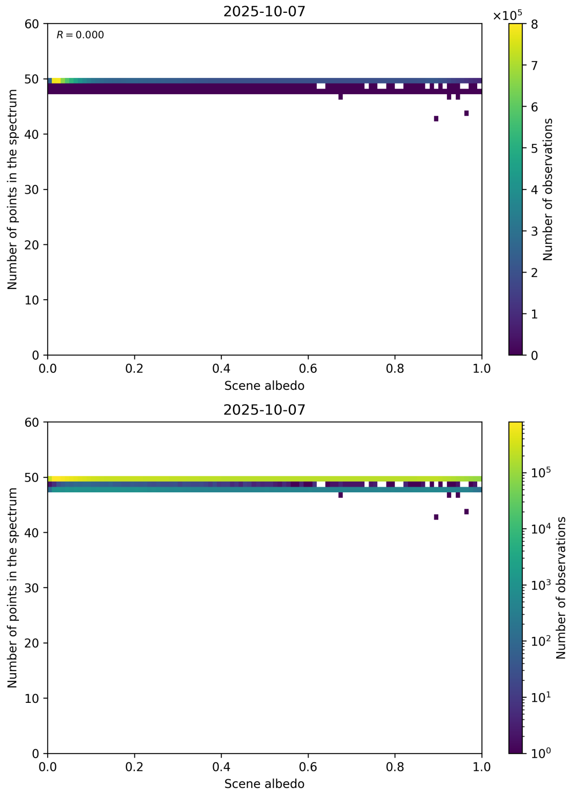
Figure 106: Scatter density plot of “Scene albedo” against “Number of points in the spectrum” for 2025-10-06 to 2025-10-08.
