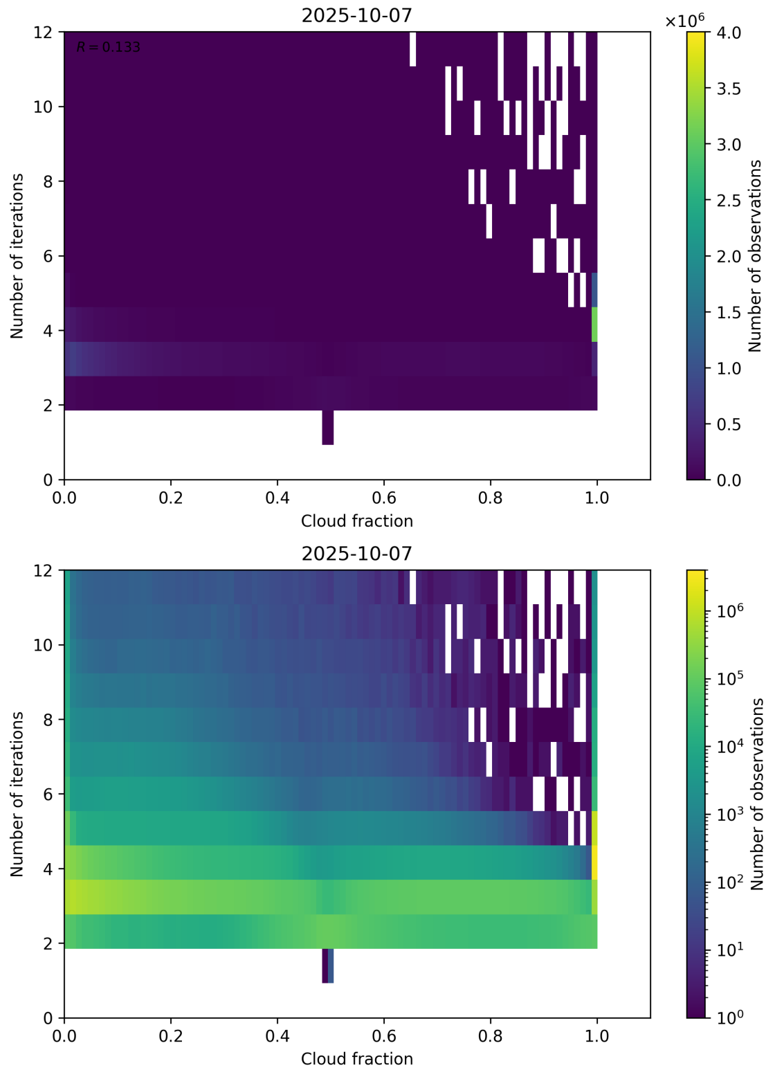
Figure 73: Scatter density plot of “Cloud fraction” against “Number of iterations” for 2025-10-06 to 2025-10-08.
