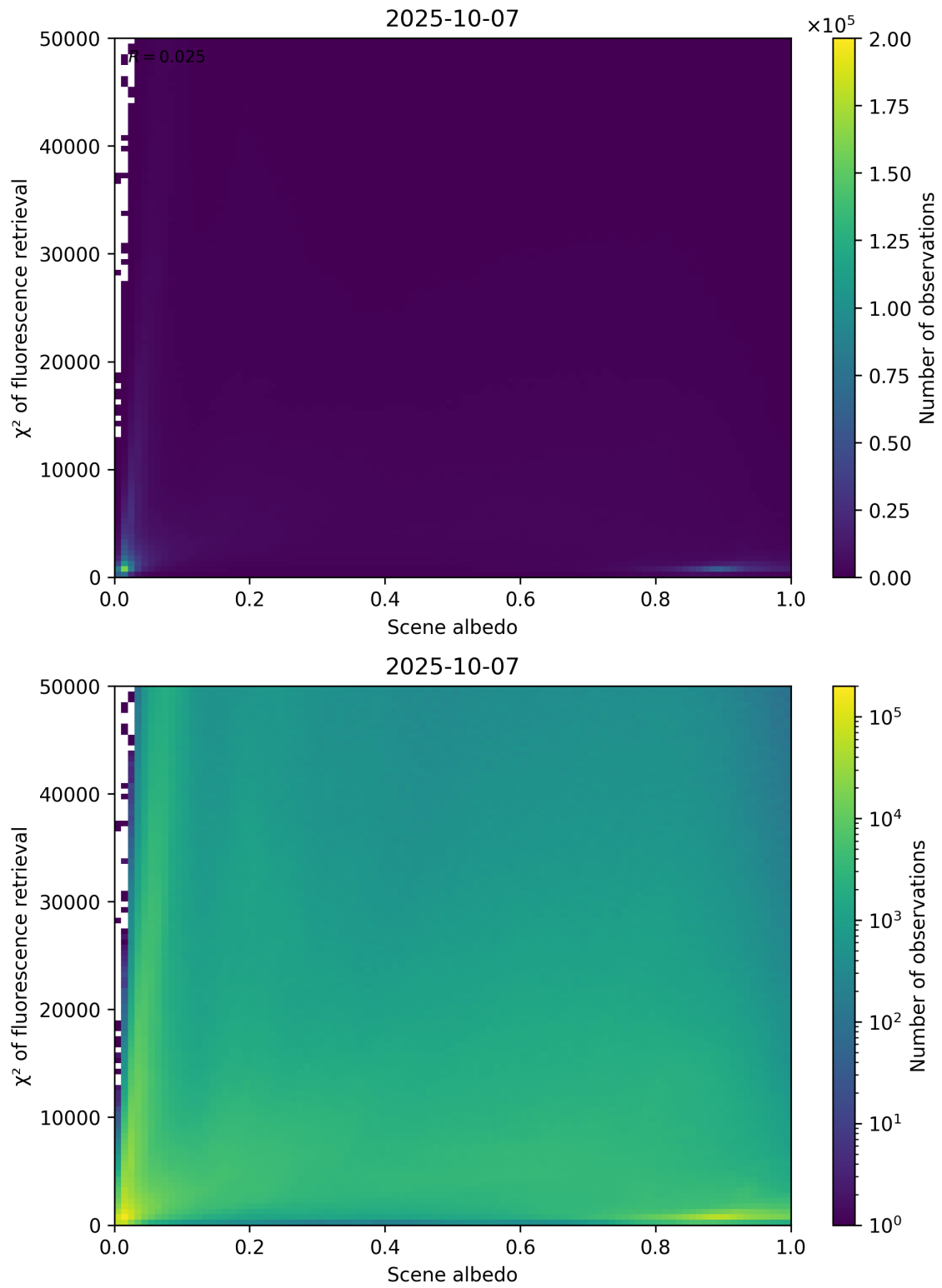
Figure 103: Scatter density plot of “Scene albedo” against “ \chi^2 of fluorescence retrieval” for 2025-10-06 to 2025-10-08.
