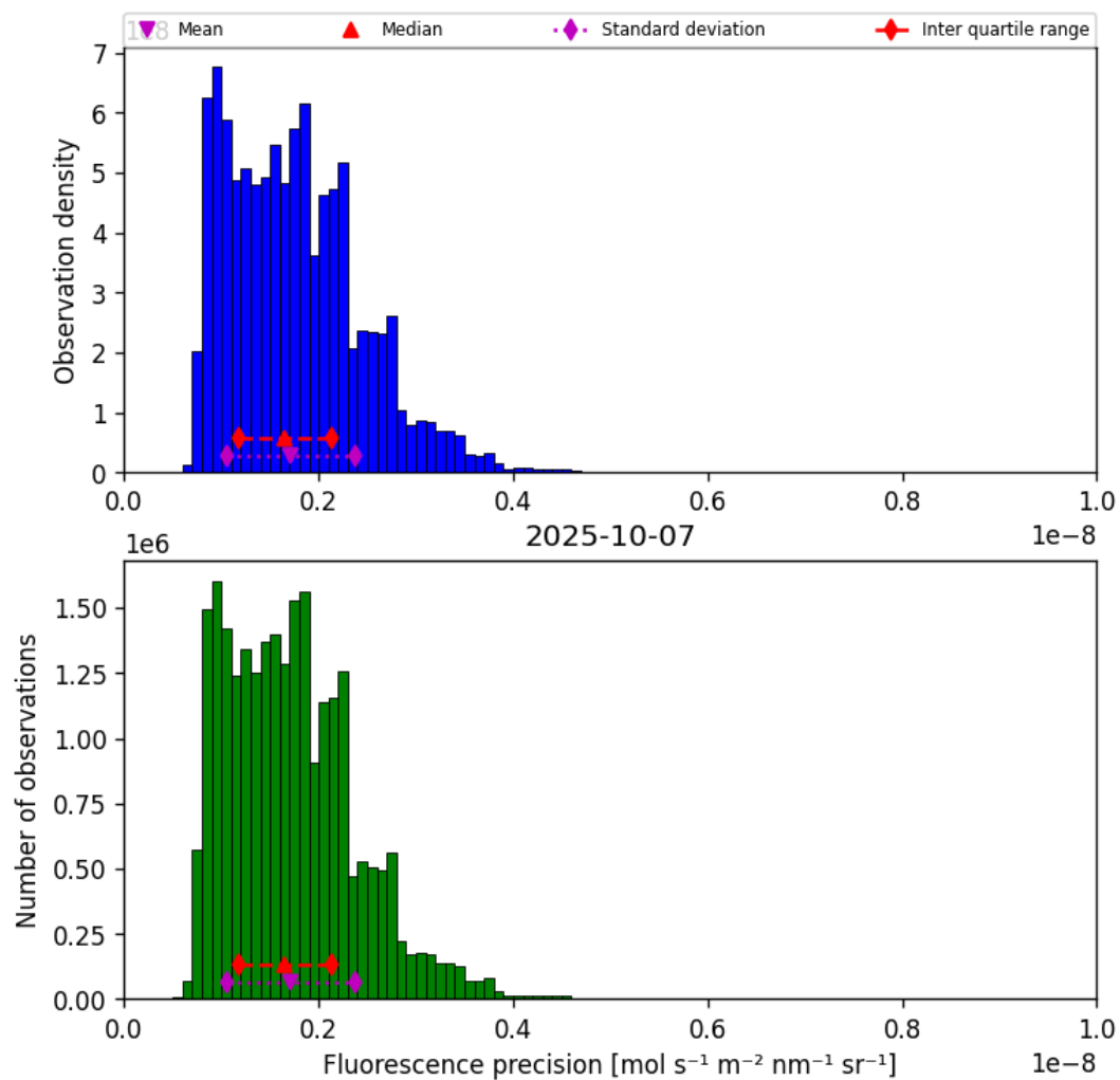
Figure 41: Histogram of “Fluorescence precision” for 2025-10-06 to 2025-10-08
