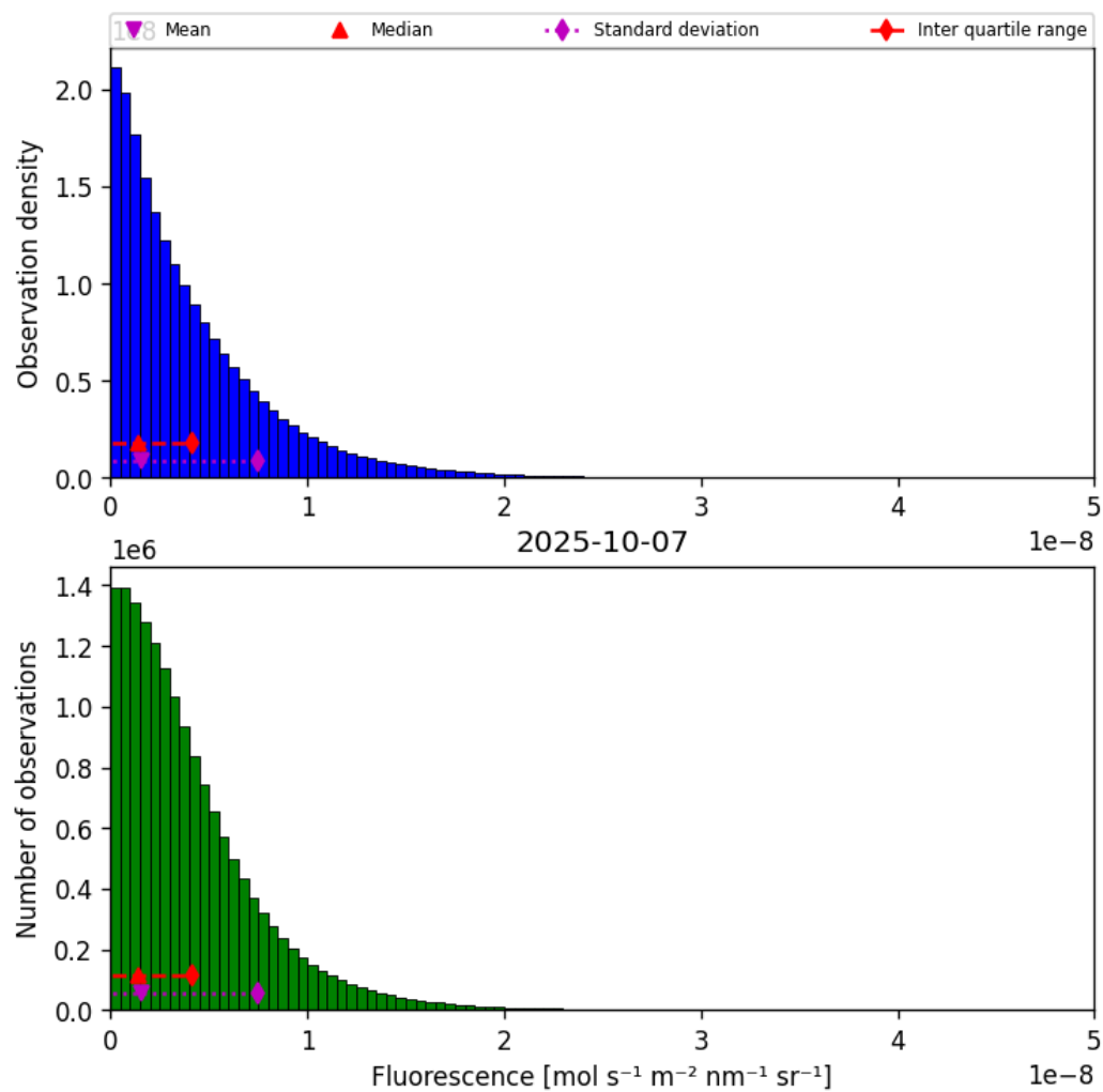
Figure 40: Histogram of “Fluorescence” for 2025-10-06 to 2025-10-08
