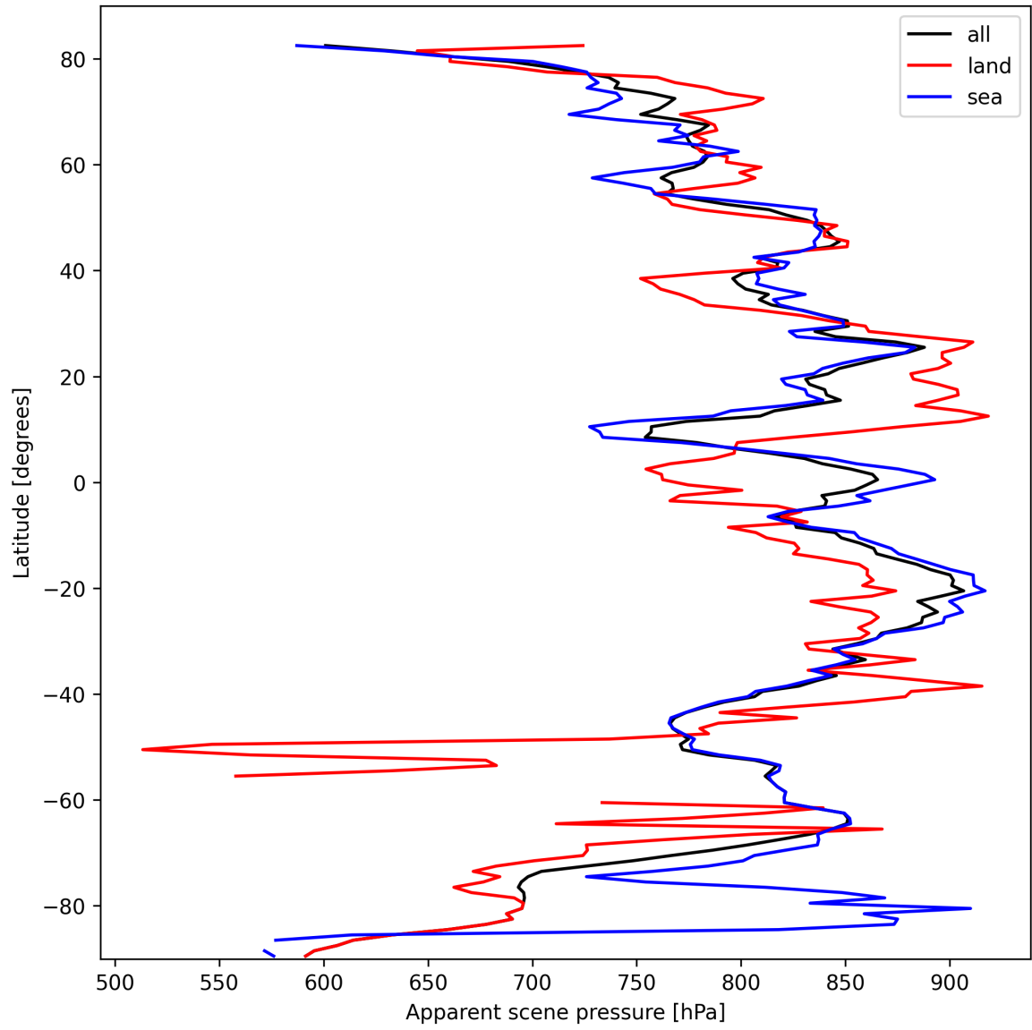
Figure 19: Zonal average of “Apparent scene pressure” for 2025-10-06 to 2025-10-08.
