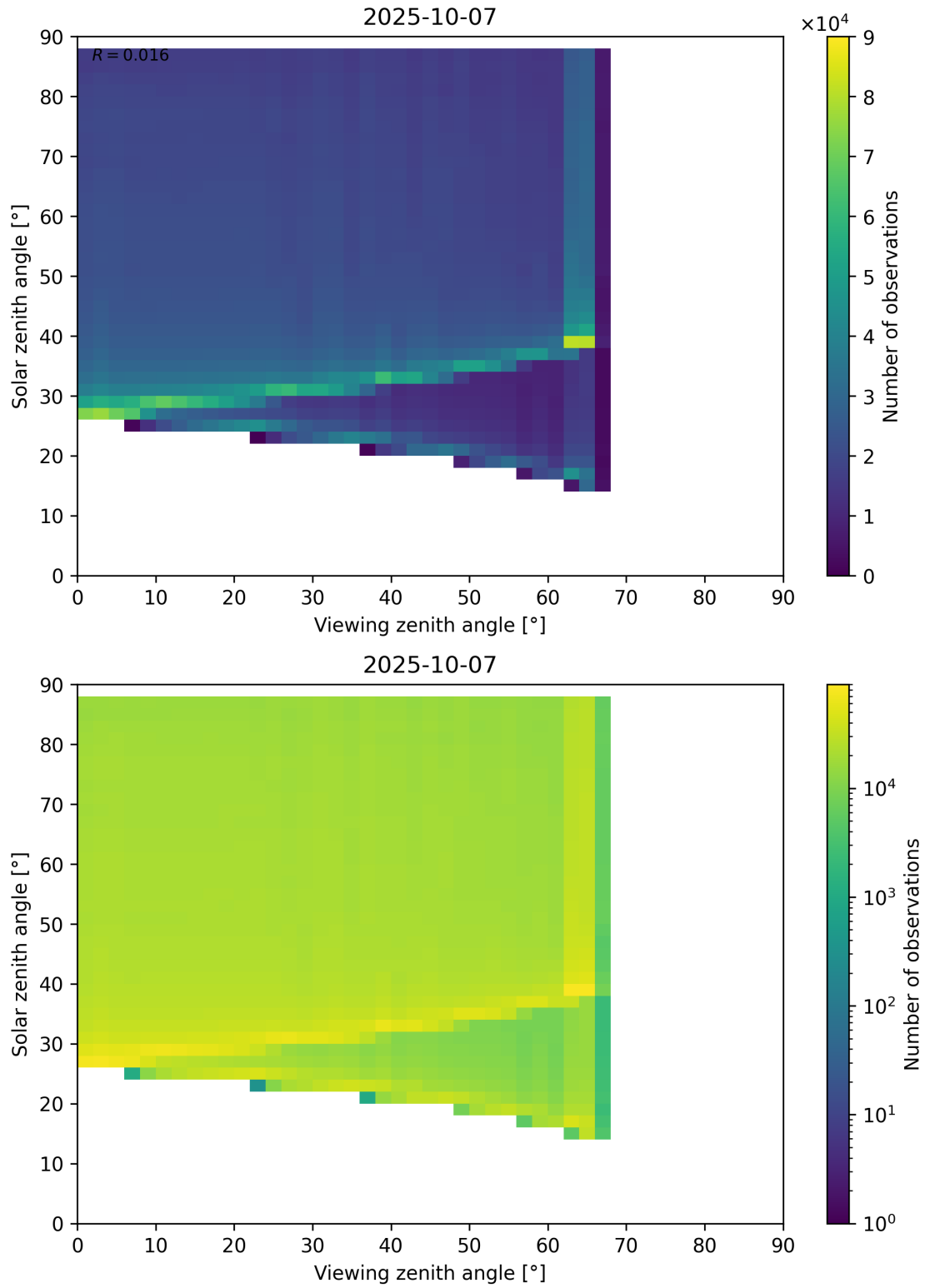
Figure 127: Scatter density plot of “Viewing zenith angle” against “Solar zenith angle” for 2025-10-06 to 2025-10-08.
