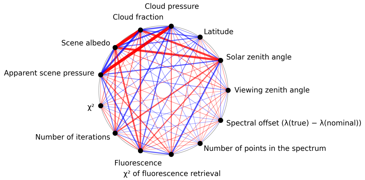
Figure 1: Map of correlation graph for 2025-10-06 to 2025-10-08.
