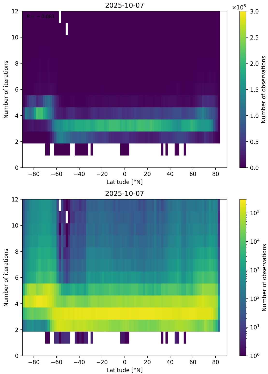
Figure 93: Scatter density plot of “Latitude” against “Number of iterations” for 2025-10-06 to 2025-10-08.
