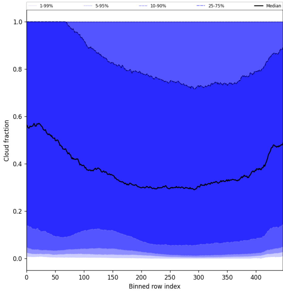
Figure 49: Along track statistics of “Cloud fraction” for 2025-10-06 to 2025-10-08
