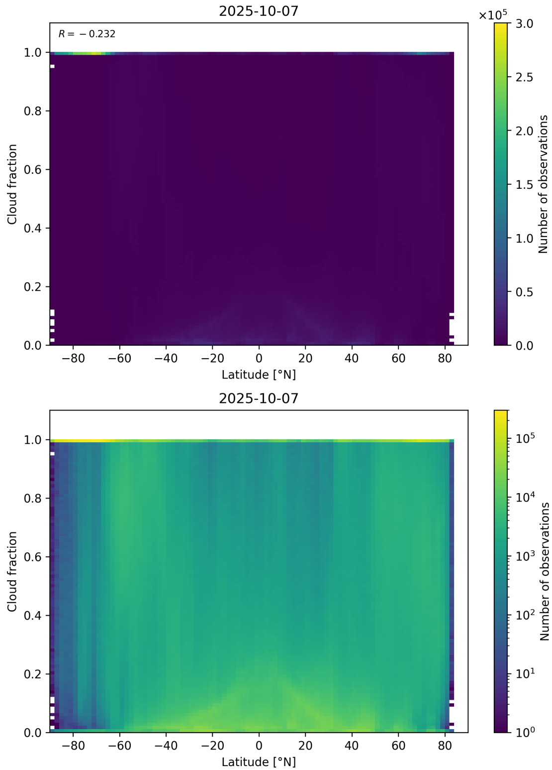
Figure 90: Scatter density plot of “Latitude” against “Cloud fraction” for 2025-10-06 to 2025-10-08.
