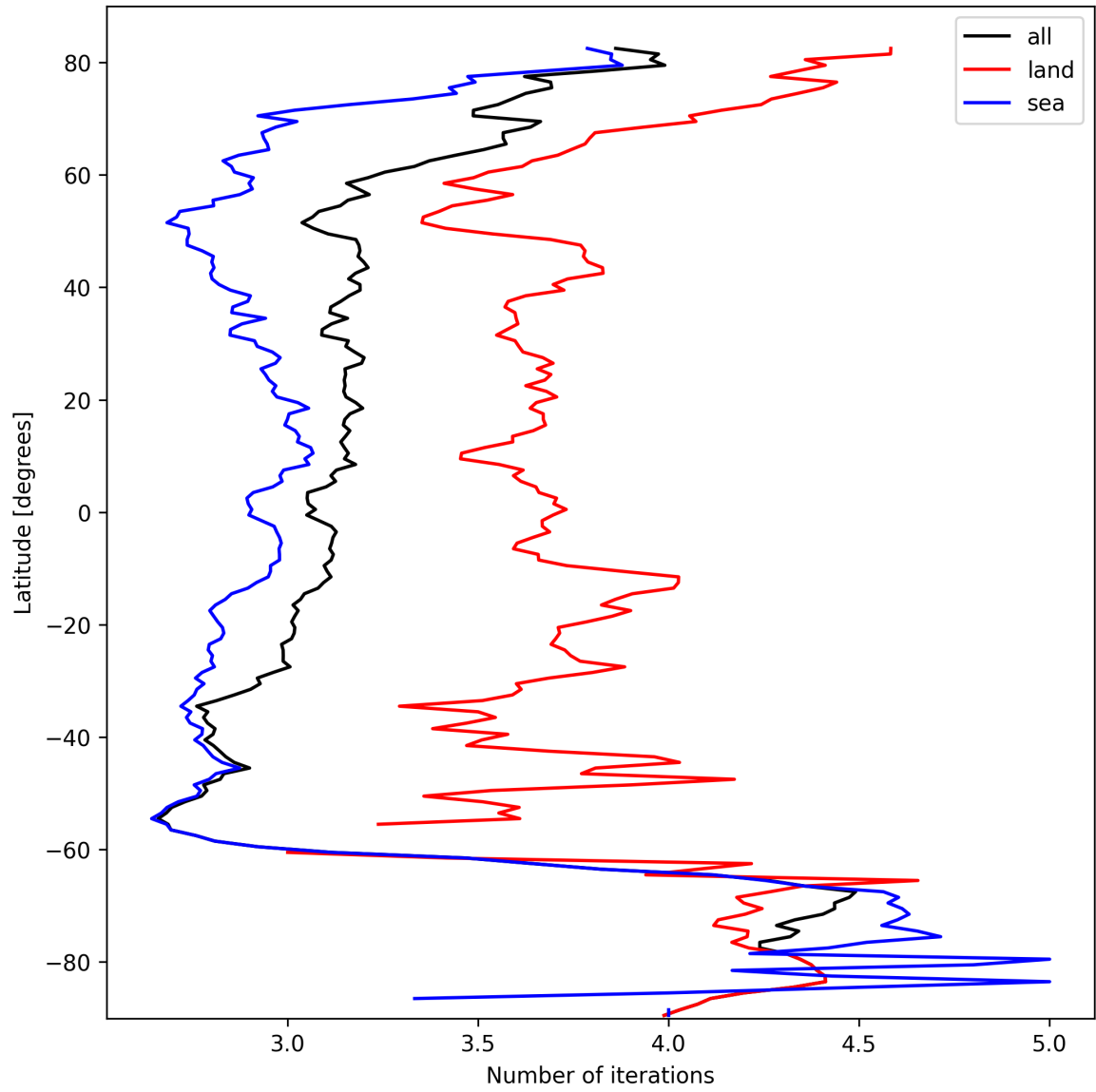
Figure 22: Zonal average of “Number of iterations” for 2025-10-06 to 2025-10-08.
