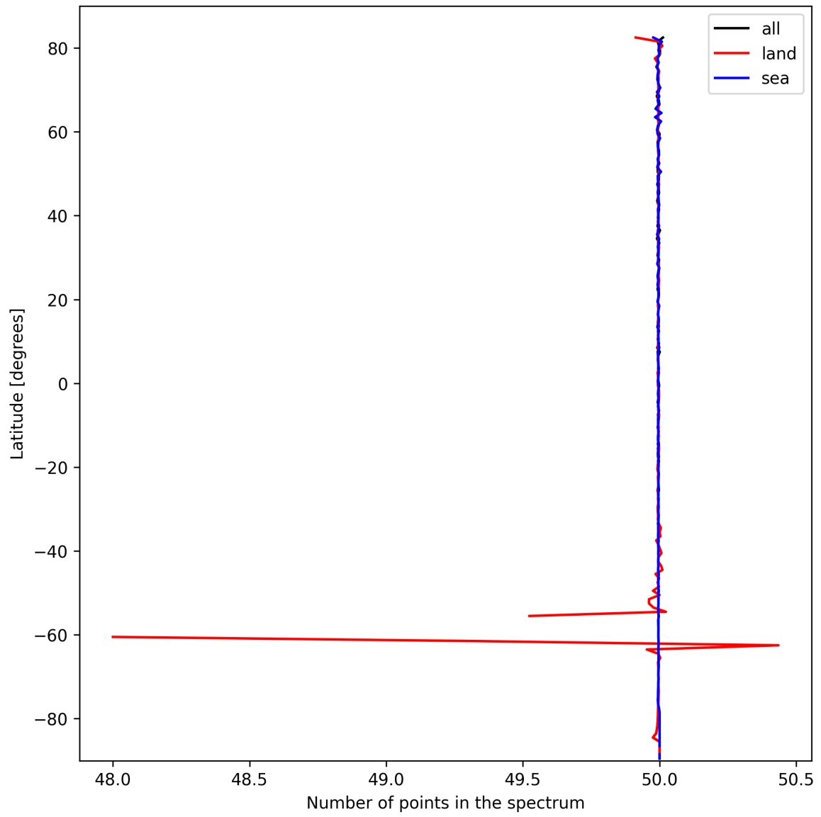
Figure 27: Zonal average of “Number of points in the spectrum” for 2025-10-06 to 2025-10-08.
