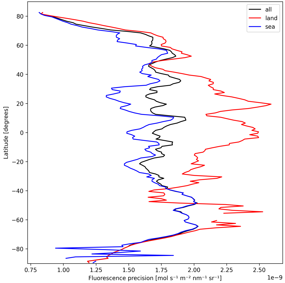
Figure 24: Zonal average of “Fluorescence precision” for 2025-10-06 to 2025-10-08.
