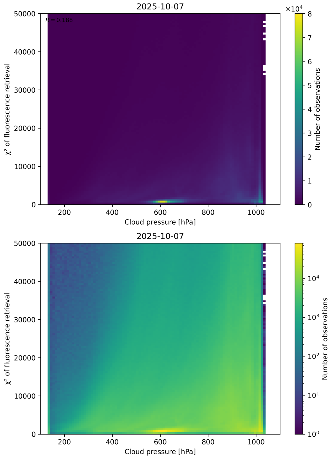
Figure 78: Scatter density plot of “Cloud pressure” against “ \chi^2 of fluorescence retrieval” for 2025-10-06 to 2025-10-08.
