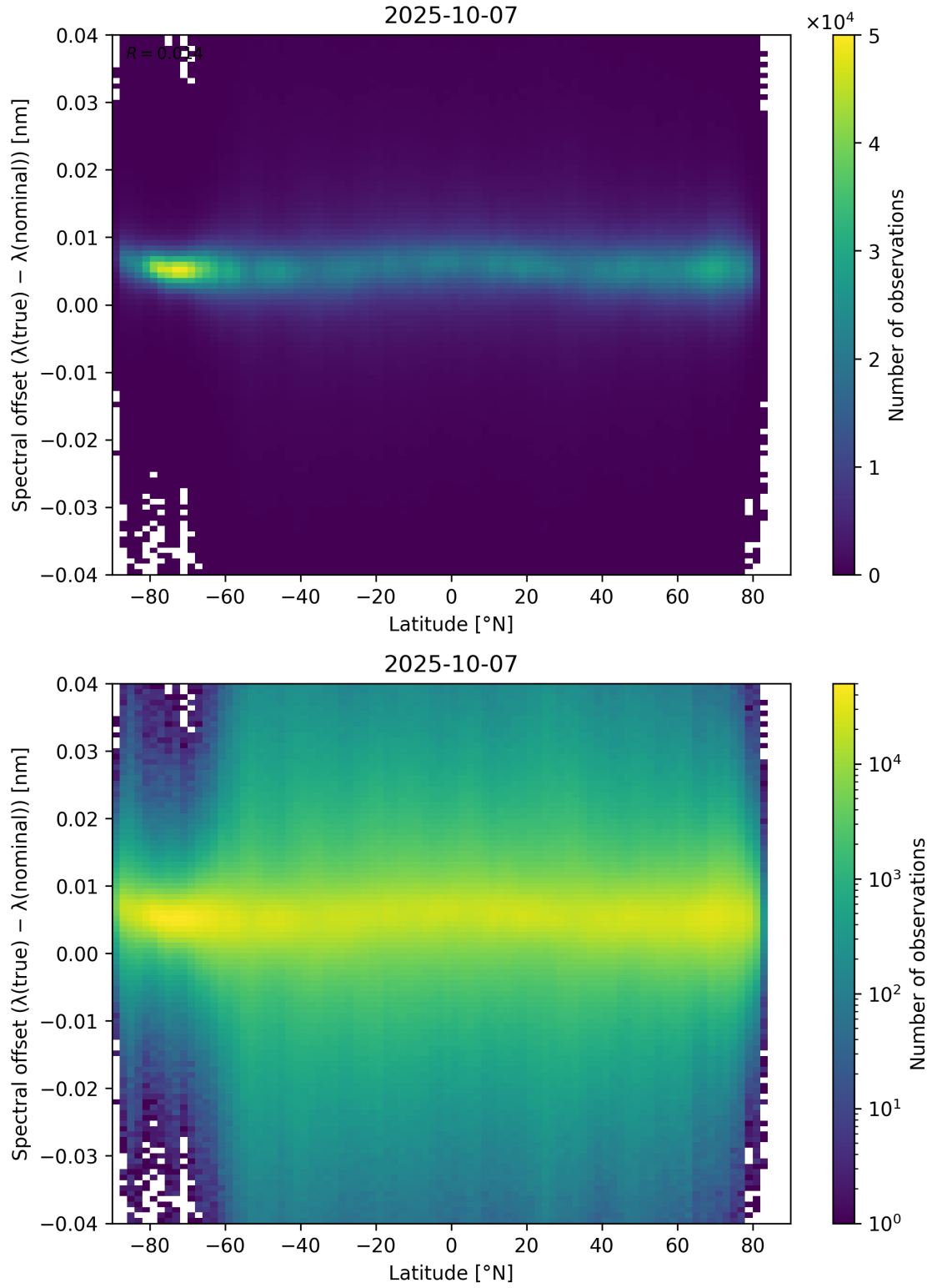
Figure 96: Scatter density plot of “Latitude” against “Spectral offset ( \lambda_{\text{true}} - \lambda_{\text{nominal}} )” for 2025-10-06 to 2025-10-08.
