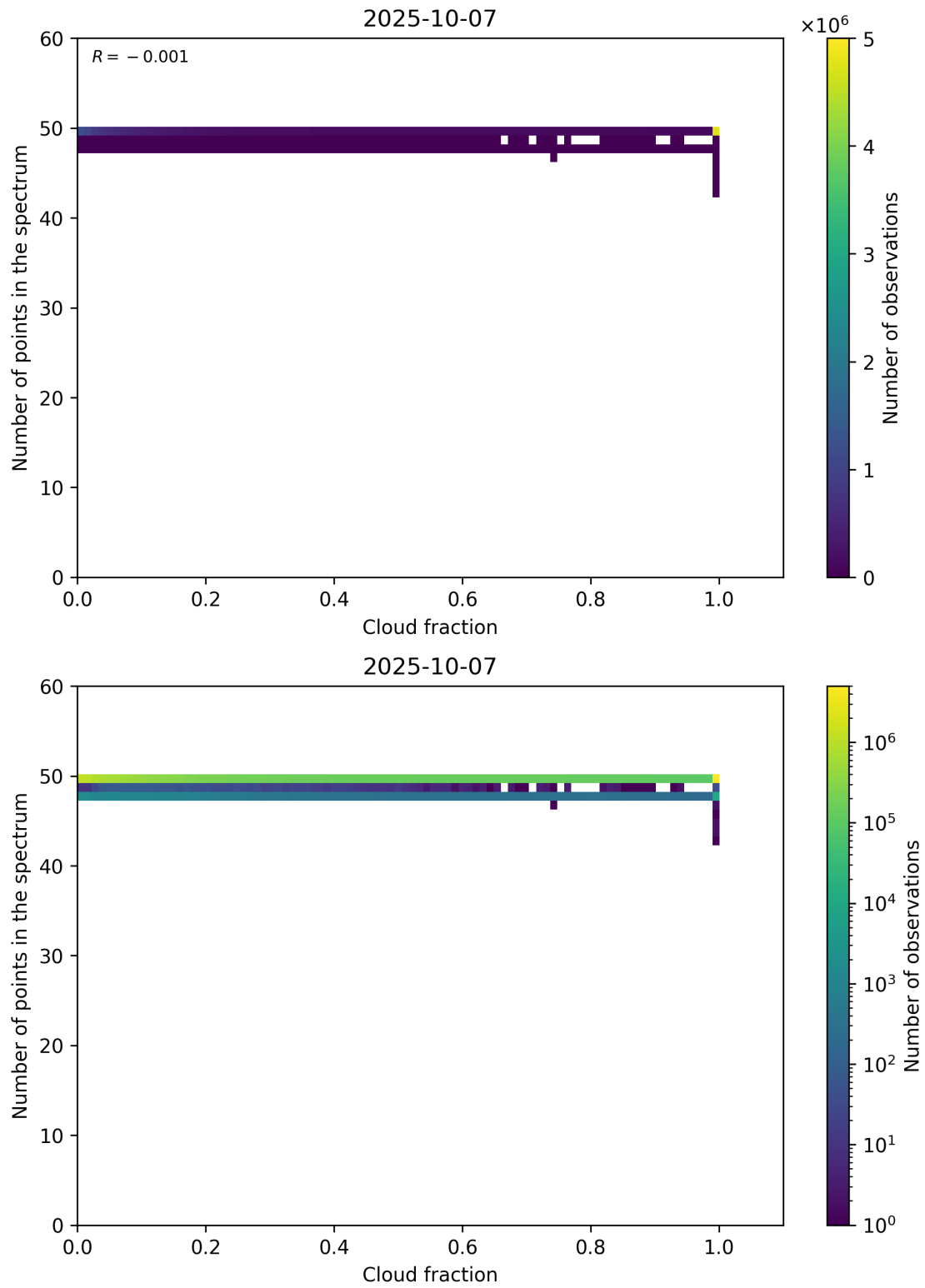
Figure 74: Scatter density plot of “Cloud fraction” against “Number of points in the spectrum” for 2025-10-06 to 2025-10-08.
