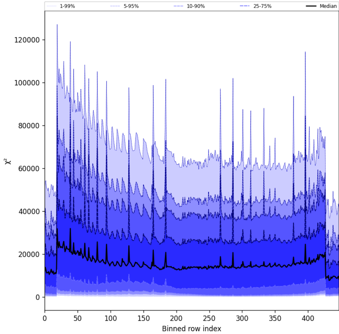
Figure 55: Along track statistics of “ \chi^2 ” for 2025-10-06 to 2025-10-08
