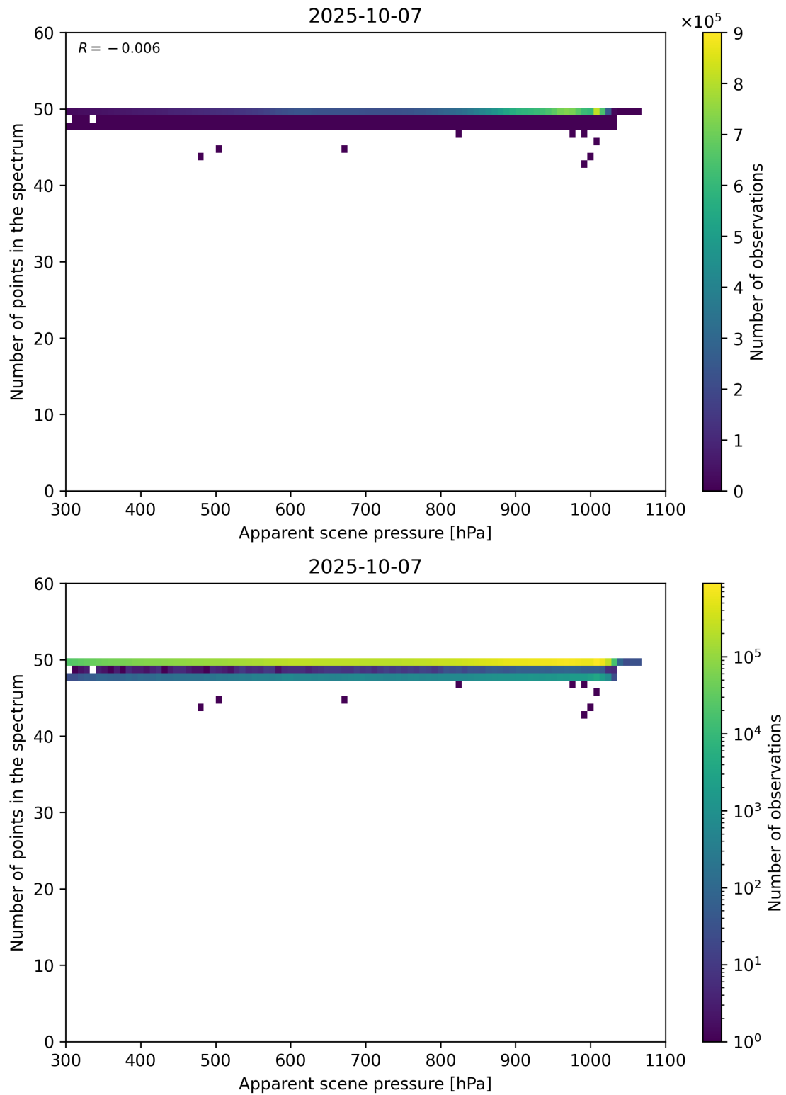
Figure 66: Scatter density plot of “Apparent scene pressure” against “Number of points in the spectrum” for 2025-10-06 to 2025-10-08.
