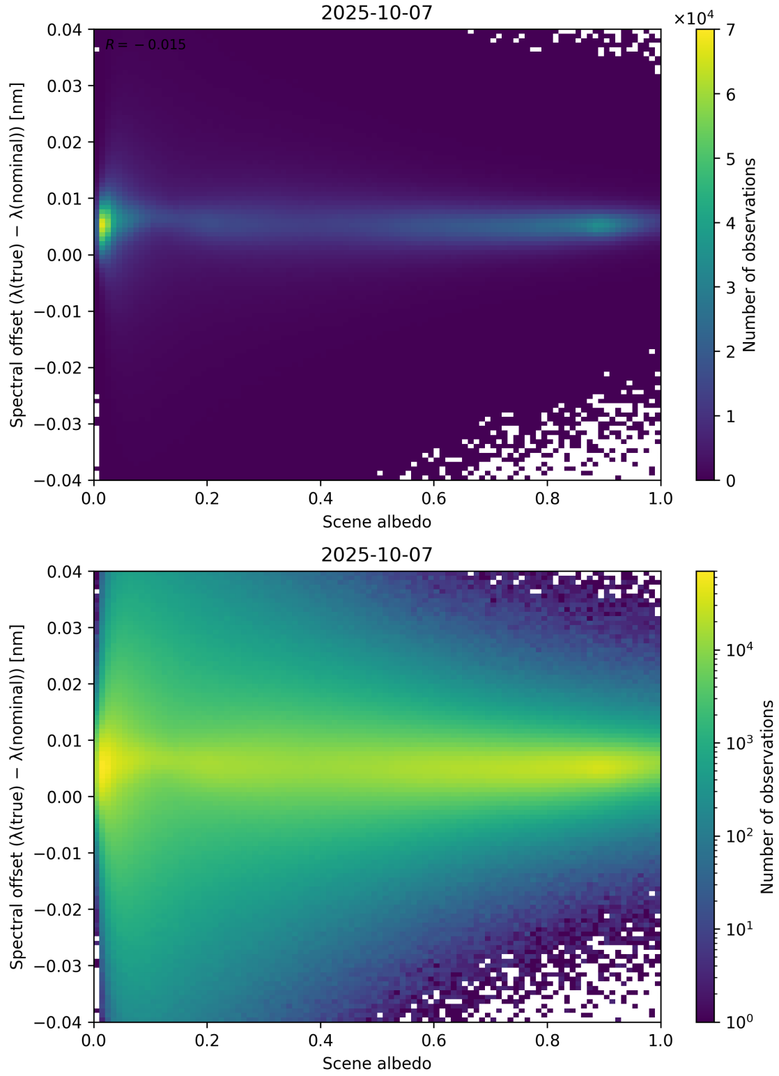
Figure 107: Scatter density plot of “Scene albedo” against “Spectral offset ( \lambda_{\text{true}} - \lambda_{\text{nominal}} )” for 2025-10-06 to 2025-10-08.
