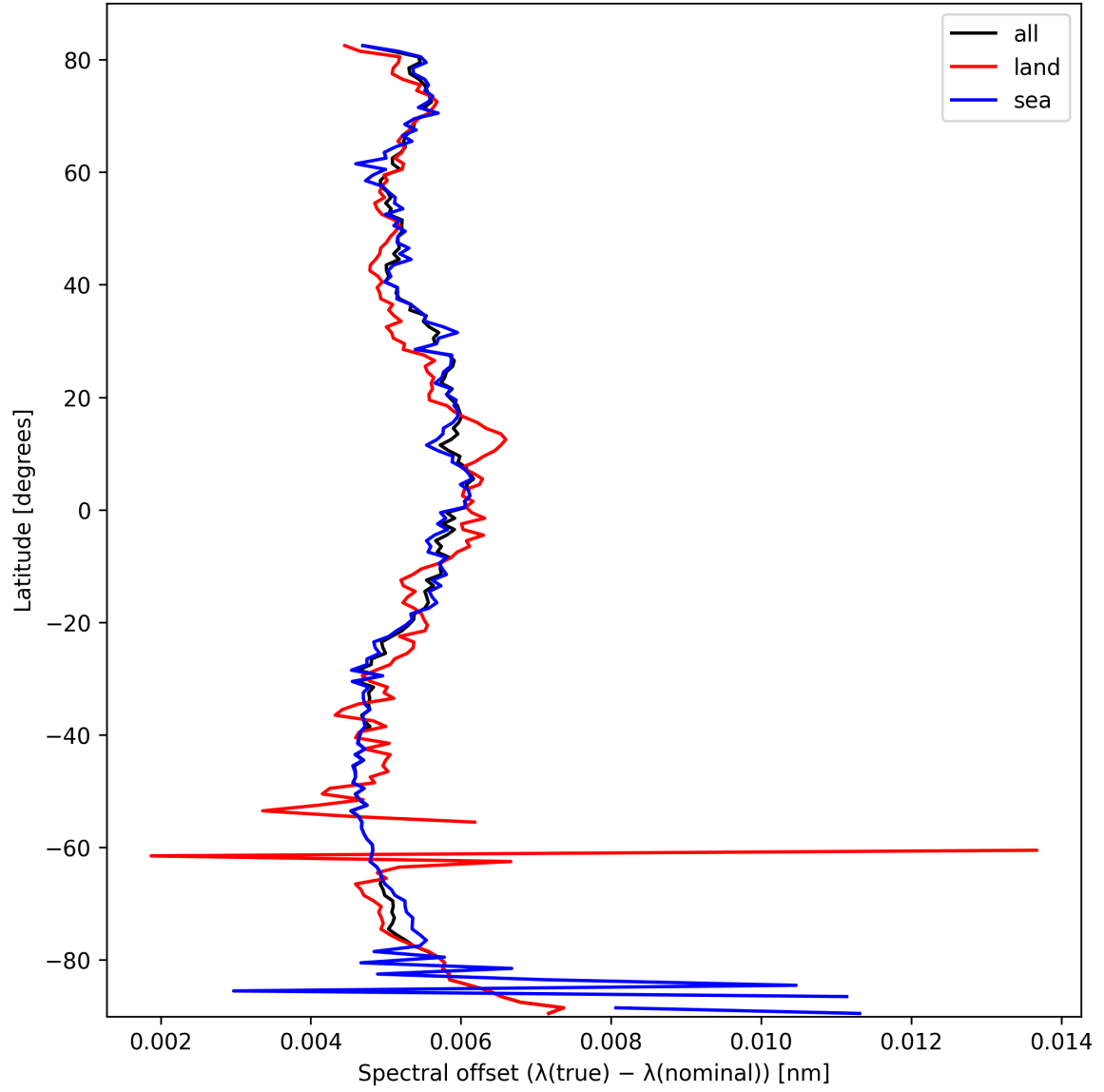
Figure 28: Zonal average of “Spectral offset ( \lambda_{\text{true}} - \lambda_{\text{nominal}} )” for 2025-10-06 to 2025-10-08.
