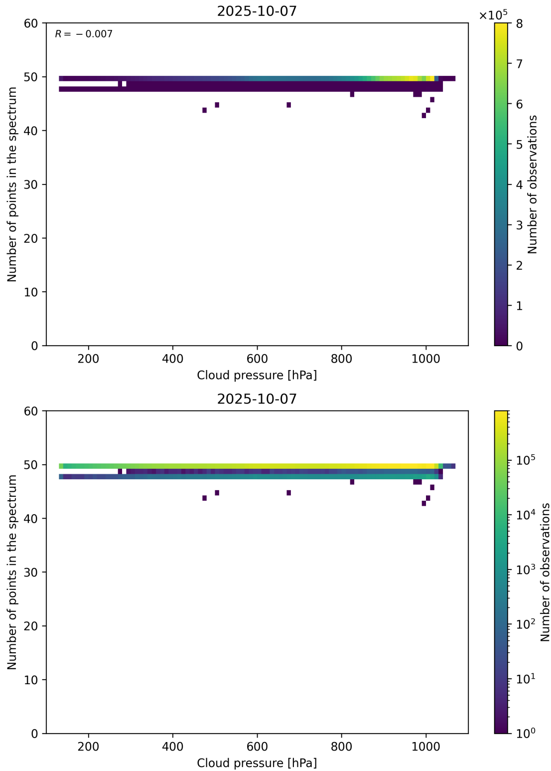
Figure 82: Scatter density plot of “Cloud pressure” against “Number of points in the spectrum” for 2025-10-06 to 2025-10-08.
