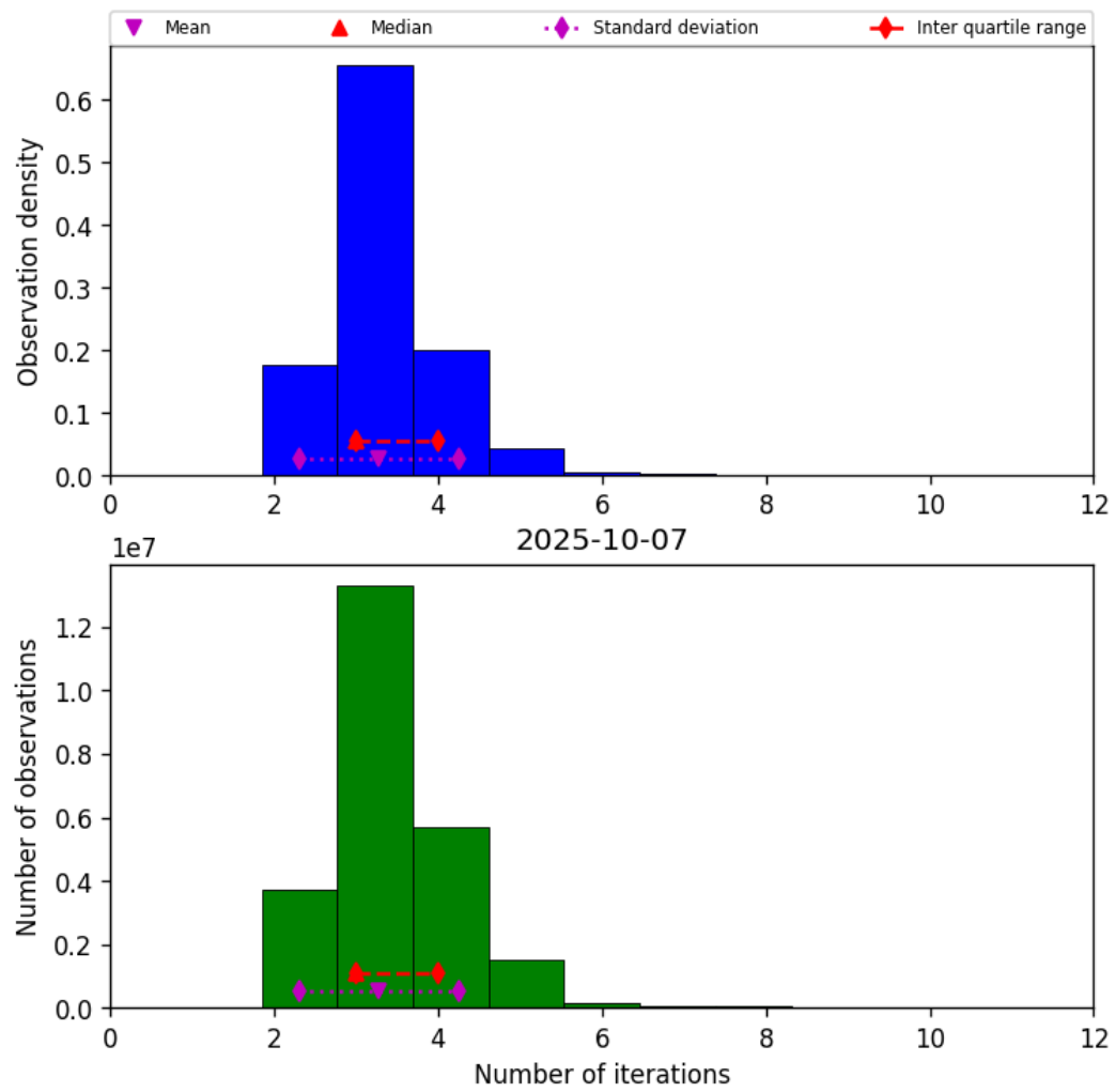
Figure 39: Histogram of “Number of iterations” for 2025-10-06 to 2025-10-08
