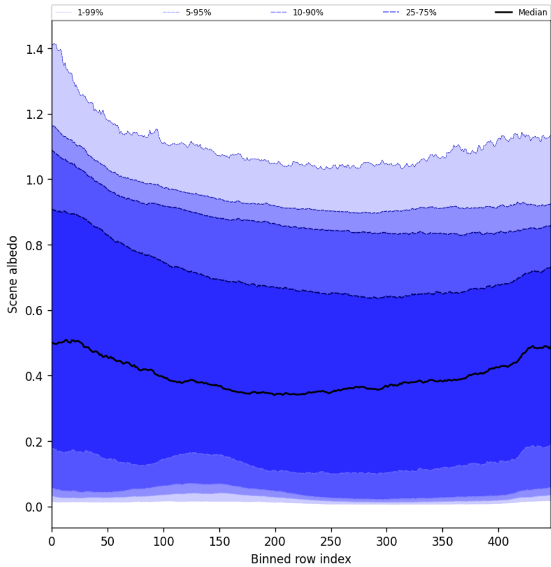
Figure 51: Along track statistics of “Scene albedo” for 2025-10-06 to 2025-10-08
