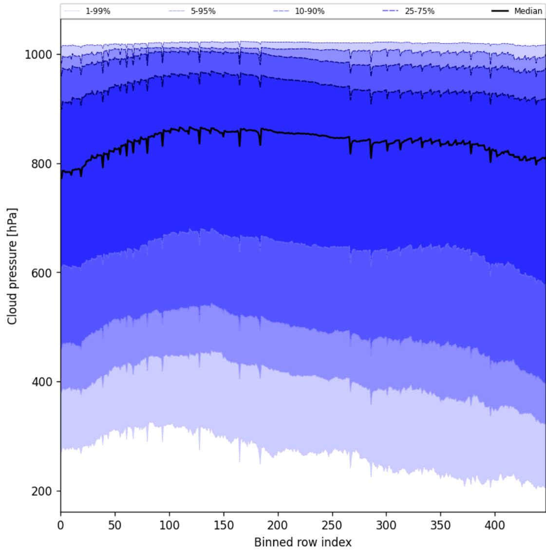
Figure 47: Along track statistics of “Cloud pressure” for 2025-10-06 to 2025-10-08
