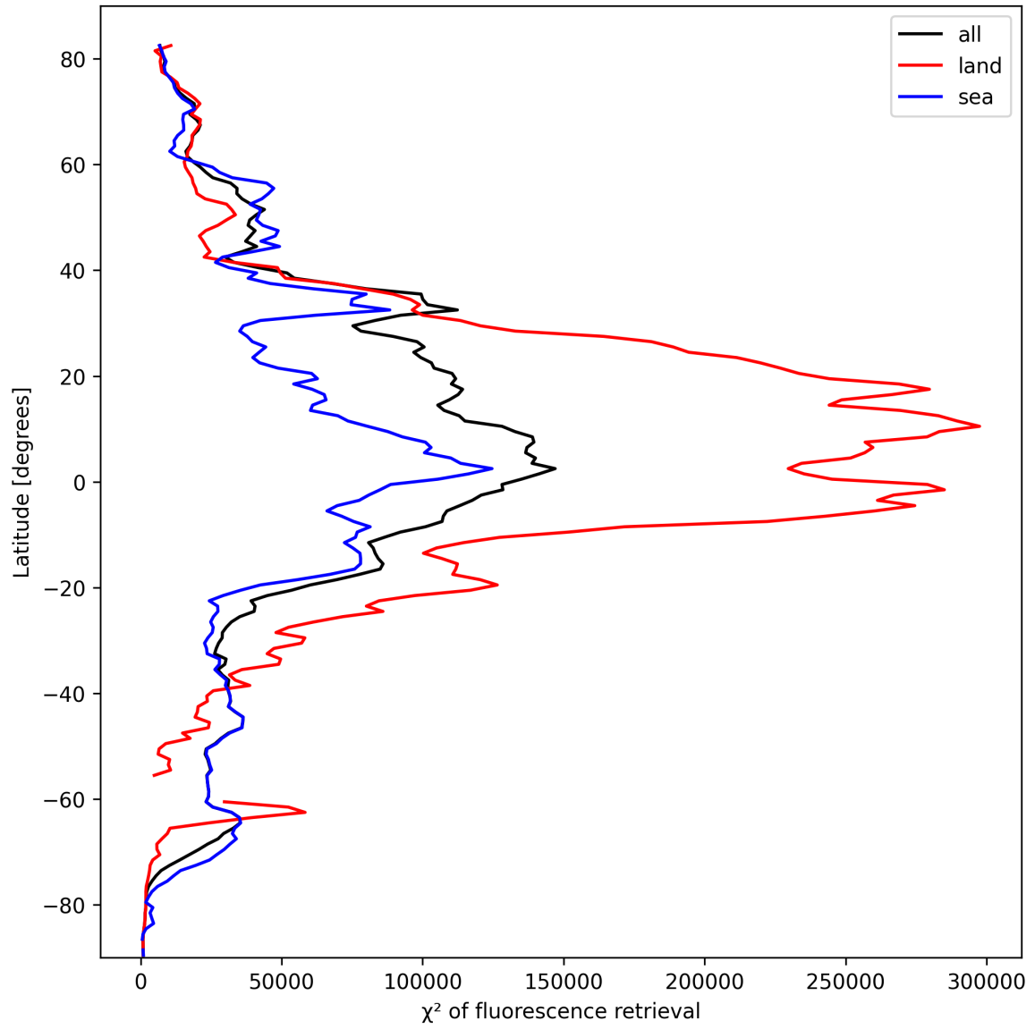
Figure 25: Zonal average of “ \chi^2 of fluorescence retrieval” for 2025-10-06 to 2025-10-08.
