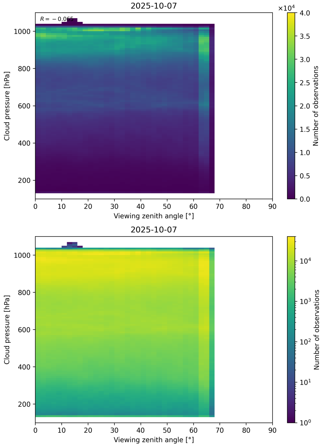
Figure 121: Scatter density plot of “Viewing zenith angle” against “Cloud pressure” for 2025-10-06 to 2025-10-08.
