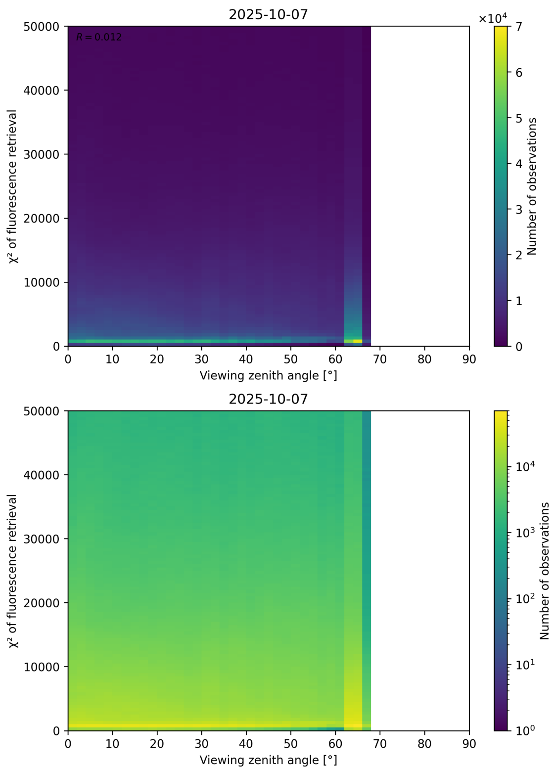
Figure 119: Scatter density plot of “Viewing zenith angle” against “ \chi^2 of fluorescence retrieval” for 2025-10-06 to 2025-10-08.
