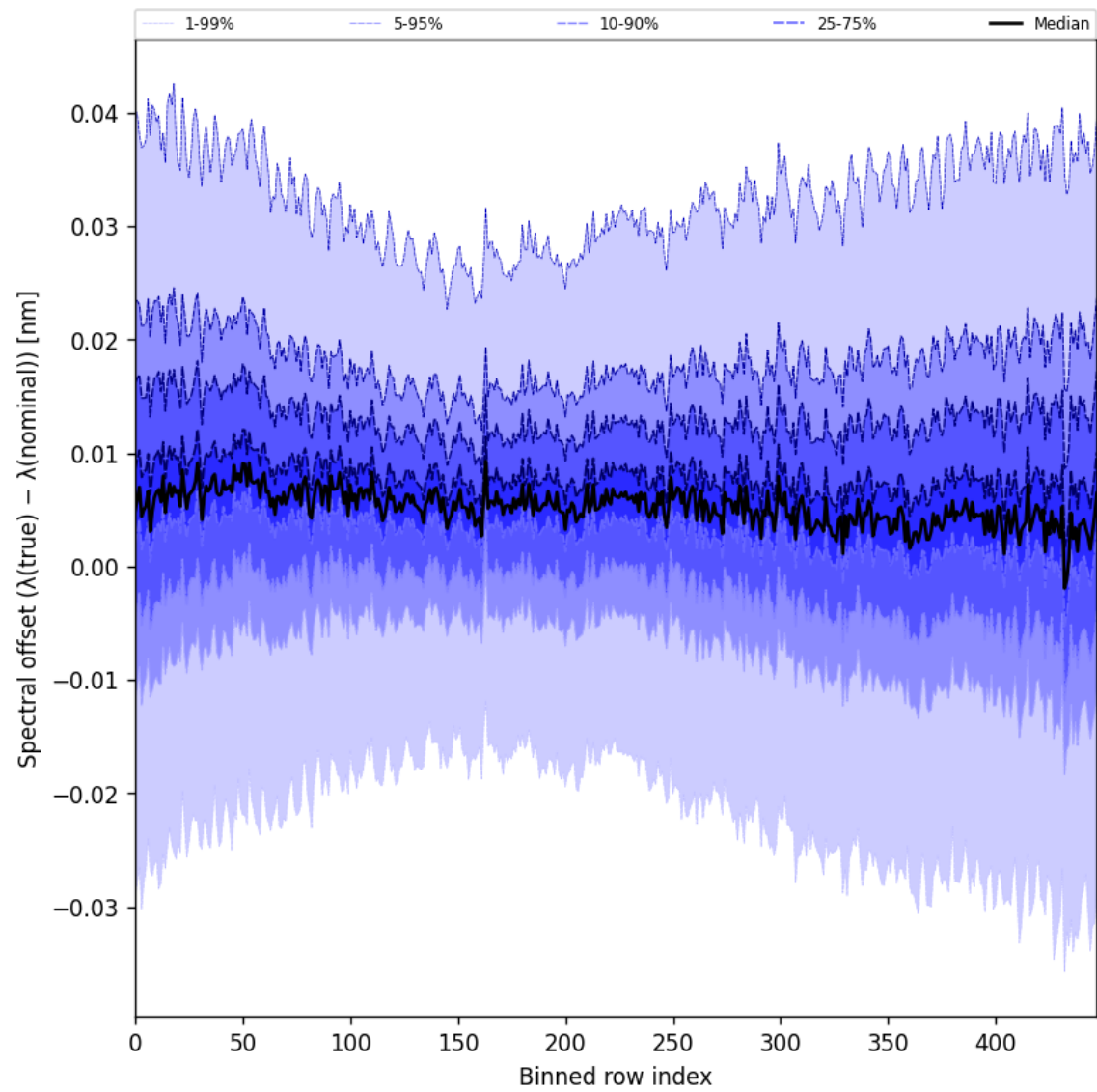
Figure 62: Along track statistics of “Spectral offset ( \lambda_{\text{true}} - \lambda_{\text{nominal}} )” for 2025-10-06 to 2025-10-08
