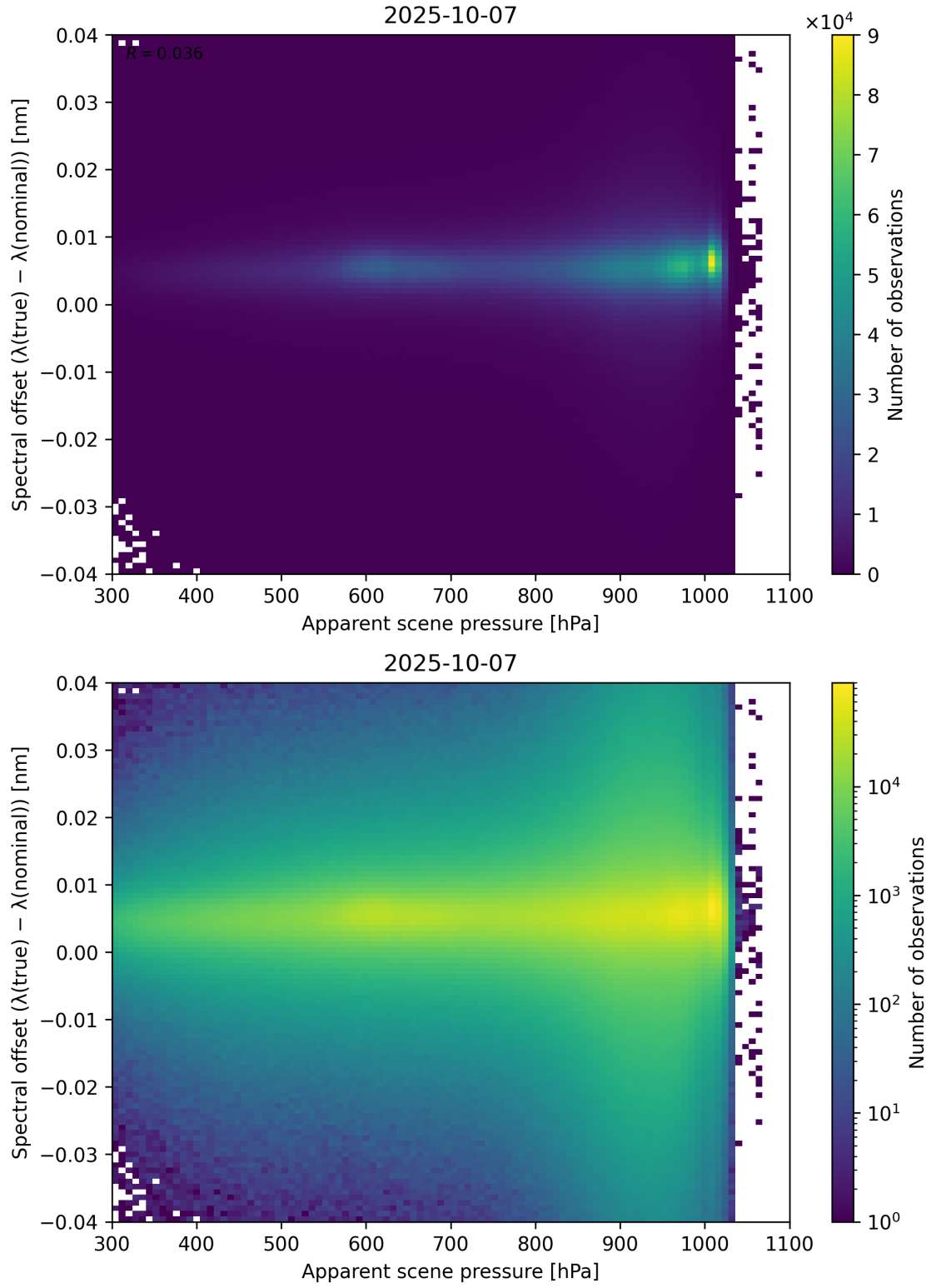
Figure 67: Scatter density plot of “Apparent scene pressure” against “Spectral offset ( \lambda_{\text{true}} - \lambda_{\text{nominal}} )” for 2025-10-06 to 2025-10-08.
