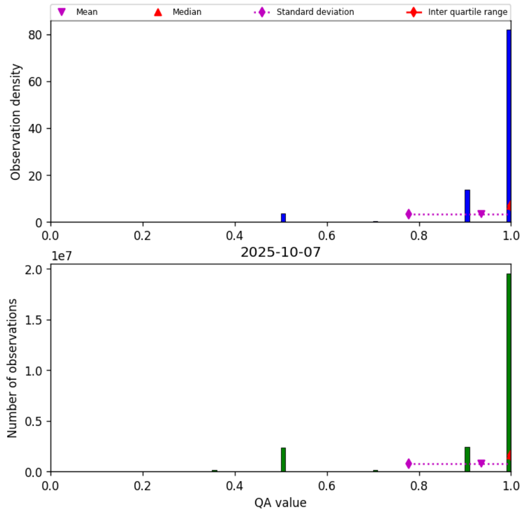
Figure 29: Histogram of “QA value” for 2025-10-06 to 2025-10-08
