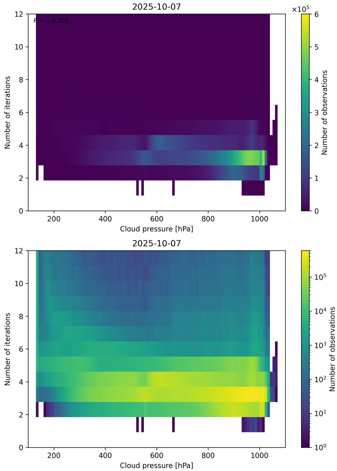
Figure 81: Scatter density plot of “Cloud pressure” against “Number of iterations” for 2025-10-06 to 2025-10-08.
