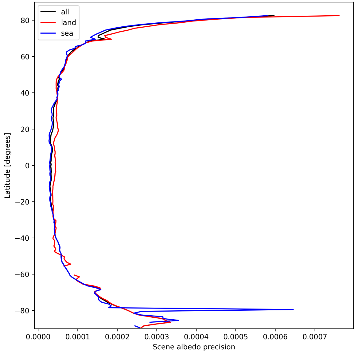
Figure 18: Zonal average of “Scene albedo precision” for 2025-10-06 to 2025-10-08.
