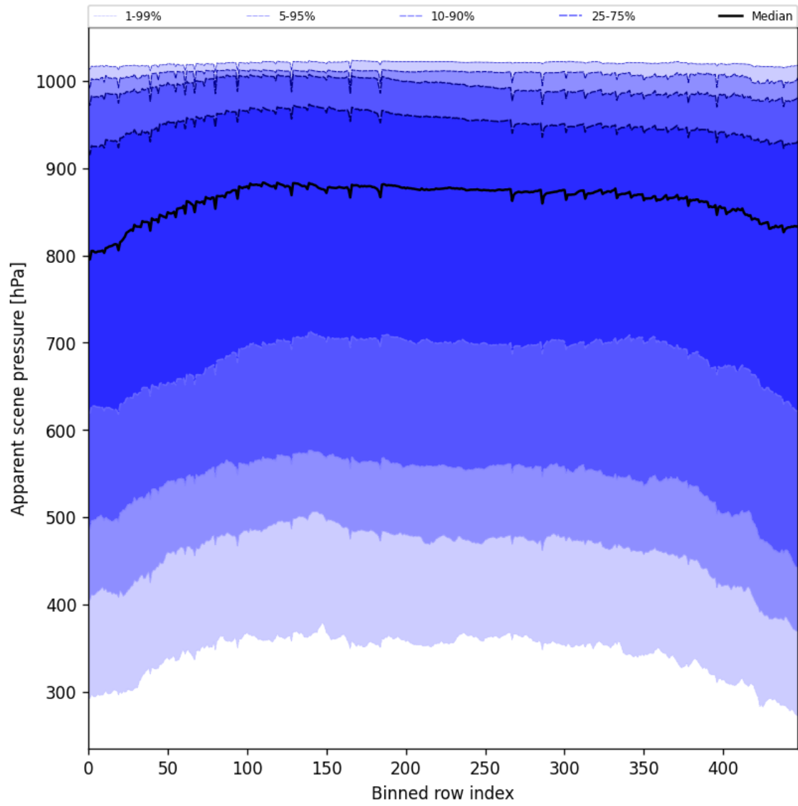
Figure 53: Along track statistics of “Apparent scene pressure” for 2025-10-06 to 2025-10-08
