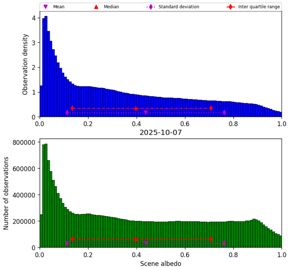
Figure 34: Histogram of “Scene albedo” for 2025-10-06 to 2025-10-08
