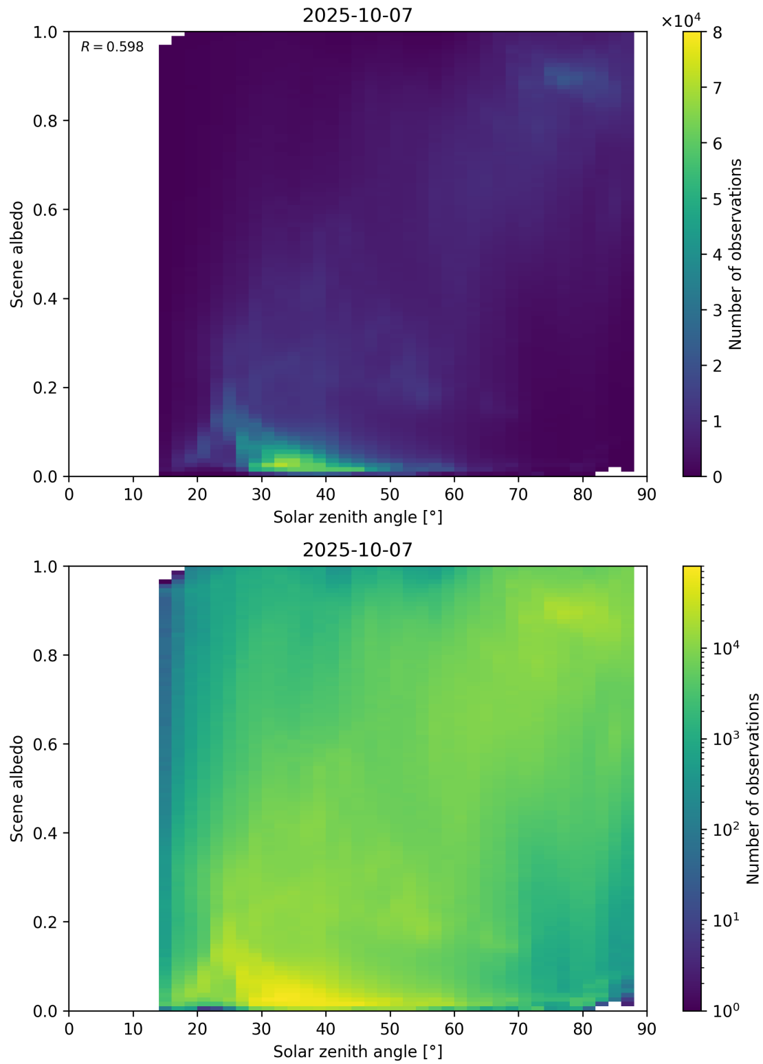
Figure 116: Scatter density plot of “Solar zenith angle” against “Scene albedo” for 2025-10-06 to 2025-10-08.
