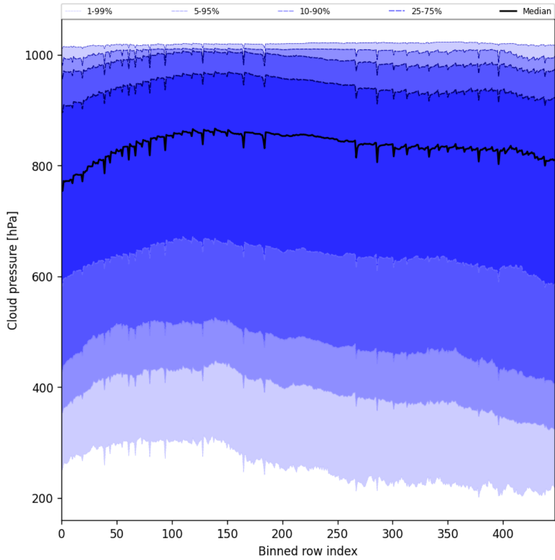
Figure 47: Along track statistics of “Cloud pressure” for 2025-10-07 to 2025-10-09
