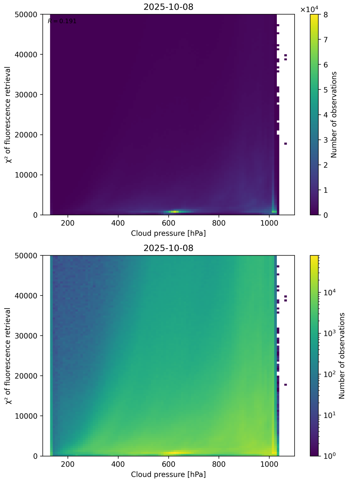
Figure 78: Scatter density plot of “Cloud pressure” against “ \chi^2 of fluorescence retrieval” for 2025-10-07 to 2025-10-09.
