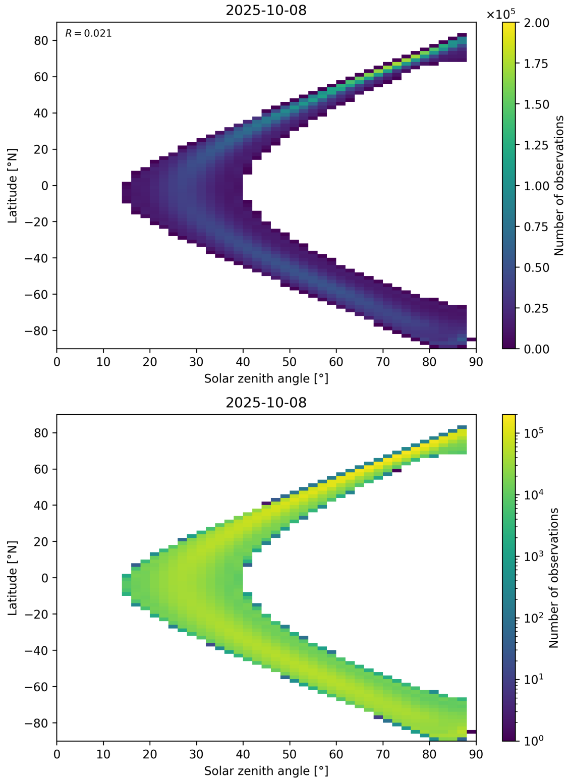
Figure 113: Scatter density plot of “Solar zenith angle” against “Latitude” for 2025-10-07 to 2025-10-09.
