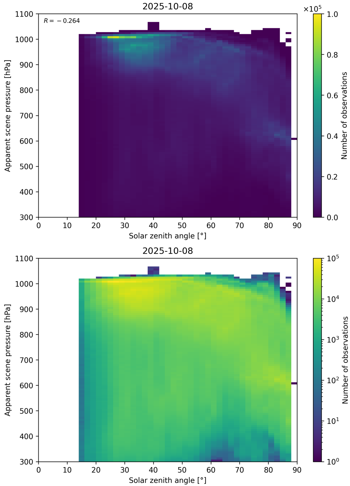
Figure 108: Scatter density plot of “Solar zenith angle” against “Apparent scene pressure” for 2025-10-07 to 2025-10-09.
