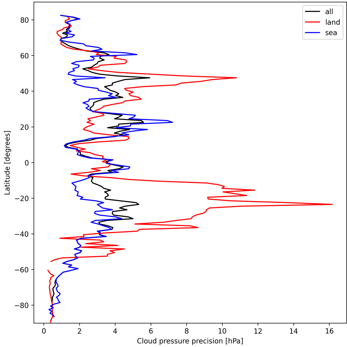
Figure 14: Zonal average of "Cloud pressure precision" for 2025-10-07 to 2025-10-09.
