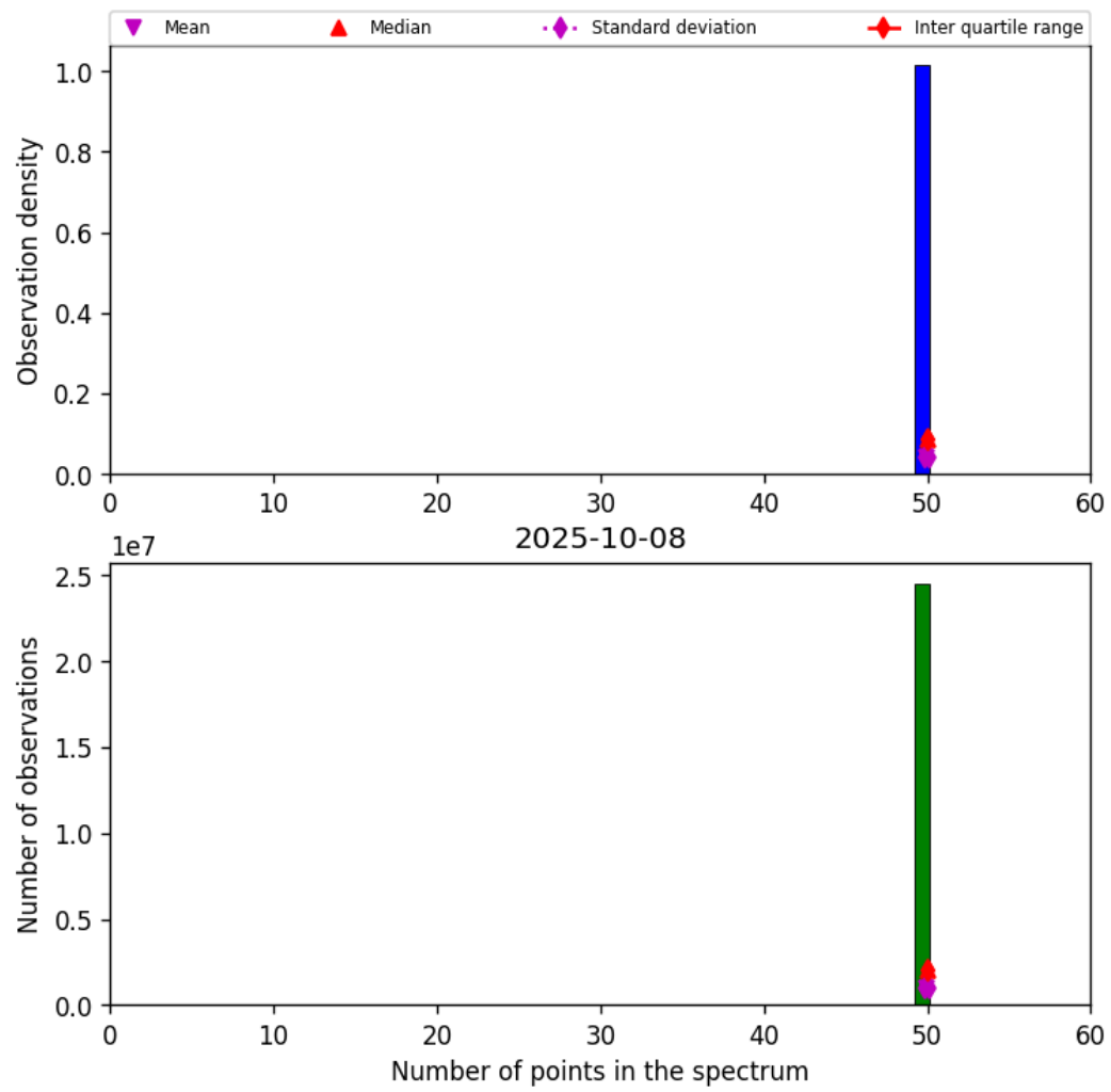
Figure 44: Histogram of "Number of points in the spectrum" for 2025-10-07 to 2025-10-09
