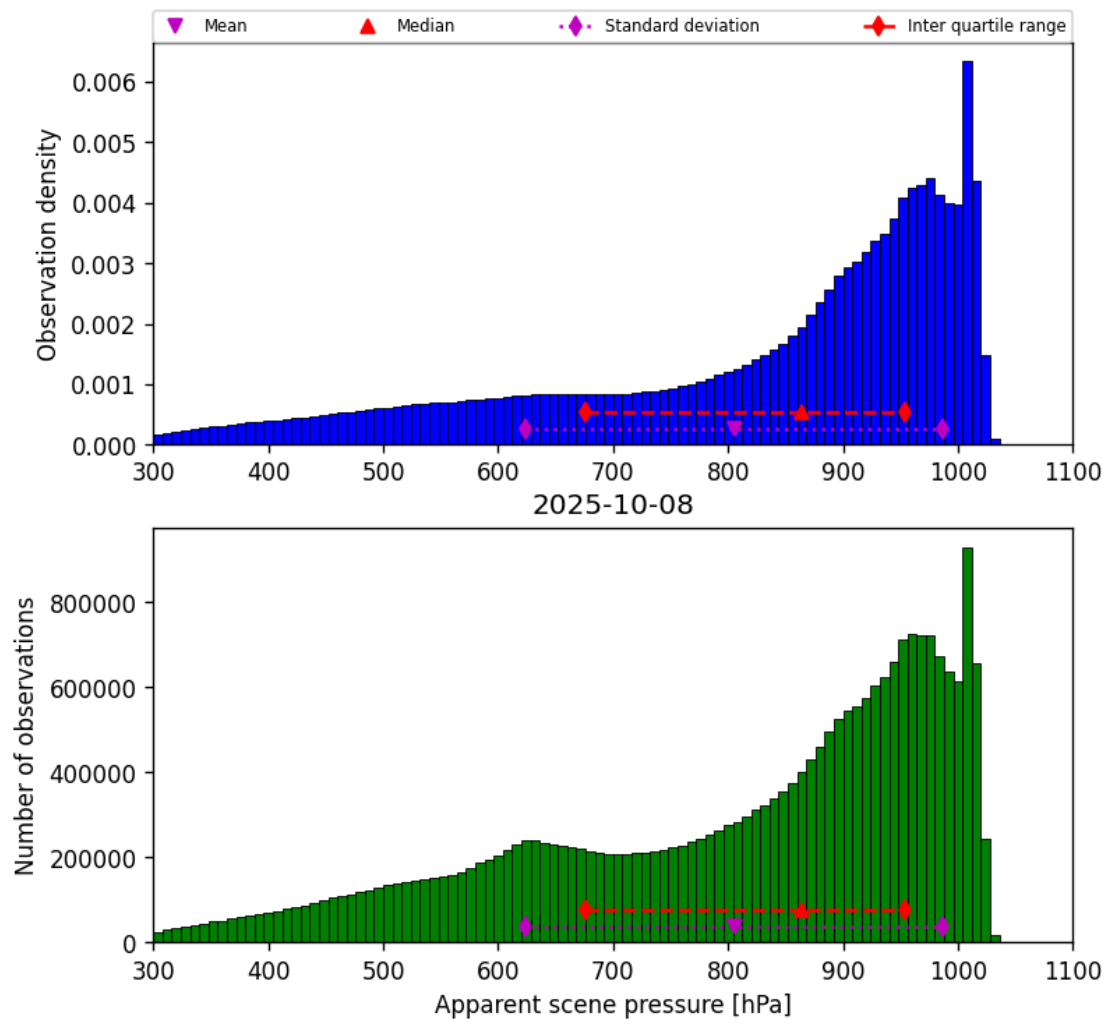
Figure 36: Histogram of “Apparent scene pressure” for 2025-10-07 to 2025-10-09
