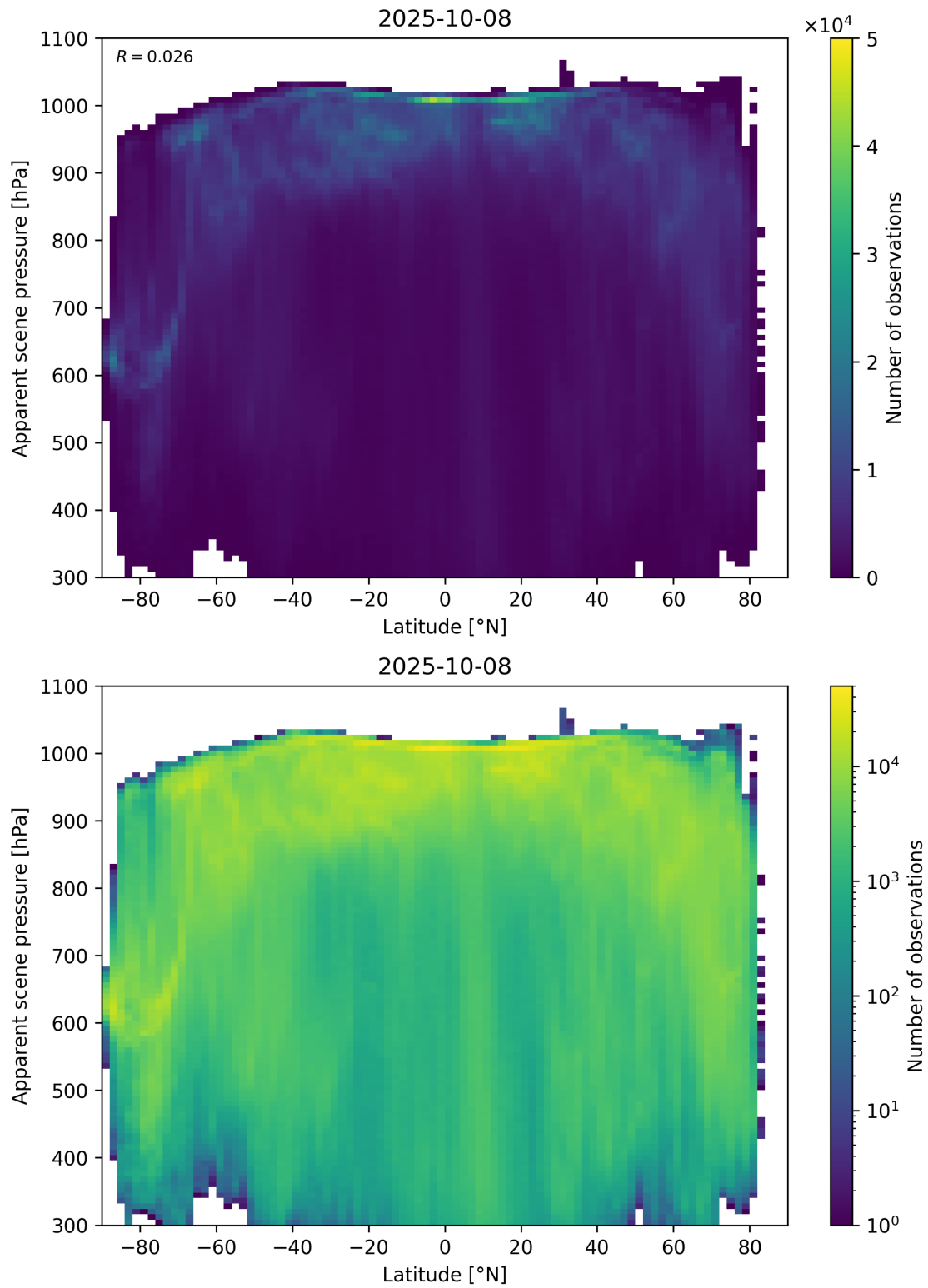
Figure 88: Scatter density plot of “Latitude” against “Apparent scene pressure” for 2025-10-07 to 2025-10-09.
