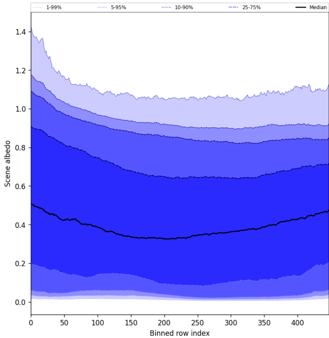
Figure 51: Along track statistics of “Scene albedo” for 2025-10-07 to 2025-10-09
