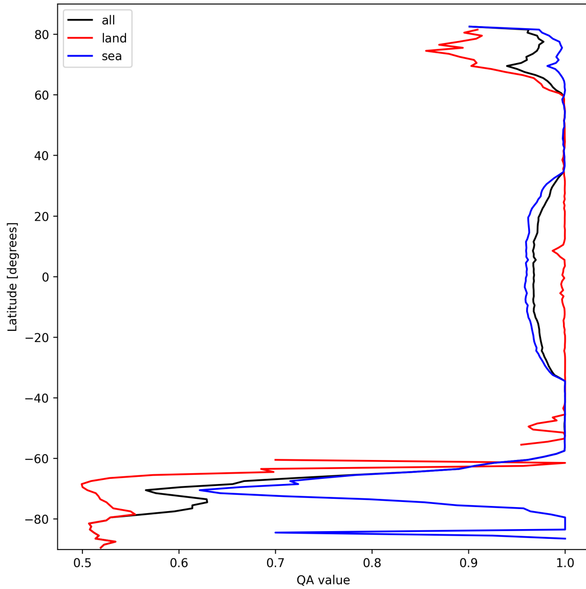
Figure 12: Zonal average of “QA value” for 2025-10-07 to 2025-10-09.
