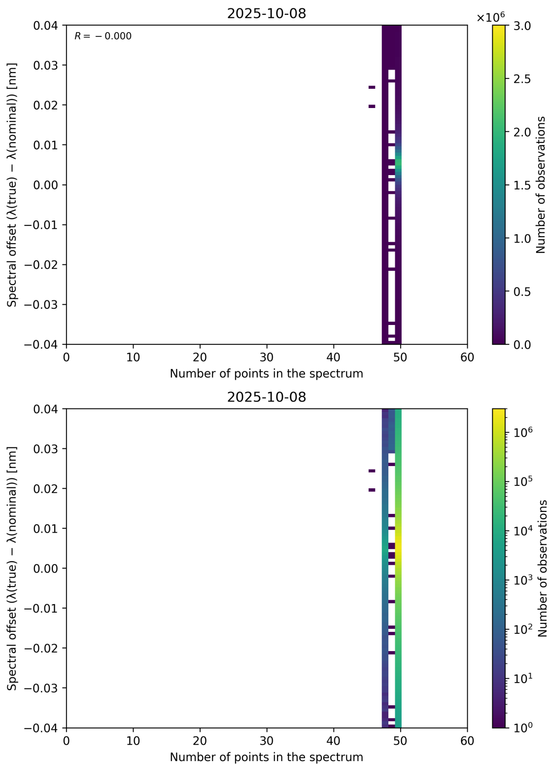
Figure 101: Scatter density plot of “Number of points in the spectrum” against “Spectral offset ( \lambda_{\text{true}} - \lambda_{\text{nominal}} )” for 2025-10-07 to 2025-10-09.
