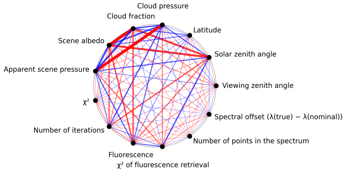
Figure 1: Map of correlation graph for 2025-10-07 to 2025-10-09.
