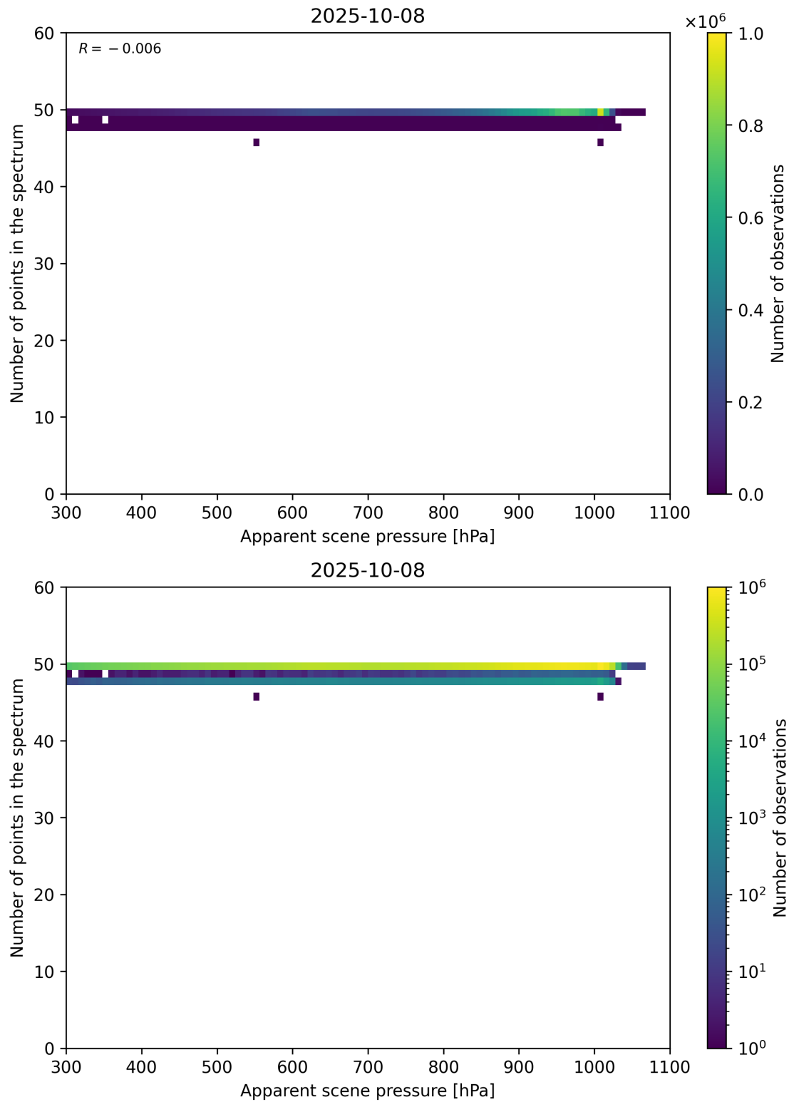
Figure 66: Scatter density plot of “Apparent scene pressure” against “Number of points in the spectrum” for 2025-10-07 to 2025-10-09.
