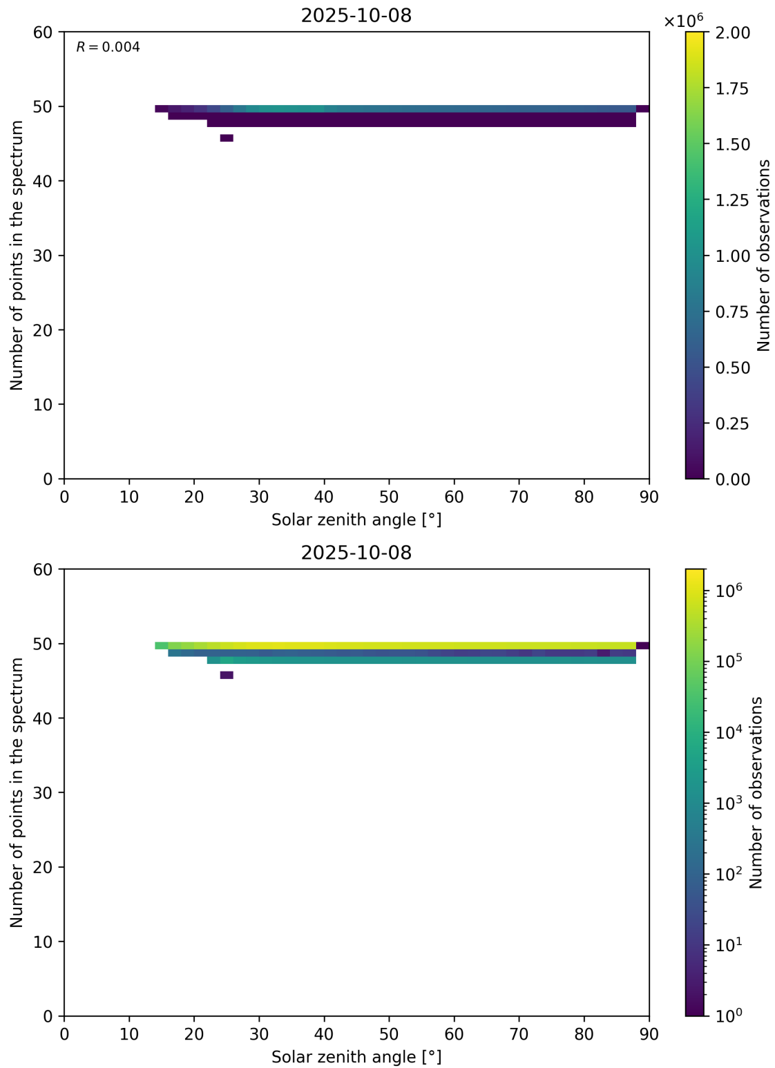
Figure 115: Scatter density plot of “Solar zenith angle” against “Number of points in the spectrum” for 2025-10-07 to 2025-10-09.
