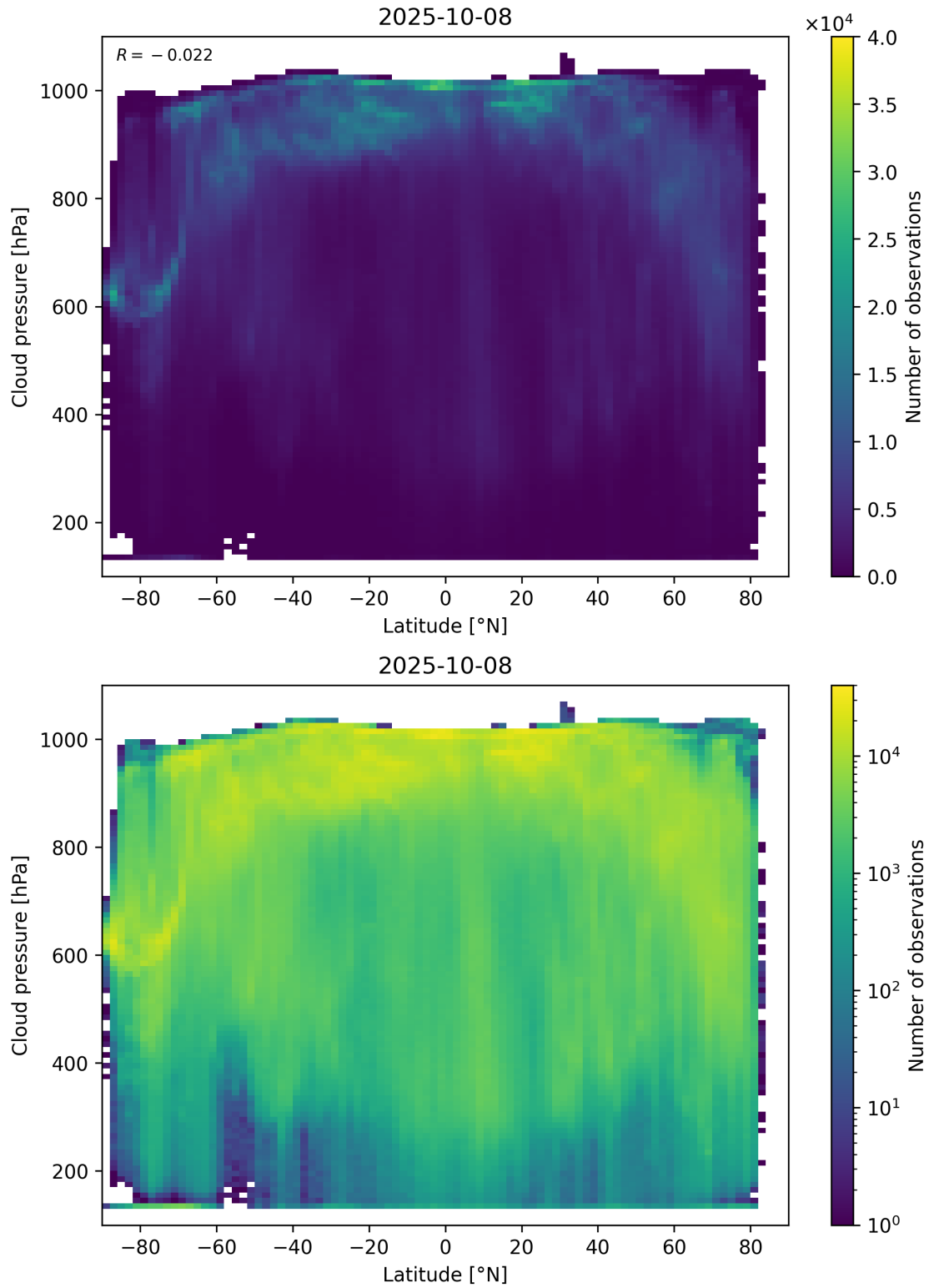
Figure 91: Scatter density plot of “Latitude” against “Cloud pressure” for 2025-10-07 to 2025-10-09.
