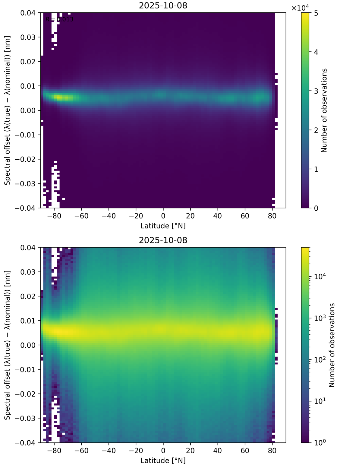
Figure 96: Scatter density plot of “Latitude” against “Spectral offset ( \lambda_{\text{true}} - \lambda_{\text{nominal}} )” for 2025-10-07 to 2025-10-09.
