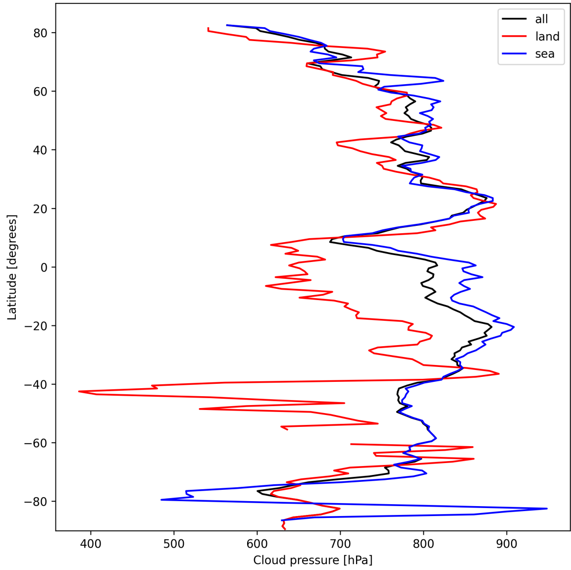
Figure 13: Zonal average of “Cloud pressure” for 2025-10-07 to 2025-10-09.
