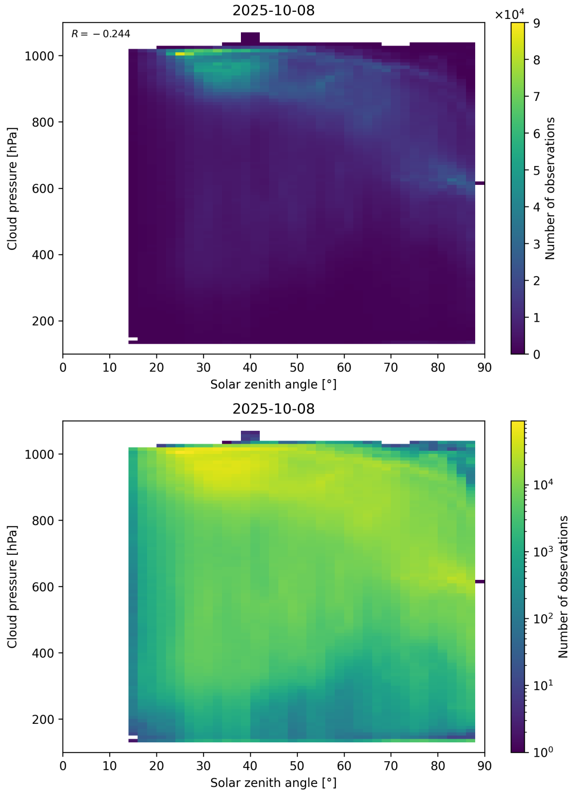
Figure 111: Scatter density plot of “Solar zenith angle” against “Cloud pressure” for 2025-10-07 to 2025-10-09.
