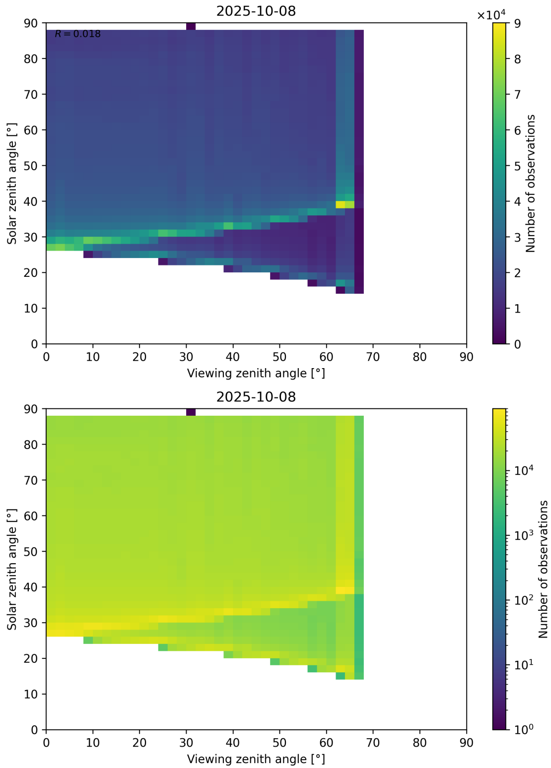
Figure 127: Scatter density plot of “Viewing zenith angle” against “Solar zenith angle” for 2025-10-07 to 2025-10-09.
