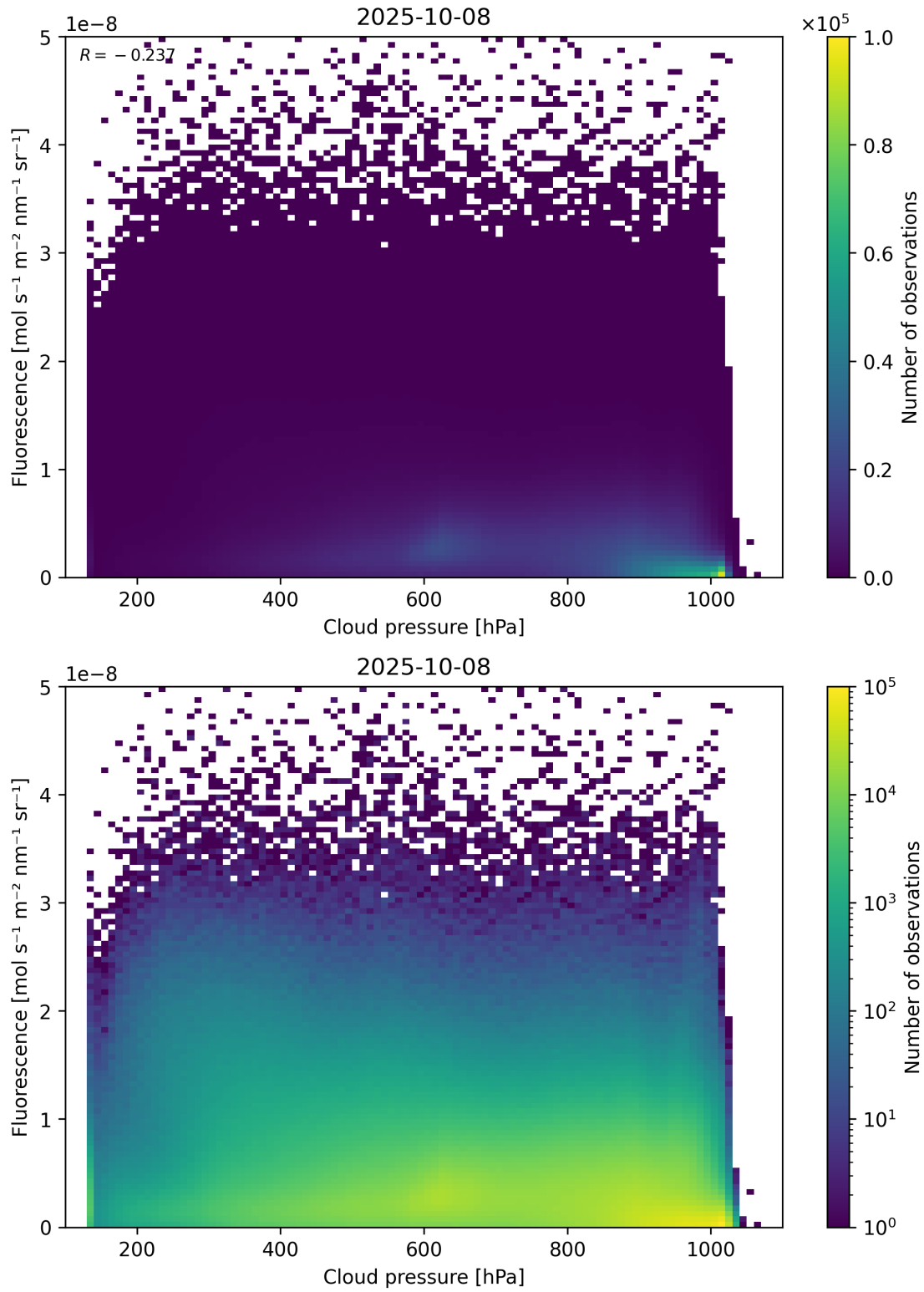
Figure 80: Scatter density plot of “Cloud pressure” against “Fluorescence” for 2025-10-07 to 2025-10-09.
