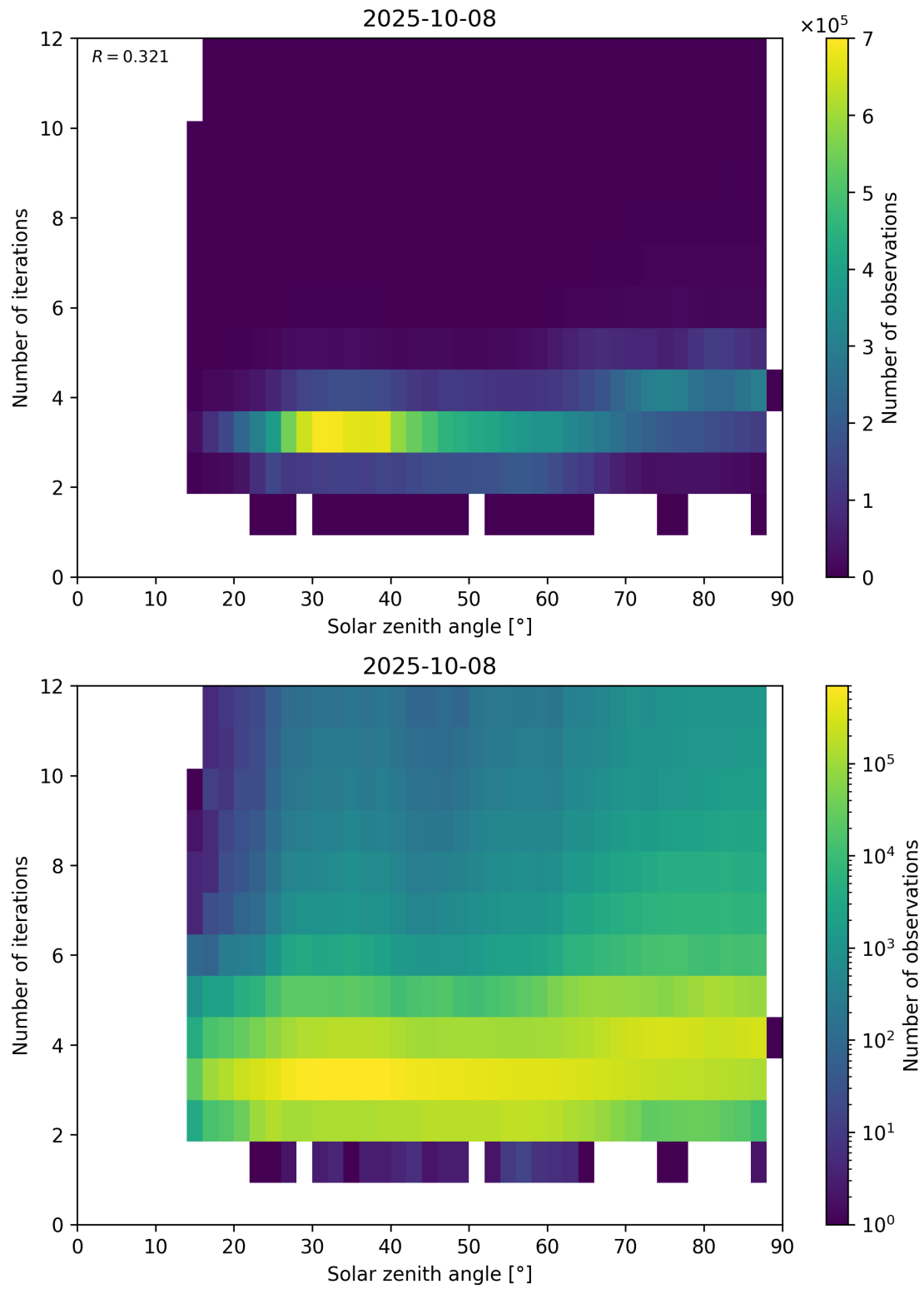
Figure 114: Scatter density plot of “Solar zenith angle” against “Number of iterations” for 2025-10-07 to 2025-10-09.
