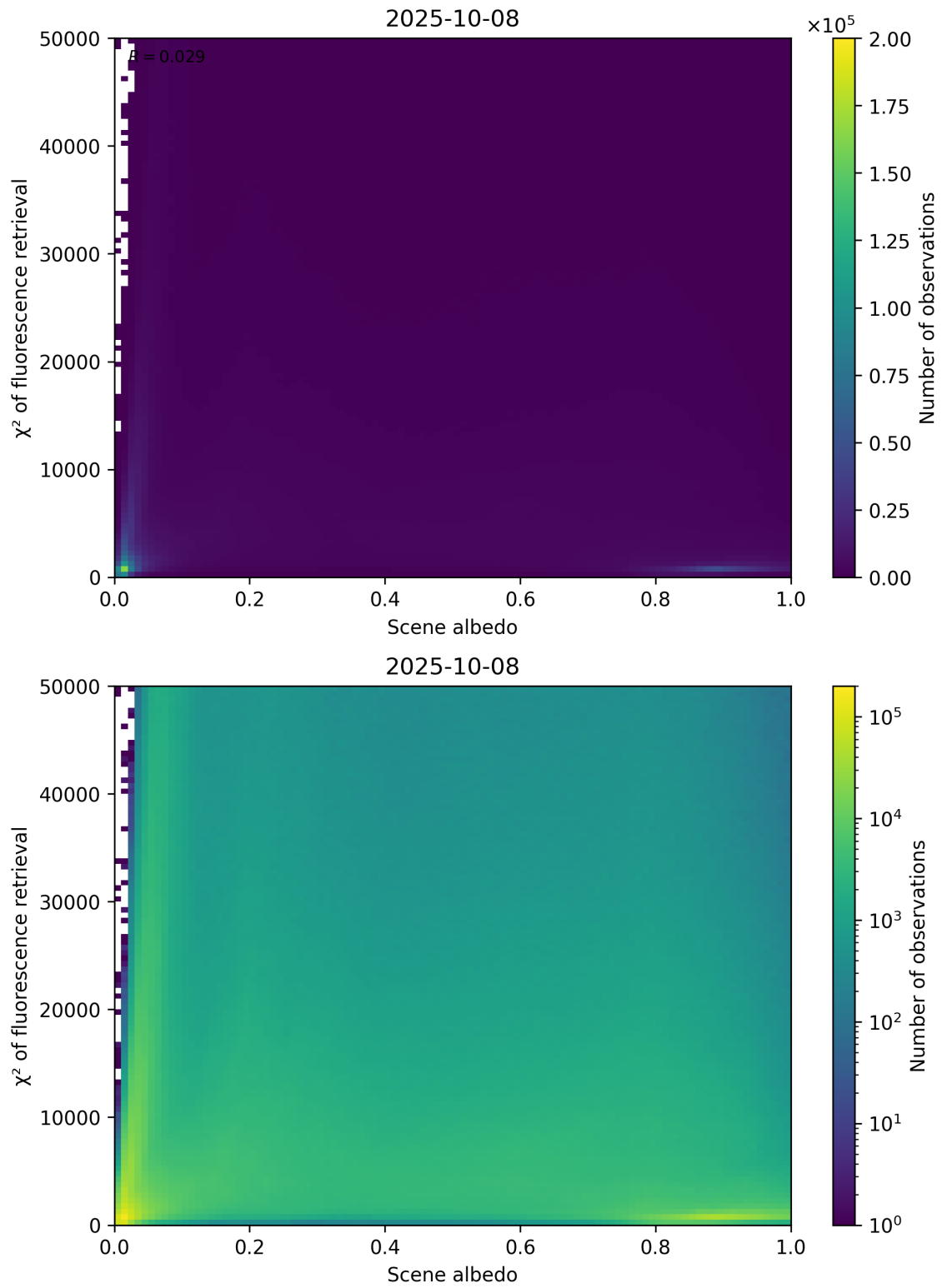
Figure 103: Scatter density plot of “Scene albedo” against “ \chi^2 of fluorescence retrieval” for 2025-10-07 to 2025-10-09.
