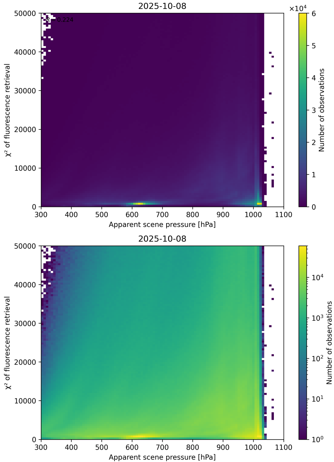
Figure 63: Scatter density plot of “Apparent scene pressure” against “ \chi^2 of fluorescence retrieval” for 2025-10-07 to 2025-10-09.
