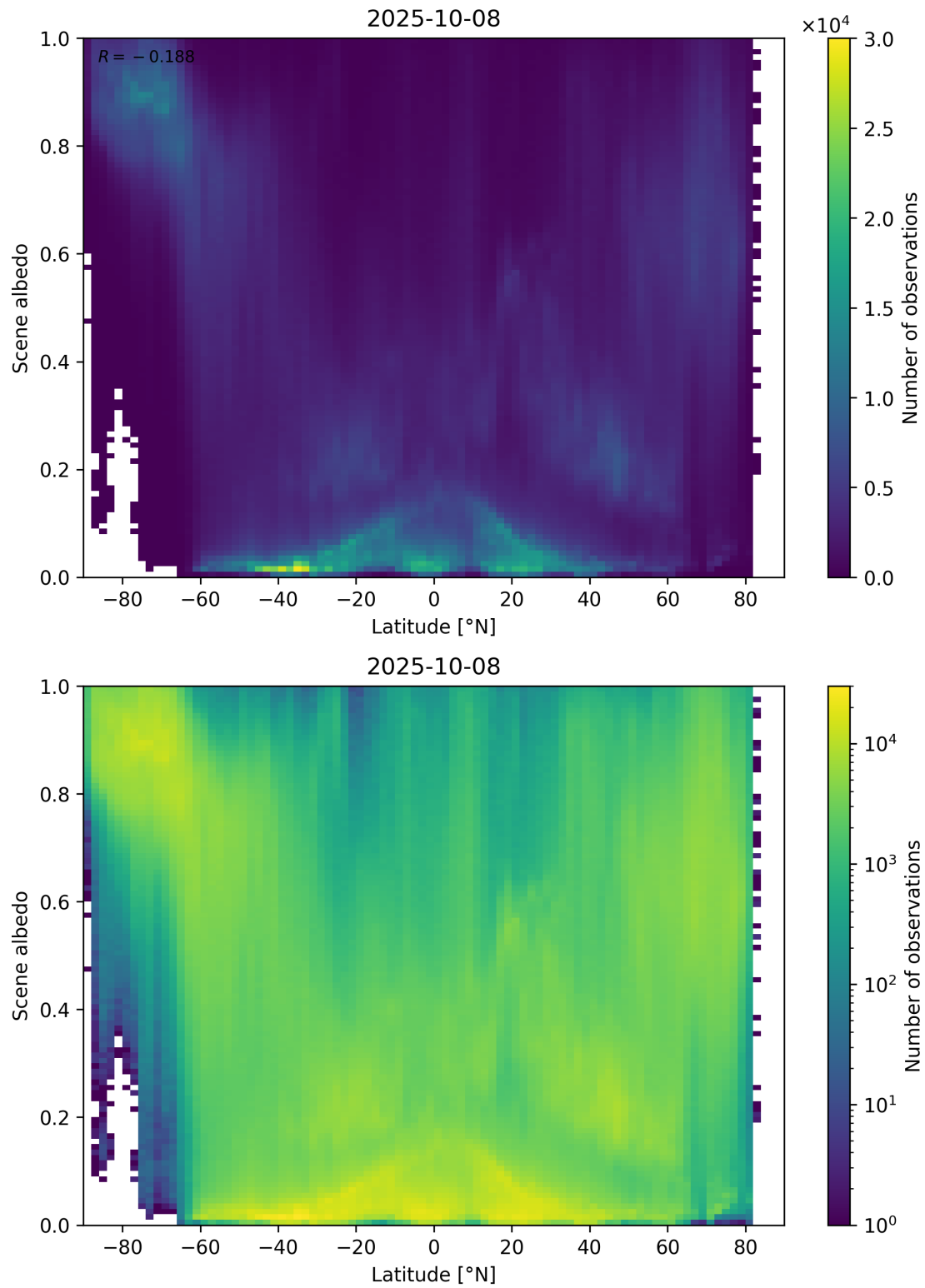
Figure 95: Scatter density plot of “Latitude” against “Scene albedo” for 2025-10-07 to 2025-10-09.
