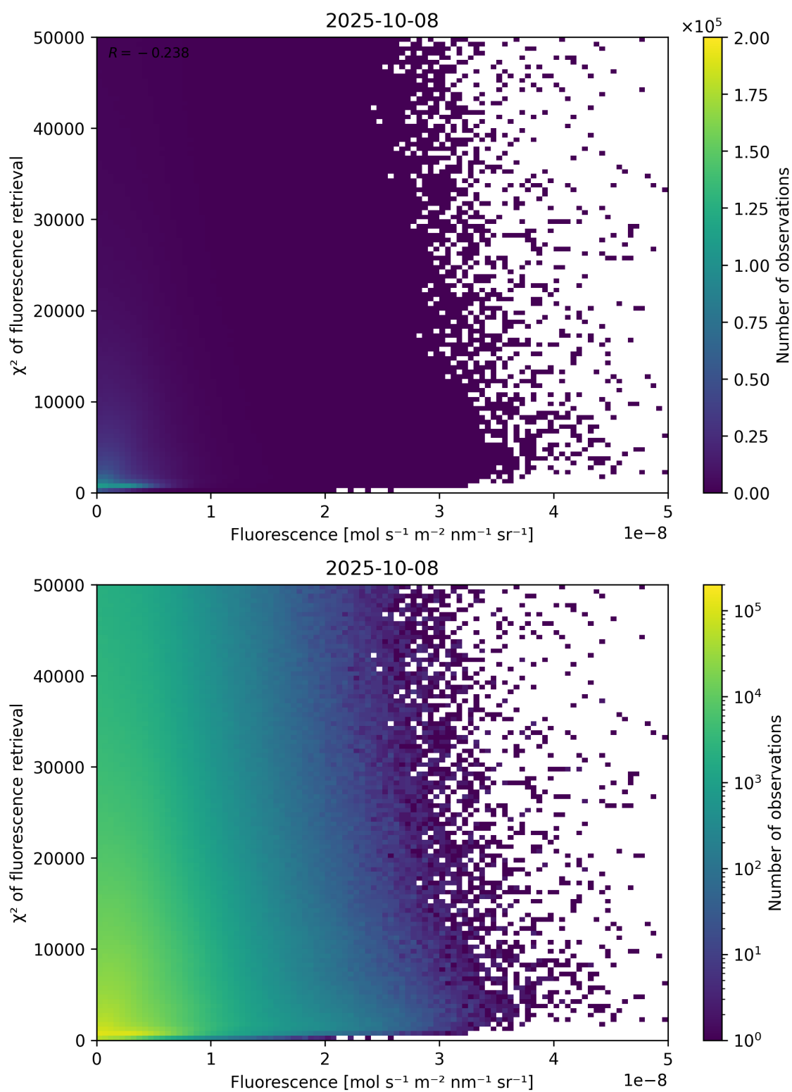
Figure 85: Scatter density plot of “Fluorescence” against “ \chi^2 of fluorescence retrieval” for 2025-10-07 to 2025-10-09.
