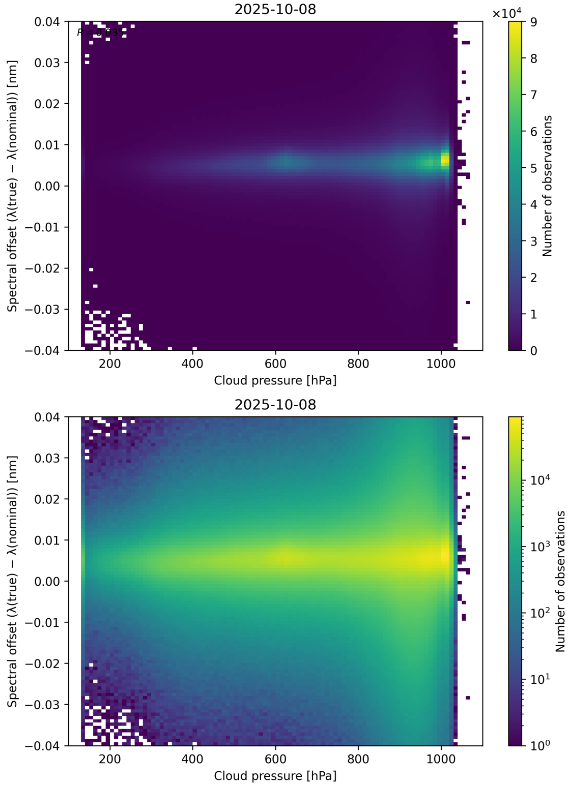
Figure 84: Scatter density plot of “Cloud pressure” against “Spectral offset ( \lambda_{\text{true}} - \lambda_{\text{nominal}} )” for 2025-10-07 to 2025-10-09.
