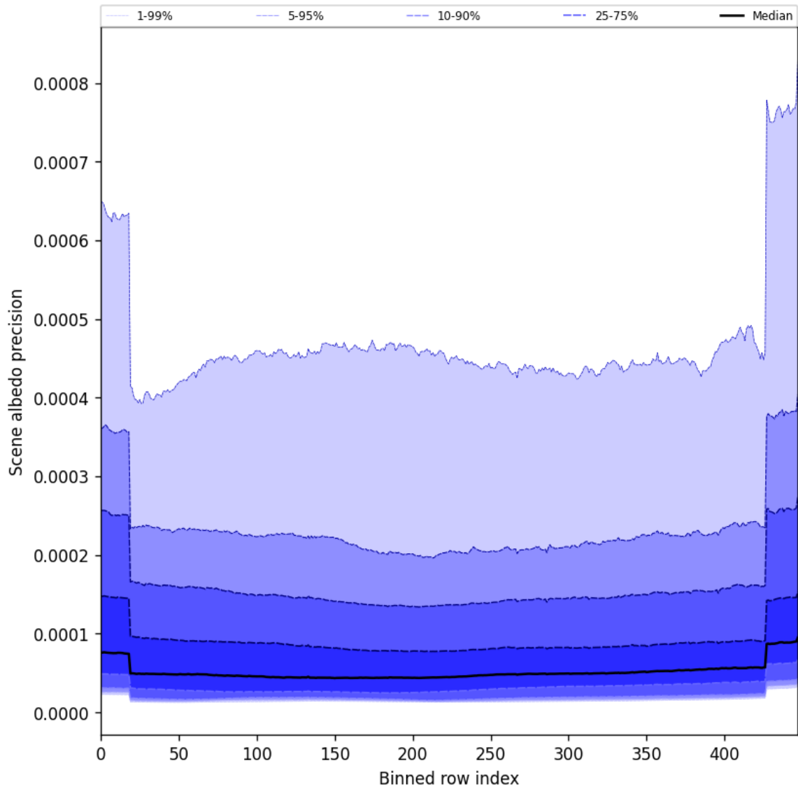
Figure 52: Along track statistics of “Scene albedo precision” for 2025-10-07 to 2025-10-09
