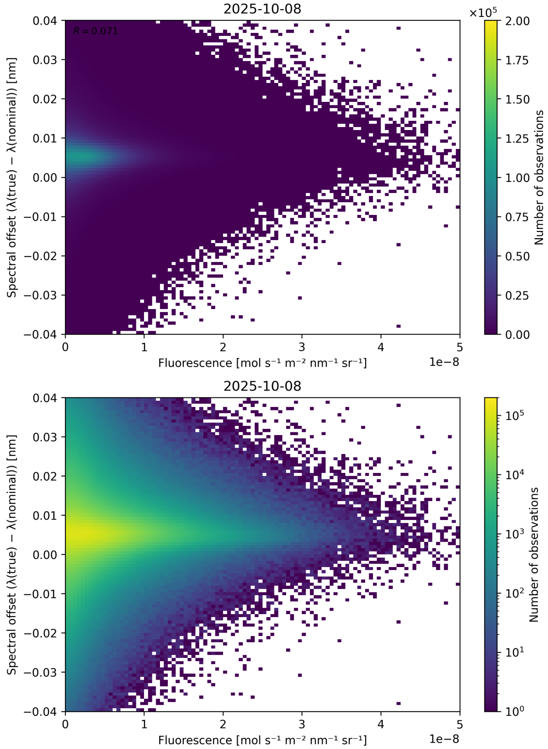
Figure 87: Scatter density plot of “Fluorescence” against “Spectral offset ( \lambda_{\text{true}} - \lambda_{\text{nominal}} )” for 2025-10-07 to 2025-10-09.
