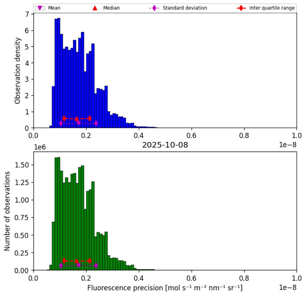
Figure 41: Histogram of “Fluorescence precision” for 2025-10-07 to 2025-10-09
