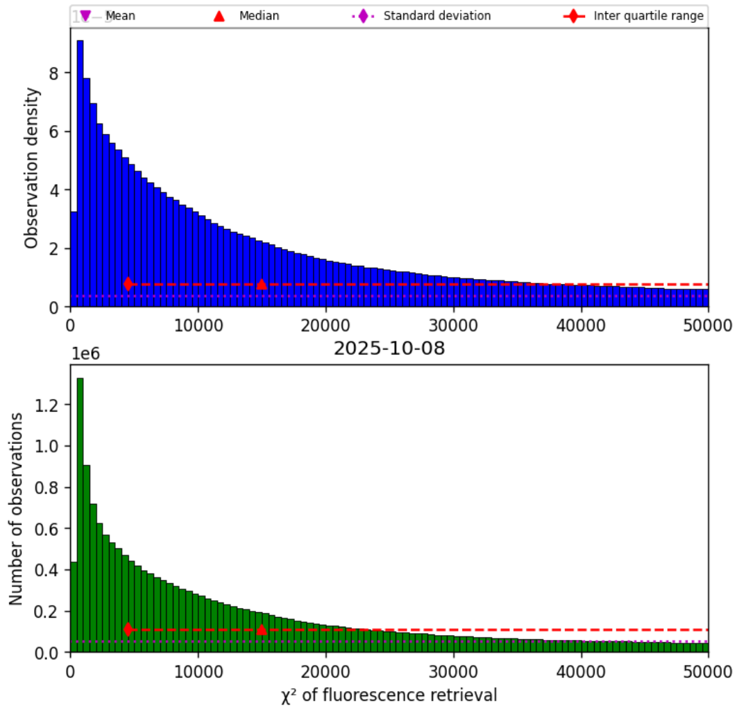
Figure 42: Histogram of “ \chi^2 of fluorescence retrieval” for 2025-10-07 to 2025-10-09
