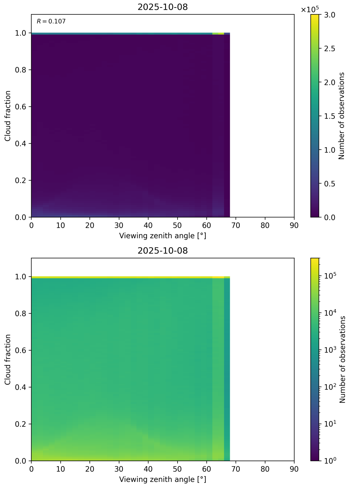
Figure 120: Scatter density plot of “Viewing zenith angle” against “Cloud fraction” for 2025-10-07 to 2025-10-09.
