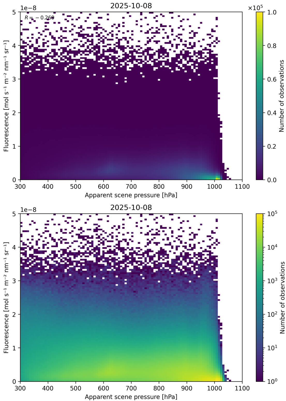
Figure 64: Scatter density plot of “Apparent scene pressure” against “Fluorescence” for 2025-10-07 to 2025-10-09.
