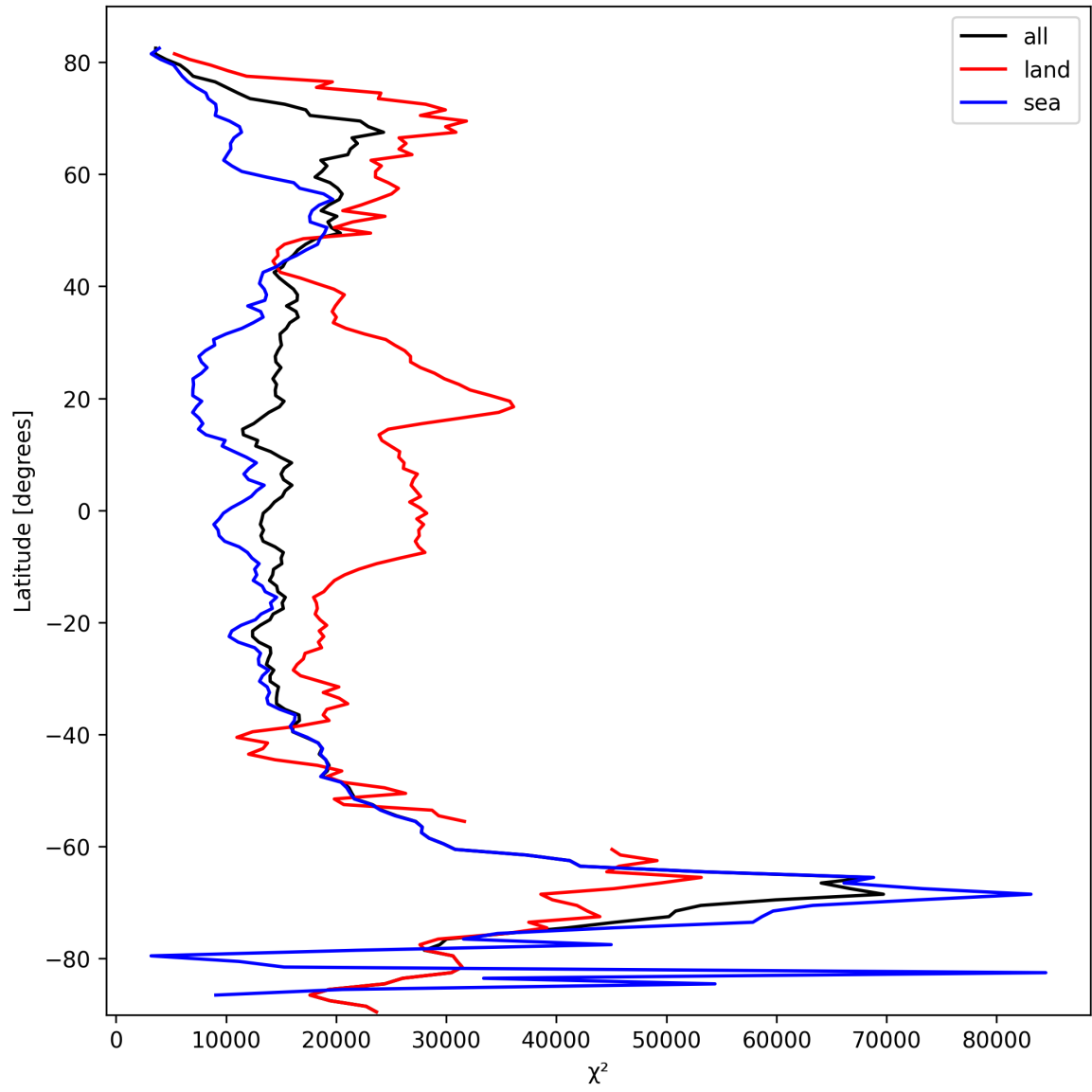
Figure 21: Zonal average of “ \chi^2 ” for 2025-10-07 to 2025-10-09.
