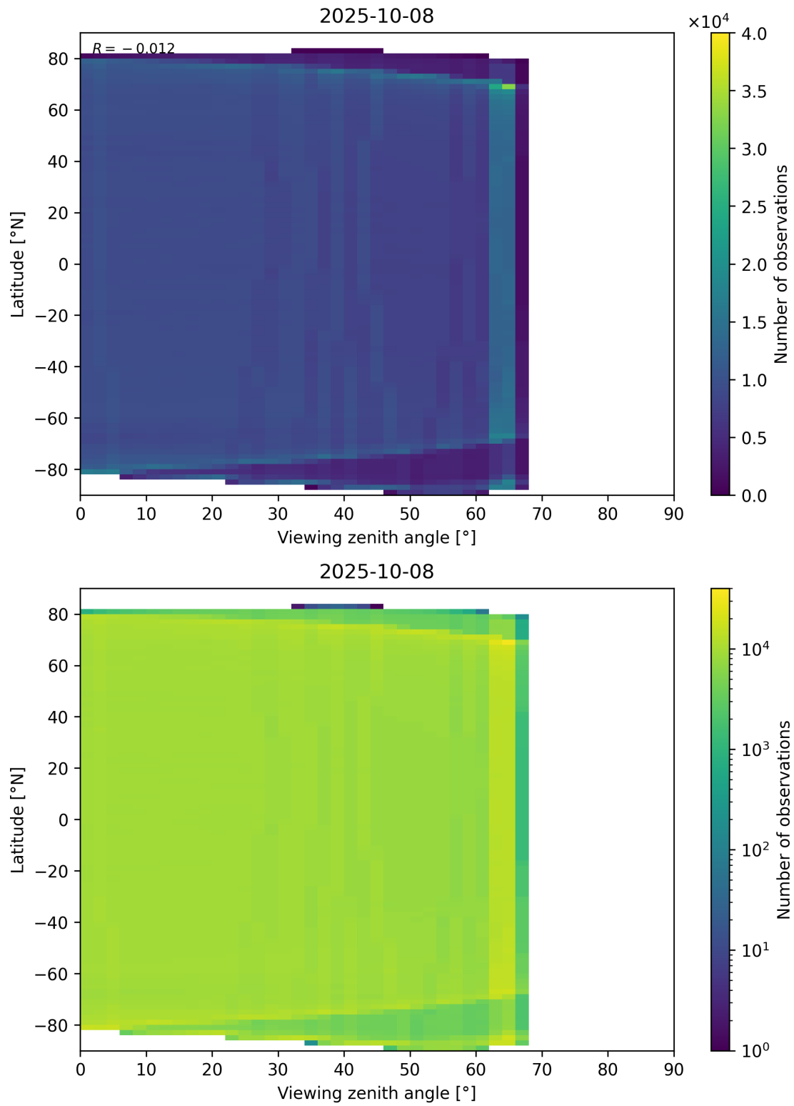
Figure 123: Scatter density plot of “Viewing zenith angle” against “Latitude” for 2025-10-07 to 2025-10-09.
