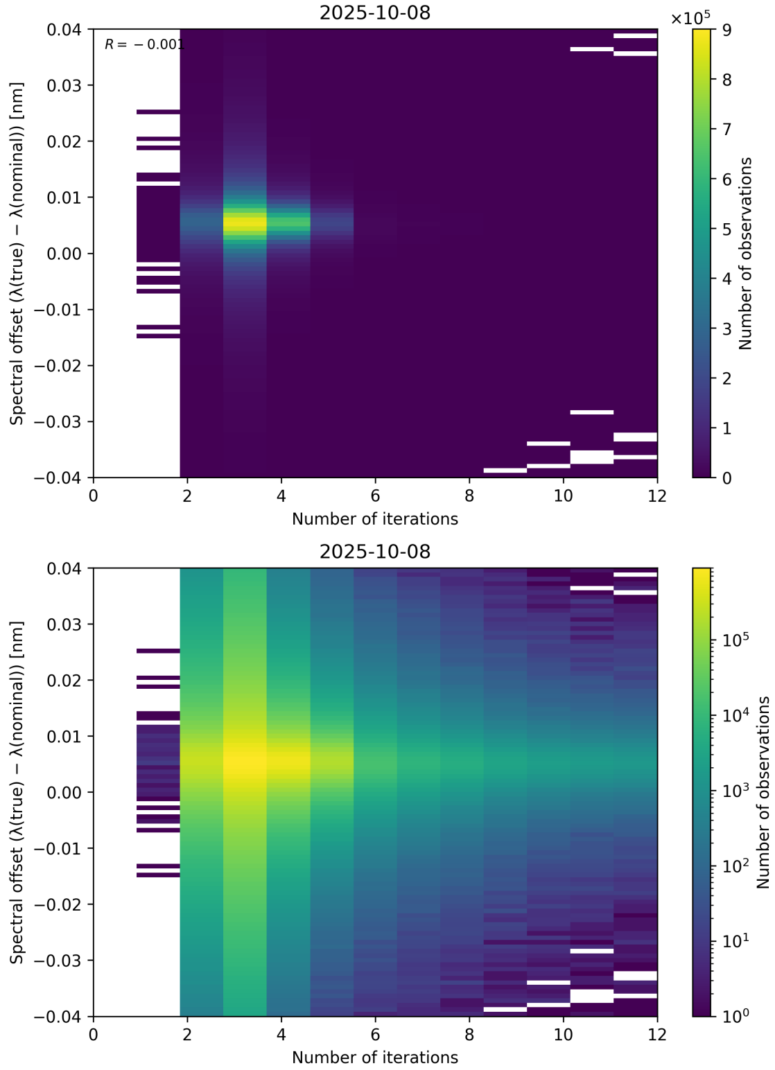
Figure 100: Scatter density plot of “Number of iterations” against “Spectral offset ( \lambda_{\text{true}} - \lambda_{\text{nominal}} )” for 2025-10-07 to 2025-10-09.
