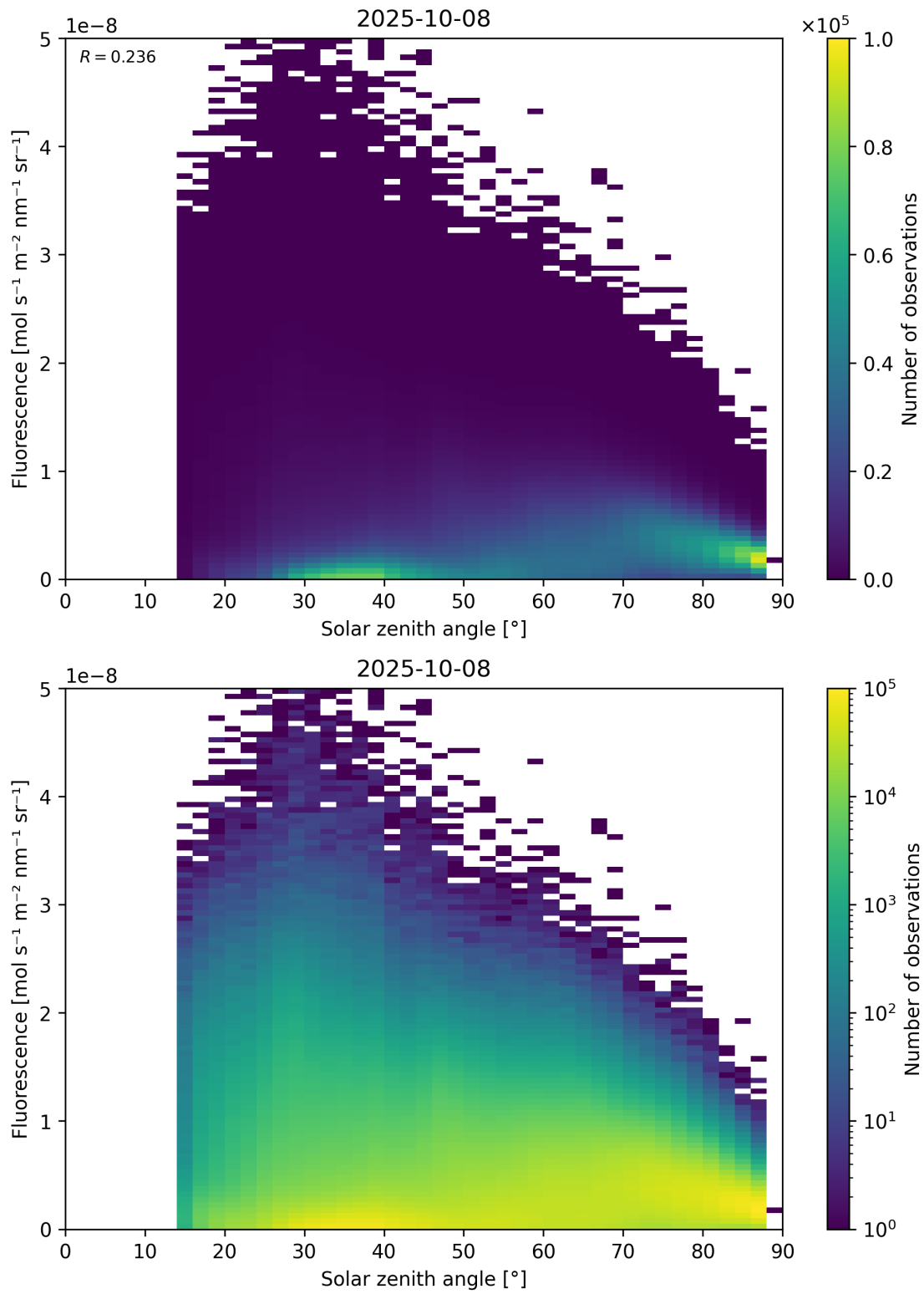
Figure 112: Scatter density plot of “Solar zenith angle” against “Fluorescence” for 2025-10-07 to 2025-10-09.
