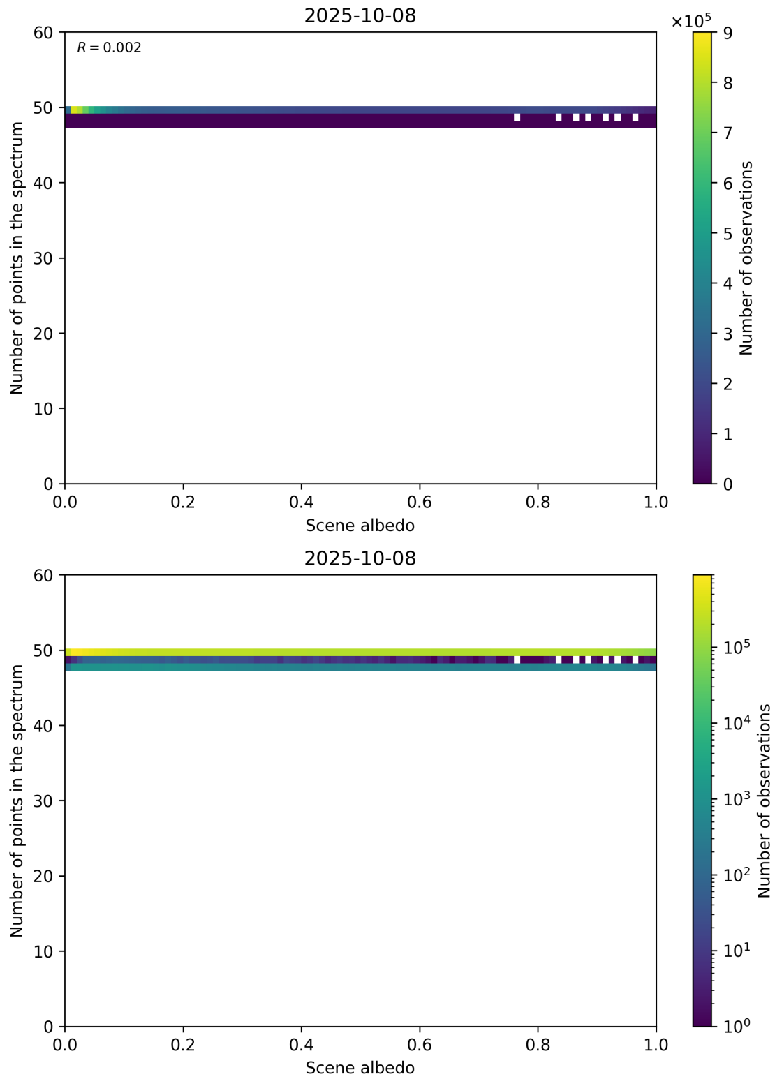
Figure 106: Scatter density plot of “Scene albedo” against “Number of points in the spectrum” for 2025-10-07 to 2025-10-09.
