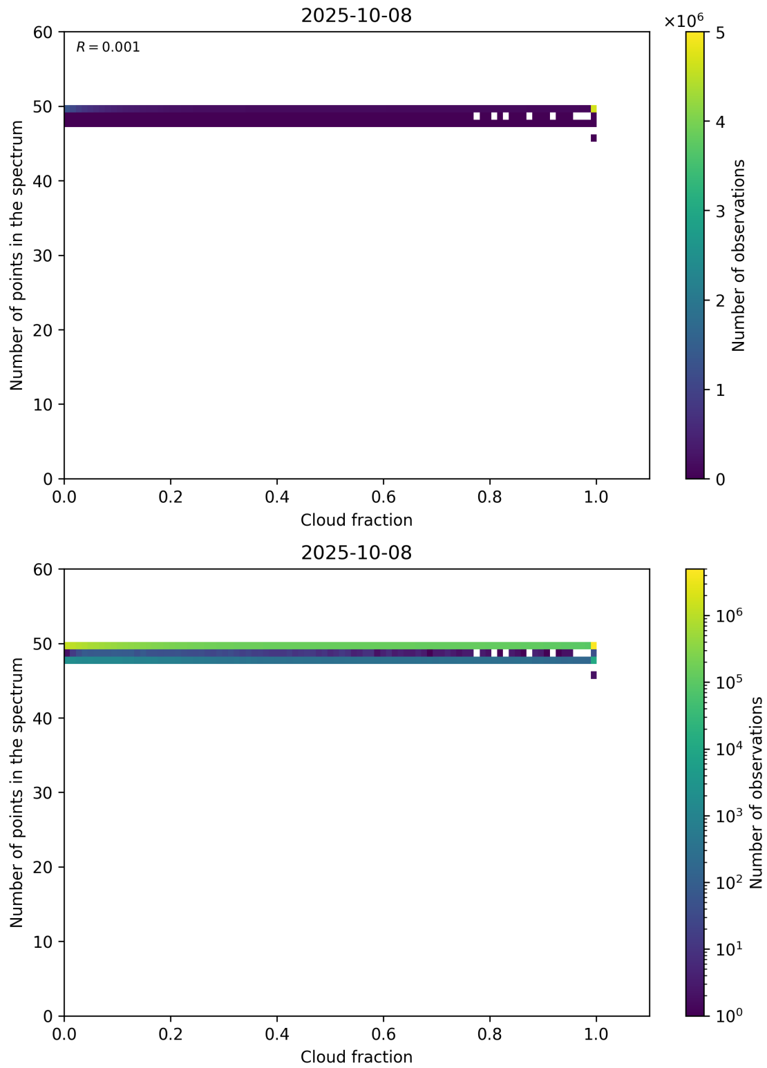
Figure 74: Scatter density plot of “Cloud fraction” against “Number of points in the spectrum” for 2025-10-07 to 2025-10-09.
