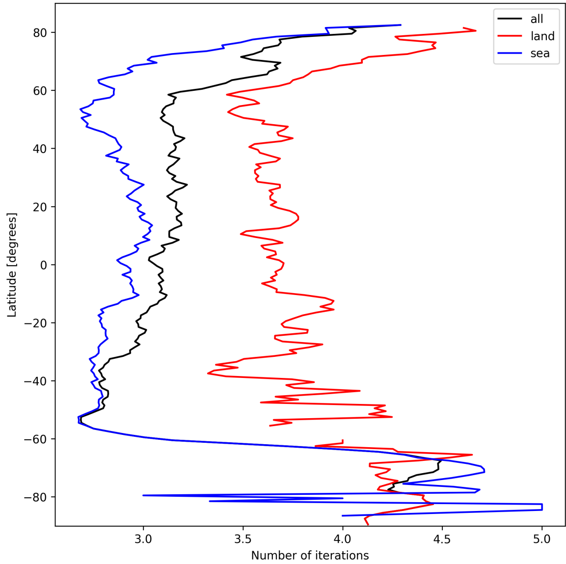
Figure 22: Zonal average of “Number of iterations” for 2025-10-07 to 2025-10-09.
