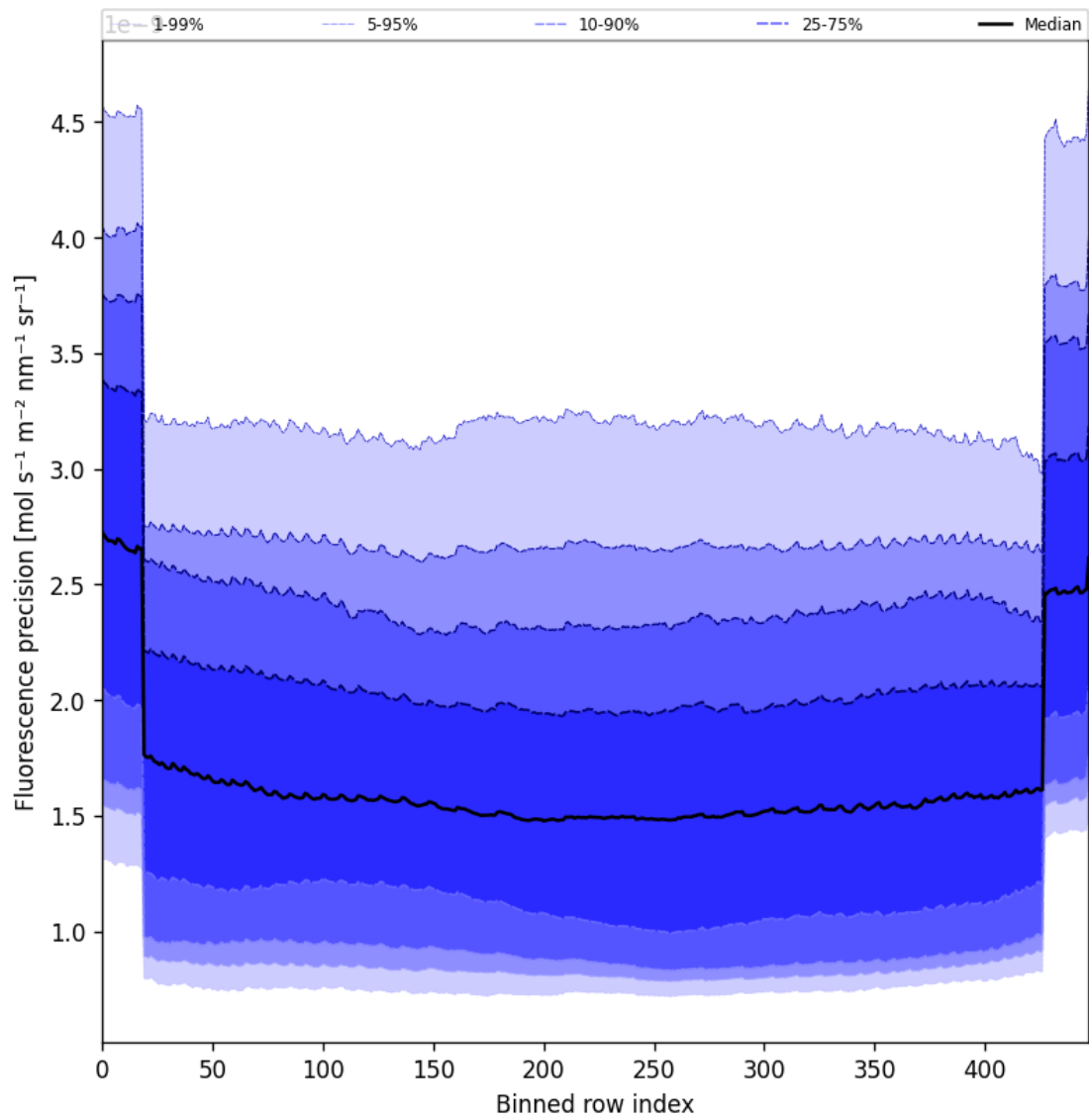
Figure 58: Along track statistics of “Fluorescence precision” for 2025-10-07 to 2025-10-09
