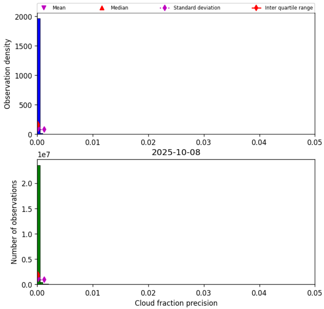
Figure 33: Histogram of “Cloud fraction precision” for 2025-10-07 to 2025-10-09
