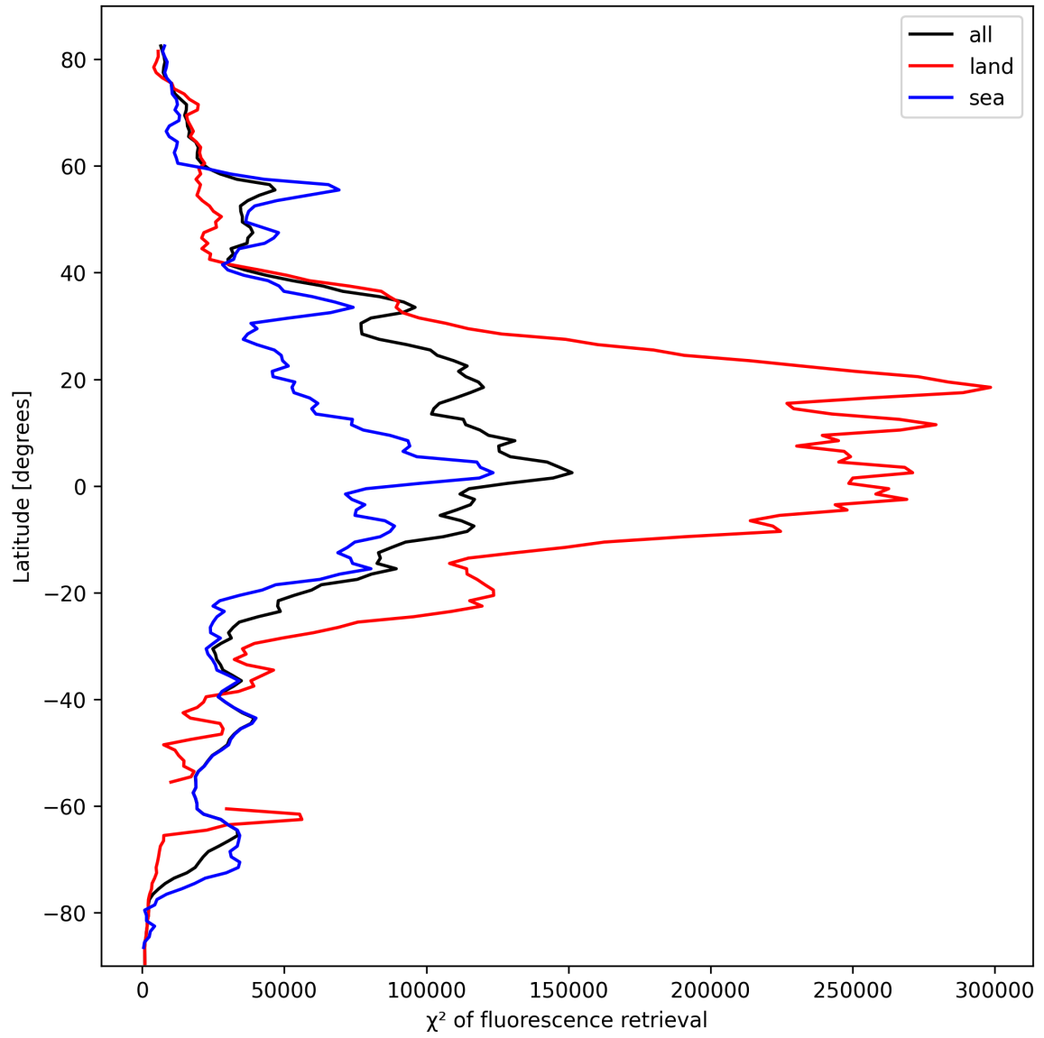
Figure 25: Zonal average of “ \chi^2 of fluorescence retrieval” for 2025-10-07 to 2025-10-09.
