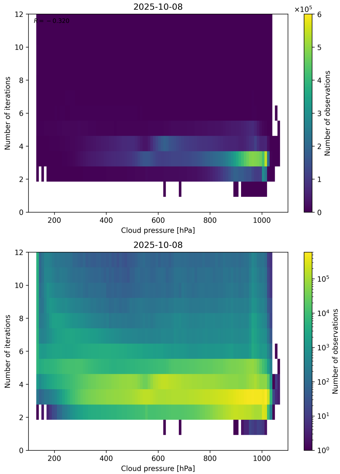
Figure 81: Scatter density plot of “Cloud pressure” against “Number of iterations” for 2025-10-07 to 2025-10-09.
