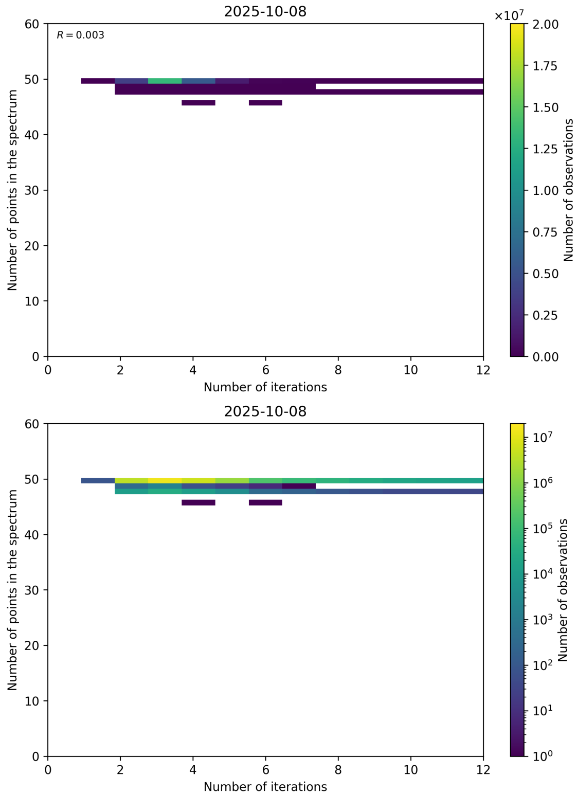
Figure 99: Scatter density plot of “Number of iterations” against “Number of points in the spectrum” for 2025-10-07 to 2025-10-09.
