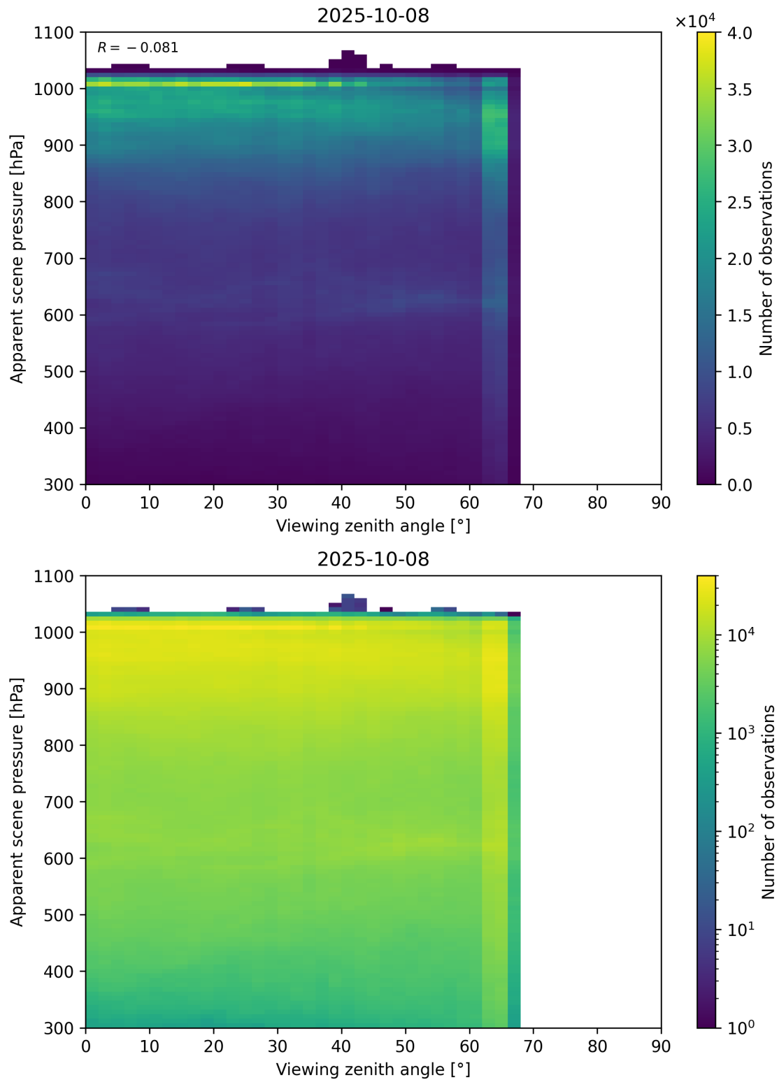
Figure 118: Scatter density plot of “Viewing zenith angle” against “Apparent scene pressure” for 2025-10-07 to 2025-10-09.
