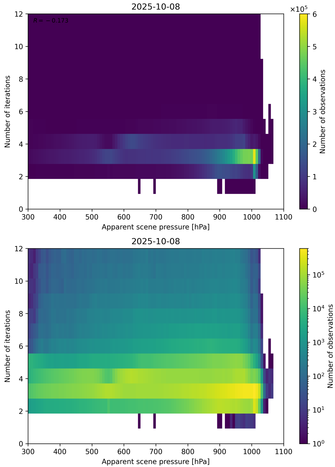
Figure 65: Scatter density plot of “Apparent scene pressure” against “Number of iterations” for 2025-10-07 to 2025-10-09.
