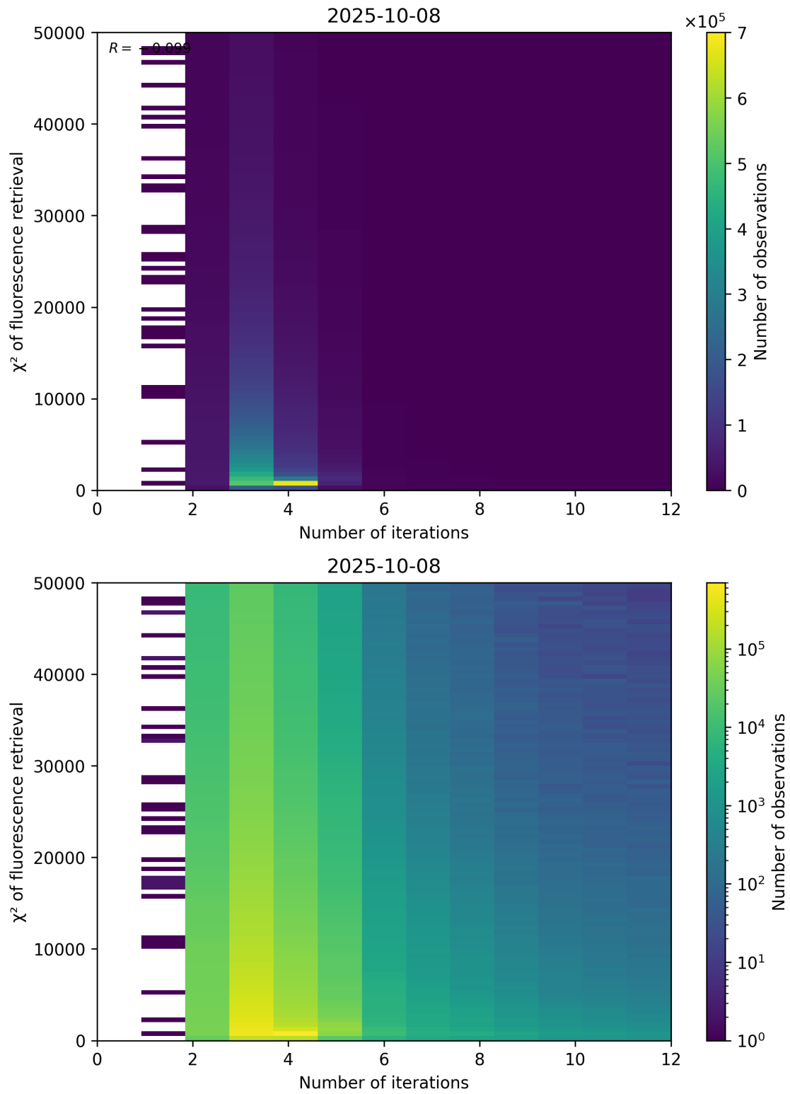
Figure 97: Scatter density plot of “Number of iterations” against “ \chi^2 of fluorescence retrieval” for 2025-10-07 to 2025-10-09.
