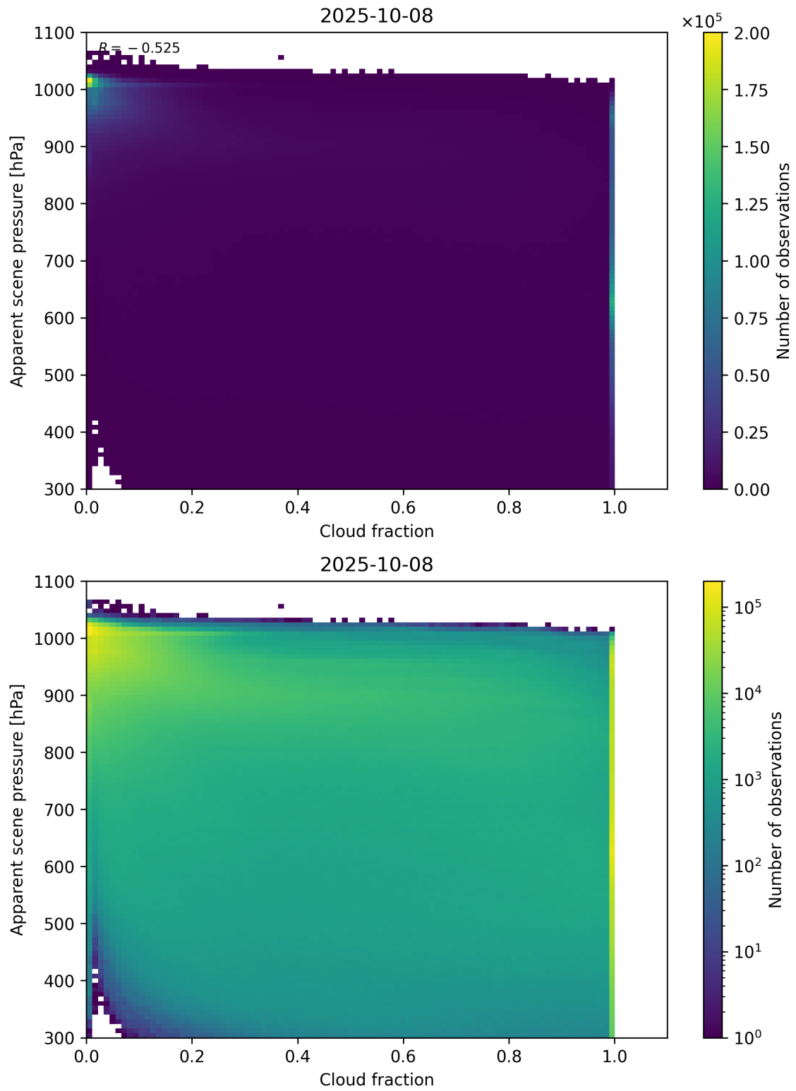
Figure 70: Scatter density plot of “Cloud fraction” against “Apparent scene pressure” for 2025-10-07 to 2025-10-09.
