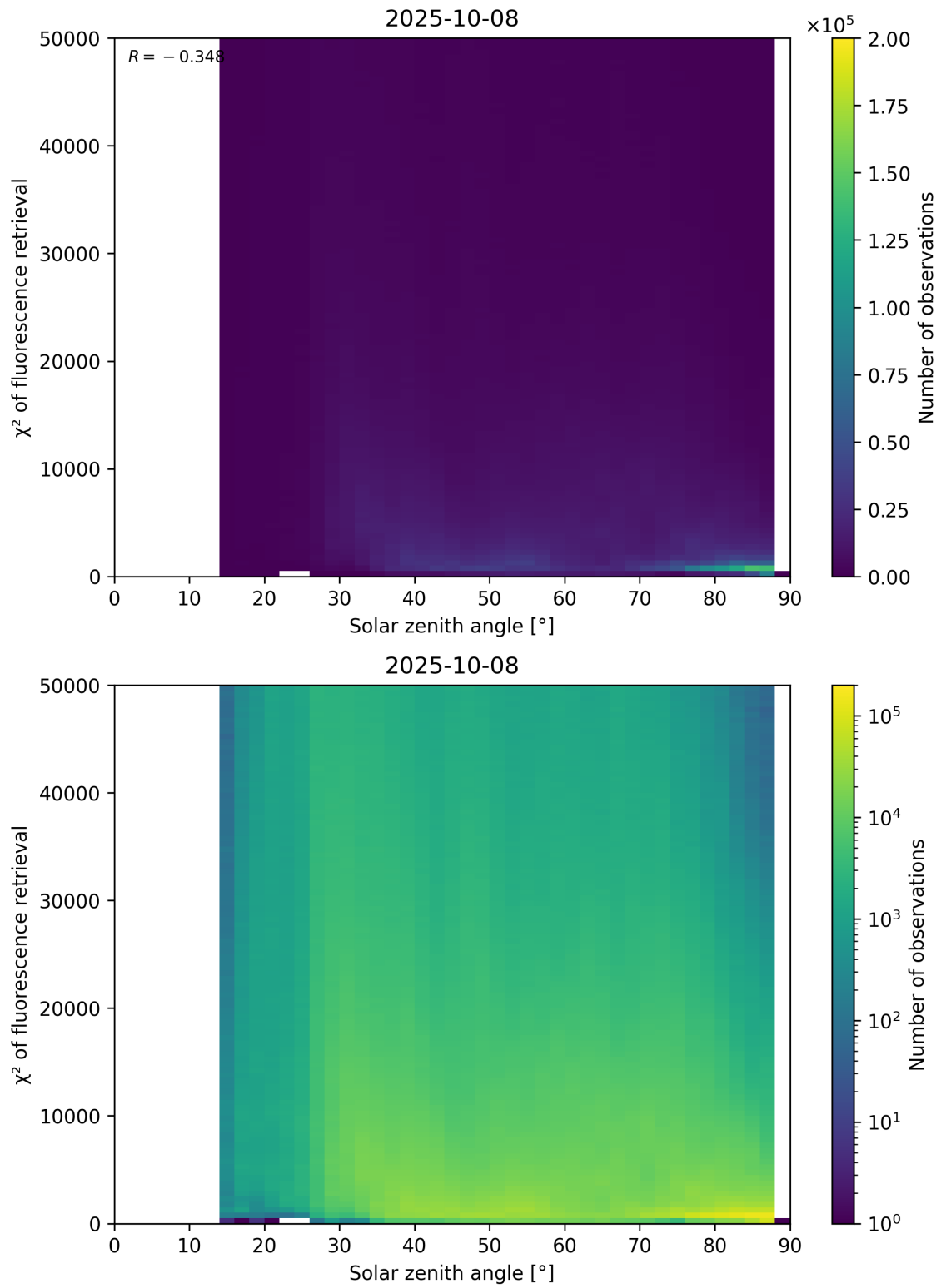
Figure 109: Scatter density plot of “Solar zenith angle” against “ \chi^2 of fluorescence retrieval” for 2025-10-07 to 2025-10-09.
