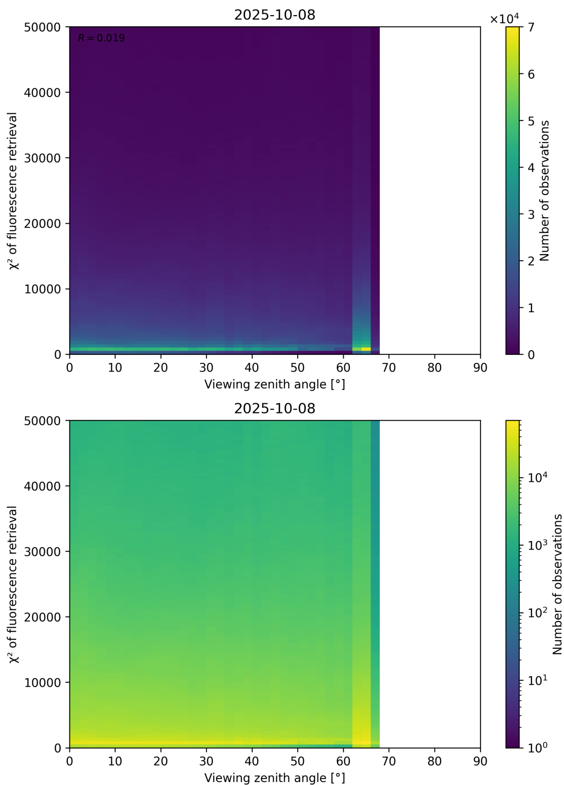
Figure 119: Scatter density plot of “Viewing zenith angle” against “ \chi^2 of fluorescence retrieval” for 2025-10-07 to 2025-10-09.
