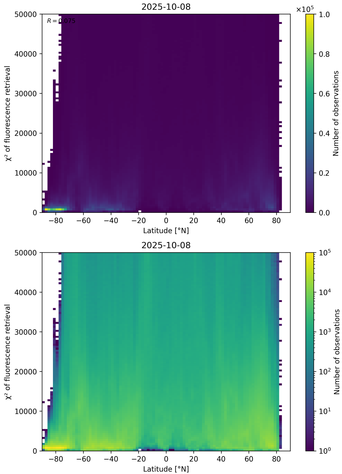
Figure 89: Scatter density plot of “Latitude” against “ \chi^2 of fluorescence retrieval” for 2025-10-07 to 2025-10-09.
