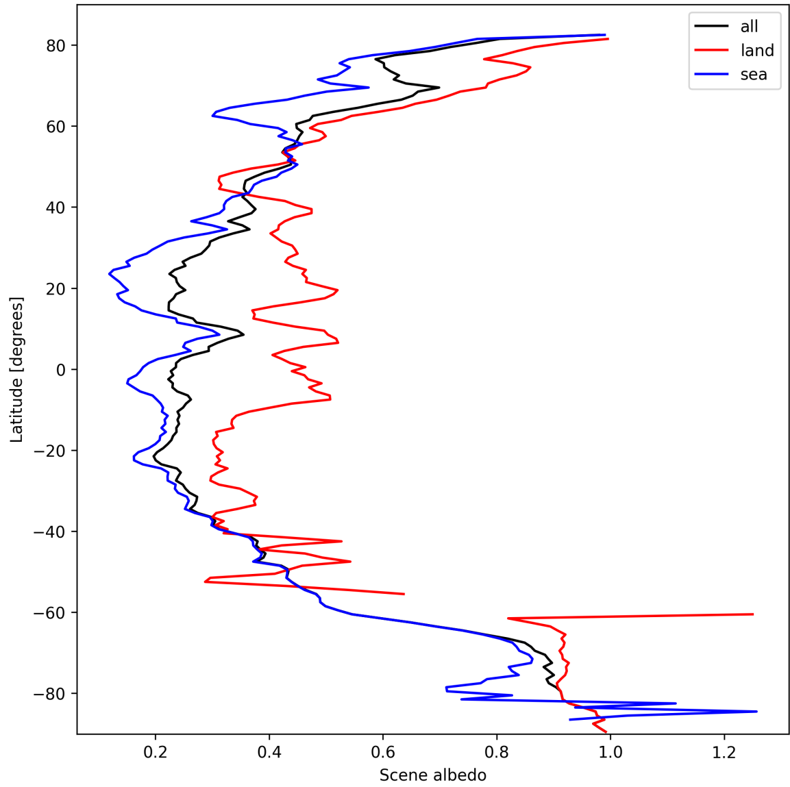
Figure 17: Zonal average of “Scene albedo” for 2025-10-07 to 2025-10-09.
