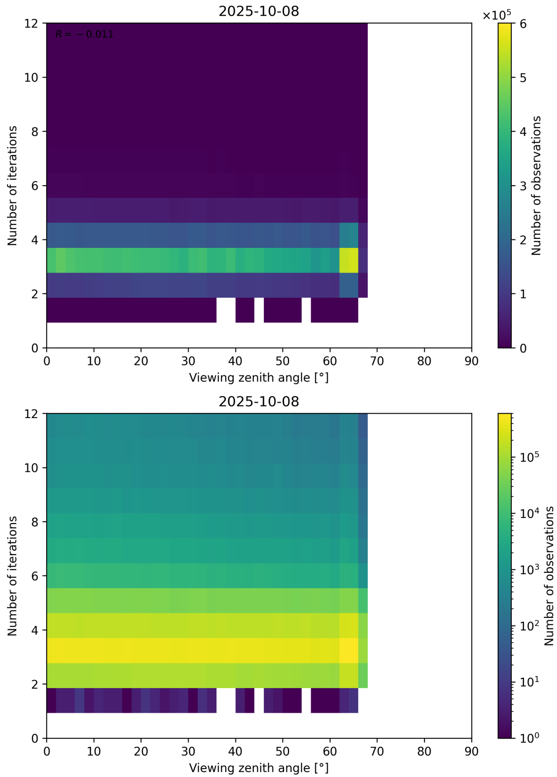
Figure 124: Scatter density plot of “Viewing zenith angle” against “Number of iterations” for 2025-10-07 to 2025-10-09.
