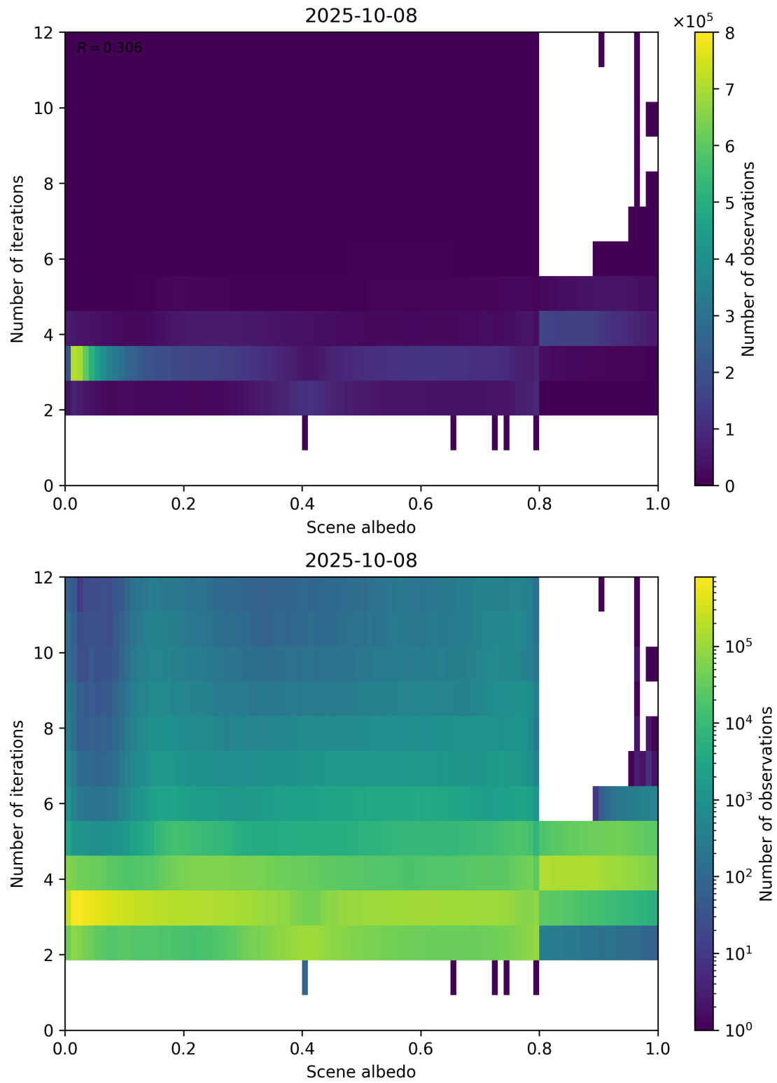
Figure 105: Scatter density plot of “Scene albedo” against “Number of iterations” for 2025-10-07 to 2025-10-09.
