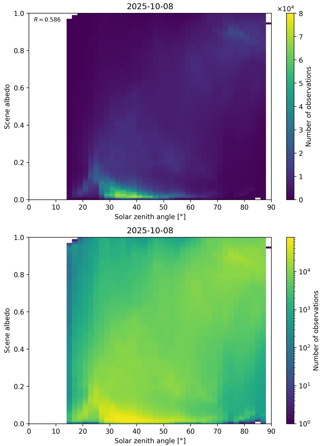
Figure 116: Scatter density plot of “Solar zenith angle” against “Scene albedo” for 2025-10-07 to 2025-10-09.
