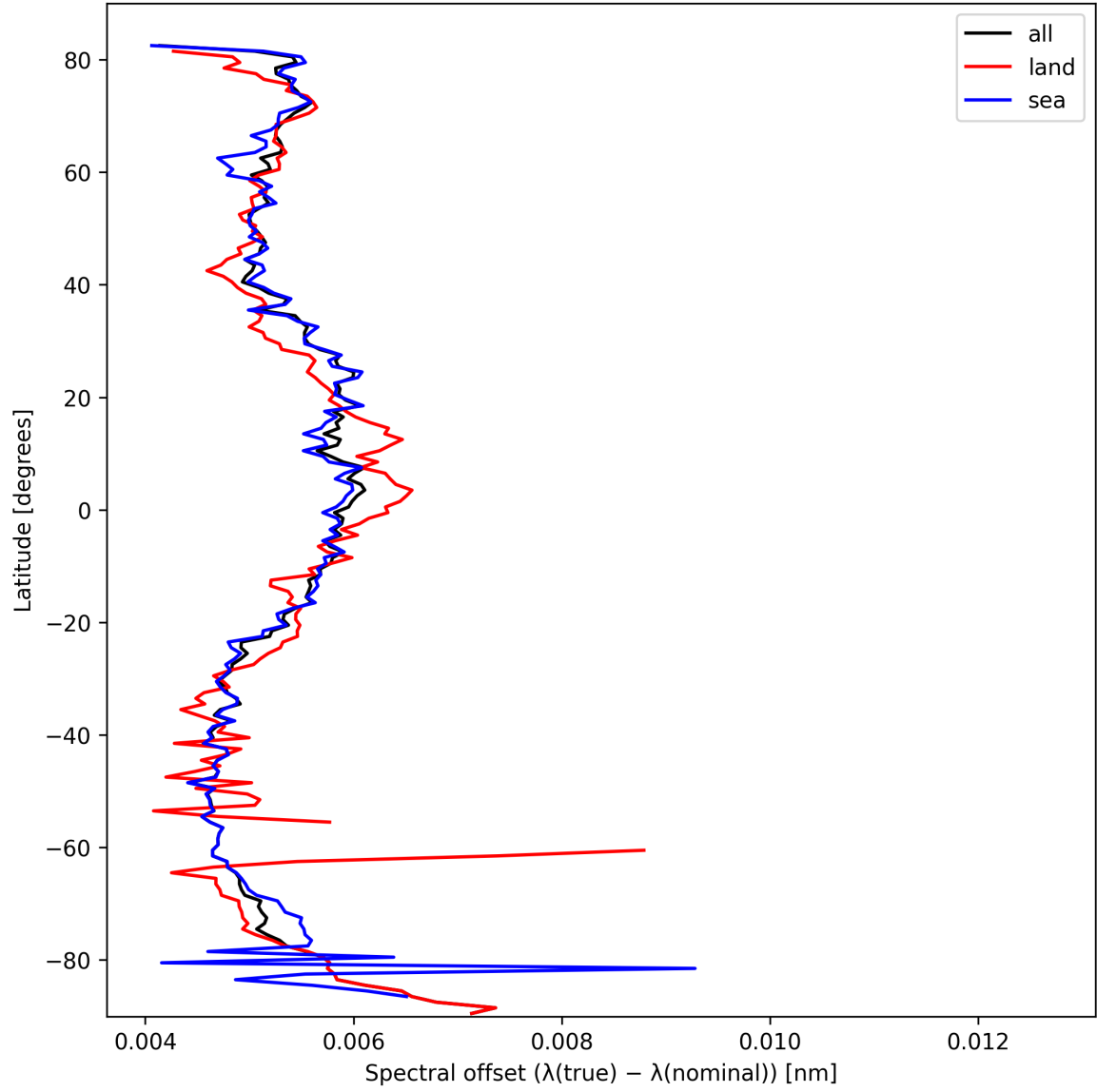
Figure 28: Zonal average of “Spectral offset ( \lambda_{\text{true}} - \lambda_{\text{nominal}} )” for 2025-10-07 to 2025-10-09.
