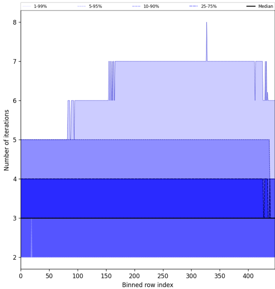
Figure 56: Along track statistics of “Number of iterations” for 2025-10-07 to 2025-10-09
