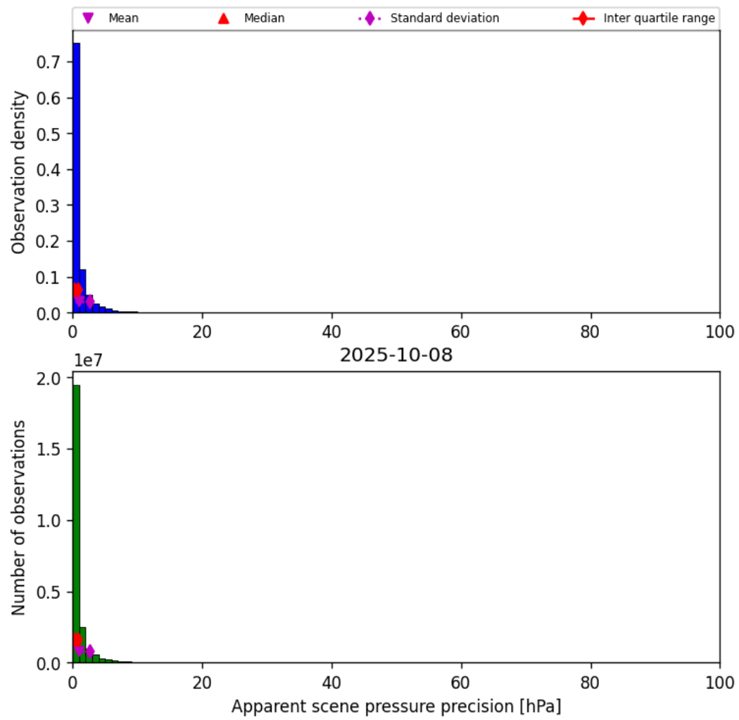
Figure 37: Histogram of “Apparent scene pressure precision” for 2025-10-07 to 2025-10-09
