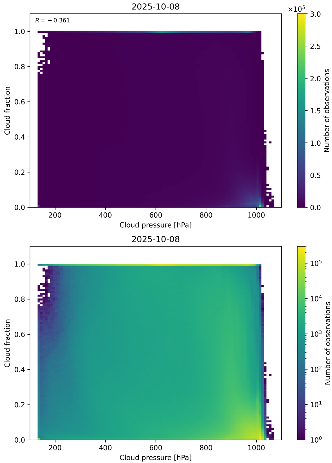
Figure 79: Scatter density plot of “Cloud pressure” against “Cloud fraction” for 2025-10-07 to 2025-10-09.
