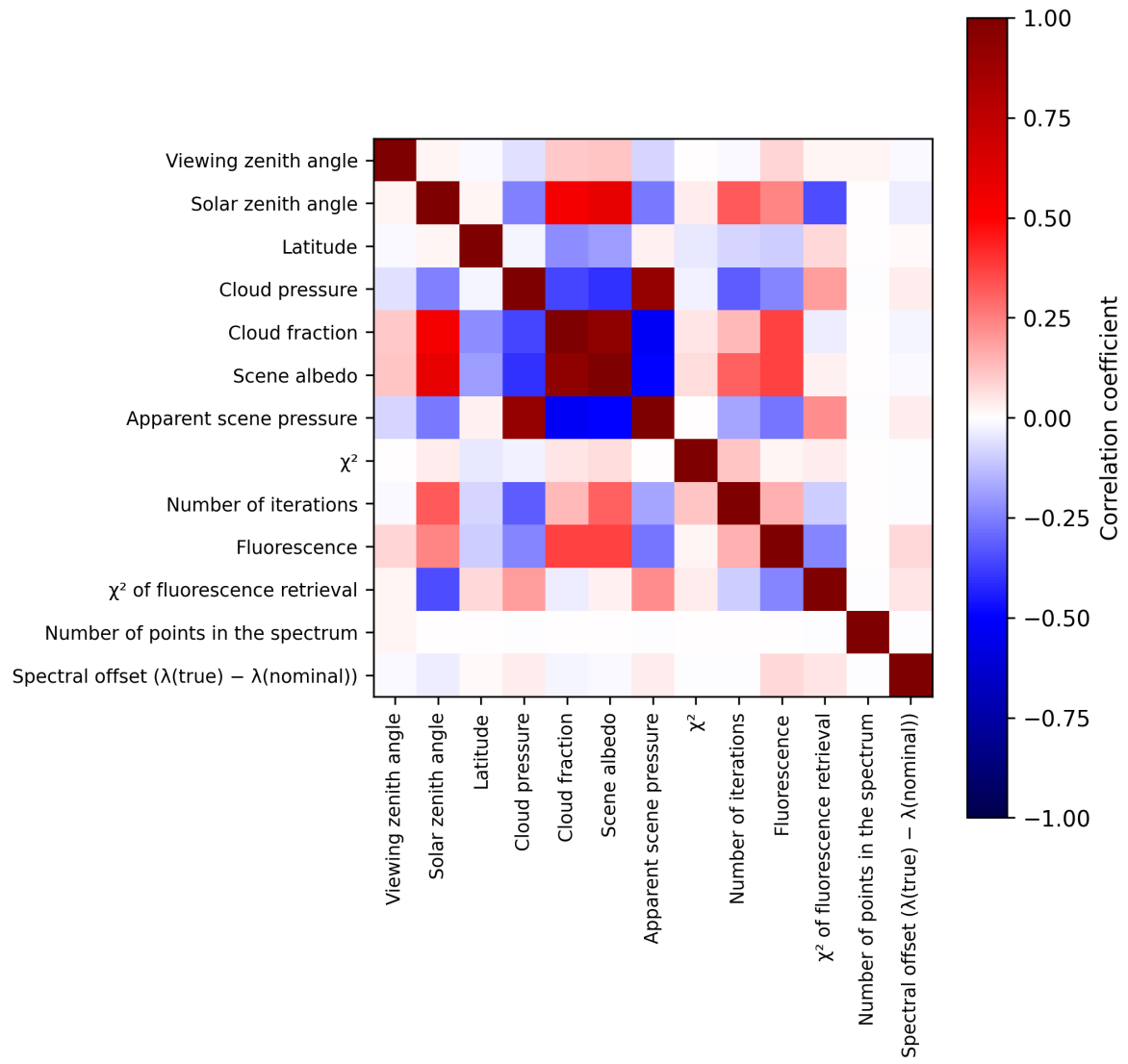
Figure 2: Map of correlation matrix for 2025-10-07 to 2025-10-09.
