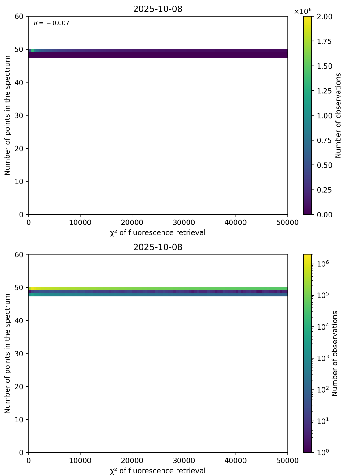
Figure 68: Scatter density plot of “ \chi^2 of fluorescence retrieval” against “Number of points in the spectrum” for 2025-10-07 to 2025-10-09.
