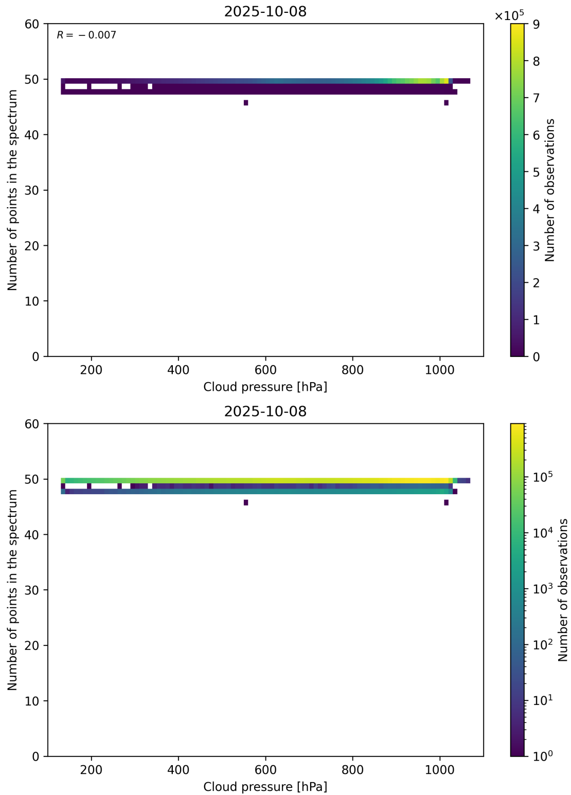
Figure 82: Scatter density plot of “Cloud pressure” against “Number of points in the spectrum” for 2025-10-07 to 2025-10-09.
