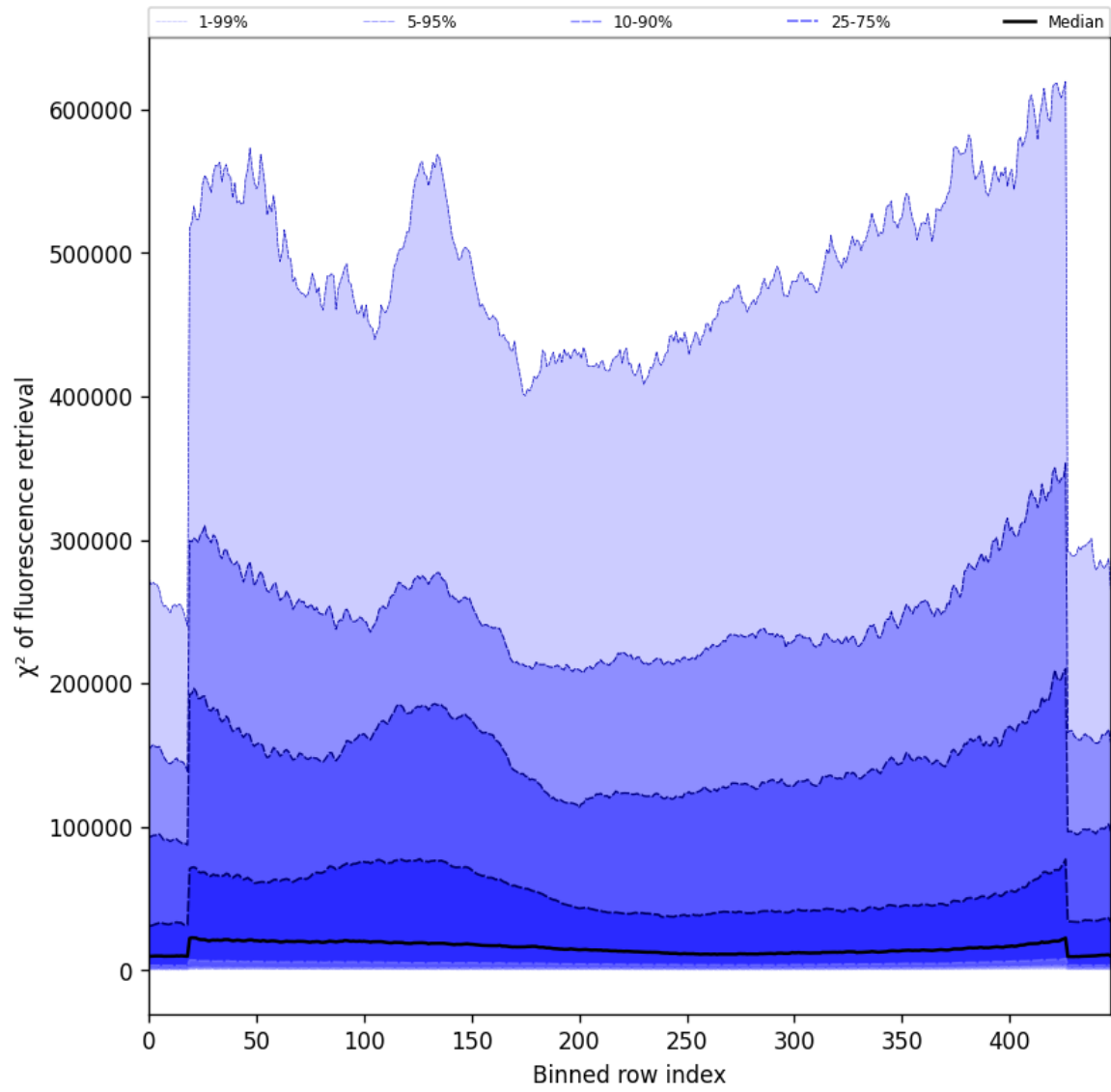
Figure 59: Along track statistics of “ \chi^2 of fluorescence retrieval” for 2025-10-07 to 2025-10-09
