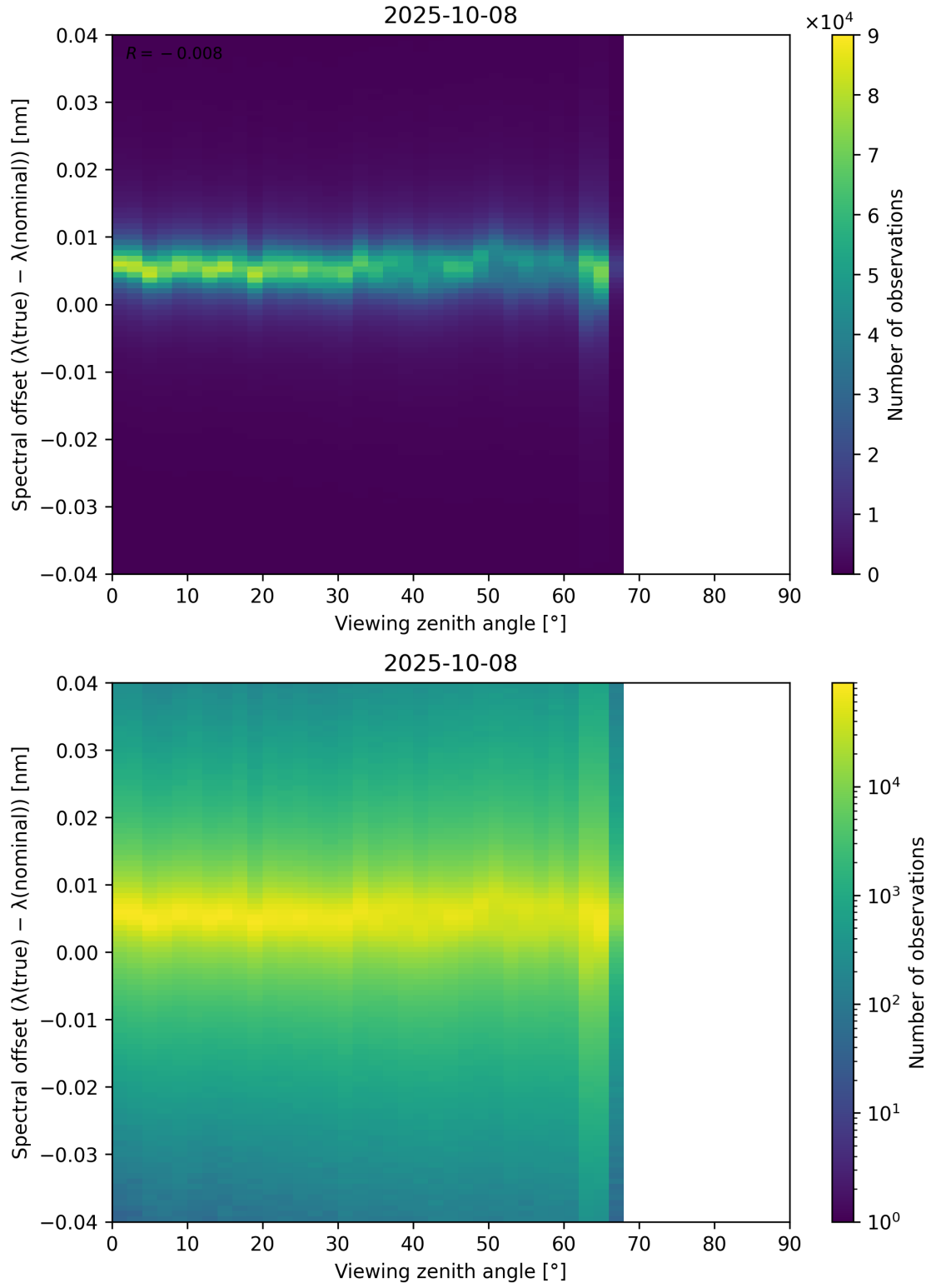
Figure 128: Scatter density plot of “Viewing zenith angle” against “Spectral offset ( \lambda_{\text{true}} - \lambda_{\text{nominal}} )” for 2025-10-07 to 2025-10-09.
