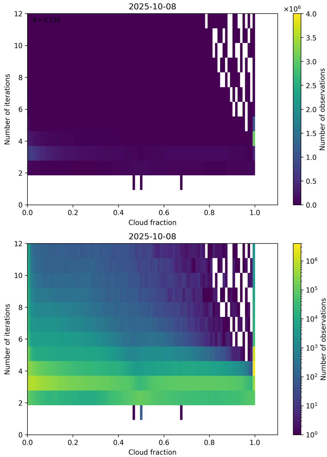
Figure 73: Scatter density plot of “Cloud fraction” against “Number of iterations” for 2025-10-07 to 2025-10-09.
