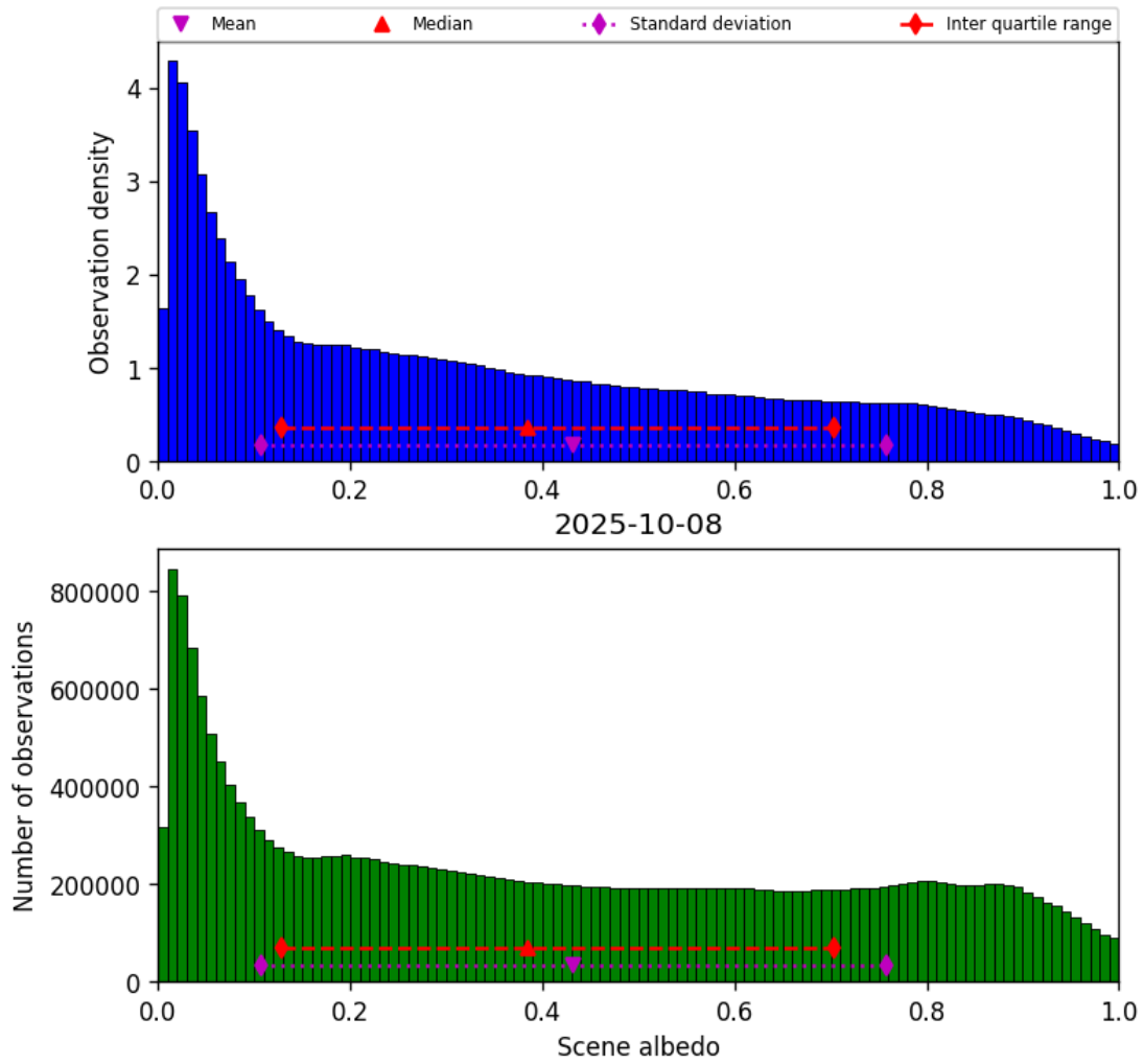
Figure 34: Histogram of “Scene albedo” for 2025-10-07 to 2025-10-09
