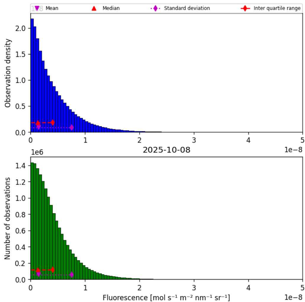
Figure 40: Histogram of “Fluorescence” for 2025-10-07 to 2025-10-09
