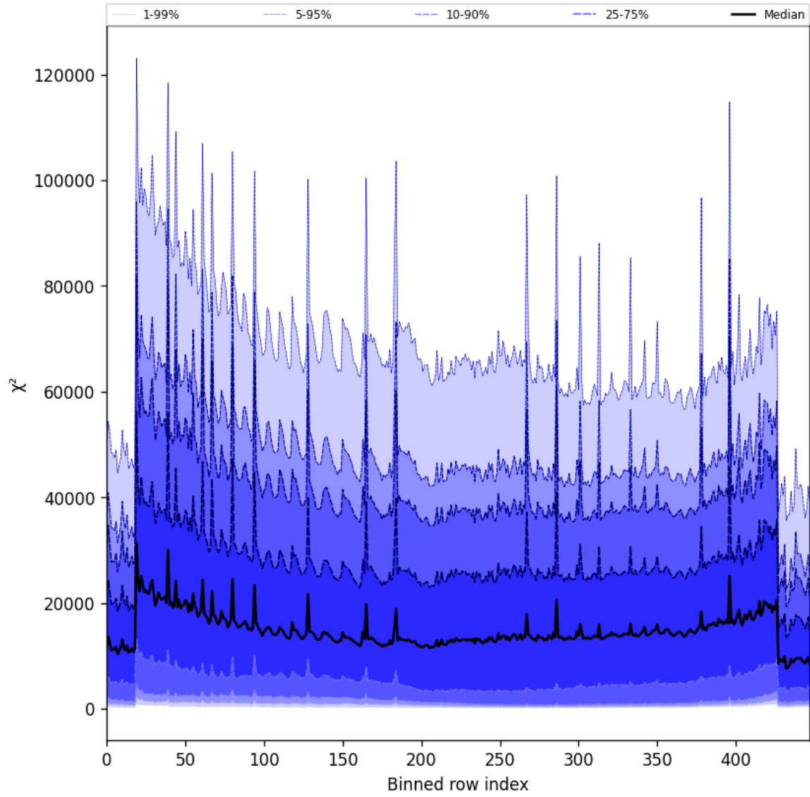
Figure 55: Along track statistics of “ \chi^2 ” for 2025-10-07 to 2025-10-09
