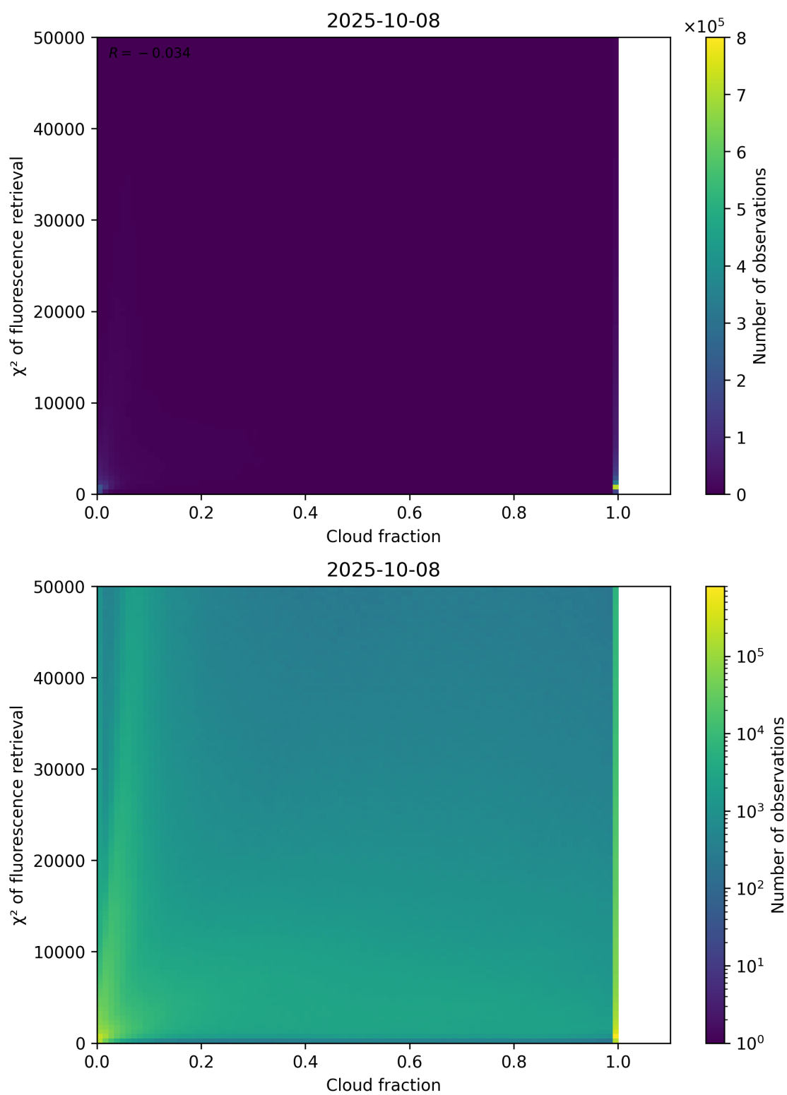
Figure 71: Scatter density plot of “Cloud fraction” against “ \chi^2 of fluorescence retrieval” for 2025-10-07 to 2025-10-09.
