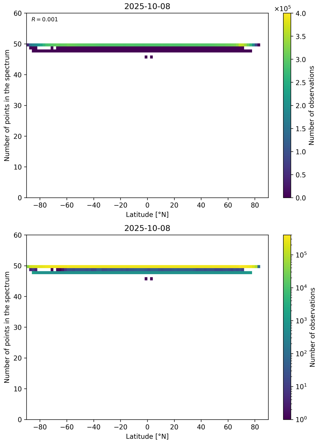
Figure 94: Scatter density plot of “Latitude” against “Number of points in the spectrum” for 2025-10-07 to 2025-10-09.
