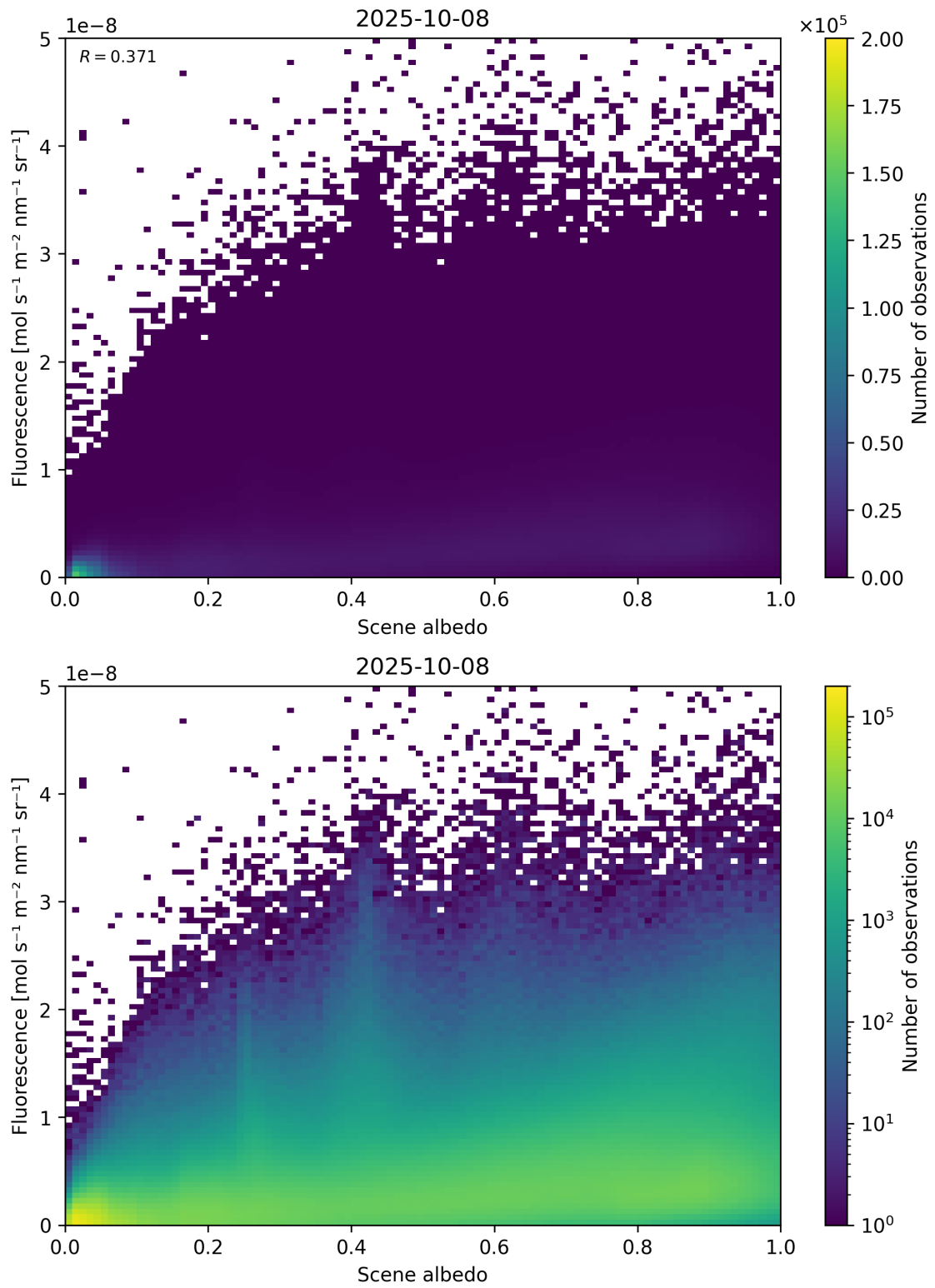
Figure 104: Scatter density plot of “Scene albedo” against “Fluorescence” for 2025-10-07 to 2025-10-09.
