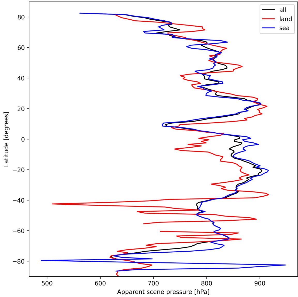
Figure 19: Zonal average of “Apparent scene pressure” for 2025-10-07 to 2025-10-09.
