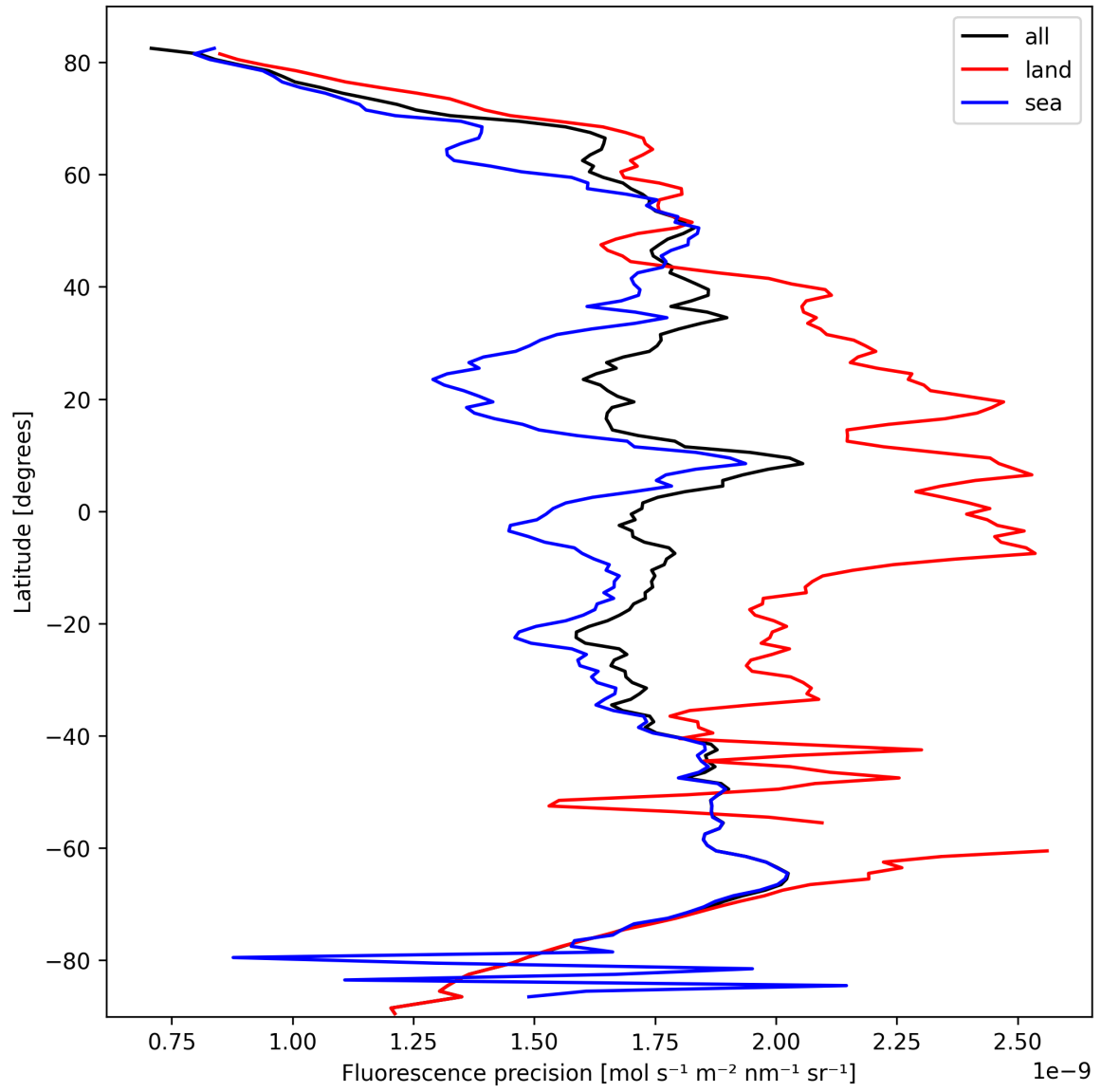
Figure 24: Zonal average of “Fluorescence precision” for 2025-10-07 to 2025-10-09.
