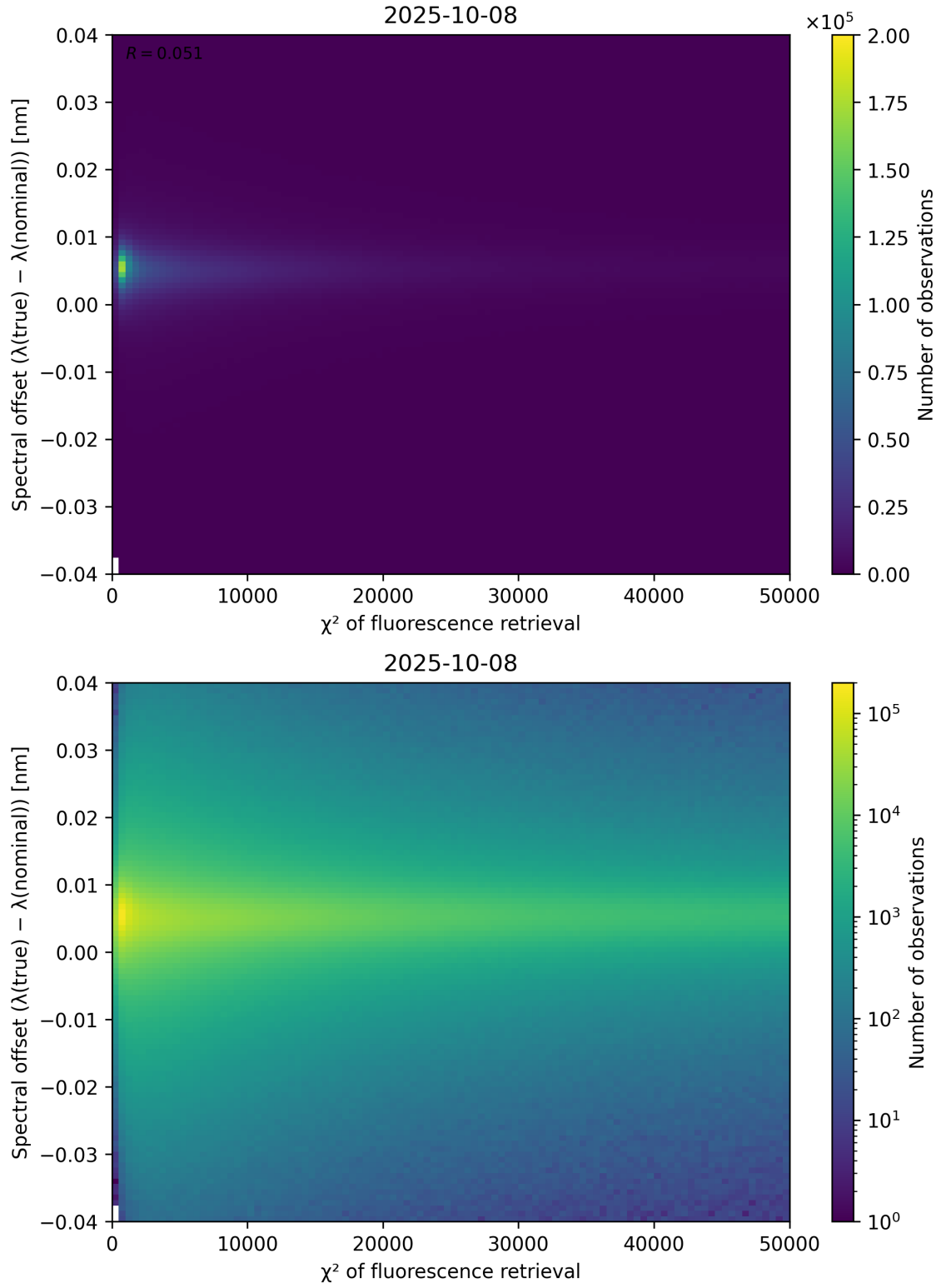
Figure 69: Scatter density plot of “ \chi^2 of fluorescence retrieval” against “Spectral offset ( \lambda_{\text{true}} - \lambda_{\text{nominal}} )” for 2025-10-07 to 2025-10-09.
