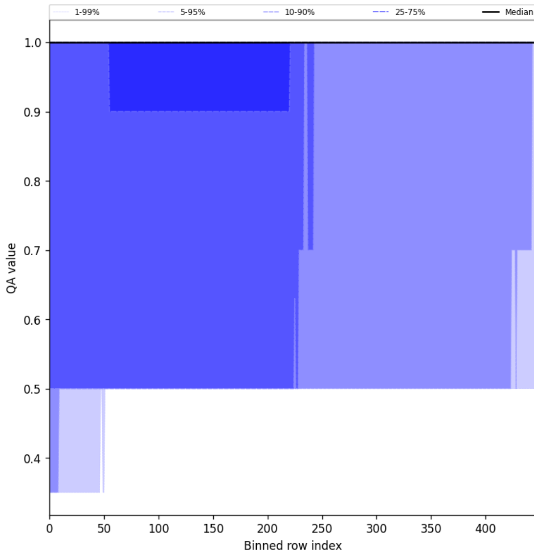
Figure 46: Along track statistics of “QA value” for 2025-10-07 to 2025-10-09
