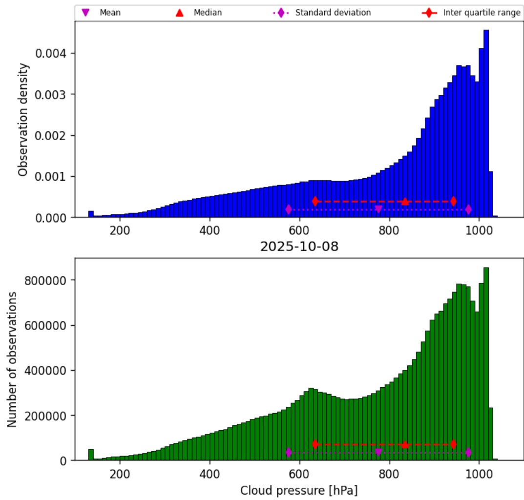
Figure 30: Histogram of “Cloud pressure” for 2025-10-07 to 2025-10-09
