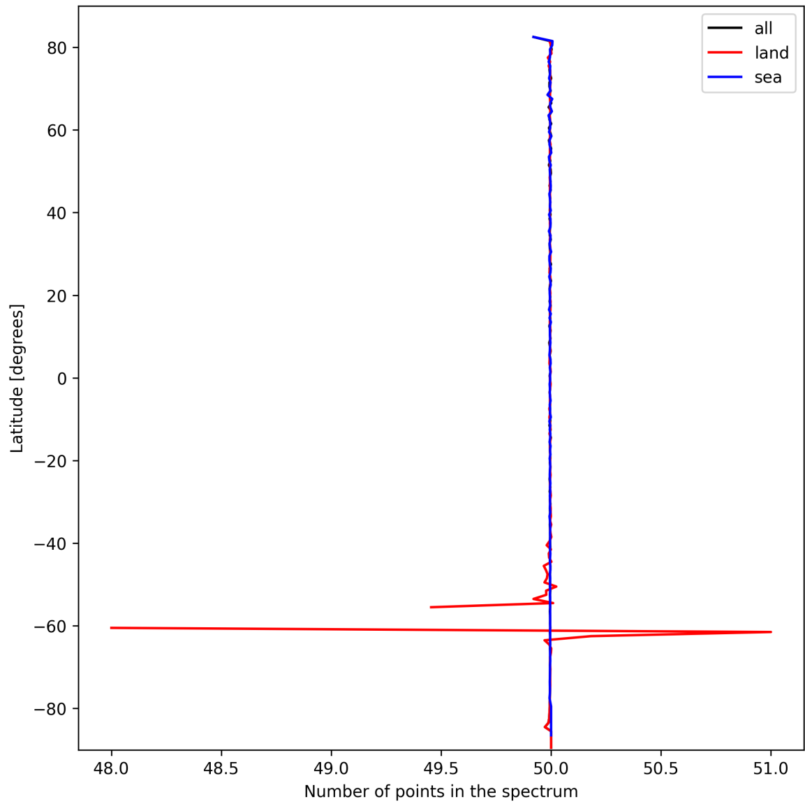
Figure 27: Zonal average of “Number of points in the spectrum” for 2025-10-07 to 2025-10-09.
