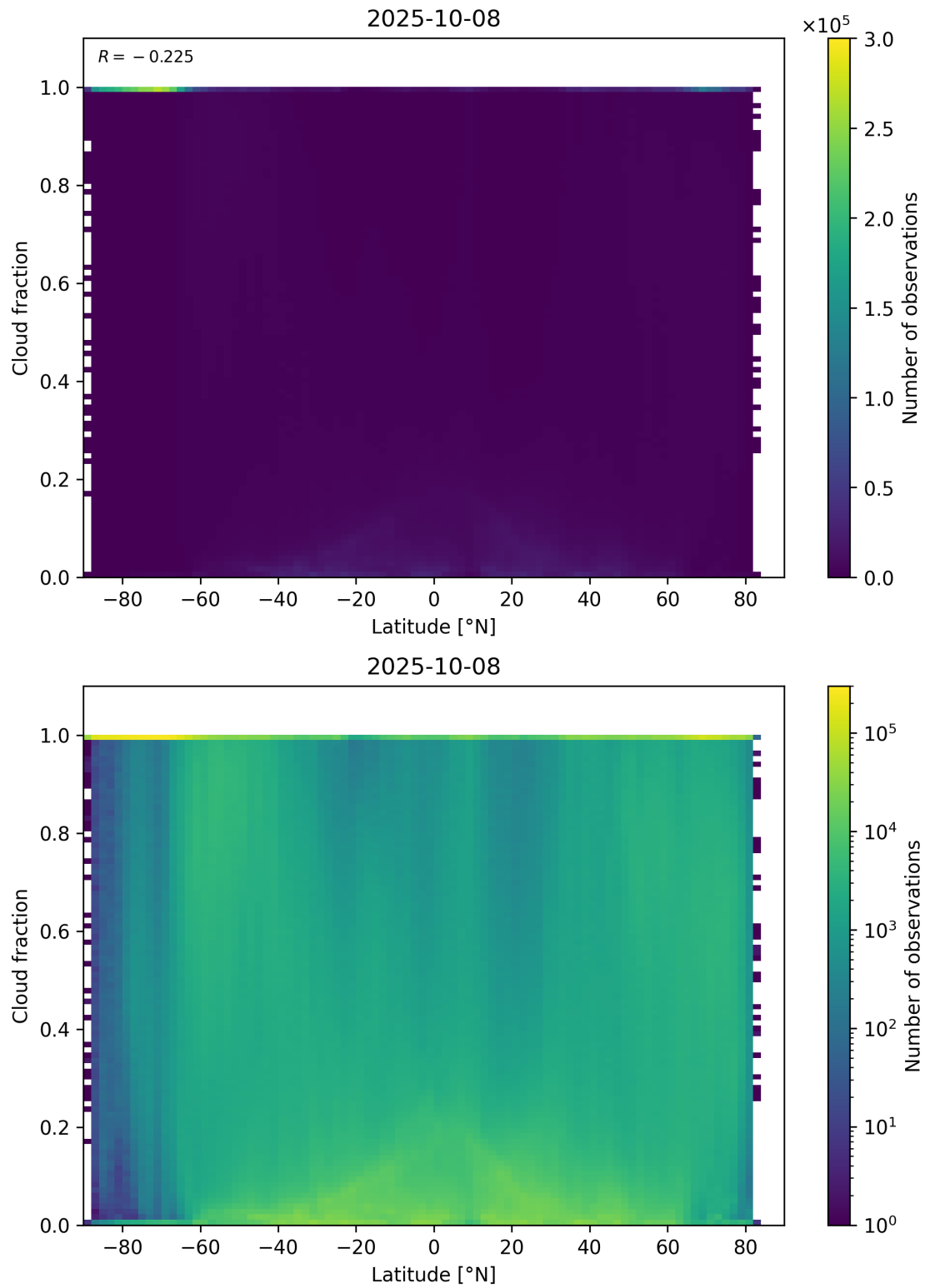
Figure 90: Scatter density plot of “Latitude” against “Cloud fraction” for 2025-10-07 to 2025-10-09.
