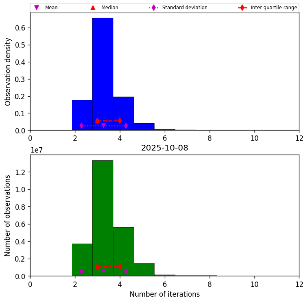
Figure 39: Histogram of “Number of iterations” for 2025-10-07 to 2025-10-09
