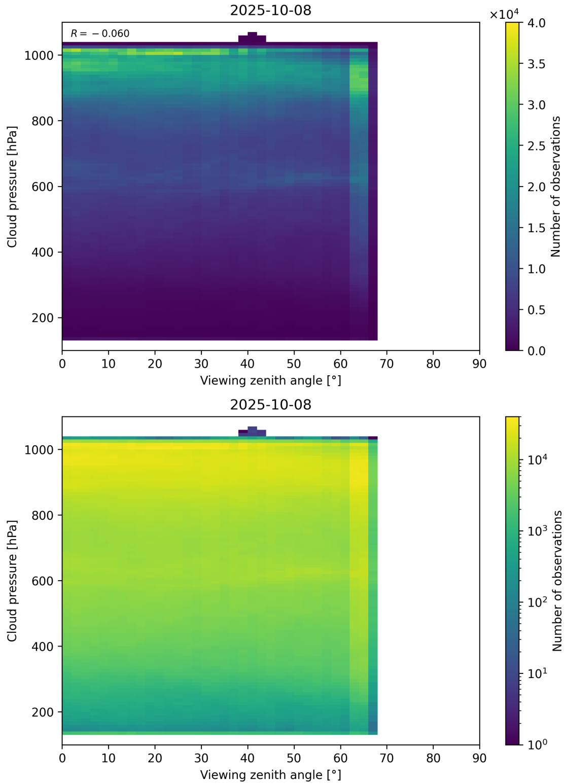
Figure 121: Scatter density plot of “Viewing zenith angle” against “Cloud pressure” for 2025-10-07 to 2025-10-09.
