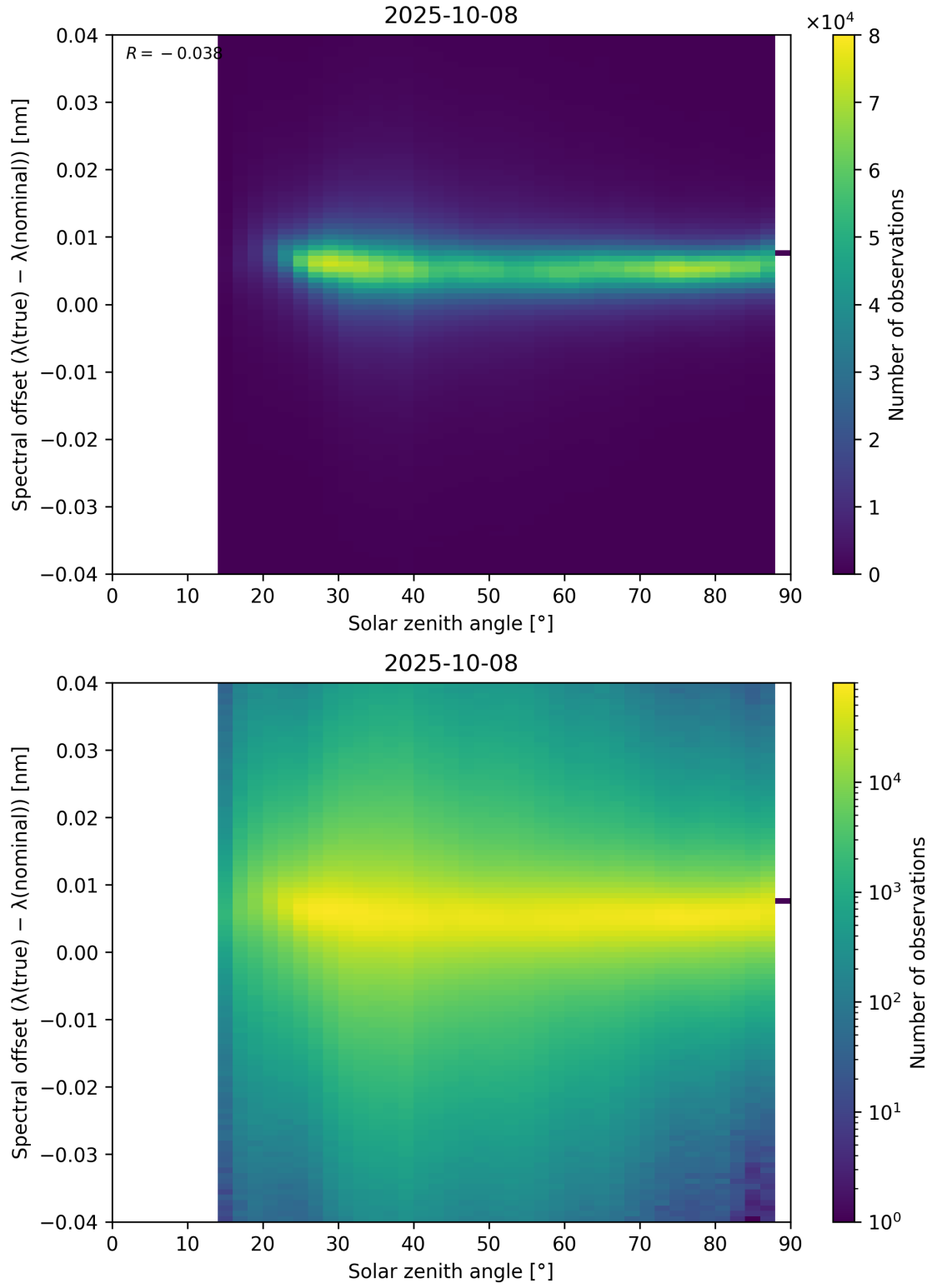
Figure 117: Scatter density plot of “Solar zenith angle” against “Spectral offset ( \lambda_{\text{true}} - \lambda_{\text{nominal}} )” for 2025-10-07 to 2025-10-09.
