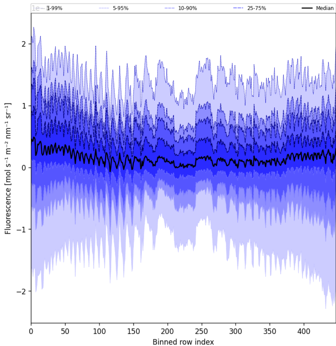
Figure 57: Along track statistics of “Fluorescence” for 2025-10-07 to 2025-10-09
