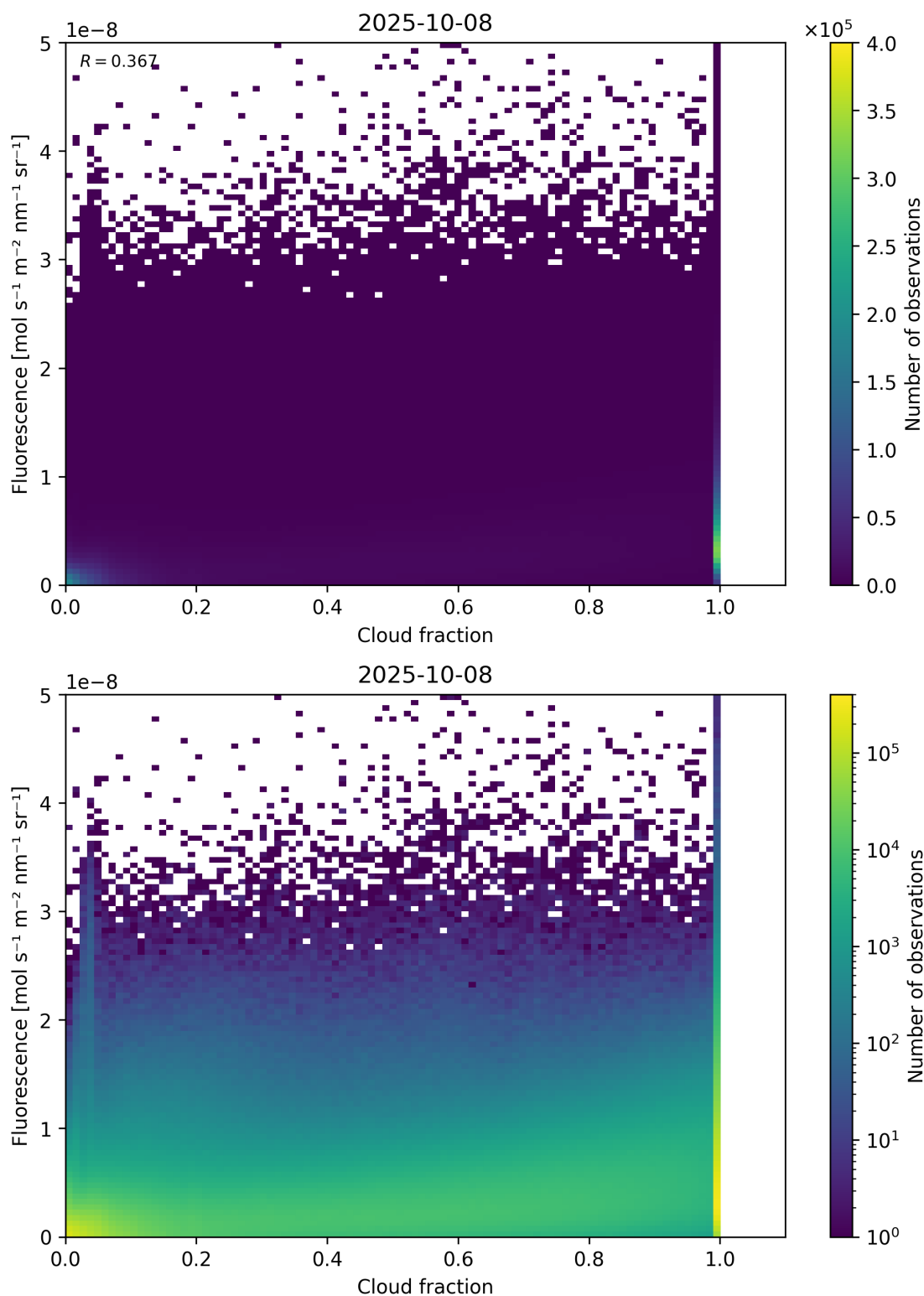
Figure 72: Scatter density plot of “Cloud fraction” against “Fluorescence” for 2025-10-07 to 2025-10-09.
