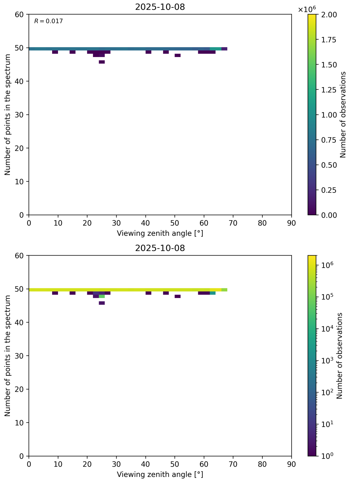
Figure 125: Scatter density plot of “Viewing zenith angle” against “Number of points in the spectrum” for 2025-10-07 to 2025-10-09.
