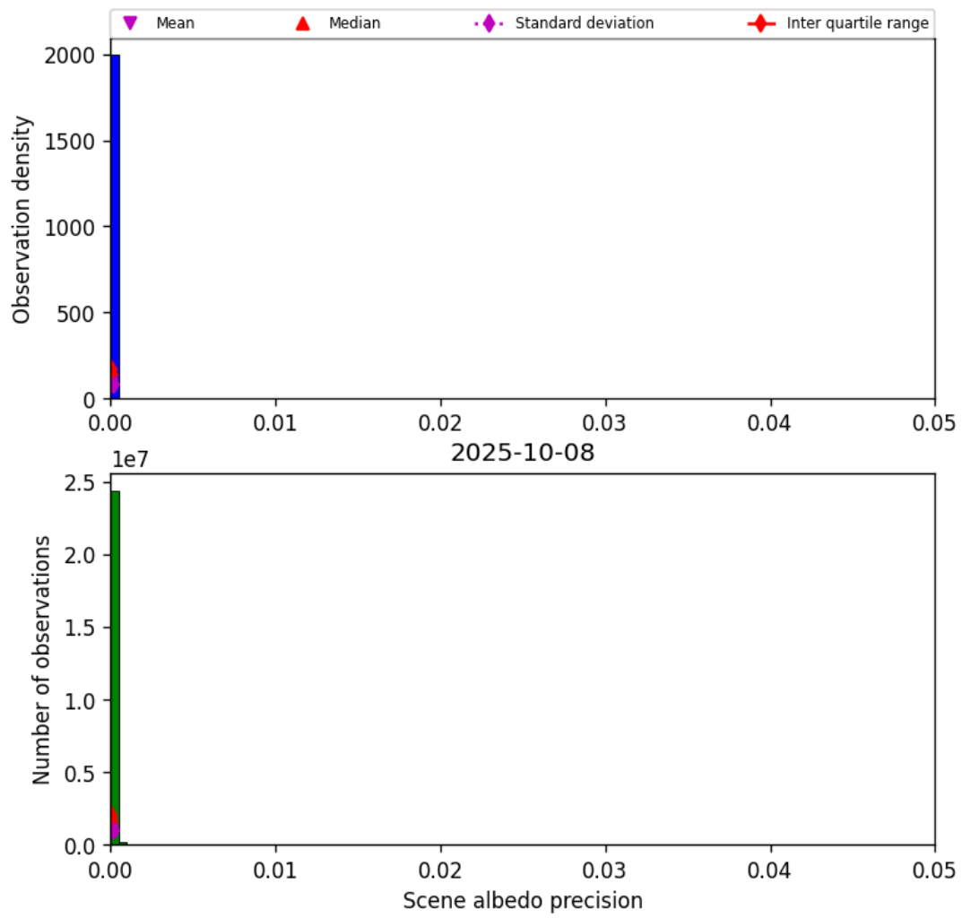
Figure 35: Histogram of “Scene albedo precision” for 2025-10-07 to 2025-10-09
