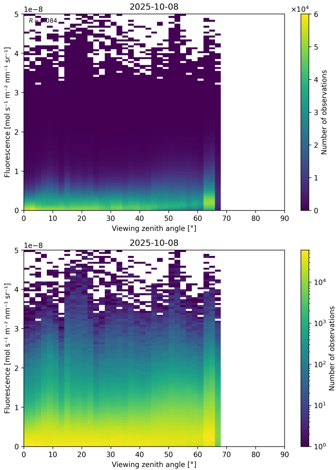
Figure 122: Scatter density plot of “Viewing zenith angle” against “Fluorescence” for 2025-10-07 to 2025-10-09.
