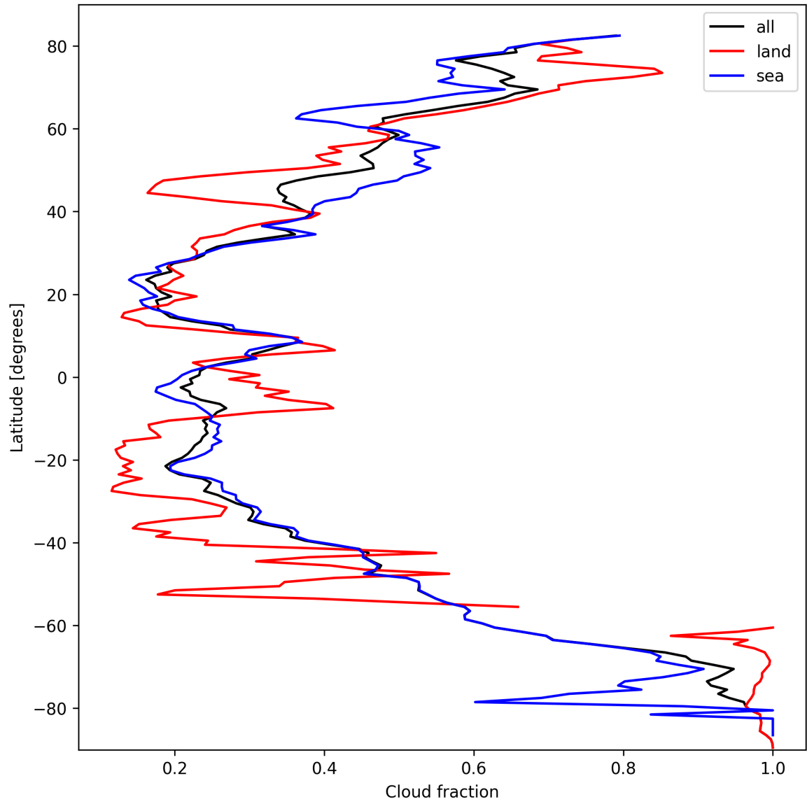
Figure 15: Zonal average of “Cloud fraction” for 2025-10-07 to 2025-10-09.
