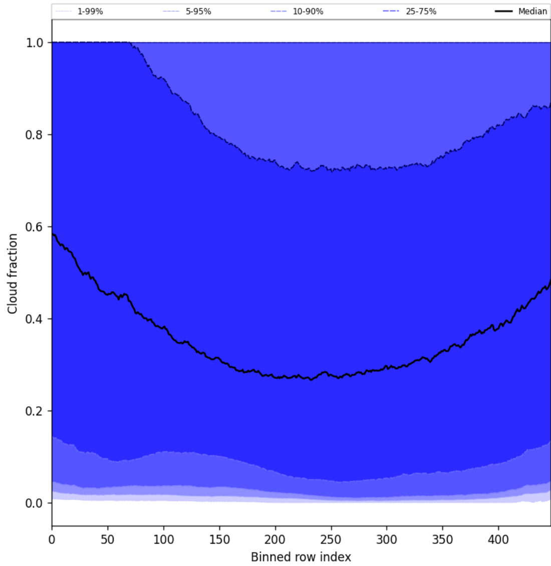
Figure 49: Along track statistics of “Cloud fraction” for 2025-10-07 to 2025-10-09
