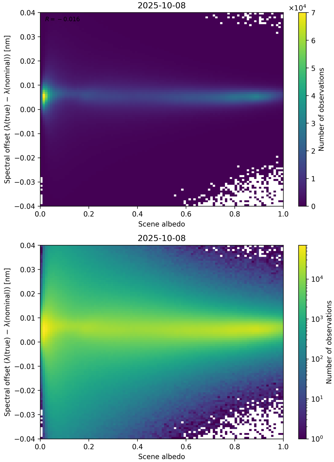
Figure 107: Scatter density plot of “Scene albedo” against “Spectral offset ( \lambda_{\text{true}} - \lambda_{\text{nominal}} )” for 2025-10-07 to 2025-10-09.
