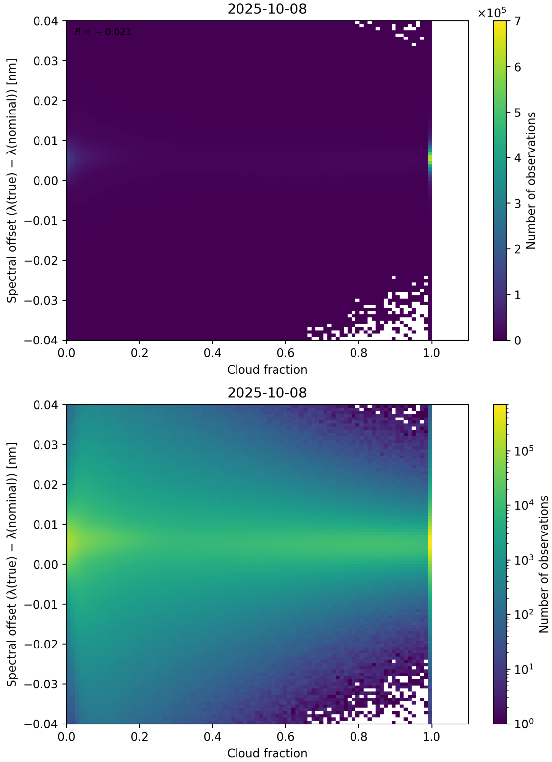
Figure 76: Scatter density plot of “Cloud fraction” against “Spectral offset ( \lambda_{\text{true}} - \lambda_{\text{nominal}} )” for 2025-10-07 to 2025-10-09.
