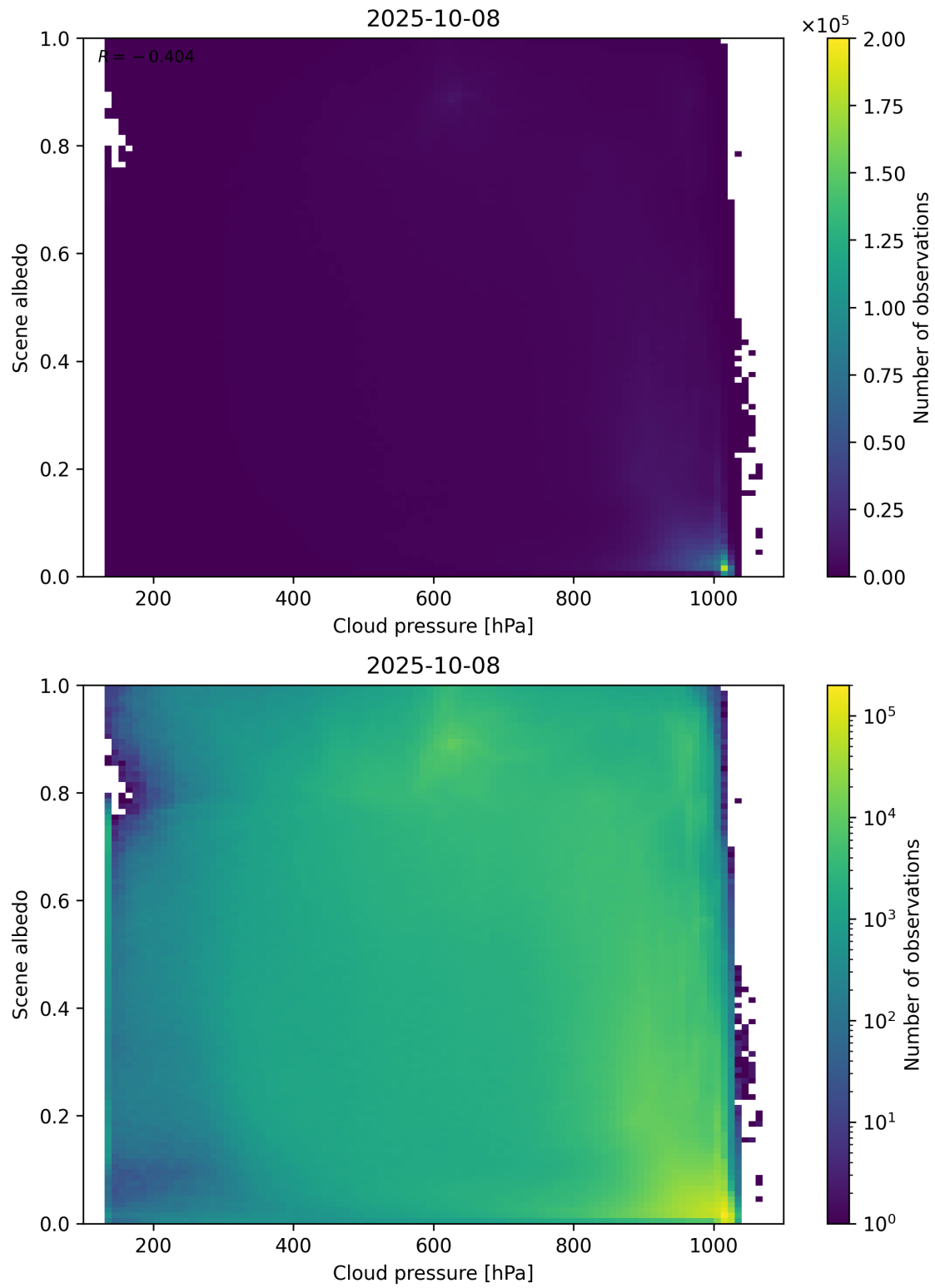
Figure 83: Scatter density plot of “Cloud pressure” against “Scene albedo” for 2025-10-07 to 2025-10-09.
