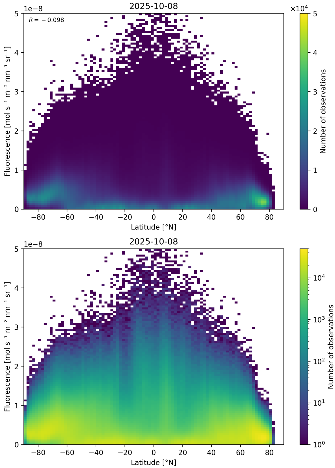
Figure 92: Scatter density plot of “Latitude” against “Fluorescence” for 2025-10-07 to 2025-10-09.
