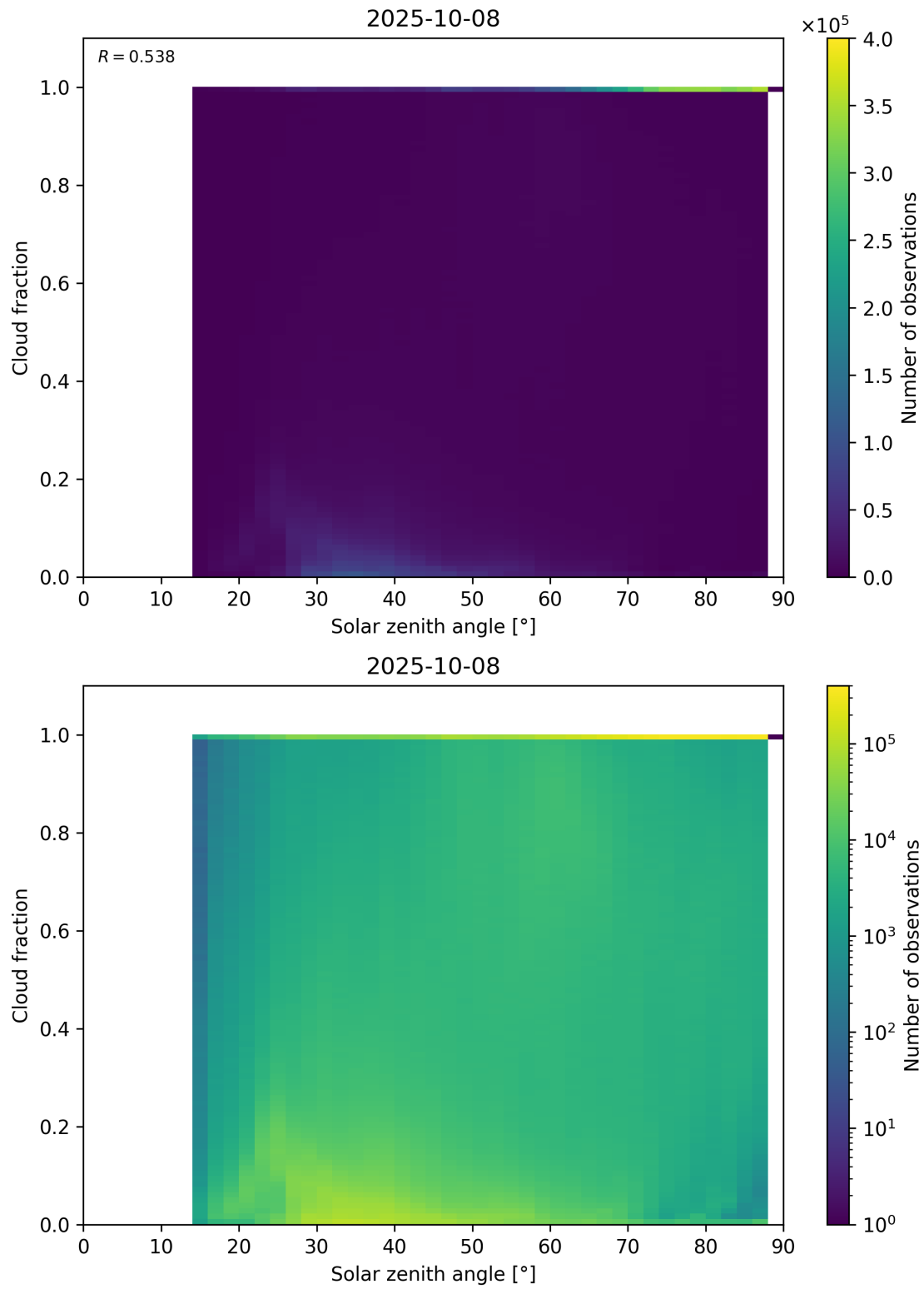
Figure 110: Scatter density plot of “Solar zenith angle” against “Cloud fraction” for 2025-10-07 to 2025-10-09.
