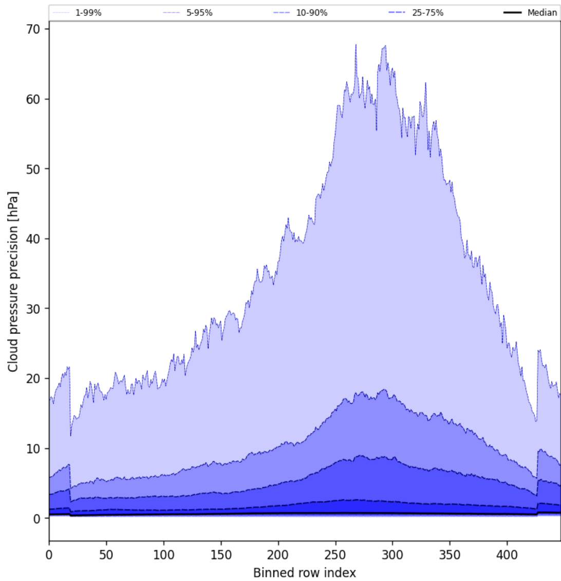
Figure 48: Along track statistics of “Cloud pressure precision” for 2025-10-07 to 2025-10-09
