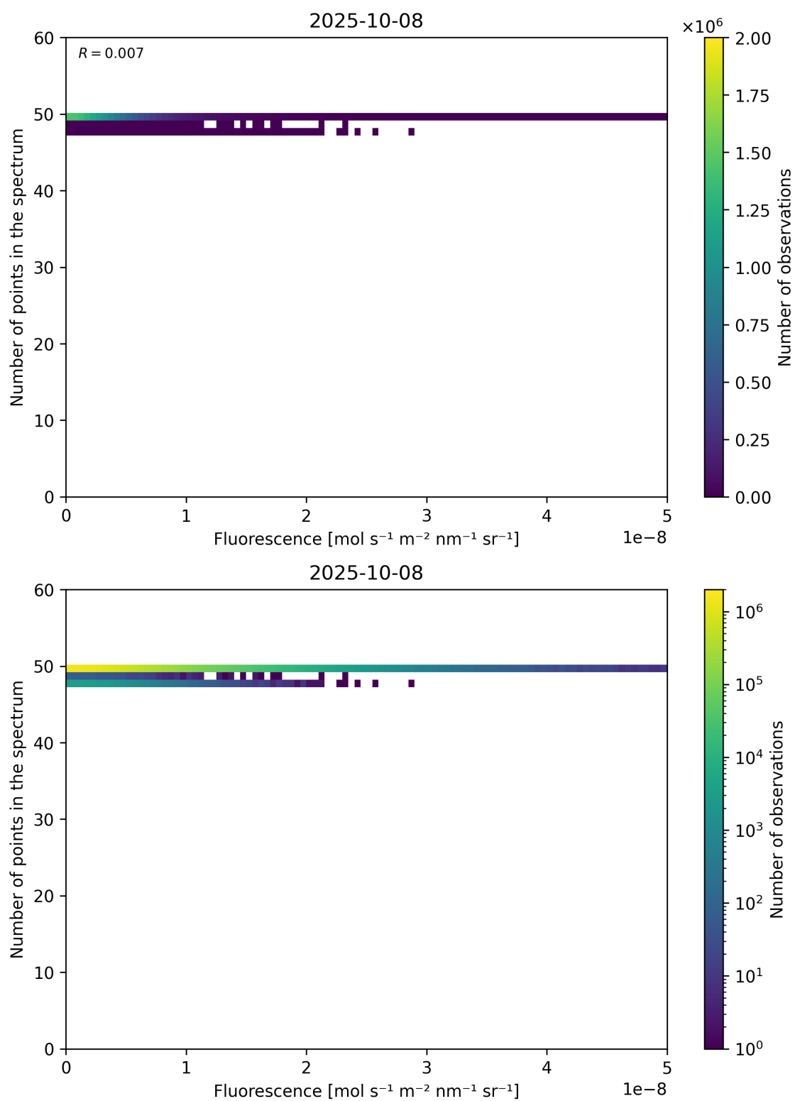
Figure 86: Scatter density plot of “Fluorescence” against “Number of points in the spectrum” for 2025-10-07 to 2025-10-09.
