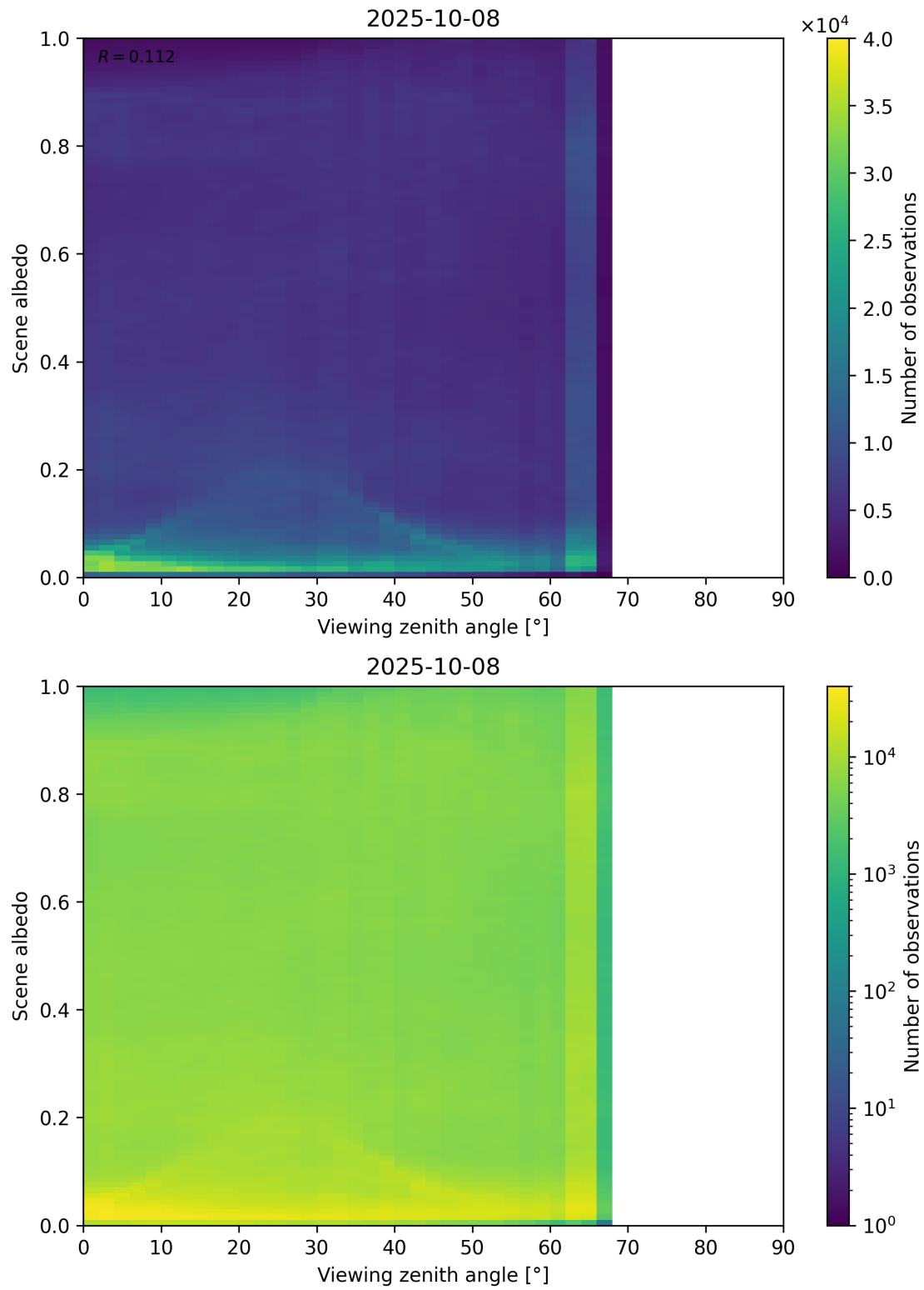
Figure 126: Scatter density plot of “Viewing zenith angle” against “Scene albedo” for 2025-10-07 to 2025-10-09.
