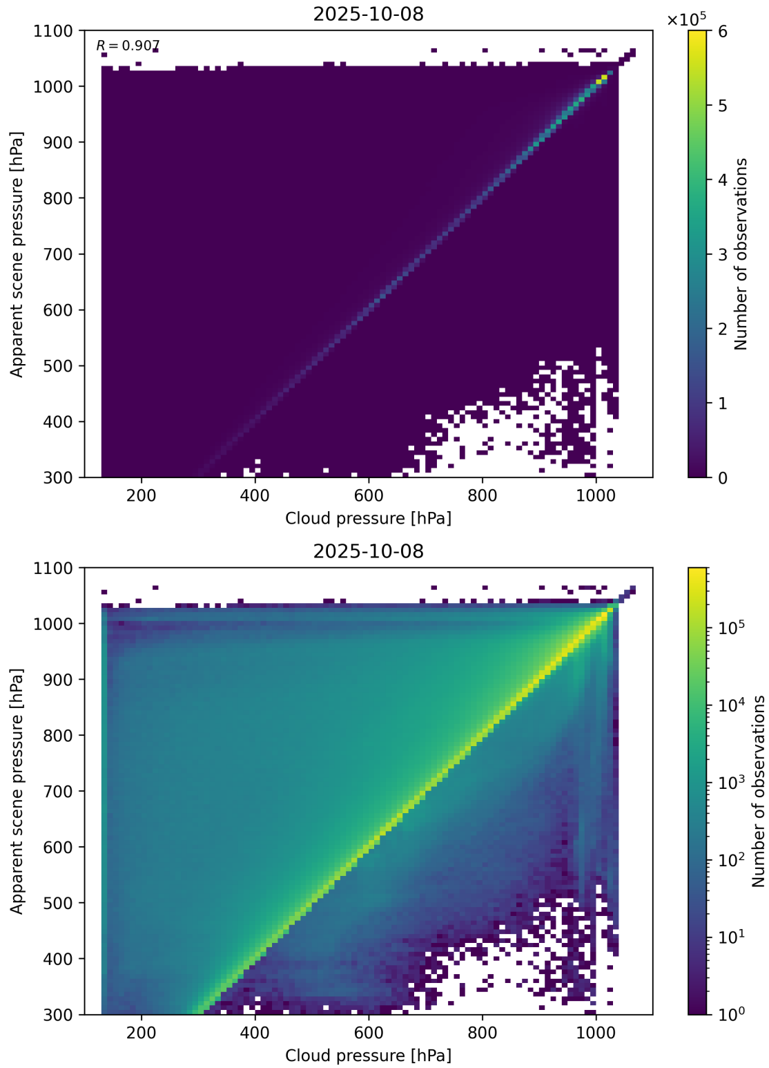
Figure 77: Scatter density plot of “Cloud pressure” against “Apparent scene pressure” for 2025-10-07 to 2025-10-09.
