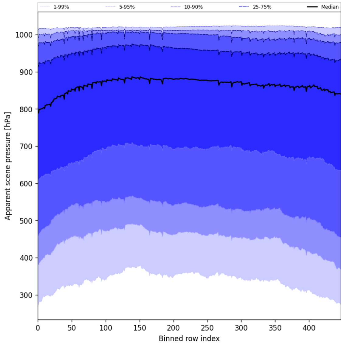
Figure 53: Along track statistics of “Apparent scene pressure” for 2025-10-07 to 2025-10-09
