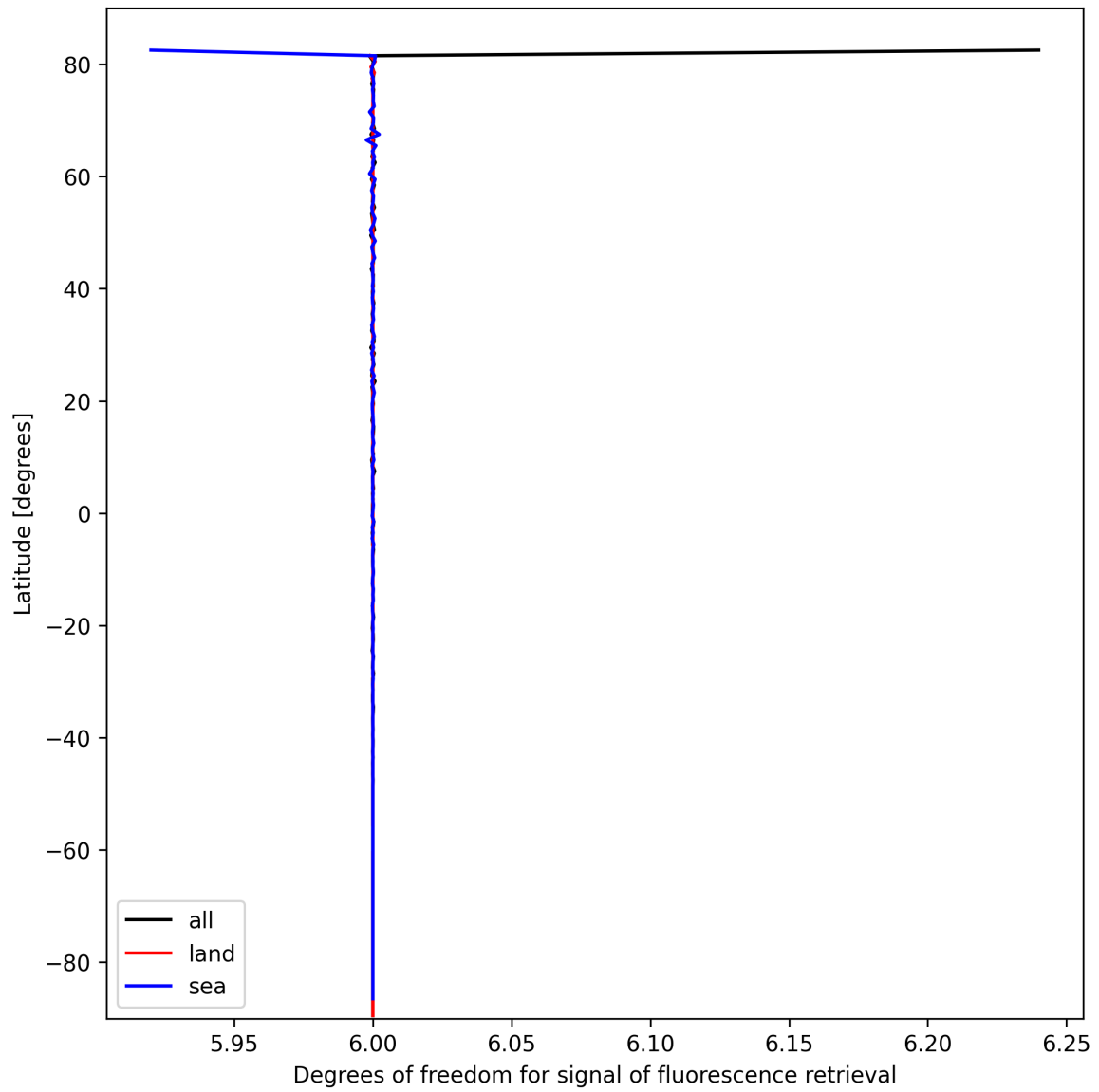
Figure 26: Zonal average of “Degrees of freedom for signal of fluorescence retrieval” for 2025-10-07 to 2025-10-09.
