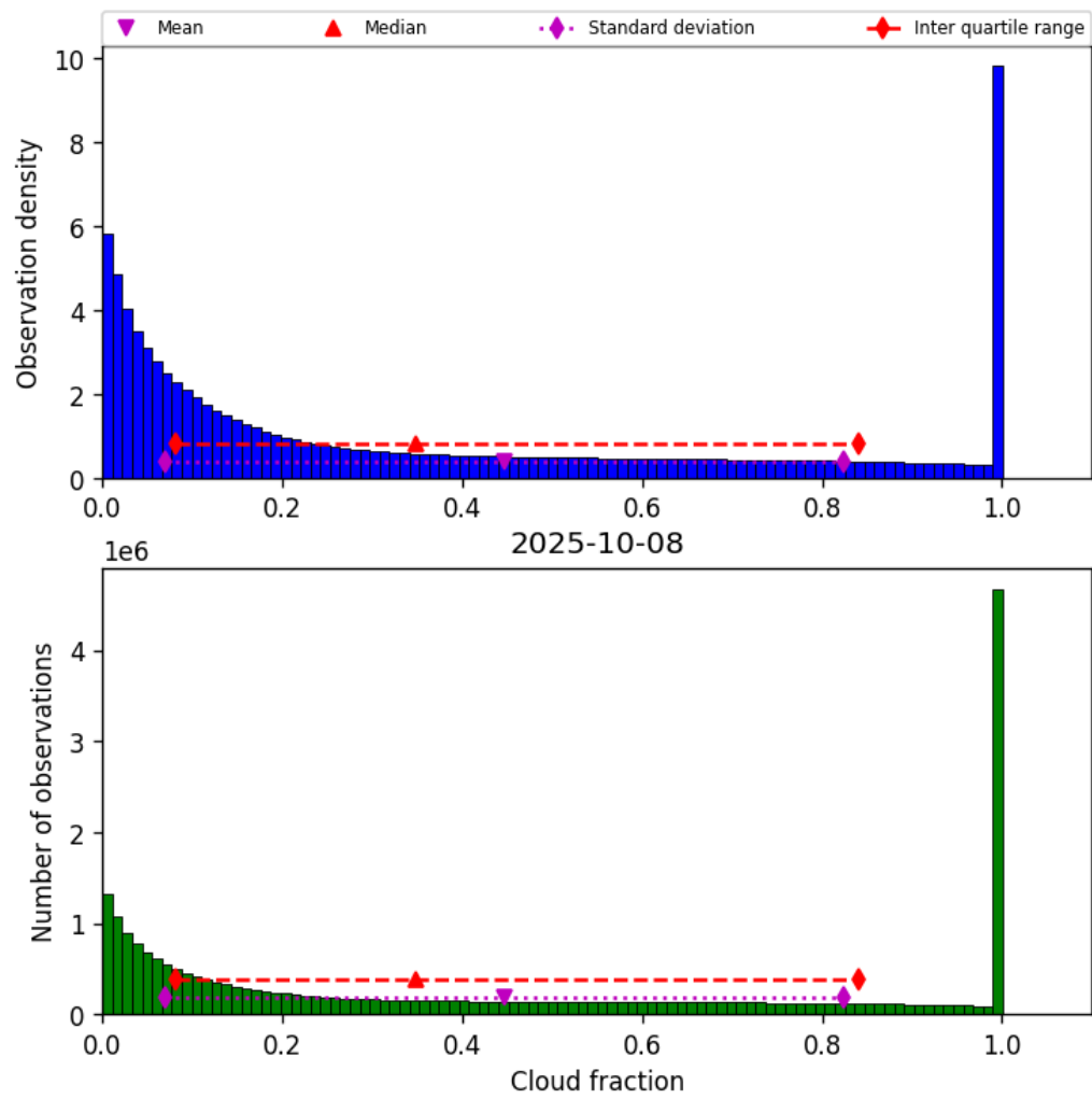
Figure 32: Histogram of “Cloud fraction” for 2025-10-07 to 2025-10-09
