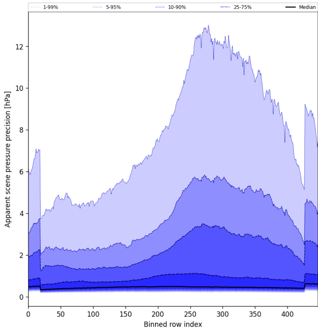
Figure 54: Along track statistics of “Apparent scene pressure precision” for 2025-10-07 to 2025-10-09
