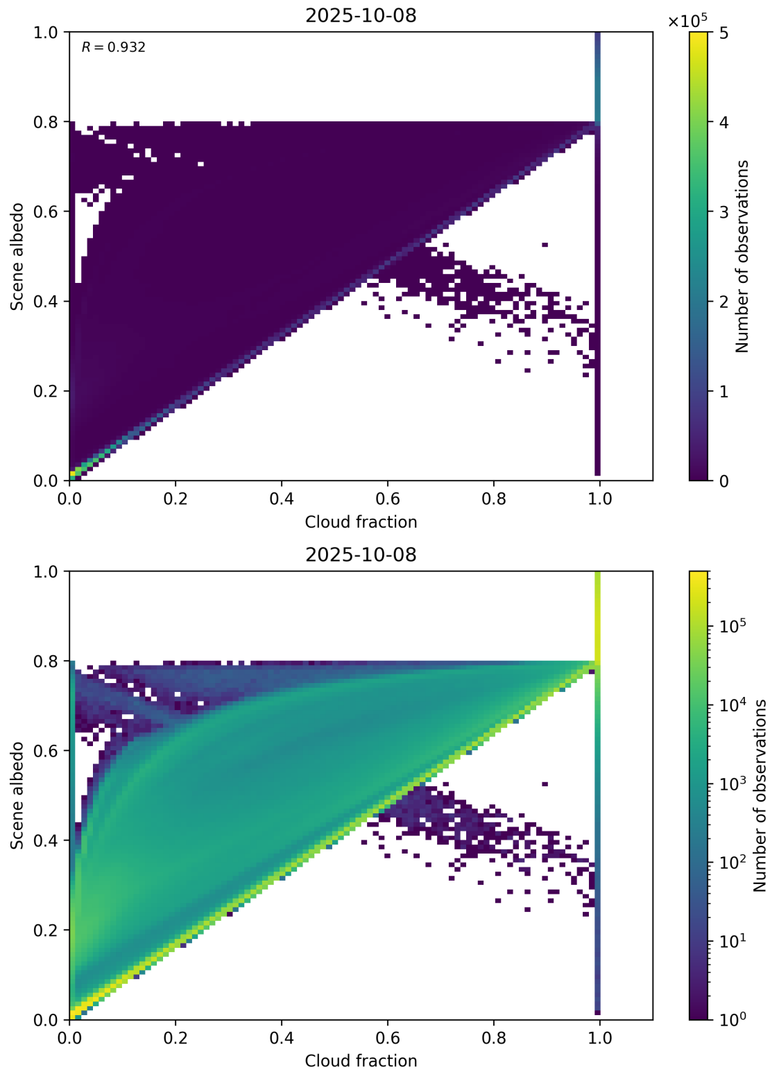
Figure 75: Scatter density plot of “Cloud fraction” against “Scene albedo” for 2025-10-07 to 2025-10-09.
