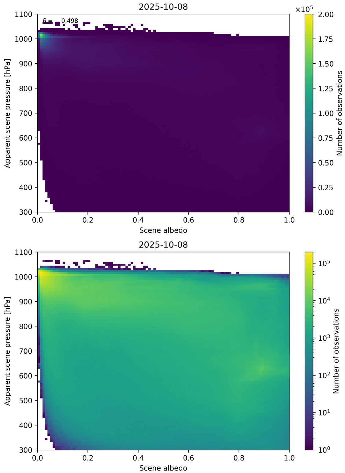
Figure 102: Scatter density plot of “Scene albedo” against “Apparent scene pressure” for 2025-10-07 to 2025-10-09.
