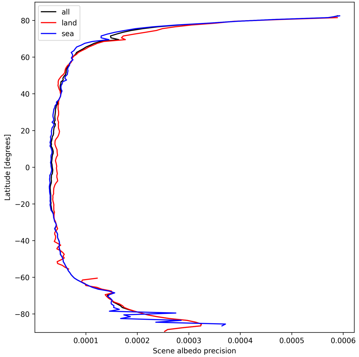
Figure 18: Zonal average of “Scene albedo precision” for 2025-10-07 to 2025-10-09.
