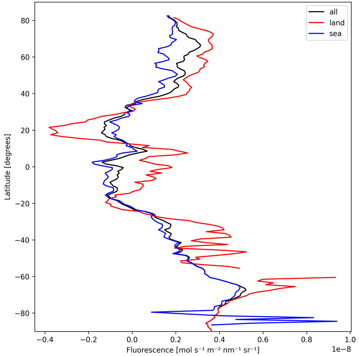
Figure 23: Zonal average of “Fluorescence” for 2025-10-07 to 2025-10-09.
