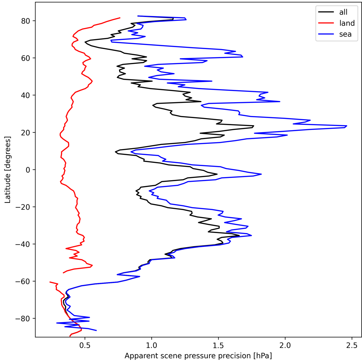
Figure 20: Zonal average of “Apparent scene pressure precision” for 2025-10-07 to 2025-10-09.
