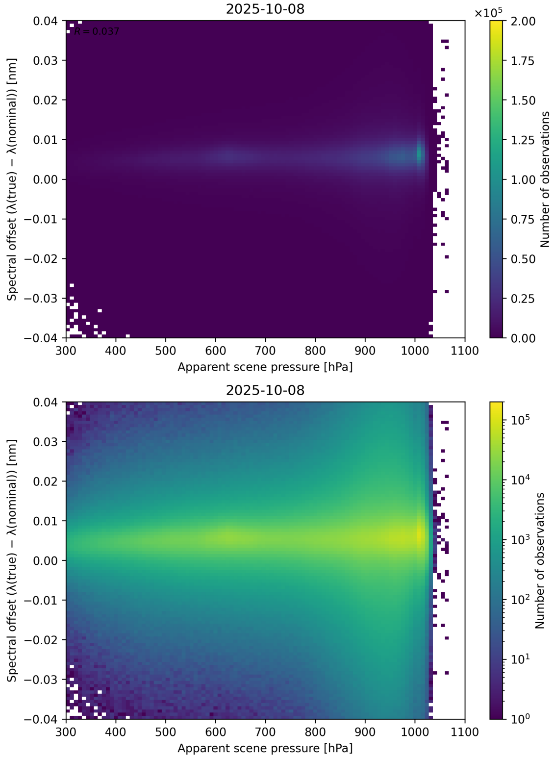
Figure 67: Scatter density plot of “Apparent scene pressure” against “Spectral offset ( \lambda_{\text{true}} - \lambda_{\text{nominal}} )” for 2025-10-07 to 2025-10-09.
