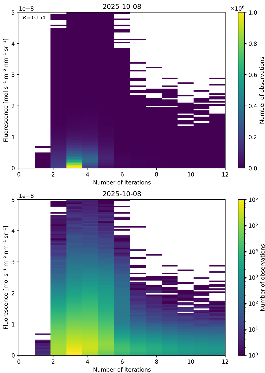
Figure 98: Scatter density plot of “Number of iterations” against “Fluorescence” for 2025-10-07 to 2025-10-09.
