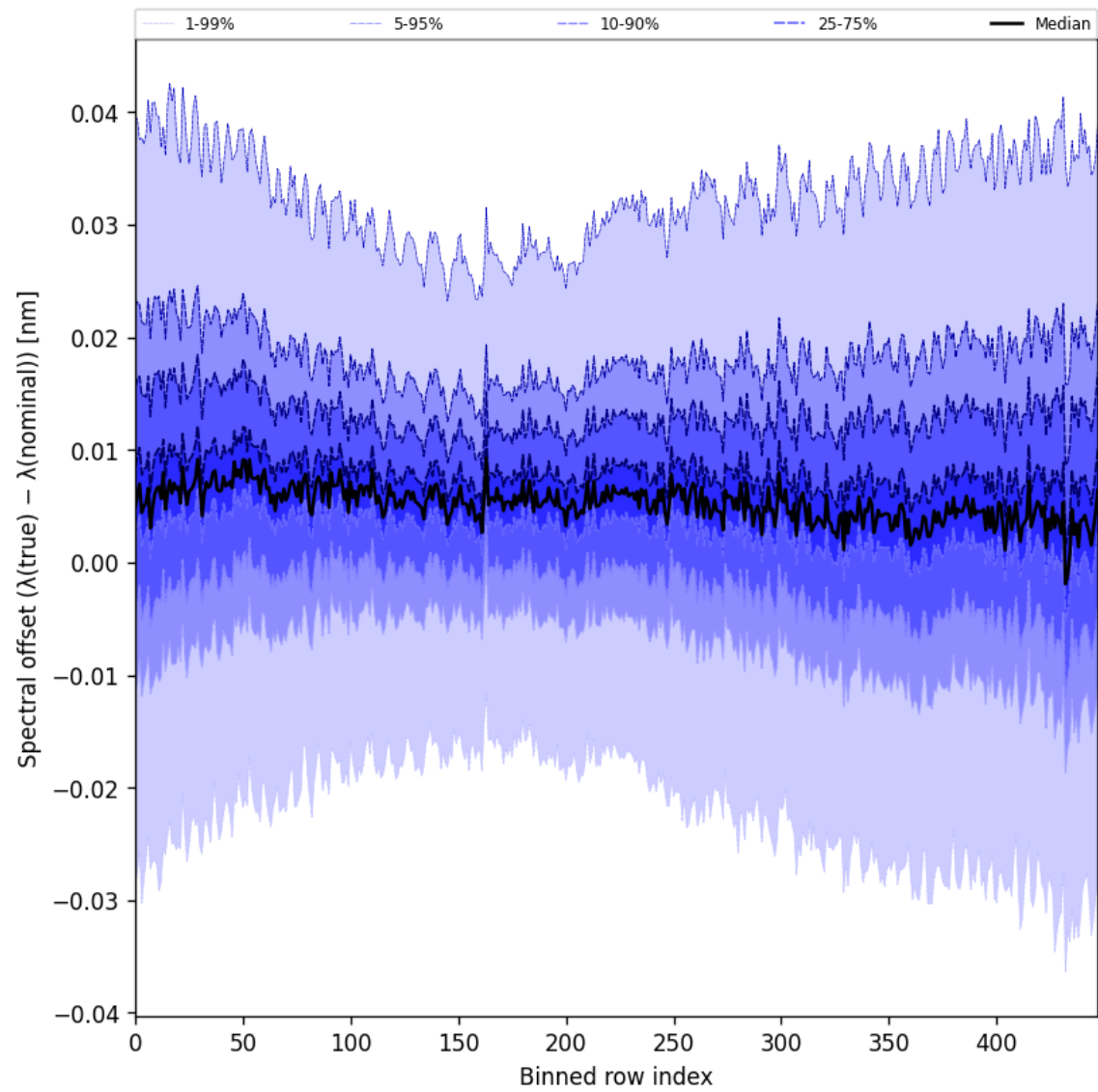
Figure 62: Along track statistics of “Spectral offset ( \lambda_{\text{true}} - \lambda_{\text{nominal}} )” for 2025-10-07 to 2025-10-09
