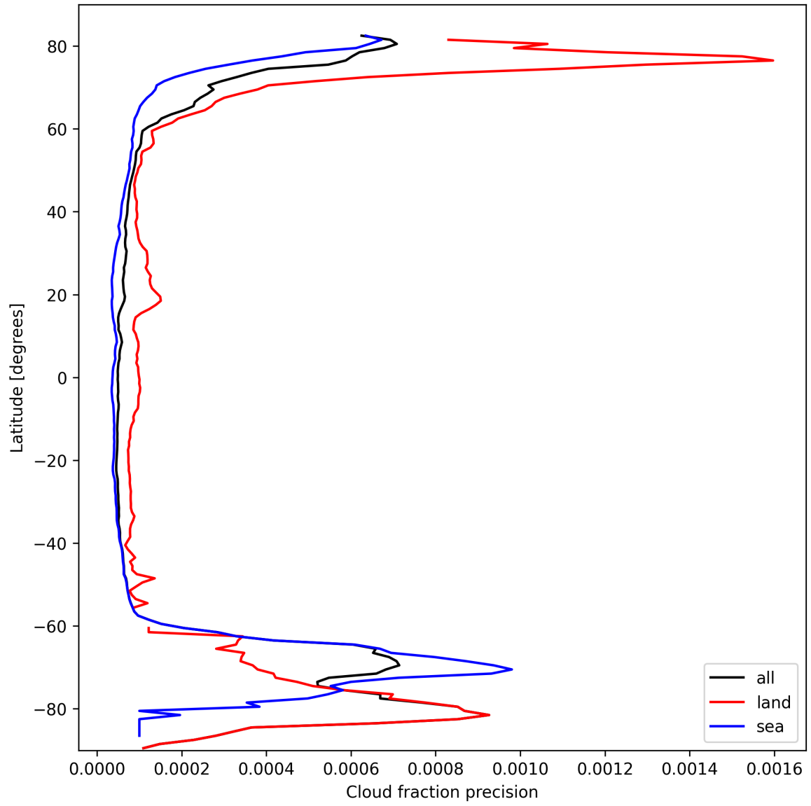
Figure 16: Zonal average of “Cloud fraction precision” for 2025-10-07 to 2025-10-09.
