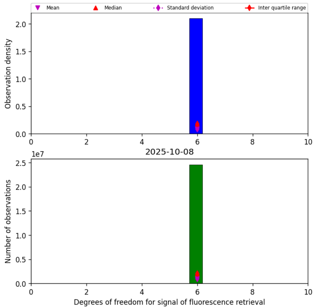
Figure 43: Histogram of "Degrees of freedom for signal of fluorescence retrieval" for 2025-10-07 to 2025-10-09
