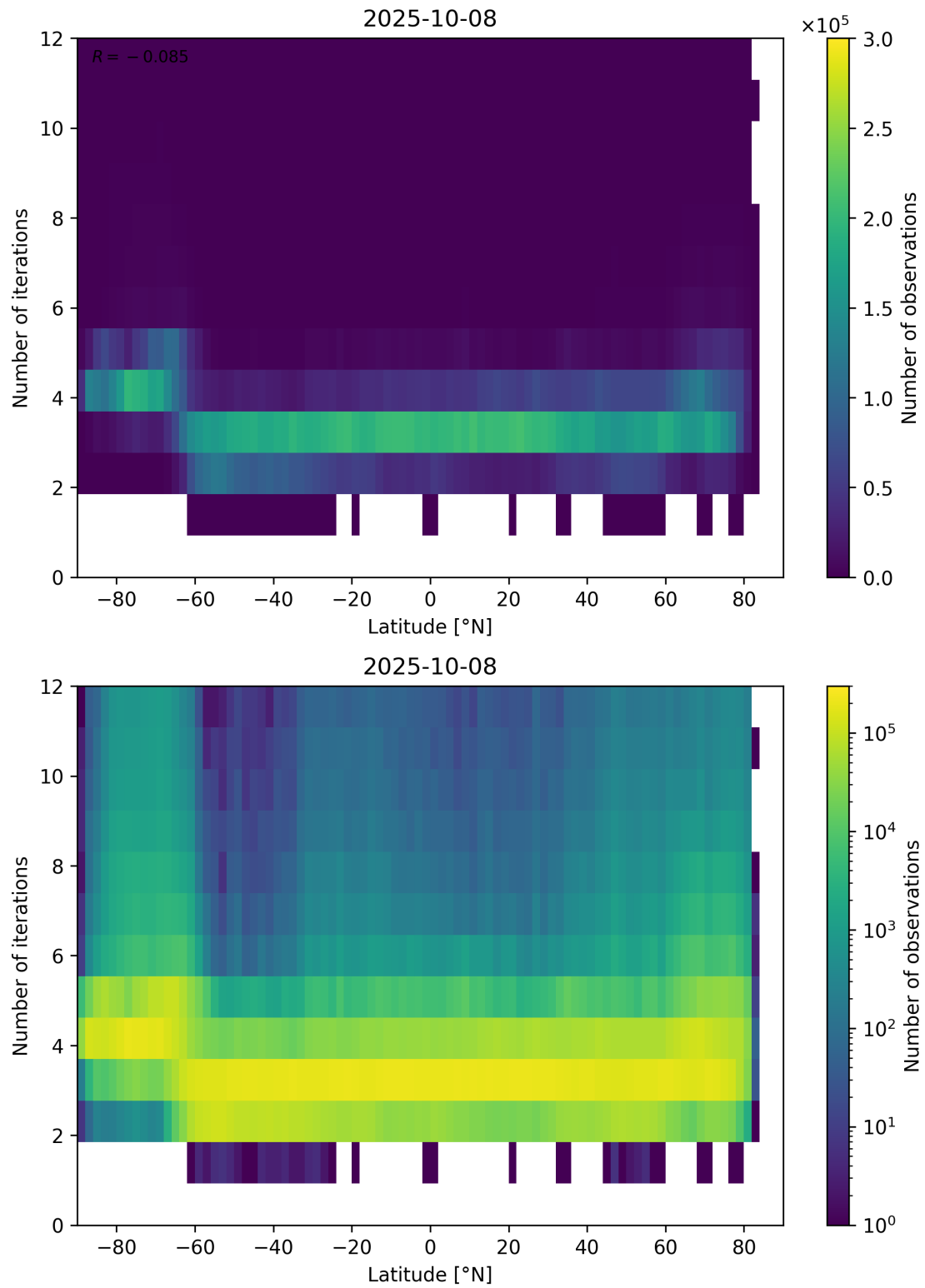
Figure 93: Scatter density plot of “Latitude” against “Number of iterations” for 2025-10-07 to 2025-10-09.
