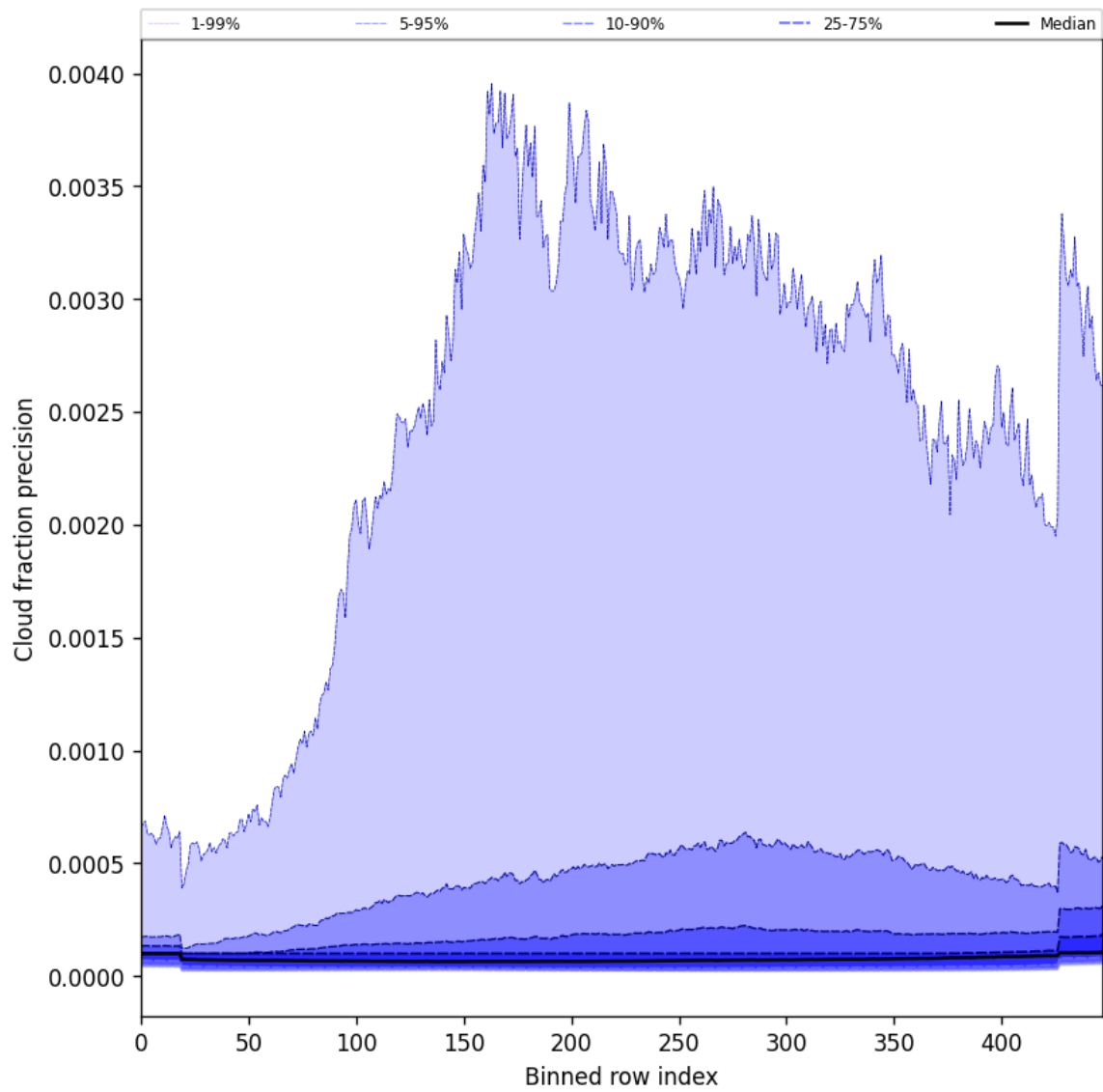
Figure 50: Along track statistics of “Cloud fraction precision” for 2025-10-07 to 2025-10-09
