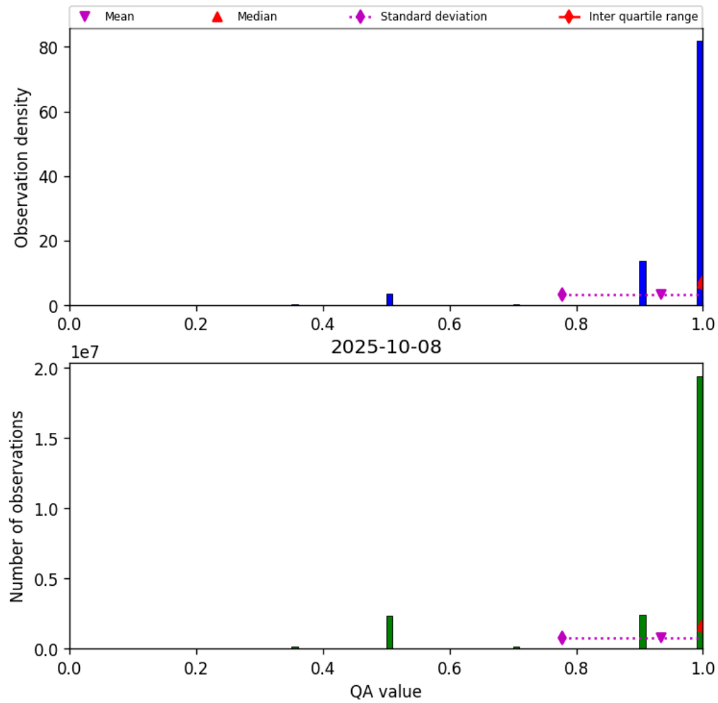
Figure 29: Histogram of "QA value" for 2025-10-07 to 2025-10-09
