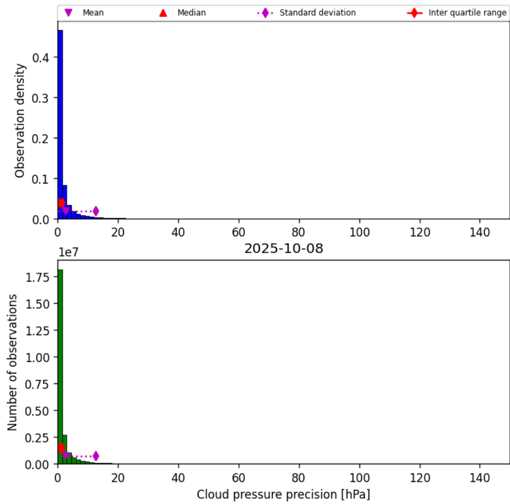
Figure 31: Histogram of “Cloud pressure precision” for 2025-10-07 to 2025-10-09
