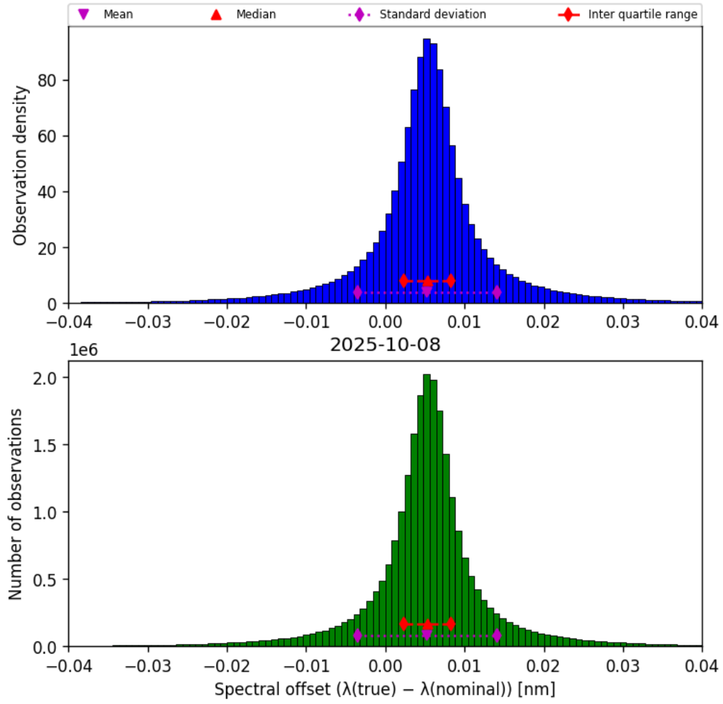
Figure 45: Histogram of “Spectral offset ( \lambda_{\text{true}} - \lambda_{\text{nominal}} )” for 2025-10-07 to 2025-10-09
