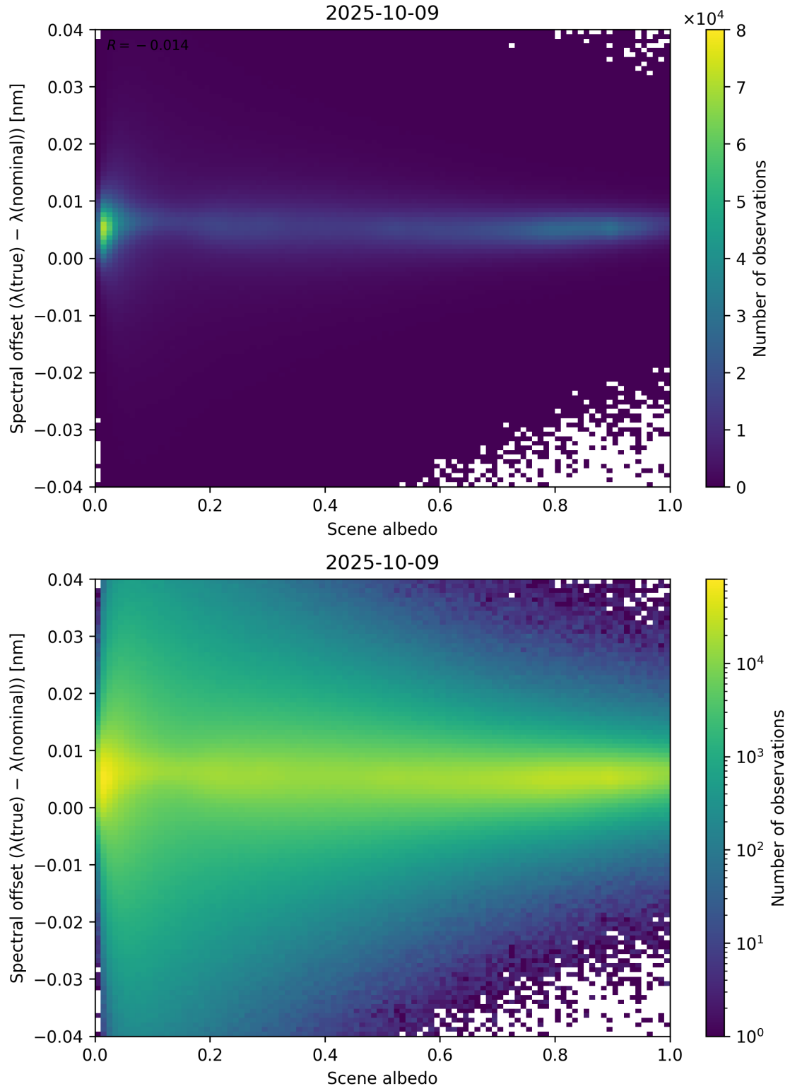
Figure 107: Scatter density plot of “Scene albedo” against “Spectral offset ( \lambda_{\text{true}} - \lambda_{\text{nominal}} )” for 2025-10-08 to 2025-10-10.
