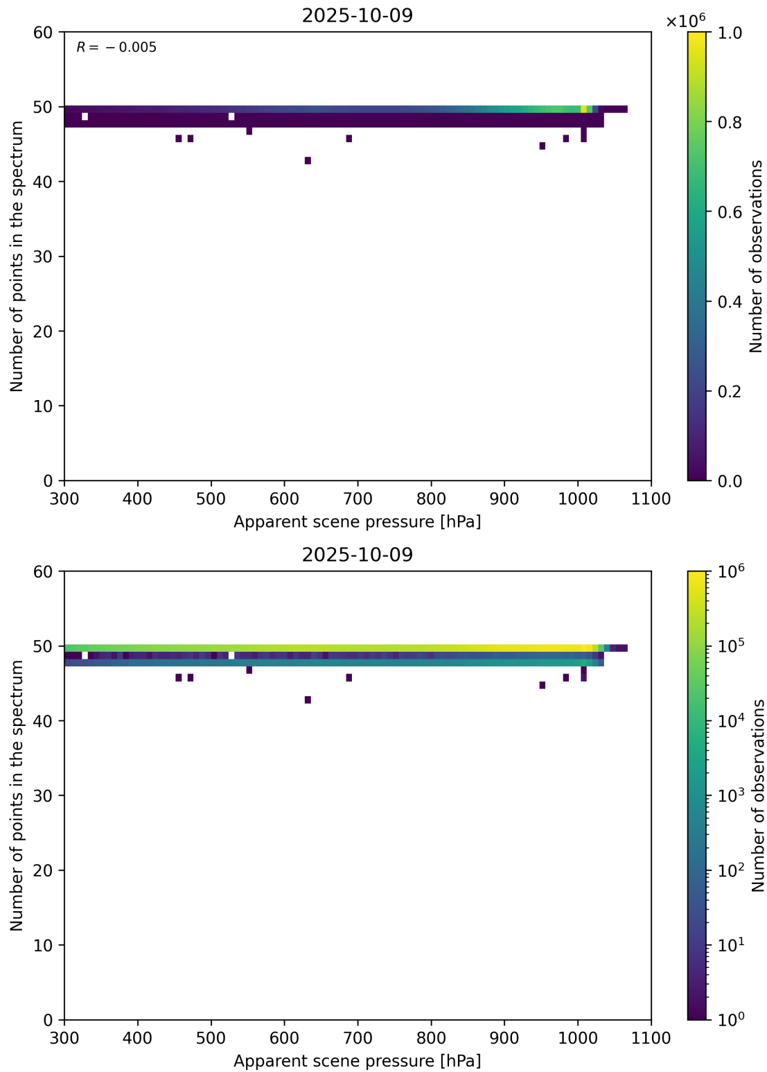
Figure 66: Scatter density plot of “Apparent scene pressure” against “Number of points in the spectrum” for 2025-10-08 to 2025-10-10.
