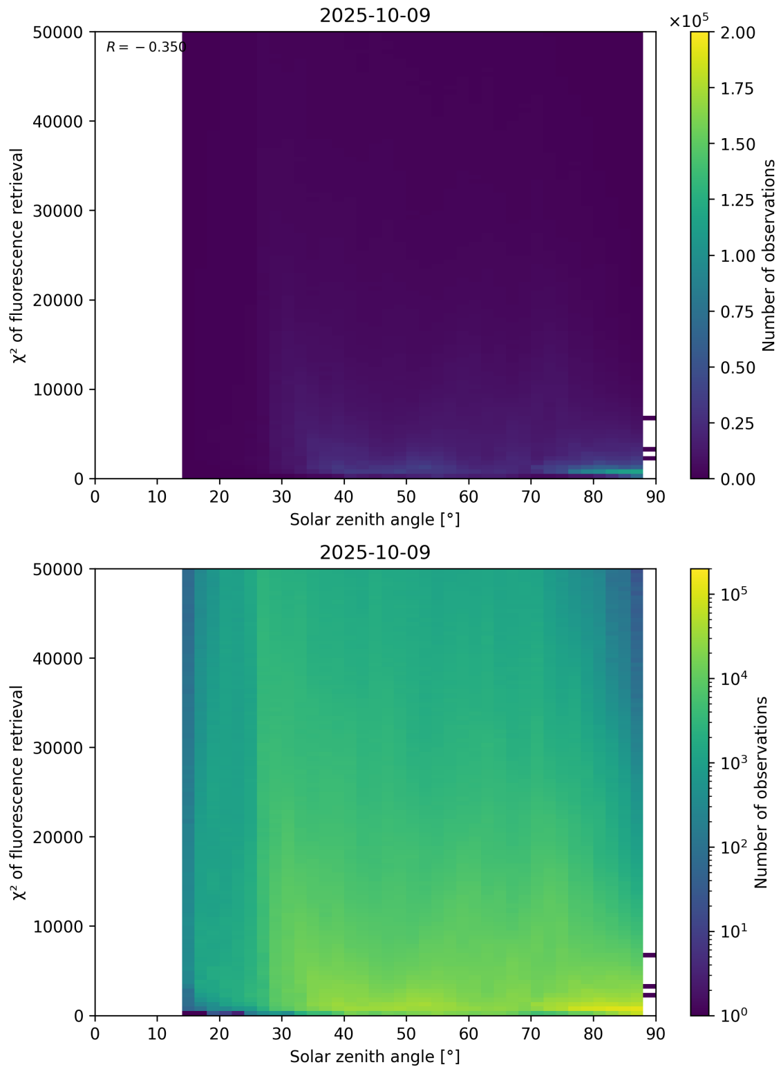
Figure 109: Scatter density plot of “Solar zenith angle” against “ \chi^2 of fluorescence retrieval” for 2025-10-08 to 2025-10-10.
