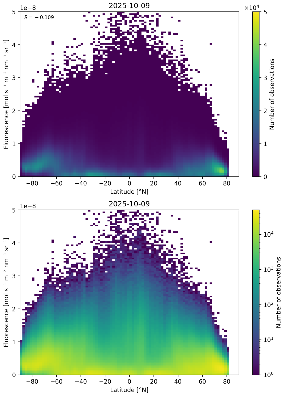
Figure 92: Scatter density plot of “Latitude” against “Fluorescence” for 2025-10-08 to 2025-10-10.
