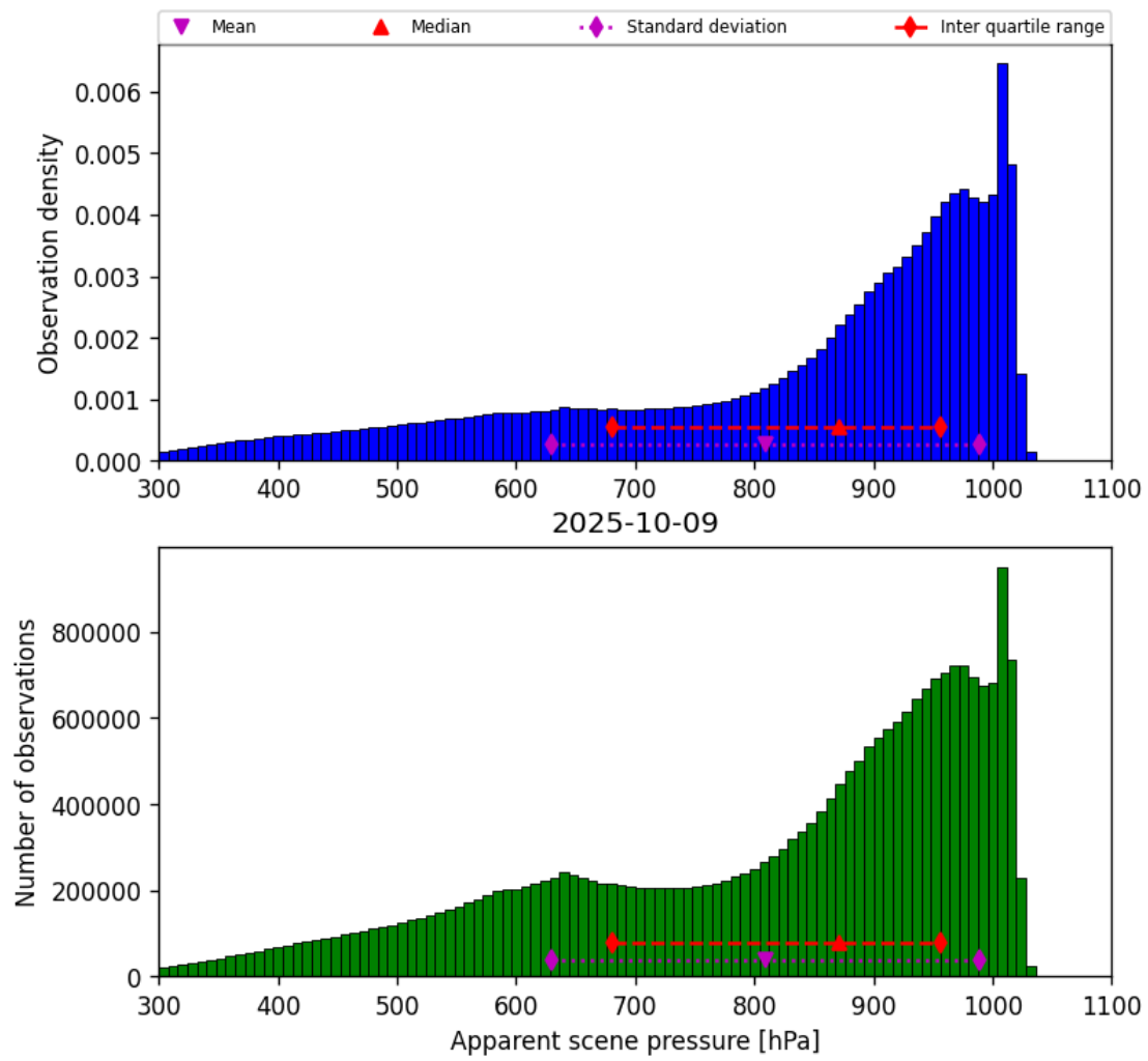
Figure 36: Histogram of “Apparent scene pressure” for 2025-10-08 to 2025-10-10
