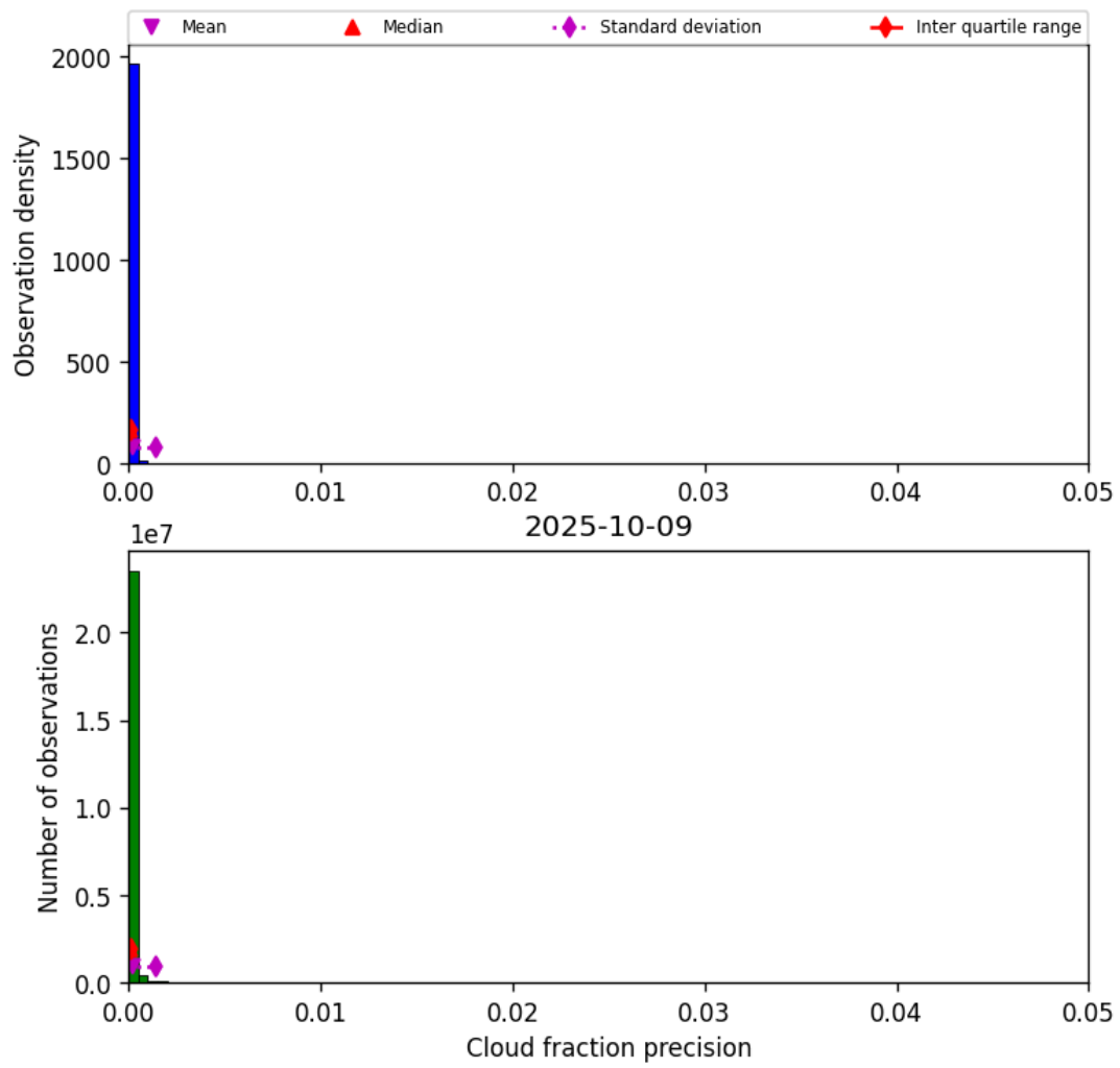
Figure 33: Histogram of “Cloud fraction precision” for 2025-10-08 to 2025-10-10
