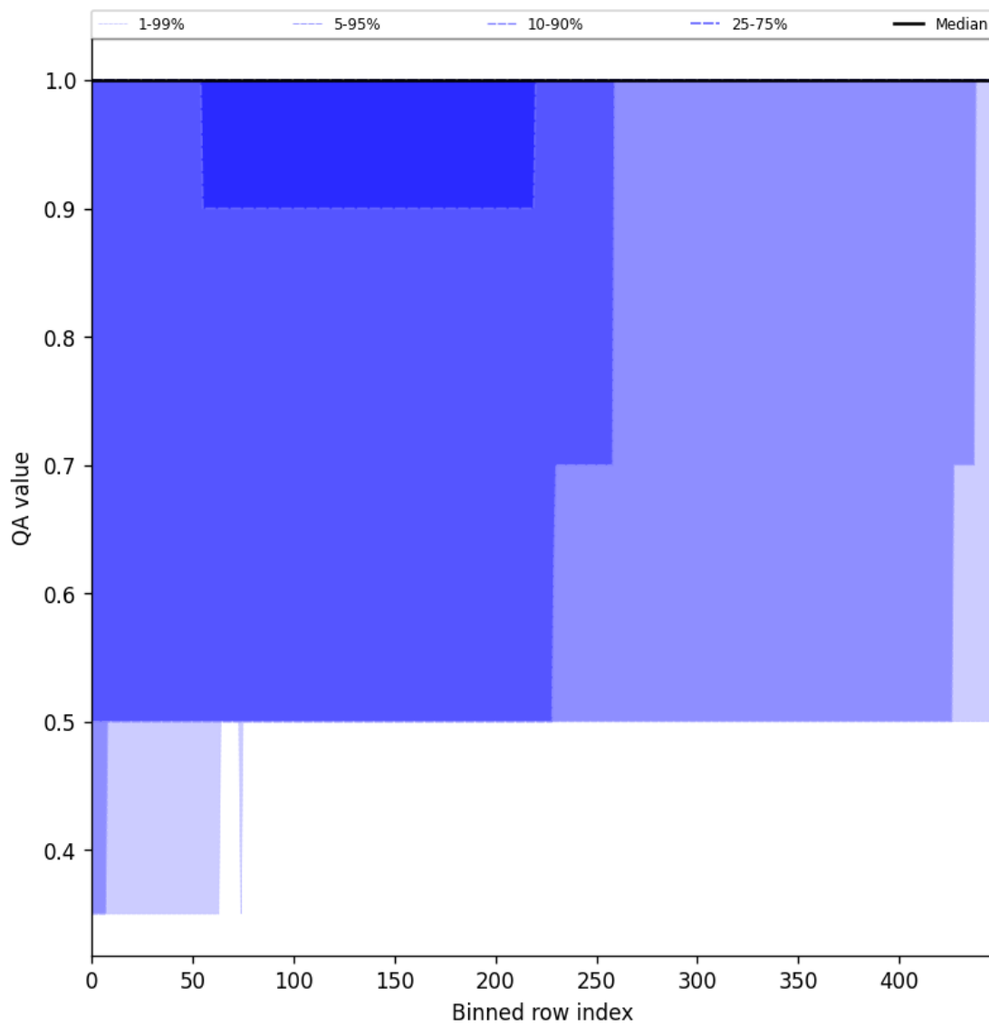
Figure 46: Along track statistics of “QA value” for 2025-10-08 to 2025-10-10
