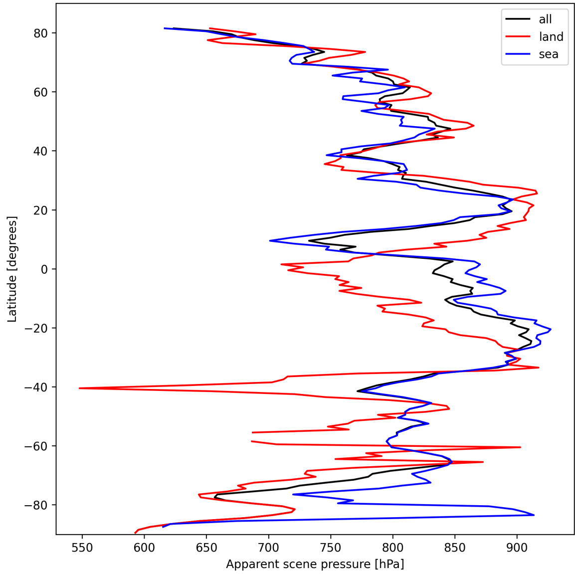
Figure 19: Zonal average of “Apparent scene pressure” for 2025-10-08 to 2025-10-10.
