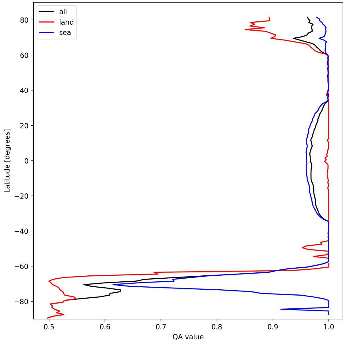
Figure 12: Zonal average of “QA value” for 2025-10-08 to 2025-10-10.
