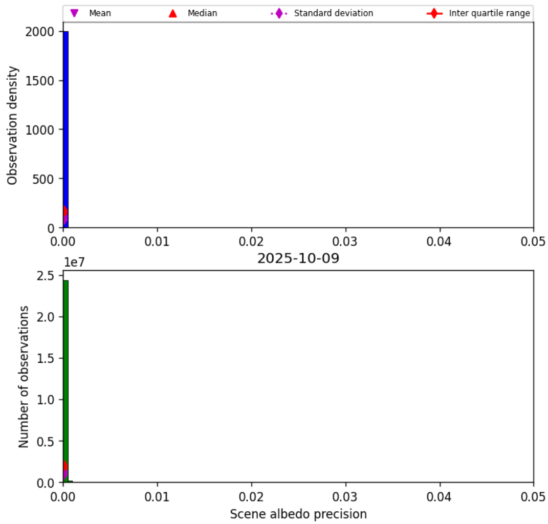
Figure 35: Histogram of “Scene albedo precision” for 2025-10-08 to 2025-10-10
