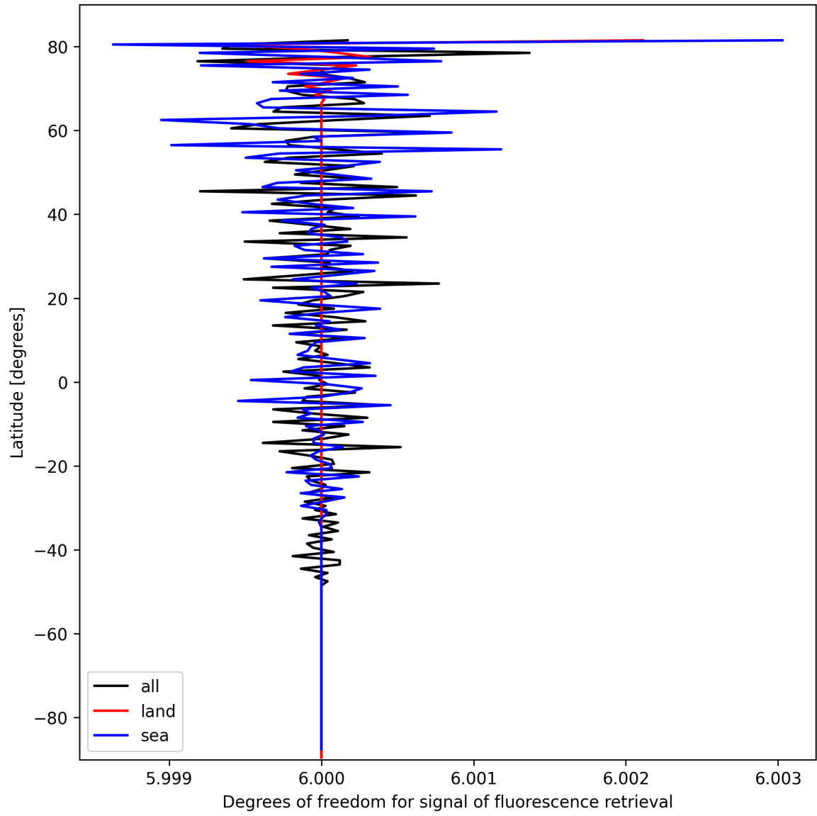
Figure 26: Zonal average of “Degrees of freedom for signal of fluorescence retrieval” for 2025-10-08 to 2025-10-10.
