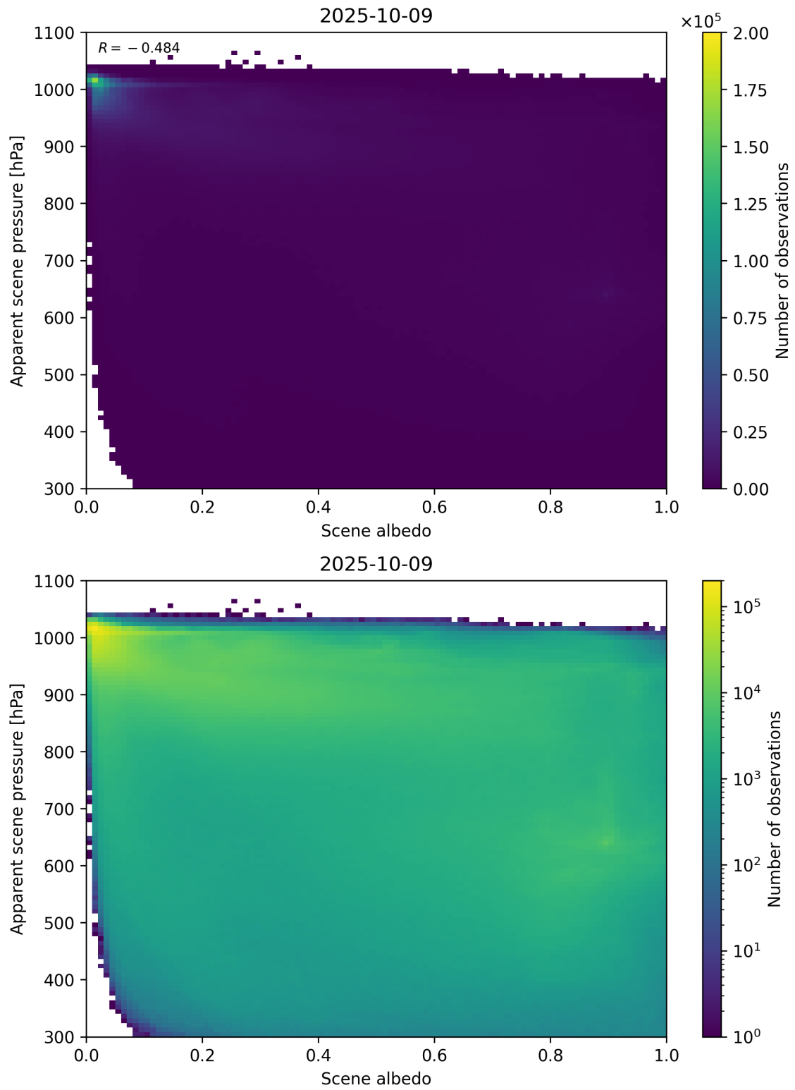
Figure 102: Scatter density plot of “Scene albedo” against “Apparent scene pressure” for 2025-10-08 to 2025-10-10.
