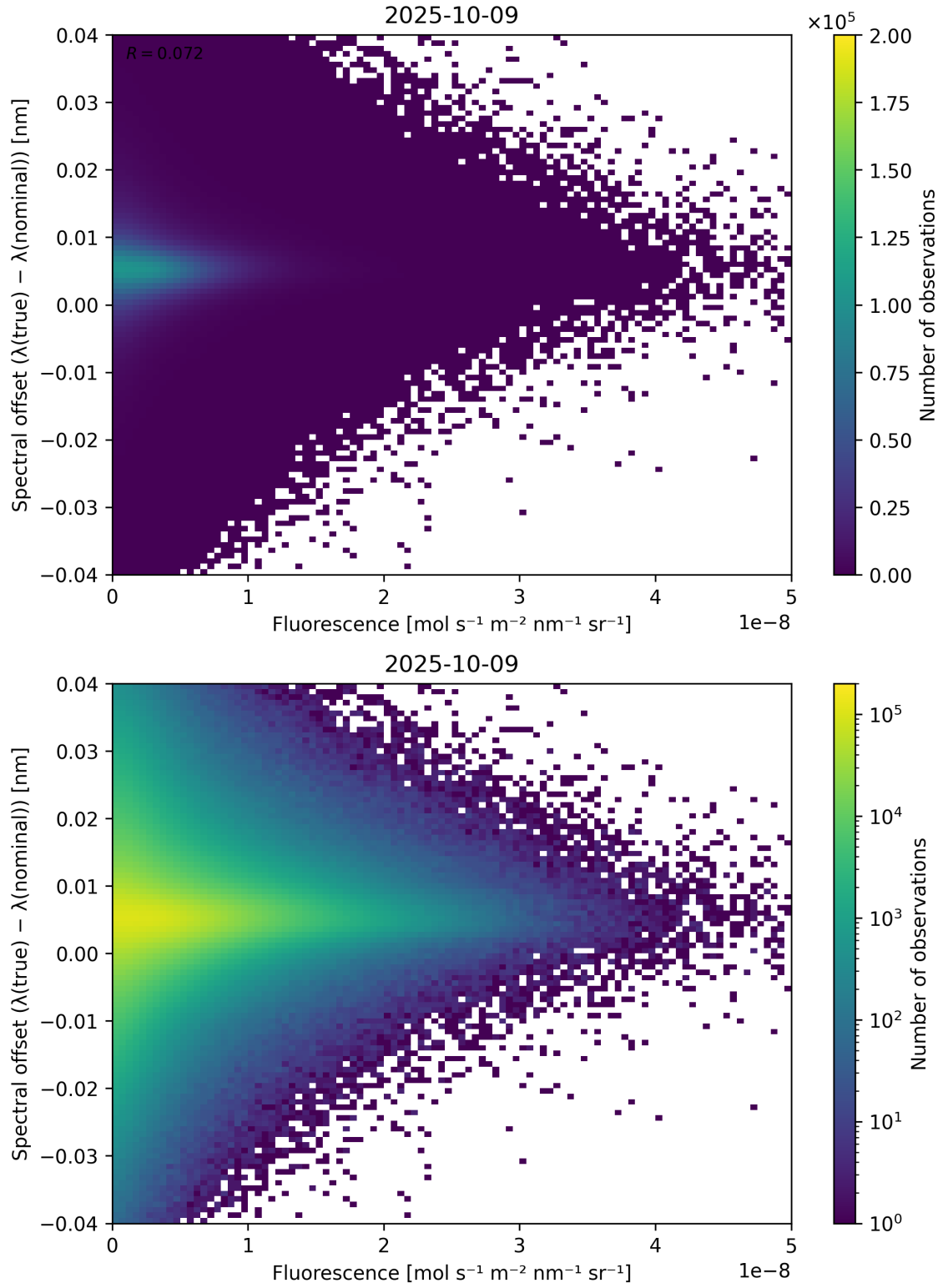
Figure 87: Scatter density plot of “Fluorescence” against “Spectral offset ( \lambda_{\text{true}} - \lambda_{\text{nominal}} )” for 2025-10-08 to 2025-10-10.
