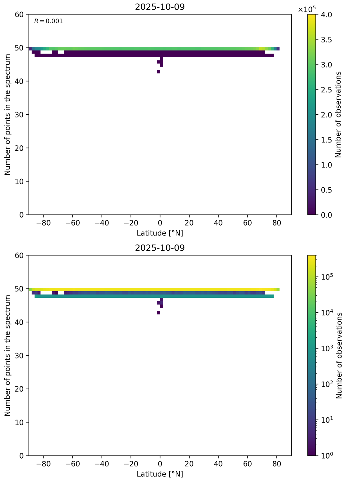
Figure 94: Scatter density plot of “Latitude” against “Number of points in the spectrum” for 2025-10-08 to 2025-10-10.
