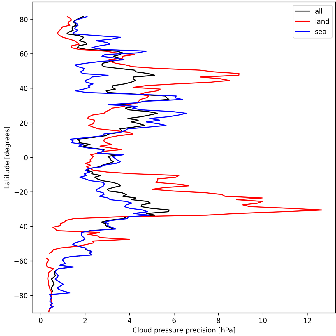
Figure 14: Zonal average of “Cloud pressure precision” for 2025-10-08 to 2025-10-10.
