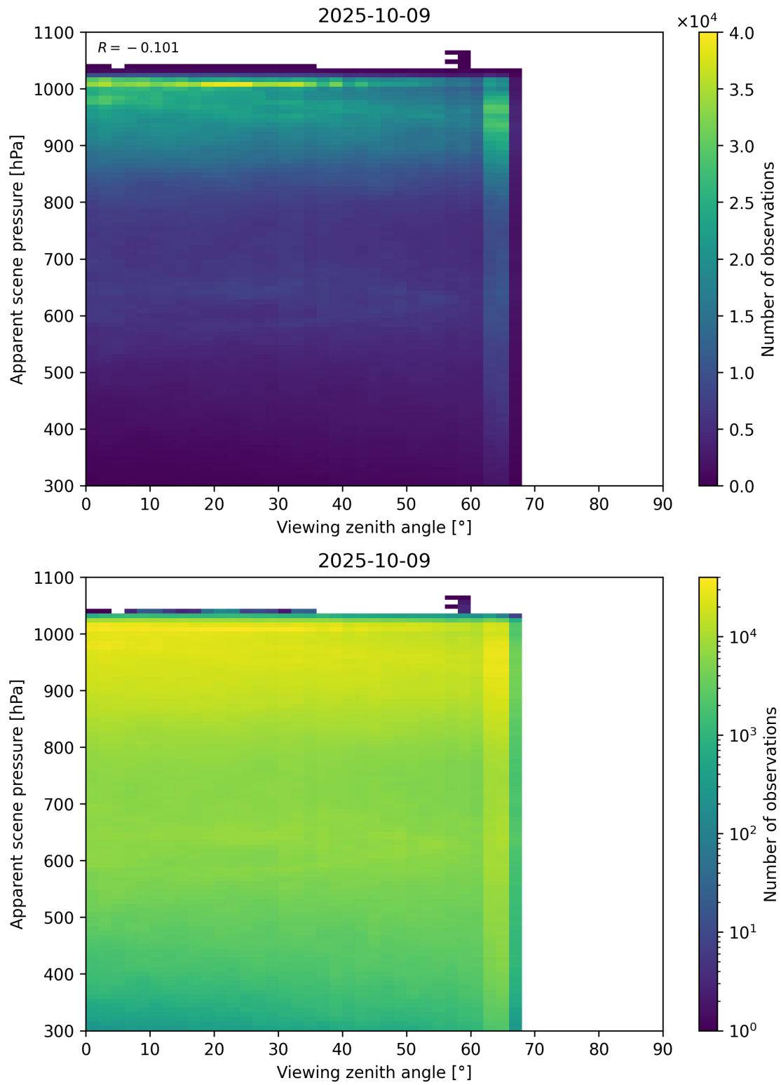
Figure 118: Scatter density plot of “Viewing zenith angle” against “Apparent scene pressure” for 2025-10-08 to 2025-10-10.
