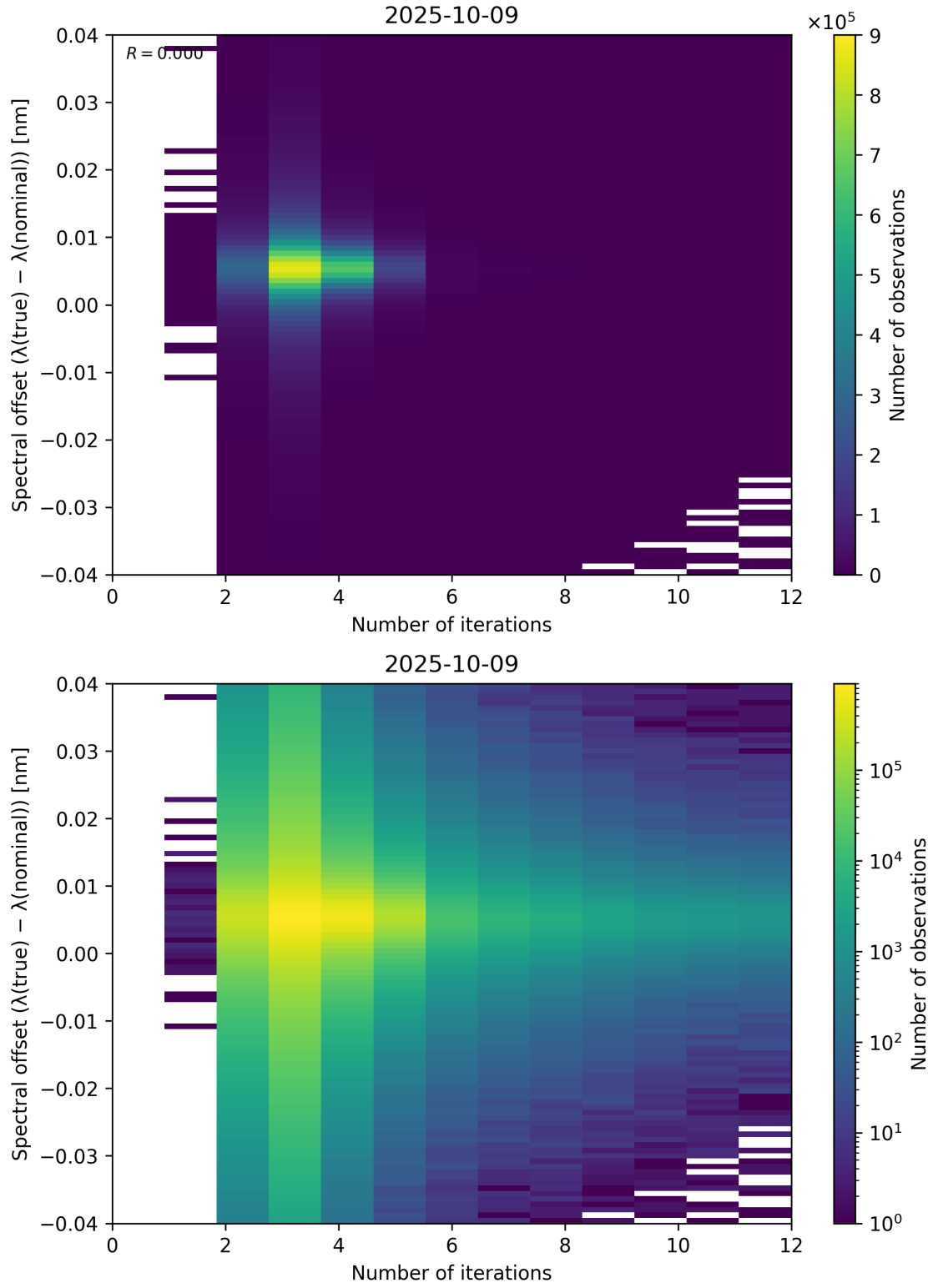
Figure 100: Scatter density plot of “Number of iterations” against “Spectral offset ( \lambda_{\text{true}} - \lambda_{\text{nominal}} )” for 2025-10-08 to 2025-10-10.
