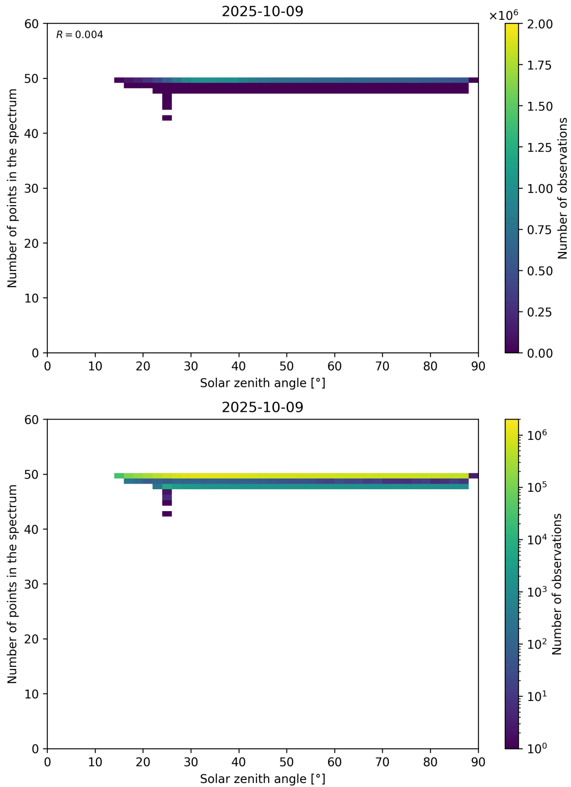
Figure 115: Scatter density plot of “Solar zenith angle” against “Number of points in the spectrum” for 2025-10-08 to 2025-10-10.
