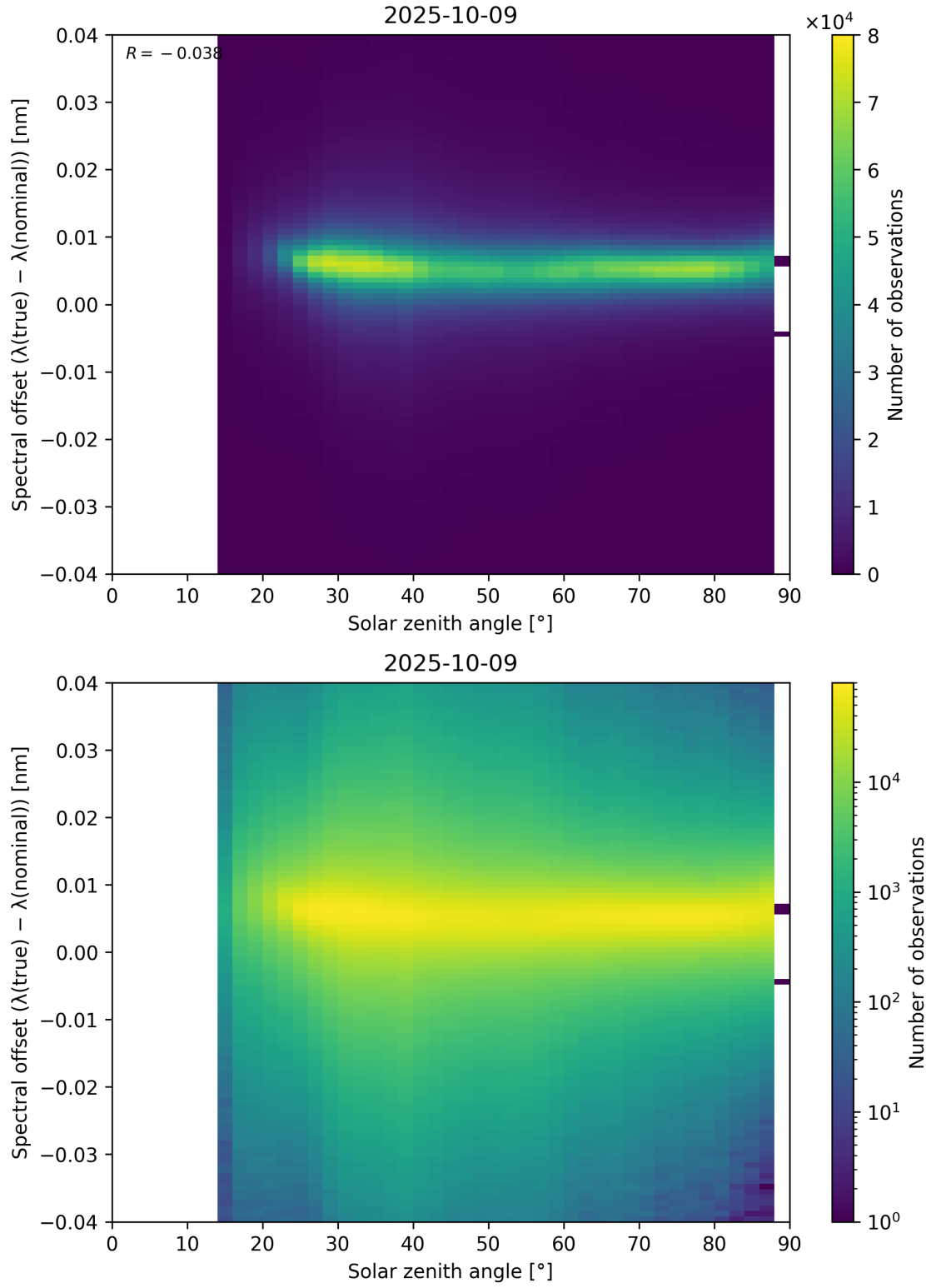
Figure 117: Scatter density plot of “Solar zenith angle” against “Spectral offset ( \lambda_{\text{true}} - \lambda_{\text{nominal}} )” for 2025-10-08 to 2025-10-10.
