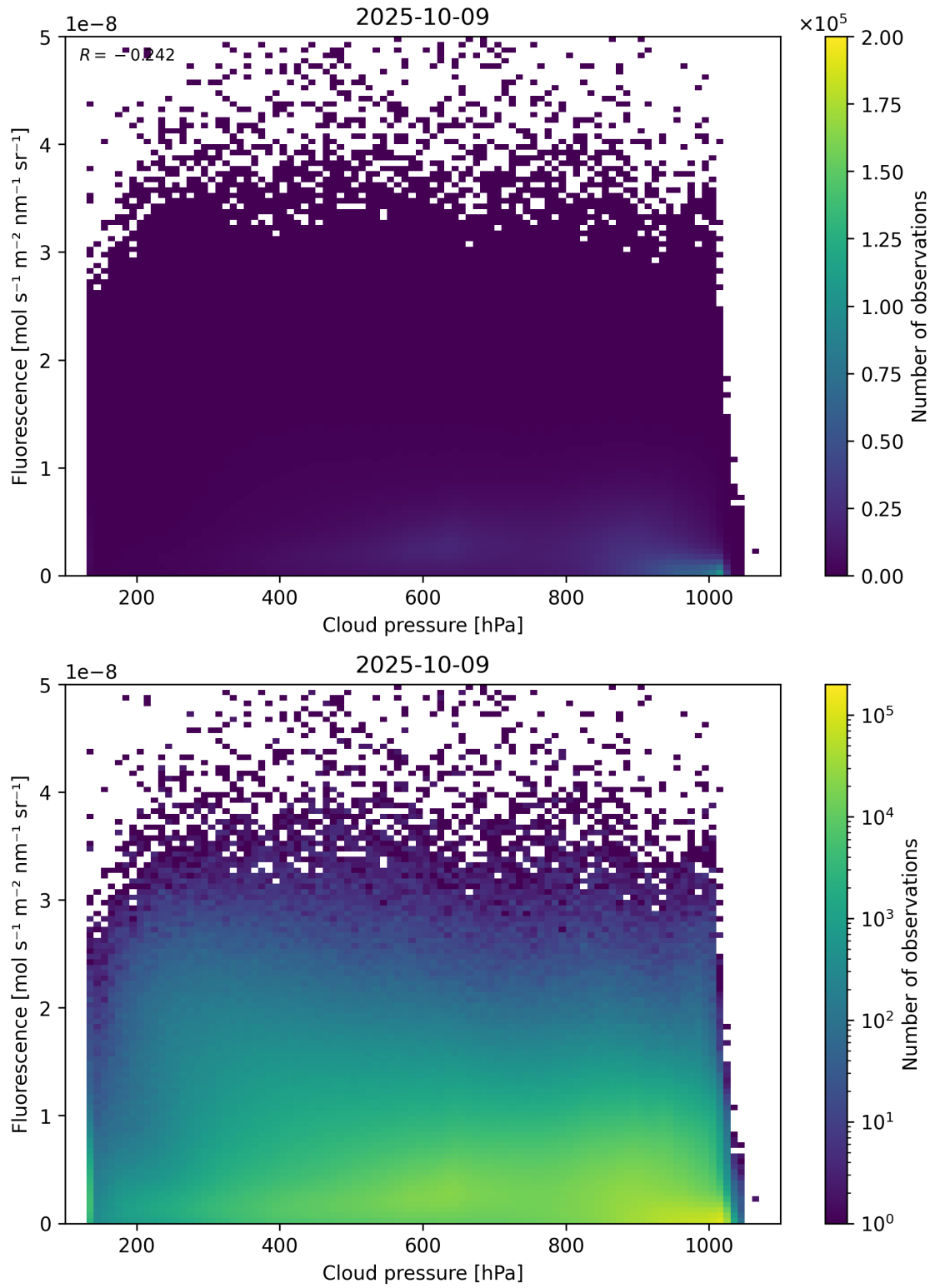
Figure 80: Scatter density plot of “Cloud pressure” against “Fluorescence” for 2025-10-08 to 2025-10-10.
