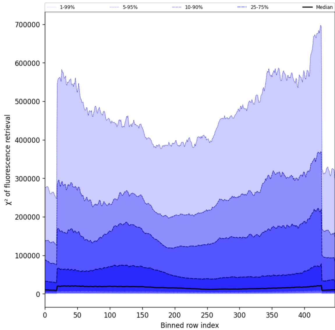
Figure 59: Along track statistics of “ \chi^2 of fluorescence retrieval” for 2025-10-08 to 2025-10-10
