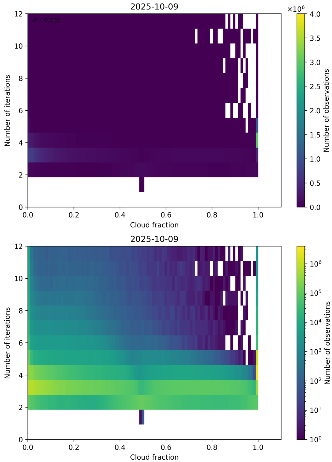
Figure 73: Scatter density plot of “Cloud fraction” against “Number of iterations” for 2025-10-08 to 2025-10-10.
