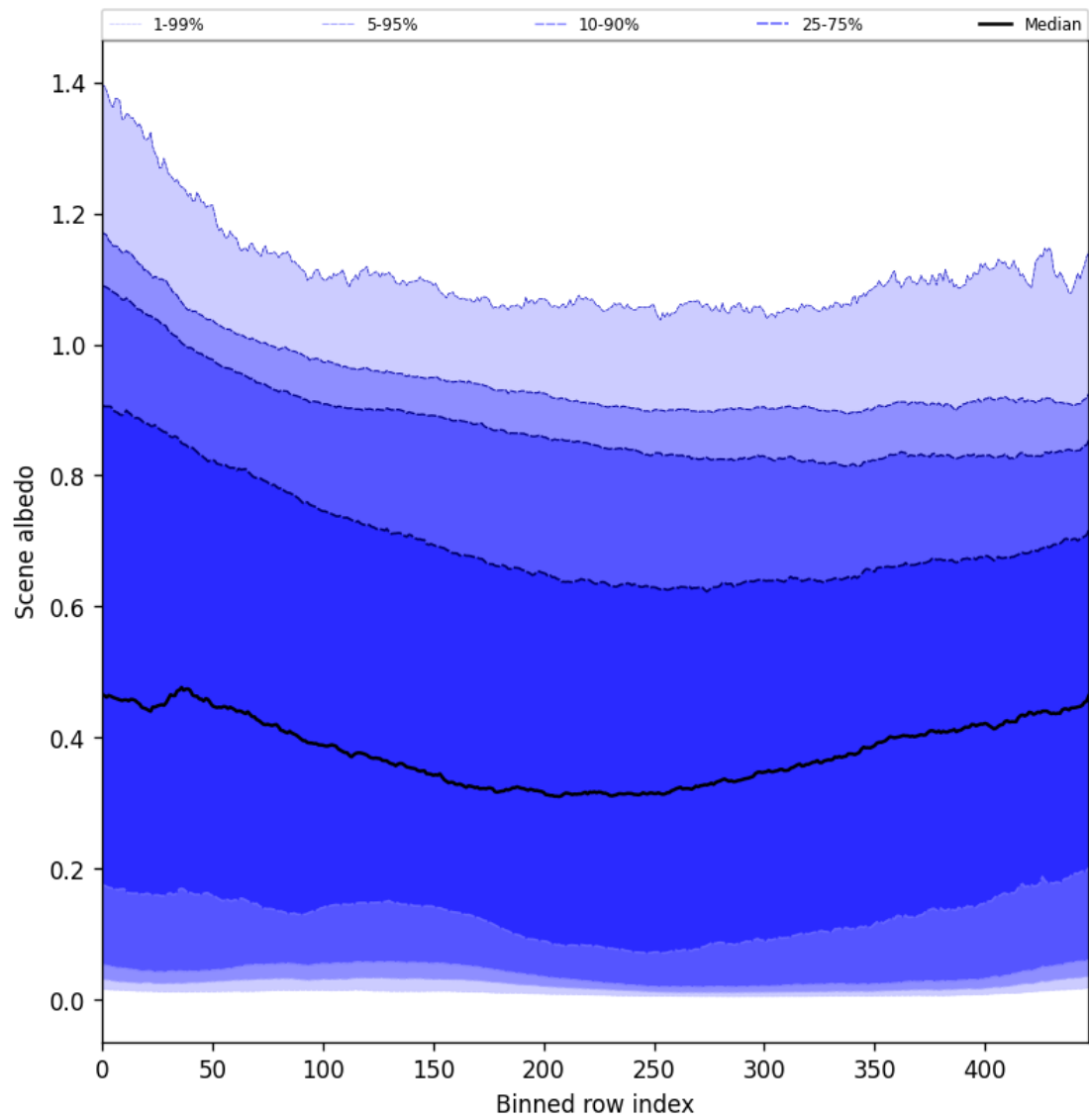
Figure 51: Along track statistics of “Scene albedo” for 2025-10-08 to 2025-10-10
