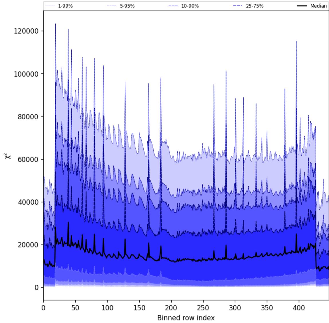
Figure 55: Along track statistics of “ \chi^2 ” for 2025-10-08 to 2025-10-10
