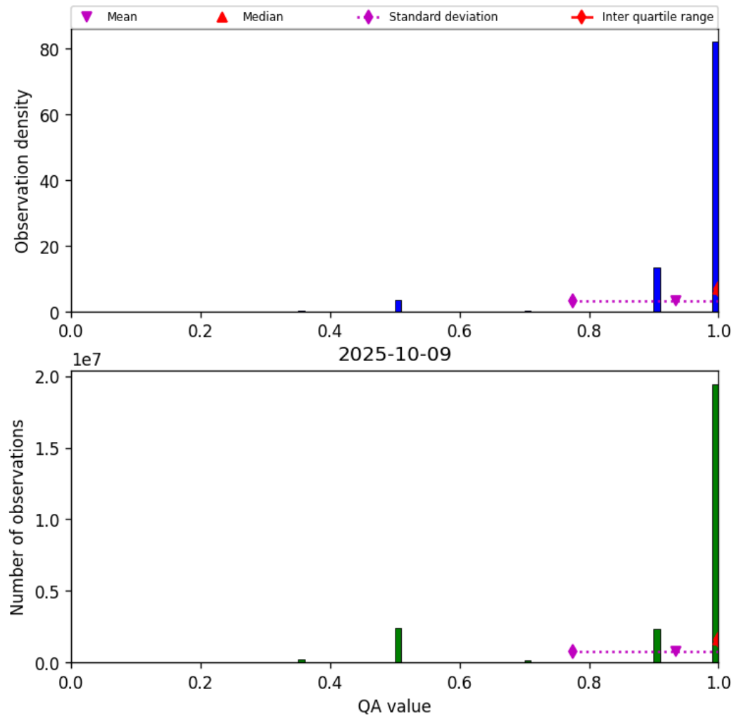
Figure 29: Histogram of “QA value” for 2025-10-08 to 2025-10-10
