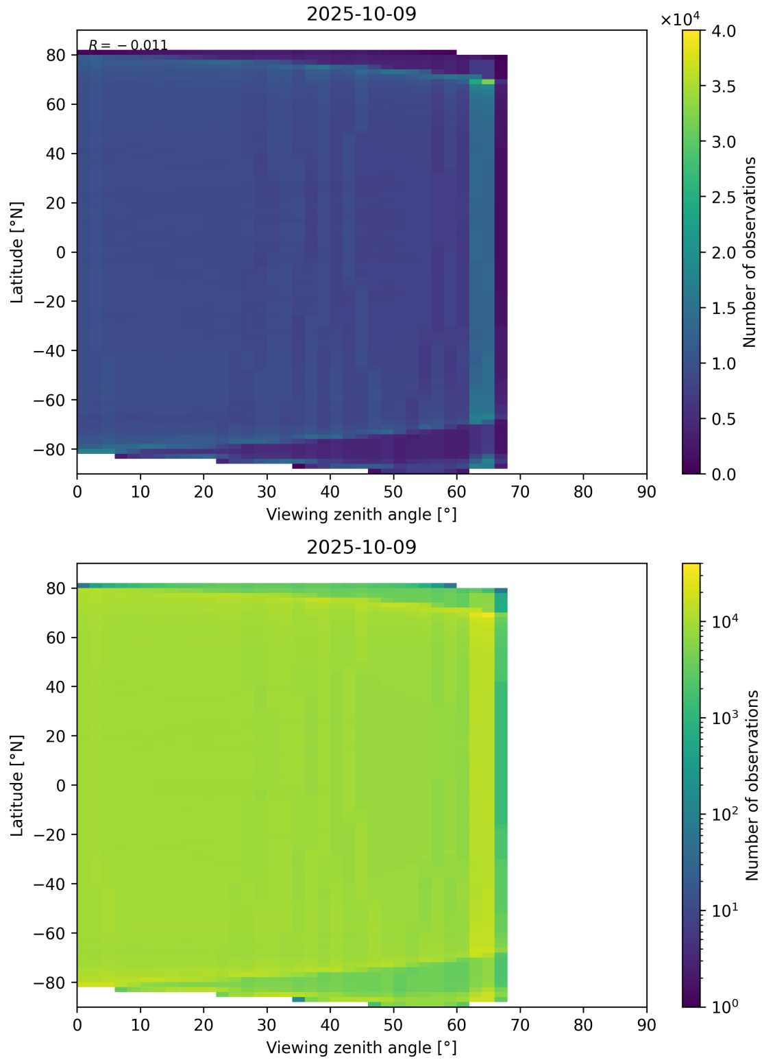
Figure 123: Scatter density plot of “Viewing zenith angle” against “Latitude” for 2025-10-08 to 2025-10-10.
