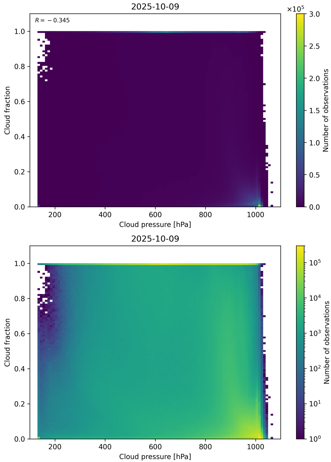
Figure 79: Scatter density plot of “Cloud pressure” against “Cloud fraction” for 2025-10-08 to 2025-10-10.
