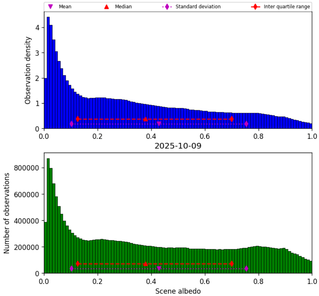
Figure 34: Histogram of “Scene albedo” for 2025-10-08 to 2025-10-10
