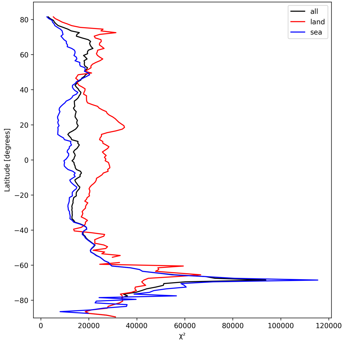
Figure 21: Zonal average of “ \chi^2 ” for 2025-10-08 to 2025-10-10.
