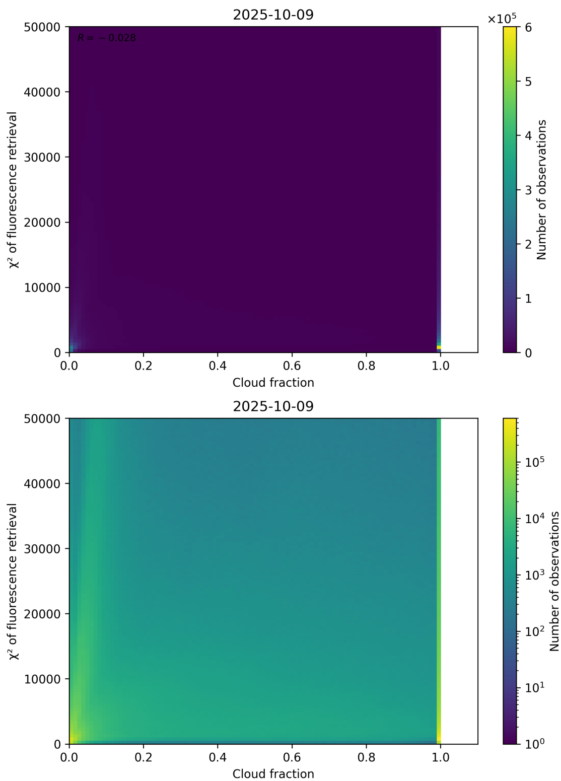
Figure 71: Scatter density plot of “Cloud fraction” against “ \chi^2 of fluorescence retrieval” for 2025-10-08 to 2025-10-10.
