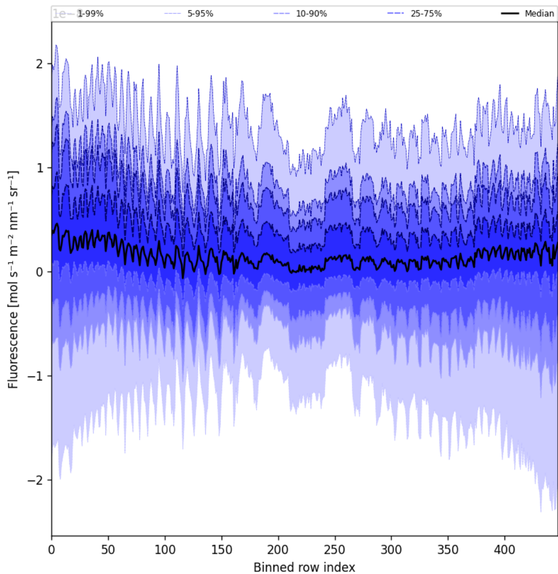
Figure 57: Along track statistics of “Fluorescence” for 2025-10-08 to 2025-10-10
