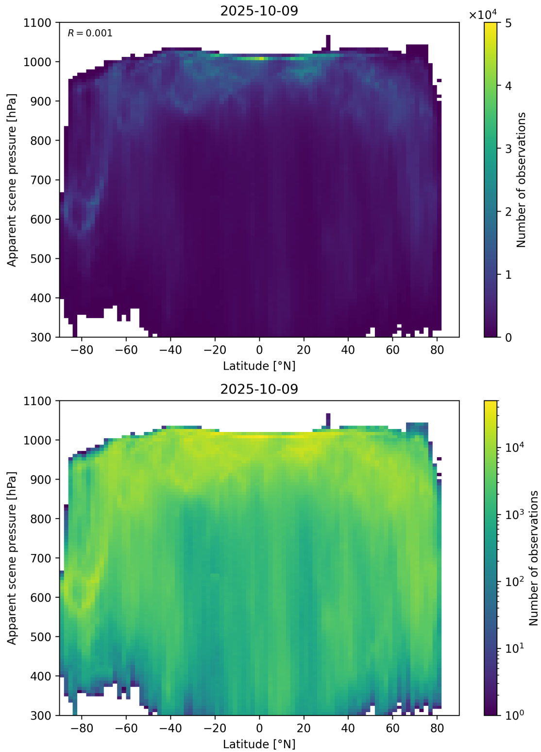
Figure 88: Scatter density plot of “Latitude” against “Apparent scene pressure” for 2025-10-08 to 2025-10-10.
