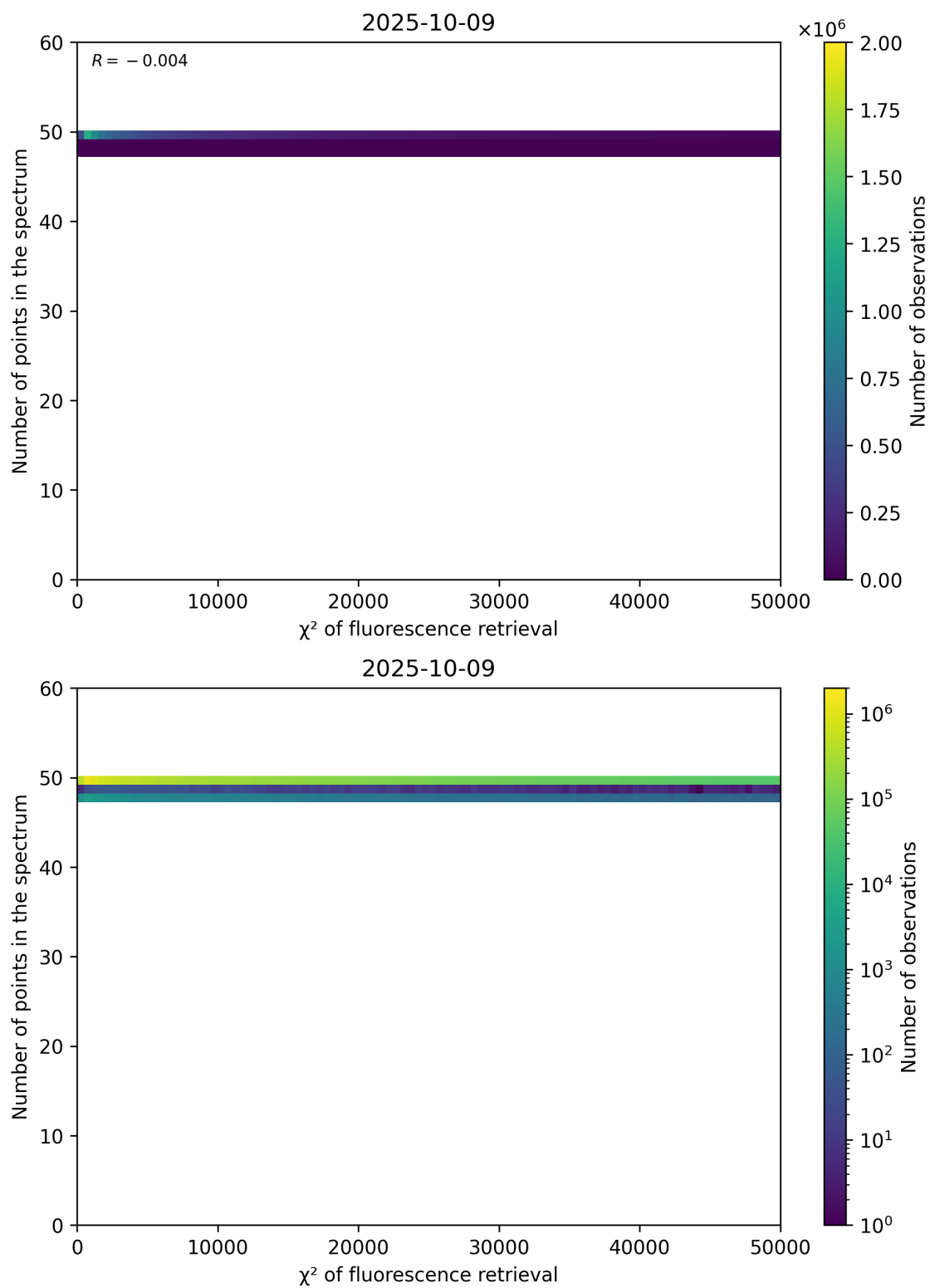
Figure 68: Scatter density plot of " \chi^2 of fluorescence retrieval" against "Number of points in the spectrum" for 2025-10-08 to 2025-10-10.
