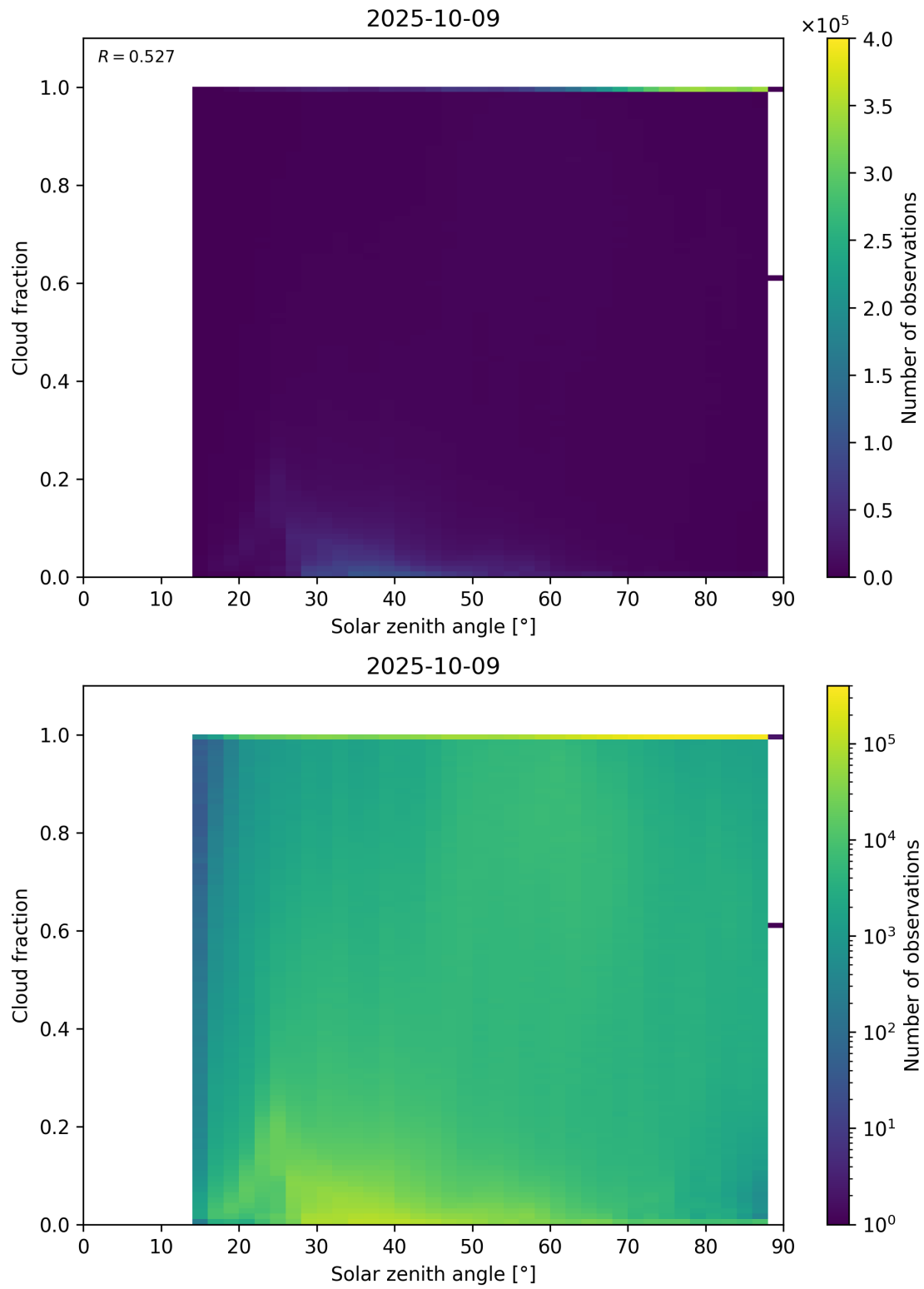
Figure 110: Scatter density plot of “Solar zenith angle” against “Cloud fraction” for 2025-10-08 to 2025-10-10.
