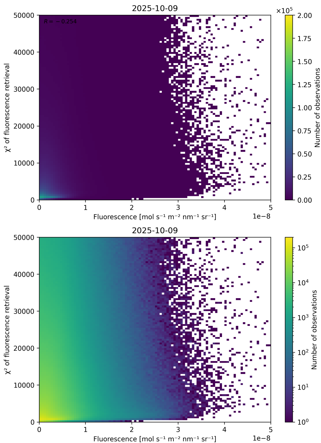
Figure 85: Scatter density plot of “Fluorescence” against “ \chi^2 of fluorescence retrieval” for 2025-10-08 to 2025-10-10.
