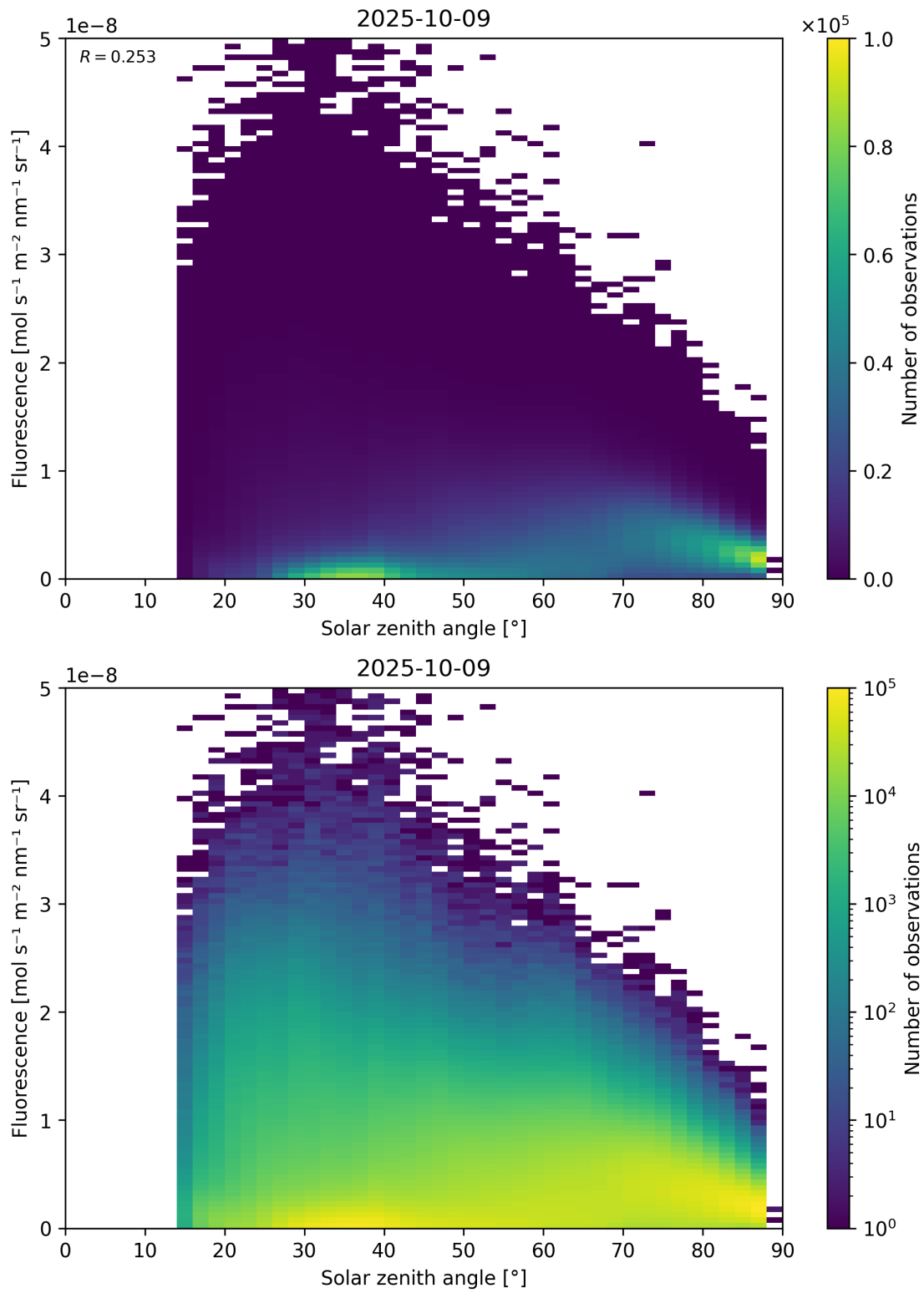
Figure 112: Scatter density plot of “Solar zenith angle” against “Fluorescence” for 2025-10-08 to 2025-10-10.
