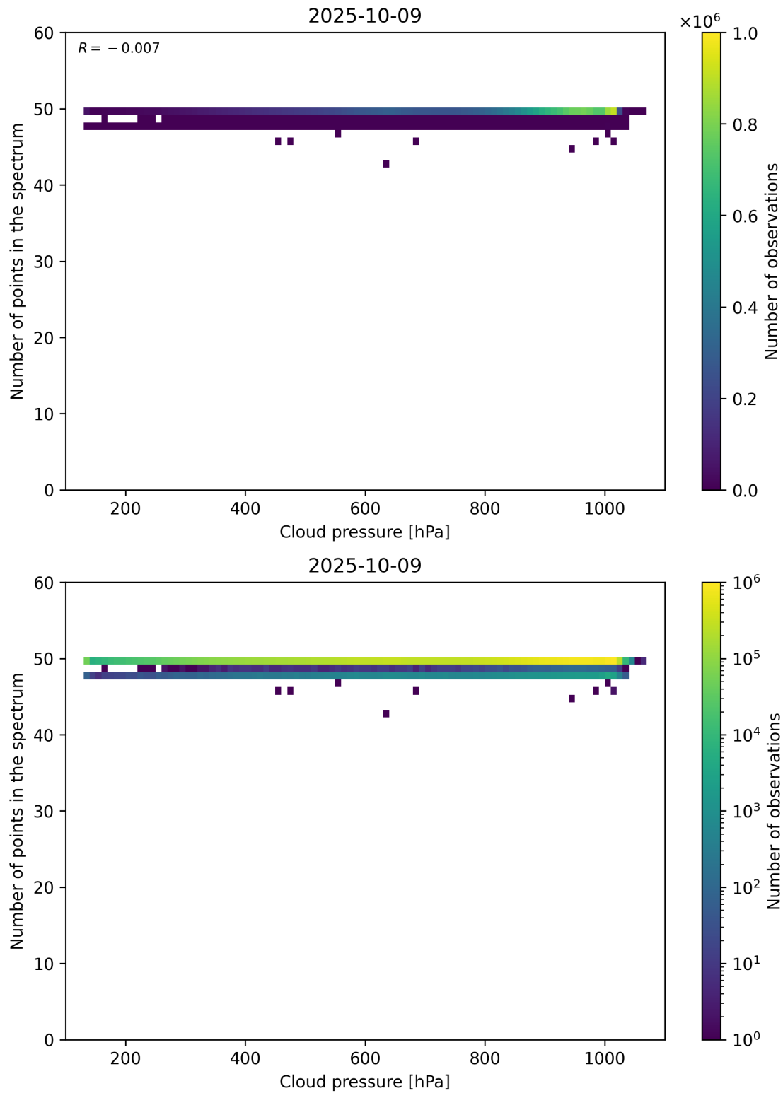
Figure 82: Scatter density plot of “Cloud pressure” against “Number of points in the spectrum” for 2025-10-08 to 2025-10-10.
