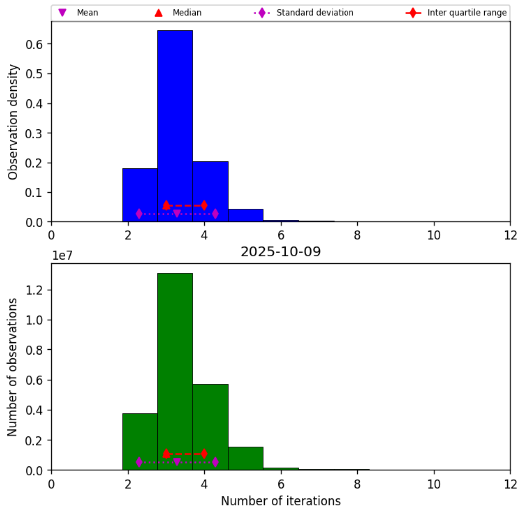
Figure 39: Histogram of “Number of iterations” for 2025-10-08 to 2025-10-10
