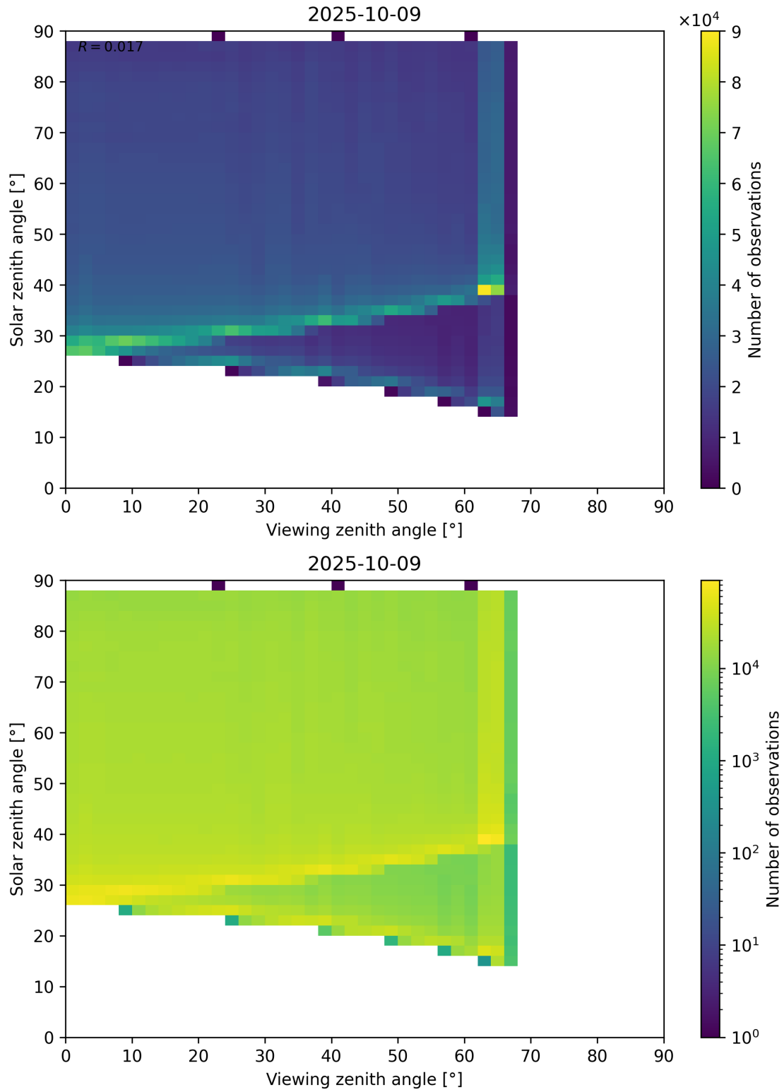
Figure 127: Scatter density plot of “Viewing zenith angle” against “Solar zenith angle” for 2025-10-08 to 2025-10-10.
