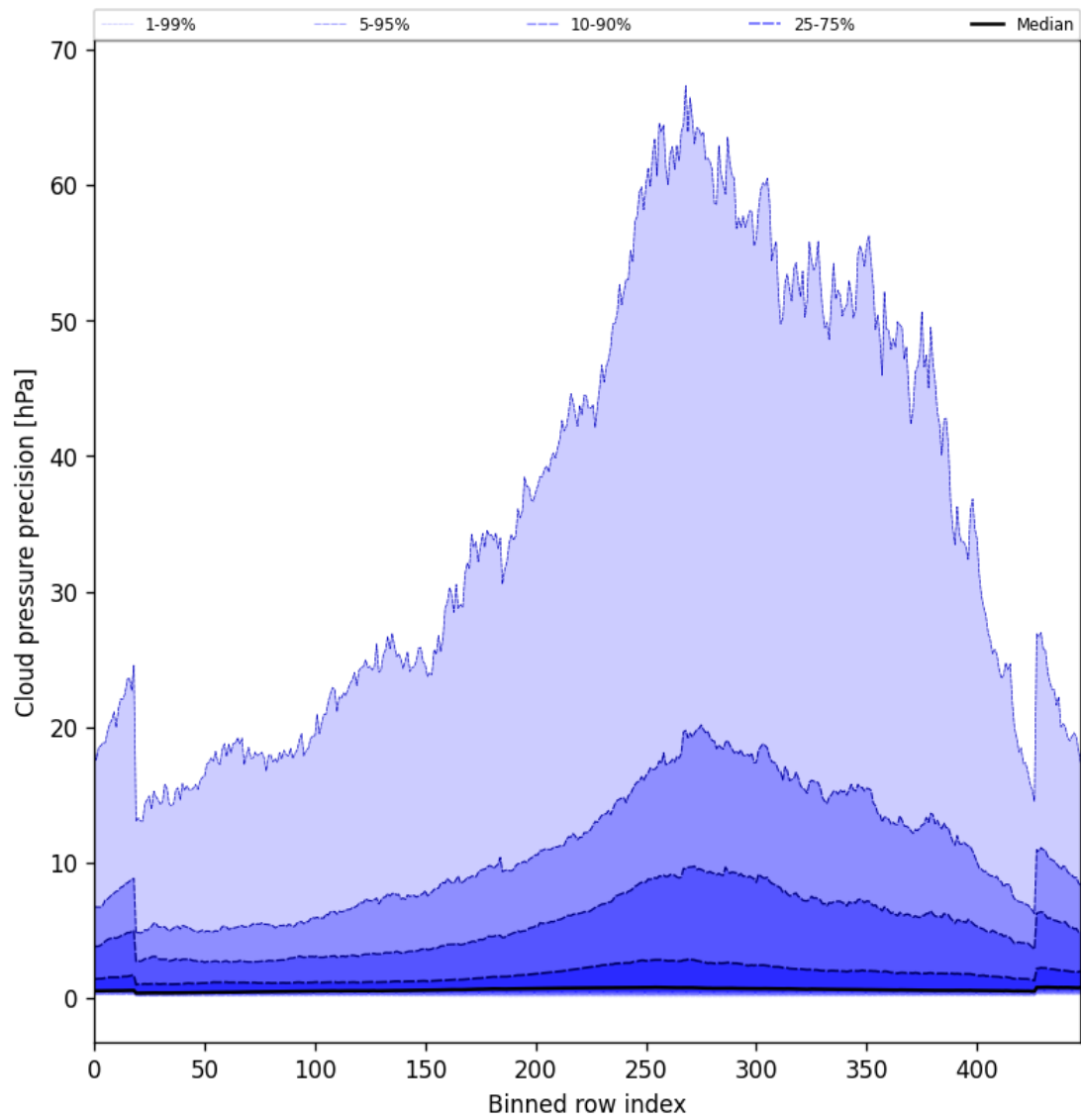
Figure 48: Along track statistics of “Cloud pressure precision” for 2025-10-08 to 2025-10-10
