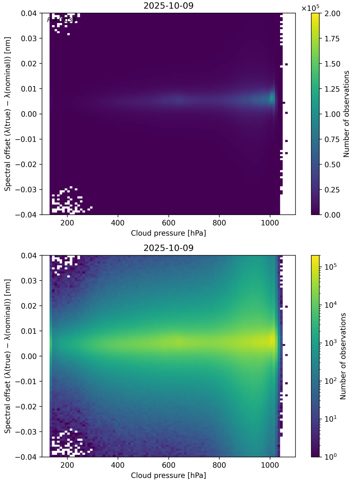
Figure 84: Scatter density plot of “Cloud pressure” against “Spectral offset ( \lambda_{\text{true}} - \lambda_{\text{nominal}} )” for 2025-10-08 to 2025-10-10.
