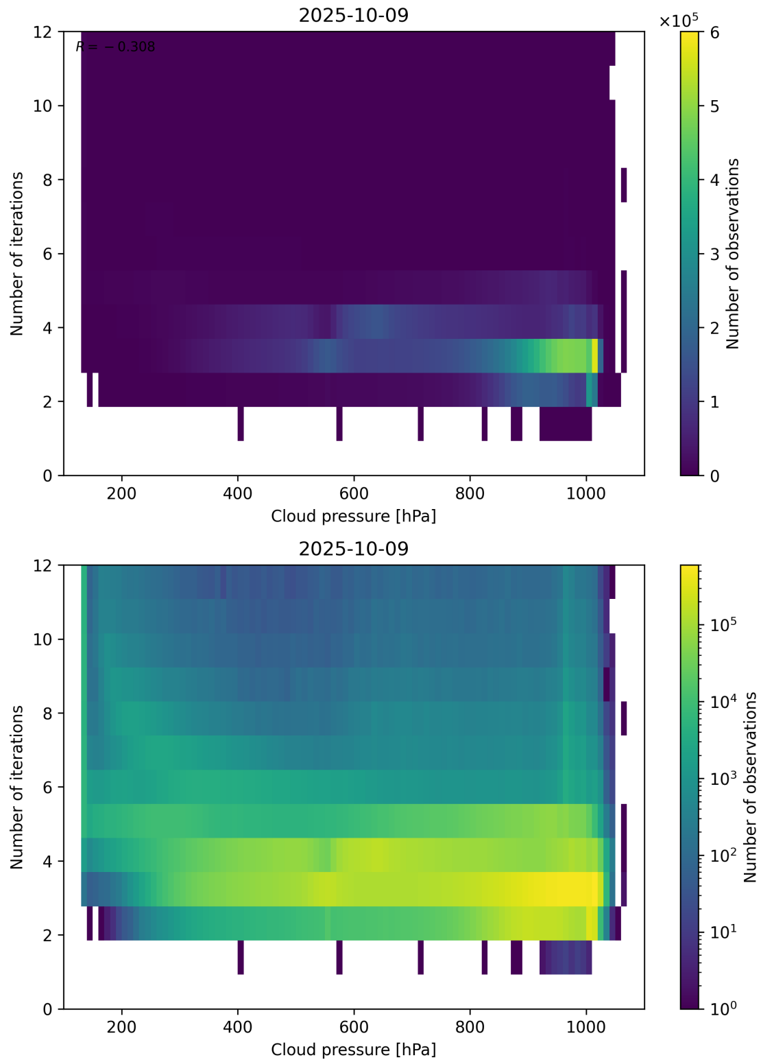
Figure 81: Scatter density plot of “Cloud pressure” against “Number of iterations” for 2025-10-08 to 2025-10-10.
