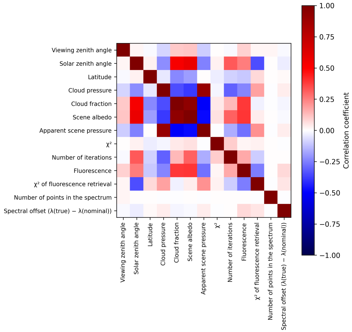
Figure 2: Map of correlation matrix for 2025-10-08 to 2025-10-10.
