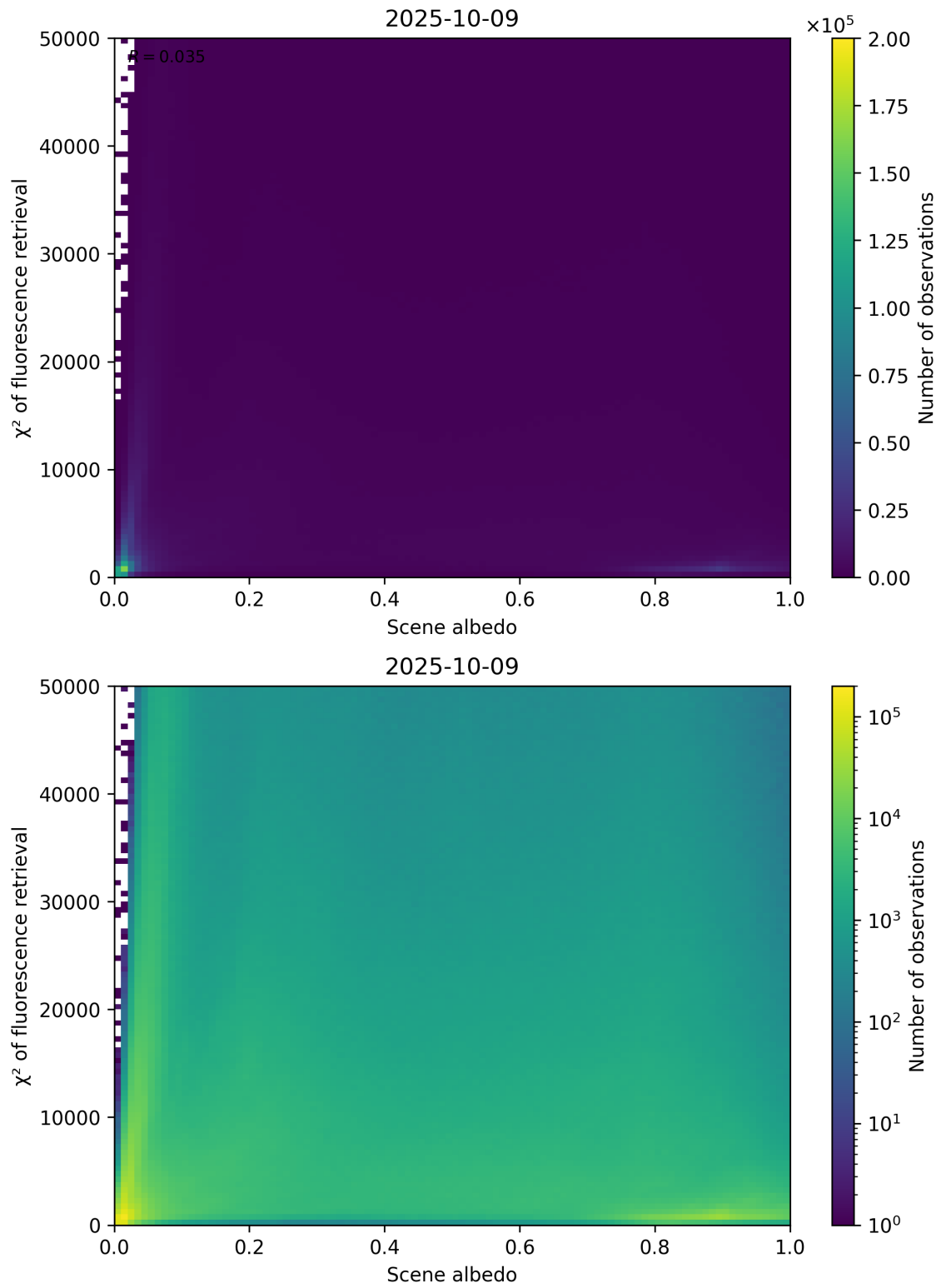
Figure 103: Scatter density plot of “Scene albedo” against “ \chi^2 of fluorescence retrieval” for 2025-10-08 to 2025-10-10.
