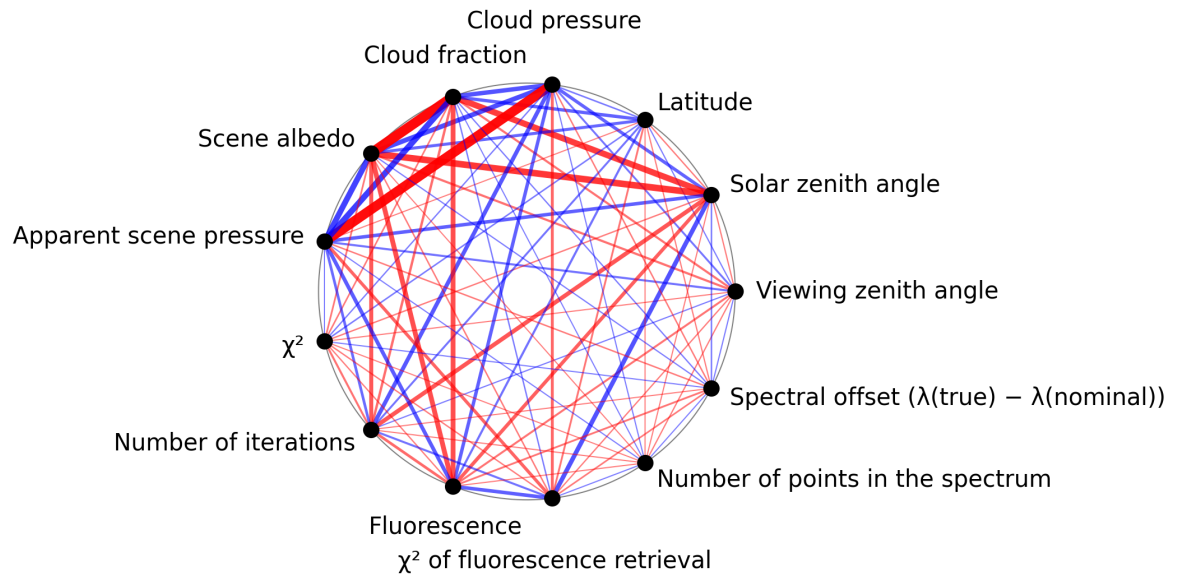
Figure 1: Map of correlation graph for 2025-10-08 to 2025-10-10.
