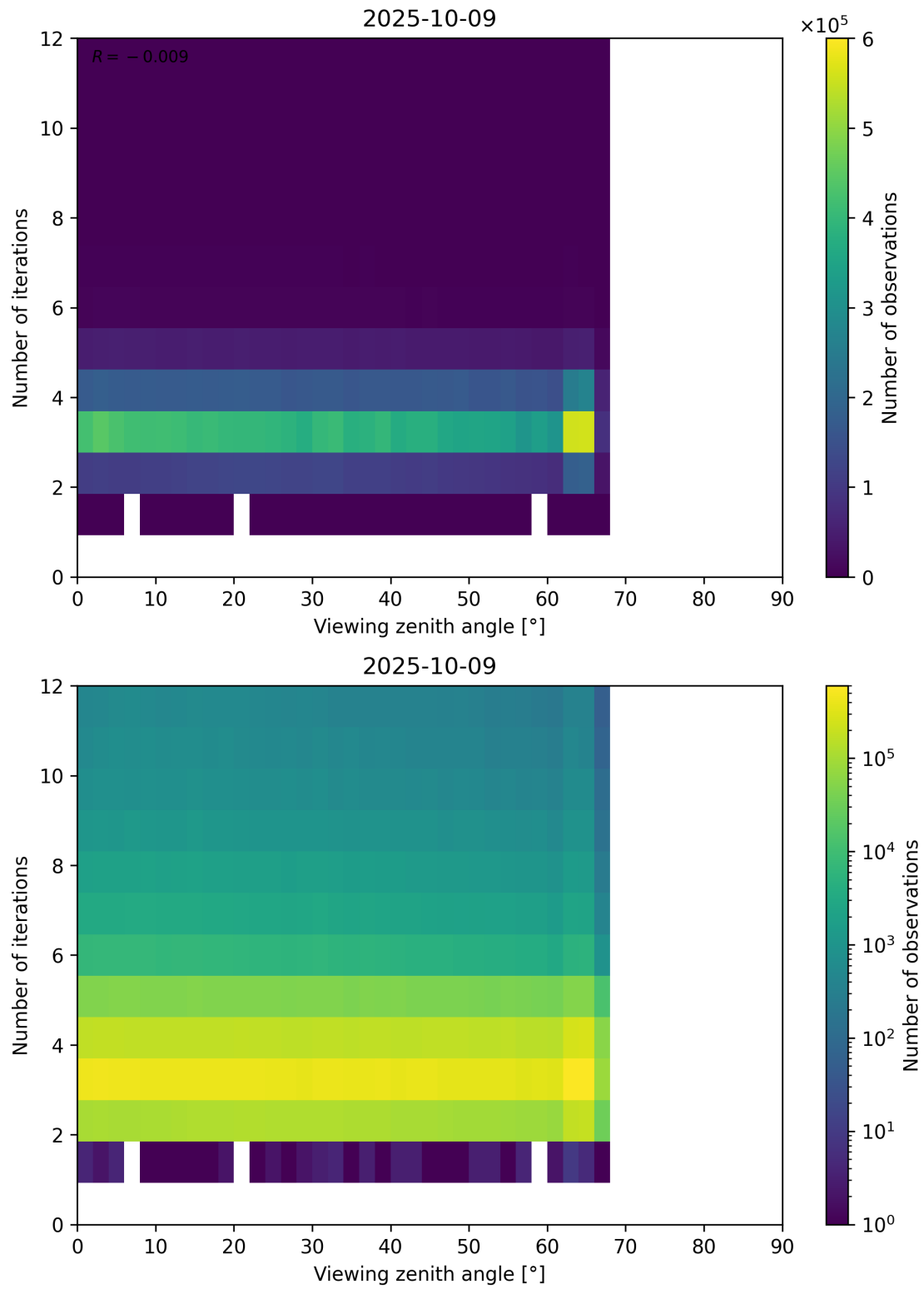
Figure 124: Scatter density plot of “Viewing zenith angle” against “Number of iterations” for 2025-10-08 to 2025-10-10.
