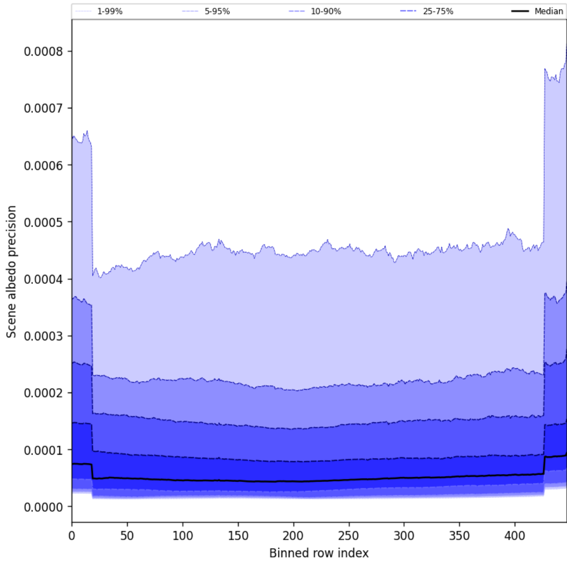
Figure 52: Along track statistics of “Scene albedo precision” for 2025-10-08 to 2025-10-10
