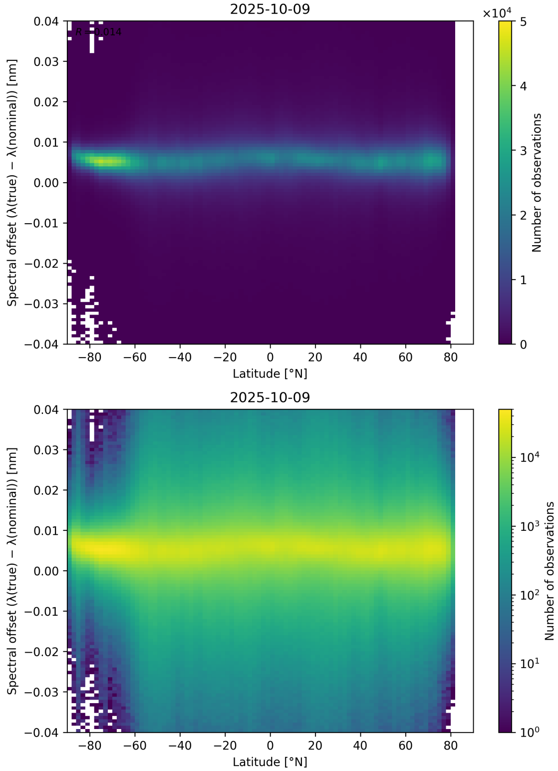
Figure 96: Scatter density plot of “Latitude” against “Spectral offset ( \lambda_{\text{true}} - \lambda_{\text{nominal}} )” for 2025-10-08 to 2025-10-10.
