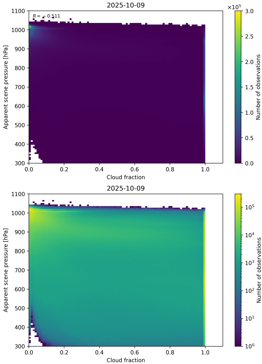
Figure 70: Scatter density plot of “Cloud fraction” against “Apparent scene pressure” for 2025-10-08 to 2025-10-10.
