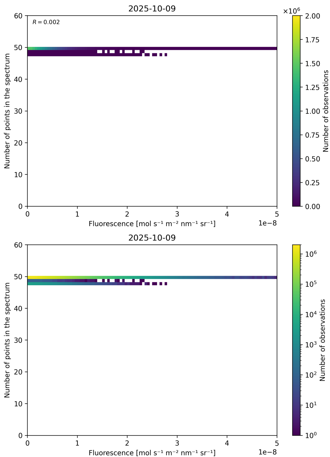
Figure 86: Scatter density plot of “Fluorescence” against “Number of points in the spectrum” for 2025-10-08 to 2025-10-10.
