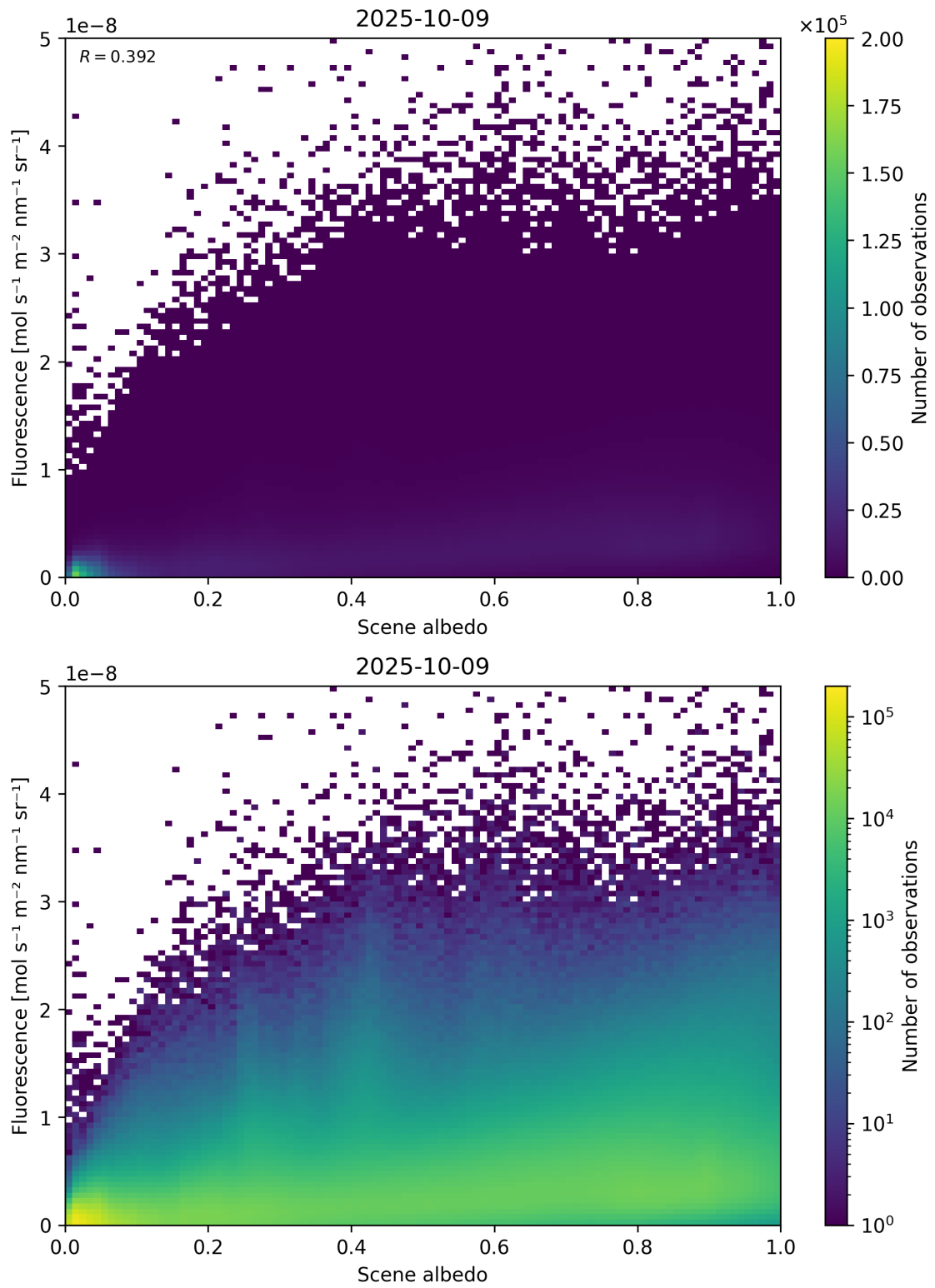
Figure 104: Scatter density plot of “Scene albedo” against “Fluorescence” for 2025-10-08 to 2025-10-10.
