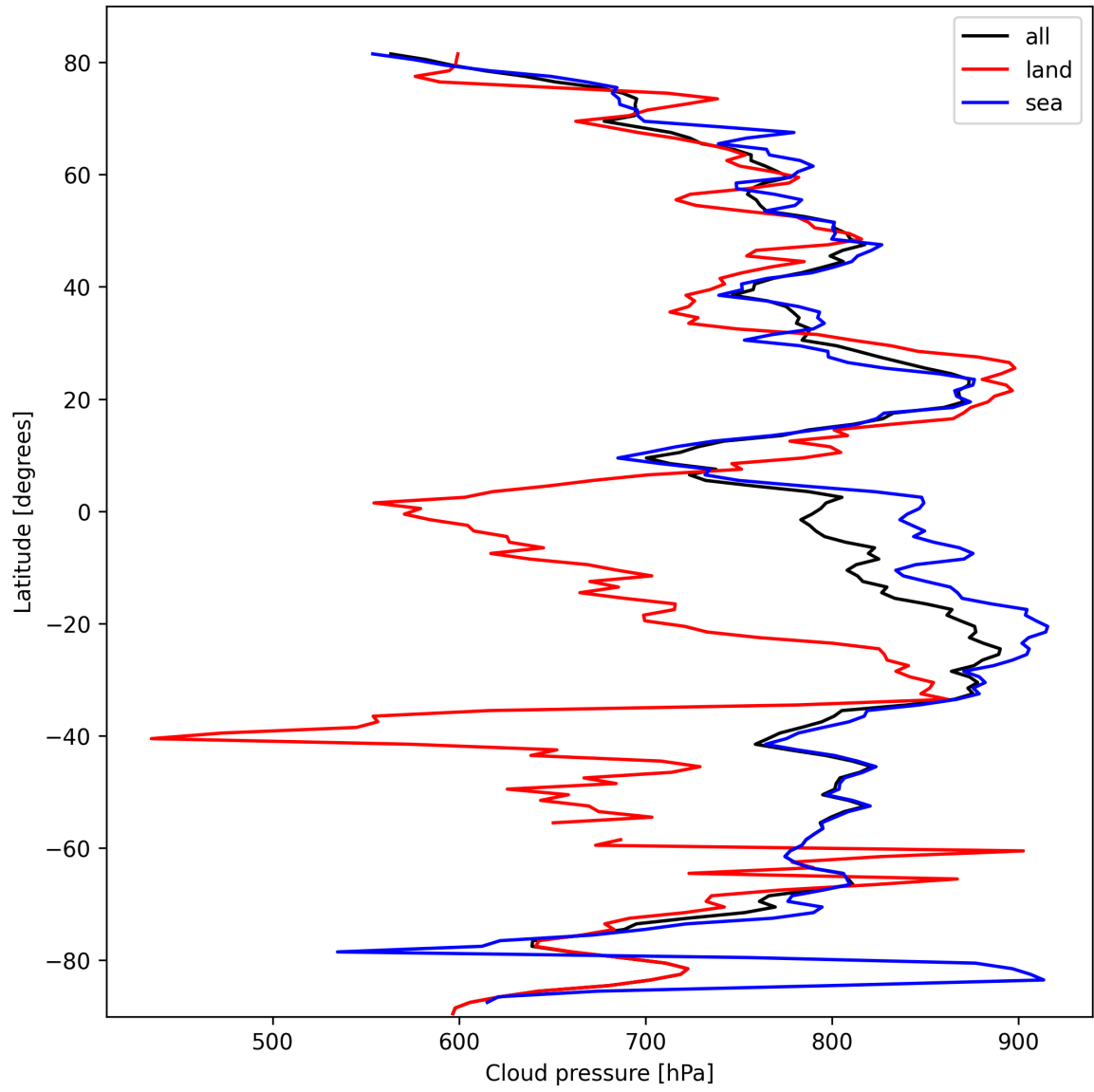
Figure 13: Zonal average of “Cloud pressure” for 2025-10-08 to 2025-10-10.
