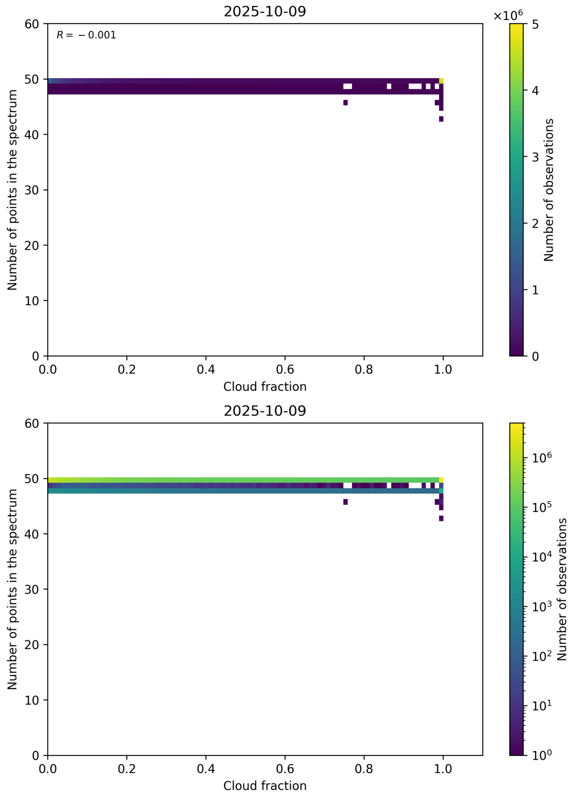
Figure 74: Scatter density plot of “Cloud fraction” against “Number of points in the spectrum” for 2025-10-08 to 2025-10-10.
