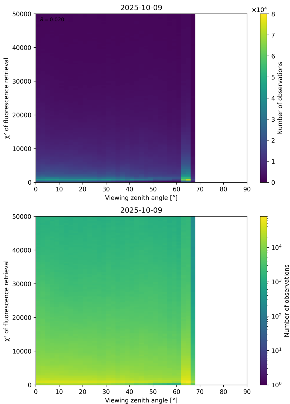
Figure 119: Scatter density plot of “Viewing zenith angle” against “ \chi^2 of fluorescence retrieval” for 2025-10-08 to 2025-10-10.
