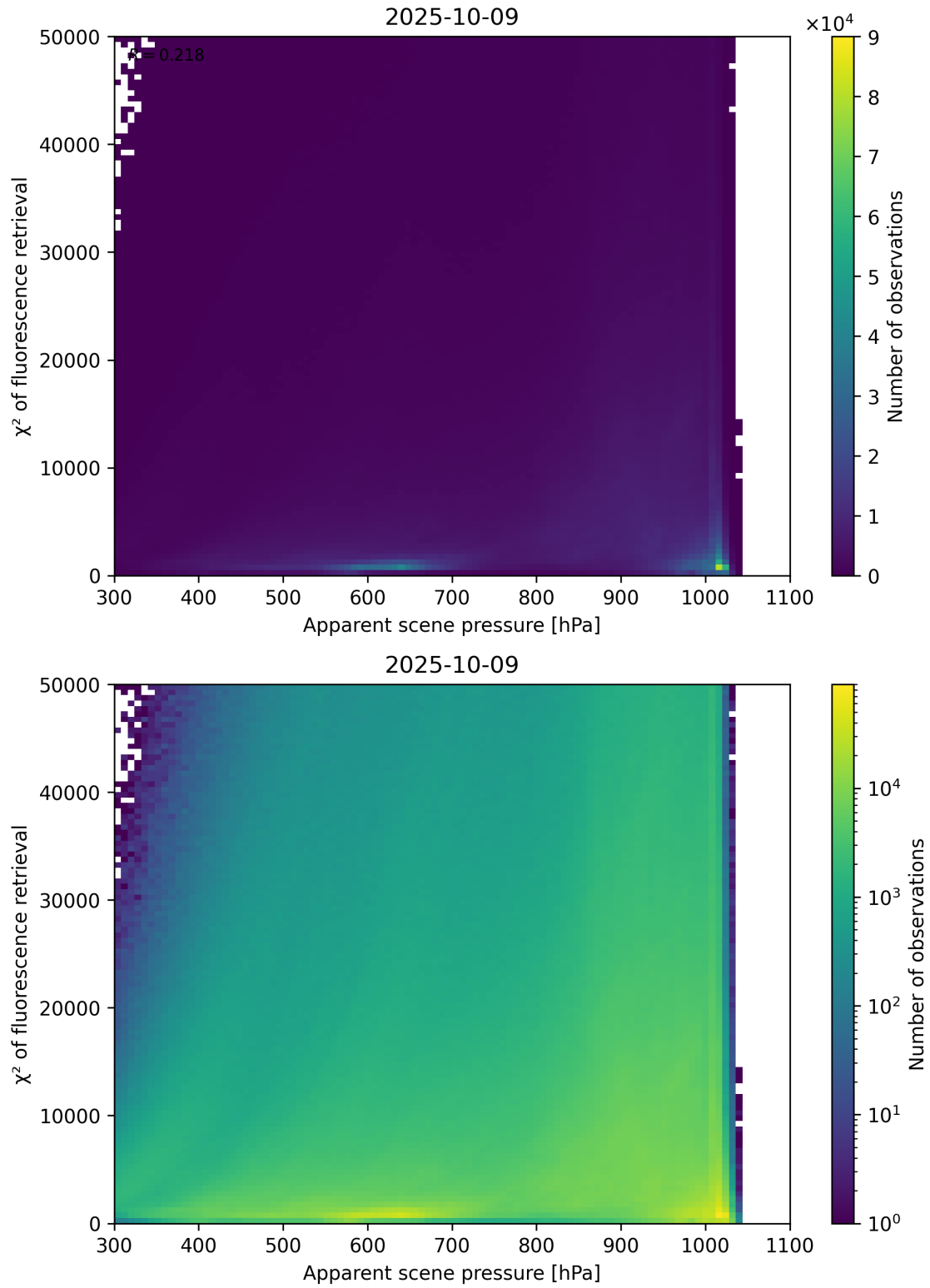
Figure 63: Scatter density plot of “Apparent scene pressure” against “ \chi^2 of fluorescence retrieval” for 2025-10-08 to 2025-10-10.
