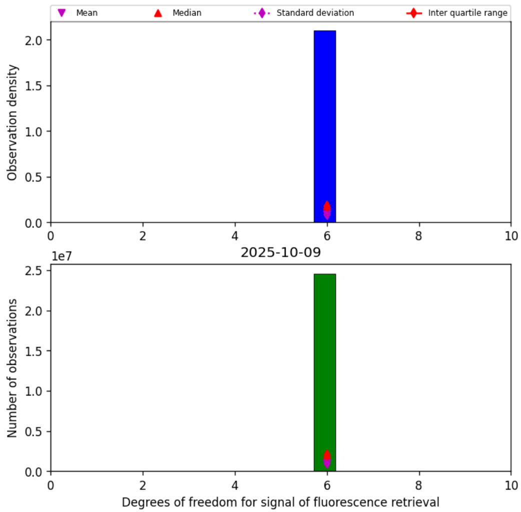
Figure 43: Histogram of “Degrees of freedom for signal of fluorescence retrieval” for 2025-10-08 to 2025-10-10
