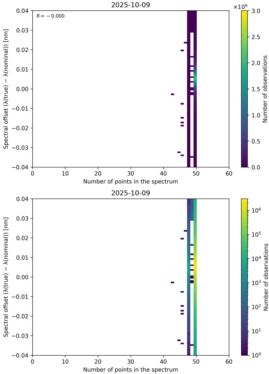
Figure 101: Scatter density plot of “Number of points in the spectrum” against “Spectral offset ( \lambda_{\text{true}} - \lambda_{\text{nominal}} )” for 2025-10-08 to 2025-10-10.
