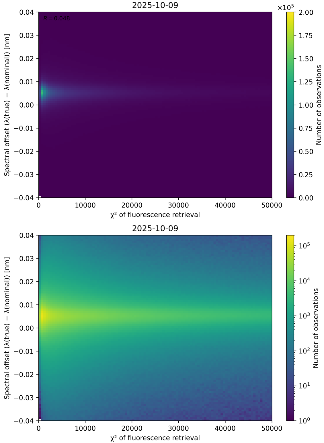
Figure 69: Scatter density plot of “ \chi^2 of fluorescence retrieval” against “Spectral offset ( \lambda_{\text{true}} - \lambda_{\text{nominal}} )” for 2025-10-08 to 2025-10-10.
