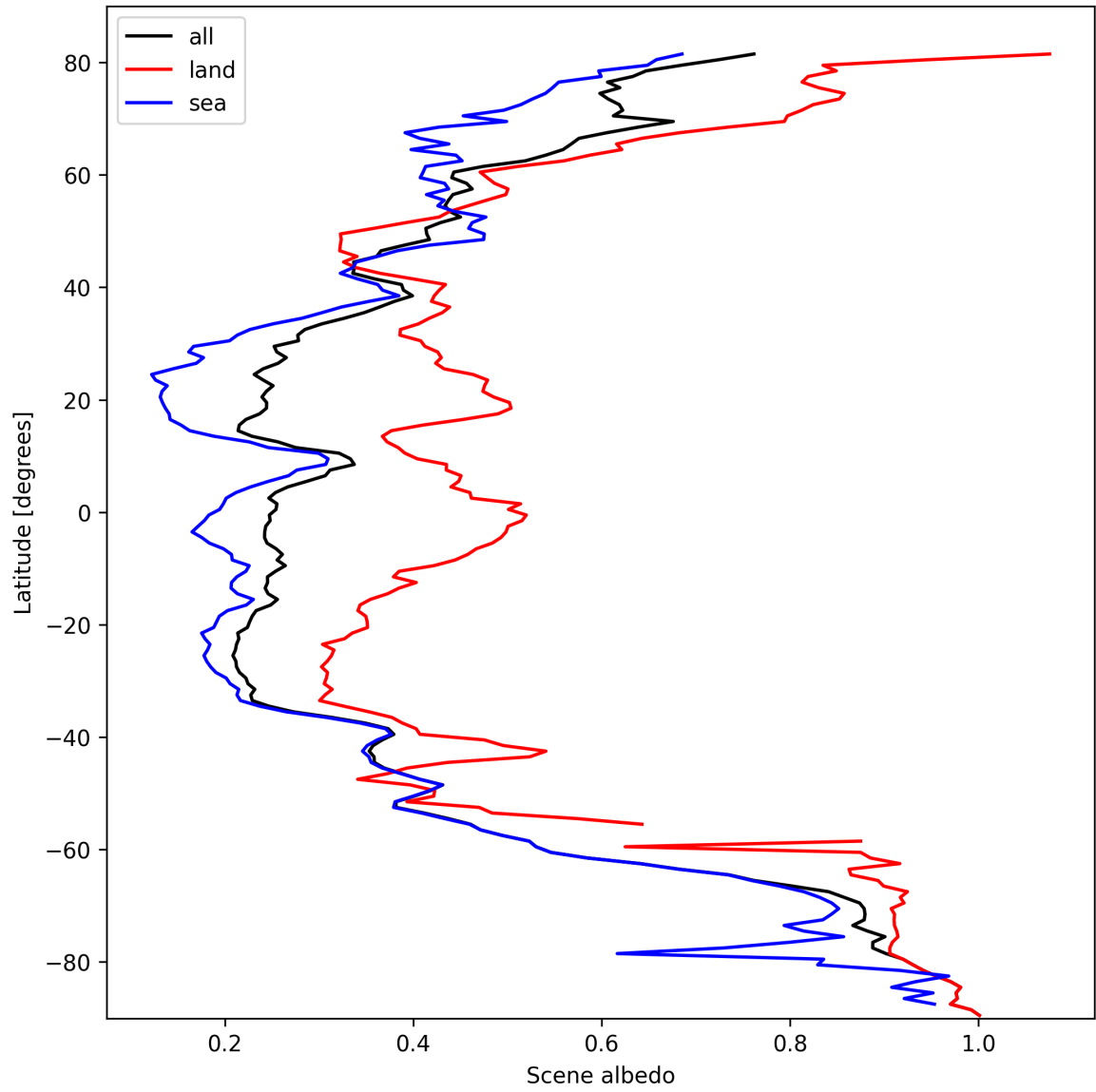
Figure 17: Zonal average of “Scene albedo” for 2025-10-08 to 2025-10-10.
