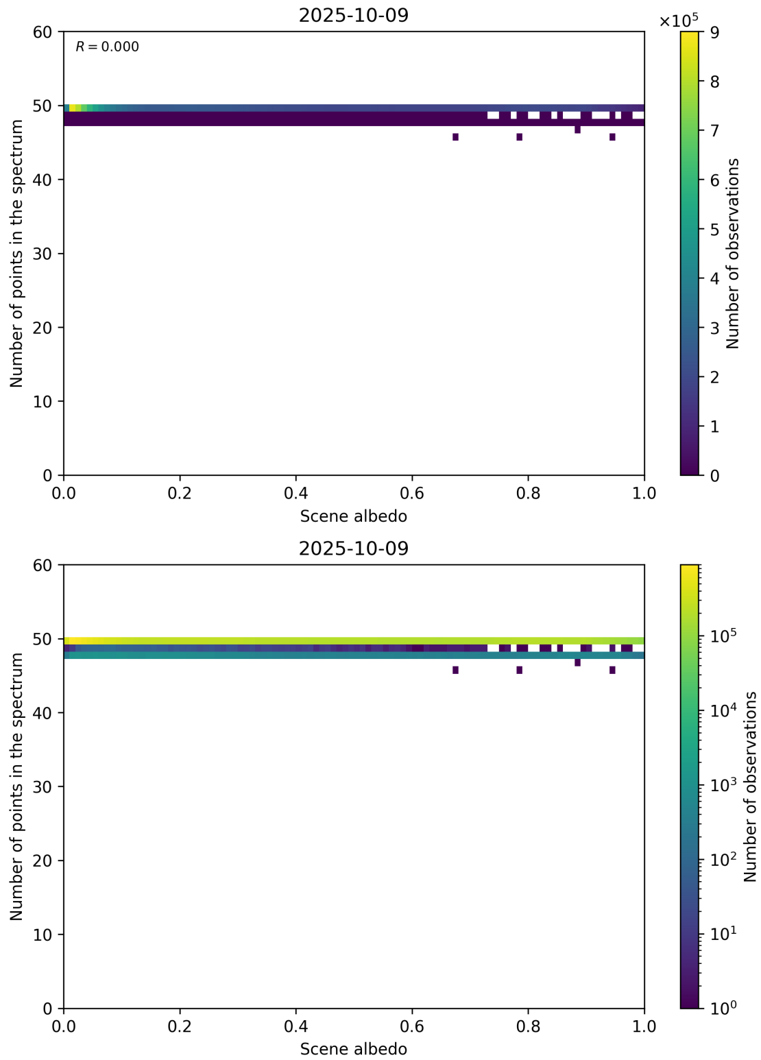
Figure 106: Scatter density plot of “Scene albedo” against “Number of points in the spectrum” for 2025-10-08 to 2025-10-10.
