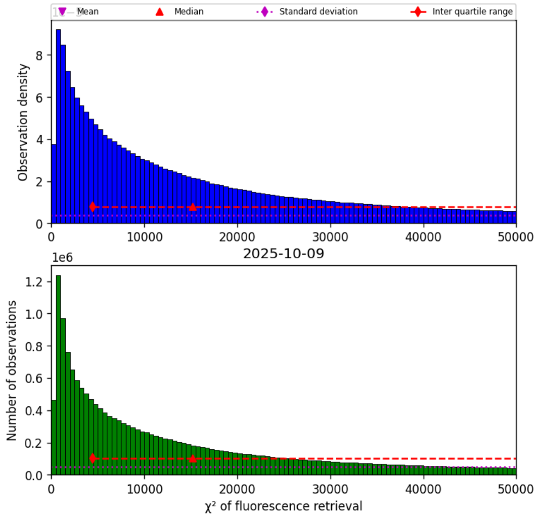
Figure 42: Histogram of “ \chi^2 of fluorescence retrieval” for 2025-10-08 to 2025-10-10
