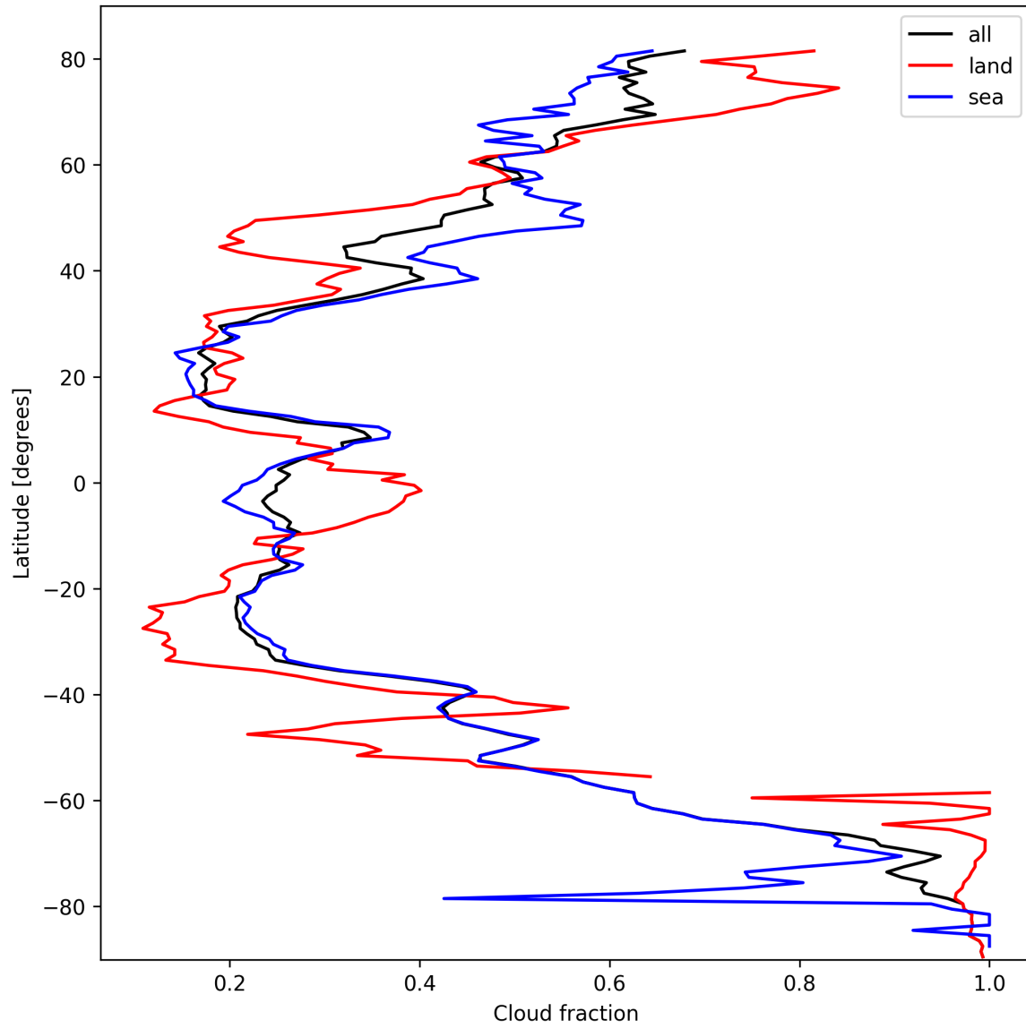
Figure 15: Zonal average of “Cloud fraction” for 2025-10-08 to 2025-10-10.
