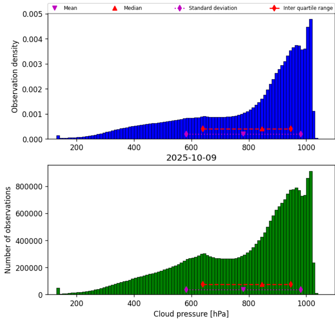
Figure 30: Histogram of “Cloud pressure” for 2025-10-08 to 2025-10-10
