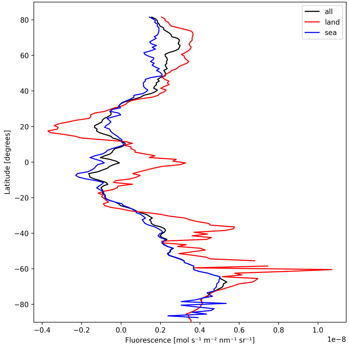
Figure 23: Zonal average of “Fluorescence” for 2025-10-08 to 2025-10-10.
