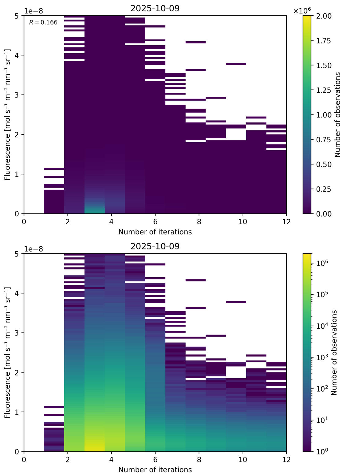
Figure 98: Scatter density plot of “Number of iterations” against “Fluorescence” for 2025-10-08 to 2025-10-10.
