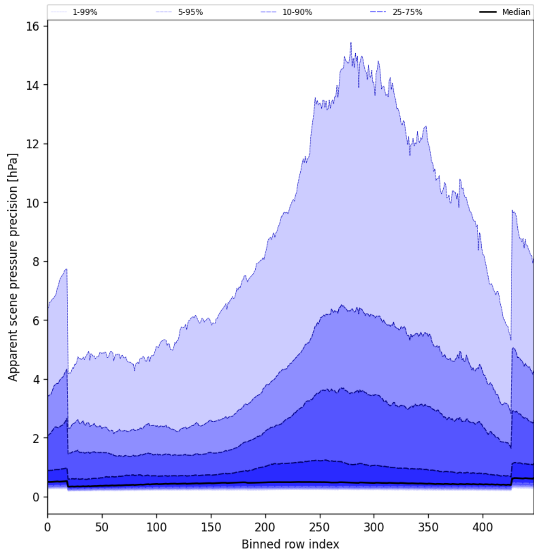
Figure 54: Along track statistics of “Apparent scene pressure precision” for 2025-10-08 to 2025-10-10
