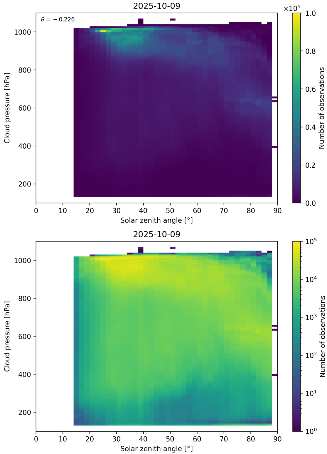
Figure 111: Scatter density plot of “Solar zenith angle” against “Cloud pressure” for 2025-10-08 to 2025-10-10.
