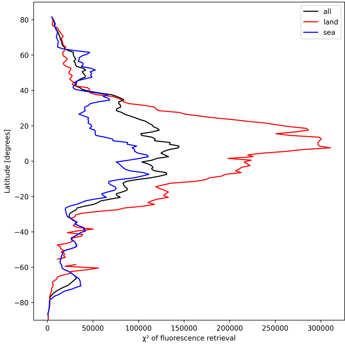
Figure 25: Zonal average of “ \chi^2 of fluorescence retrieval” for 2025-10-08 to 2025-10-10.
