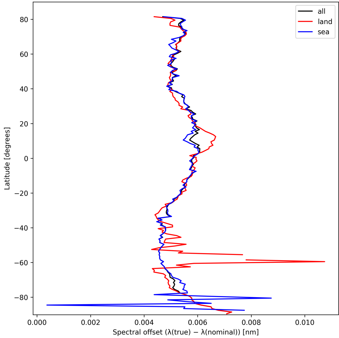
Figure 28: Zonal average of “Spectral offset ( \lambda_{\text{true}} - \lambda_{\text{nominal}} )” for 2025-10-08 to 2025-10-10.
