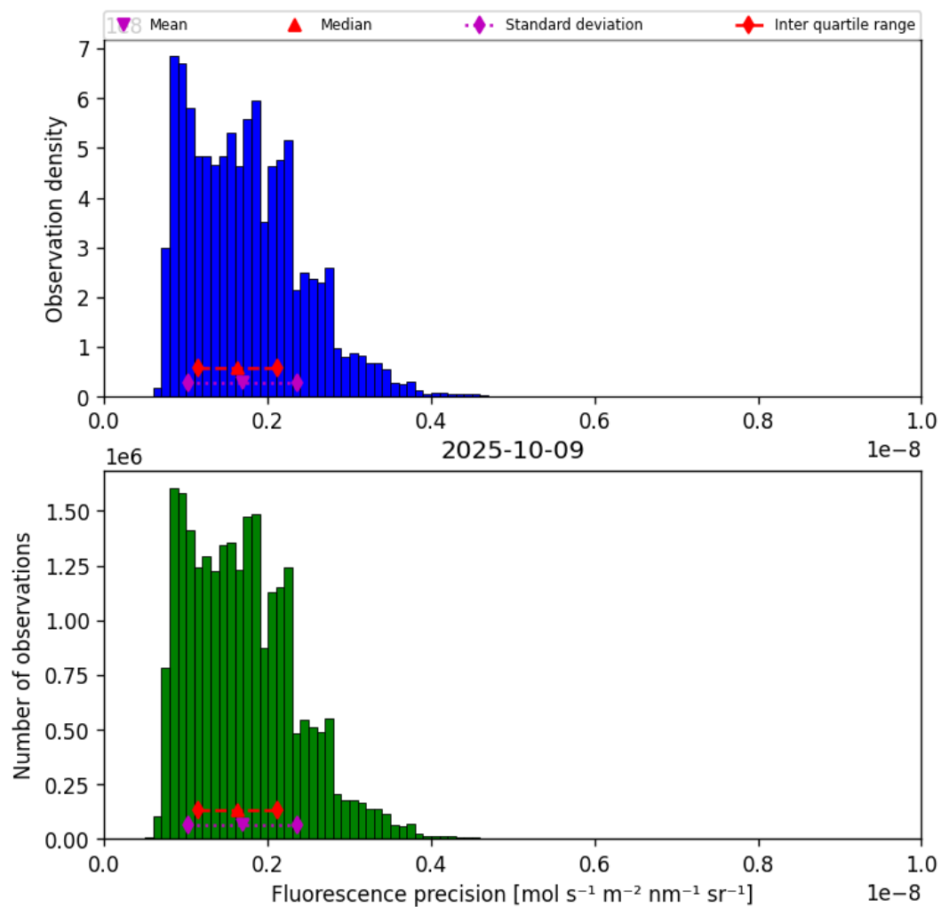
Figure 41: Histogram of “Fluorescence precision” for 2025-10-08 to 2025-10-10
