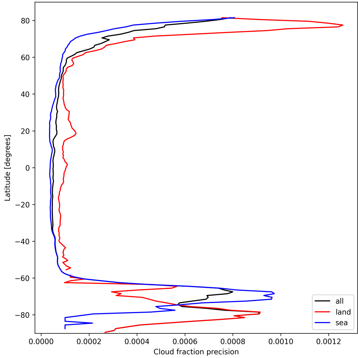
Figure 16: Zonal average of “Cloud fraction precision” for 2025-10-08 to 2025-10-10.
