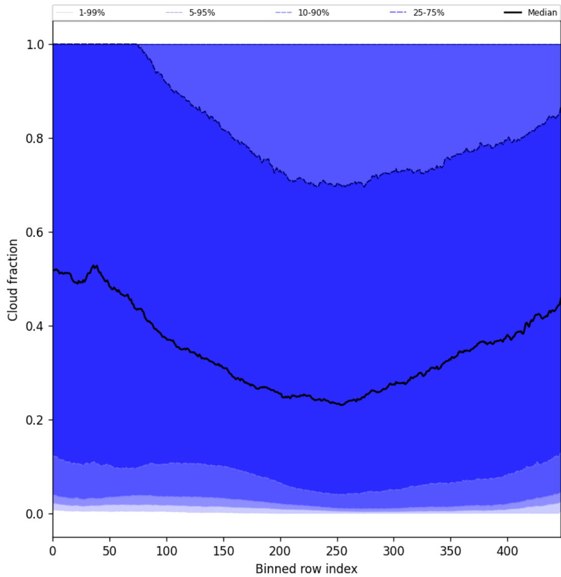
Figure 49: Along track statistics of “Cloud fraction” for 2025-10-08 to 2025-10-10
