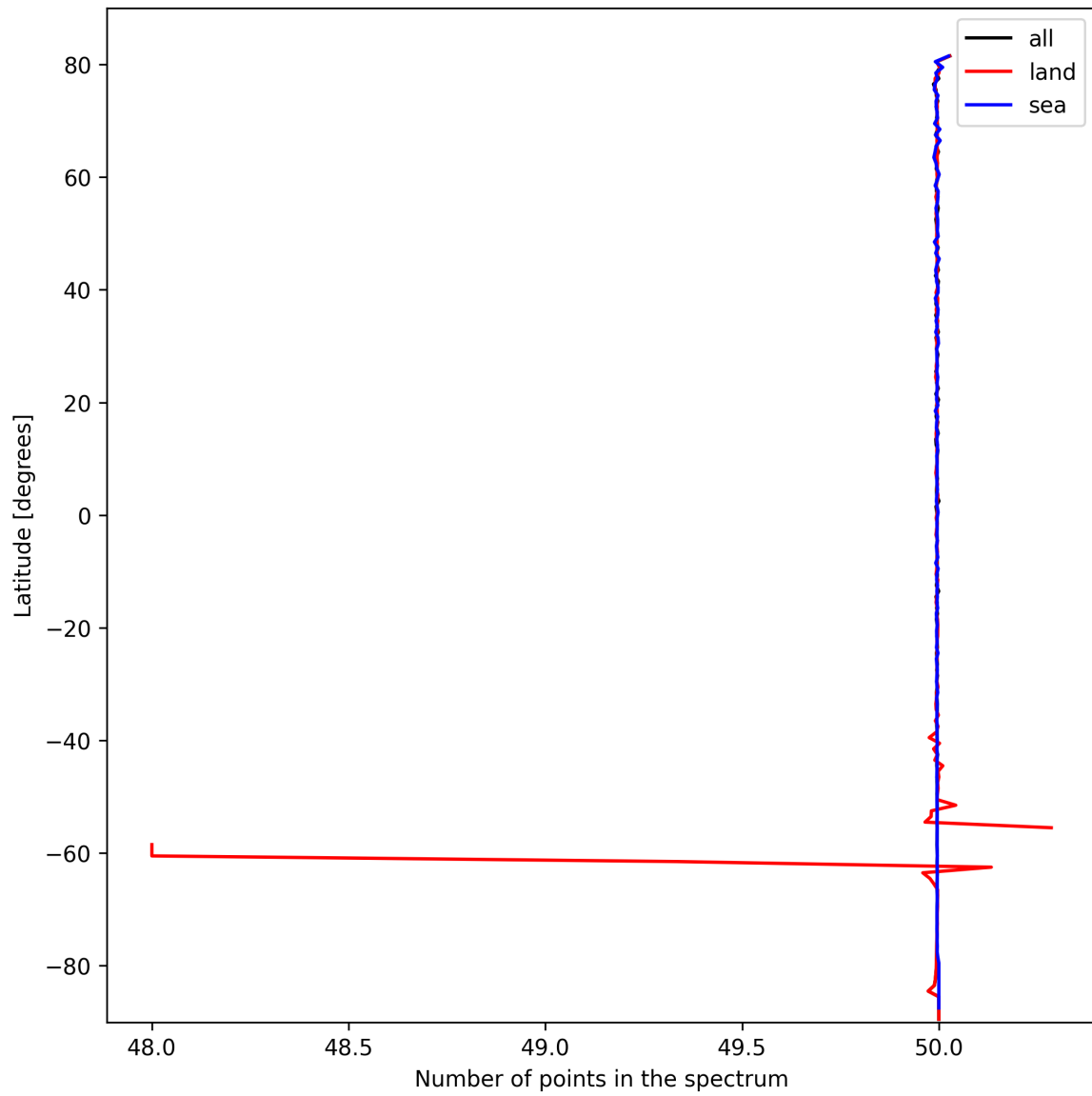
Figure 27: Zonal average of “Number of points in the spectrum” for 2025-10-08 to 2025-10-10.
