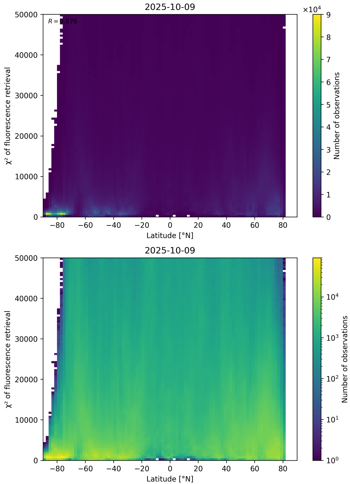
Figure 89: Scatter density plot of “Latitude” against “ \chi^2 of fluorescence retrieval” for 2025-10-08 to 2025-10-10.
