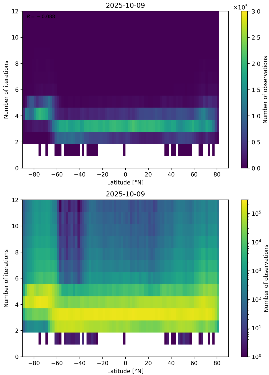
Figure 93: Scatter density plot of “Latitude” against “Number of iterations” for 2025-10-08 to 2025-10-10.
