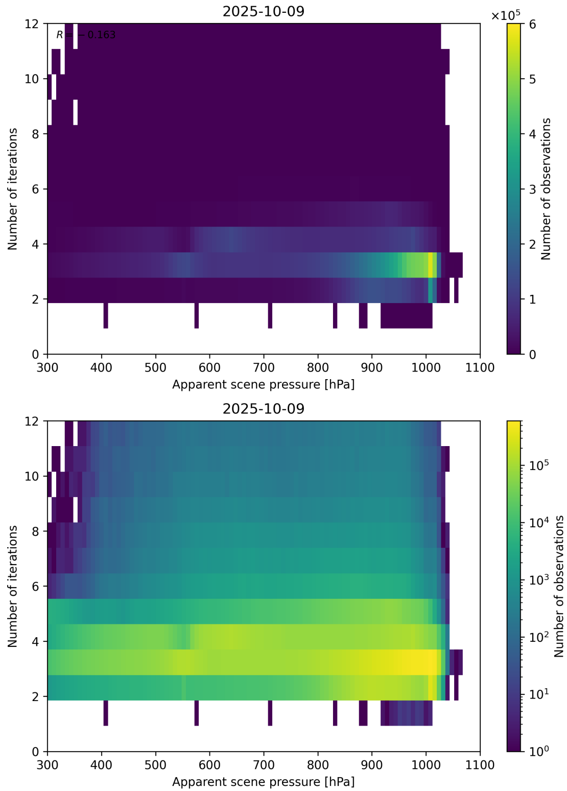
Figure 65: Scatter density plot of “Apparent scene pressure” against “Number of iterations” for 2025-10-08 to 2025-10-10.
