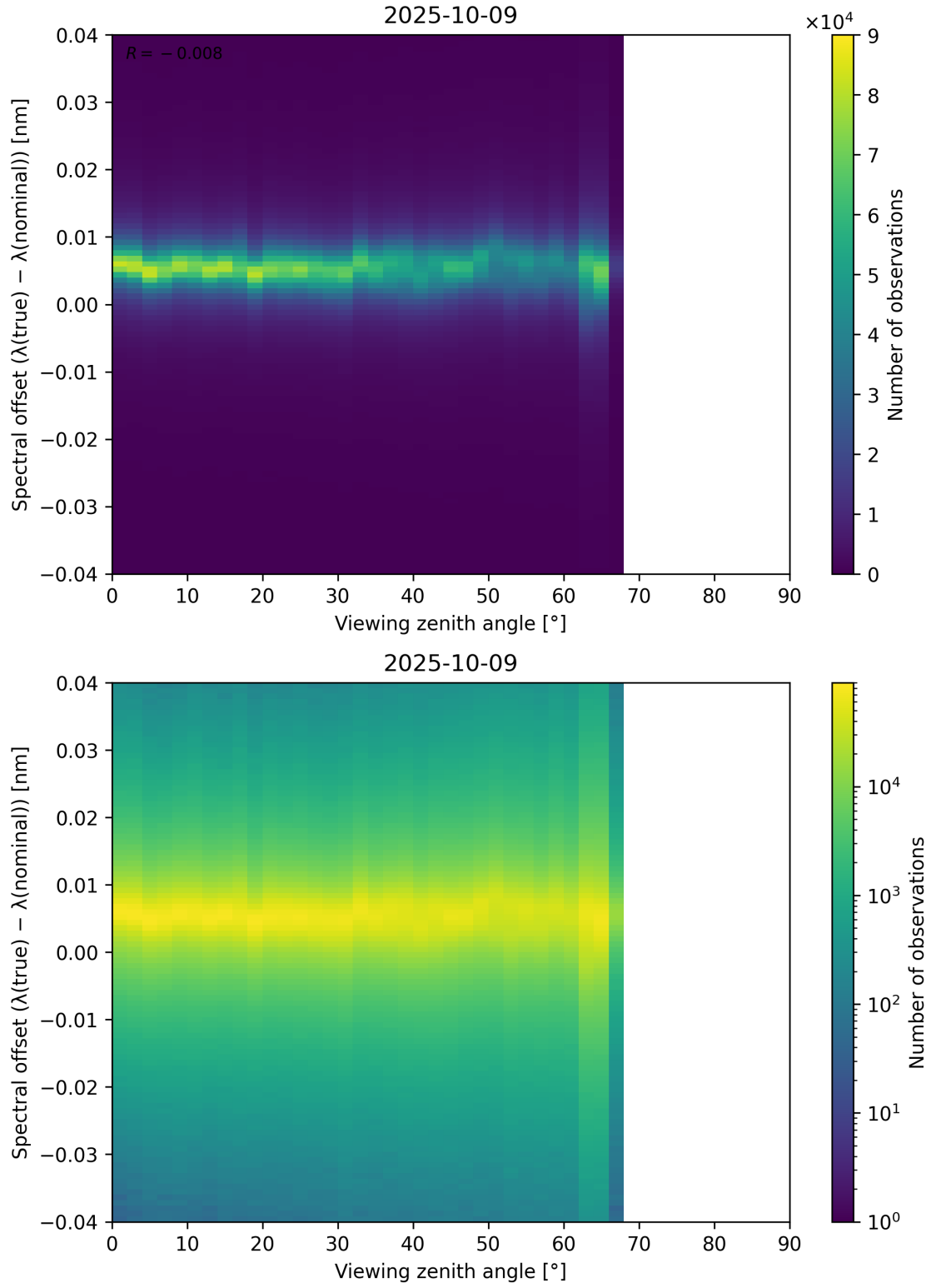
Figure 128: Scatter density plot of “Viewing zenith angle” against “Spectral offset ( \lambda_{\text{true}} - \lambda_{\text{nominal}} )” for 2025-10-08 to 2025-10-10.
