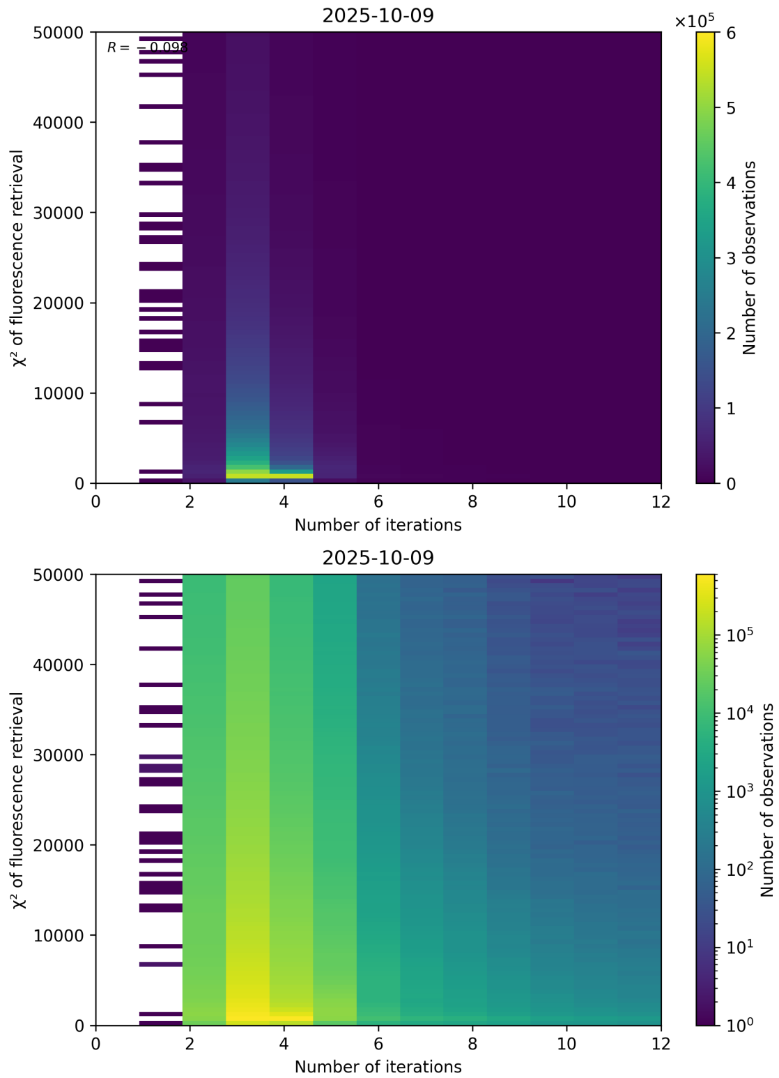
Figure 97: Scatter density plot of “Number of iterations” against “ \chi^2 of fluorescence retrieval” for 2025-10-08 to 2025-10-10.
