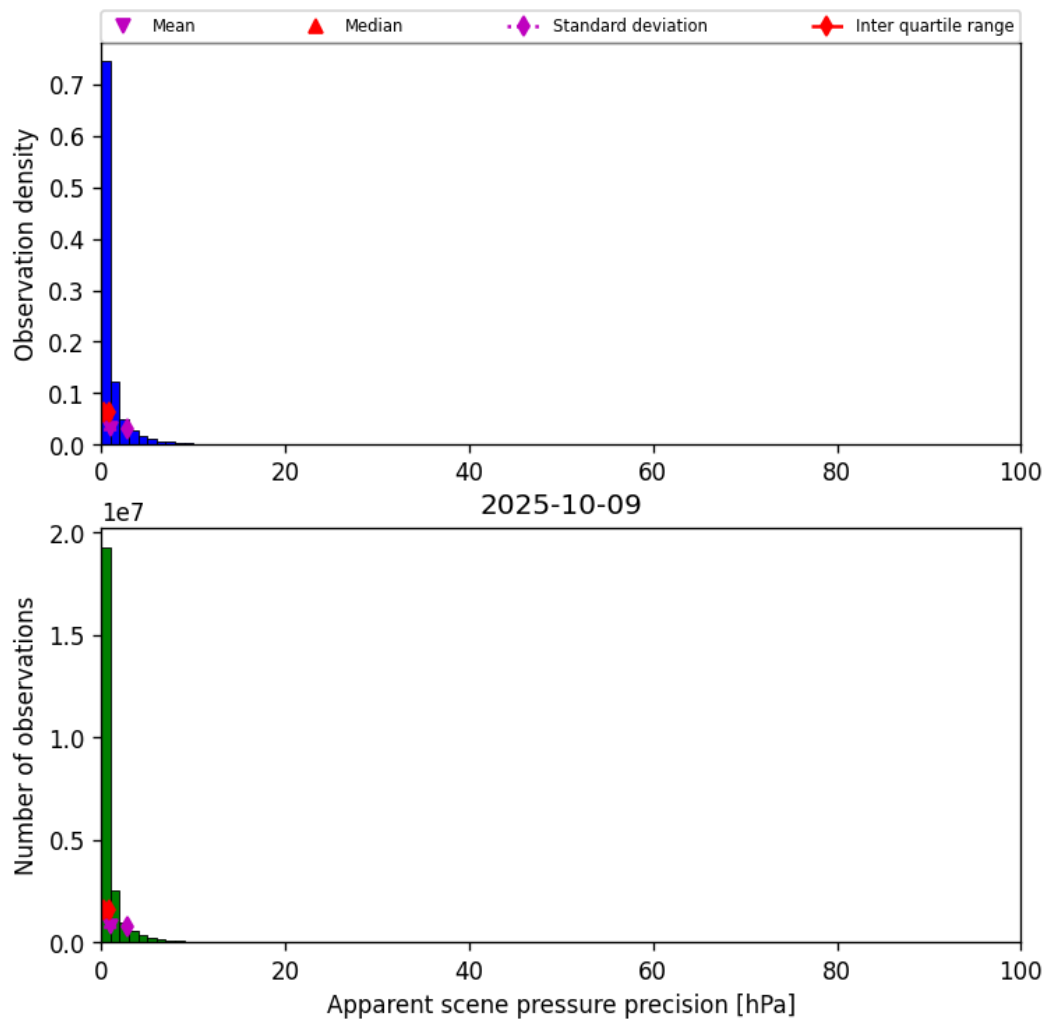
Figure 37: Histogram of “Apparent scene pressure precision” for 2025-10-08 to 2025-10-10
