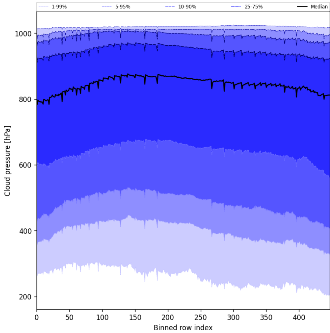
Figure 47: Along track statistics of “Cloud pressure” for 2025-10-08 to 2025-10-10
