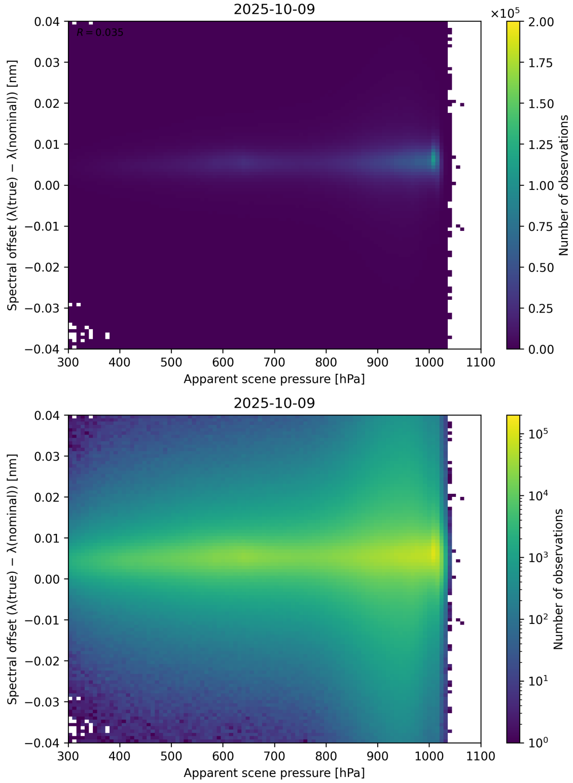
Figure 67: Scatter density plot of “Apparent scene pressure” against “Spectral offset ( \lambda_{\text{true}} - \lambda_{\text{nominal}} )” for 2025-10-08 to 2025-10-10.
