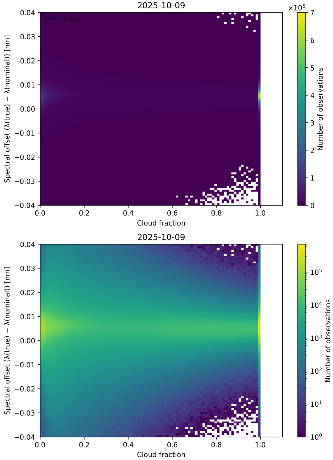
Figure 76: Scatter density plot of “Cloud fraction” against “Spectral offset ( \lambda_{\text{true}} - \lambda_{\text{nominal}} )” for 2025-10-08 to 2025-10-10.
