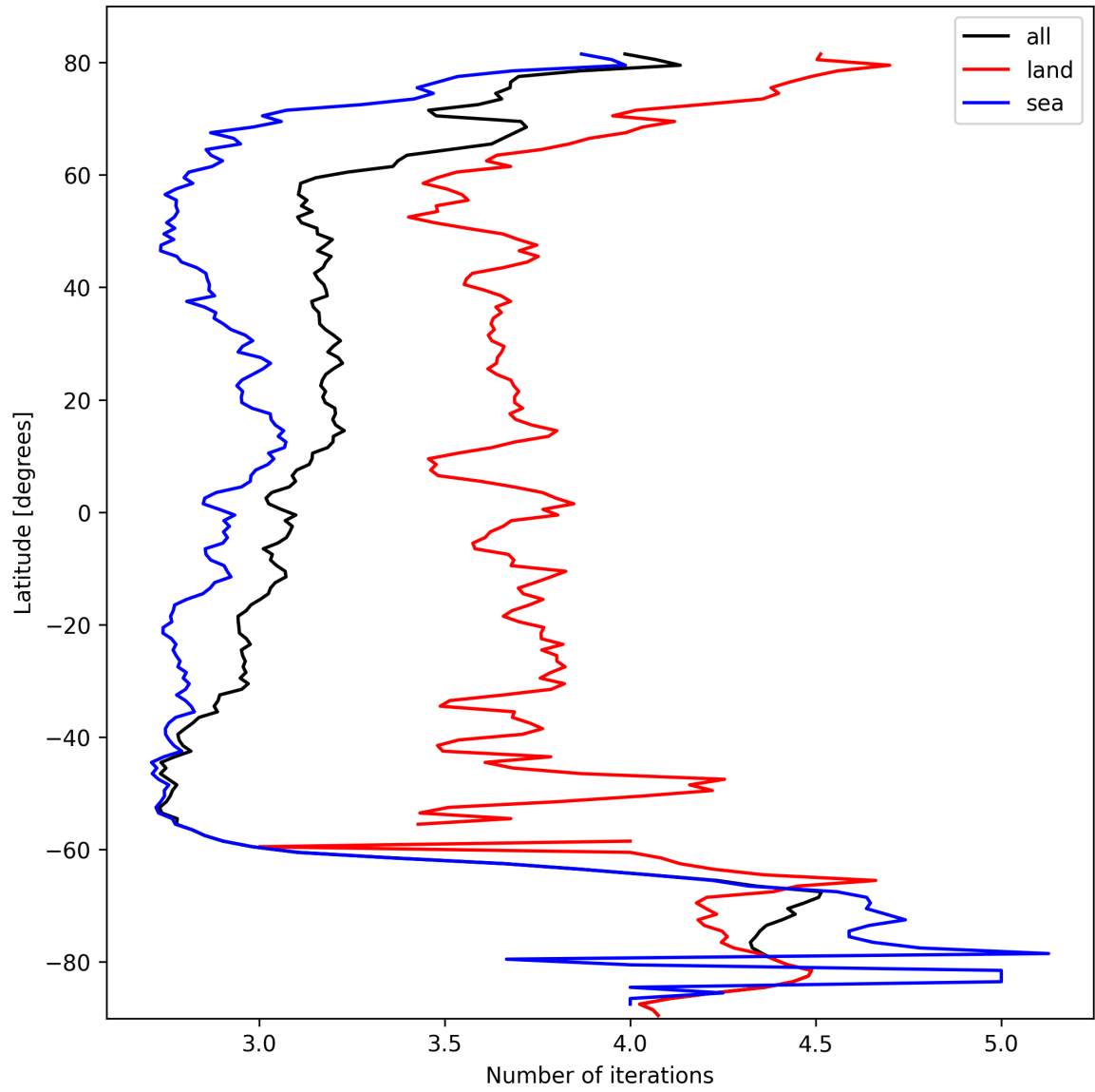
Figure 22: Zonal average of “Number of iterations” for 2025-10-08 to 2025-10-10.
