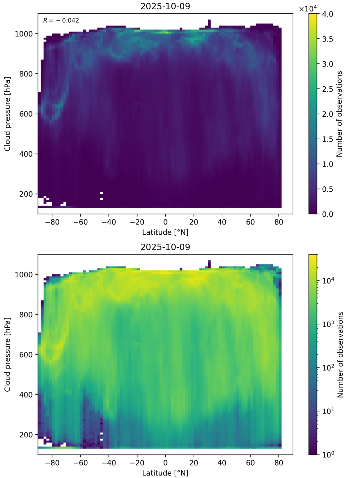
Figure 91: Scatter density plot of “Latitude” against “Cloud pressure” for 2025-10-08 to 2025-10-10.
