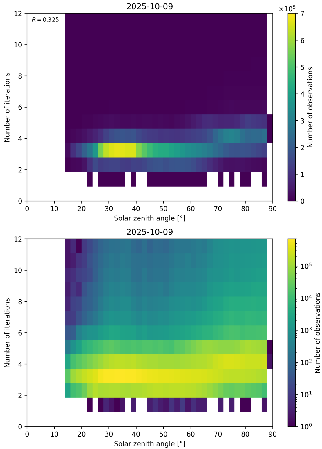
Figure 114: Scatter density plot of “Solar zenith angle” against “Number of iterations” for 2025-10-08 to 2025-10-10.
