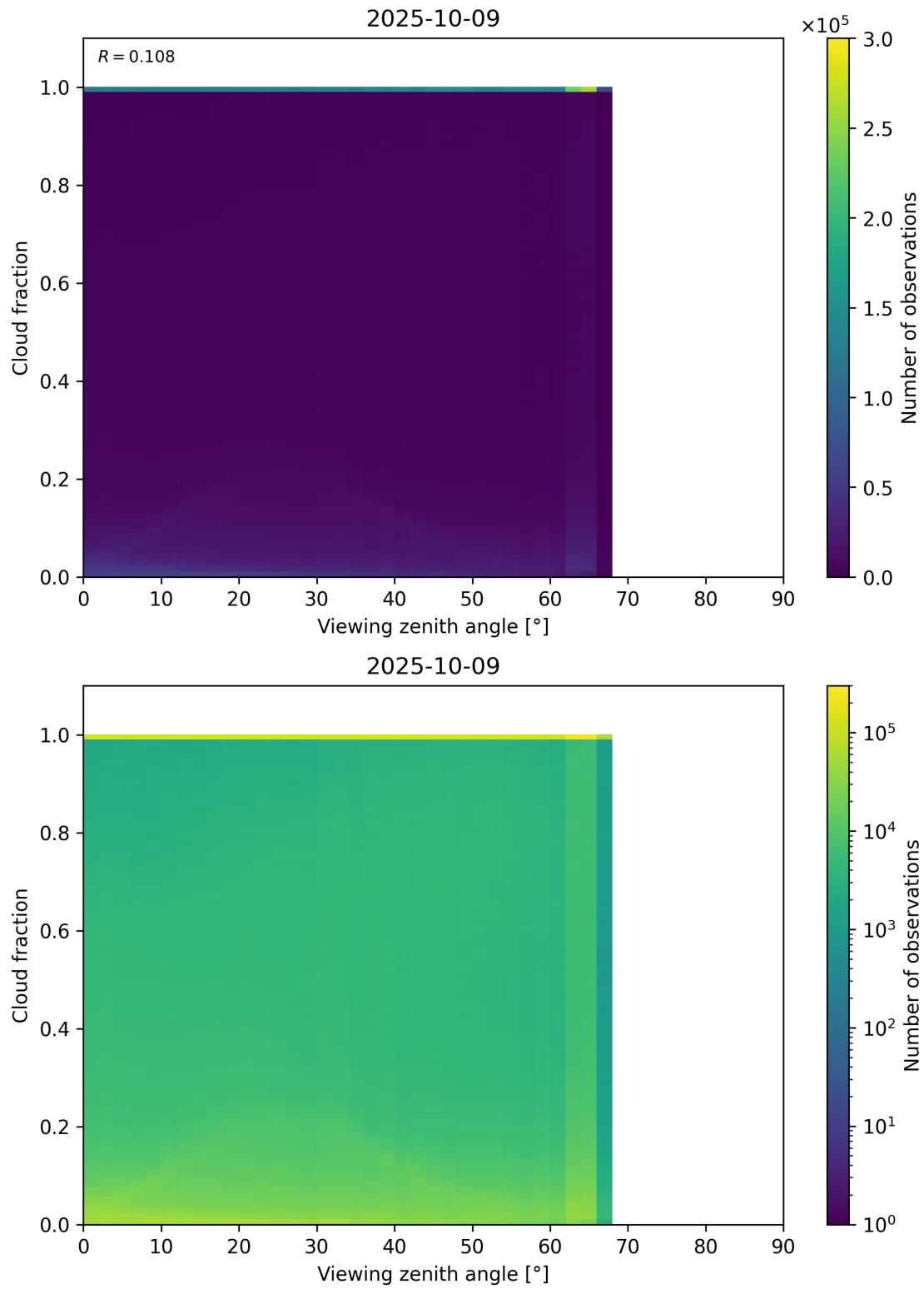
Figure 120: Scatter density plot of “Viewing zenith angle” against “Cloud fraction” for 2025-10-08 to 2025-10-10.
