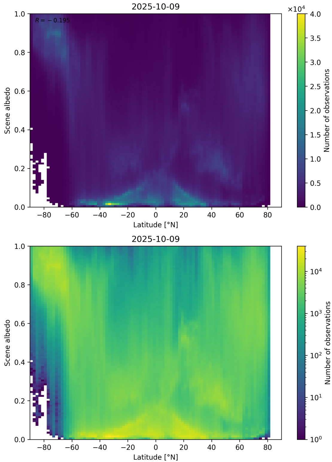
Figure 95: Scatter density plot of “Latitude” against “Scene albedo” for 2025-10-08 to 2025-10-10.
