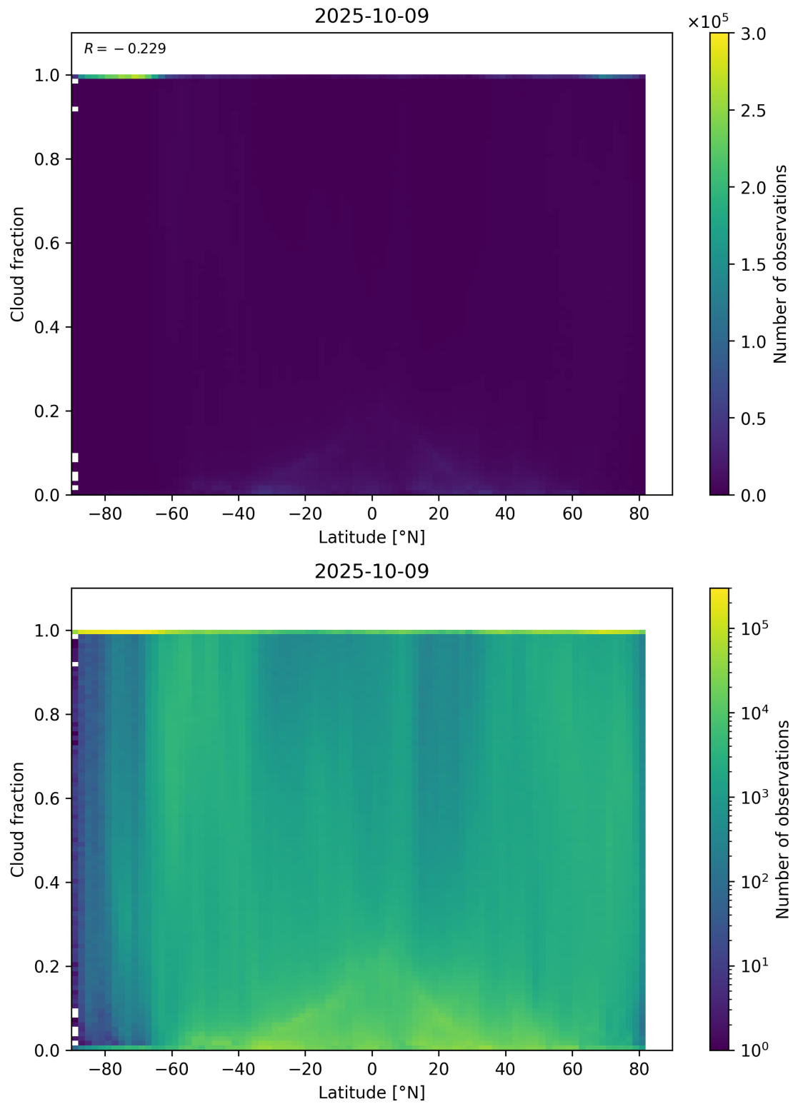
Figure 90: Scatter density plot of “Latitude” against “Cloud fraction” for 2025-10-08 to 2025-10-10.
