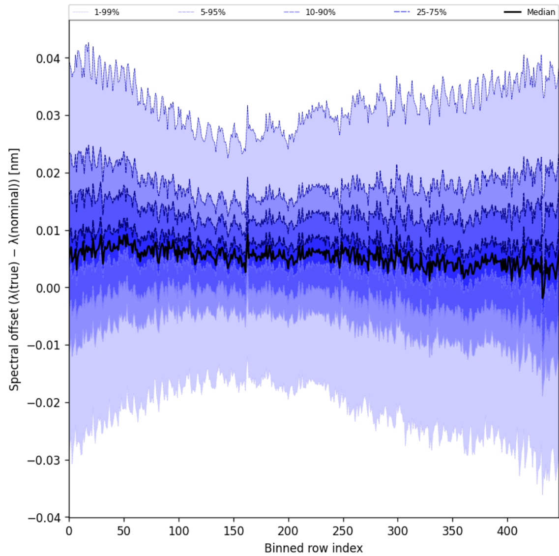
Figure 62: Along track statistics of “Spectral offset ( \lambda_{\text{true}} - \lambda_{\text{nominal}} )” for 2025-10-08 to 2025-10-10
