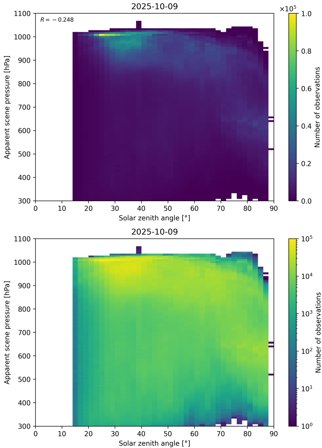
Figure 108: Scatter density plot of “Solar zenith angle” against “Apparent scene pressure” for 2025-10-08 to 2025-10-10.
