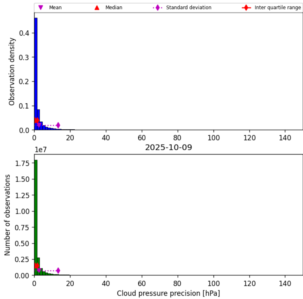
Figure 31: Histogram of “Cloud pressure precision” for 2025-10-08 to 2025-10-10
