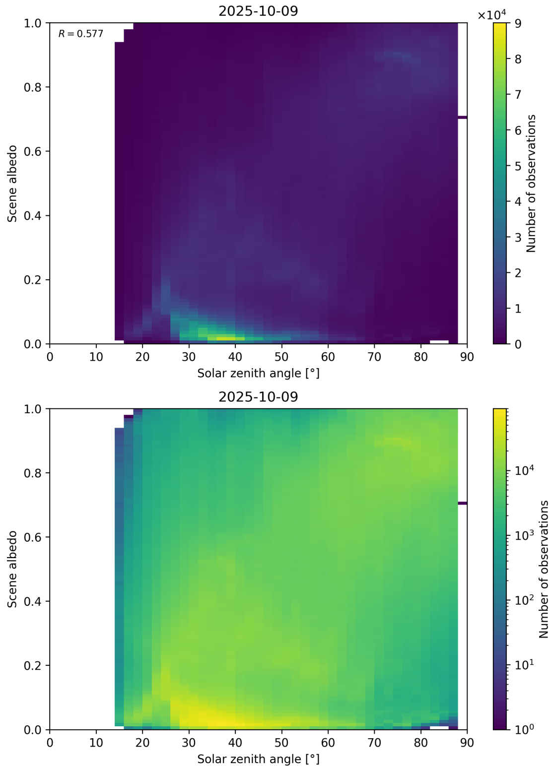
Figure 116: Scatter density plot of “Solar zenith angle” against “Scene albedo” for 2025-10-08 to 2025-10-10.
