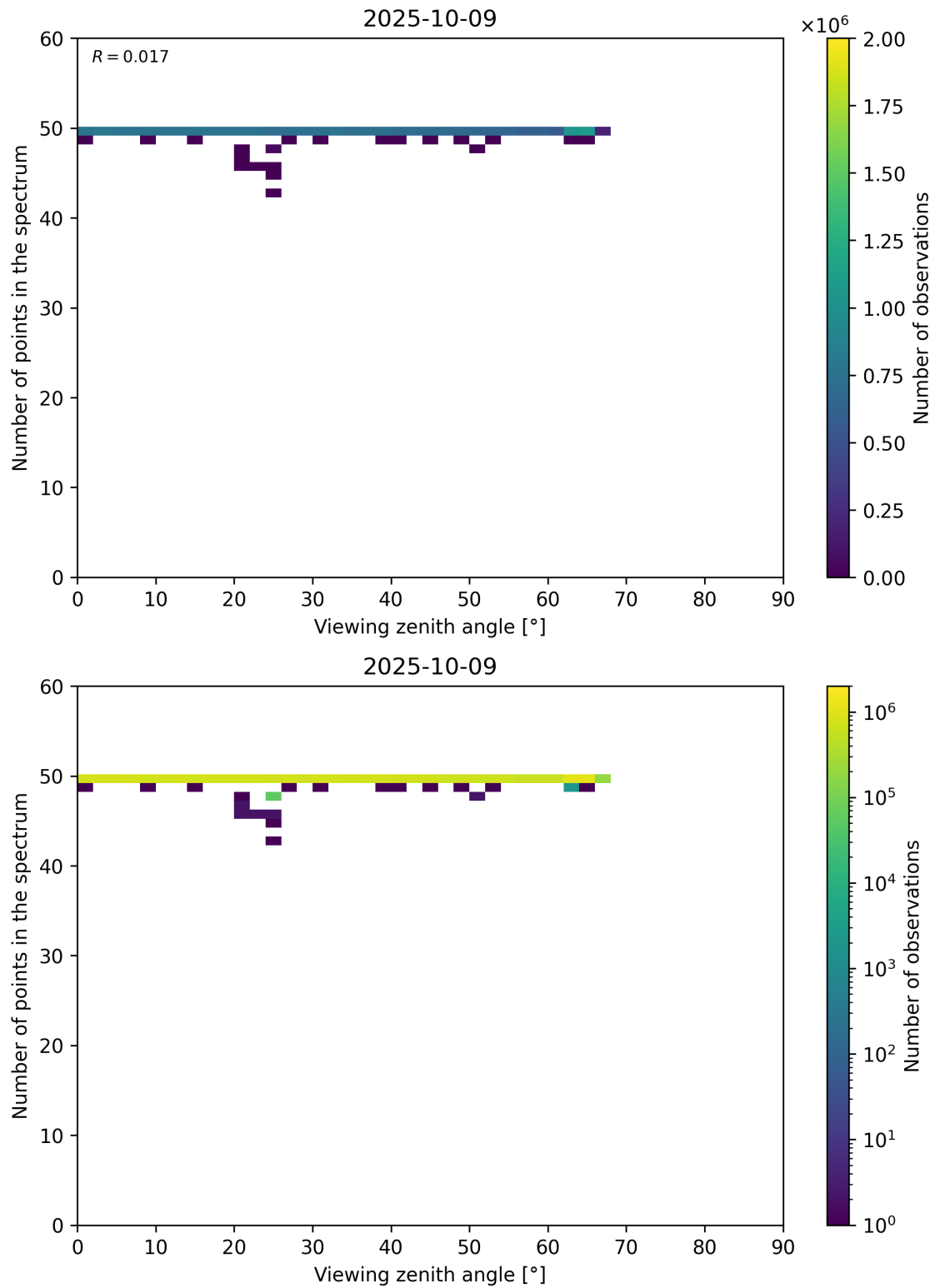
Figure 125: Scatter density plot of “Viewing zenith angle” against “Number of points in the spectrum” for 2025-10-08 to 2025-10-10.
