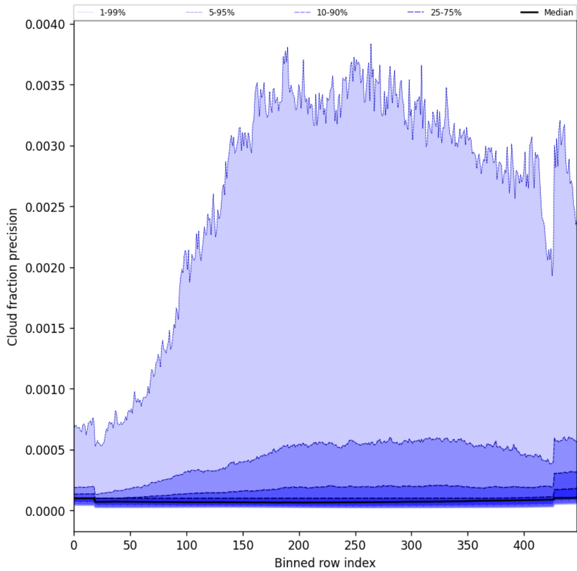
Figure 50: Along track statistics of “Cloud fraction precision” for 2025-10-08 to 2025-10-10
