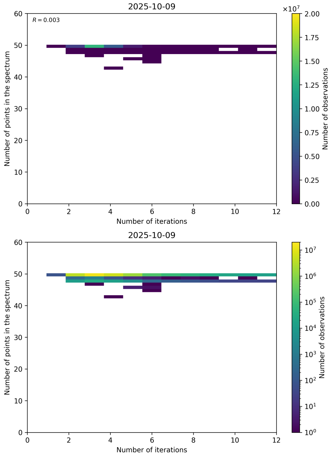
Figure 99: Scatter density plot of “Number of iterations” against “Number of points in the spectrum” for 2025-10-08 to 2025-10-10.
