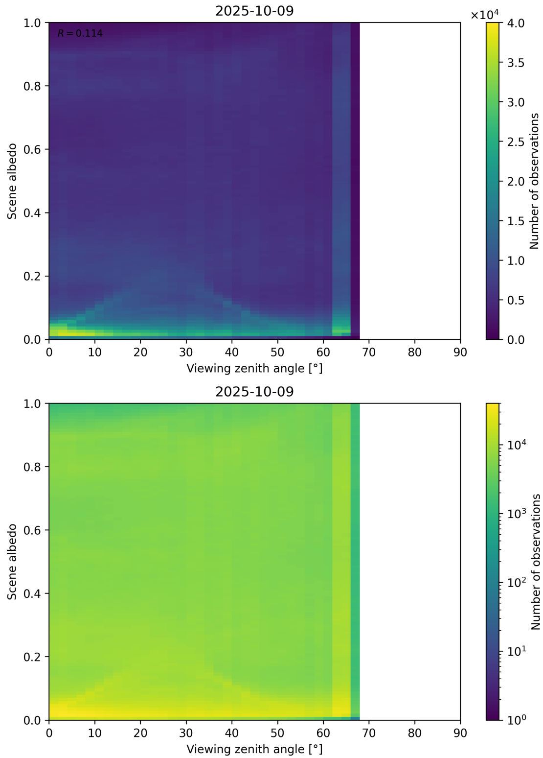
Figure 126: Scatter density plot of “Viewing zenith angle” against “Scene albedo” for 2025-10-08 to 2025-10-10.
