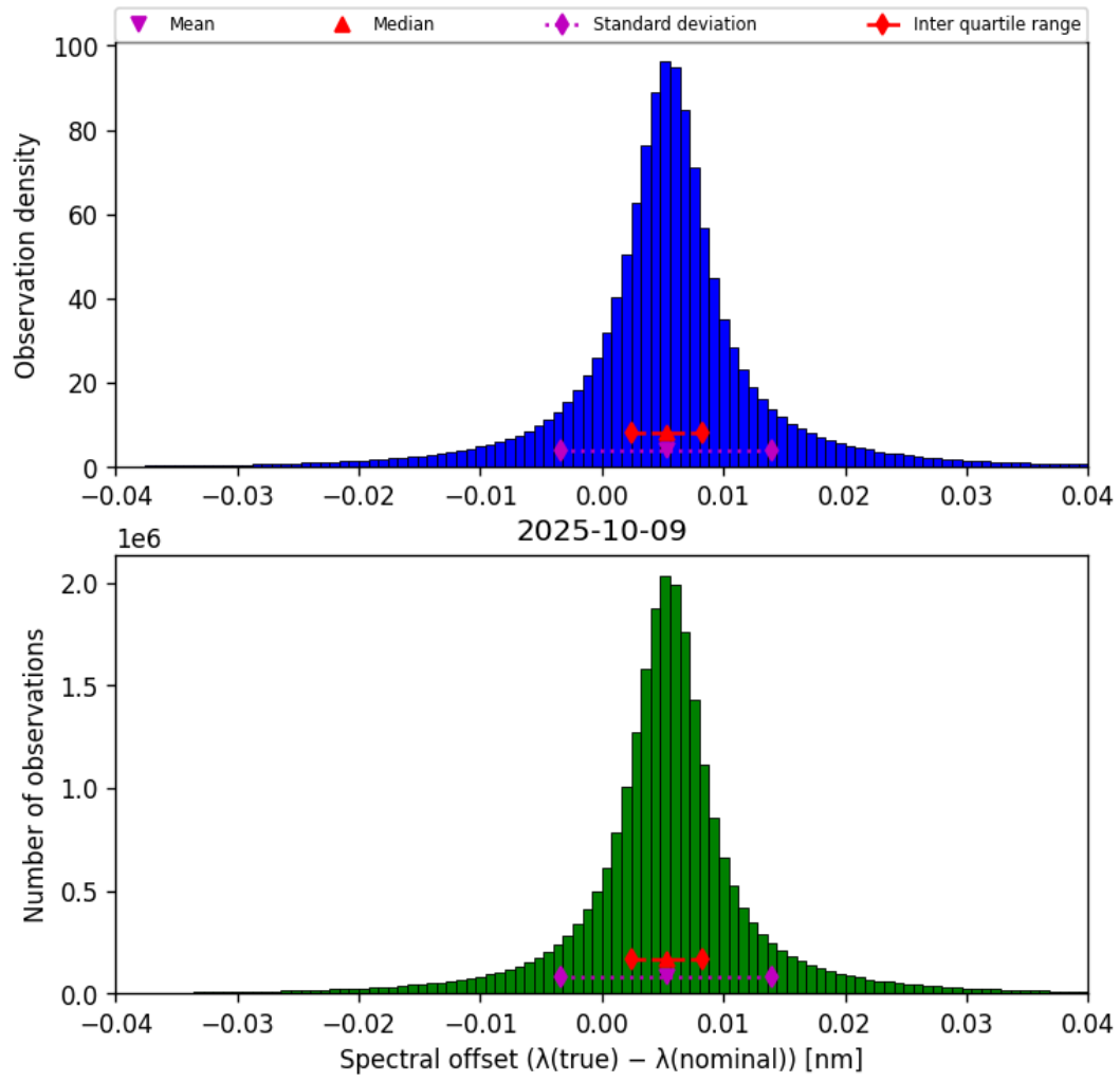
Figure 45: Histogram of “Spectral offset ( \lambda_{\text{true}} - \lambda_{\text{nominal}} )” for 2025-10-08 to 2025-10-10
