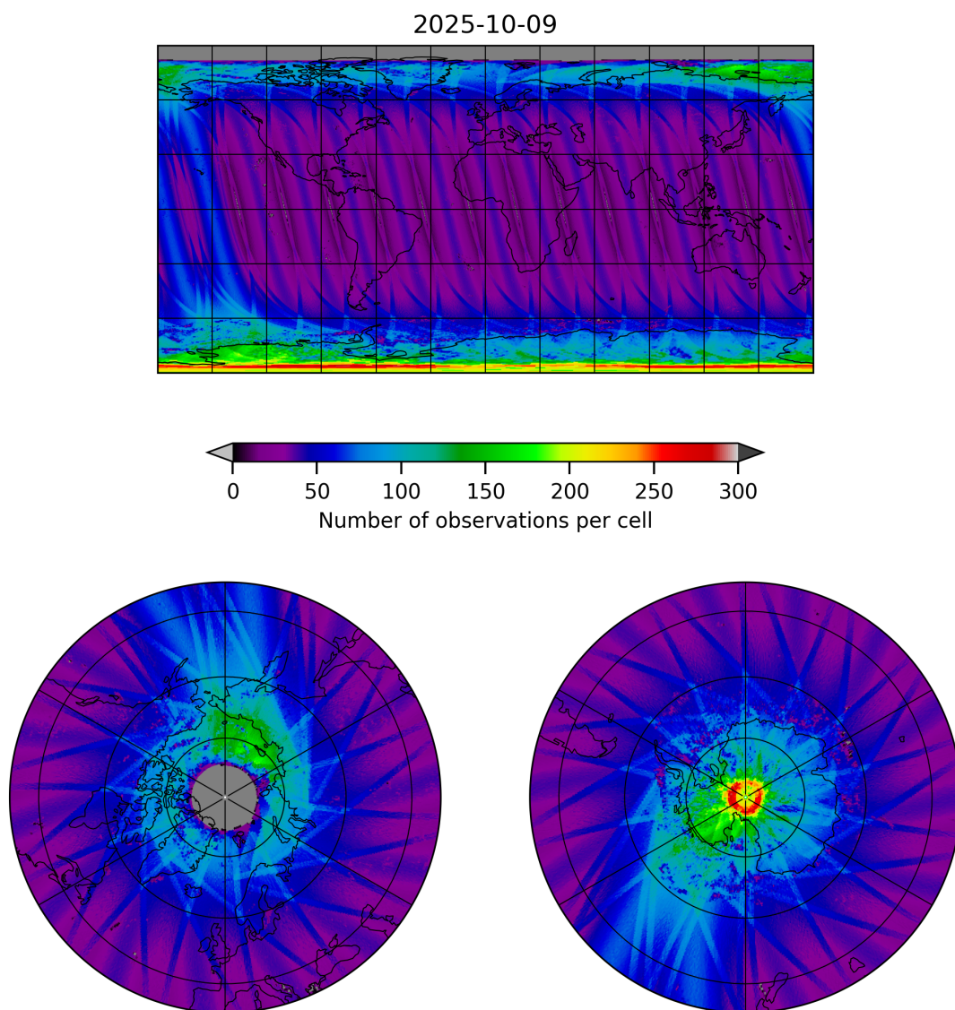
Figure 11: Map of the number of observations for 2025-10-08 to 2025-10-10
