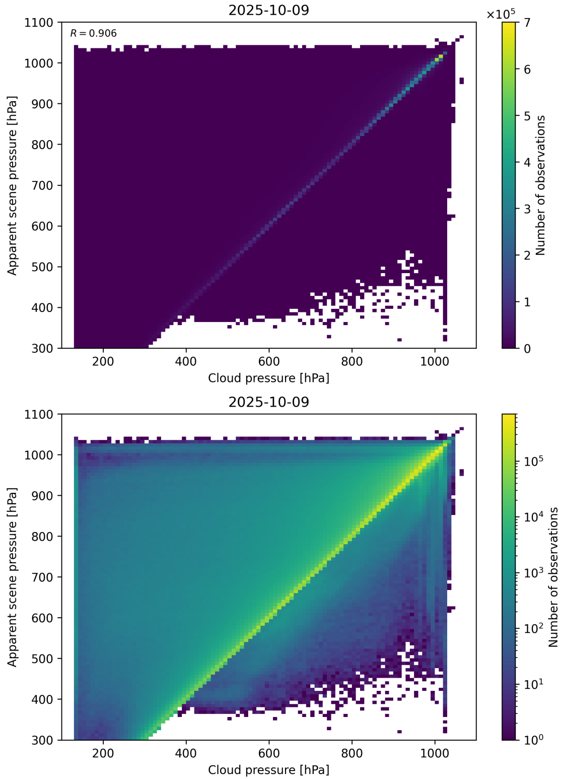
Figure 77: Scatter density plot of “Cloud pressure” against “Apparent scene pressure” for 2025-10-08 to 2025-10-10.
