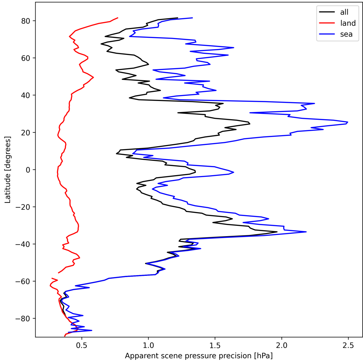
Figure 20: Zonal average of “Apparent scene pressure precision” for 2025-10-08 to 2025-10-10.
