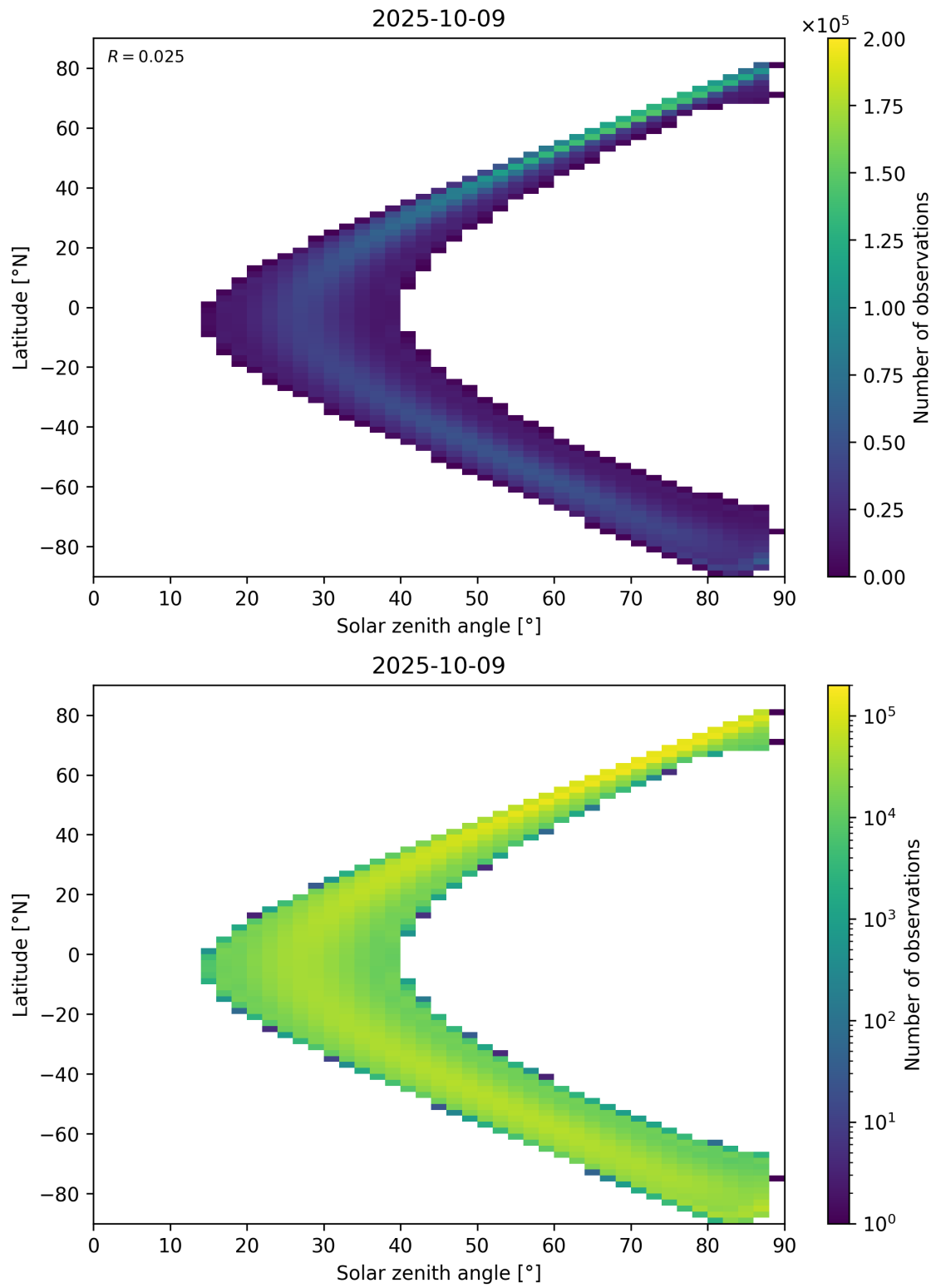
Figure 113: Scatter density plot of “Solar zenith angle” against “Latitude” for 2025-10-08 to 2025-10-10.
