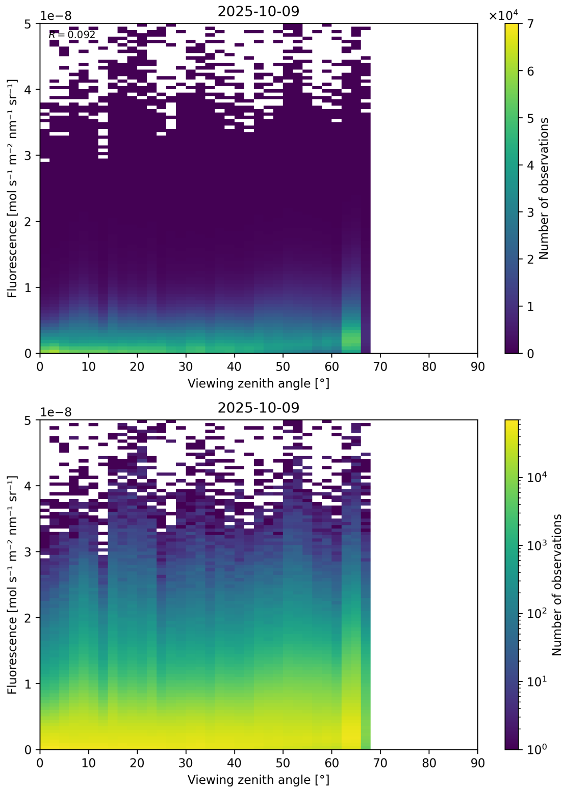
Figure 122: Scatter density plot of “Viewing zenith angle” against “Fluorescence” for 2025-10-08 to 2025-10-10.
