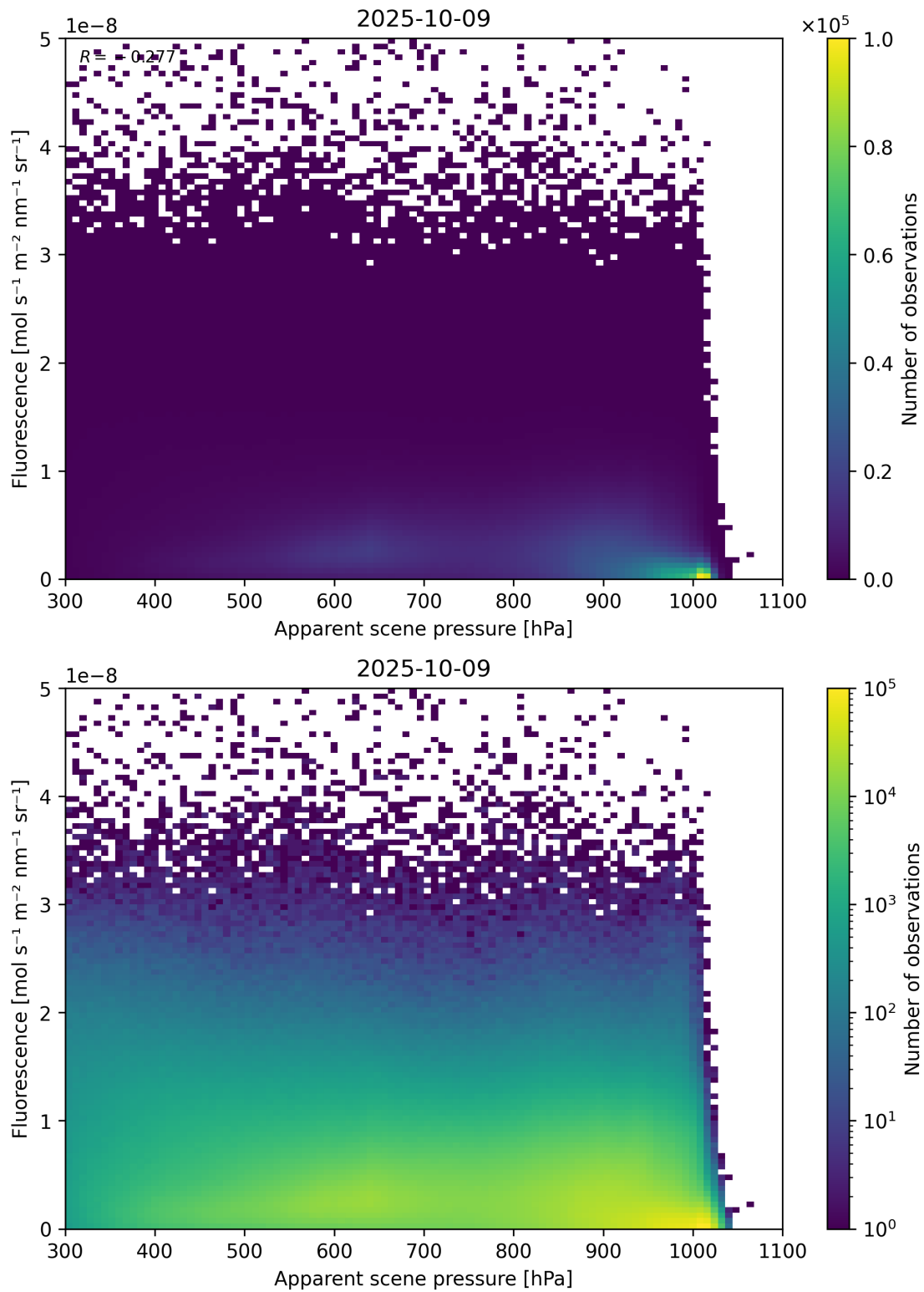
Figure 64: Scatter density plot of “Apparent scene pressure” against “Fluorescence” for 2025-10-08 to 2025-10-10.
