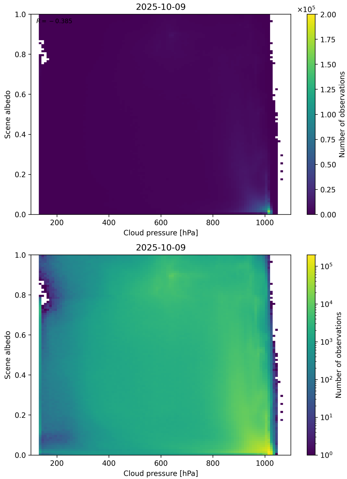
Figure 83: Scatter density plot of “Cloud pressure” against “Scene albedo” for 2025-10-08 to 2025-10-10.
