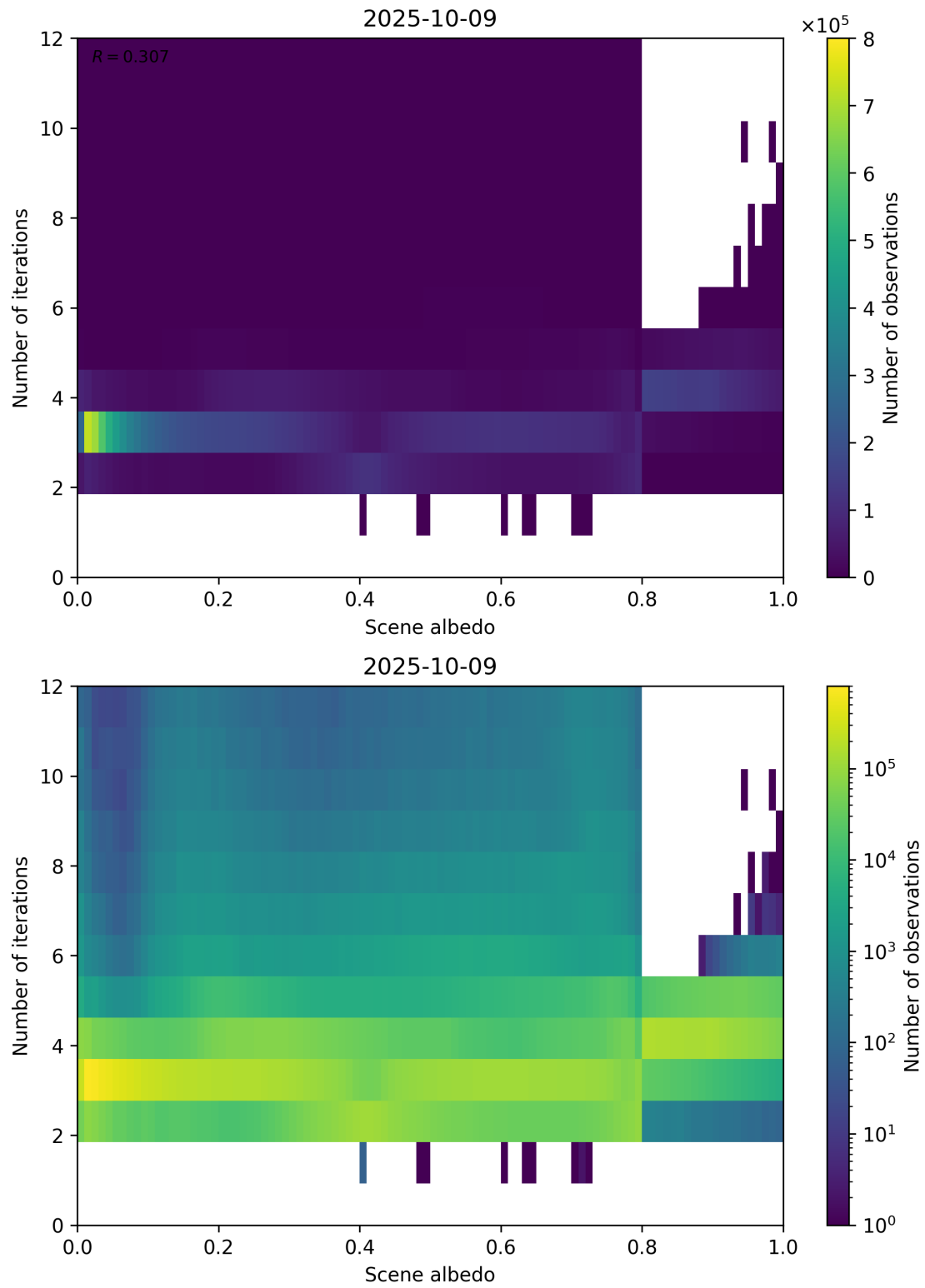
Figure 105: Scatter density plot of “Scene albedo” against “Number of iterations” for 2025-10-08 to 2025-10-10.
