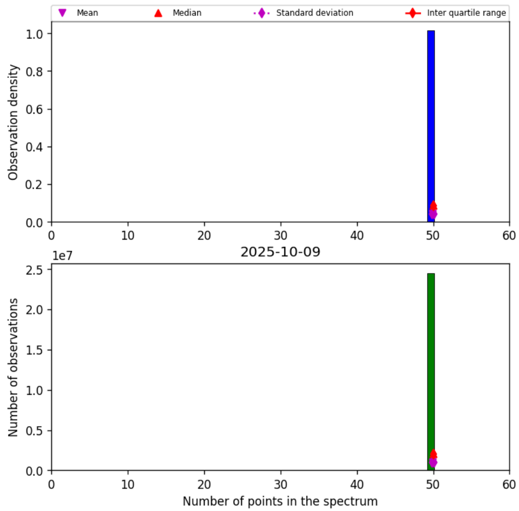
Figure 44: Histogram of “Number of points in the spectrum” for 2025-10-08 to 2025-10-10
