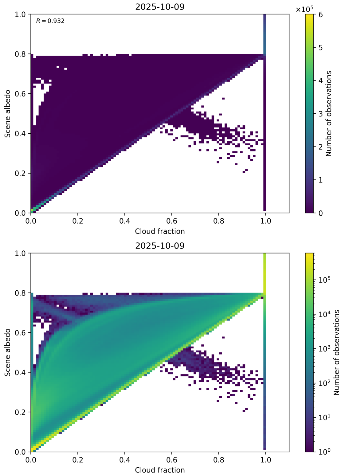
Figure 75: Scatter density plot of “Cloud fraction” against “Scene albedo” for 2025-10-08 to 2025-10-10.
