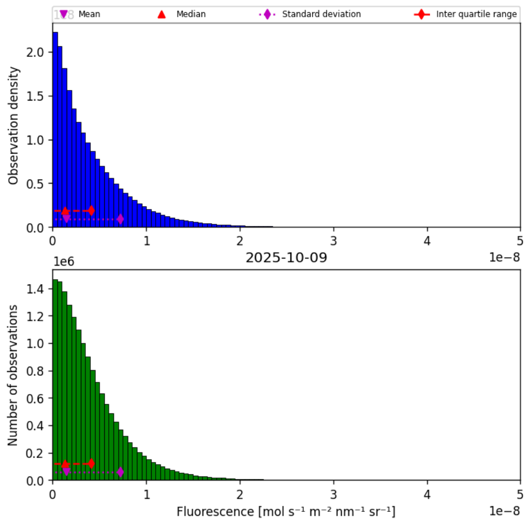
Figure 40: Histogram of “Fluorescence” for 2025-10-08 to 2025-10-10
