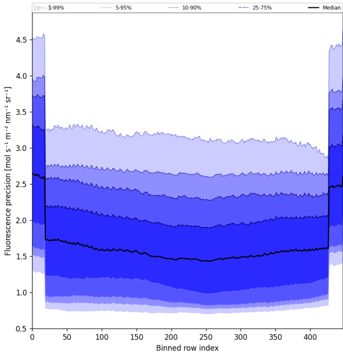
Figure 58: Along track statistics of "Fluorescence precision" for 2025-10-08 to 2025-10-10
