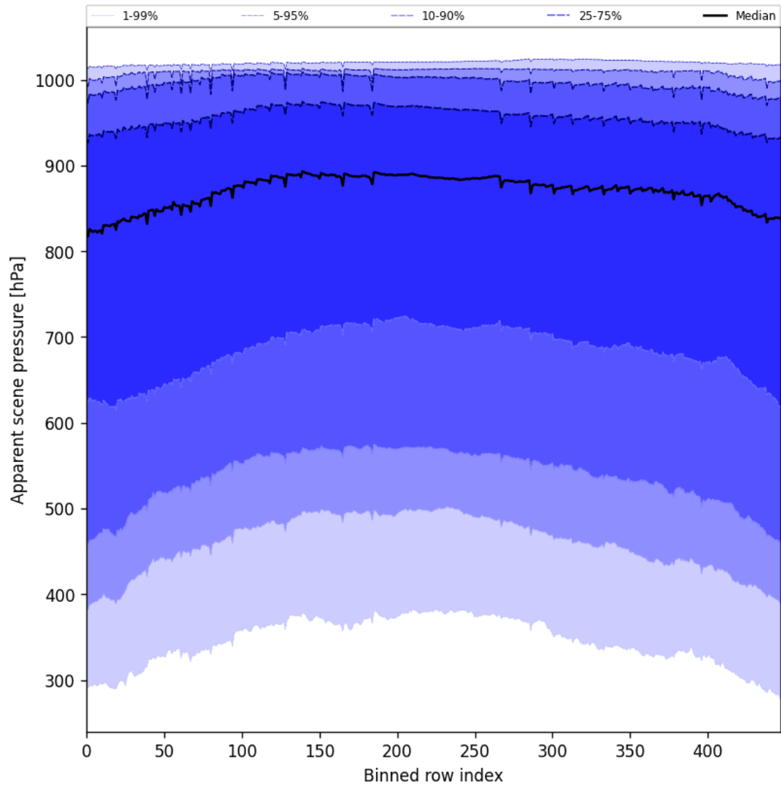
Figure 53: Along track statistics of “Apparent scene pressure” for 2025-10-08 to 2025-10-10
