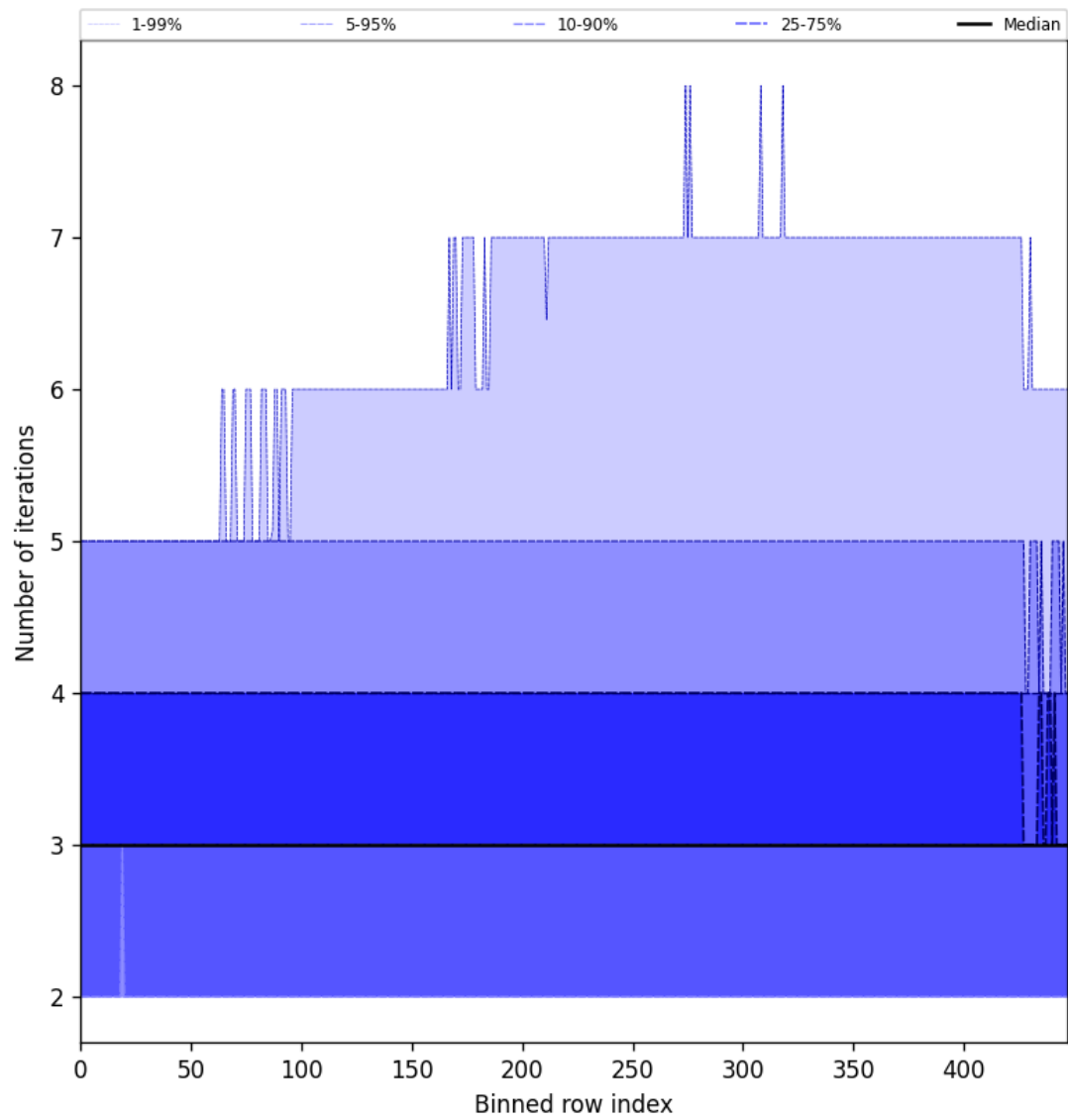
Figure 56: Along track statistics of “Number of iterations” for 2025-10-08 to 2025-10-10
