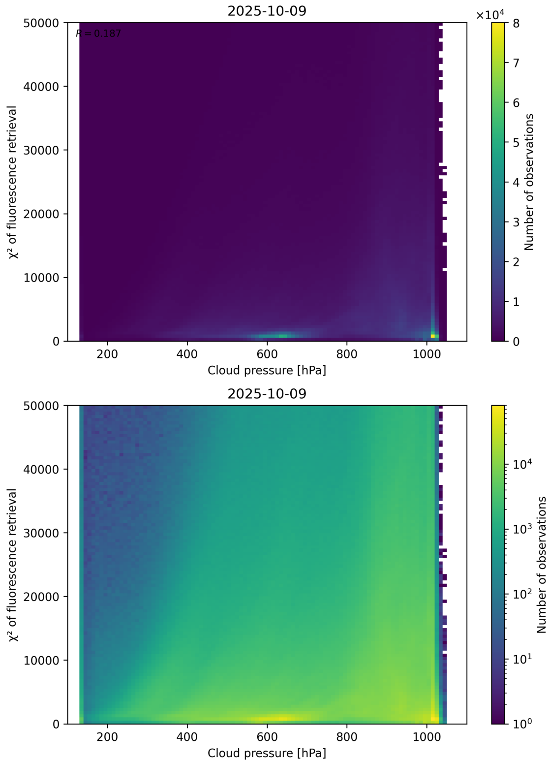
Figure 78: Scatter density plot of “Cloud pressure” against “ \chi^2 of fluorescence retrieval” for 2025-10-08 to 2025-10-10.
