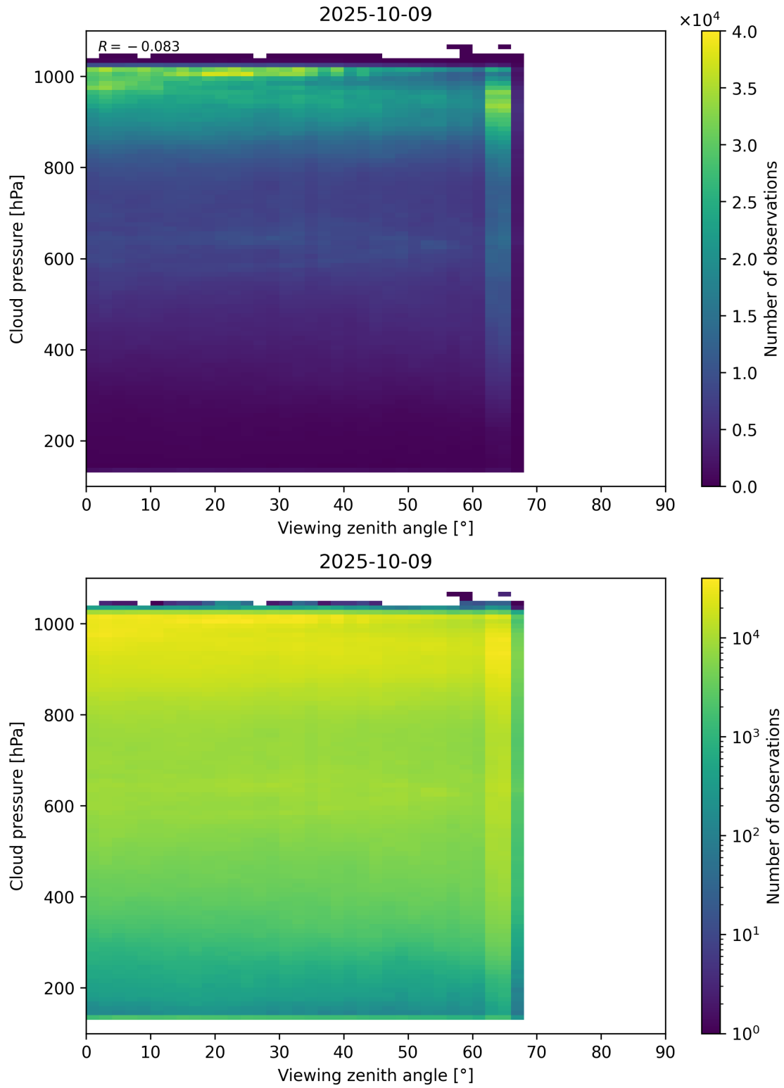
Figure 121: Scatter density plot of “Viewing zenith angle” against “Cloud pressure” for 2025-10-08 to 2025-10-10.
