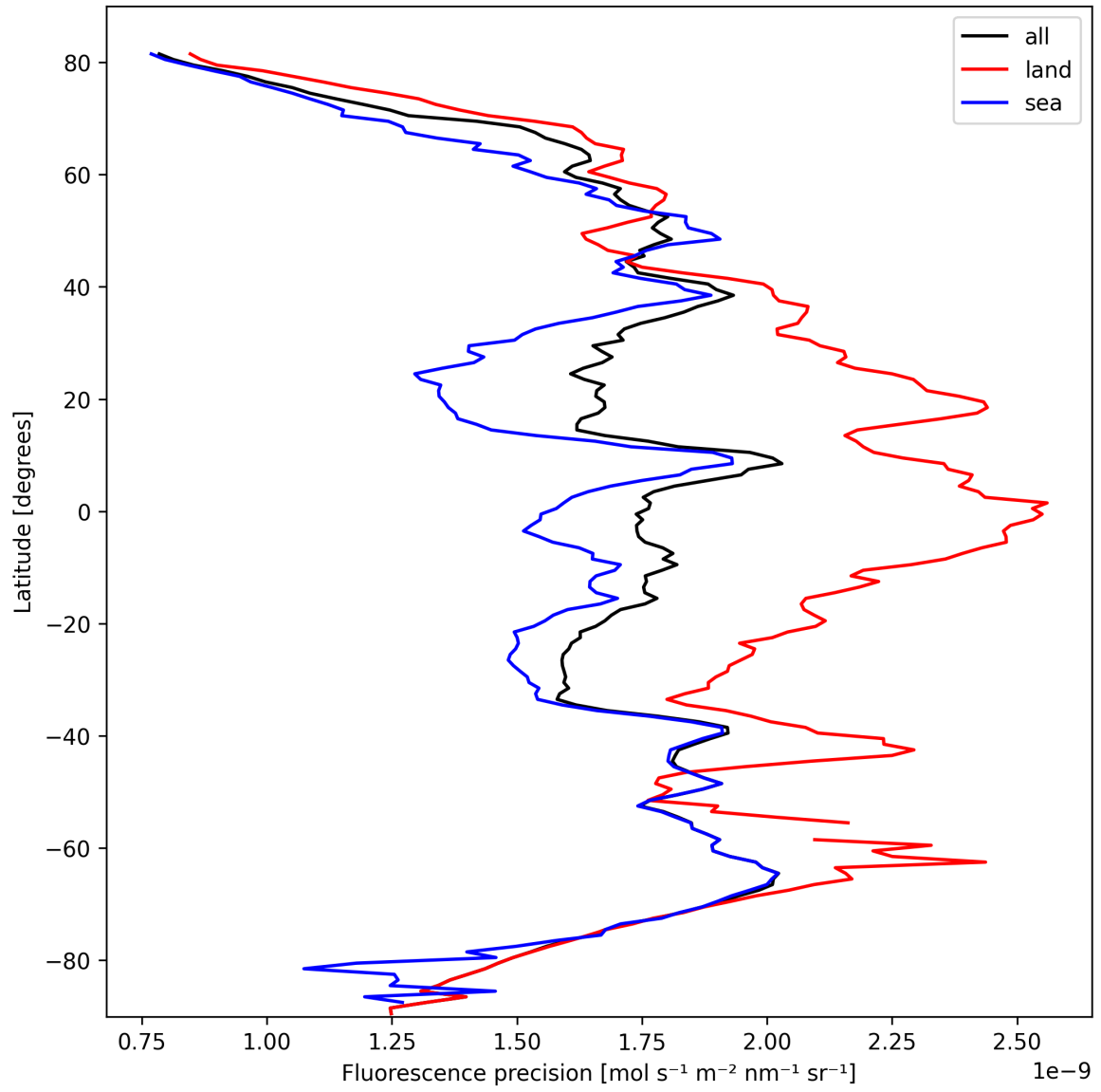
Figure 24: Zonal average of “Fluorescence precision” for 2025-10-08 to 2025-10-10.
