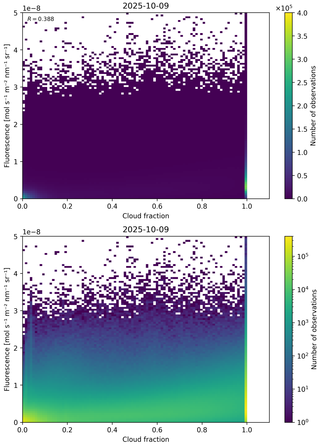
Figure 72: Scatter density plot of “Cloud fraction” against “Fluorescence” for 2025-10-08 to 2025-10-10.
