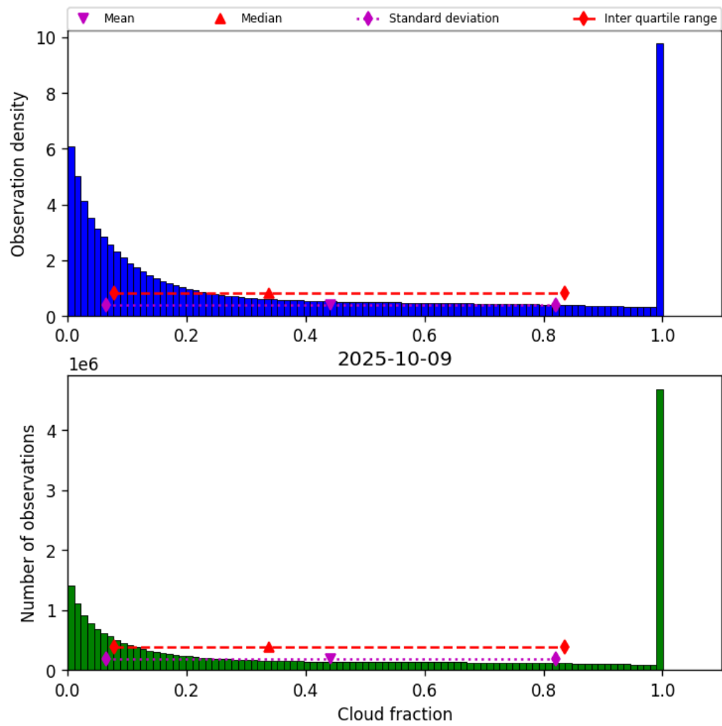
Figure 32: Histogram of “Cloud fraction” for 2025-10-08 to 2025-10-10
