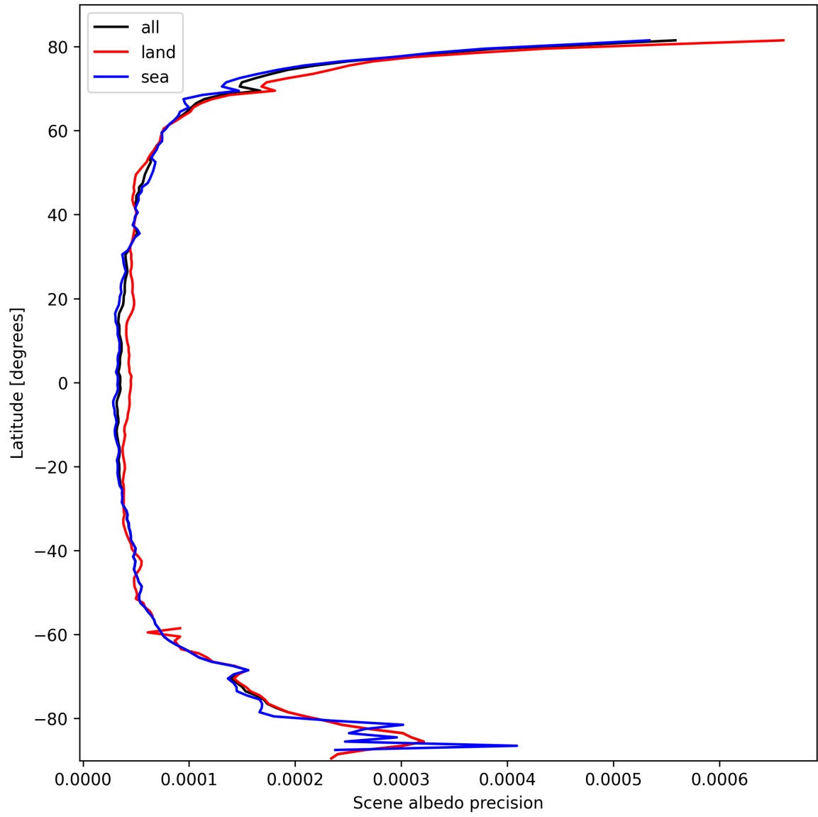
Figure 18: Zonal average of “Scene albedo precision” for 2025-10-08 to 2025-10-10.
