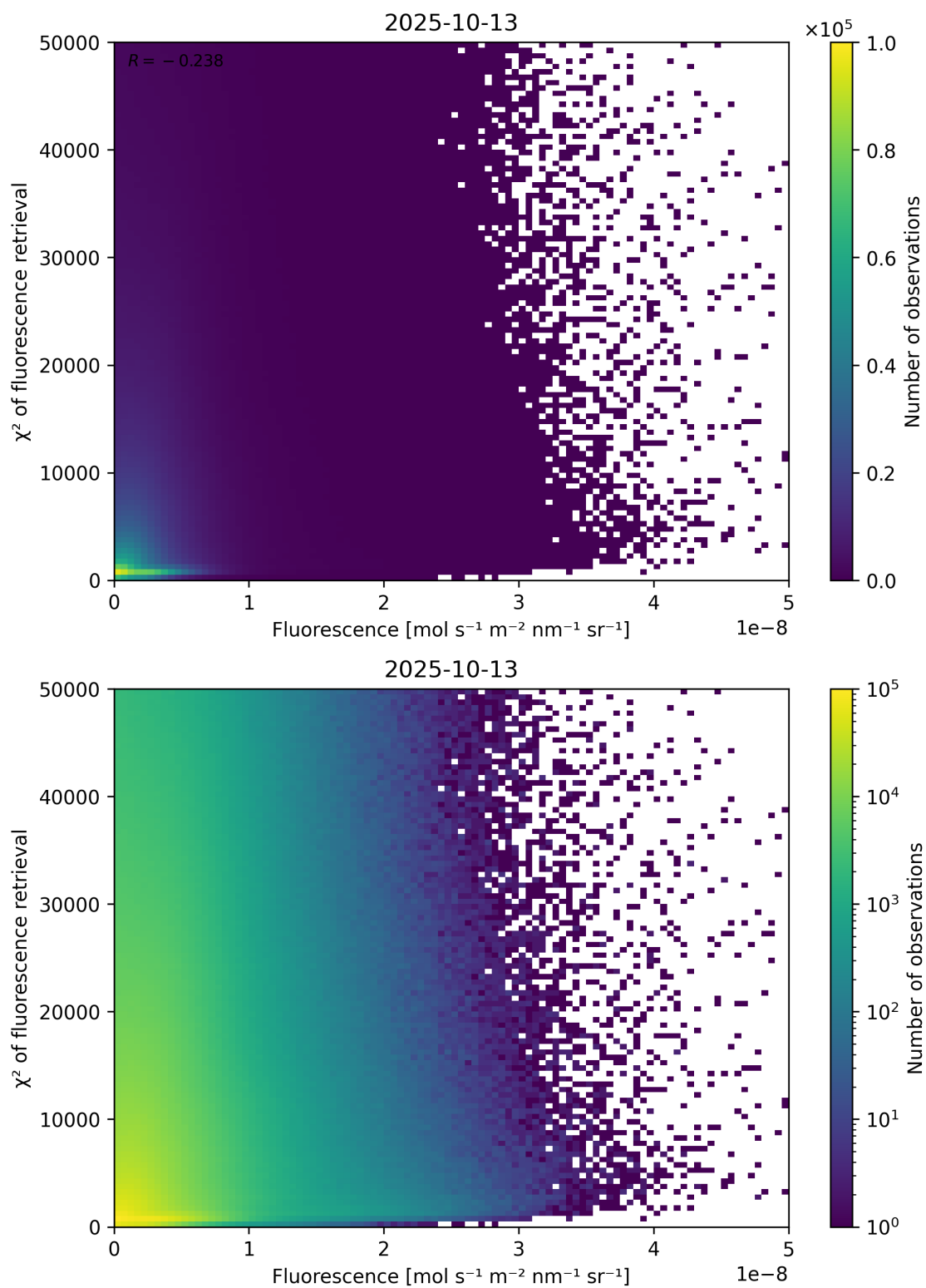
Figure 85: Scatter density plot of “Fluorescence” against “ \chi^2 of fluorescence retrieval” for 2025-10-12 to 2025-10-14.
