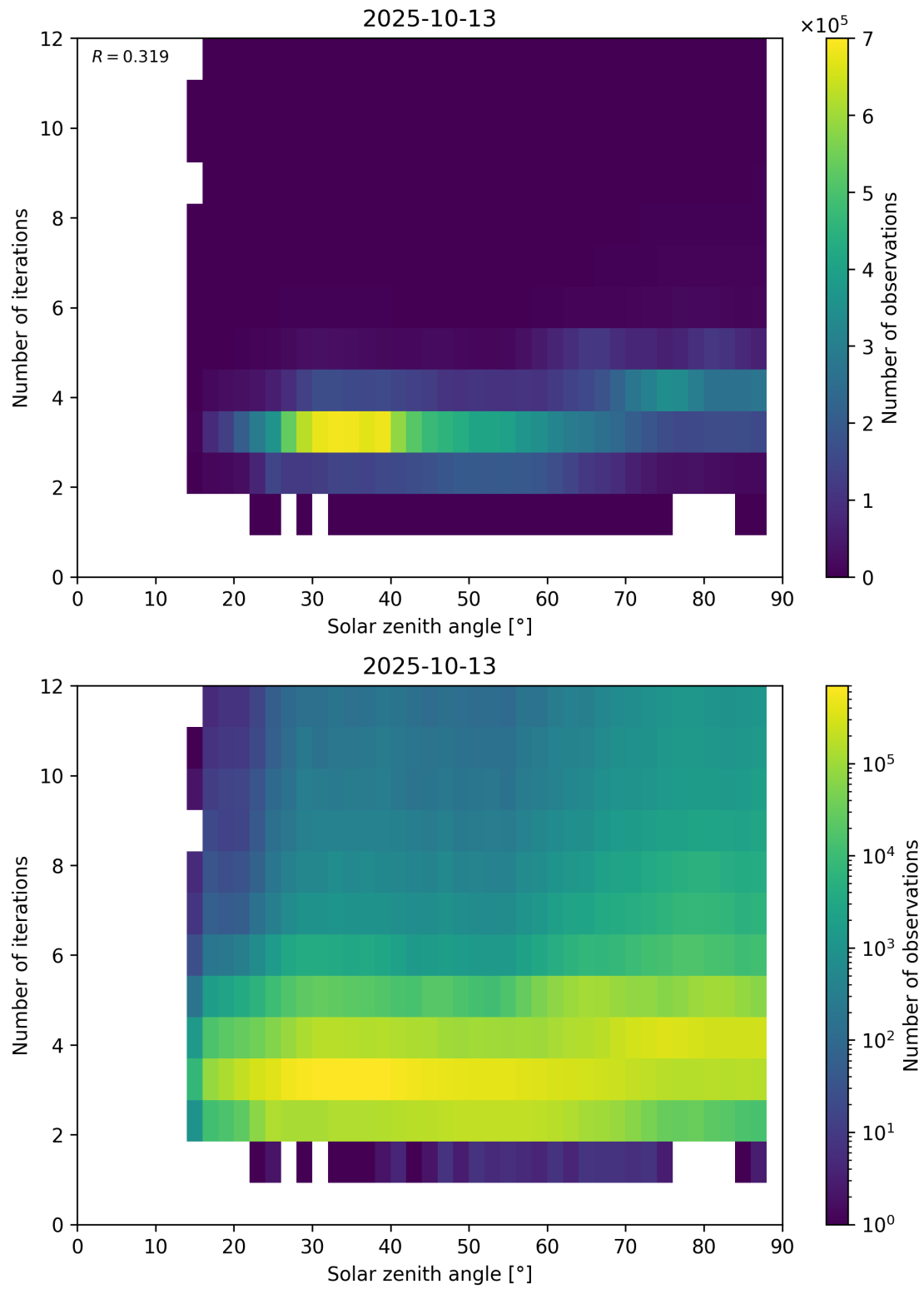
Figure 114: Scatter density plot of “Solar zenith angle” against “Number of iterations” for 2025-10-12 to 2025-10-14.
