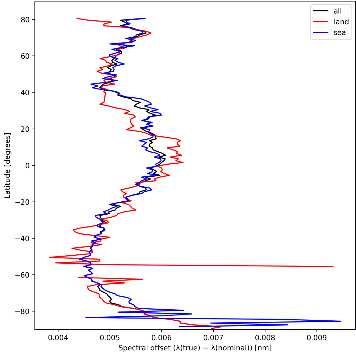
Figure 28: Zonal average of “Spectral offset ( \lambda_{\text{true}} - \lambda_{\text{nominal}} )” for 2025-10-12 to 2025-10-14.
