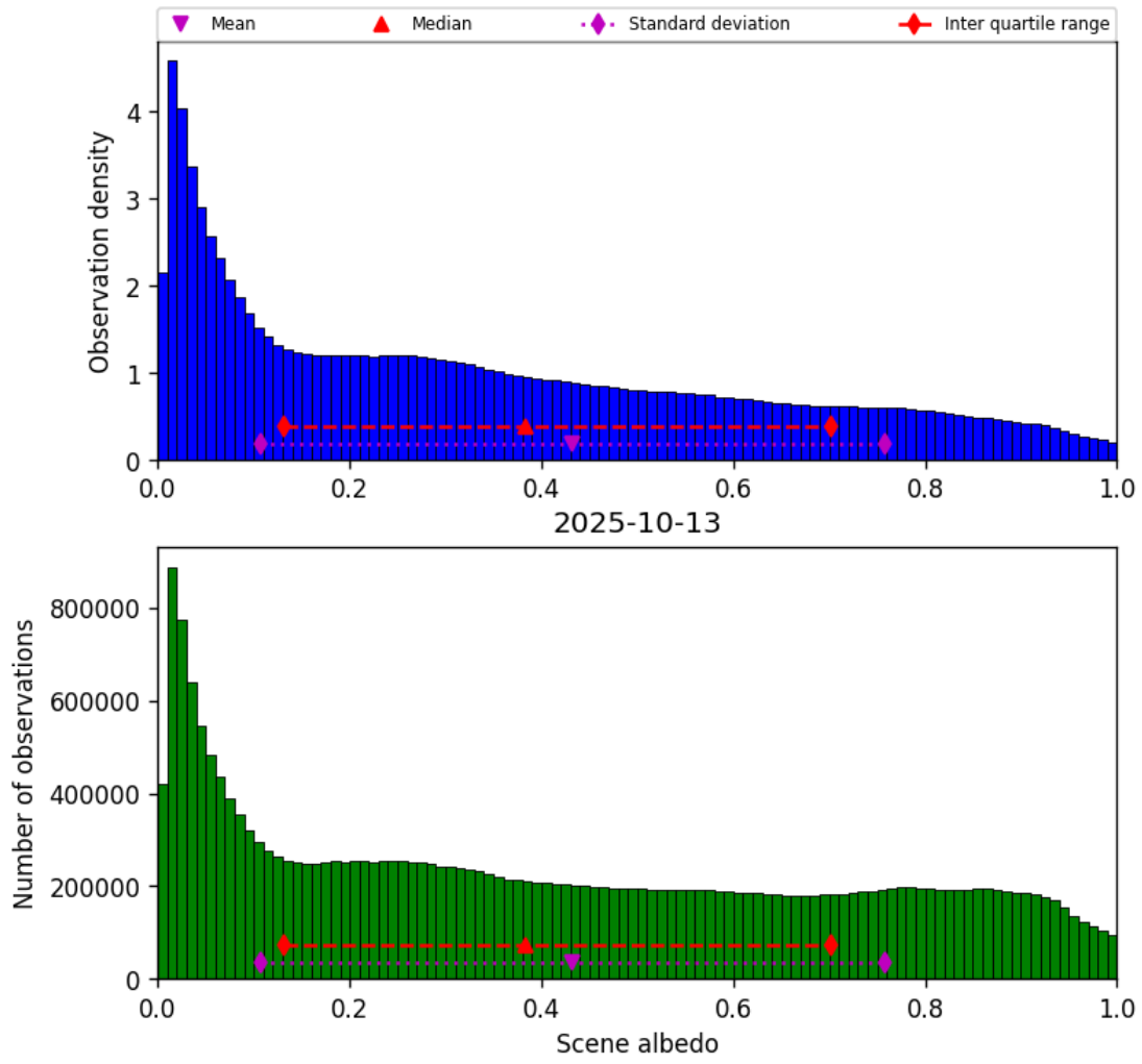
Figure 34: Histogram of “Scene albedo” for 2025-10-12 to 2025-10-14
