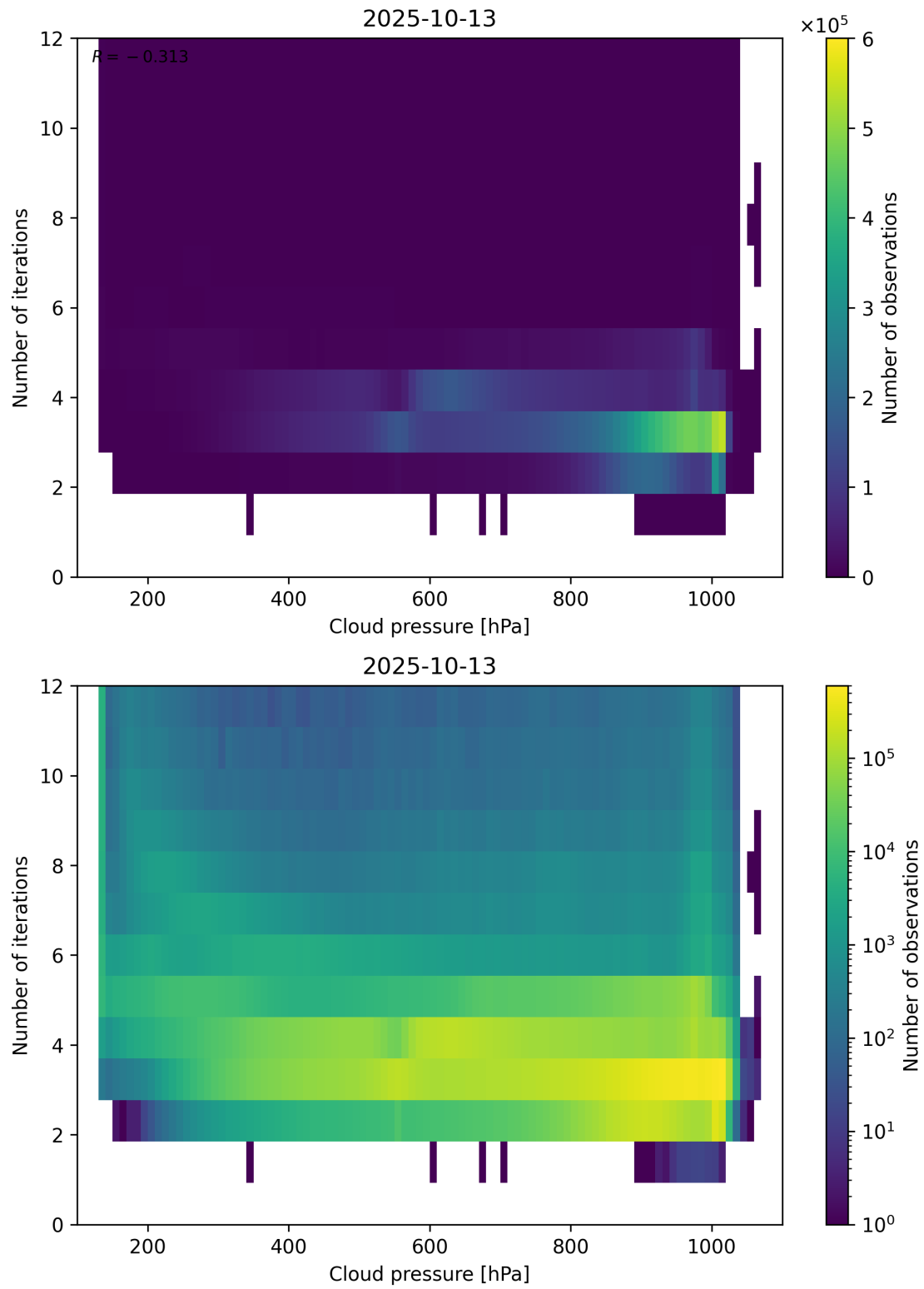
Figure 81: Scatter density plot of “Cloud pressure” against “Number of iterations” for 2025-10-12 to 2025-10-14.
