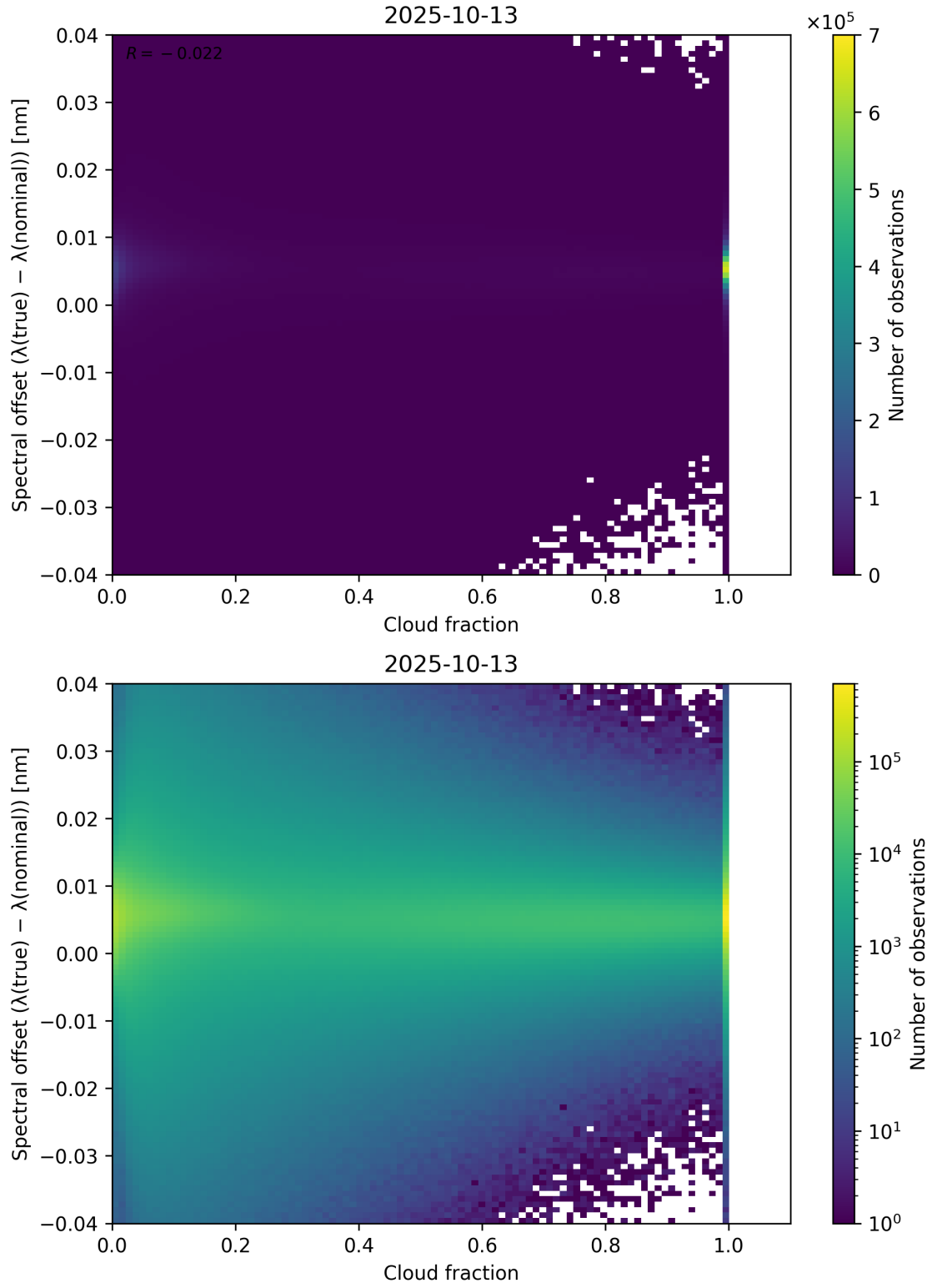
Figure 76: Scatter density plot of “Cloud fraction” against “Spectral offset ( \lambda_{\text{true}} - \lambda_{\text{nominal}} )” for 2025-10-12 to 2025-10-14.
