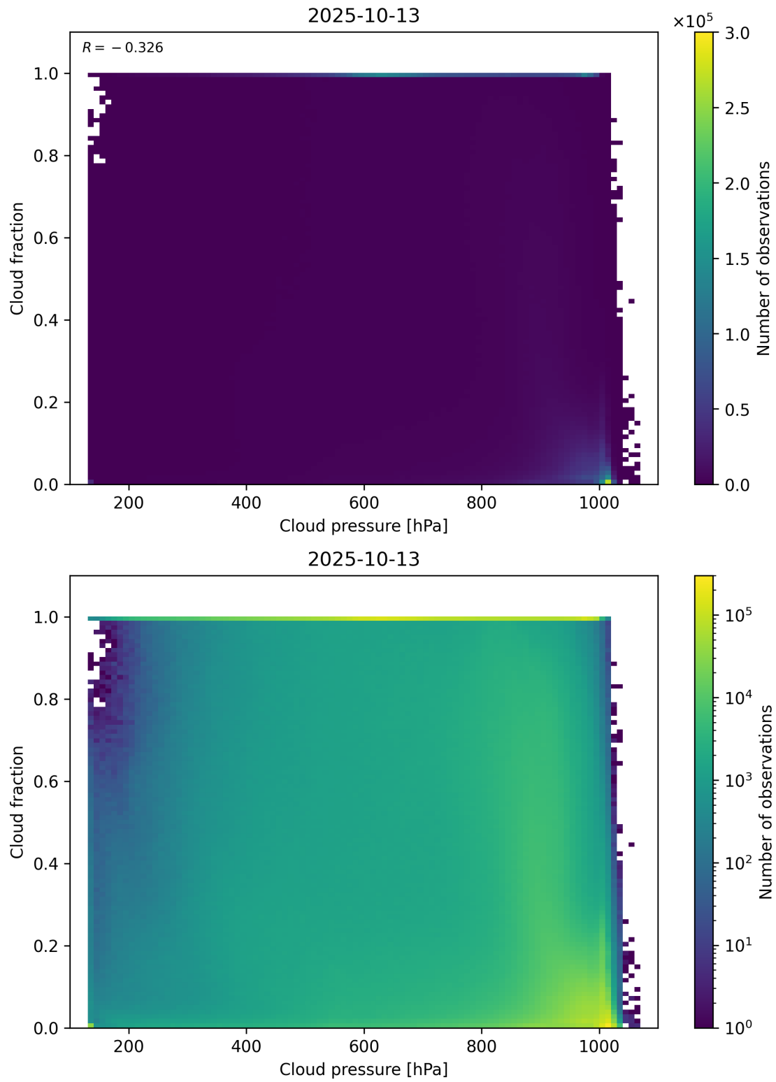
Figure 79: Scatter density plot of “Cloud pressure” against “Cloud fraction” for 2025-10-12 to 2025-10-14.
