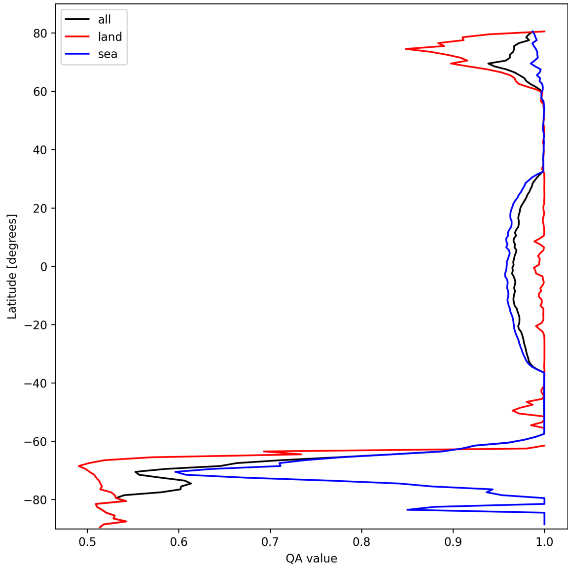
Figure 12: Zonal average of “QA value” for 2025-10-12 to 2025-10-14.
