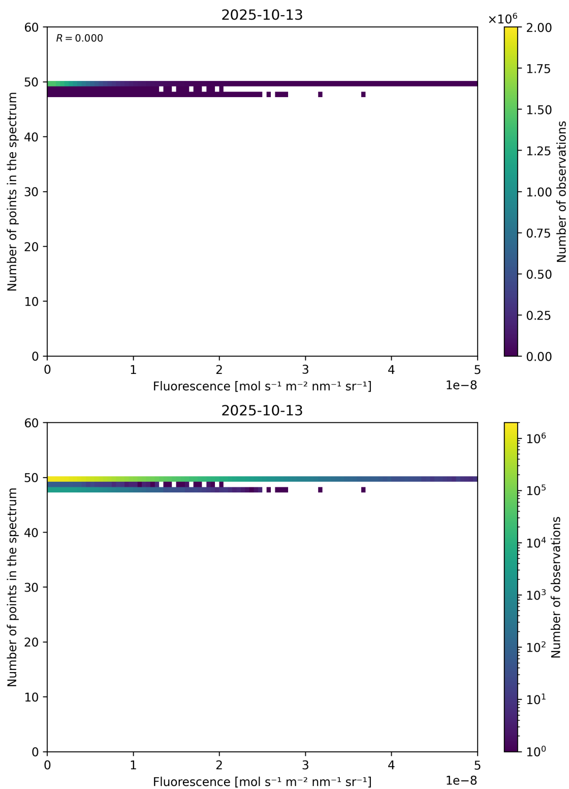
Figure 86: Scatter density plot of “Fluorescence” against “Number of points in the spectrum” for 2025-10-12 to 2025-10-14.
