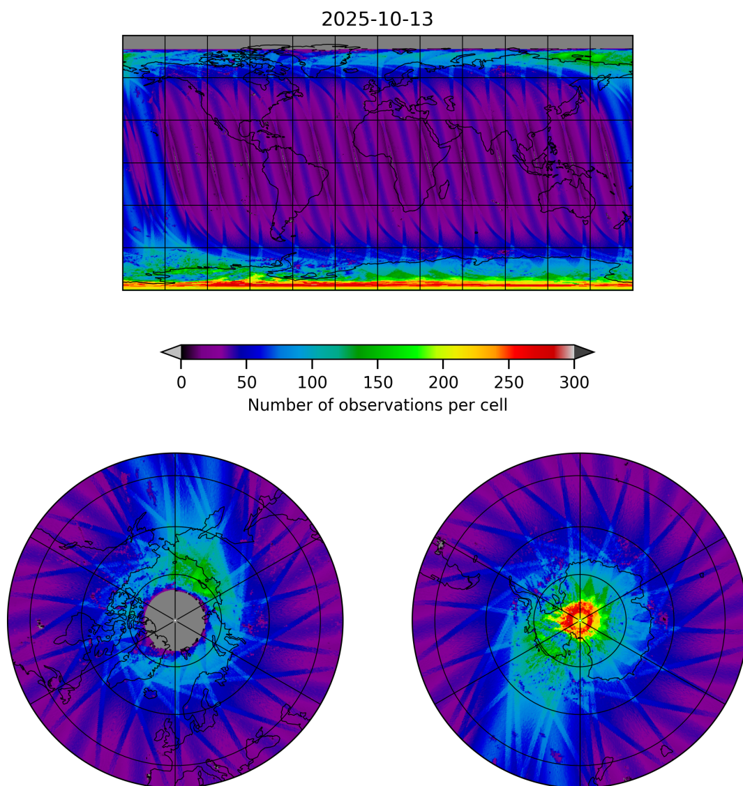
Figure 11: Map of the number of observations for 2025-10-12 to 2025-10-14
