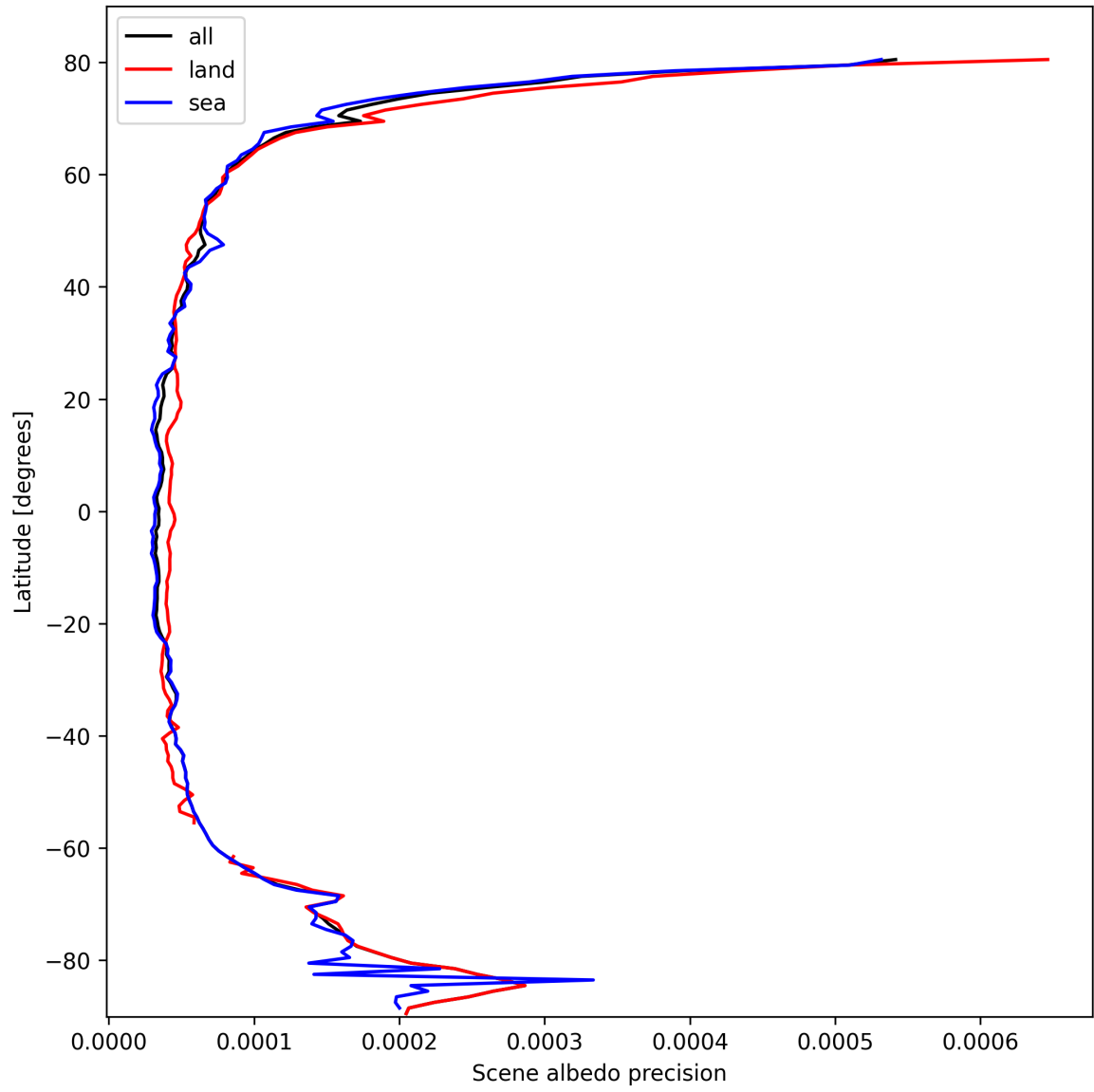
Figure 18: Zonal average of “Scene albedo precision” for 2025-10-12 to 2025-10-14.
