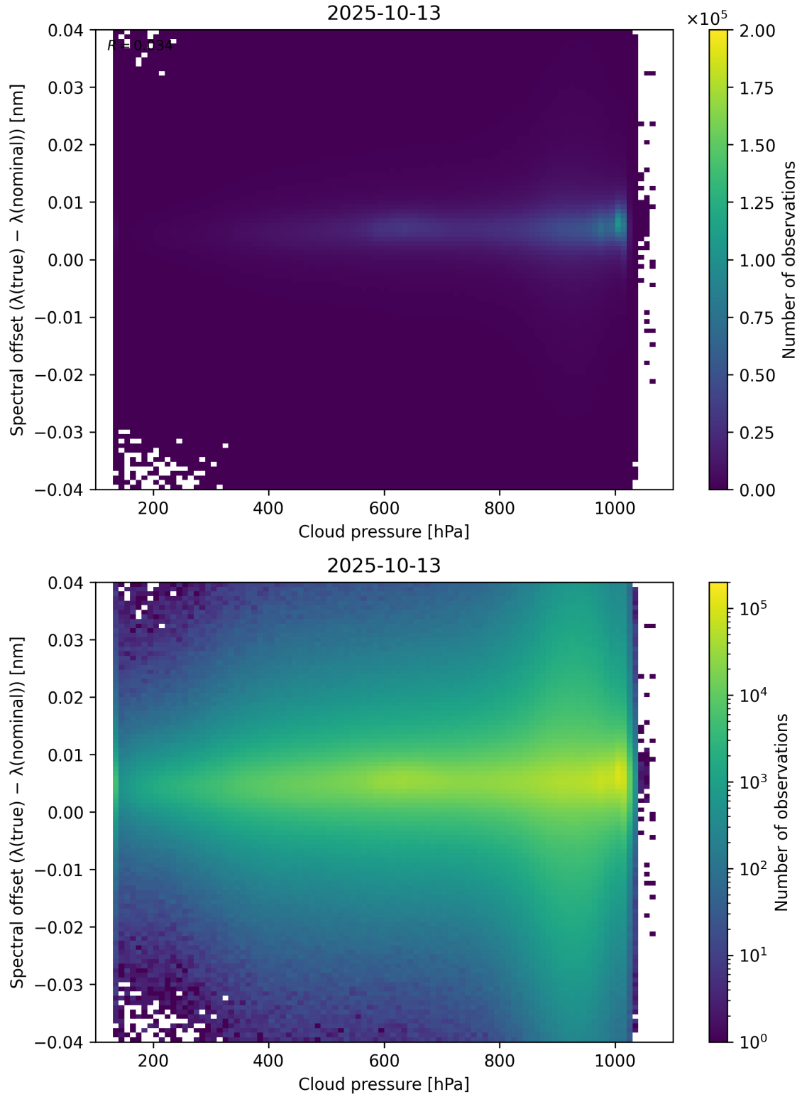
Figure 84: Scatter density plot of “Cloud pressure” against “Spectral offset ( \lambda_{\text{true}} - \lambda_{\text{nominal}} )” for 2025-10-12 to 2025-10-14.
