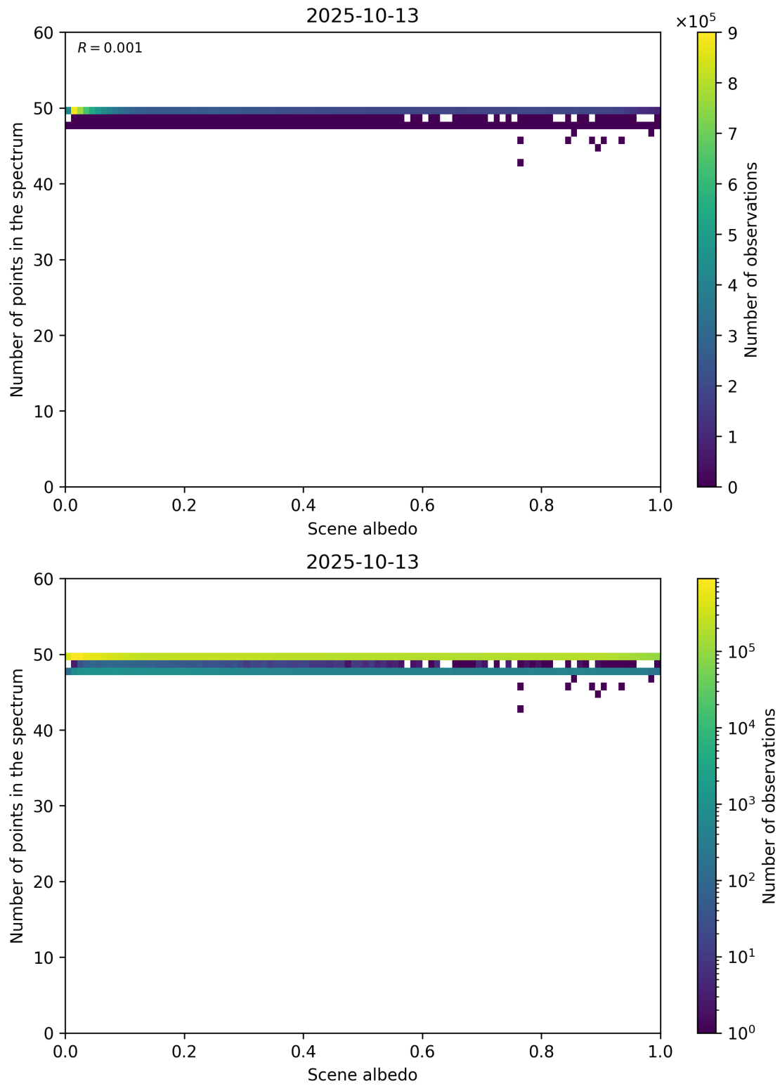
Figure 106: Scatter density plot of “Scene albedo” against “Number of points in the spectrum” for 2025-10-12 to 2025-10-14.
