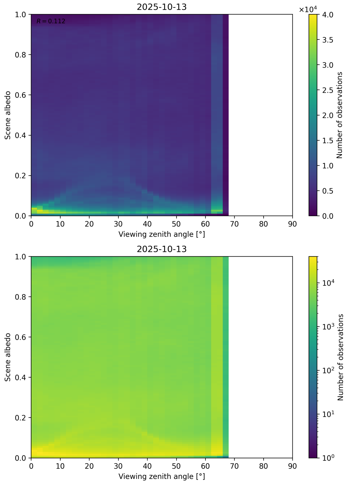
Figure 126: Scatter density plot of “Viewing zenith angle” against “Scene albedo” for 2025-10-12 to 2025-10-14.
