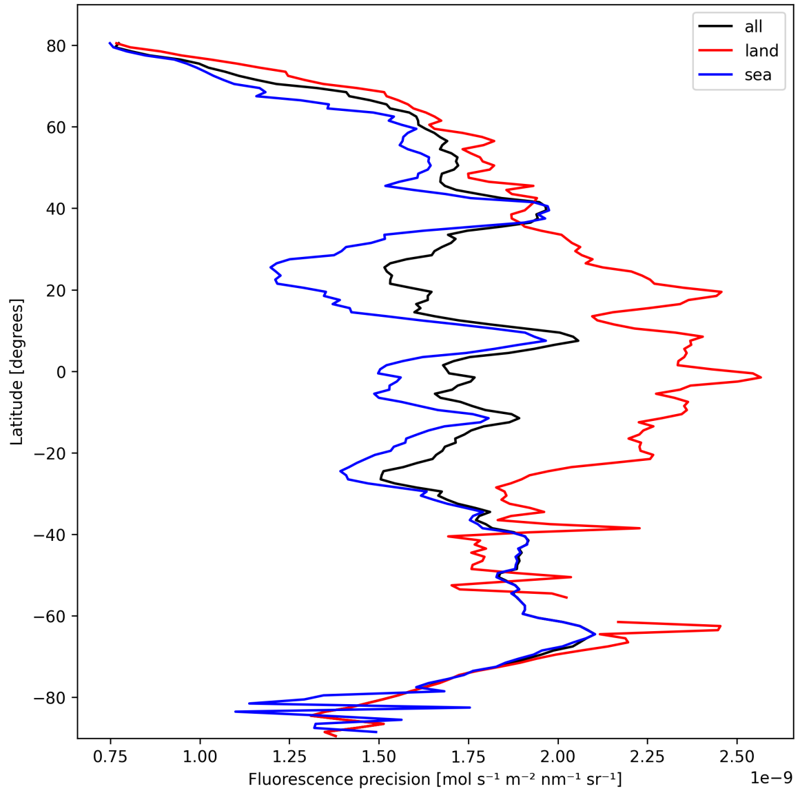
Figure 24: Zonal average of “Fluorescence precision” for 2025-10-12 to 2025-10-14.
