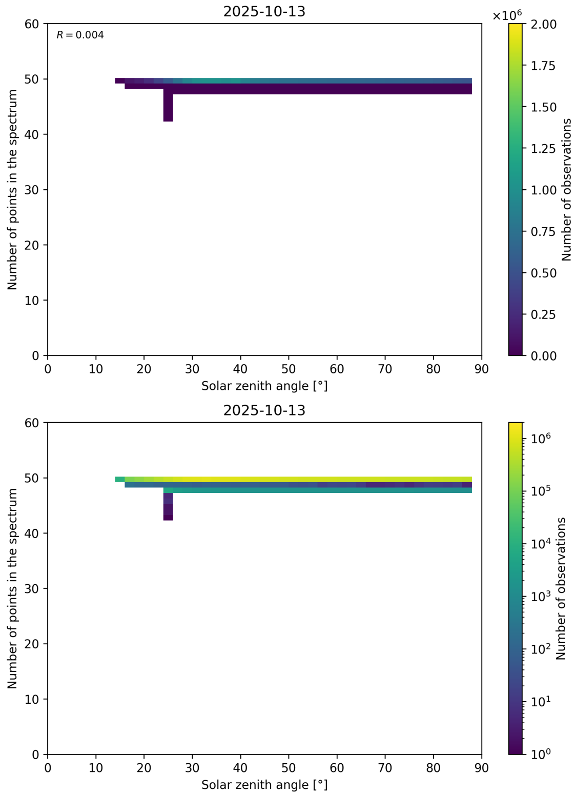
Figure 115: Scatter density plot of “Solar zenith angle” against “Number of points in the spectrum” for 2025-10-12 to 2025-10-14.
