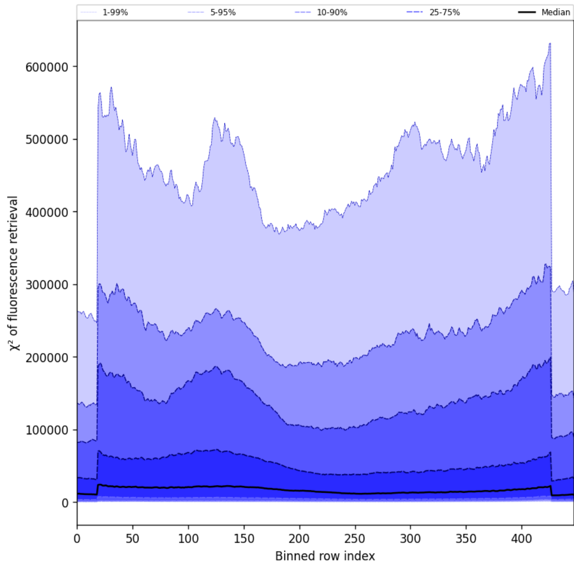
Figure 59: Along track statistics of “ \chi^2 of fluorescence retrieval” for 2025-10-12 to 2025-10-14
