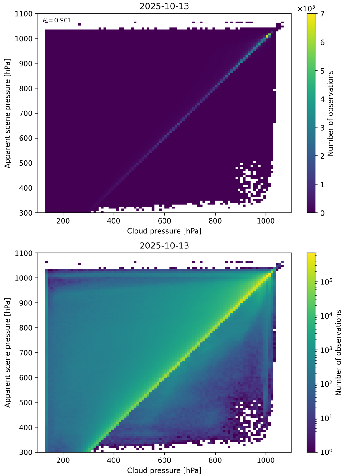
Figure 77: Scatter density plot of “Cloud pressure” against “Apparent scene pressure” for 2025-10-12 to 2025-10-14.
