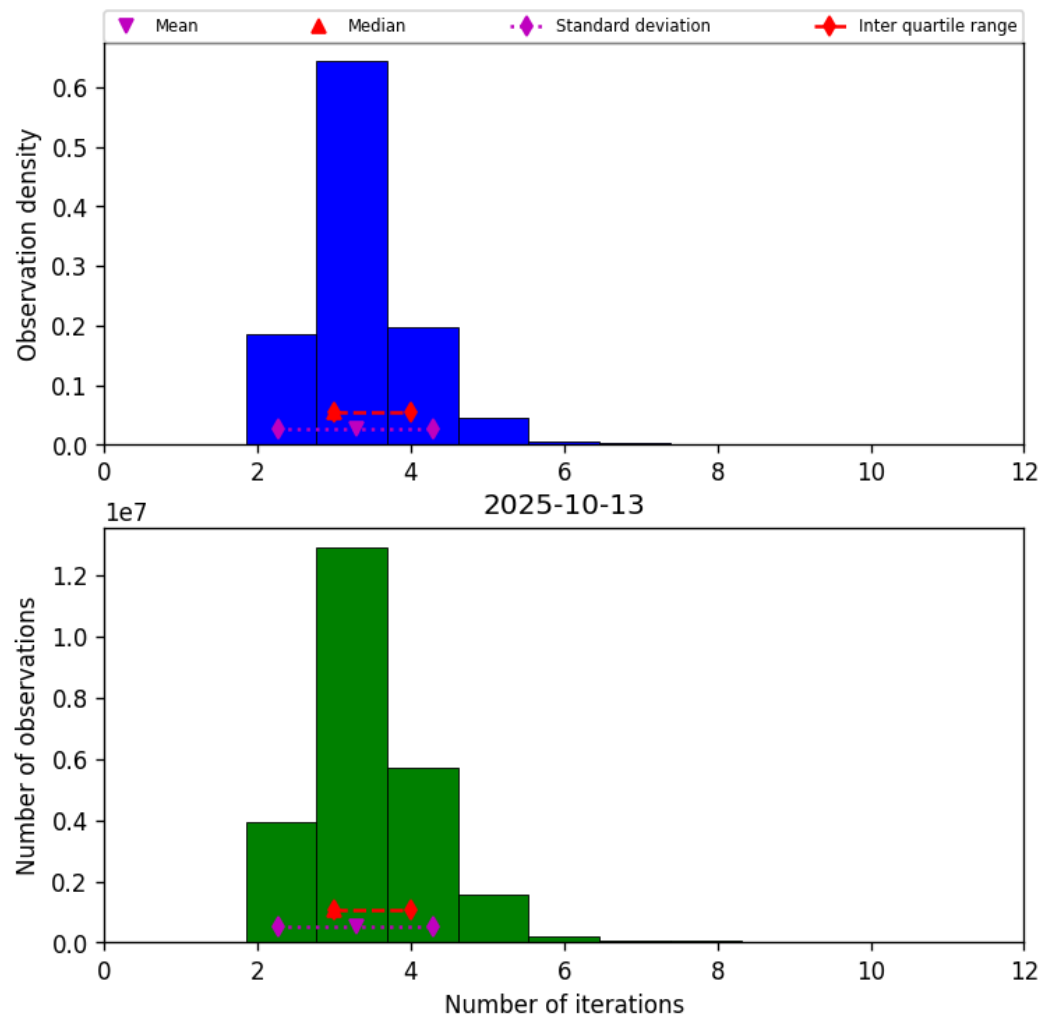
Figure 39: Histogram of “Number of iterations” for 2025-10-12 to 2025-10-14
