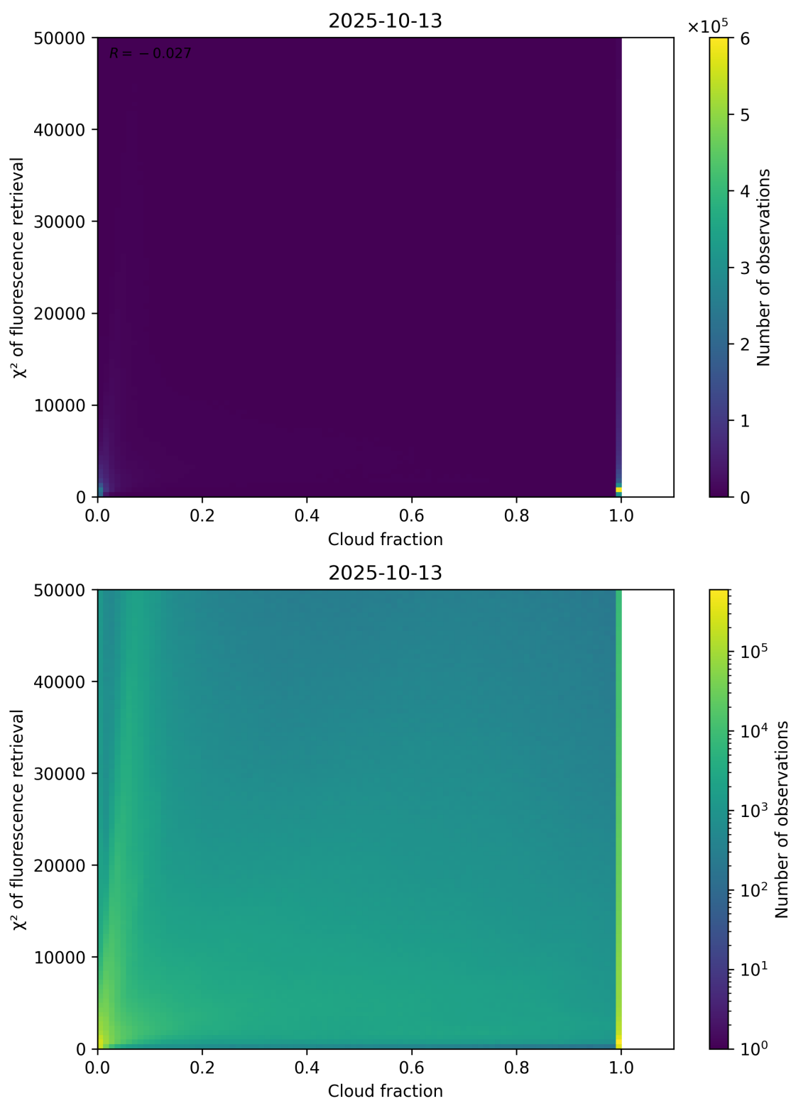
Figure 71: Scatter density plot of “Cloud fraction” against “ \chi^2 of fluorescence retrieval” for 2025-10-12 to 2025-10-14.
