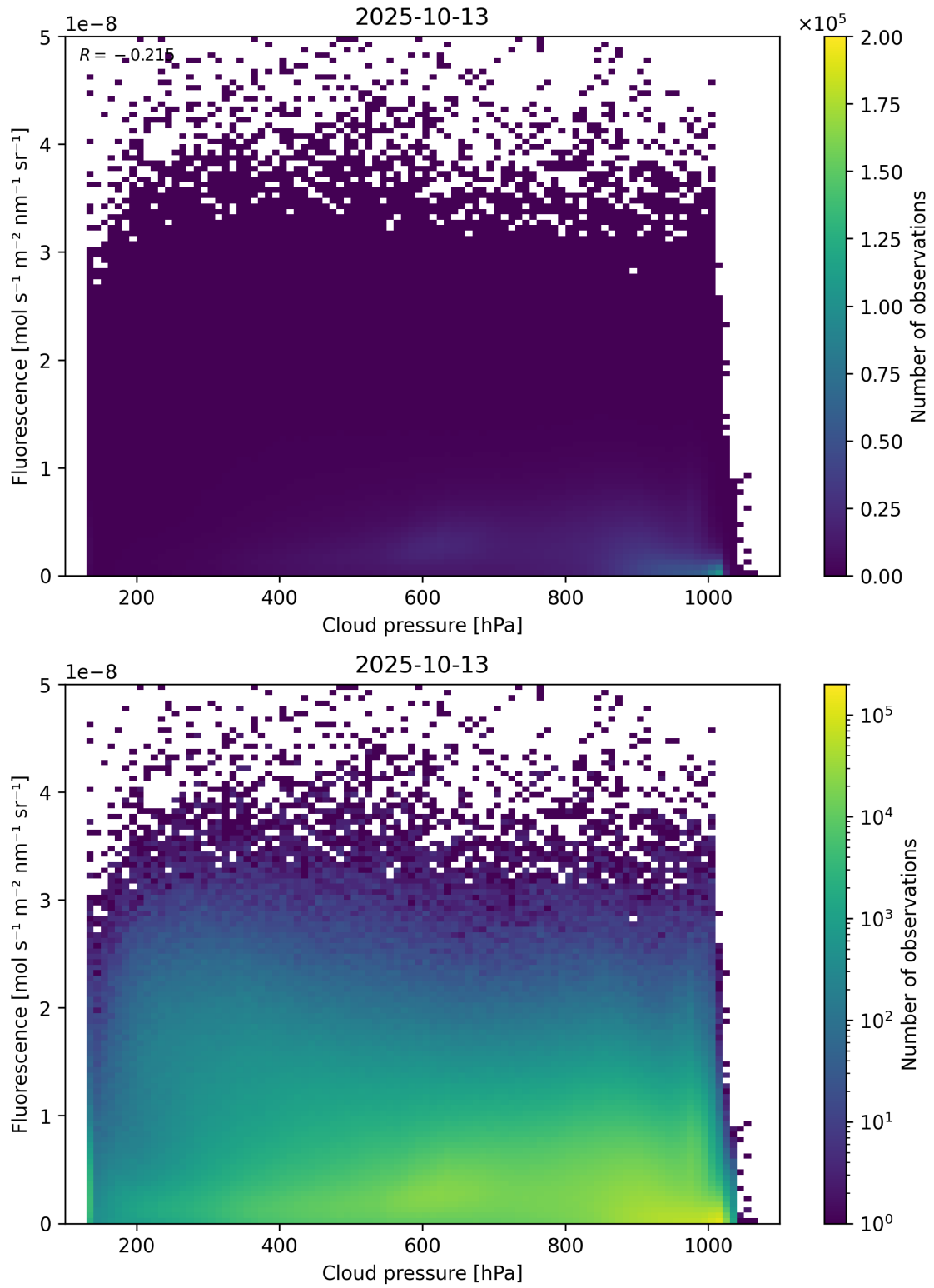
Figure 80: Scatter density plot of “Cloud pressure” against “Fluorescence” for 2025-10-12 to 2025-10-14.
