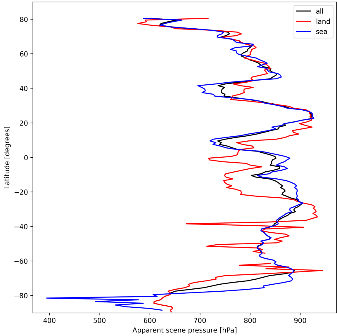
Figure 19: Zonal average of “Apparent scene pressure” for 2025-10-12 to 2025-10-14.
