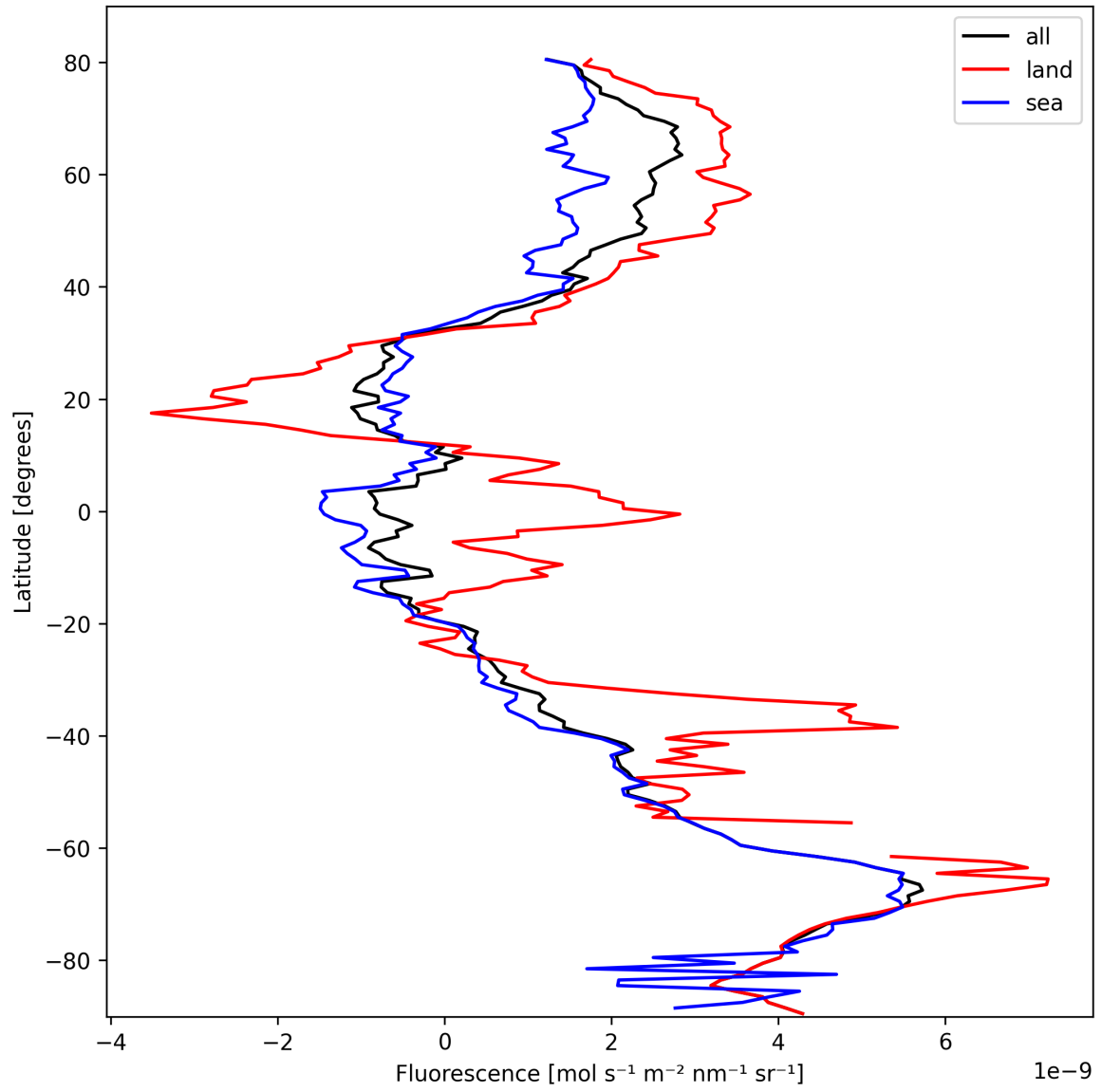
Figure 23: Zonal average of “Fluorescence” for 2025-10-12 to 2025-10-14.
