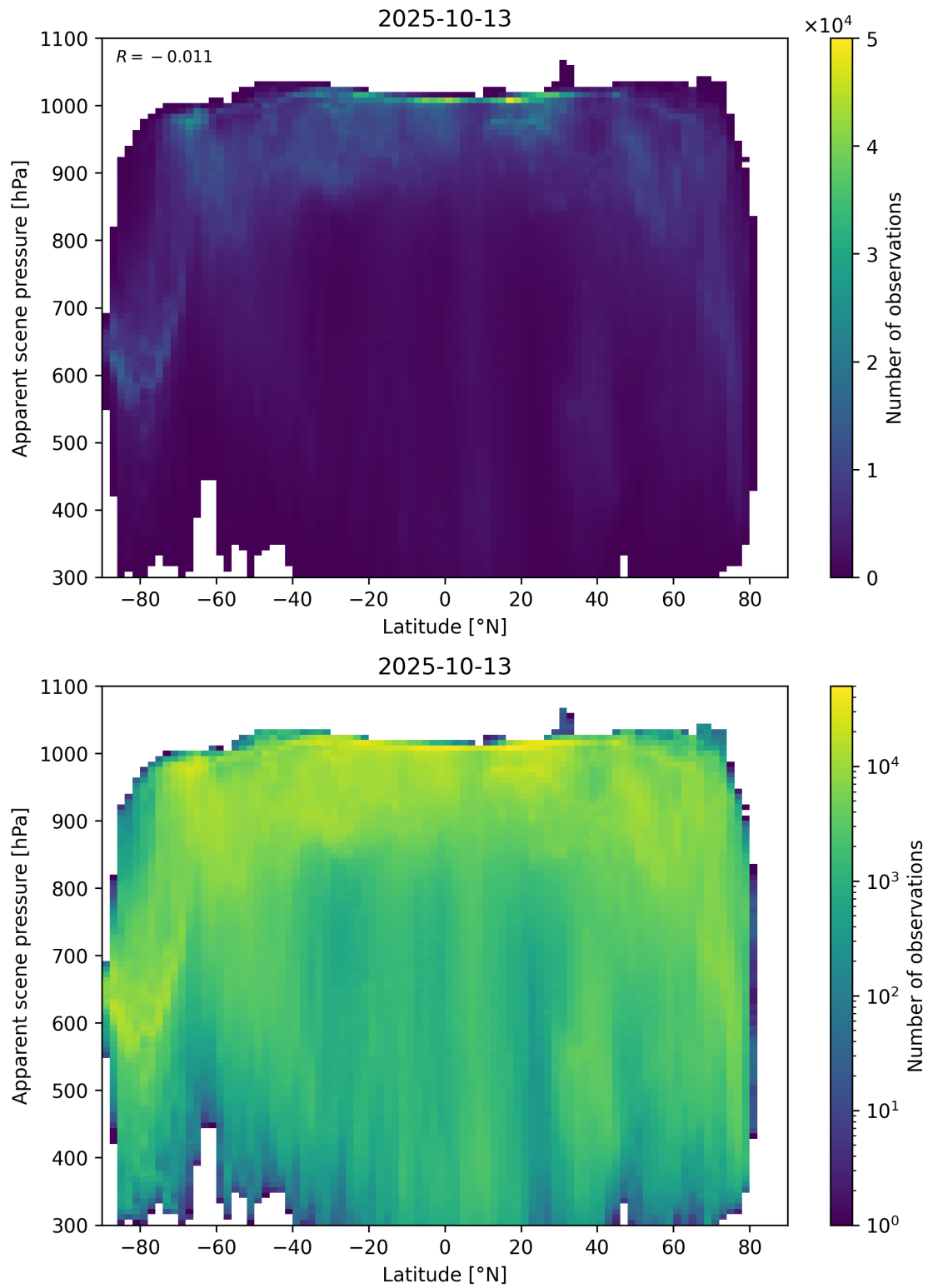
Figure 88: Scatter density plot of “Latitude” against “Apparent scene pressure” for 2025-10-12 to 2025-10-14.
