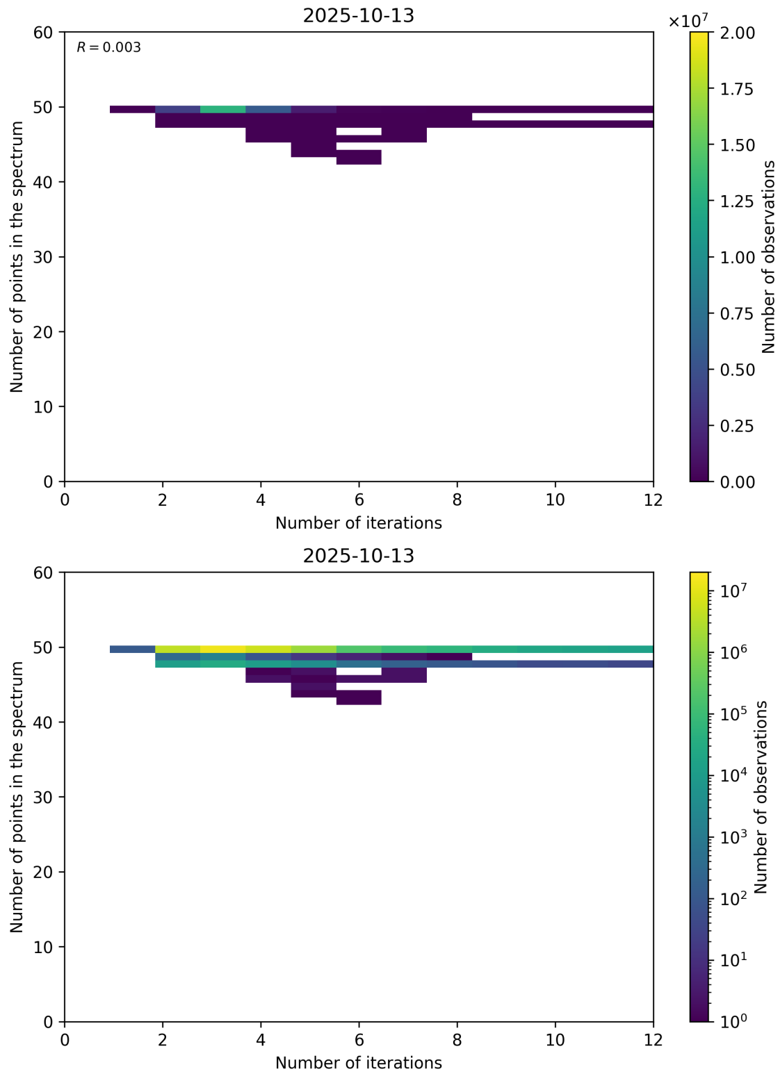
Figure 99: Scatter density plot of “Number of iterations” against “Number of points in the spectrum” for 2025-10-12 to 2025-10-14.
