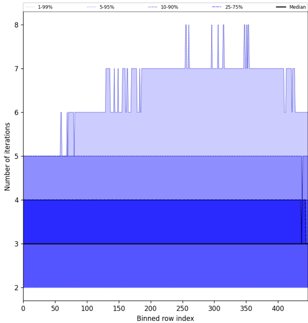
Figure 56: Along track statistics of “Number of iterations” for 2025-10-12 to 2025-10-14
