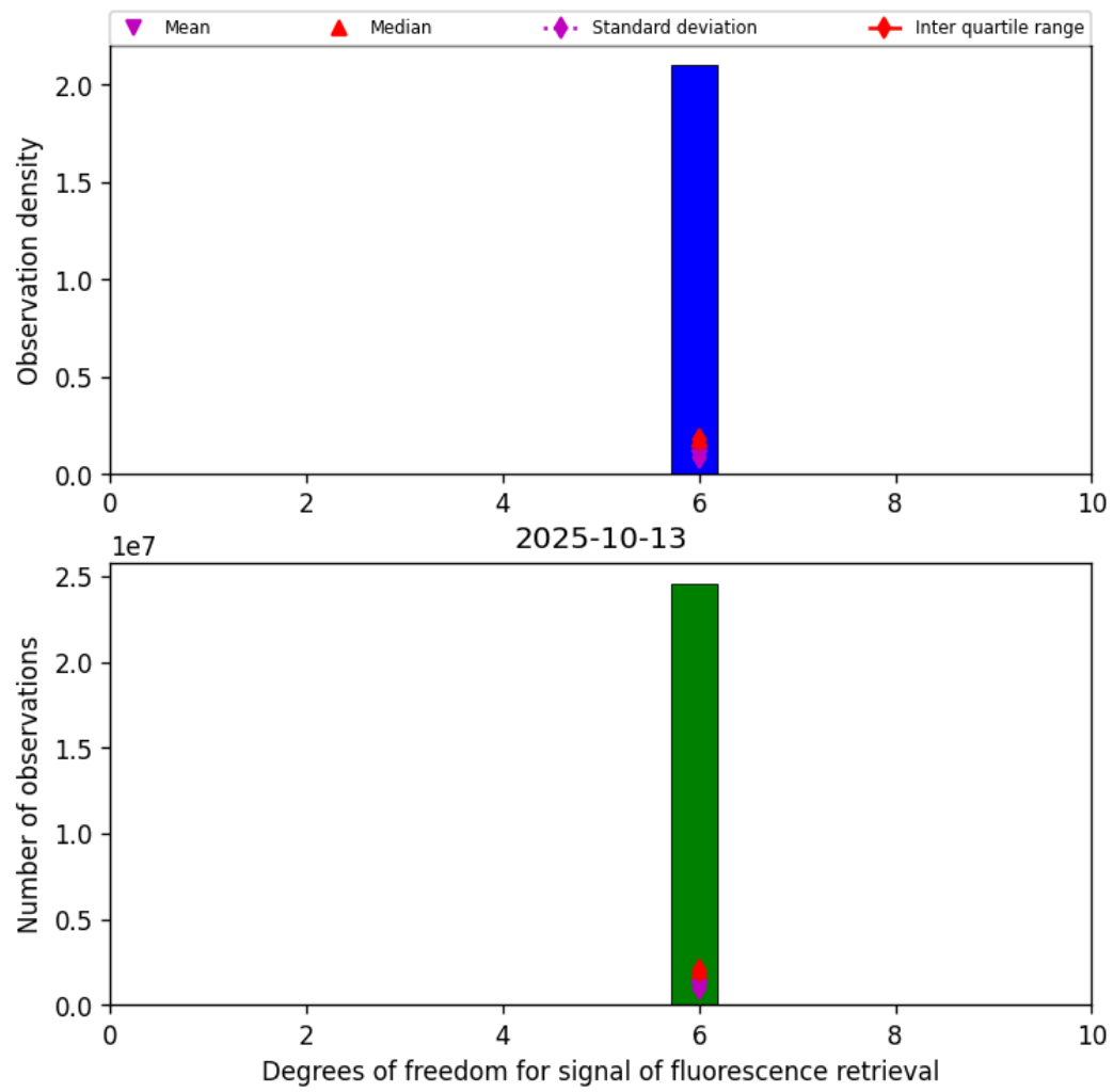
Figure 43: Histogram of "Degrees of freedom for signal of fluorescence retrieval" for 2025-10-12 to 2025-10-14
