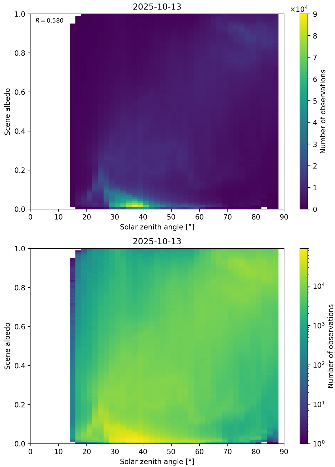
Figure 116: Scatter density plot of “Solar zenith angle” against “Scene albedo” for 2025-10-12 to 2025-10-14.
