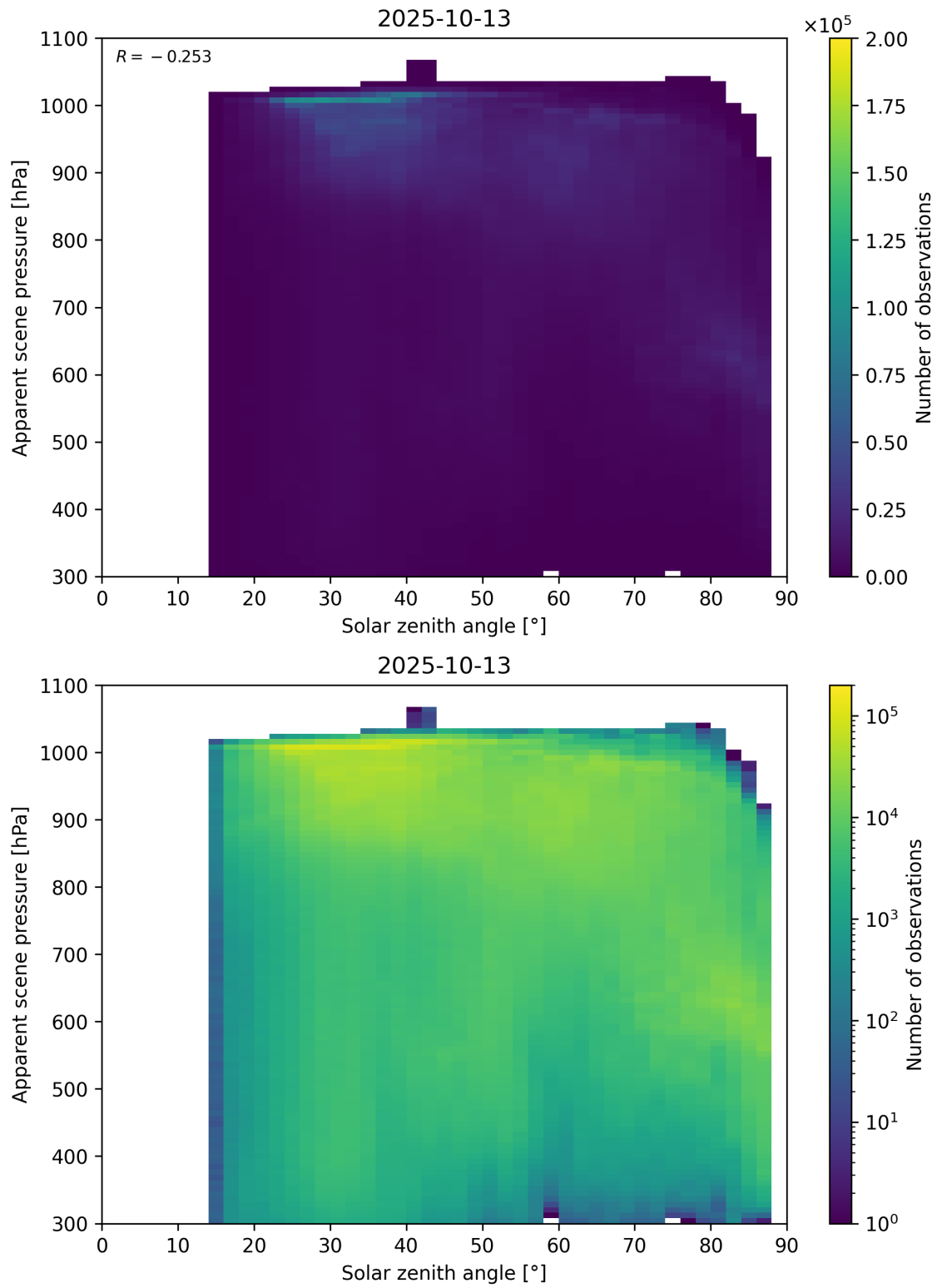
Figure 108: Scatter density plot of “Solar zenith angle” against “Apparent scene pressure” for 2025-10-12 to 2025-10-14.
