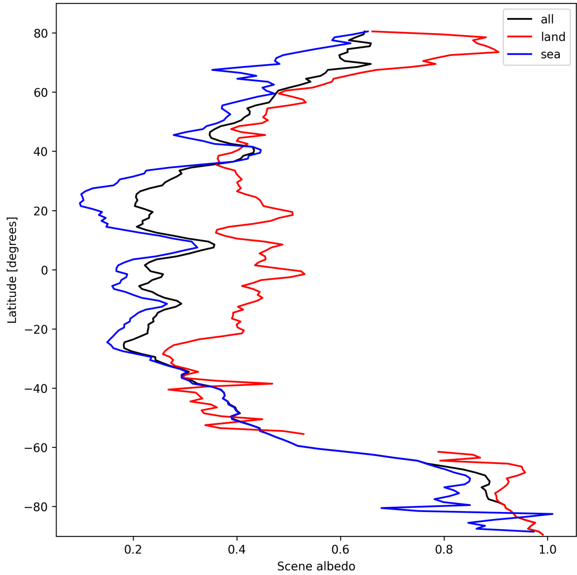
Figure 17: Zonal average of “Scene albedo” for 2025-10-12 to 2025-10-14.
