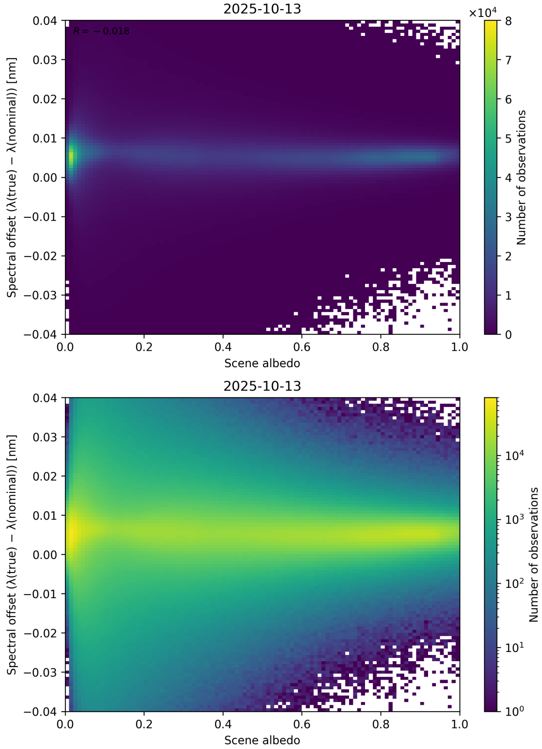
Figure 107: Scatter density plot of “Scene albedo” against “Spectral offset ( \lambda_{\text{true}} - \lambda_{\text{nominal}} )” for 2025-10-12 to 2025-10-14.
