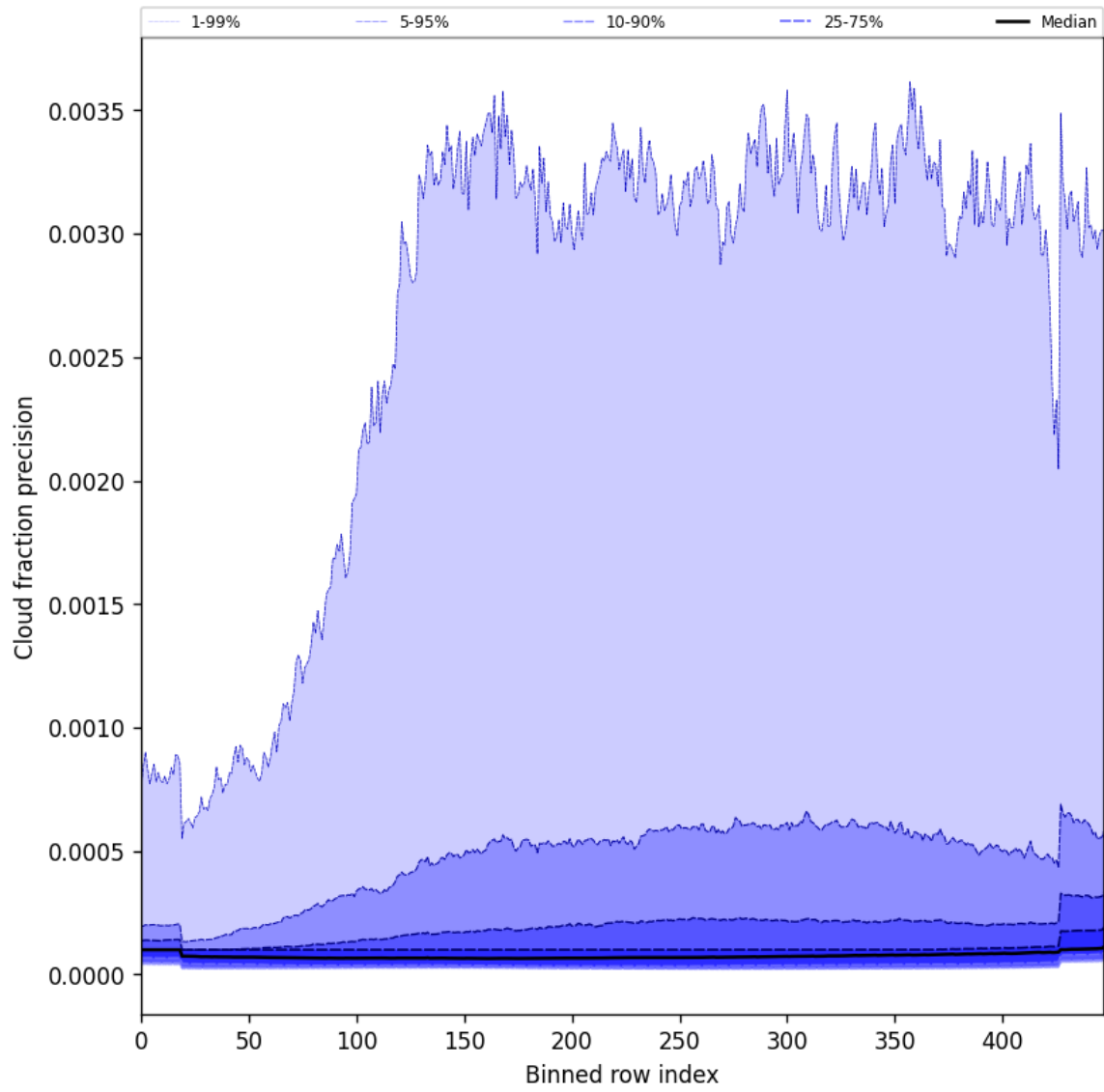
Figure 50: Along track statistics of “Cloud fraction precision” for 2025-10-12 to 2025-10-14
