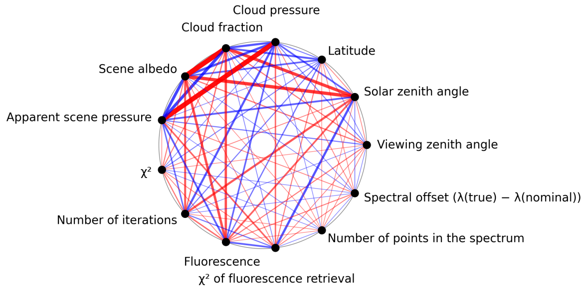
Figure 1: Map of correlation graph for 2025-10-12 to 2025-10-14.
