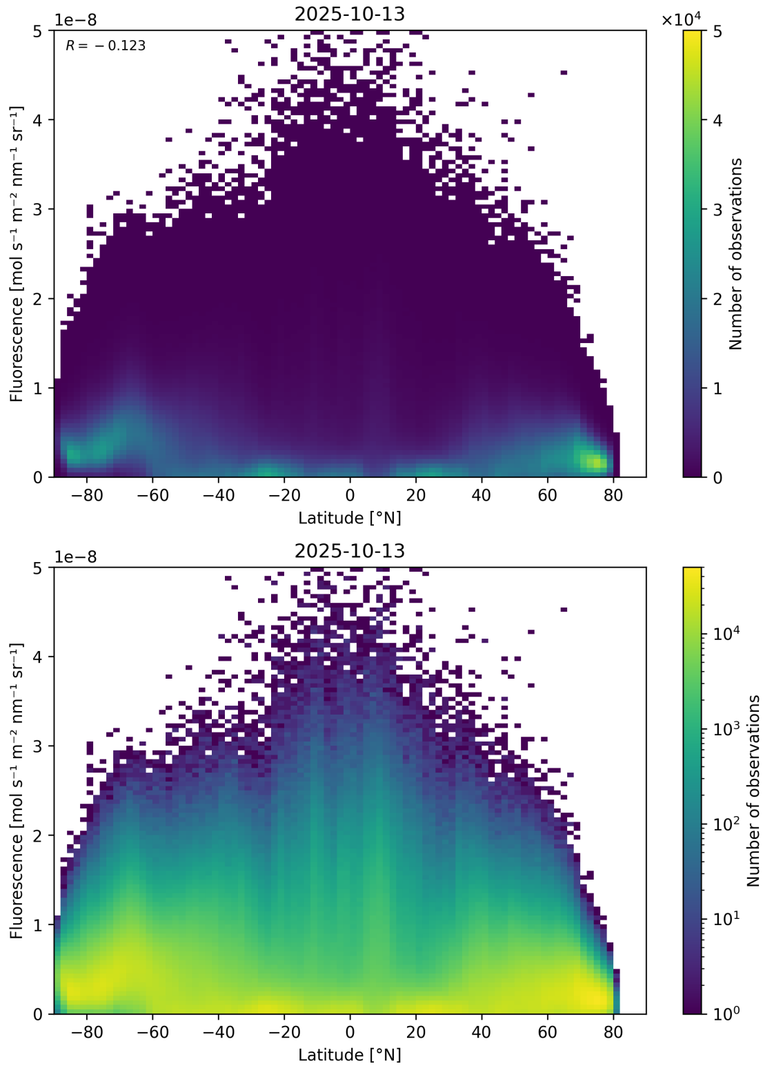
Figure 92: Scatter density plot of “Latitude” against “Fluorescence” for 2025-10-12 to 2025-10-14.
