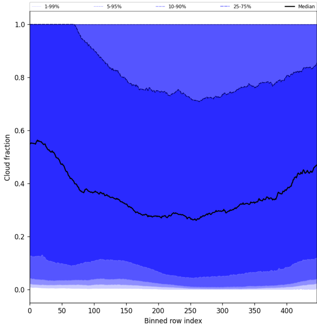
Figure 49: Along track statistics of “Cloud fraction” for 2025-10-12 to 2025-10-14
