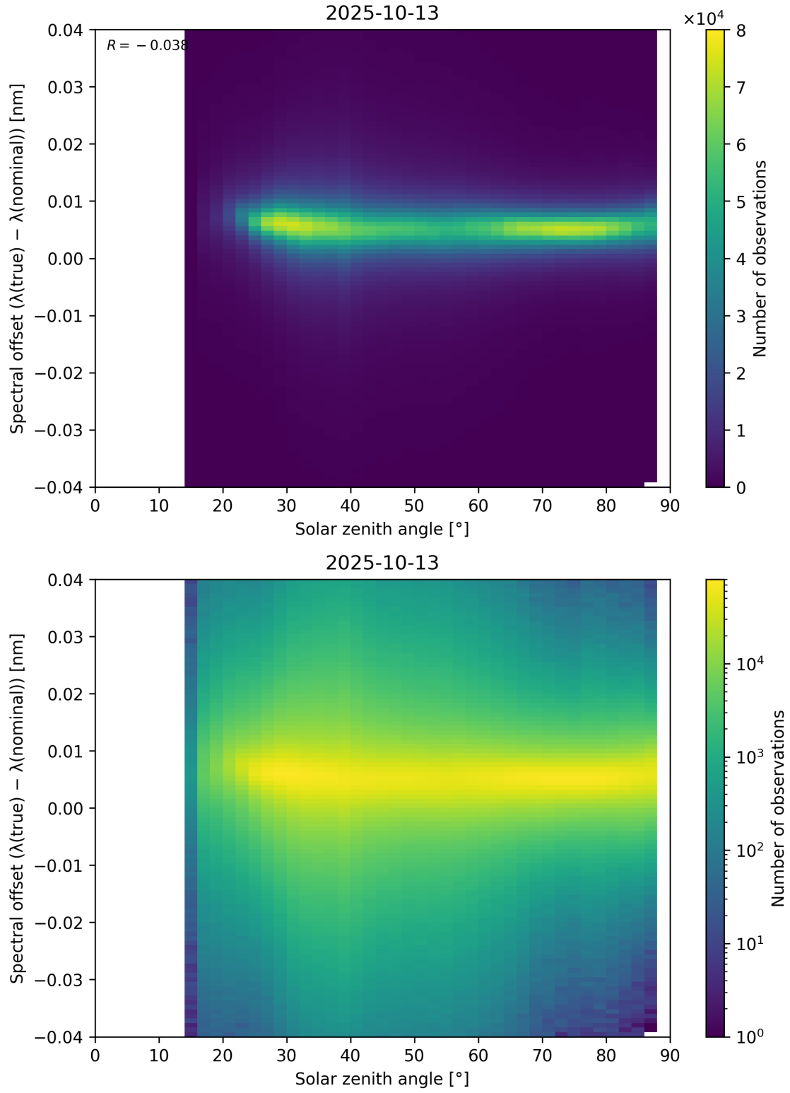
Figure 117: Scatter density plot of “Solar zenith angle” against “Spectral offset ( \lambda_{\text{true}} - \lambda_{\text{nominal}} )” for 2025-10-12 to 2025-10-14.
