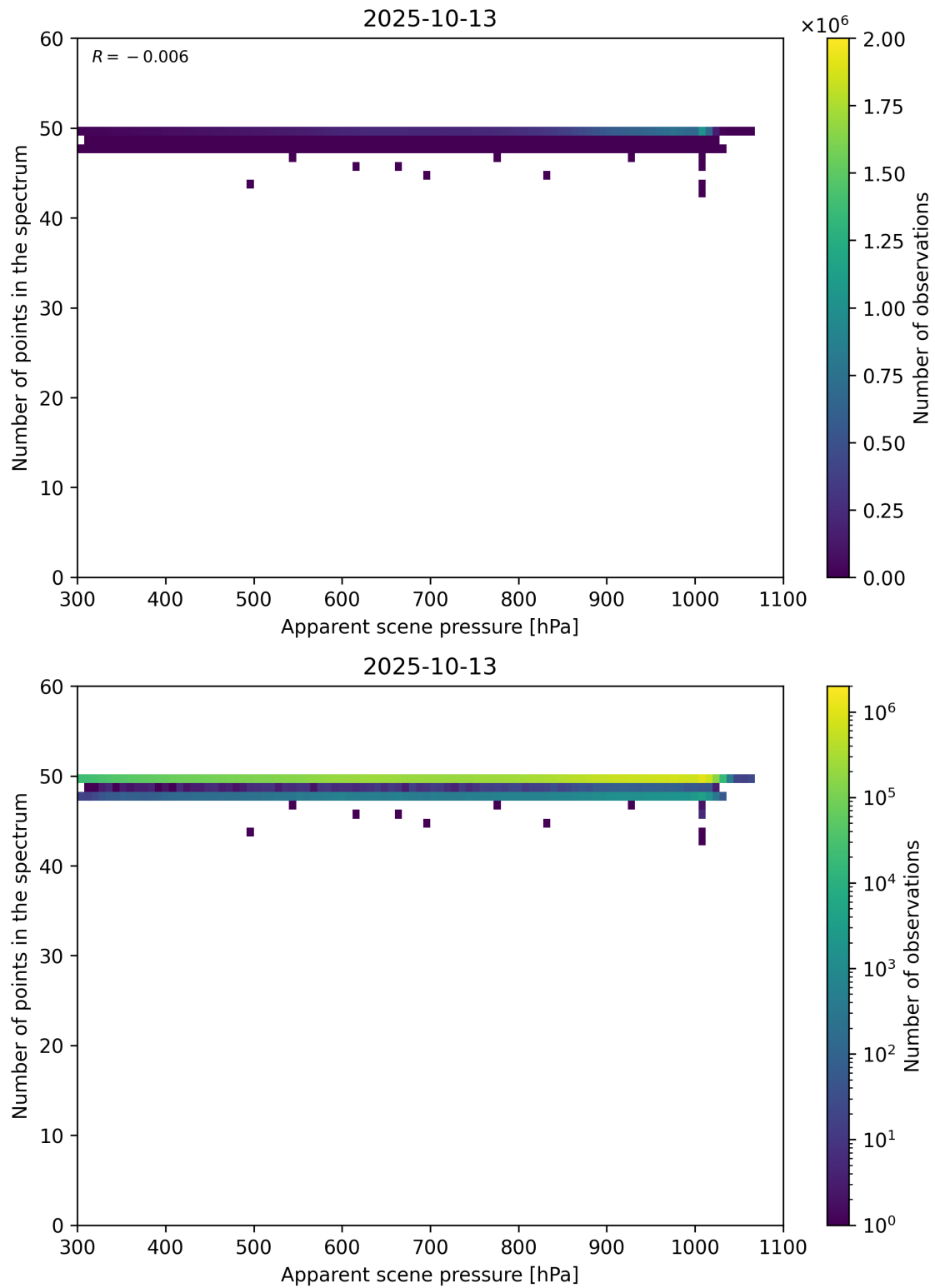
Figure 66: Scatter density plot of “Apparent scene pressure” against “Number of points in the spectrum” for 2025-10-12 to 2025-10-14.
