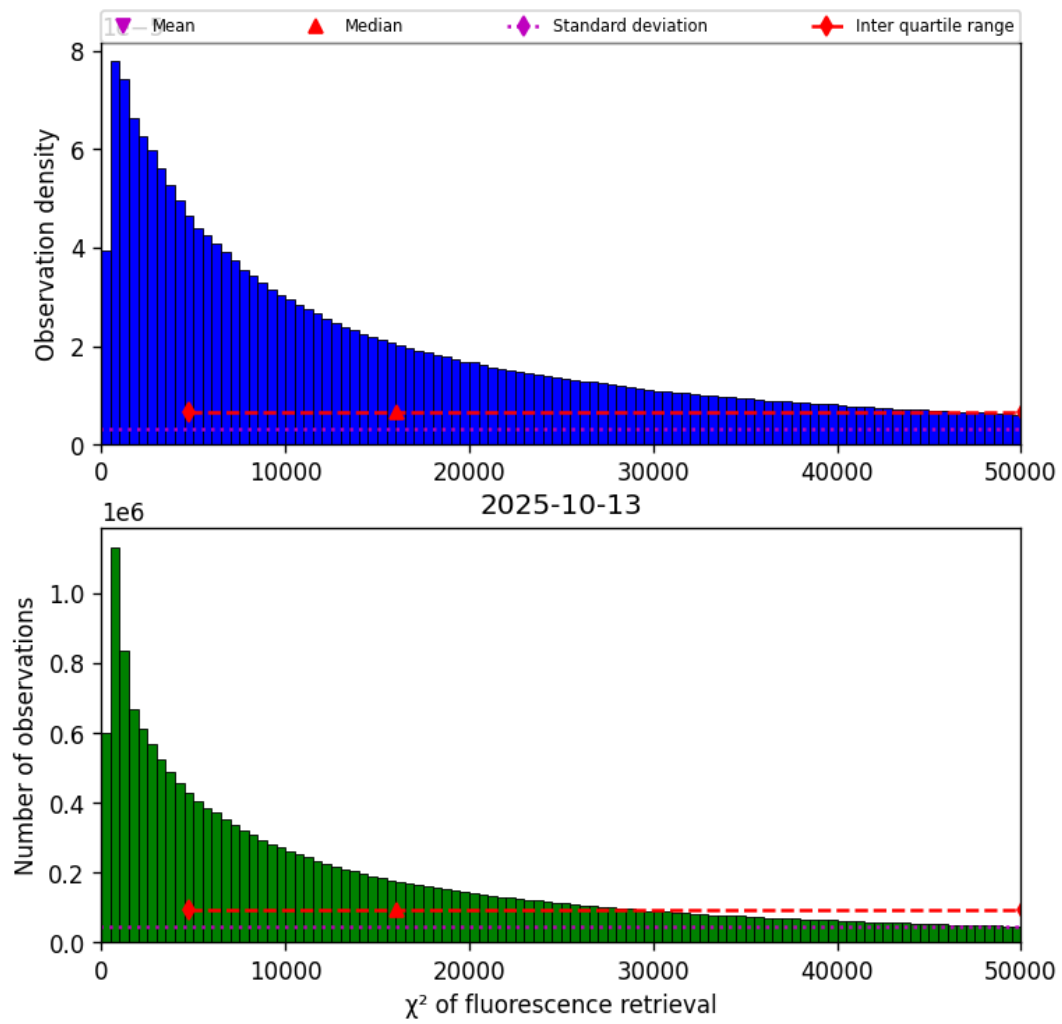
Figure 42: Histogram of “ \chi^2 of fluorescence retrieval” for 2025-10-12 to 2025-10-14
