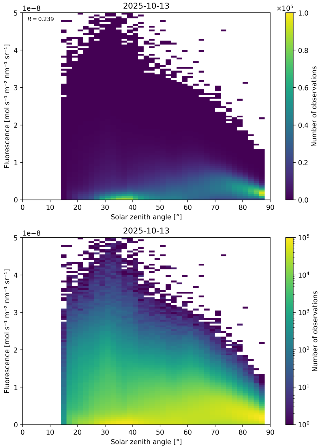
Figure 112: Scatter density plot of “Solar zenith angle” against “Fluorescence” for 2025-10-12 to 2025-10-14.
