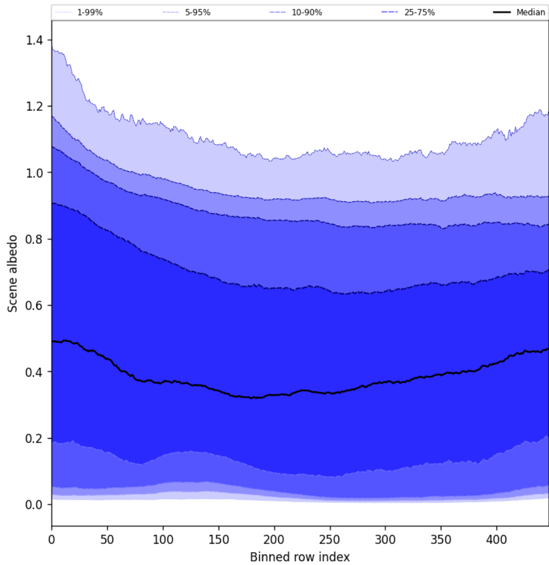
Figure 51: Along track statistics of “Scene albedo” for 2025-10-12 to 2025-10-14
