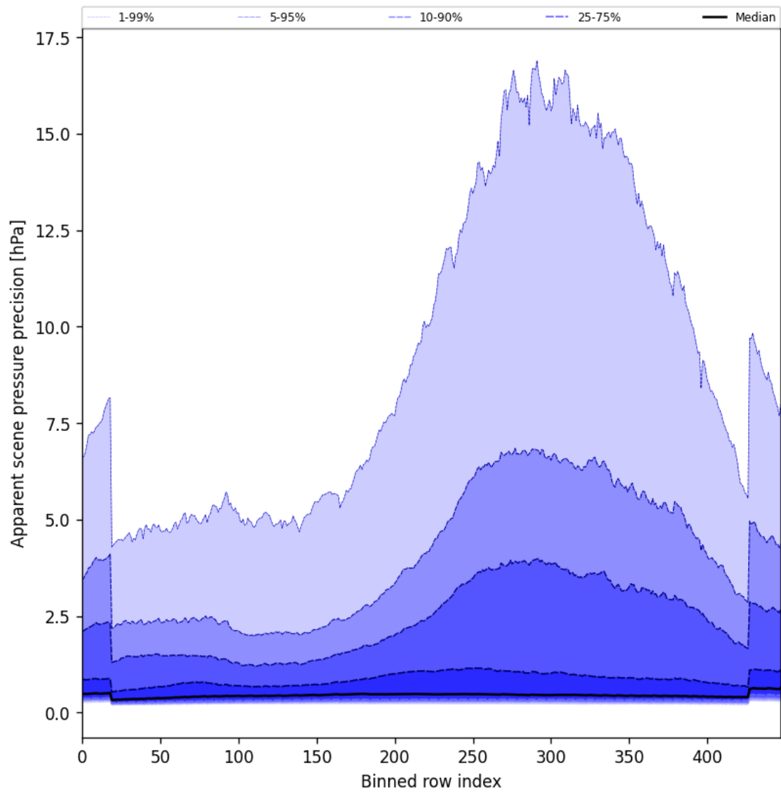
Figure 54: Along track statistics of “Apparent scene pressure precision” for 2025-10-12 to 2025-10-14
