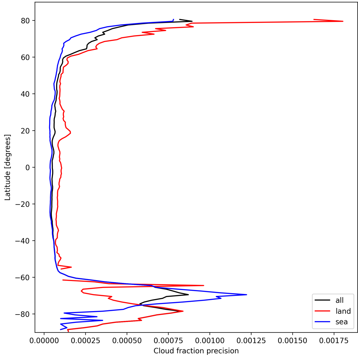
Figure 16: Zonal average of “Cloud fraction precision” for 2025-10-12 to 2025-10-14.
