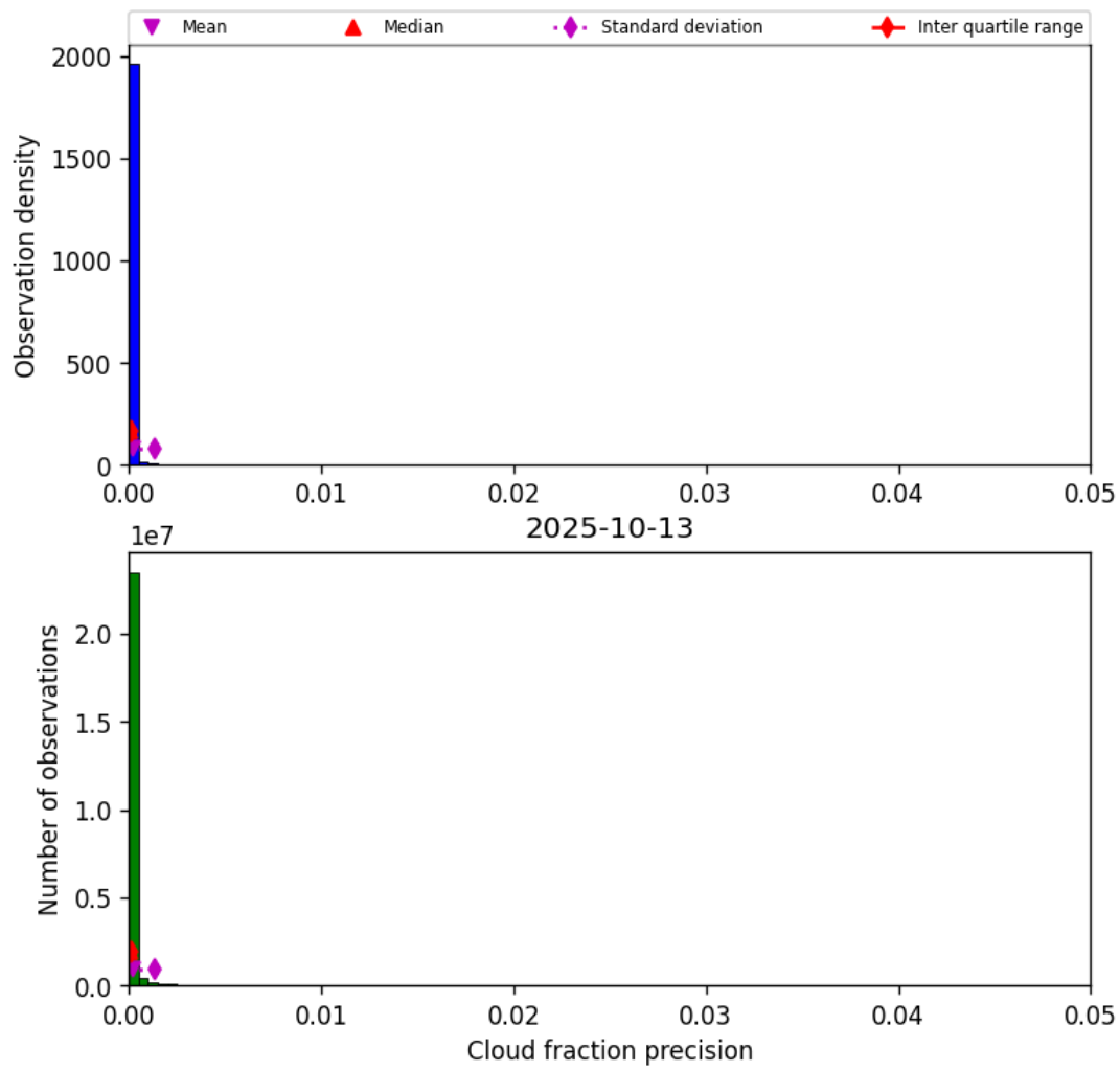
Figure 33: Histogram of “Cloud fraction precision” for 2025-10-12 to 2025-10-14
