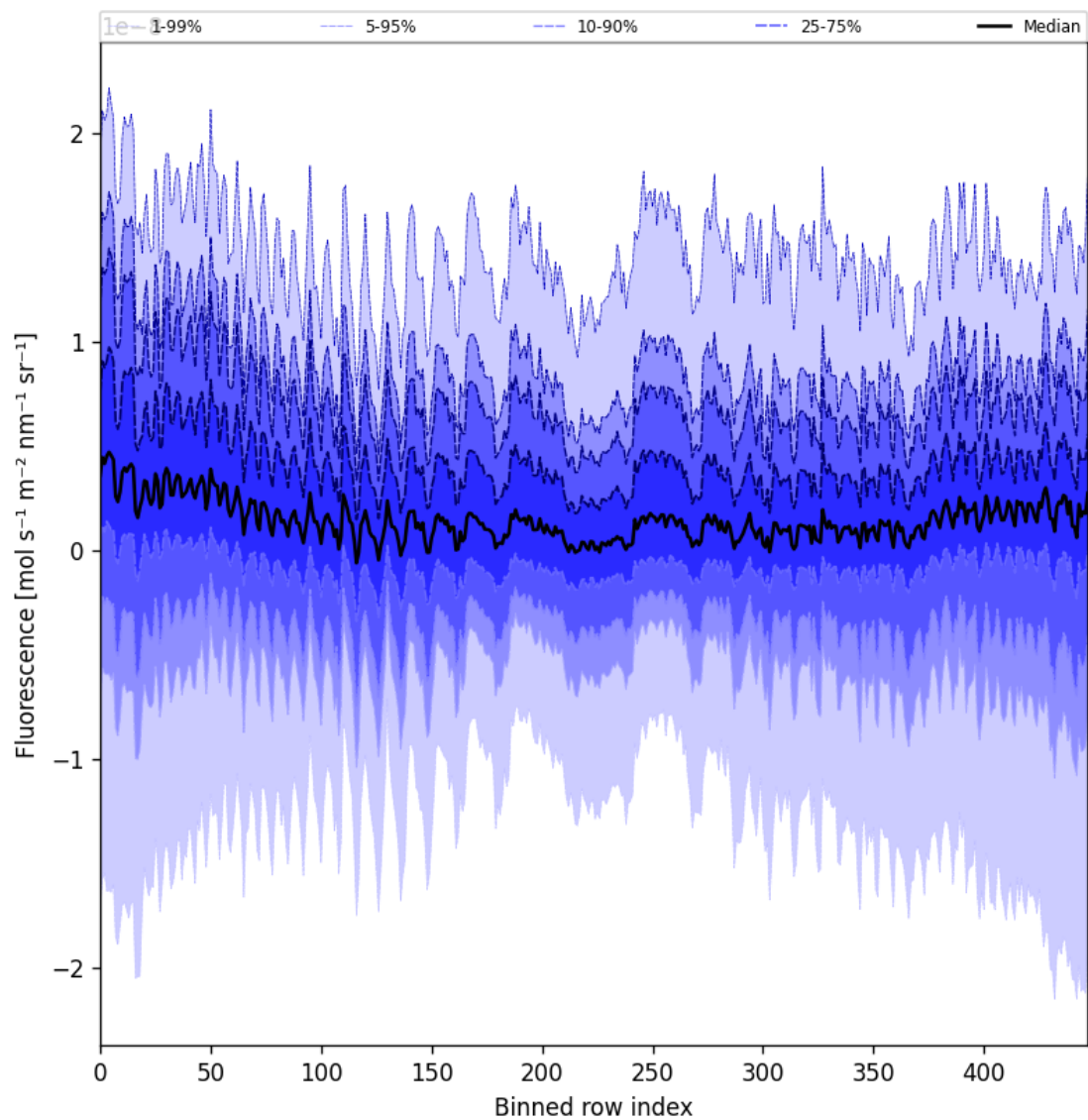
Figure 57: Along track statistics of “Fluorescence” for 2025-10-12 to 2025-10-14
