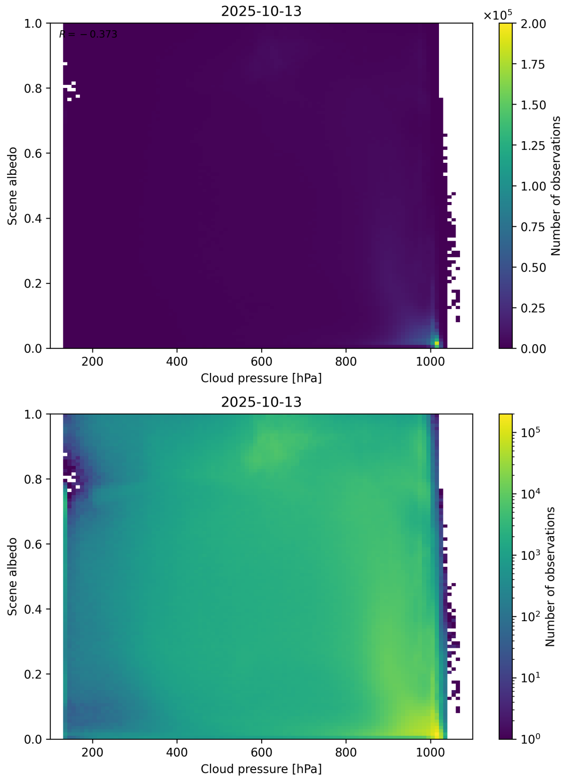
Figure 83: Scatter density plot of “Cloud pressure” against “Scene albedo” for 2025-10-12 to 2025-10-14.
