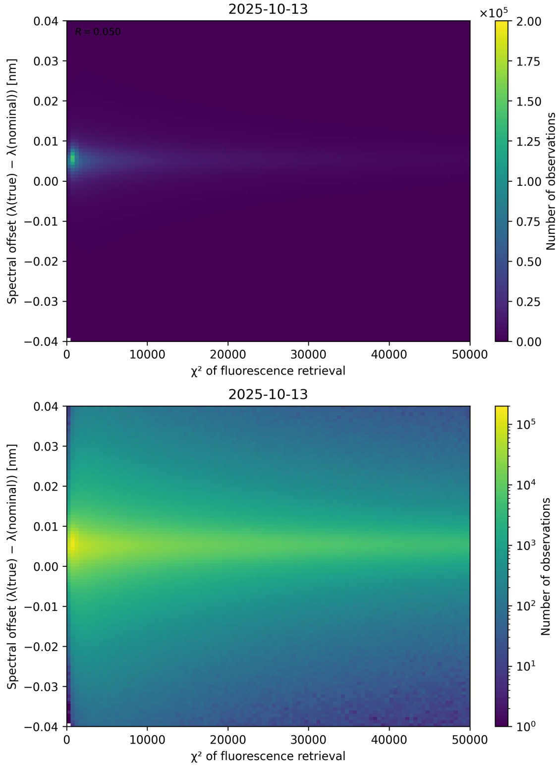
Figure 69: Scatter density plot of “ \chi^2 of fluorescence retrieval” against “Spectral offset ( \lambda_{\text{true}} - \lambda_{\text{nominal}} )” for 2025-10-12 to 2025-10-14.
