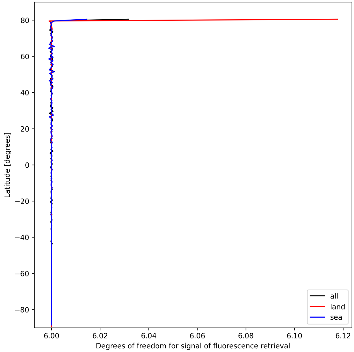
Figure 26: Zonal average of “Degrees of freedom for signal of fluorescence retrieval” for 2025-10-12 to 2025-10-14.
