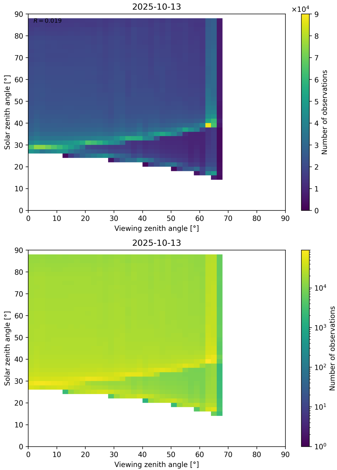
Figure 127: Scatter density plot of “Viewing zenith angle” against “Solar zenith angle” for 2025-10-12 to 2025-10-14.
