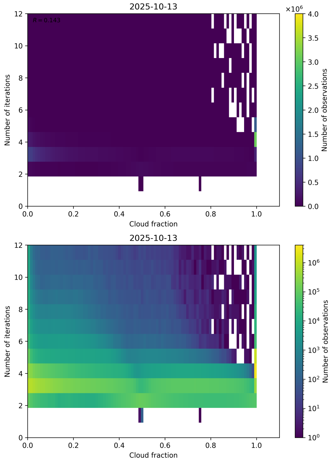
Figure 73: Scatter density plot of “Cloud fraction” against “Number of iterations” for 2025-10-12 to 2025-10-14.
