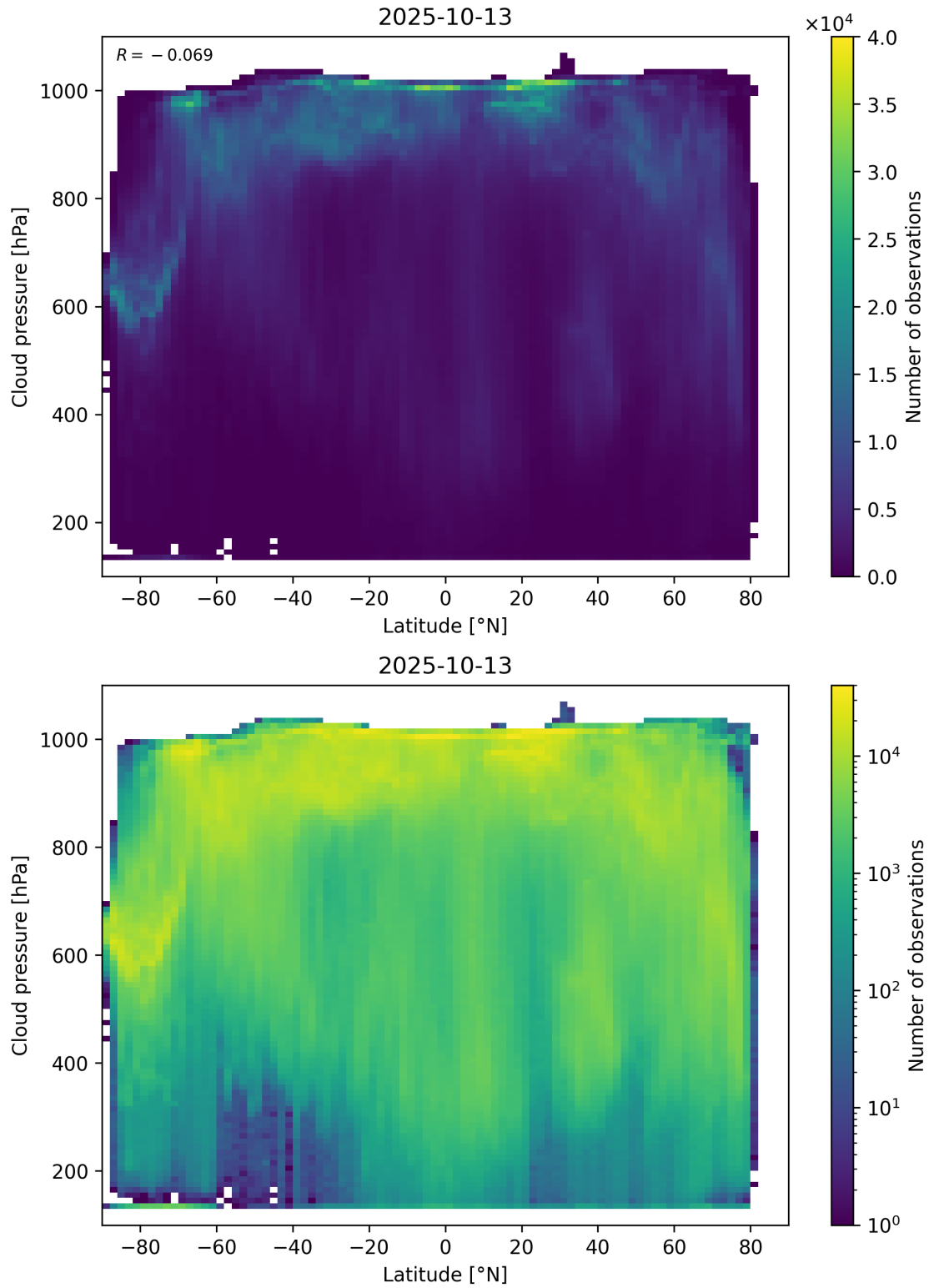
Figure 91: Scatter density plot of “Latitude” against “Cloud pressure” for 2025-10-12 to 2025-10-14.
