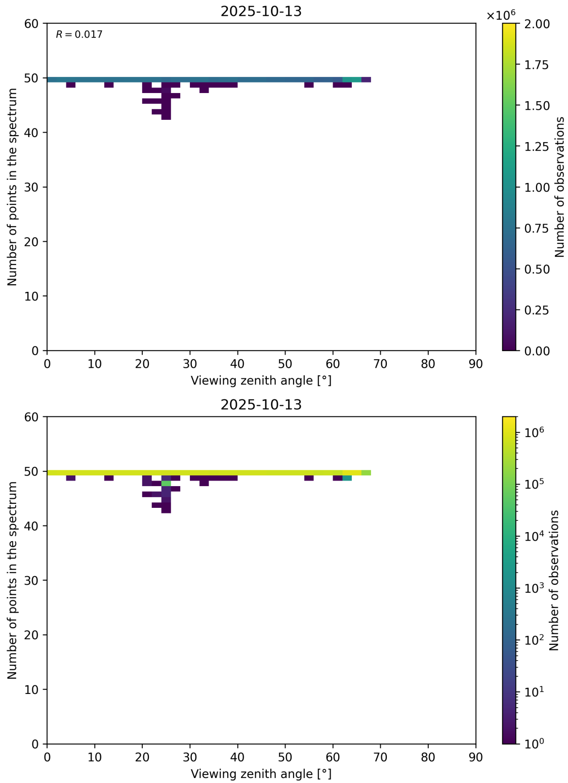
Figure 125: Scatter density plot of “Viewing zenith angle” against “Number of points in the spectrum” for 2025-10-12 to 2025-10-14.
