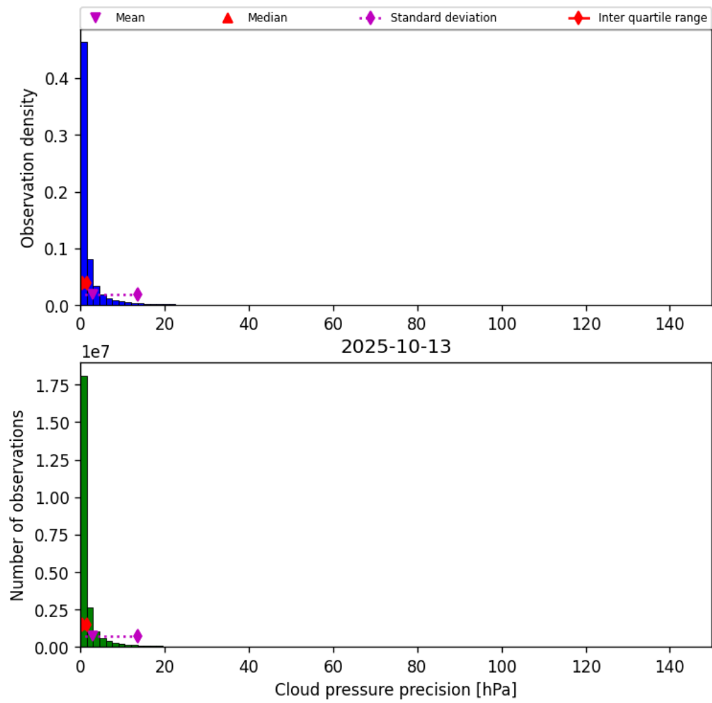
Figure 31: Histogram of “Cloud pressure precision” for 2025-10-12 to 2025-10-14
