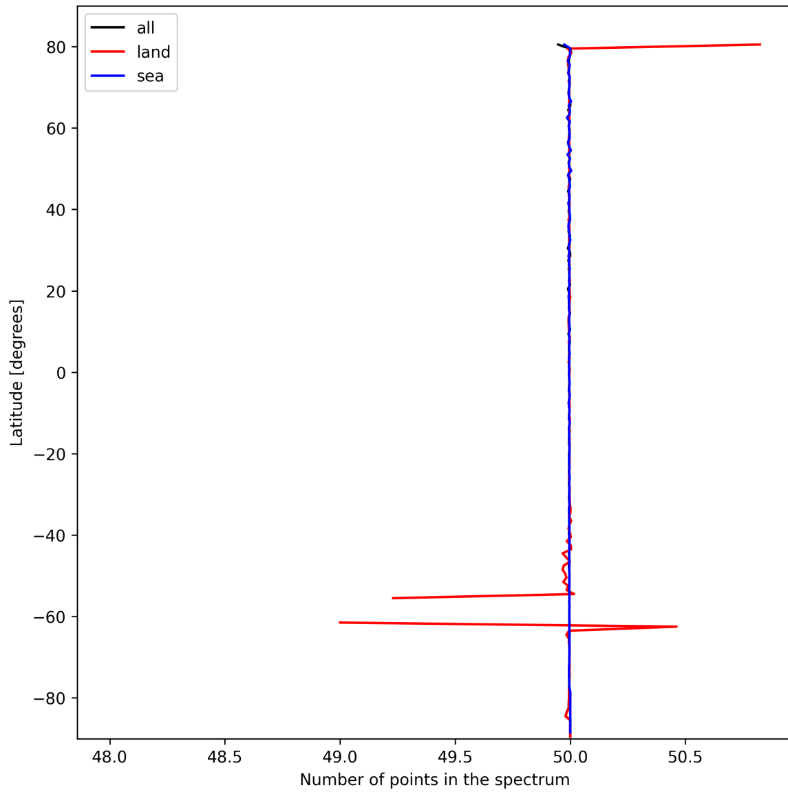
Figure 27: Zonal average of “Number of points in the spectrum” for 2025-10-12 to 2025-10-14.
