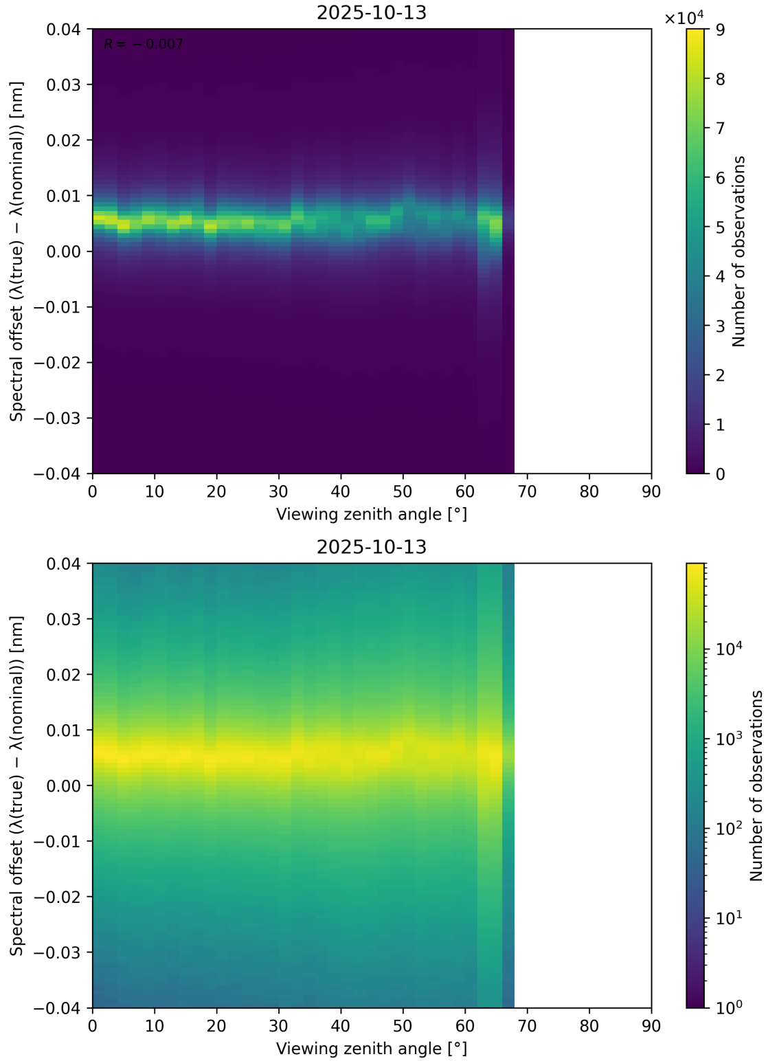
Figure 128: Scatter density plot of “Viewing zenith angle” against “Spectral offset ( \lambda_{\text{true}} - \lambda_{\text{nominal}} )” for 2025-10-12 to 2025-10-14.
