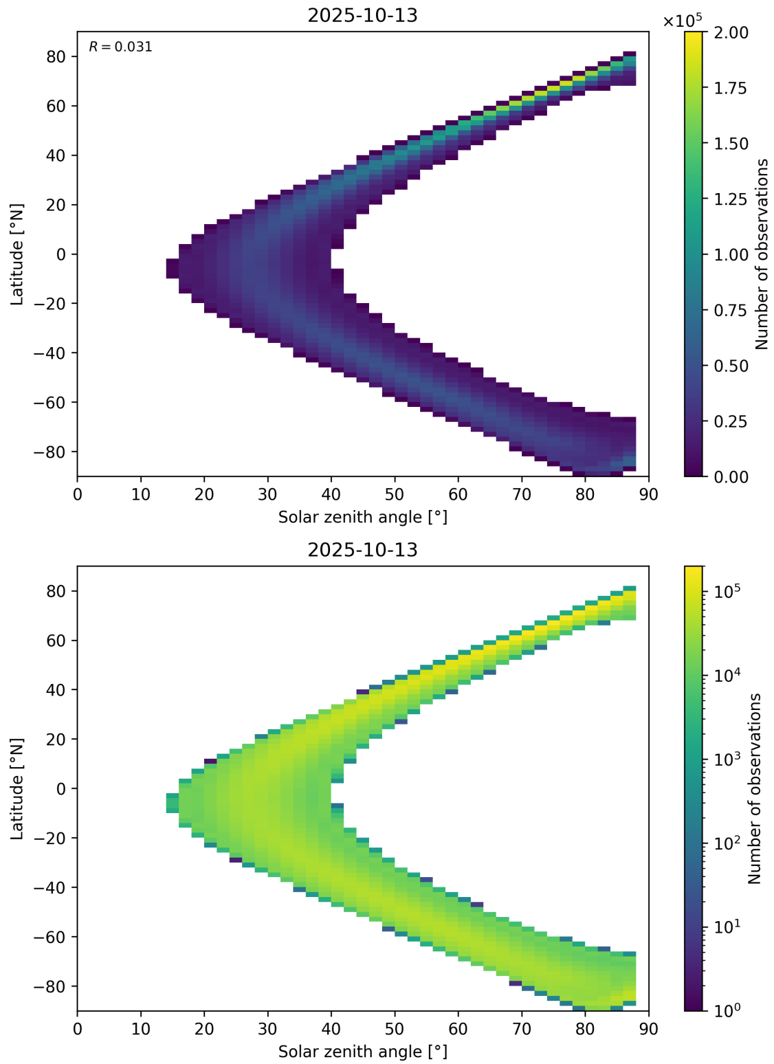
Figure 113: Scatter density plot of “Solar zenith angle” against “Latitude” for 2025-10-12 to 2025-10-14.
