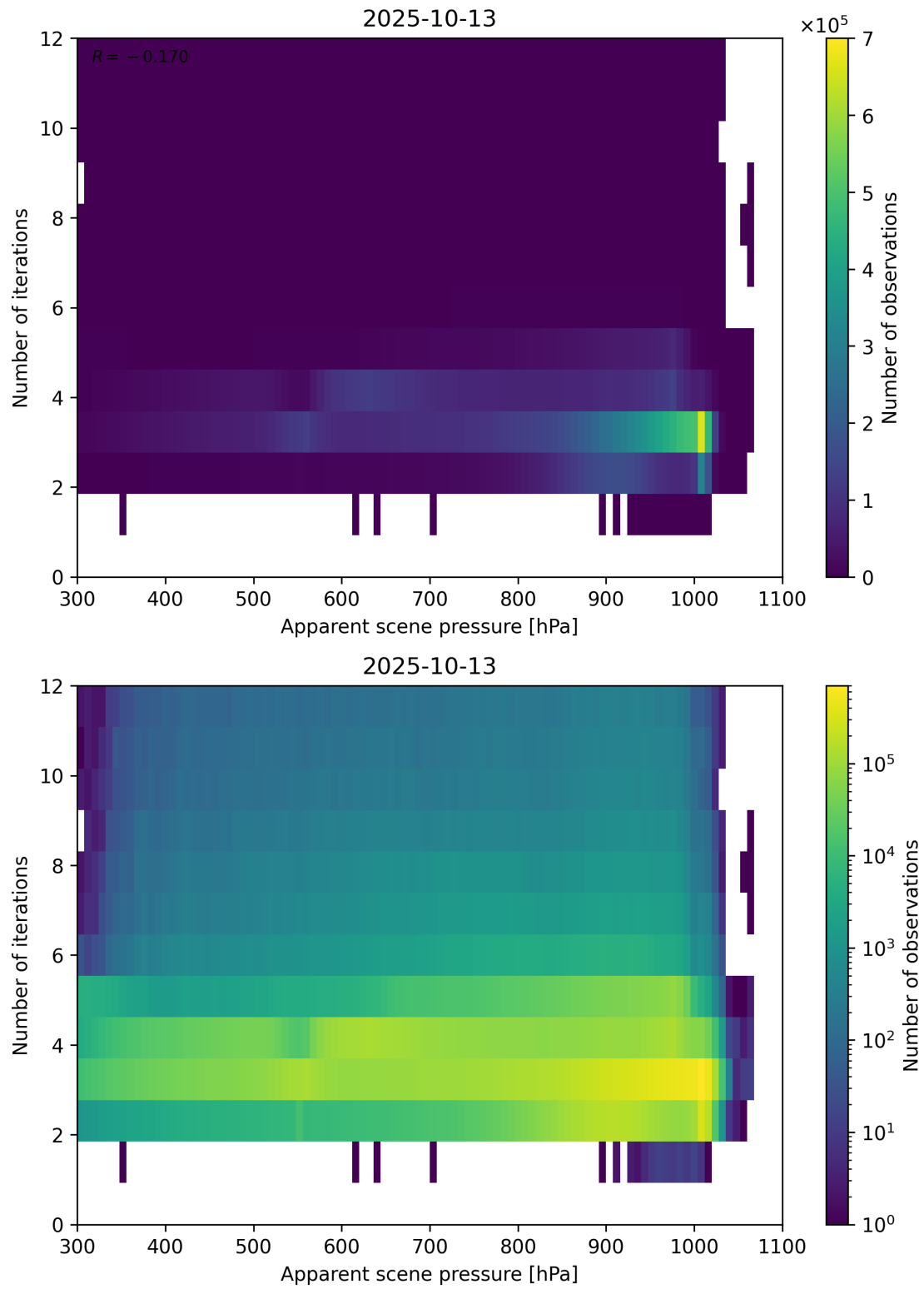
Figure 65: Scatter density plot of “Apparent scene pressure” against “Number of iterations” for 2025-10-12 to 2025-10-14.
