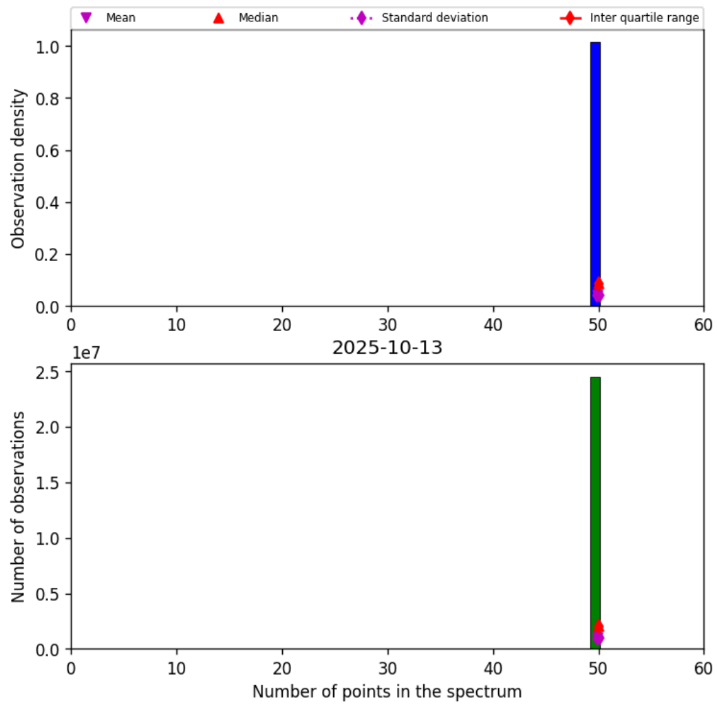
Figure 44: Histogram of “Number of points in the spectrum” for 2025-10-12 to 2025-10-14
