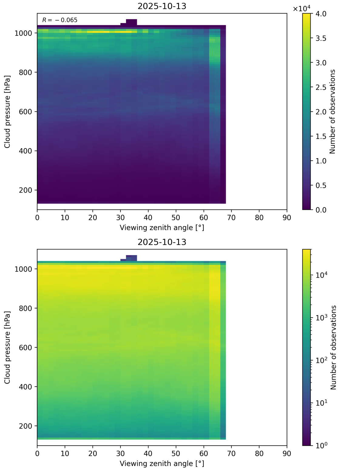
Figure 121: Scatter density plot of “Viewing zenith angle” against “Cloud pressure” for 2025-10-12 to 2025-10-14.
