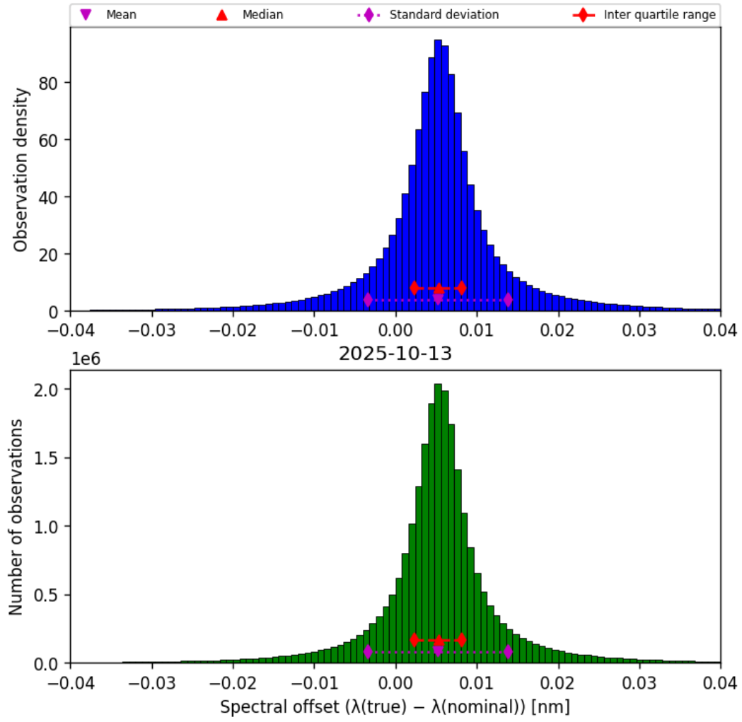
Figure 45: Histogram of “Spectral offset ( \lambda_{\text{true}} - \lambda_{\text{nominal}} )” for 2025-10-12 to 2025-10-14
