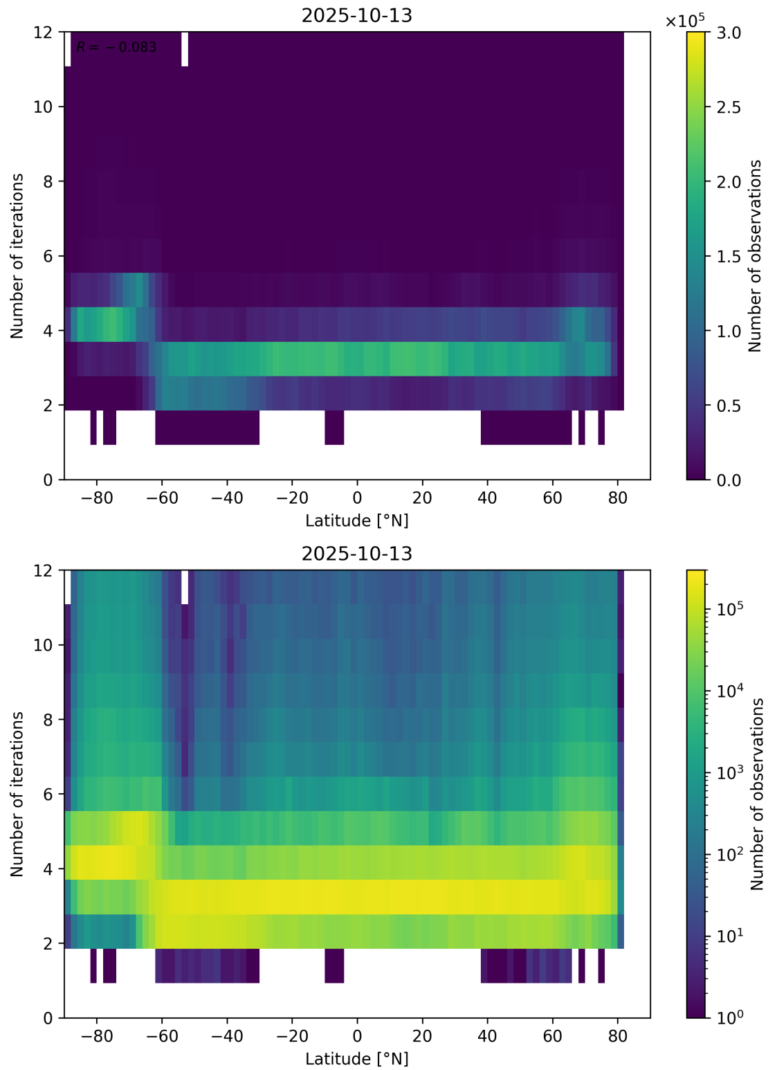
Figure 93: Scatter density plot of “Latitude” against “Number of iterations” for 2025-10-12 to 2025-10-14.
