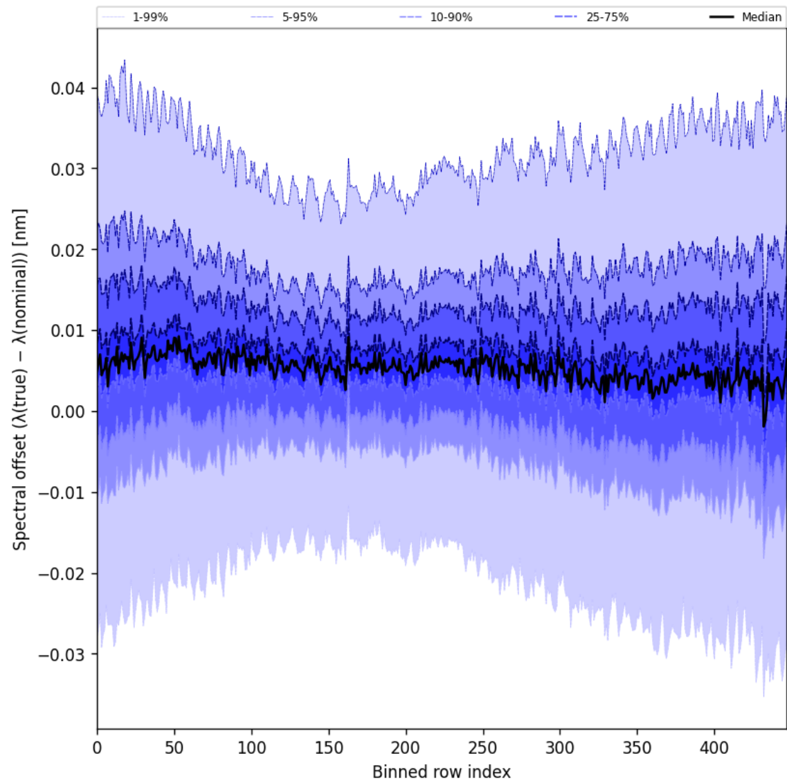
Figure 62: Along track statistics of “Spectral offset ( \lambda_{\text{true}} - \lambda_{\text{nominal}} )” for 2025-10-12 to 2025-10-14
