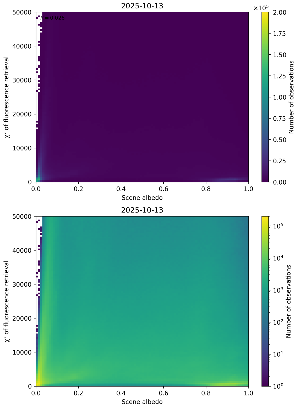
Figure 103: Scatter density plot of “Scene albedo” against “ \chi^2 of fluorescence retrieval” for 2025-10-12 to 2025-10-14.
