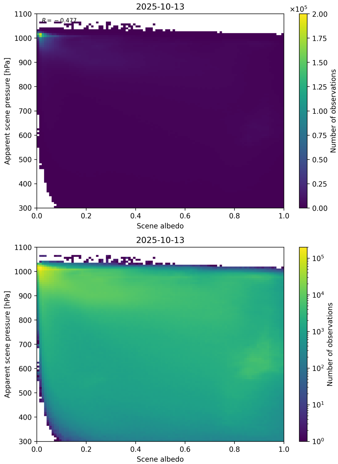
Figure 102: Scatter density plot of “Scene albedo” against “Apparent scene pressure” for 2025-10-12 to 2025-10-14.
