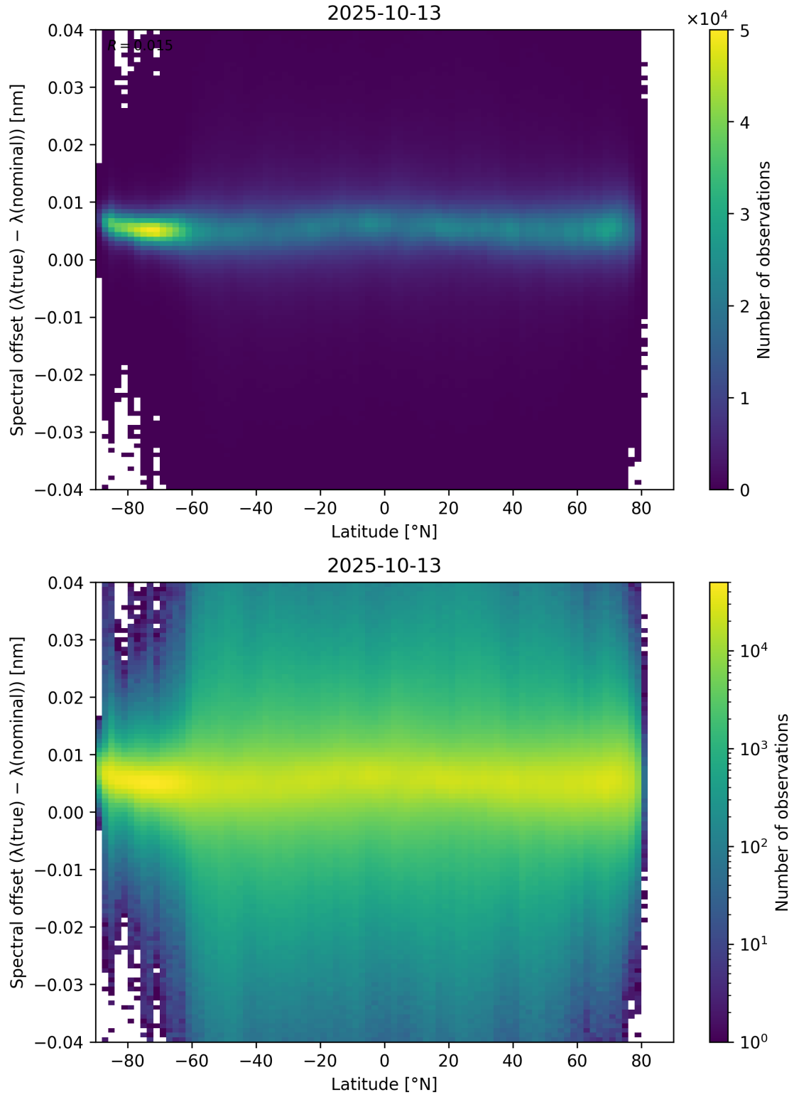
Figure 96: Scatter density plot of “Latitude” against “Spectral offset ( \lambda_{\text{true}} - \lambda_{\text{nominal}} )” for 2025-10-12 to 2025-10-14.
