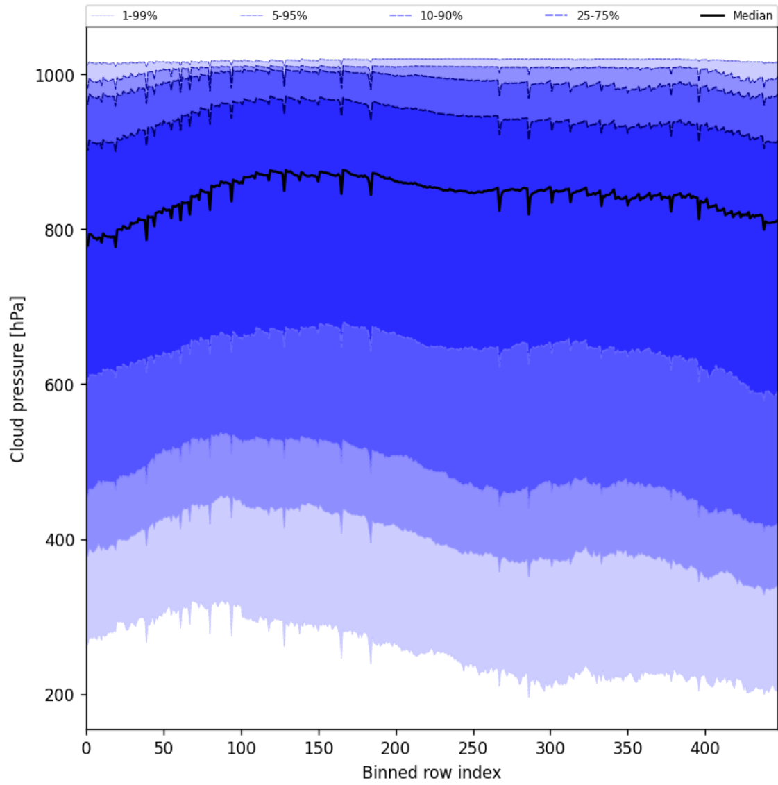
Figure 47: Along track statistics of “Cloud pressure” for 2025-10-12 to 2025-10-14
