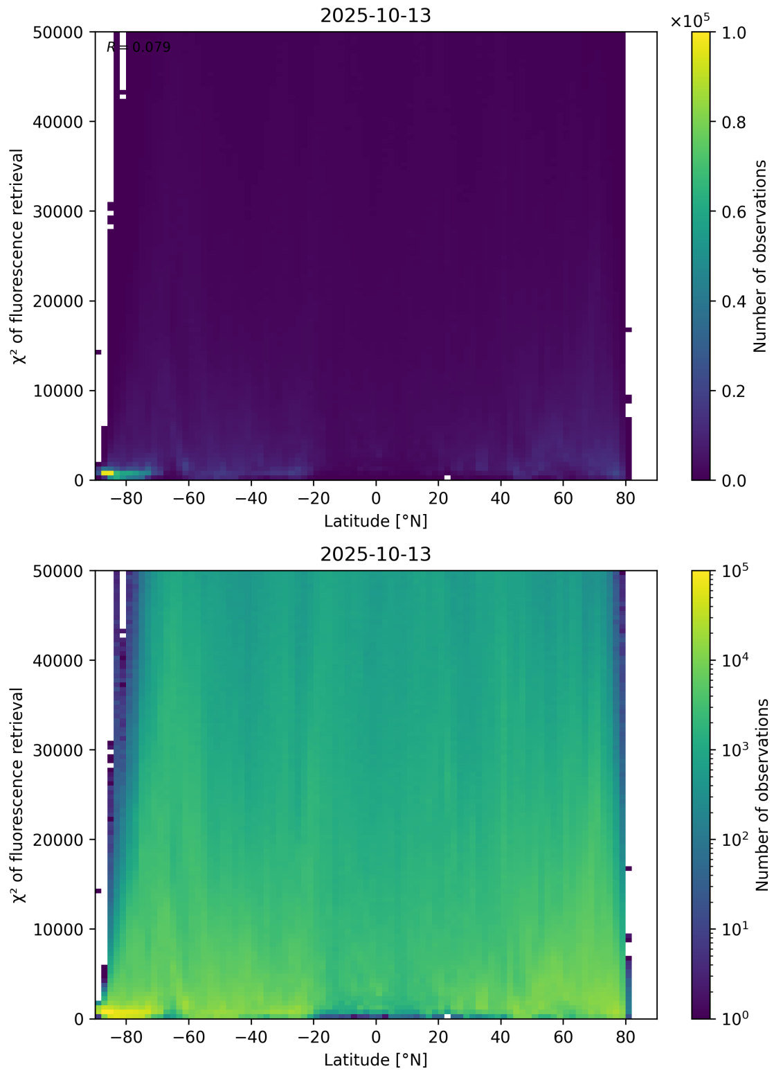
Figure 89: Scatter density plot of “Latitude” against “ \chi^2 of fluorescence retrieval” for 2025-10-12 to 2025-10-14.
