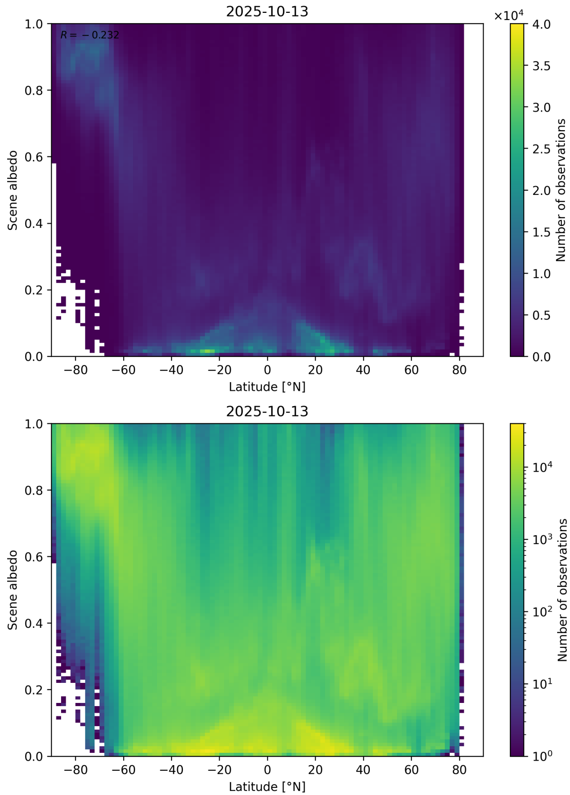
Figure 95: Scatter density plot of “Latitude” against “Scene albedo” for 2025-10-12 to 2025-10-14.
