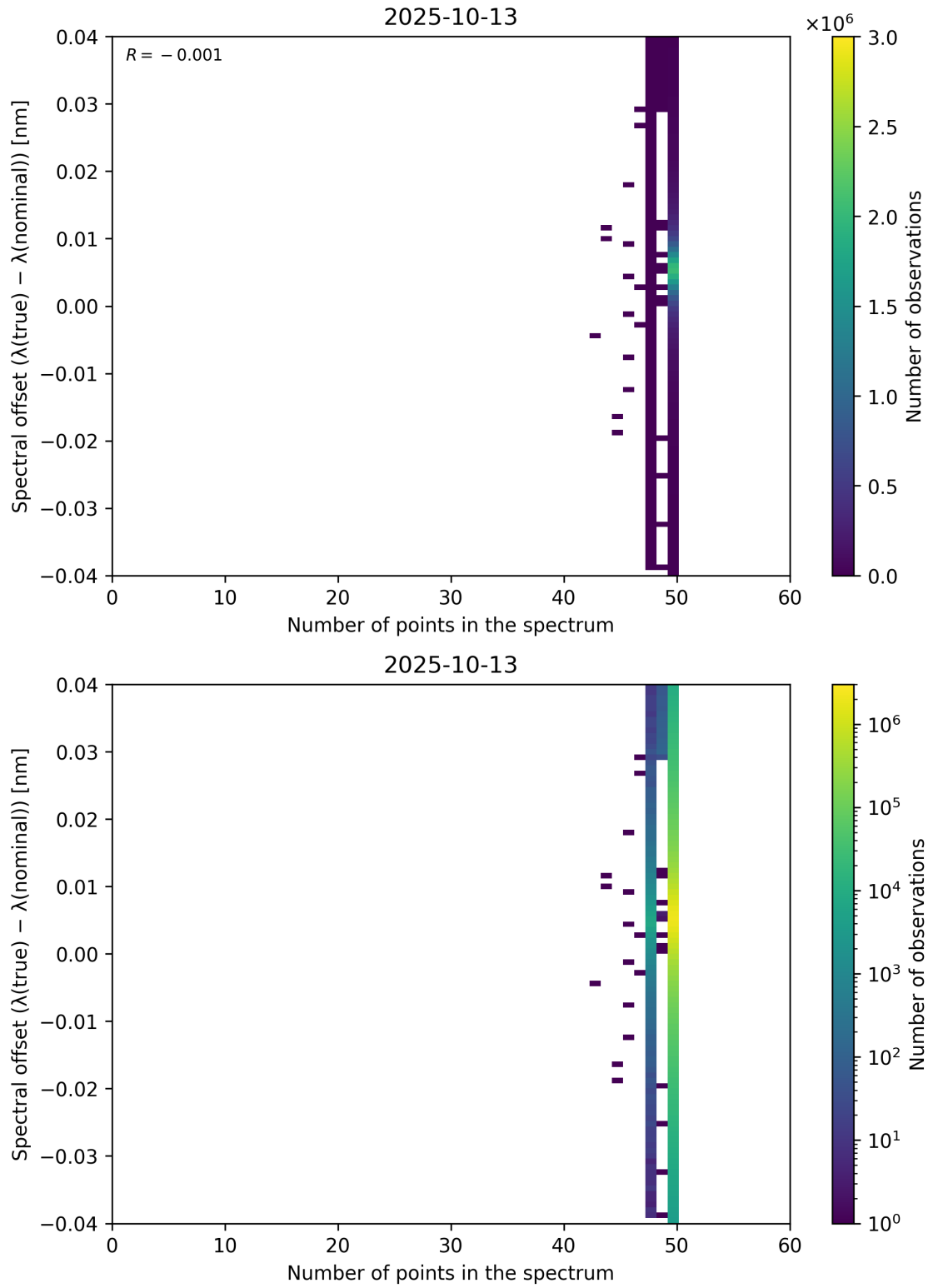
Figure 101: Scatter density plot of “Number of points in the spectrum” against “Spectral offset ( \lambda_{\text{true}} - \lambda_{\text{nominal}} )” for 2025-10-12 to 2025-10-14.
