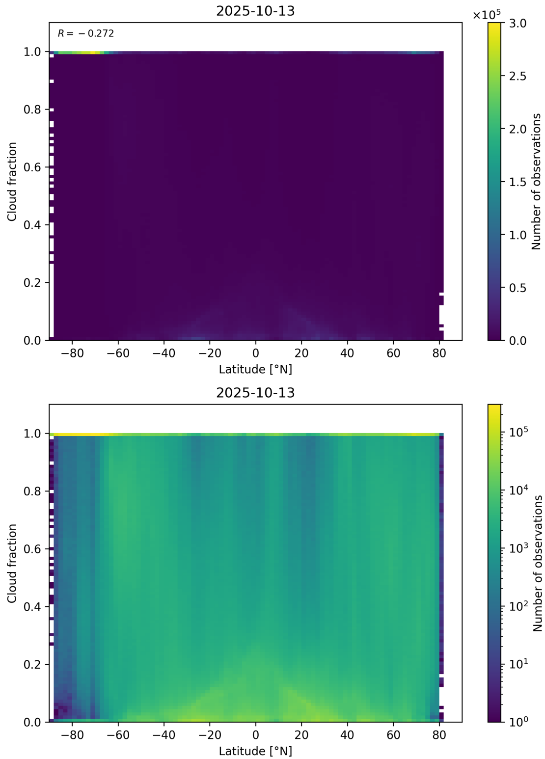
Figure 90: Scatter density plot of “Latitude” against “Cloud fraction” for 2025-10-12 to 2025-10-14.
