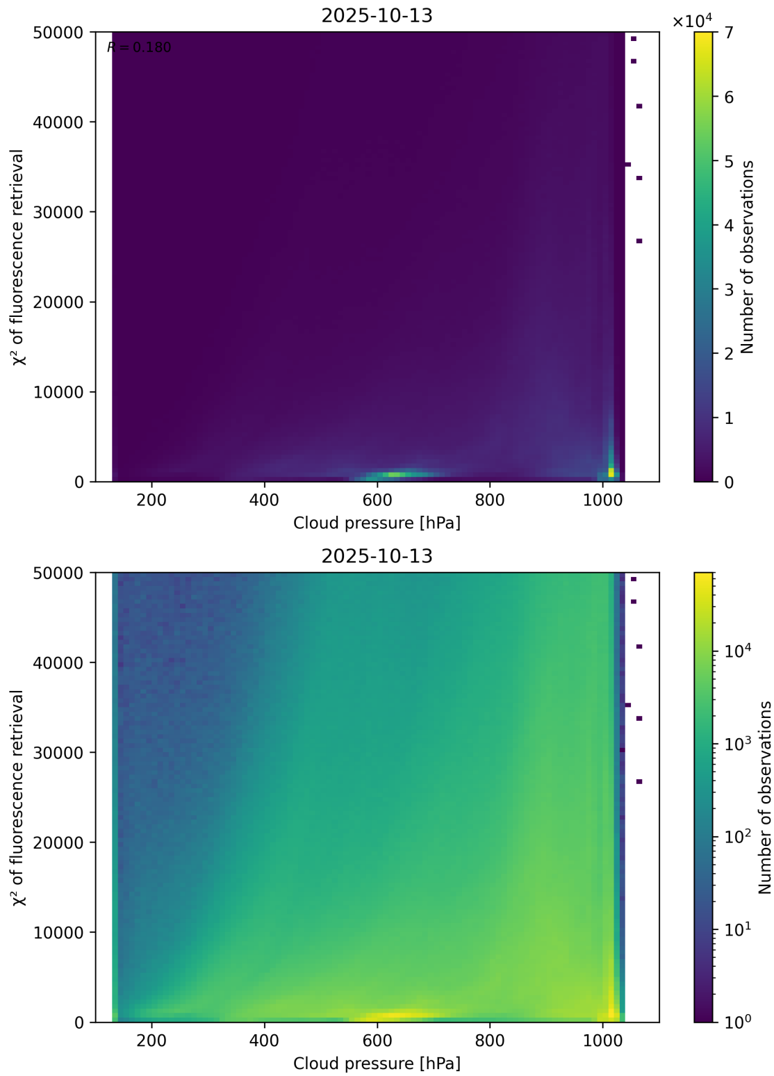
Figure 78: Scatter density plot of “Cloud pressure” against “ \chi^2 of fluorescence retrieval” for 2025-10-12 to 2025-10-14.
