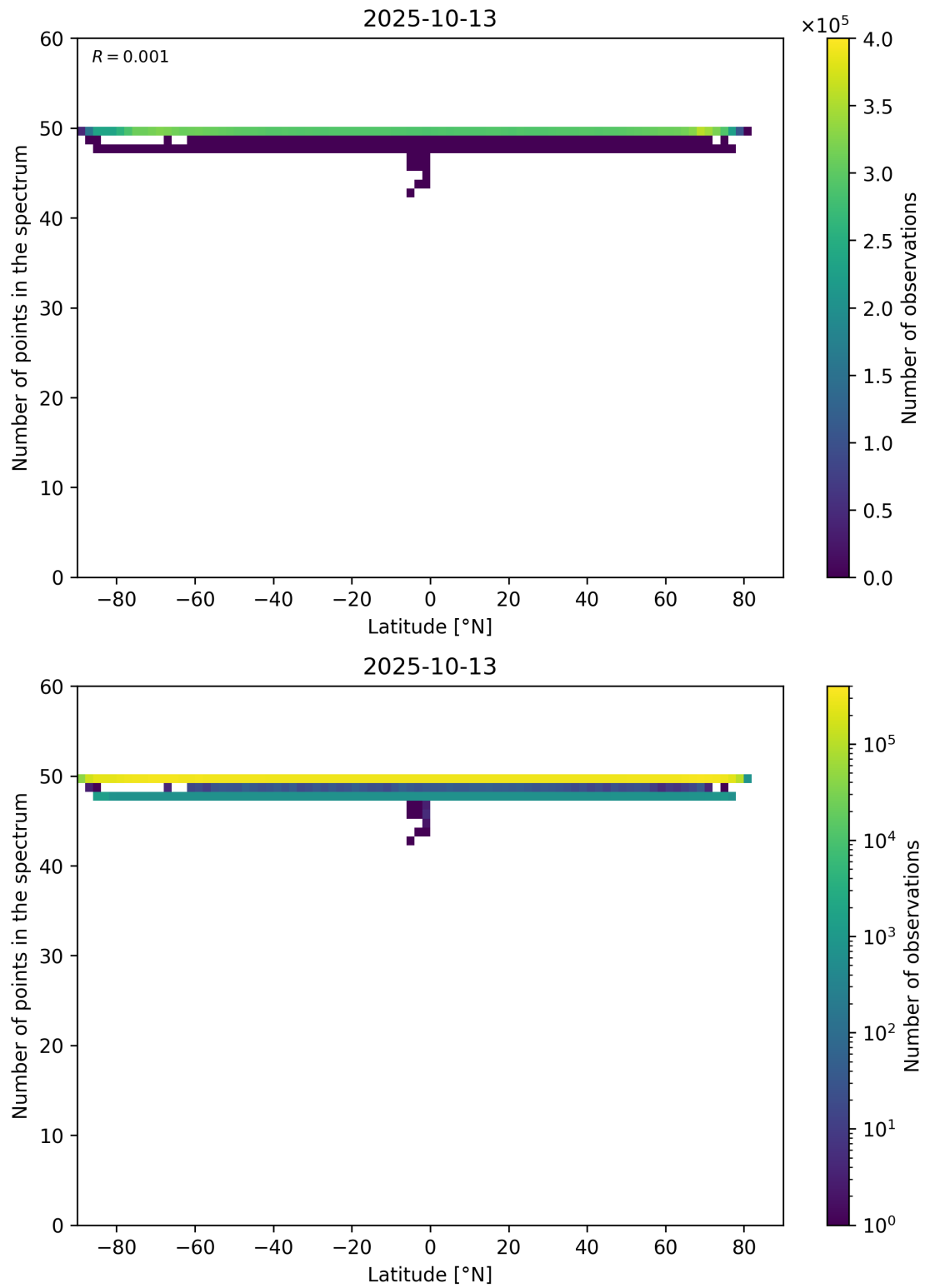
Figure 94: Scatter density plot of “Latitude” against “Number of points in the spectrum” for 2025-10-12 to 2025-10-14.
