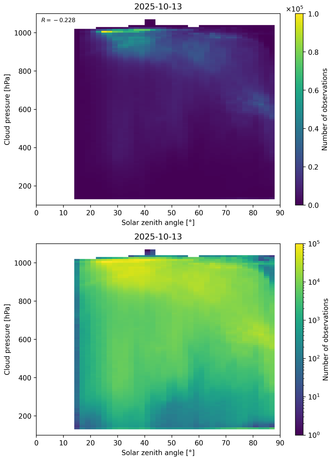
Figure 111: Scatter density plot of “Solar zenith angle” against “Cloud pressure” for 2025-10-12 to 2025-10-14.
