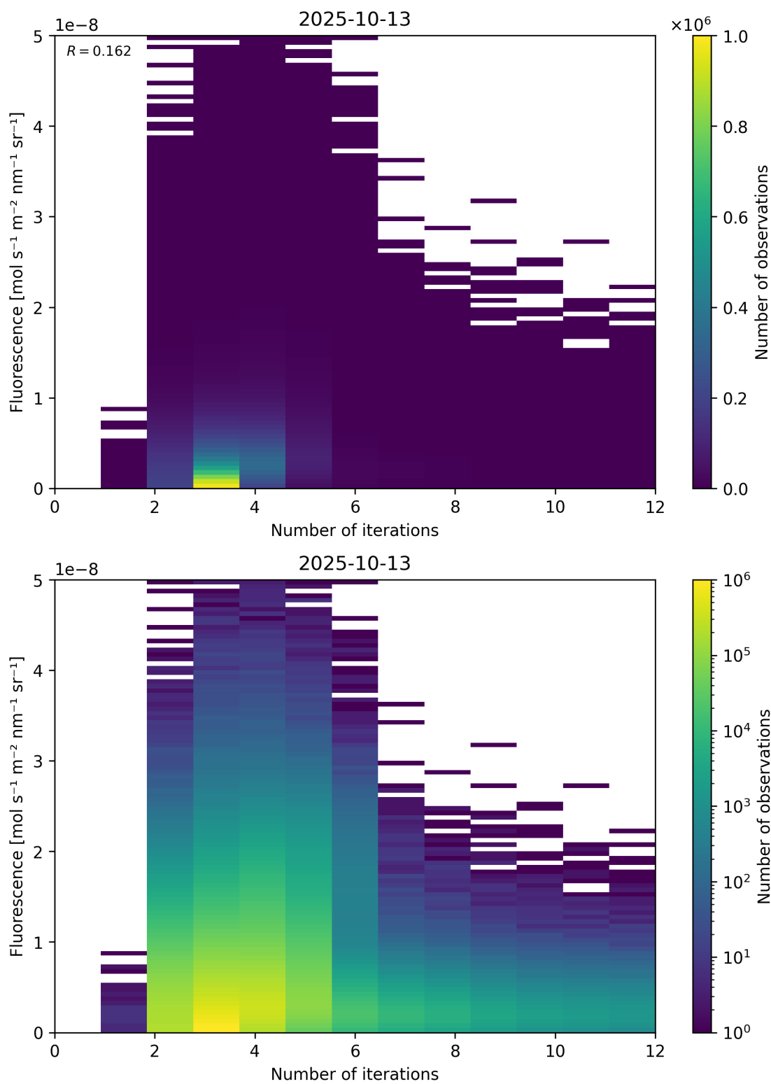
Figure 98: Scatter density plot of “Number of iterations” against “Fluorescence” for 2025-10-12 to 2025-10-14.
