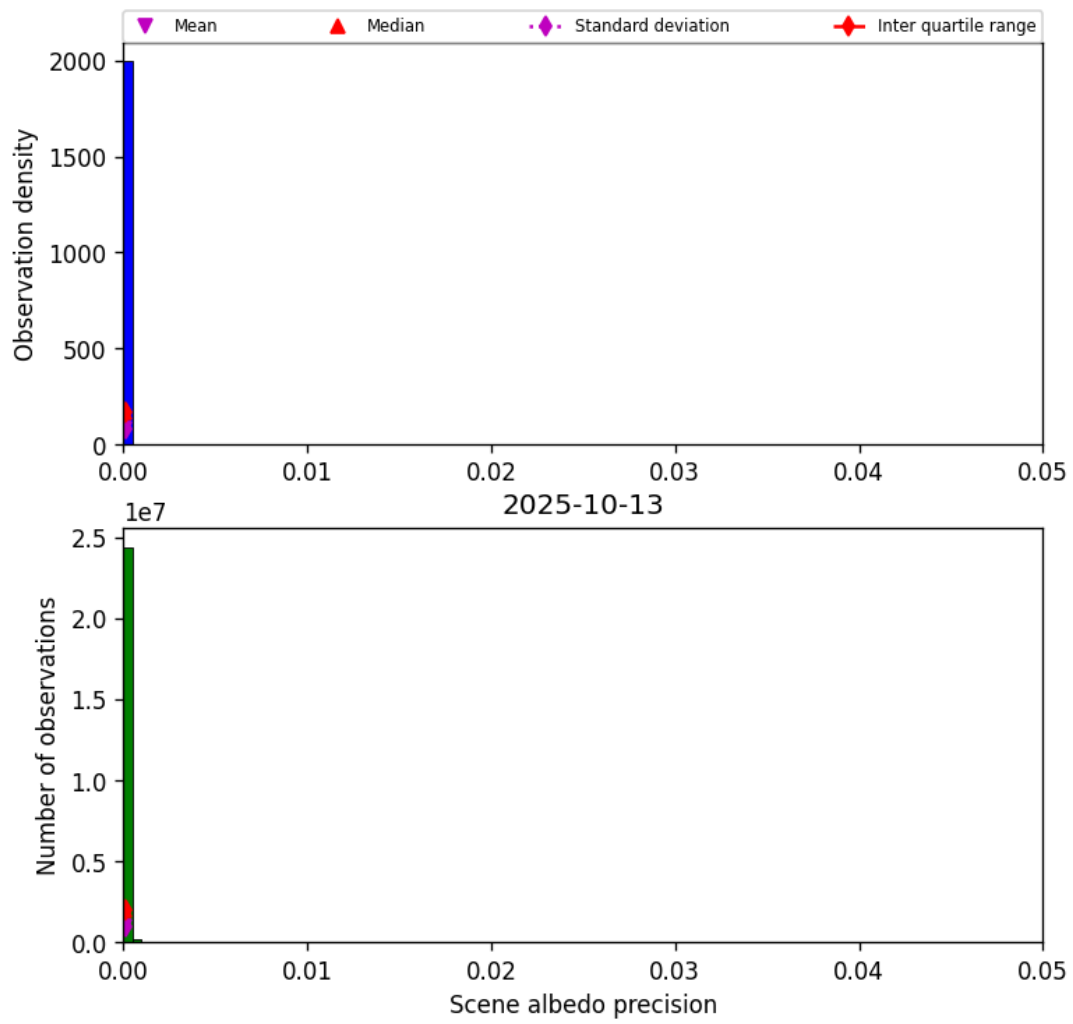
Figure 35: Histogram of “Scene albedo precision” for 2025-10-12 to 2025-10-14
