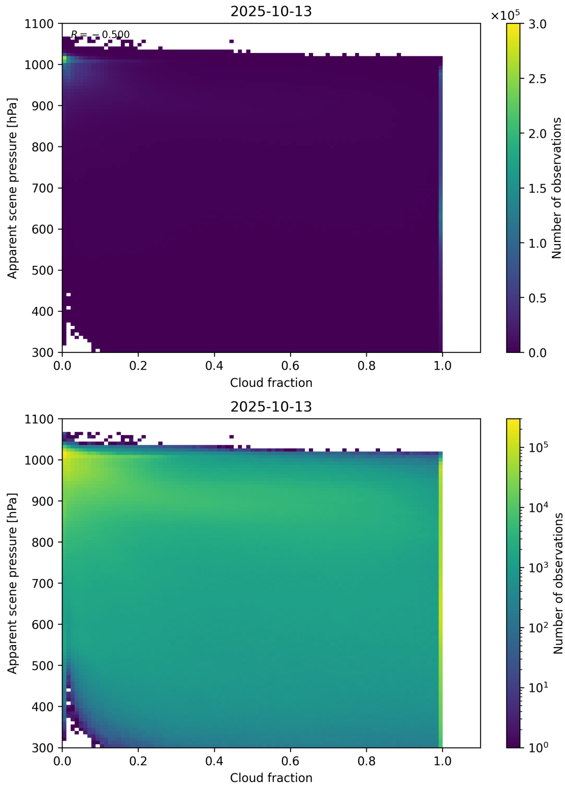
Figure 70: Scatter density plot of “Cloud fraction” against “Apparent scene pressure” for 2025-10-12 to 2025-10-14.
