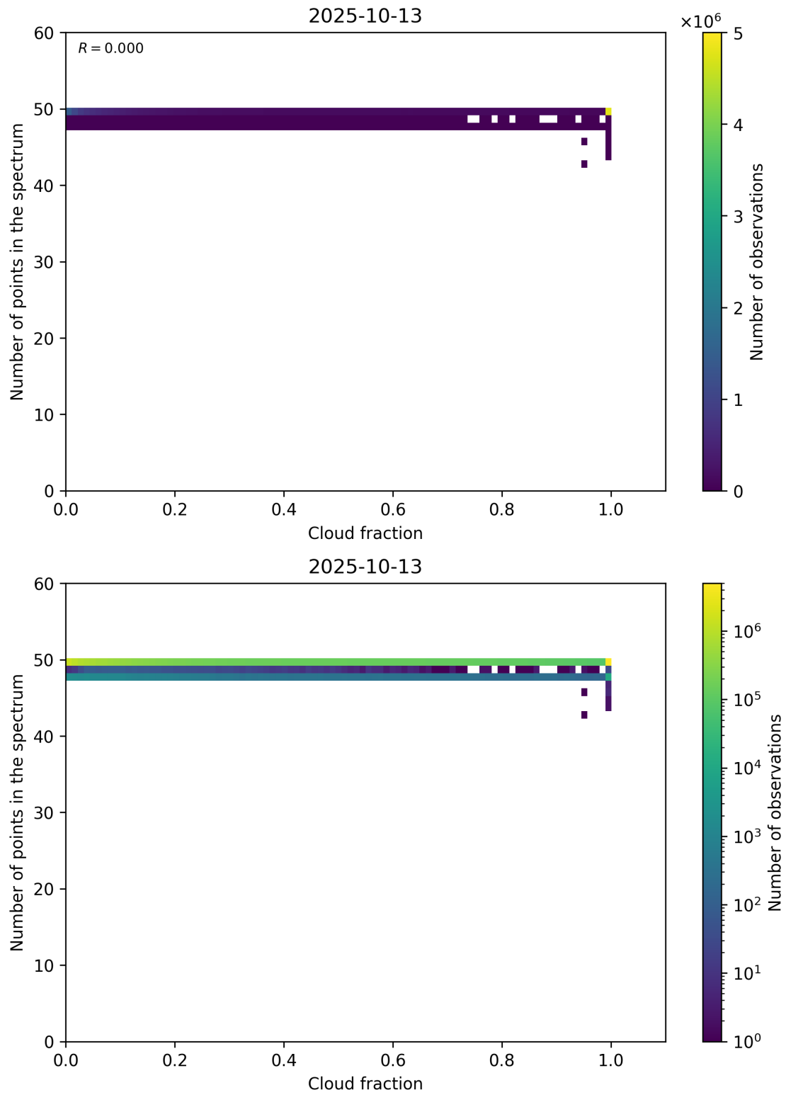
Figure 74: Scatter density plot of “Cloud fraction” against “Number of points in the spectrum” for 2025-10-12 to 2025-10-14.
