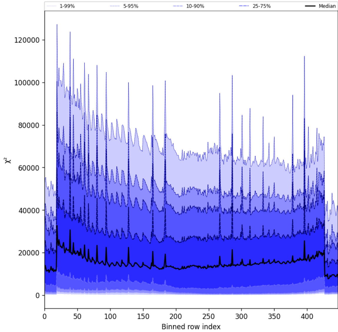
Figure 55: Along track statistics of “ \chi^2 ” for 2025-10-12 to 2025-10-14
