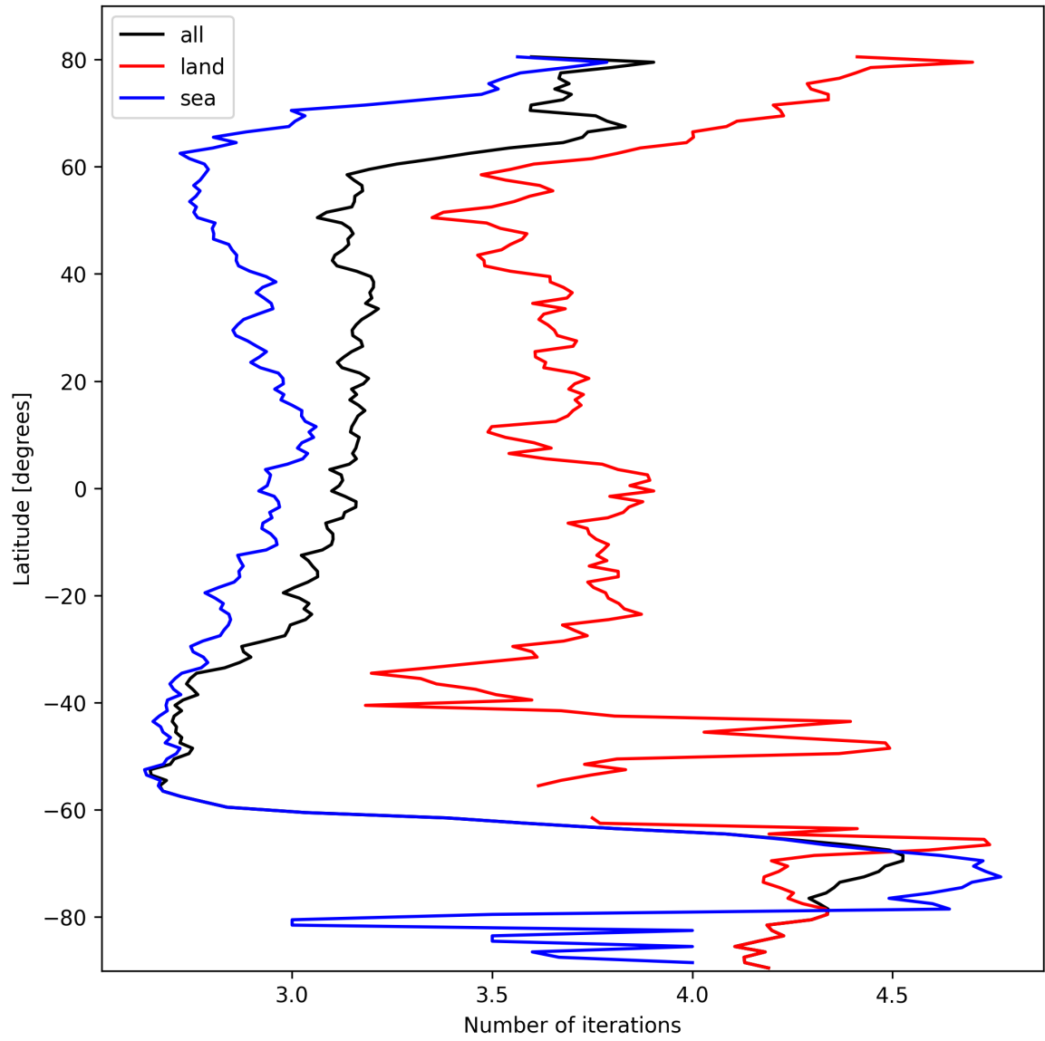
Figure 22: Zonal average of “Number of iterations” for 2025-10-12 to 2025-10-14.
