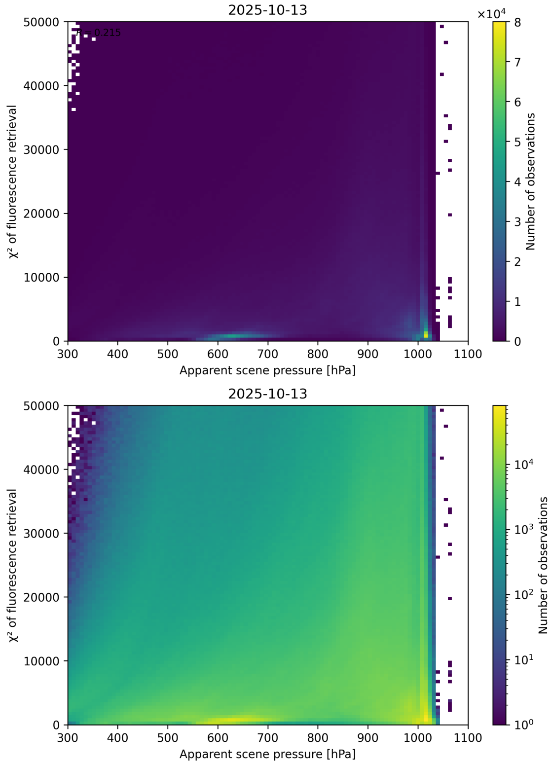
Figure 63: Scatter density plot of “Apparent scene pressure” against “ \chi^2 of fluorescence retrieval” for 2025-10-12 to 2025-10-14.
