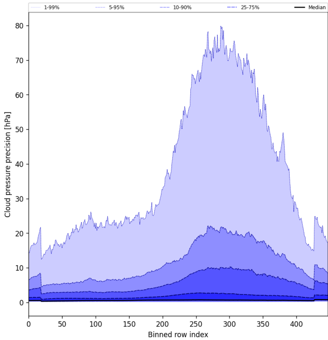
Figure 48: Along track statistics of “Cloud pressure precision” for 2025-10-12 to 2025-10-14
