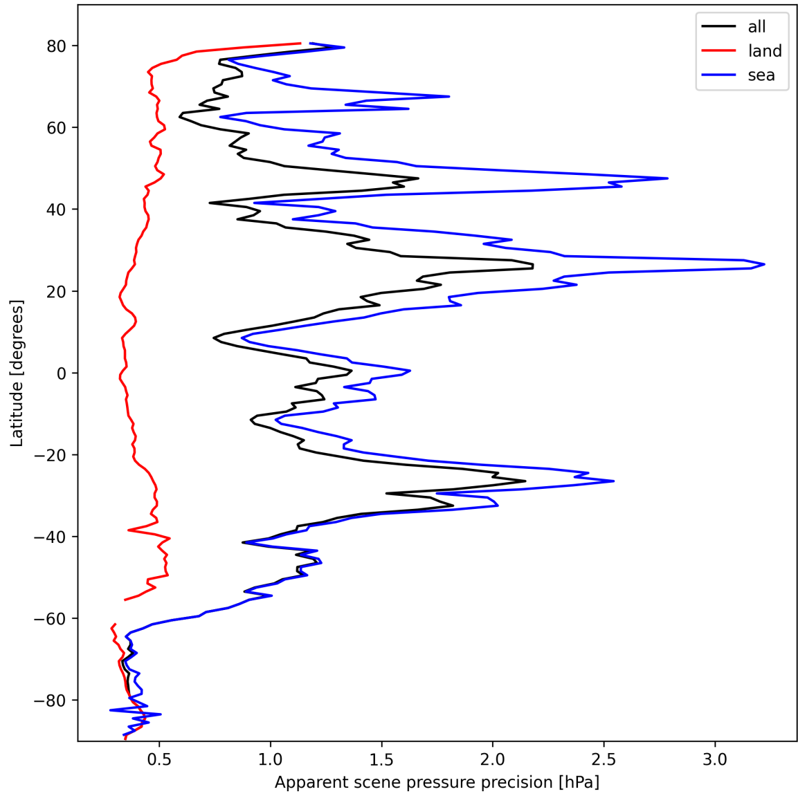
Figure 20: Zonal average of “Apparent scene pressure precision” for 2025-10-12 to 2025-10-14.
