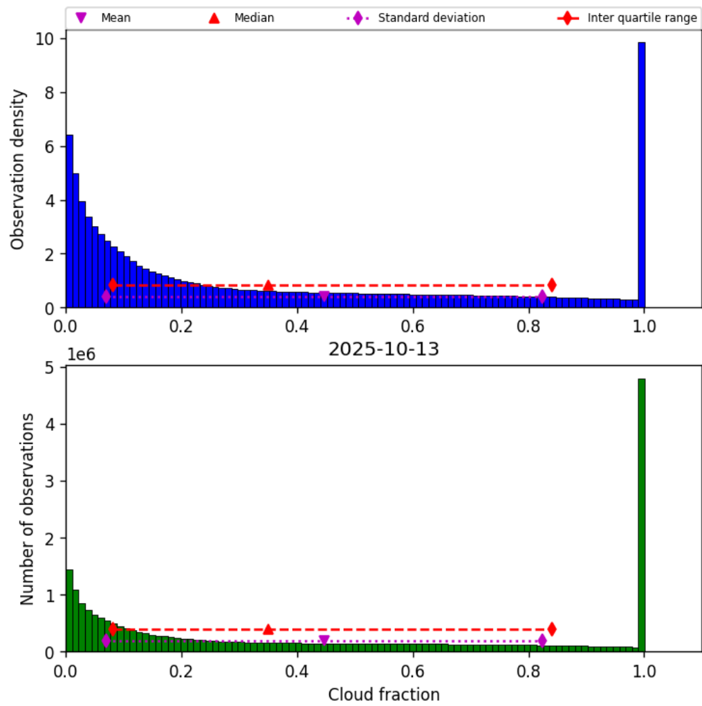
Figure 32: Histogram of “Cloud fraction” for 2025-10-12 to 2025-10-14
