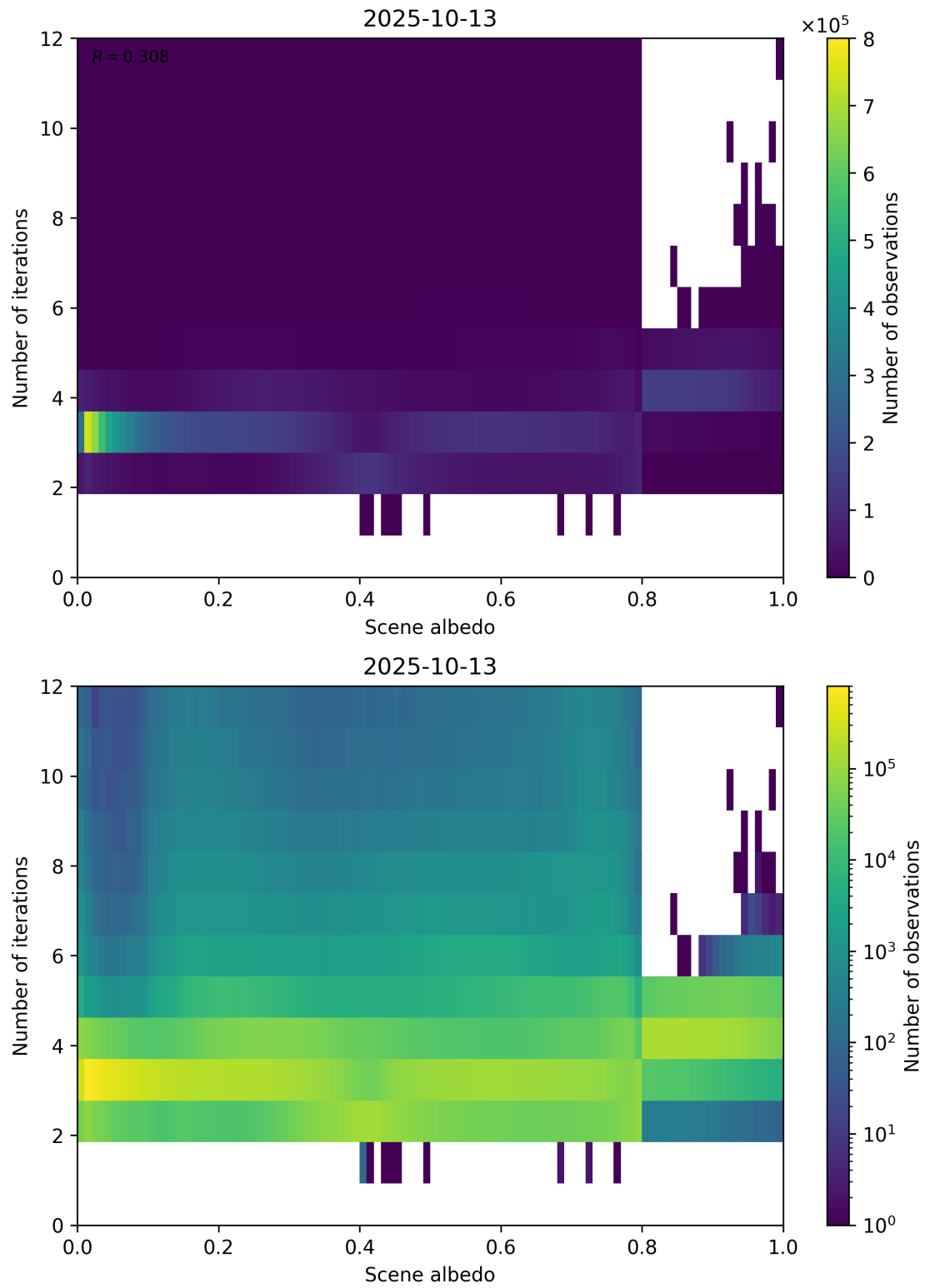
Figure 105: Scatter density plot of “Scene albedo” against “Number of iterations” for 2025-10-12 to 2025-10-14.
