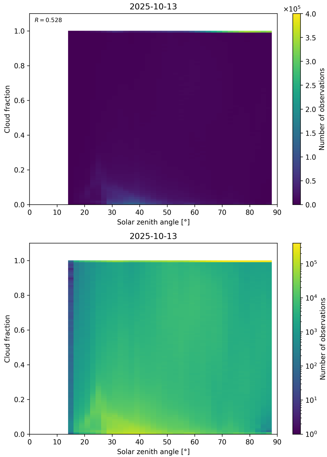
Figure 110: Scatter density plot of “Solar zenith angle” against “Cloud fraction” for 2025-10-12 to 2025-10-14.
