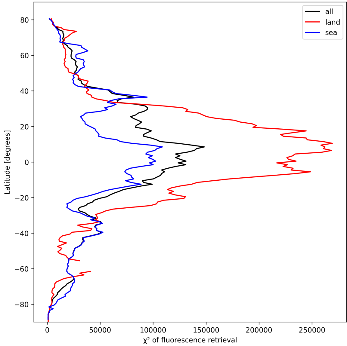
Figure 25: Zonal average of “ \chi^2 of fluorescence retrieval” for 2025-10-12 to 2025-10-14.
