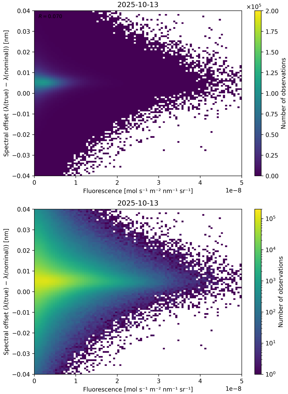
Figure 87: Scatter density plot of “Fluorescence” against “Spectral offset ( \lambda_{\text{true}} - \lambda_{\text{nominal}} )” for 2025-10-12 to 2025-10-14.
