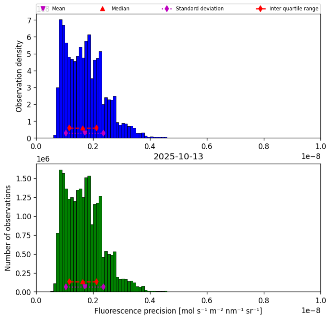
Figure 41: Histogram of “Fluorescence precision” for 2025-10-12 to 2025-10-14
