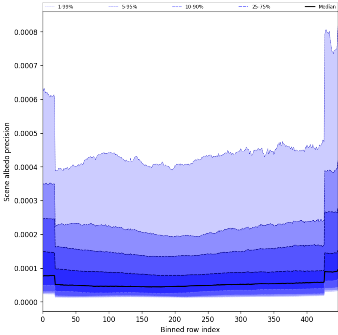
Figure 52: Along track statistics of “Scene albedo precision” for 2025-10-12 to 2025-10-14
