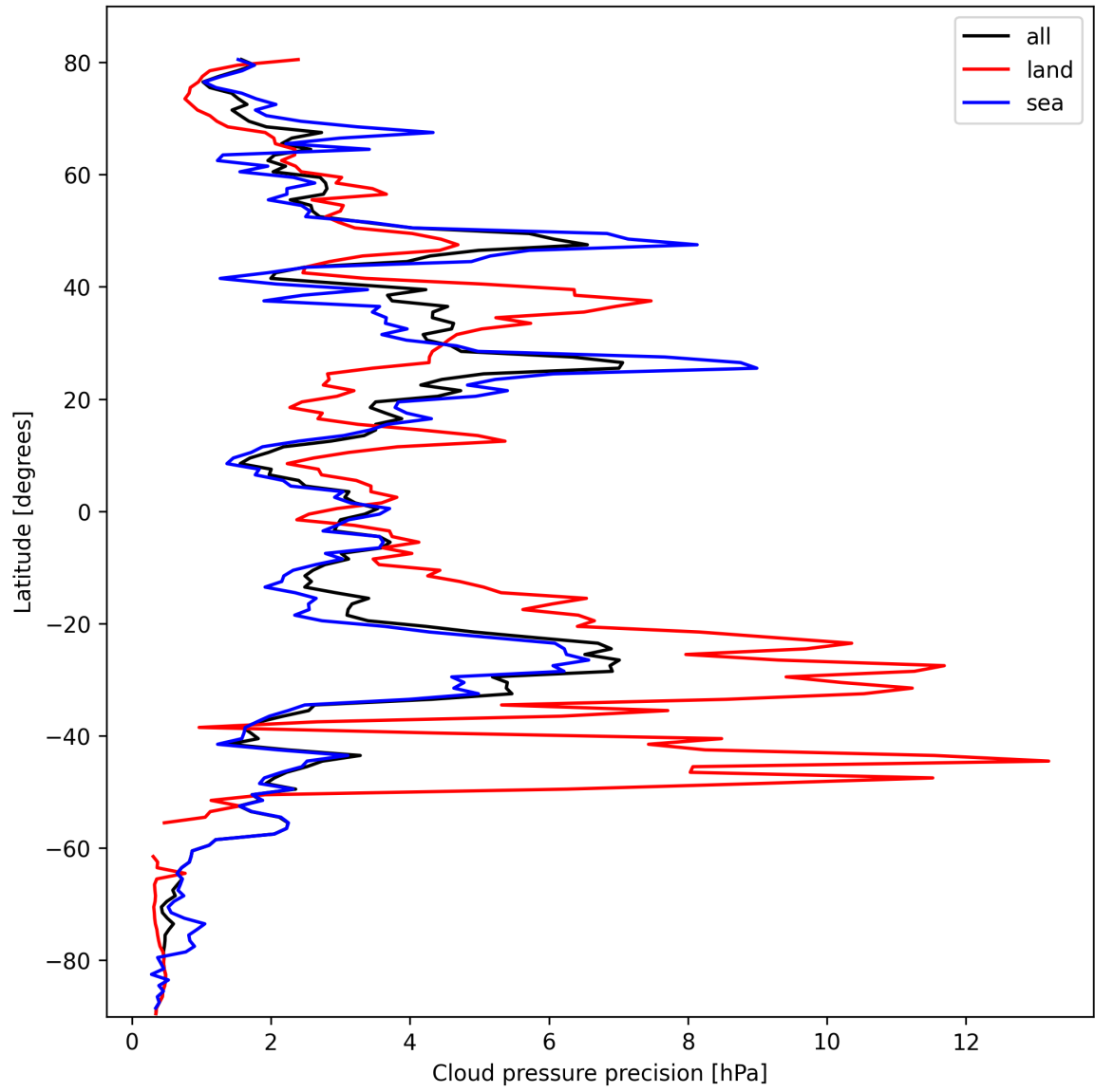
Figure 14: Zonal average of “Cloud pressure precision” for 2025-10-12 to 2025-10-14.
