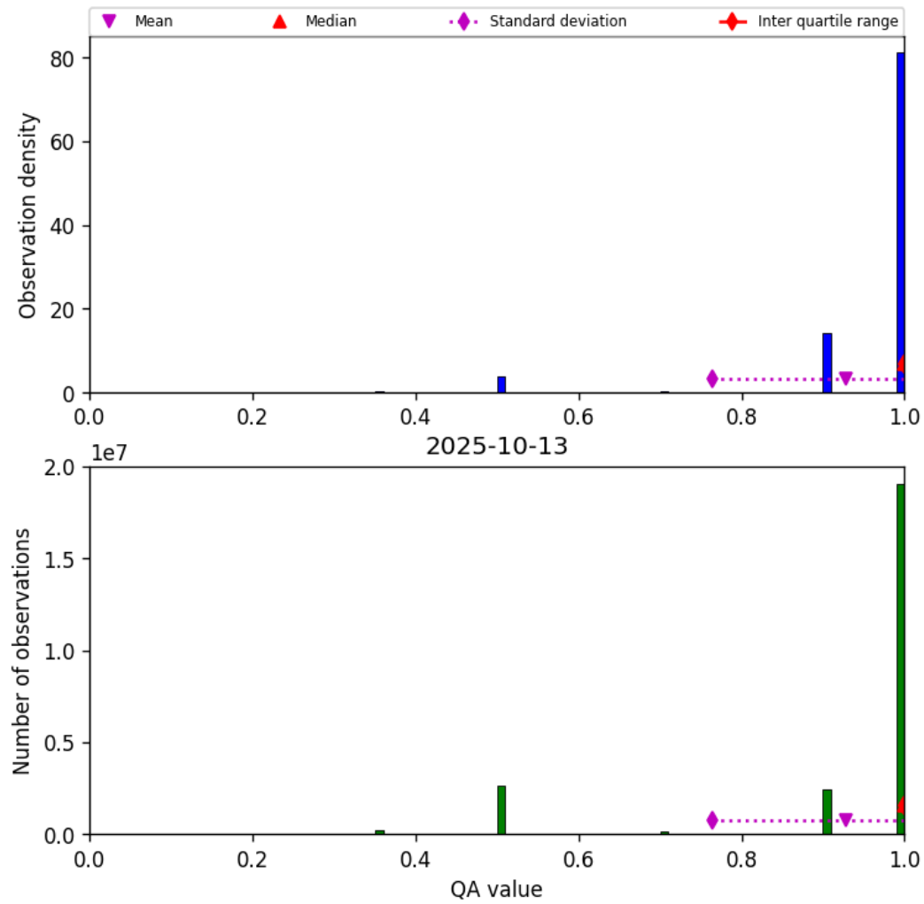
Figure 29: Histogram of “QA value” for 2025-10-12 to 2025-10-14
