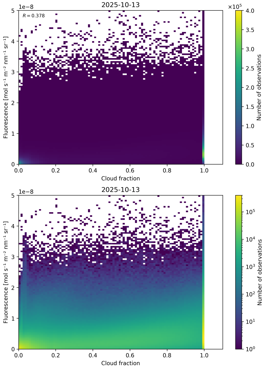
Figure 72: Scatter density plot of “Cloud fraction” against “Fluorescence” for 2025-10-12 to 2025-10-14.
