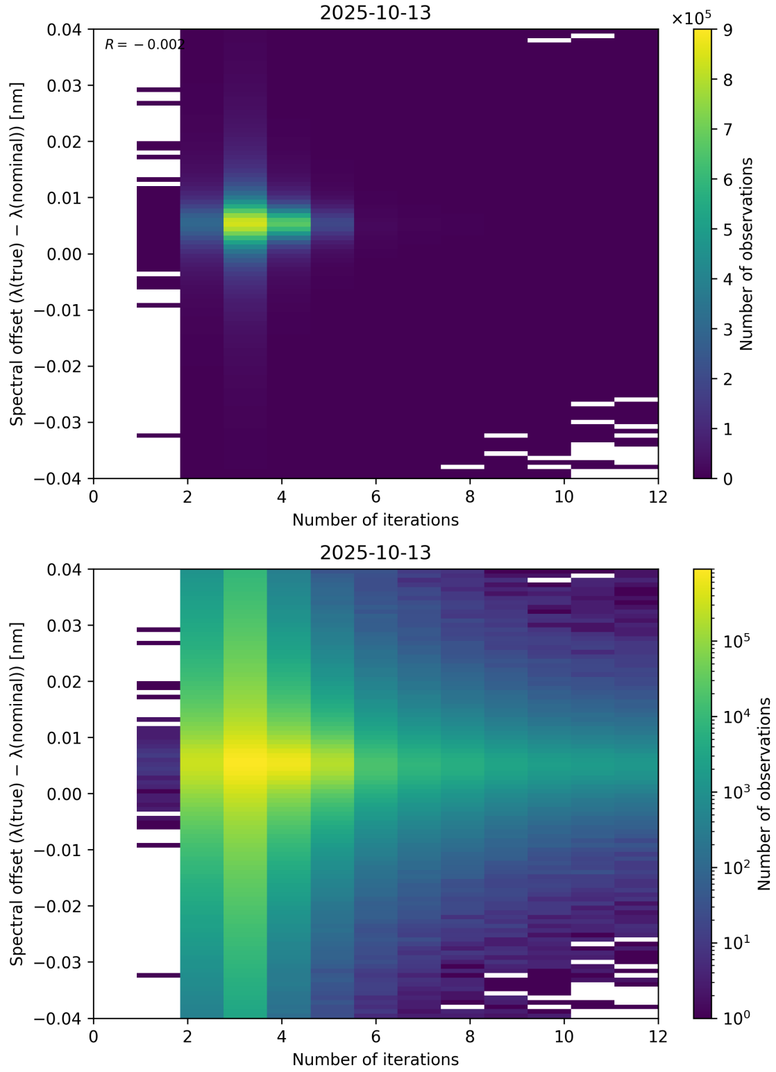
Figure 100: Scatter density plot of “Number of iterations” against “Spectral offset ( \lambda_{\text{true}} - \lambda_{\text{nominal}} )” for 2025-10-12 to 2025-10-14.
