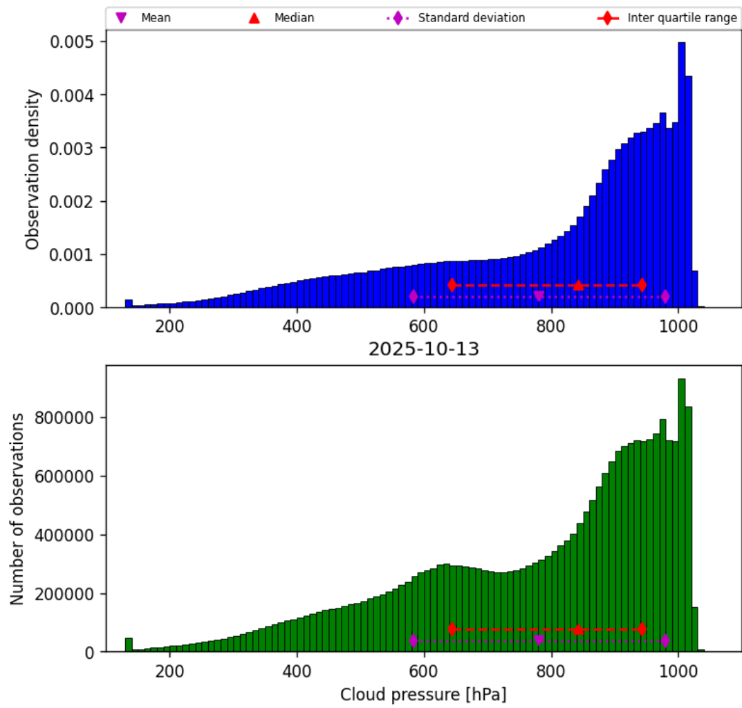
Figure 30: Histogram of “Cloud pressure” for 2025-10-12 to 2025-10-14
