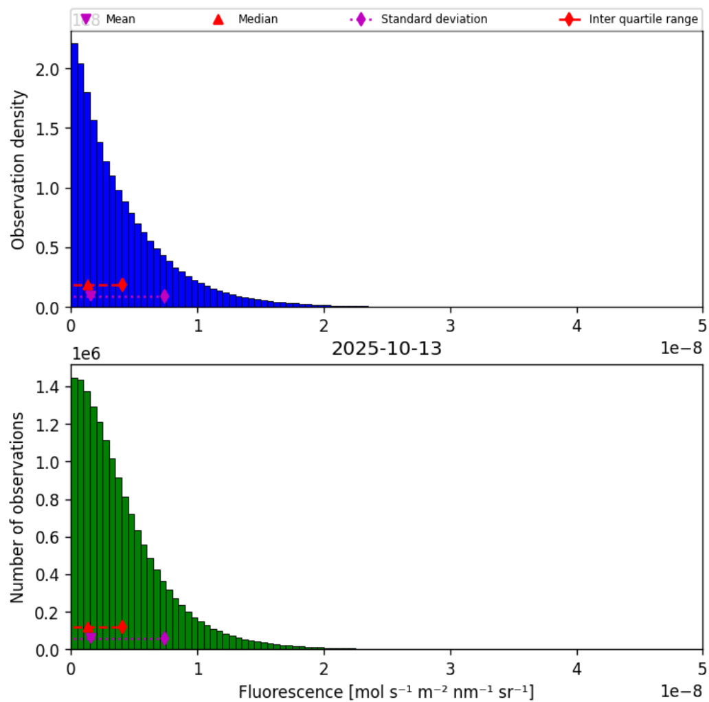
Figure 40: Histogram of “Fluorescence” for 2025-10-12 to 2025-10-14
