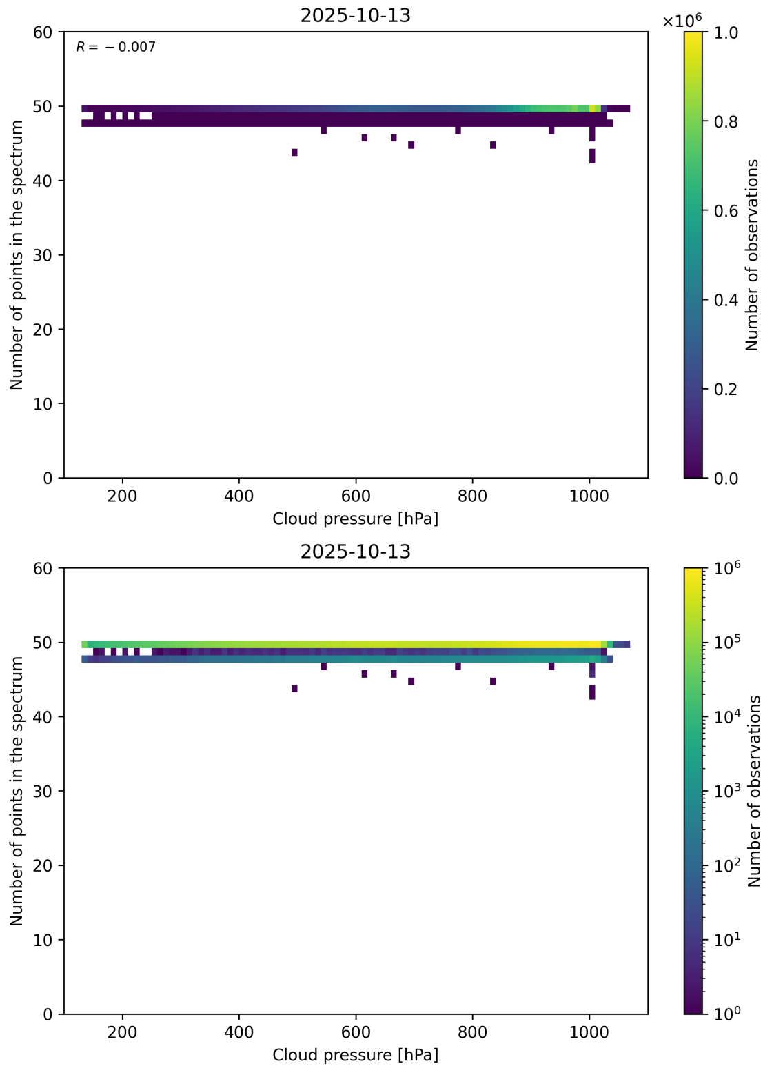
Figure 82: Scatter density plot of “Cloud pressure” against “Number of points in the spectrum” for 2025-10-12 to 2025-10-14.
