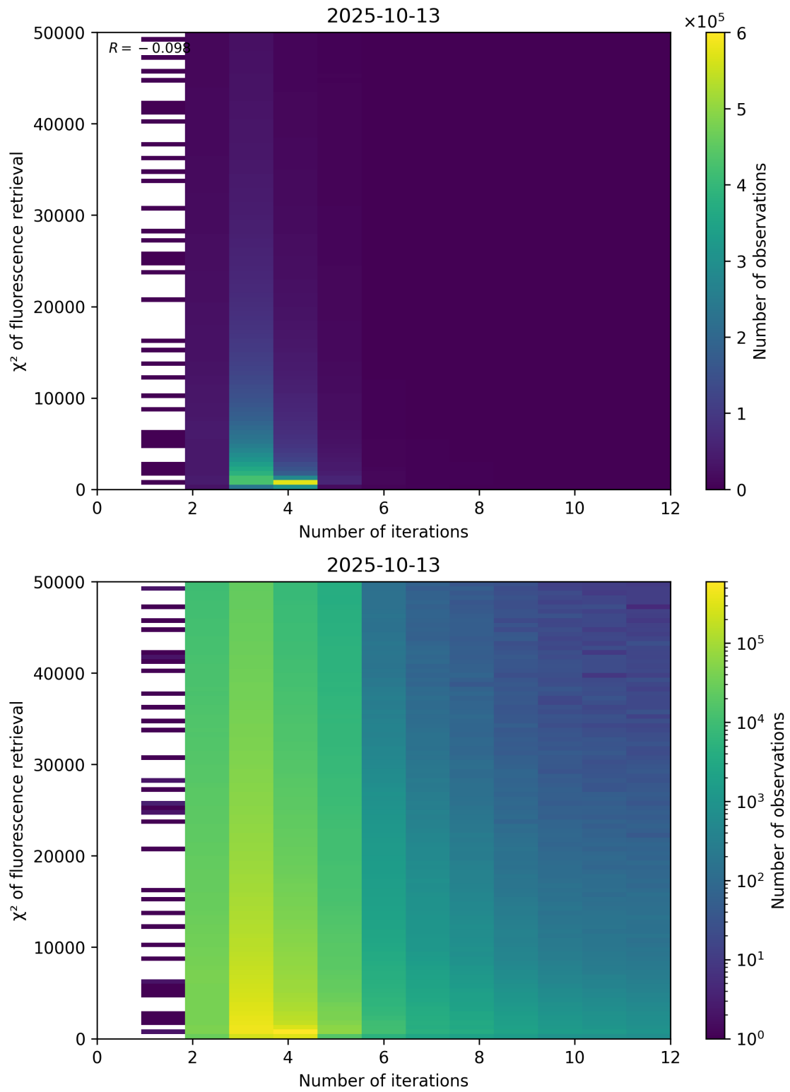
Figure 97: Scatter density plot of “Number of iterations” against “ \chi^2 of fluorescence retrieval” for 2025-10-12 to 2025-10-14.
