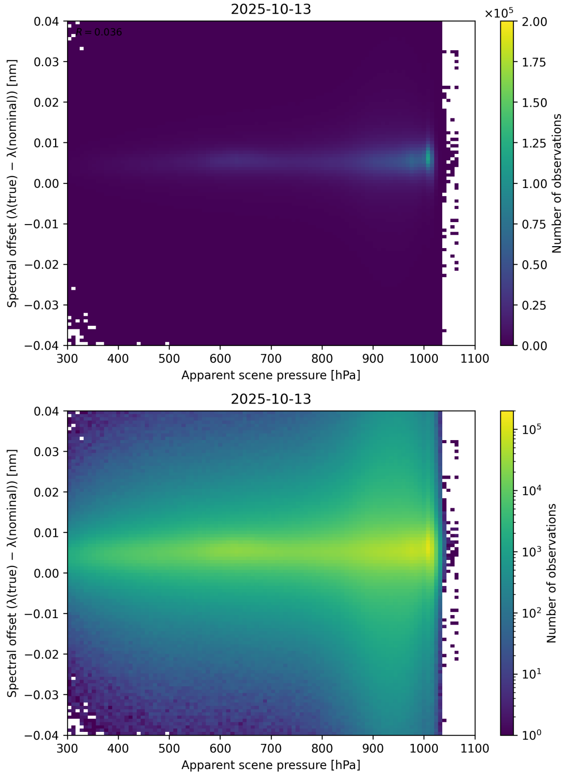
Figure 67: Scatter density plot of “Apparent scene pressure” against “Spectral offset ( \lambda_{\text{true}} - \lambda_{\text{nominal}} )” for 2025-10-12 to 2025-10-14.
