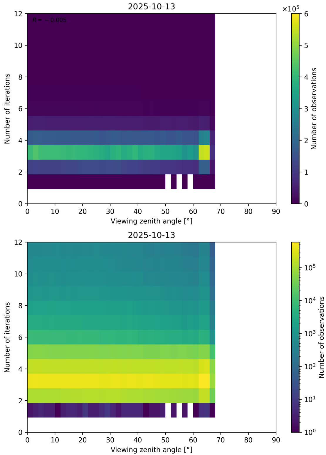
Figure 124: Scatter density plot of “Viewing zenith angle” against “Number of iterations” for 2025-10-12 to 2025-10-14.
