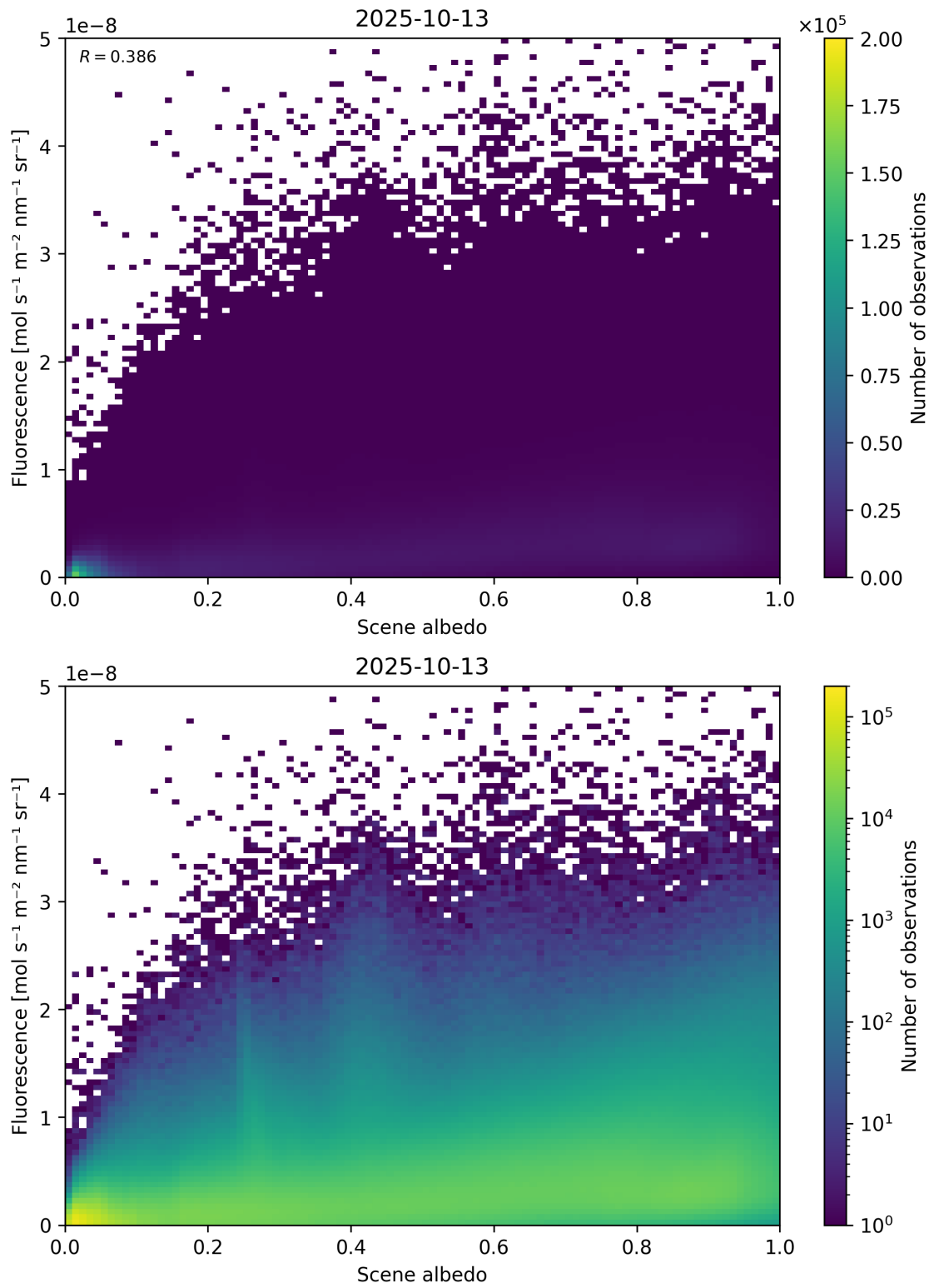
Figure 104: Scatter density plot of “Scene albedo” against “Fluorescence” for 2025-10-12 to 2025-10-14.
