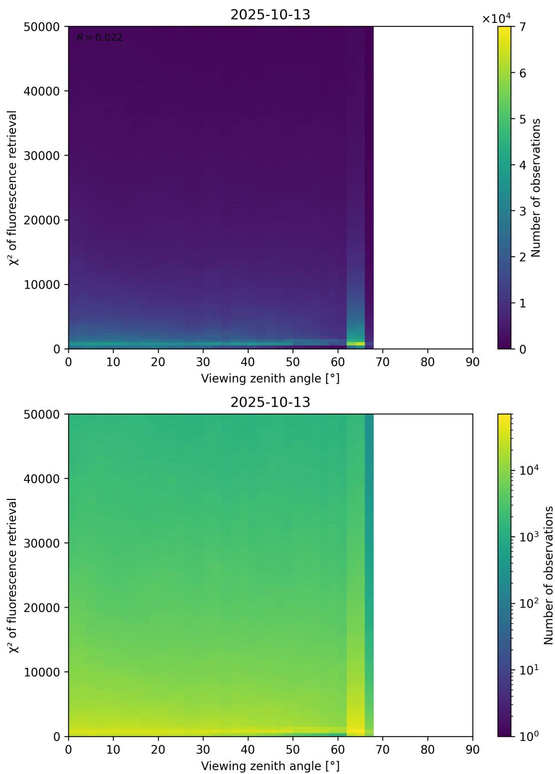
Figure 119: Scatter density plot of “Viewing zenith angle” against “ \chi^2 of fluorescence retrieval” for 2025-10-12 to 2025-10-14.
