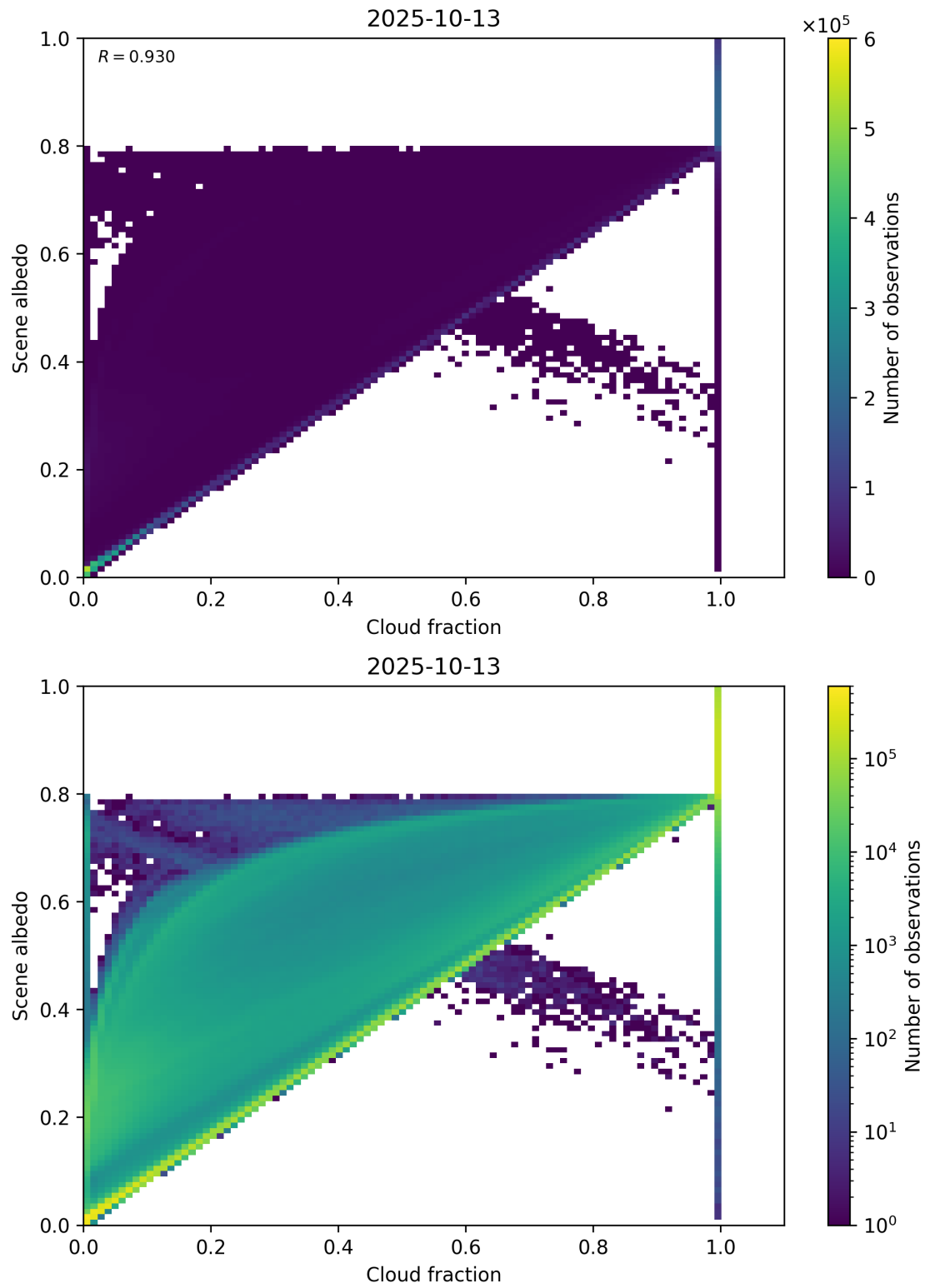
Figure 75: Scatter density plot of “Cloud fraction” against “Scene albedo” for 2025-10-12 to 2025-10-14.
