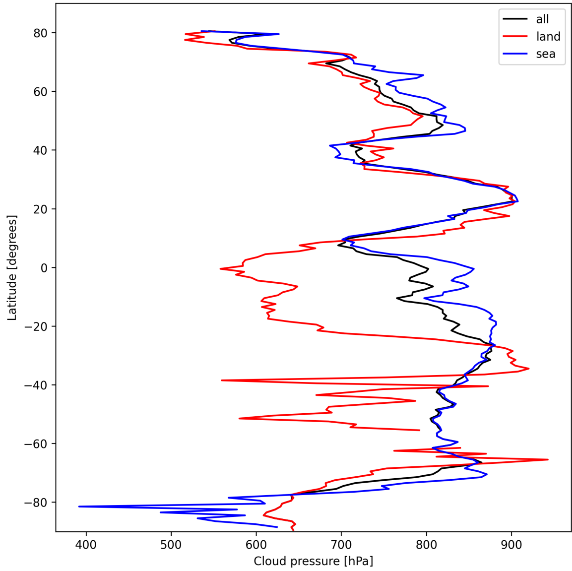
Figure 13: Zonal average of “Cloud pressure” for 2025-10-12 to 2025-10-14.
