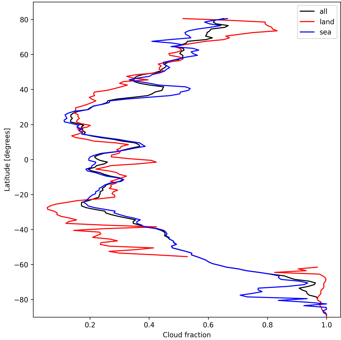
Figure 15: Zonal average of “Cloud fraction” for 2025-10-12 to 2025-10-14.
