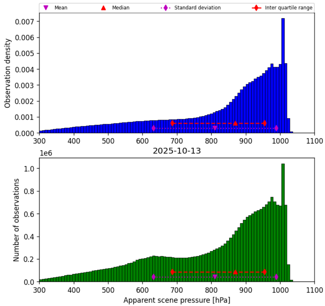
Figure 36: Histogram of “Apparent scene pressure” for 2025-10-12 to 2025-10-14
