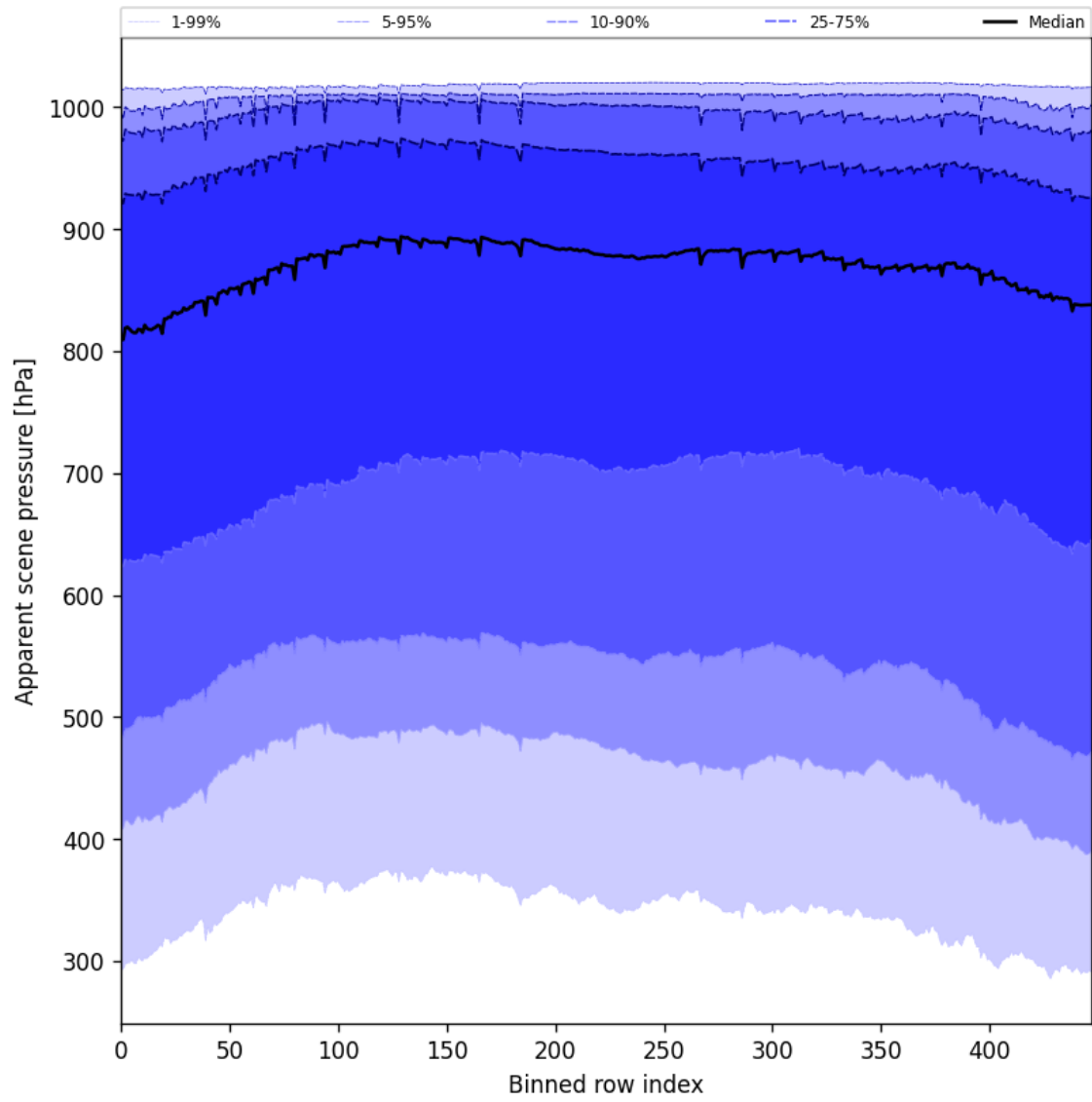
Figure 53: Along track statistics of “Apparent scene pressure” for 2025-10-12 to 2025-10-14
