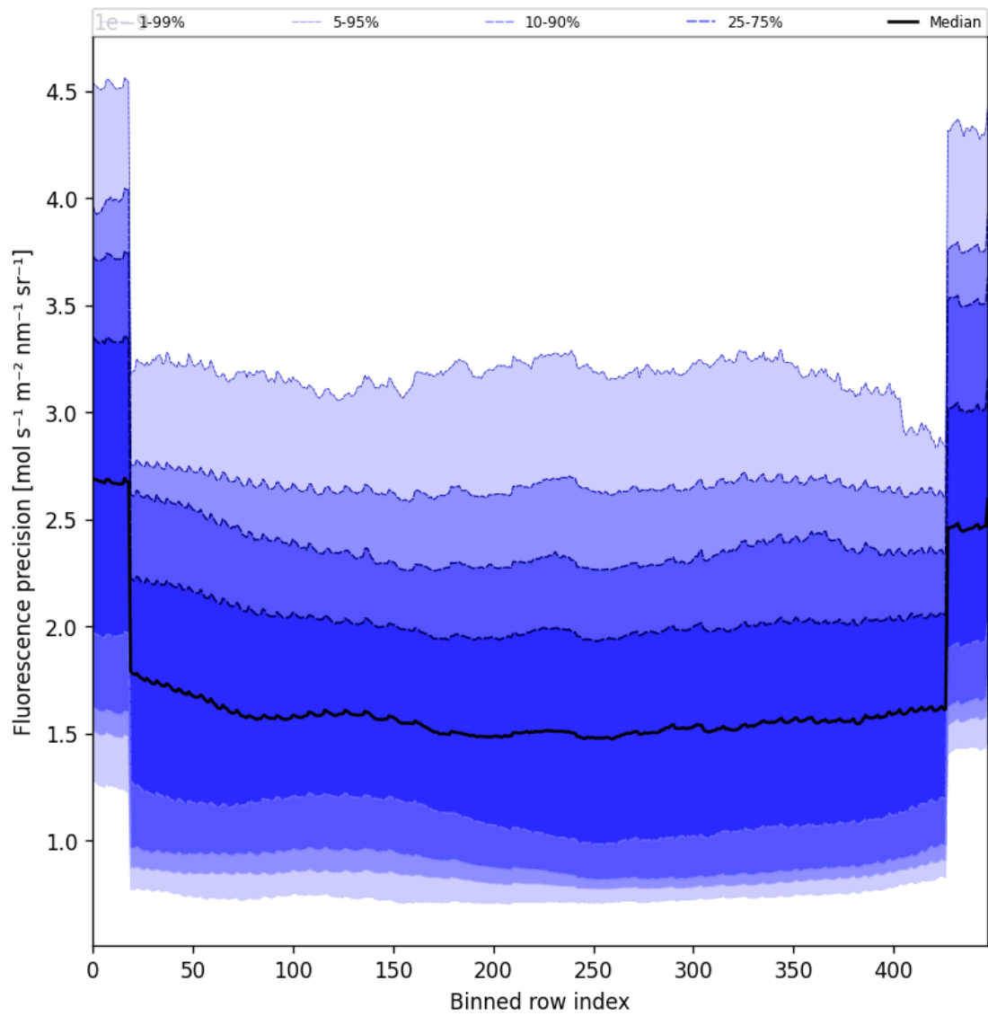
Figure 58: Along track statistics of “Fluorescence precision” for 2025-10-12 to 2025-10-14
