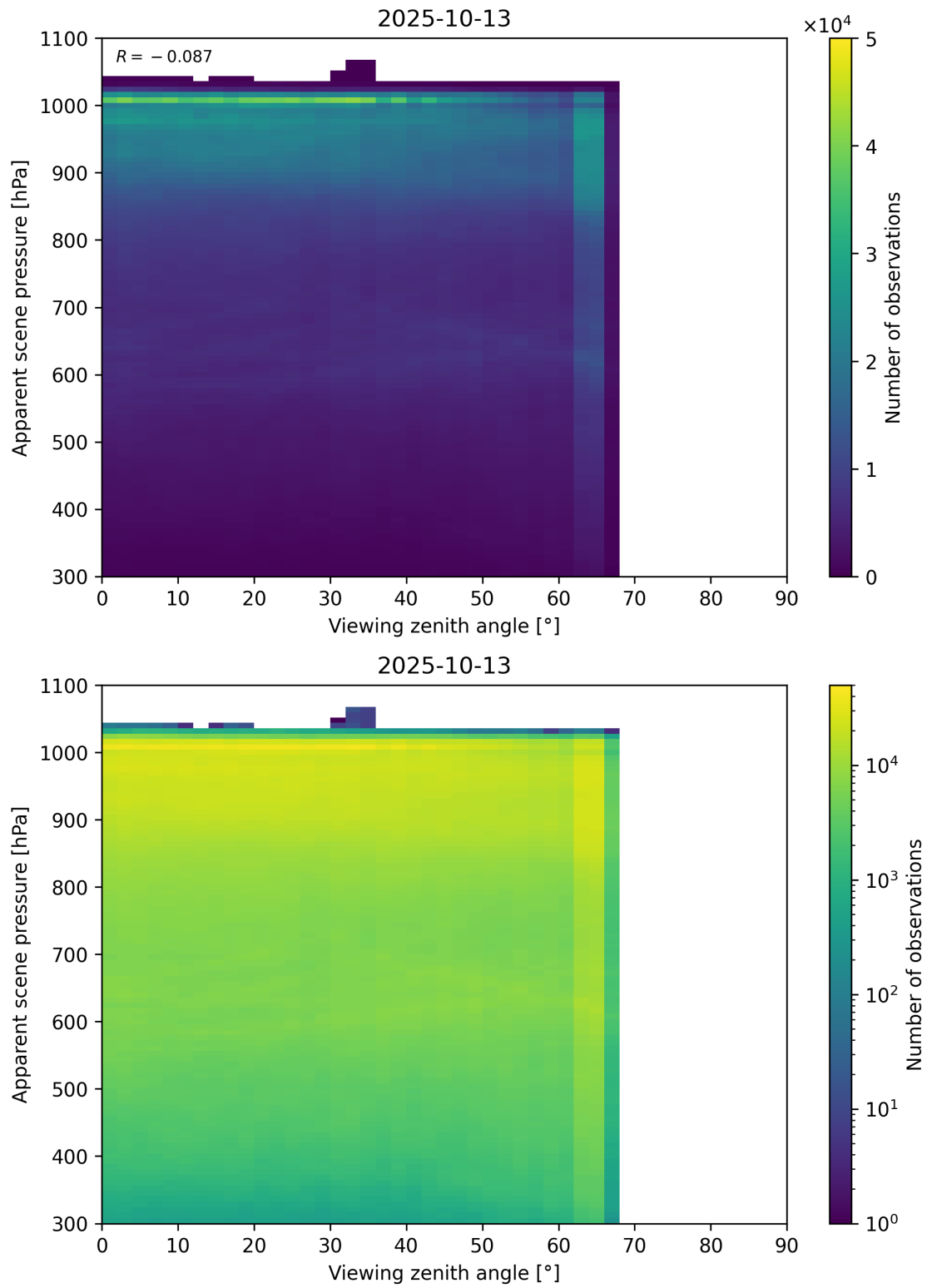
Figure 118: Scatter density plot of “Viewing zenith angle” against “Apparent scene pressure” for 2025-10-12 to 2025-10-14.
