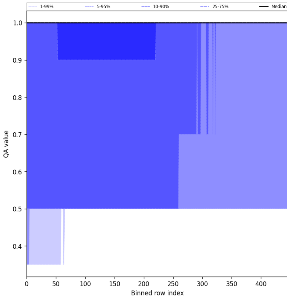
Figure 46: Along track statistics of “QA value” for 2025-10-12 to 2025-10-14
