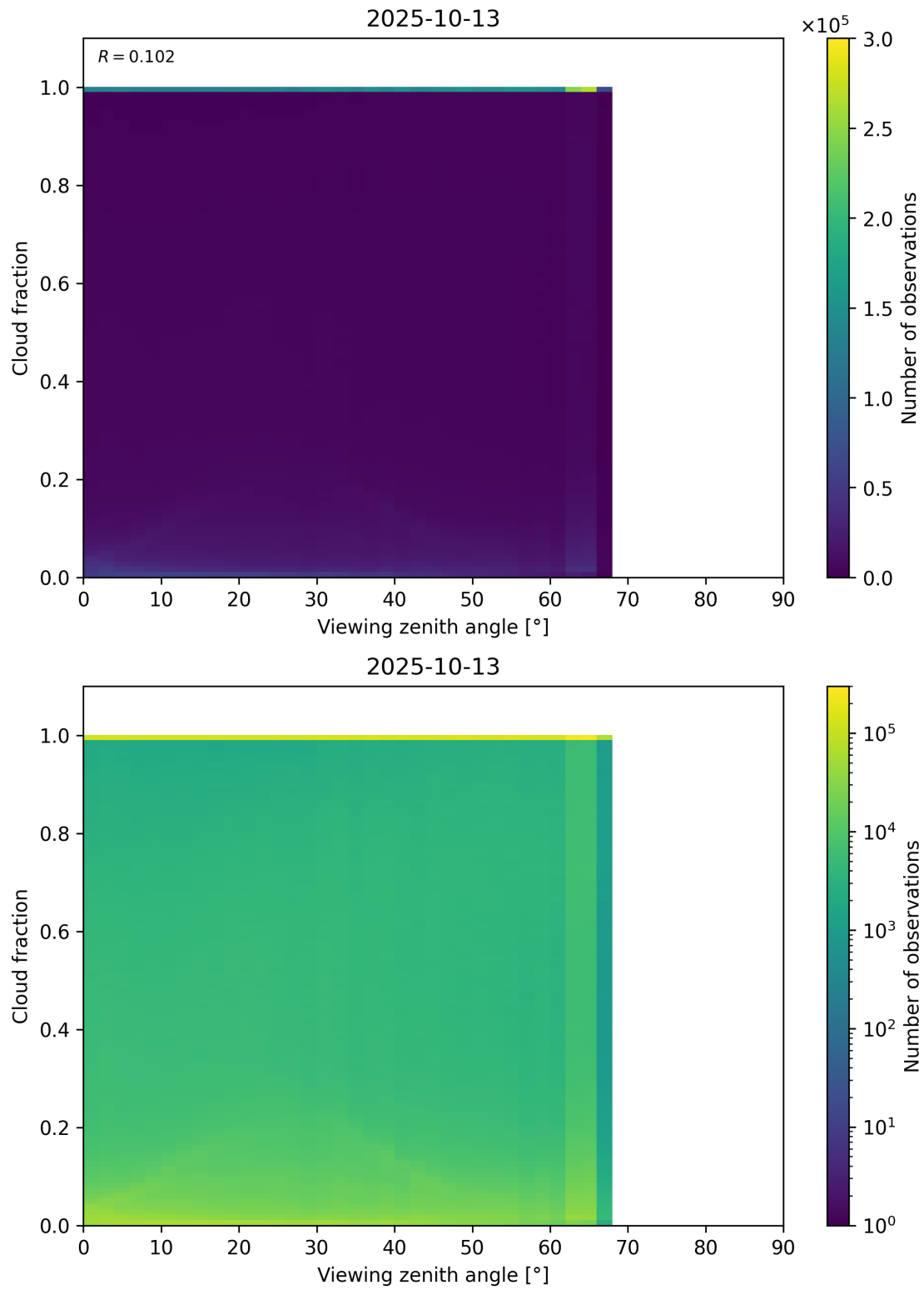
Figure 120: Scatter density plot of “Viewing zenith angle” against “Cloud fraction” for 2025-10-12 to 2025-10-14.
