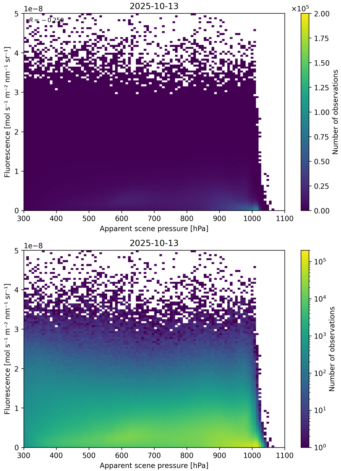
Figure 64: Scatter density plot of “Apparent scene pressure” against “Fluorescence” for 2025-10-12 to 2025-10-14.
