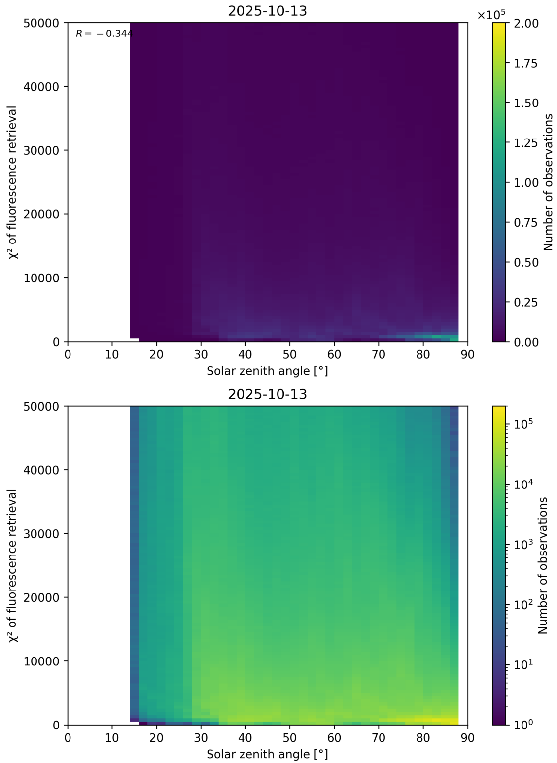
Figure 109: Scatter density plot of “Solar zenith angle” against “ \chi^2 of fluorescence retrieval” for 2025-10-12 to 2025-10-14.
