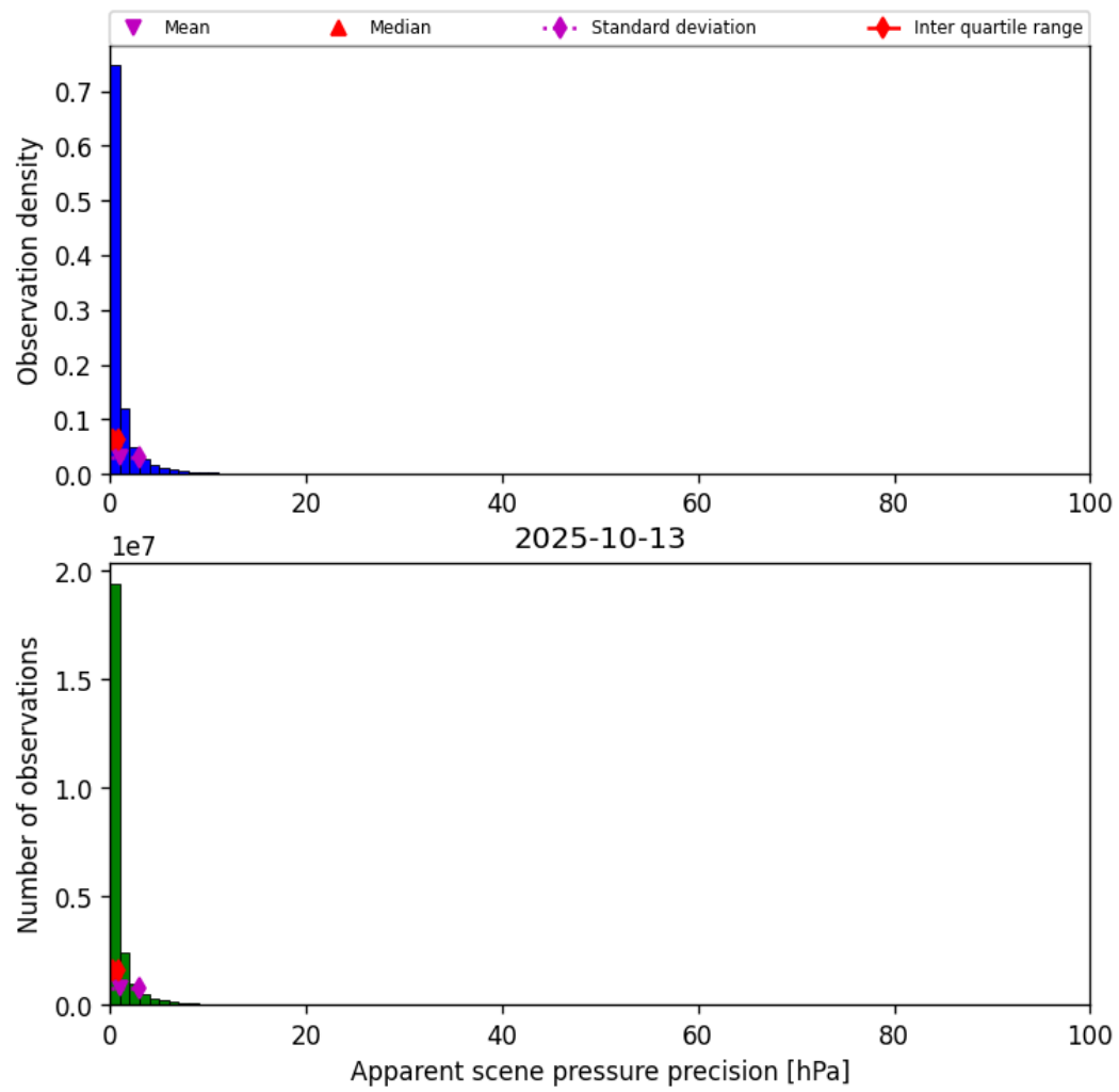
Figure 37: Histogram of “Apparent scene pressure precision” for 2025-10-12 to 2025-10-14
