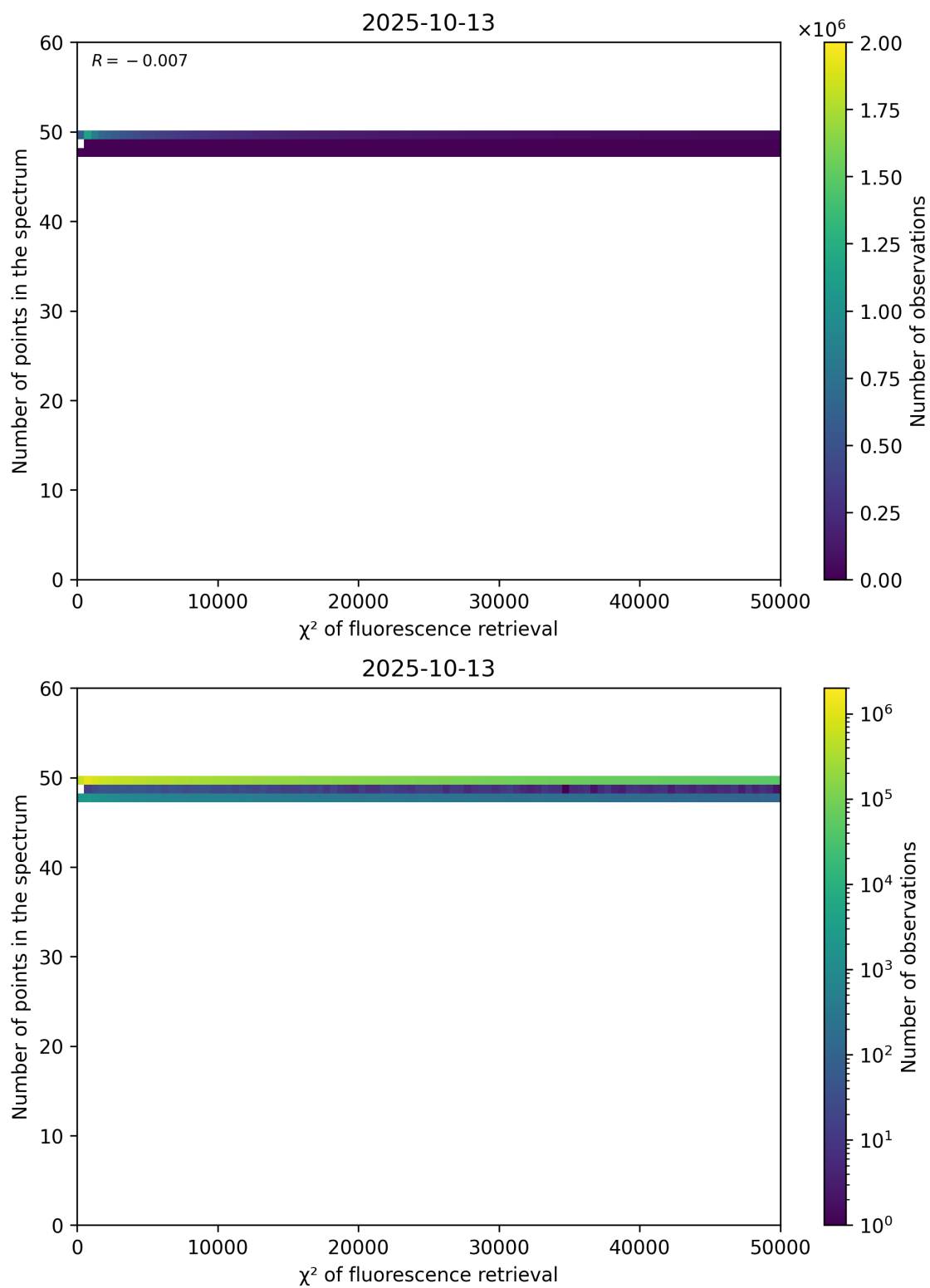
Figure 68: Scatter density plot of “ \chi^2 of fluorescence retrieval” against “Number of points in the spectrum” for 2025-10-12 to 2025-10-14.
