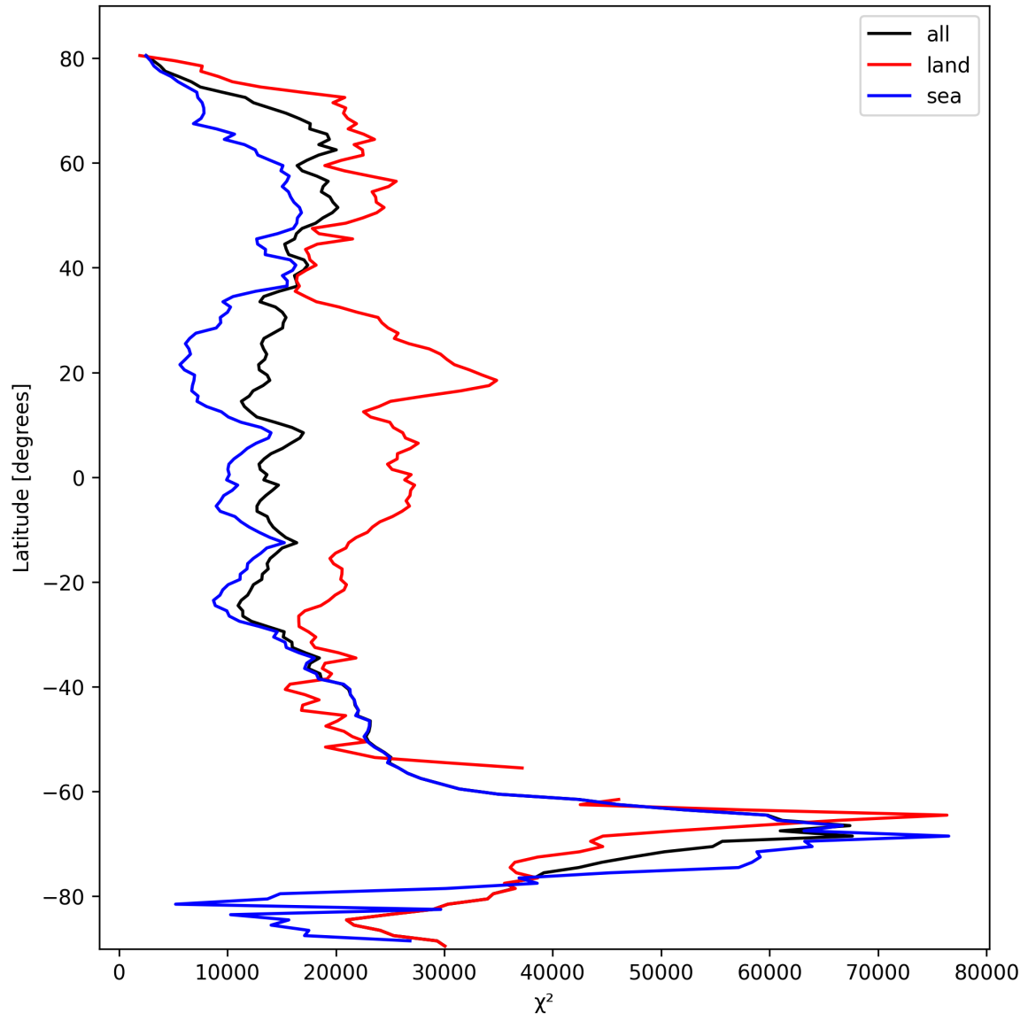
Figure 21: Zonal average of “ \chi^2 ” for 2025-10-12 to 2025-10-14.
