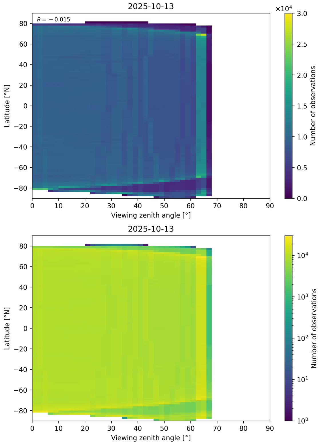
Figure 123: Scatter density plot of “Viewing zenith angle” against “Latitude” for 2025-10-12 to 2025-10-14.
