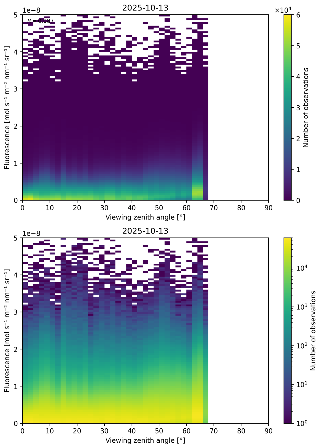
Figure 122: Scatter density plot of “Viewing zenith angle” against “Fluorescence” for 2025-10-12 to 2025-10-14.
