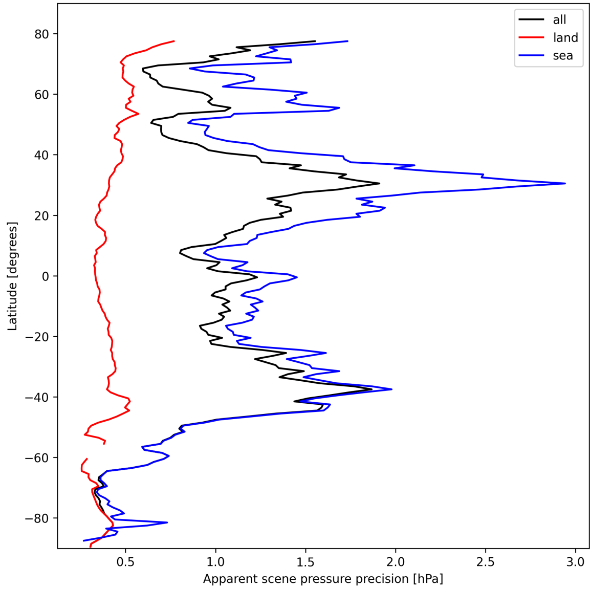
Figure 20: Zonal average of “Apparent scene pressure precision” for 2025-10-18 to 2025-10-20.
