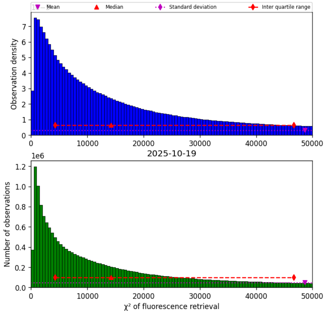
Figure 42: Histogram of “ \chi^2 of fluorescence retrieval” for 2025-10-18 to 2025-10-20
