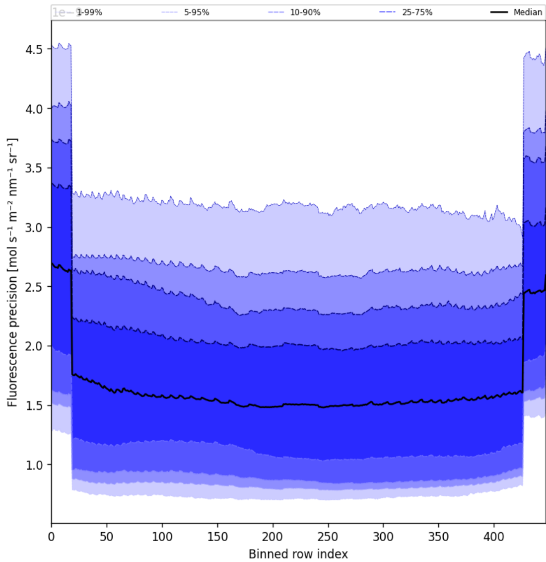
Figure 58: Along track statistics of “Fluorescence precision” for 2025-10-18 to 2025-10-20
