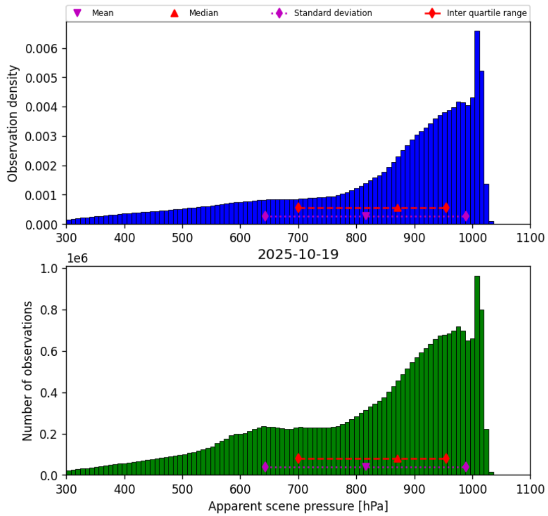
Figure 36: Histogram of “Apparent scene pressure” for 2025-10-18 to 2025-10-20
