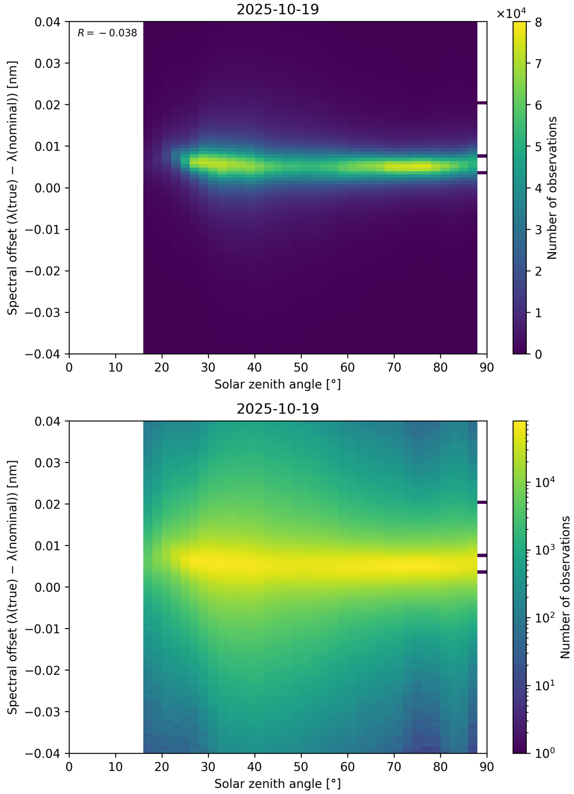
Figure 117: Scatter density plot of “Solar zenith angle” against “Spectral offset ( \lambda_{\text{true}} - \lambda_{\text{nominal}} )” for 2025-10-18 to 2025-10-20.
