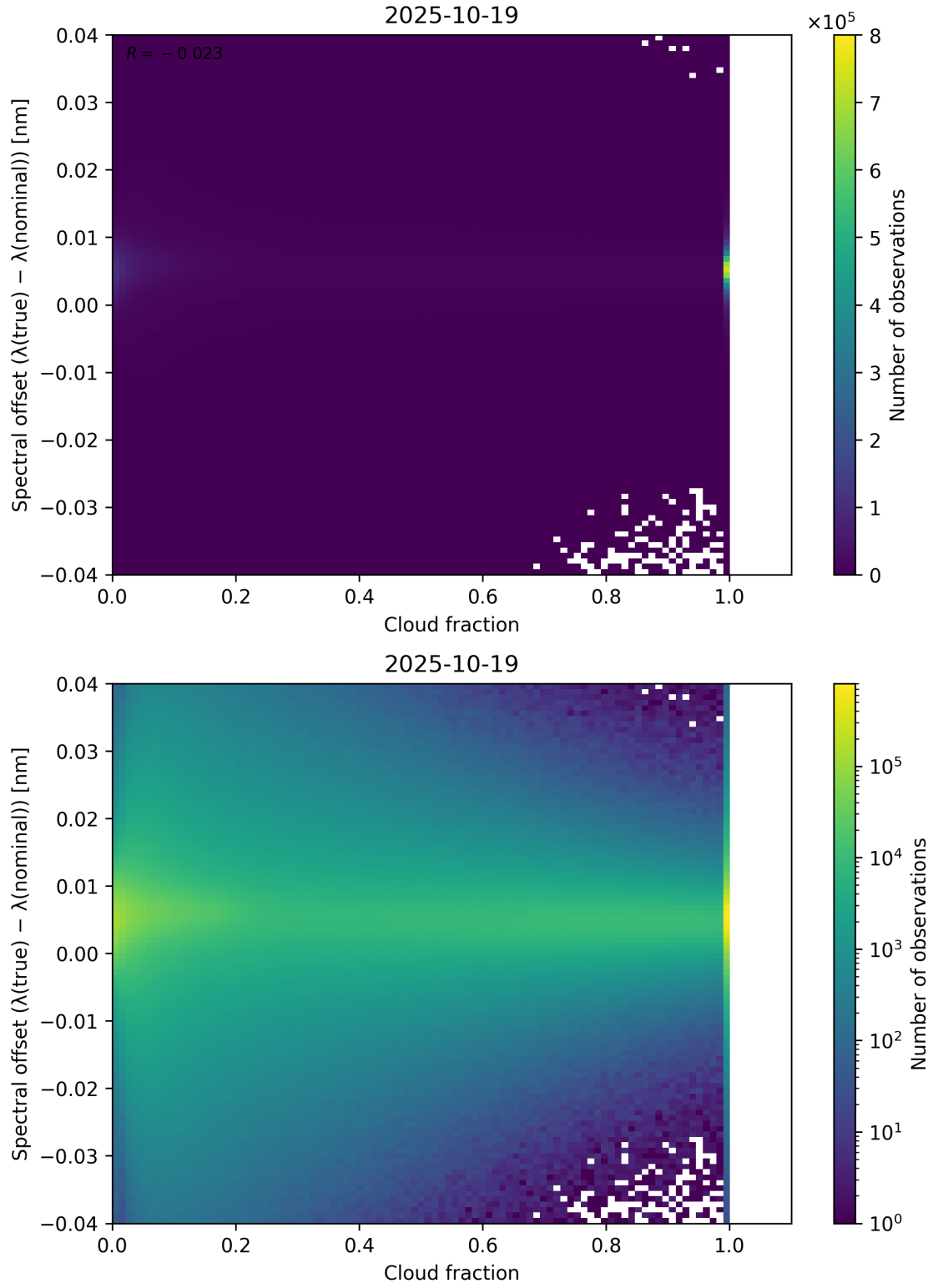
Figure 76: Scatter density plot of “Cloud fraction” against “Spectral offset ( \lambda_{\text{true}} - \lambda_{\text{nominal}} )” for 2025-10-18 to 2025-10-20.
