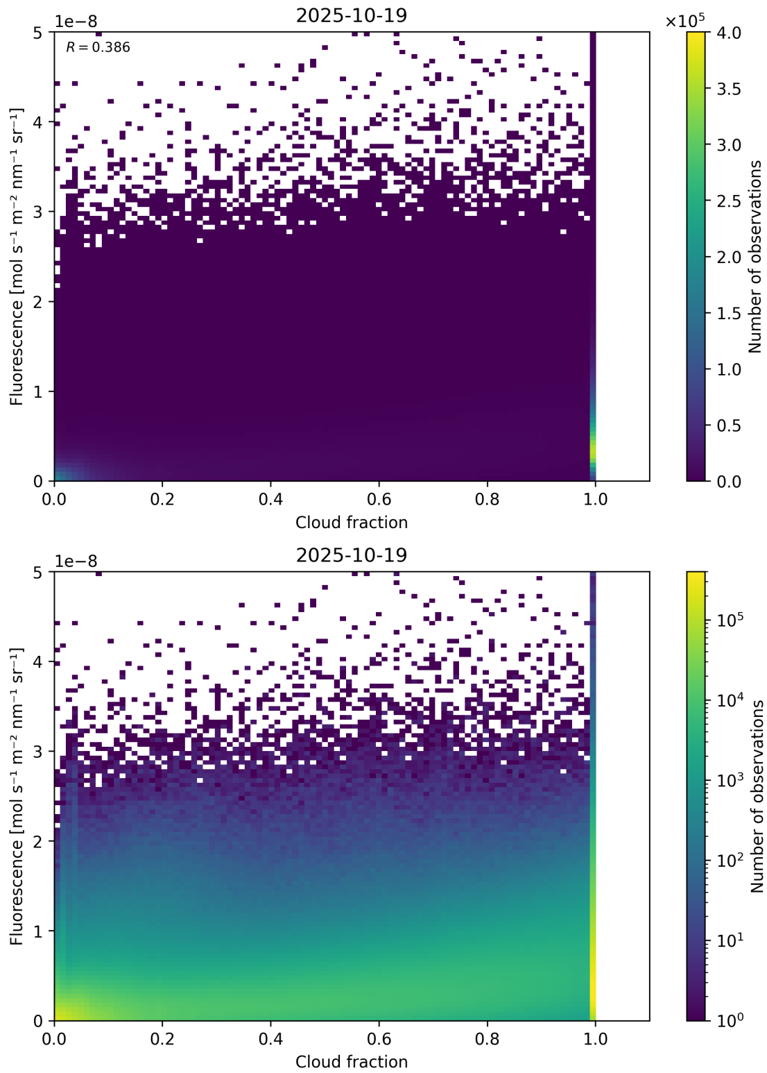
Figure 72: Scatter density plot of “Cloud fraction” against “Fluorescence” for 2025-10-18 to 2025-10-20.
