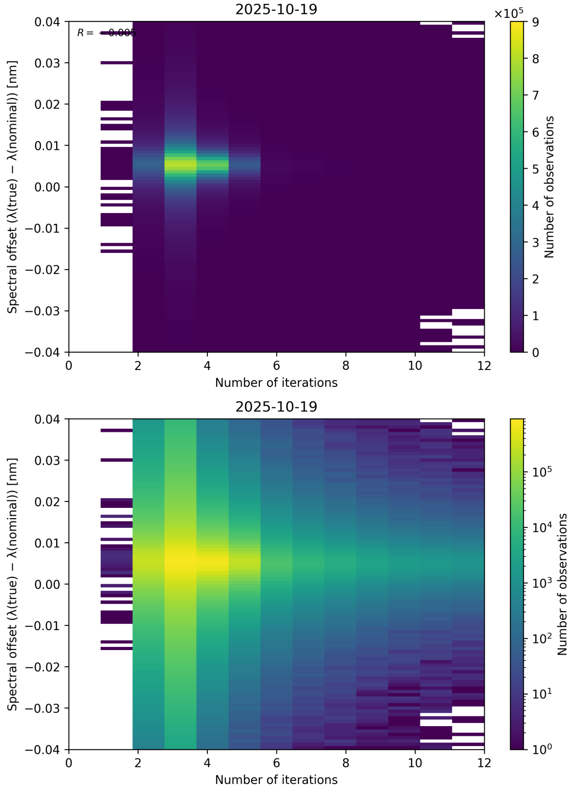
Figure 100: Scatter density plot of “Number of iterations” against “Spectral offset ( \lambda_{\text{true}} - \lambda_{\text{nominal}} )” for 2025-10-18 to 2025-10-20.
