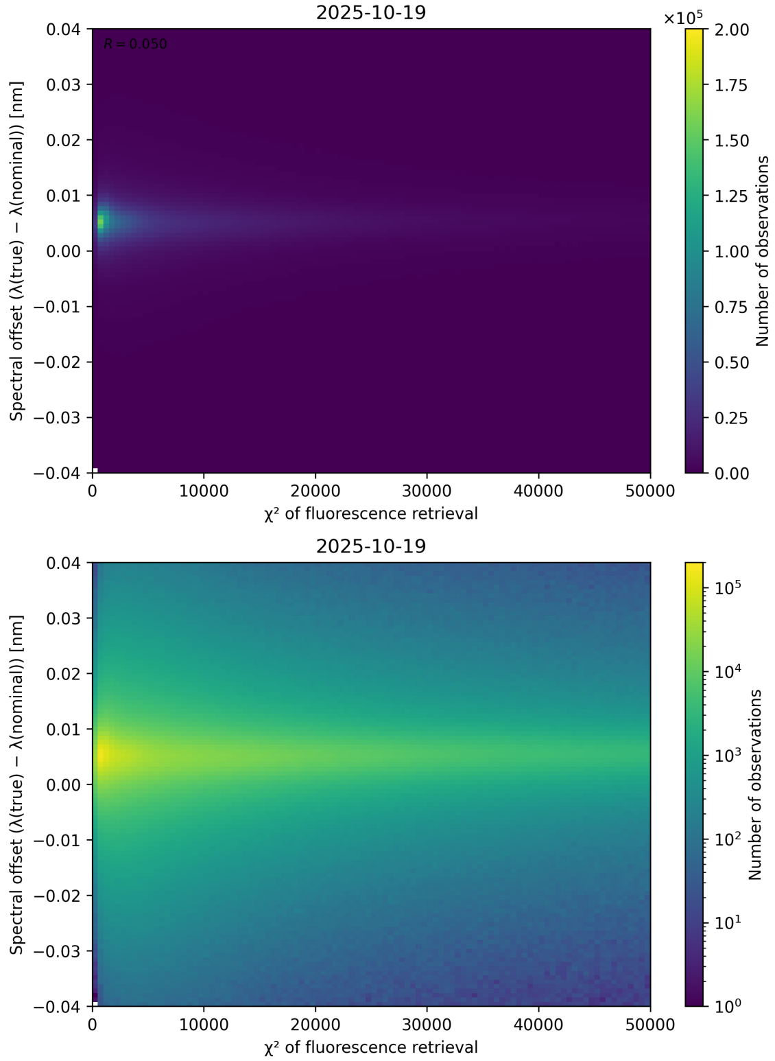
Figure 69: Scatter density plot of “ \chi^2 of fluorescence retrieval” against “Spectral offset ( \lambda_{\text{true}} - \lambda_{\text{nominal}} )” for 2025-10-18 to 2025-10-20.
