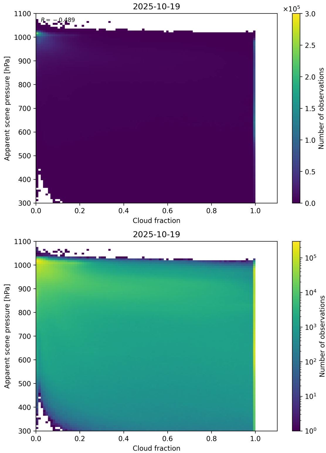
Figure 70: Scatter density plot of “Cloud fraction” against “Apparent scene pressure” for 2025-10-18 to 2025-10-20.
