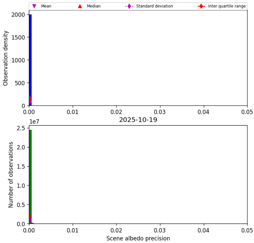
Figure 35: Histogram of “Scene albedo precision” for 2025-10-18 to 2025-10-20
