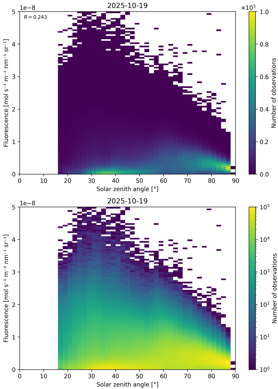
Figure 112: Scatter density plot of “Solar zenith angle” against “Fluorescence” for 2025-10-18 to 2025-10-20.
