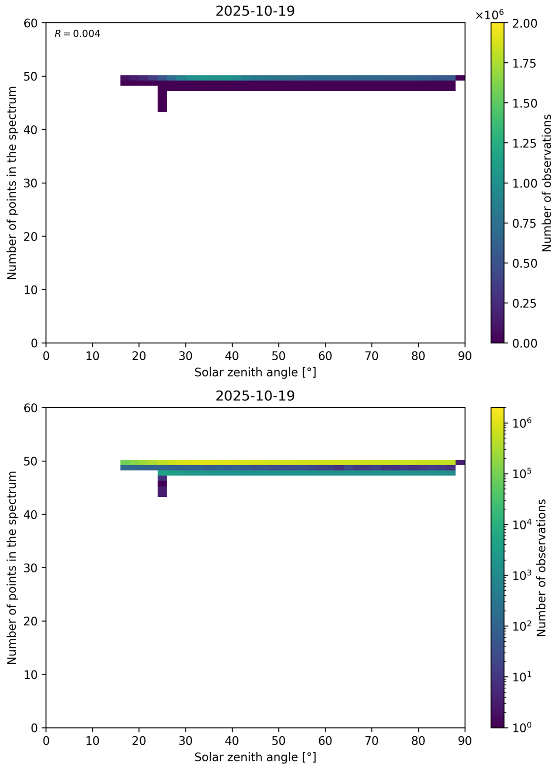
Figure 115: Scatter density plot of “Solar zenith angle” against “Number of points in the spectrum” for 2025-10-18 to 2025-10-20.
