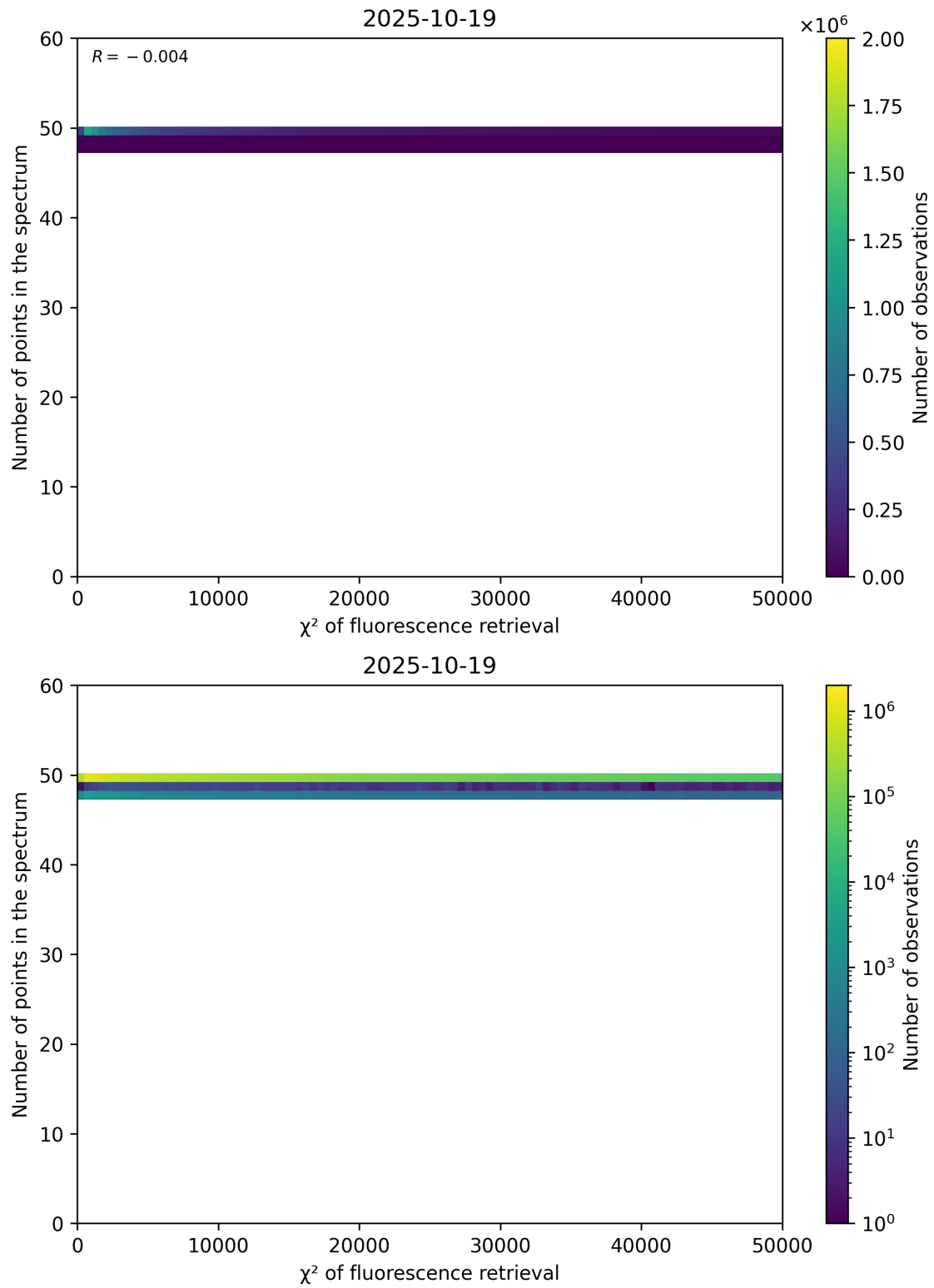
Figure 68: Scatter density plot of " \chi^2 of fluorescence retrieval" against "Number of points in the spectrum" for 2025-10-18 to 2025-10-20.
