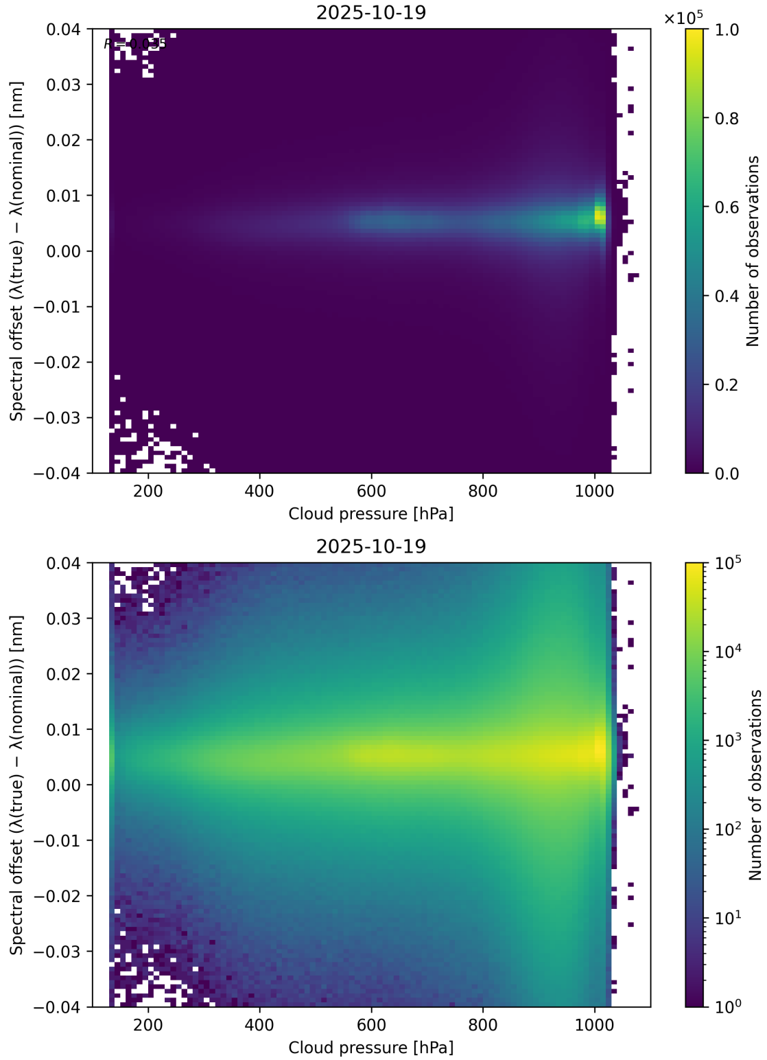
Figure 84: Scatter density plot of “Cloud pressure” against “Spectral offset ( \lambda_{\text{true}} - \lambda_{\text{nominal}} )” for 2025-10-18 to 2025-10-20.
