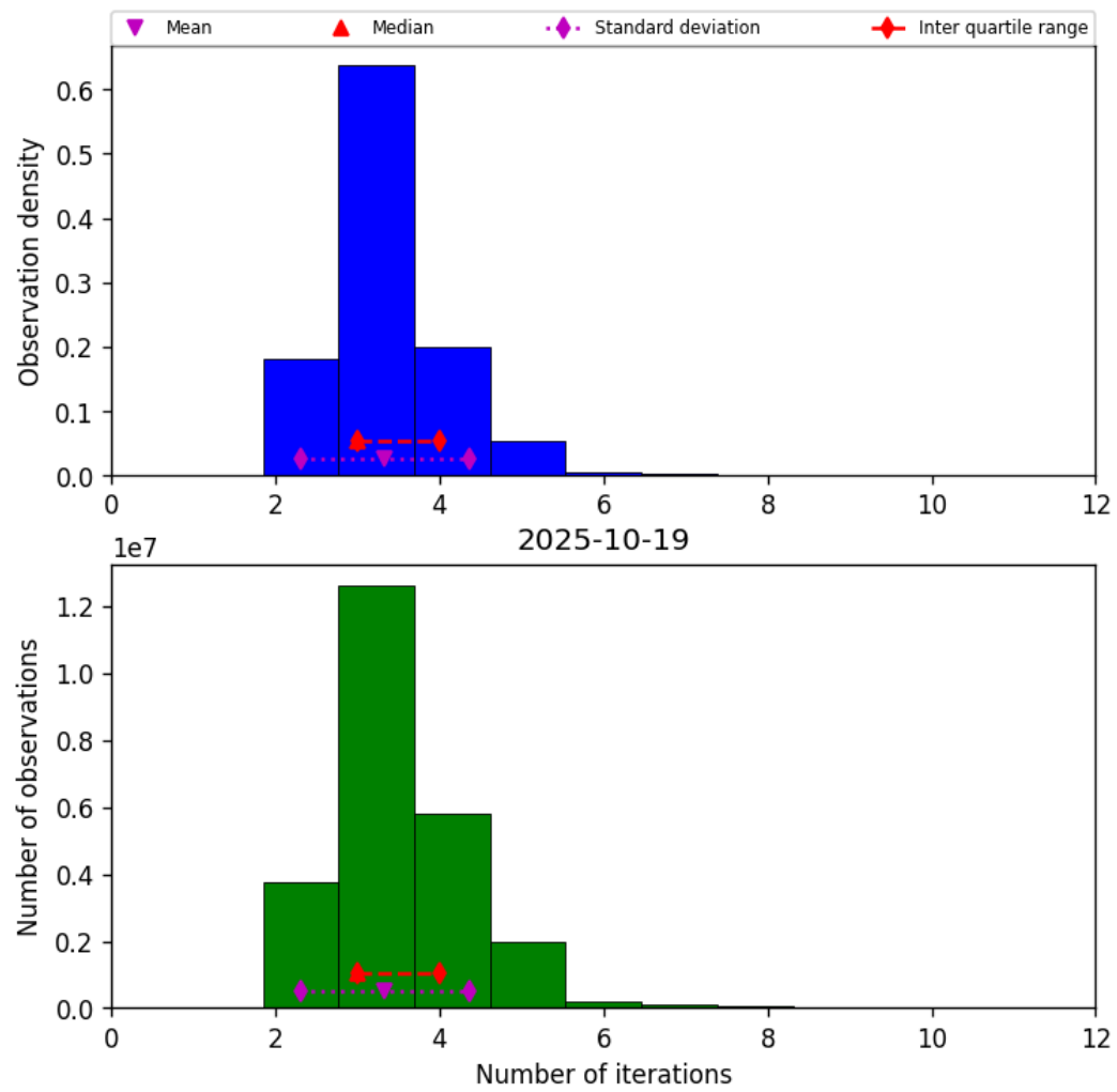
Figure 39: Histogram of “Number of iterations” for 2025-10-18 to 2025-10-20
