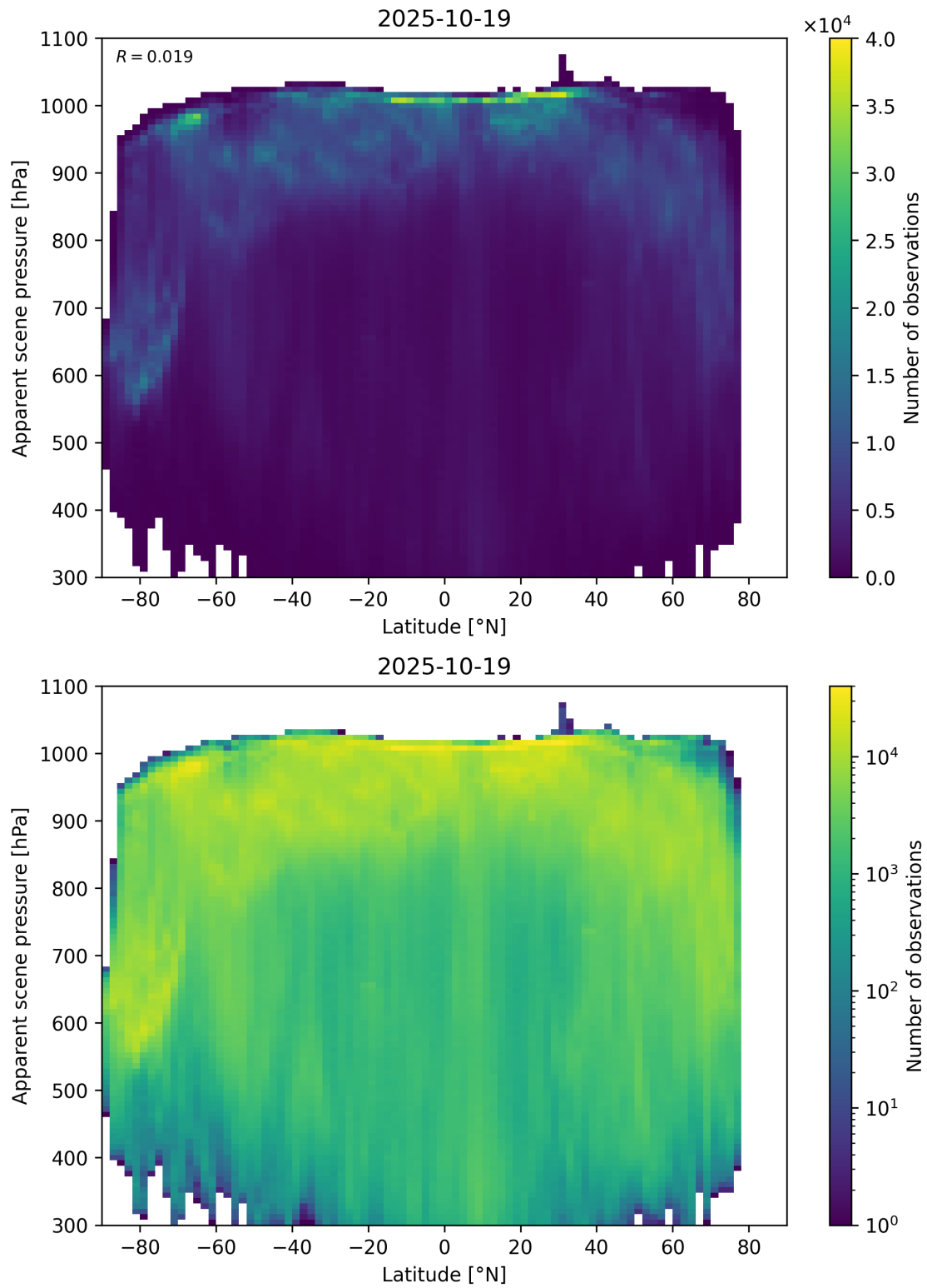
Figure 88: Scatter density plot of “Latitude” against “Apparent scene pressure” for 2025-10-18 to 2025-10-20.
