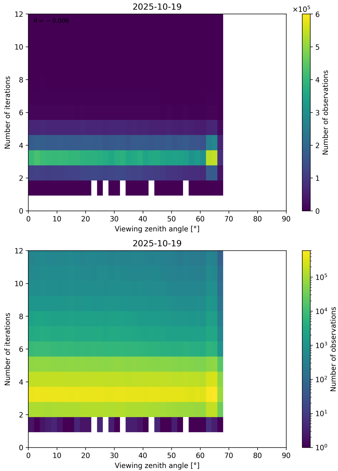
Figure 124: Scatter density plot of “Viewing zenith angle” against “Number of iterations” for 2025-10-18 to 2025-10-20.
