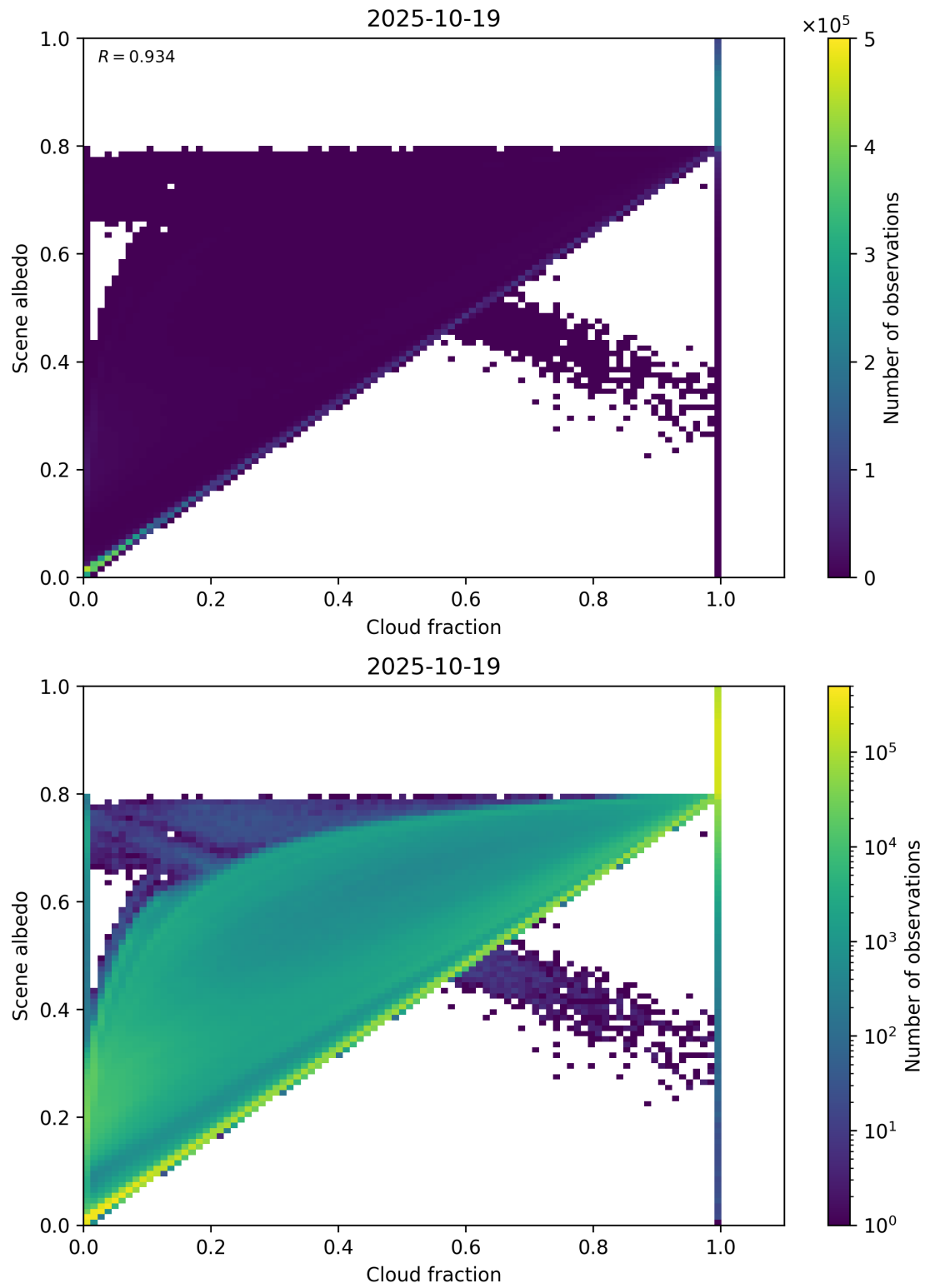
Figure 75: Scatter density plot of “Cloud fraction” against “Scene albedo” for 2025-10-18 to 2025-10-20.
