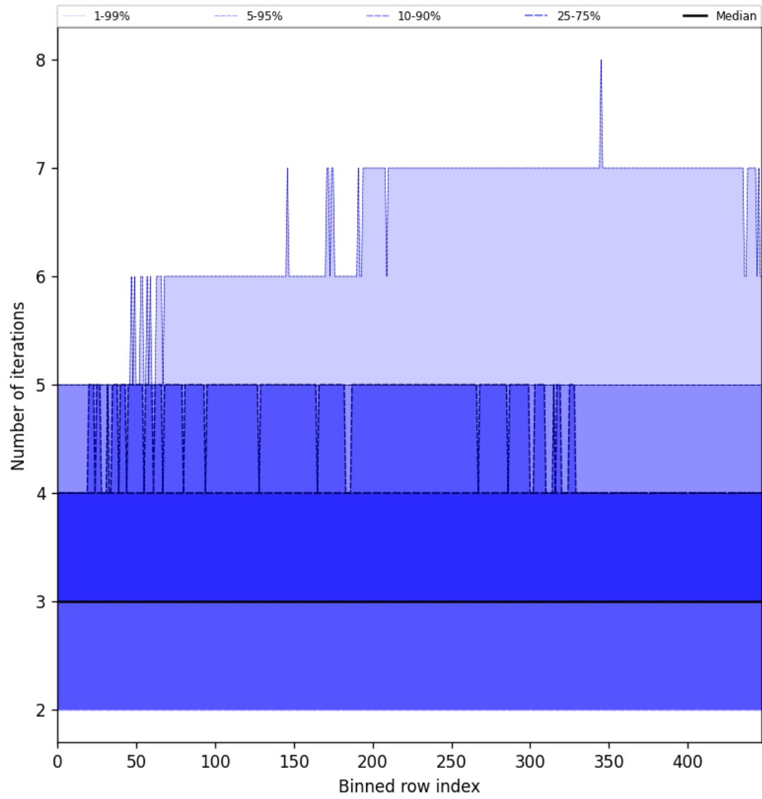
Figure 56: Along track statistics of “Number of iterations” for 2025-10-18 to 2025-10-20
