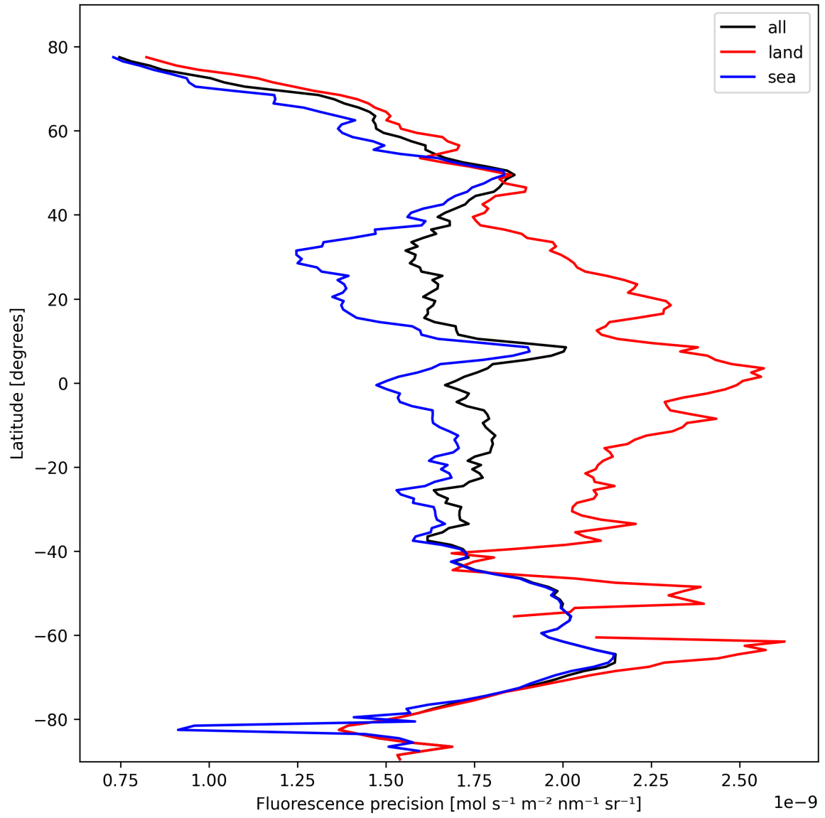
Figure 24: Zonal average of “Fluorescence precision” for 2025-10-18 to 2025-10-20.
