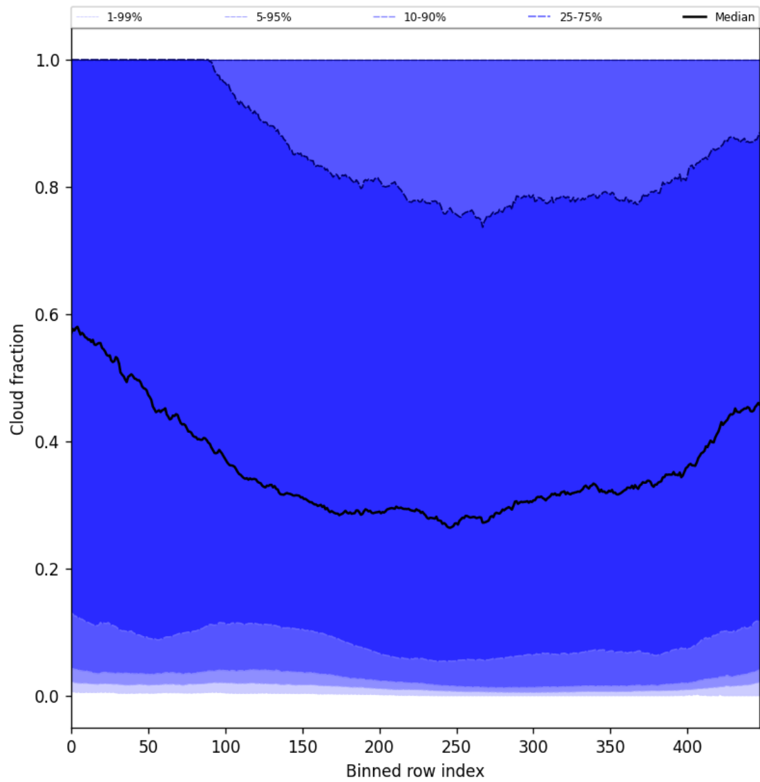
Figure 49: Along track statistics of “Cloud fraction” for 2025-10-18 to 2025-10-20
