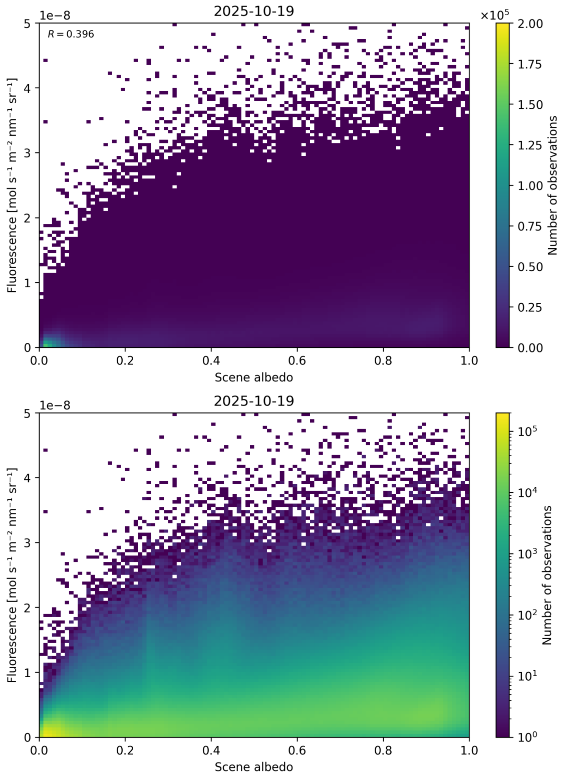
Figure 104: Scatter density plot of “Scene albedo” against “Fluorescence” for 2025-10-18 to 2025-10-20.
