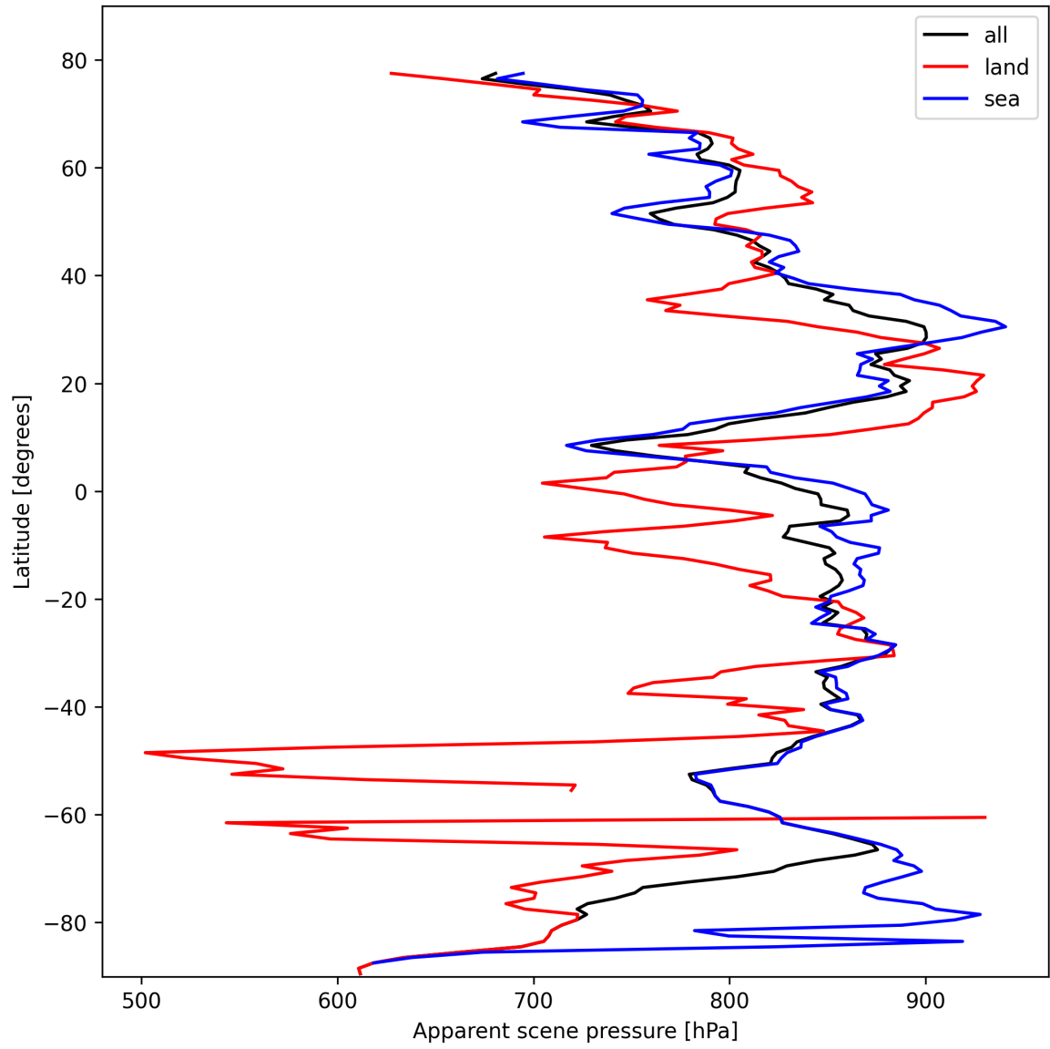
Figure 19: Zonal average of “Apparent scene pressure” for 2025-10-18 to 2025-10-20.
