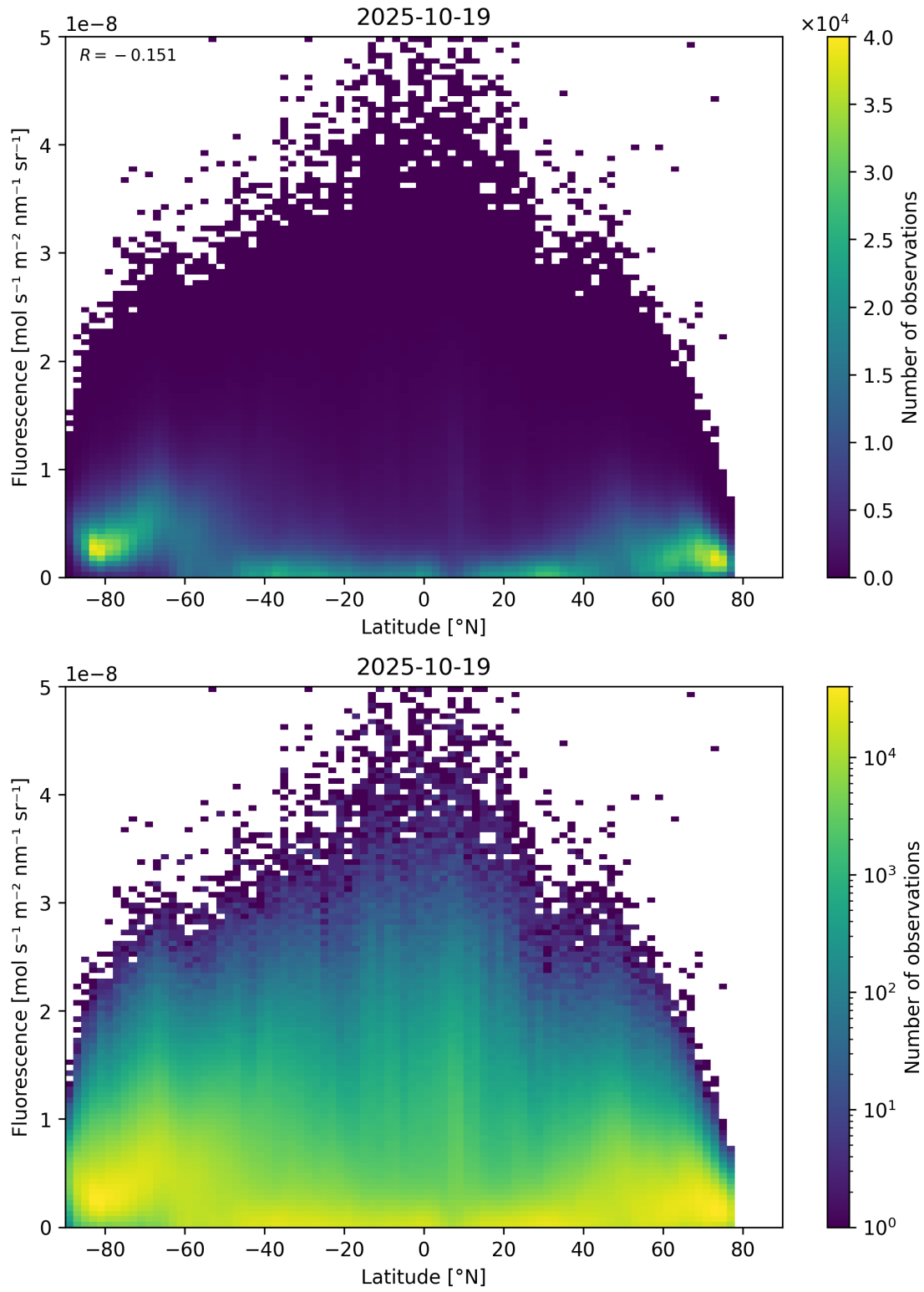
Figure 92: Scatter density plot of “Latitude” against “Fluorescence” for 2025-10-18 to 2025-10-20.
