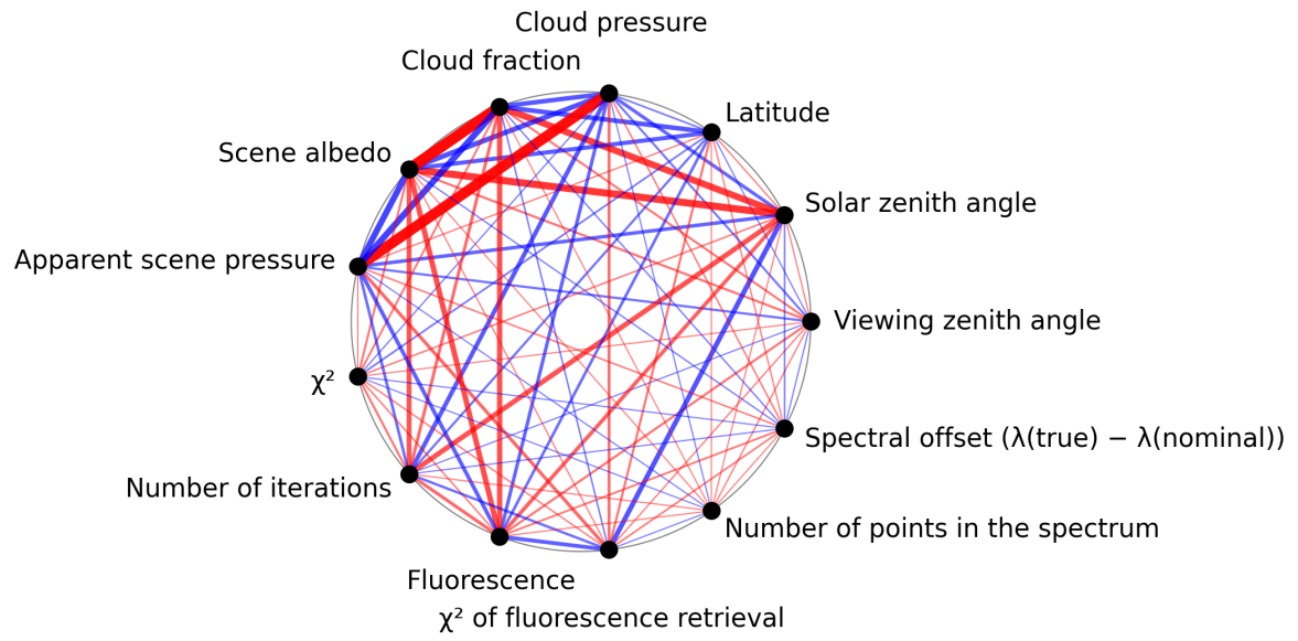
Figure 1: Map of correlation graph for 2025-10-18 to 2025-10-20.
