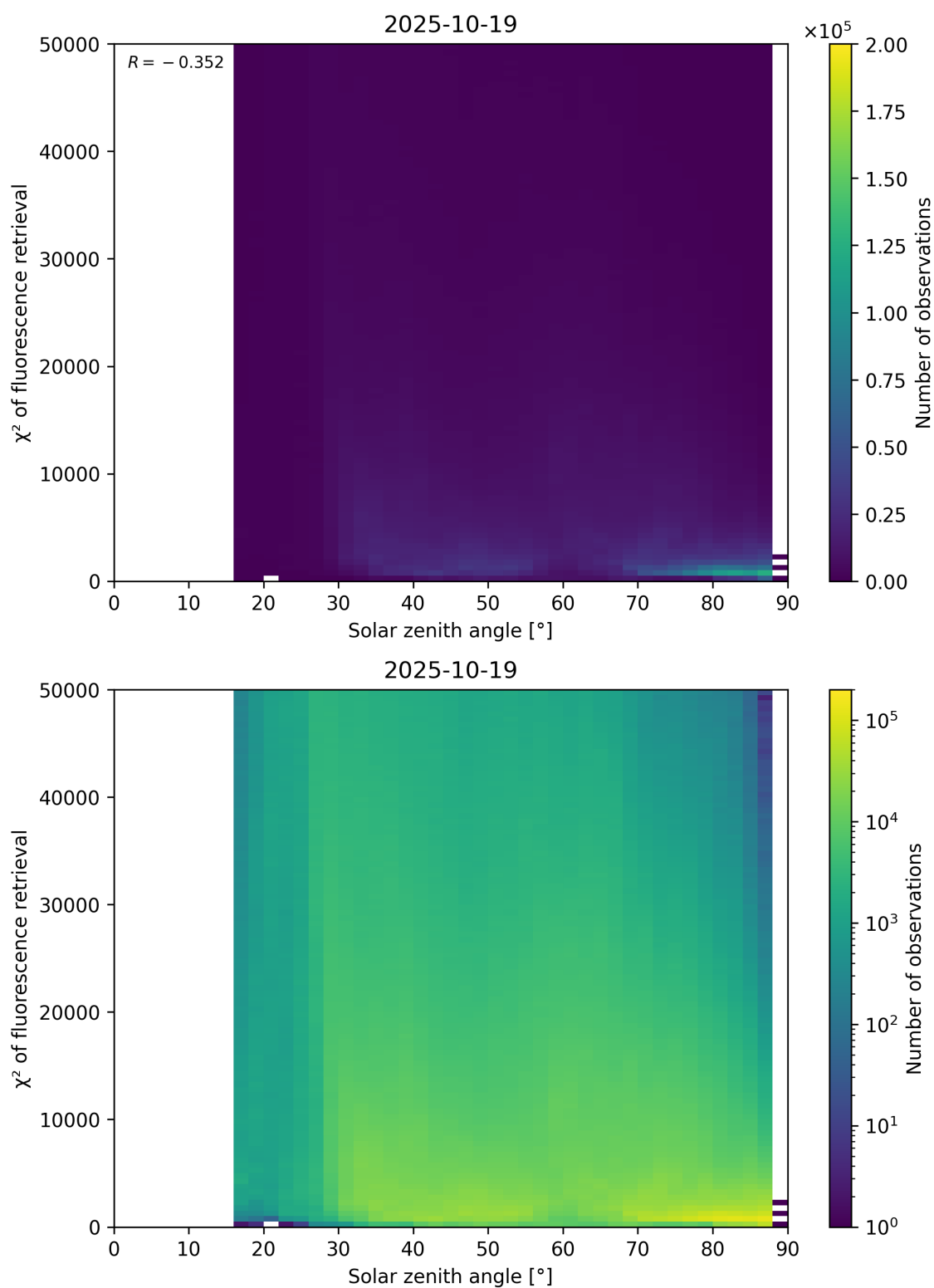
Figure 109: Scatter density plot of “Solar zenith angle” against “ \chi^2 of fluorescence retrieval” for 2025-10-18 to 2025-10-20.
