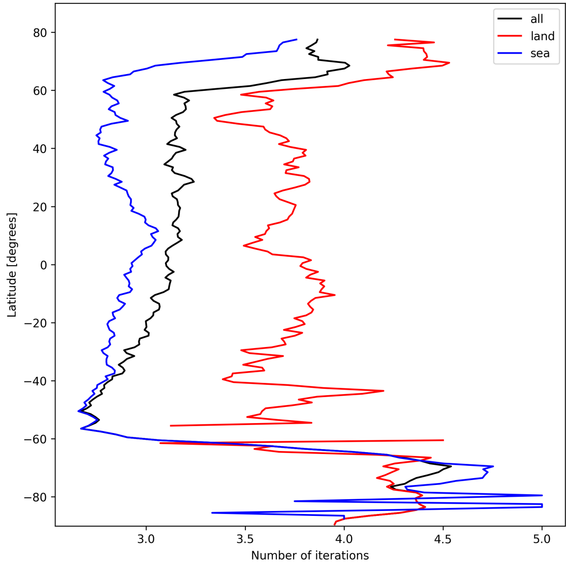
Figure 22: Zonal average of “Number of iterations” for 2025-10-18 to 2025-10-20.
