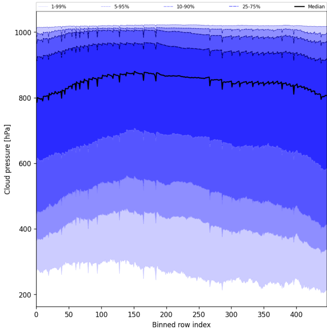
Figure 47: Along track statistics of “Cloud pressure” for 2025-10-18 to 2025-10-20
