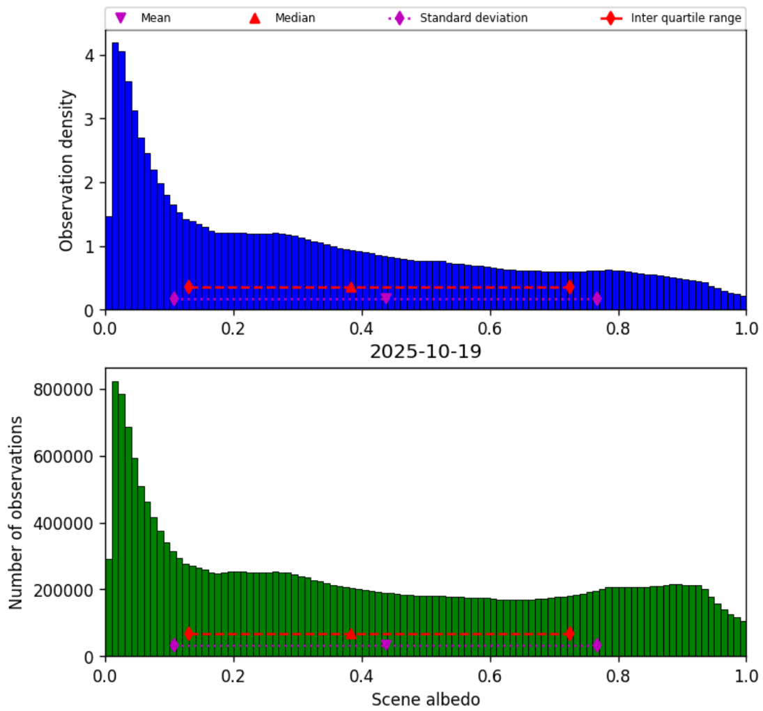
Figure 34: Histogram of “Scene albedo” for 2025-10-18 to 2025-10-20
