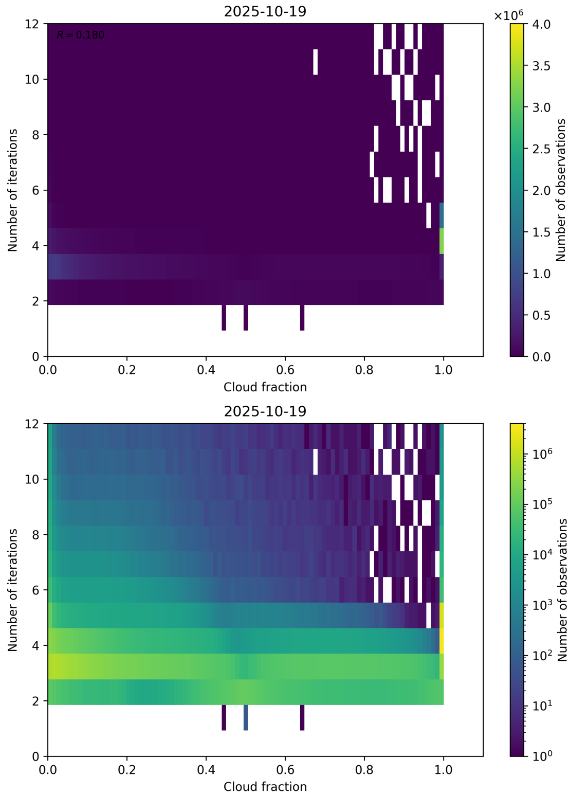
Figure 73: Scatter density plot of “Cloud fraction” against “Number of iterations” for 2025-10-18 to 2025-10-20.
