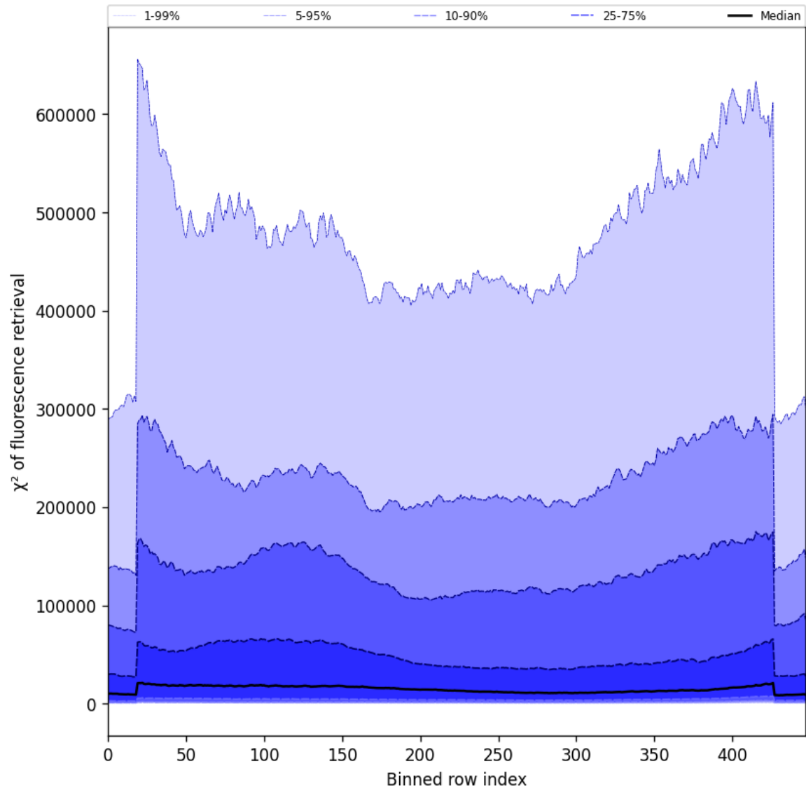
Figure 59: Along track statistics of " \chi^2 of fluorescence retrieval" for 2025-10-18 to 2025-10-20
