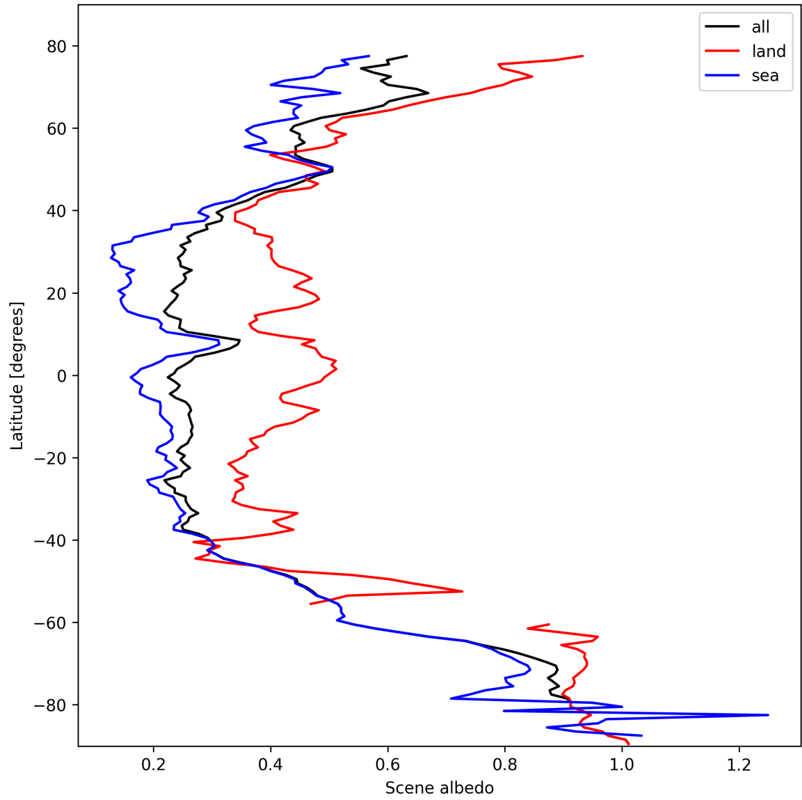
Figure 17: Zonal average of “Scene albedo” for 2025-10-18 to 2025-10-20.
