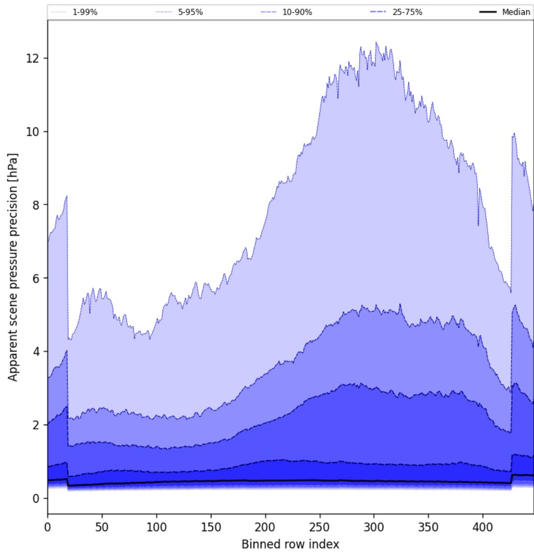
Figure 54: Along track statistics of “Apparent scene pressure precision” for 2025-10-18 to 2025-10-20
