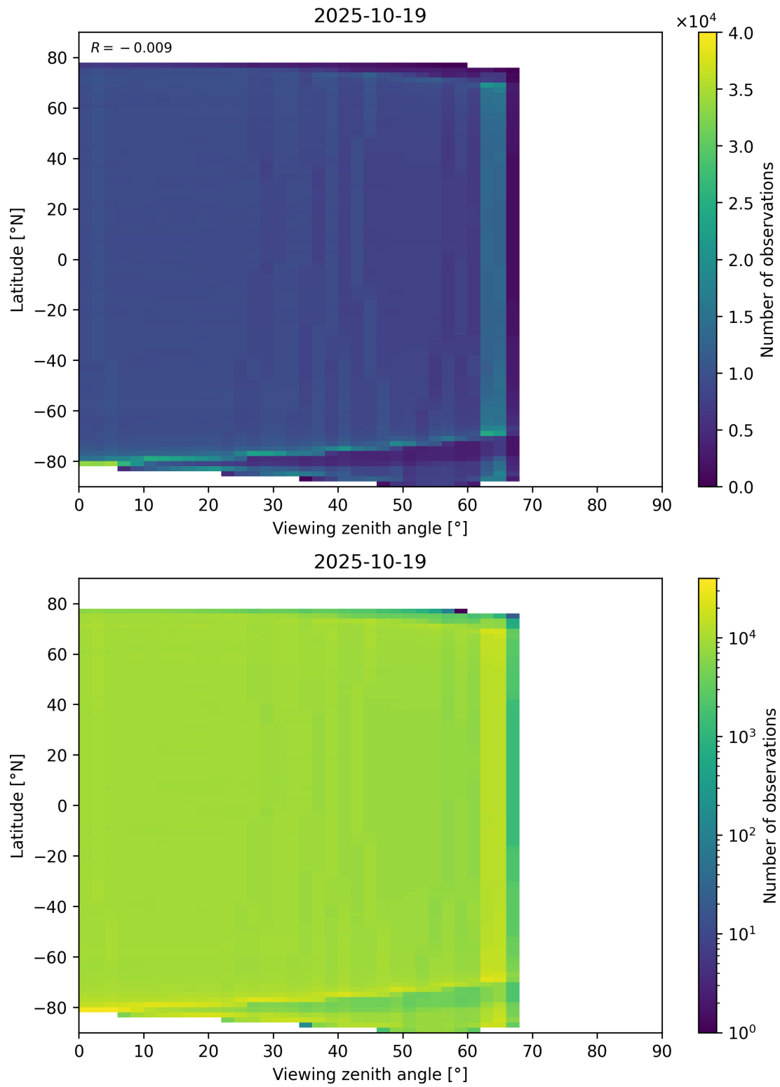
Figure 123: Scatter density plot of “Viewing zenith angle” against “Latitude” for 2025-10-18 to 2025-10-20.
