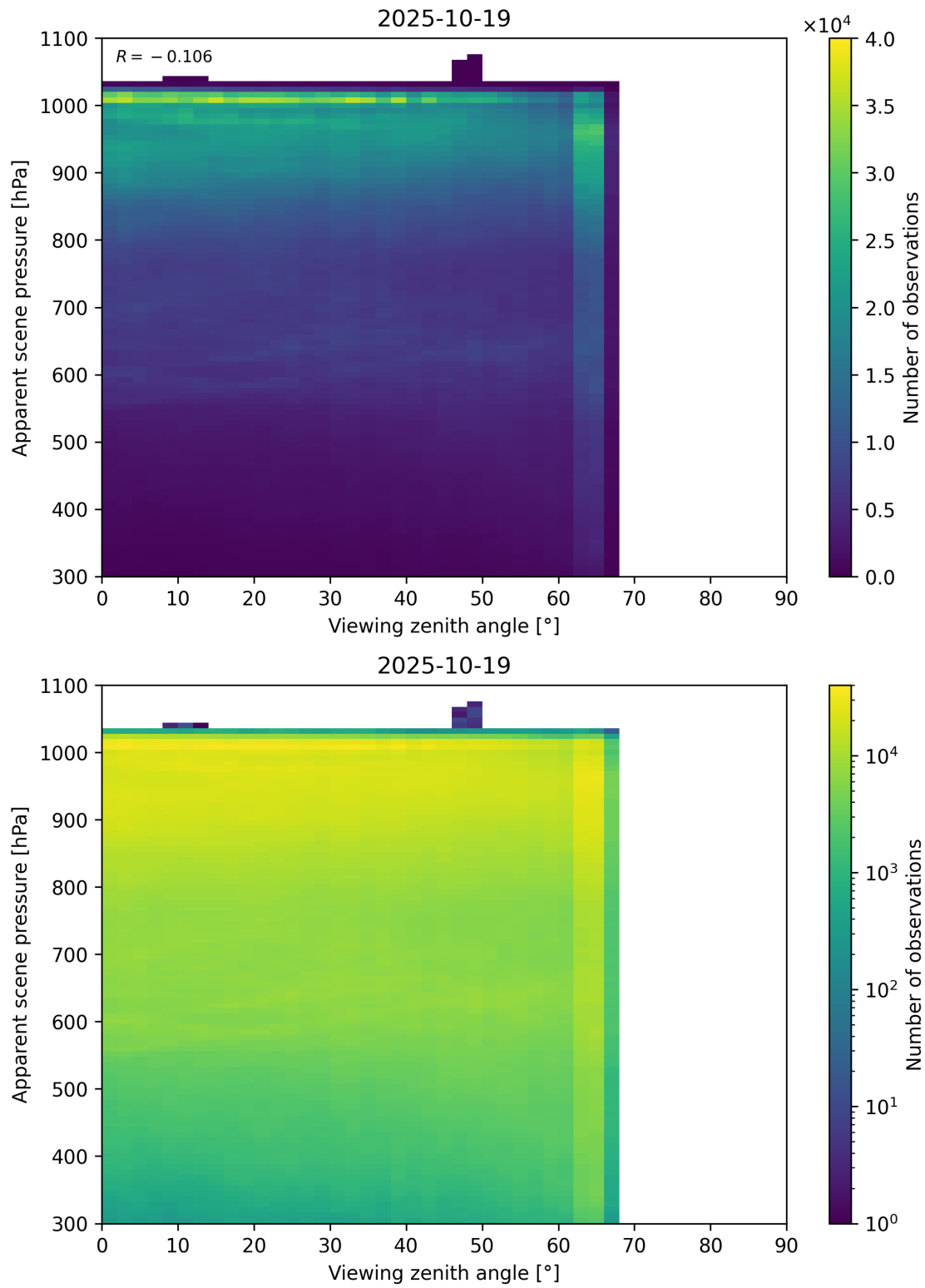
Figure 118: Scatter density plot of “Viewing zenith angle” against “Apparent scene pressure” for 2025-10-18 to 2025-10-20.
