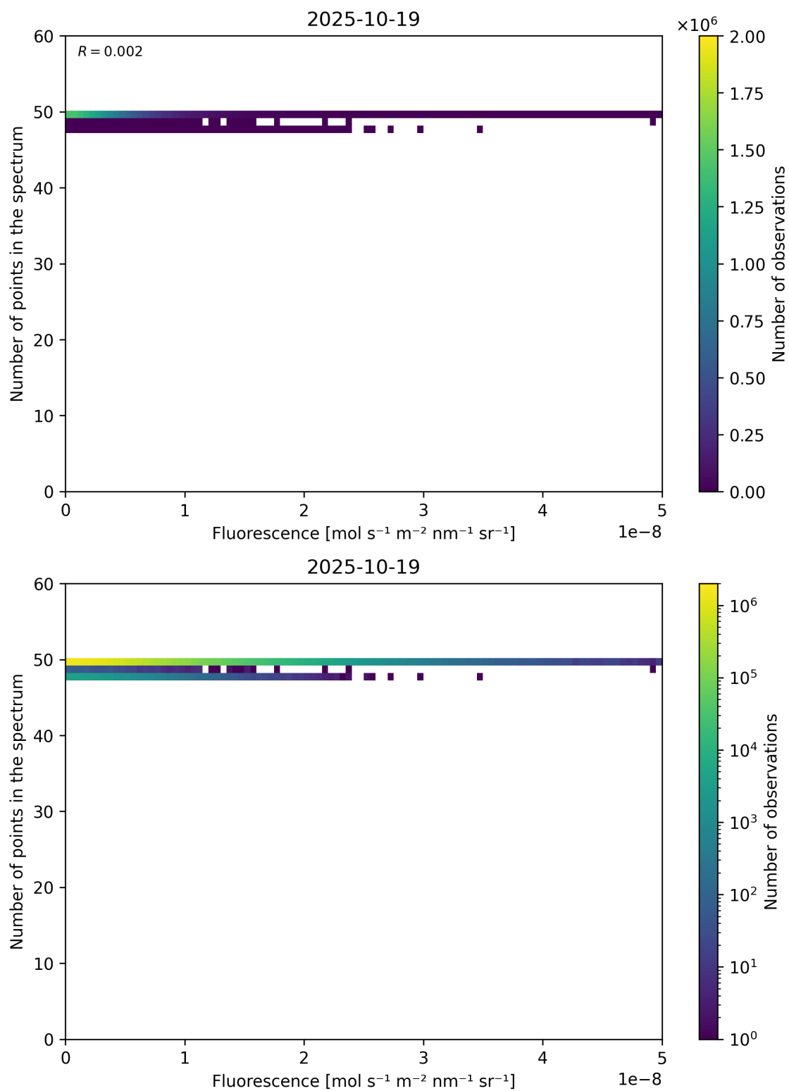
Figure 86: Scatter density plot of “Fluorescence” against “Number of points in the spectrum” for 2025-10-18 to 2025-10-20.
