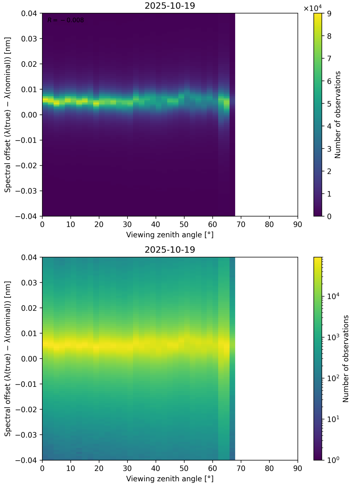
Figure 128: Scatter density plot of “Viewing zenith angle” against “Spectral offset ( \lambda_{\text{true}} - \lambda_{\text{nominal}} )” for 2025-10-18 to 2025-10-20.
