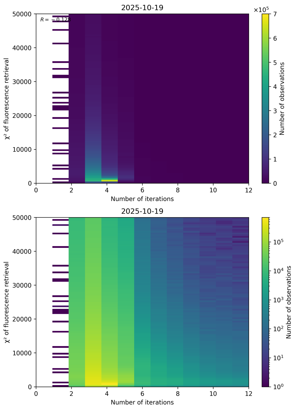
Figure 97: Scatter density plot of “Number of iterations” against “ \chi^2 of fluorescence retrieval” for 2025-10-18 to 2025-10-20.
