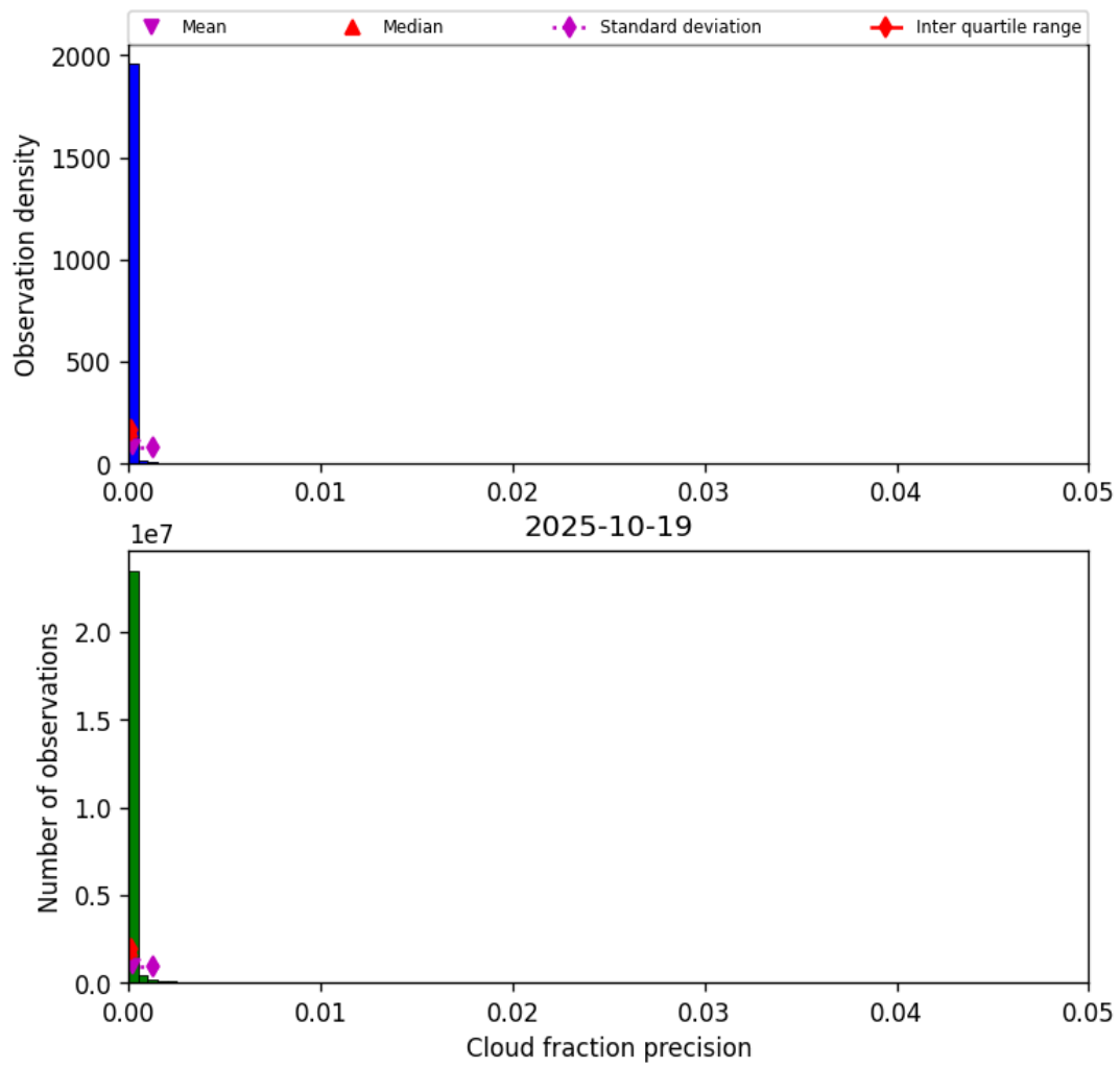
Figure 33: Histogram of “Cloud fraction precision” for 2025-10-18 to 2025-10-20
