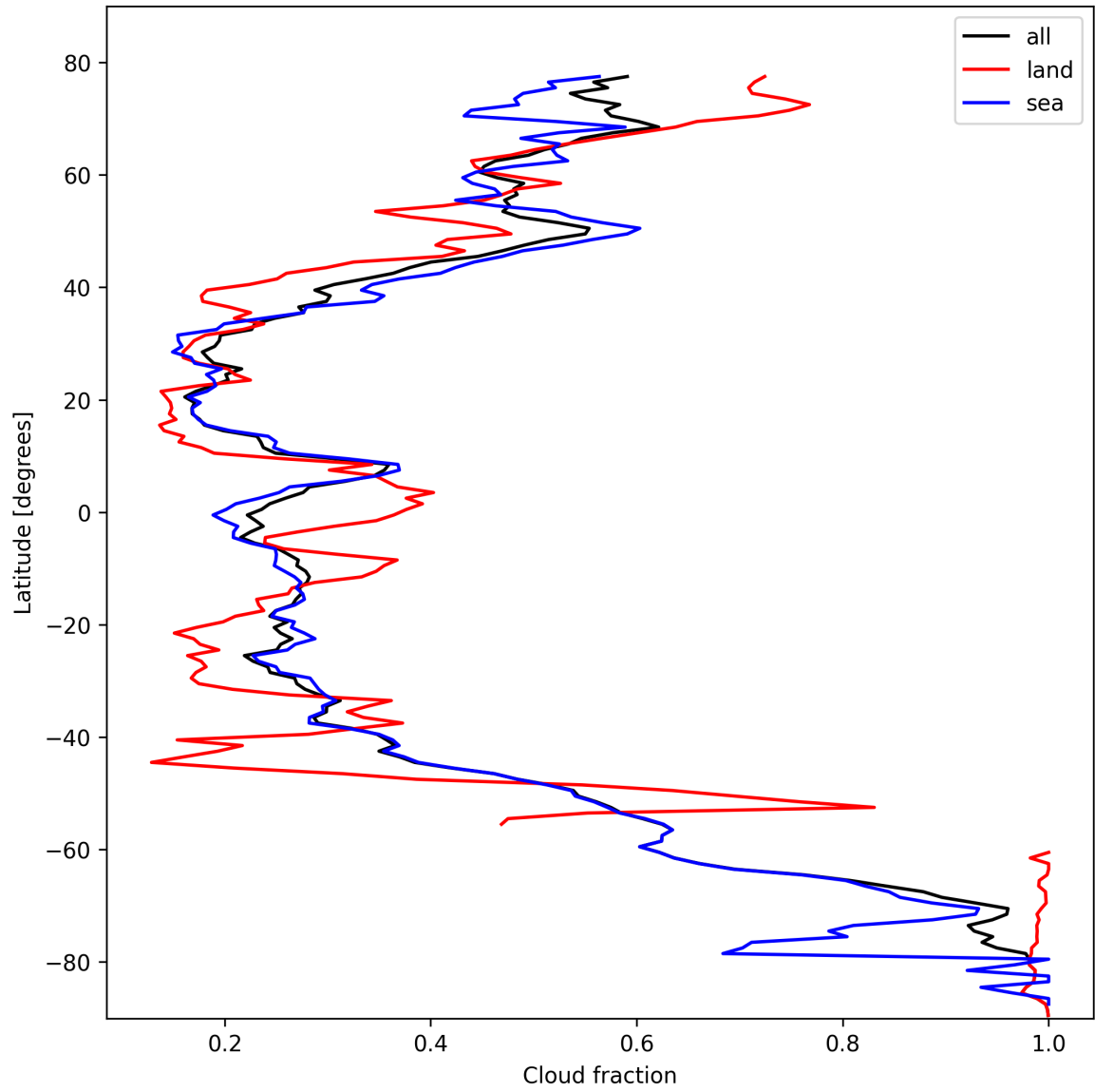
Figure 15: Zonal average of “Cloud fraction” for 2025-10-18 to 2025-10-20.
