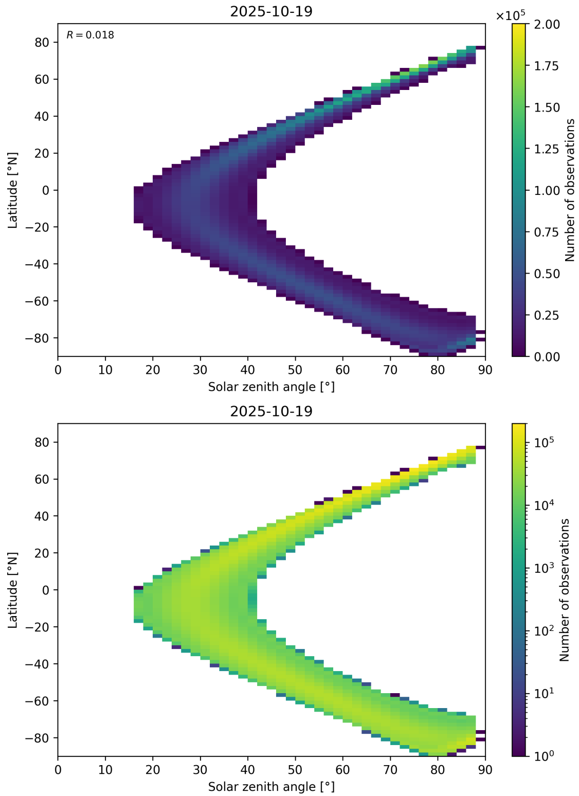
Figure 113: Scatter density plot of “Solar zenith angle” against “Latitude” for 2025-10-18 to 2025-10-20.
