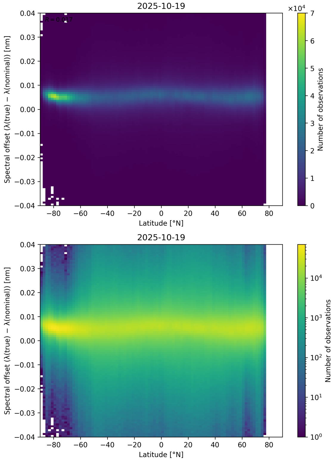
Figure 96: Scatter density plot of “Latitude” against “Spectral offset ( \lambda_{\text{true}} - \lambda_{\text{nominal}} )” for 2025-10-18 to 2025-10-20.
