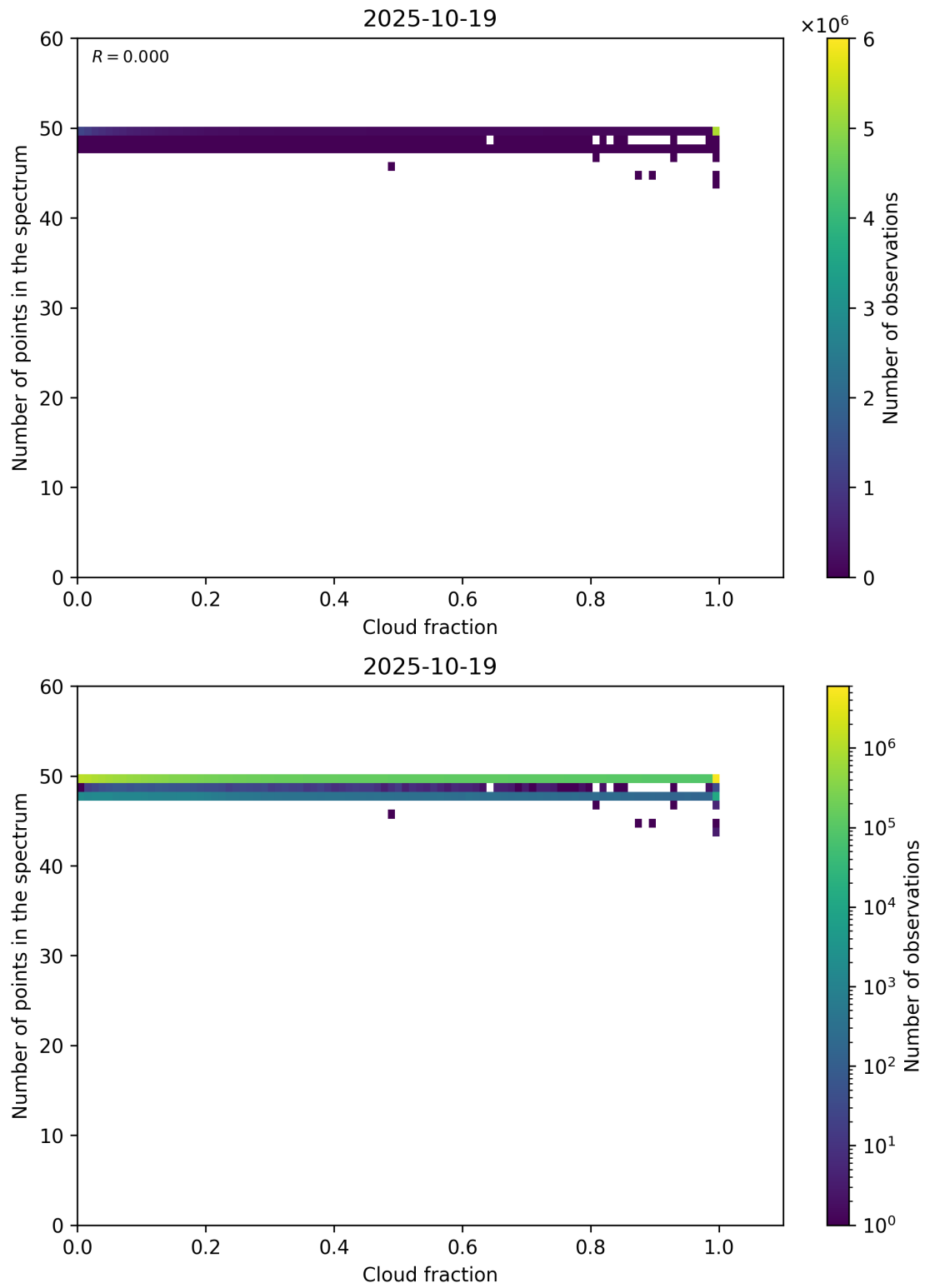
Figure 74: Scatter density plot of “Cloud fraction” against “Number of points in the spectrum” for 2025-10-18 to 2025-10-20.
