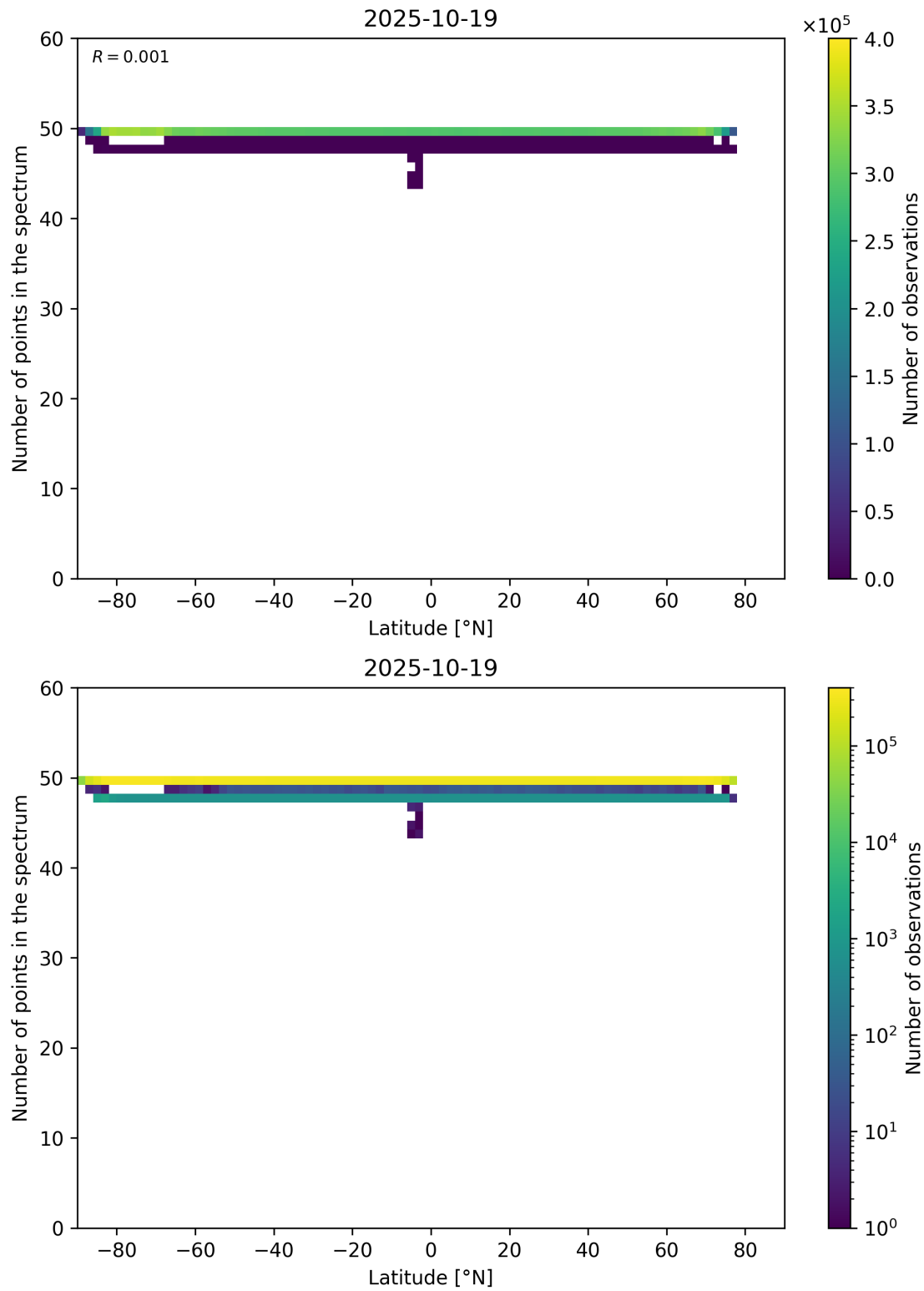
Figure 94: Scatter density plot of “Latitude” against “Number of points in the spectrum” for 2025-10-18 to 2025-10-20.
