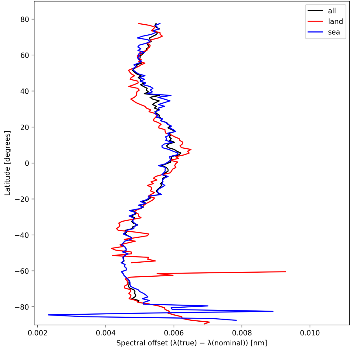
Figure 28: Zonal average of “Spectral offset ( \lambda_{\text{true}} - \lambda_{\text{nominal}} )” for 2025-10-18 to 2025-10-20.
