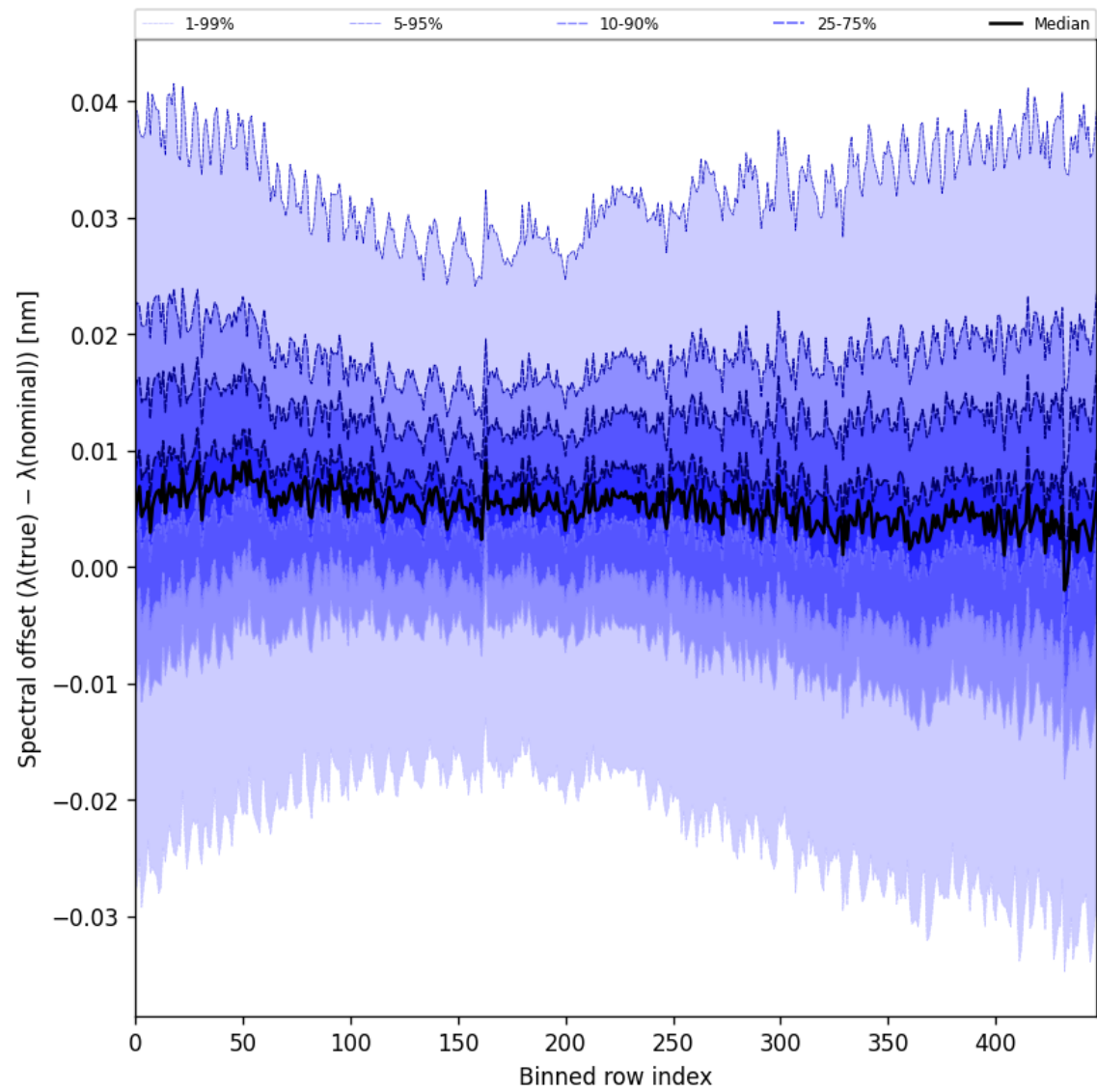
Figure 62: Along track statistics of “Spectral offset ( \lambda_{\text{true}} - \lambda_{\text{nominal}} )” for 2025-10-18 to 2025-10-20
