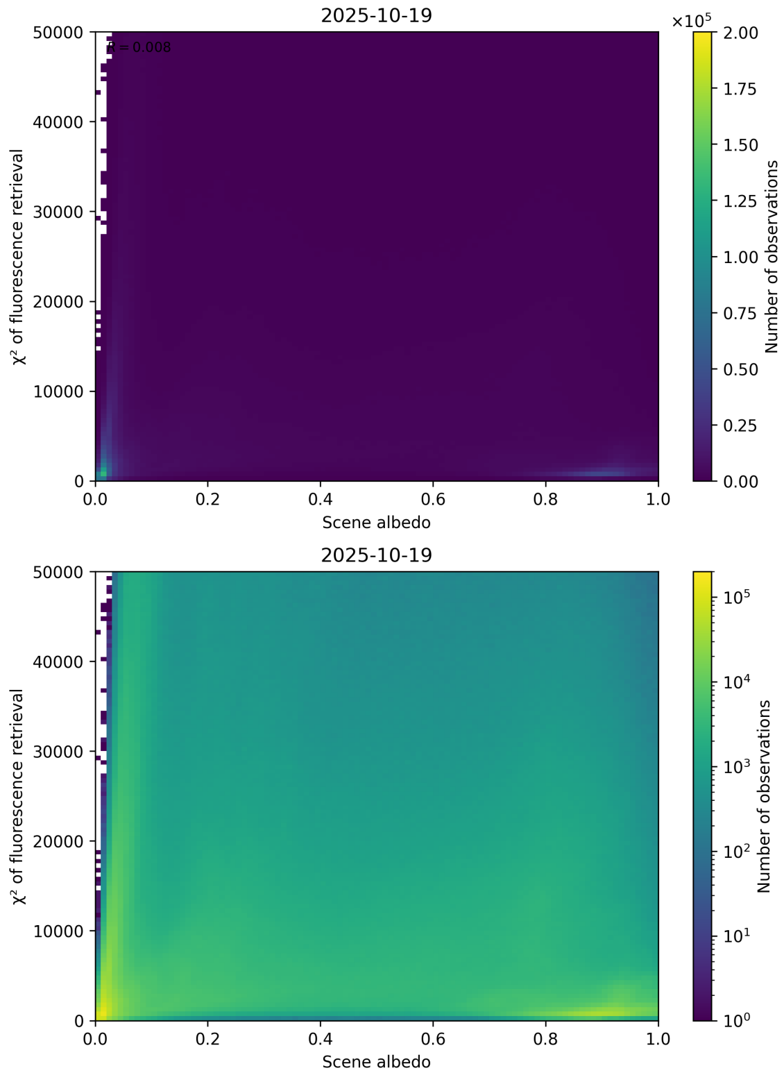
Figure 103: Scatter density plot of “Scene albedo” against “ \chi^2 of fluorescence retrieval” for 2025-10-18 to 2025-10-20.
