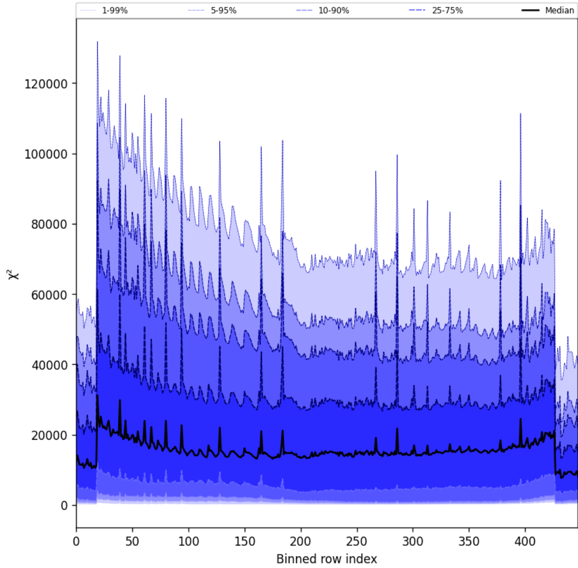
Figure 55: Along track statistics of “ \chi^2 ” for 2025-10-18 to 2025-10-20
