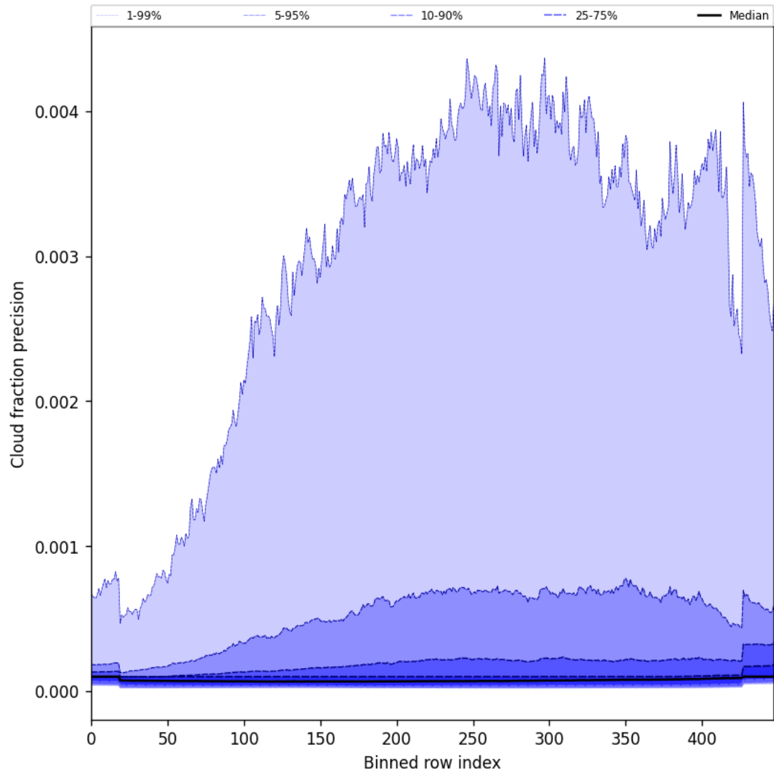
Figure 50: Along track statistics of “Cloud fraction precision” for 2025-10-18 to 2025-10-20
