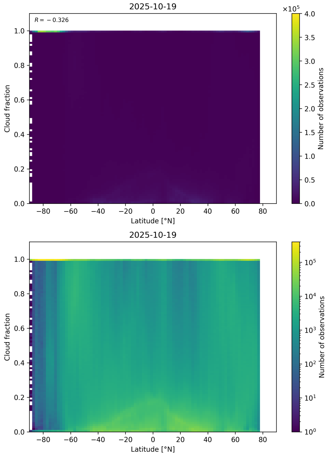
Figure 90: Scatter density plot of “Latitude” against “Cloud fraction” for 2025-10-18 to 2025-10-20.
