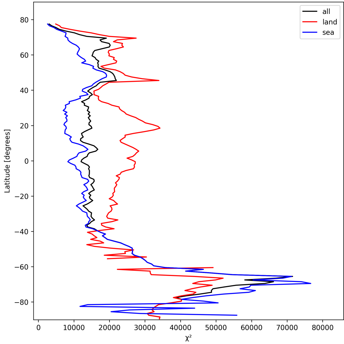
Figure 21: Zonal average of “ \chi^2 ” for 2025-10-18 to 2025-10-20.
