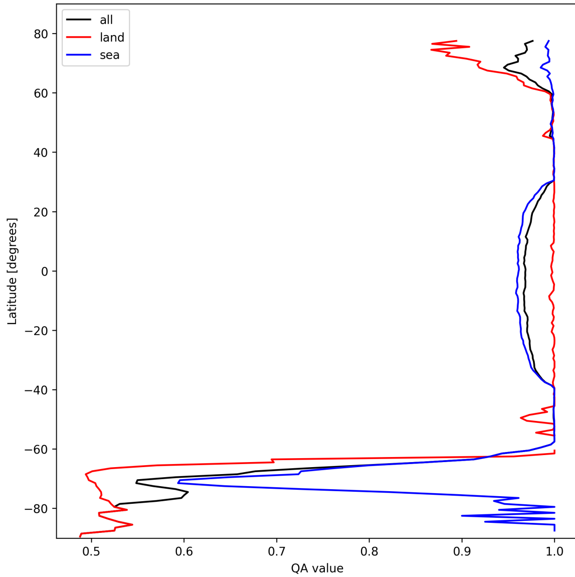
Figure 12: Zonal average of “QA value” for 2025-10-18 to 2025-10-20.
