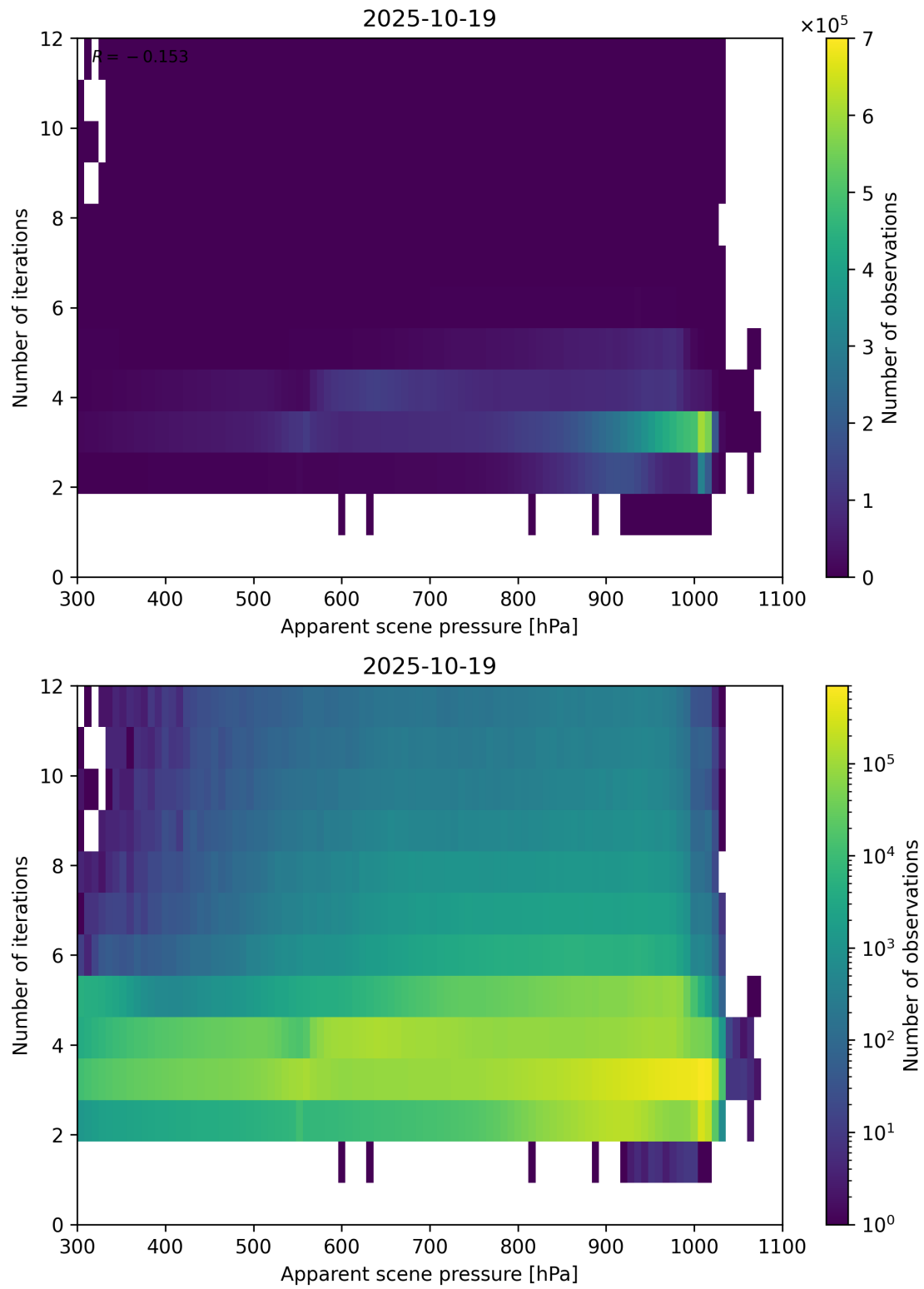
Figure 65: Scatter density plot of “Apparent scene pressure” against “Number of iterations” for 2025-10-18 to 2025-10-20.
