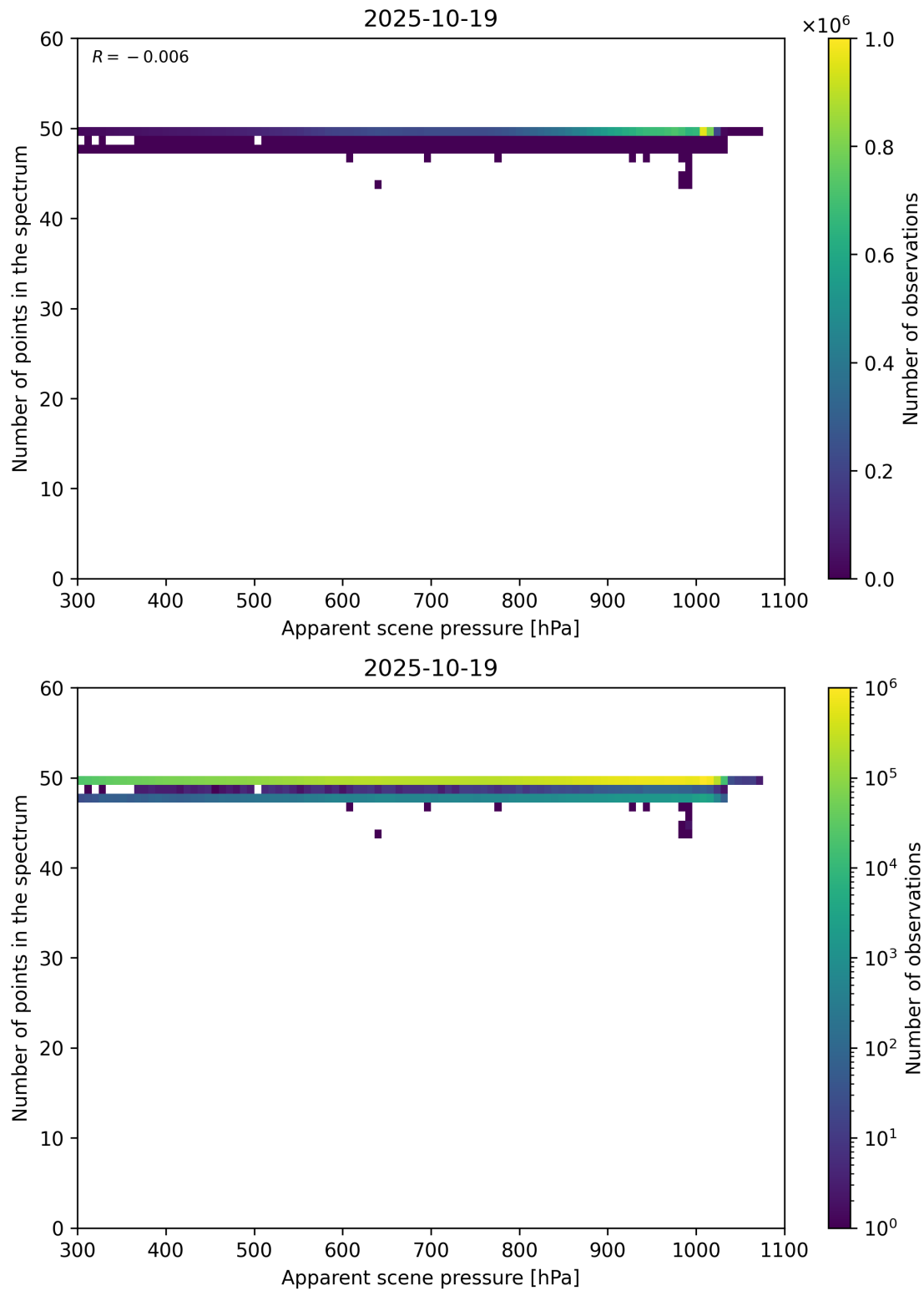
Figure 66: Scatter density plot of “Apparent scene pressure” against “Number of points in the spectrum” for 2025-10-18 to 2025-10-20.
