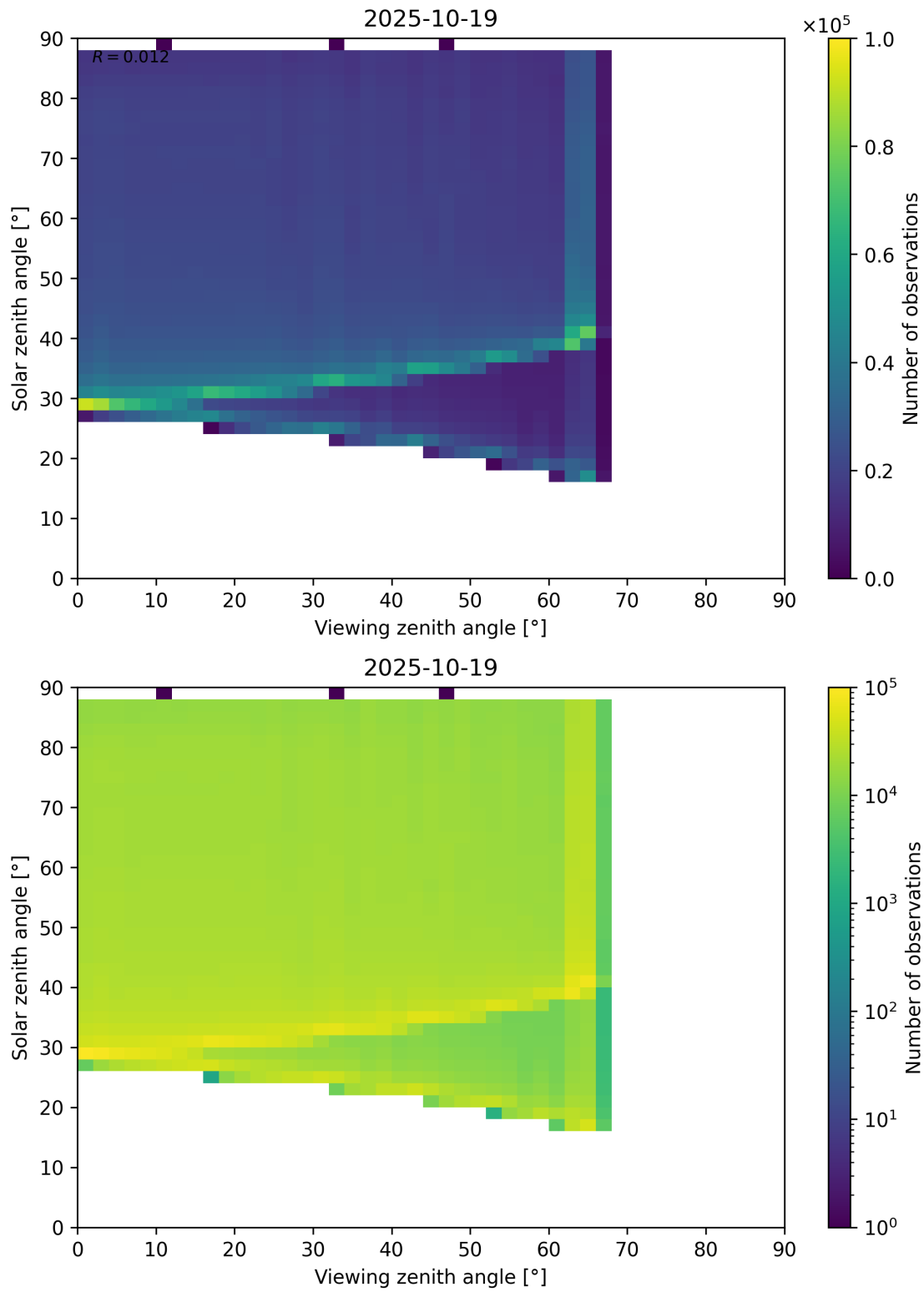
Figure 127: Scatter density plot of “Viewing zenith angle” against “Solar zenith angle” for 2025-10-18 to 2025-10-20.
