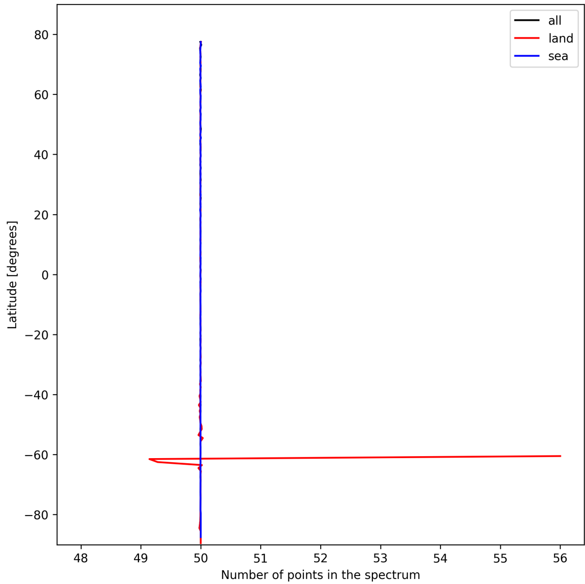
Figure 27: Zonal average of “Number of points in the spectrum” for 2025-10-18 to 2025-10-20.
