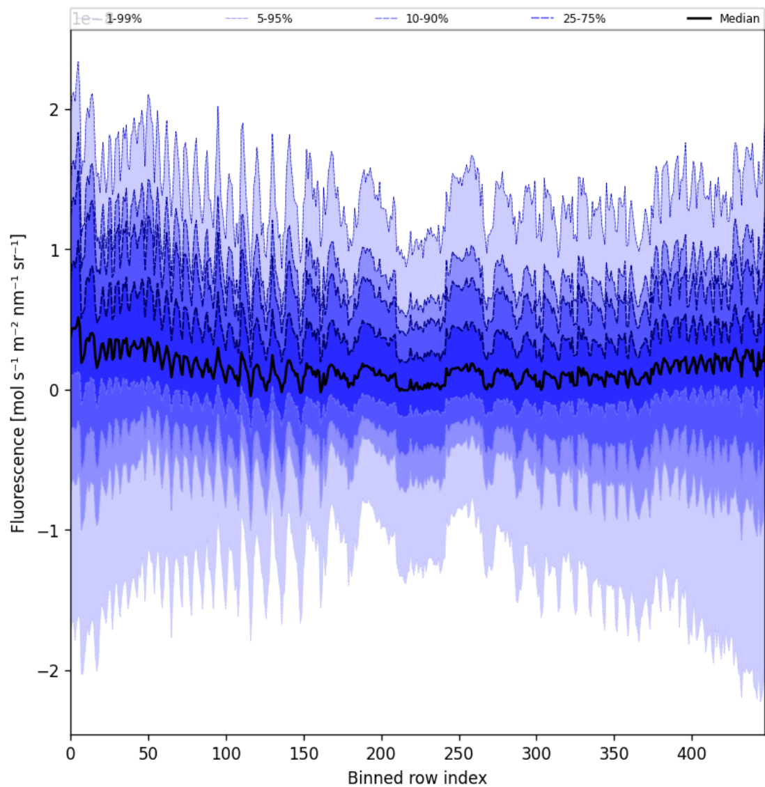
Figure 57: Along track statistics of “Fluorescence” for 2025-10-18 to 2025-10-20
