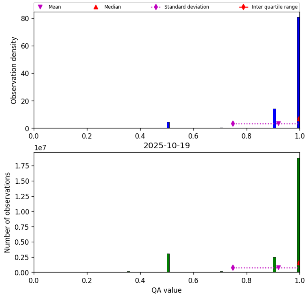
Figure 29: Histogram of “QA value” for 2025-10-18 to 2025-10-20
