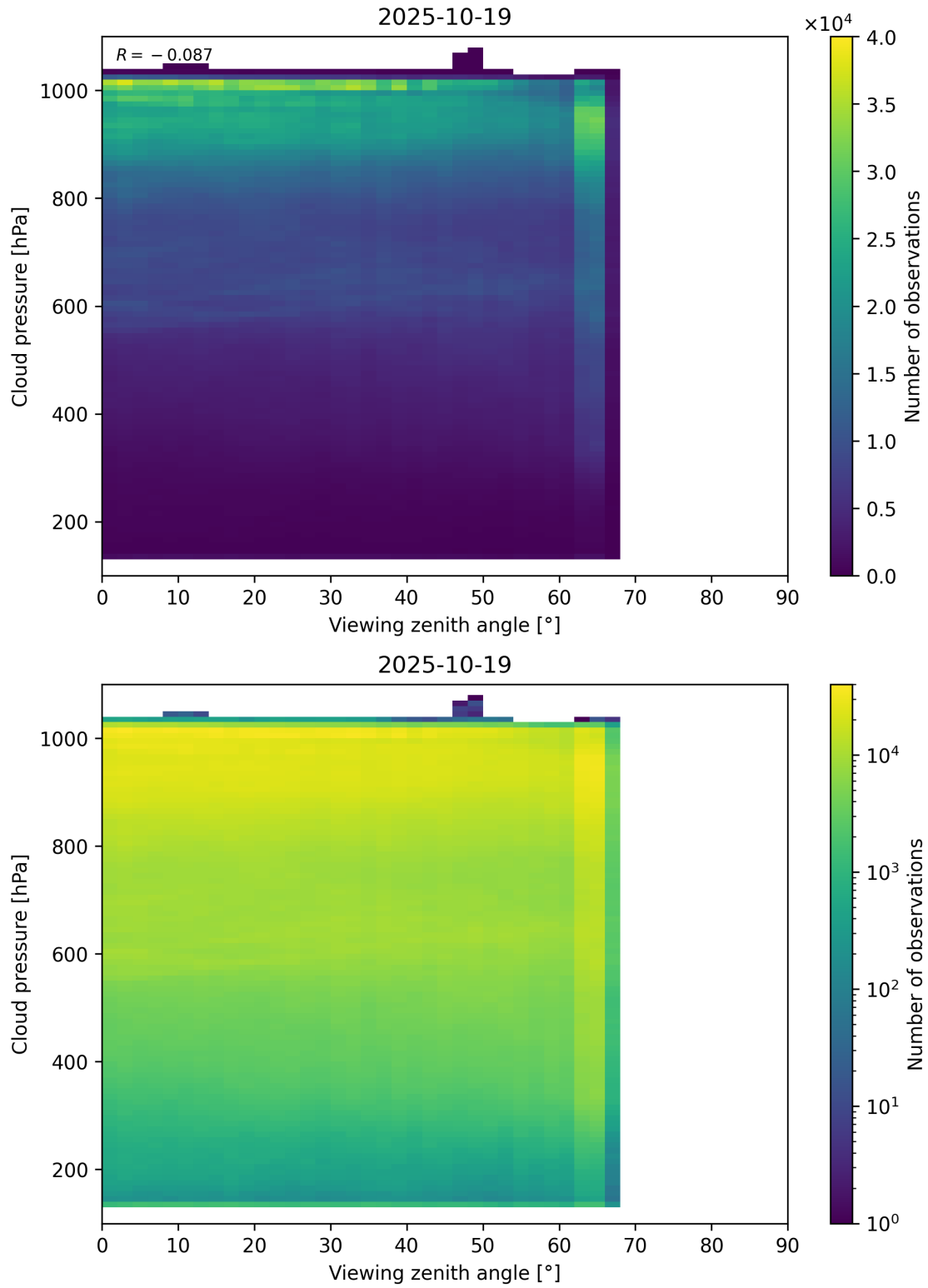
Figure 121: Scatter density plot of “Viewing zenith angle” against “Cloud pressure” for 2025-10-18 to 2025-10-20.
