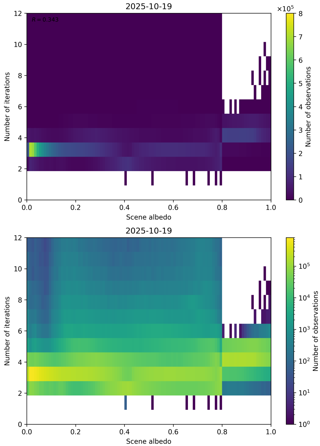
Figure 105: Scatter density plot of “Scene albedo” against “Number of iterations” for 2025-10-18 to 2025-10-20.
