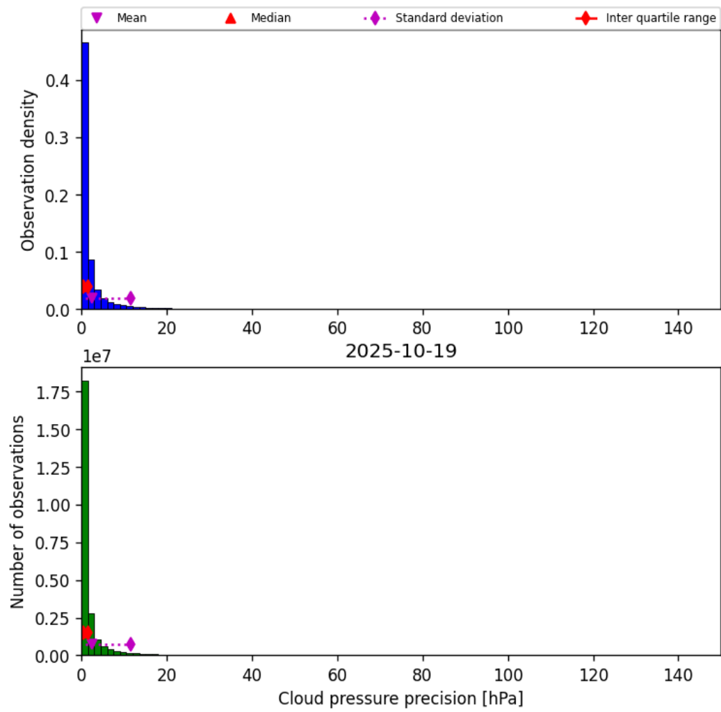
Figure 31: Histogram of “Cloud pressure precision” for 2025-10-18 to 2025-10-20
