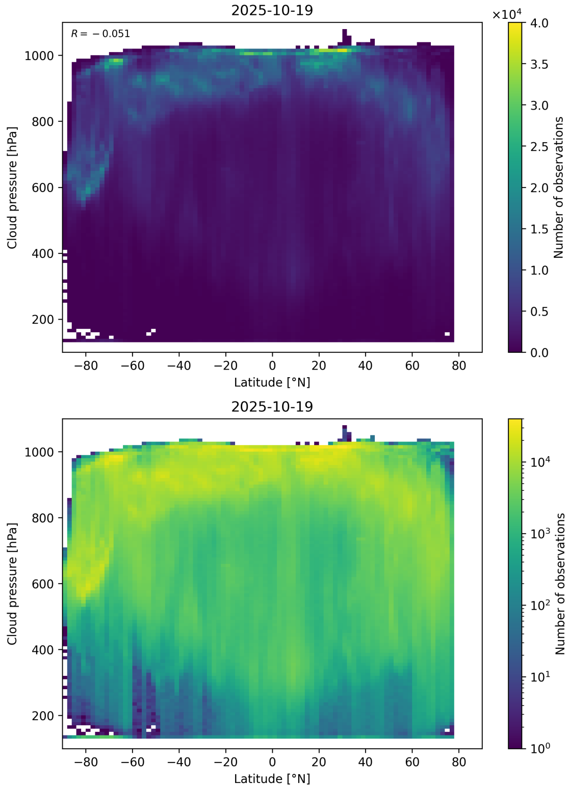
Figure 91: Scatter density plot of “Latitude” against “Cloud pressure” for 2025-10-18 to 2025-10-20.
