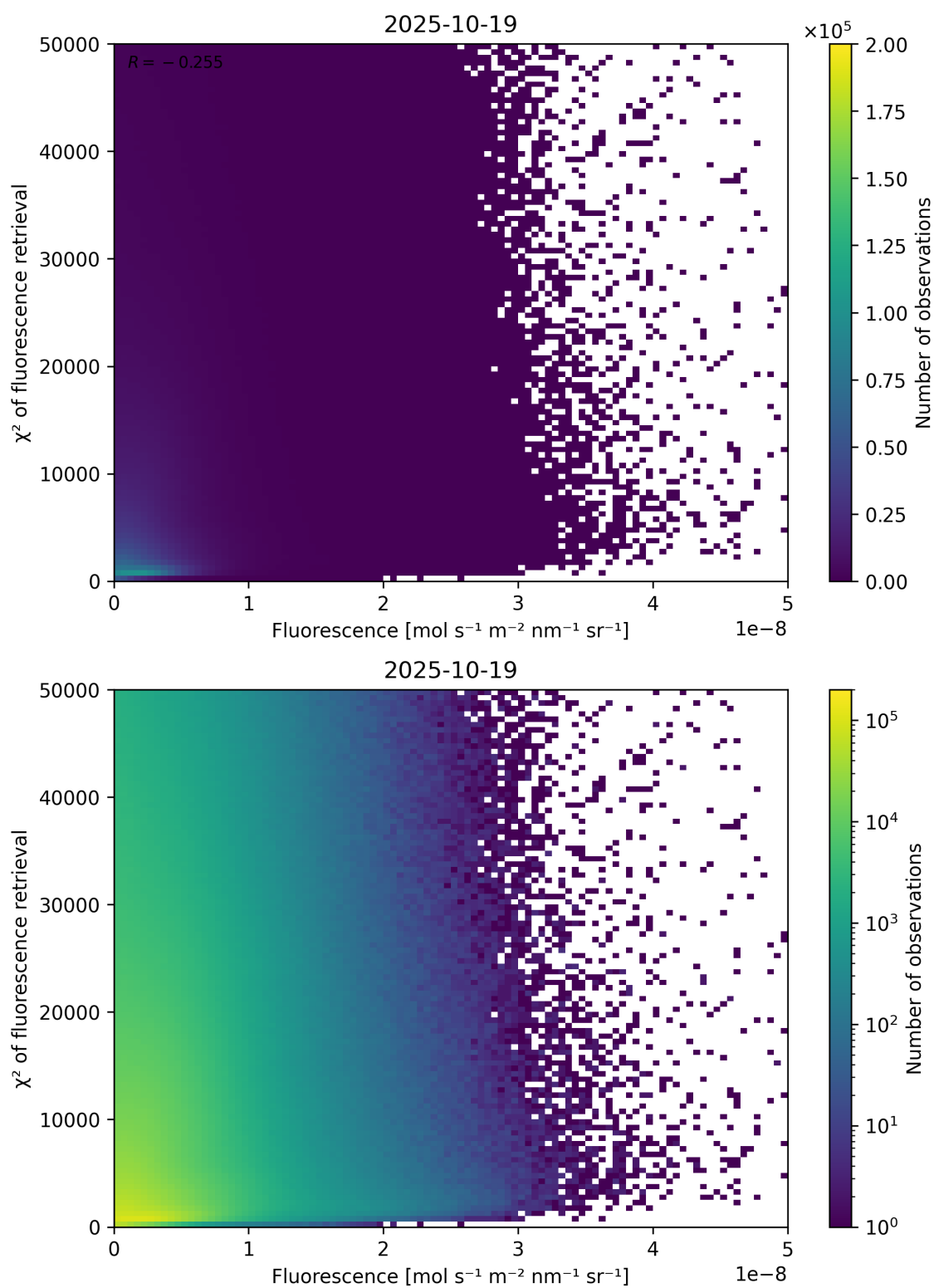
Figure 85: Scatter density plot of “Fluorescence” against “ \chi^2 of fluorescence retrieval” for 2025-10-18 to 2025-10-20.
