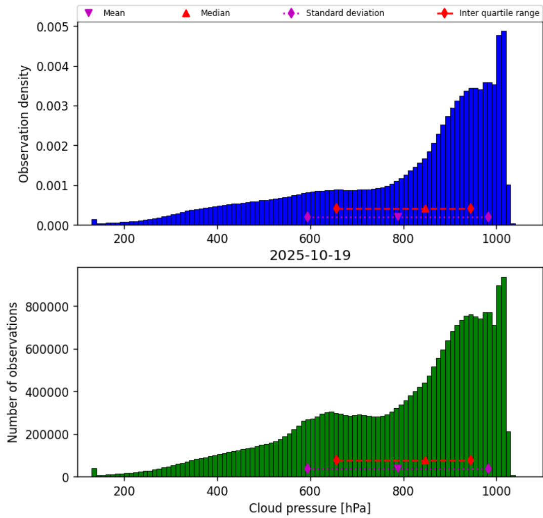
Figure 30: Histogram of “Cloud pressure” for 2025-10-18 to 2025-10-20
