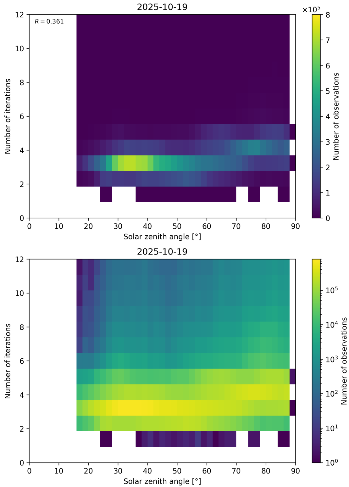
Figure 114: Scatter density plot of “Solar zenith angle” against “Number of iterations” for 2025-10-18 to 2025-10-20.
