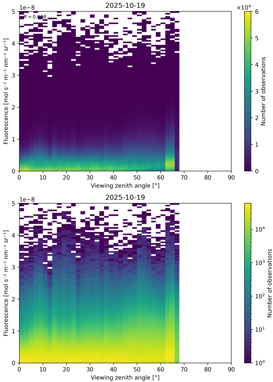
Figure 122: Scatter density plot of “Viewing zenith angle” against “Fluorescence” for 2025-10-18 to 2025-10-20.
