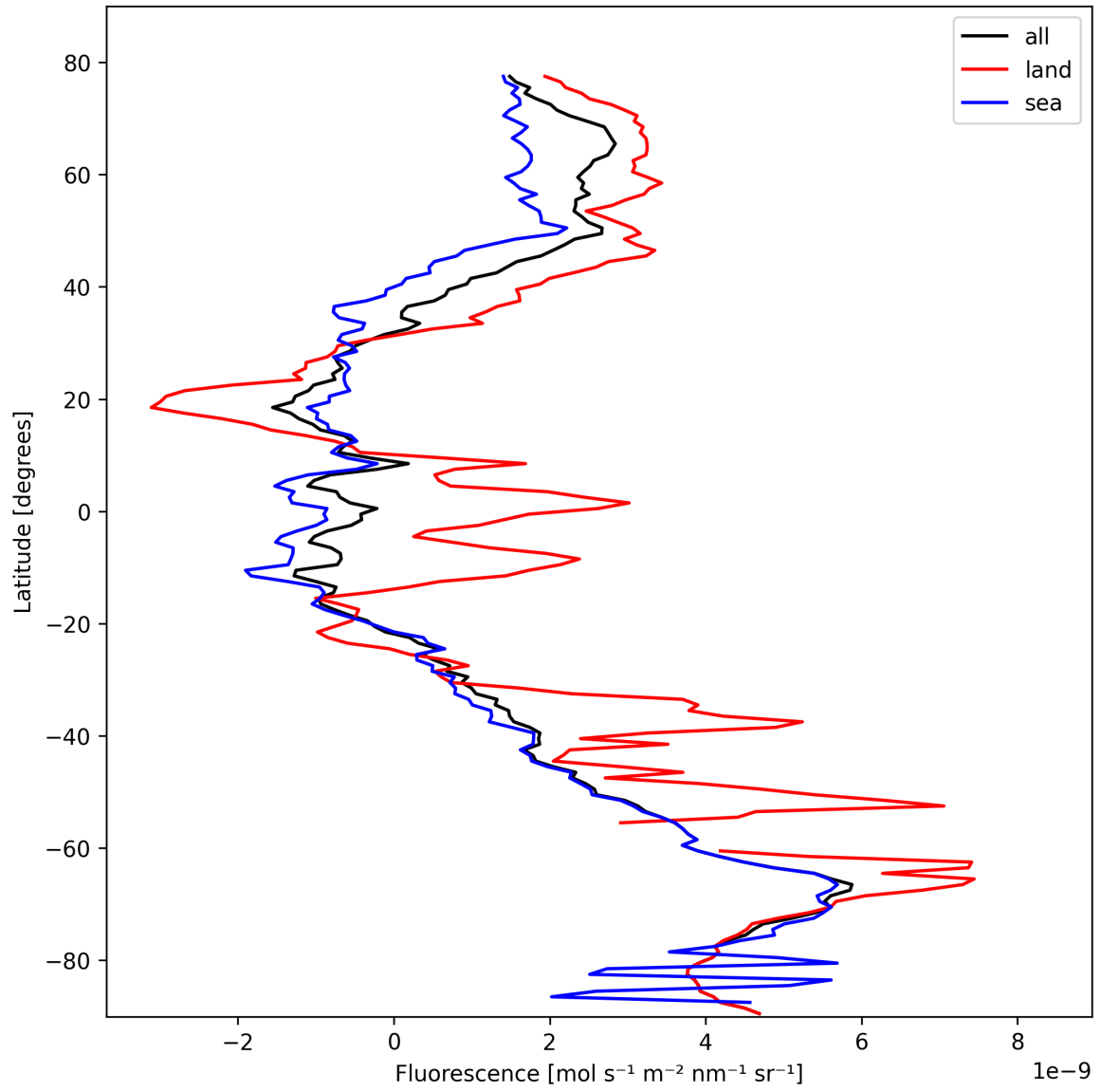
Figure 23: Zonal average of “Fluorescence” for 2025-10-18 to 2025-10-20.
