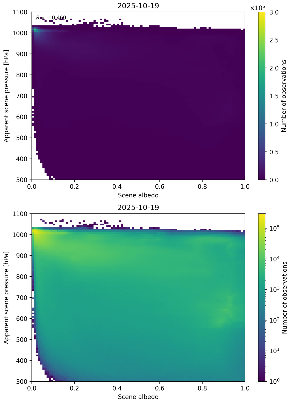
Figure 102: Scatter density plot of “Scene albedo” against “Apparent scene pressure” for 2025-10-18 to 2025-10-20.
