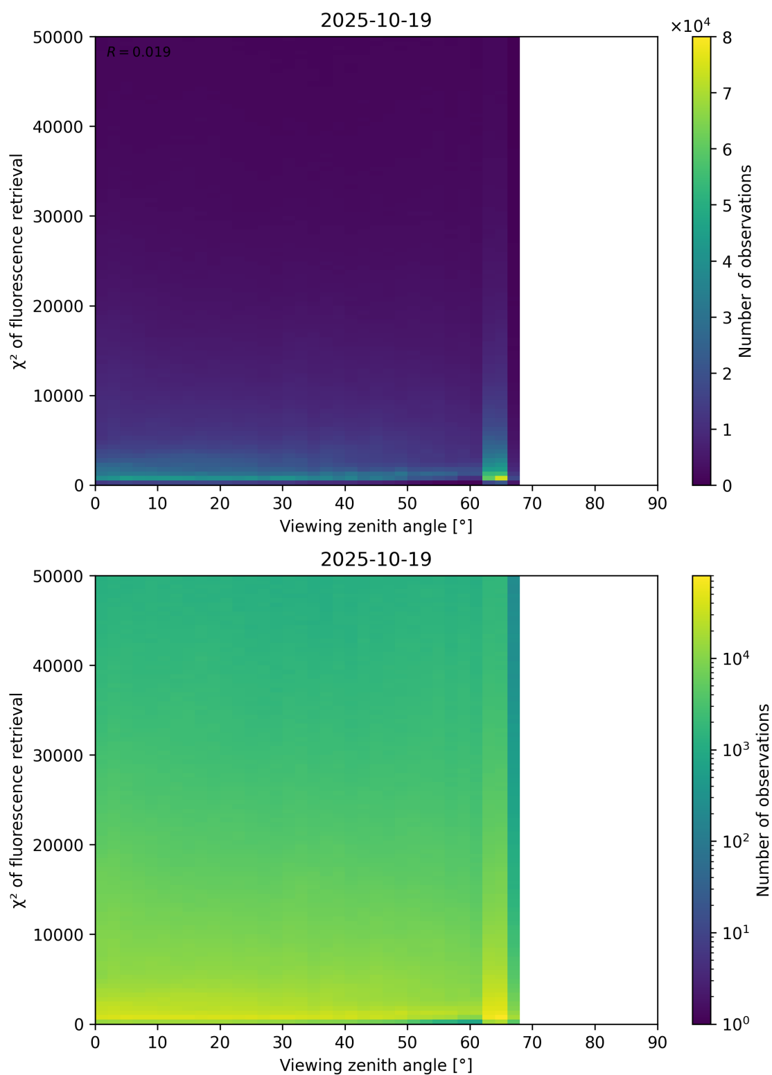
Figure 119: Scatter density plot of “Viewing zenith angle” against “ \chi^2 of fluorescence retrieval” for 2025-10-18 to 2025-10-20.
