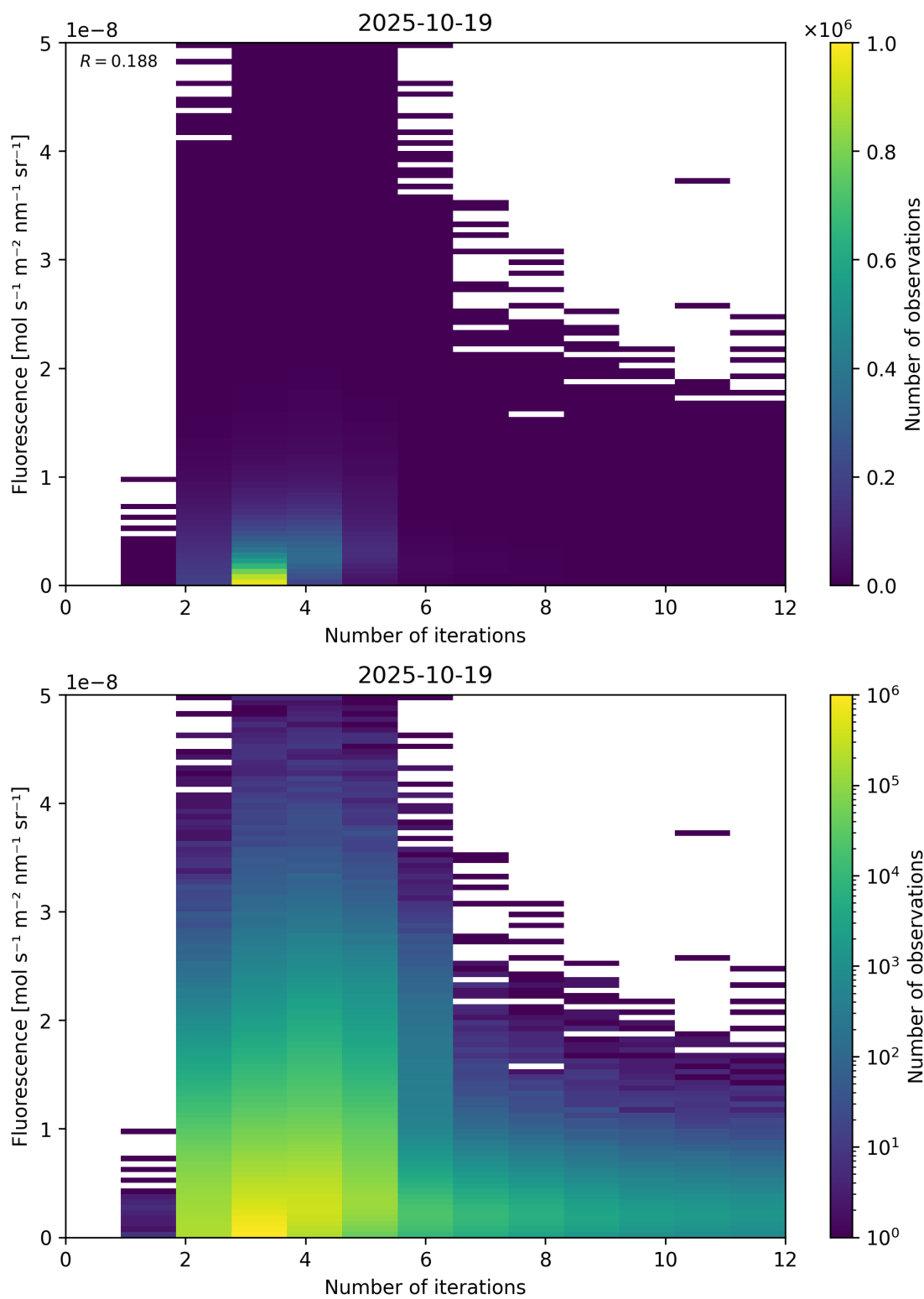
Figure 98: Scatter density plot of “Number of iterations” against “Fluorescence” for 2025-10-18 to 2025-10-20.
