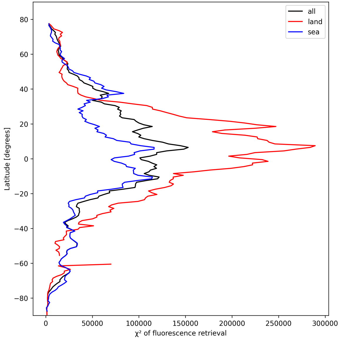
Figure 25: Zonal average of “ \chi^2 of fluorescence retrieval” for 2025-10-18 to 2025-10-20.
