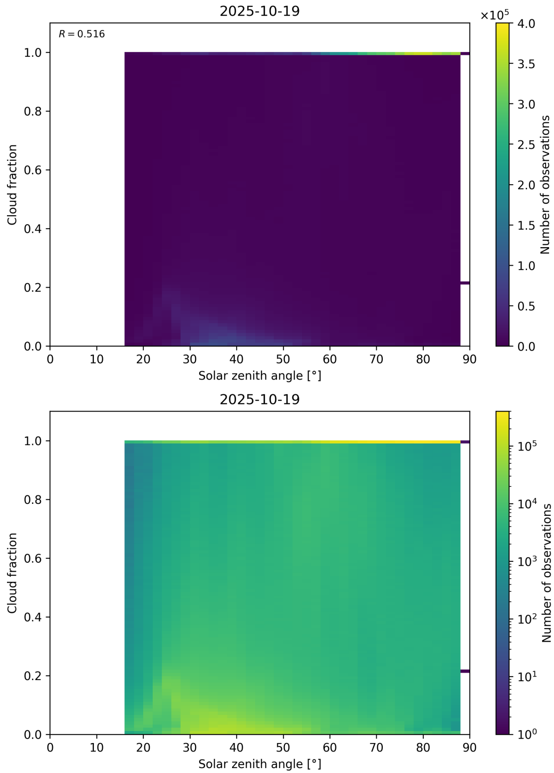
Figure 110: Scatter density plot of “Solar zenith angle” against “Cloud fraction” for 2025-10-18 to 2025-10-20.
