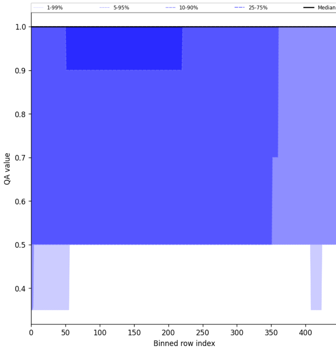
Figure 46: Along track statistics of “QA value” for 2025-10-18 to 2025-10-20
