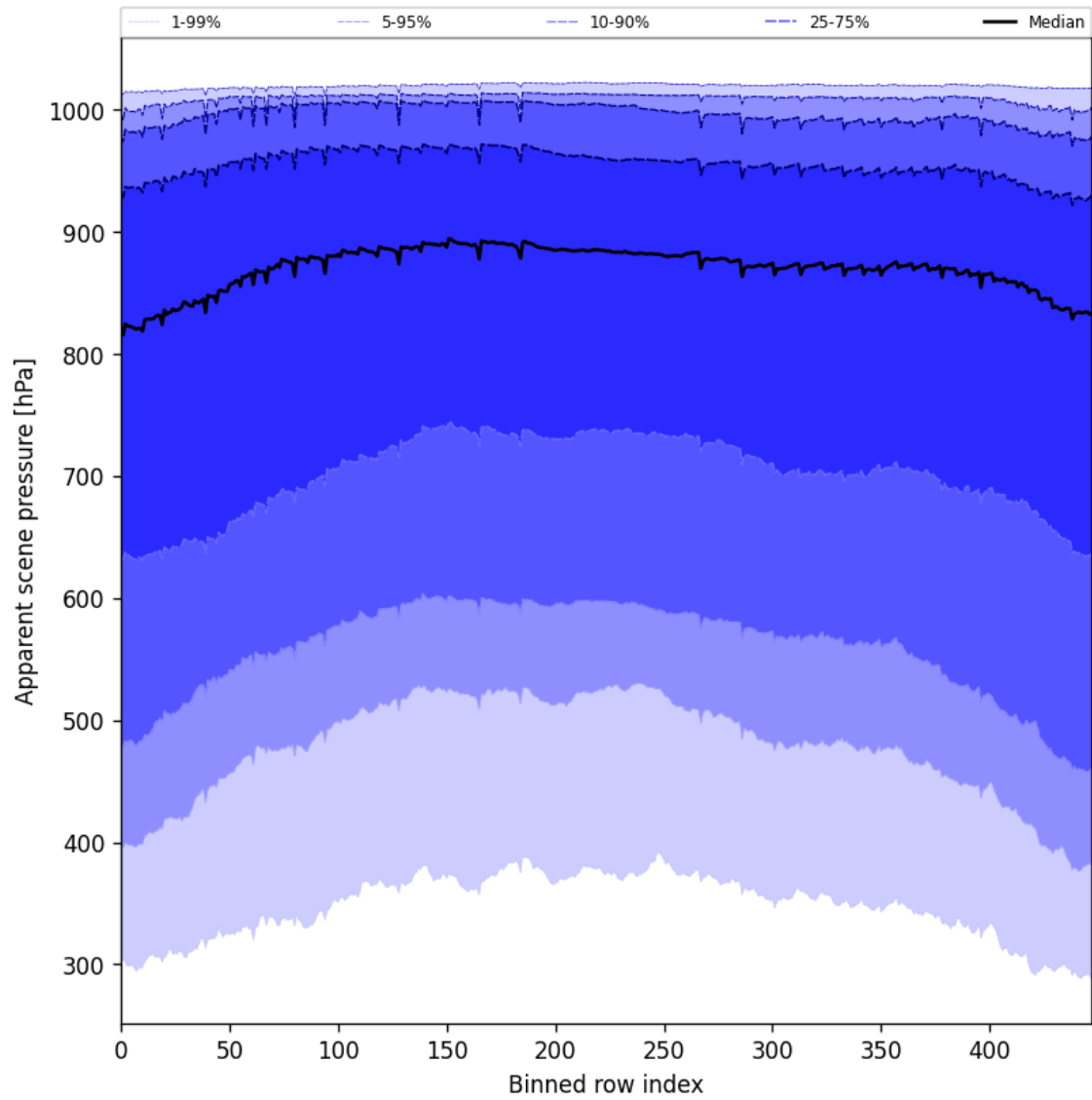
Figure 53: Along track statistics of “Apparent scene pressure” for 2025-10-18 to 2025-10-20
