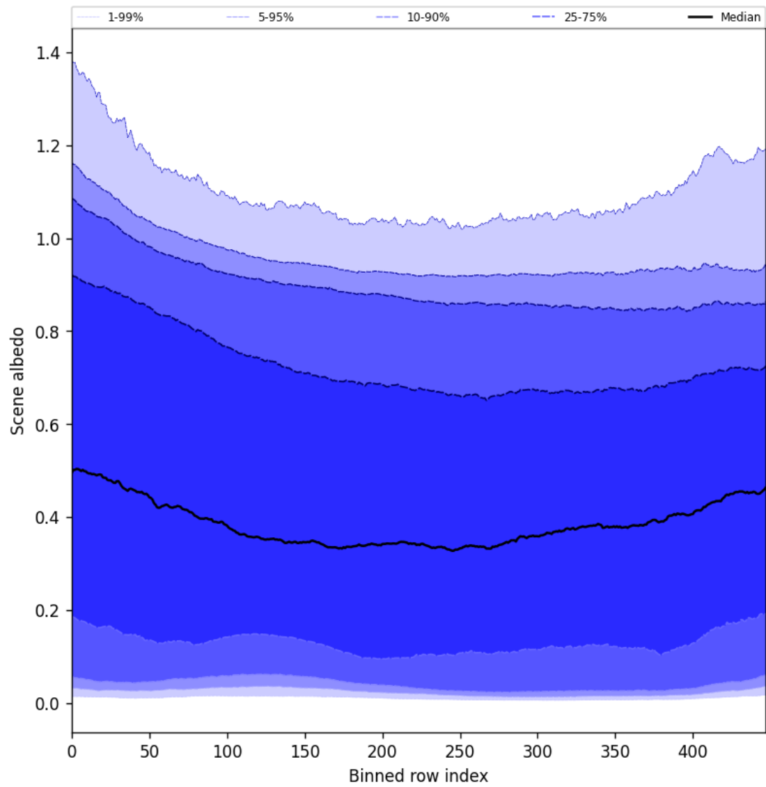
Figure 51: Along track statistics of “Scene albedo” for 2025-10-18 to 2025-10-20
