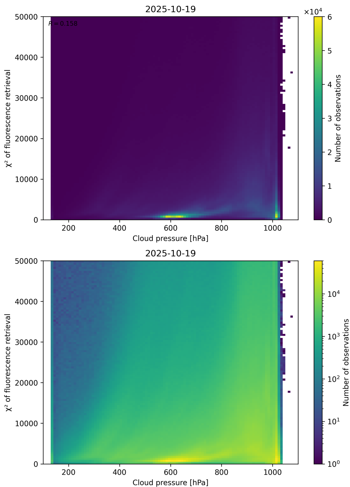
Figure 78: Scatter density plot of “Cloud pressure” against “ \chi^2 of fluorescence retrieval” for 2025-10-18 to 2025-10-20.
