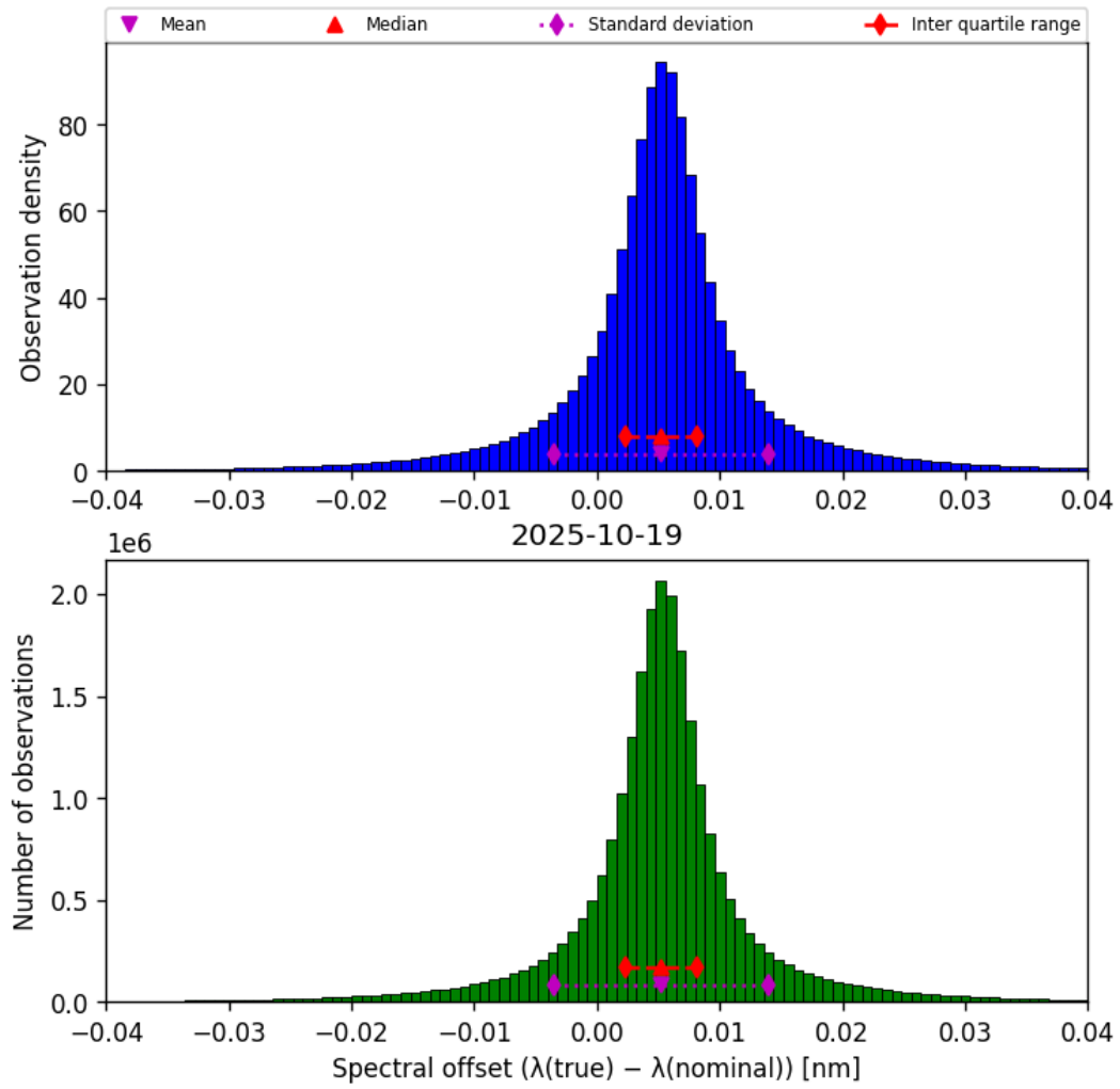
Figure 45: Histogram of “Spectral offset ( \lambda_{\text{true}} - \lambda_{\text{nominal}} )” for 2025-10-18 to 2025-10-20
