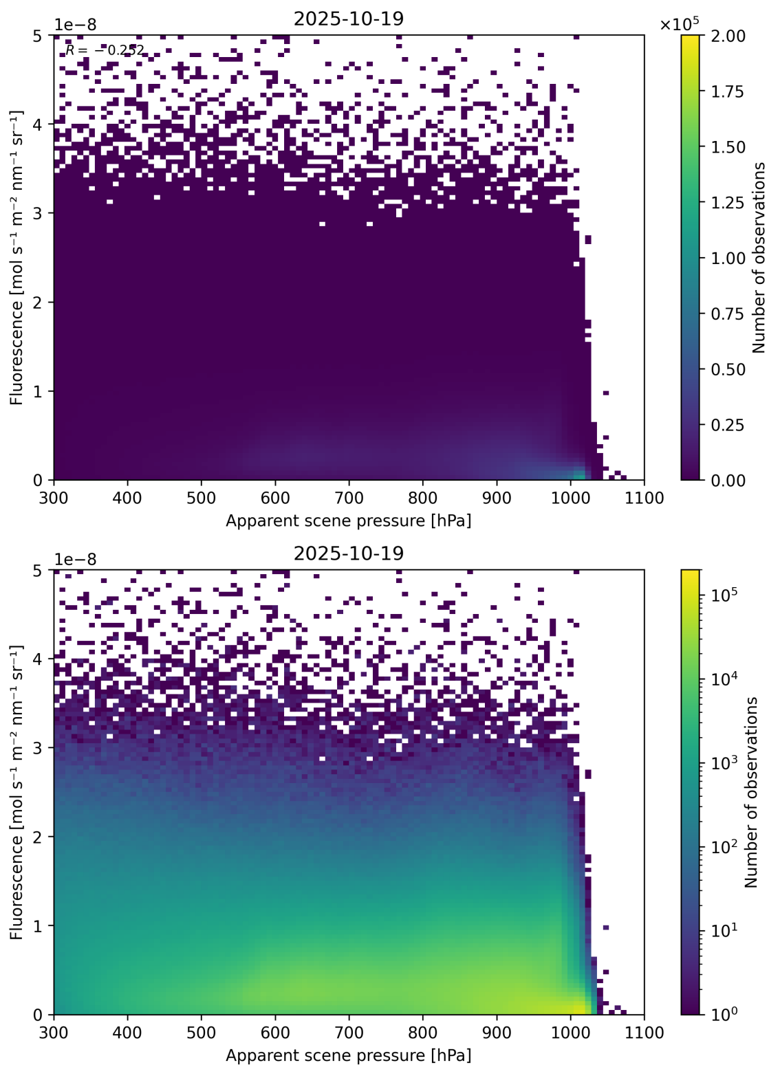
Figure 64: Scatter density plot of “Apparent scene pressure” against “Fluorescence” for 2025-10-18 to 2025-10-20.
