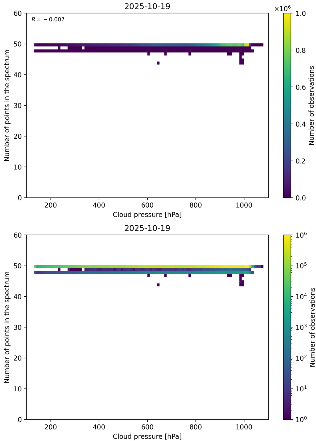
Figure 82: Scatter density plot of “Cloud pressure” against “Number of points in the spectrum” for 2025-10-18 to 2025-10-20.
