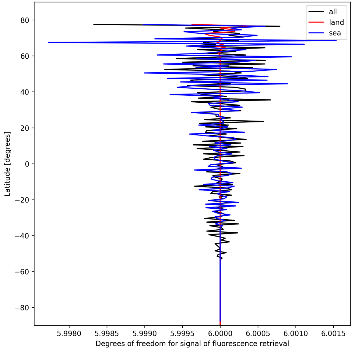
Figure 26: Zonal average of “Degrees of freedom for signal of fluorescence retrieval” for 2025-10-18 to 2025-10-20.
