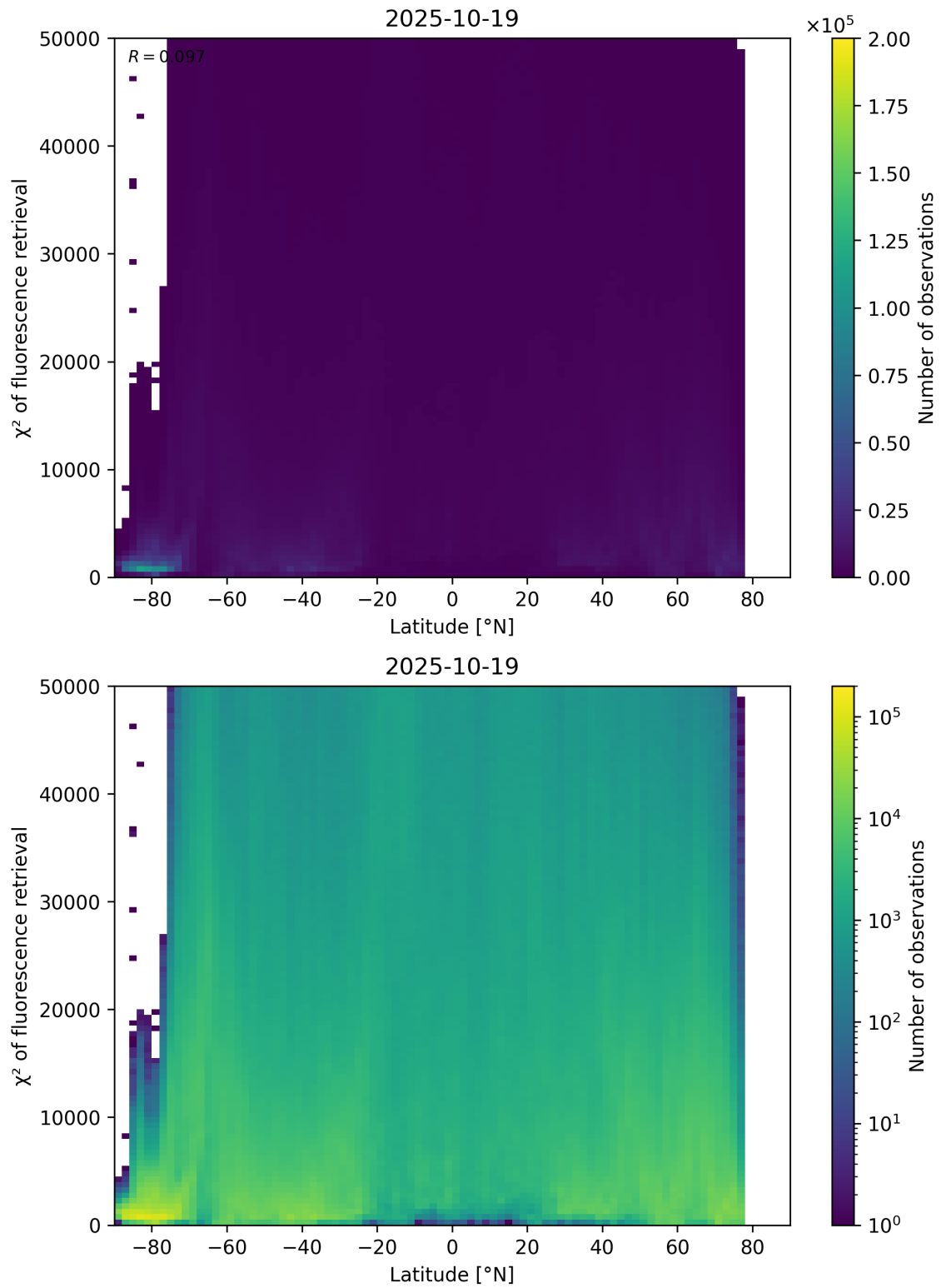
Figure 89: Scatter density plot of “Latitude” against “ \chi^2 of fluorescence retrieval” for 2025-10-18 to 2025-10-20.
