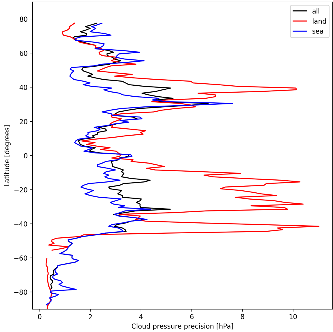
Figure 14: Zonal average of “Cloud pressure precision” for 2025-10-18 to 2025-10-20.
