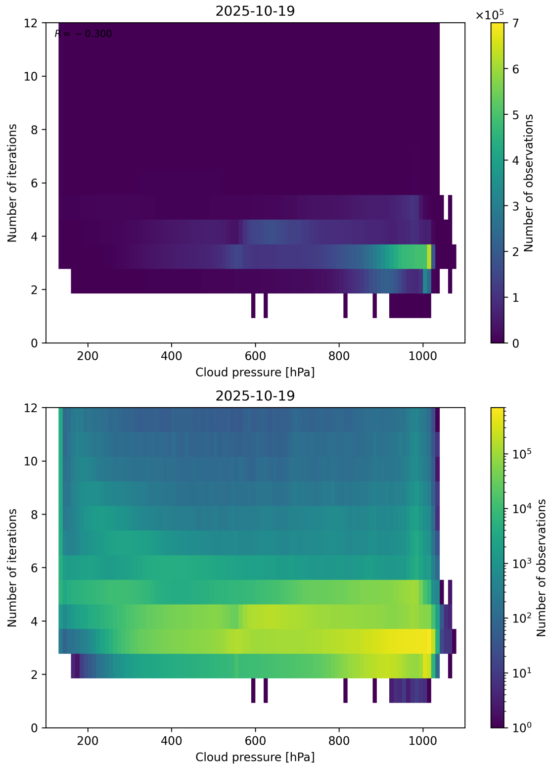
Figure 81: Scatter density plot of “Cloud pressure” against “Number of iterations” for 2025-10-18 to 2025-10-20.
