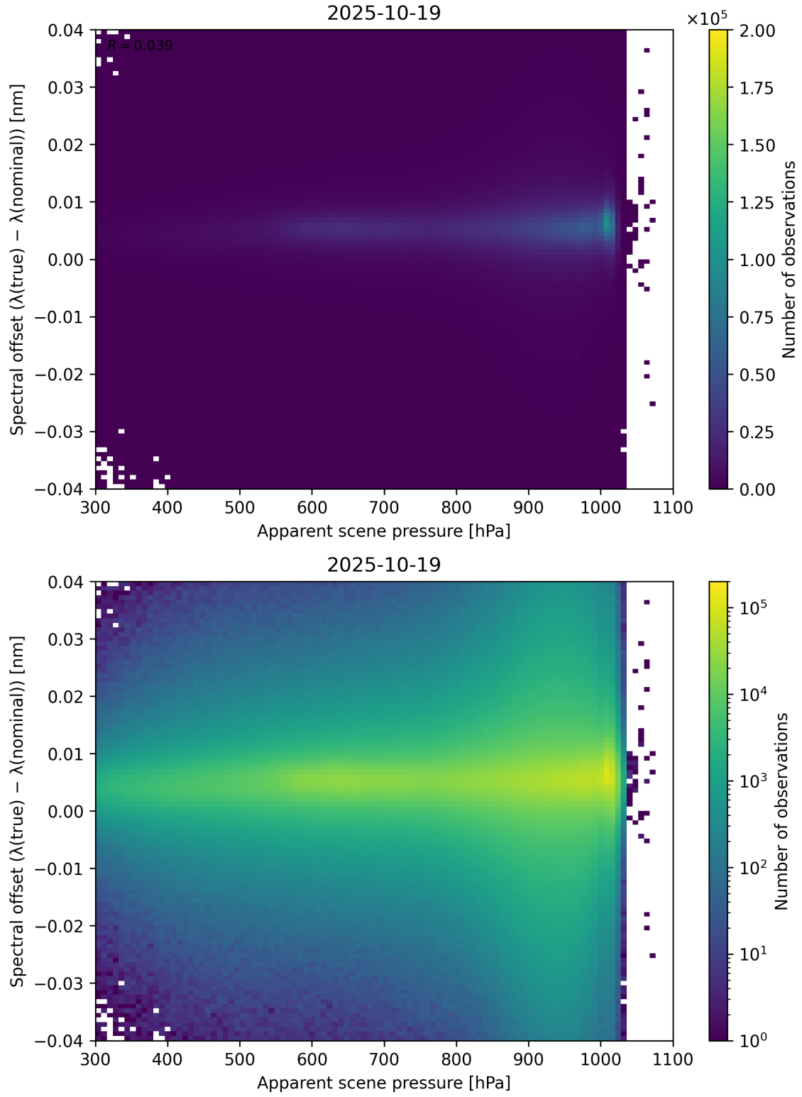
Figure 67: Scatter density plot of “Apparent scene pressure” against “Spectral offset ( \lambda_{\text{true}} - \lambda_{\text{nominal}} )” for 2025-10-18 to 2025-10-20.
