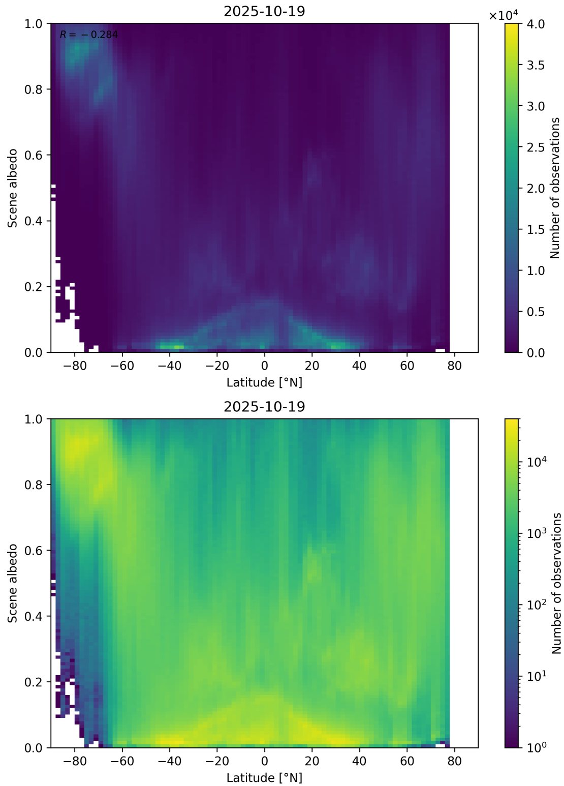
Figure 95: Scatter density plot of “Latitude” against “Scene albedo” for 2025-10-18 to 2025-10-20.
