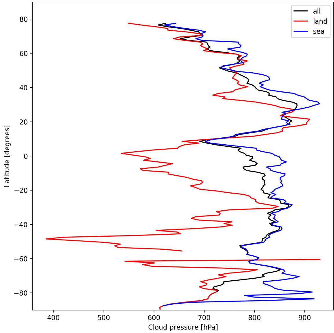
Figure 13: Zonal average of “Cloud pressure” for 2025-10-18 to 2025-10-20.
