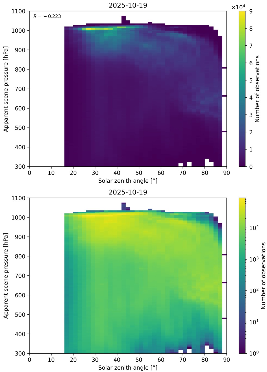
Figure 108: Scatter density plot of “Solar zenith angle” against “Apparent scene pressure” for 2025-10-18 to 2025-10-20.
