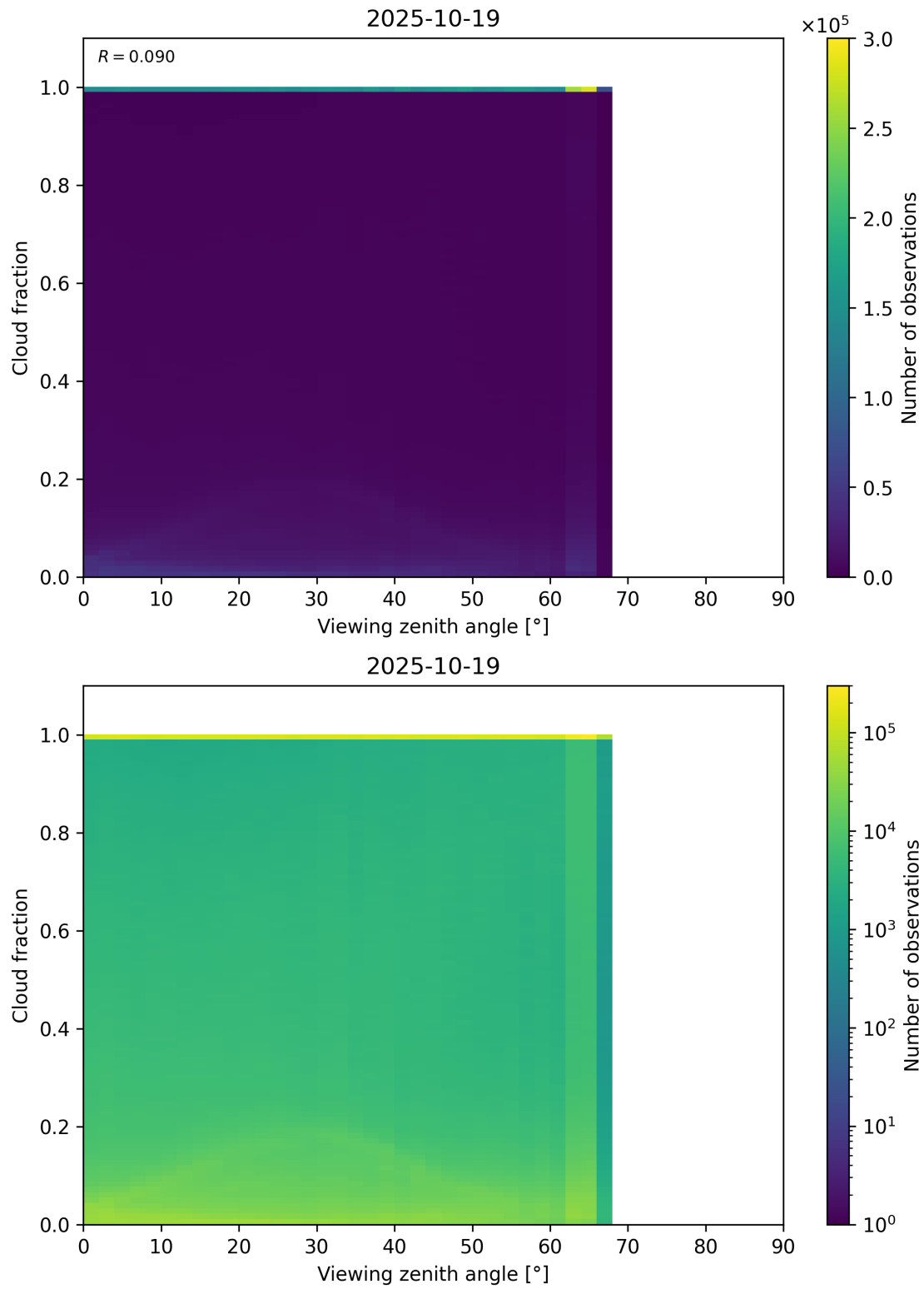
Figure 120: Scatter density plot of “Viewing zenith angle” against “Cloud fraction” for 2025-10-18 to 2025-10-20.
