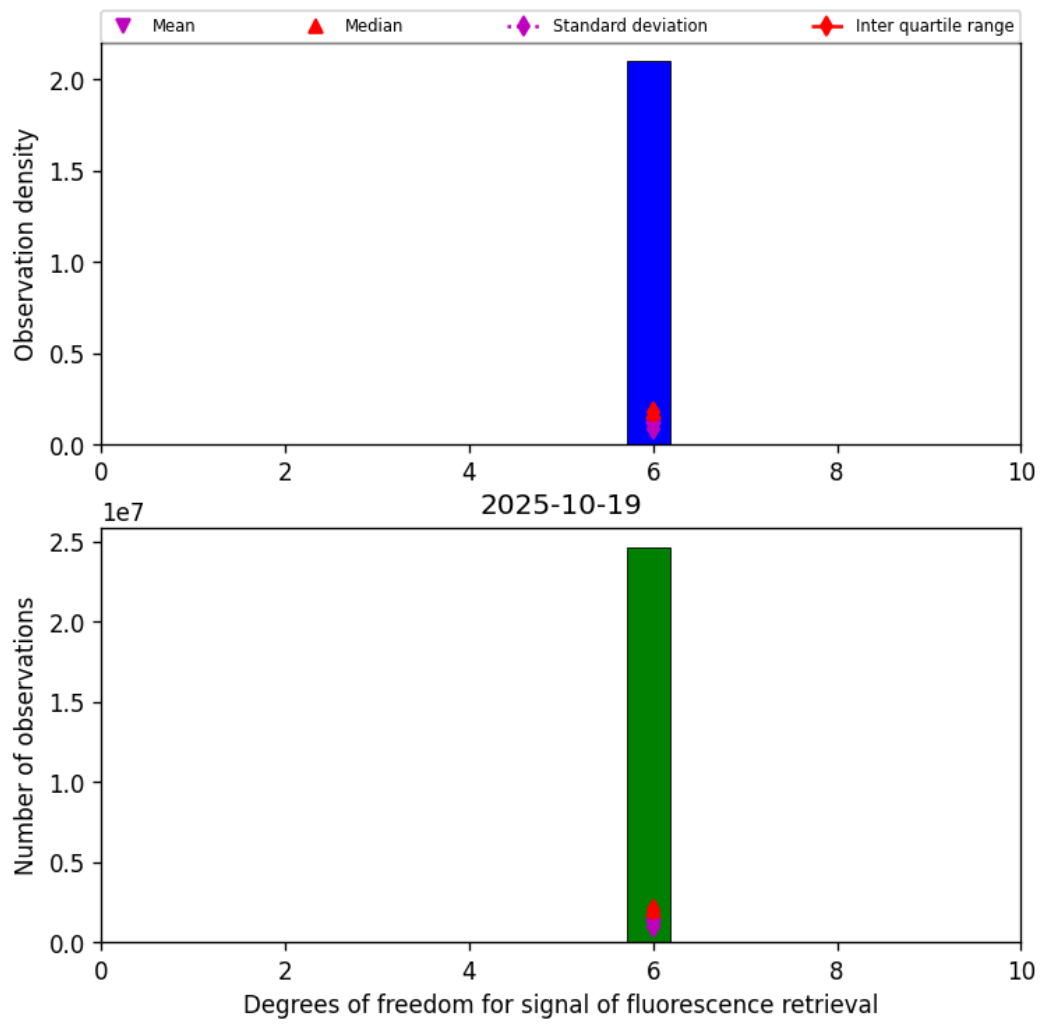
Figure 43: Histogram of "Degrees of freedom for signal of fluorescence retrieval" for 2025-10-18 to 2025-10-20
