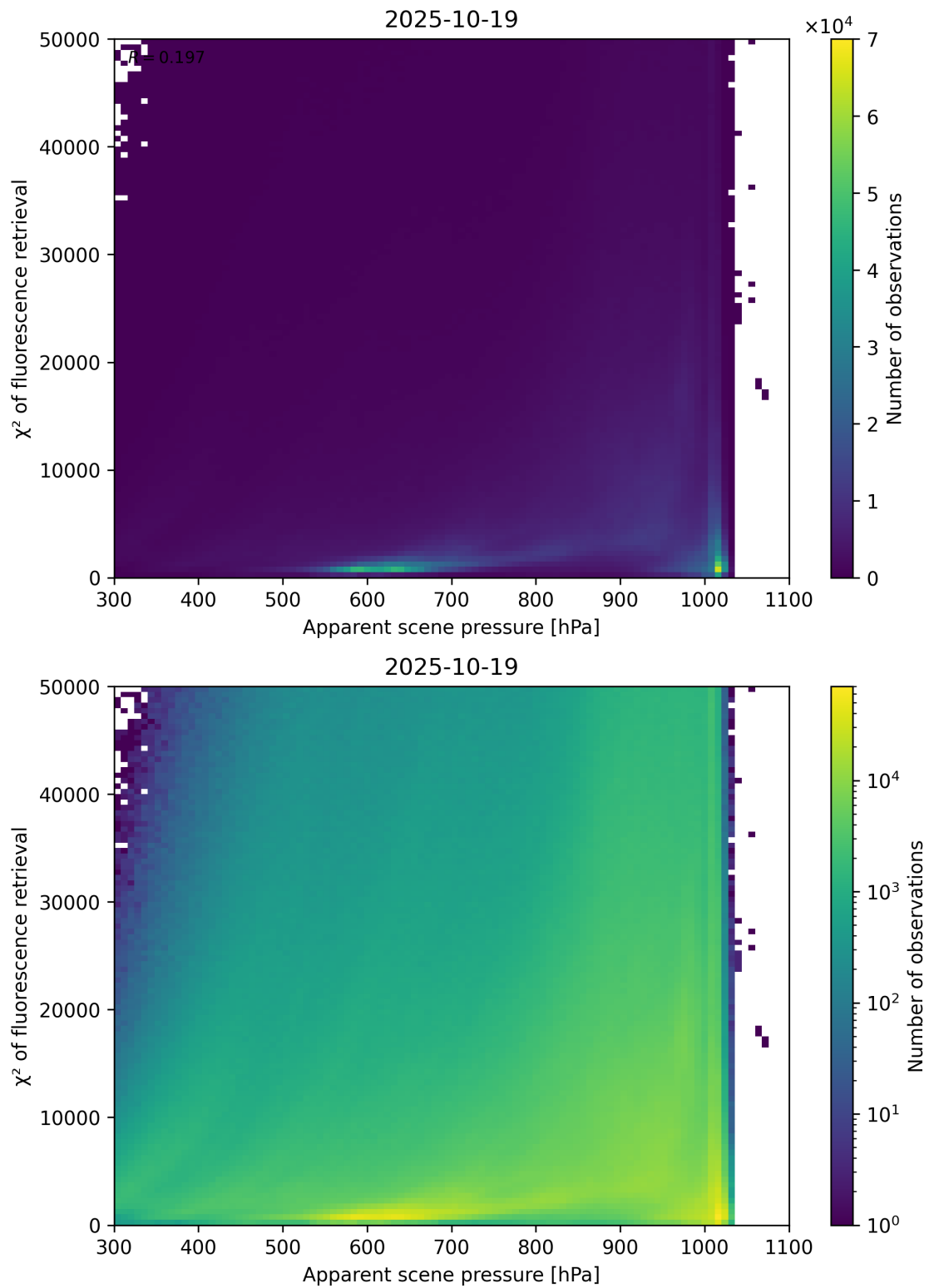
Figure 63: Scatter density plot of “Apparent scene pressure” against “ \chi^2 of fluorescence retrieval” for 2025-10-18 to 2025-10-20.
