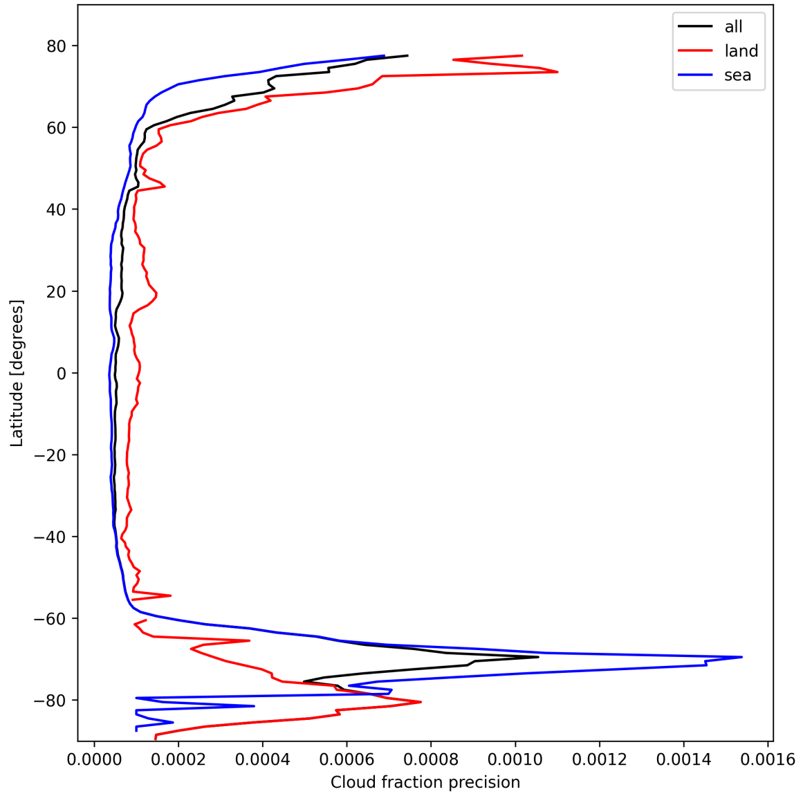
Figure 16: Zonal average of “Cloud fraction precision” for 2025-10-18 to 2025-10-20.
