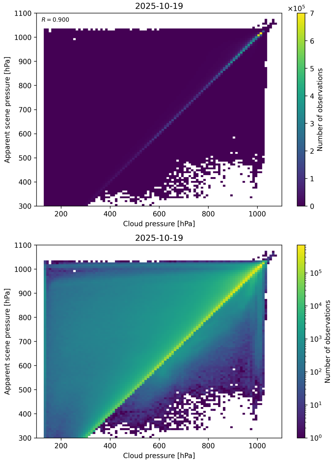
Figure 77: Scatter density plot of “Cloud pressure” against “Apparent scene pressure” for 2025-10-18 to 2025-10-20.
