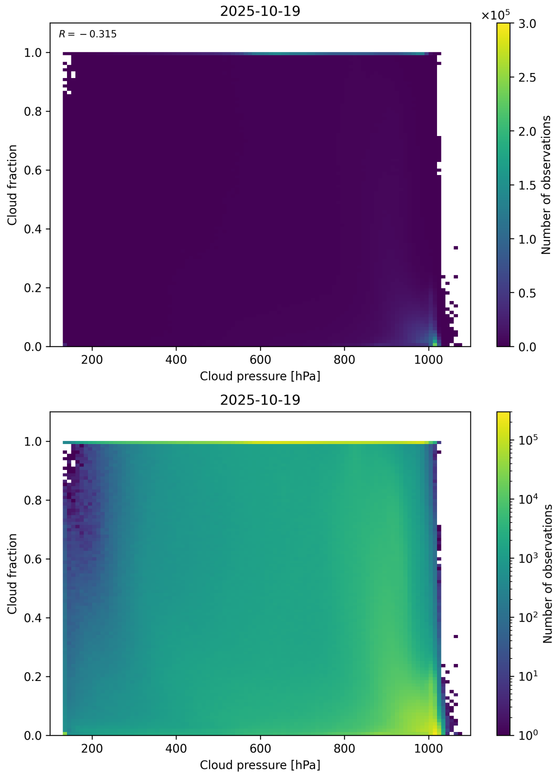
Figure 79: Scatter density plot of “Cloud pressure” against “Cloud fraction” for 2025-10-18 to 2025-10-20.
