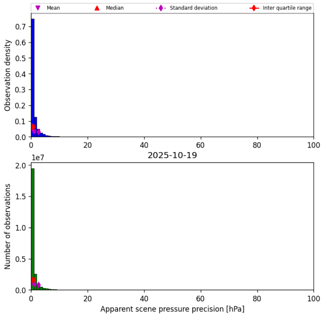
Figure 37: Histogram of “Apparent scene pressure precision” for 2025-10-18 to 2025-10-20
