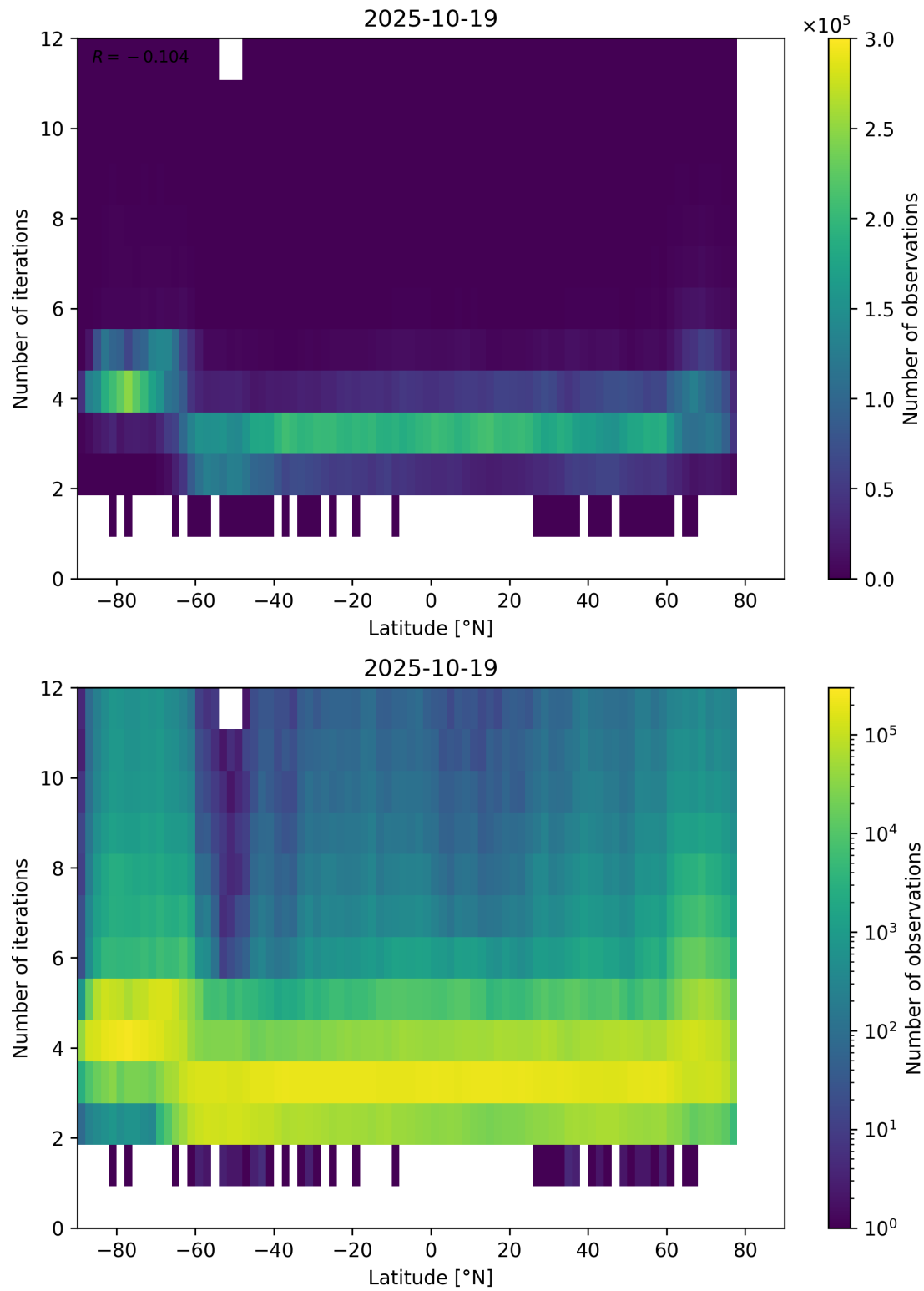
Figure 93: Scatter density plot of “Latitude” against “Number of iterations” for 2025-10-18 to 2025-10-20.
