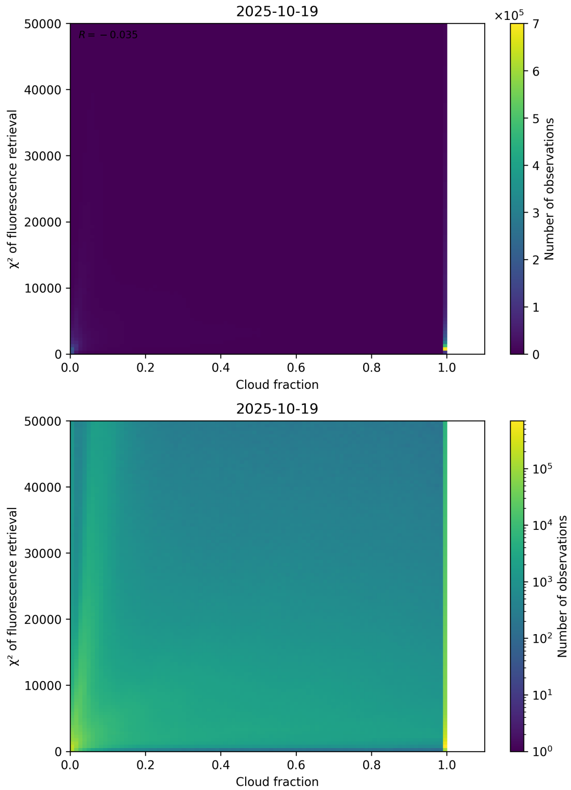
Figure 71: Scatter density plot of “Cloud fraction” against “ \chi^2 of fluorescence retrieval” for 2025-10-18 to 2025-10-20.
