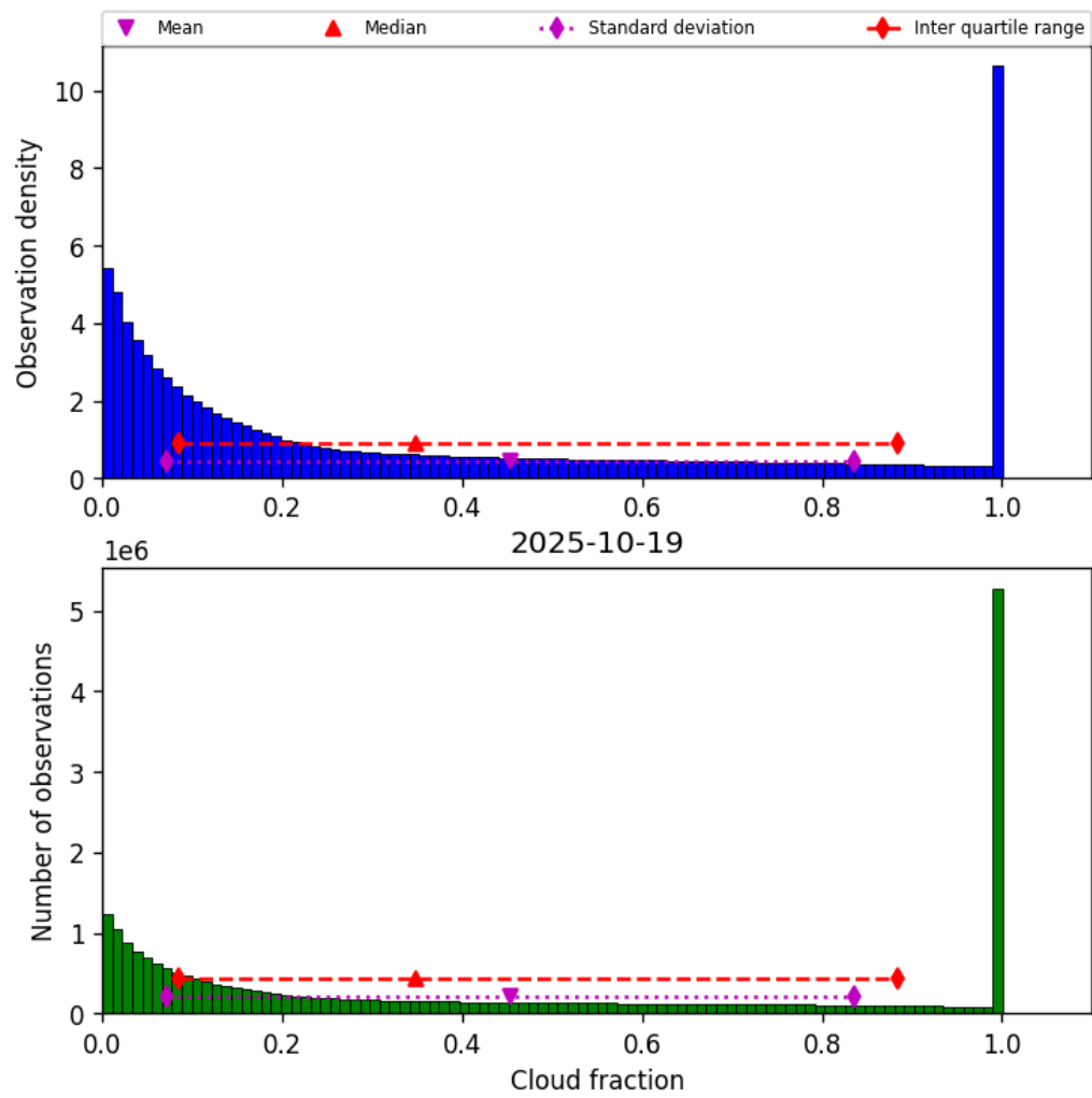
Figure 32: Histogram of “Cloud fraction” for 2025-10-18 to 2025-10-20
