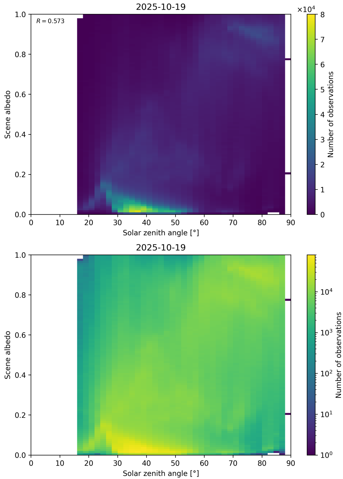
Figure 116: Scatter density plot of “Solar zenith angle” against “Scene albedo” for 2025-10-18 to 2025-10-20.
