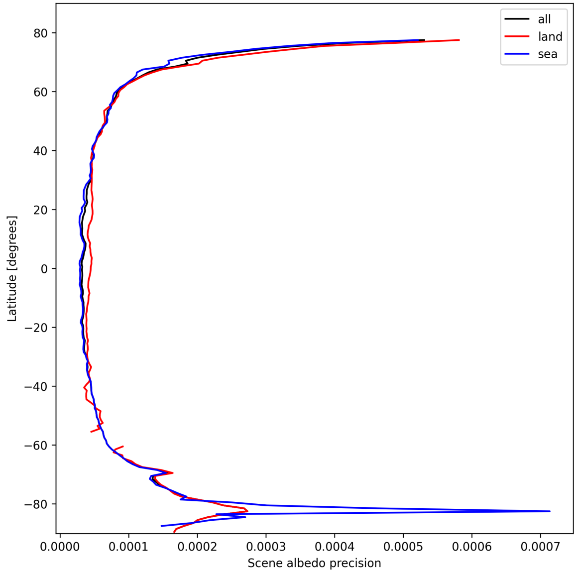
Figure 18: Zonal average of “Scene albedo precision” for 2025-10-18 to 2025-10-20.
