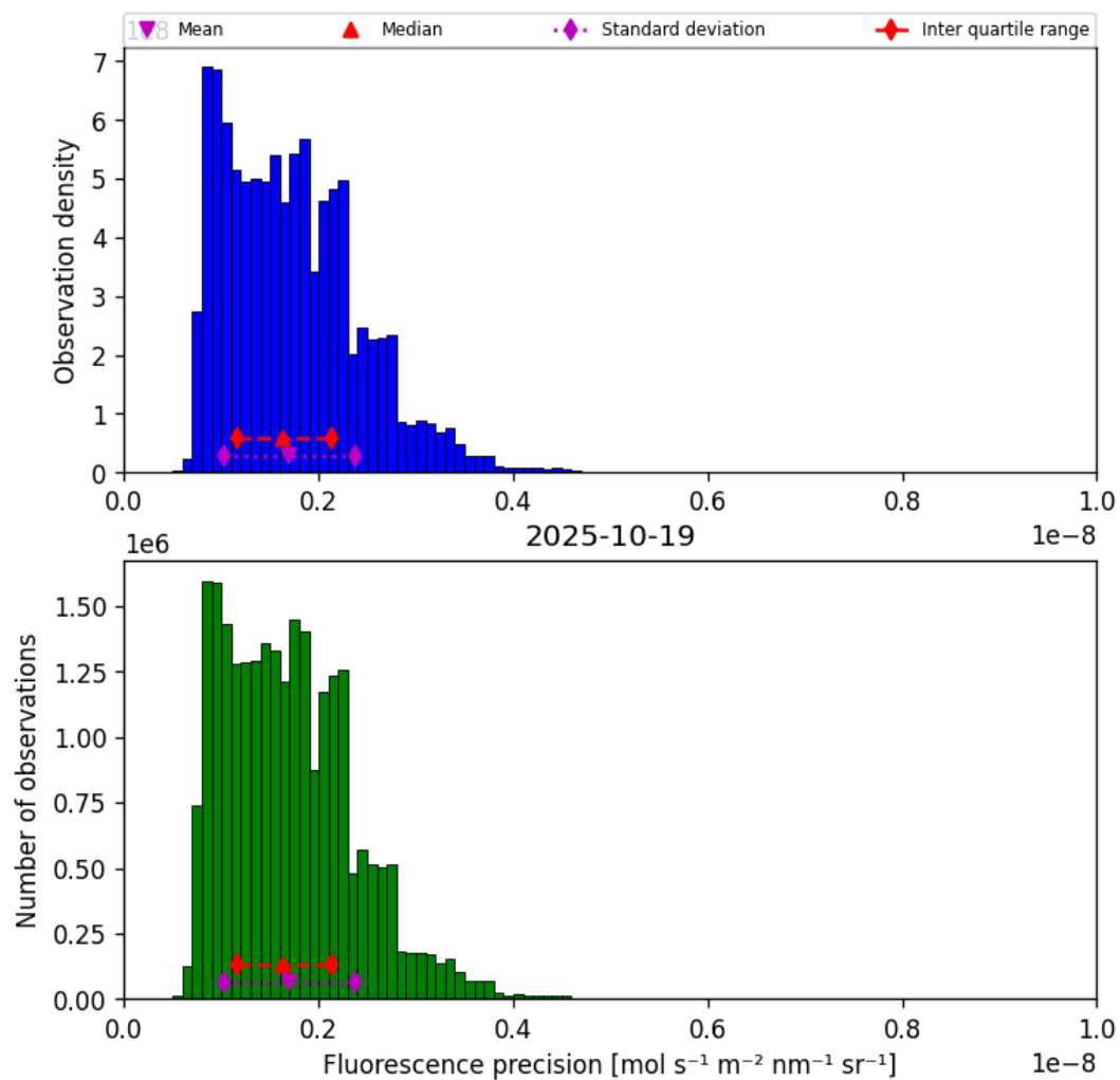
Figure 41: Histogram of “Fluorescence precision” for 2025-10-18 to 2025-10-20
