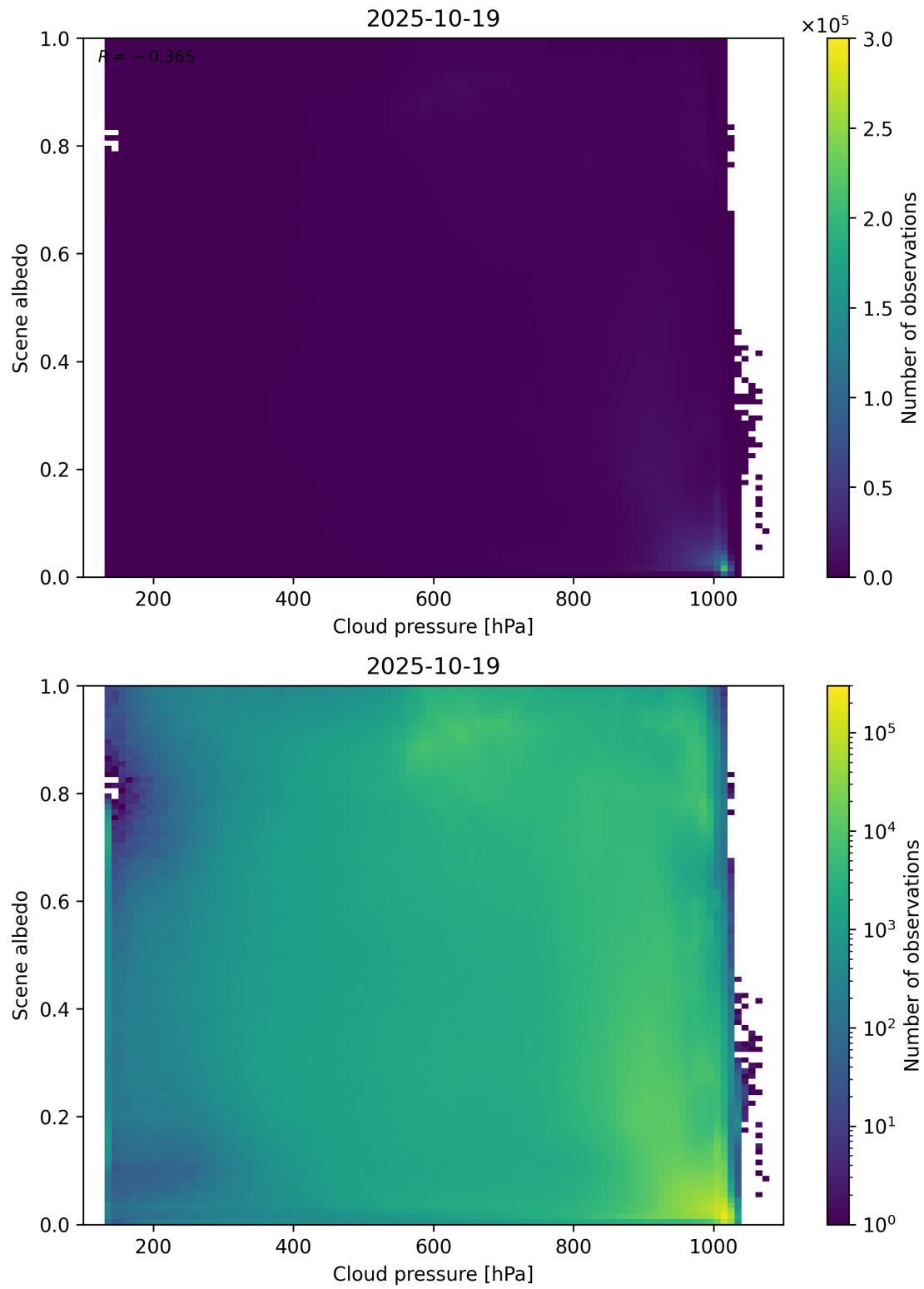
Figure 83: Scatter density plot of “Cloud pressure” against “Scene albedo” for 2025-10-18 to 2025-10-20.
