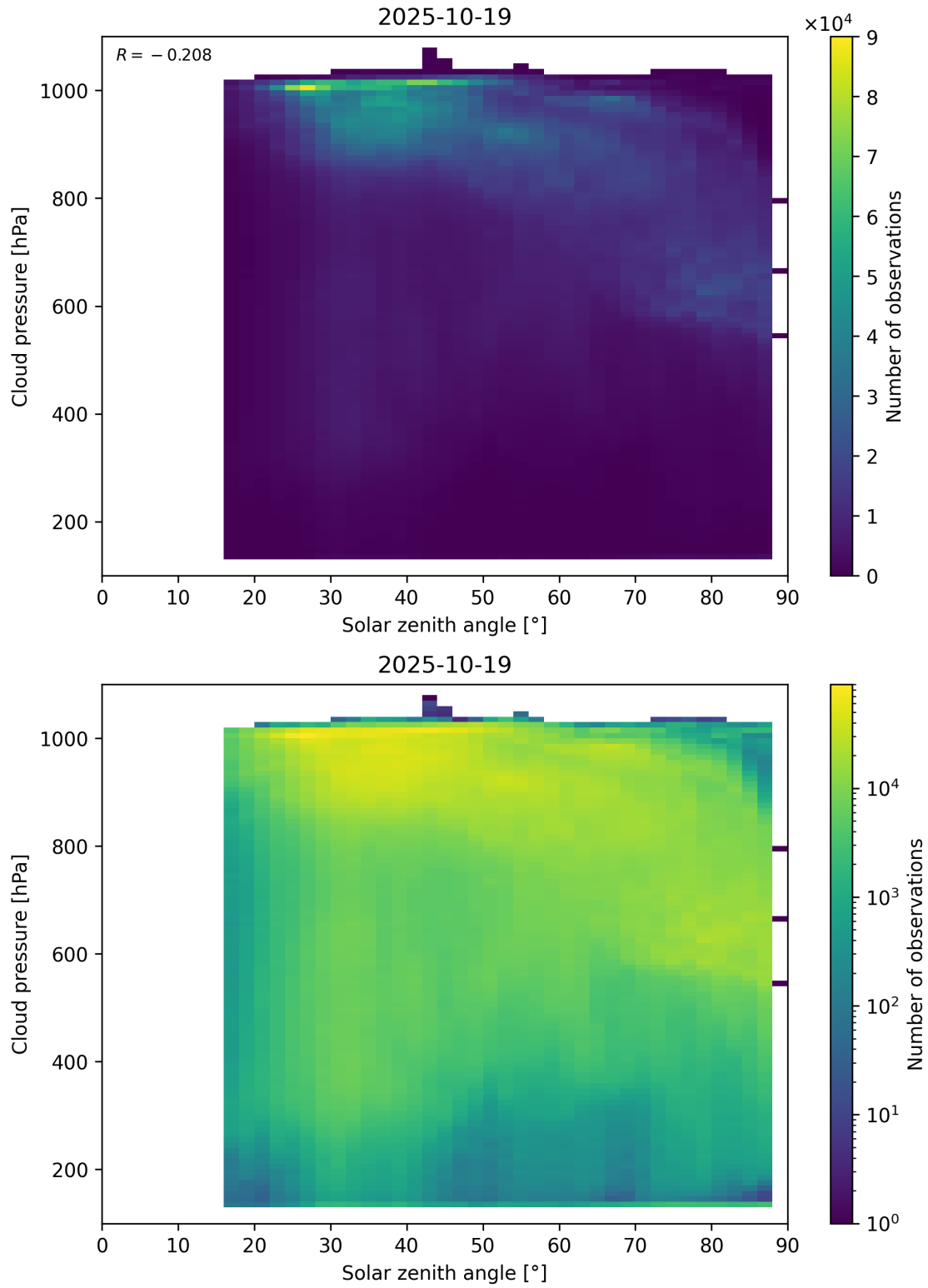
Figure 111: Scatter density plot of “Solar zenith angle” against “Cloud pressure” for 2025-10-18 to 2025-10-20.
