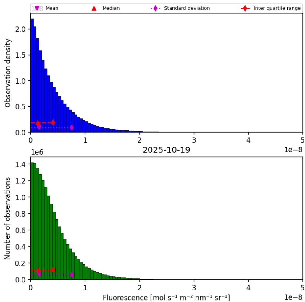
Figure 40: Histogram of “Fluorescence” for 2025-10-18 to 2025-10-20
