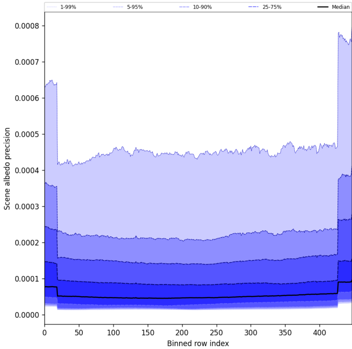
Figure 52: Along track statistics of “Scene albedo precision” for 2025-10-18 to 2025-10-20
