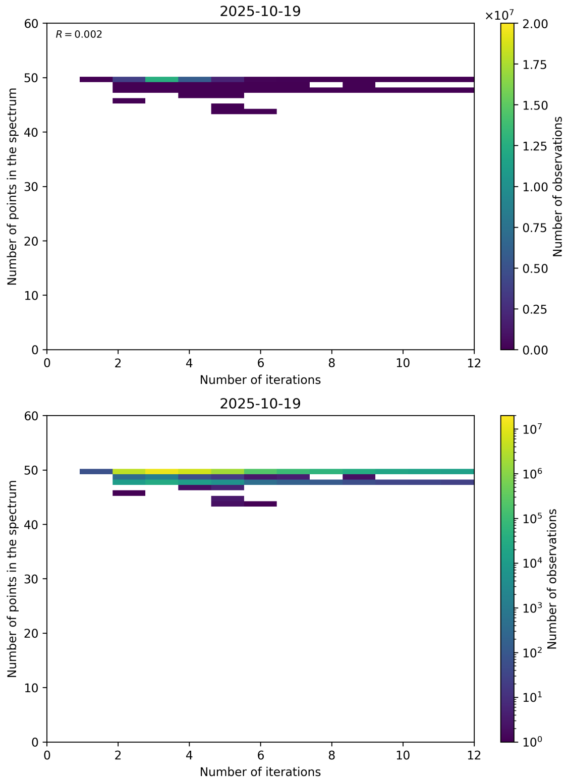
Figure 99: Scatter density plot of “Number of iterations” against “Number of points in the spectrum” for 2025-10-18 to 2025-10-20.
