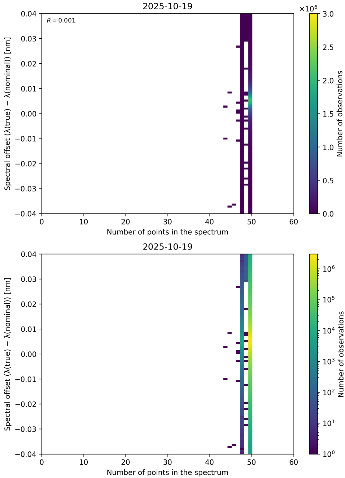
Figure 101: Scatter density plot of “Number of points in the spectrum” against “Spectral offset ( \lambda_{\text{true}} - \lambda_{\text{nominal}} )” for 2025-10-18 to 2025-10-20.
