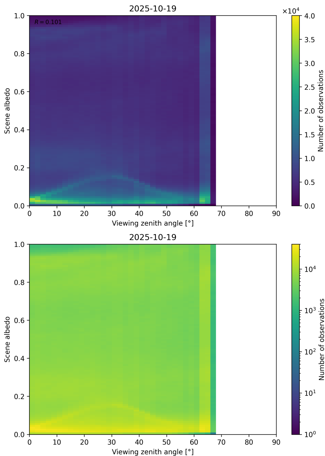
Figure 126: Scatter density plot of “Viewing zenith angle” against “Scene albedo” for 2025-10-18 to 2025-10-20.
