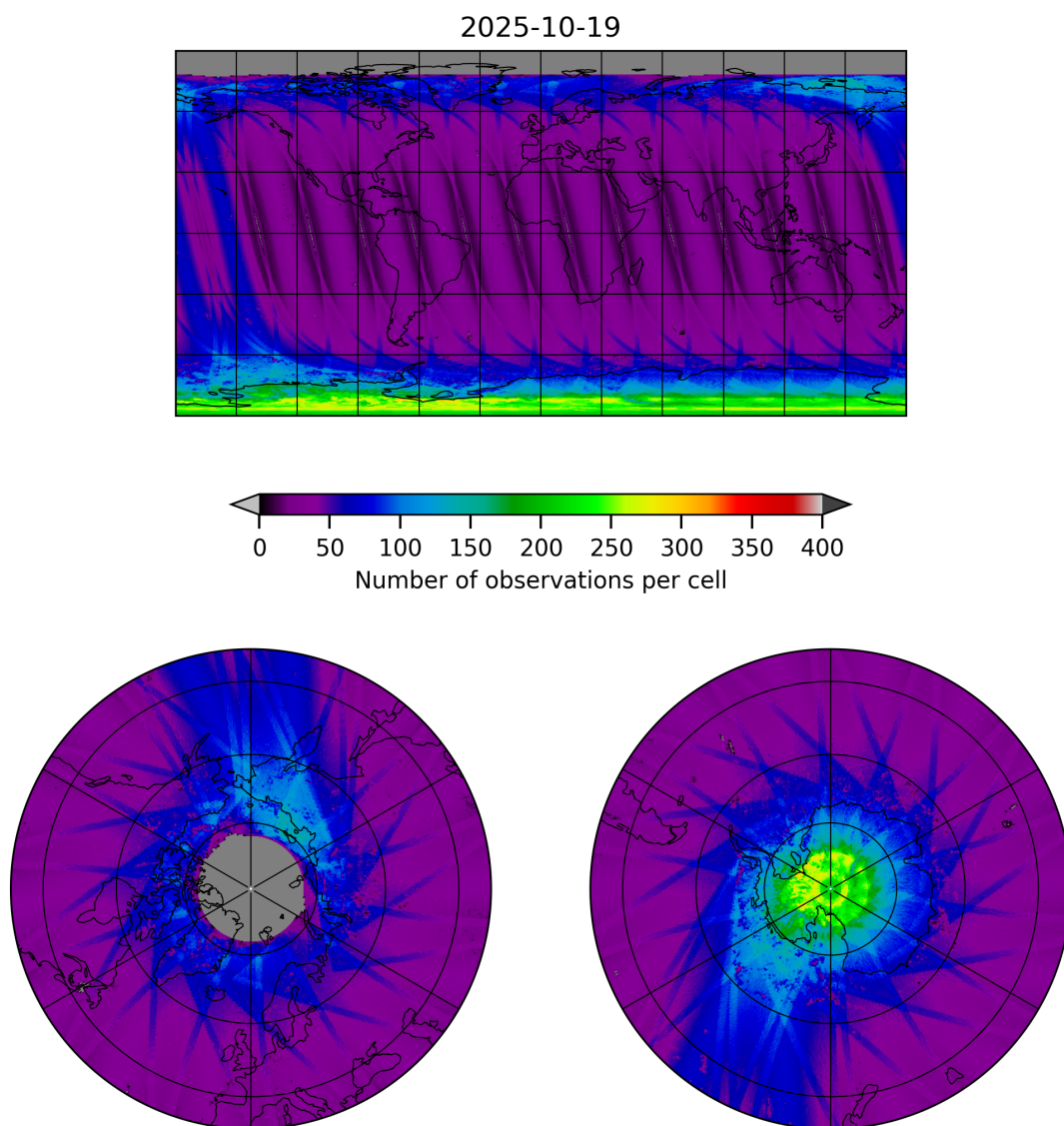
Figure 11: Map of the number of observations for 2025-10-18 to 2025-10-20
