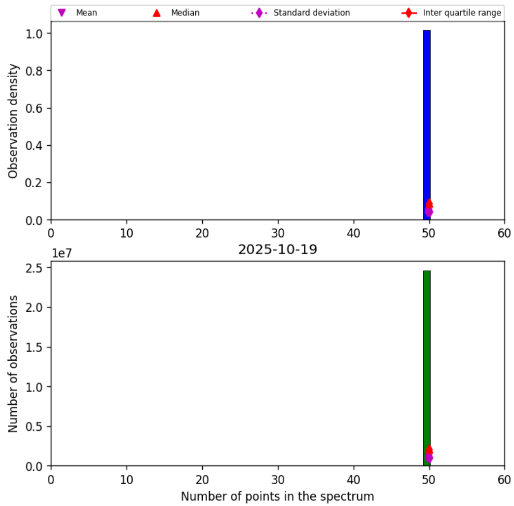
Figure 44: Histogram of “Number of points in the spectrum” for 2025-10-18 to 2025-10-20
