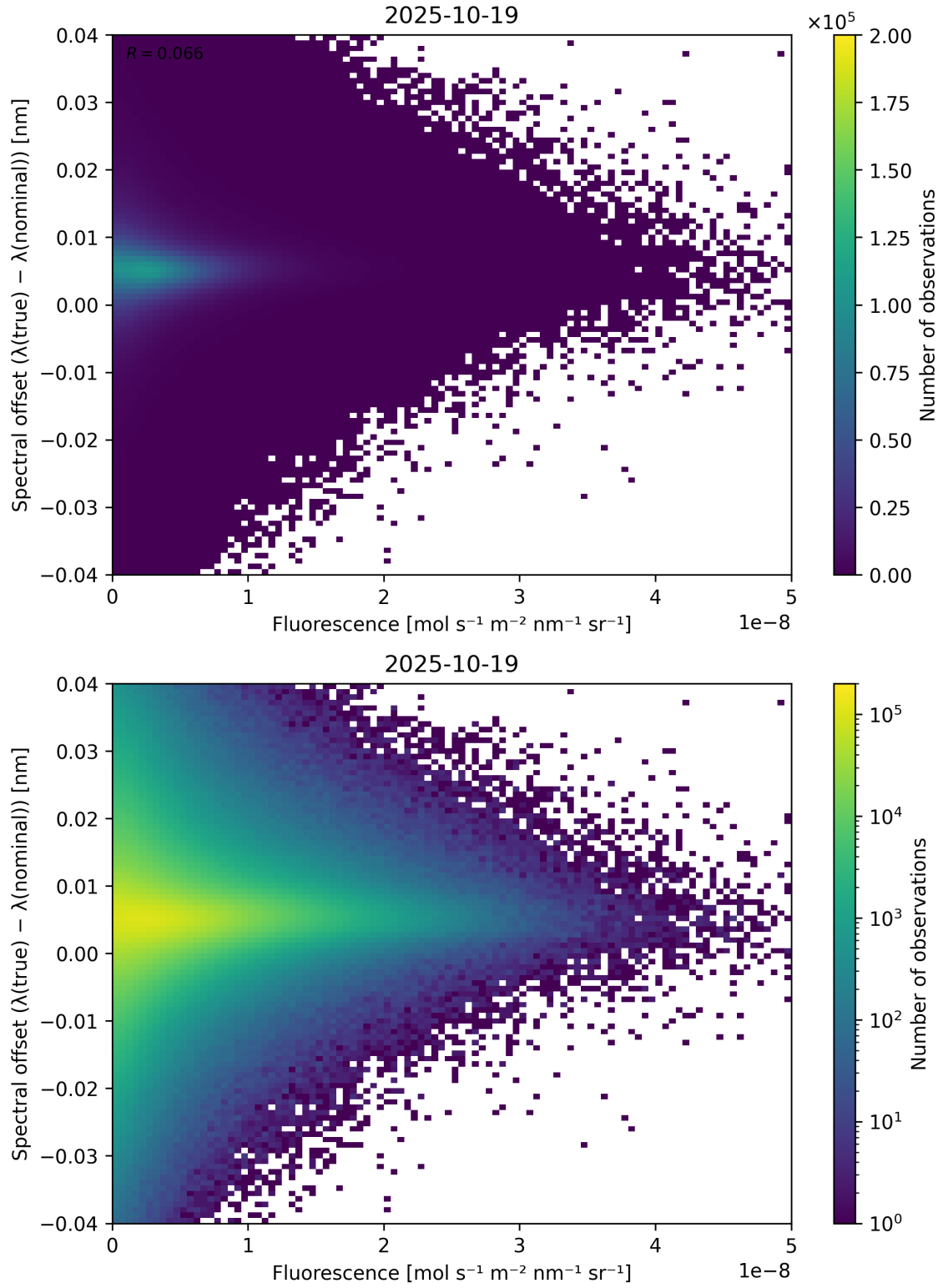
Figure 87: Scatter density plot of “Fluorescence” against “Spectral offset ( \lambda_{\text{true}} - \lambda_{\text{nominal}} )” for 2025-10-18 to 2025-10-20.
