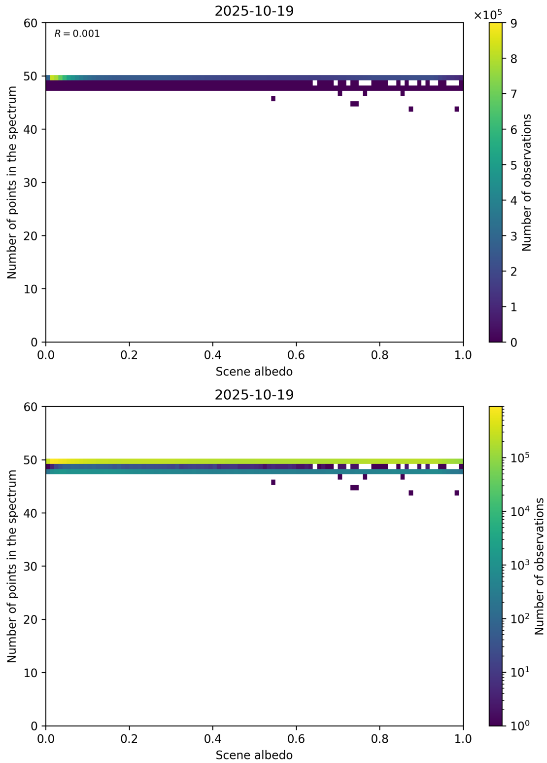
Figure 106: Scatter density plot of “Scene albedo” against “Number of points in the spectrum” for 2025-10-18 to 2025-10-20.
