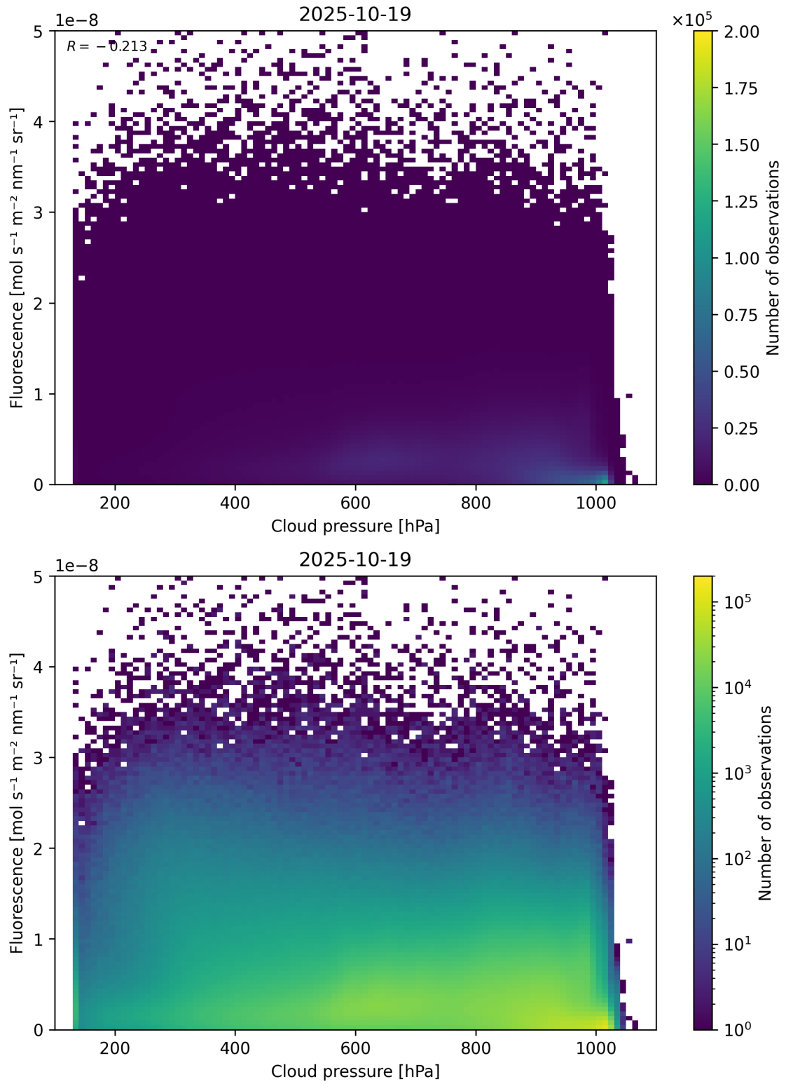
Figure 80: Scatter density plot of “Cloud pressure” against “Fluorescence” for 2025-10-18 to 2025-10-20.
