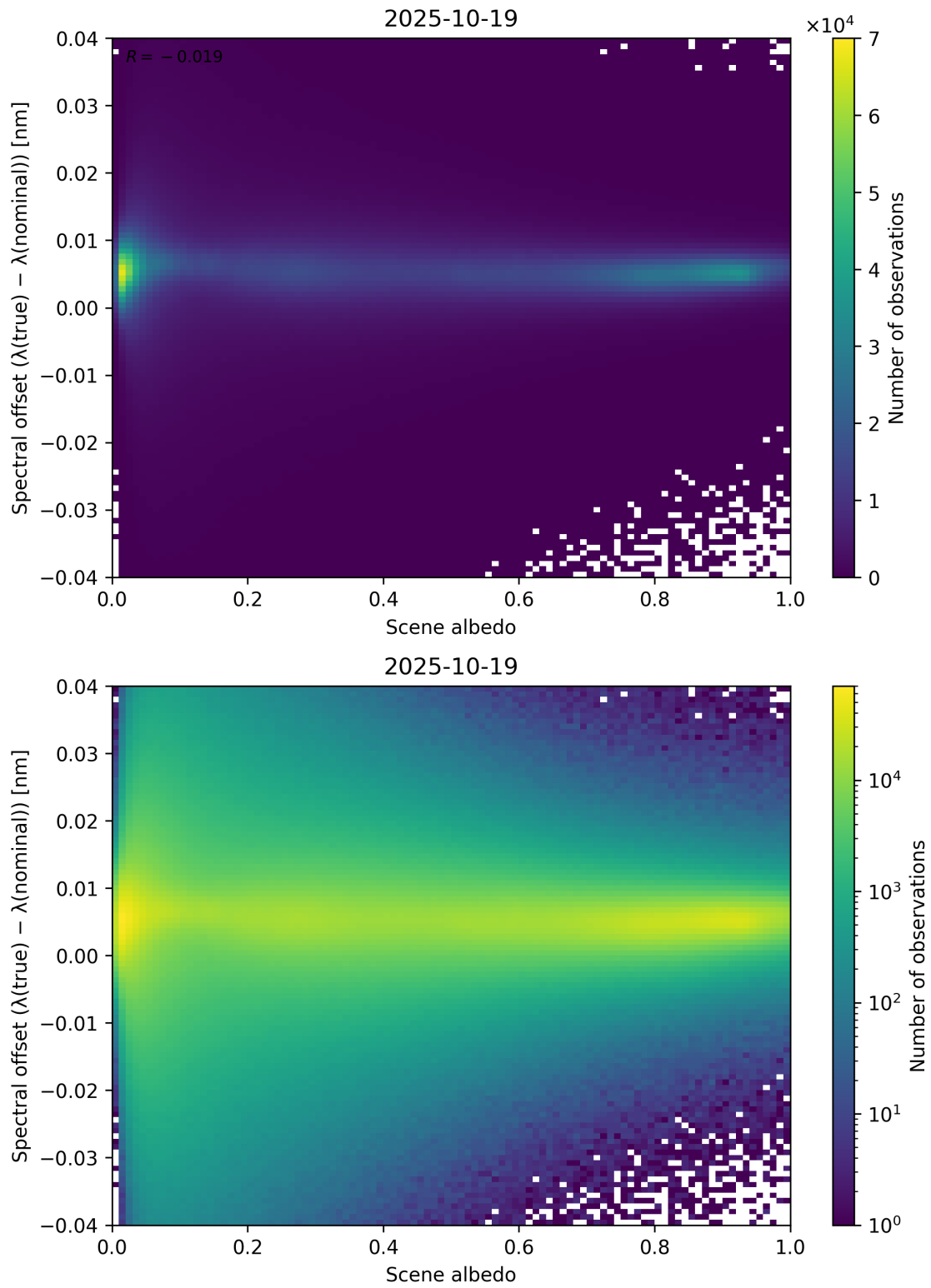
Figure 107: Scatter density plot of “Scene albedo” against “Spectral offset ( \lambda_{\text{true}} - \lambda_{\text{nominal}} )” for 2025-10-18 to 2025-10-20.
