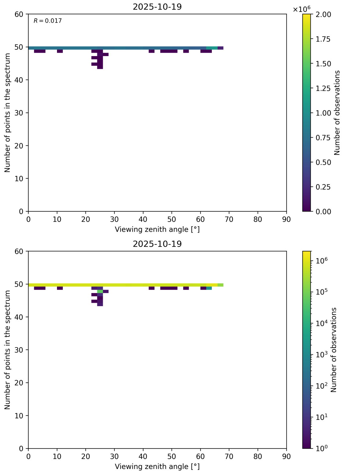
Figure 125: Scatter density plot of “Viewing zenith angle” against “Number of points in the spectrum” for 2025-10-18 to 2025-10-20.
