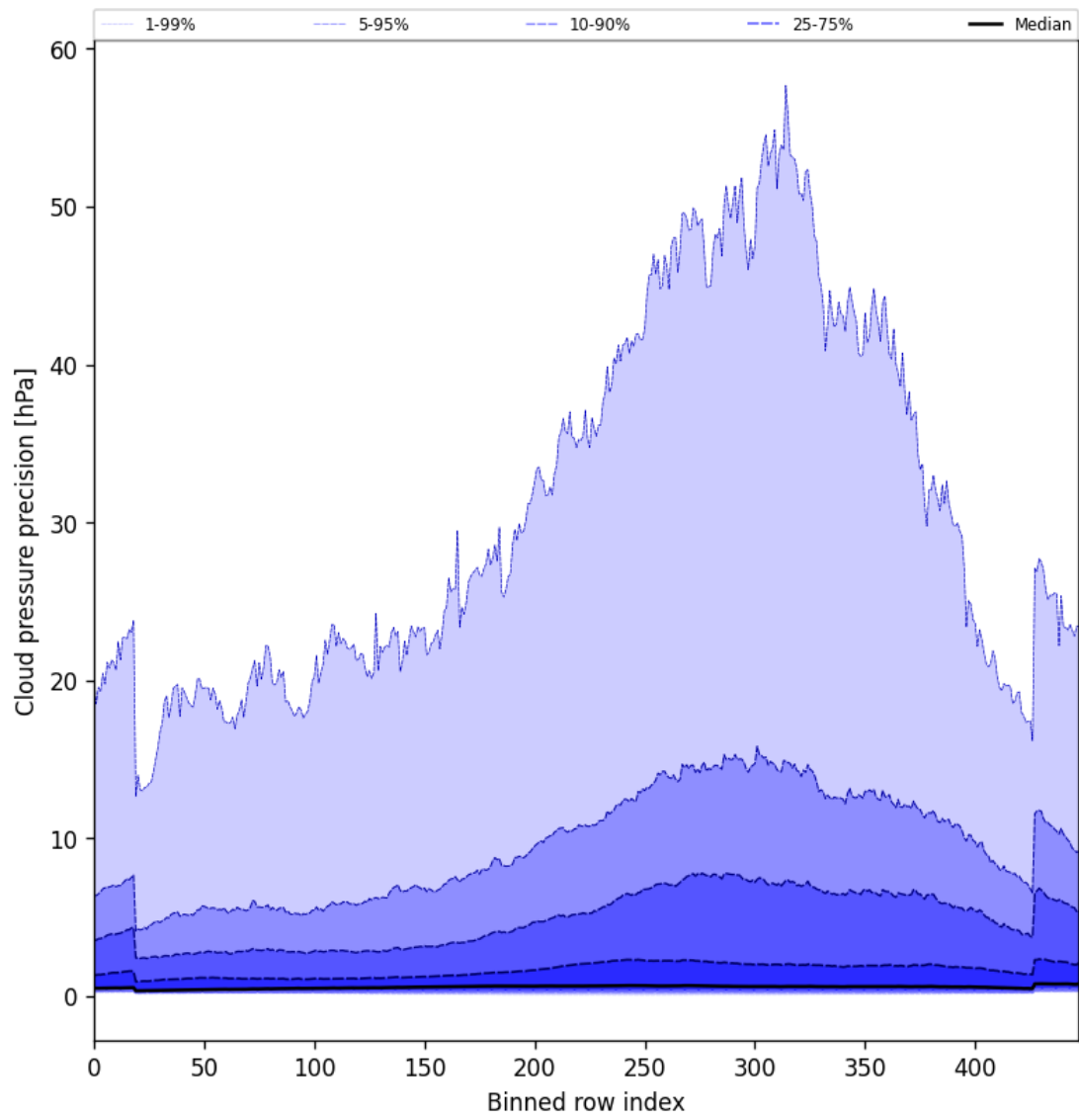
Figure 48: Along track statistics of “Cloud pressure precision” for 2025-10-18 to 2025-10-20
