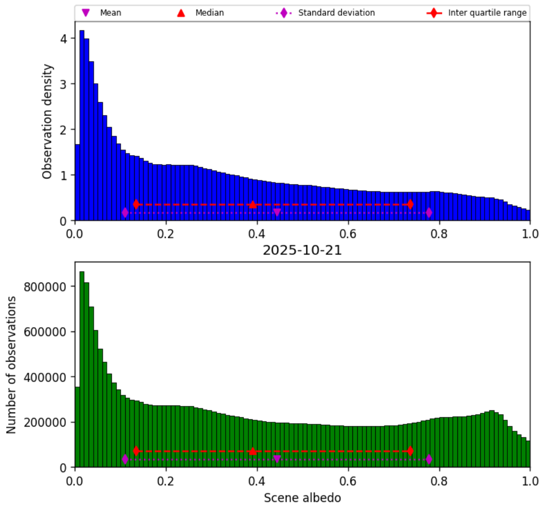
Figure 34: Histogram of “Scene albedo” for 2025-10-20 to 2025-10-22
