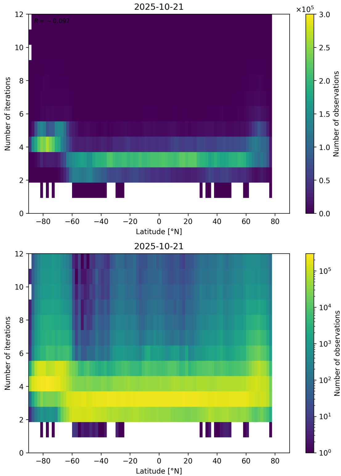
Figure 93: Scatter density plot of “Latitude” against “Number of iterations” for 2025-10-20 to 2025-10-22.
