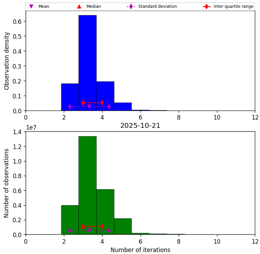
Figure 39: Histogram of “Number of iterations” for 2025-10-20 to 2025-10-22
