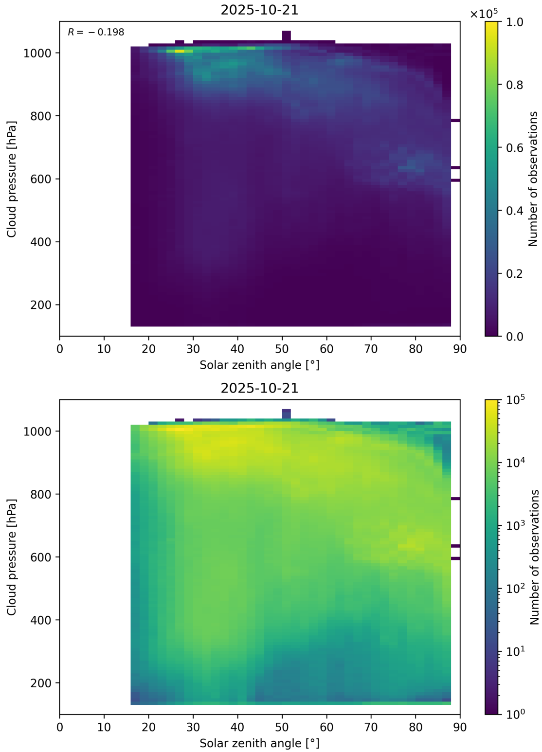
Figure 111: Scatter density plot of “Solar zenith angle” against “Cloud pressure” for 2025-10-20 to 2025-10-22.
