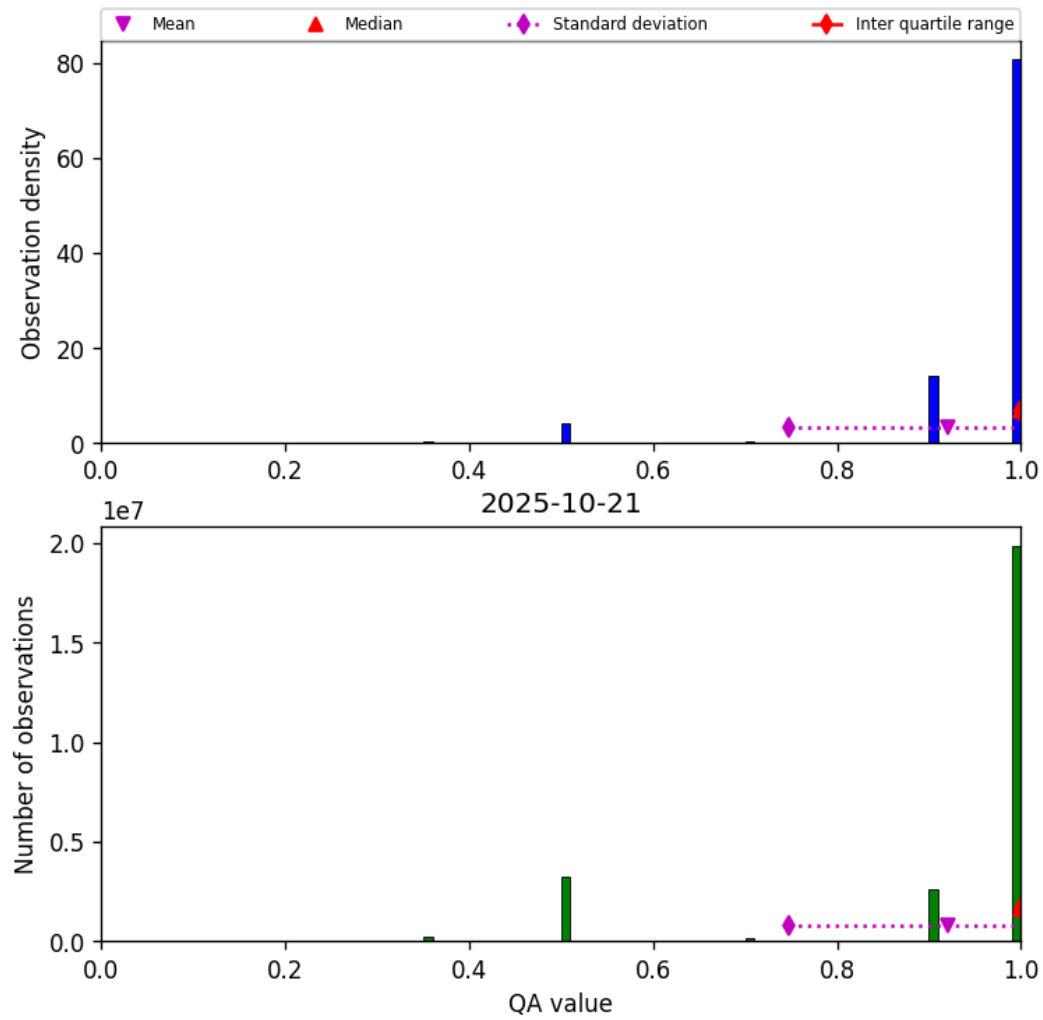
Figure 29: Histogram of “QA value” for 2025-10-20 to 2025-10-22
