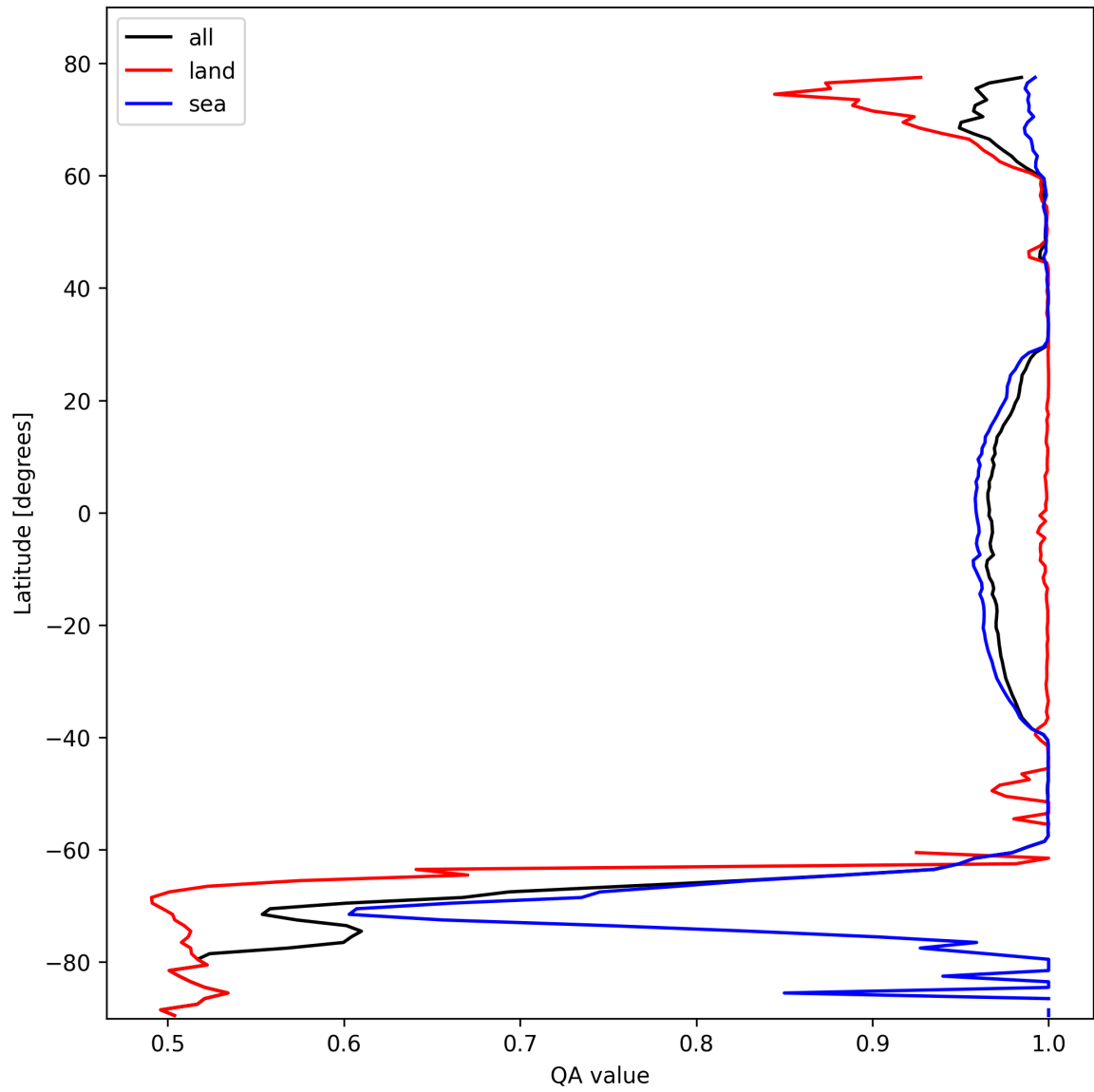
Figure 12: Zonal average of “QA value” for 2025-10-20 to 2025-10-22.
