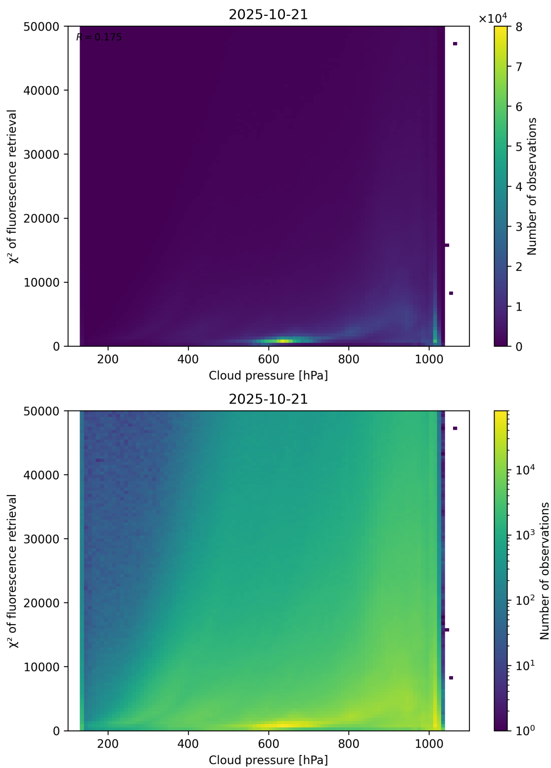
Figure 78: Scatter density plot of “Cloud pressure” against “ \chi^2 of fluorescence retrieval” for 2025-10-20 to 2025-10-22.
