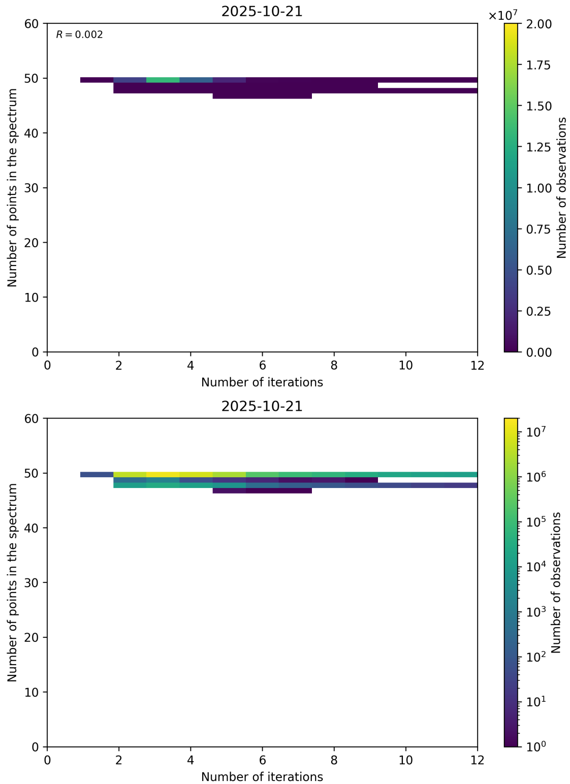
Figure 99: Scatter density plot of “Number of iterations” against “Number of points in the spectrum” for 2025-10-20 to 2025-10-22.
