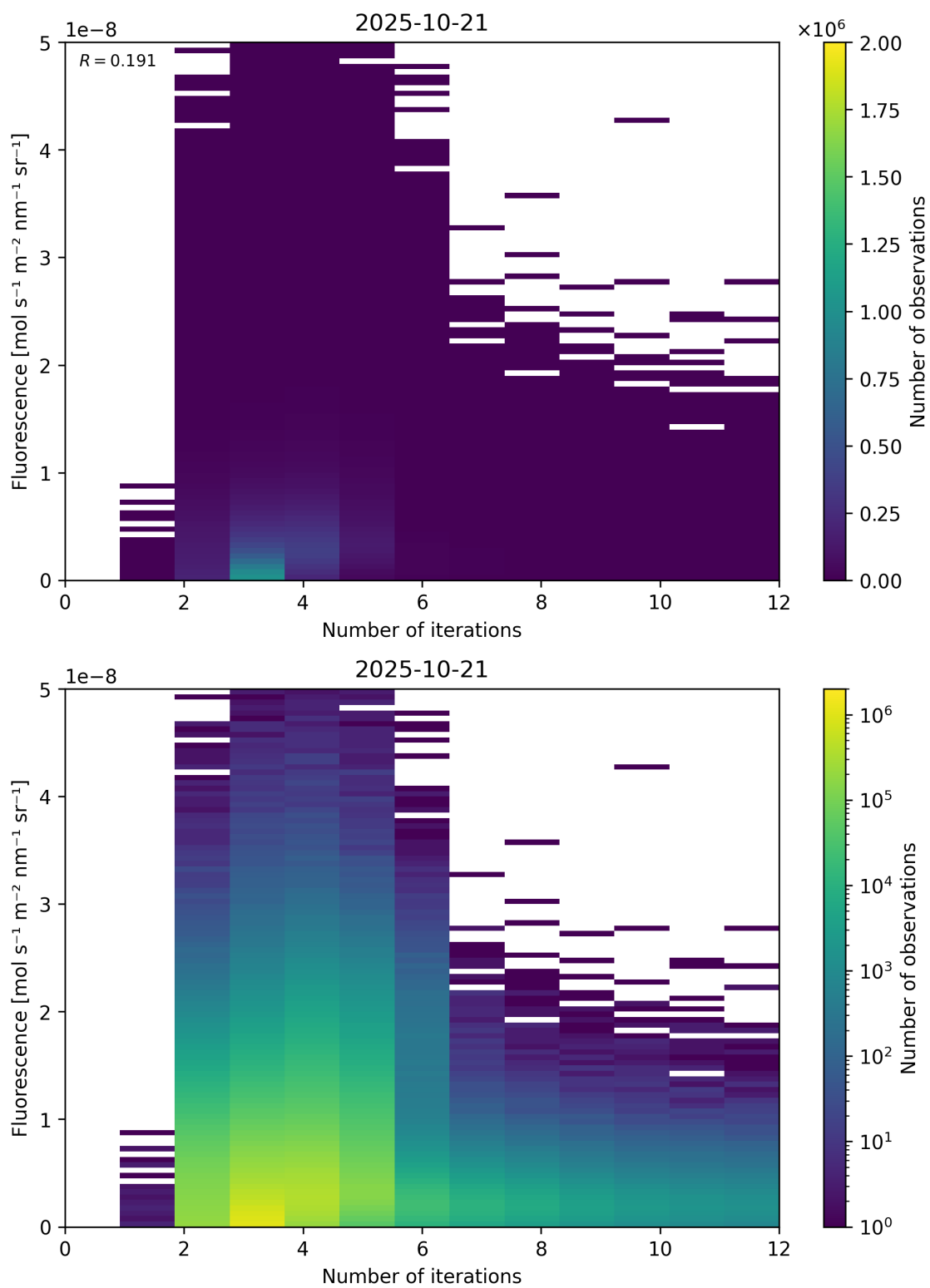
Figure 98: Scatter density plot of “Number of iterations” against “Fluorescence” for 2025-10-20 to 2025-10-22.
