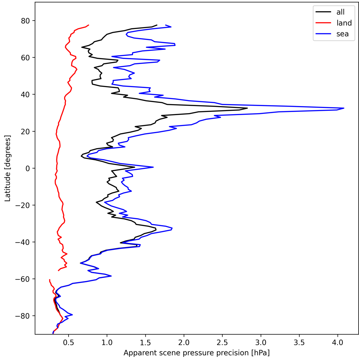
Figure 20: Zonal average of “Apparent scene pressure precision” for 2025-10-20 to 2025-10-22.
