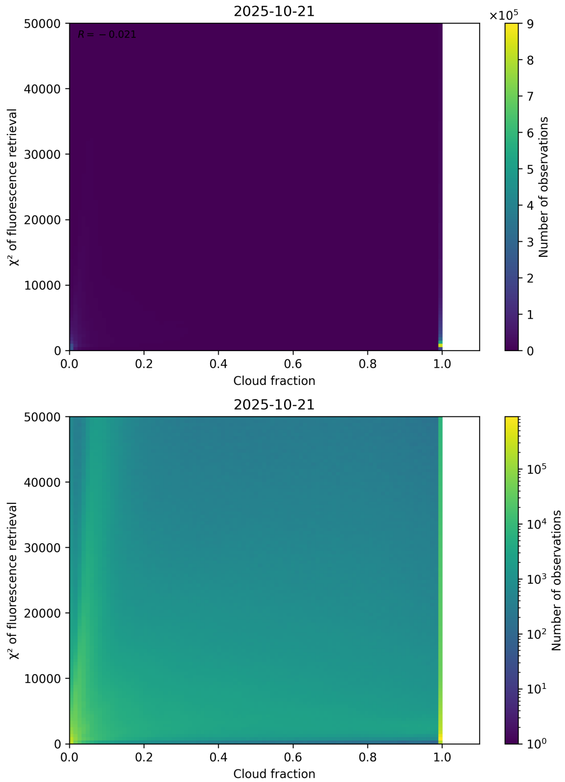
Figure 71: Scatter density plot of “Cloud fraction” against “ \chi^2 of fluorescence retrieval” for 2025-10-20 to 2025-10-22.
