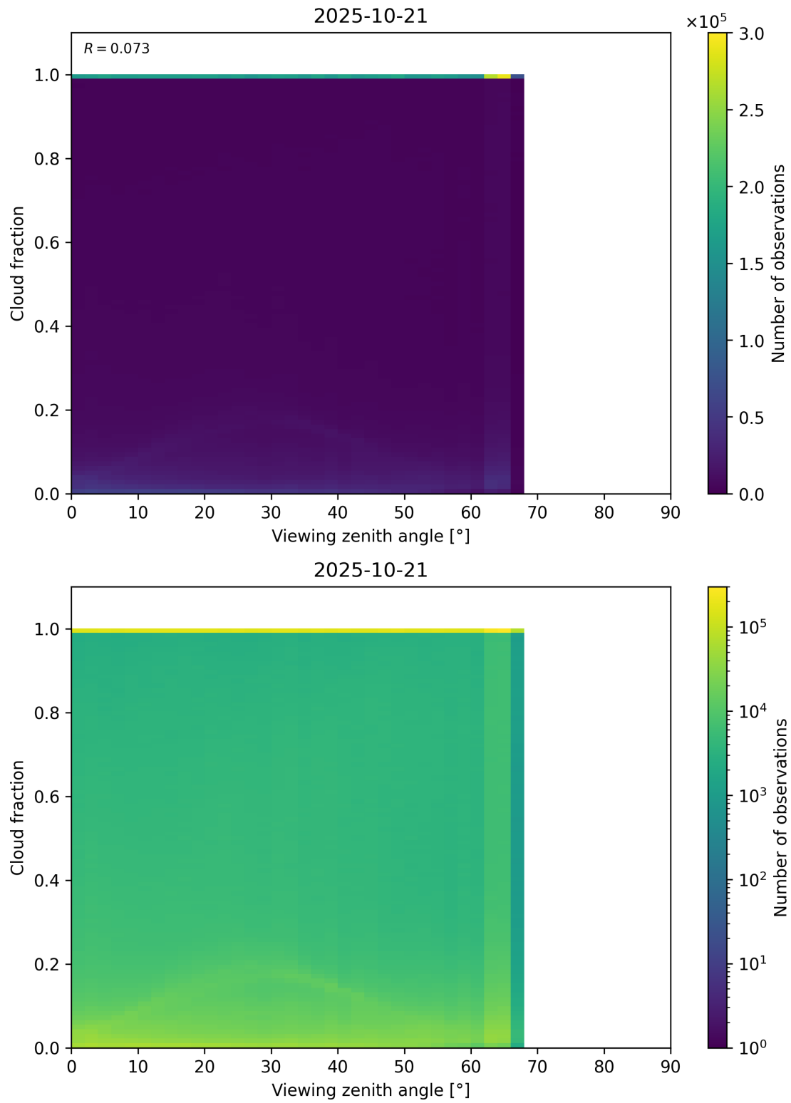
Figure 120: Scatter density plot of “Viewing zenith angle” against “Cloud fraction” for 2025-10-20 to 2025-10-22.
