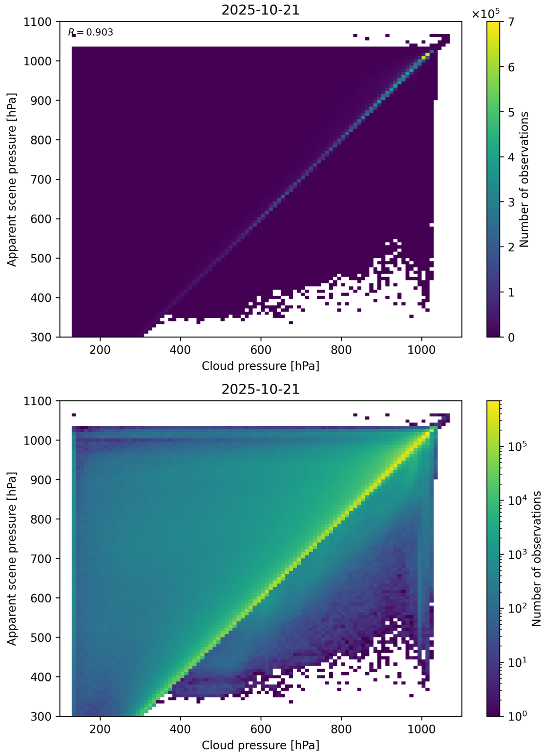
Figure 77: Scatter density plot of “Cloud pressure” against “Apparent scene pressure” for 2025-10-20 to 2025-10-22.
