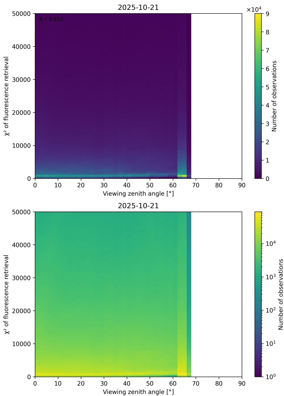
Figure 119: Scatter density plot of “Viewing zenith angle” against “ \chi^2 of fluorescence retrieval” for 2025-10-20 to 2025-10-22.
