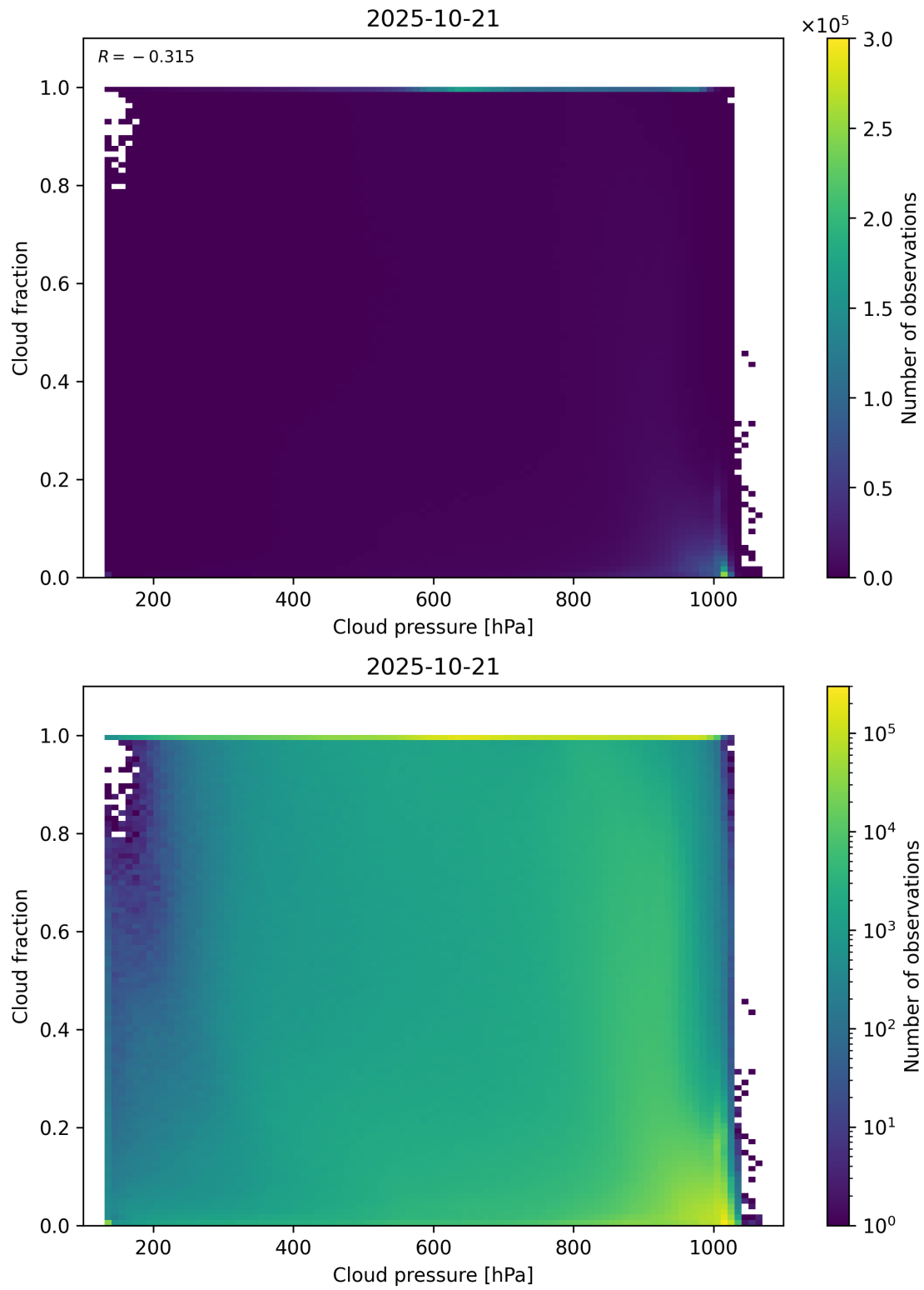
Figure 79: Scatter density plot of “Cloud pressure” against “Cloud fraction” for 2025-10-20 to 2025-10-22.
