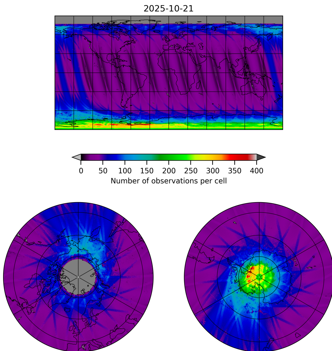
Figure 11: Map of the number of observations for 2025-10-20 to 2025-10-22
