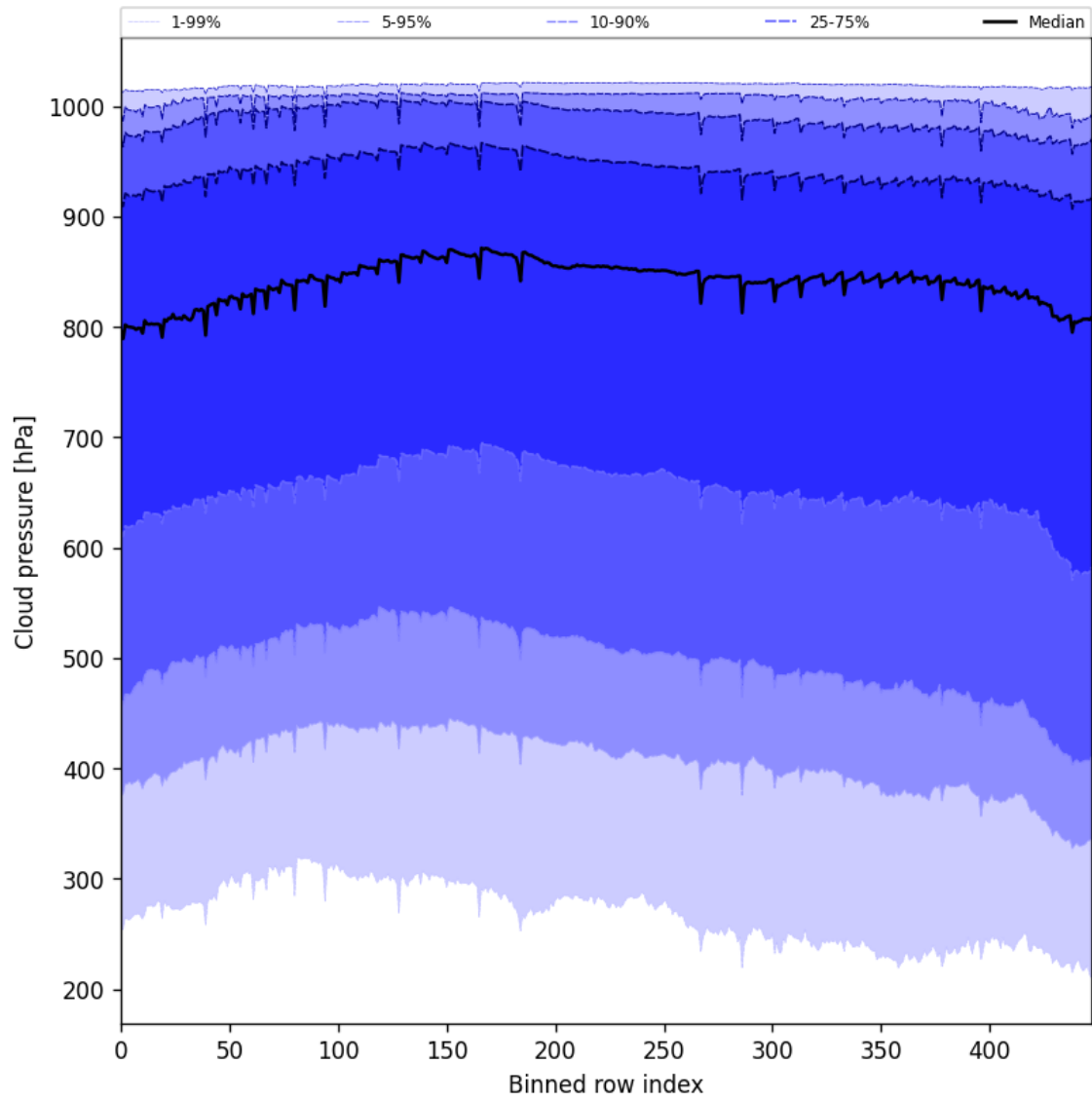
Figure 47: Along track statistics of “Cloud pressure” for 2025-10-20 to 2025-10-22
