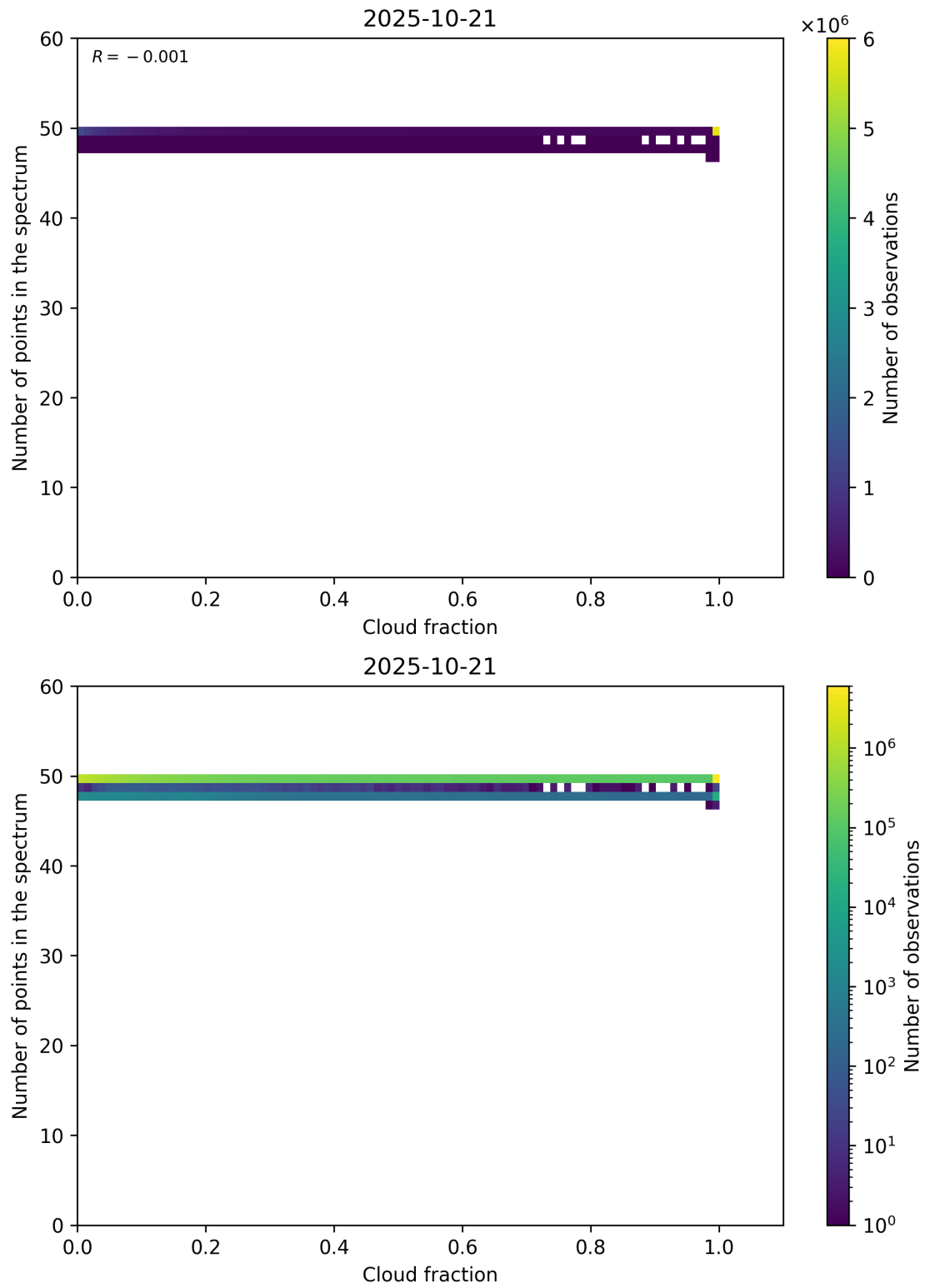
Figure 74: Scatter density plot of “Cloud fraction” against “Number of points in the spectrum” for 2025-10-20 to 2025-10-22.
