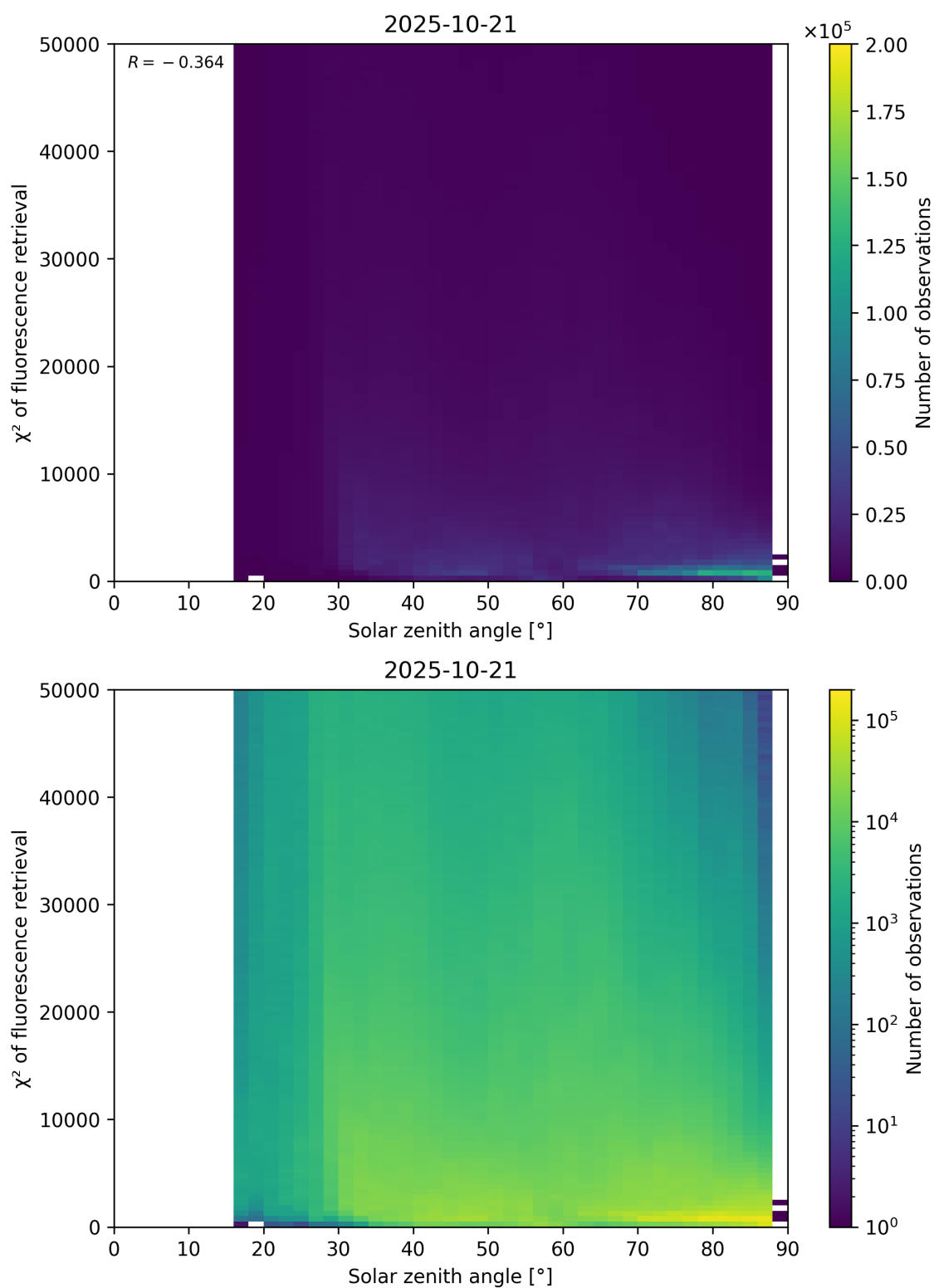
Figure 109: Scatter density plot of “Solar zenith angle” against “ \chi^2 of fluorescence retrieval” for 2025-10-20 to 2025-10-22.
