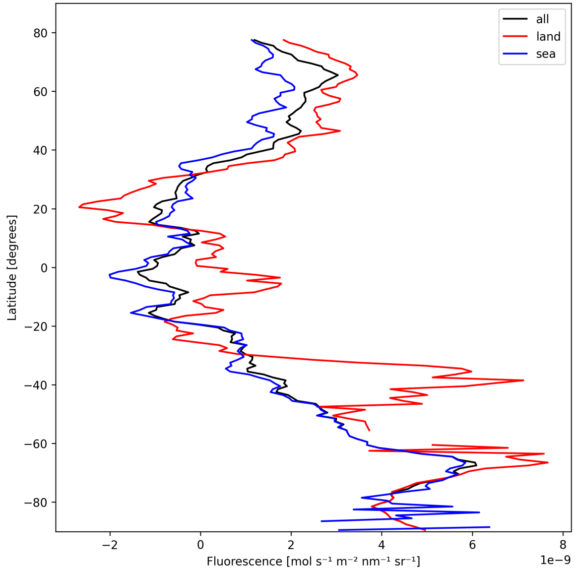
Figure 23: Zonal average of “Fluorescence” for 2025-10-20 to 2025-10-22.
