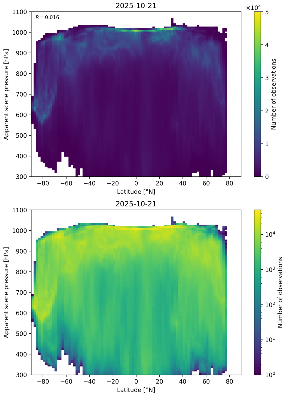
Figure 88: Scatter density plot of “Latitude” against “Apparent scene pressure” for 2025-10-20 to 2025-10-22.
