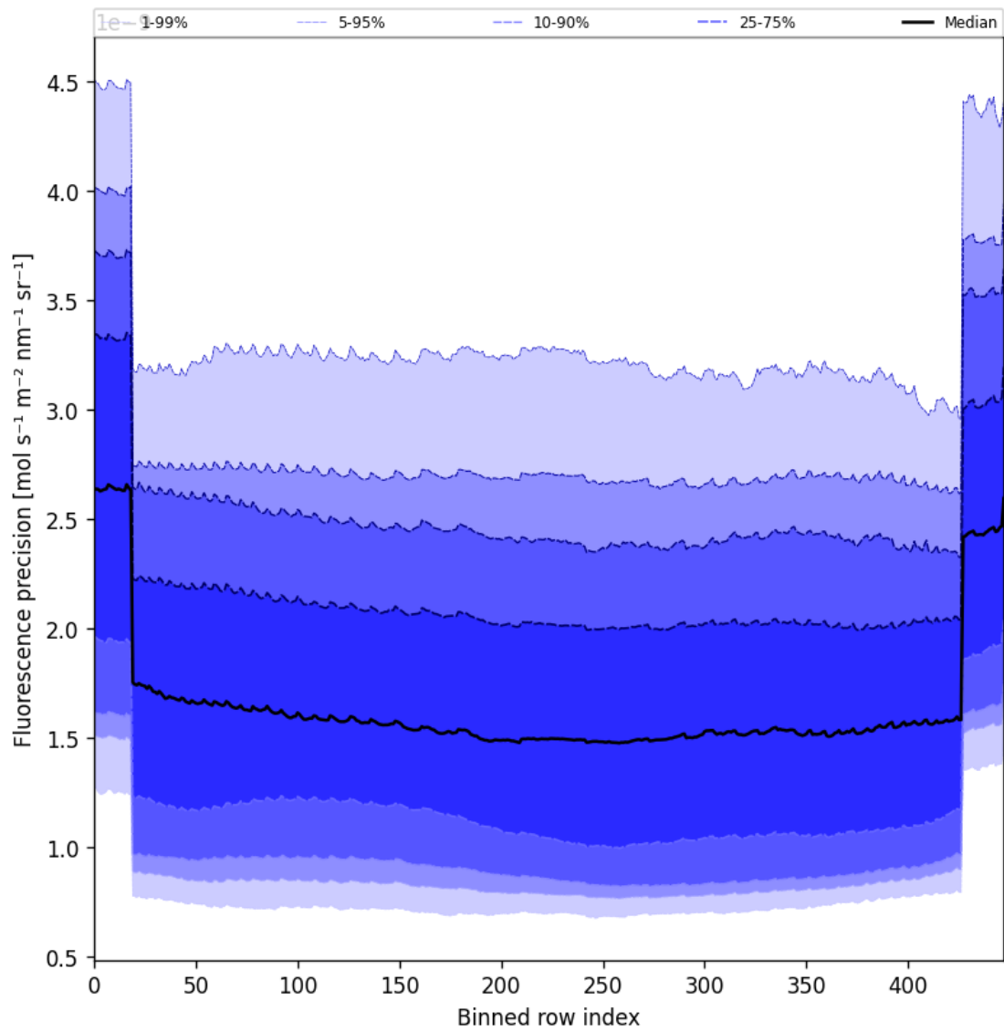
Figure 58: Along track statistics of “Fluorescence precision” for 2025-10-20 to 2025-10-22
