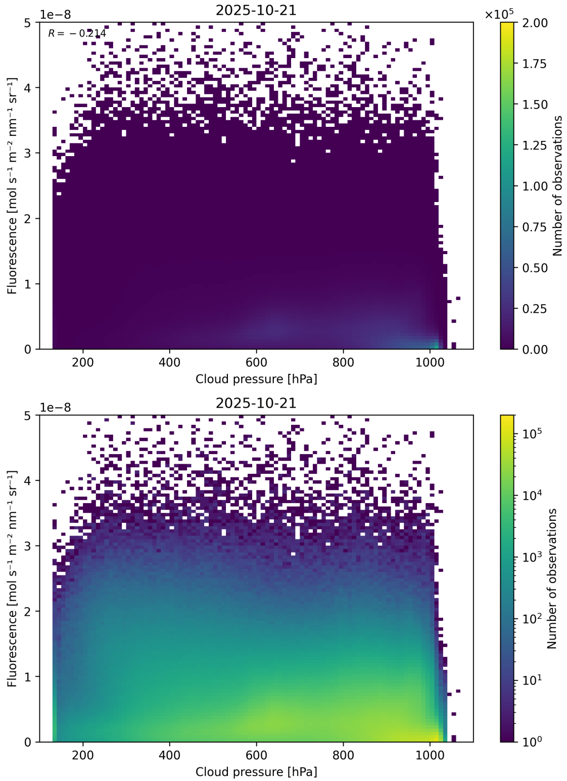
Figure 80: Scatter density plot of “Cloud pressure” against “Fluorescence” for 2025-10-20 to 2025-10-22.
