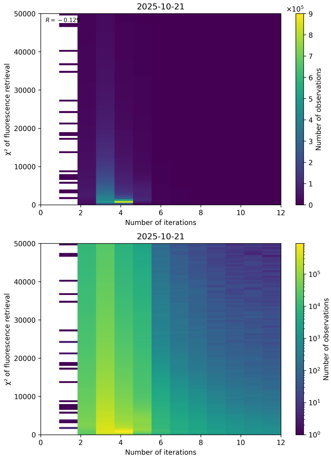
Figure 97: Scatter density plot of “Number of iterations” against “ \chi^2 of fluorescence retrieval” for 2025-10-20 to 2025-10-22.
