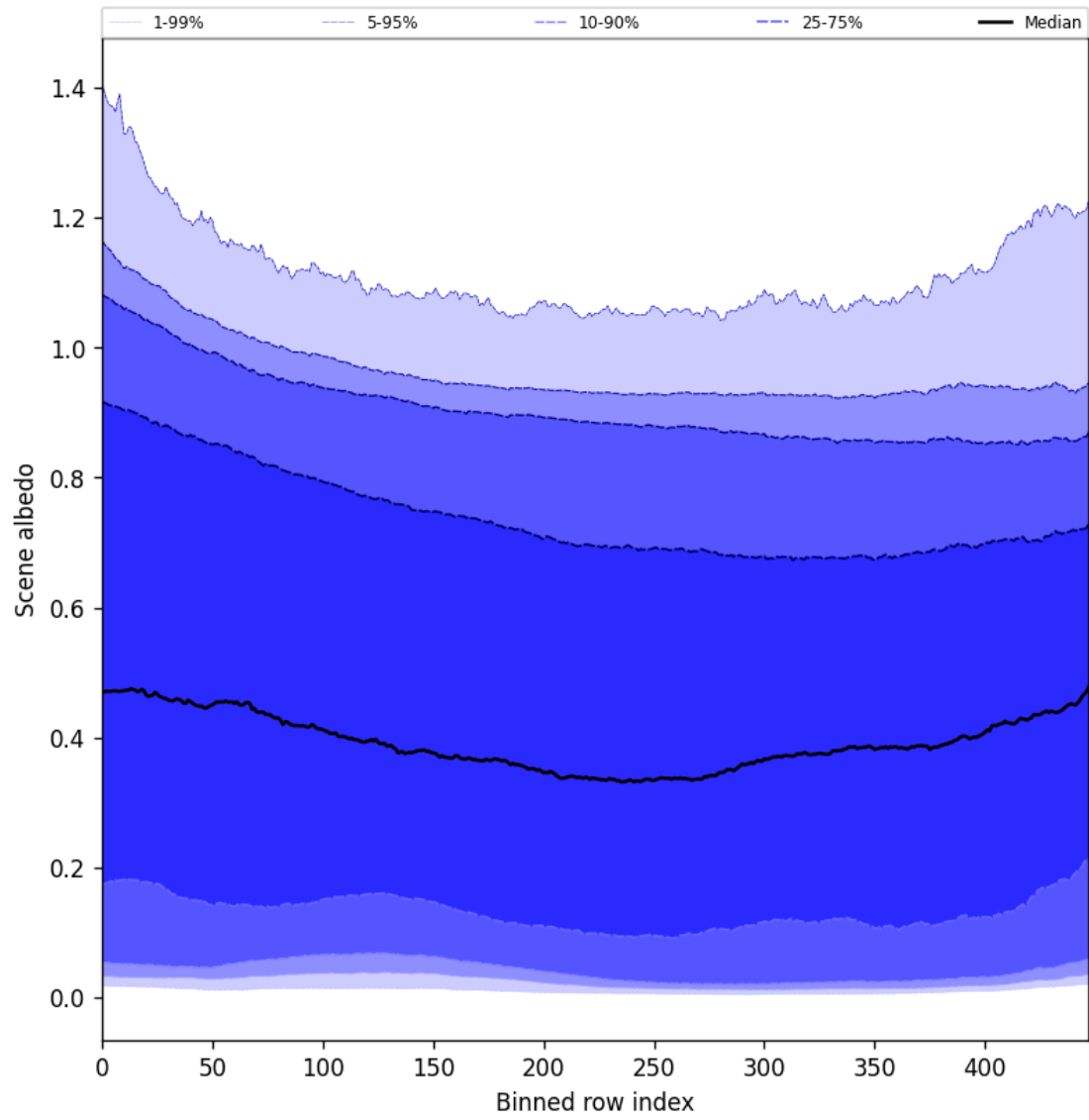
Figure 51: Along track statistics of “Scene albedo” for 2025-10-20 to 2025-10-22
