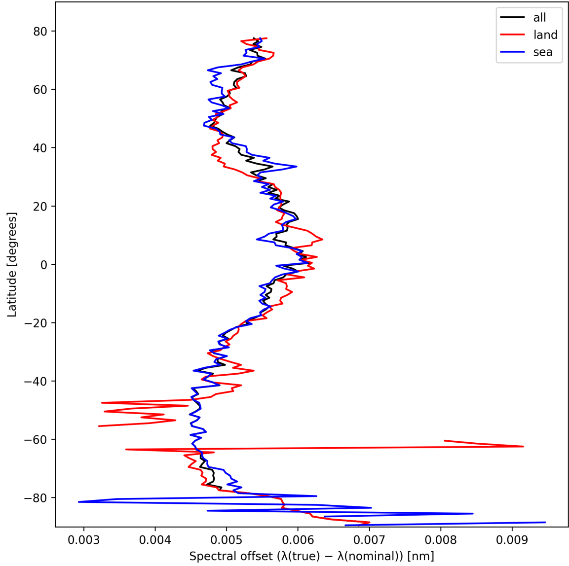
Figure 28: Zonal average of “Spectral offset ( \lambda_{\text{true}} - \lambda_{\text{nominal}} )” for 2025-10-20 to 2025-10-22.
