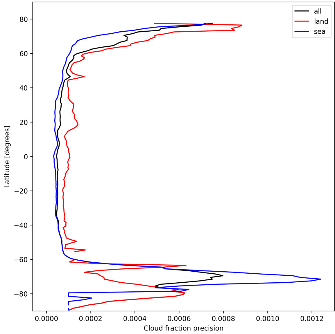
Figure 16: Zonal average of “Cloud fraction precision” for 2025-10-20 to 2025-10-22.
