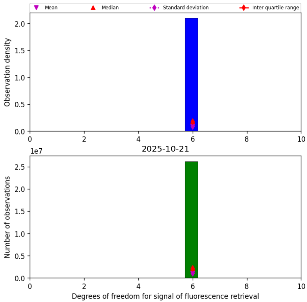
Figure 43: Histogram of "Degrees of freedom for signal of fluorescence retrieval" for 2025-10-20 to 2025-10-22
