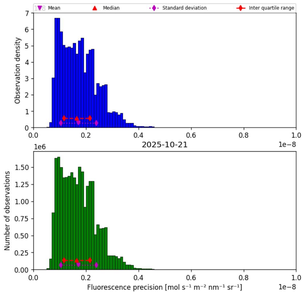
Figure 41: Histogram of “Fluorescence precision” for 2025-10-20 to 2025-10-22
