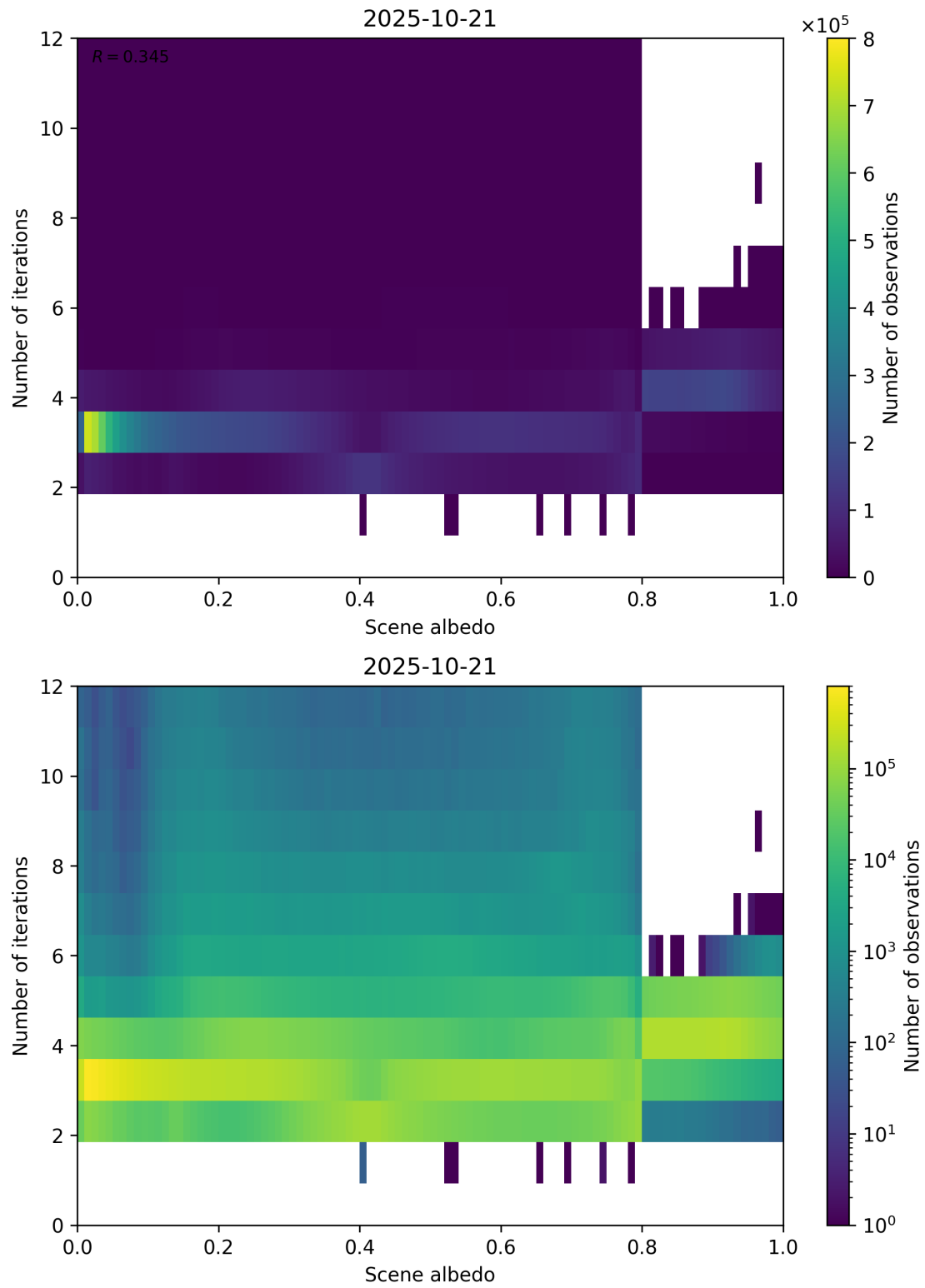
Figure 105: Scatter density plot of “Scene albedo” against “Number of iterations” for 2025-10-20 to 2025-10-22.
