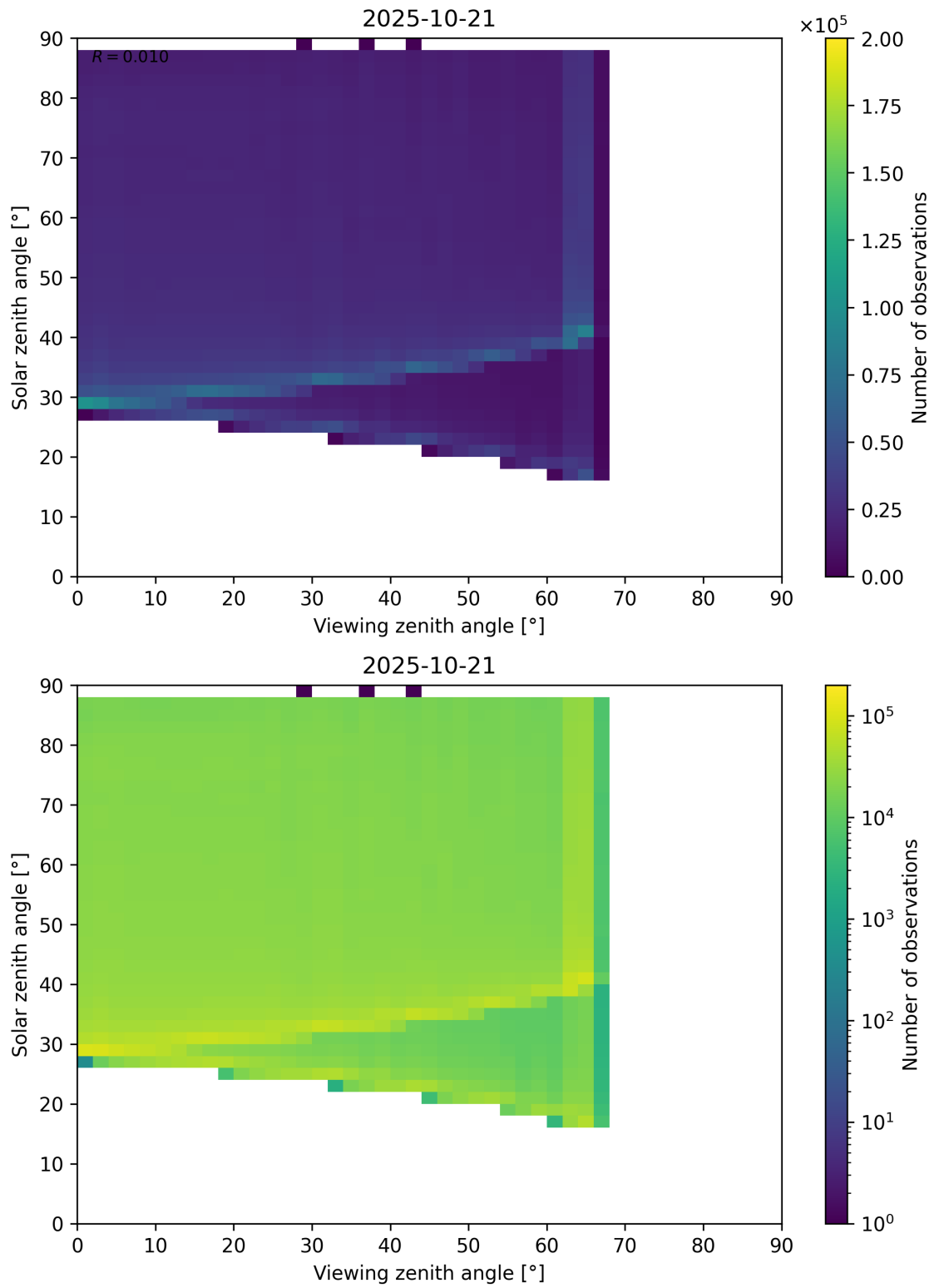
Figure 127: Scatter density plot of “Viewing zenith angle” against “Solar zenith angle” for 2025-10-20 to 2025-10-22.
