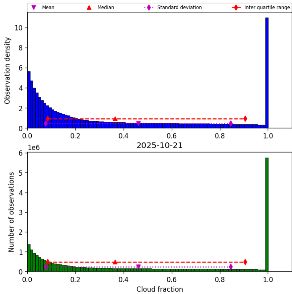
Figure 32: Histogram of “Cloud fraction” for 2025-10-20 to 2025-10-22
