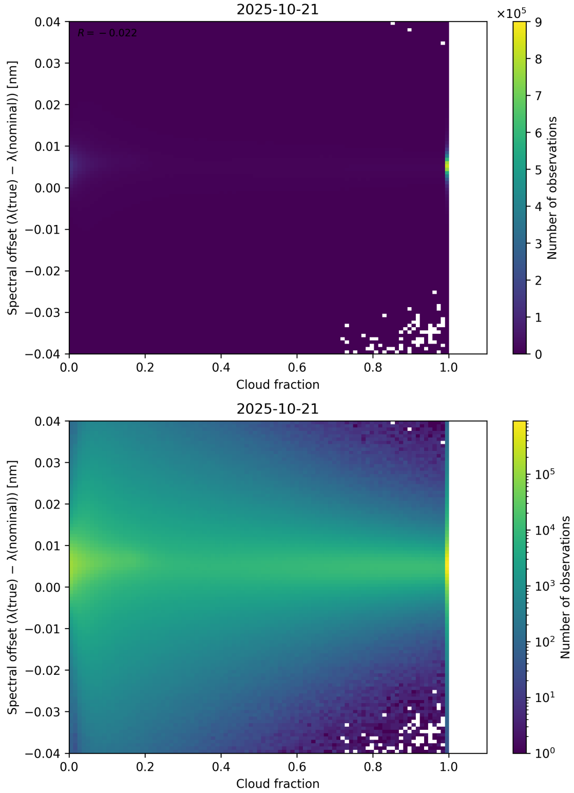
Figure 76: Scatter density plot of “Cloud fraction” against “Spectral offset ( \lambda_{\text{true}} - \lambda_{\text{nominal}} )” for 2025-10-20 to 2025-10-22.
