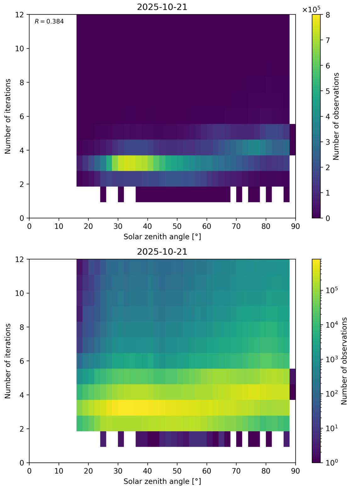
Figure 114: Scatter density plot of “Solar zenith angle” against “Number of iterations” for 2025-10-20 to 2025-10-22.
