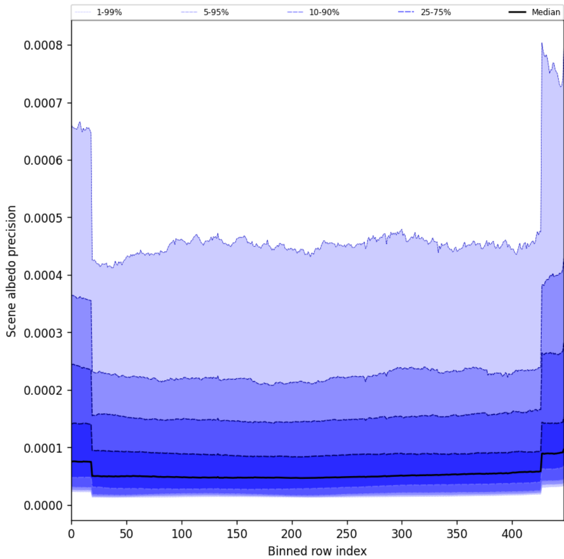
Figure 52: Along track statistics of “Scene albedo precision” for 2025-10-20 to 2025-10-22
