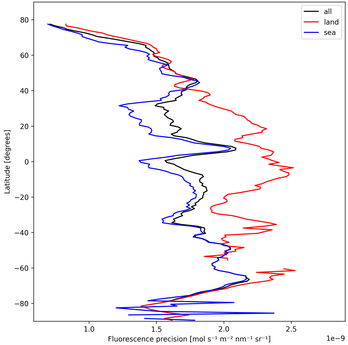
Figure 24: Zonal average of “Fluorescence precision” for 2025-10-20 to 2025-10-22.
