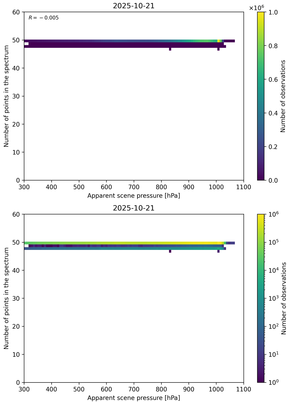
Figure 66: Scatter density plot of “Apparent scene pressure” against “Number of points in the spectrum” for 2025-10-20 to 2025-10-22.
