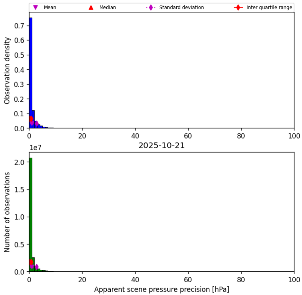
Figure 37: Histogram of “Apparent scene pressure precision” for 2025-10-20 to 2025-10-22
