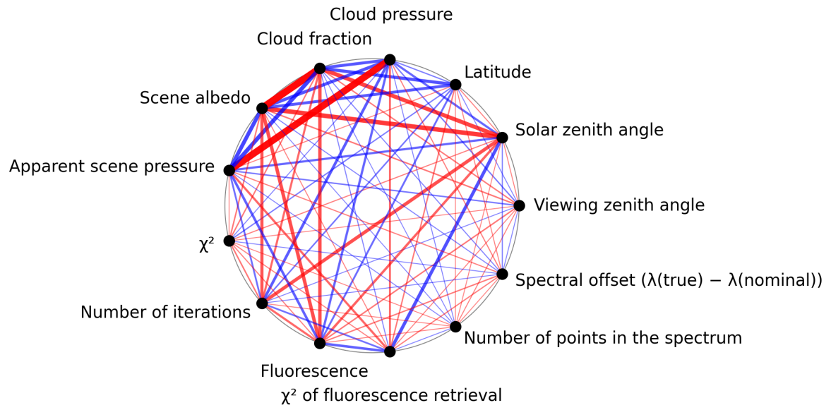
Figure 1: Map of correlation graph for 2025-10-20 to 2025-10-22.
