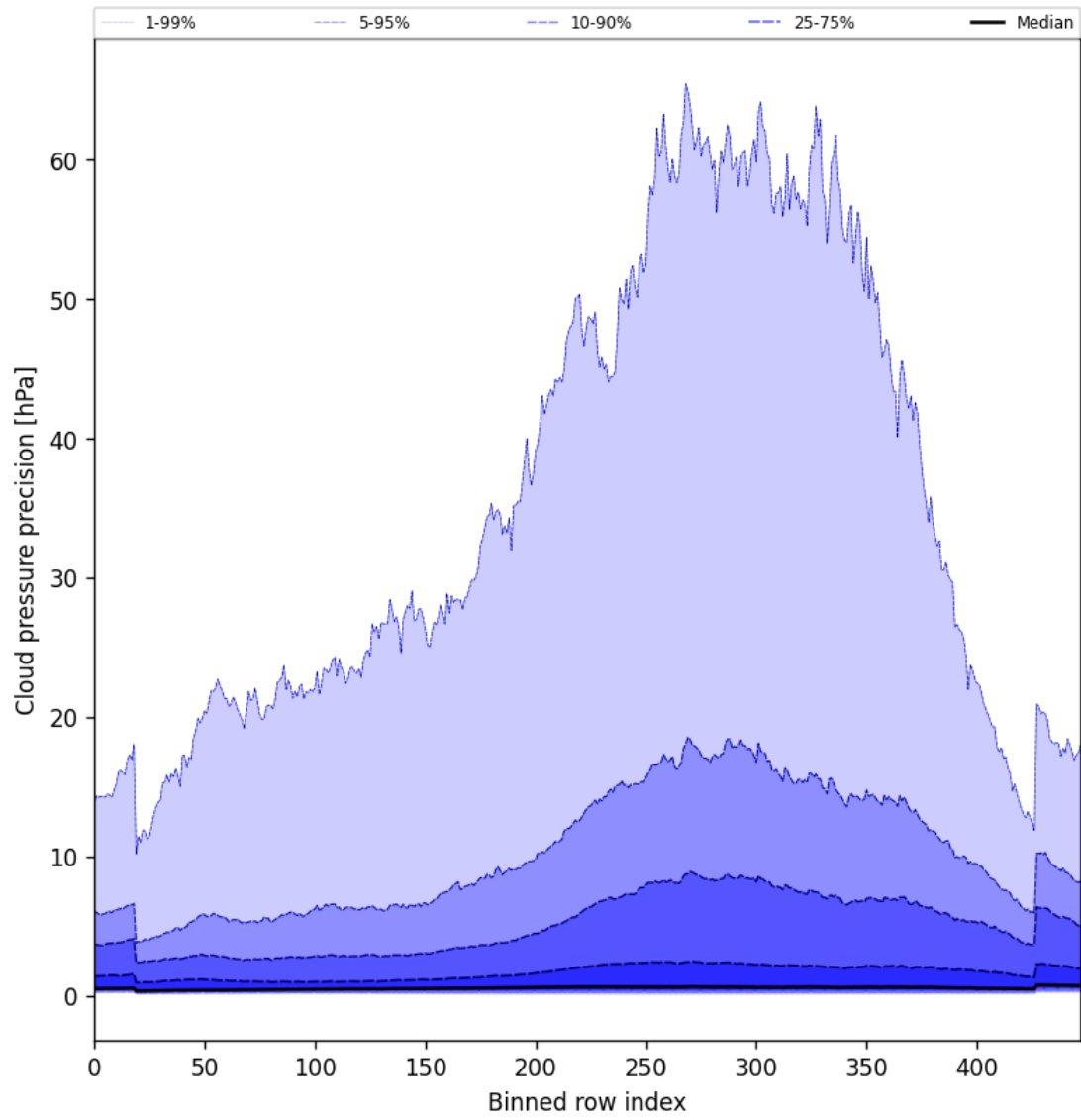
Figure 48: Along track statistics of “Cloud pressure precision” for 2025-10-20 to 2025-10-22
