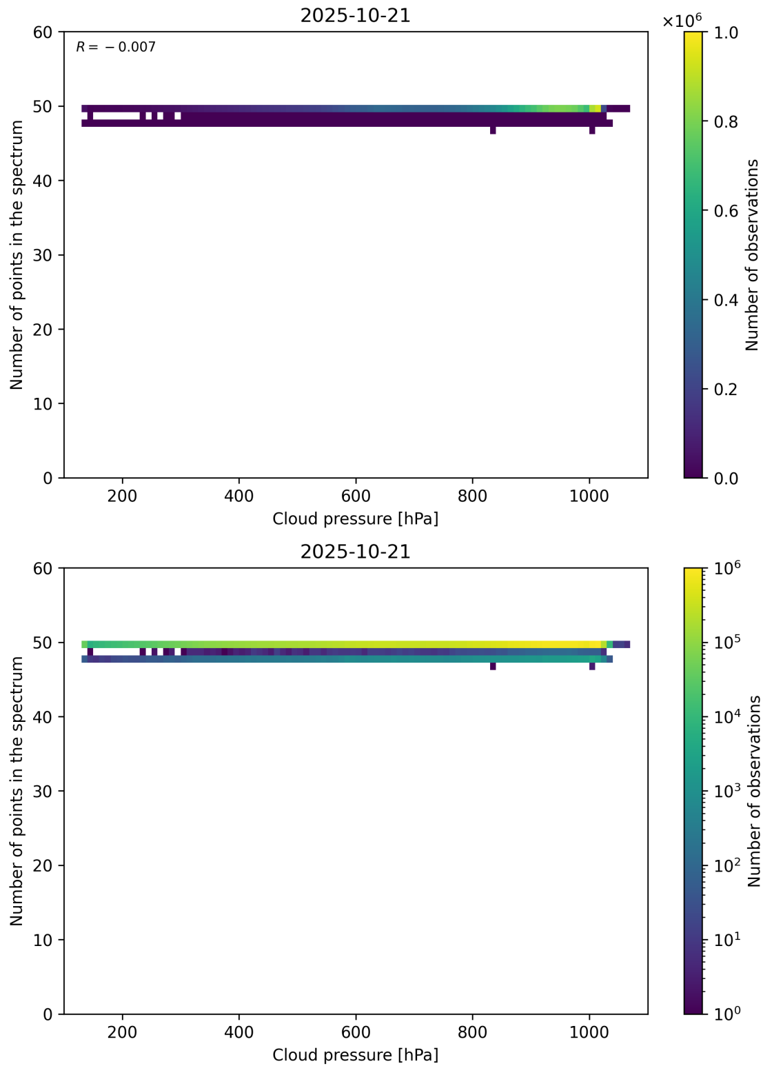
Figure 82: Scatter density plot of “Cloud pressure” against “Number of points in the spectrum” for 2025-10-20 to 2025-10-22.
