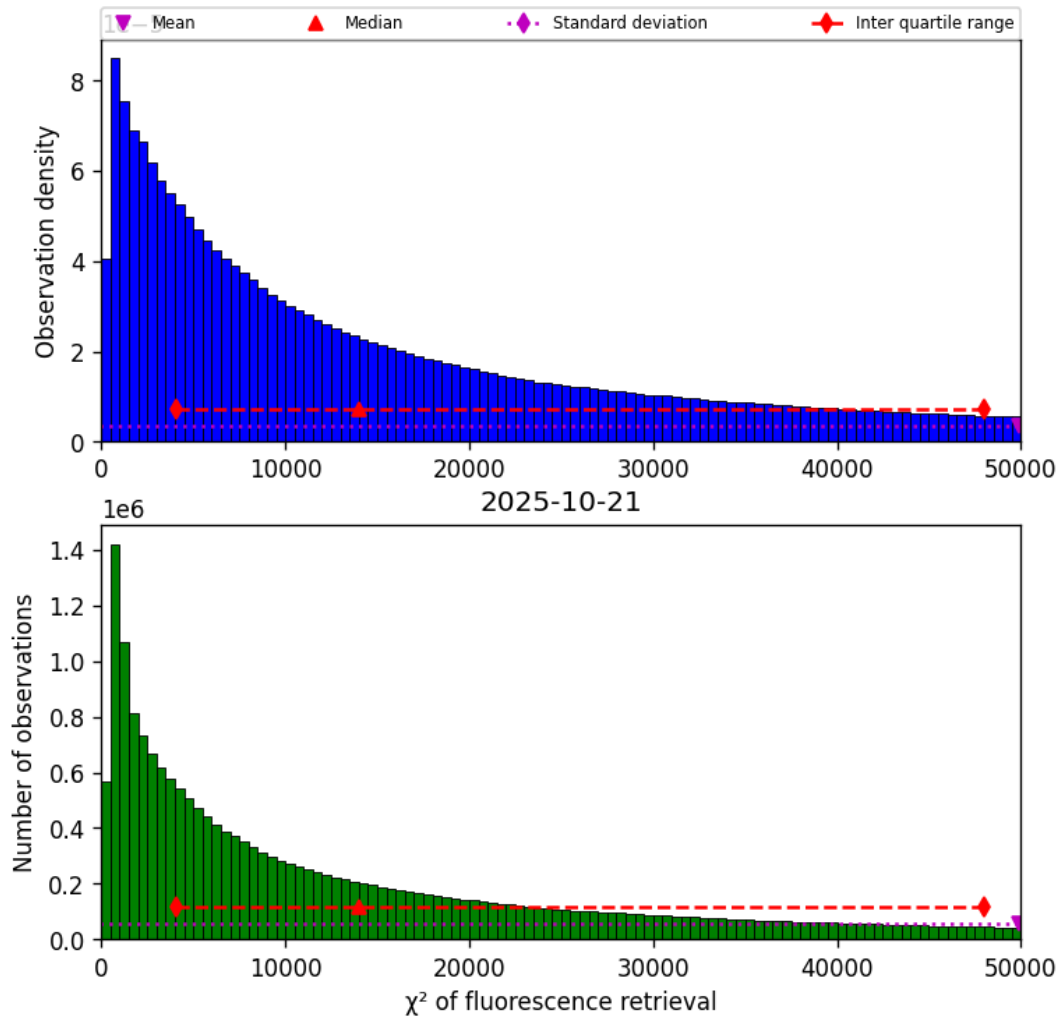
Figure 42: Histogram of “ \chi^2 of fluorescence retrieval” for 2025-10-20 to 2025-10-22
