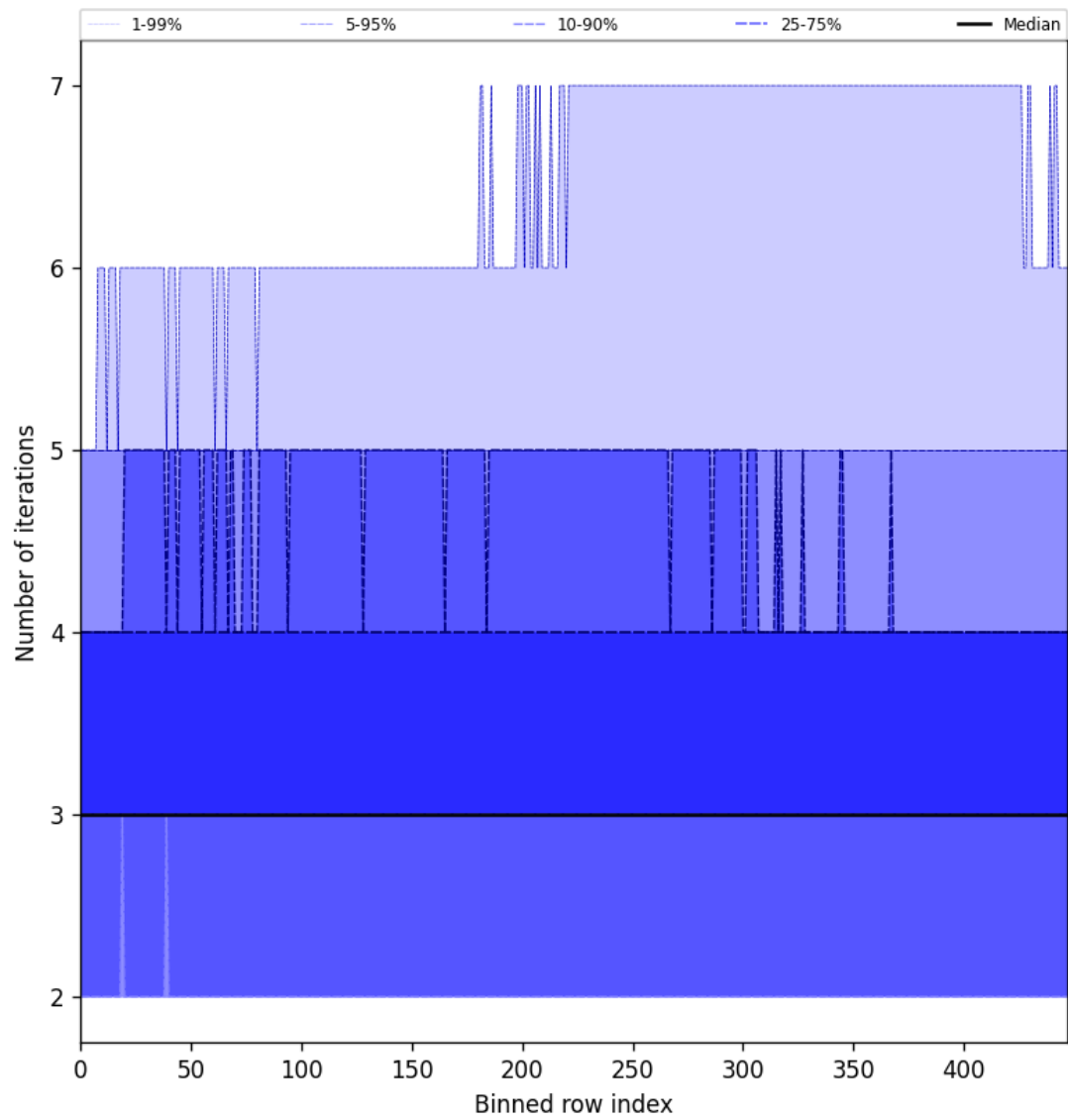
Figure 56: Along track statistics of “Number of iterations” for 2025-10-20 to 2025-10-22
