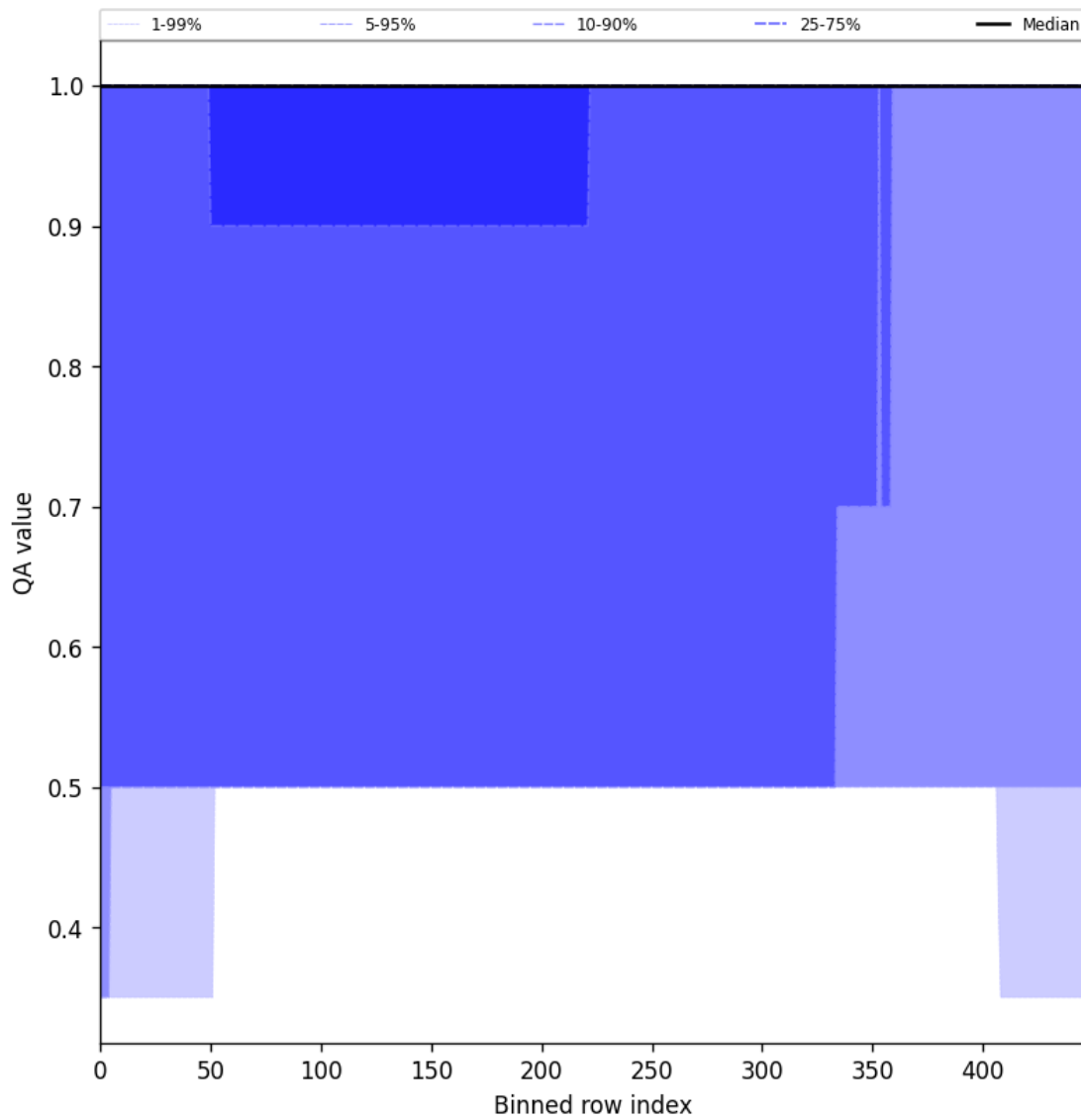
Figure 46: Along track statistics of “QA value” for 2025-10-20 to 2025-10-22
