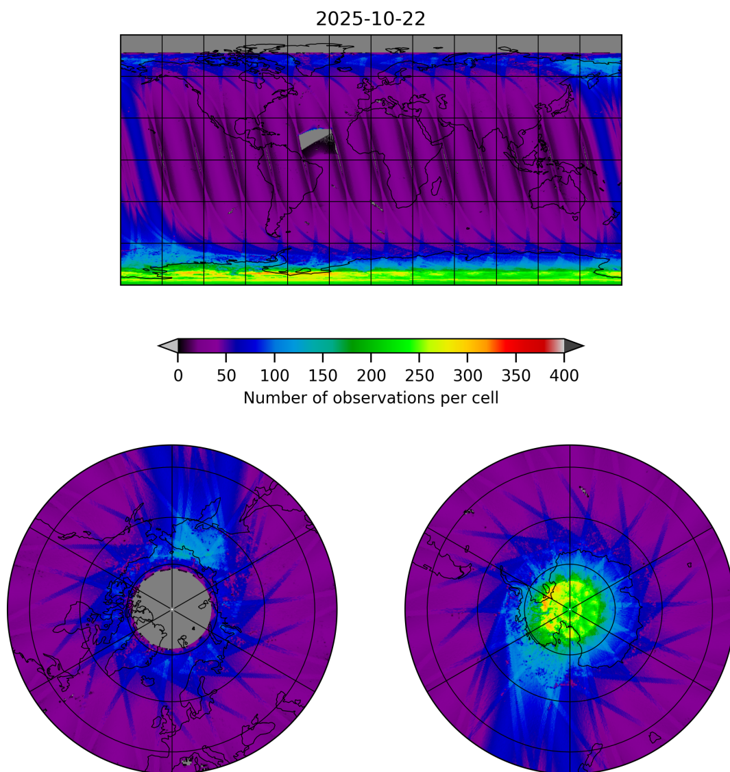
Figure 11: Map of the number of observations for 2025-10-22 to 2025-10-23
