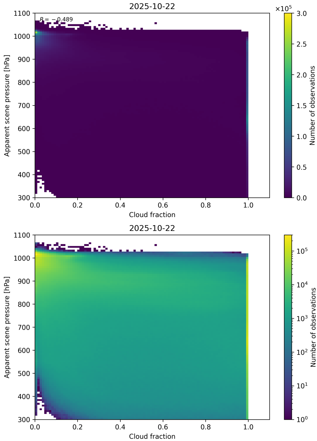
Figure 70: Scatter density plot of “Cloud fraction” against “Apparent scene pressure” for 2025-10-22 to 2025-10-23.
