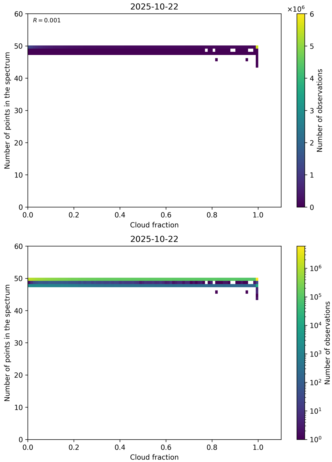
Figure 74: Scatter density plot of “Cloud fraction” against “Number of points in the spectrum” for 2025-10-22 to 2025-10-23.
