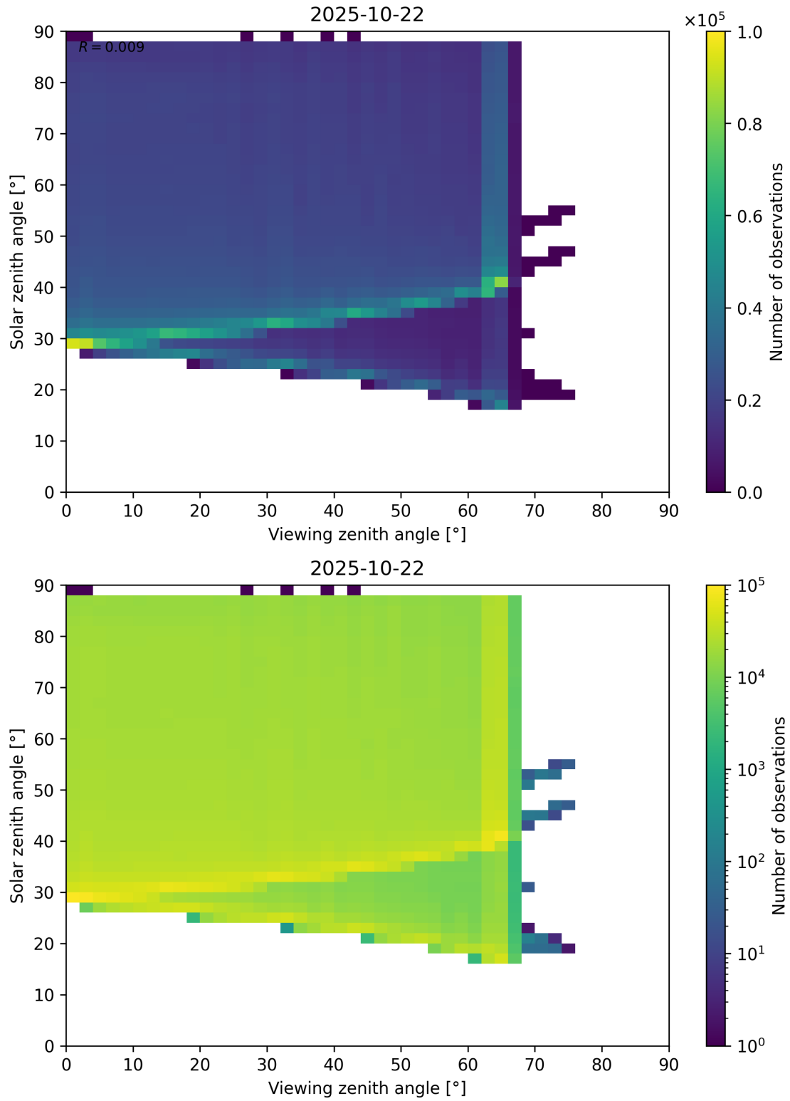
Figure 127: Scatter density plot of “Viewing zenith angle” against “Solar zenith angle” for 2025-10-22 to 2025-10-23.
