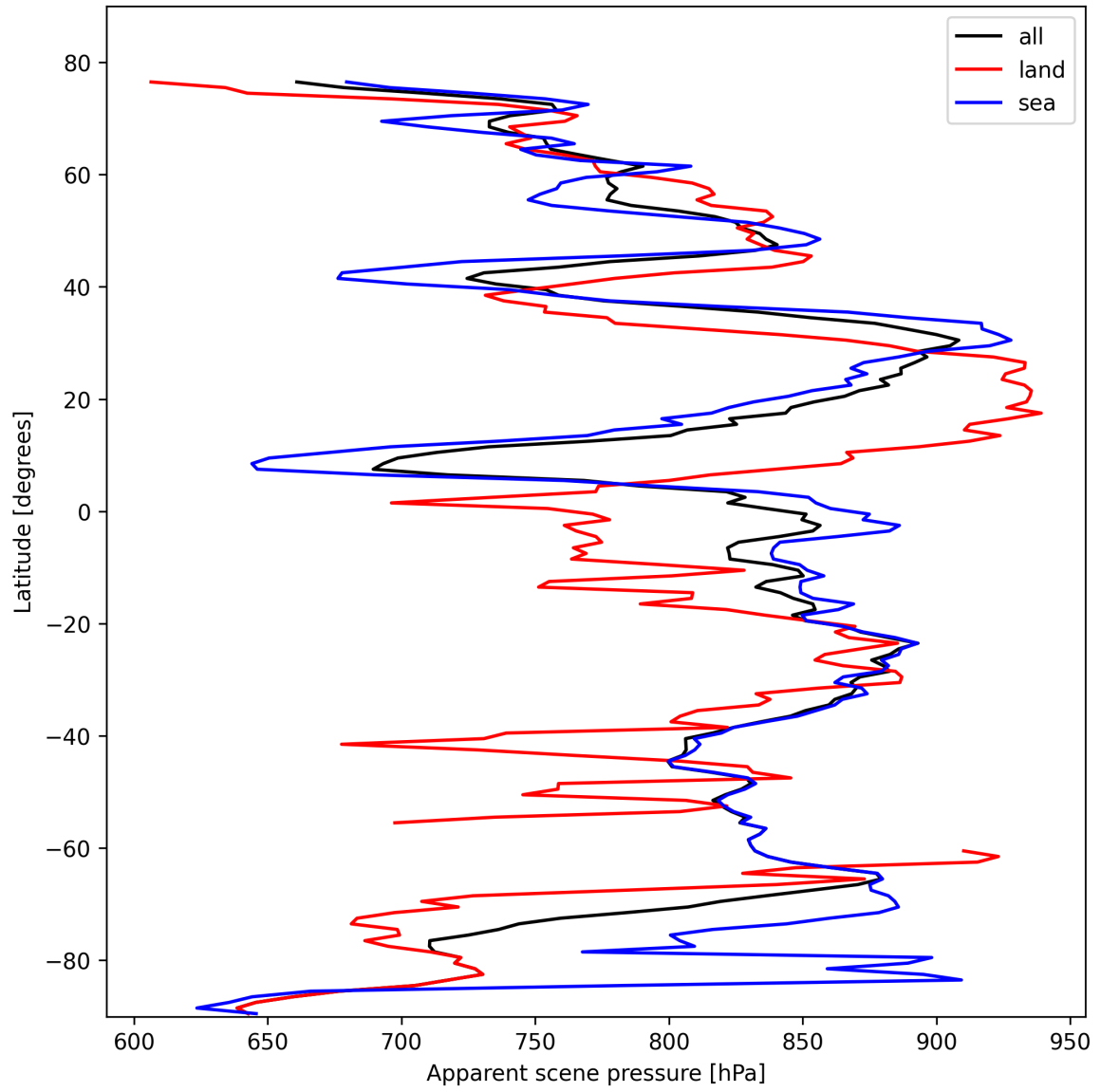
Figure 19: Zonal average of “Apparent scene pressure” for 2025-10-22 to 2025-10-23.
