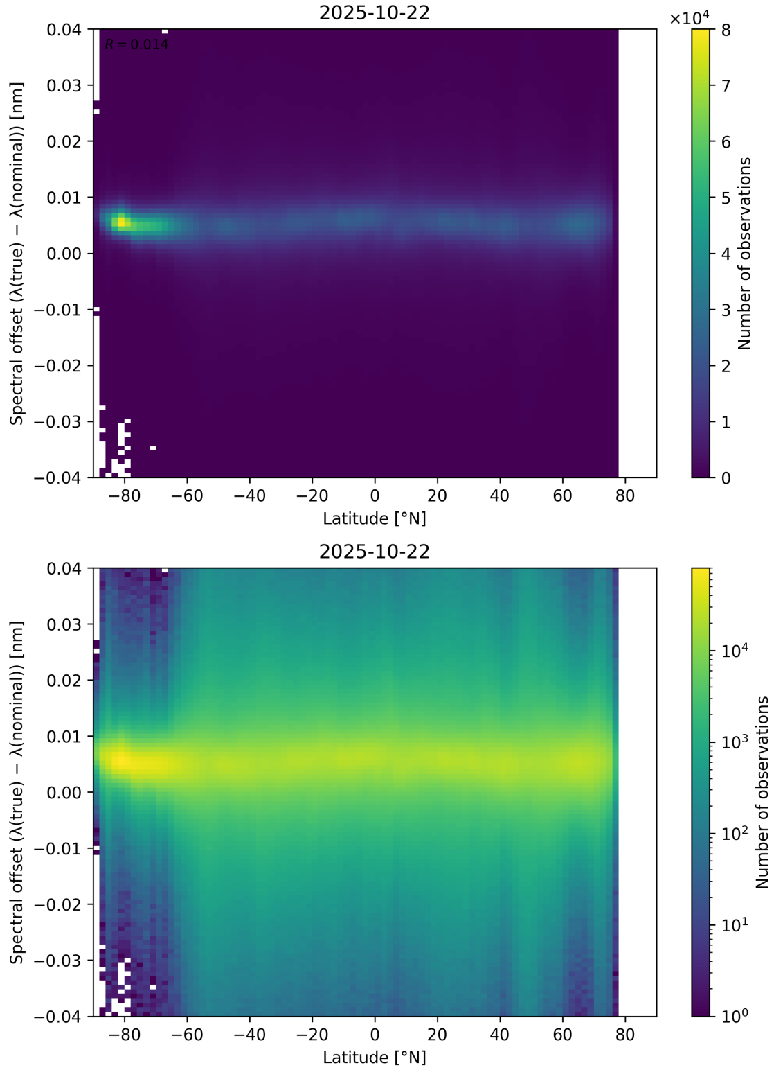
Figure 96: Scatter density plot of “Latitude” against “Spectral offset ( \lambda_{\text{true}} - \lambda_{\text{nominal}} )” for 2025-10-22 to 2025-10-23.
