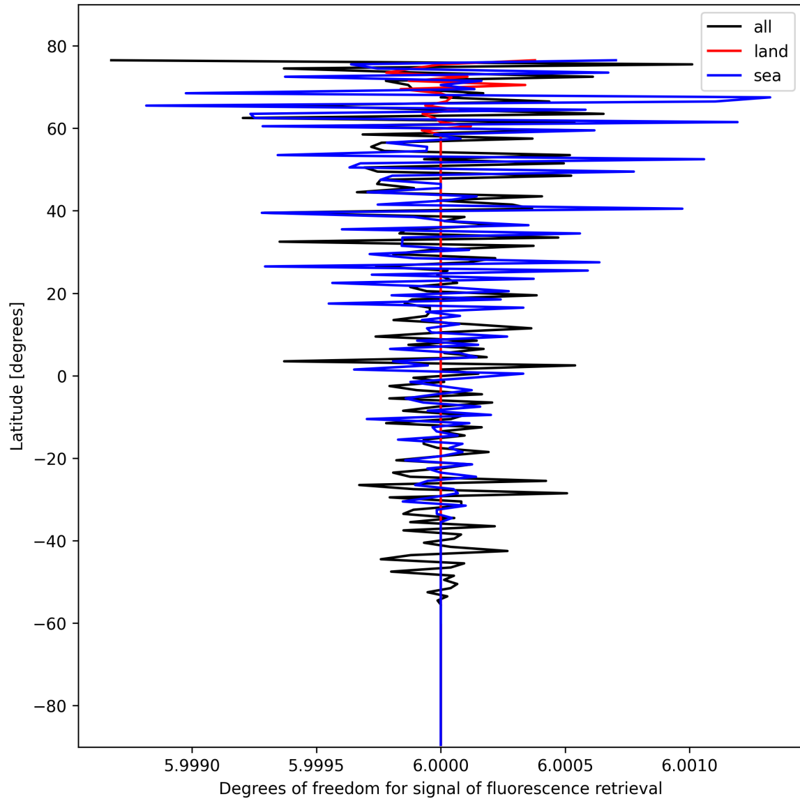
Figure 26: Zonal average of “Degrees of freedom for signal of fluorescence retrieval” for 2025-10-22 to 2025-10-23.
