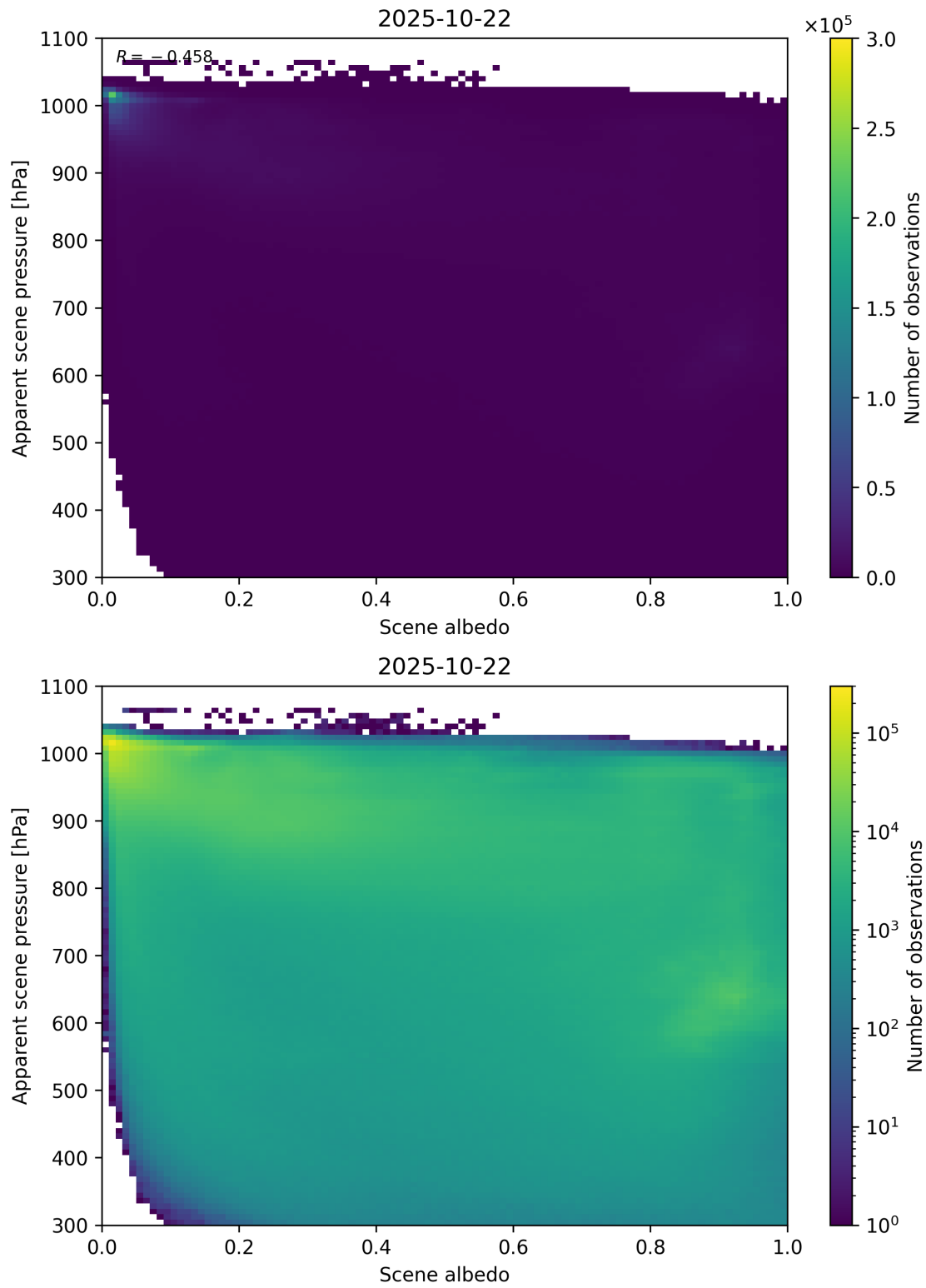
Figure 102: Scatter density plot of “Scene albedo” against “Apparent scene pressure” for 2025-10-22 to 2025-10-23.
