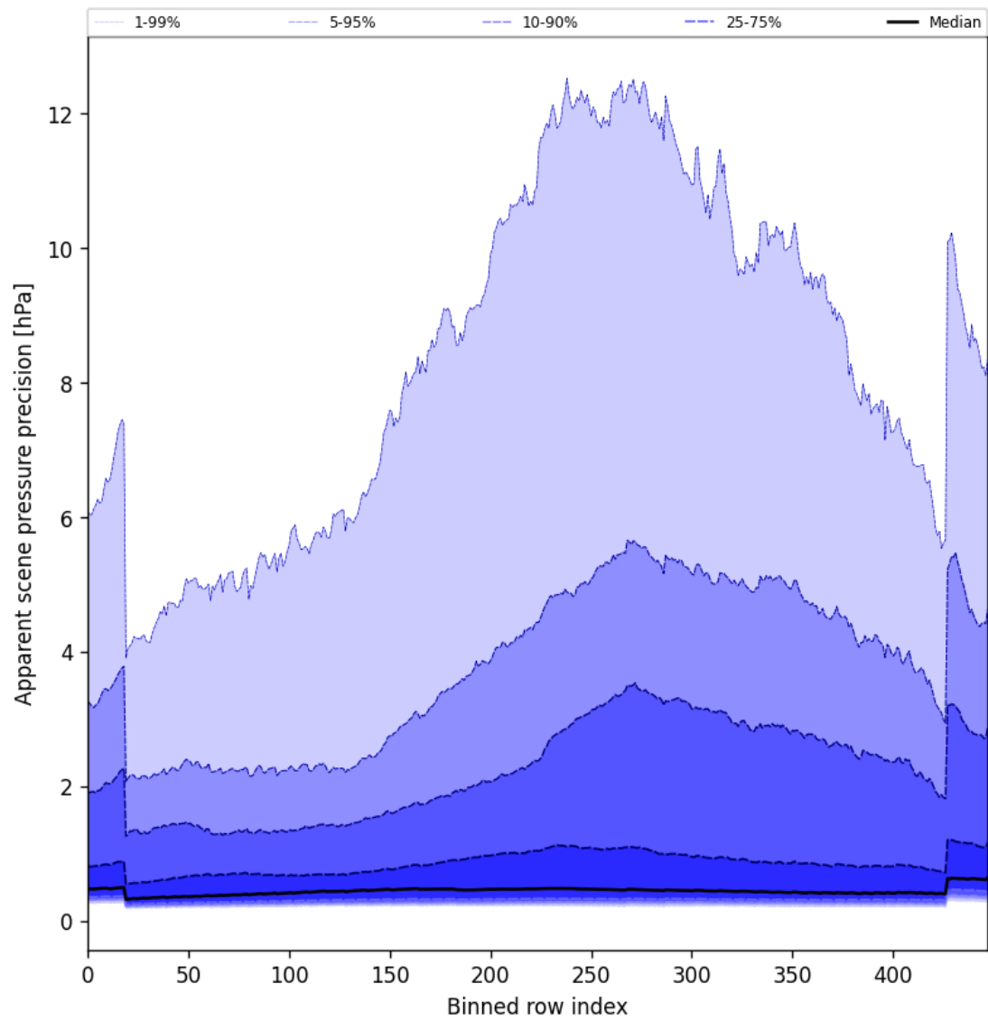
Figure 54: Along track statistics of “Apparent scene pressure precision” for 2025-10-22 to 2025-10-23
