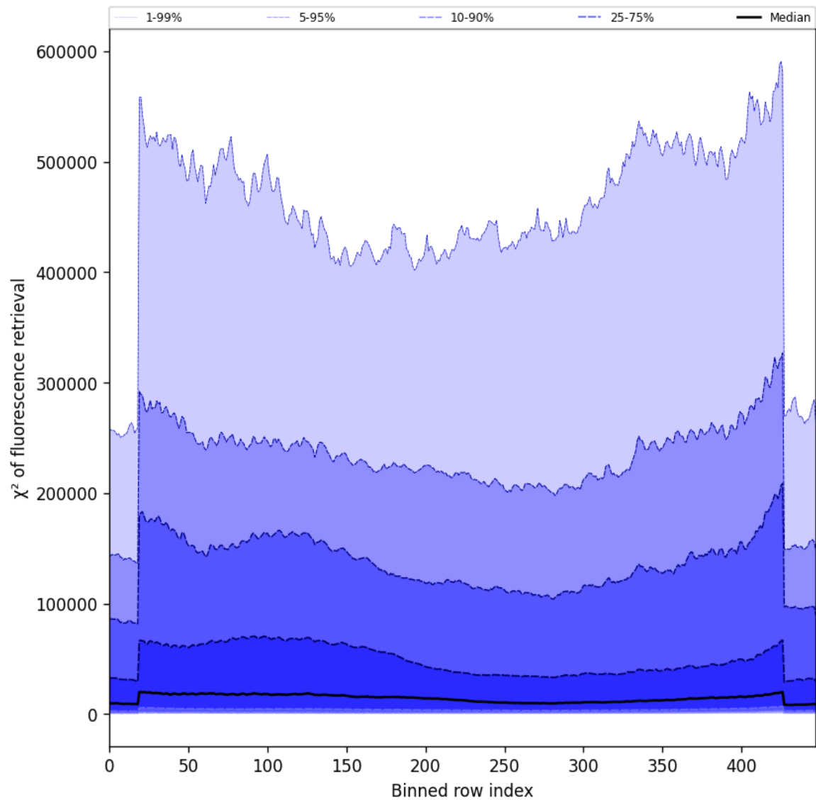
Figure 59: Along track statistics of “ \chi^2 of fluorescence retrieval” for 2025-10-22 to 2025-10-23
