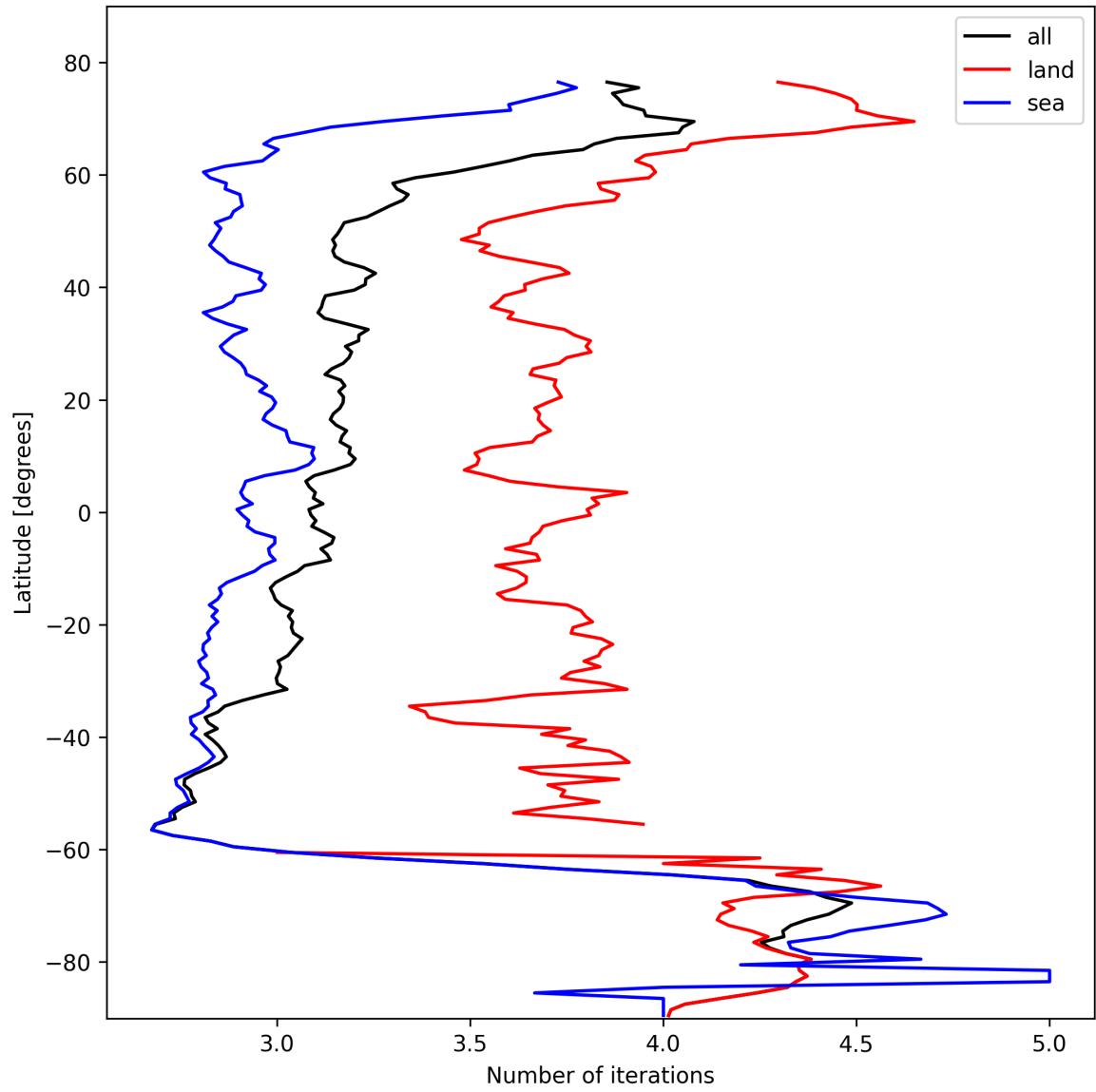
Figure 22: Zonal average of “Number of iterations” for 2025-10-22 to 2025-10-23.
