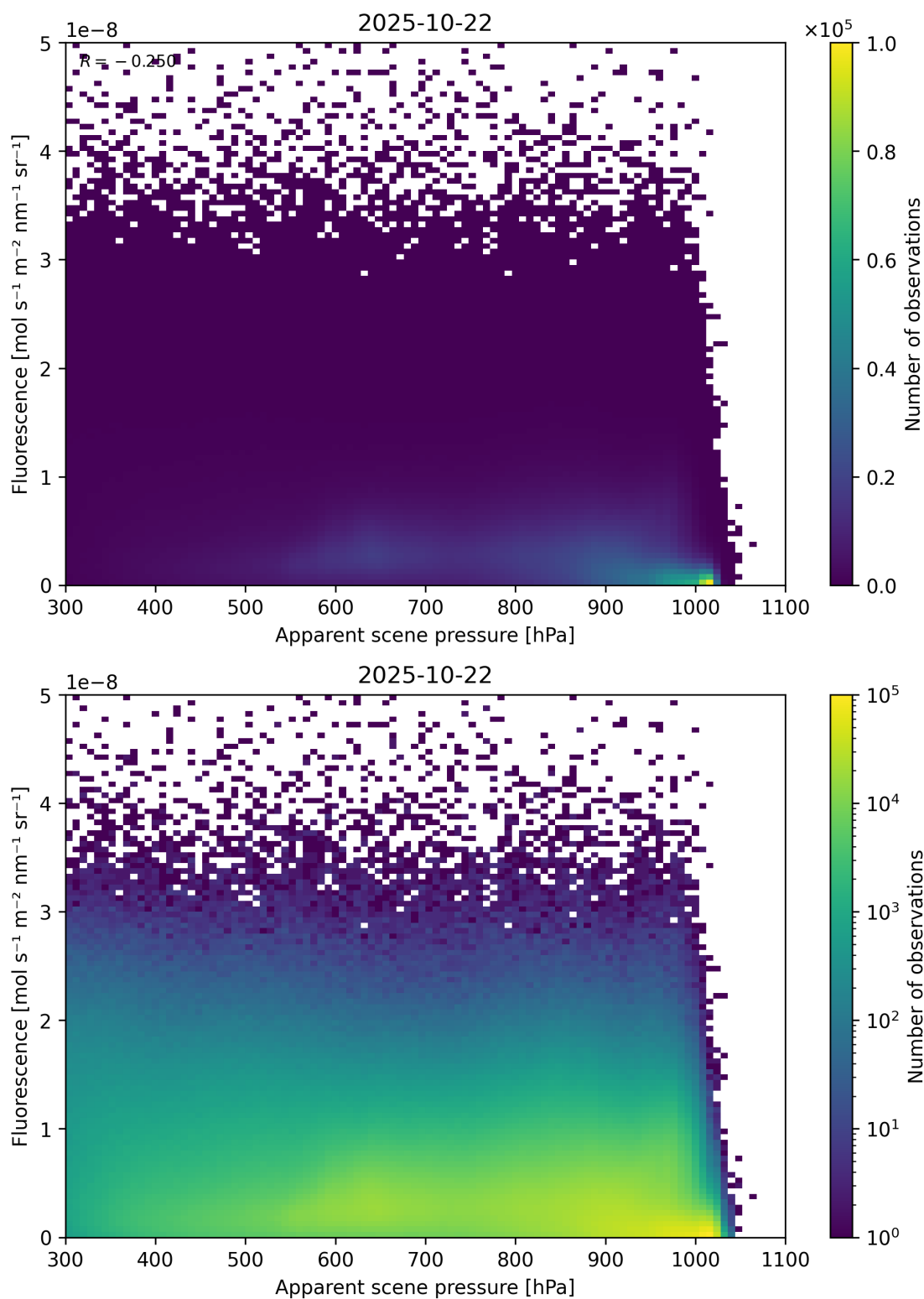
Figure 64: Scatter density plot of “Apparent scene pressure” against “Fluorescence” for 2025-10-22 to 2025-10-23.
