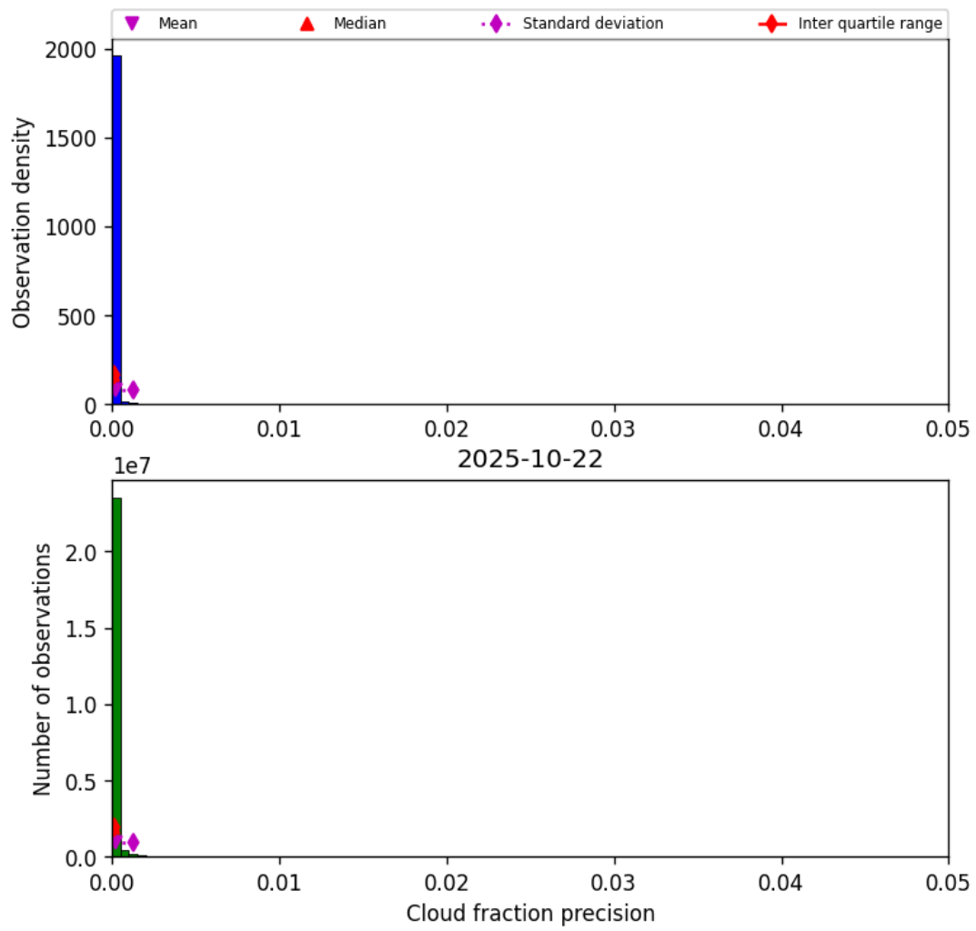
Figure 33: Histogram of “Cloud fraction precision” for 2025-10-22 to 2025-10-23
