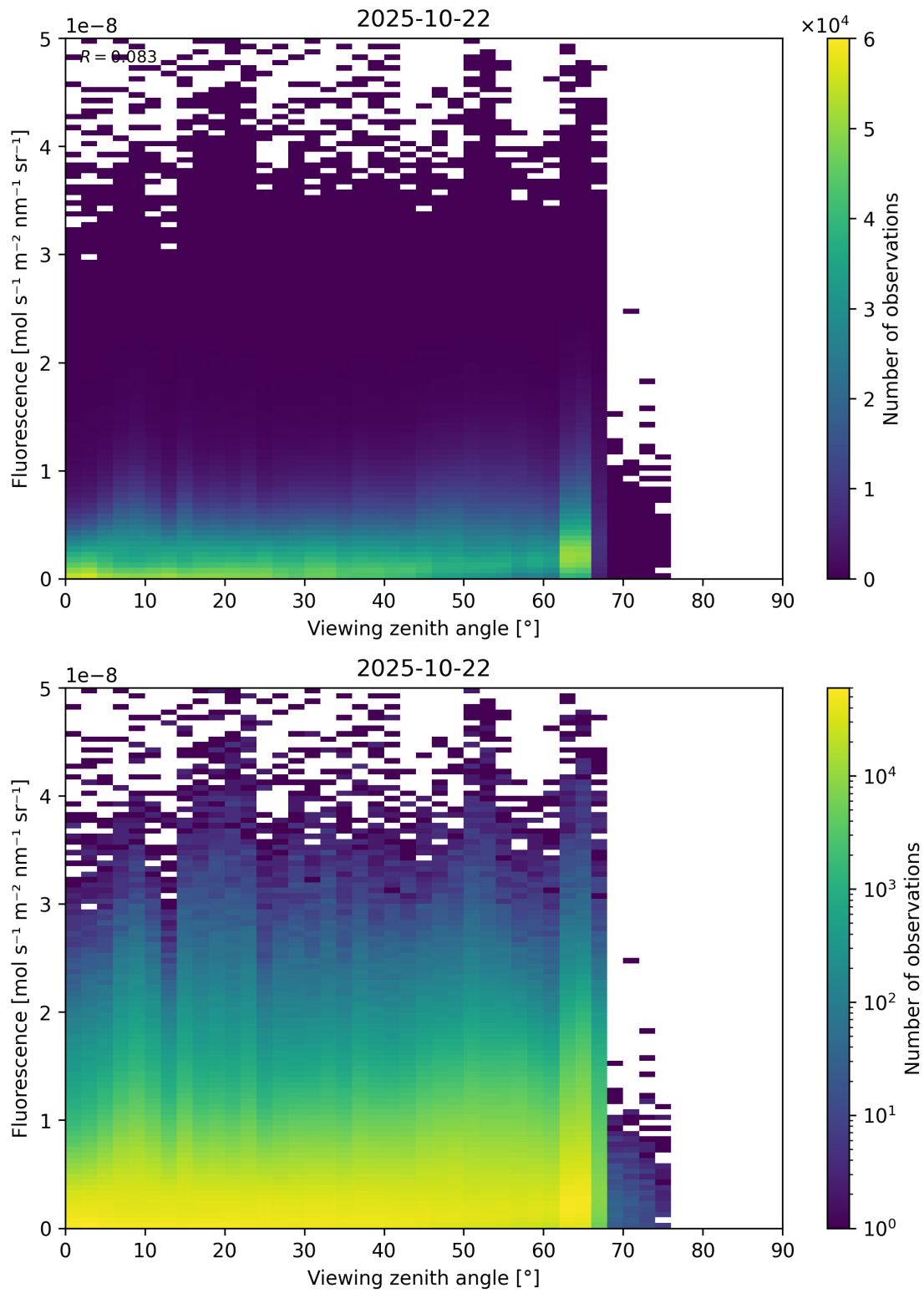
Figure 122: Scatter density plot of “Viewing zenith angle” against “Fluorescence” for 2025-10-22 to 2025-10-23.
