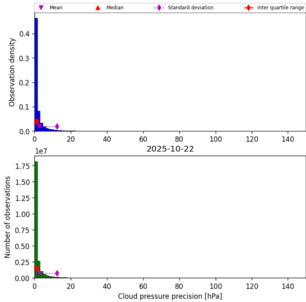
Figure 31: Histogram of "Cloud pressure precision" for 2025-10-22 to 2025-10-23
