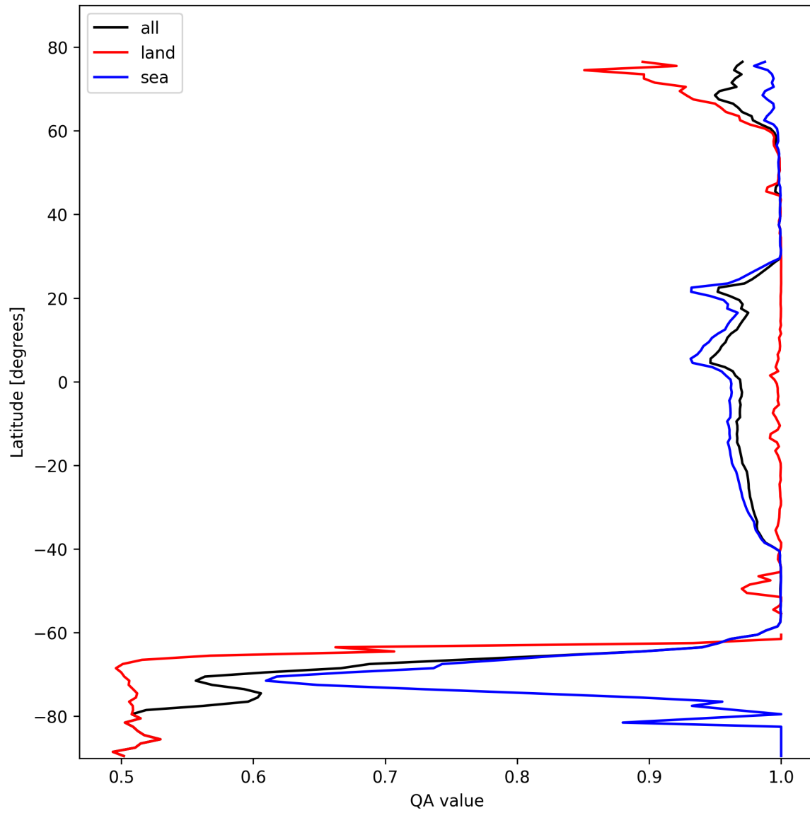
Figure 12: Zonal average of "QA value" for 2025-10-22 to 2025-10-23.
