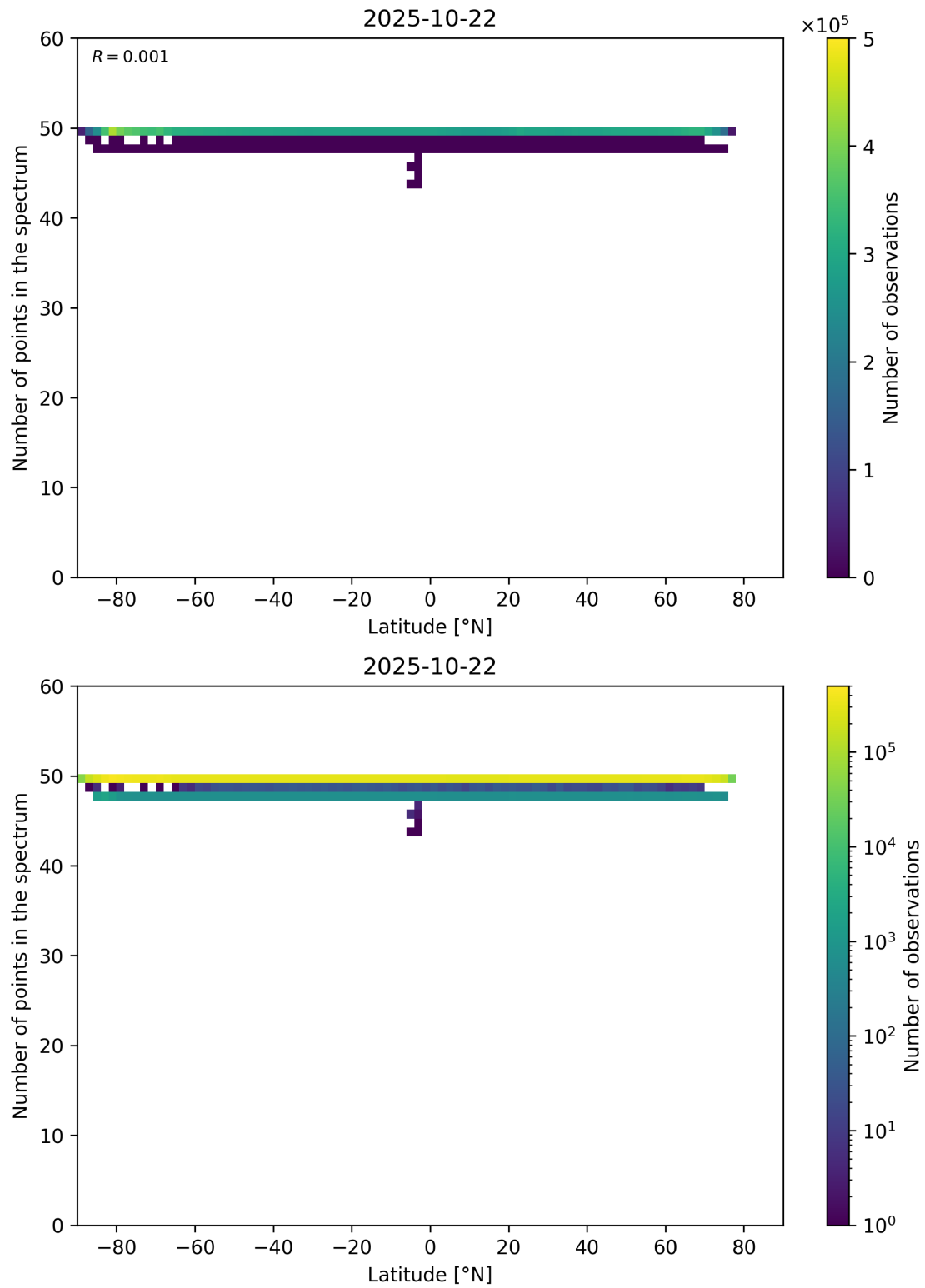
Figure 94: Scatter density plot of “Latitude” against “Number of points in the spectrum” for 2025-10-22 to 2025-10-23.
