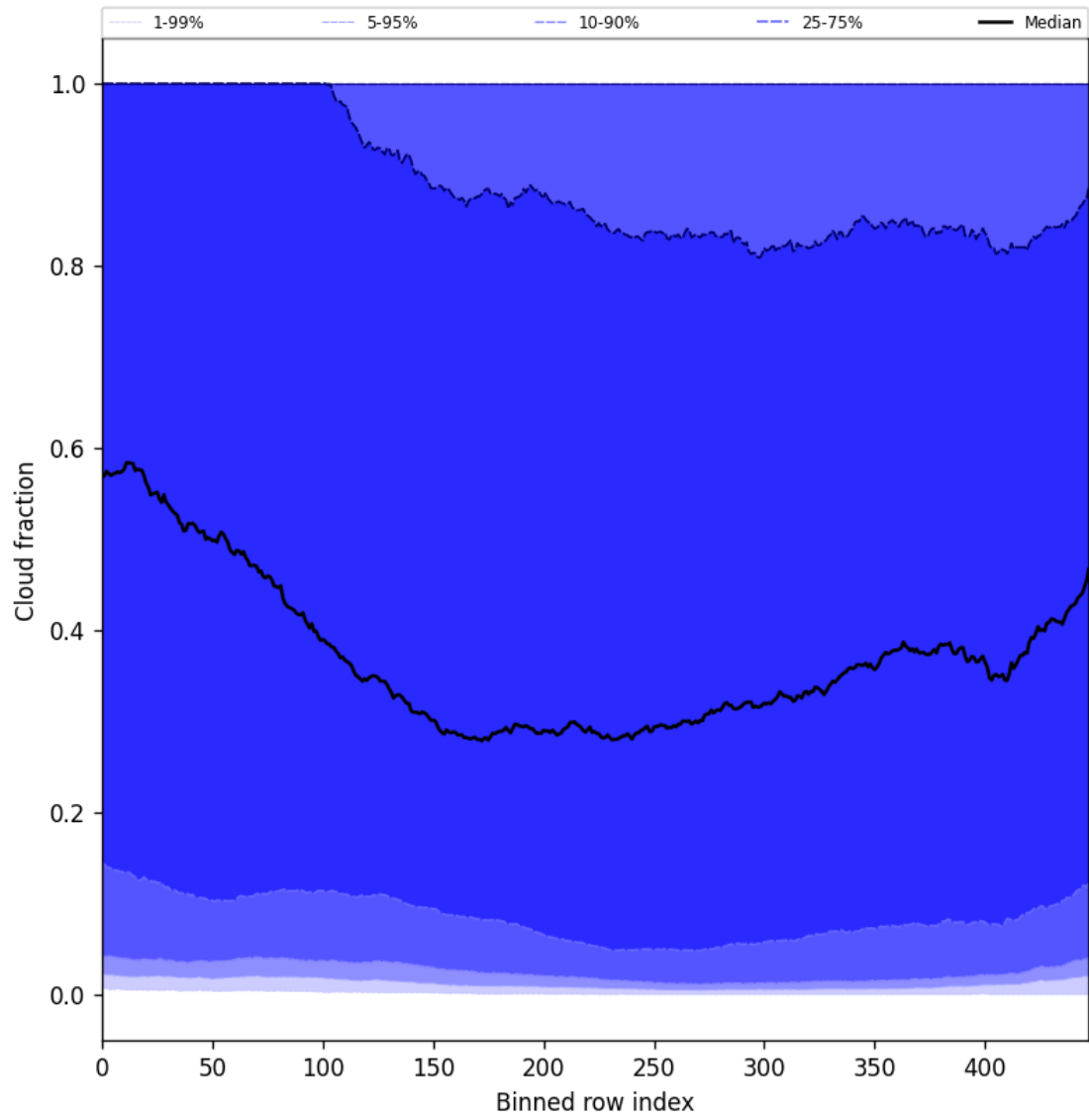
Figure 49: Along track statistics of “Cloud fraction” for 2025-10-22 to 2025-10-23
