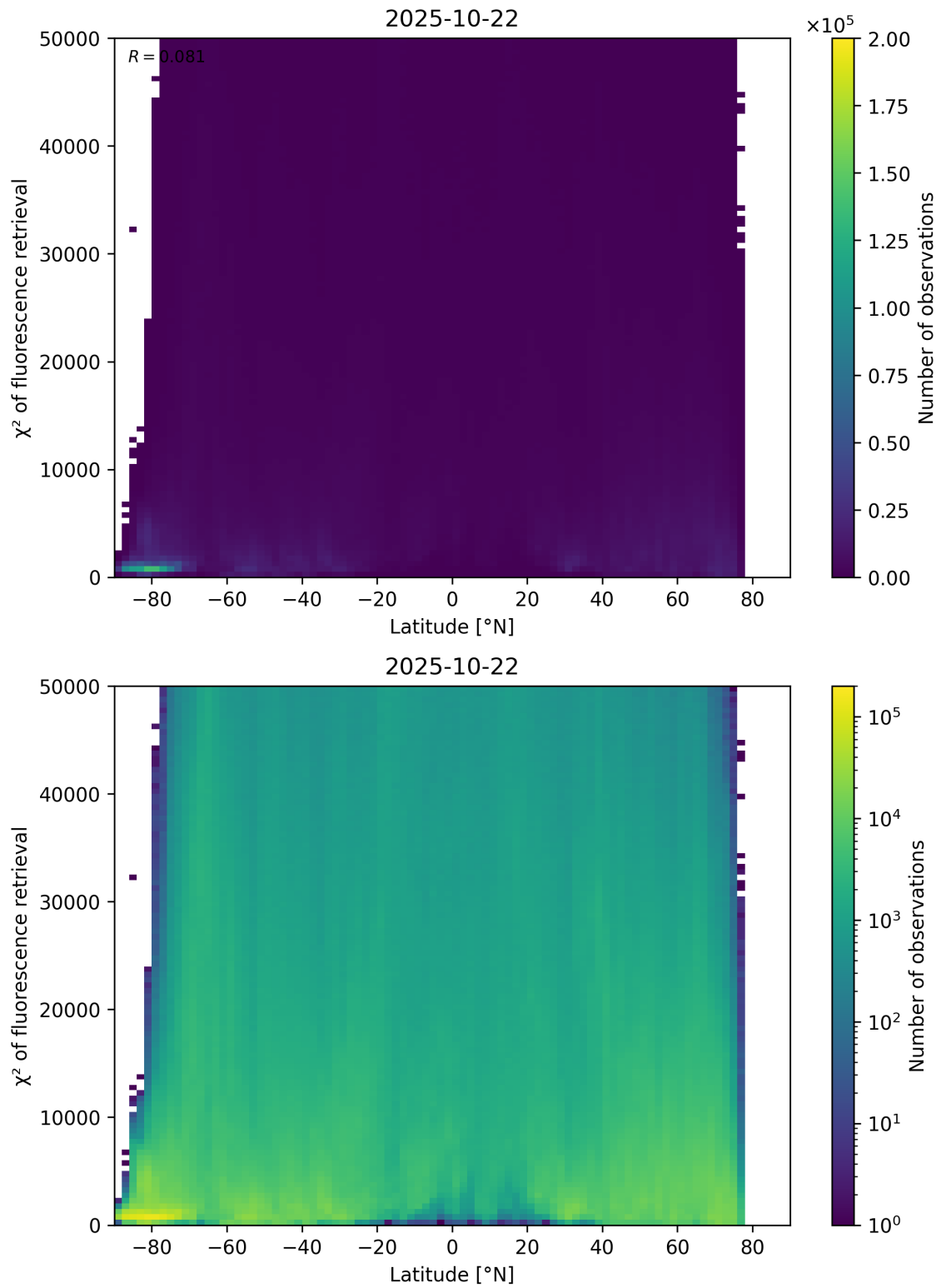
Figure 89: Scatter density plot of “Latitude” against “ \chi^2 of fluorescence retrieval” for 2025-10-22 to 2025-10-23.
