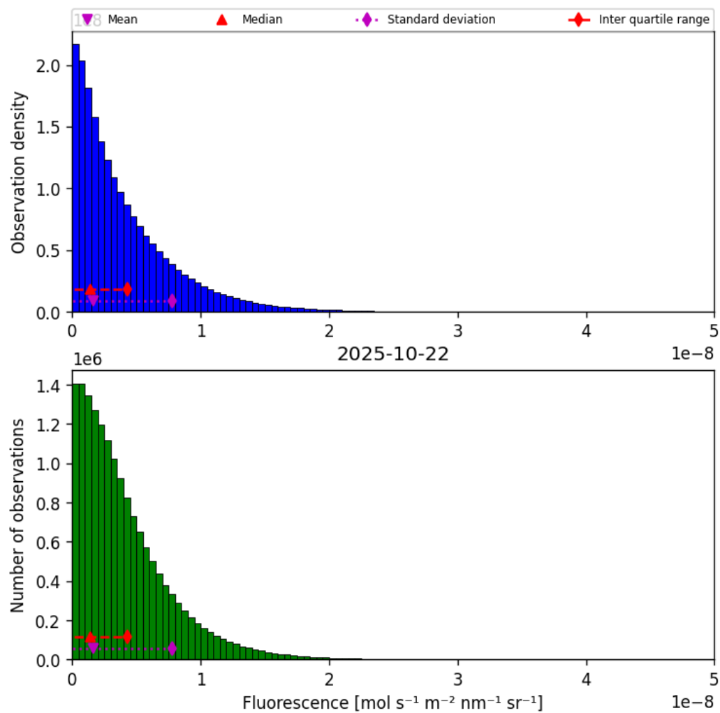
Figure 40: Histogram of “Fluorescence” for 2025-10-22 to 2025-10-23
