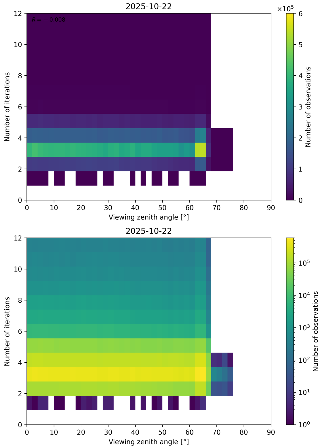
Figure 124: Scatter density plot of “Viewing zenith angle” against “Number of iterations” for 2025-10-22 to 2025-10-23.
