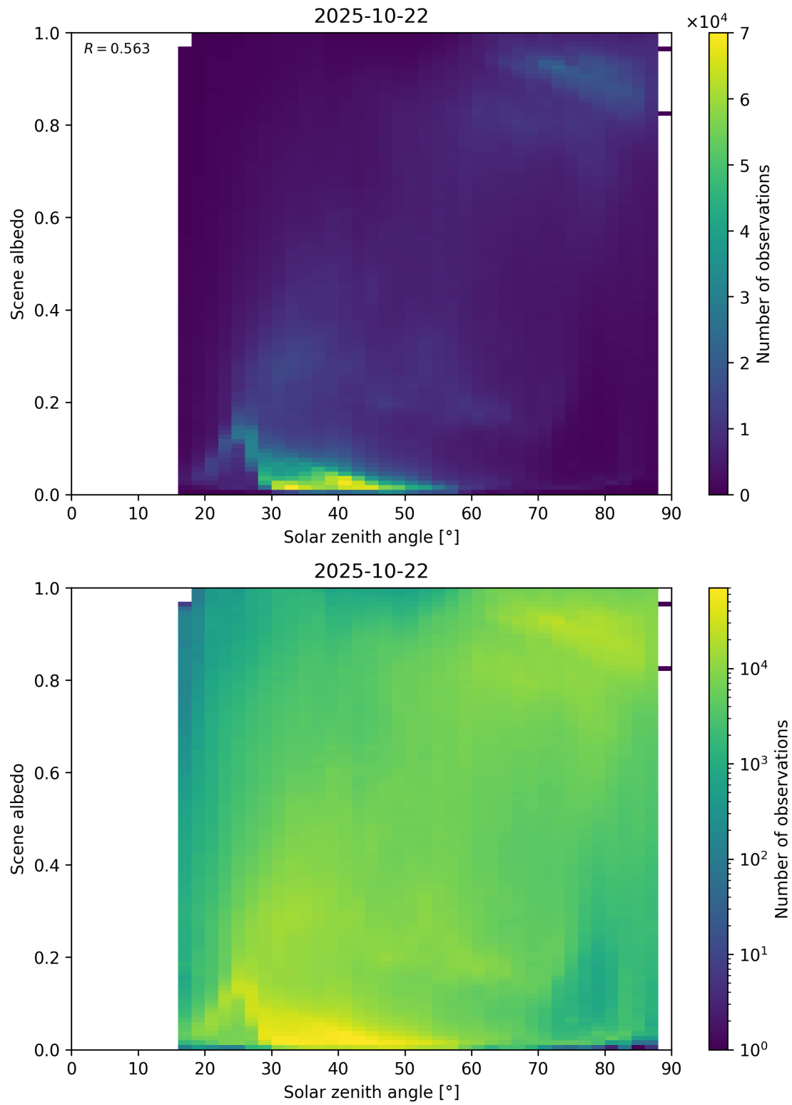
Figure 116: Scatter density plot of “Solar zenith angle” against “Scene albedo” for 2025-10-22 to 2025-10-23.
