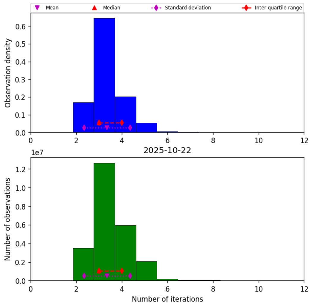
Figure 39: Histogram of “Number of iterations” for 2025-10-22 to 2025-10-23
