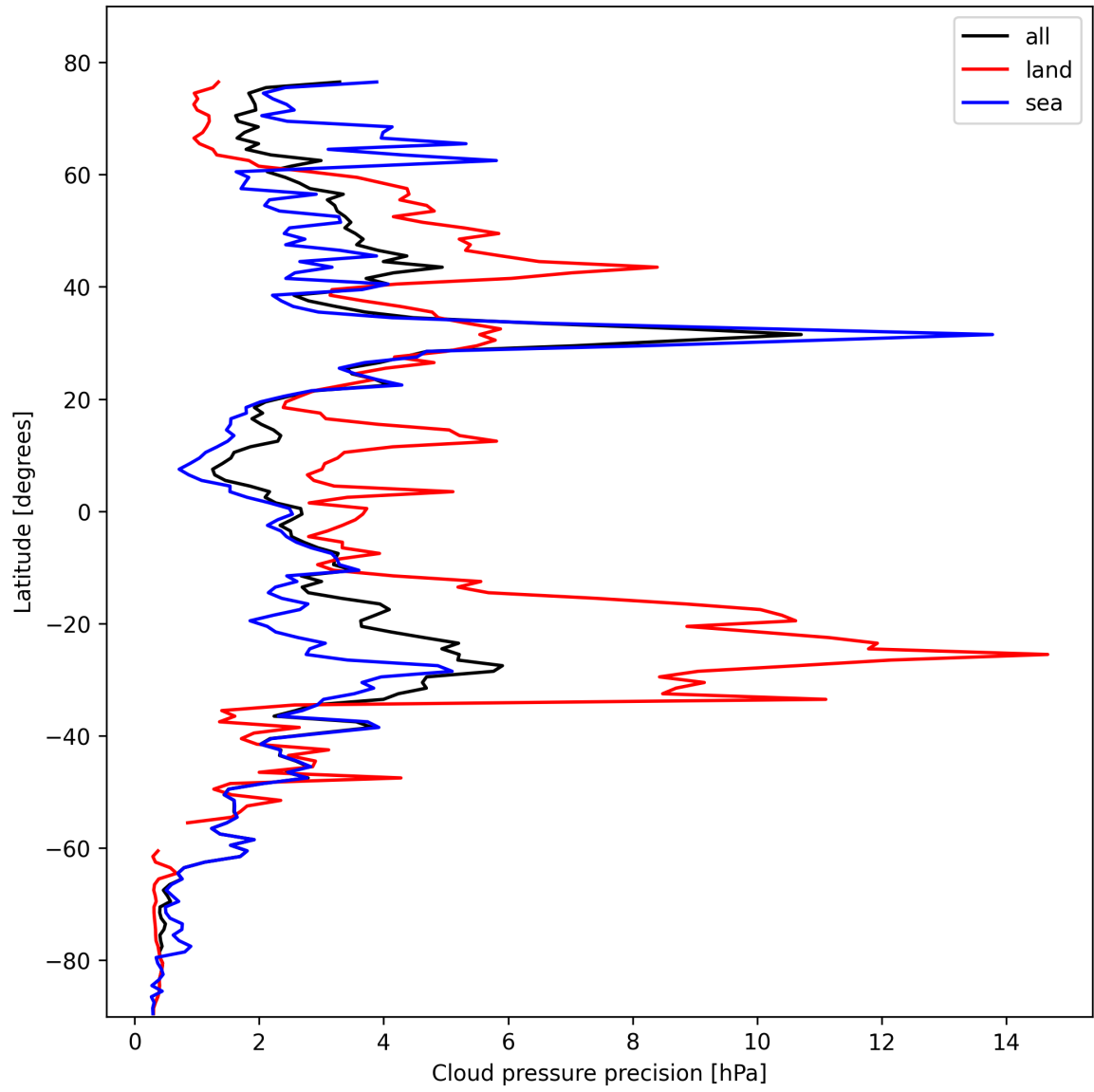
Figure 14: Zonal average of "Cloud pressure precision" for 2025-10-22 to 2025-10-23.
