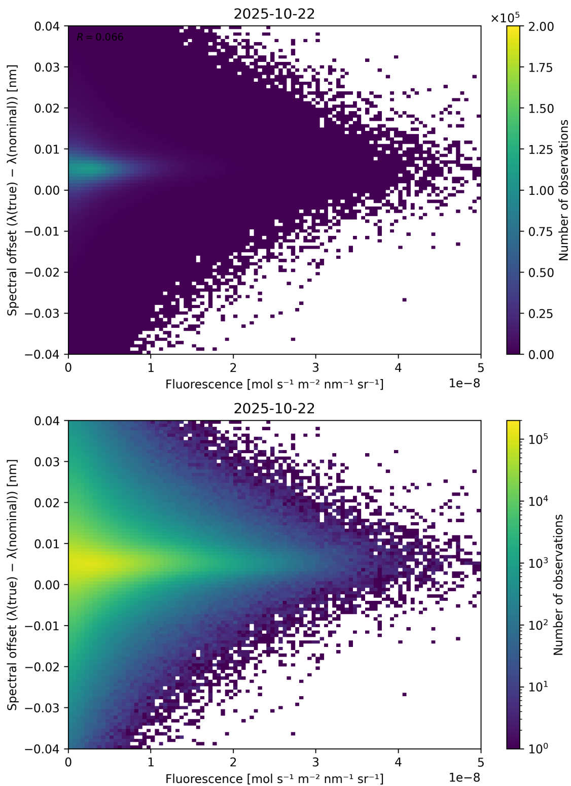
Figure 87: Scatter density plot of “Fluorescence” against “Spectral offset ( \lambda_{\text{true}} - \lambda_{\text{nominal}} )” for 2025-10-22 to 2025-10-23.
