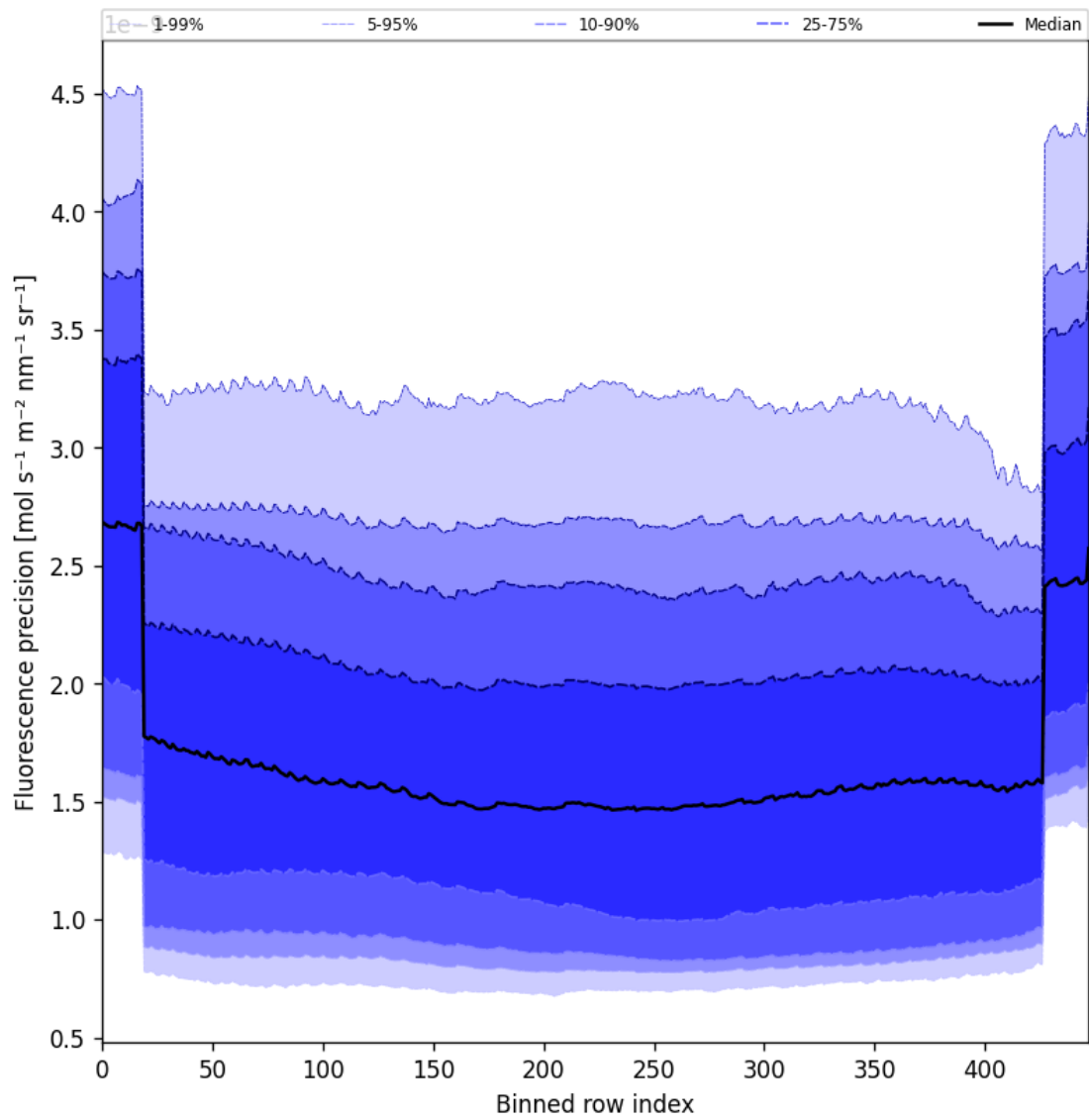
Figure 58: Along track statistics of “Fluorescence precision” for 2025-10-22 to 2025-10-23
