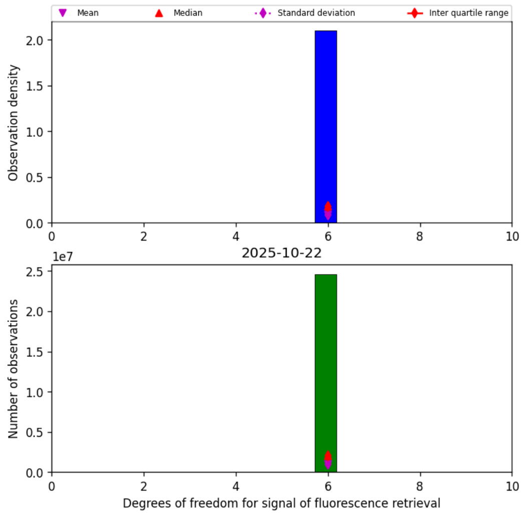
Figure 43: Histogram of “Degrees of freedom for signal of fluorescence retrieval” for 2025-10-22 to 2025-10-23
