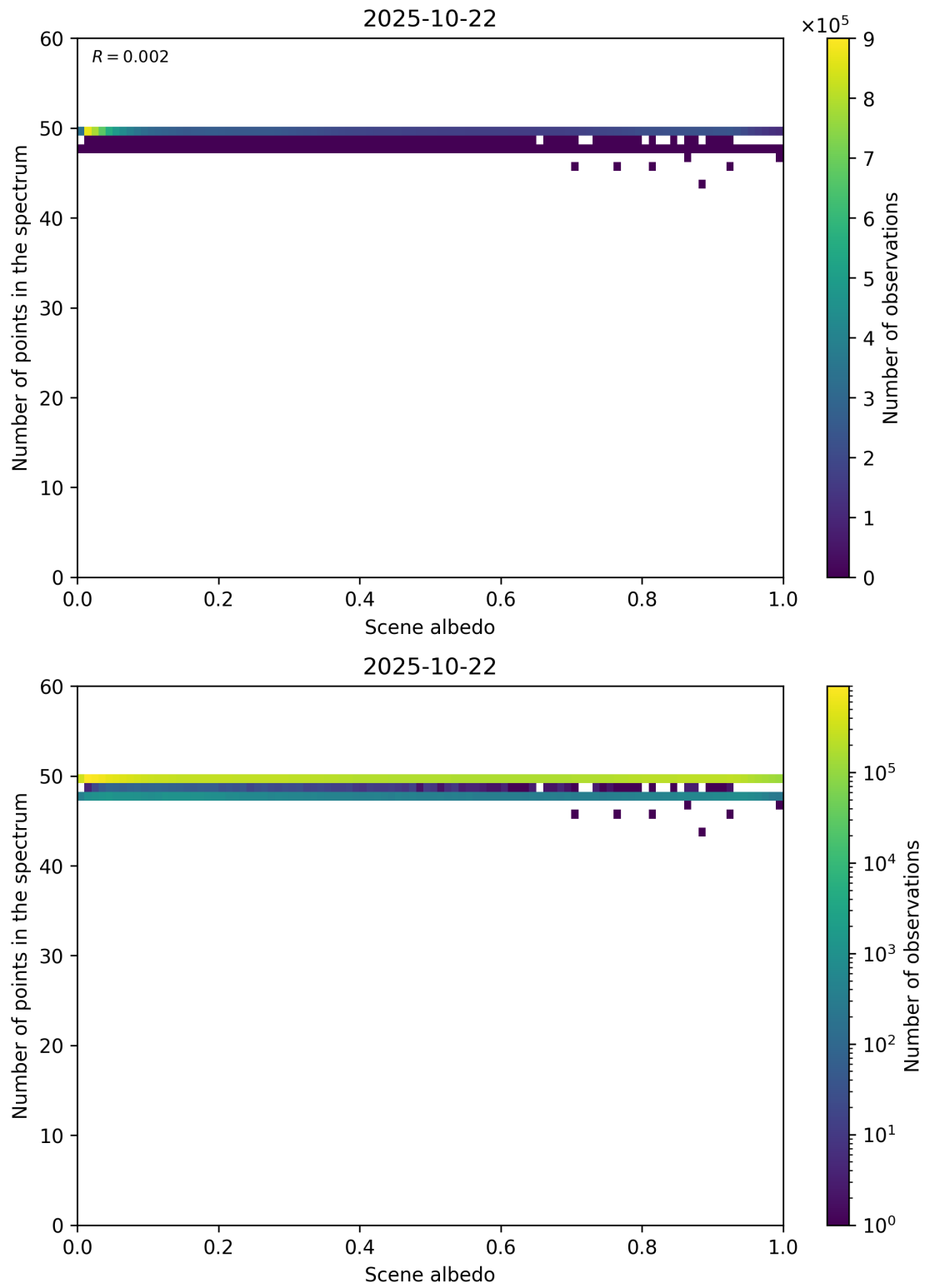
Figure 106: Scatter density plot of “Scene albedo” against “Number of points in the spectrum” for 2025-10-22 to 2025-10-23.
