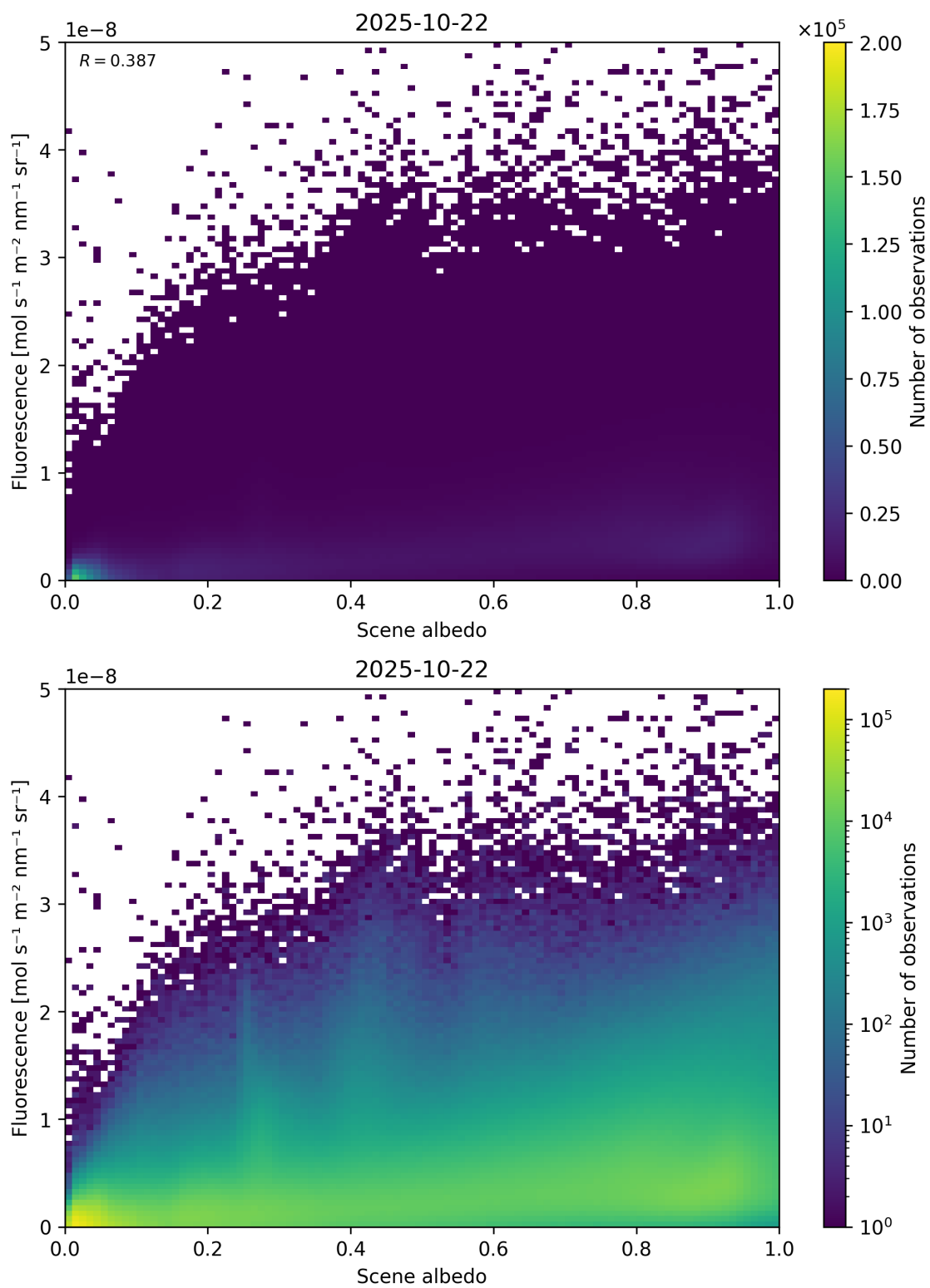
Figure 104: Scatter density plot of “Scene albedo” against “Fluorescence” for 2025-10-22 to 2025-10-23.
