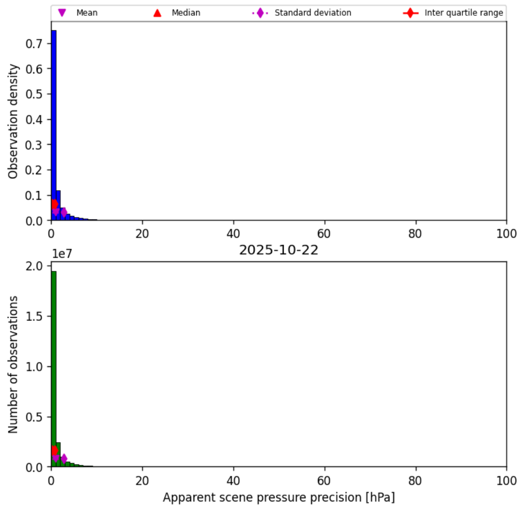
Figure 37: Histogram of "Apparent scene pressure precision" for 2025-10-22 to 2025-10-23
