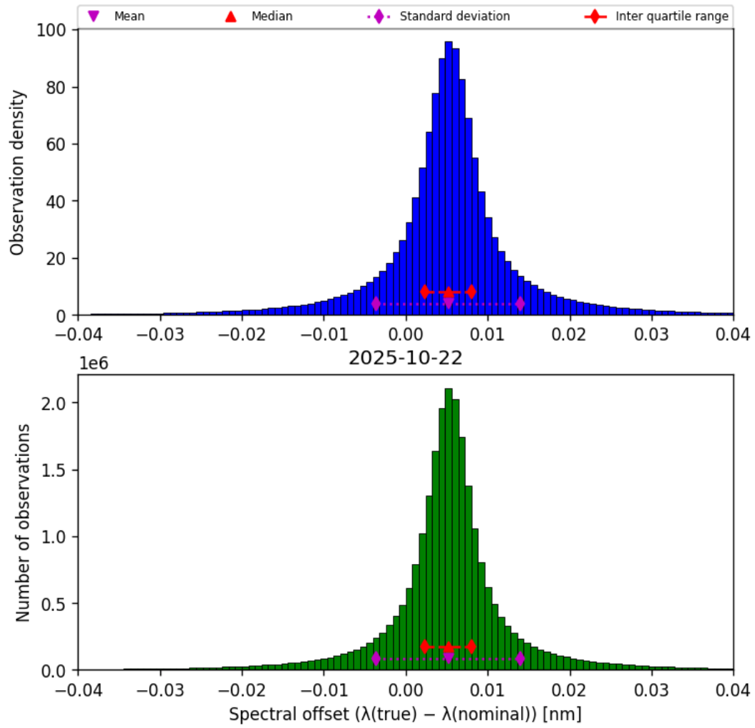
Figure 45: Histogram of “Spectral offset ( \lambda_{\text{true}} - \lambda_{\text{nominal}} )” for 2025-10-22 to 2025-10-23
