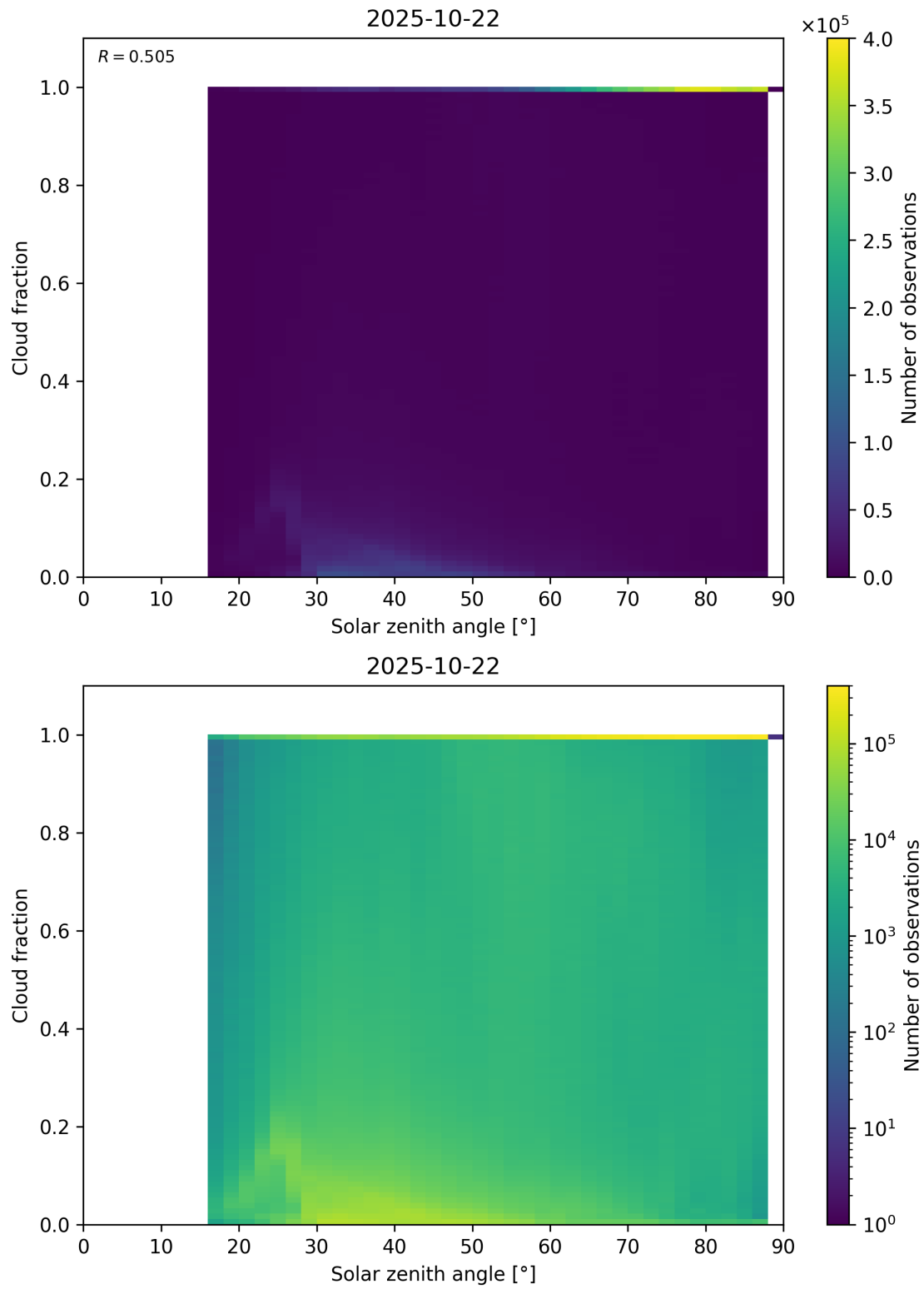
Figure 110: Scatter density plot of “Solar zenith angle” against “Cloud fraction” for 2025-10-22 to 2025-10-23.
