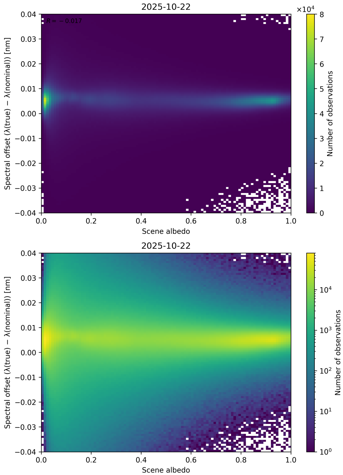
Figure 107: Scatter density plot of “Scene albedo” against “Spectral offset ( \lambda_{\text{true}} - \lambda_{\text{nominal}} )” for 2025-10-22 to 2025-10-23.
