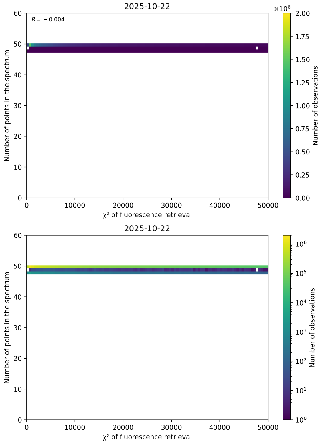
Figure 68: Scatter density plot of “ \chi^2 of fluorescence retrieval” against “Number of points in the spectrum” for 2025-10-22 to 2025-10-23.
