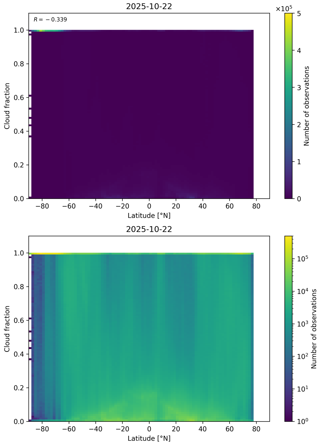
Figure 90: Scatter density plot of “Latitude” against “Cloud fraction” for 2025-10-22 to 2025-10-23.
