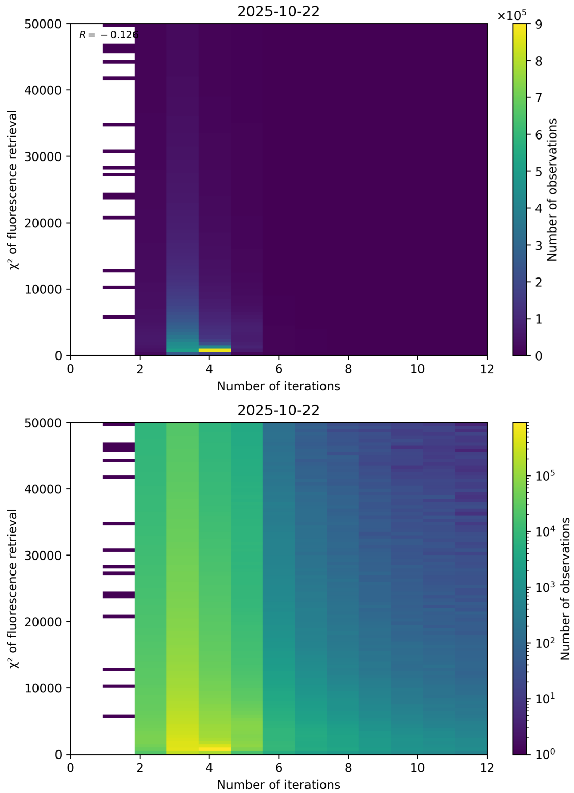
Figure 97: Scatter density plot of “Number of iterations” against “ \chi^2 of fluorescence retrieval” for 2025-10-22 to 2025-10-23.
