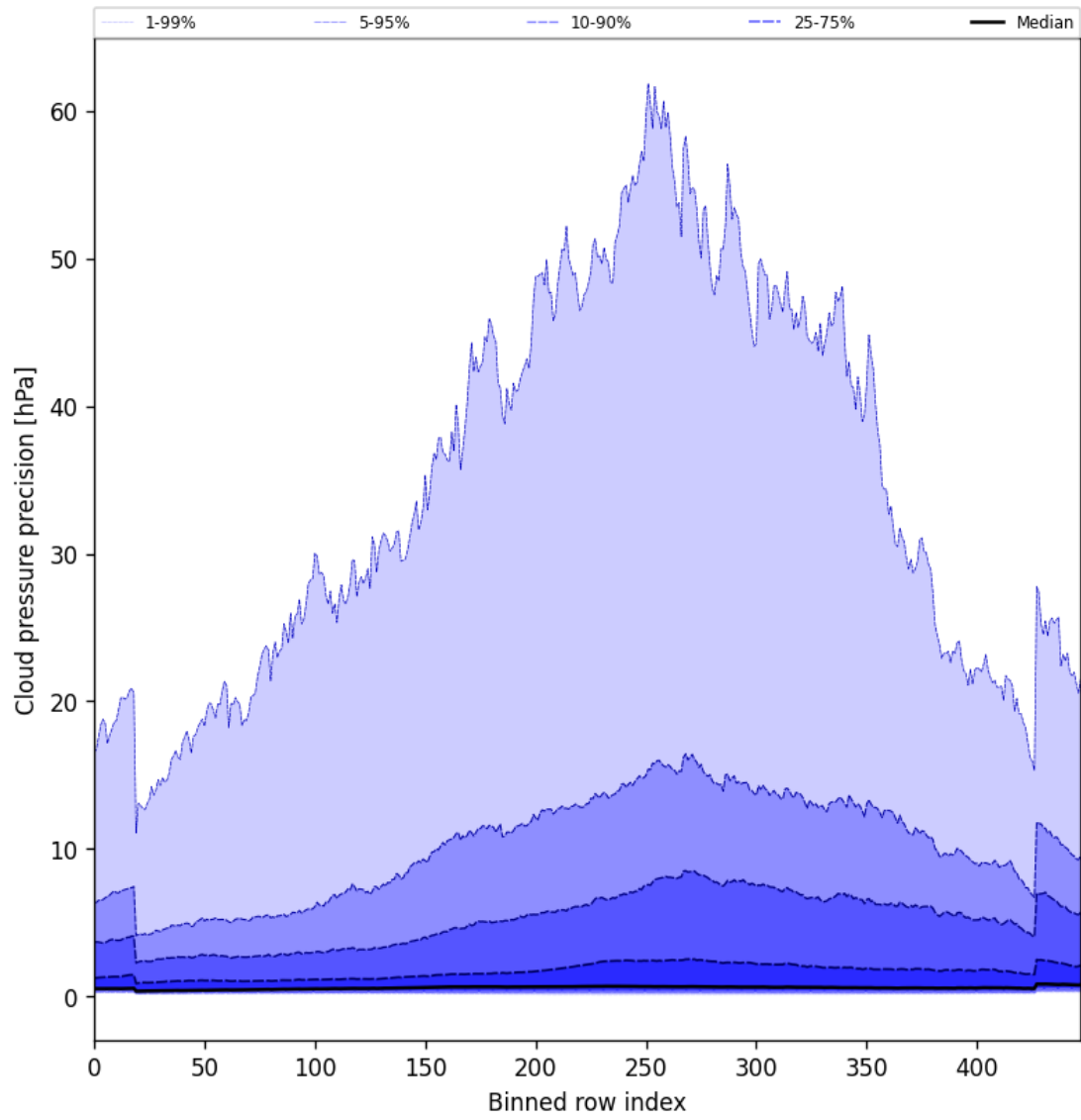
Figure 48: Along track statistics of “Cloud pressure precision” for 2025-10-22 to 2025-10-23
