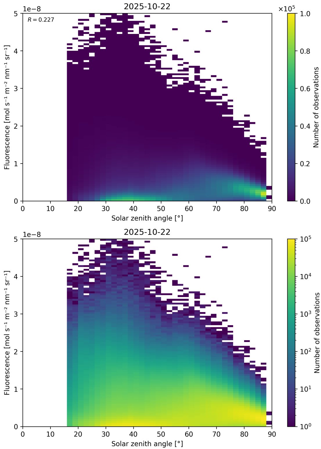
Figure 112: Scatter density plot of “Solar zenith angle” against “Fluorescence” for 2025-10-22 to 2025-10-23.
