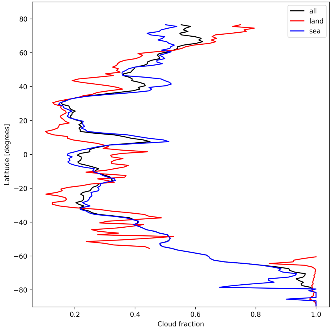
Figure 15: Zonal average of “Cloud fraction” for 2025-10-22 to 2025-10-23.
