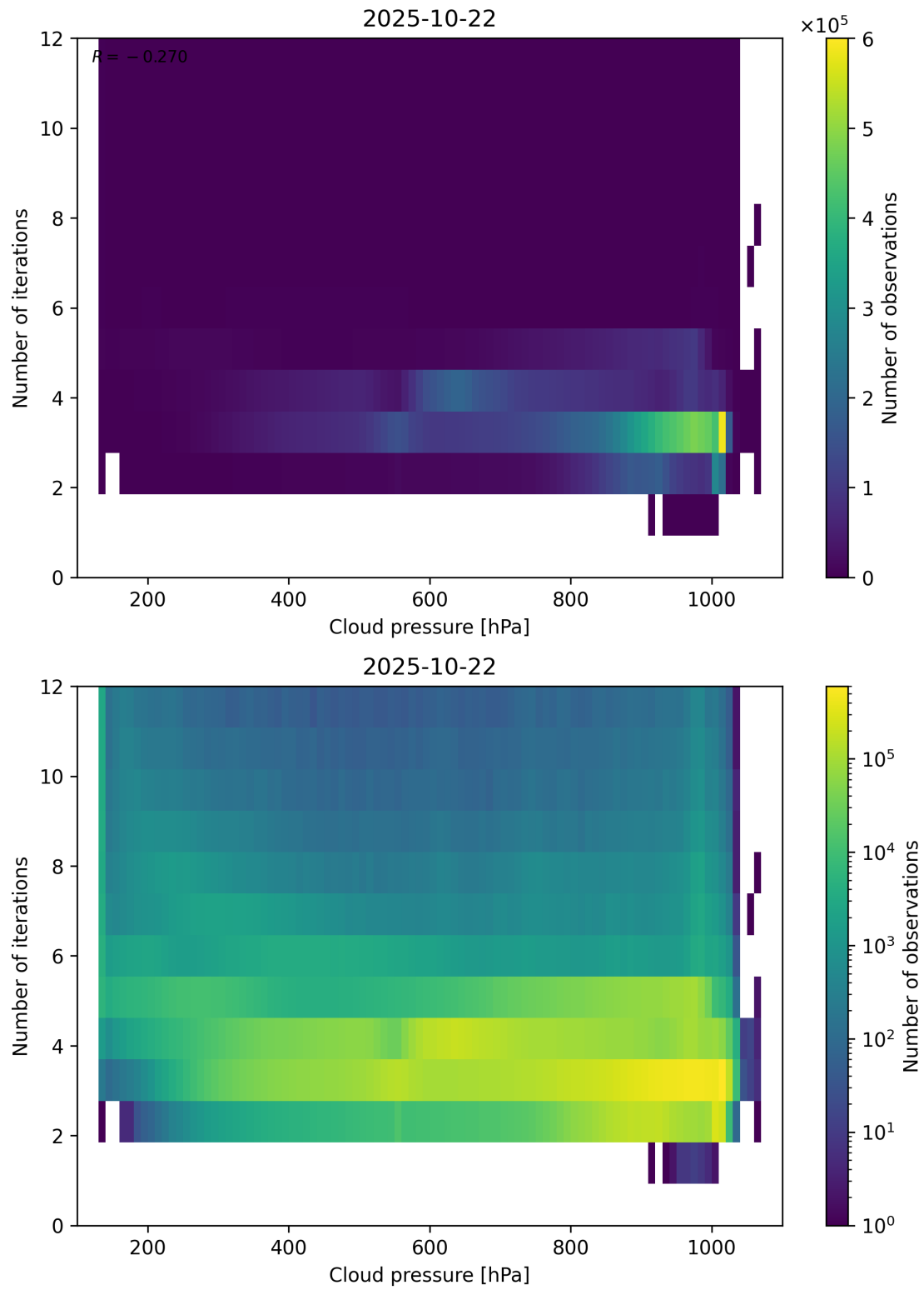
Figure 81: Scatter density plot of “Cloud pressure” against “Number of iterations” for 2025-10-22 to 2025-10-23.
