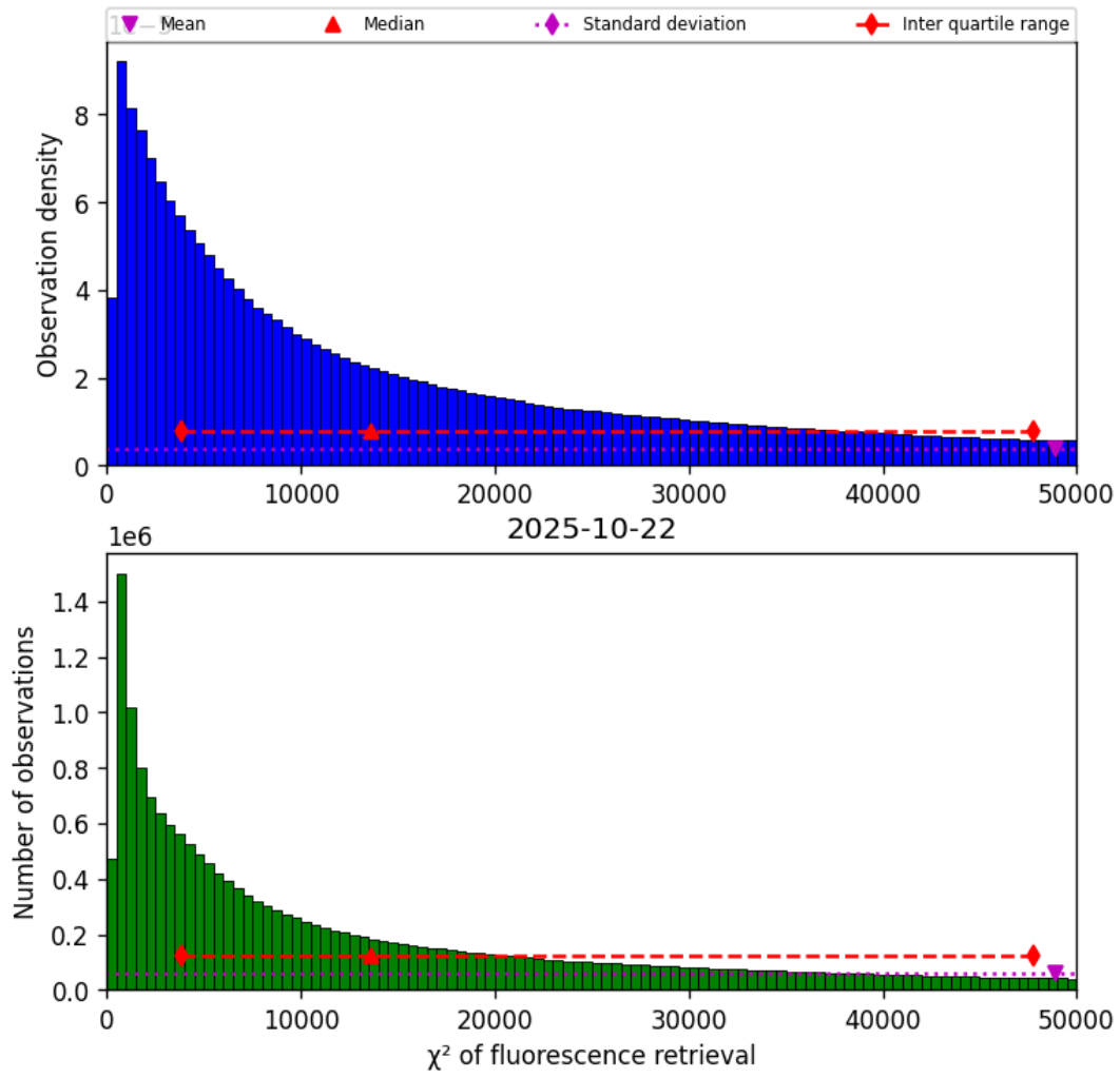
Figure 42: Histogram of “ \chi^2 of fluorescence retrieval” for 2025-10-22 to 2025-10-23
