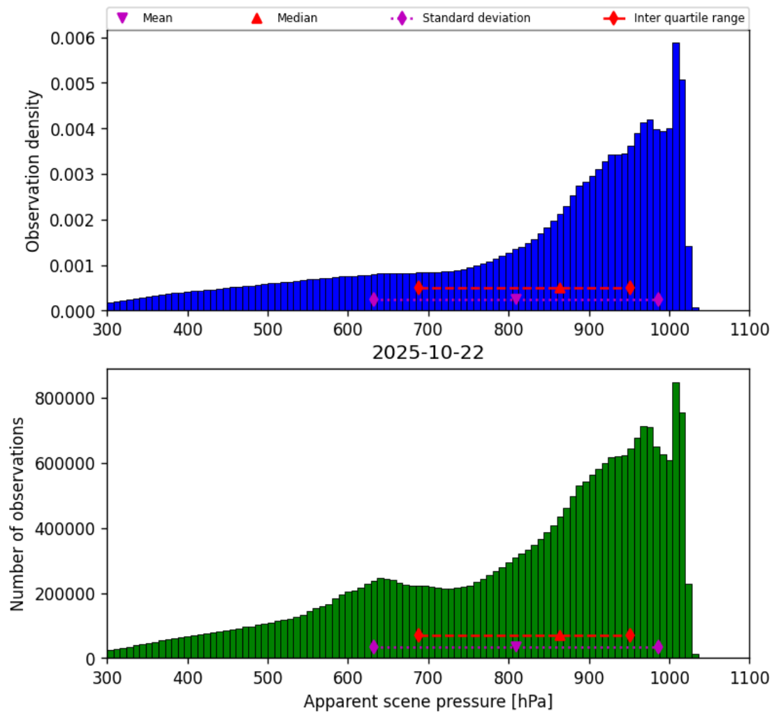
Figure 36: Histogram of “Apparent scene pressure” for 2025-10-22 to 2025-10-23
