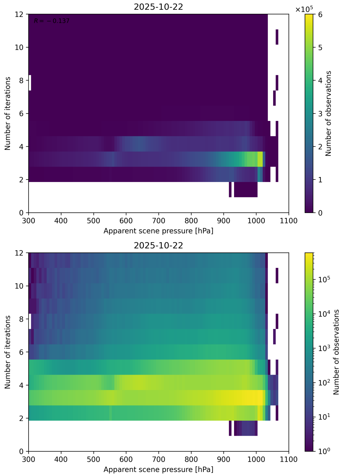
Figure 65: Scatter density plot of “Apparent scene pressure” against “Number of iterations” for 2025-10-22 to 2025-10-23.
