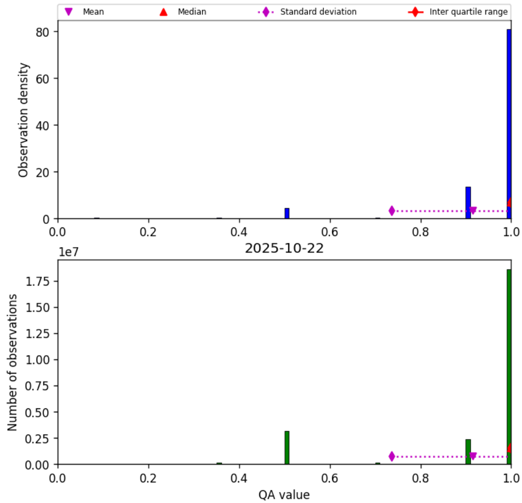
Figure 29: Histogram of “QA value” for 2025-10-22 to 2025-10-23
