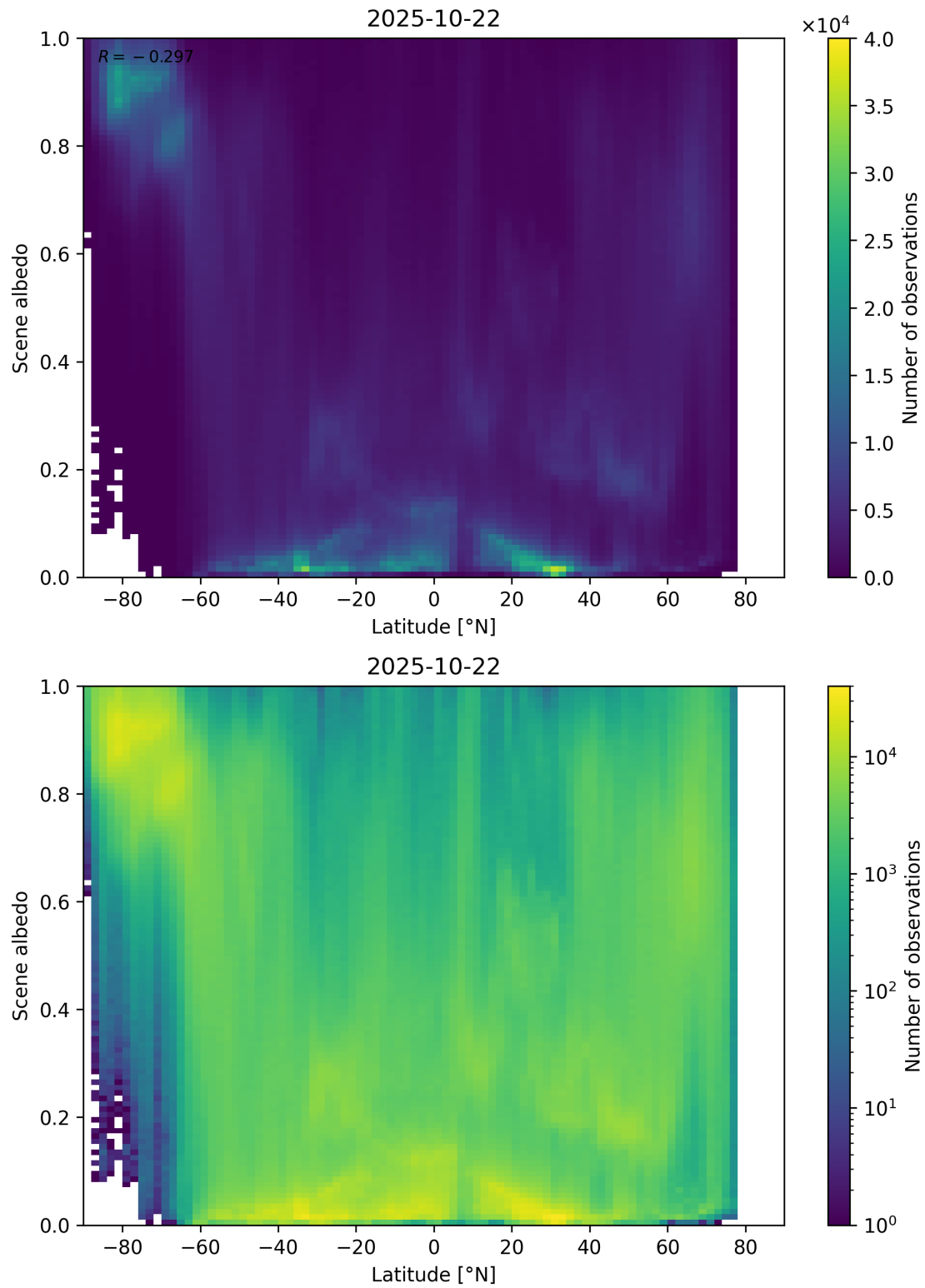
Figure 95: Scatter density plot of “Latitude” against “Scene albedo” for 2025-10-22 to 2025-10-23.
