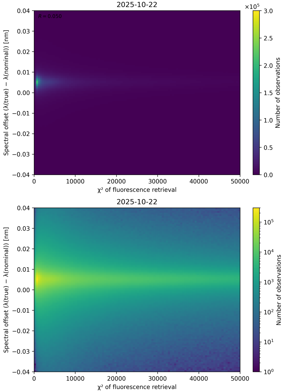
Figure 69: Scatter density plot of “ \chi^2 of fluorescence retrieval” against “Spectral offset ( \lambda_{\text{true}} - \lambda_{\text{nominal}} )” for 2025-10-22 to 2025-10-23.
