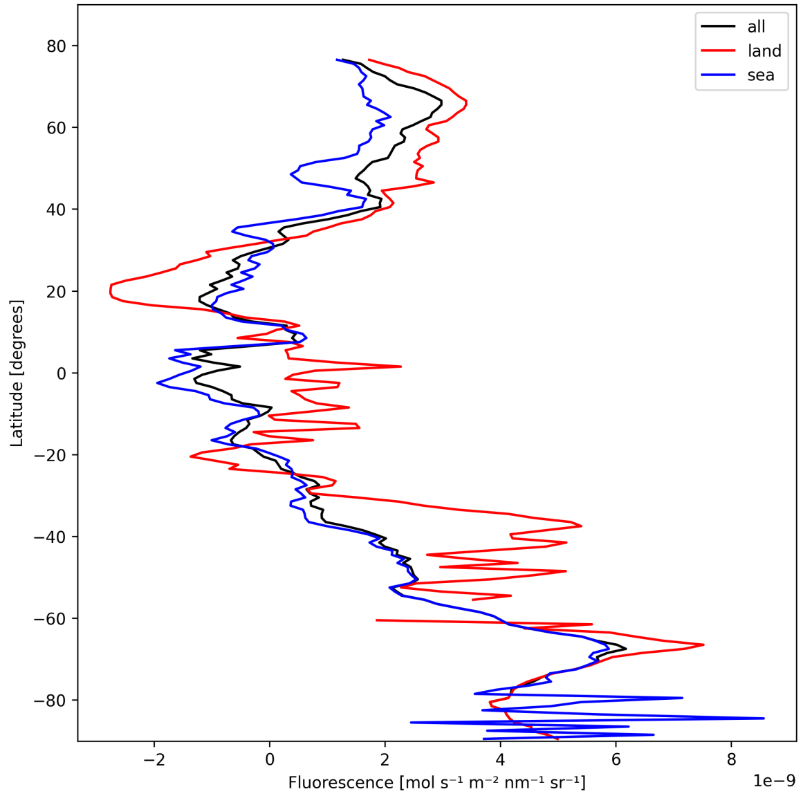
Figure 23: Zonal average of “Fluorescence” for 2025-10-22 to 2025-10-23.
