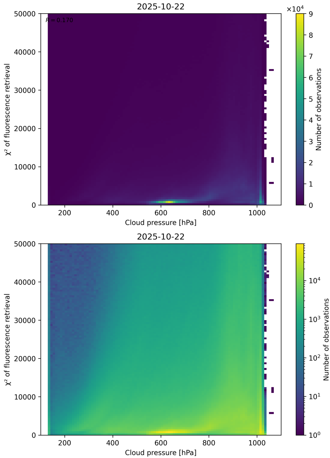
Figure 78: Scatter density plot of “Cloud pressure” against “ \chi^2 of fluorescence retrieval” for 2025-10-22 to 2025-10-23.
