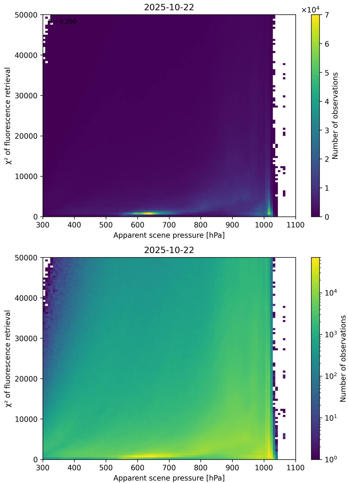
Figure 63: Scatter density plot of “Apparent scene pressure” against “ \chi^2 of fluorescence retrieval” for 2025-10-22 to 2025-10-23.
