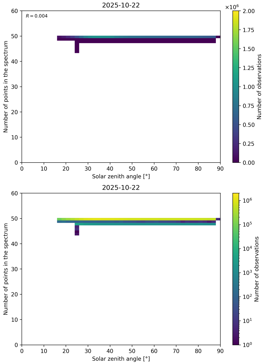
Figure 115: Scatter density plot of “Solar zenith angle” against “Number of points in the spectrum” for 2025-10-22 to 2025-10-23.
