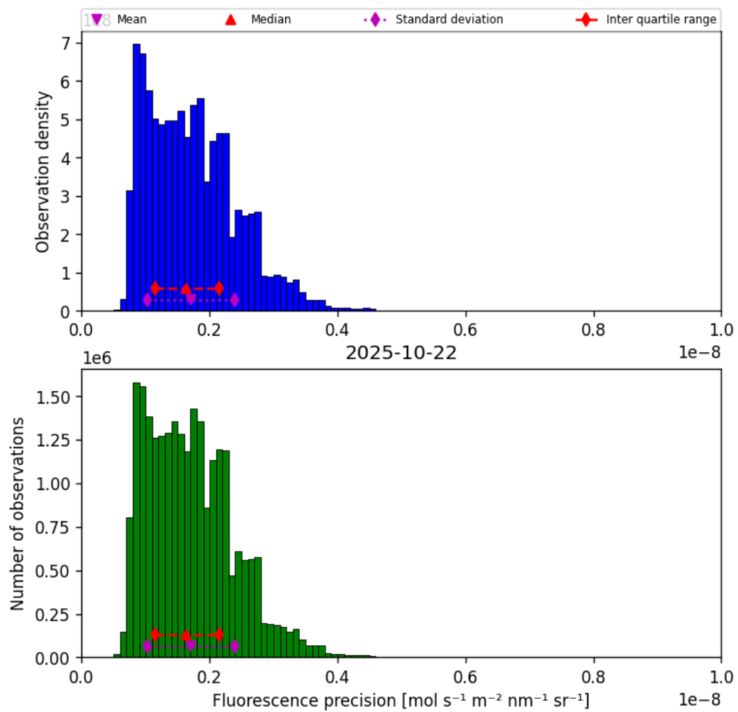
Figure 41: Histogram of “Fluorescence precision” for 2025-10-22 to 2025-10-23
