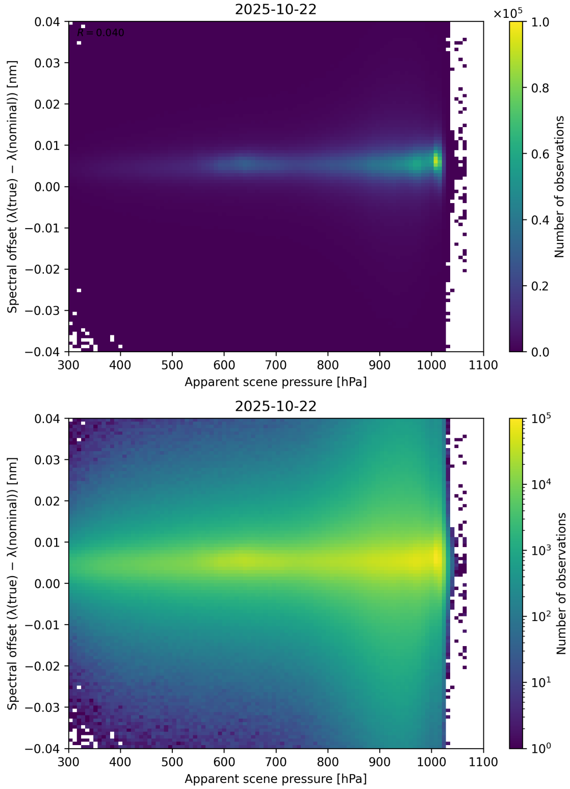
Figure 67: Scatter density plot of “Apparent scene pressure” against “Spectral offset ( \lambda_{\text{true}} - \lambda_{\text{nominal}} )” for 2025-10-22 to 2025-10-23.
