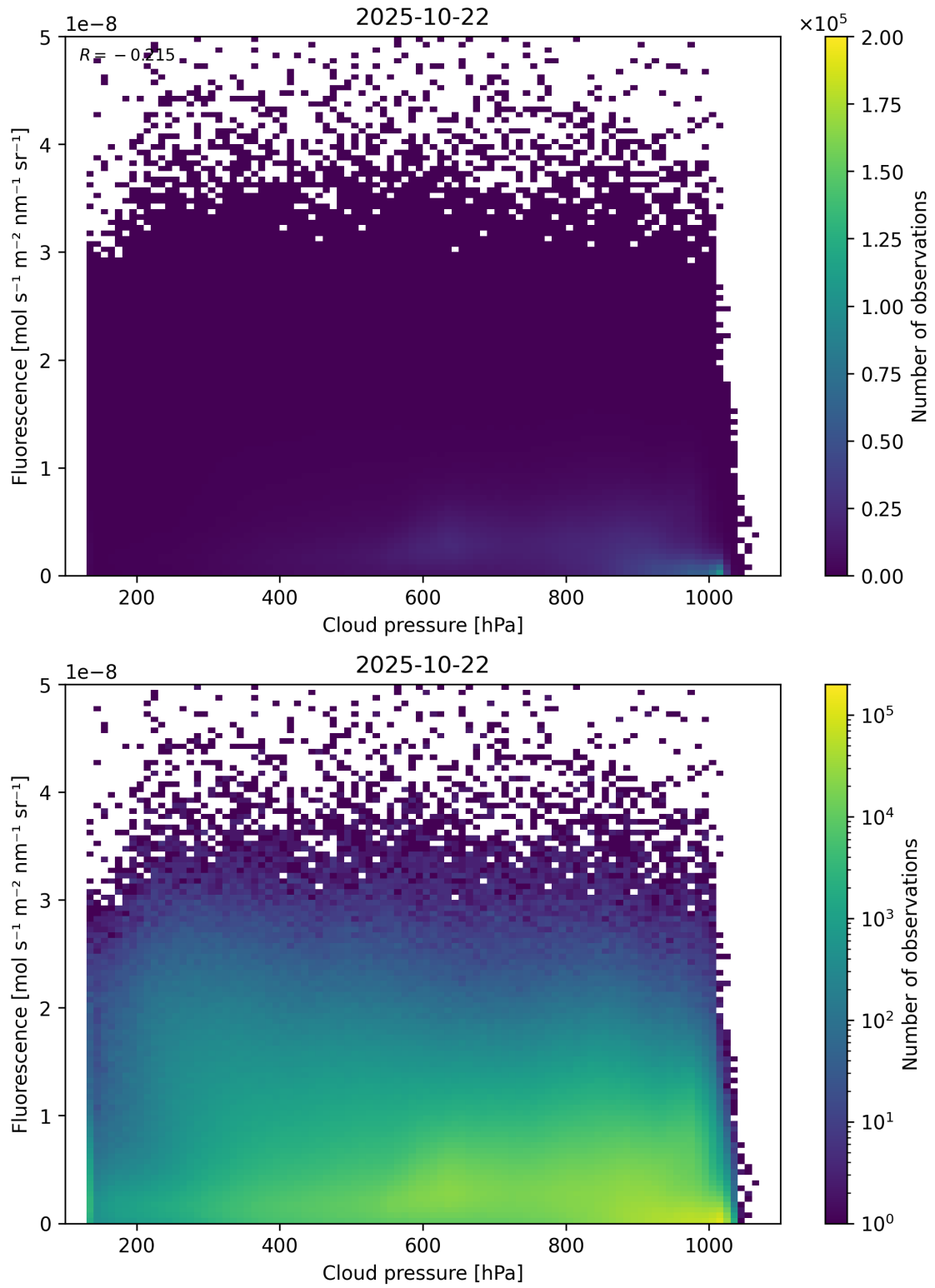
Figure 80: Scatter density plot of “Cloud pressure” against “Fluorescence” for 2025-10-22 to 2025-10-23.
