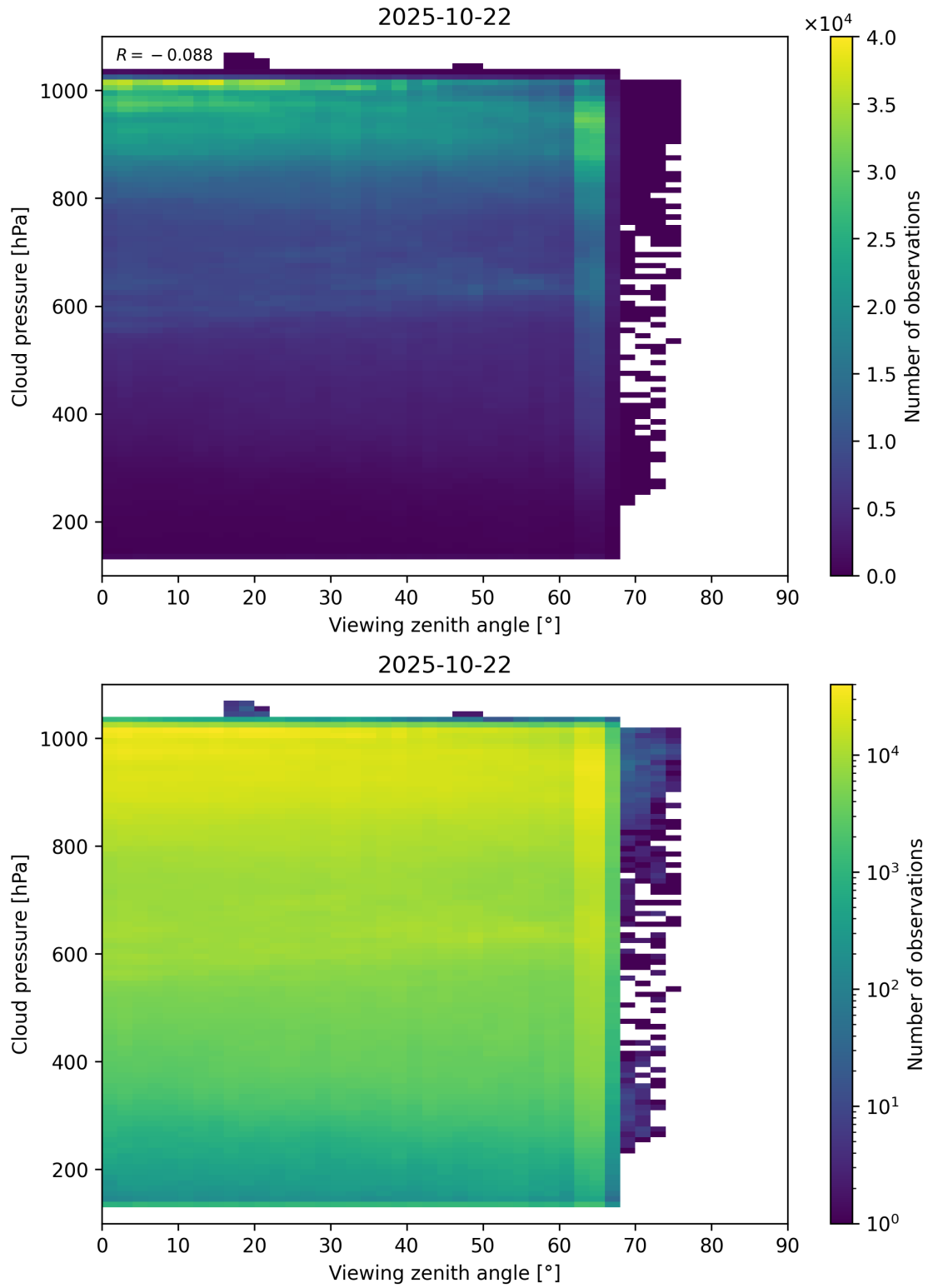
Figure 121: Scatter density plot of “Viewing zenith angle” against “Cloud pressure” for 2025-10-22 to 2025-10-23.
