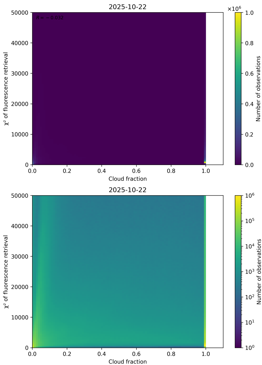
Figure 71: Scatter density plot of “Cloud fraction” against “ \chi^2 of fluorescence retrieval” for 2025-10-22 to 2025-10-23.
