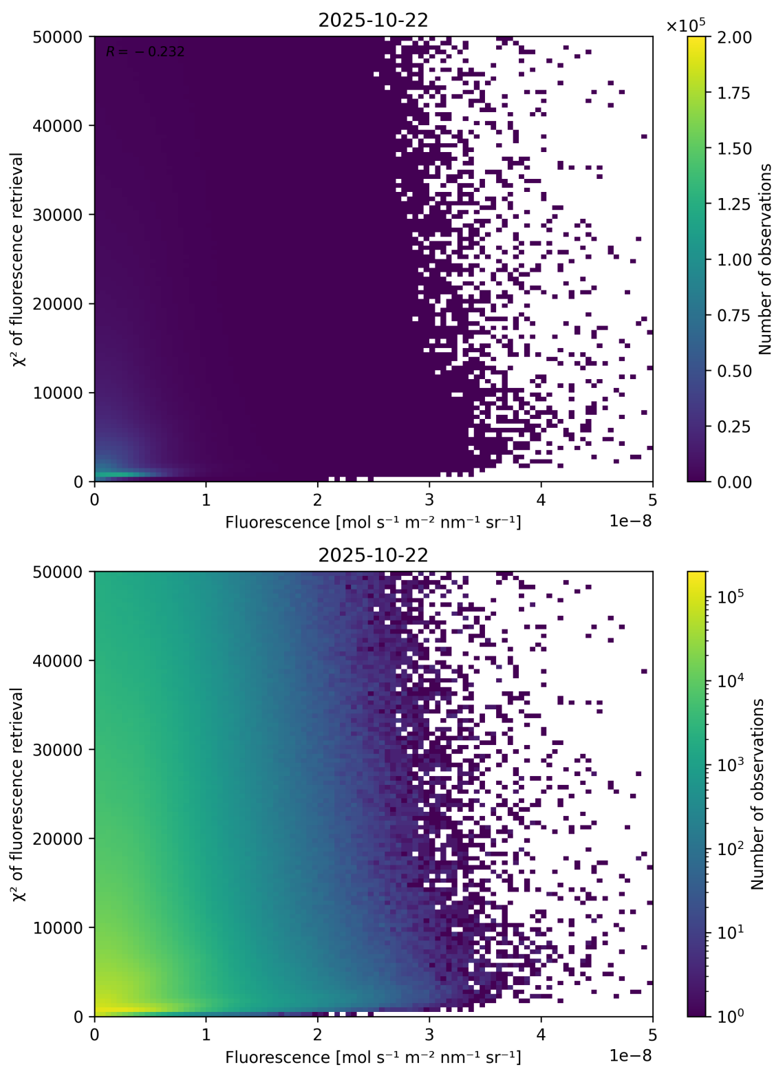
Figure 85: Scatter density plot of “Fluorescence” against “ \chi^2 of fluorescence retrieval” for 2025-10-22 to 2025-10-23.
