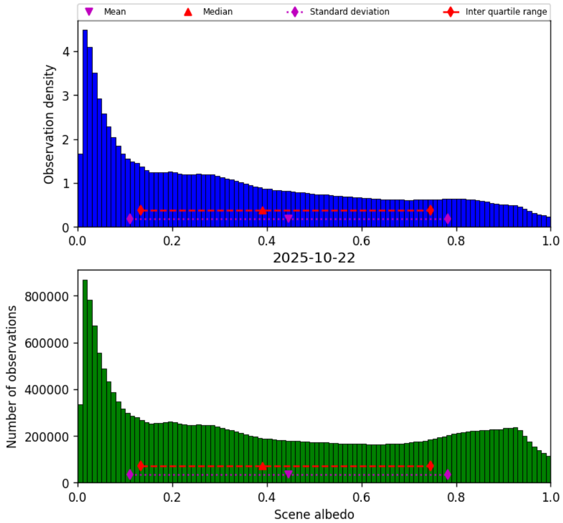
Figure 34: Histogram of “Scene albedo” for 2025-10-22 to 2025-10-23
