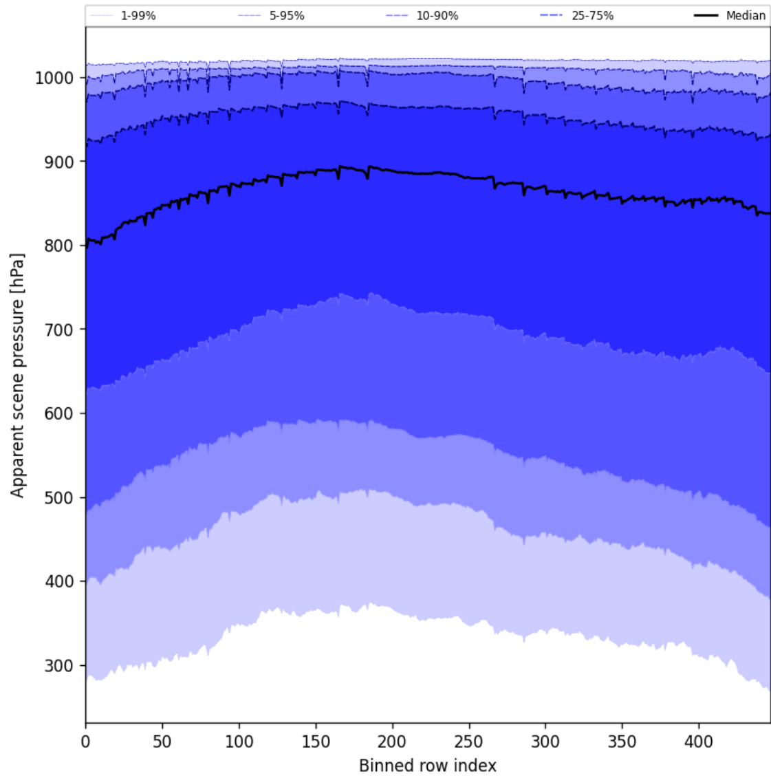
Figure 53: Along track statistics of “Apparent scene pressure” for 2025-10-22 to 2025-10-23
