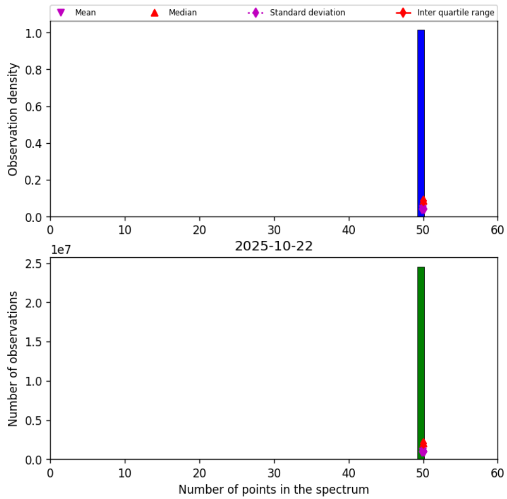
Figure 44: Histogram of “Number of points in the spectrum” for 2025-10-22 to 2025-10-23
