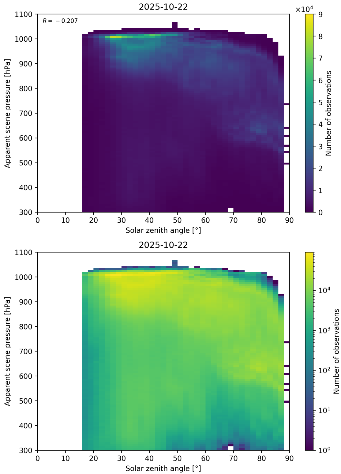
Figure 108: Scatter density plot of “Solar zenith angle” against “Apparent scene pressure” for 2025-10-22 to 2025-10-23.
