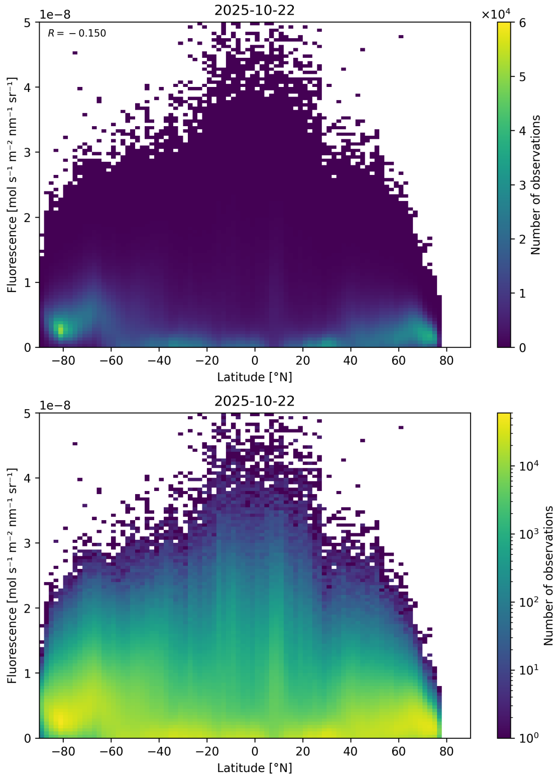
Figure 92: Scatter density plot of “Latitude” against “Fluorescence” for 2025-10-22 to 2025-10-23.
