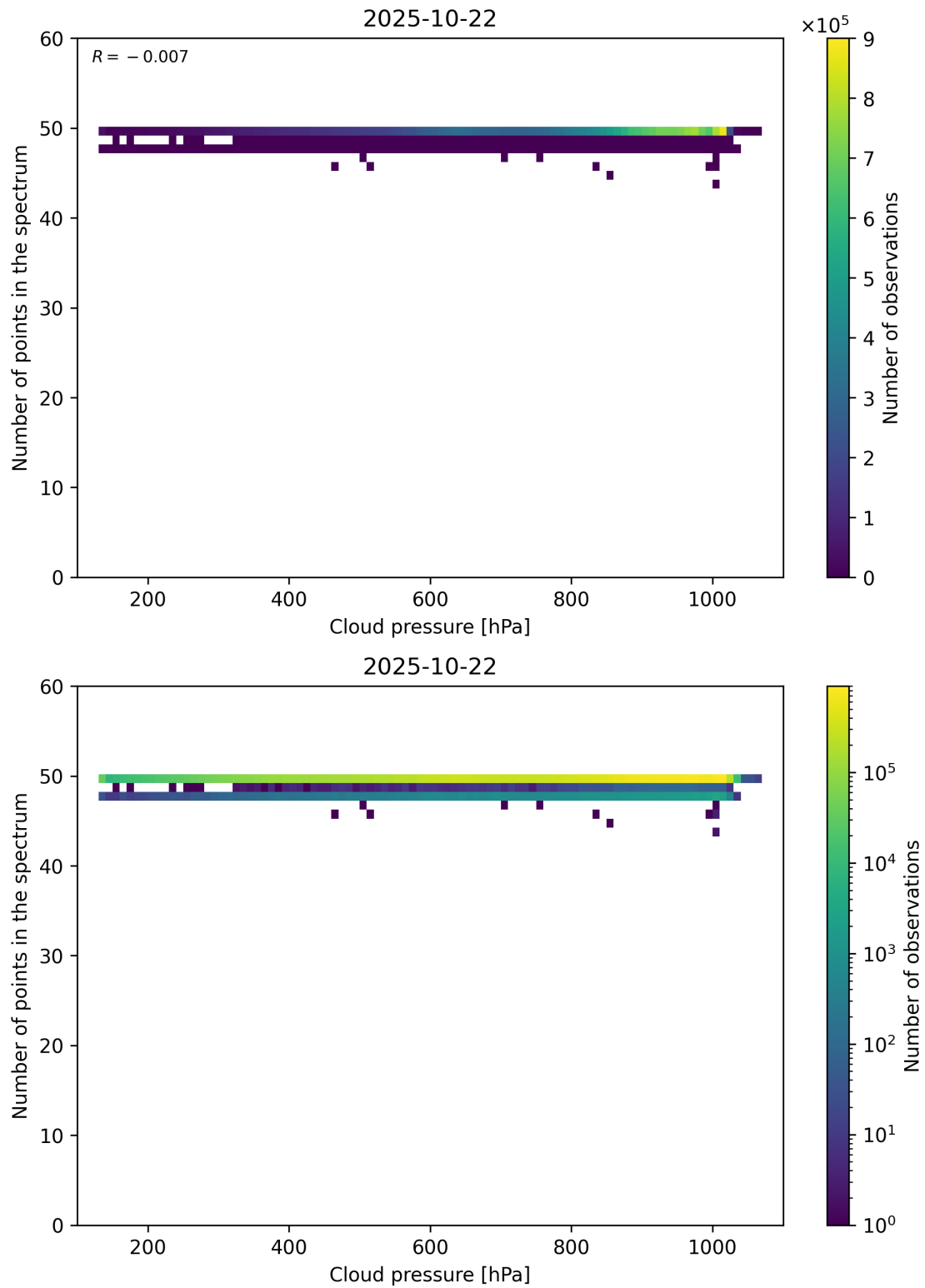
Figure 82: Scatter density plot of “Cloud pressure” against “Number of points in the spectrum” for 2025-10-22 to 2025-10-23.
