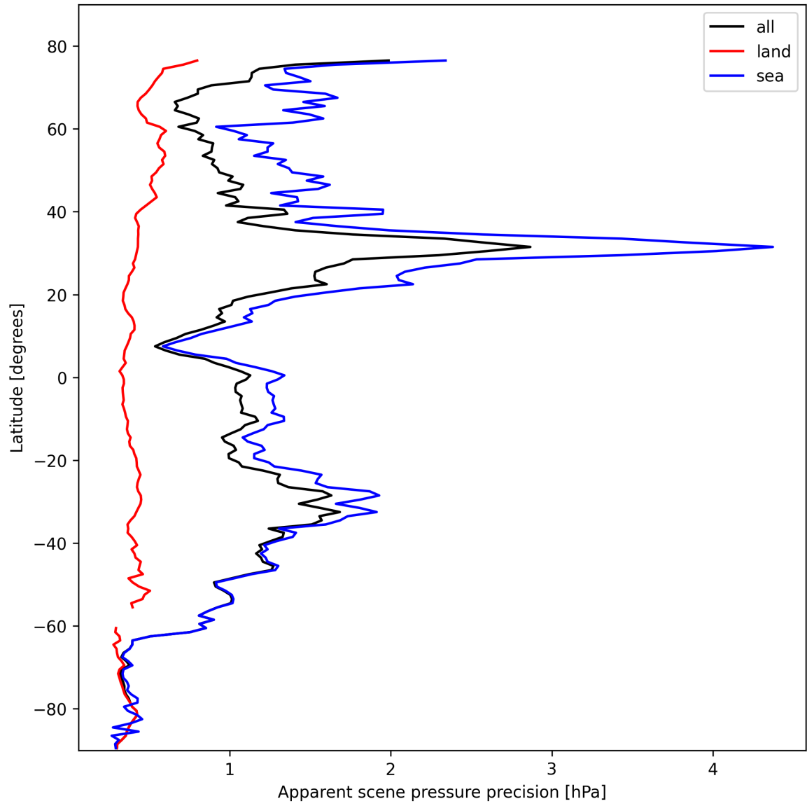
Figure 20: Zonal average of “Apparent scene pressure precision” for 2025-10-22 to 2025-10-23.
