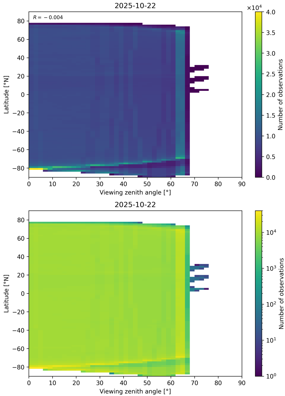
Figure 123: Scatter density plot of “Viewing zenith angle” against “Latitude” for 2025-10-22 to 2025-10-23.
