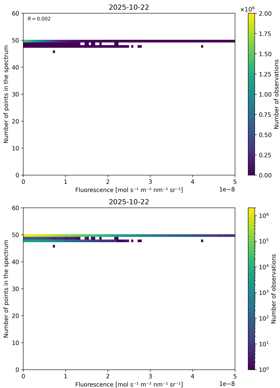
Figure 86: Scatter density plot of “Fluorescence” against “Number of points in the spectrum” for 2025-10-22 to 2025-10-23.
