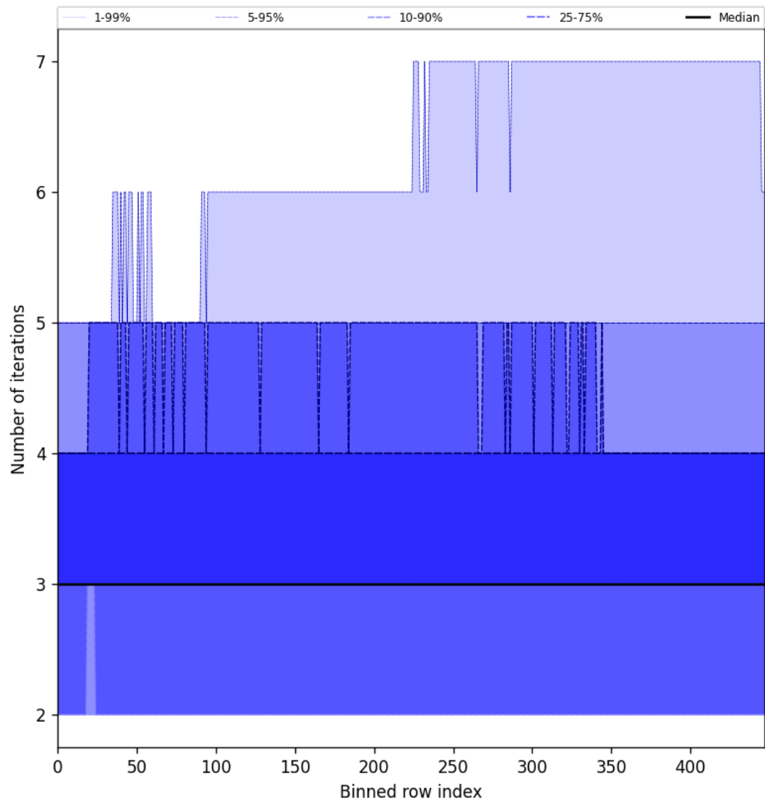
Figure 56: Along track statistics of “Number of iterations” for 2025-10-22 to 2025-10-23
