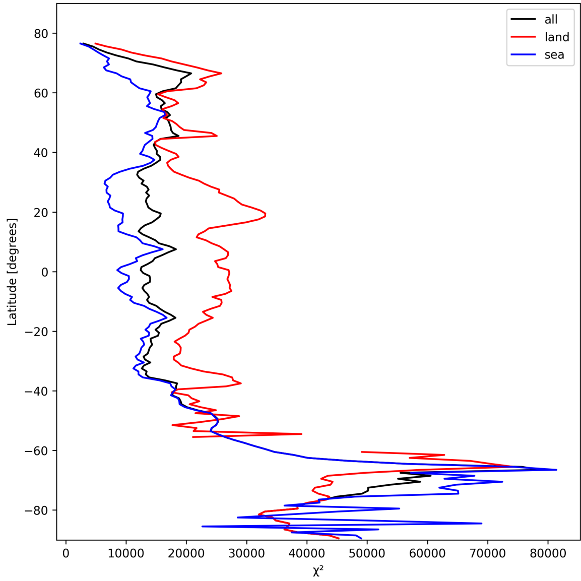
Figure 21: Zonal average of “ \chi^2 ” for 2025-10-22 to 2025-10-23.
