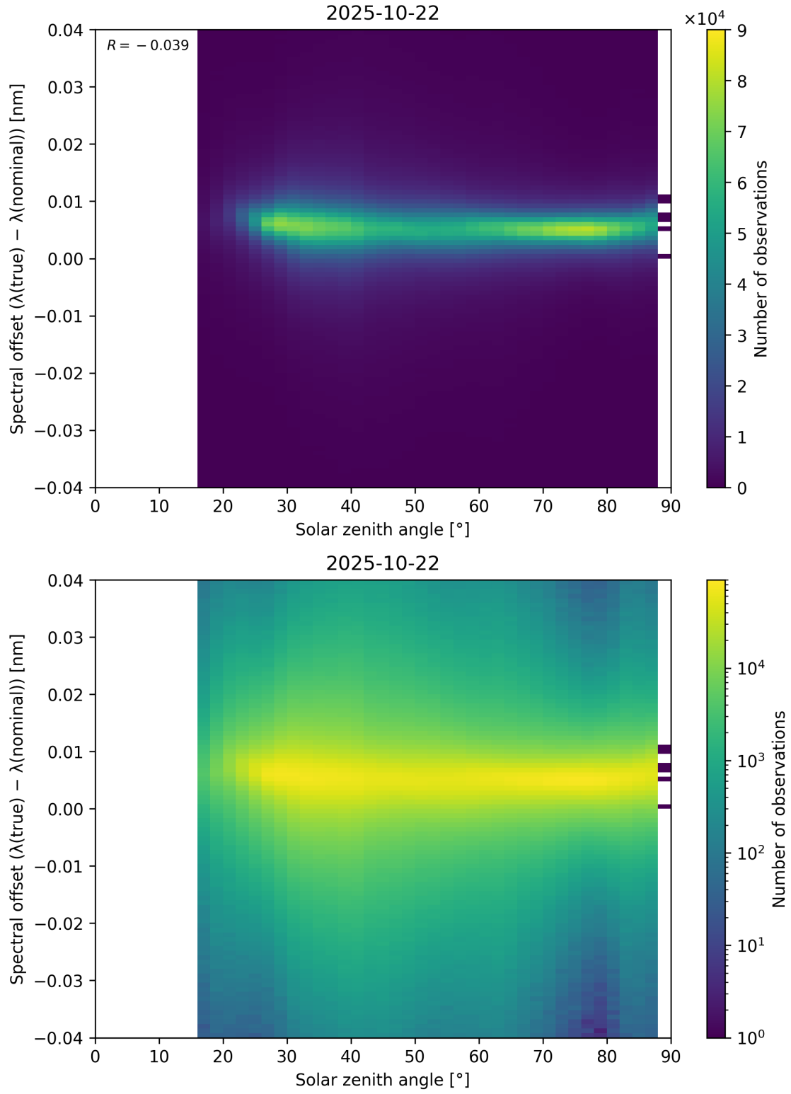
Figure 117: Scatter density plot of “Solar zenith angle” against “Spectral offset ( \lambda_{\text{true}} - \lambda_{\text{nominal}} )” for 2025-10-22 to 2025-10-23.
