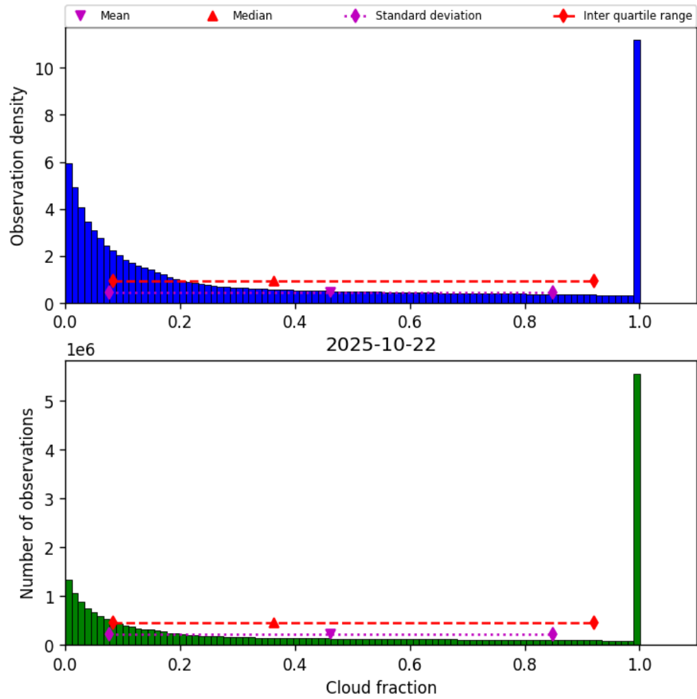
Figure 32: Histogram of “Cloud fraction” for 2025-10-22 to 2025-10-23
