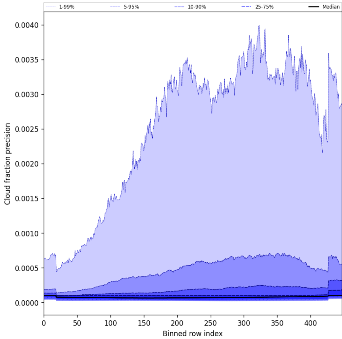
Figure 50: Along track statistics of “Cloud fraction precision” for 2025-10-22 to 2025-10-23
