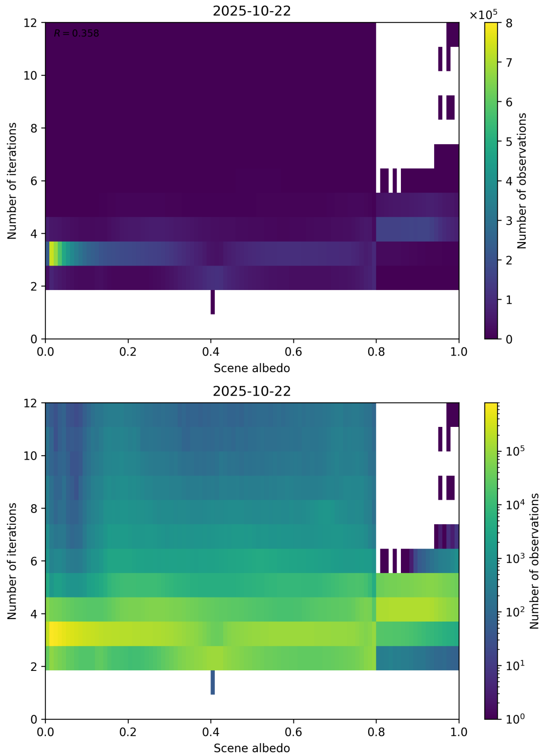
Figure 105: Scatter density plot of “Scene albedo” against “Number of iterations” for 2025-10-22 to 2025-10-23.
