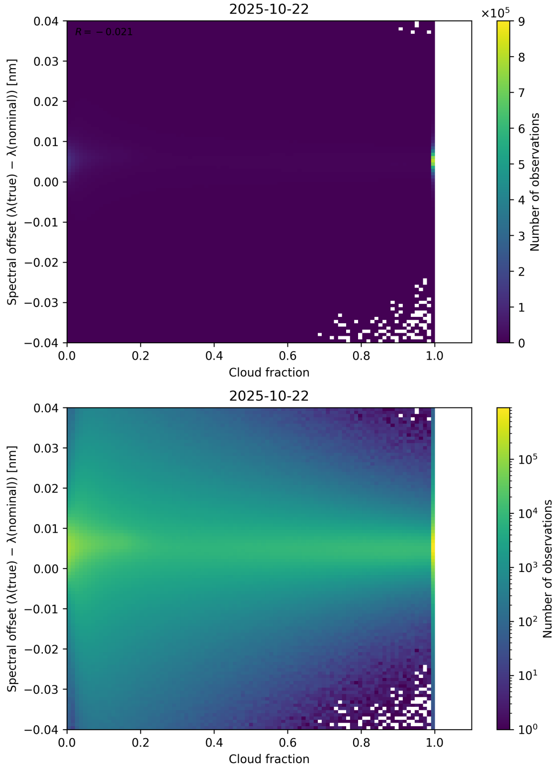
Figure 76: Scatter density plot of “Cloud fraction” against “Spectral offset ( \lambda_{\text{true}} - \lambda_{\text{nominal}} )” for 2025-10-22 to 2025-10-23.
