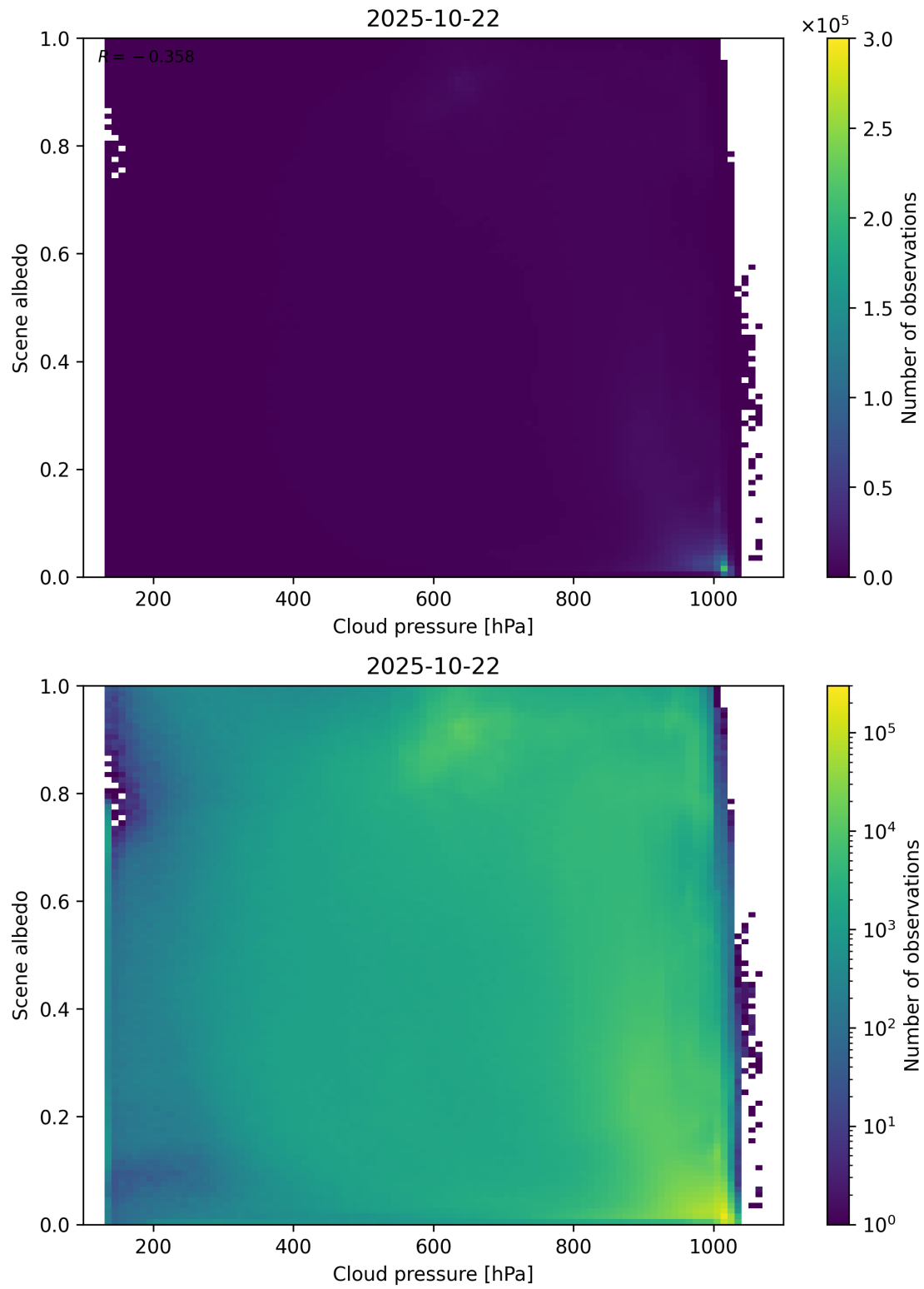
Figure 83: Scatter density plot of “Cloud pressure” against “Scene albedo” for 2025-10-22 to 2025-10-23.
