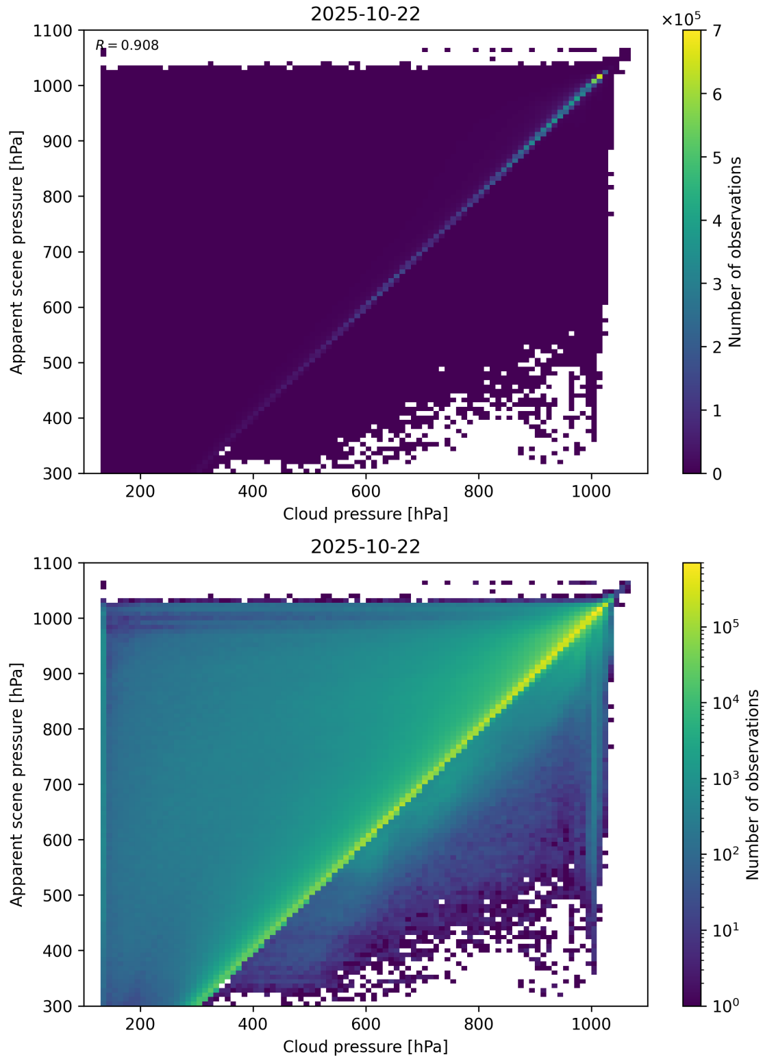
Figure 77: Scatter density plot of “Cloud pressure” against “Apparent scene pressure” for 2025-10-22 to 2025-10-23.
