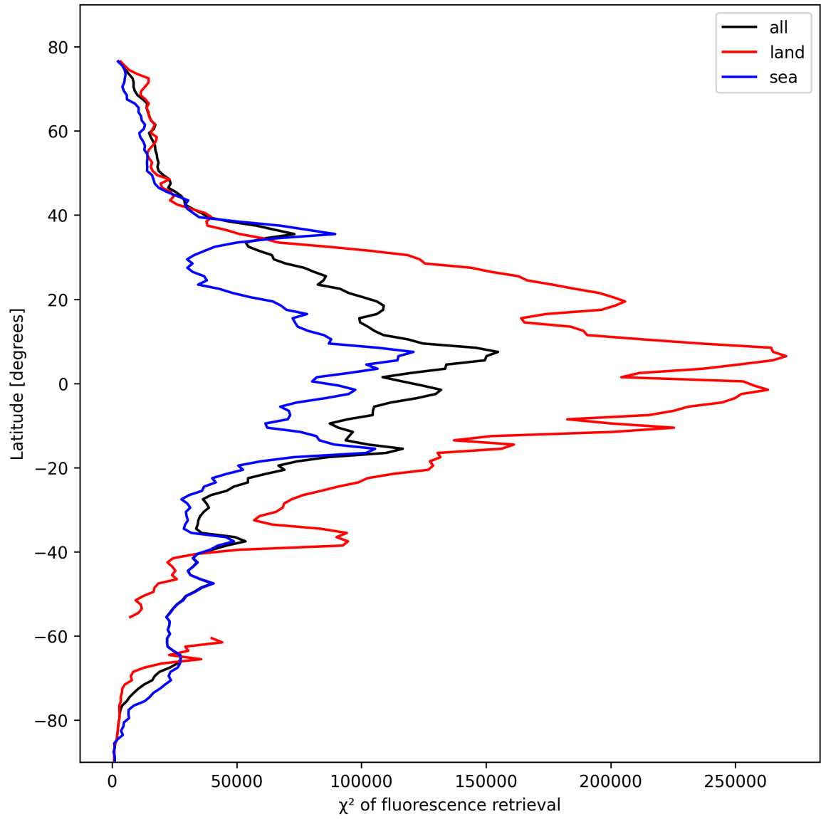
Figure 25: Zonal average of “ \chi^2 of fluorescence retrieval” for 2025-10-22 to 2025-10-23.
