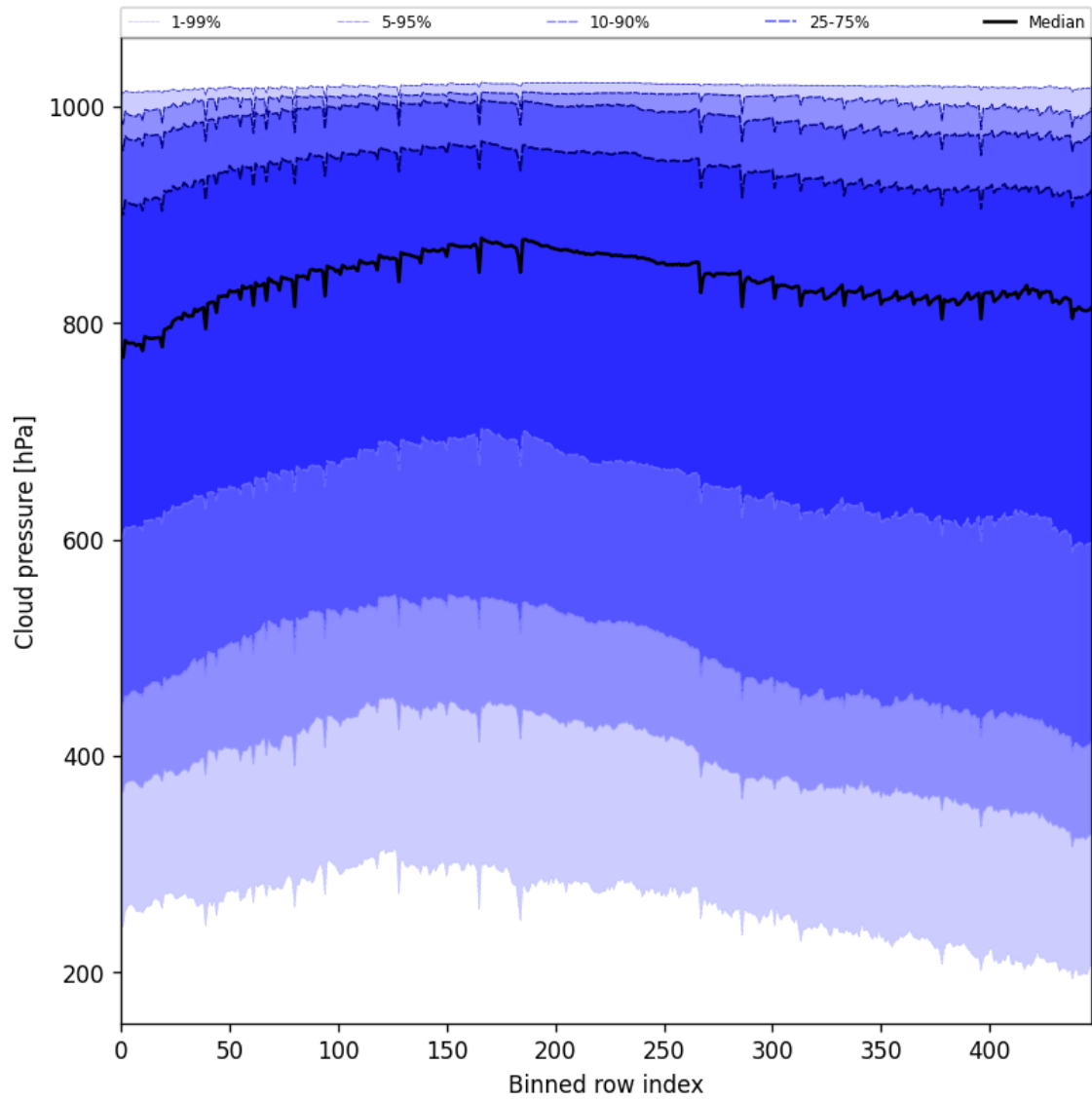
Figure 47: Along track statistics of “Cloud pressure” for 2025-10-22 to 2025-10-23
