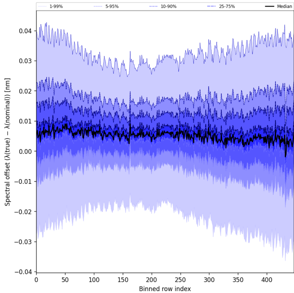
Figure 62: Along track statistics of “Spectral offset (\lambda_{\text{true}} - \lambda_{\text{nominal}}) ” for 2025-10-22 to 2025-10-23
