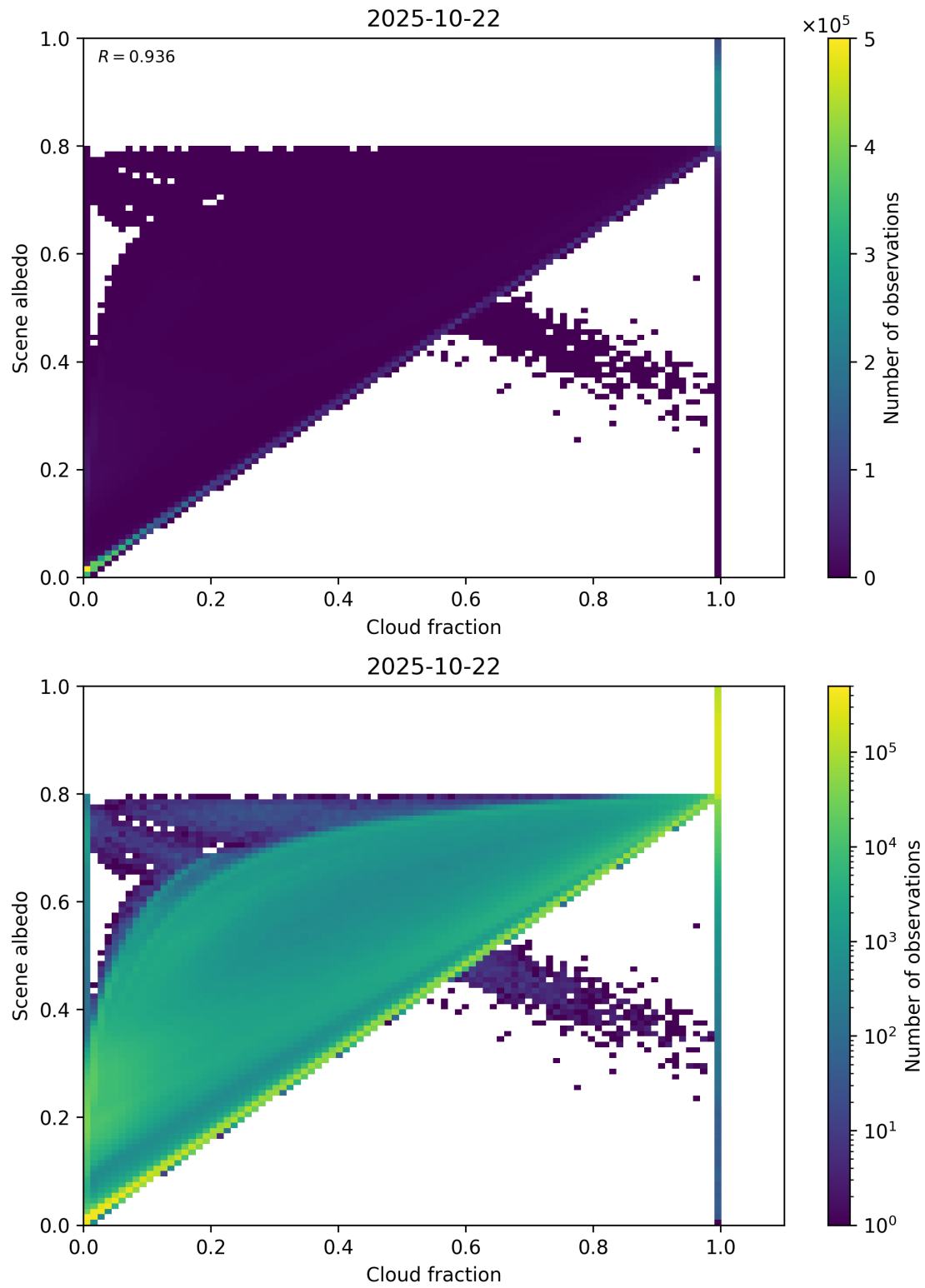
Figure 75: Scatter density plot of “Cloud fraction” against “Scene albedo” for 2025-10-22 to 2025-10-23.
