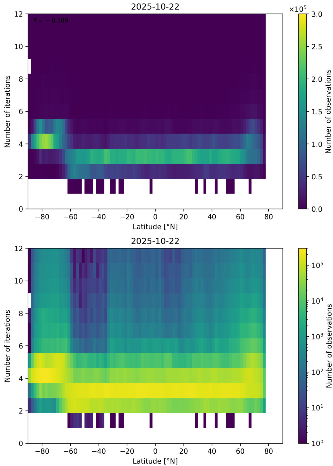
Figure 93: Scatter density plot of “Latitude” against “Number of iterations” for 2025-10-22 to 2025-10-23.
