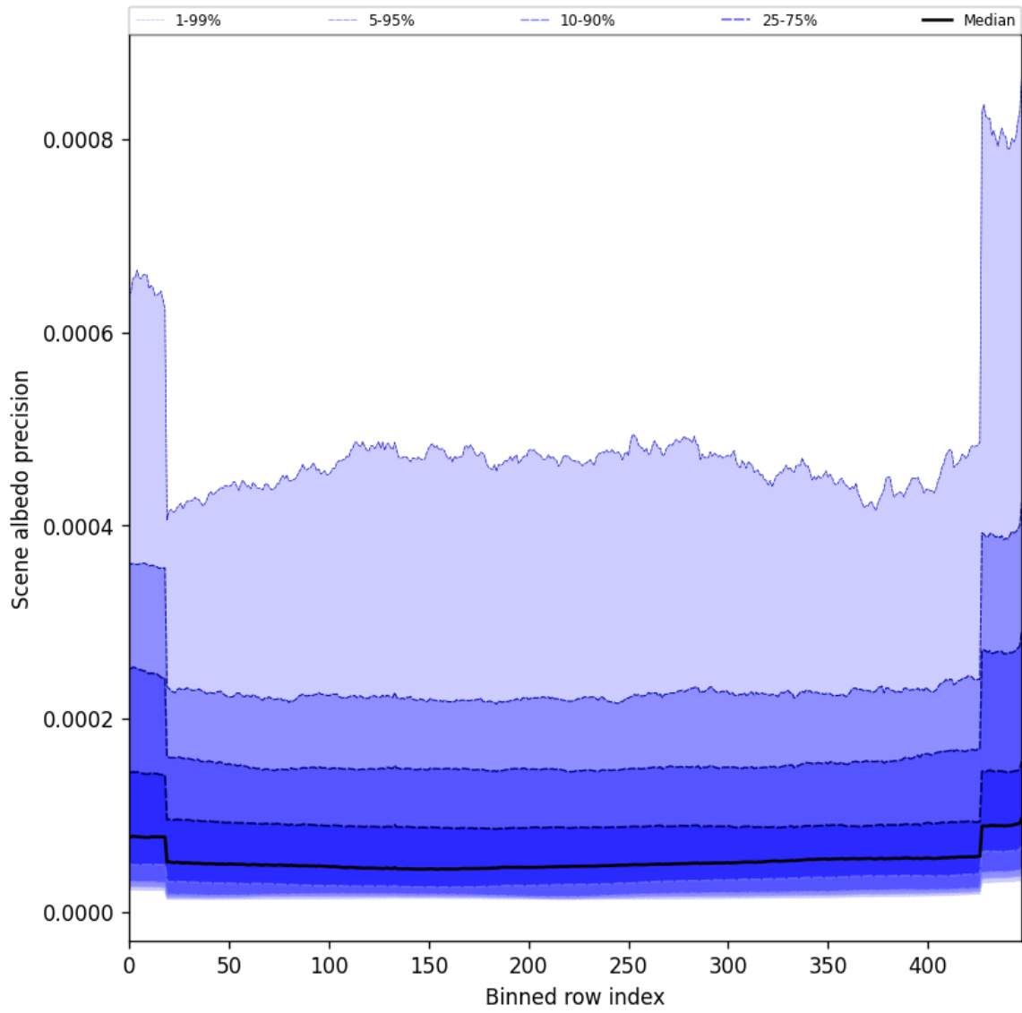
Figure 52: Along track statistics of “Scene albedo precision” for 2025-10-22 to 2025-10-23
