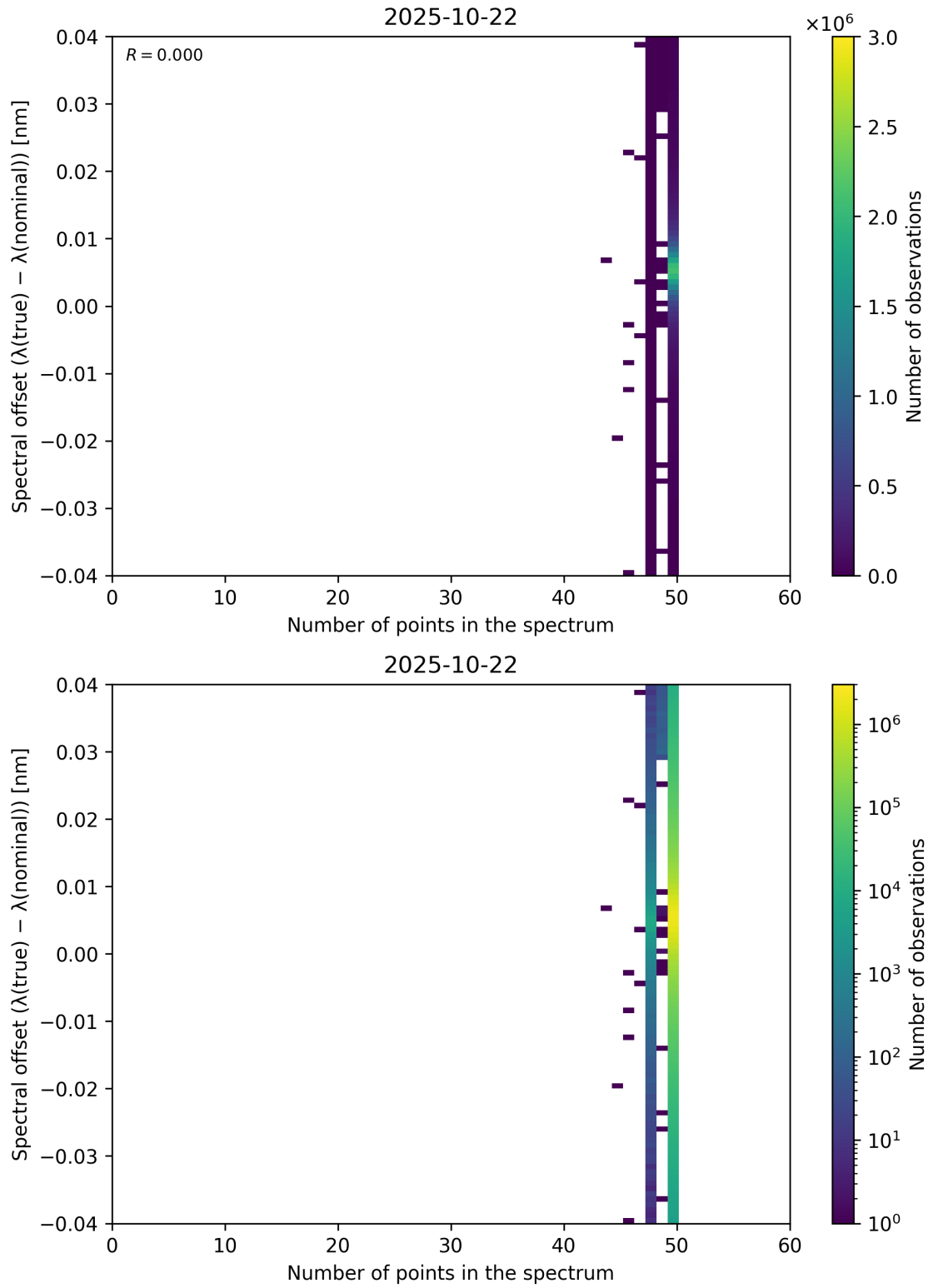
Figure 101: Scatter density plot of “Number of points in the spectrum” against “Spectral offset ( \lambda_{\text{true}} - \lambda_{\text{nominal}} )” for 2025-10-22 to 2025-10-23.
