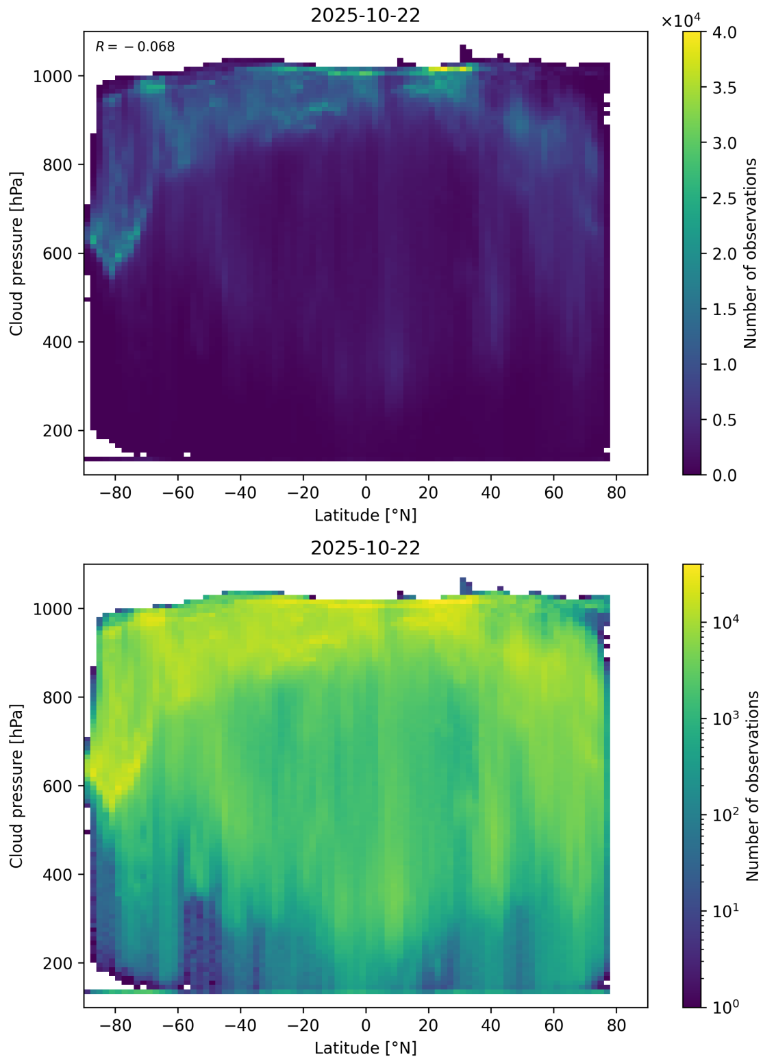
Figure 91: Scatter density plot of “Latitude” against “Cloud pressure” for 2025-10-22 to 2025-10-23.
