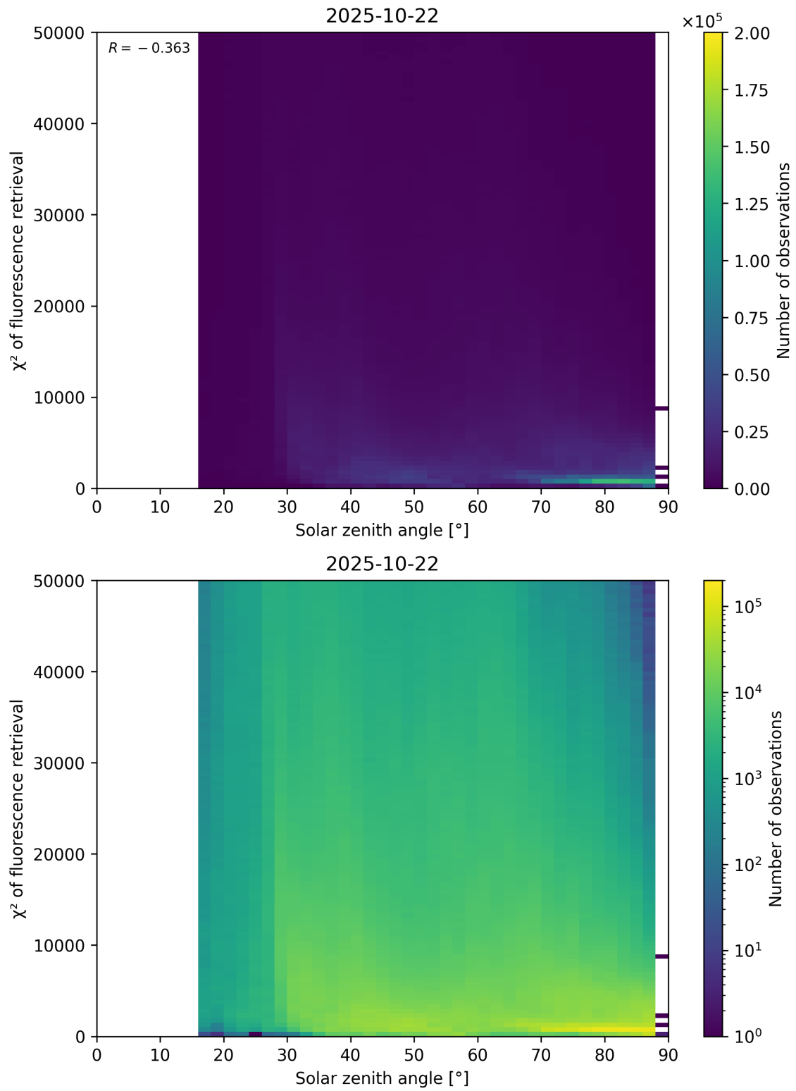
Figure 109: Scatter density plot of “Solar zenith angle” against “ \chi^2 of fluorescence retrieval” for 2025-10-22 to 2025-10-23.
