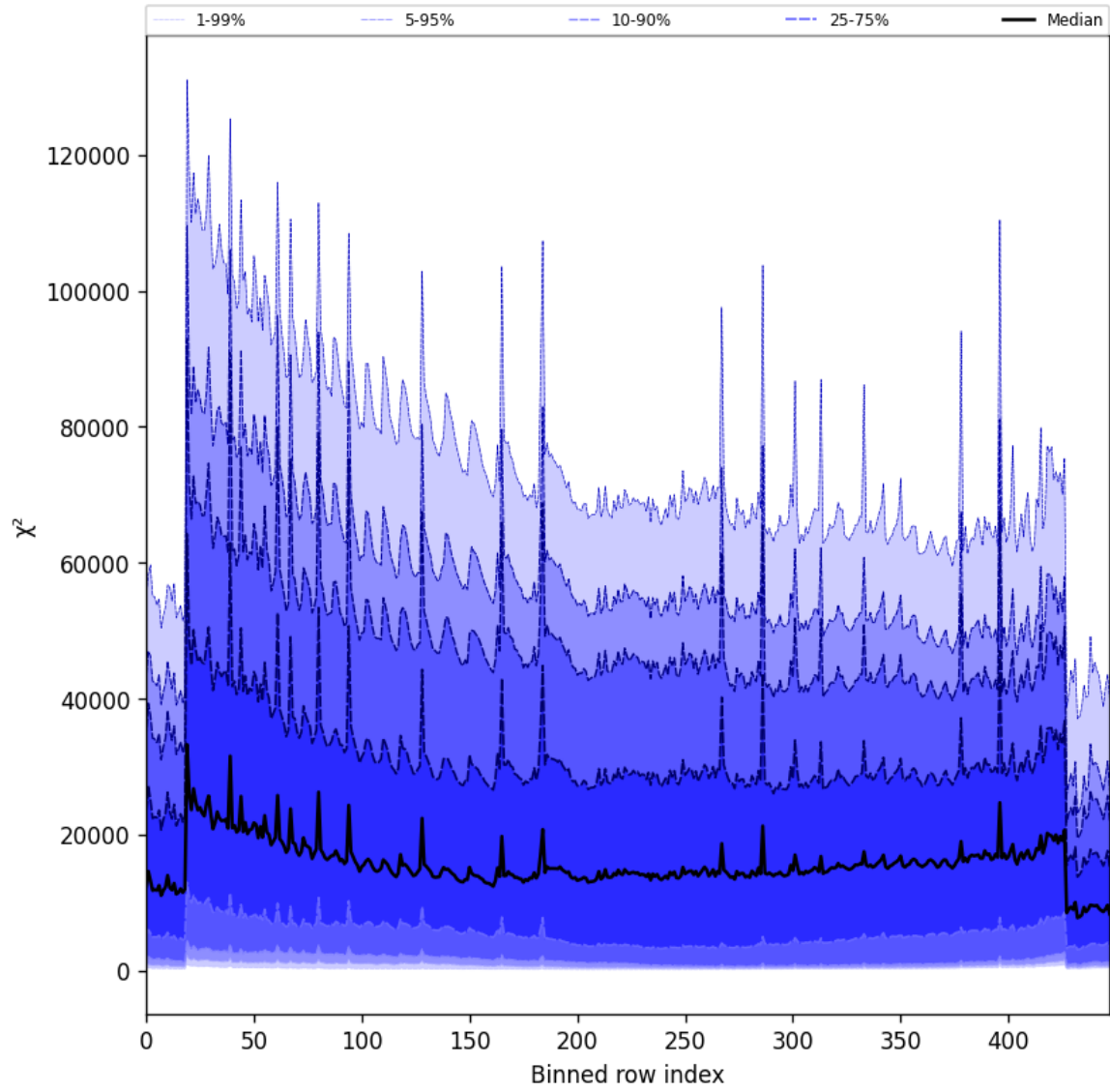
Figure 55: Along track statistics of “ \chi^2 ” for 2025-10-22 to 2025-10-23
