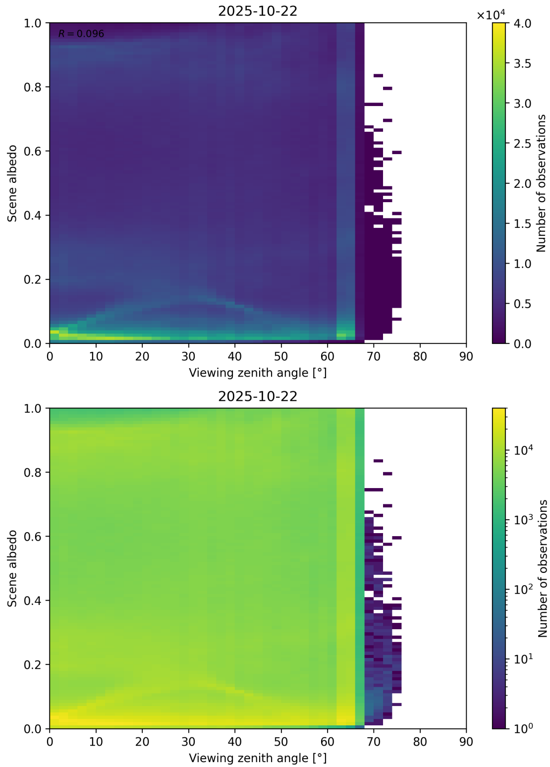
Figure 126: Scatter density plot of “Viewing zenith angle” against “Scene albedo” for 2025-10-22 to 2025-10-23.
