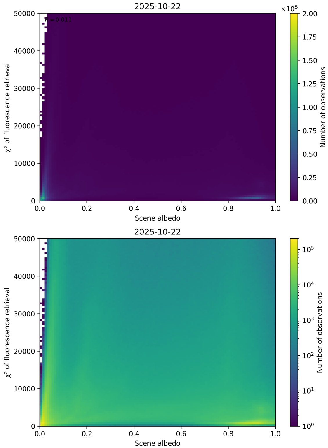
Figure 103: Scatter density plot of “Scene albedo” against “ \chi^2 of fluorescence retrieval” for 2025-10-22 to 2025-10-23.
