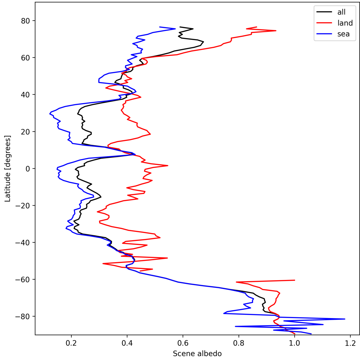
Figure 17: Zonal average of “Scene albedo” for 2025-10-22 to 2025-10-23.
