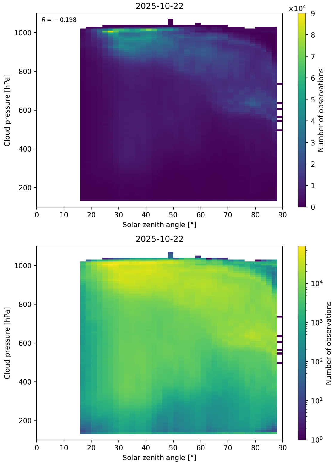
Figure 111: Scatter density plot of “Solar zenith angle” against “Cloud pressure” for 2025-10-22 to 2025-10-23.
