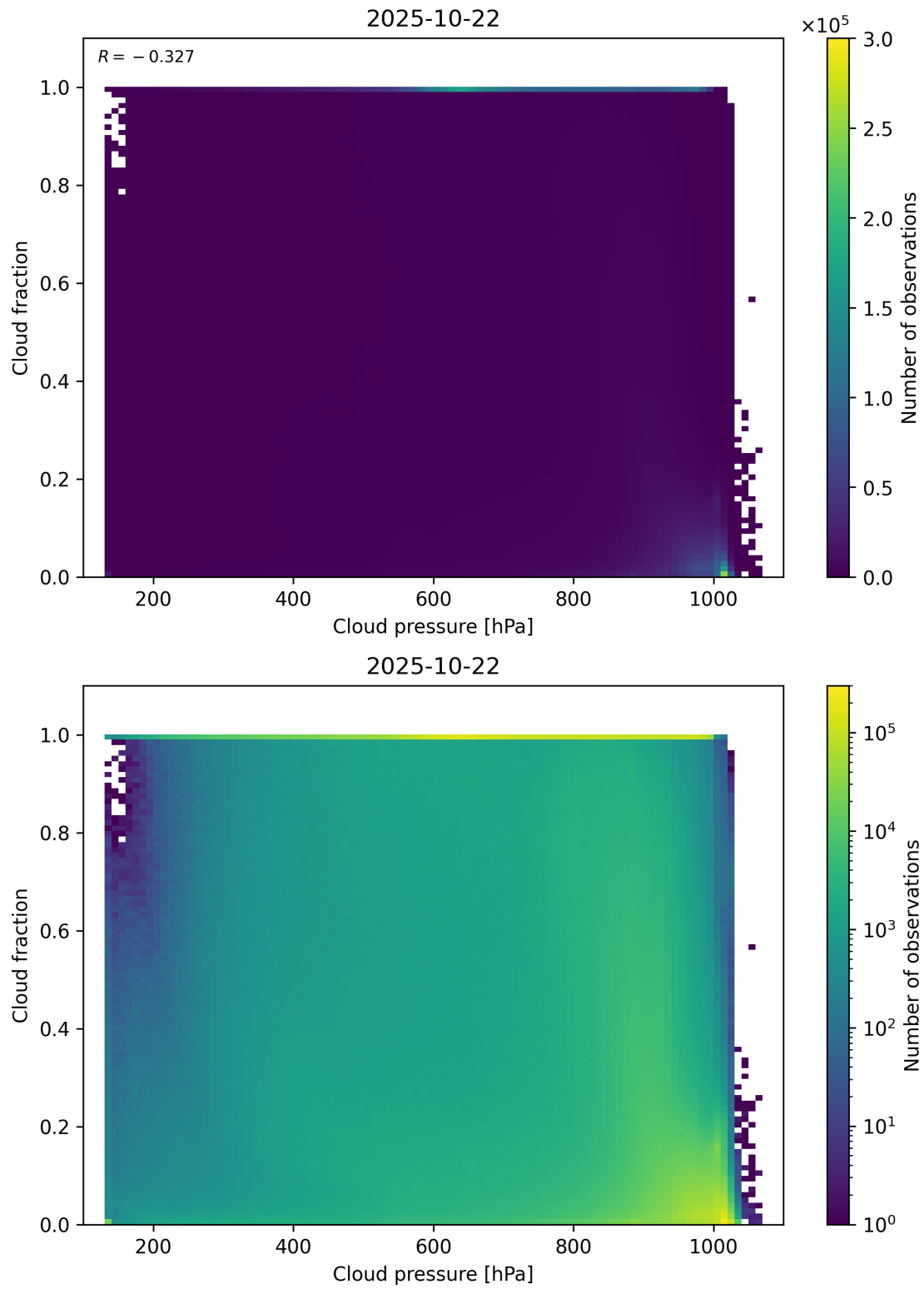
Figure 79: Scatter density plot of “Cloud pressure” against “Cloud fraction” for 2025-10-22 to 2025-10-23.
