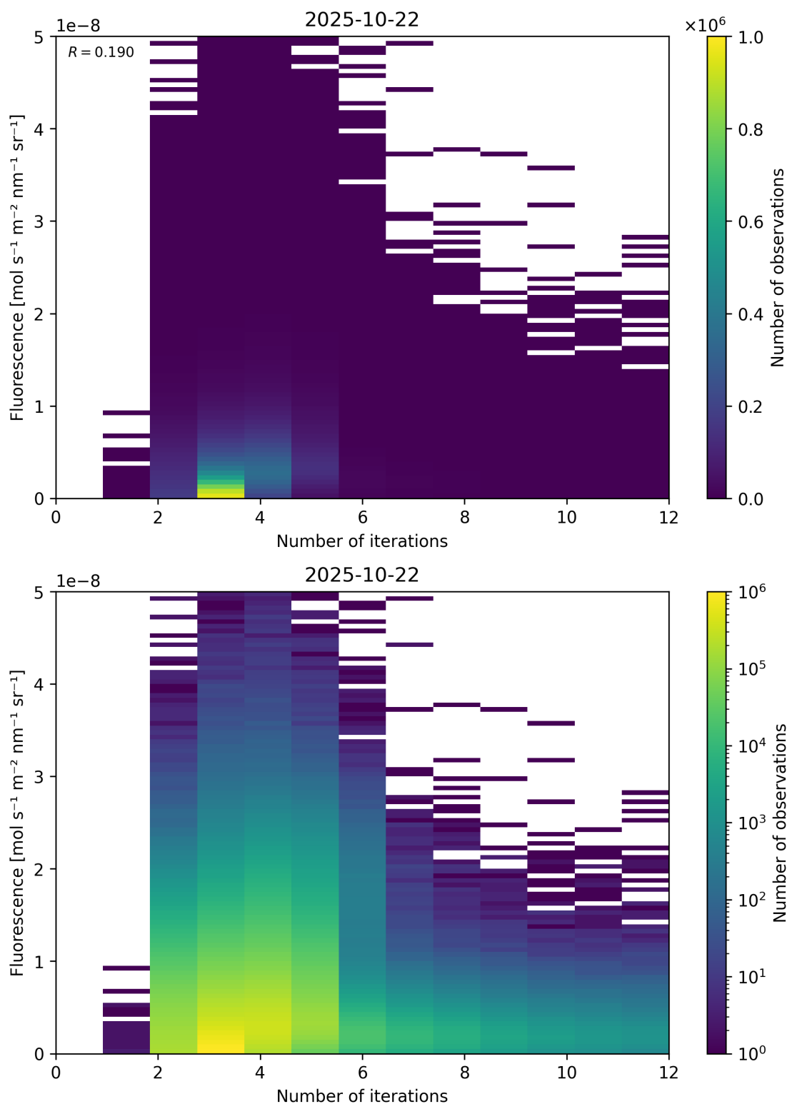
Figure 98: Scatter density plot of “Number of iterations” against “Fluorescence” for 2025-10-22 to 2025-10-23.
