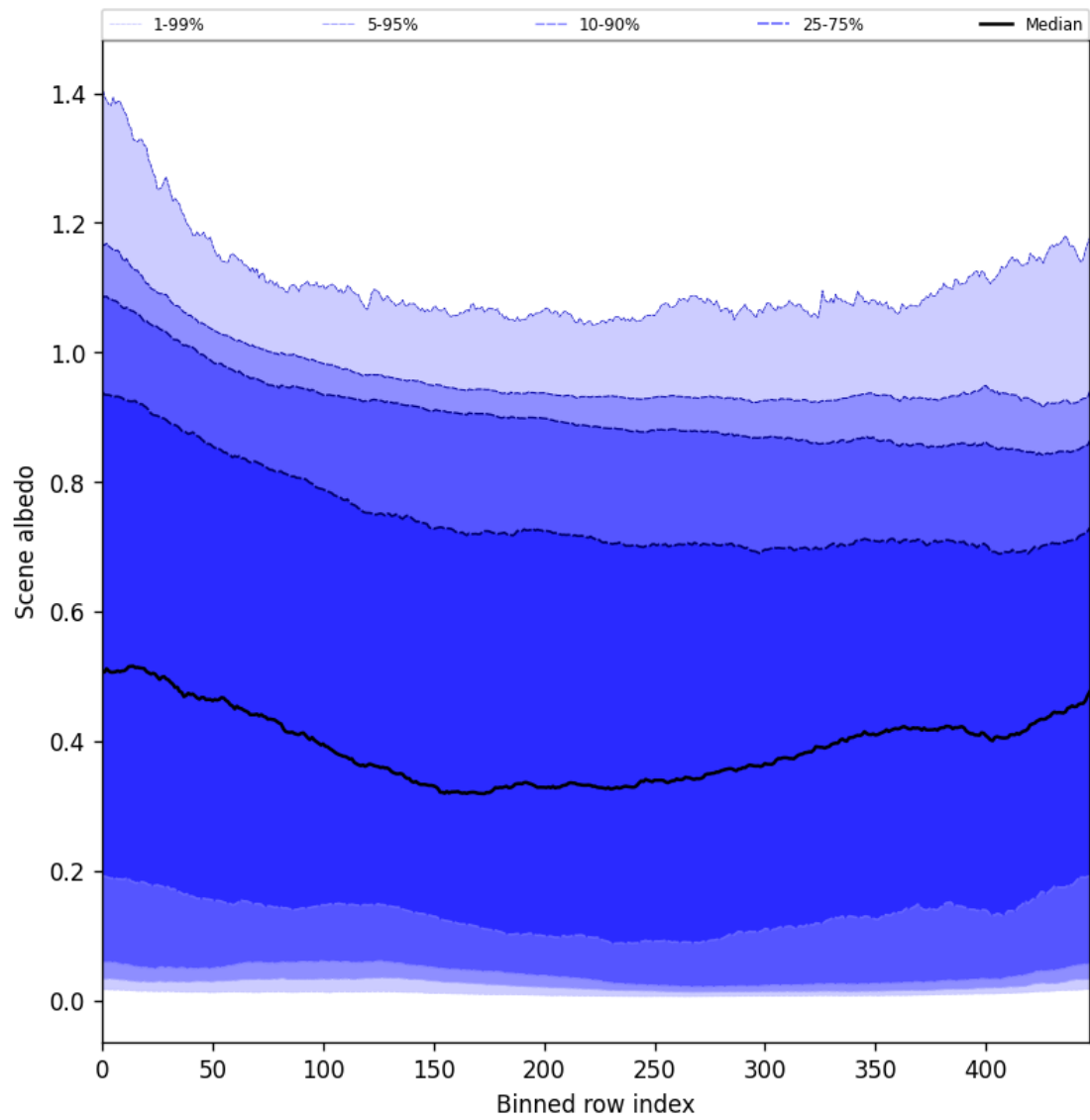
Figure 51: Along track statistics of “Scene albedo” for 2025-10-22 to 2025-10-23
