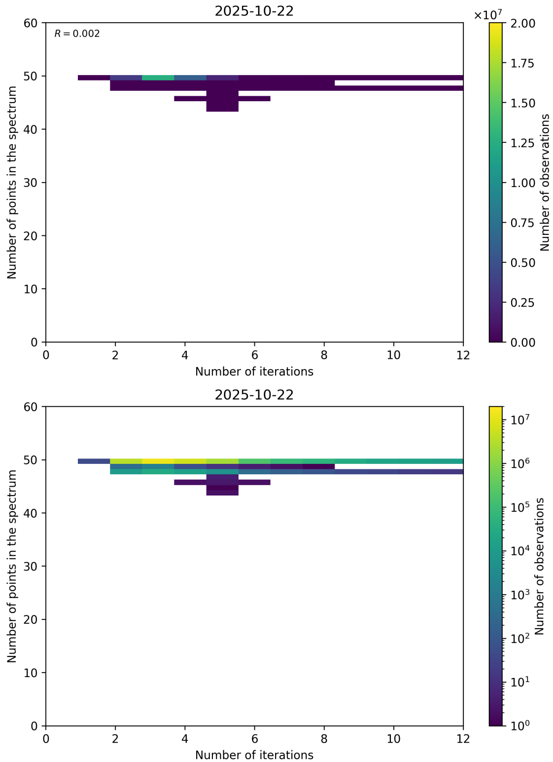
Figure 99: Scatter density plot of “Number of iterations” against “Number of points in the spectrum” for 2025-10-22 to 2025-10-23.
