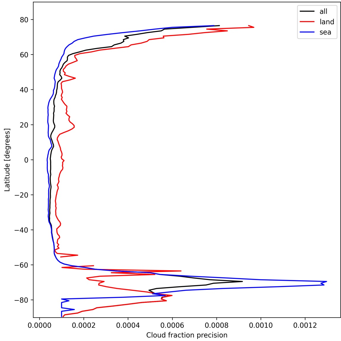
Figure 16: Zonal average of “Cloud fraction precision” for 2025-10-22 to 2025-10-23.
