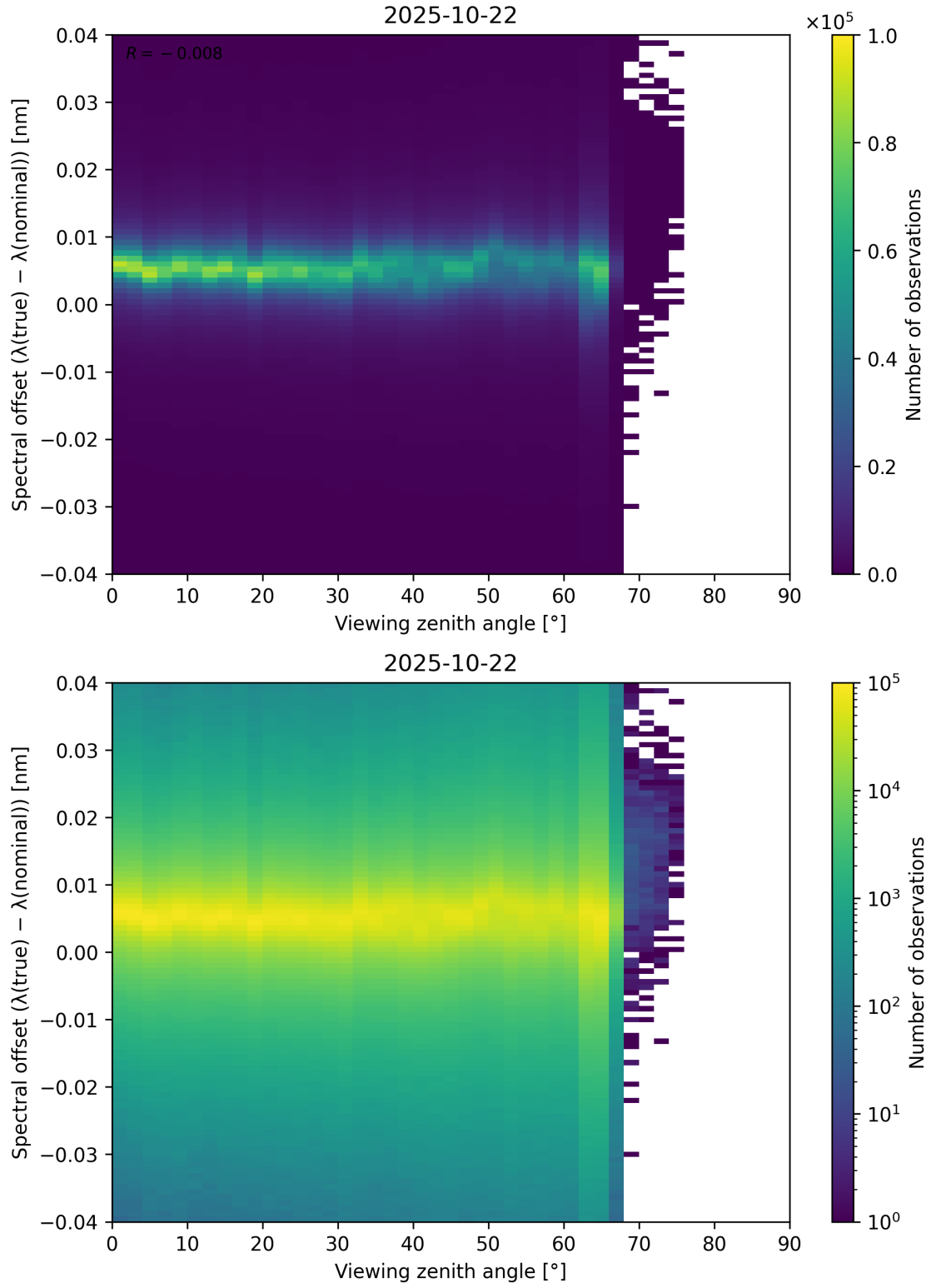
Figure 128: Scatter density plot of “Viewing zenith angle” against “Spectral offset ( \lambda_{\text{true}} - \lambda_{\text{nominal}} )” for 2025-10-22 to 2025-10-23.
