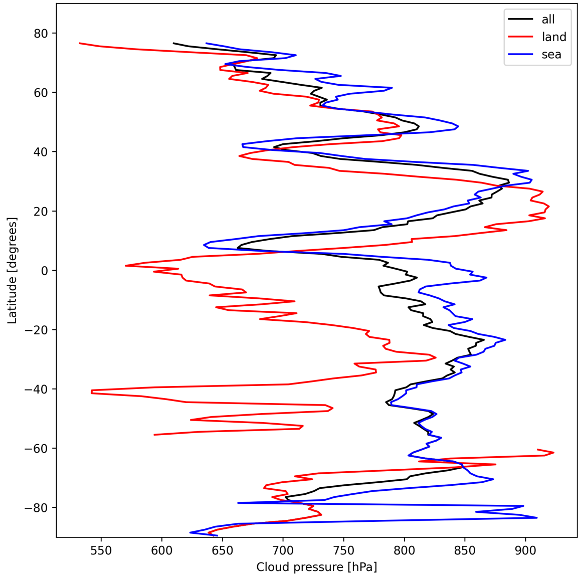
Figure 13: Zonal average of “Cloud pressure” for 2025-10-22 to 2025-10-23.
