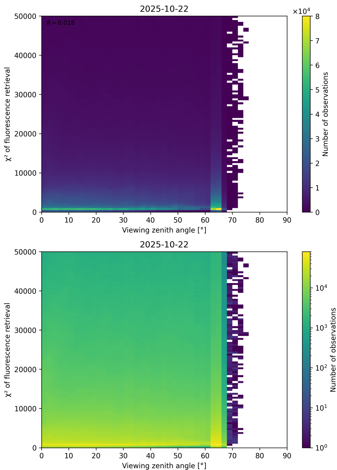
Figure 119: Scatter density plot of “Viewing zenith angle” against “ \chi^2 of fluorescence retrieval” for 2025-10-22 to 2025-10-23.
