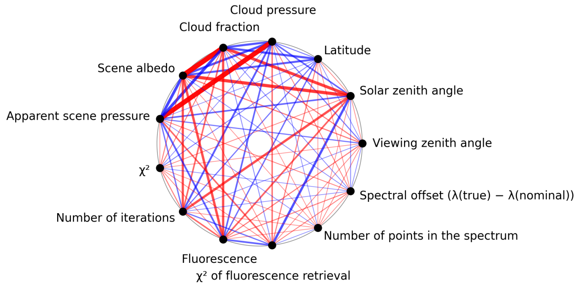
Figure 1: Map of correlation graph for 2025-10-22 to 2025-10-23.
