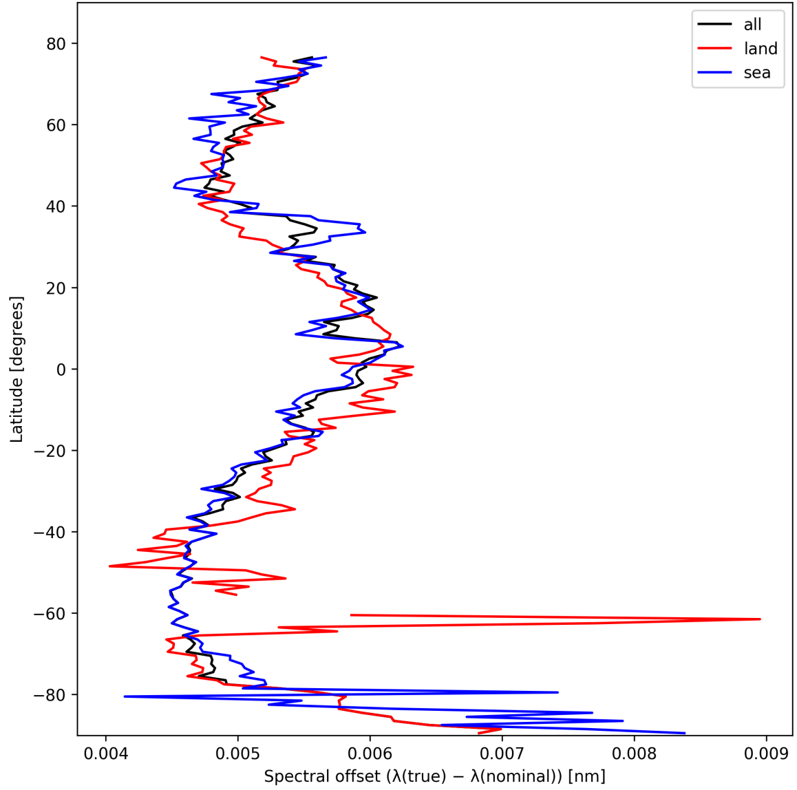
Figure 28: Zonal average of “Spectral offset ( \lambda_{\text{true}} - \lambda_{\text{nominal}} )” for 2025-10-22 to 2025-10-23.
