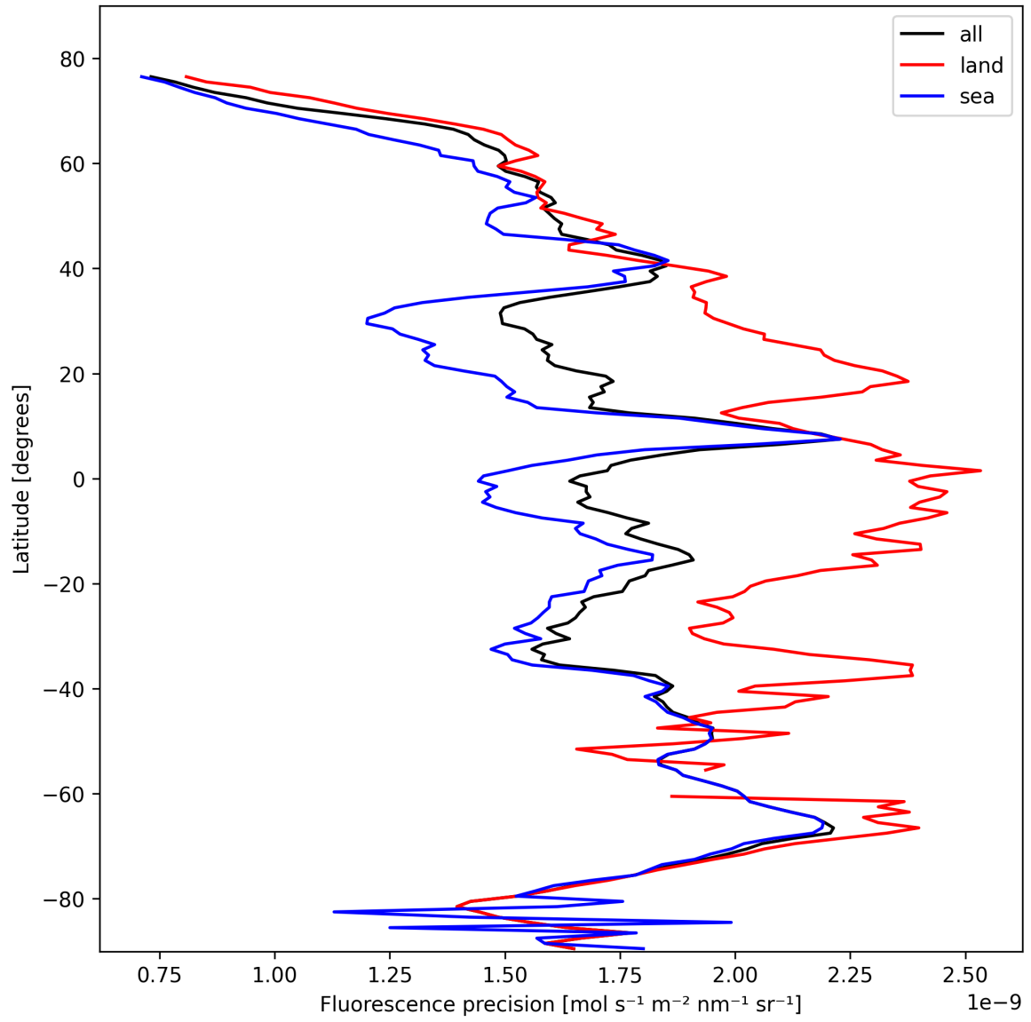
Figure 24: Zonal average of “Fluorescence precision” for 2025-10-22 to 2025-10-23.
