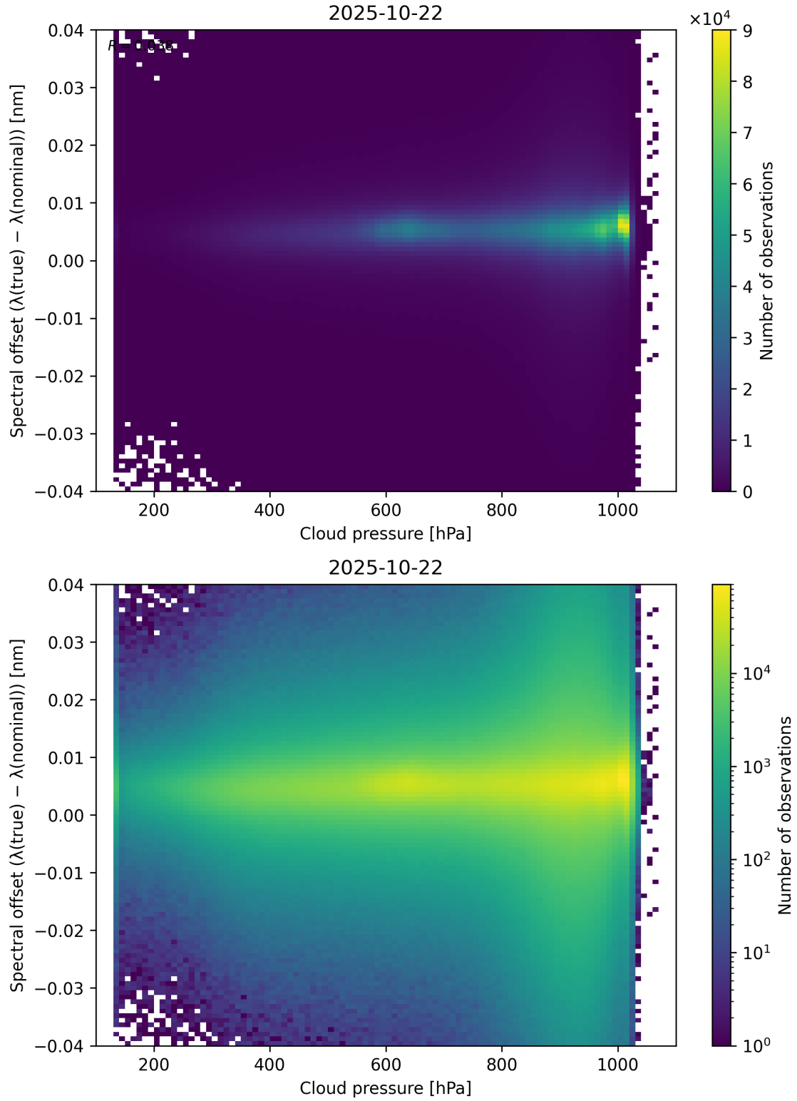
Figure 84: Scatter density plot of “Cloud pressure” against “Spectral offset ( \lambda_{\text{true}} - \lambda_{\text{nominal}} )” for 2025-10-22 to 2025-10-23.
