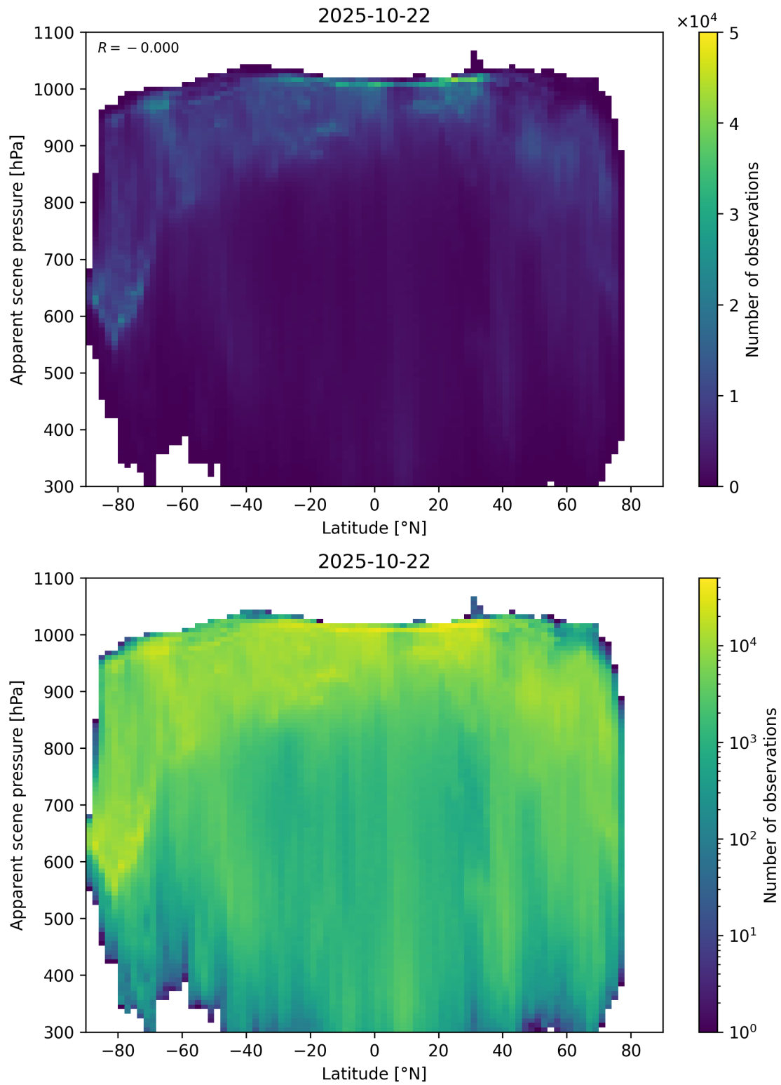
Figure 88: Scatter density plot of “Latitude” against “Apparent scene pressure” for 2025-10-22 to 2025-10-23.
