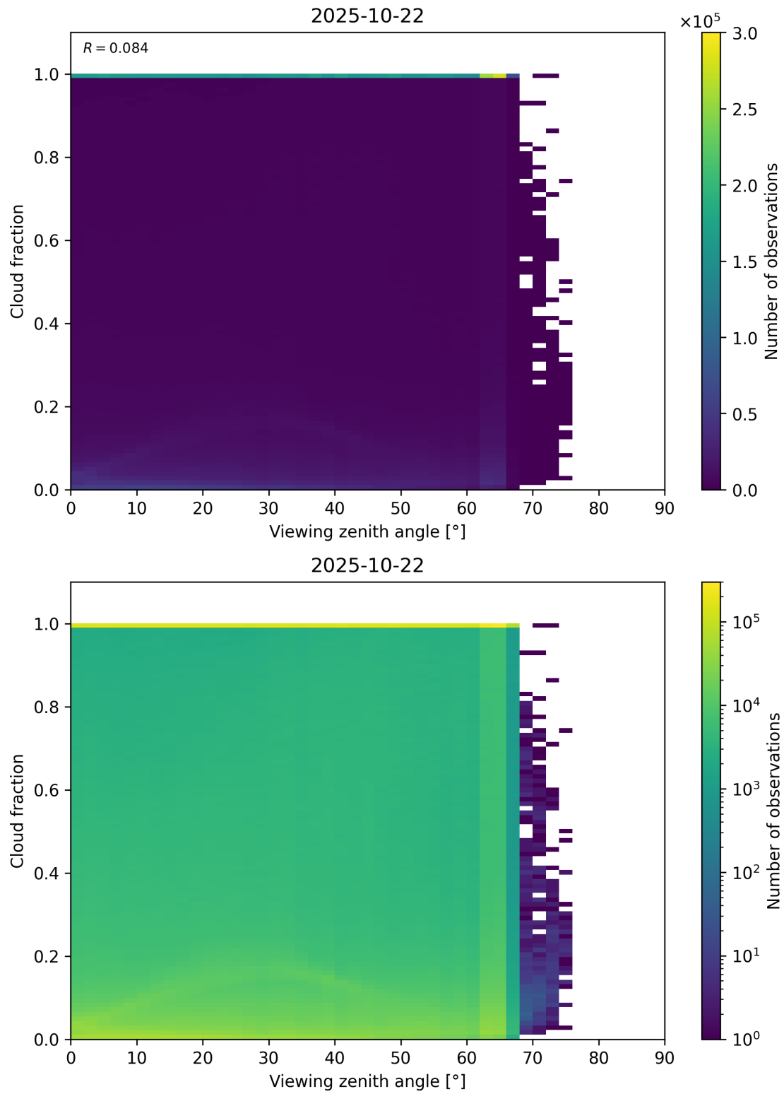
Figure 120: Scatter density plot of “Viewing zenith angle” against “Cloud fraction” for 2025-10-22 to 2025-10-23.
