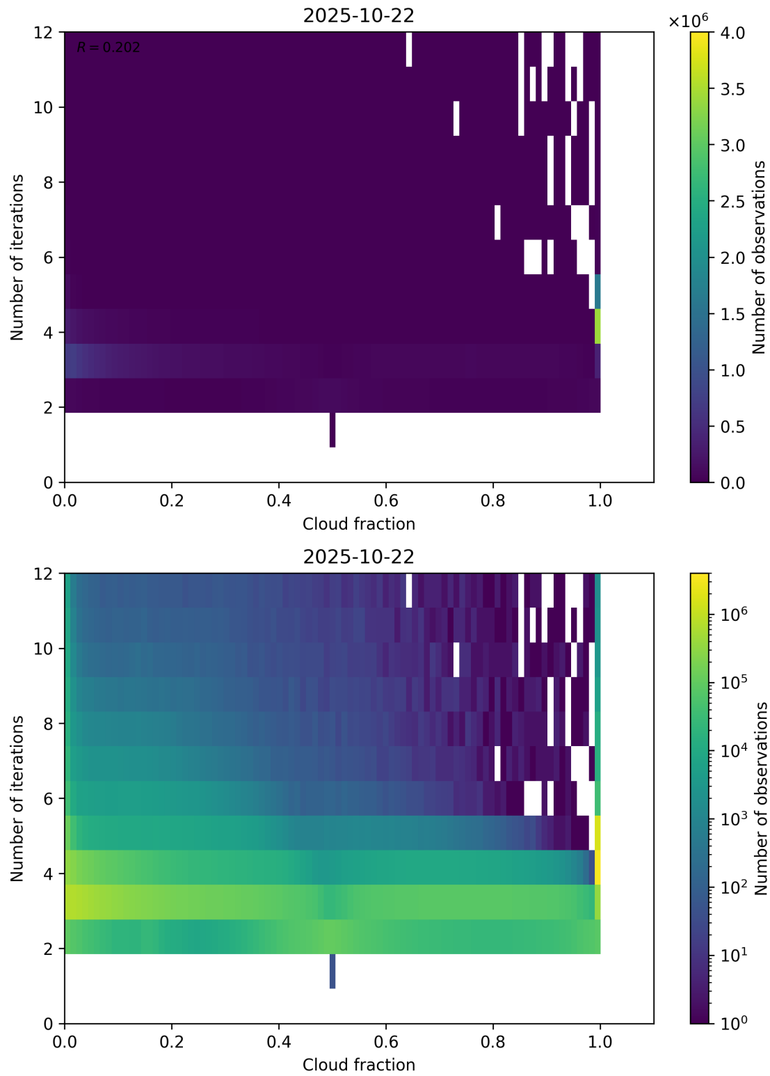
Figure 73: Scatter density plot of “Cloud fraction” against “Number of iterations” for 2025-10-22 to 2025-10-23.
