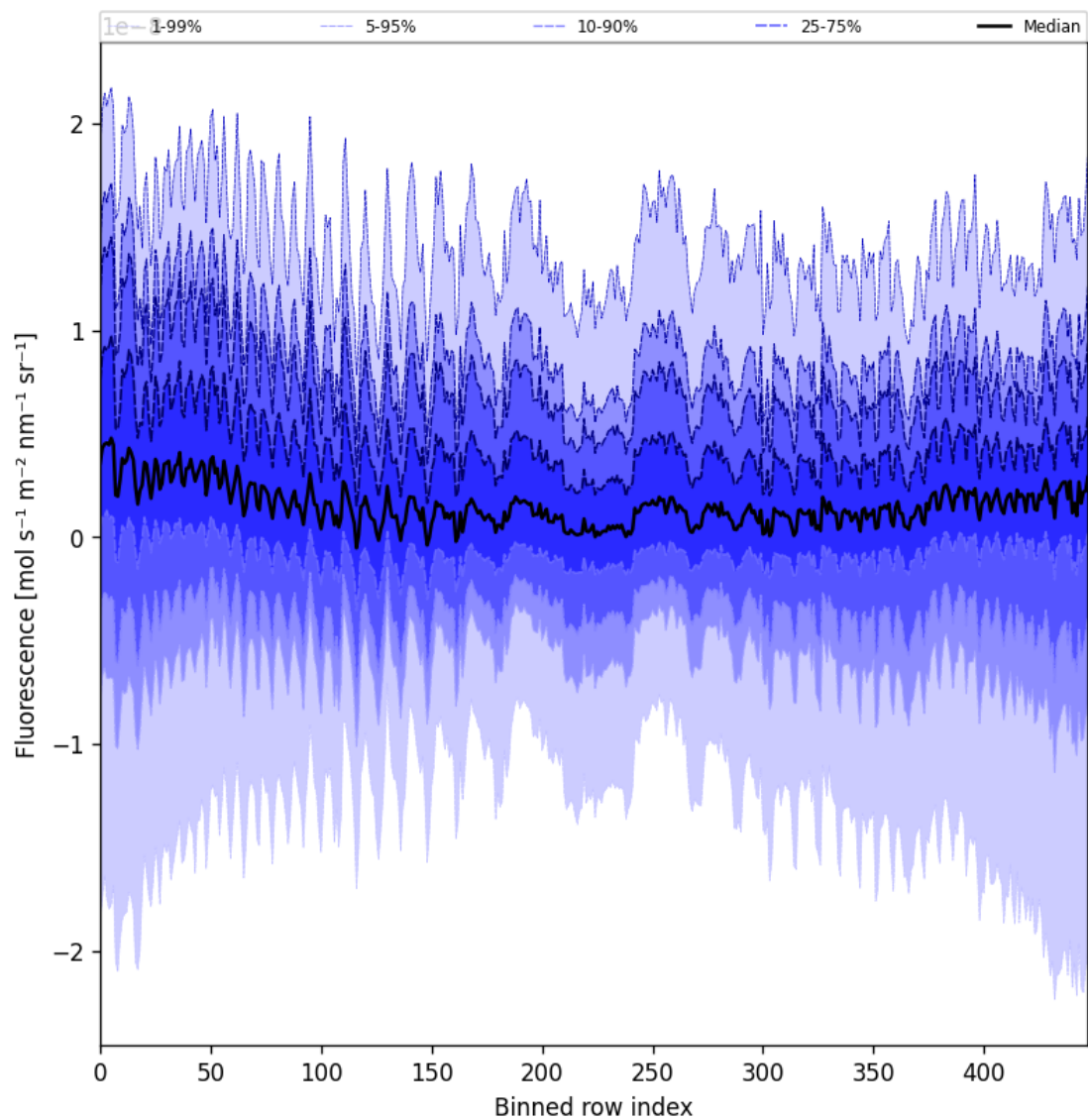
Figure 57: Along track statistics of “Fluorescence” for 2025-10-22 to 2025-10-23
