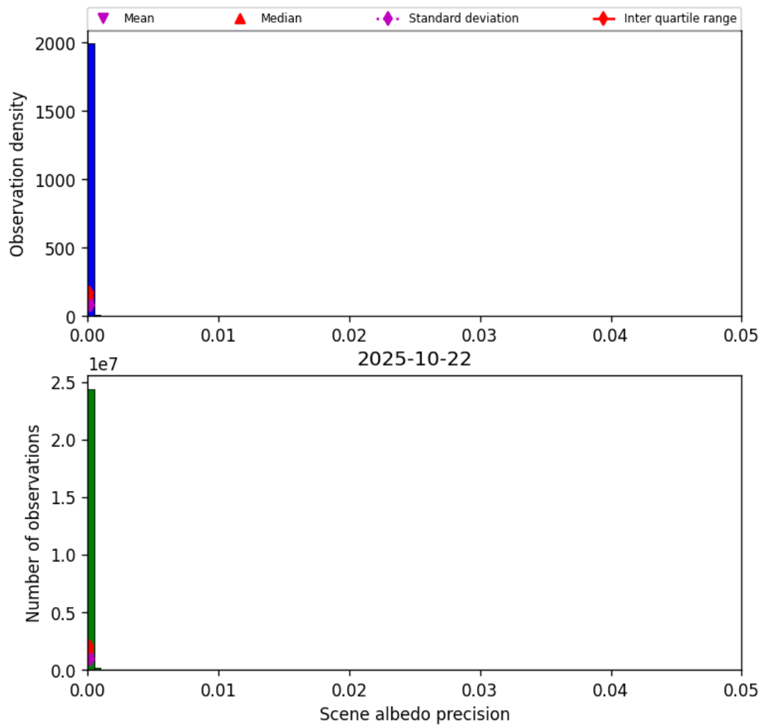
Figure 35: Histogram of “Scene albedo precision” for 2025-10-22 to 2025-10-23
