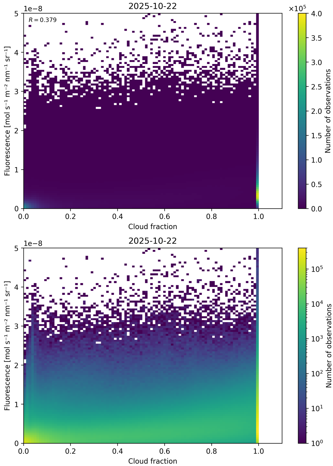
Figure 72: Scatter density plot of “Cloud fraction” against “Fluorescence” for 2025-10-22 to 2025-10-23.
