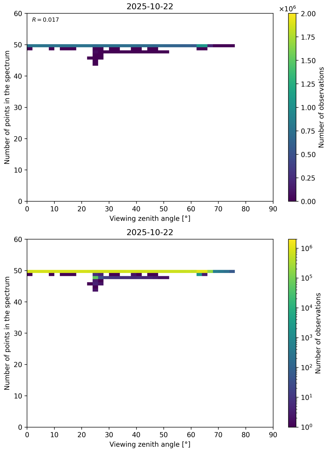
Figure 125: Scatter density plot of “Viewing zenith angle” against “Number of points in the spectrum” for 2025-10-22 to 2025-10-23.
