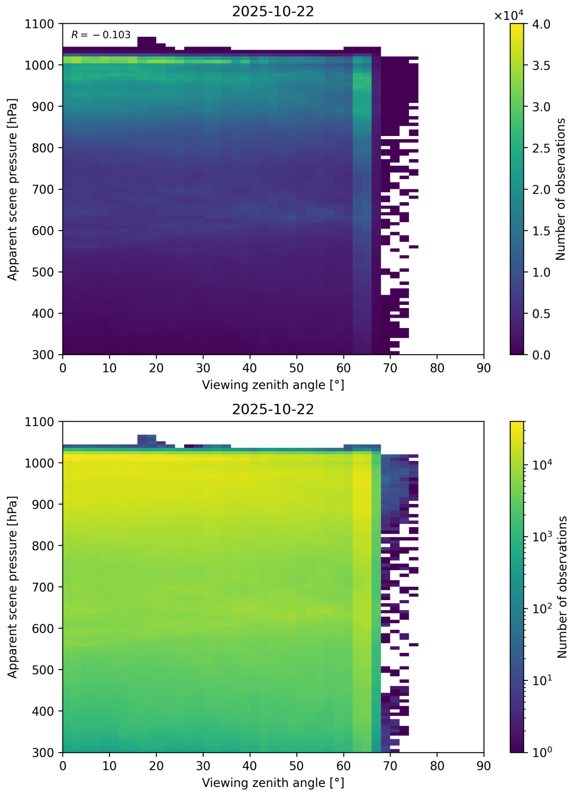
Figure 118: Scatter density plot of “Viewing zenith angle” against “Apparent scene pressure” for 2025-10-22 to 2025-10-23.
