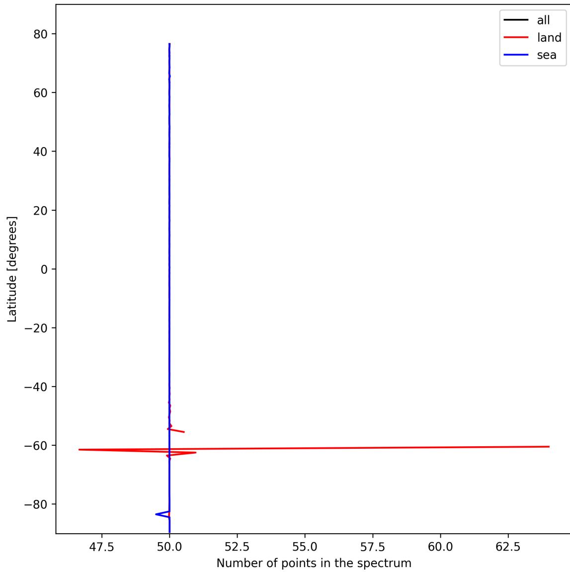
Figure 27: Zonal average of “Number of points in the spectrum” for 2025-10-22 to 2025-10-23.
