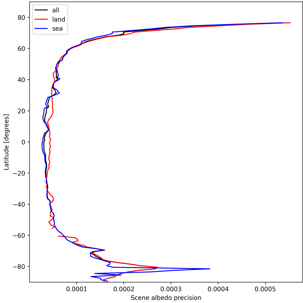
Figure 18: Zonal average of “Scene albedo precision” for 2025-10-22 to 2025-10-23.
