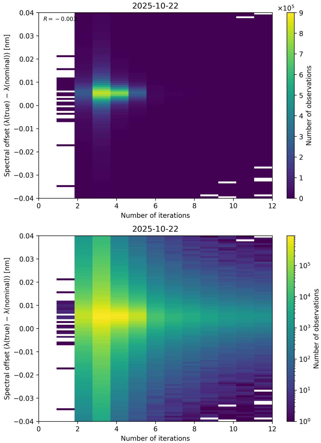
Figure 100: Scatter density plot of “Number of iterations” against “Spectral offset ( \lambda_{\text{true}} - \lambda_{\text{nominal}} )” for 2025-10-22 to 2025-10-23.
