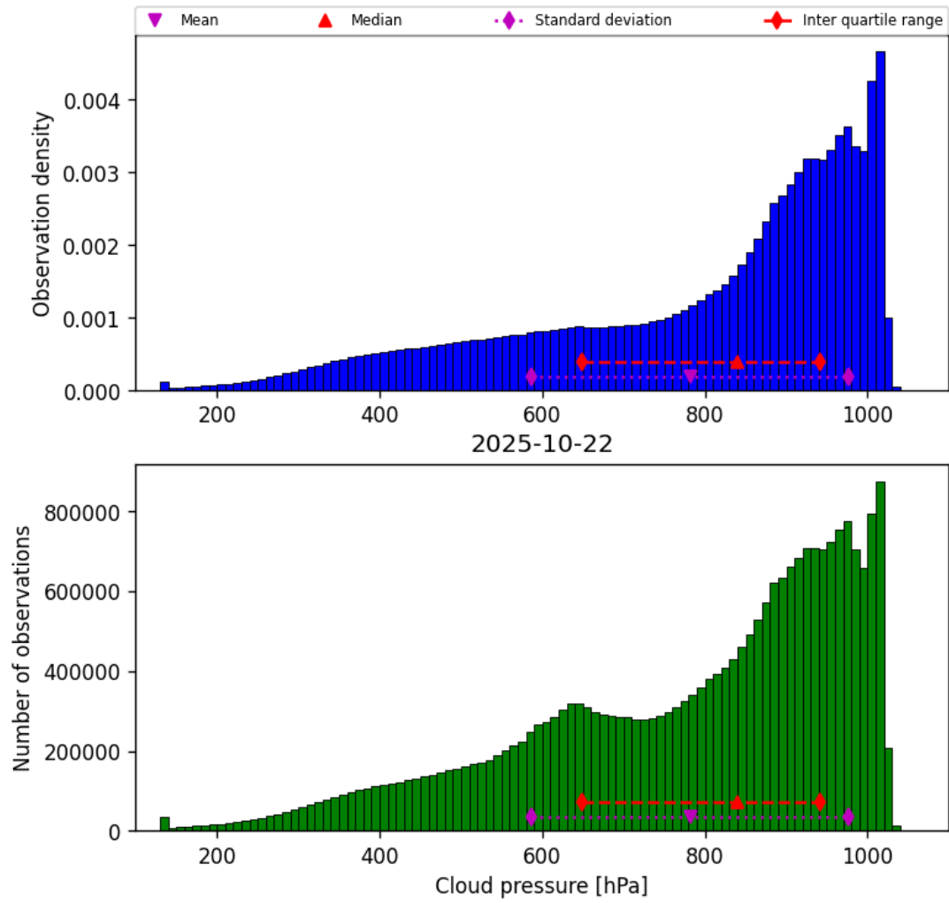
Figure 30: Histogram of “Cloud pressure” for 2025-10-22 to 2025-10-23
