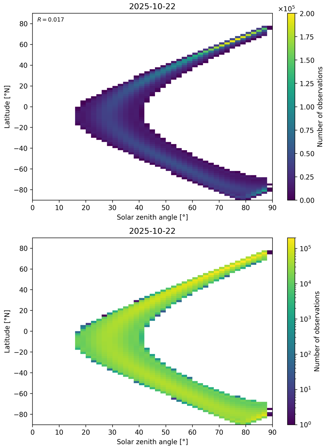
Figure 113: Scatter density plot of “Solar zenith angle” against “Latitude” for 2025-10-22 to 2025-10-23.
