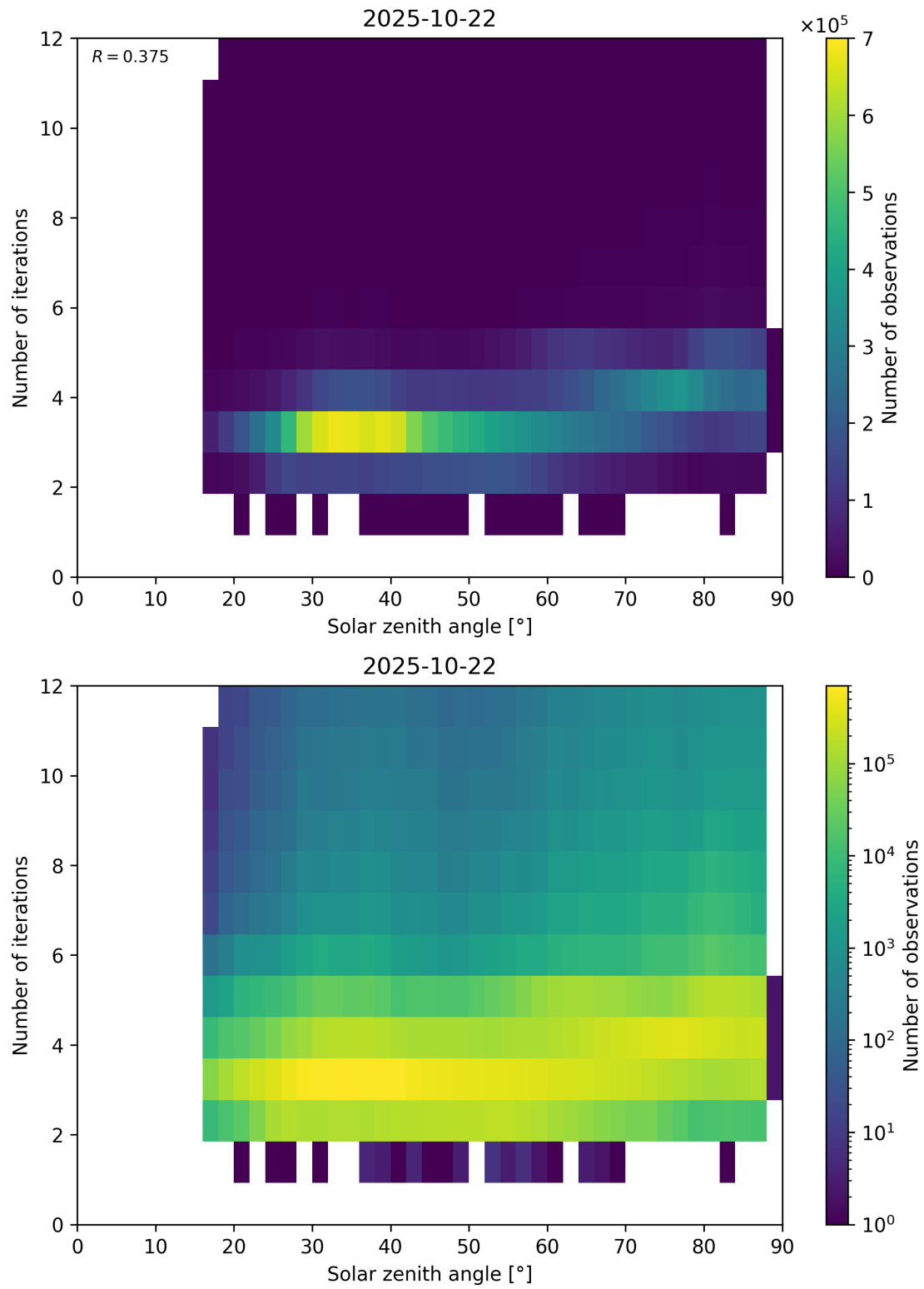
Figure 114: Scatter density plot of “Solar zenith angle” against “Number of iterations” for 2025-10-22 to 2025-10-23.
