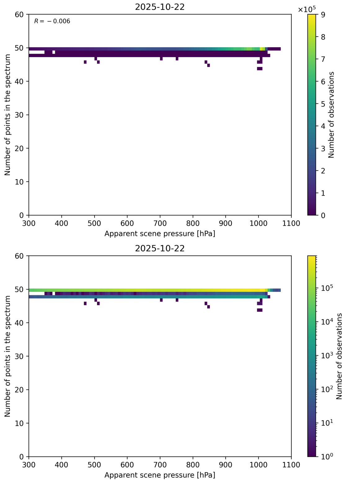
Figure 66: Scatter density plot of “Apparent scene pressure” against “Number of points in the spectrum” for 2025-10-22 to 2025-10-23.
