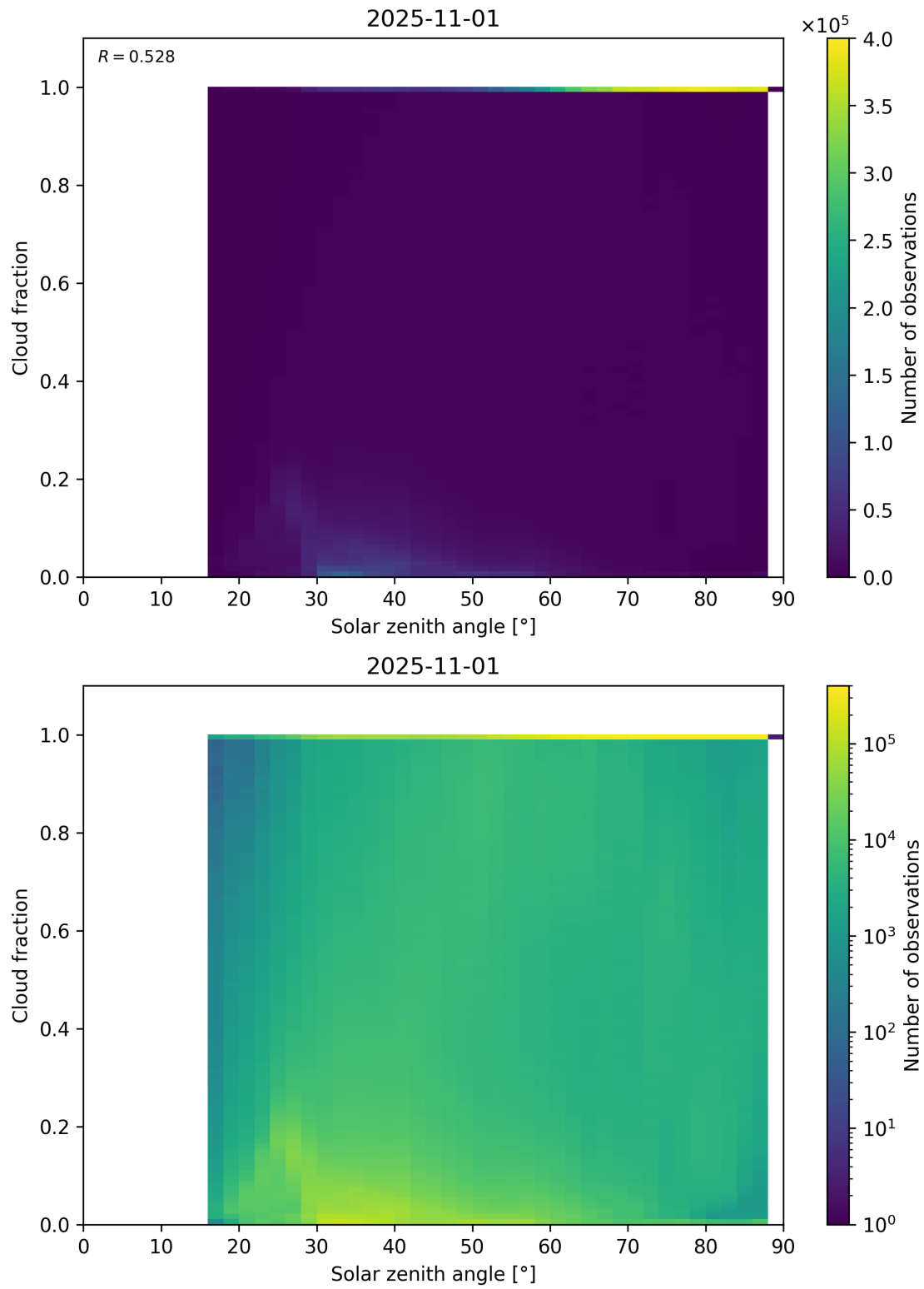
Figure 110: Scatter density plot of “Solar zenith angle” against “Cloud fraction” for 2025-10-31 to 2025-11-02.
