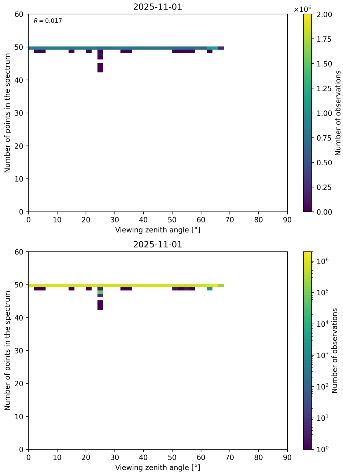
Figure 125: Scatter density plot of “Viewing zenith angle” against “Number of points in the spectrum” for 2025-10-31 to 2025-11-02.
