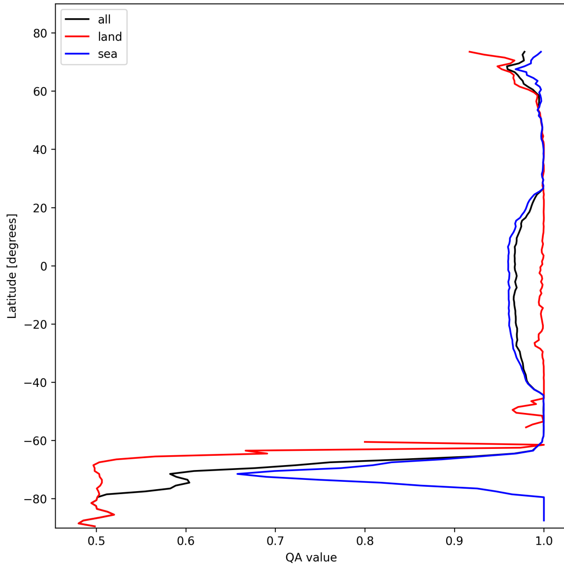
Figure 12: Zonal average of “QA value” for 2025-10-31 to 2025-11-02.
