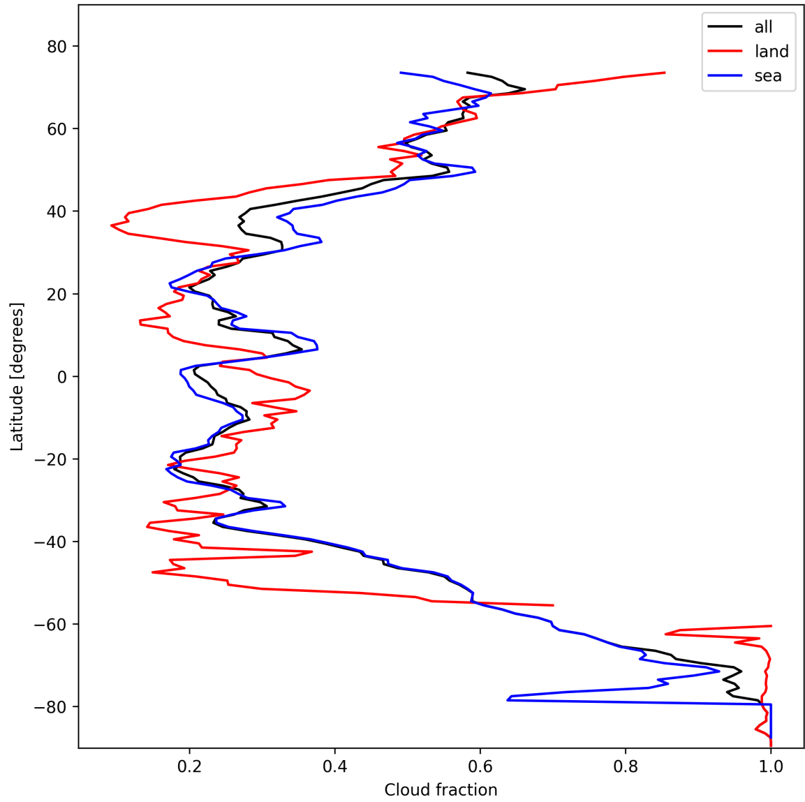
Figure 15: Zonal average of “Cloud fraction” for 2025-10-31 to 2025-11-02.
