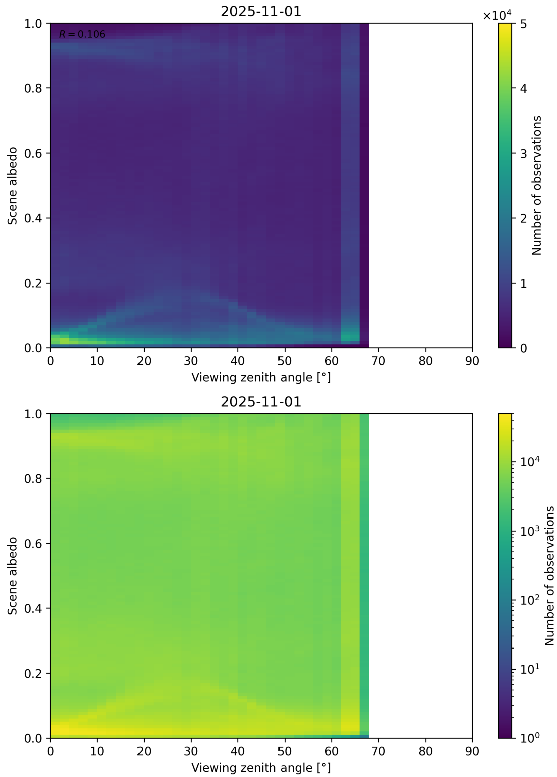
Figure 126: Scatter density plot of “Viewing zenith angle” against “Scene albedo” for 2025-10-31 to 2025-11-02.
