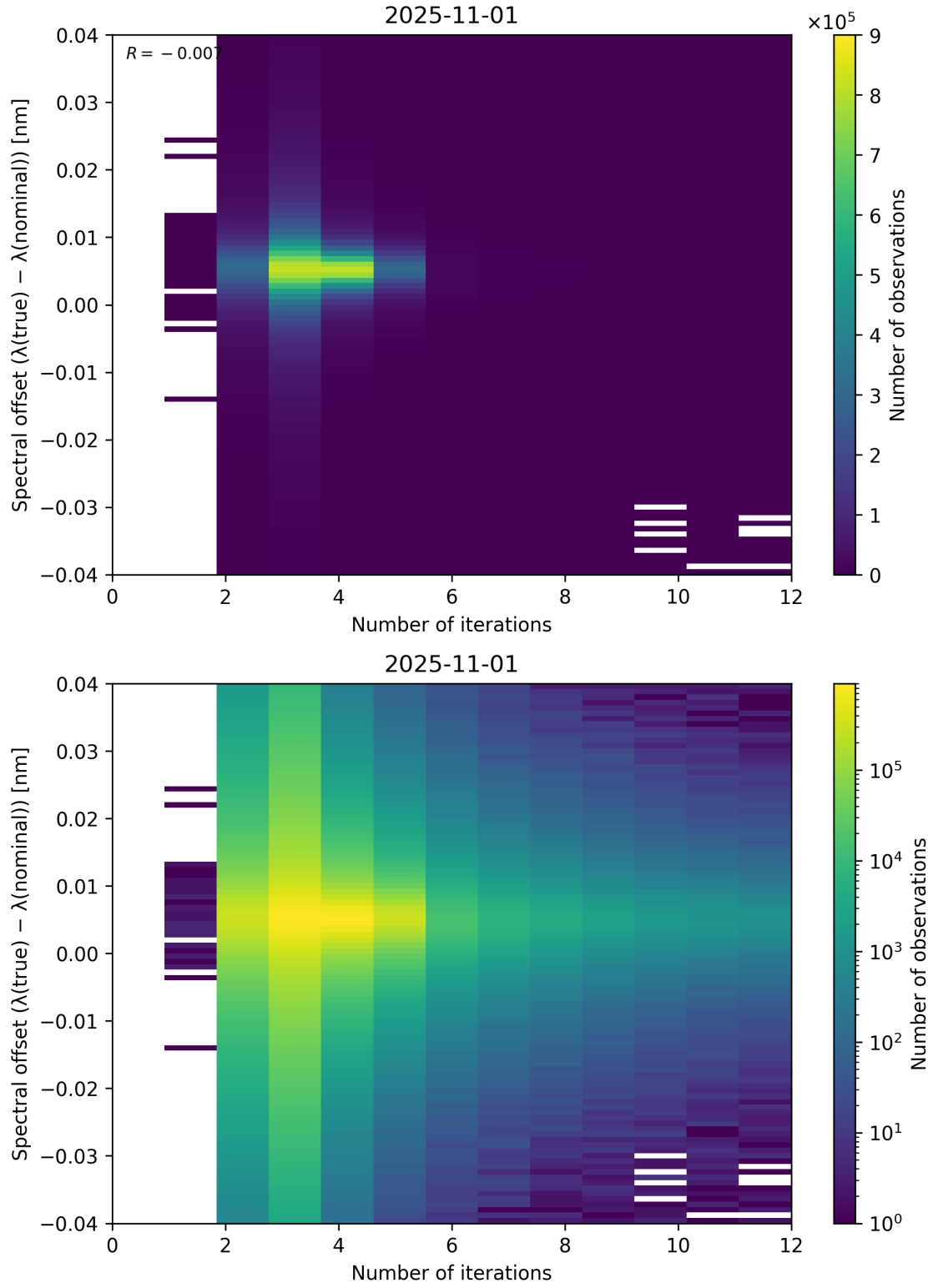
Figure 100: Scatter density plot of “Number of iterations” against “Spectral offset ( \lambda_{\text{true}} - \lambda_{\text{nominal}} )” for 2025-10-31 to 2025-11-02.
