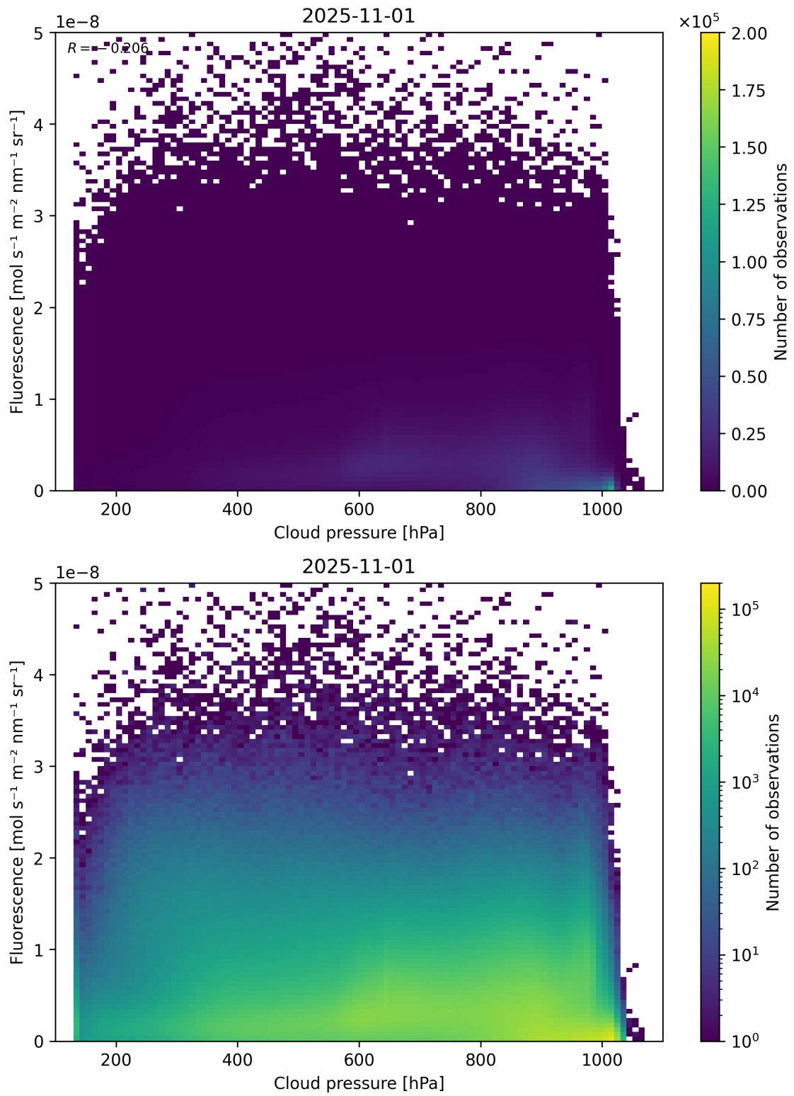
Figure 80: Scatter density plot of “Cloud pressure” against “Fluorescence” for 2025-10-31 to 2025-11-02.
