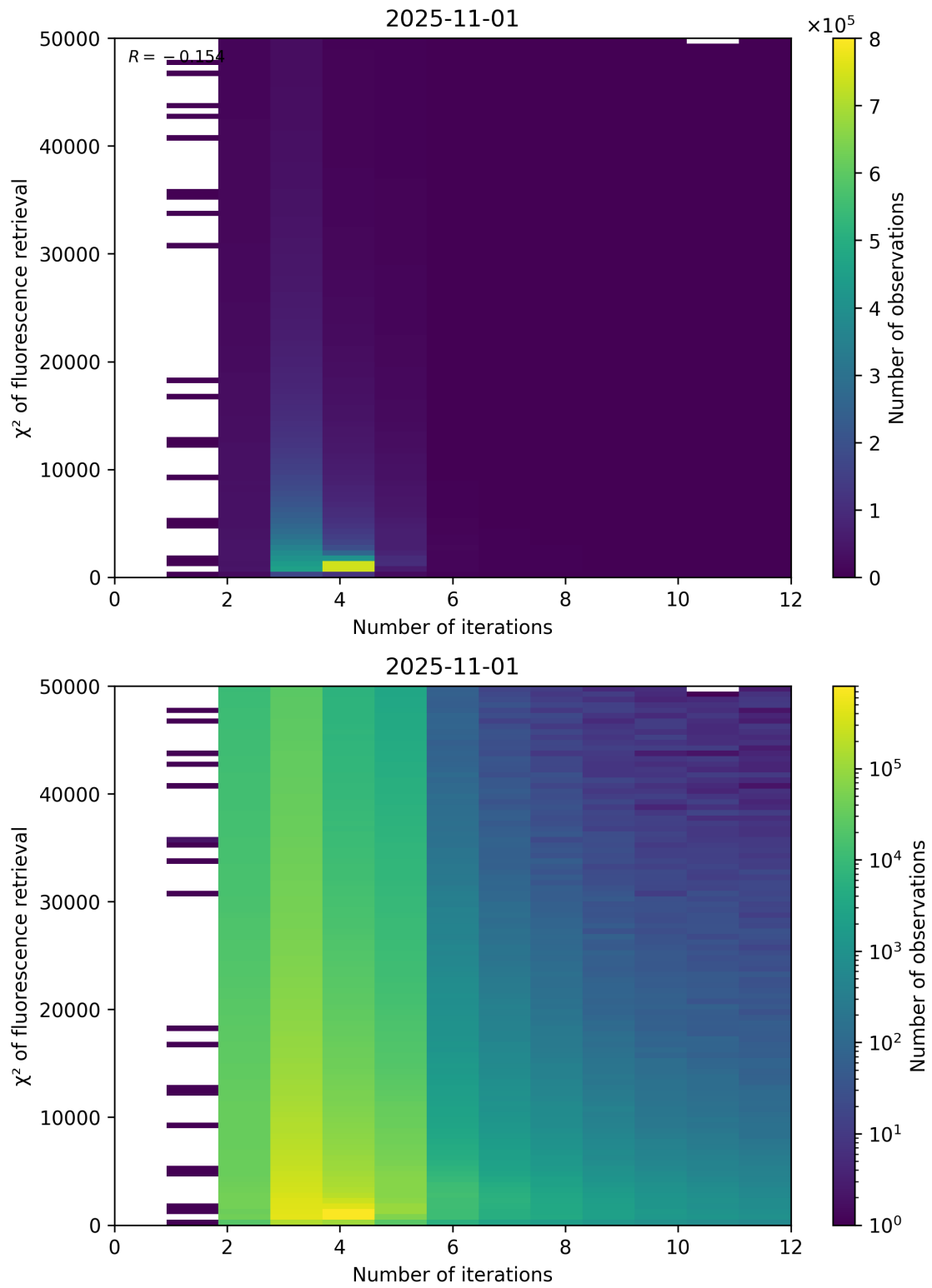
Figure 97: Scatter density plot of “Number of iterations” against “ \chi^2 of fluorescence retrieval” for 2025-10-31 to 2025-11-02.
