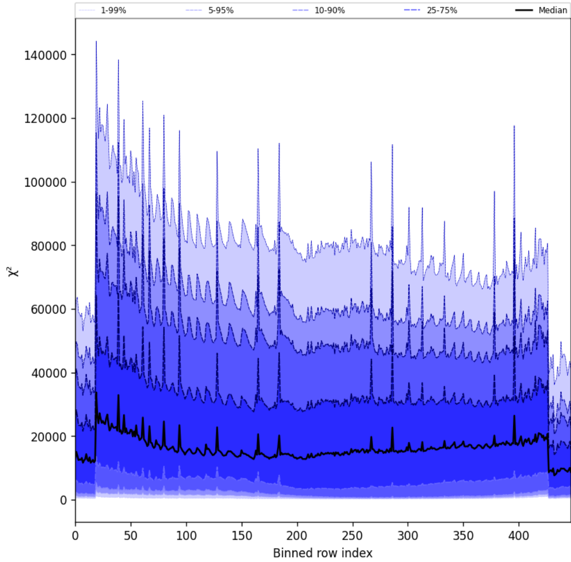
Figure 55: Along track statistics of “ \chi^2 ” for 2025-10-31 to 2025-11-02
