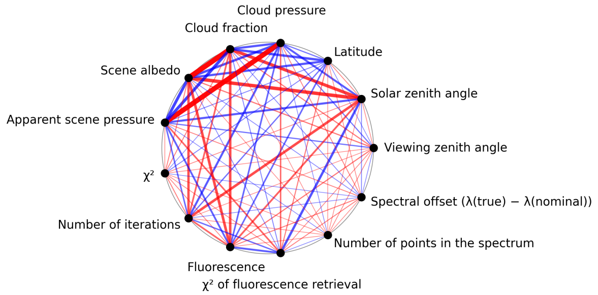
Figure 1: Map of correlation graph for 2025-10-31 to 2025-11-02.
