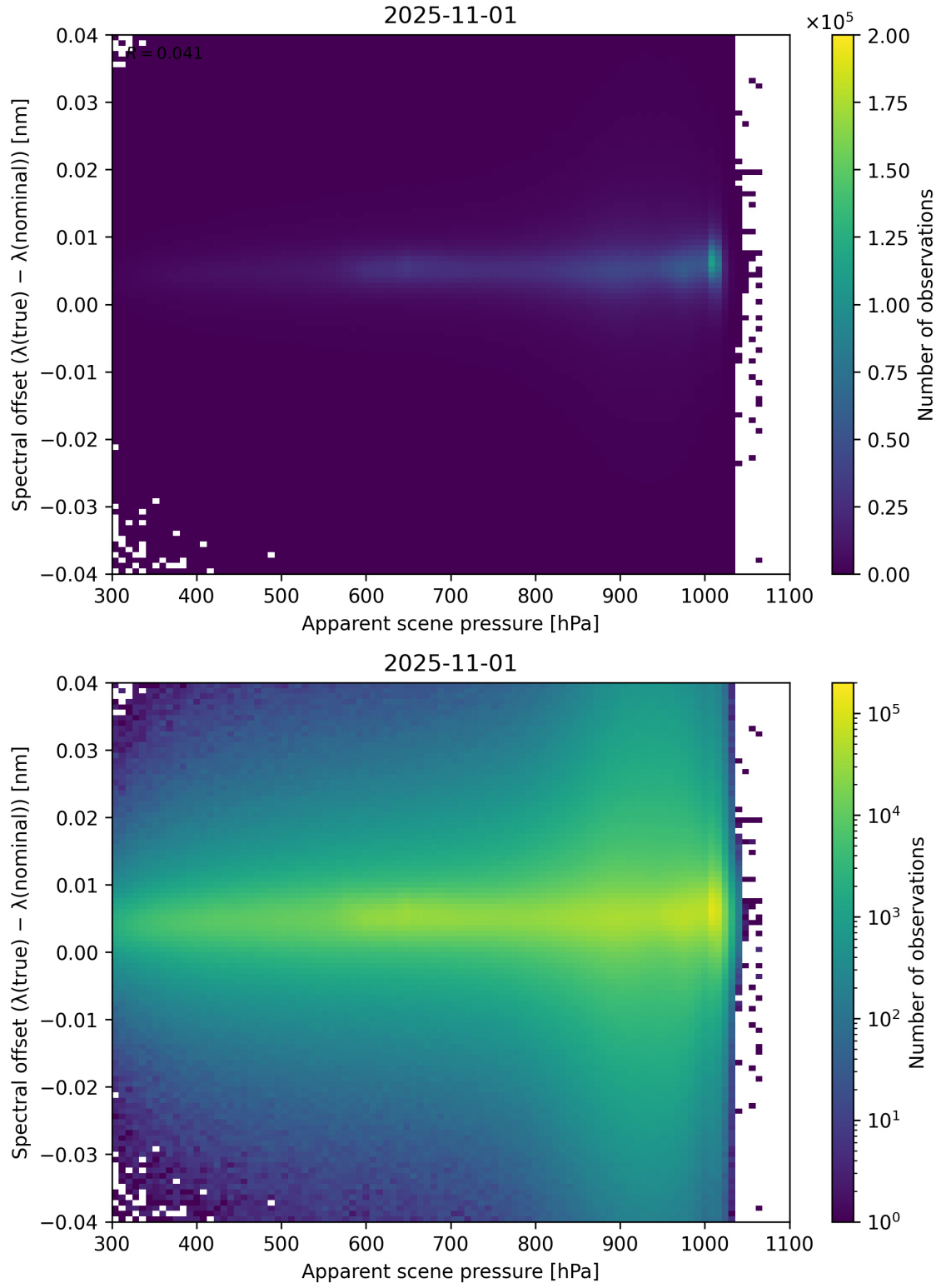
Figure 67: Scatter density plot of “Apparent scene pressure” against “Spectral offset ( \lambda_{\text{true}} - \lambda_{\text{nominal}} )” for 2025-10-31 to 2025-11-02.
