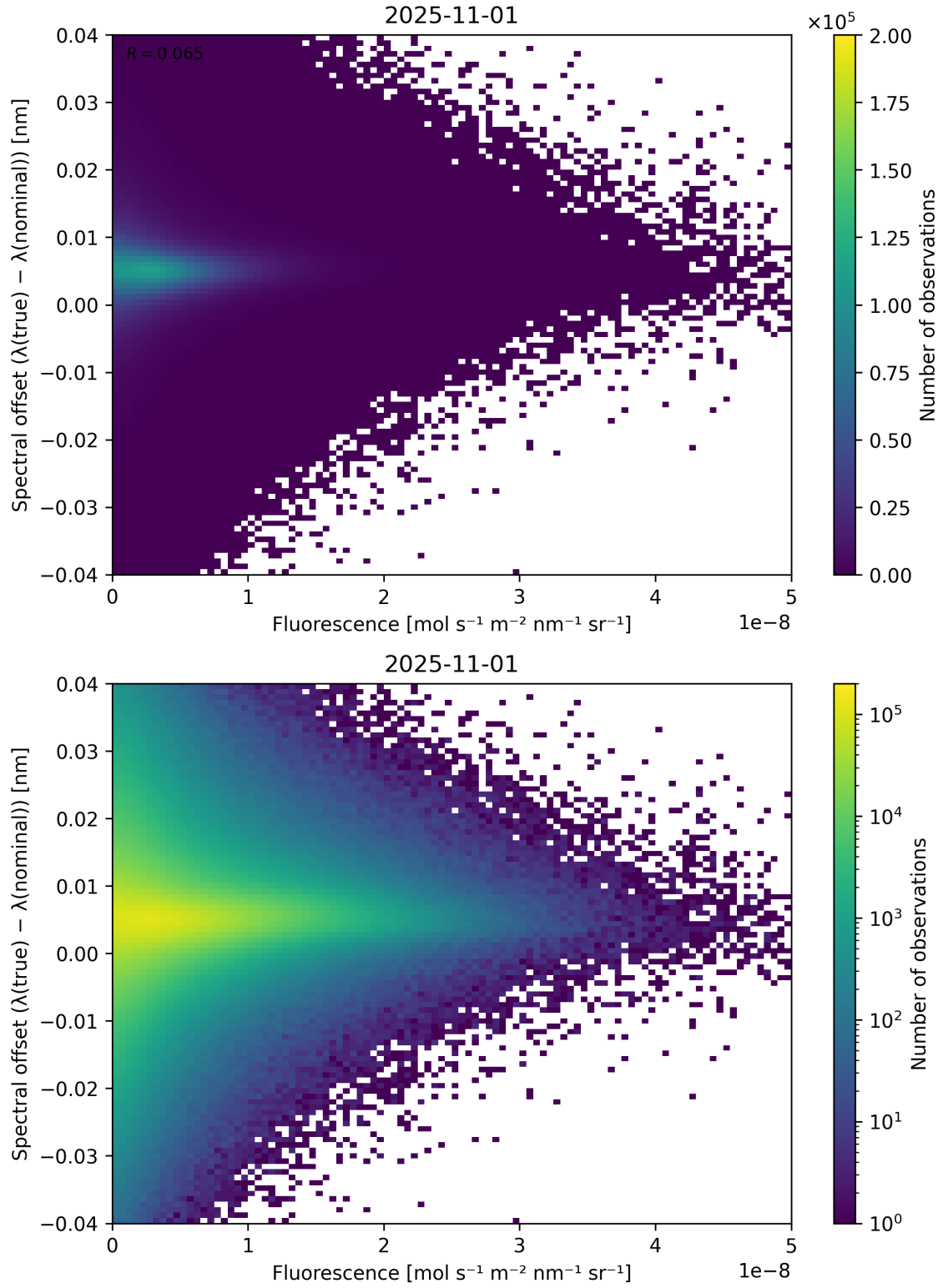
Figure 87: Scatter density plot of “Fluorescence” against “Spectral offset ( \lambda_{\text{true}} - \lambda_{\text{nominal}} )” for 2025-10-31 to 2025-11-02.
