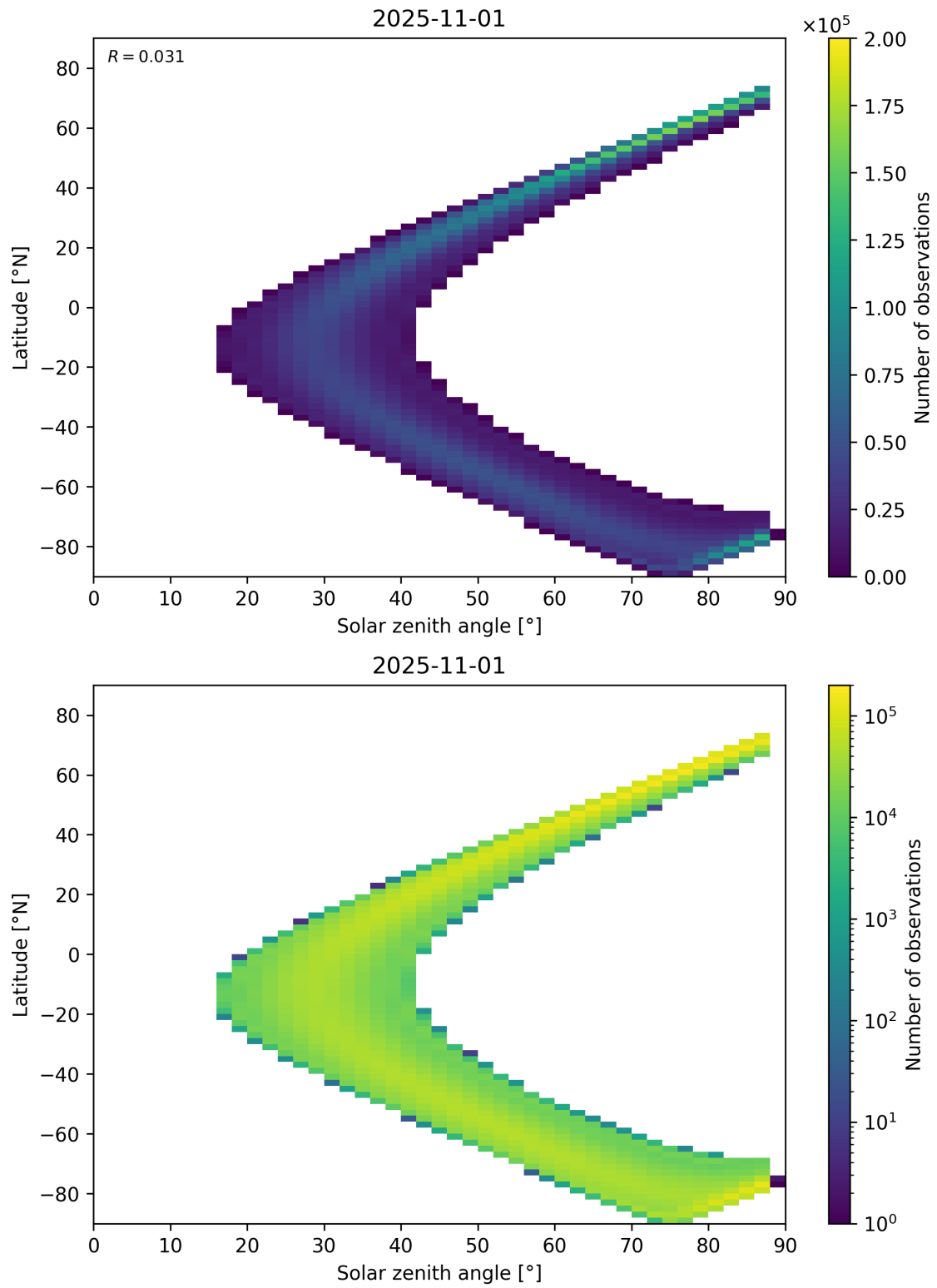
Figure 113: Scatter density plot of “Solar zenith angle” against “Latitude” for 2025-10-31 to 2025-11-02.
