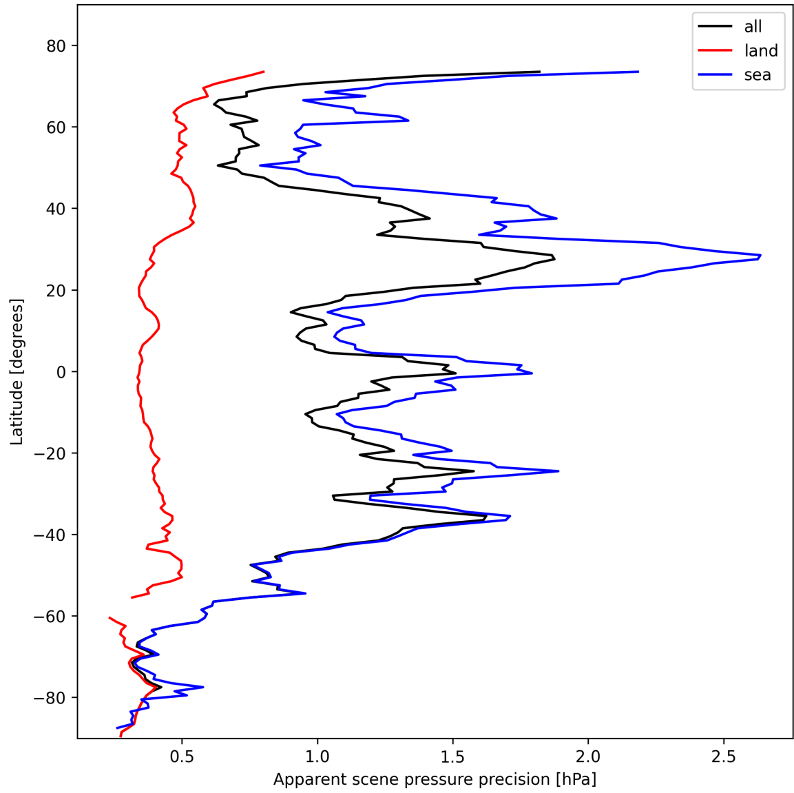
Figure 20: Zonal average of “Apparent scene pressure precision” for 2025-10-31 to 2025-11-02.
