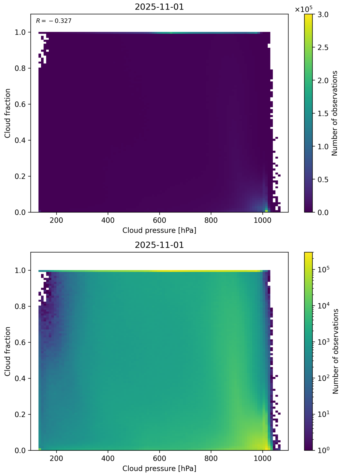
Figure 79: Scatter density plot of “Cloud pressure” against “Cloud fraction” for 2025-10-31 to 2025-11-02.
