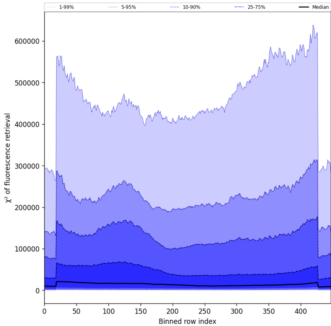
Figure 59: Along track statistics of “ \chi^2 of fluorescence retrieval” for 2025-10-31 to 2025-11-02
