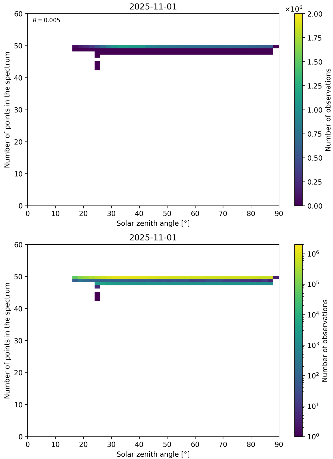
Figure 115: Scatter density plot of “Solar zenith angle” against “Number of points in the spectrum” for 2025-10-31 to 2025-11-02.
