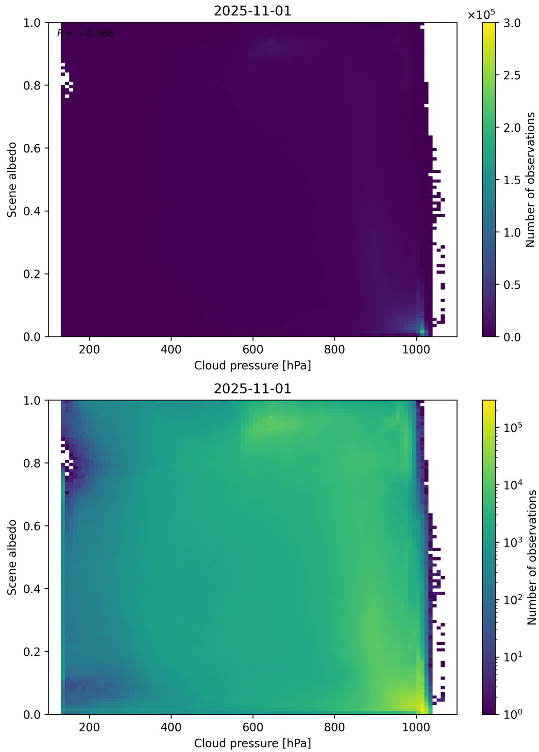
Figure 83: Scatter density plot of “Cloud pressure” against “Scene albedo” for 2025-10-31 to 2025-11-02.
