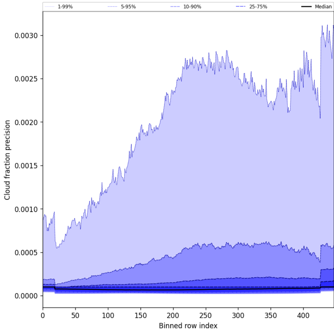
Figure 50: Along track statistics of “Cloud fraction precision” for 2025-10-31 to 2025-11-02
