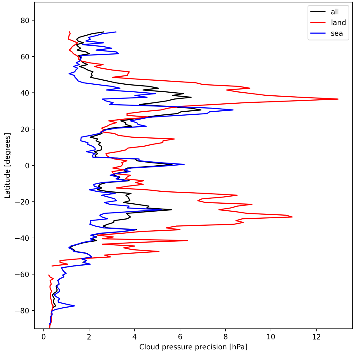
Figure 14: Zonal average of “Cloud pressure precision” for 2025-10-31 to 2025-11-02.
