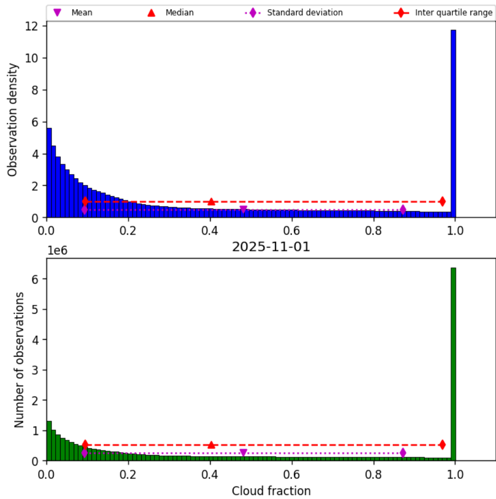
Figure 32: Histogram of “Cloud fraction” for 2025-10-31 to 2025-11-02
