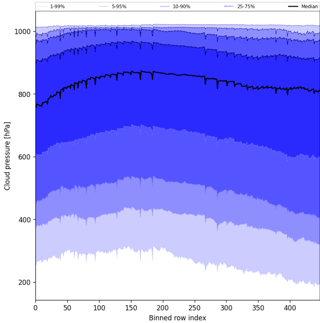
Figure 47: Along track statistics of “Cloud pressure” for 2025-10-31 to 2025-11-02
