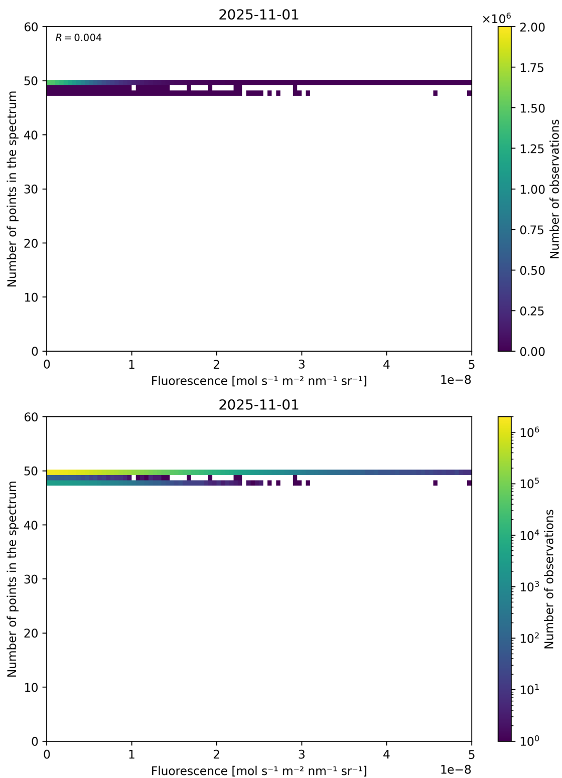
Figure 86: Scatter density plot of “Fluorescence” against “Number of points in the spectrum” for 2025-10-31 to 2025-11-02.
