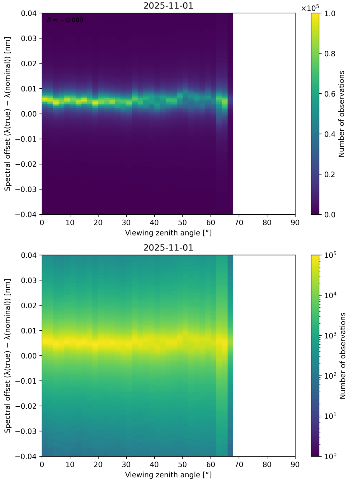
Figure 128: Scatter density plot of “Viewing zenith angle” against “Spectral offset ( \lambda_{\text{true}} - \lambda_{\text{nominal}} )” for 2025-10-31 to 2025-11-02.
