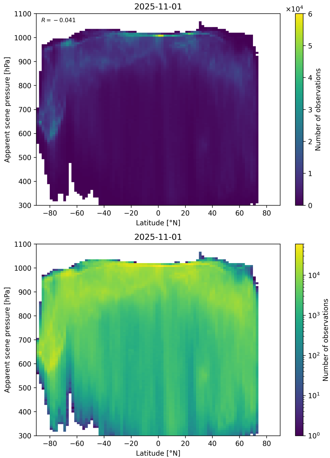
Figure 88: Scatter density plot of “Latitude” against “Apparent scene pressure” for 2025-10-31 to 2025-11-02.
