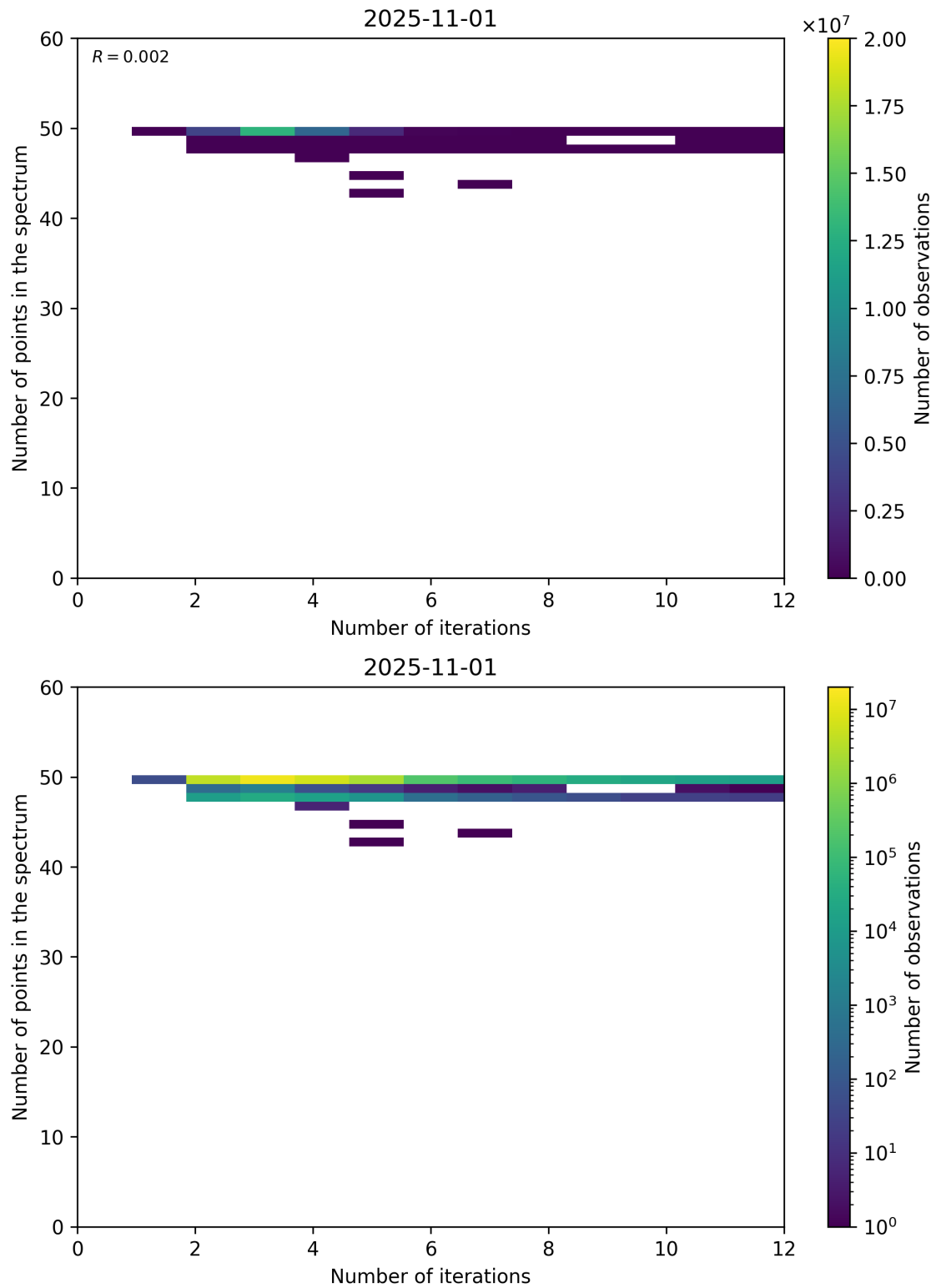
Figure 99: Scatter density plot of “Number of iterations” against “Number of points in the spectrum” for 2025-10-31 to 2025-11-02.
