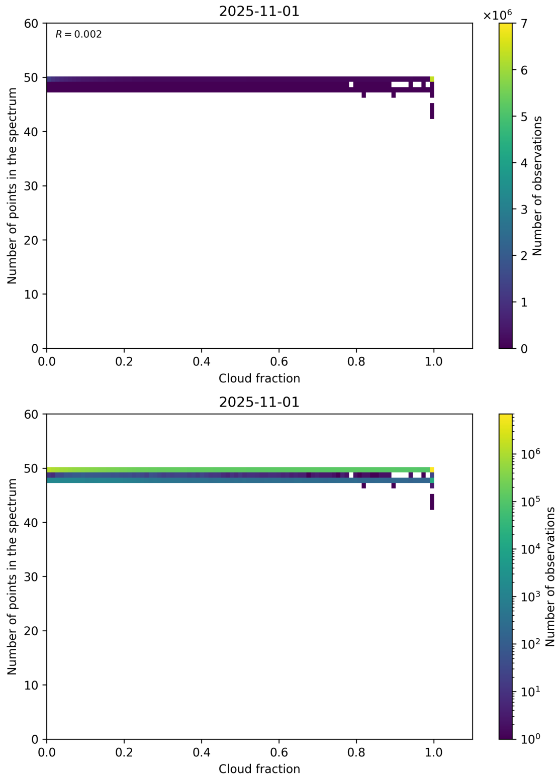
Figure 74: Scatter density plot of “Cloud fraction” against “Number of points in the spectrum” for 2025-10-31 to 2025-11-02.
