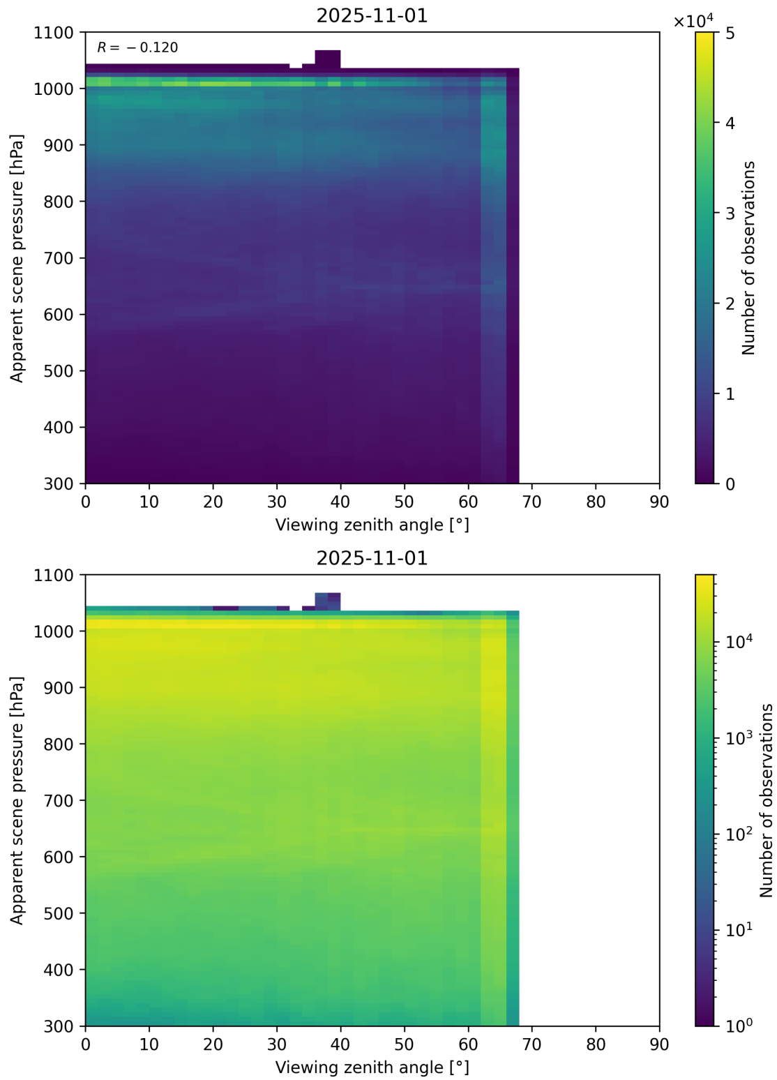
Figure 118: Scatter density plot of “Viewing zenith angle” against “Apparent scene pressure” for 2025-10-31 to 2025-11-02.
