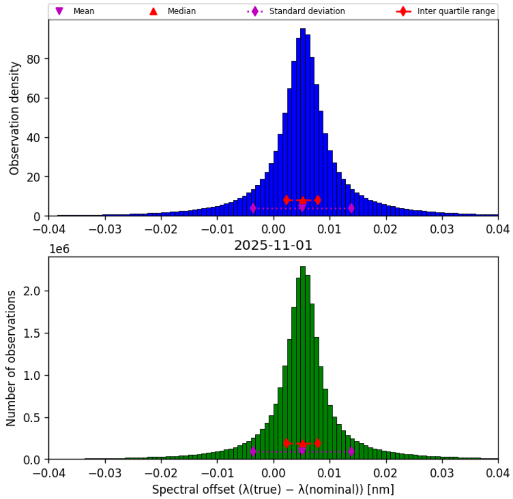
Figure 45: Histogram of “Spectral offset ( \lambda_{\text{true}} - \lambda_{\text{nominal}} )” for 2025-10-31 to 2025-11-02
