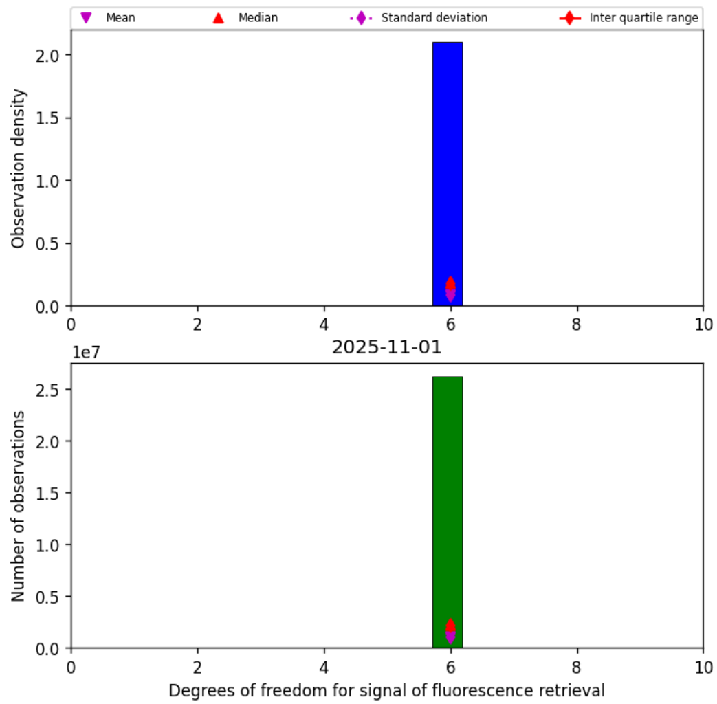
Figure 43: Histogram of "Degrees of freedom for signal of fluorescence retrieval" for 2025-10-31 to 2025-11-02
