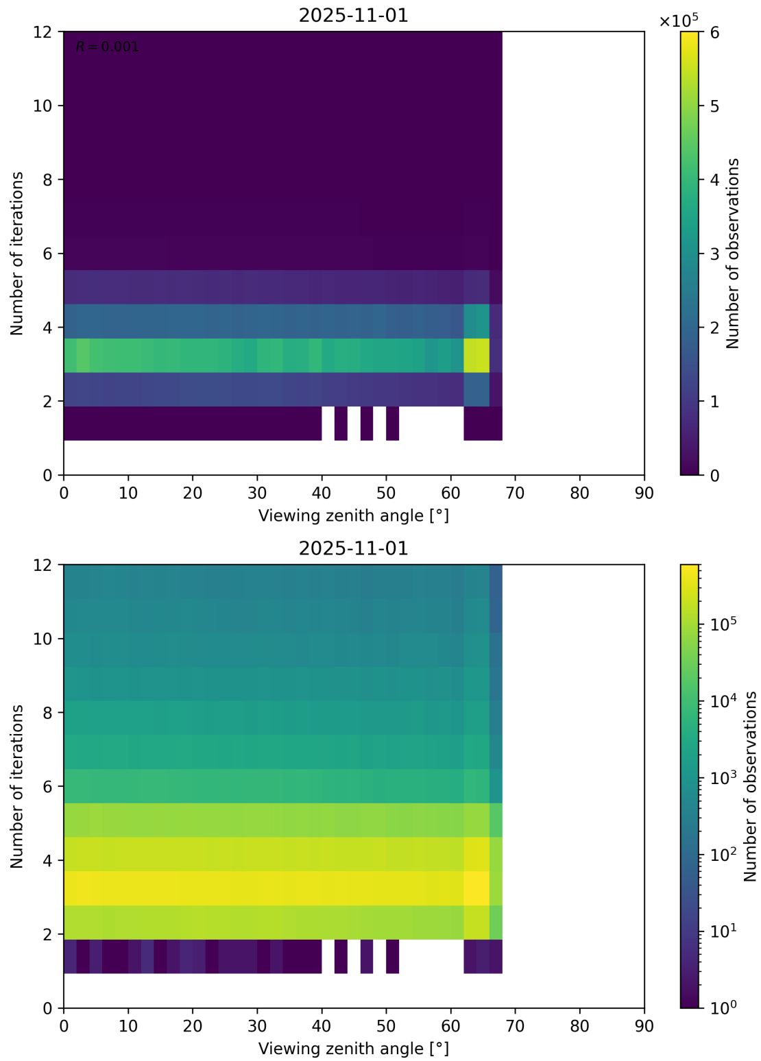
Figure 124: Scatter density plot of “Viewing zenith angle” against “Number of iterations” for 2025-10-31 to 2025-11-02.
