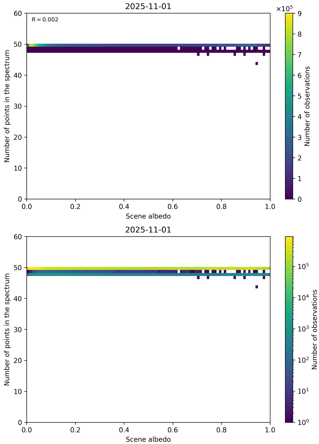
Figure 106: Scatter density plot of “Scene albedo” against “Number of points in the spectrum” for 2025-10-31 to 2025-11-02.
