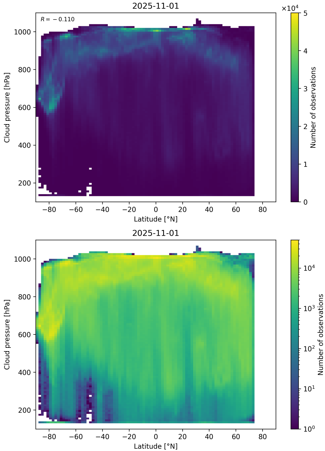
Figure 91: Scatter density plot of “Latitude” against “Cloud pressure” for 2025-10-31 to 2025-11-02.
