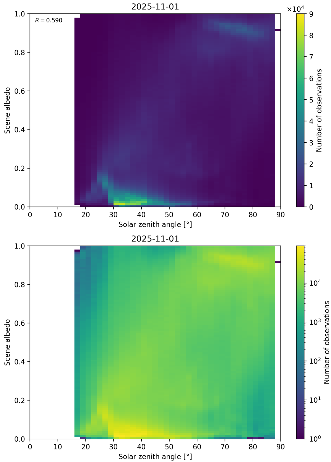
Figure 116: Scatter density plot of “Solar zenith angle” against “Scene albedo” for 2025-10-31 to 2025-11-02.
