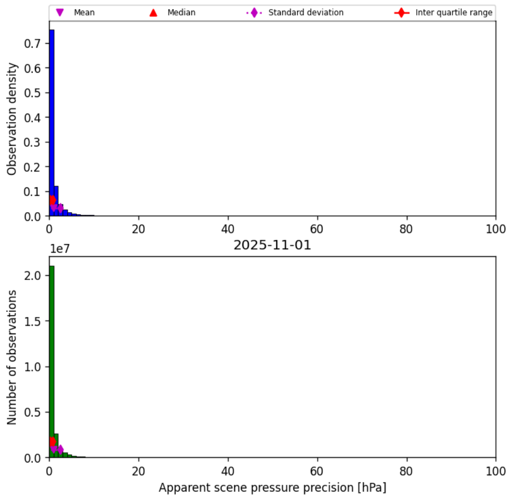
Figure 37: Histogram of “Apparent scene pressure precision” for 2025-10-31 to 2025-11-02
