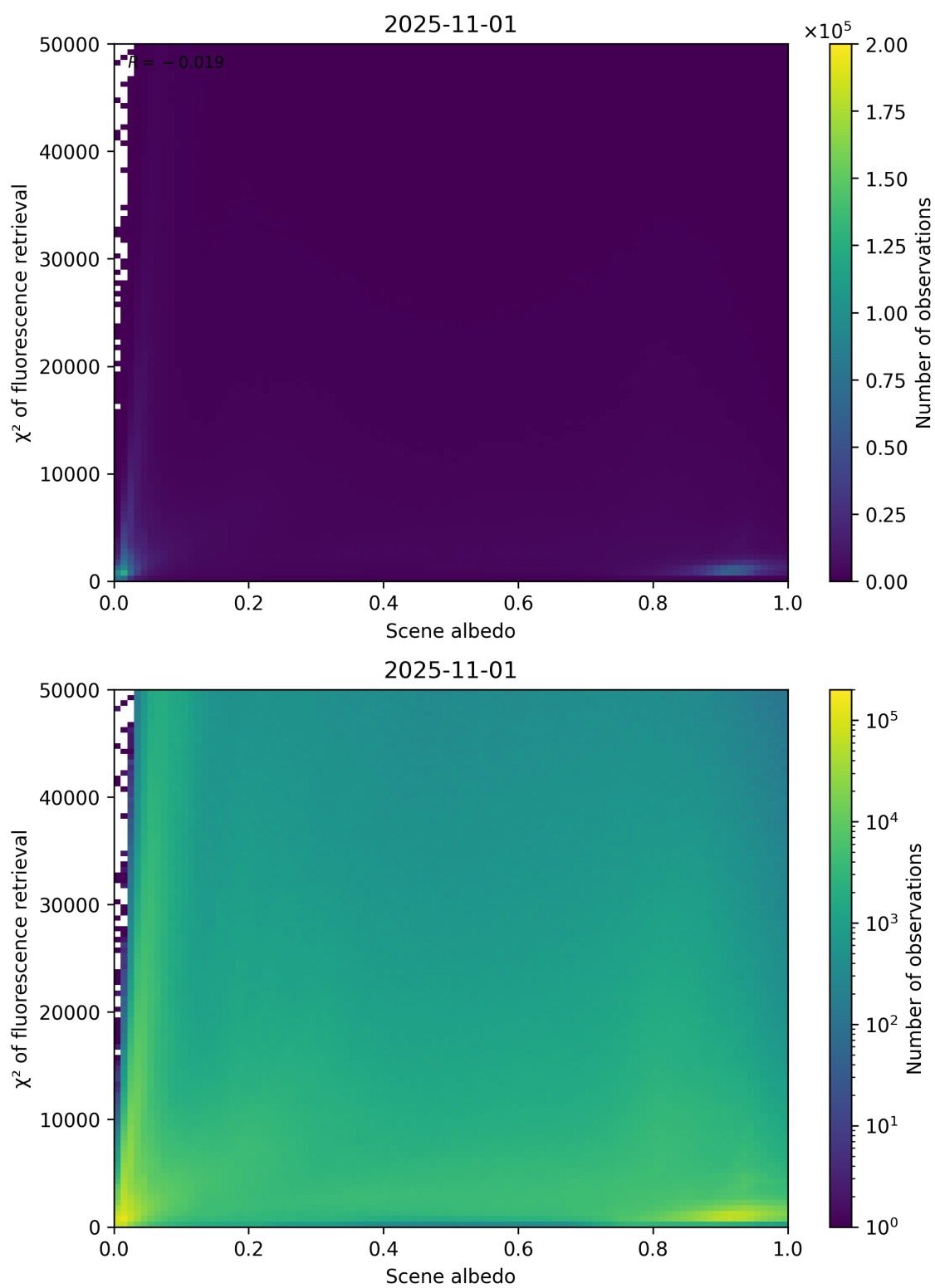
Figure 103: Scatter density plot of “Scene albedo” against “ \chi^2 of fluorescence retrieval” for 2025-10-31 to 2025-11-02.
