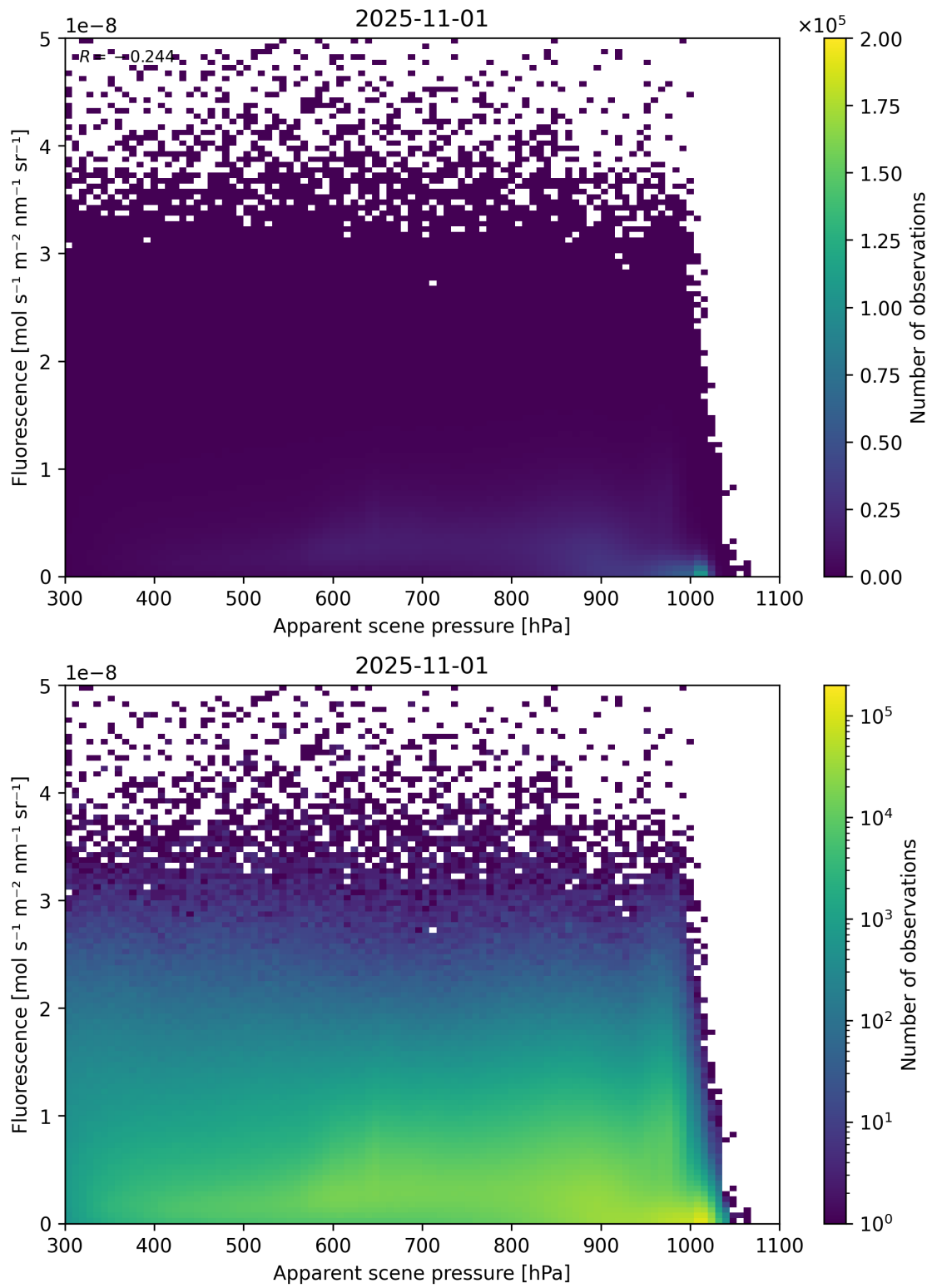
Figure 64: Scatter density plot of “Apparent scene pressure” against “Fluorescence” for 2025-10-31 to 2025-11-02.
