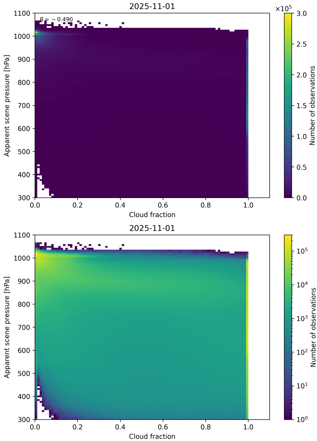
Figure 70: Scatter density plot of “Cloud fraction” against “Apparent scene pressure” for 2025-10-31 to 2025-11-02.
