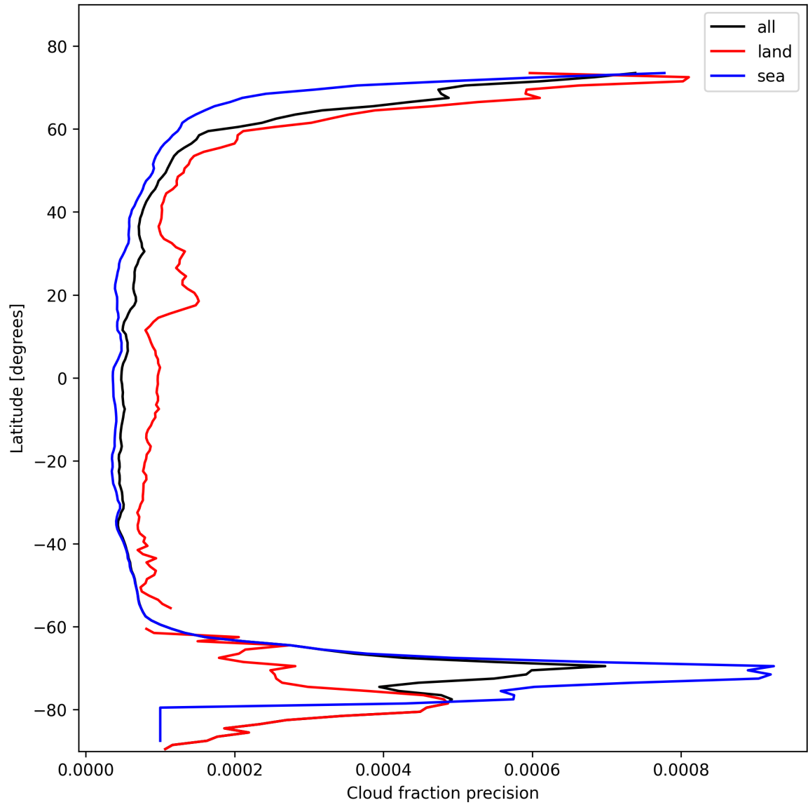
Figure 16: Zonal average of “Cloud fraction precision” for 2025-10-31 to 2025-11-02.
