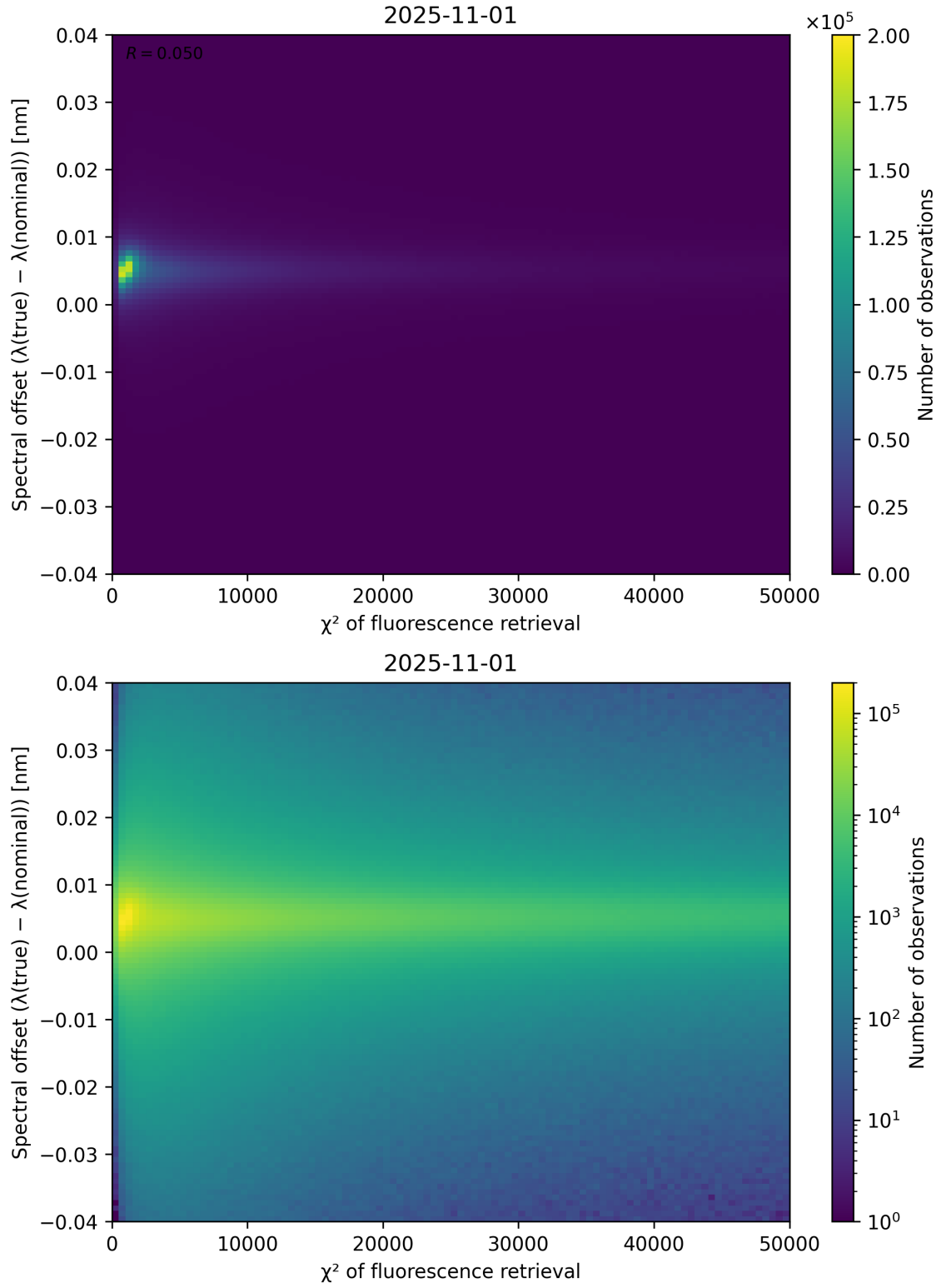
Figure 69: Scatter density plot of “ \chi^2 of fluorescence retrieval” against “Spectral offset ( \lambda_{\text{true}} - \lambda_{\text{nominal}} )” for 2025-10-31 to 2025-11-02.
