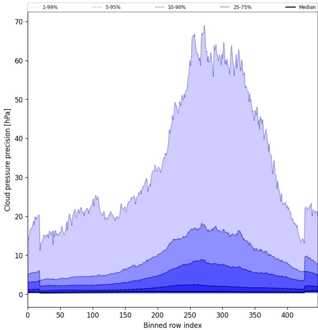
Figure 48: Along track statistics of “Cloud pressure precision” for 2025-10-31 to 2025-11-02
