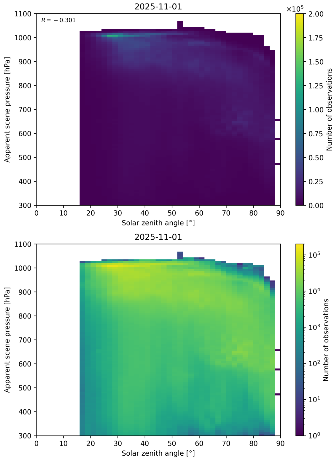
Figure 108: Scatter density plot of “Solar zenith angle” against “Apparent scene pressure” for 2025-10-31 to 2025-11-02.
