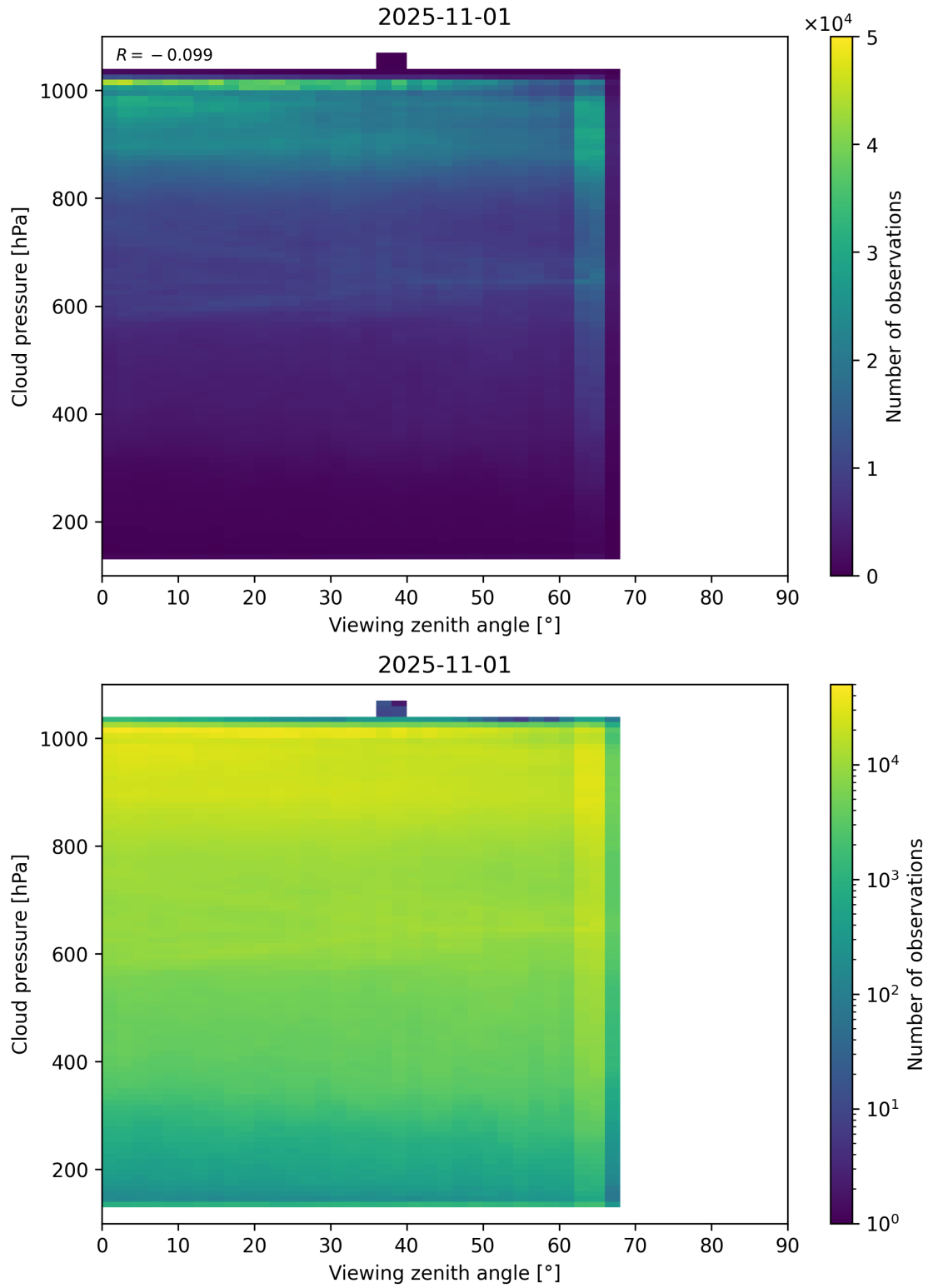
Figure 121: Scatter density plot of “Viewing zenith angle” against “Cloud pressure” for 2025-10-31 to 2025-11-02.
