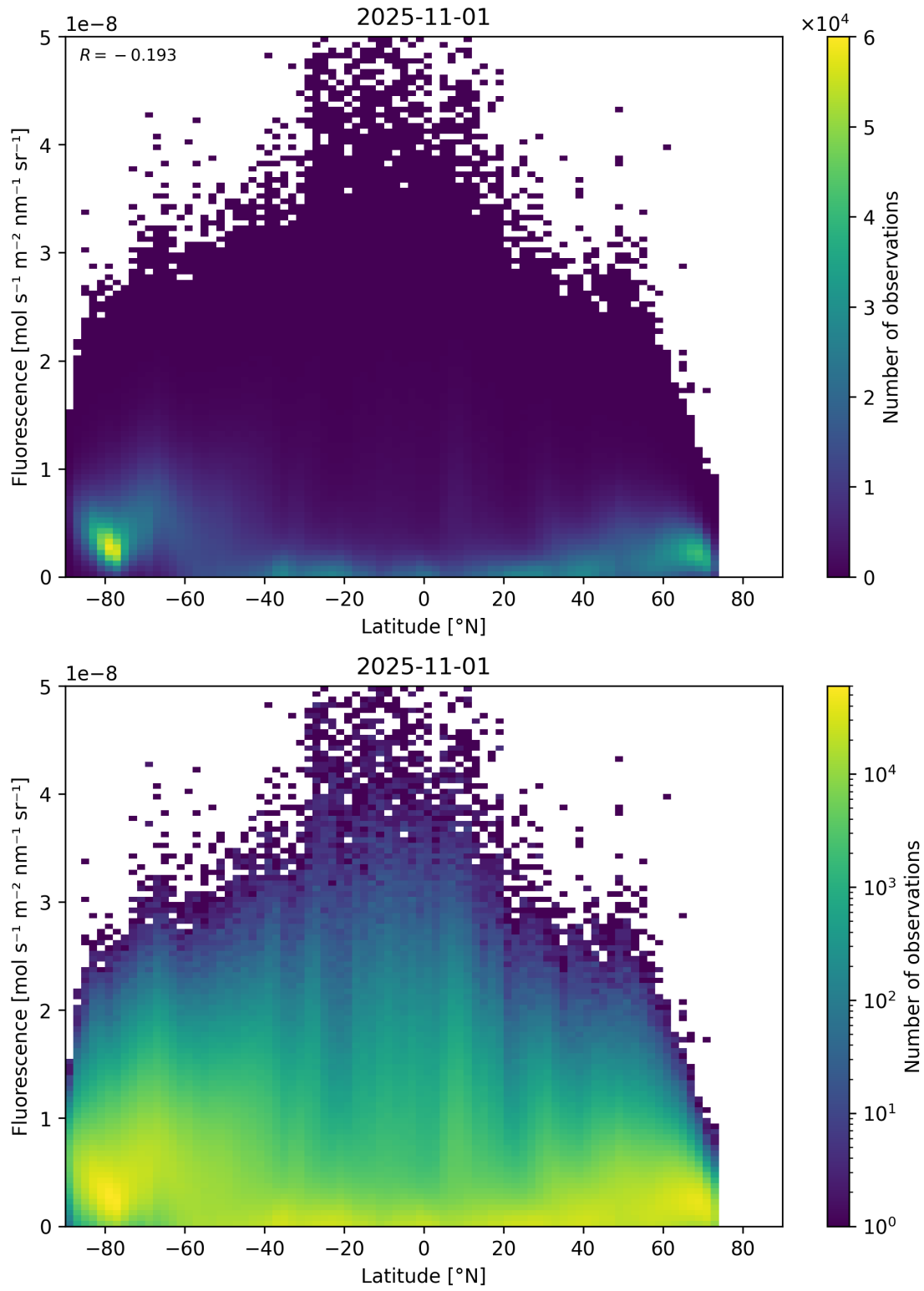
Figure 92: Scatter density plot of “Latitude” against “Fluorescence” for 2025-10-31 to 2025-11-02.
