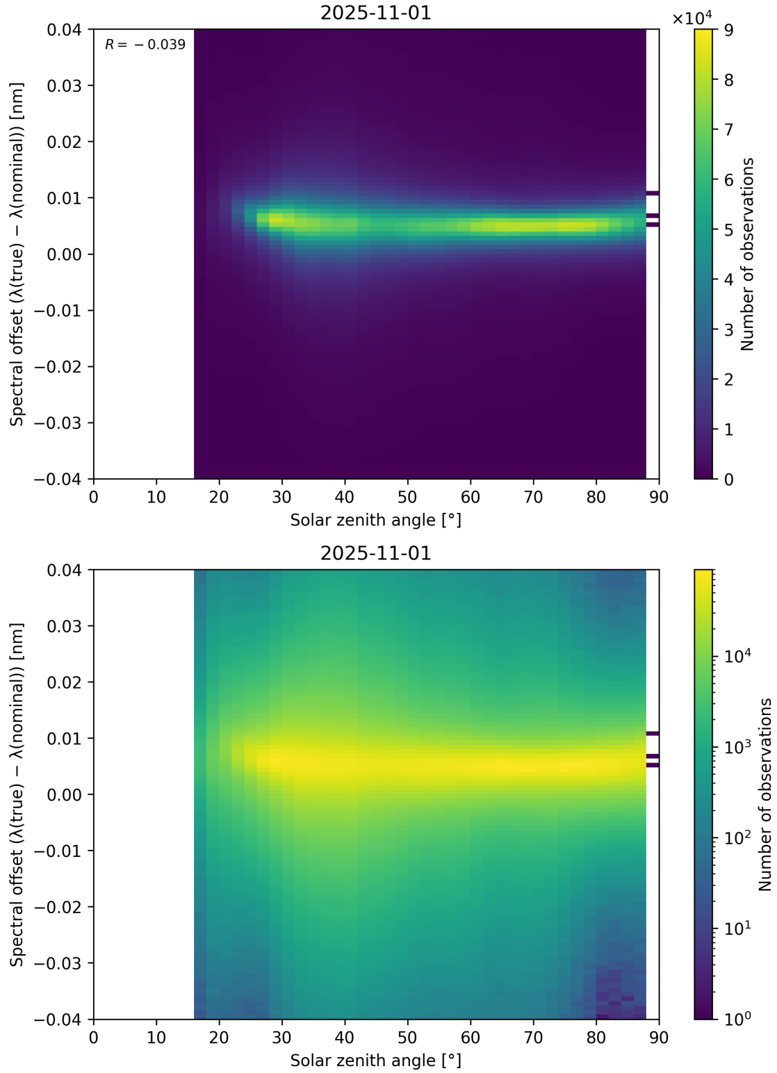
Figure 117: Scatter density plot of “Solar zenith angle” against “Spectral offset ( \lambda_{\text{true}} - \lambda_{\text{nominal}} )” for 2025-10-31 to 2025-11-02.
