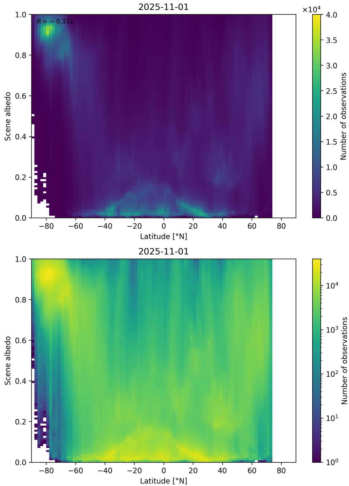
Figure 95: Scatter density plot of “Latitude” against “Scene albedo” for 2025-10-31 to 2025-11-02.
