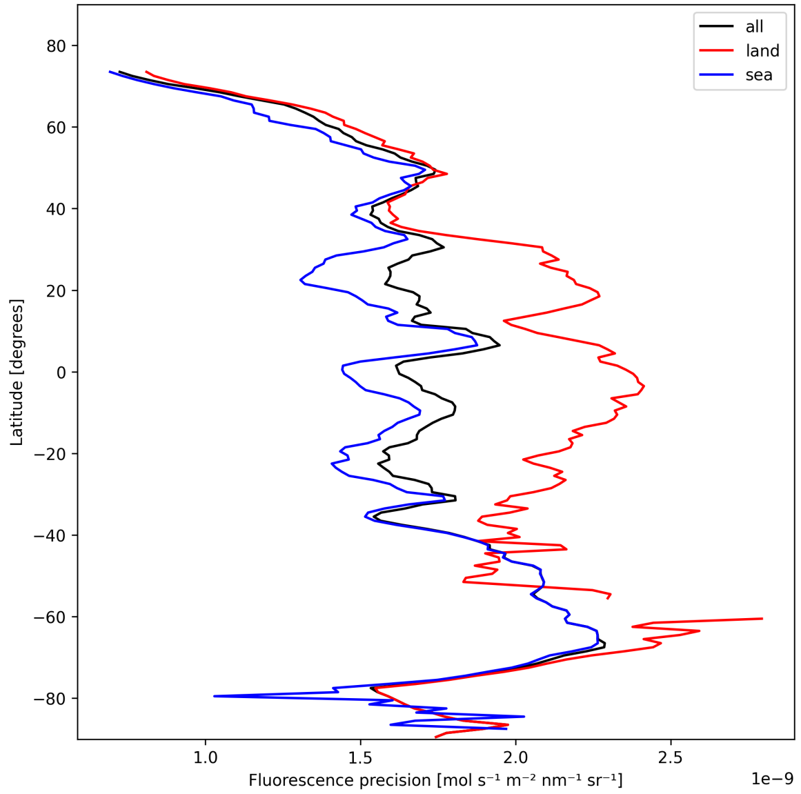
Figure 24: Zonal average of “Fluorescence precision” for 2025-10-31 to 2025-11-02.
