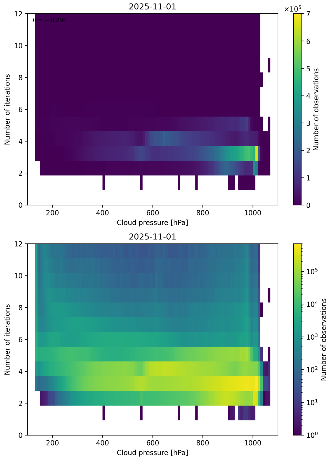
Figure 81: Scatter density plot of “Cloud pressure” against “Number of iterations” for 2025-10-31 to 2025-11-02.
