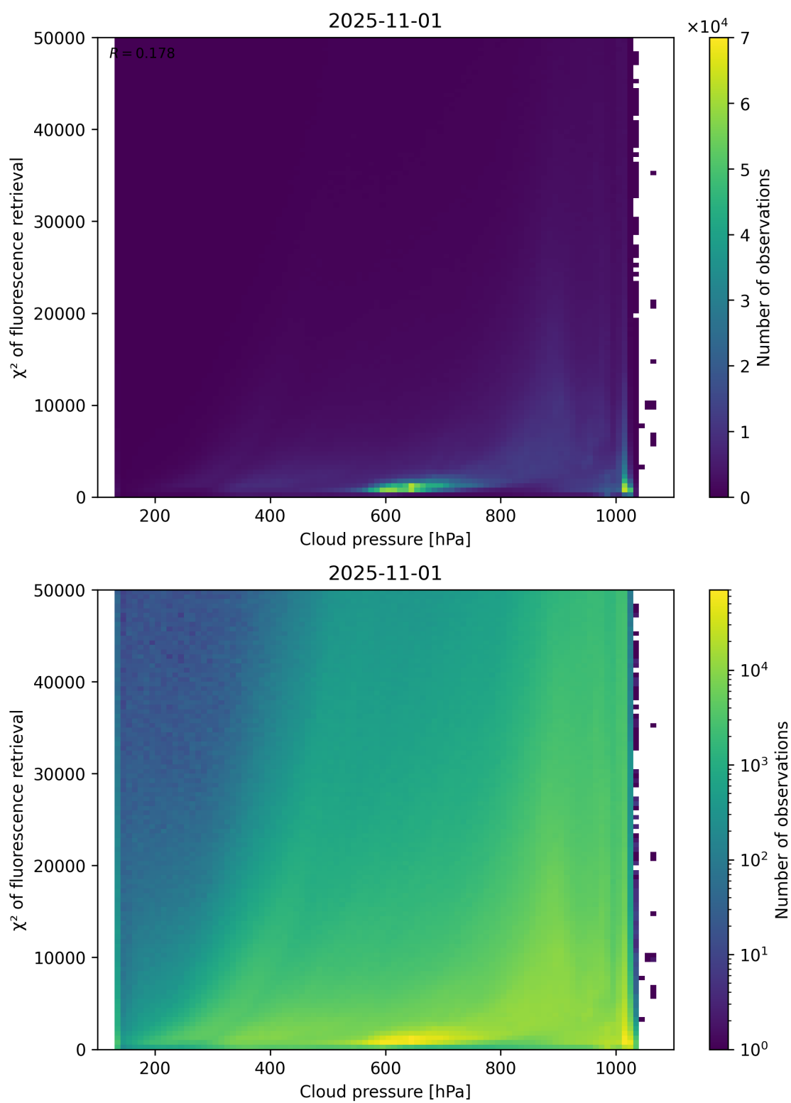
Figure 78: Scatter density plot of “Cloud pressure” against “ \chi^2 of fluorescence retrieval” for 2025-10-31 to 2025-11-02.
