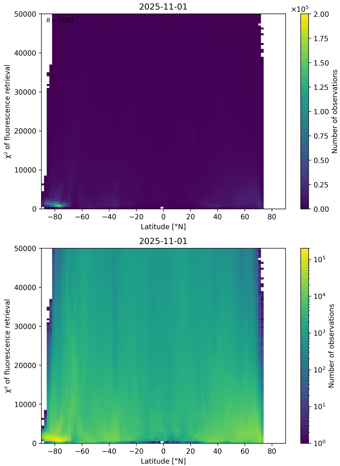
Figure 89: Scatter density plot of “Latitude” against “ \chi^2 of fluorescence retrieval” for 2025-10-31 to 2025-11-02.
