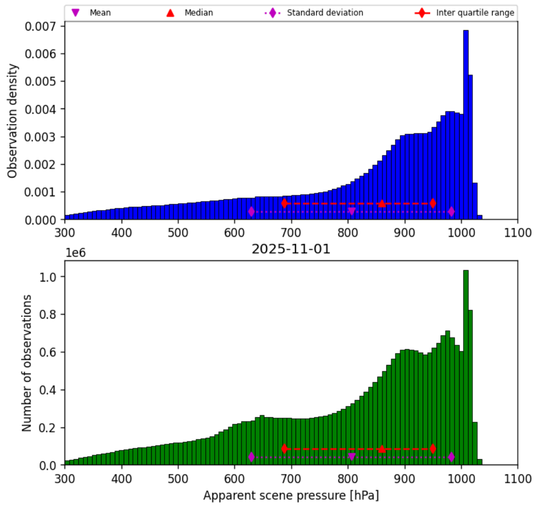
Figure 36: Histogram of “Apparent scene pressure” for 2025-10-31 to 2025-11-02
