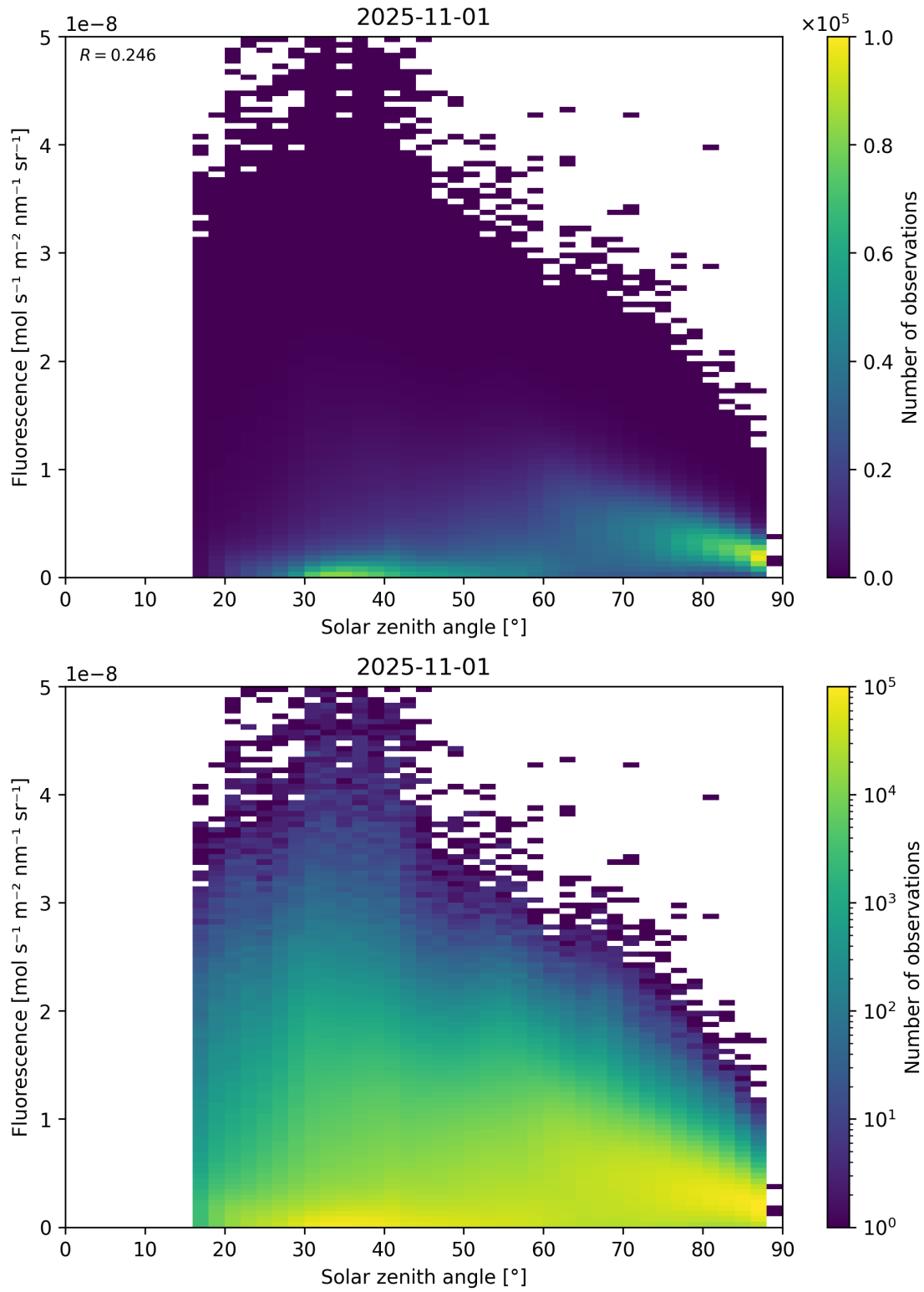
Figure 112: Scatter density plot of “Solar zenith angle” against “Fluorescence” for 2025-10-31 to 2025-11-02.
