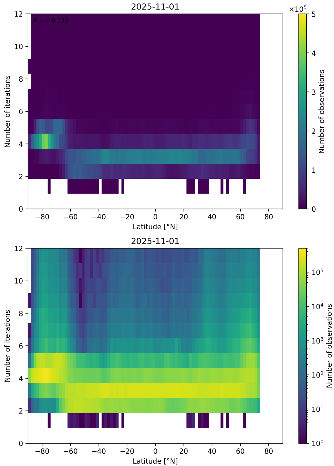
Figure 93: Scatter density plot of “Latitude” against “Number of iterations” for 2025-10-31 to 2025-11-02.
