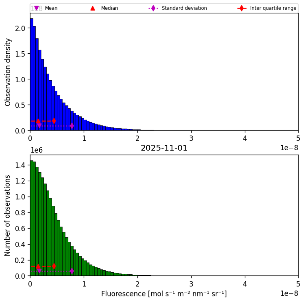
Figure 40: Histogram of “Fluorescence” for 2025-10-31 to 2025-11-02
