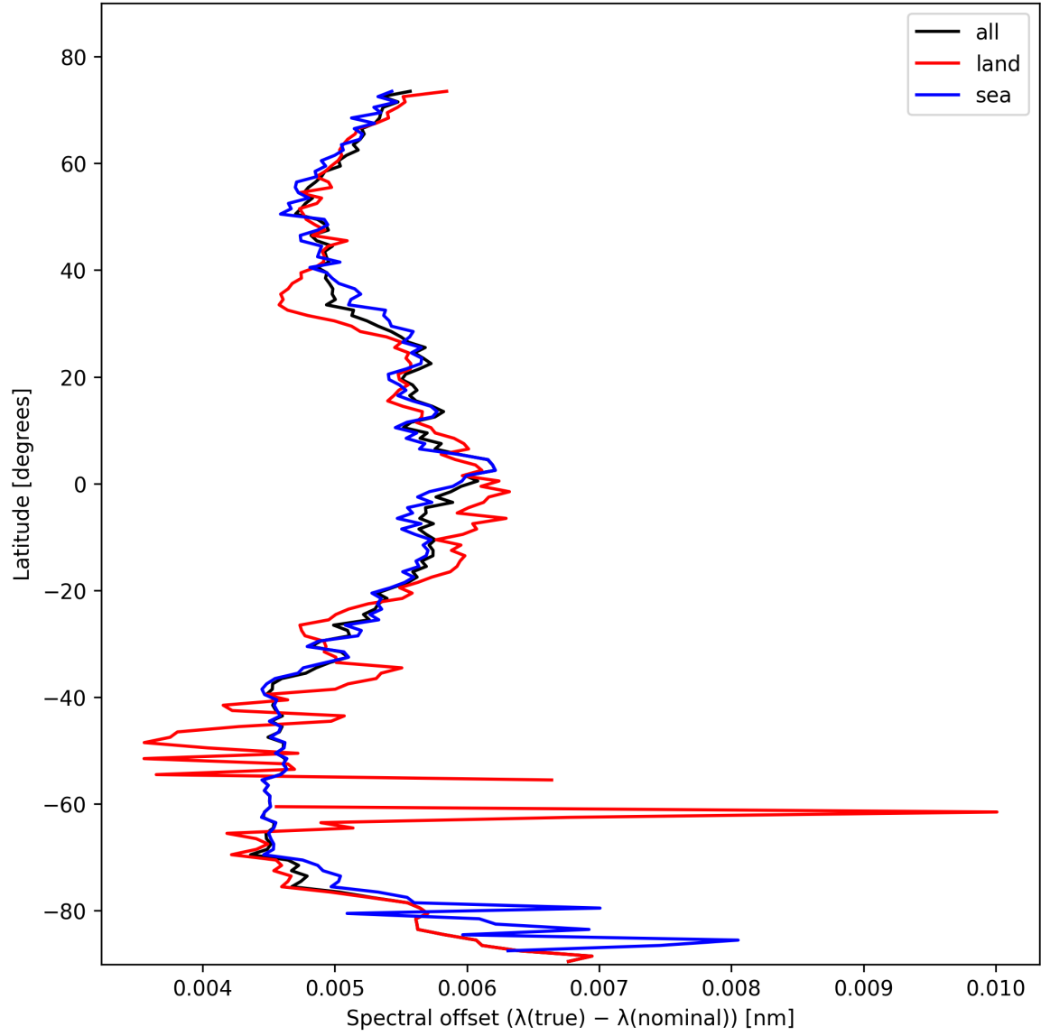
Figure 28: Zonal average of “Spectral offset ( \lambda_{\text{true}} - \lambda_{\text{nominal}} )” for 2025-10-31 to 2025-11-02.
