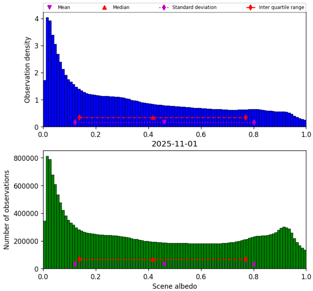
Figure 34: Histogram of “Scene albedo” for 2025-10-31 to 2025-11-02
