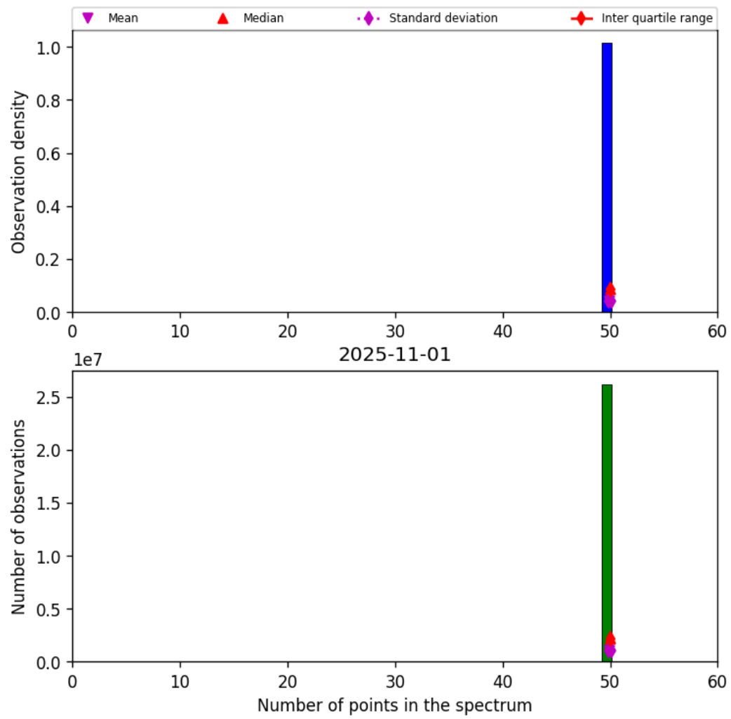
Figure 44: Histogram of “Number of points in the spectrum” for 2025-10-31 to 2025-11-02
