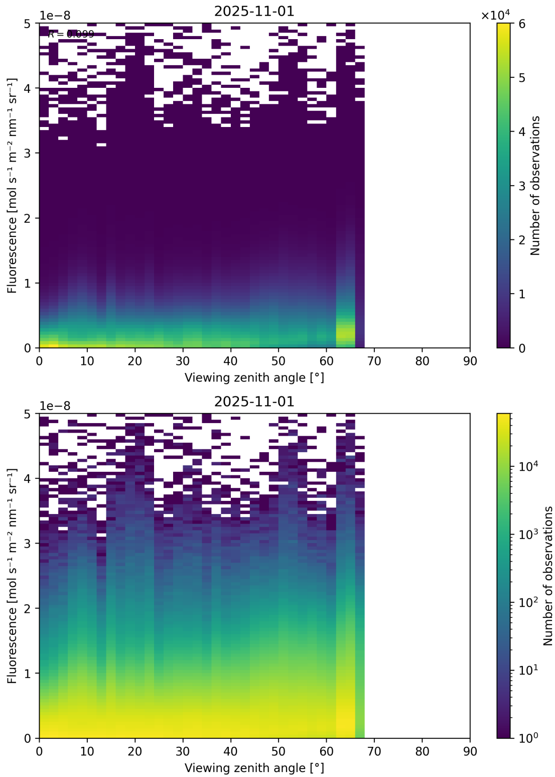
Figure 122: Scatter density plot of “Viewing zenith angle” against “Fluorescence” for 2025-10-31 to 2025-11-02.
