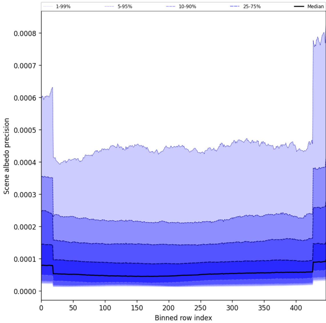
Figure 52: Along track statistics of “Scene albedo precision” for 2025-10-31 to 2025-11-02
