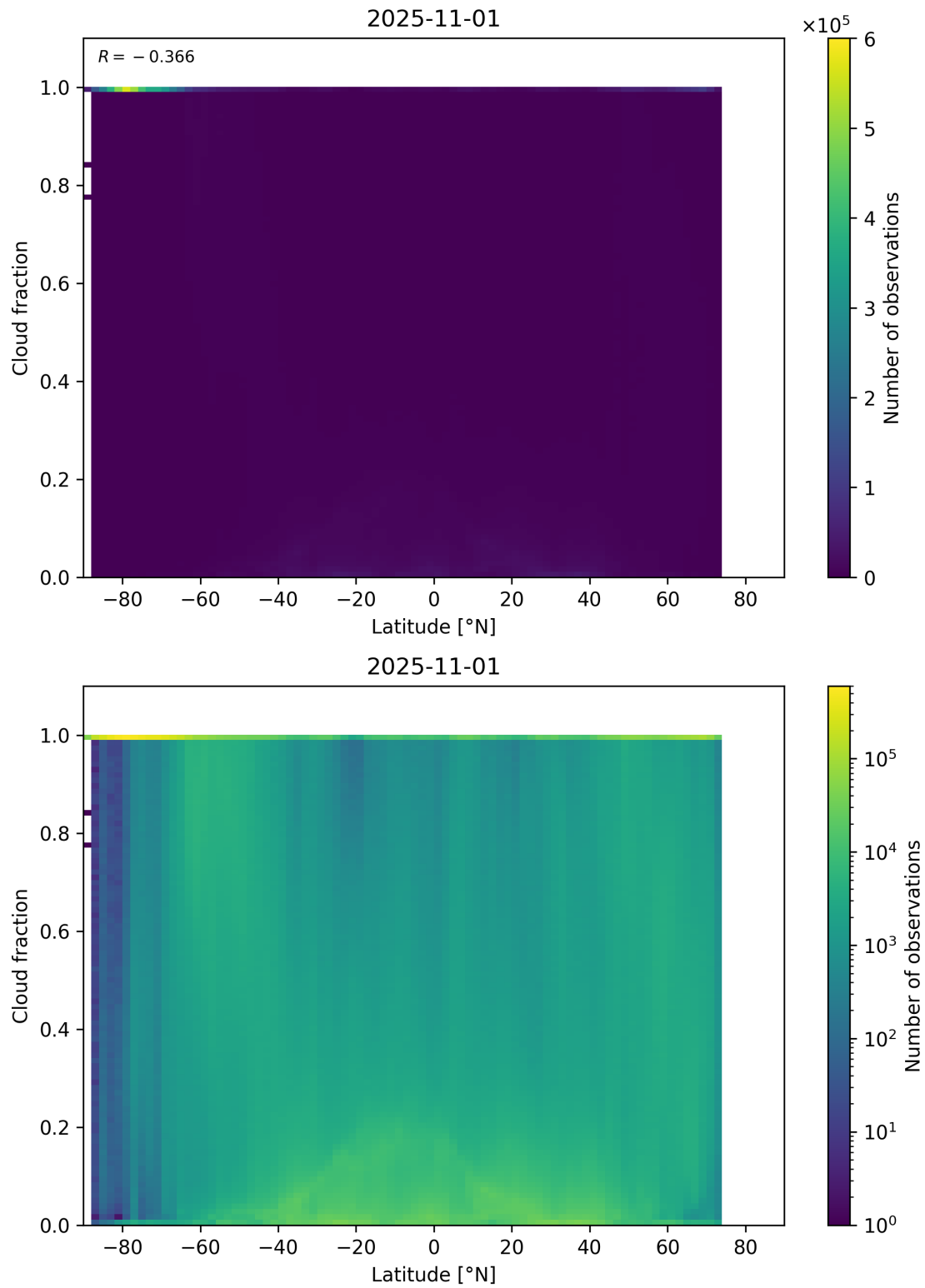
Figure 90: Scatter density plot of “Latitude” against “Cloud fraction” for 2025-10-31 to 2025-11-02.
