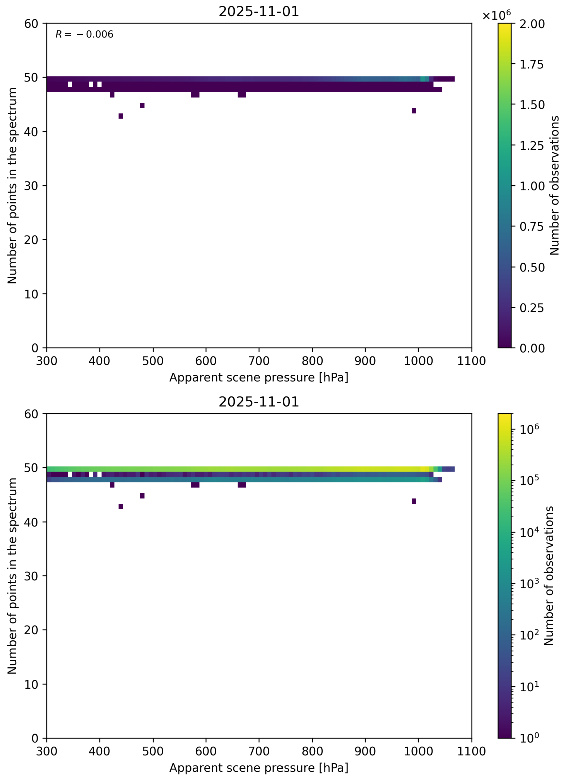
Figure 66: Scatter density plot of “Apparent scene pressure” against “Number of points in the spectrum” for 2025-10-31 to 2025-11-02.
