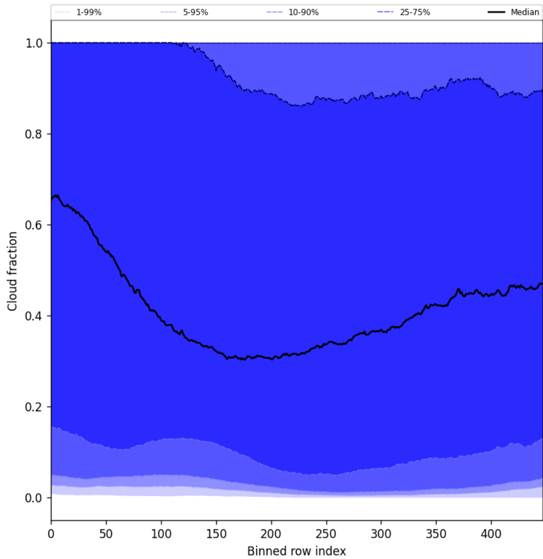
Figure 49: Along track statistics of “Cloud fraction” for 2025-10-31 to 2025-11-02
