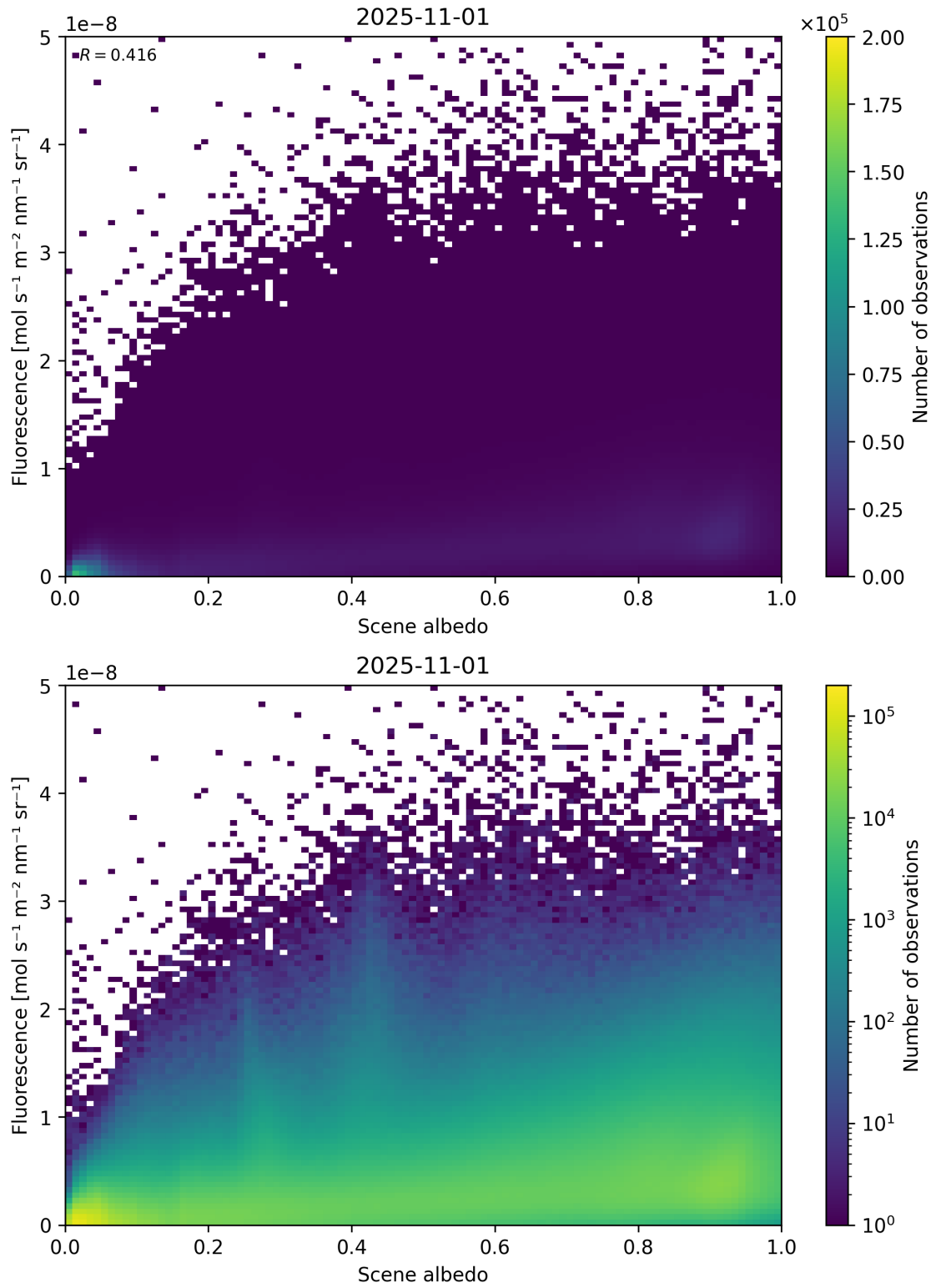
Figure 104: Scatter density plot of "Scene albedo" against "Fluorescence" for 2025-10-31 to 2025-11-02.
