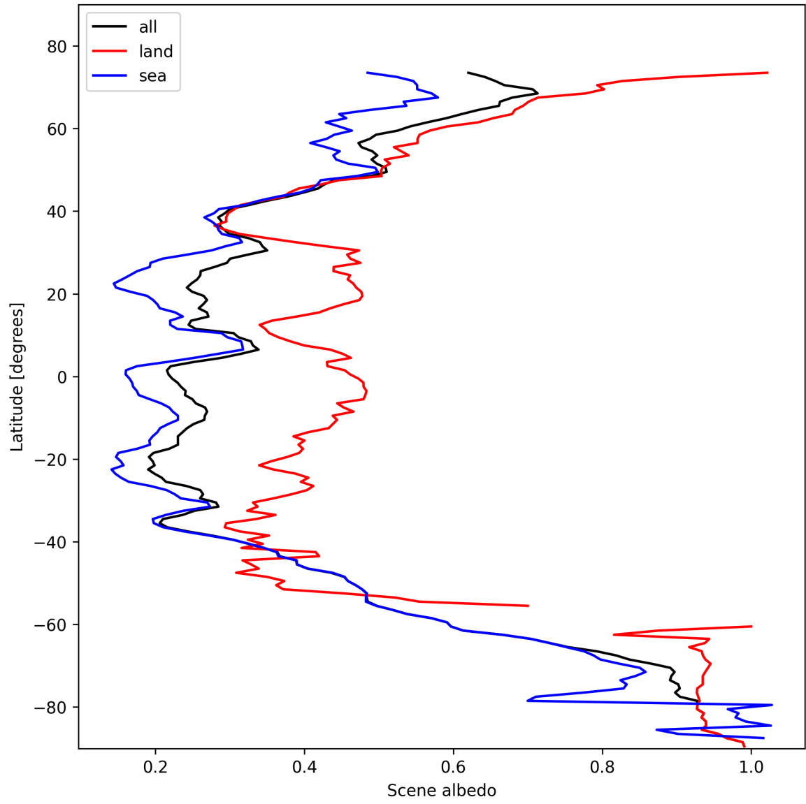
Figure 17: Zonal average of “Scene albedo” for 2025-10-31 to 2025-11-02.
