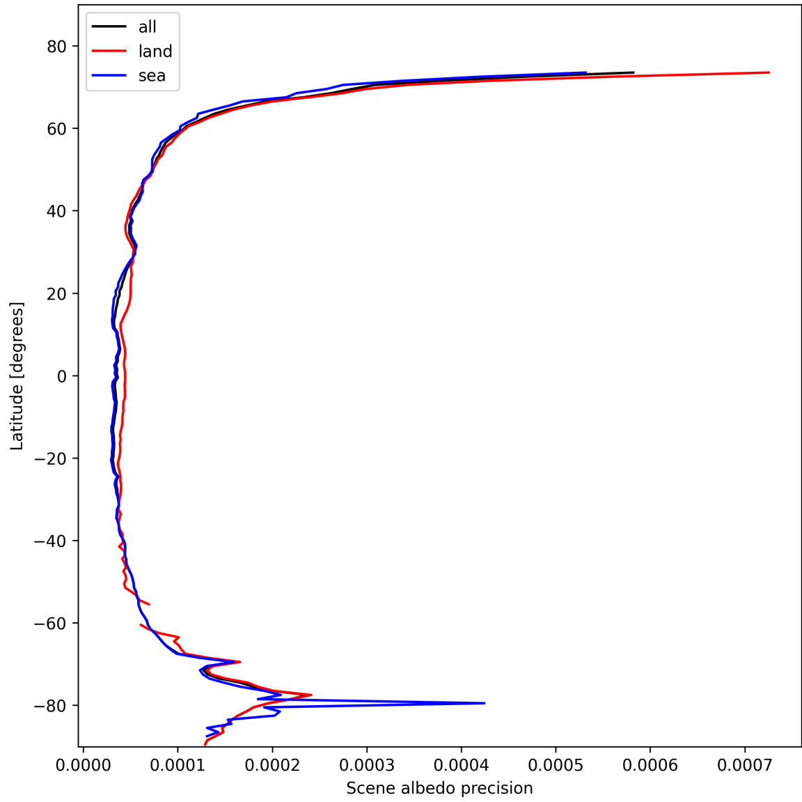
Figure 18: Zonal average of “Scene albedo precision” for 2025-10-31 to 2025-11-02.
