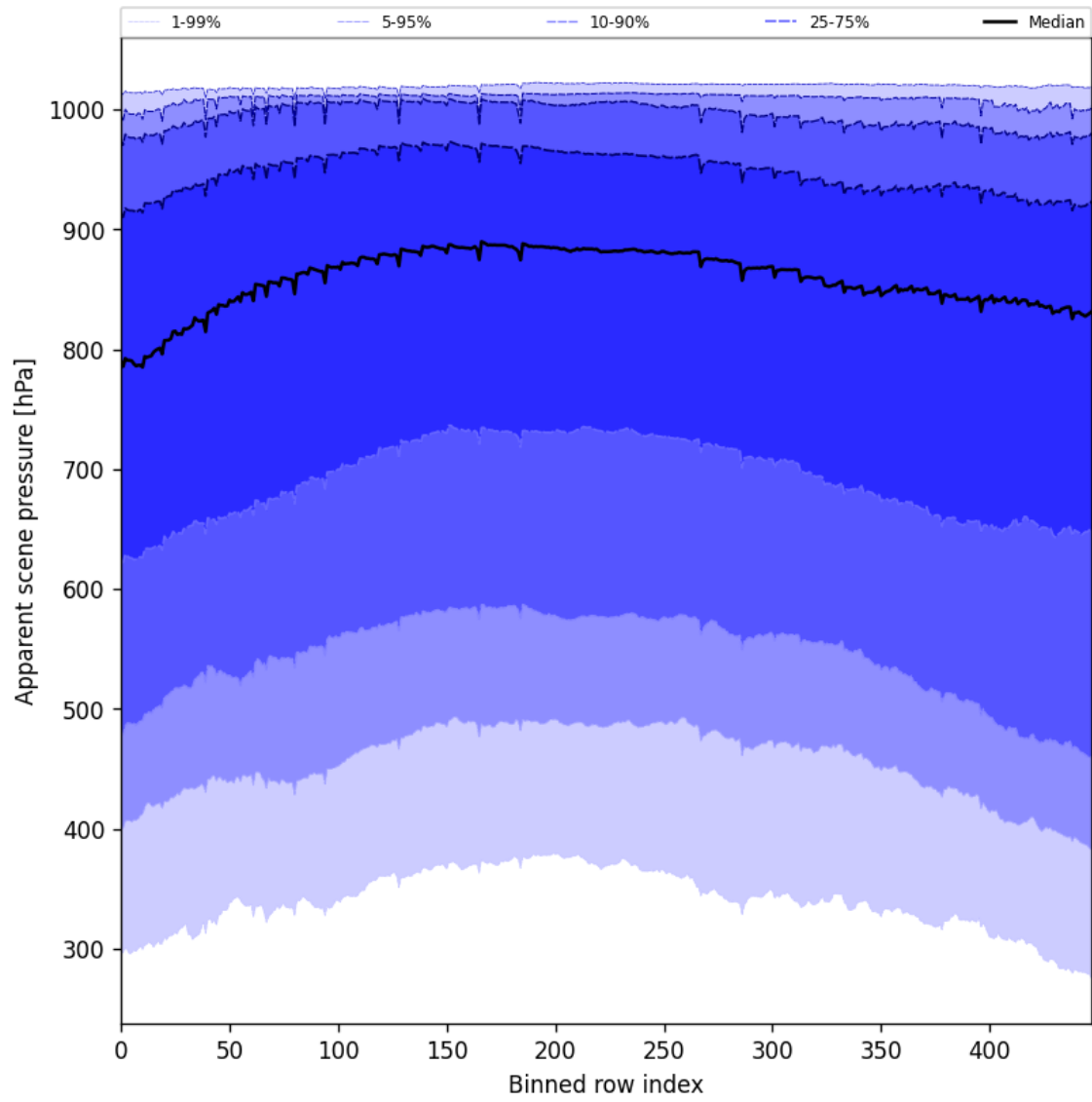
Figure 53: Along track statistics of “Apparent scene pressure” for 2025-10-31 to 2025-11-02
