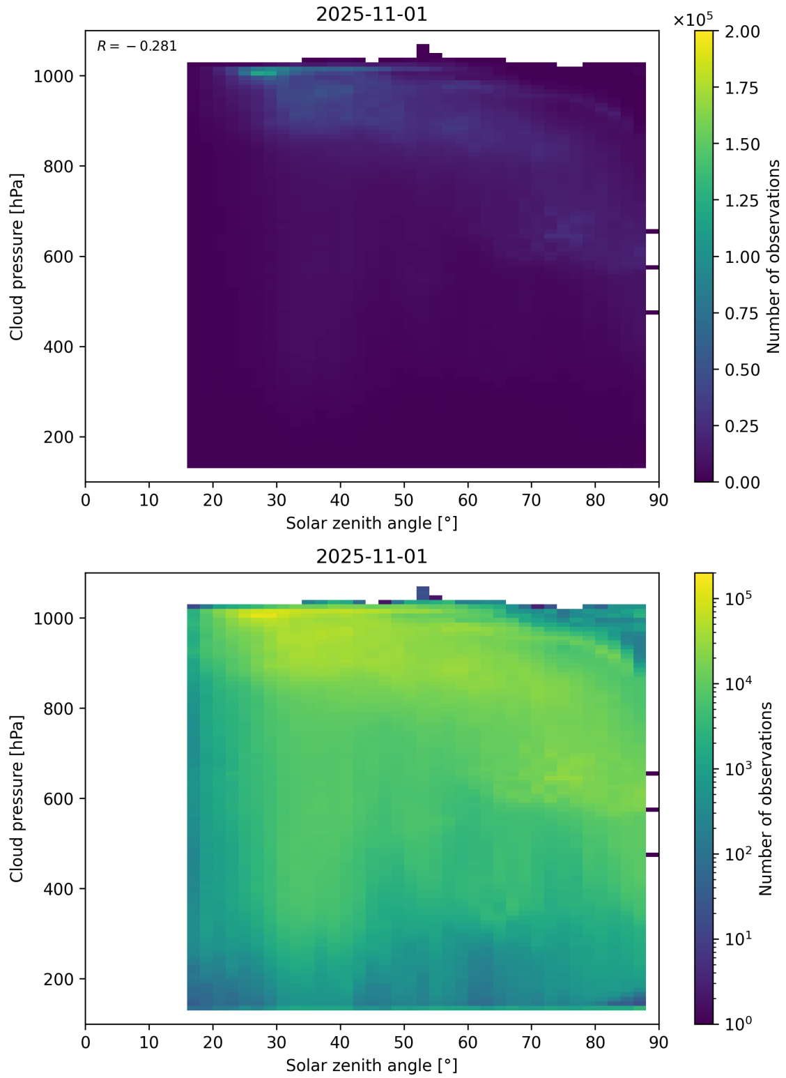
Figure 111: Scatter density plot of “Solar zenith angle” against “Cloud pressure” for 2025-10-31 to 2025-11-02.
