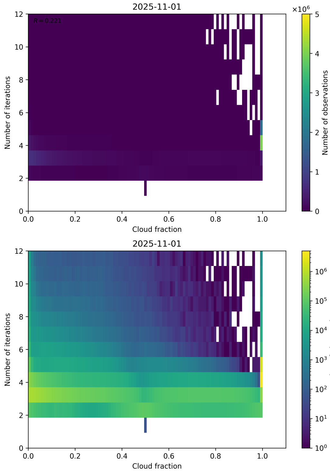
Figure 73: Scatter density plot of “Cloud fraction” against “Number of iterations” for 2025-10-31 to 2025-11-02.
