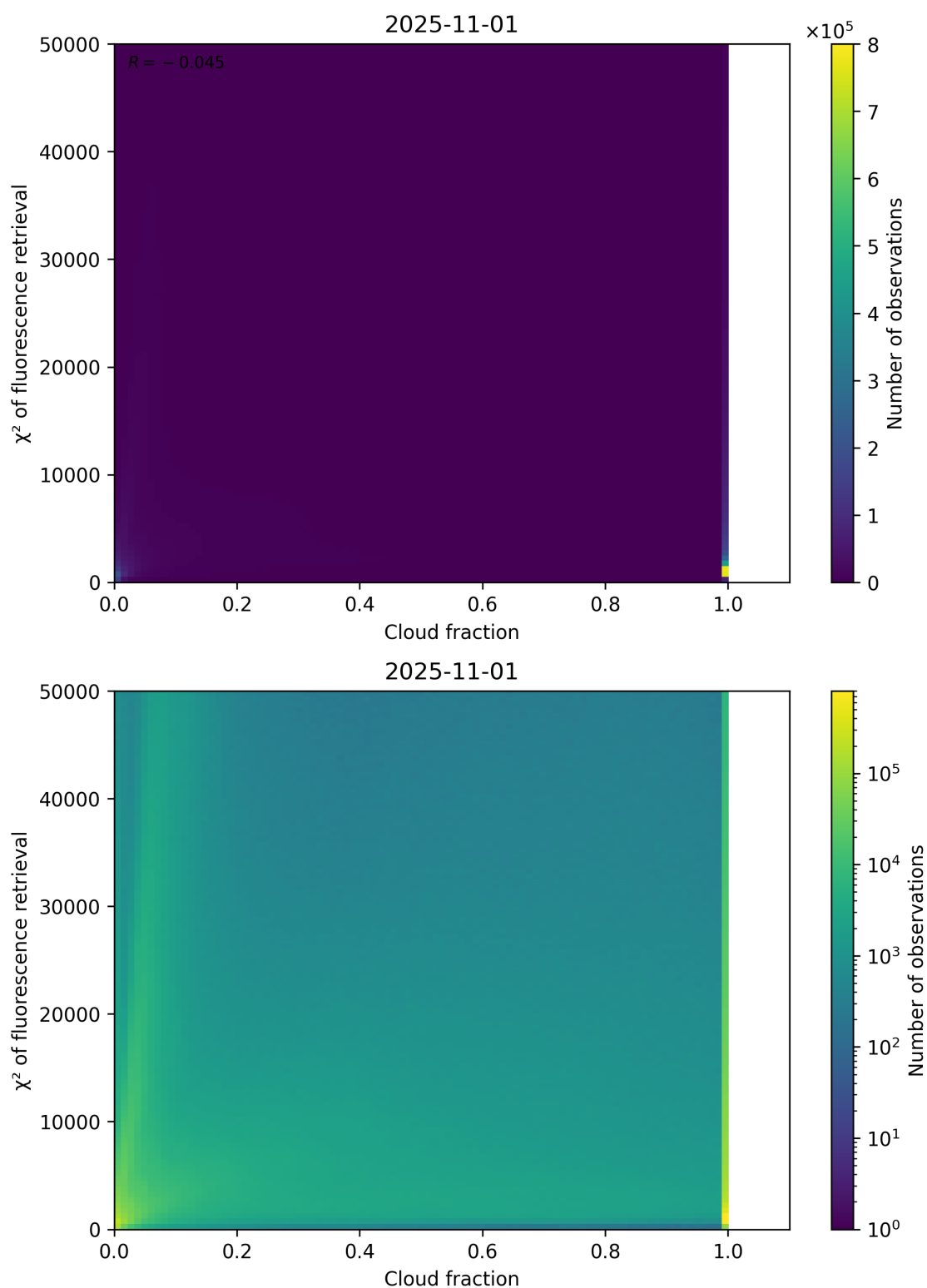
Figure 71: Scatter density plot of “Cloud fraction” against “ \chi^2 of fluorescence retrieval” for 2025-10-31 to 2025-11-02.
