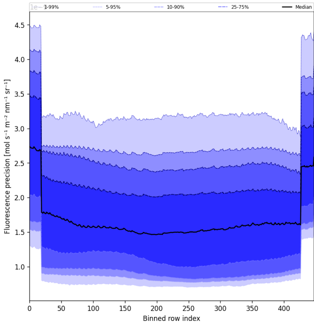
Figure 58: Along track statistics of “Fluorescence precision” for 2025-10-31 to 2025-11-02
