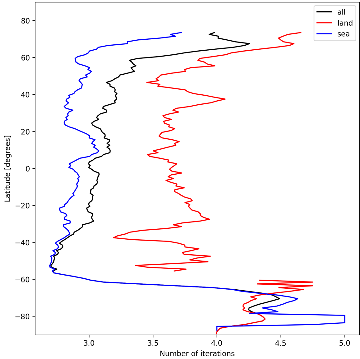
Figure 22: Zonal average of “Number of iterations” for 2025-10-31 to 2025-11-02.
