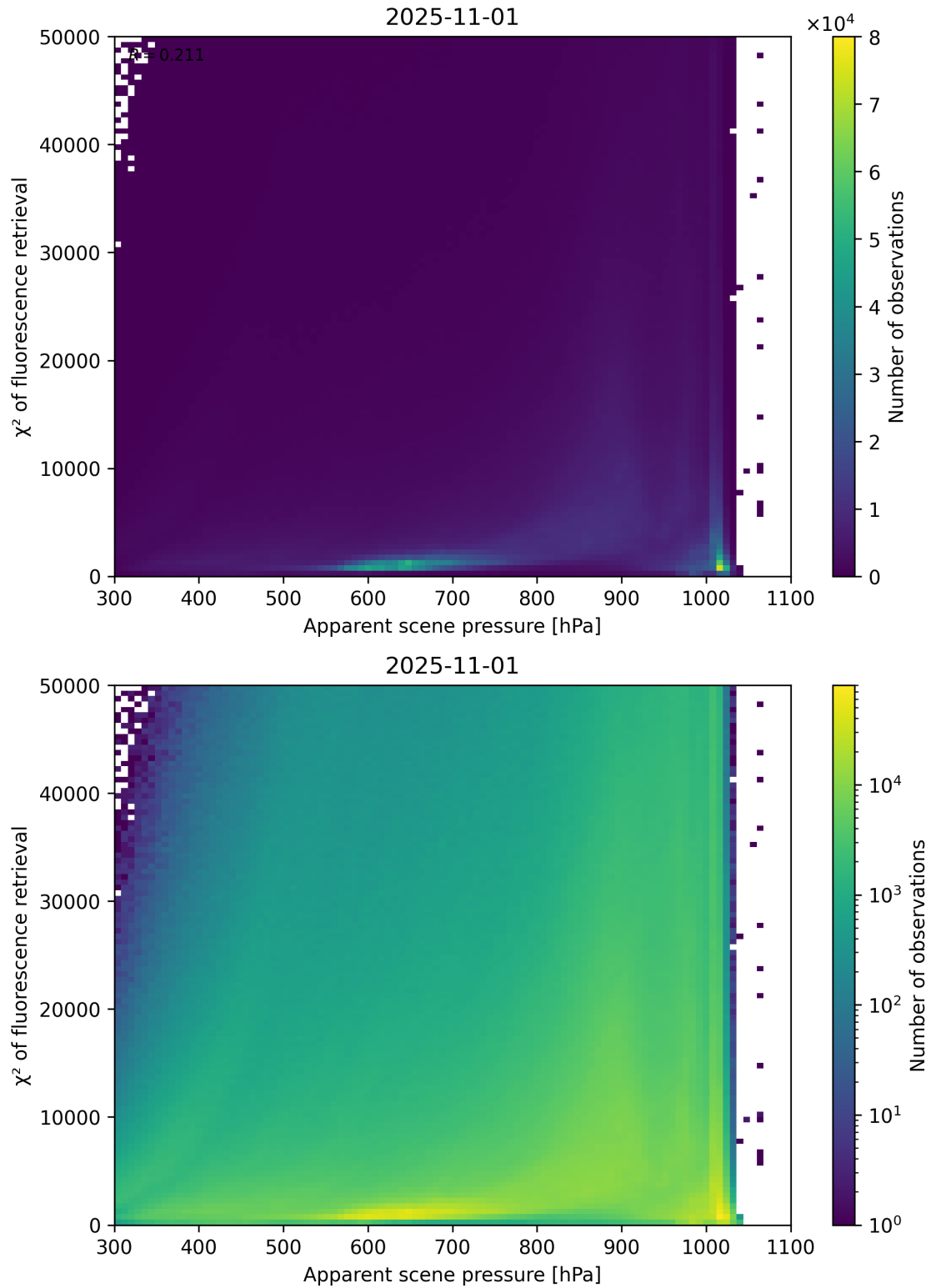
Figure 63: Scatter density plot of “Apparent scene pressure” against “ \chi^2 of fluorescence retrieval” for 2025-10-31 to 2025-11-02.
