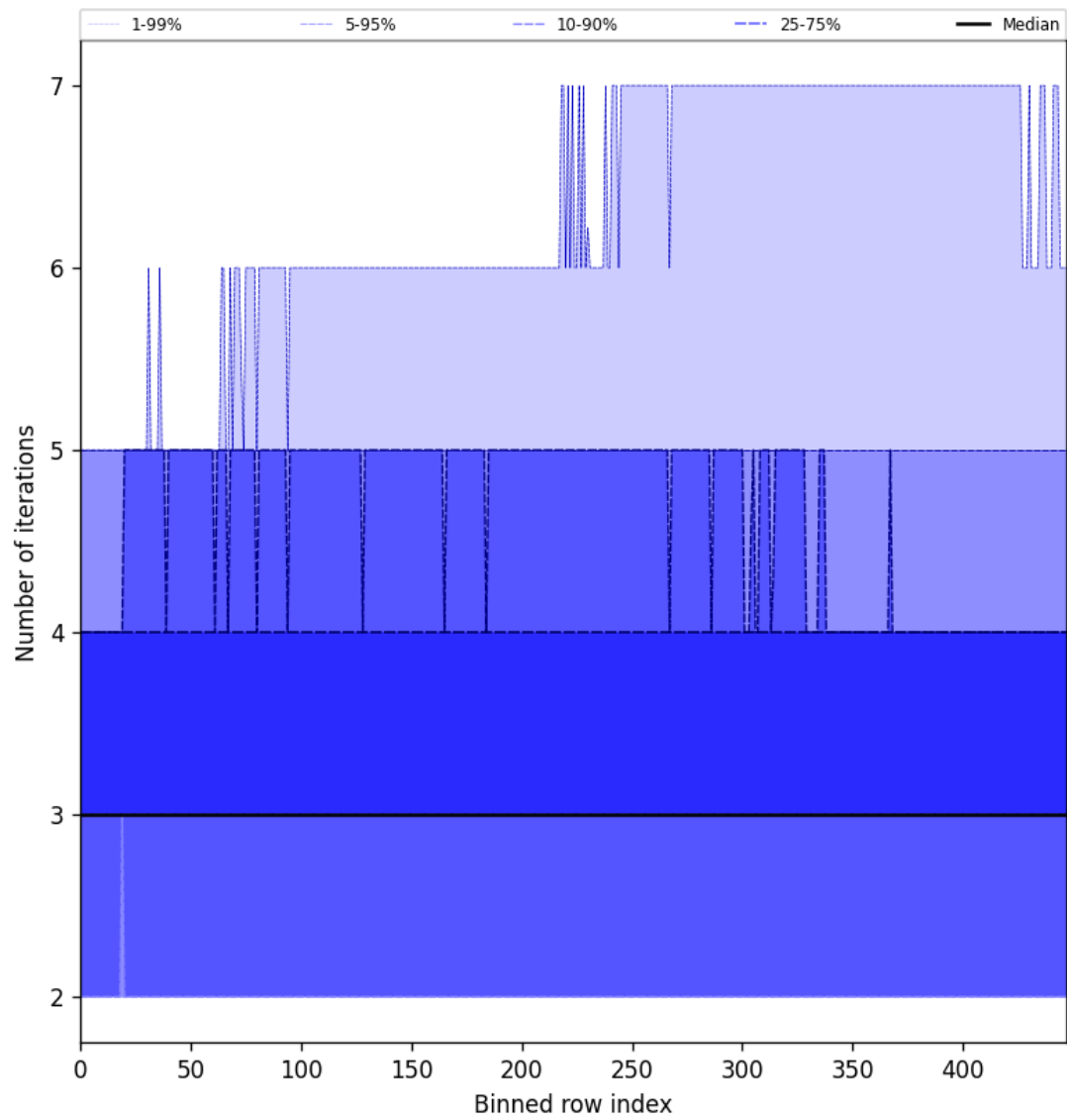
Figure 56: Along track statistics of “Number of iterations” for 2025-10-31 to 2025-11-02
