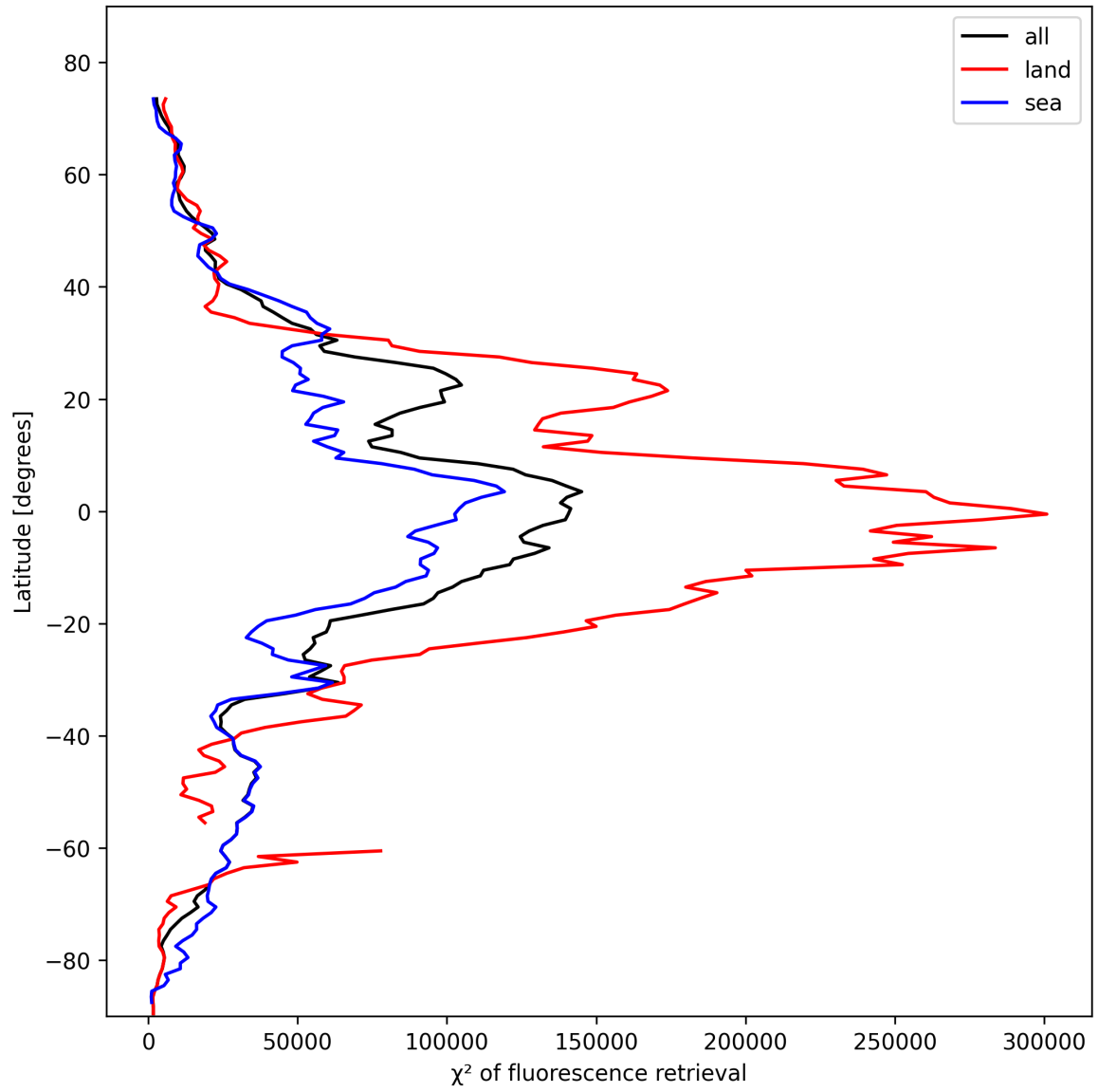
Figure 25: Zonal average of “ \chi^2 of fluorescence retrieval” for 2025-10-31 to 2025-11-02.
