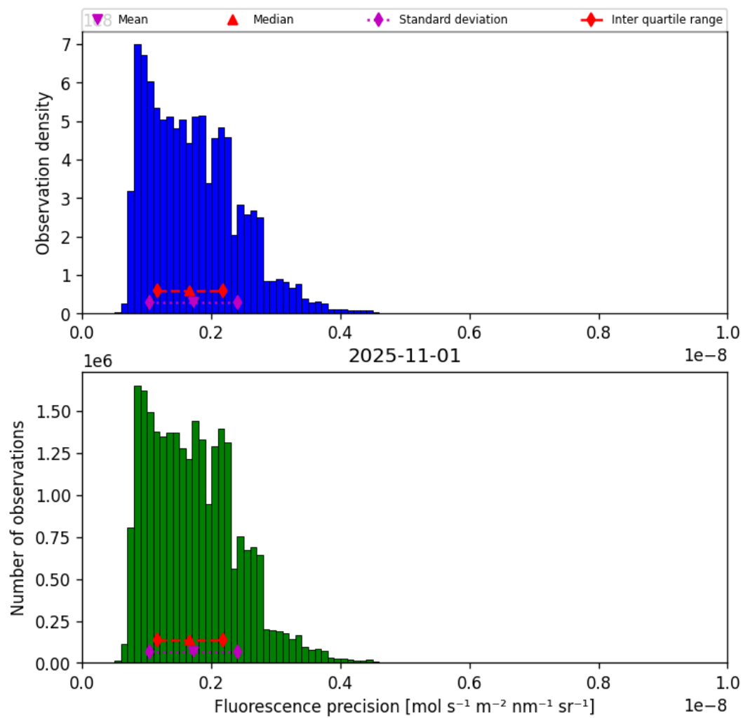
Figure 41: Histogram of “Fluorescence precision” for 2025-10-31 to 2025-11-02
