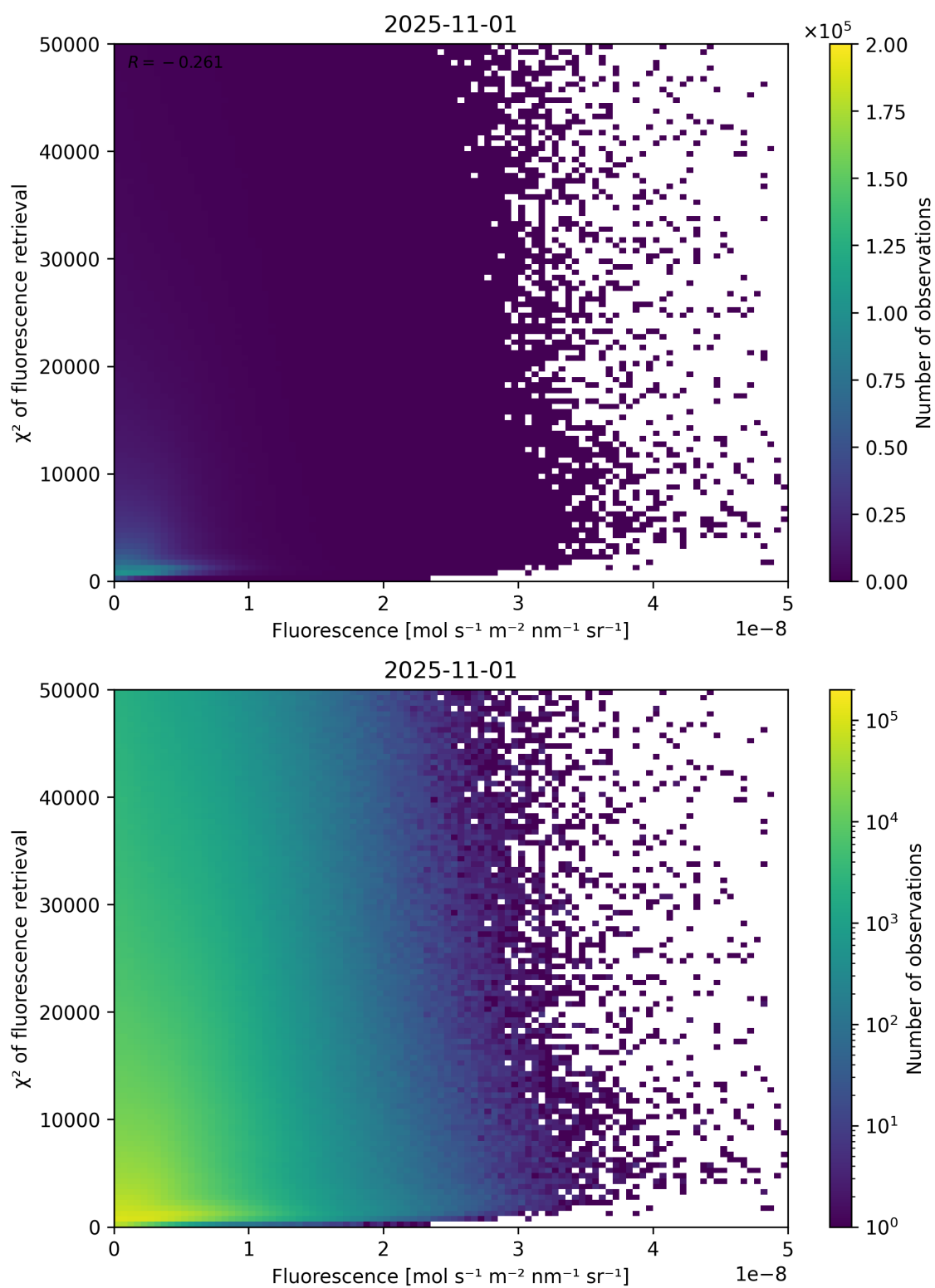
Figure 85: Scatter density plot of “Fluorescence” against “ \chi^2 of fluorescence retrieval” for 2025-10-31 to 2025-11-02.
