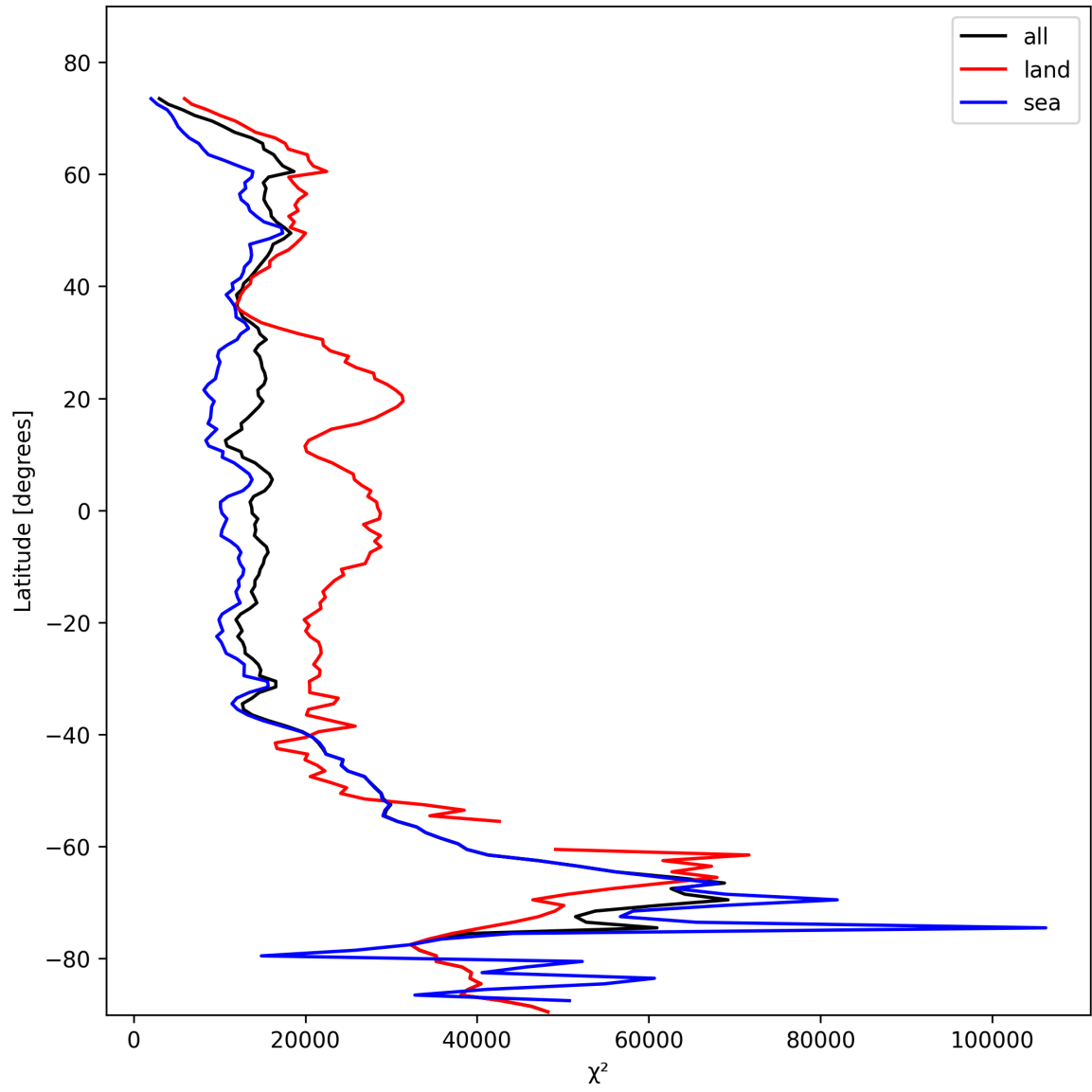
Figure 21: Zonal average of “ \chi^2 ” for 2025-10-31 to 2025-11-02.
