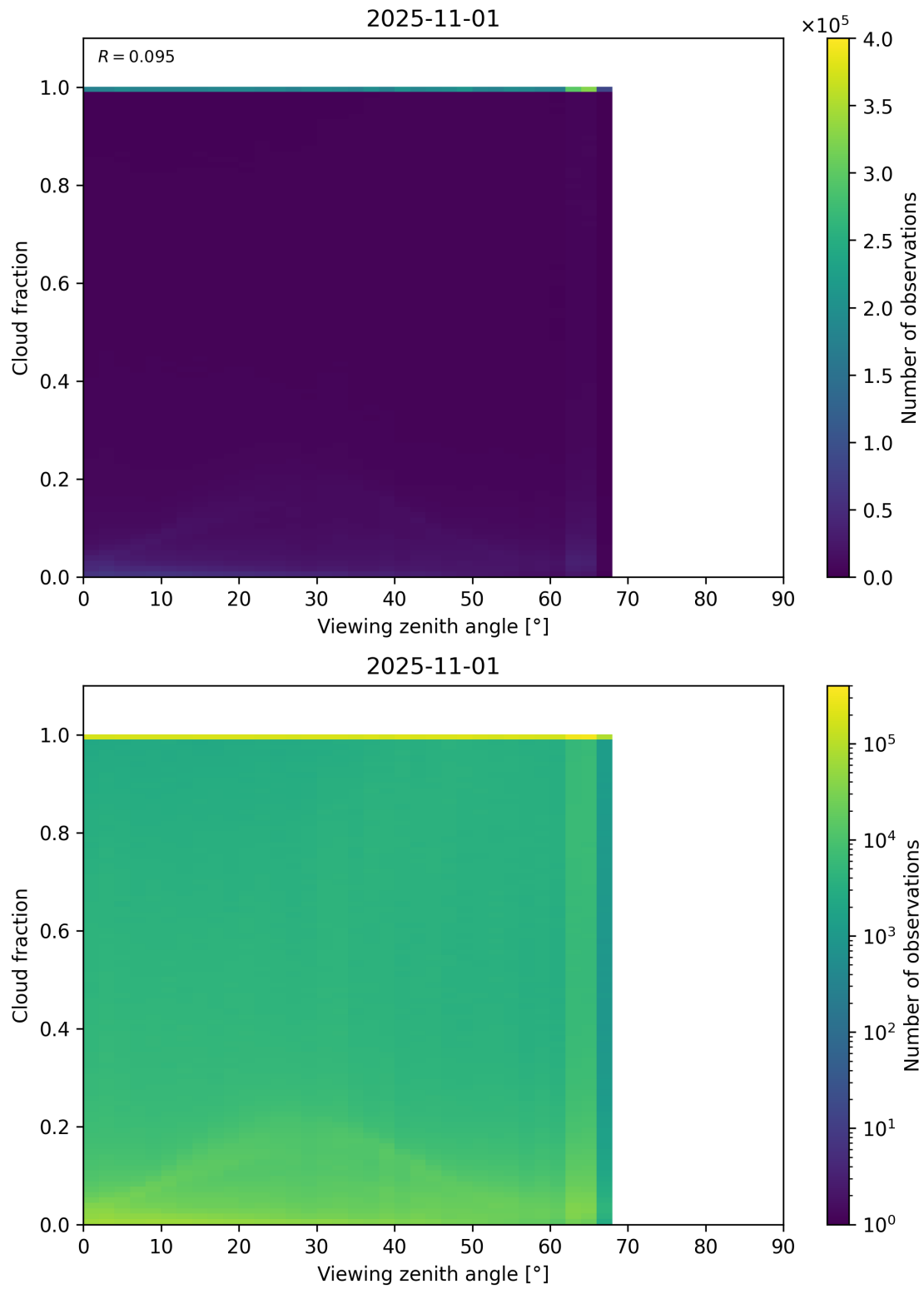
Figure 120: Scatter density plot of “Viewing zenith angle” against “Cloud fraction” for 2025-10-31 to 2025-11-02.
