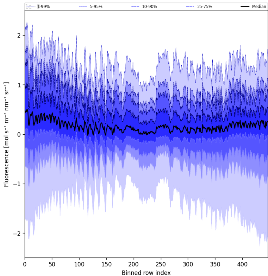
Figure 57: Along track statistics of “Fluorescence” for 2025-10-31 to 2025-11-02
