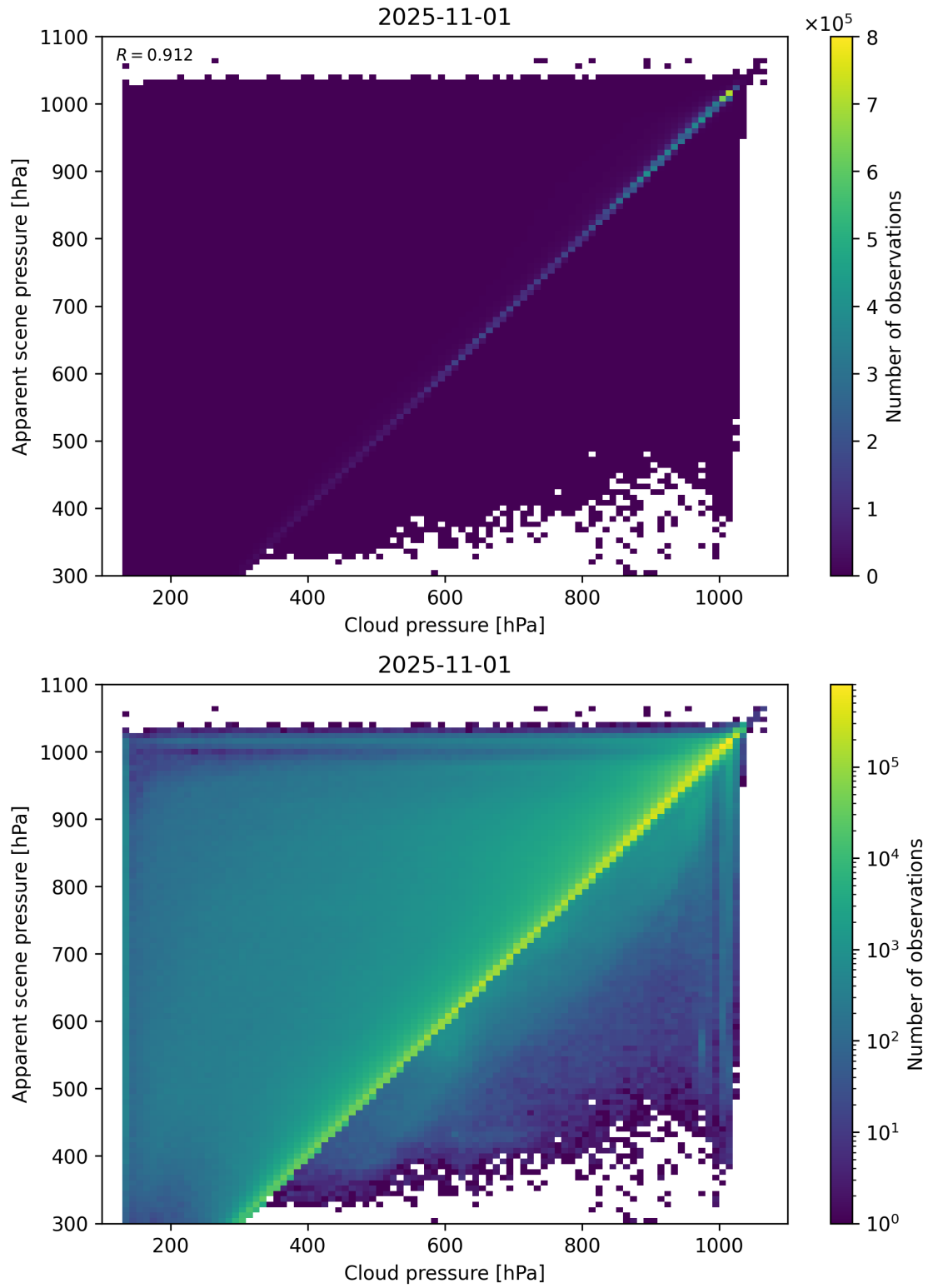
Figure 77: Scatter density plot of “Cloud pressure” against “Apparent scene pressure” for 2025-10-31 to 2025-11-02.
