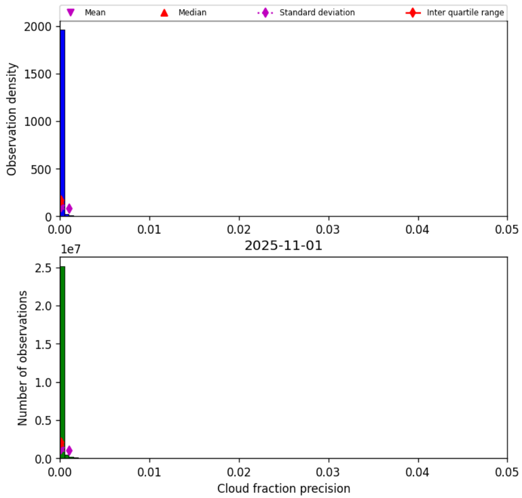
Figure 33: Histogram of “Cloud fraction precision” for 2025-10-31 to 2025-11-02
