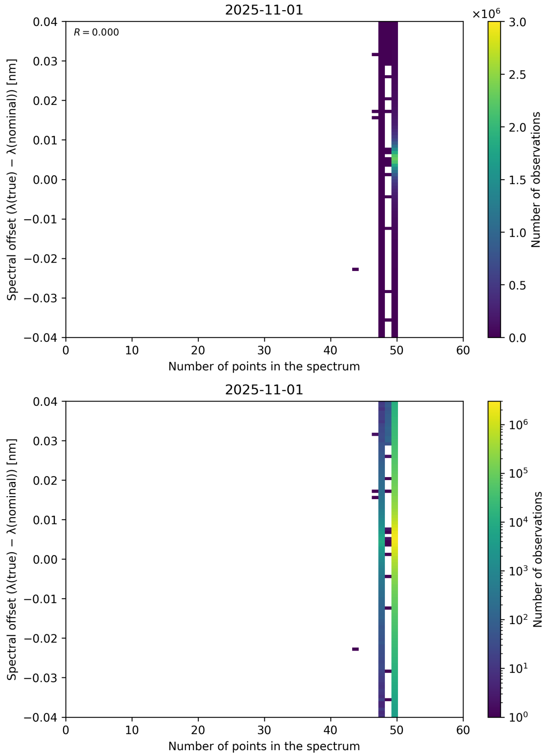
Figure 101: Scatter density plot of “Number of points in the spectrum” against “Spectral offset ( \lambda_{\text{true}} - \lambda_{\text{nominal}} )” for 2025-10-31 to 2025-11-02.
