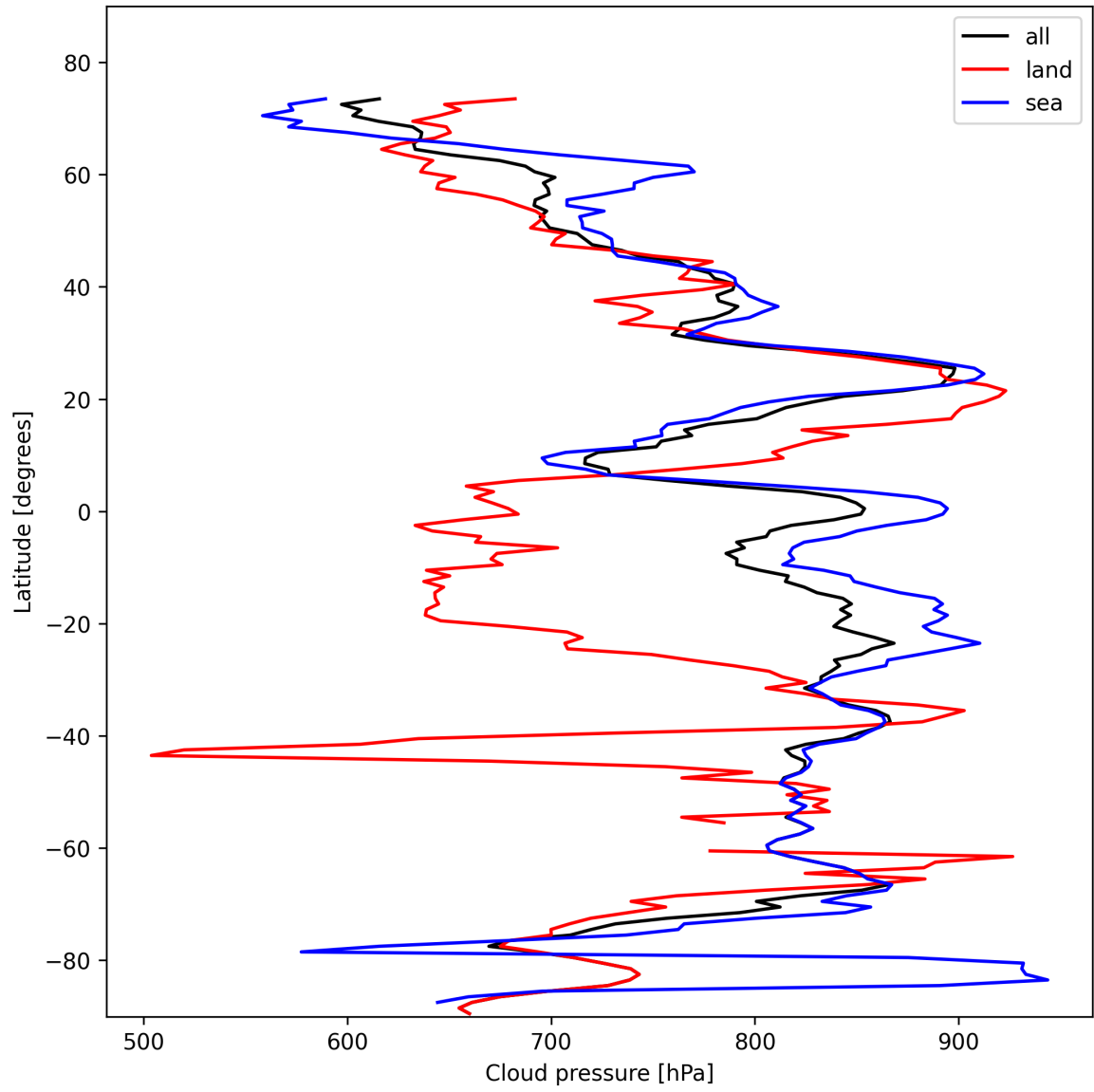
Figure 13: Zonal average of “Cloud pressure” for 2025-10-31 to 2025-11-02.
