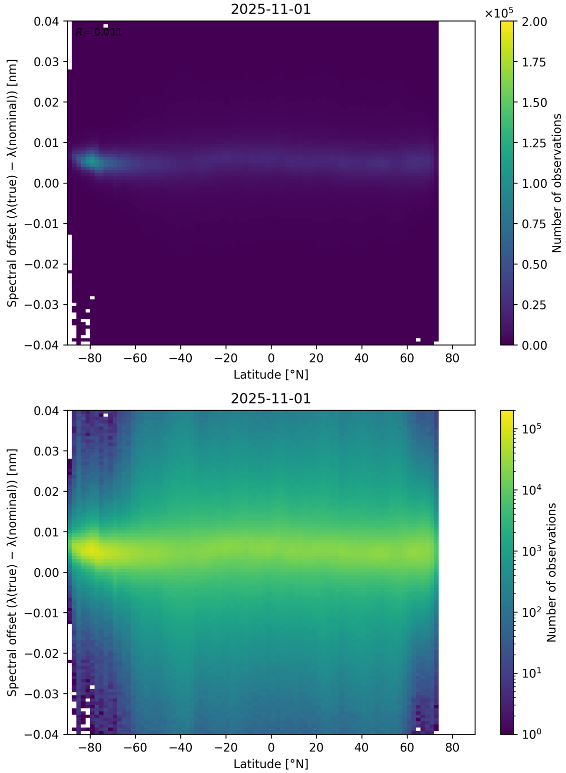
Figure 96: Scatter density plot of “Latitude” against “Spectral offset ( \lambda_{\text{true}} - \lambda_{\text{nominal}} )” for 2025-10-31 to 2025-11-02.
