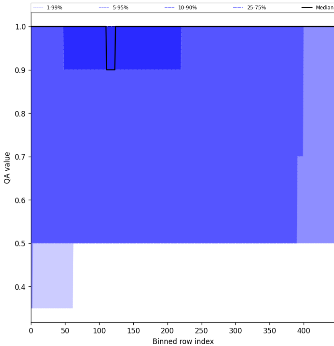
Figure 46: Along track statistics of “QA value” for 2025-10-31 to 2025-11-02
