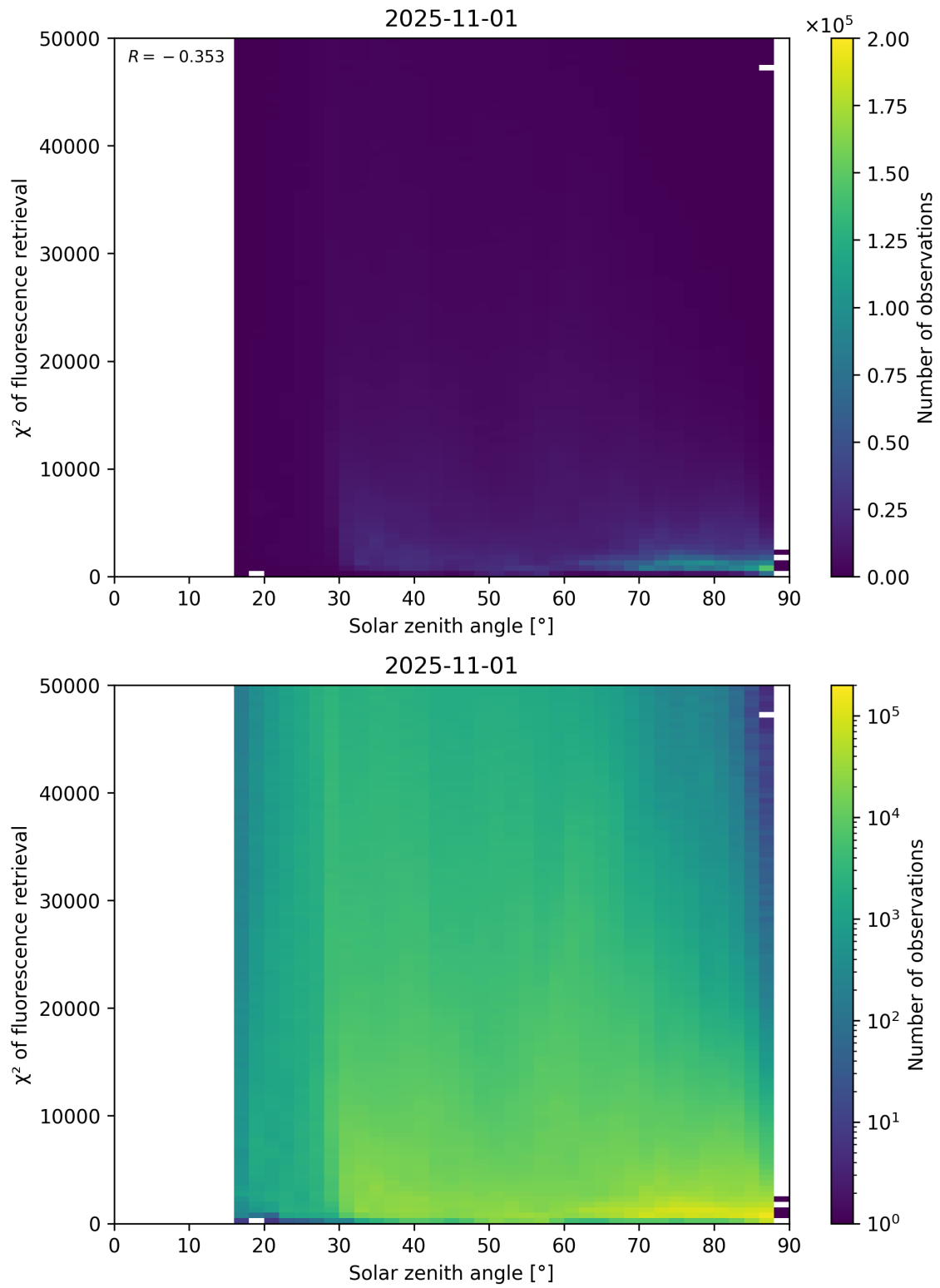
Figure 109: Scatter density plot of “Solar zenith angle” against “ \chi^2 of fluorescence retrieval” for 2025-10-31 to 2025-11-02.
