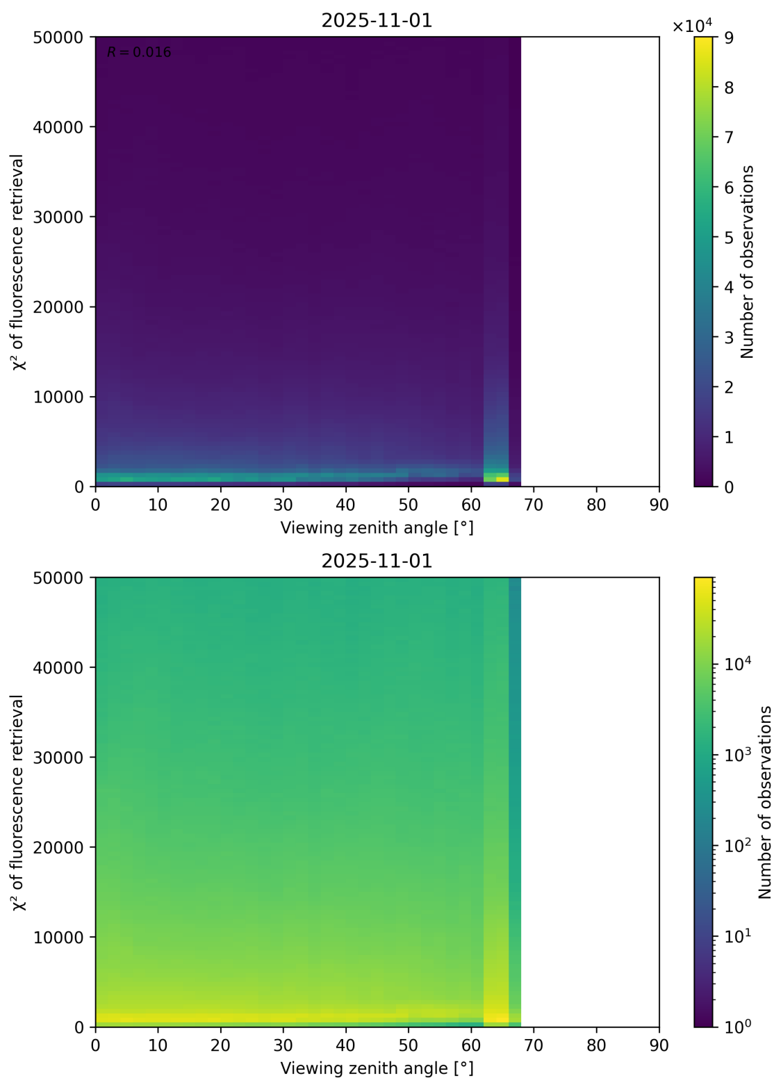
Figure 119: Scatter density plot of “Viewing zenith angle” against “ \chi^2 of fluorescence retrieval” for 2025-10-31 to 2025-11-02.
