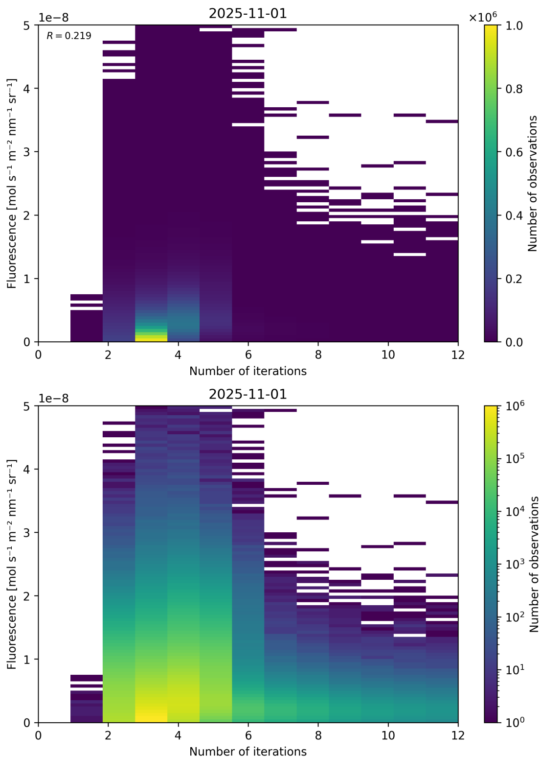
Figure 98: Scatter density plot of “Number of iterations” against “Fluorescence” for 2025-10-31 to 2025-11-02.
