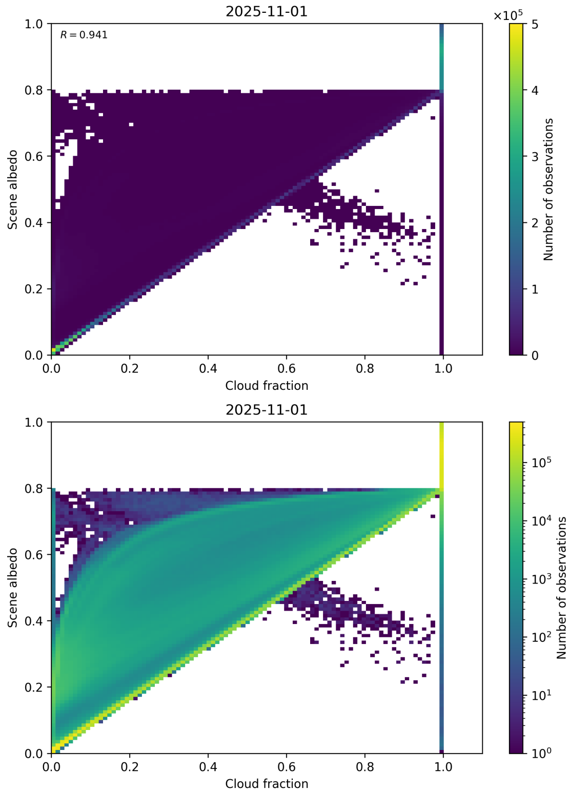
Figure 75: Scatter density plot of “Cloud fraction” against “Scene albedo” for 2025-10-31 to 2025-11-02.
