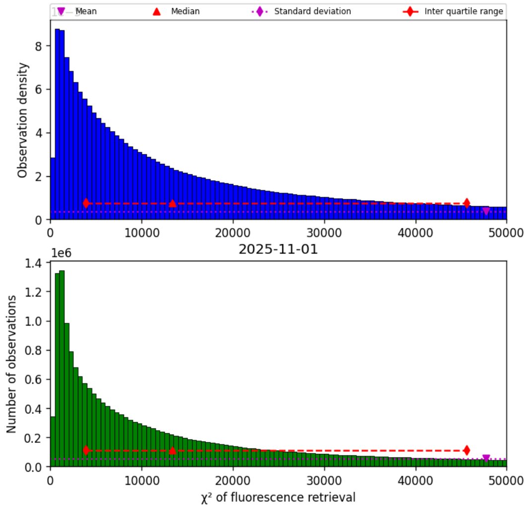
Figure 42: Histogram of “ \chi^2 of fluorescence retrieval” for 2025-10-31 to 2025-11-02
