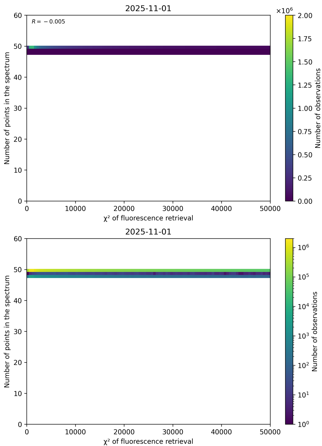
Figure 68: Scatter density plot of “ \chi^2 of fluorescence retrieval” against “Number of points in the spectrum” for 2025-10-31 to 2025-11-02.
