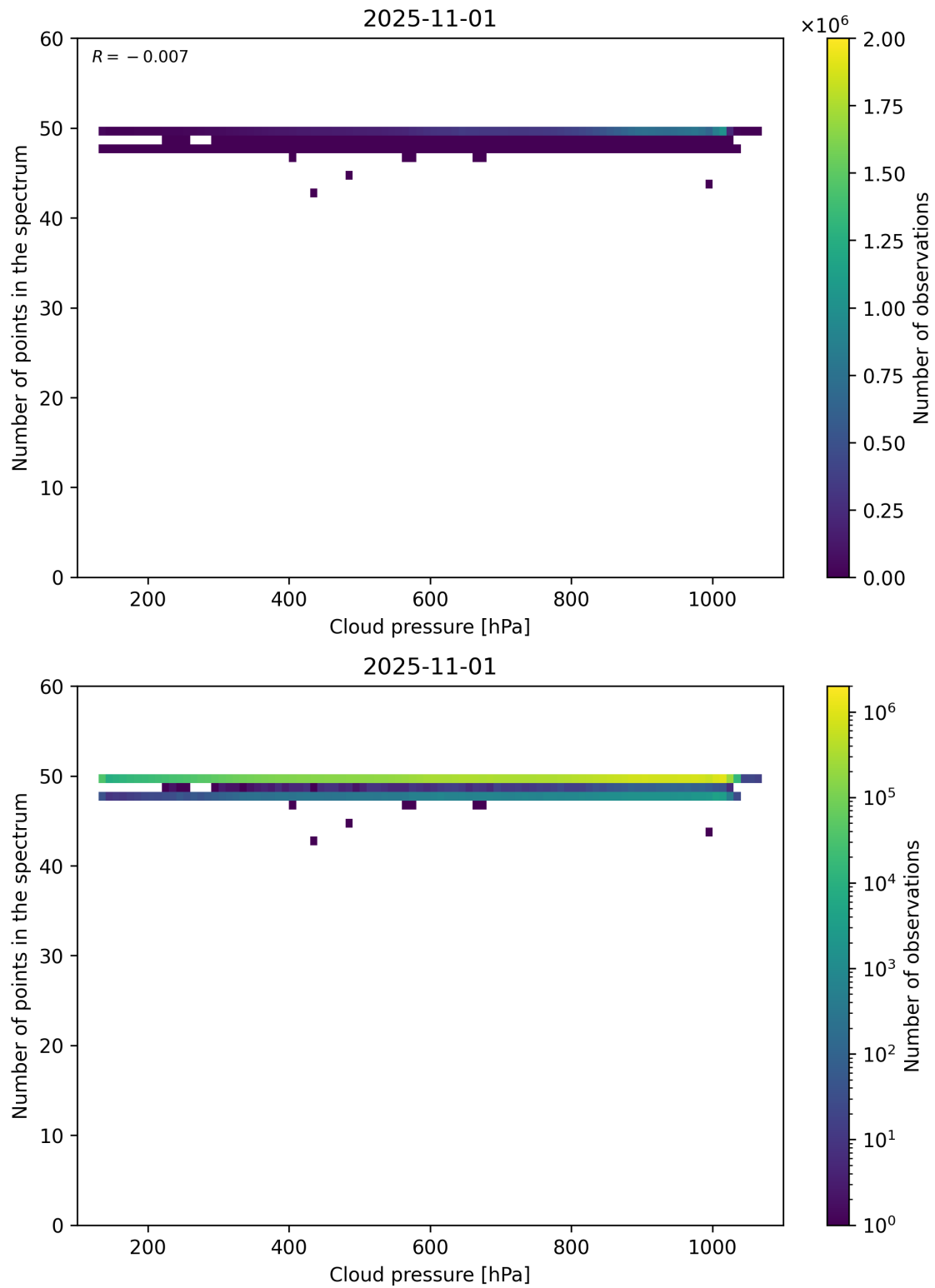
Figure 82: Scatter density plot of “Cloud pressure” against “Number of points in the spectrum” for 2025-10-31 to 2025-11-02.
