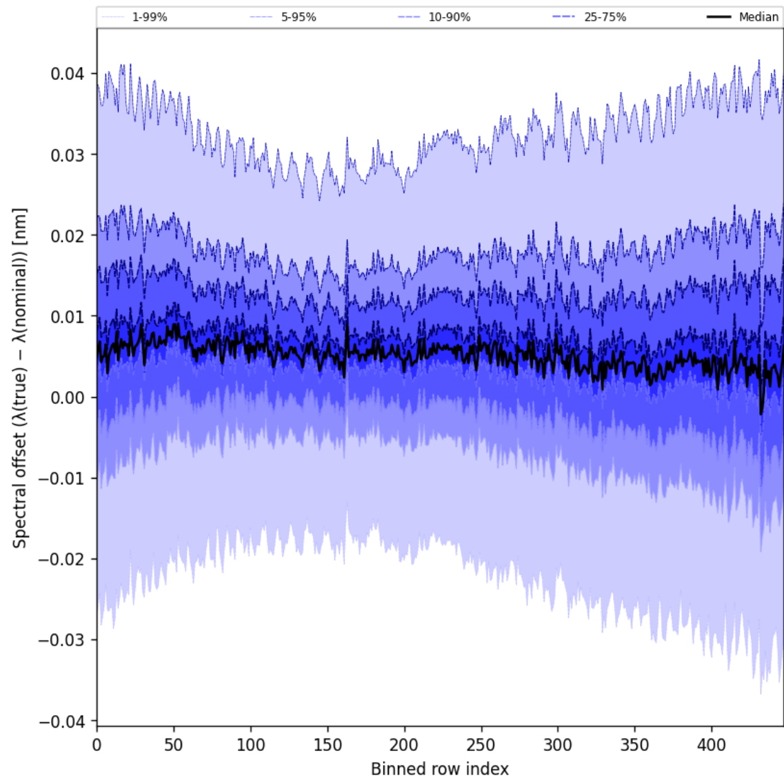
Figure 62: Along track statistics of “Spectral offset ( \lambda_{\text{true}} - \lambda_{\text{nominal}} )” for 2025-10-31 to 2025-11-02
