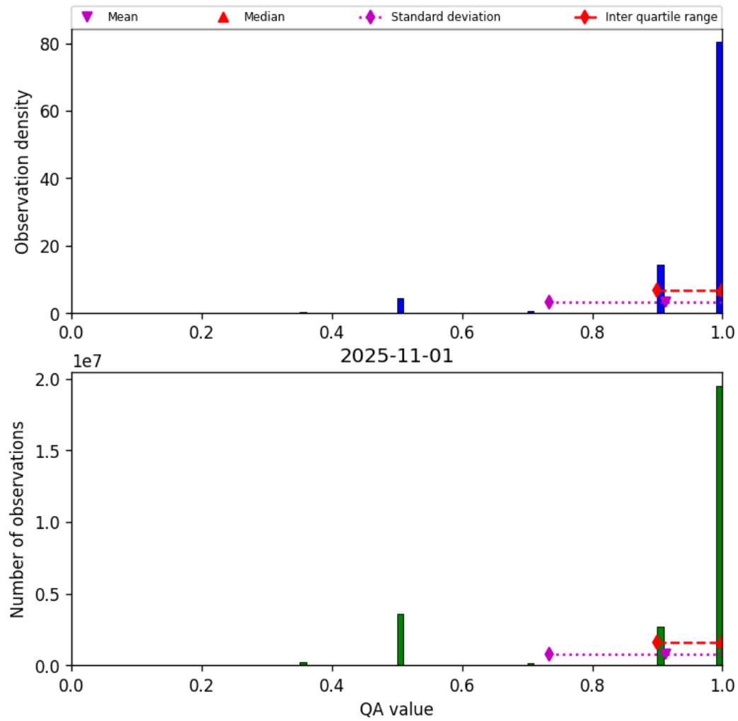
Figure 29: Histogram of “QA value” for 2025-10-31 to 2025-11-02
