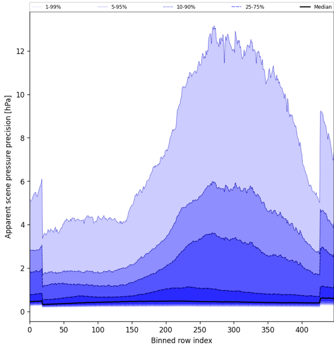
Figure 54: Along track statistics of “Apparent scene pressure precision” for 2025-10-31 to 2025-11-02
