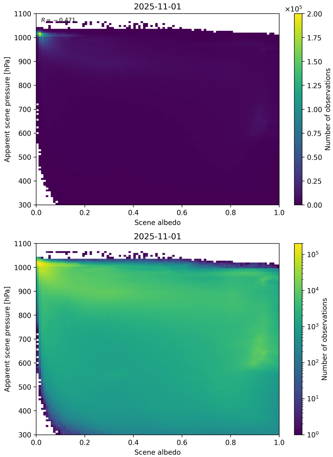
Figure 102: Scatter density plot of “Scene albedo” against “Apparent scene pressure” for 2025-10-31 to 2025-11-02.
