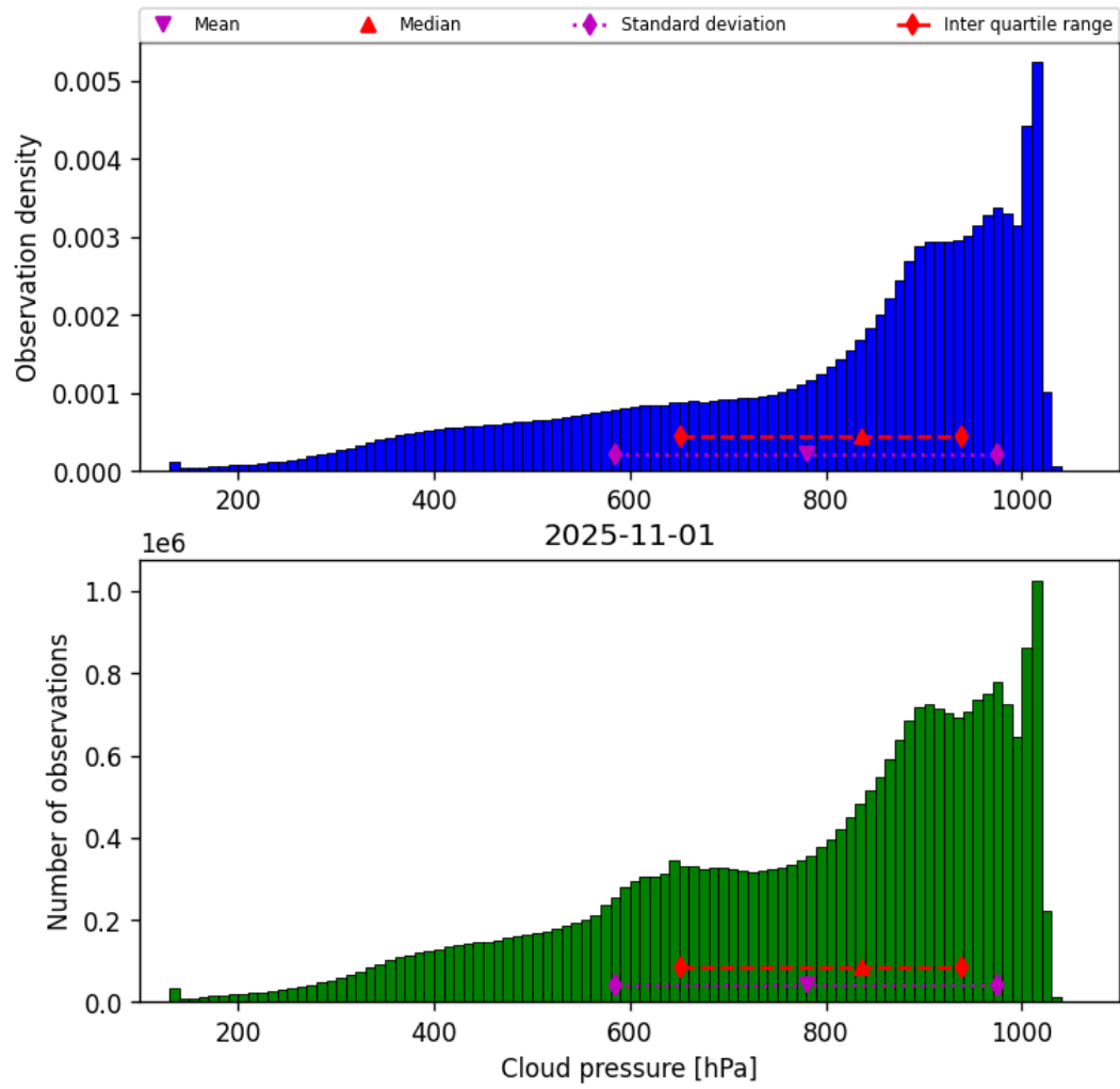
Figure 30: Histogram of “Cloud pressure” for 2025-10-31 to 2025-11-02
