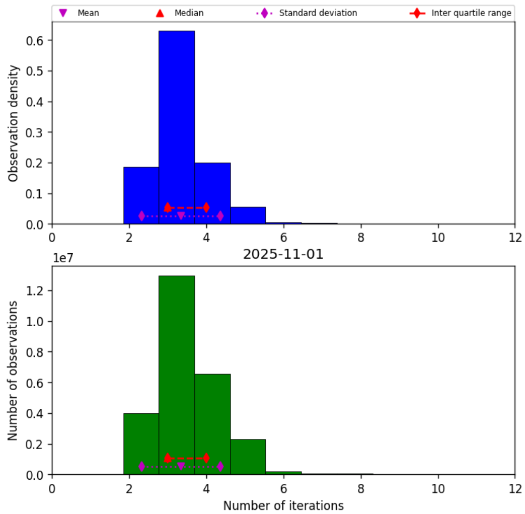
Figure 39: Histogram of “Number of iterations” for 2025-10-31 to 2025-11-02
