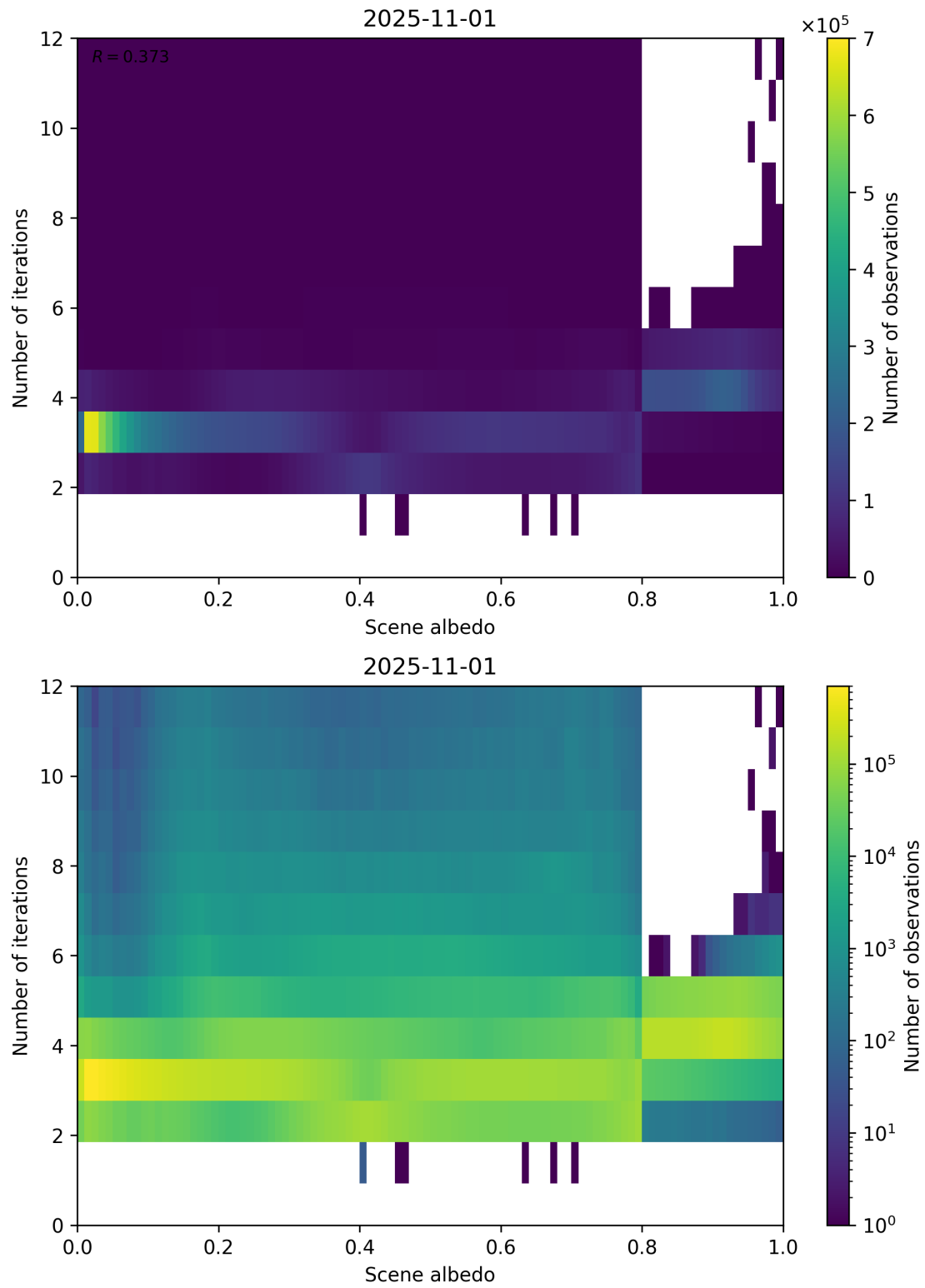
Figure 105: Scatter density plot of “Scene albedo” against “Number of iterations” for 2025-10-31 to 2025-11-02.
