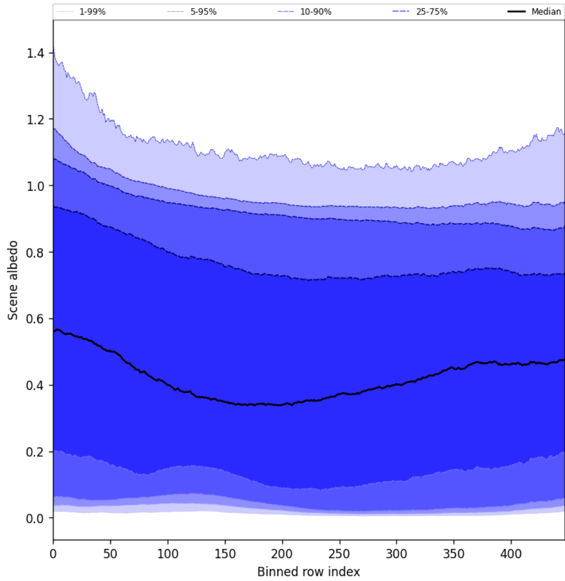
Figure 51: Along track statistics of “Scene albedo” for 2025-10-31 to 2025-11-02
