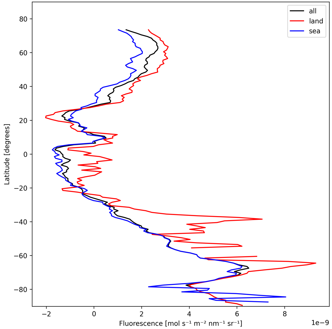
Figure 23: Zonal average of “Fluorescence” for 2025-10-31 to 2025-11-02.
