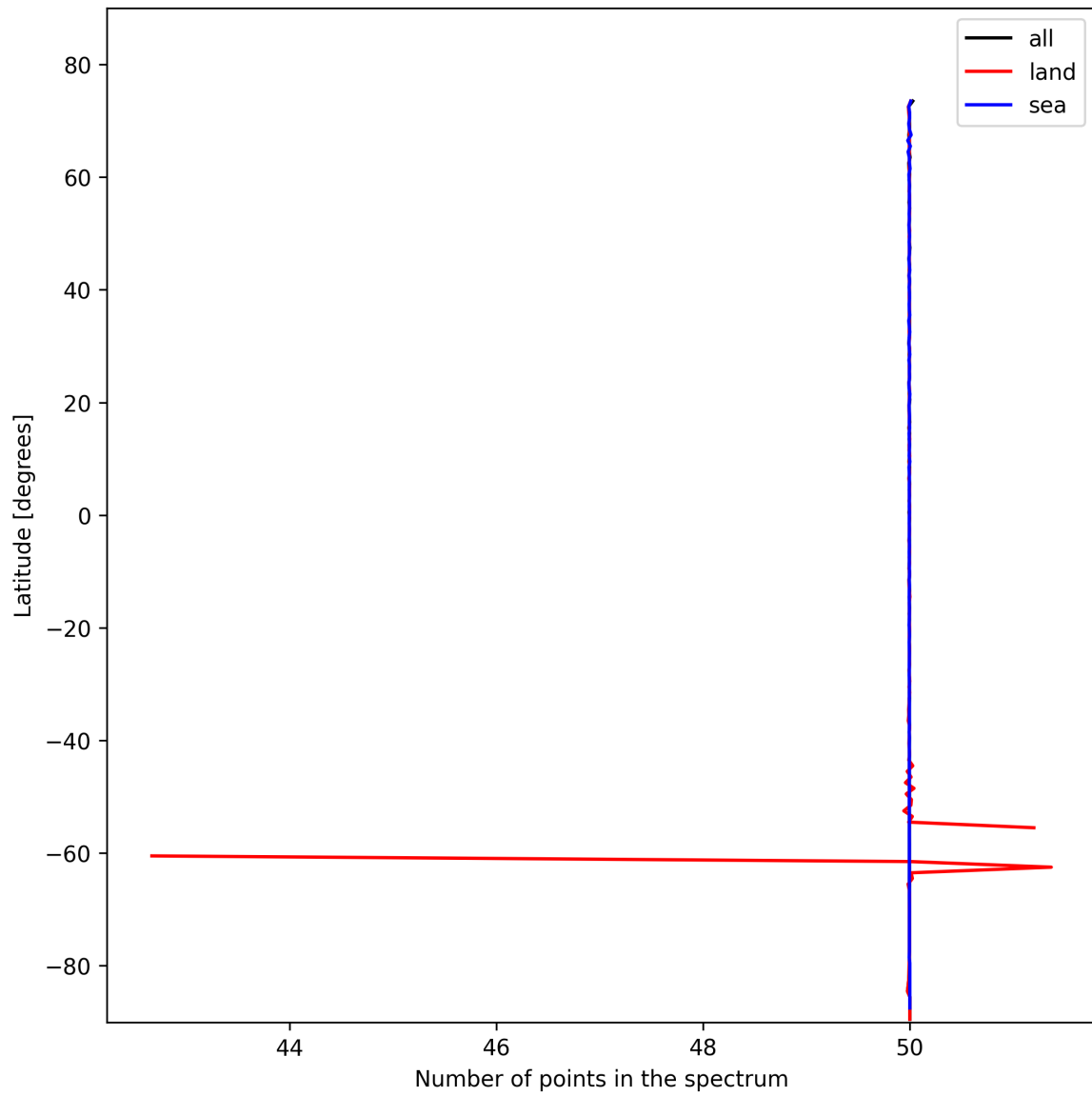
Figure 27: Zonal average of “Number of points in the spectrum” for 2025-10-31 to 2025-11-02.
