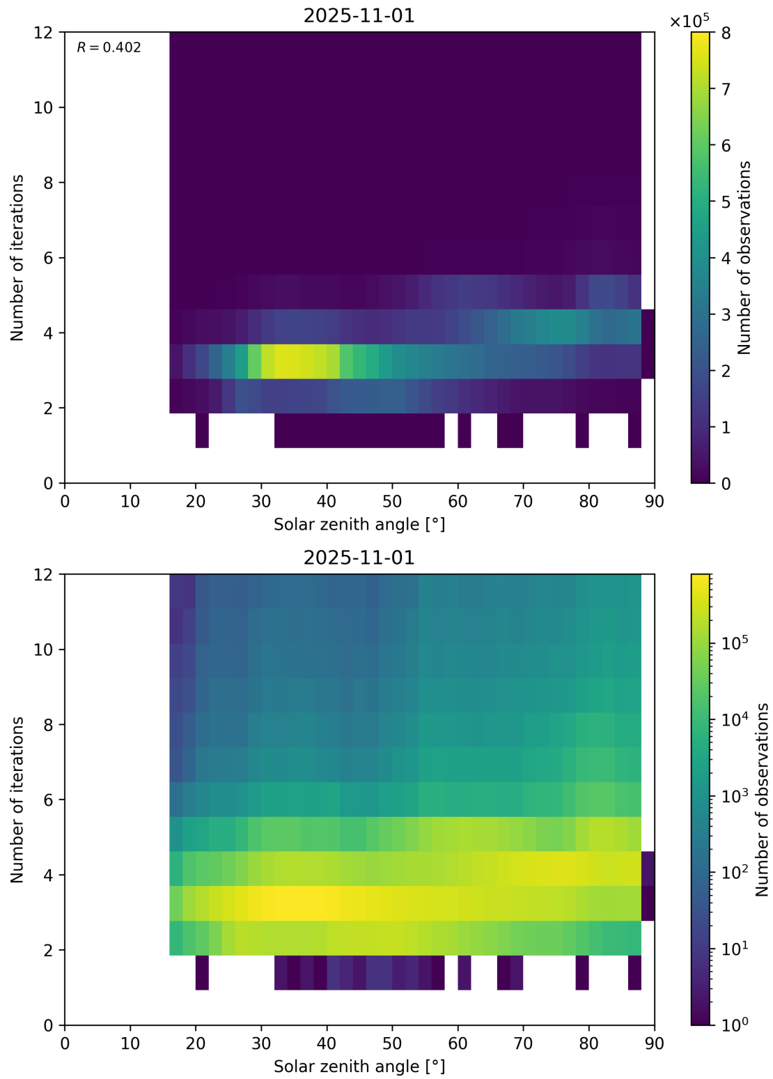
Figure 114: Scatter density plot of “Solar zenith angle” against “Number of iterations” for 2025-10-31 to 2025-11-02.
