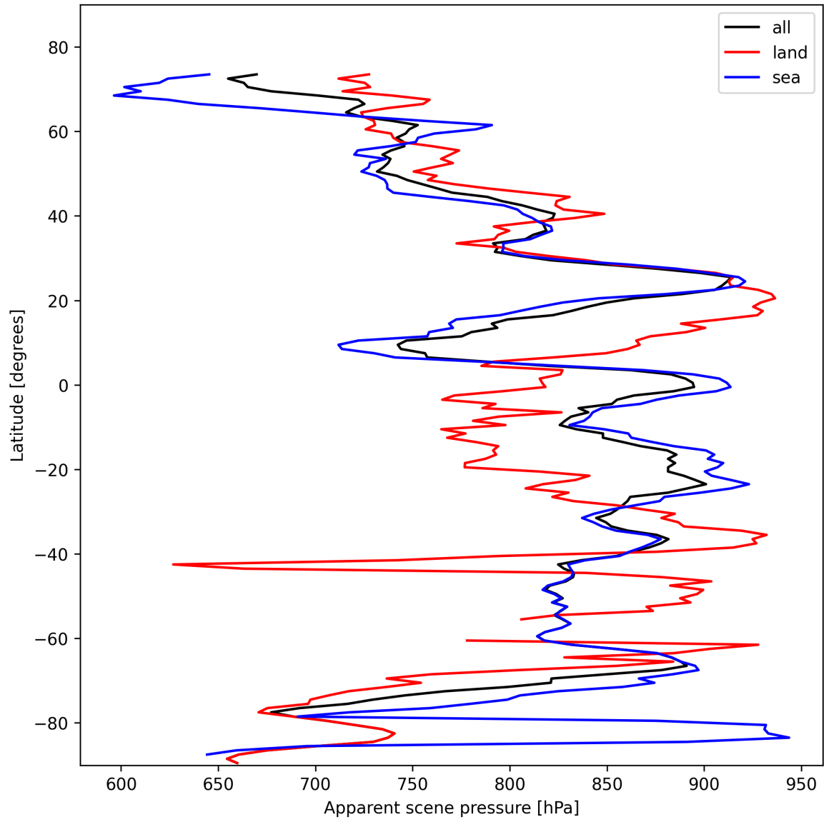
Figure 19: Zonal average of “Apparent scene pressure” for 2025-10-31 to 2025-11-02.
