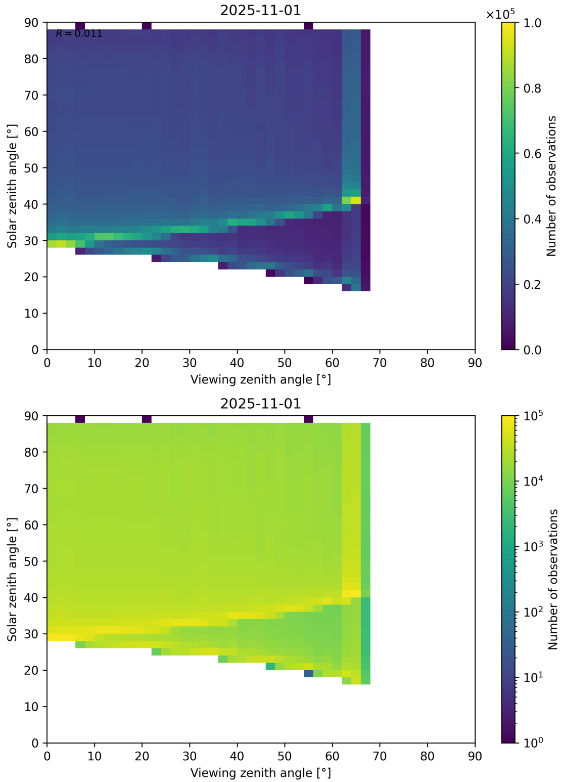
Figure 127: Scatter density plot of “Viewing zenith angle” against “Solar zenith angle” for 2025-10-31 to 2025-11-02.
