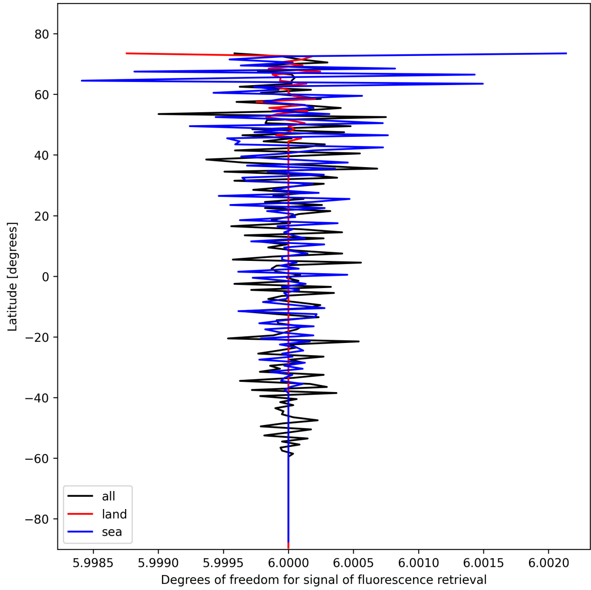
Figure 26: Zonal average of “Degrees of freedom for signal of fluorescence retrieval” for 2025-10-31 to 2025-11-02.
