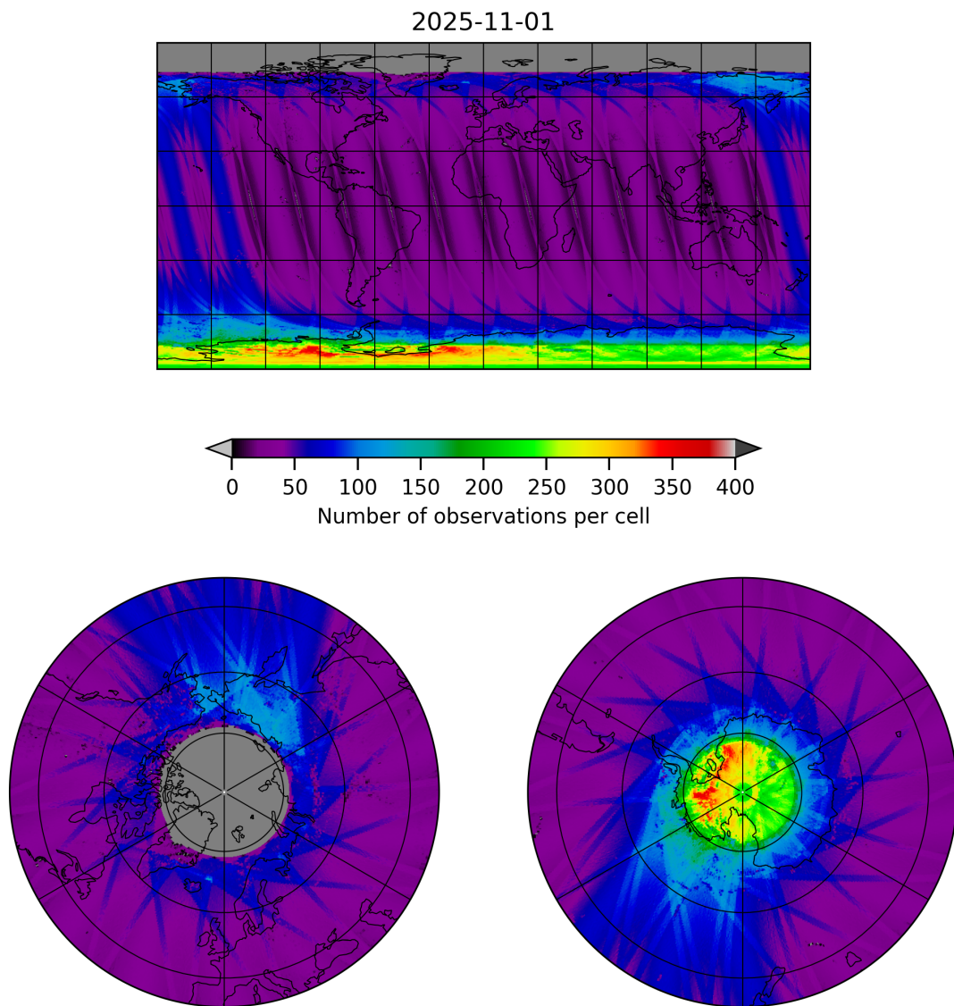
Figure 11: Map of the number of observations for 2025-10-31 to 2025-11-02
