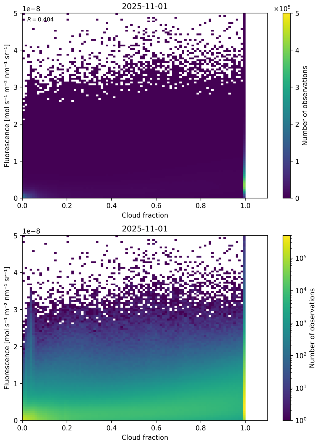
Figure 72: Scatter density plot of “Cloud fraction” against “Fluorescence” for 2025-10-31 to 2025-11-02.
