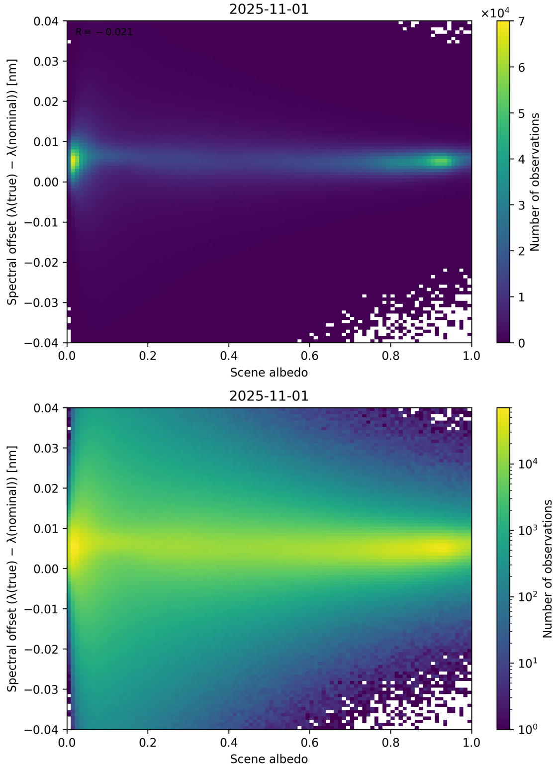
Figure 107: Scatter density plot of “Scene albedo” against “Spectral offset ( \lambda_{\text{true}} - \lambda_{\text{nominal}} )” for 2025-10-31 to 2025-11-02.
