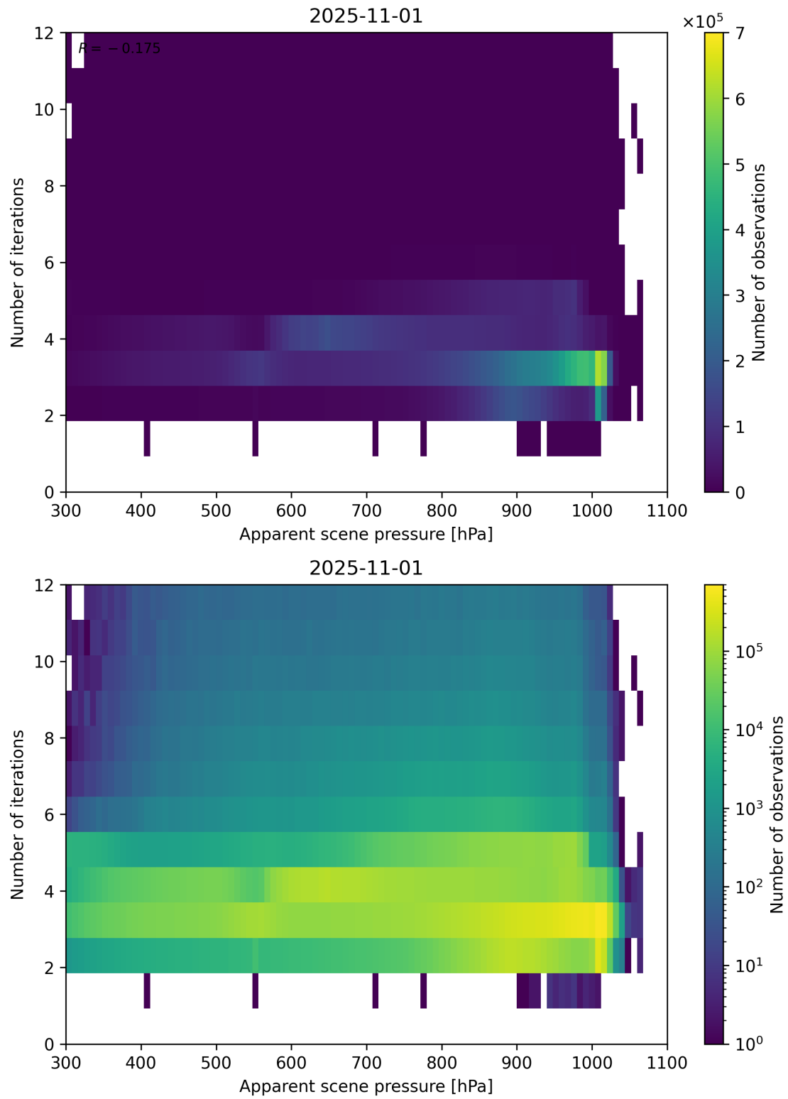
Figure 65: Scatter density plot of “Apparent scene pressure” against “Number of iterations” for 2025-10-31 to 2025-11-02.
