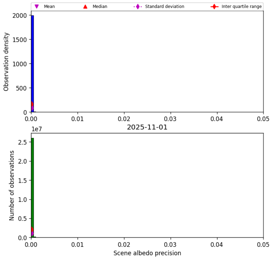
Figure 35: Histogram of “Scene albedo precision” for 2025-10-31 to 2025-11-02
