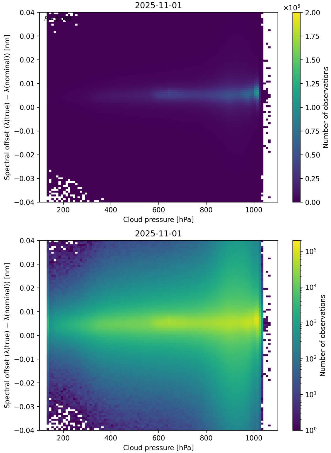
Figure 84: Scatter density plot of “Cloud pressure” against “Spectral offset ( \lambda_{\text{true}} - \lambda_{\text{nominal}} )” for 2025-10-31 to 2025-11-02.
