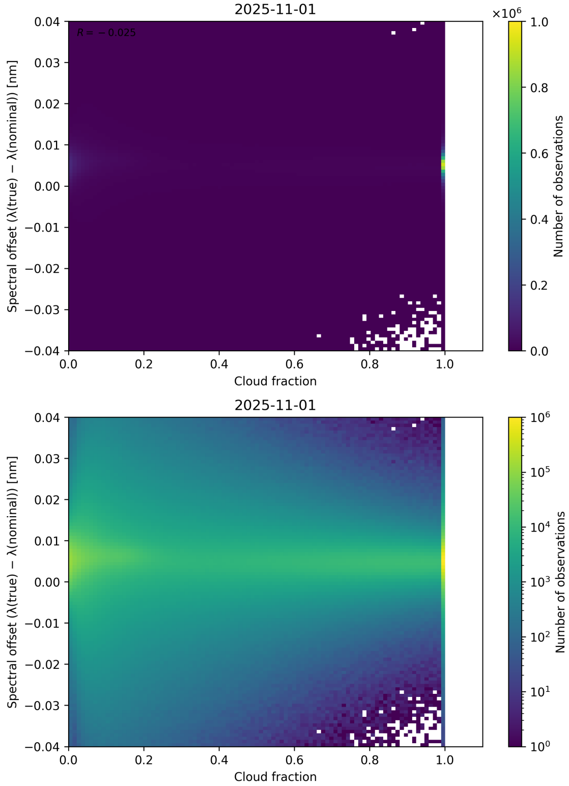
Figure 76: Scatter density plot of “Cloud fraction” against “Spectral offset ( \lambda_{\text{true}} - \lambda_{\text{nominal}} )” for 2025-10-31 to 2025-11-02.
