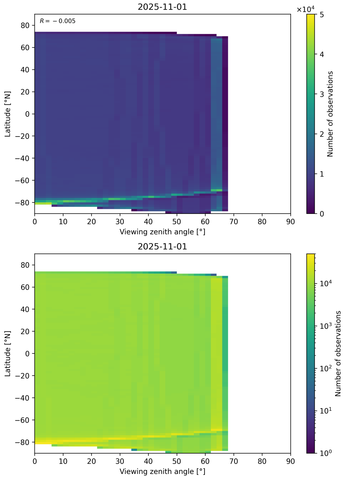
Figure 123: Scatter density plot of “Viewing zenith angle” against “Latitude” for 2025-10-31 to 2025-11-02.
