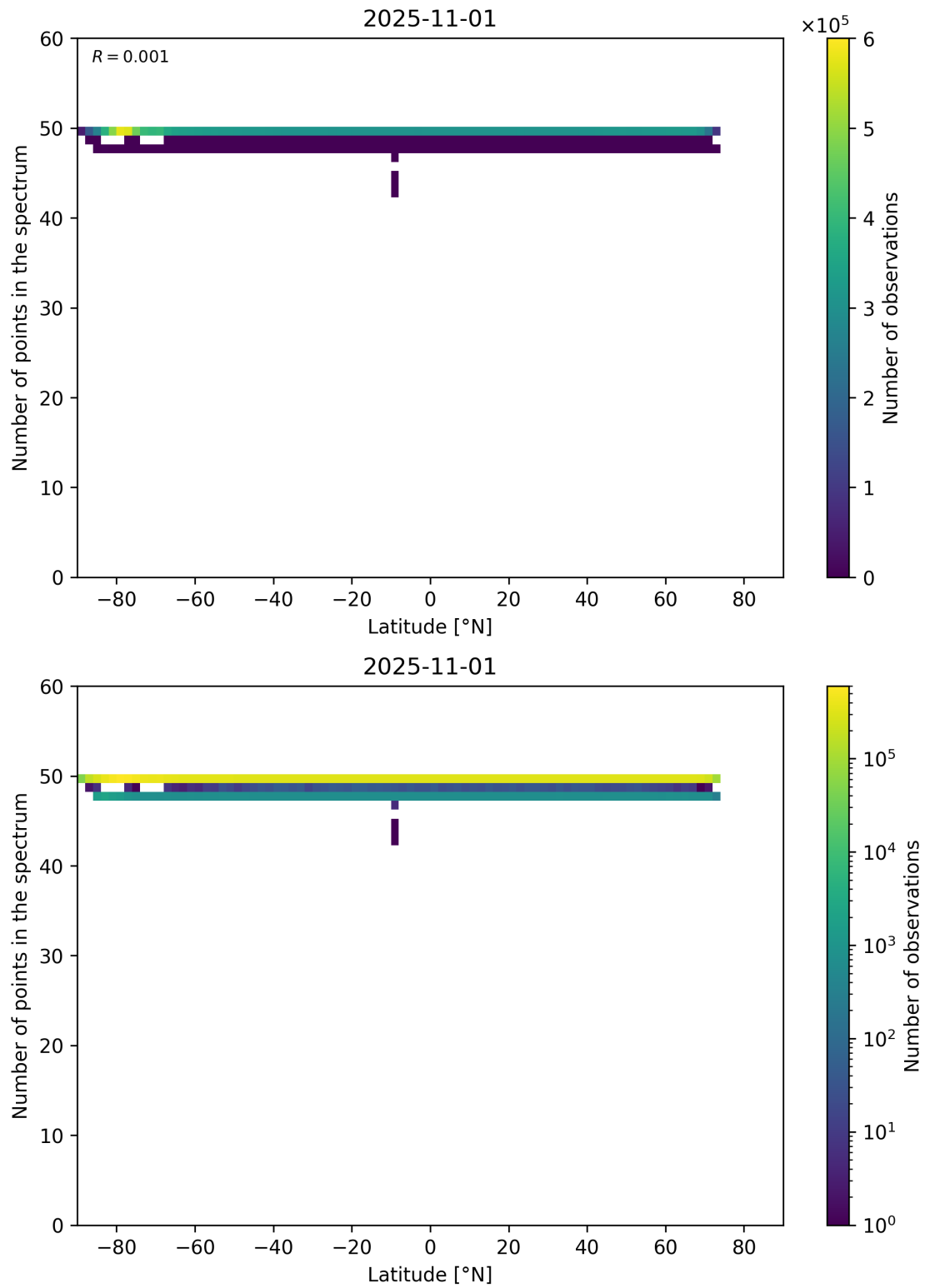
Figure 94: Scatter density plot of “Latitude” against “Number of points in the spectrum” for 2025-10-31 to 2025-11-02.
