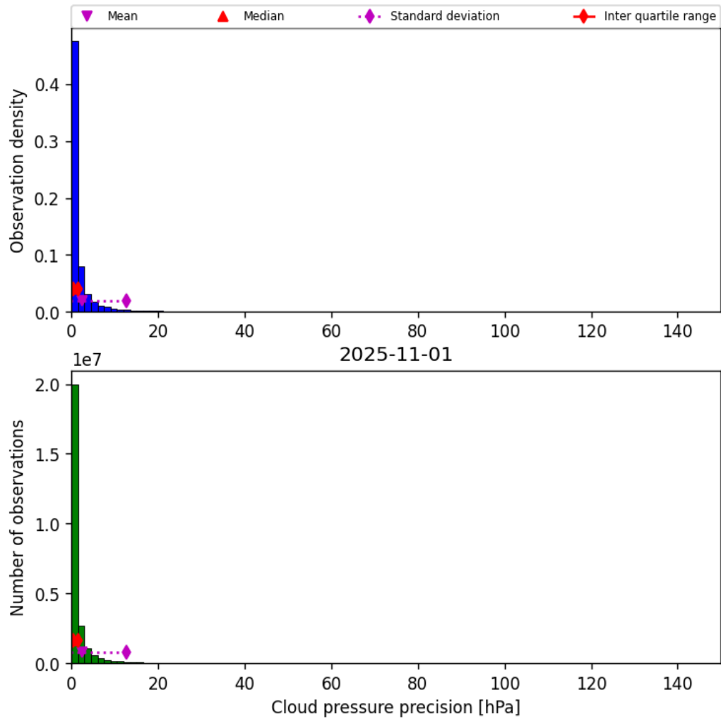
Figure 31: Histogram of “Cloud pressure precision” for 2025-10-31 to 2025-11-02
