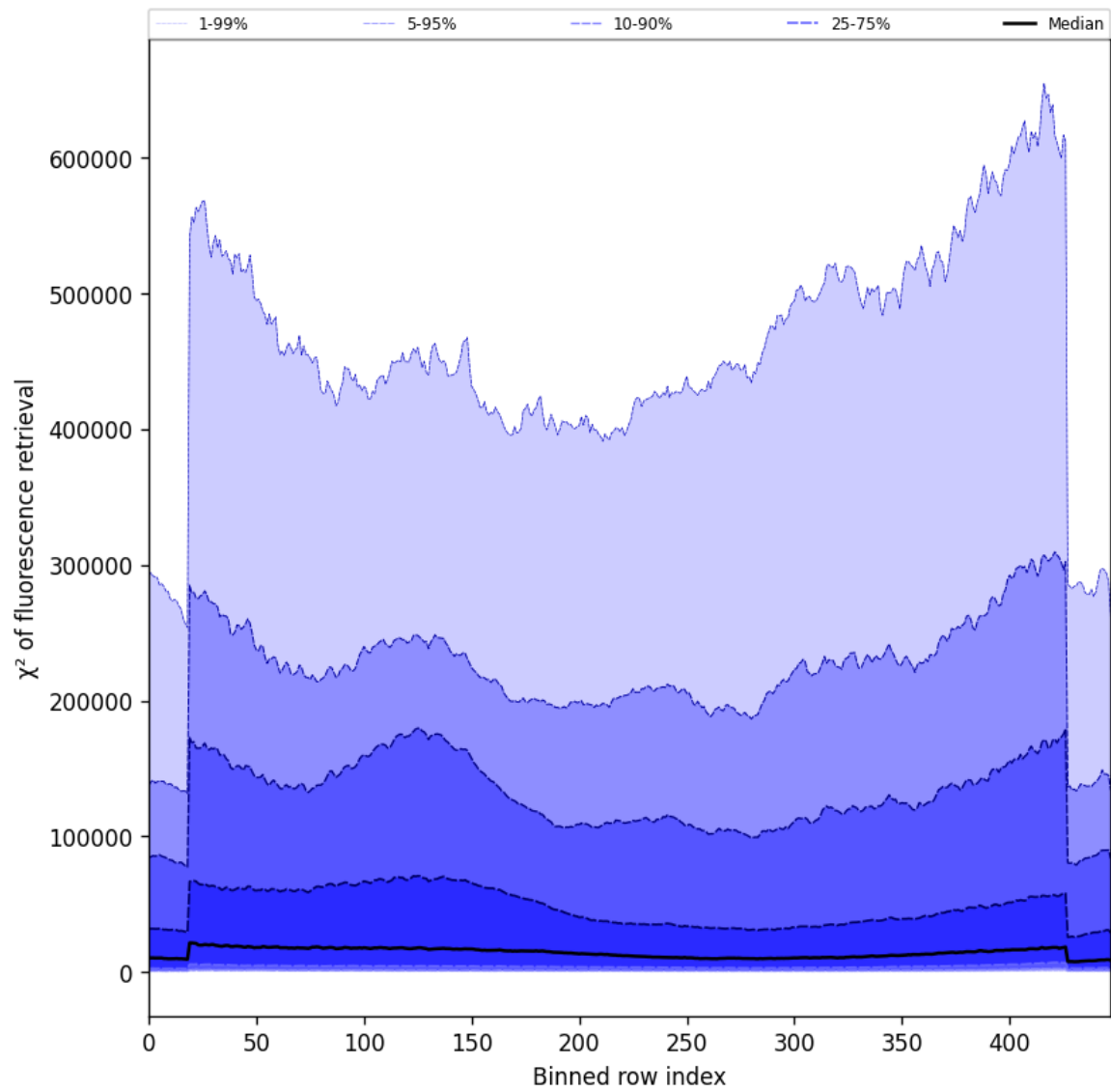
Figure 59: Along track statistics of “ \chi^2 of fluorescence retrieval” for 2025-11-02 to 2025-11-03
