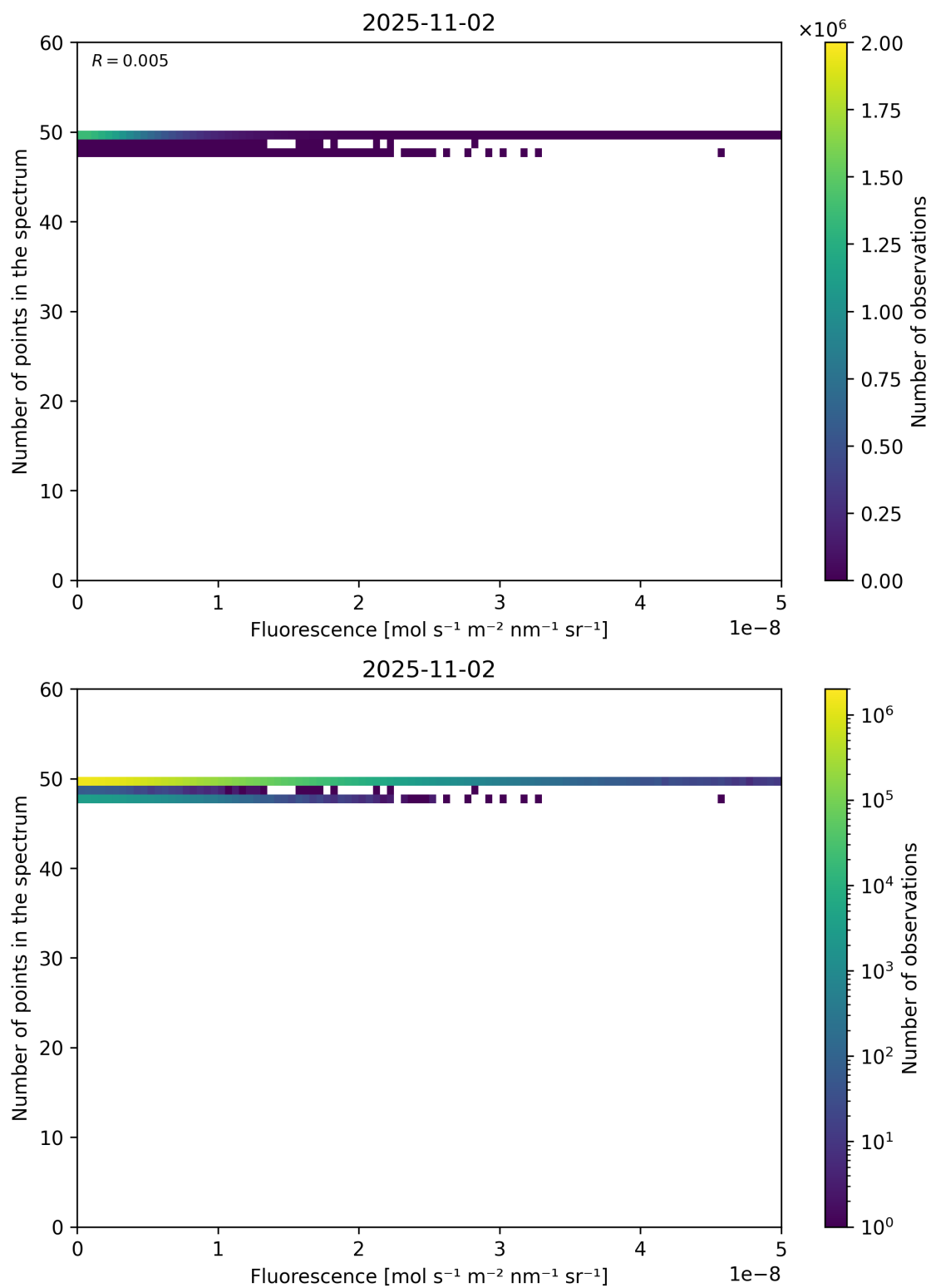
Figure 86: Scatter density plot of “Fluorescence” against “Number of points in the spectrum” for 2025-11-02 to 2025-11-03.
