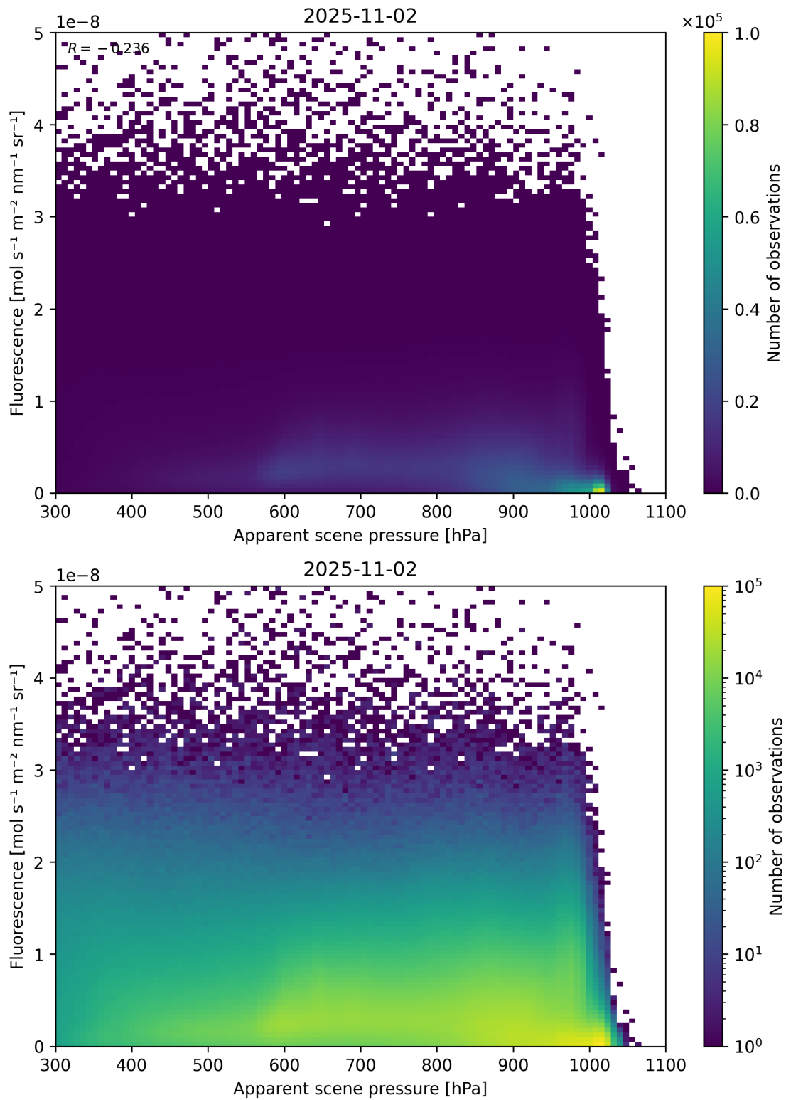
Figure 64: Scatter density plot of “Apparent scene pressure” against “Fluorescence” for 2025-11-02 to 2025-11-03.
