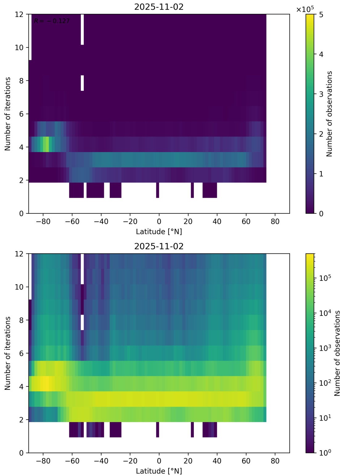
Figure 93: Scatter density plot of “Latitude” against “Number of iterations” for 2025-11-02 to 2025-11-03.
