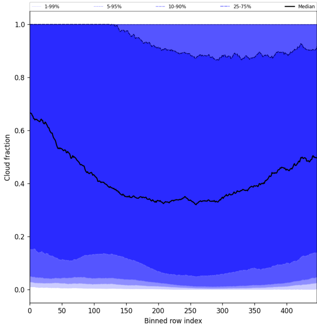
Figure 49: Along track statistics of “Cloud fraction” for 2025-11-02 to 2025-11-03
