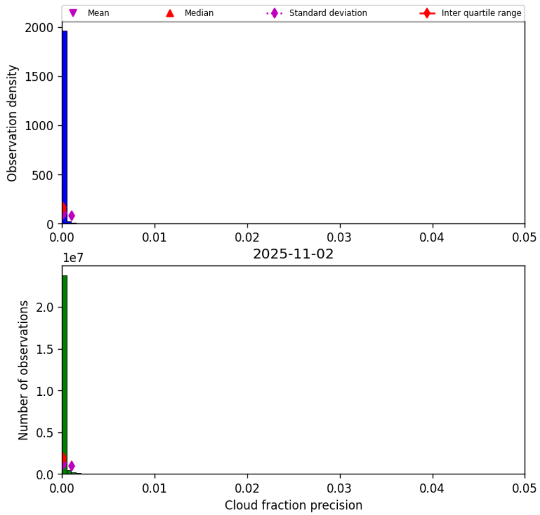
Figure 33: Histogram of “Cloud fraction precision” for 2025-11-02 to 2025-11-03
