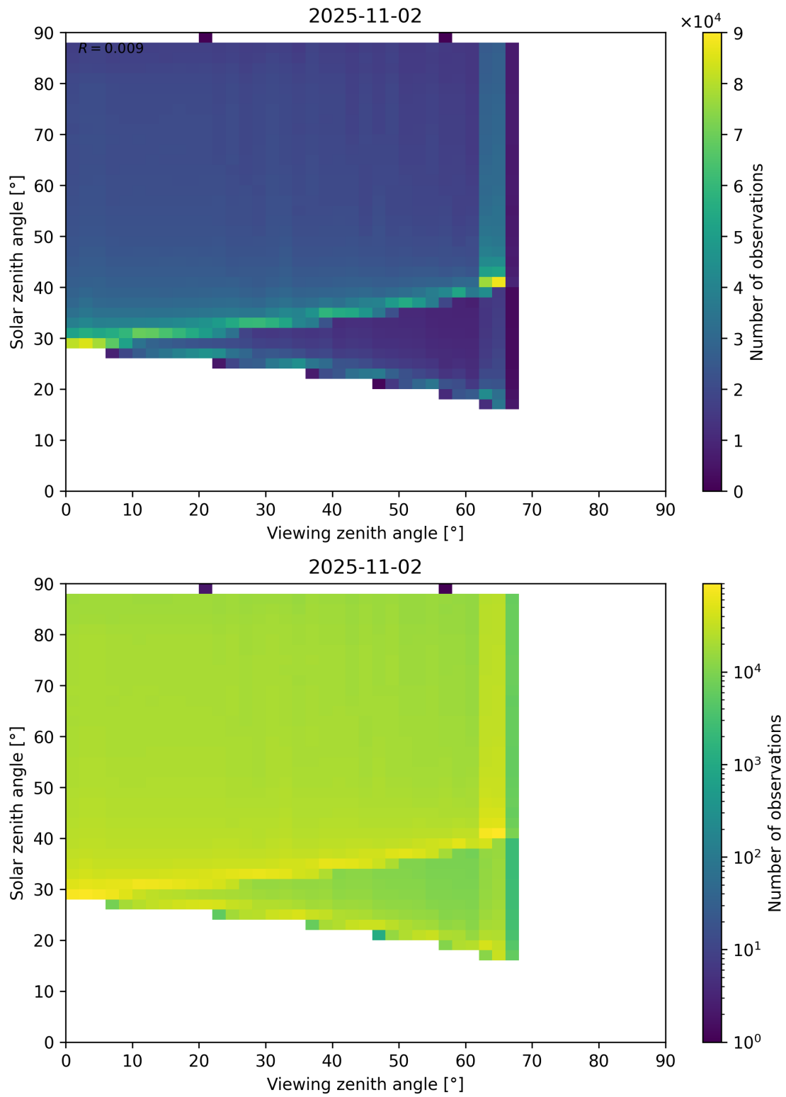
Figure 127: Scatter density plot of “Viewing zenith angle” against “Solar zenith angle” for 2025-11-02 to 2025-11-03.
