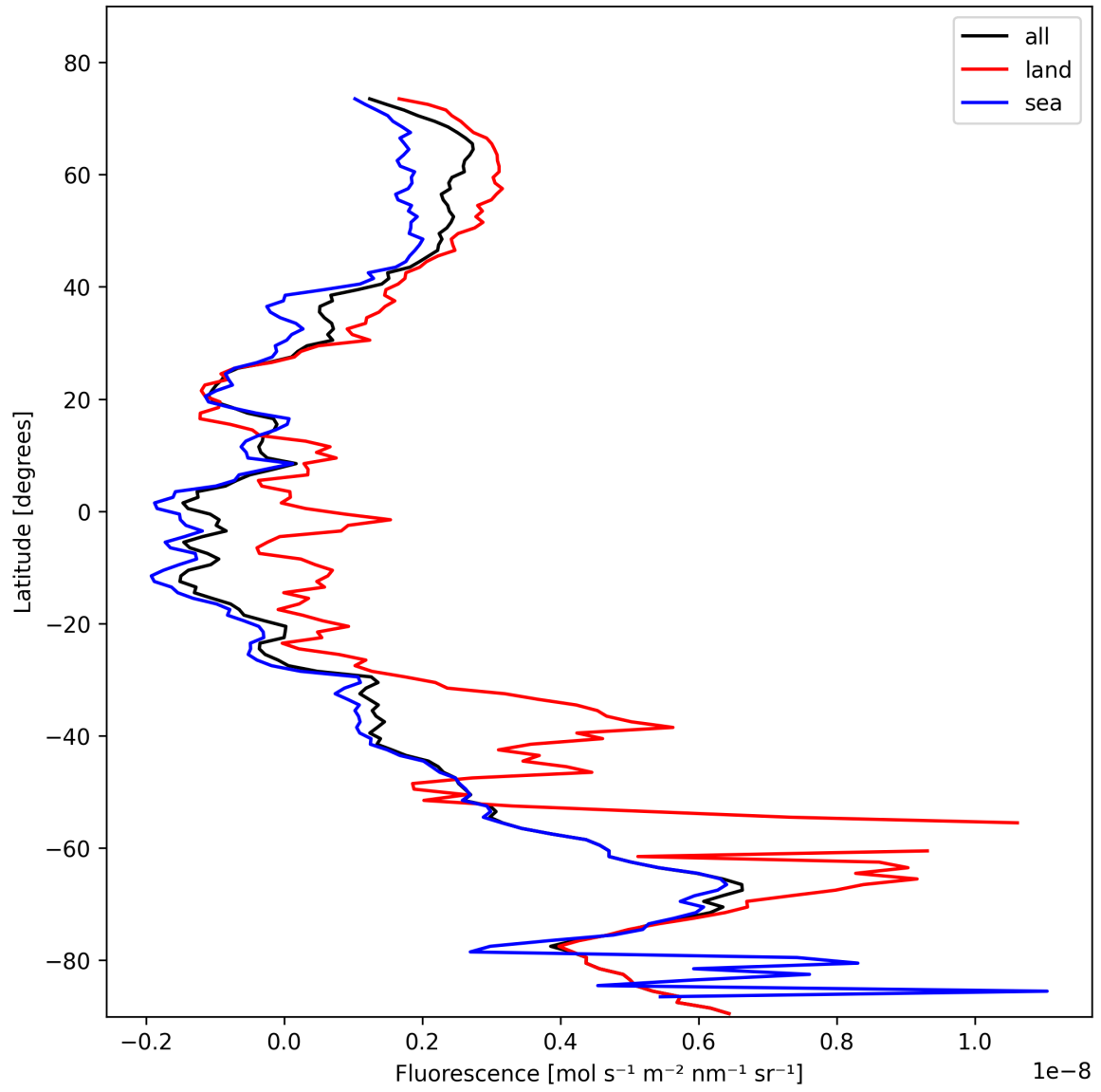
Figure 23: Zonal average of “Fluorescence” for 2025-11-02 to 2025-11-03.
