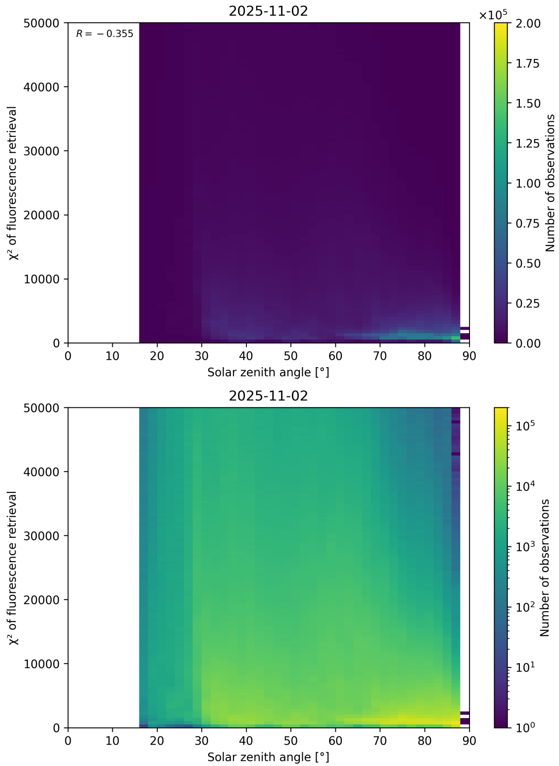
Figure 109: Scatter density plot of “Solar zenith angle” against “ \chi^2 of fluorescence retrieval” for 2025-11-02 to 2025-11-03.
