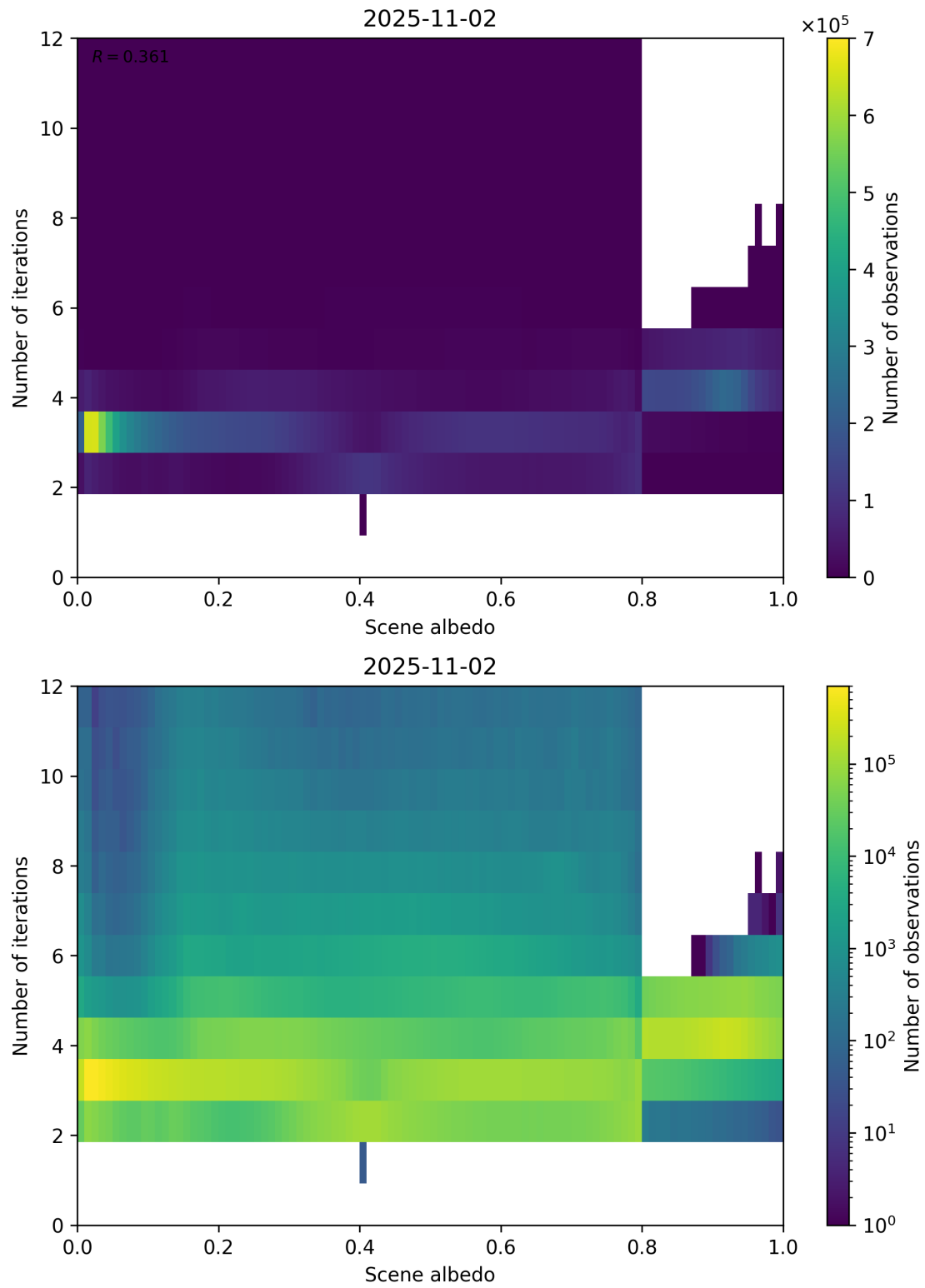
Figure 105: Scatter density plot of “Scene albedo” against “Number of iterations” for 2025-11-02 to 2025-11-03.
