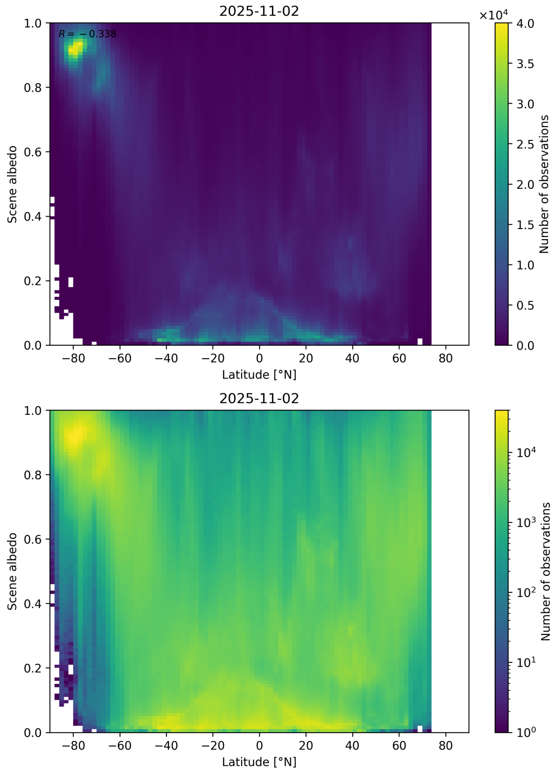
Figure 95: Scatter density plot of “Latitude” against “Scene albedo” for 2025-11-02 to 2025-11-03.
