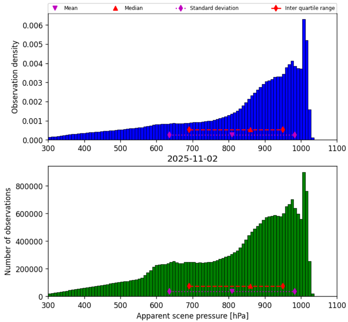
Figure 36: Histogram of “Apparent scene pressure” for 2025-11-02 to 2025-11-03
