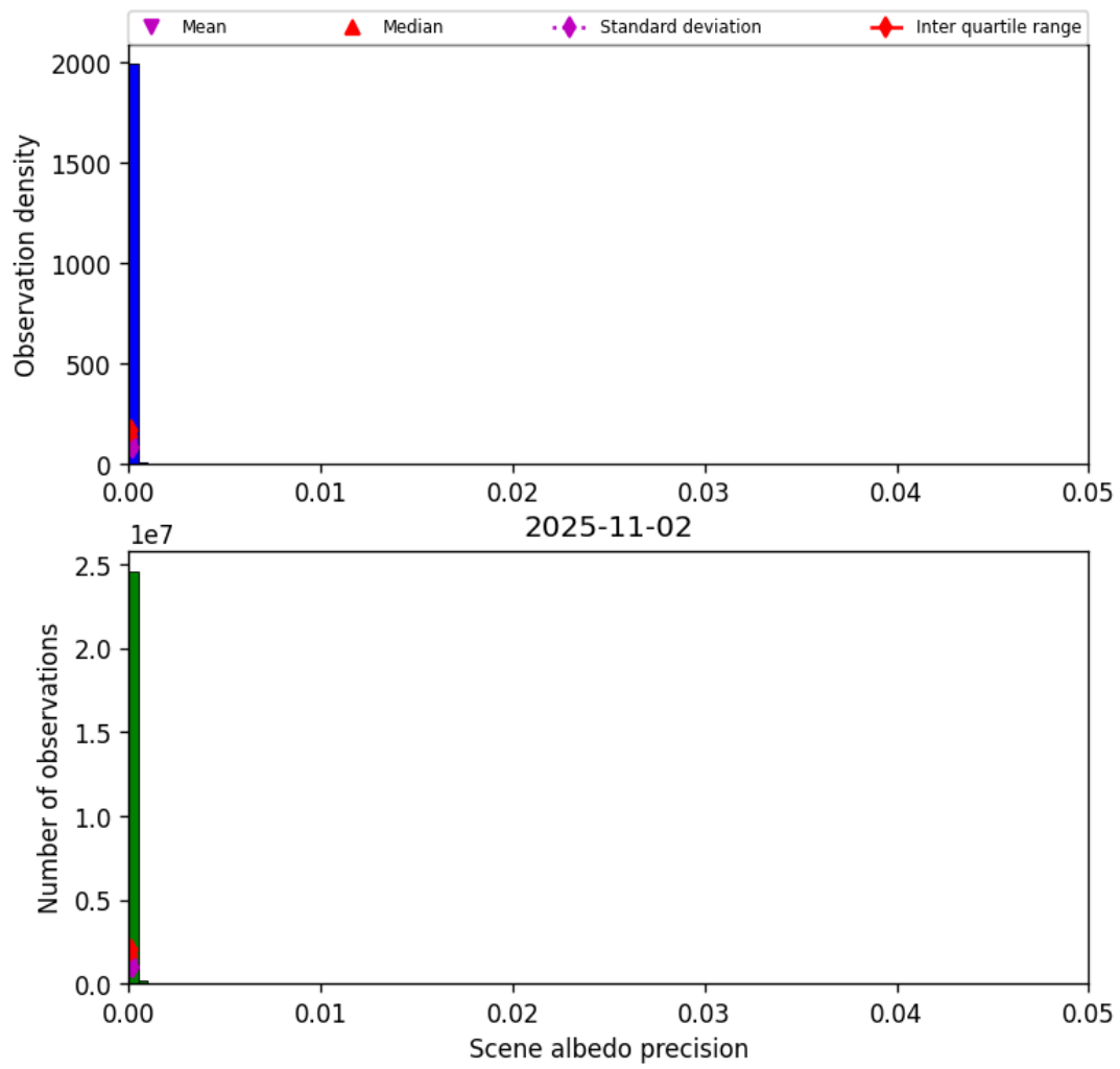
Figure 35: Histogram of “Scene albedo precision” for 2025-11-02 to 2025-11-03
