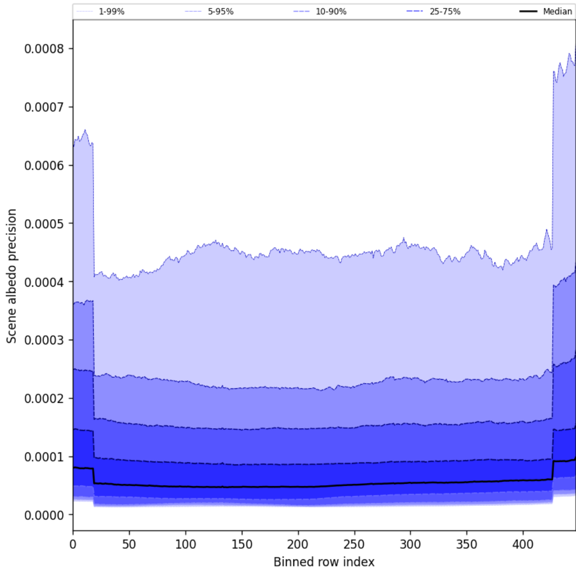
Figure 52: Along track statistics of “Scene albedo precision” for 2025-11-02 to 2025-11-03
