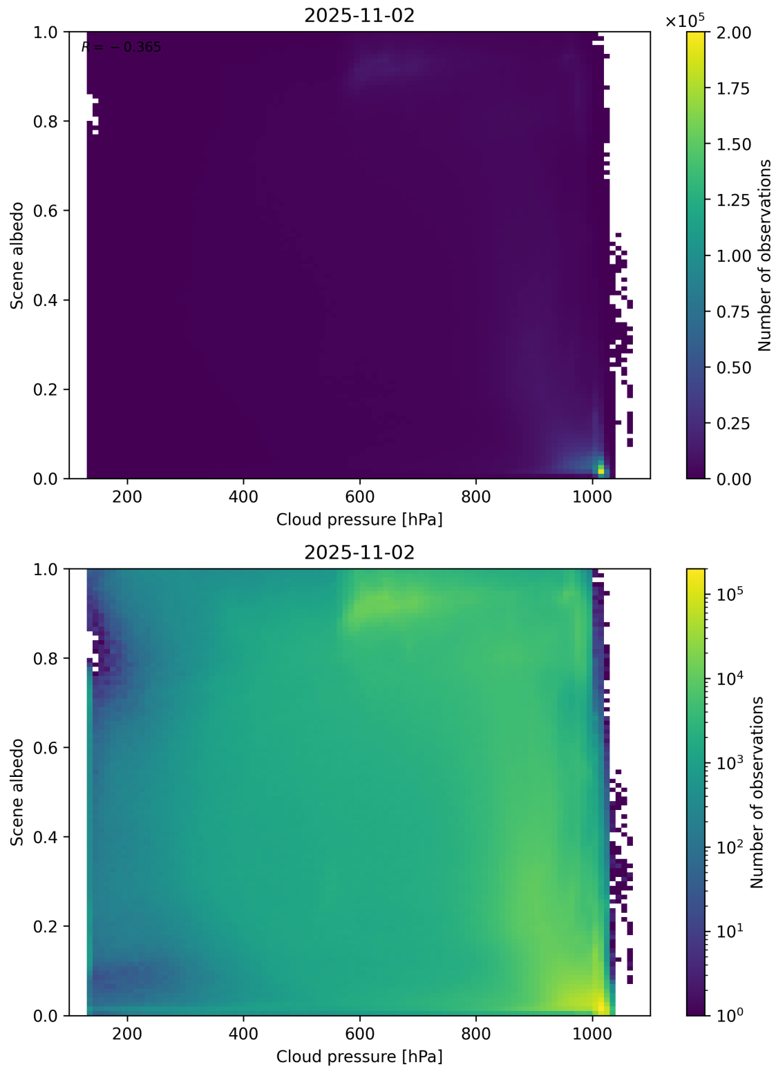
Figure 83: Scatter density plot of “Cloud pressure” against “Scene albedo” for 2025-11-02 to 2025-11-03.
