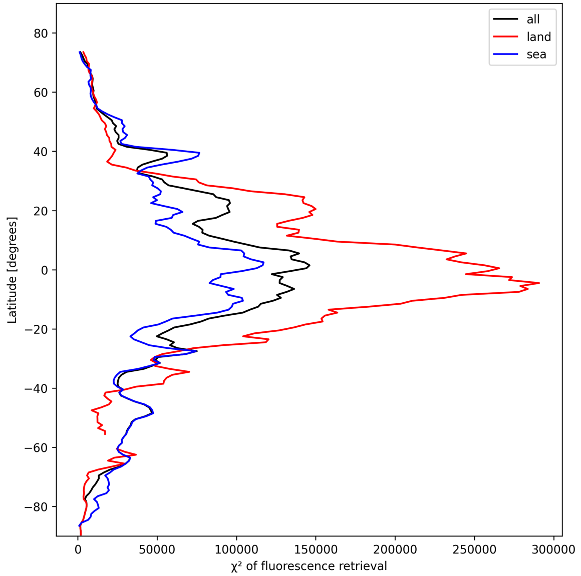
Figure 25: Zonal average of “ \chi^2 of fluorescence retrieval” for 2025-11-02 to 2025-11-03.
