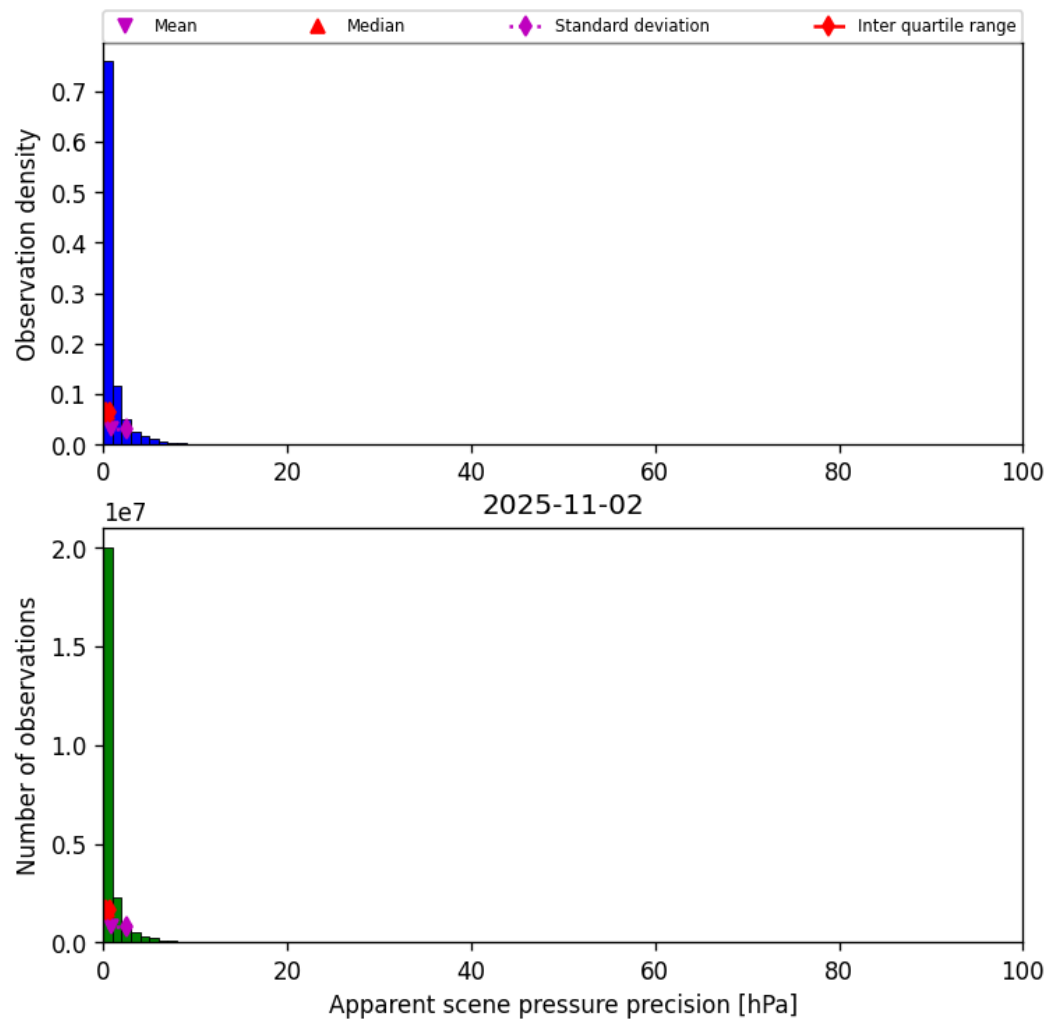
Figure 37: Histogram of “Apparent scene pressure precision” for 2025-11-02 to 2025-11-03
