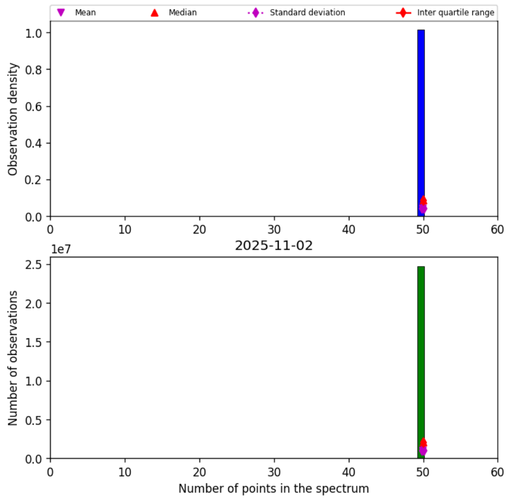
Figure 44: Histogram of “Number of points in the spectrum” for 2025-11-02 to 2025-11-03
