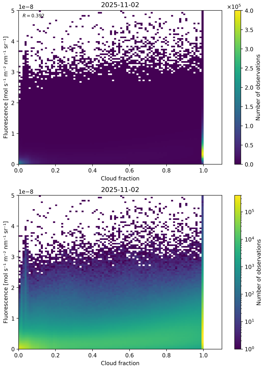
Figure 72: Scatter density plot of “Cloud fraction” against “Fluorescence” for 2025-11-02 to 2025-11-03.
