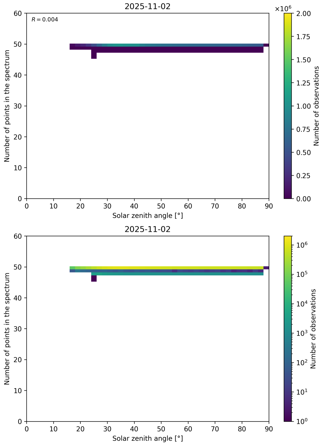
Figure 115: Scatter density plot of “Solar zenith angle” against “Number of points in the spectrum” for 2025-11-02 to 2025-11-03.
