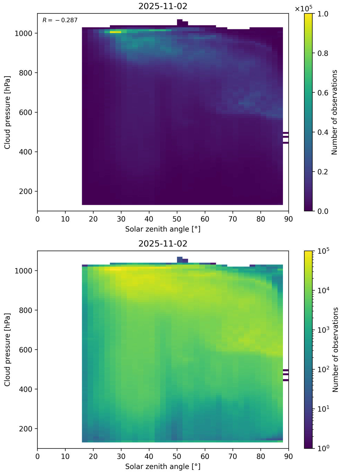
Figure 111: Scatter density plot of “Solar zenith angle” against “Cloud pressure” for 2025-11-02 to 2025-11-03.
