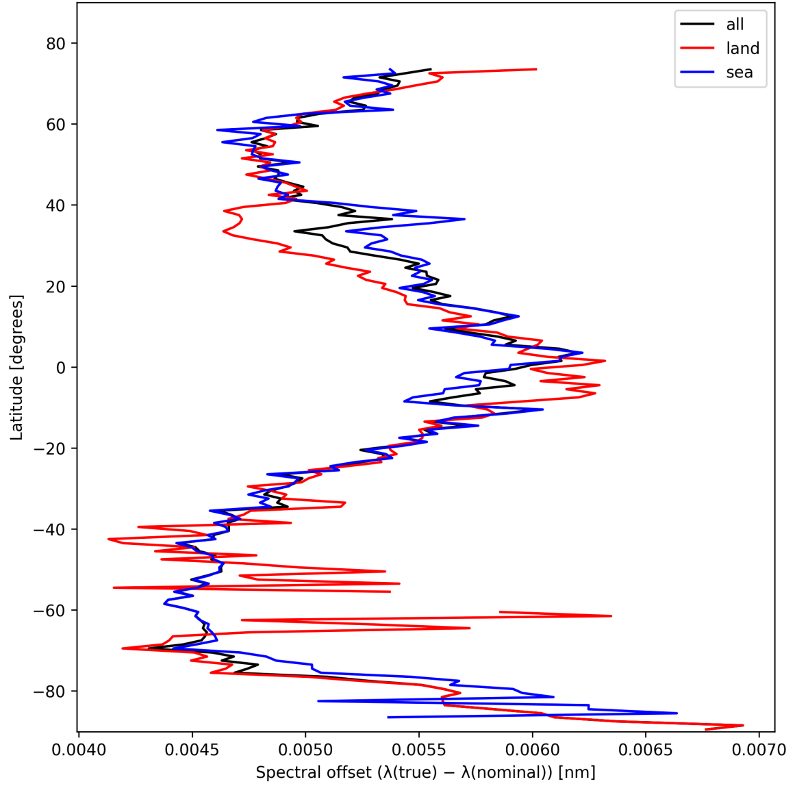
Figure 28: Zonal average of “Spectral offset ( \lambda_{\text{true}} - \lambda_{\text{nominal}} )” for 2025-11-02 to 2025-11-03.
