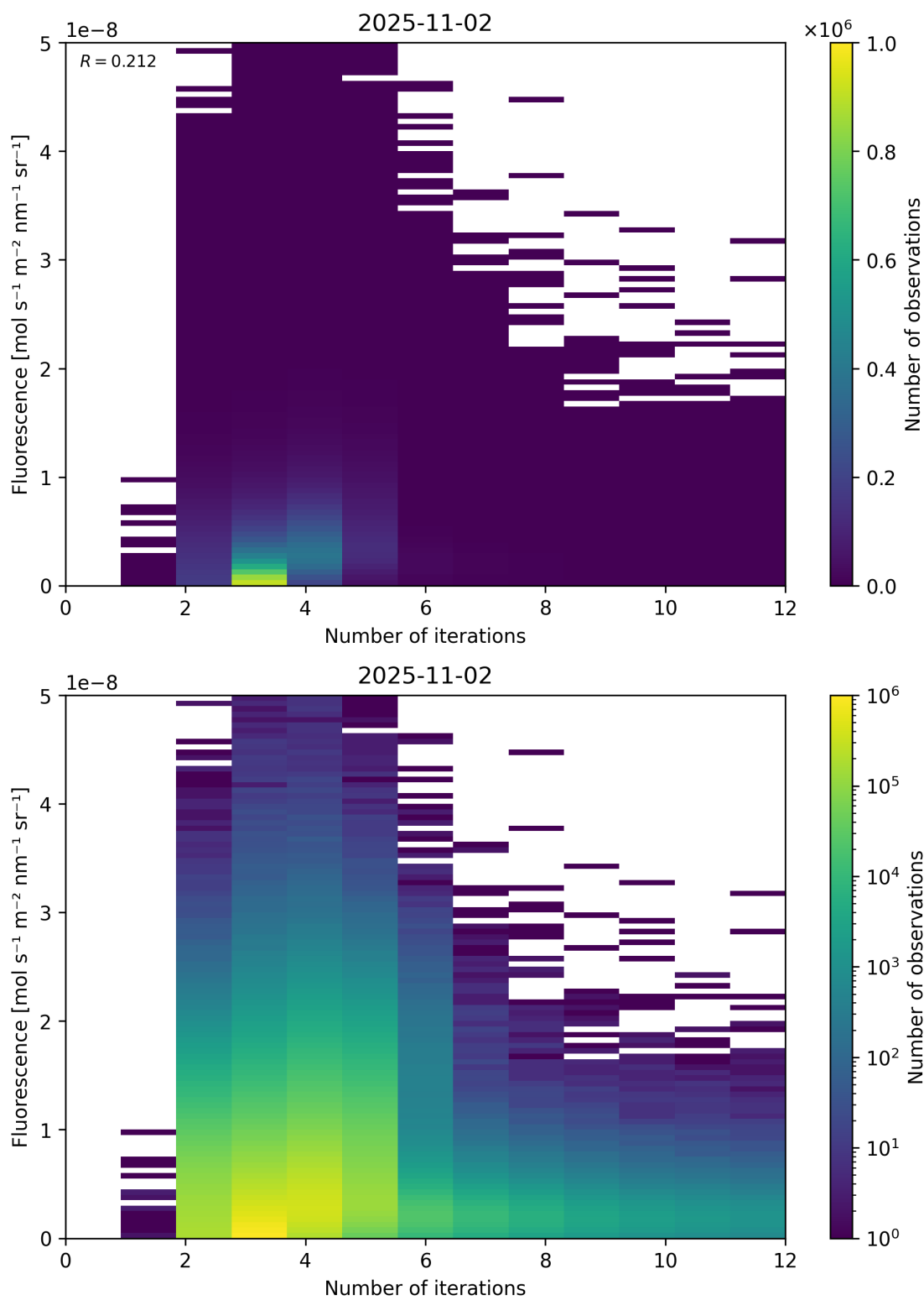
Figure 98: Scatter density plot of “Number of iterations” against “Fluorescence” for 2025-11-02 to 2025-11-03.
