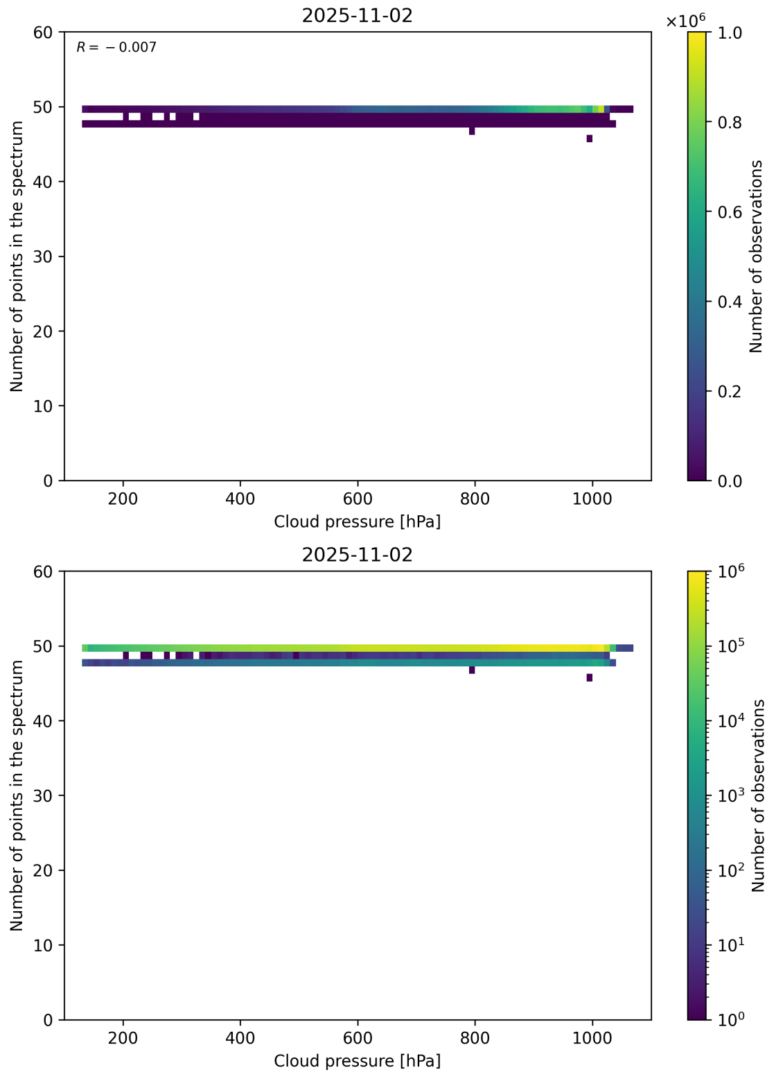
Figure 82: Scatter density plot of “Cloud pressure” against “Number of points in the spectrum” for 2025-11-02 to 2025-11-03.
