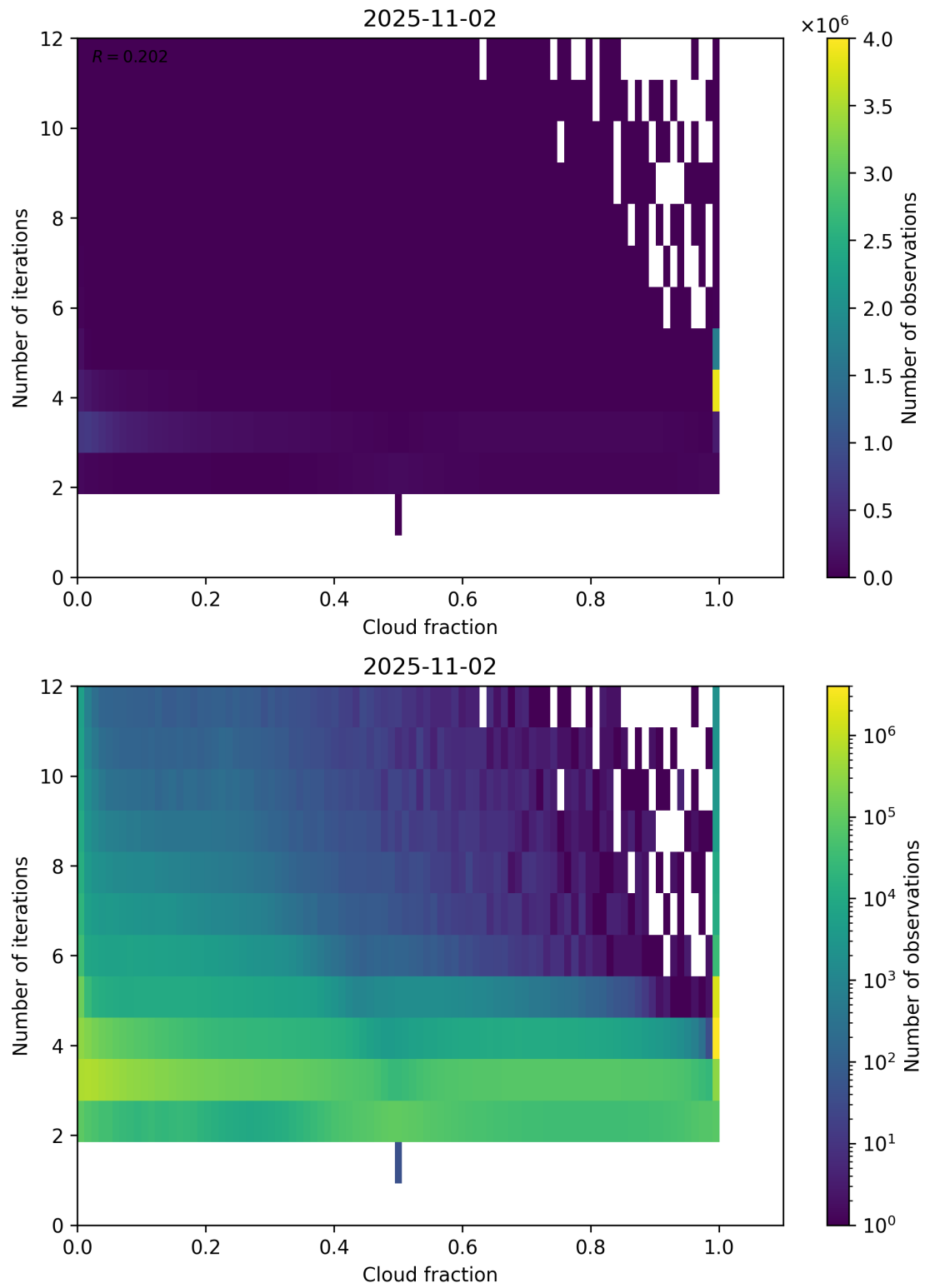
Figure 73: Scatter density plot of “Cloud fraction” against “Number of iterations” for 2025-11-02 to 2025-11-03.
