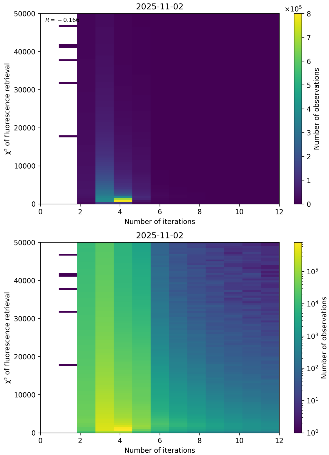
Figure 97: Scatter density plot of “Number of iterations” against “ \chi^2 of fluorescence retrieval” for 2025-11-02 to 2025-11-03.
