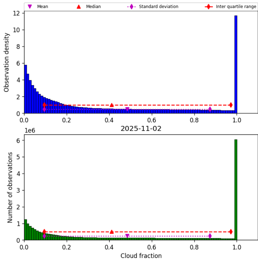
Figure 32: Histogram of “Cloud fraction” for 2025-11-02 to 2025-11-03
