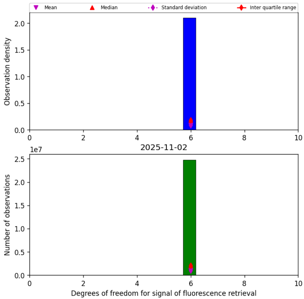
Figure 43: Histogram of “Degrees of freedom for signal of fluorescence retrieval” for 2025-11-02 to 2025-11-03
