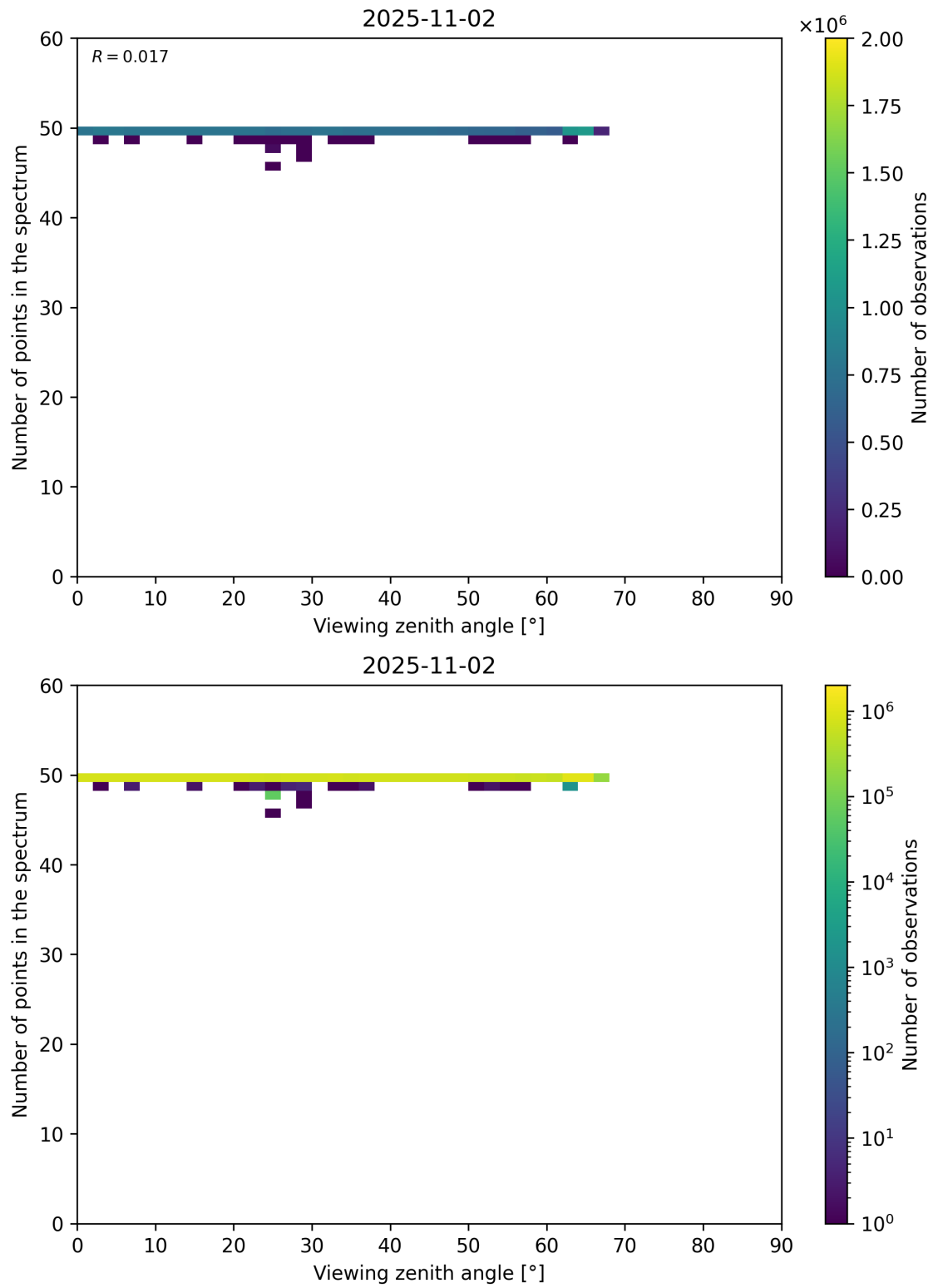
Figure 125: Scatter density plot of “Viewing zenith angle” against “Number of points in the spectrum” for 2025-11-02 to 2025-11-03.
