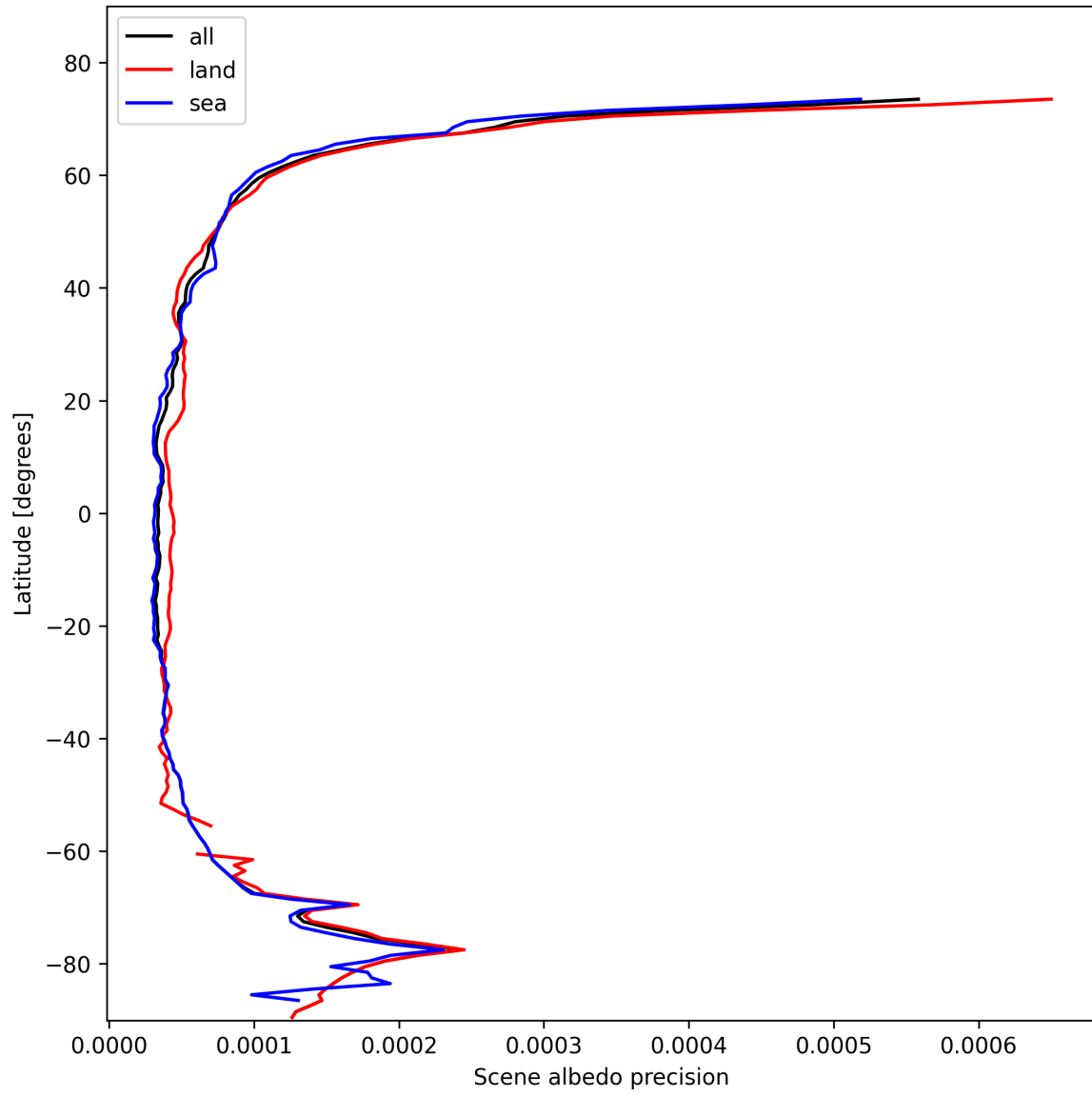
Figure 18: Zonal average of “Scene albedo precision” for 2025-11-02 to 2025-11-03.
