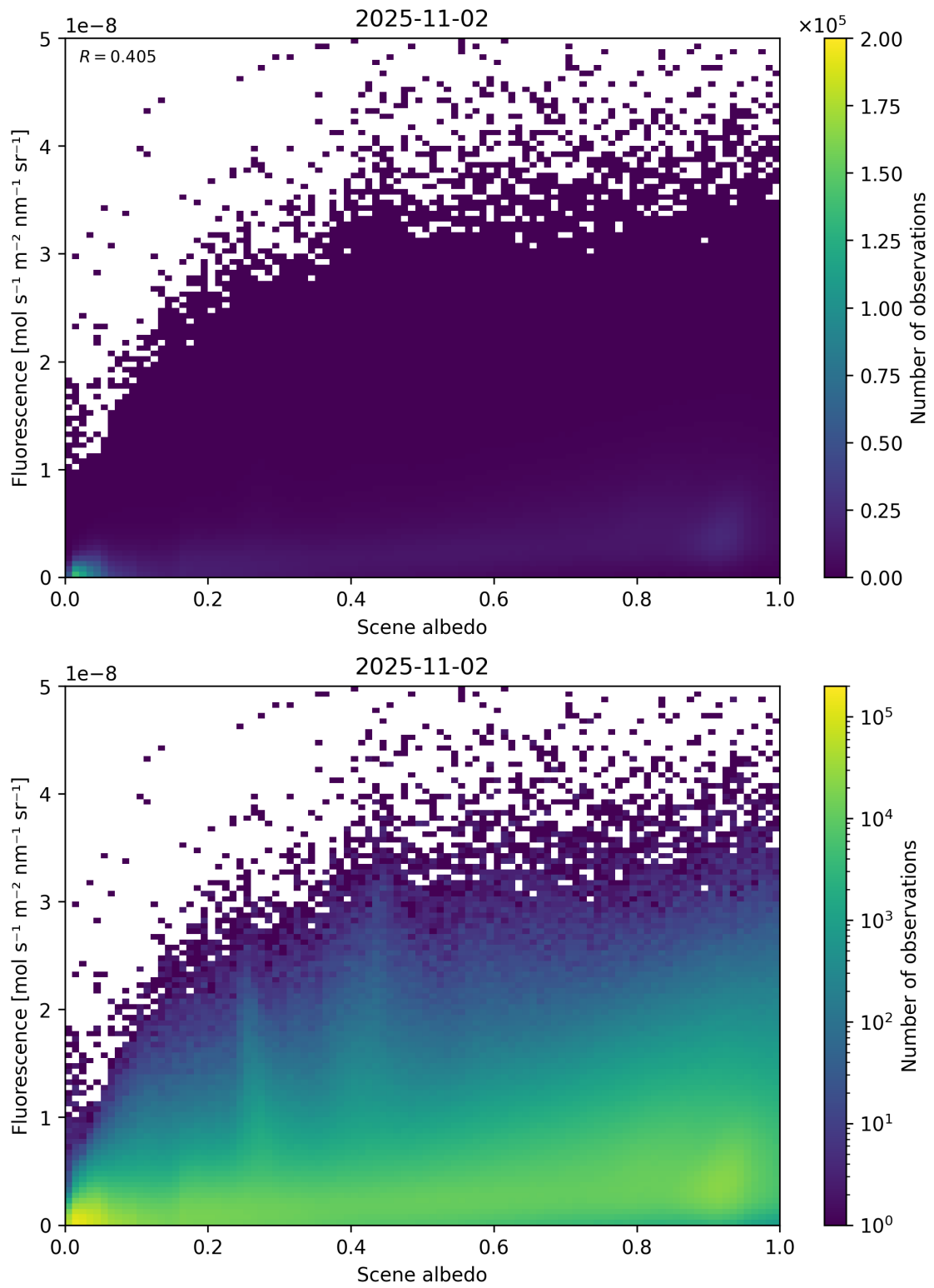
Figure 104: Scatter density plot of “Scene albedo” against “Fluorescence” for 2025-11-02 to 2025-11-03.
