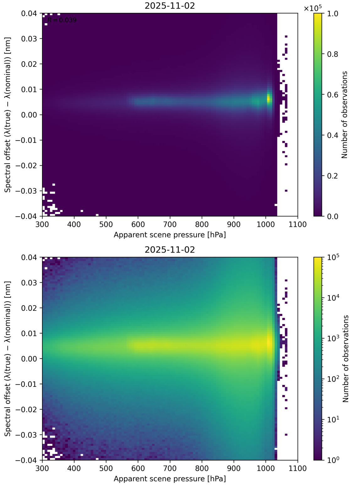
Figure 67: Scatter density plot of “Apparent scene pressure” against “Spectral offset ( \lambda_{\text{true}} - \lambda_{\text{nominal}} )” for 2025-11-02 to 2025-11-03.
