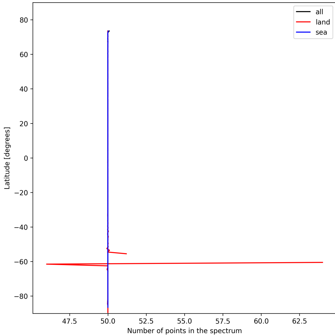
Figure 27: Zonal average of “Number of points in the spectrum” for 2025-11-02 to 2025-11-03.
