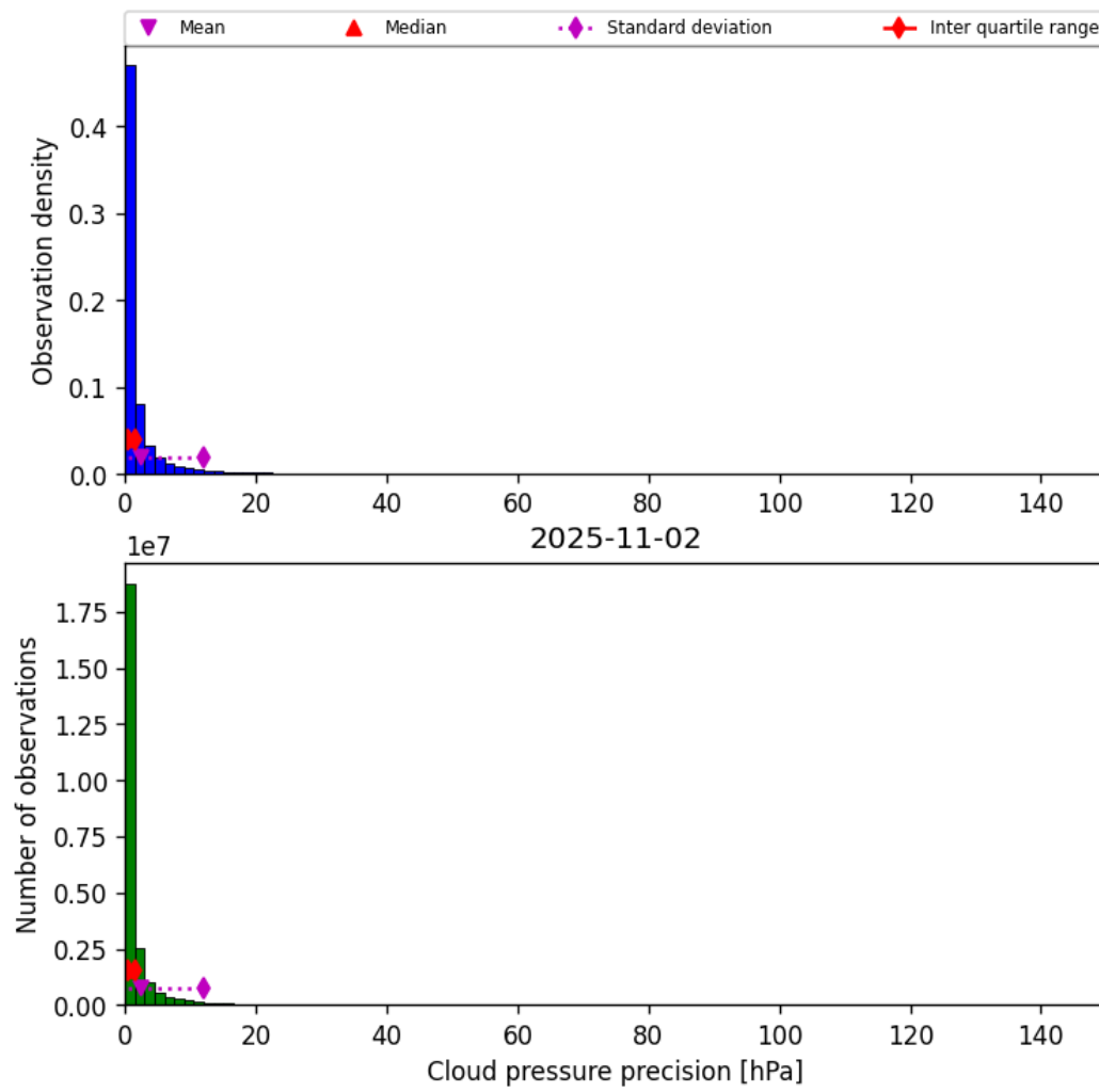
Figure 31: Histogram of “Cloud pressure precision” for 2025-11-02 to 2025-11-03
