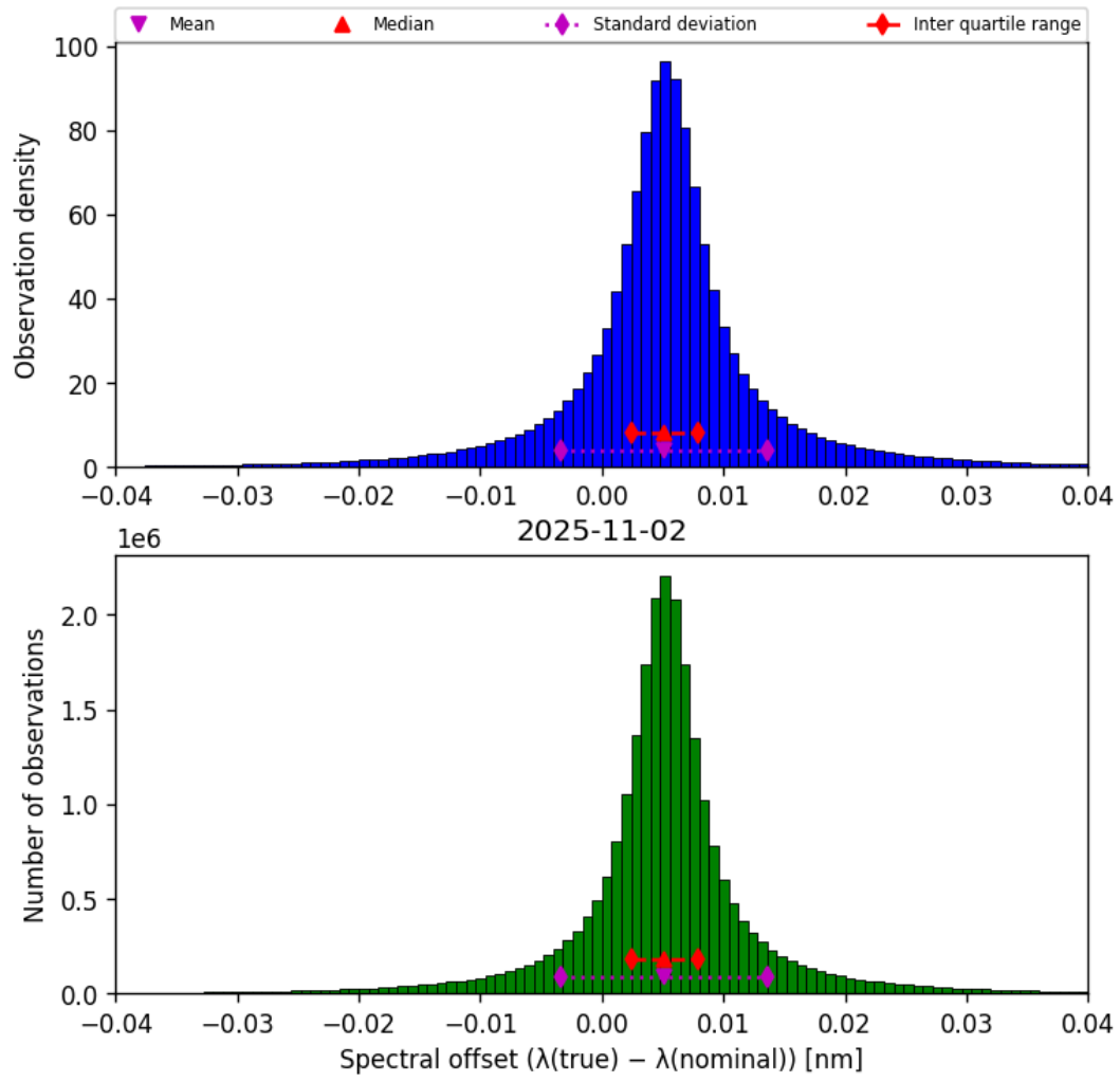
Figure 45: Histogram of “Spectral offset ( \lambda_{\text{true}} - \lambda_{\text{nominal}} )” for 2025-11-02 to 2025-11-03
