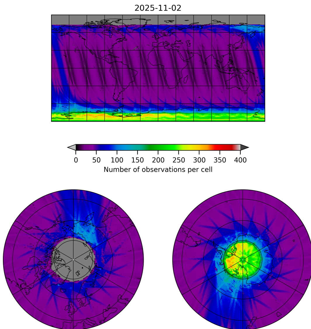
Figure 11: Map of the number of observations for 2025-11-02 to 2025-11-03
