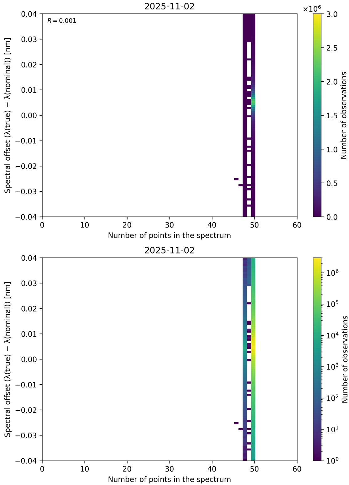
Figure 101: Scatter density plot of “Number of points in the spectrum” against “Spectral offset ( \lambda_{\text{true}} - \lambda_{\text{nominal}} )” for 2025-11-02 to 2025-11-03.
