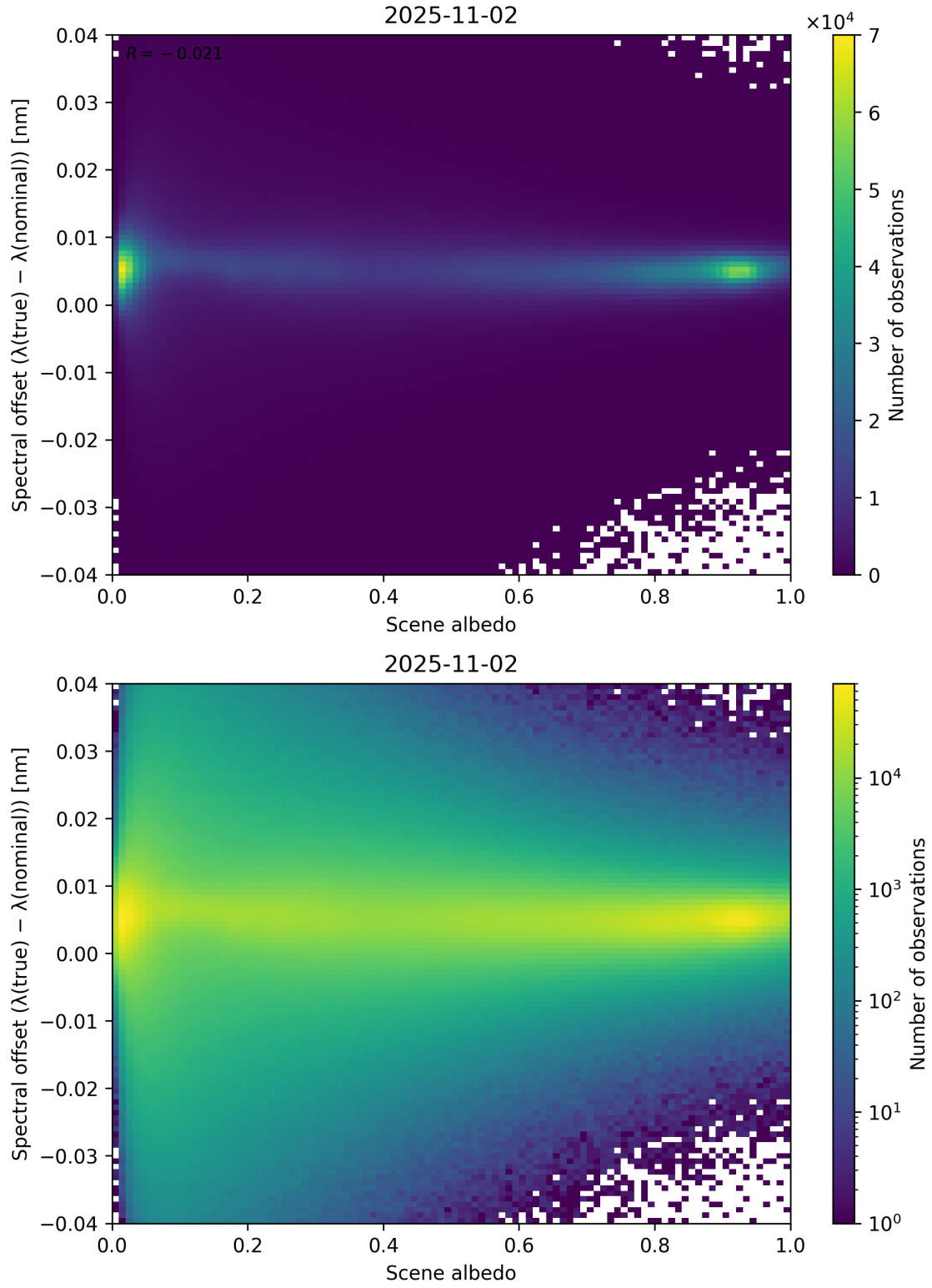
Figure 107: Scatter density plot of “Scene albedo” against “Spectral offset ( \lambda_{\text{true}} - \lambda_{\text{nominal}} )” for 2025-11-02 to 2025-11-03.
