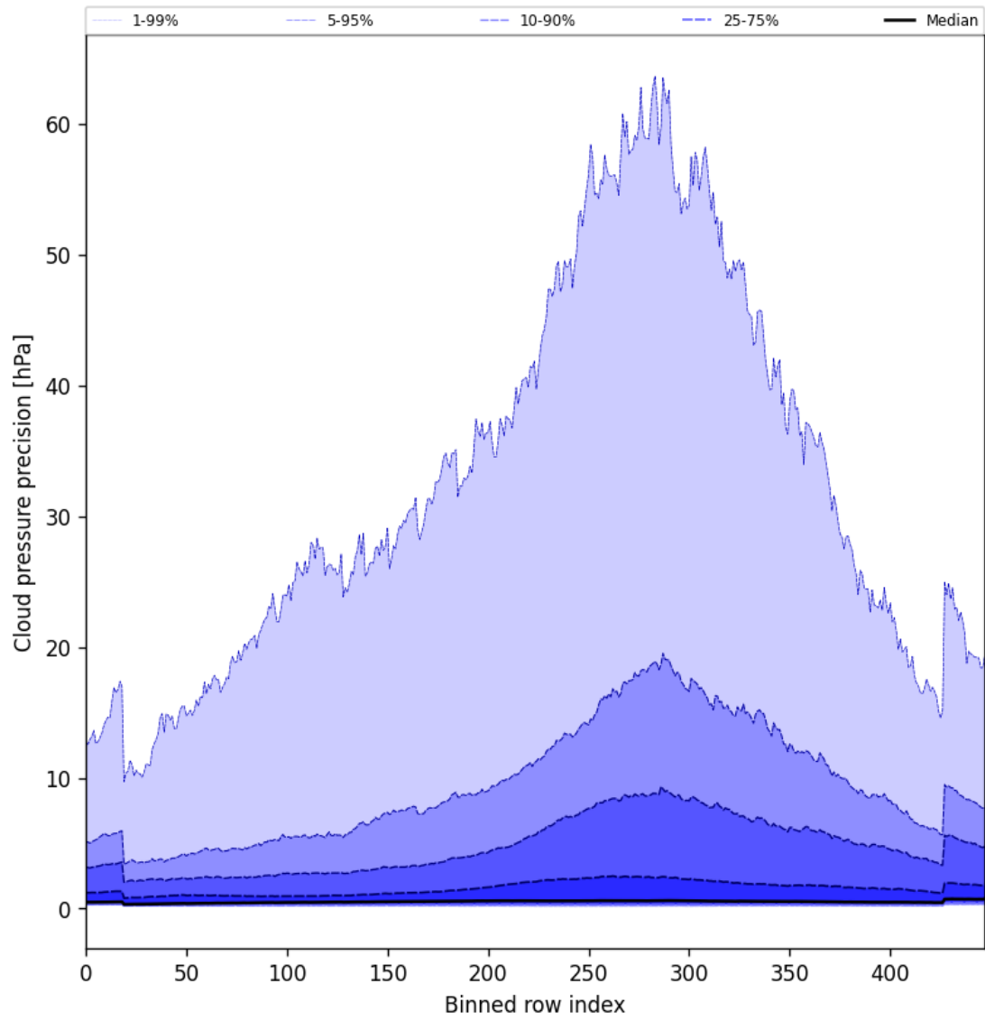
Figure 48: Along track statistics of “Cloud pressure precision” for 2025-11-02 to 2025-11-03
