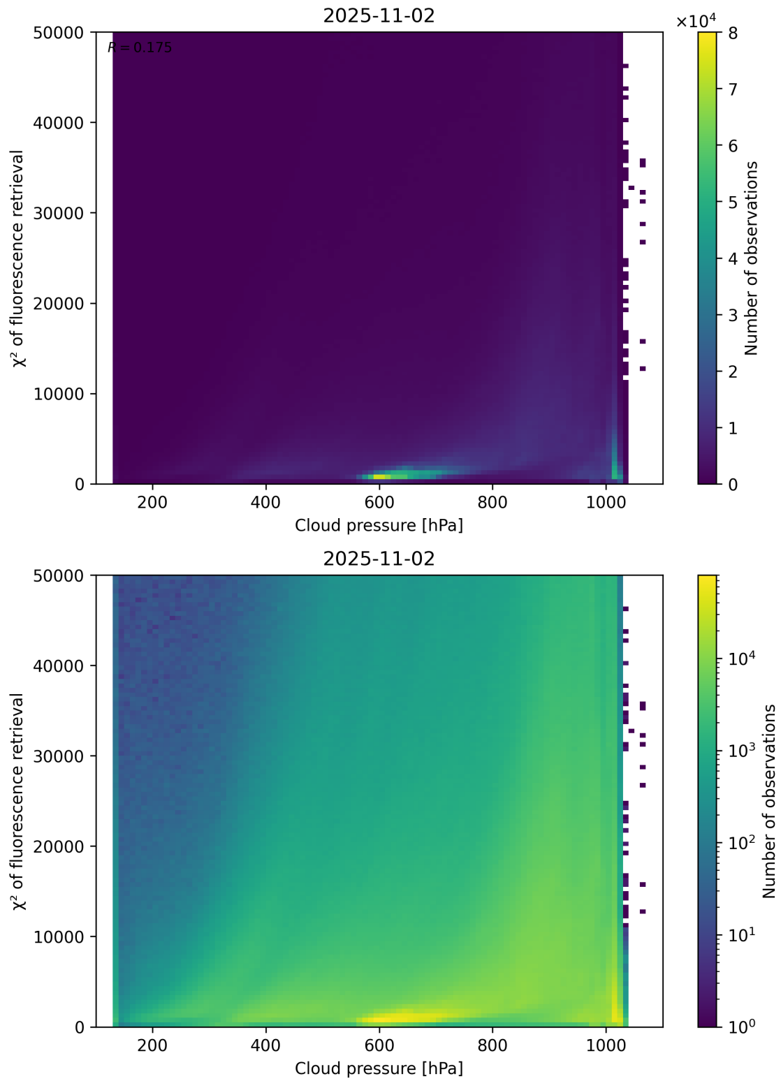
Figure 78: Scatter density plot of “Cloud pressure” against “ \chi^2 of fluorescence retrieval” for 2025-11-02 to 2025-11-03.
