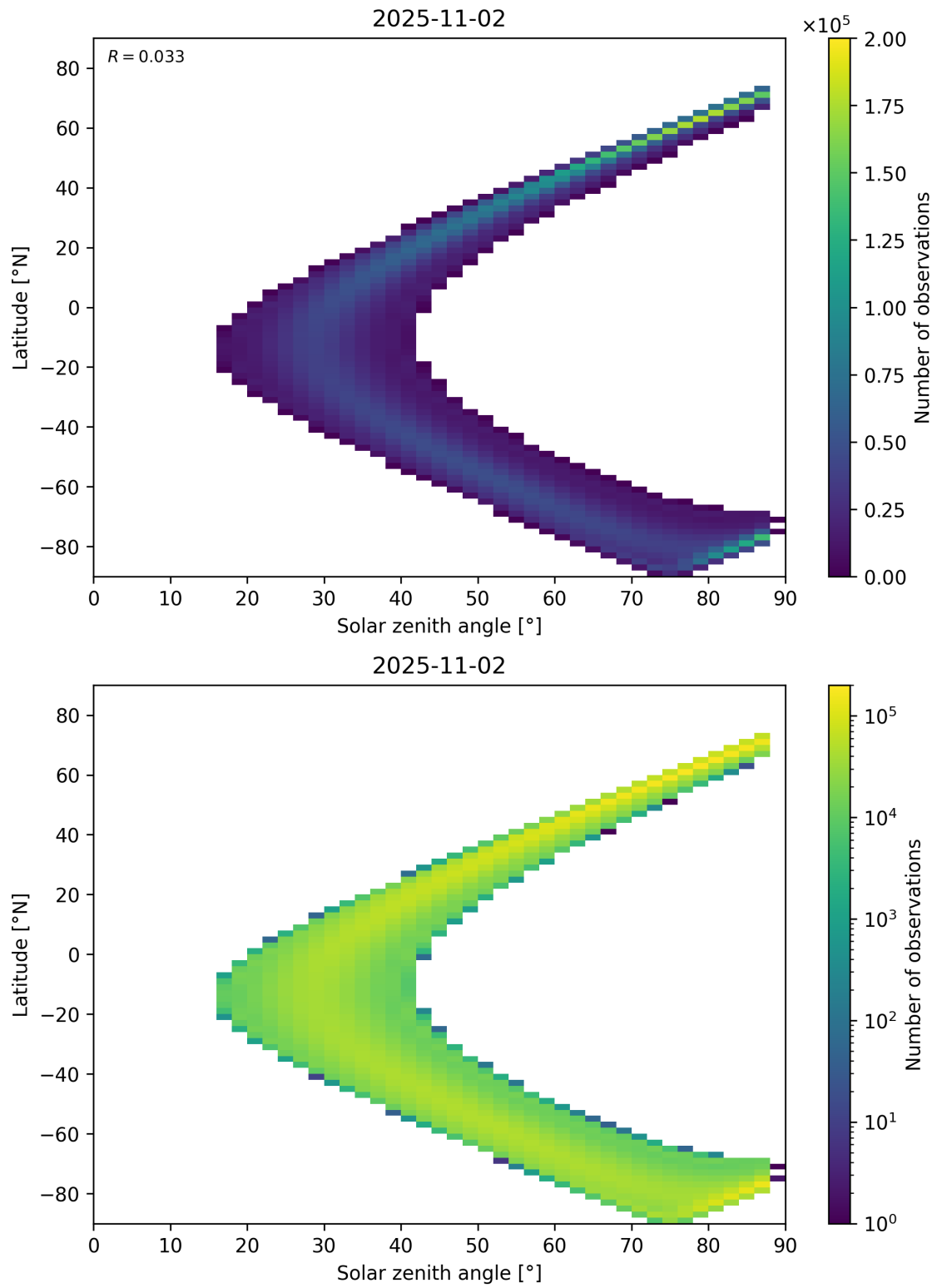
Figure 113: Scatter density plot of “Solar zenith angle” against “Latitude” for 2025-11-02 to 2025-11-03.
