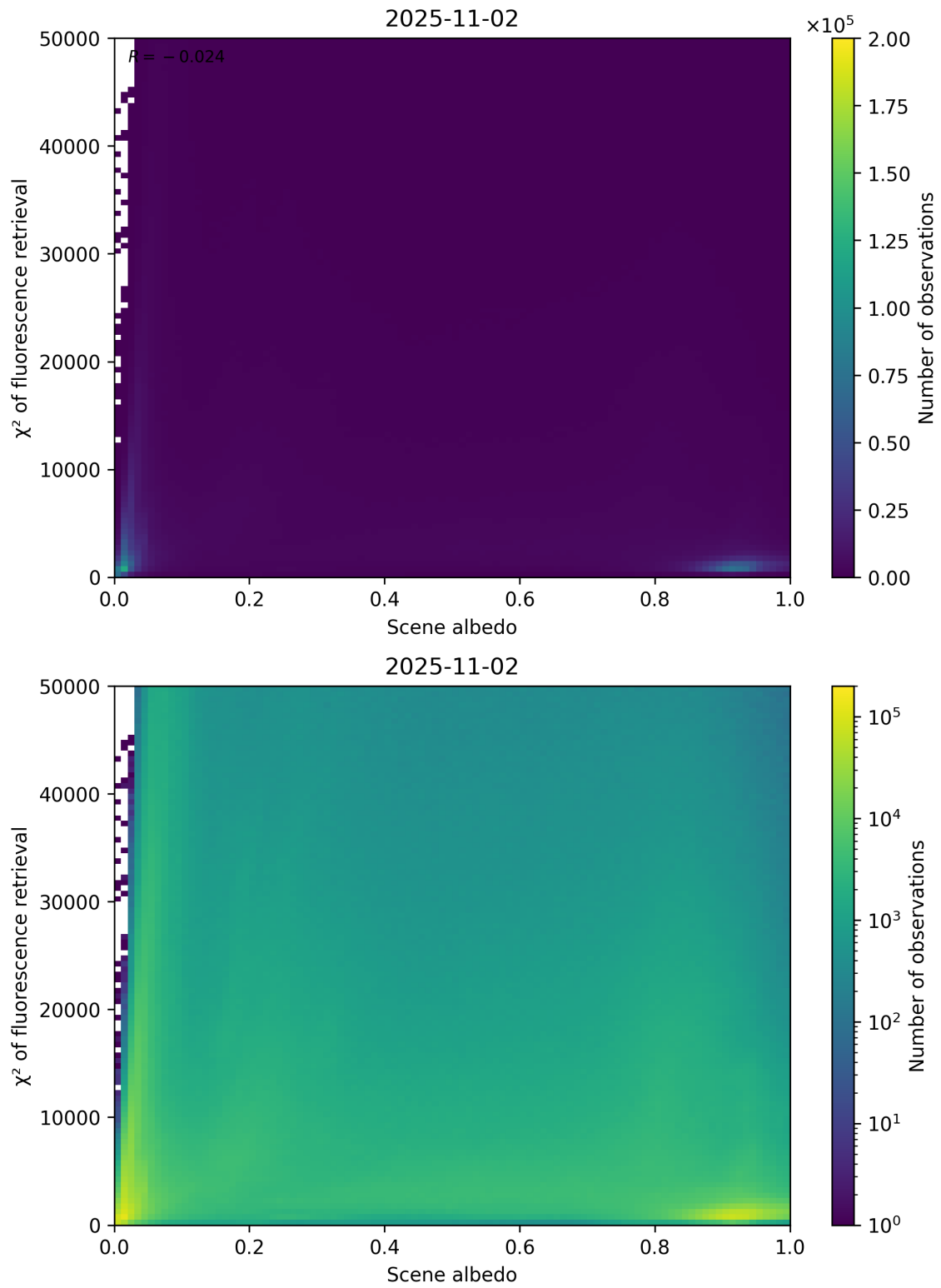
Figure 103: Scatter density plot of “Scene albedo” against “ \chi^2 of fluorescence retrieval” for 2025-11-02 to 2025-11-03.
