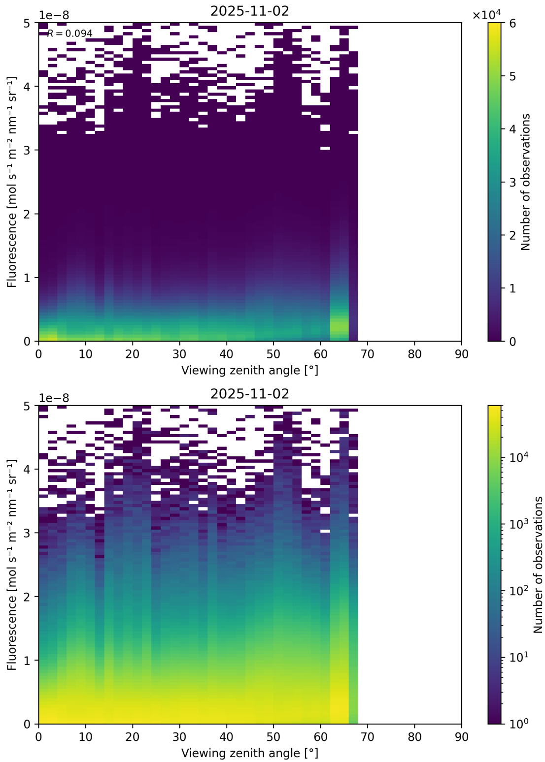
Figure 122: Scatter density plot of “Viewing zenith angle” against “Fluorescence” for 2025-11-02 to 2025-11-03.
