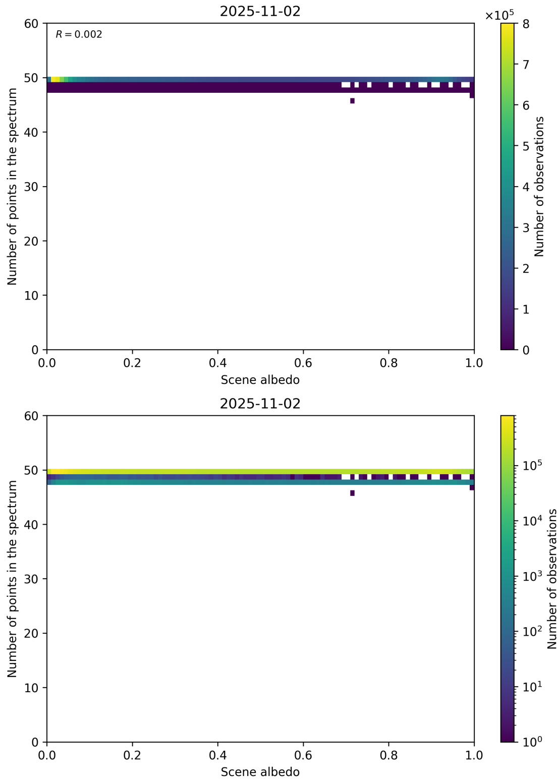
Figure 106: Scatter density plot of “Scene albedo” against “Number of points in the spectrum” for 2025-11-02 to 2025-11-03.
