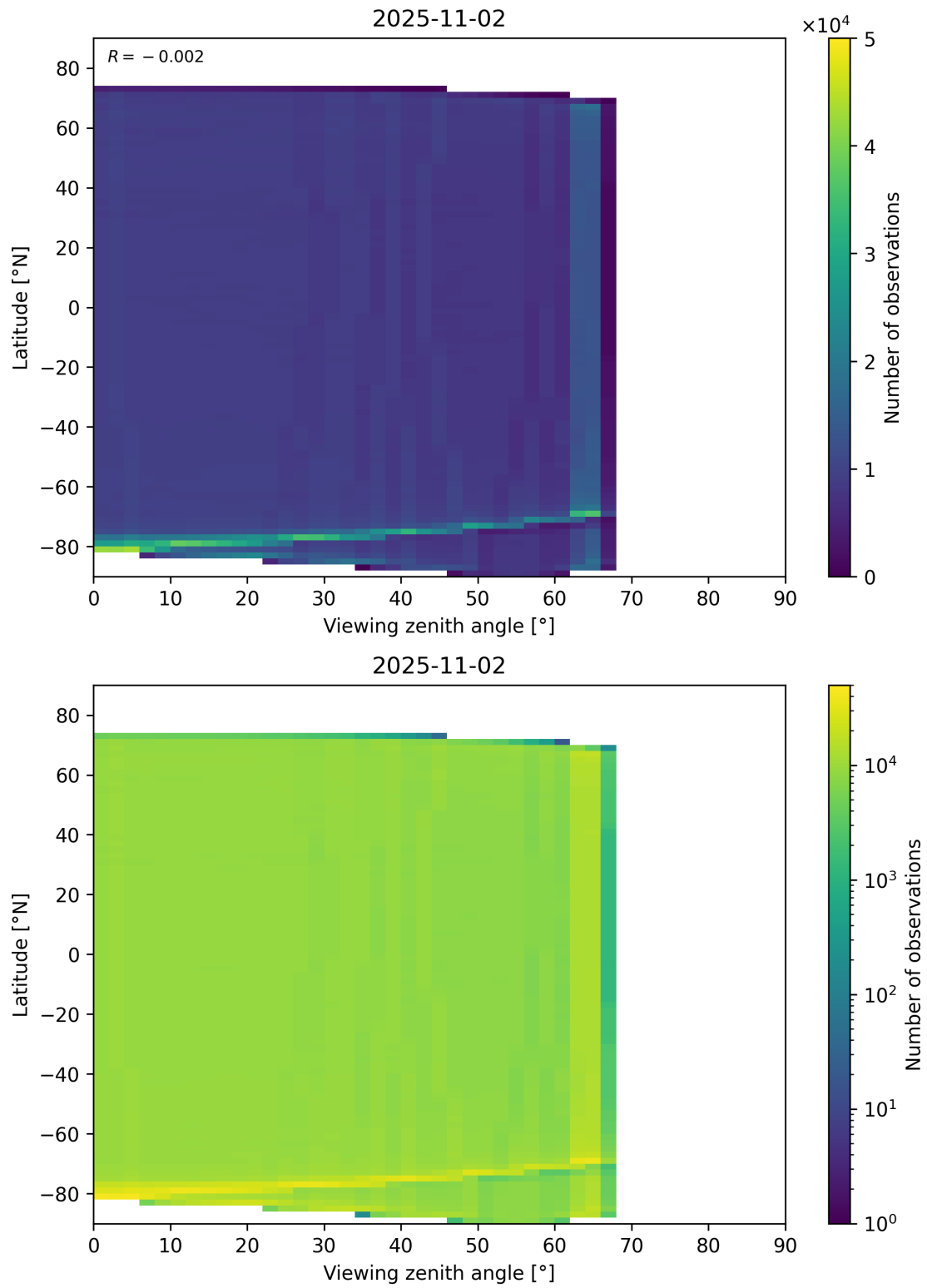
Figure 123: Scatter density plot of “Viewing zenith angle” against “Latitude” for 2025-11-02 to 2025-11-03.
