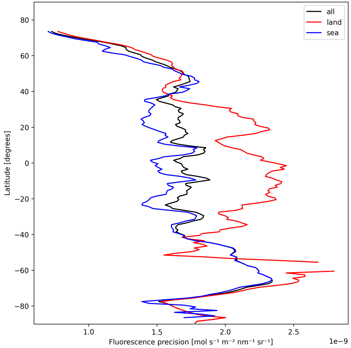
Figure 24: Zonal average of “Fluorescence precision” for 2025-11-02 to 2025-11-03.
