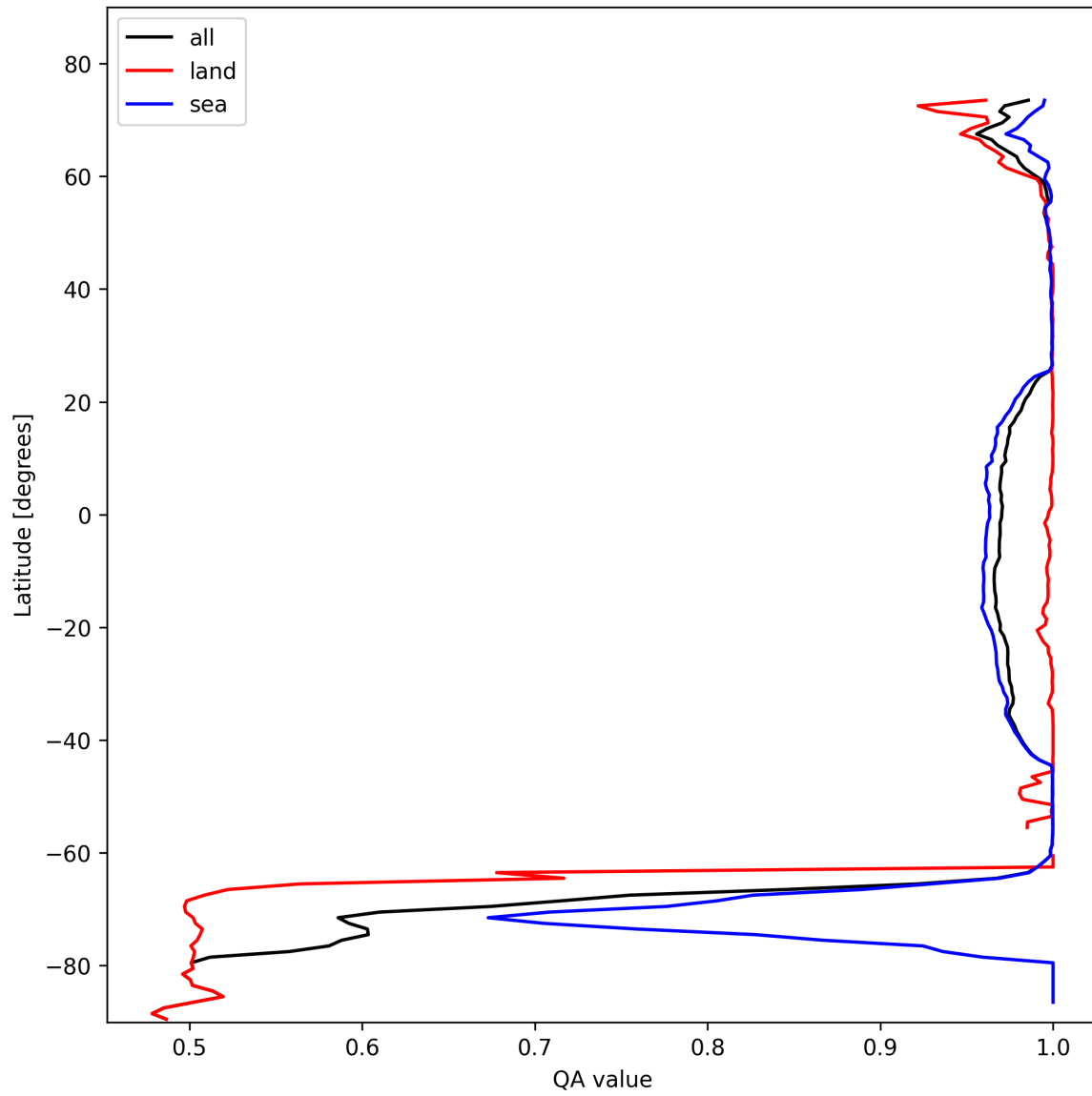
Figure 12: Zonal average of “QA value” for 2025-11-02 to 2025-11-03.
