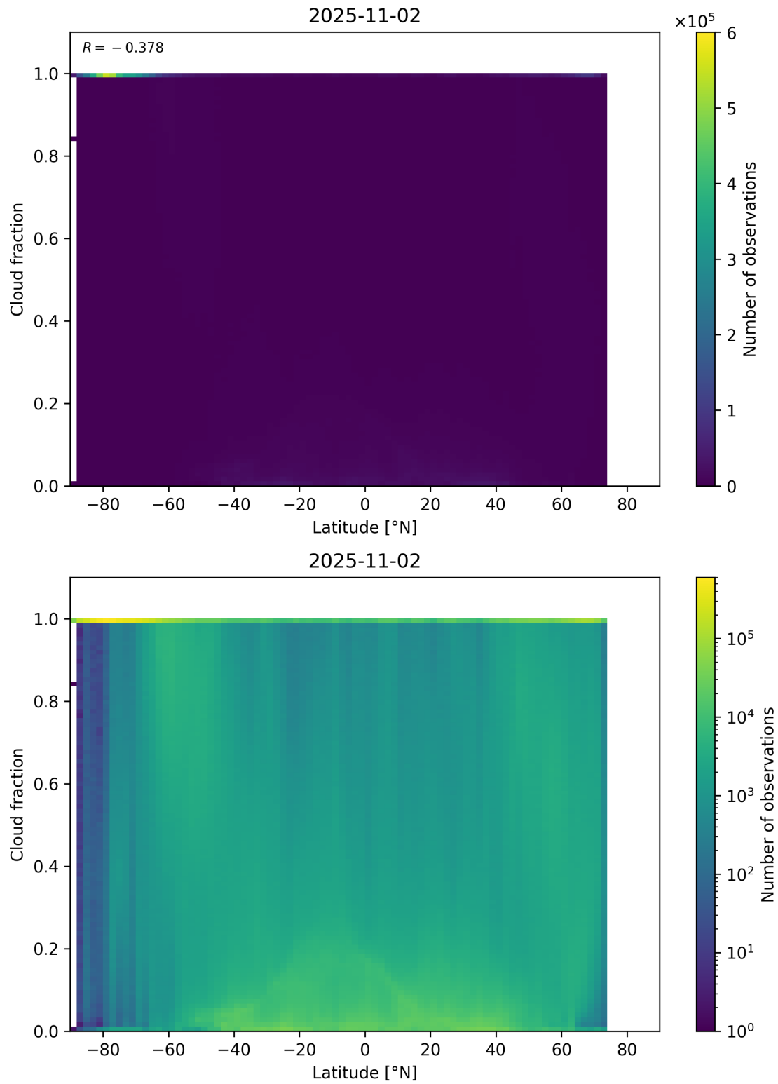
Figure 90: Scatter density plot of “Latitude” against “Cloud fraction” for 2025-11-02 to 2025-11-03.
