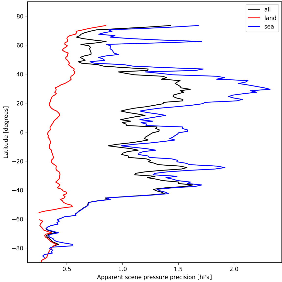
Figure 20: Zonal average of “Apparent scene pressure precision” for 2025-11-02 to 2025-11-03.
