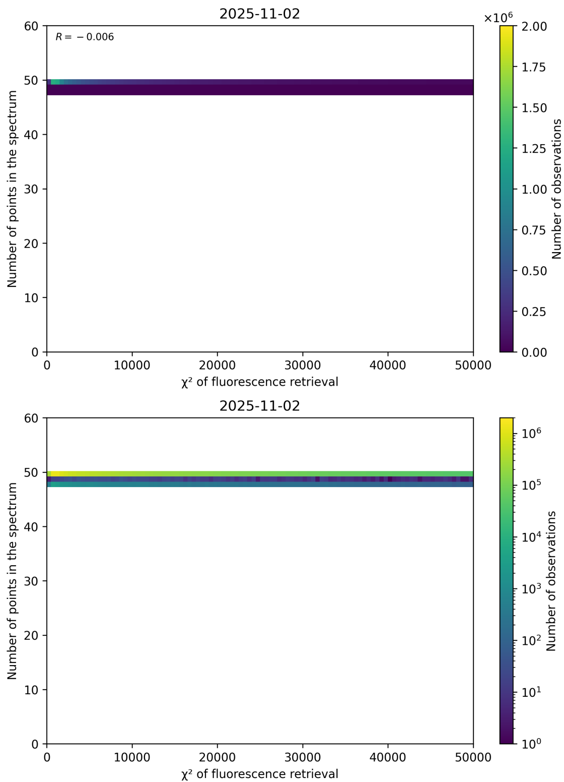
Figure 68: Scatter density plot of “ \chi^2 of fluorescence retrieval” against “Number of points in the spectrum” for 2025-11-02 to 2025-11-03.
