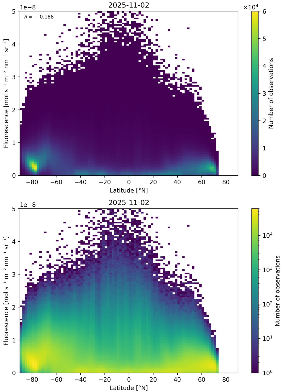
Figure 92: Scatter density plot of “Latitude” against “Fluorescence” for 2025-11-02 to 2025-11-03.
