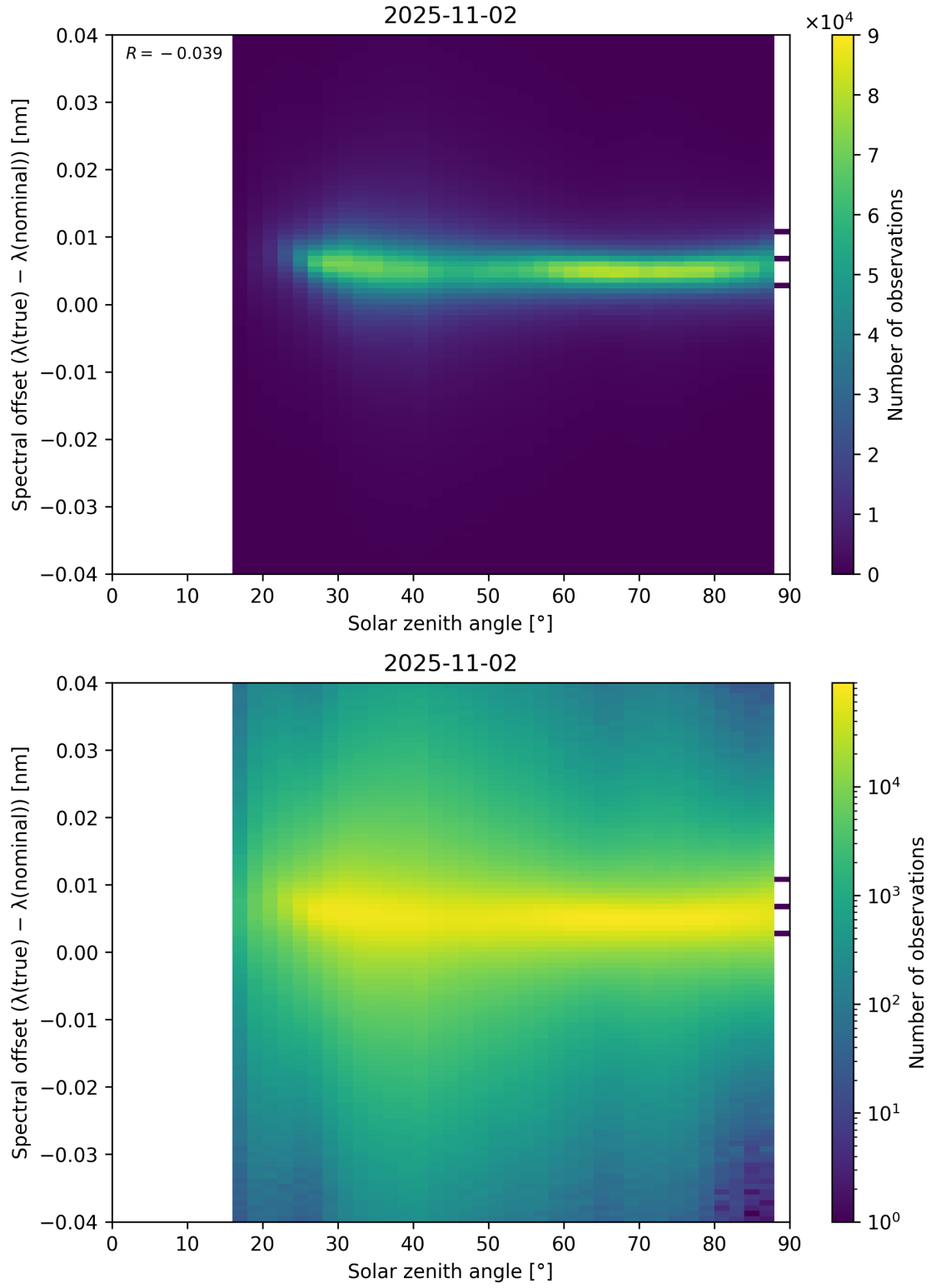
Figure 117: Scatter density plot of “Solar zenith angle” against “Spectral offset ( \lambda_{\text{true}} - \lambda_{\text{nominal}} )” for 2025-11-02 to 2025-11-03.
