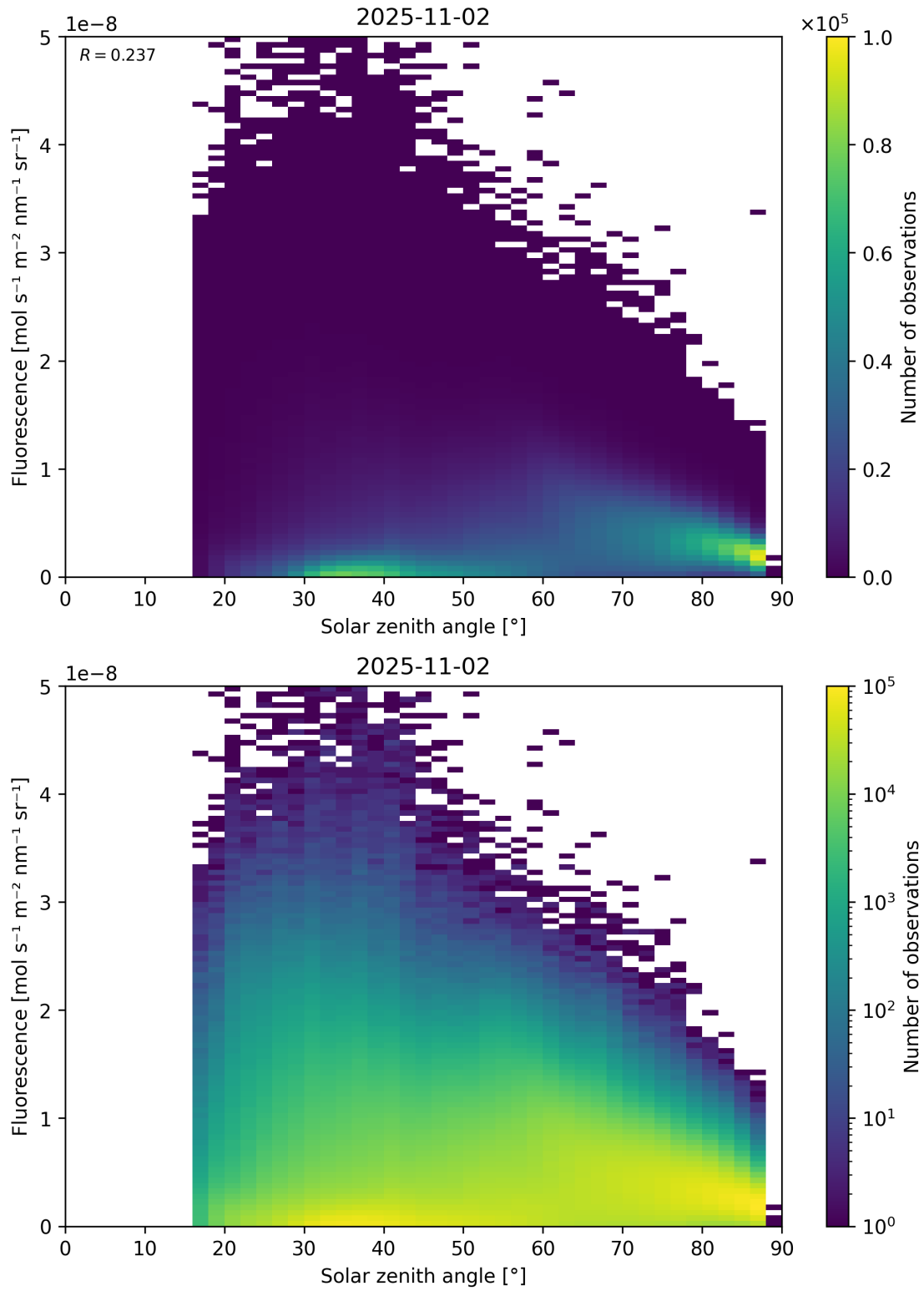
Figure 112: Scatter density plot of “Solar zenith angle” against “Fluorescence” for 2025-11-02 to 2025-11-03.
