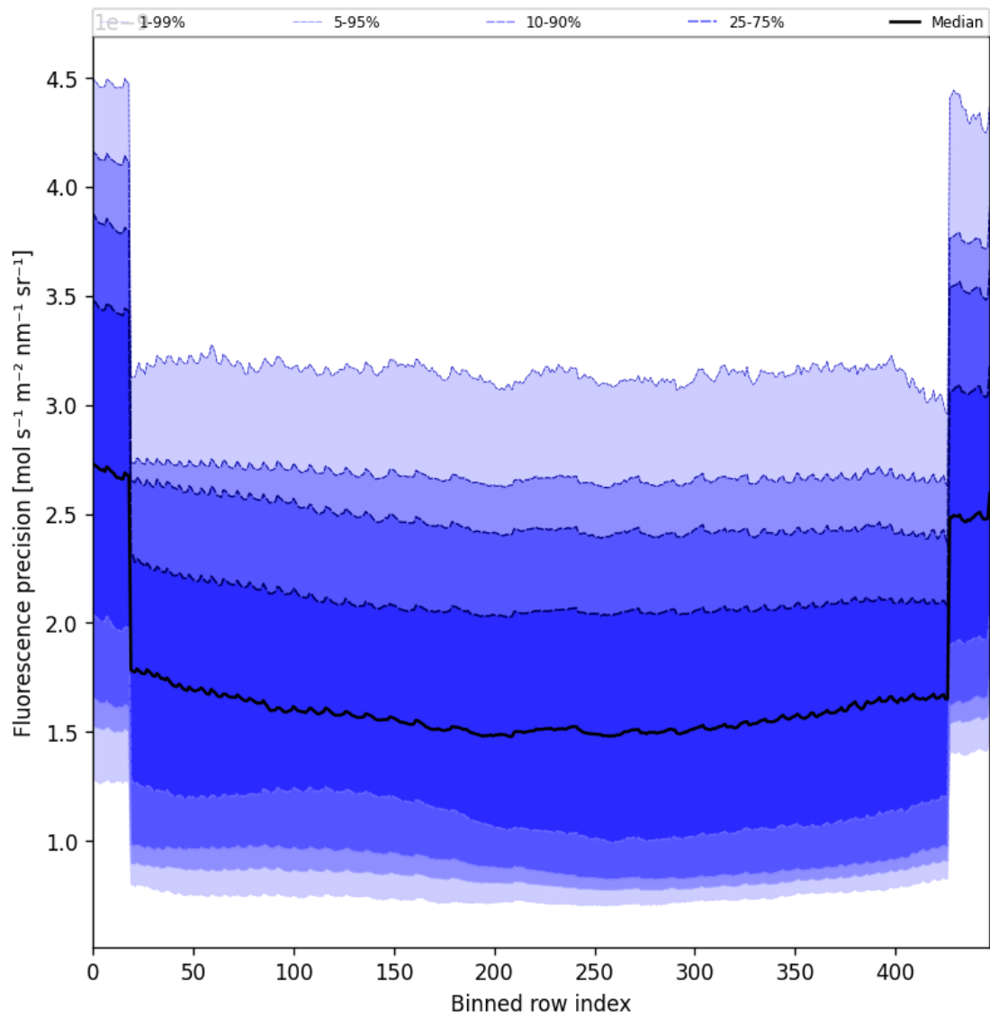
Figure 58: Along track statistics of “Fluorescence precision” for 2025-11-02 to 2025-11-03
