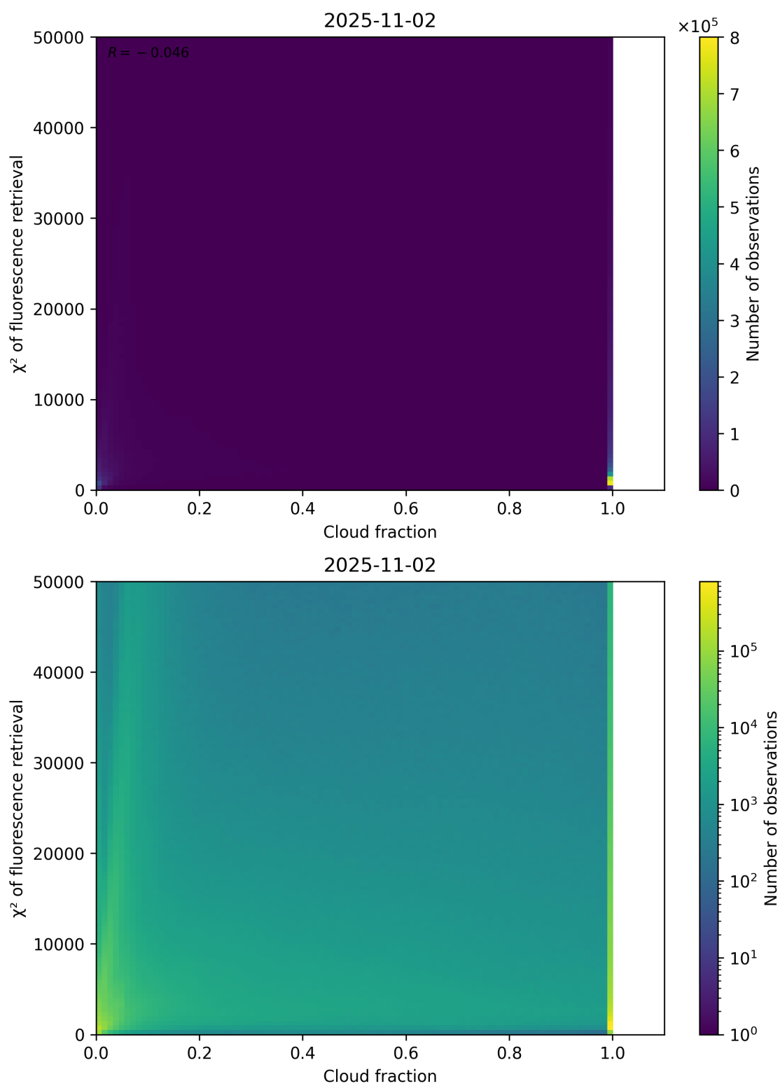
Figure 71: Scatter density plot of “Cloud fraction” against “ \chi^2 of fluorescence retrieval” for 2025-11-02 to 2025-11-03.
