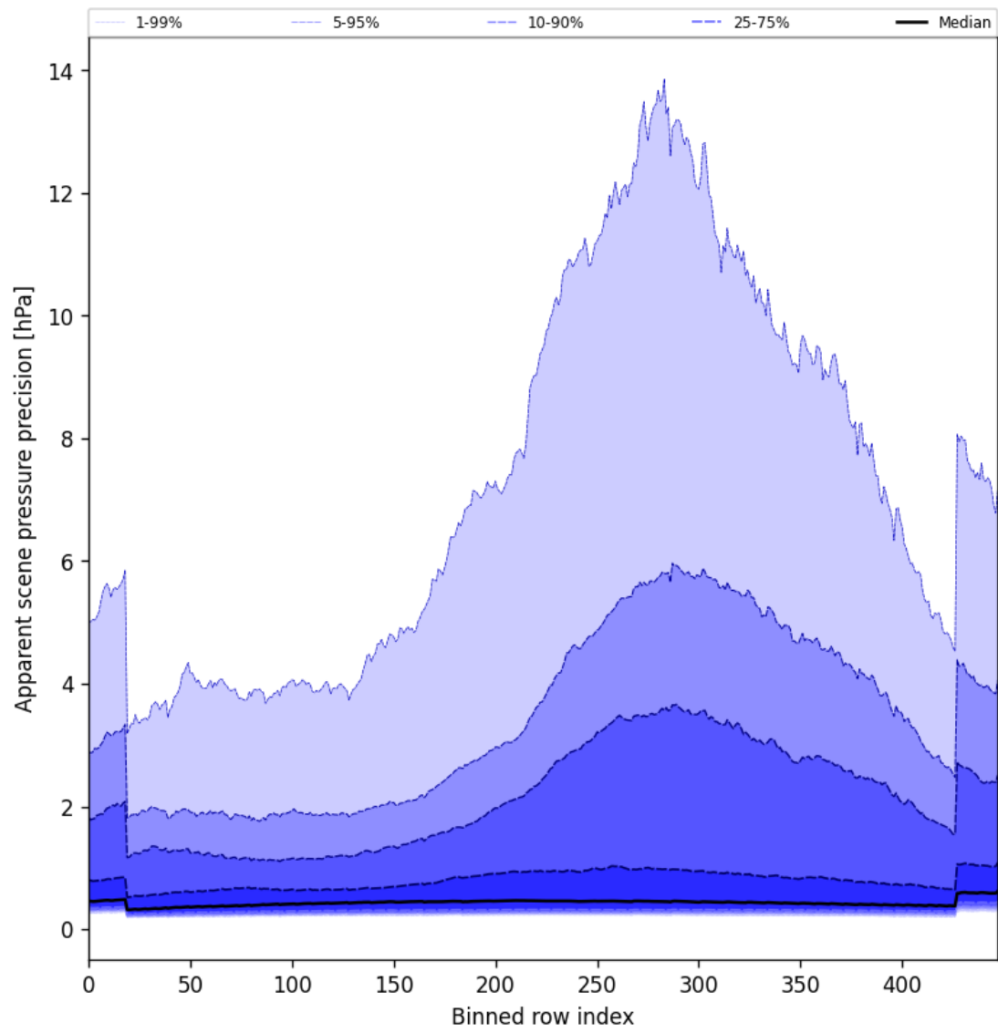
Figure 54: Along track statistics of “Apparent scene pressure precision” for 2025-11-02 to 2025-11-03
