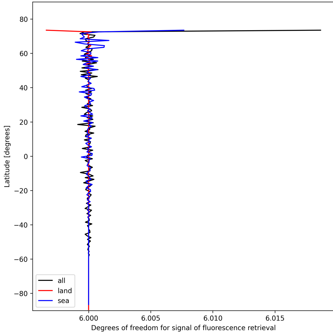
Figure 26: Zonal average of “Degrees of freedom for signal of fluorescence retrieval” for 2025-11-02 to 2025-11-03.
