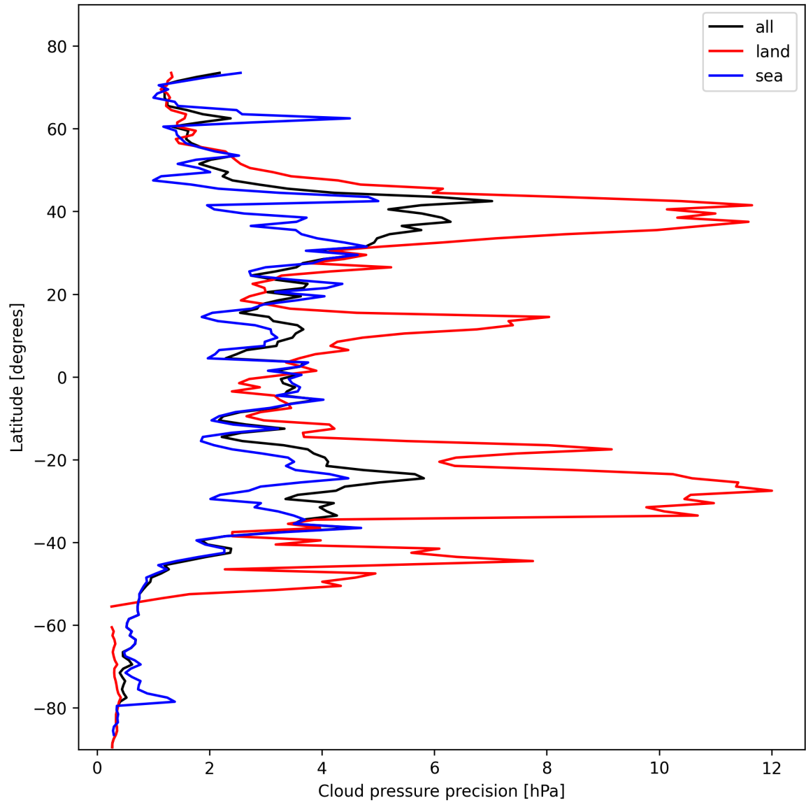
Figure 14: Zonal average of “Cloud pressure precision” for 2025-11-02 to 2025-11-03.
