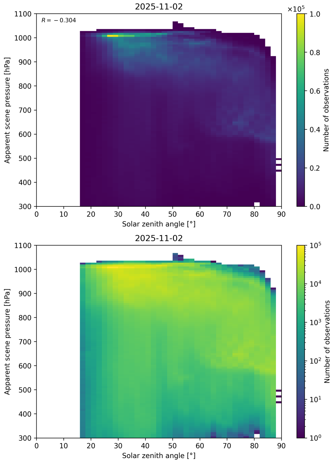
Figure 108: Scatter density plot of “Solar zenith angle” against “Apparent scene pressure” for 2025-11-02 to 2025-11-03.
