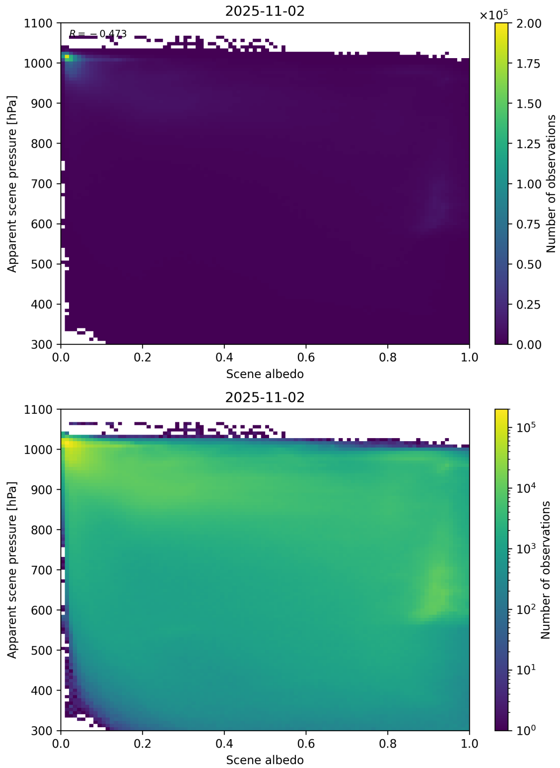
Figure 102: Scatter density plot of “Scene albedo” against “Apparent scene pressure” for 2025-11-02 to 2025-11-03.
