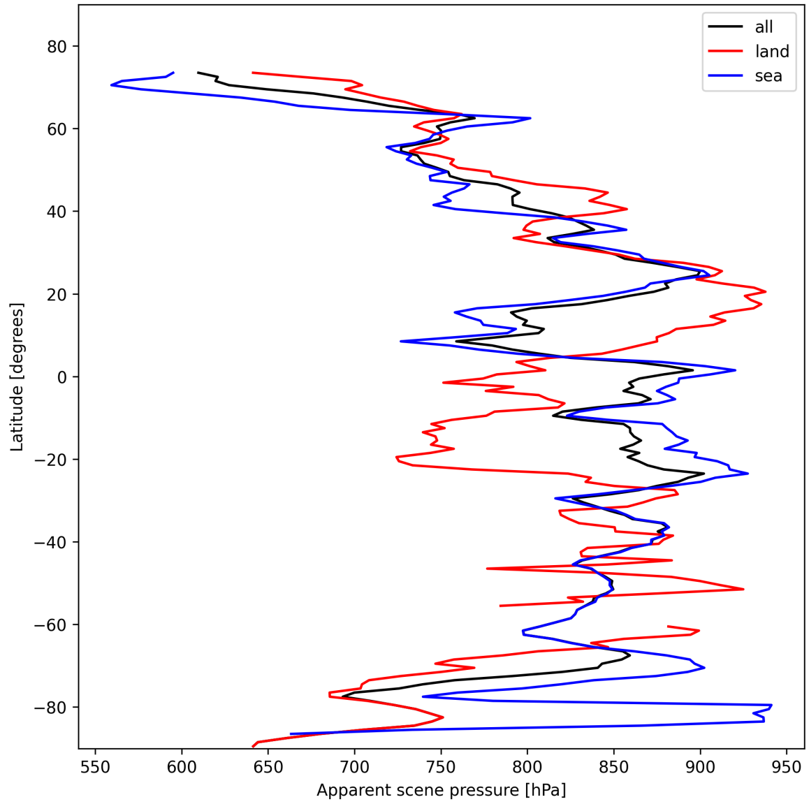
Figure 19: Zonal average of “Apparent scene pressure” for 2025-11-02 to 2025-11-03.
