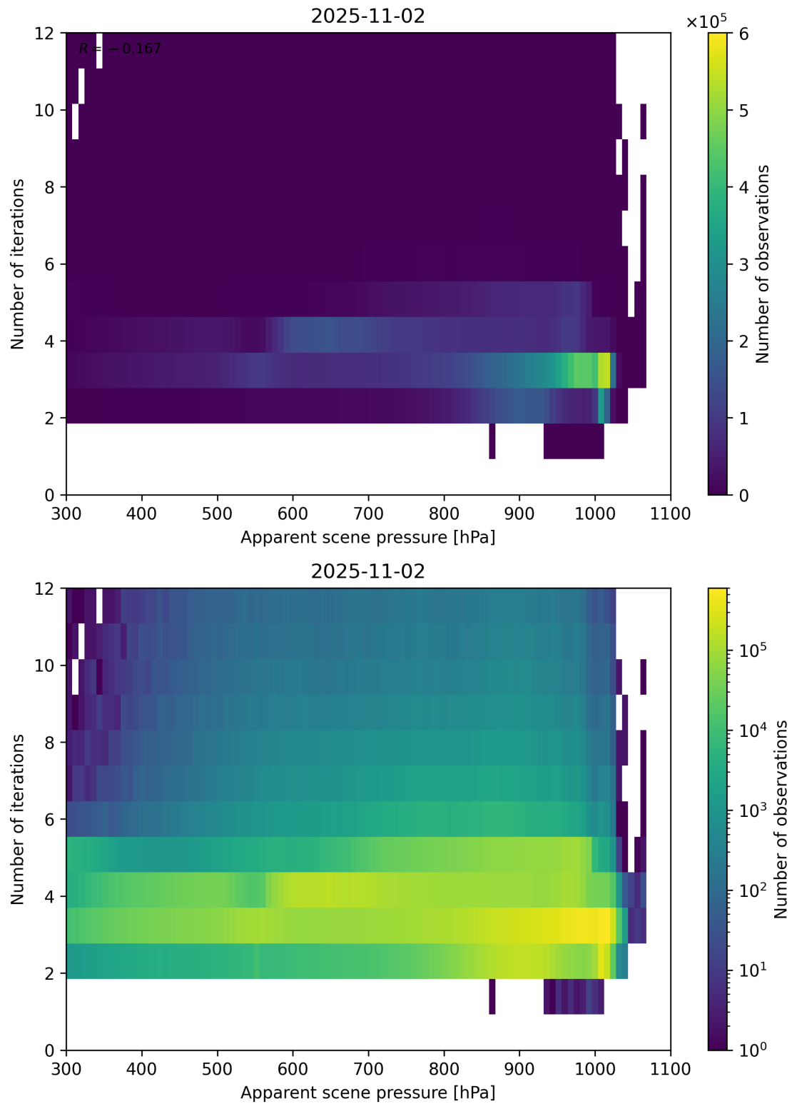
Figure 65: Scatter density plot of “Apparent scene pressure” against “Number of iterations” for 2025-11-02 to 2025-11-03.
