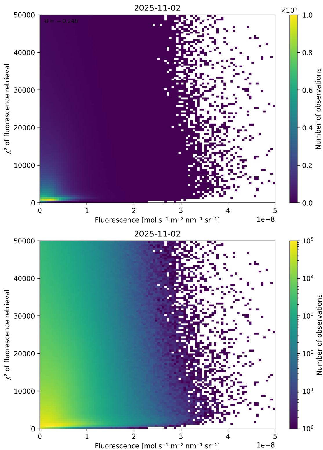
Figure 85: Scatter density plot of “Fluorescence” against “ \chi^2 of fluorescence retrieval” for 2025-11-02 to 2025-11-03.
