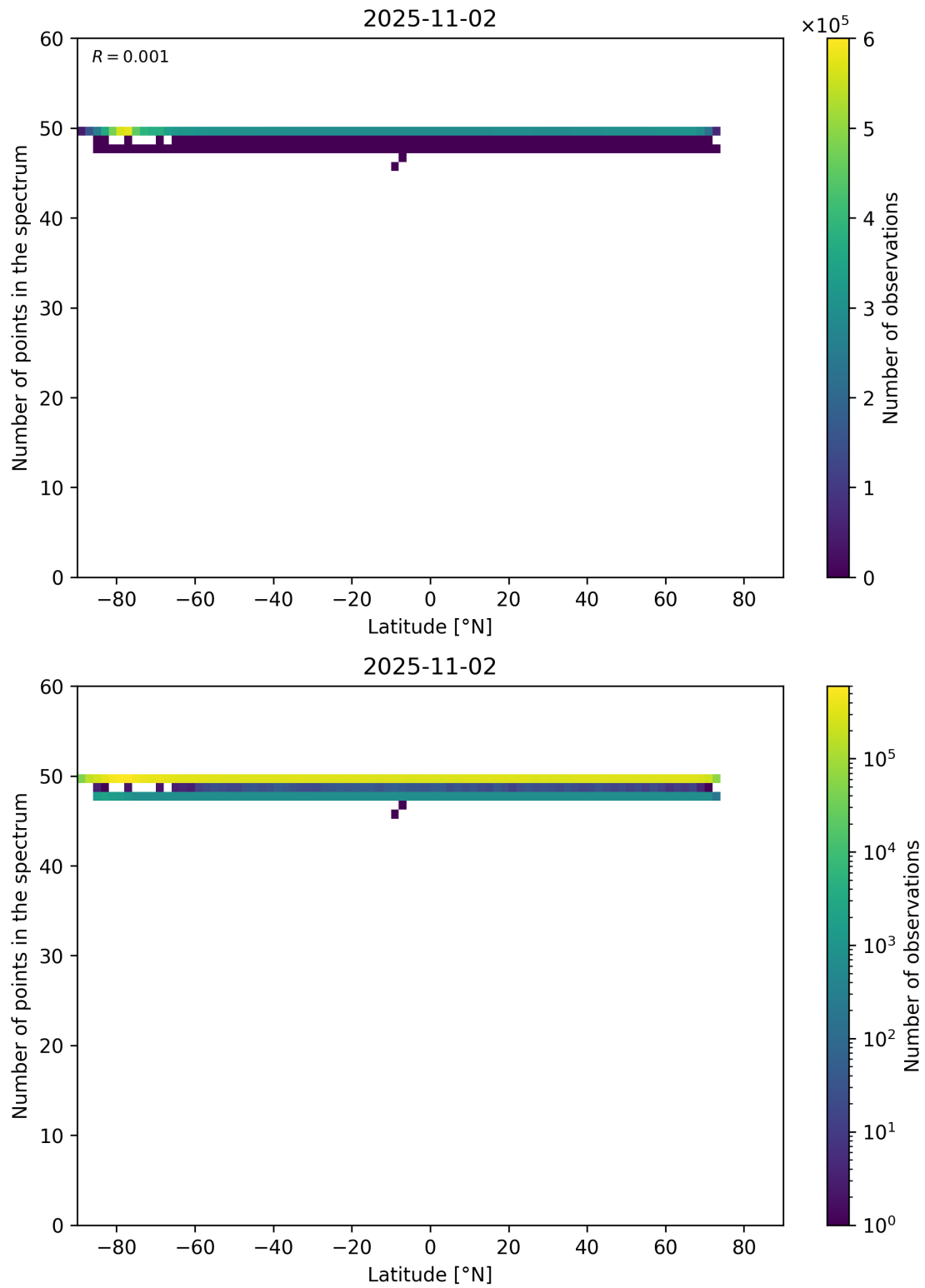
Figure 94: Scatter density plot of “Latitude” against “Number of points in the spectrum” for 2025-11-02 to 2025-11-03.
