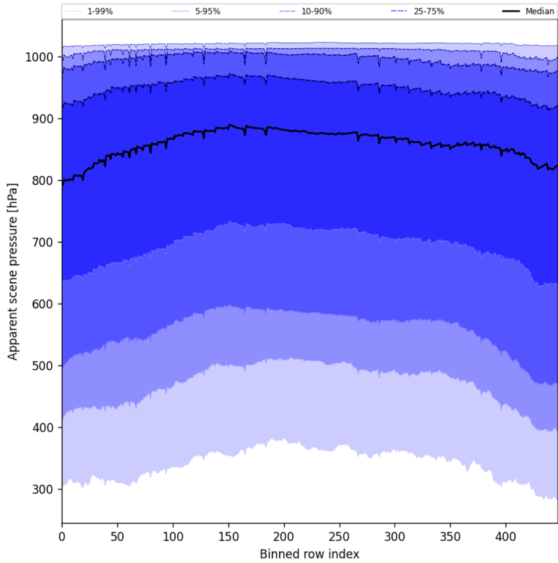
Figure 53: Along track statistics of “Apparent scene pressure” for 2025-11-02 to 2025-11-03
