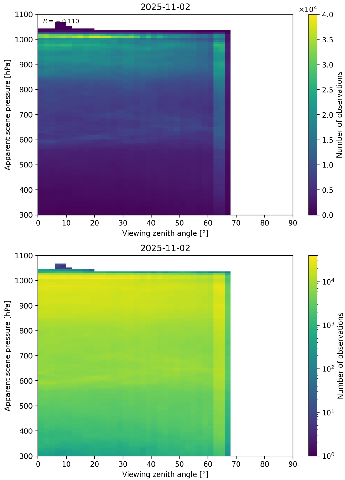
Figure 118: Scatter density plot of “Viewing zenith angle” against “Apparent scene pressure” for 2025-11-02 to 2025-11-03.
