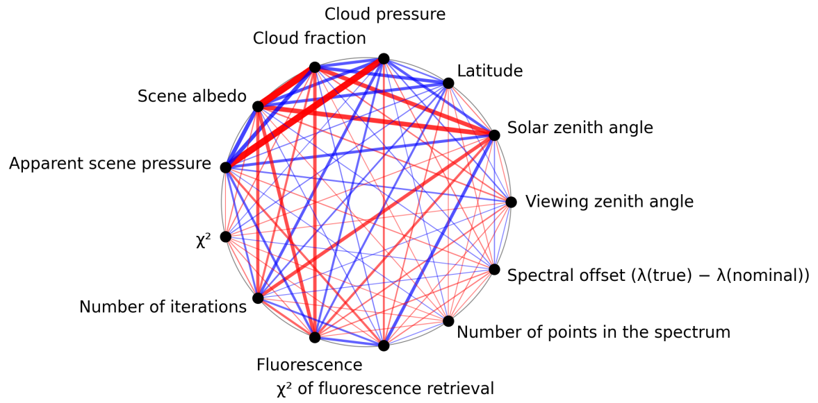
Figure 1: Map of correlation graph for 2025-11-02 to 2025-11-03.
