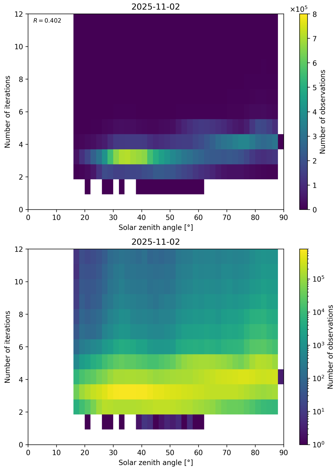
Figure 114: Scatter density plot of “Solar zenith angle” against “Number of iterations” for 2025-11-02 to 2025-11-03.
