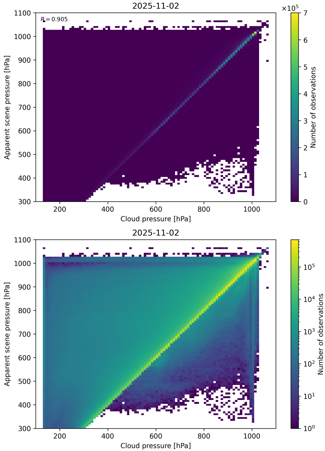
Figure 77: Scatter density plot of “Cloud pressure” against “Apparent scene pressure” for 2025-11-02 to 2025-11-03.
