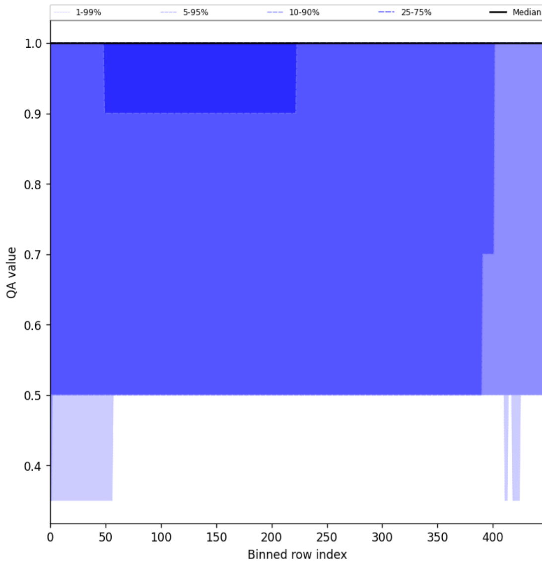
Figure 46: Along track statistics of “QA value” for 2025-11-02 to 2025-11-03
