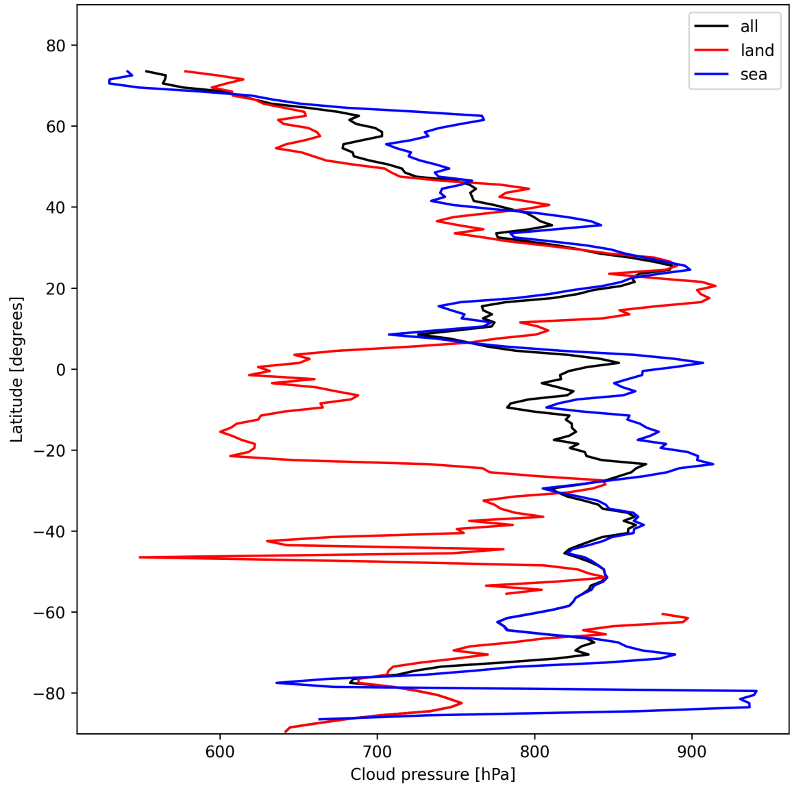
Figure 13: Zonal average of “Cloud pressure” for 2025-11-02 to 2025-11-03.
