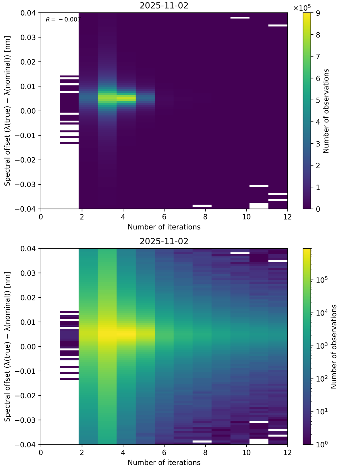
Figure 100: Scatter density plot of “Number of iterations” against “Spectral offset ( \lambda_{\text{true}} - \lambda_{\text{nominal}} )” for 2025-11-02 to 2025-11-03.
