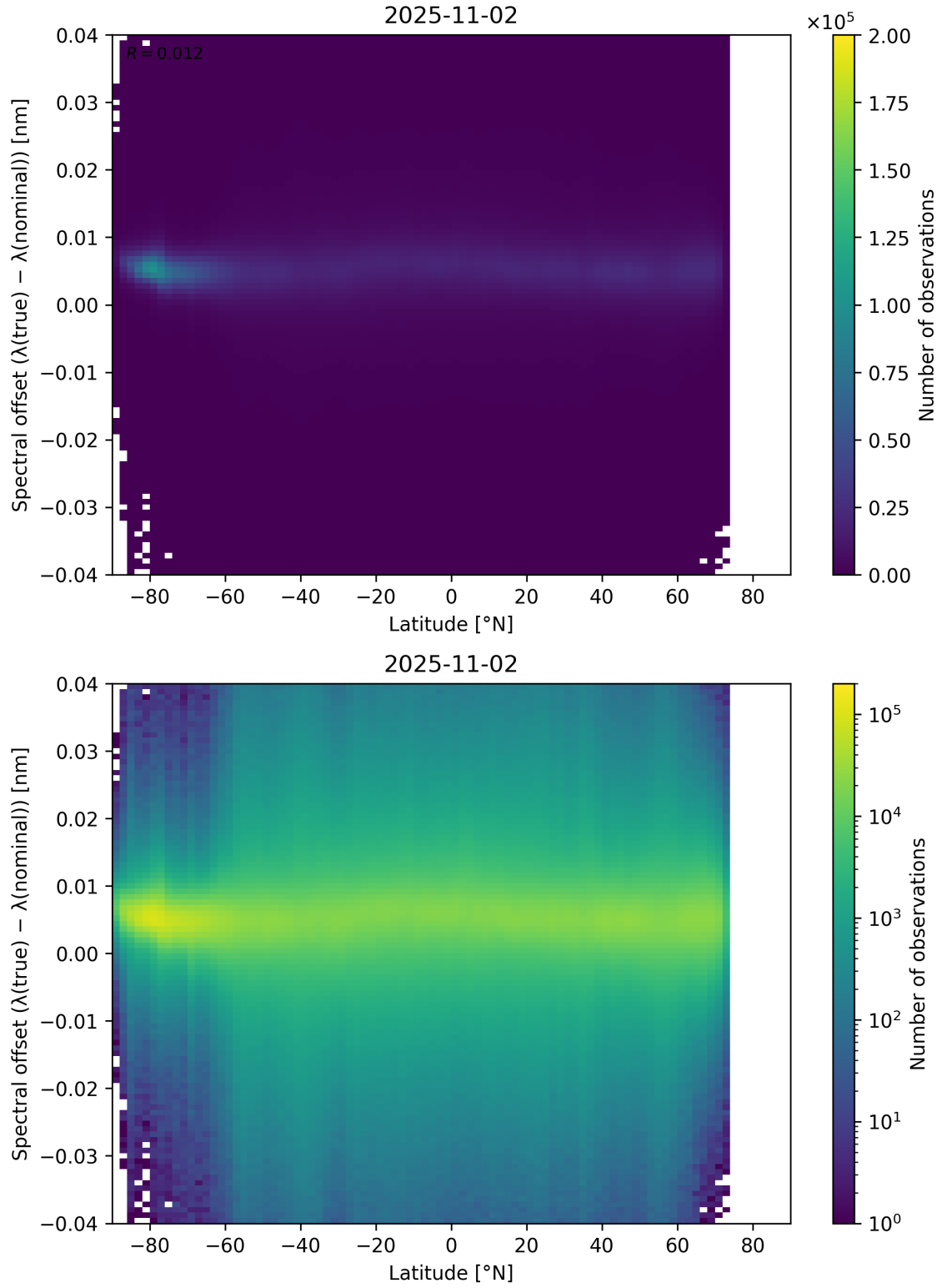
Figure 96: Scatter density plot of “Latitude” against “Spectral offset ( \lambda_{\text{true}} - \lambda_{\text{nominal}} )” for 2025-11-02 to 2025-11-03.
