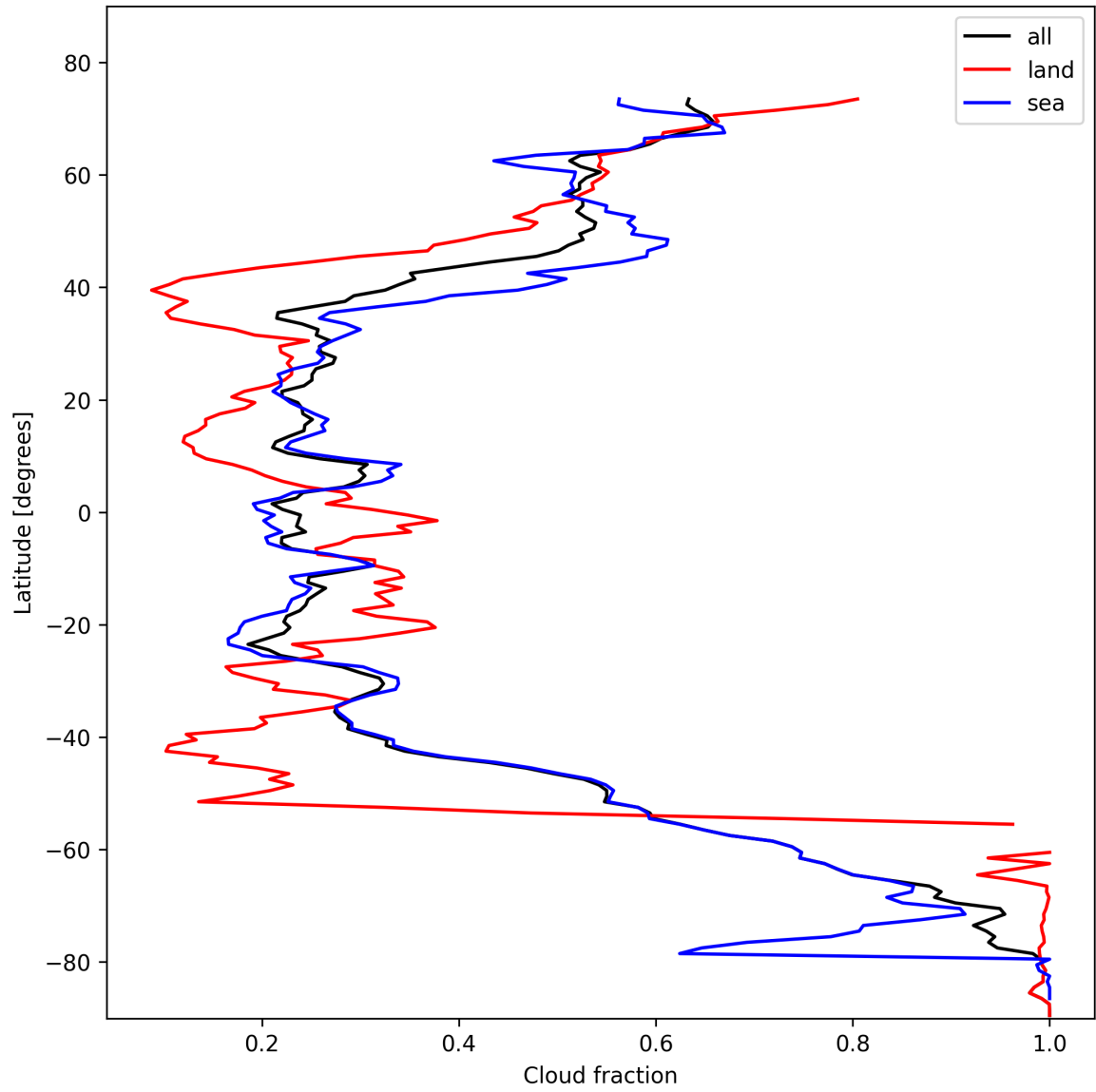
Figure 15: Zonal average of “Cloud fraction” for 2025-11-02 to 2025-11-03.
