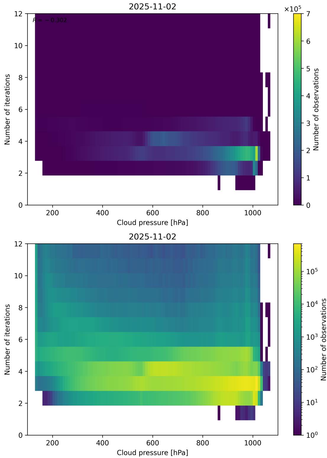
Figure 81: Scatter density plot of “Cloud pressure” against “Number of iterations” for 2025-11-02 to 2025-11-03.
