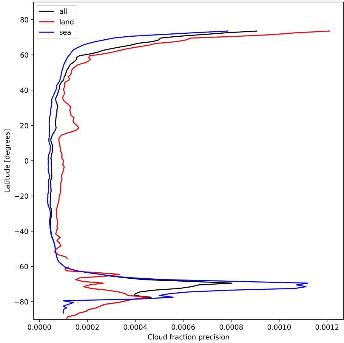
Figure 16: Zonal average of “Cloud fraction precision” for 2025-11-02 to 2025-11-03.
