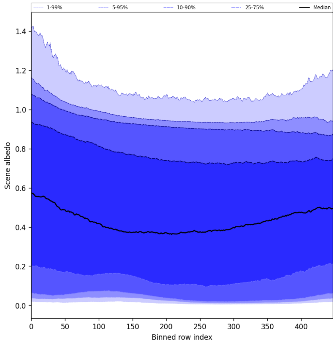
Figure 51: Along track statistics of “Scene albedo” for 2025-11-02 to 2025-11-03
