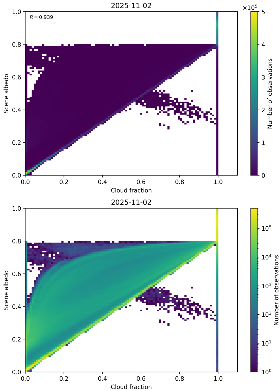
Figure 75: Scatter density plot of “Cloud fraction” against “Scene albedo” for 2025-11-02 to 2025-11-03.
