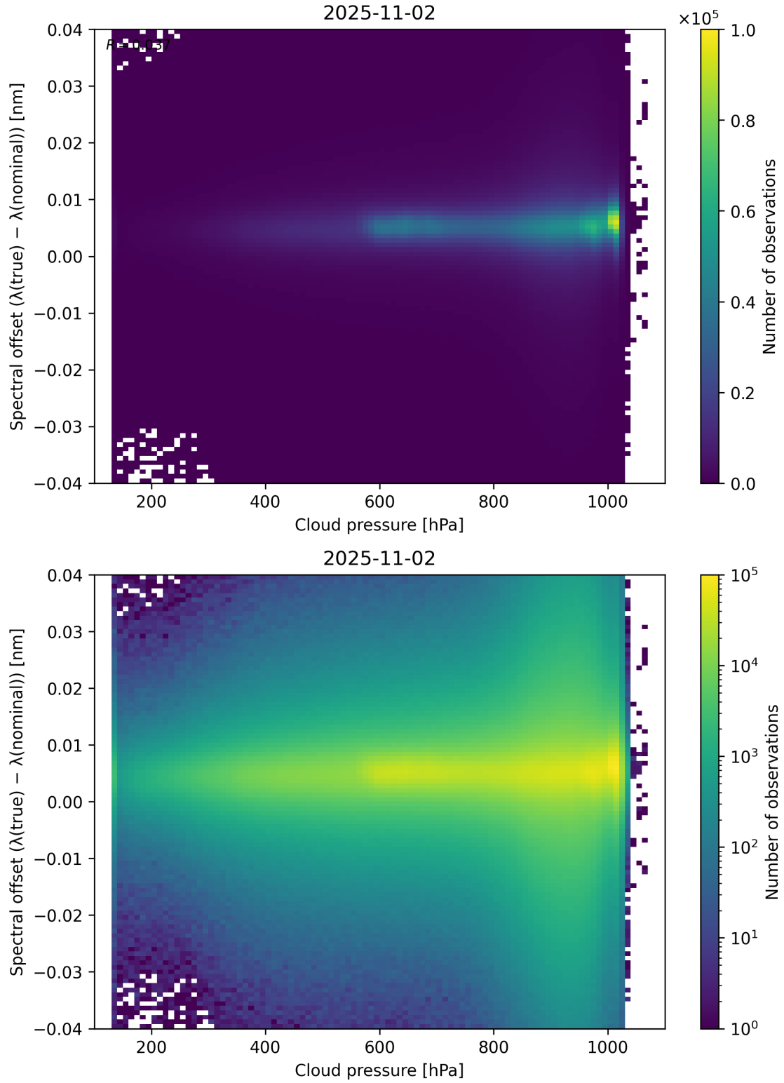
Figure 84: Scatter density plot of “Cloud pressure” against “Spectral offset ( \lambda_{\text{true}} - \lambda_{\text{nominal}} )” for 2025-11-02 to 2025-11-03.
