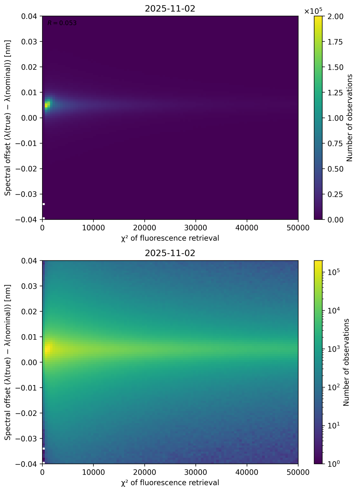
Figure 69: Scatter density plot of “ \chi^2 of fluorescence retrieval” against “Spectral offset ( \lambda_{\text{true}} - \lambda_{\text{nominal}} )” for 2025-11-02 to 2025-11-03.
