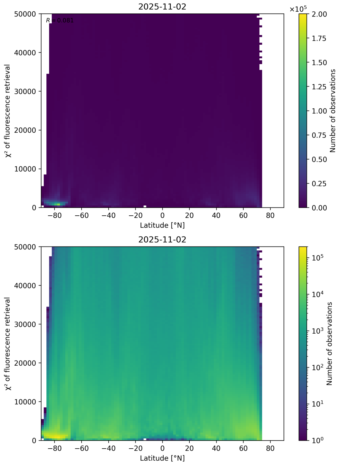
Figure 89: Scatter density plot of “Latitude” against “ \chi^2 of fluorescence retrieval” for 2025-11-02 to 2025-11-03.
