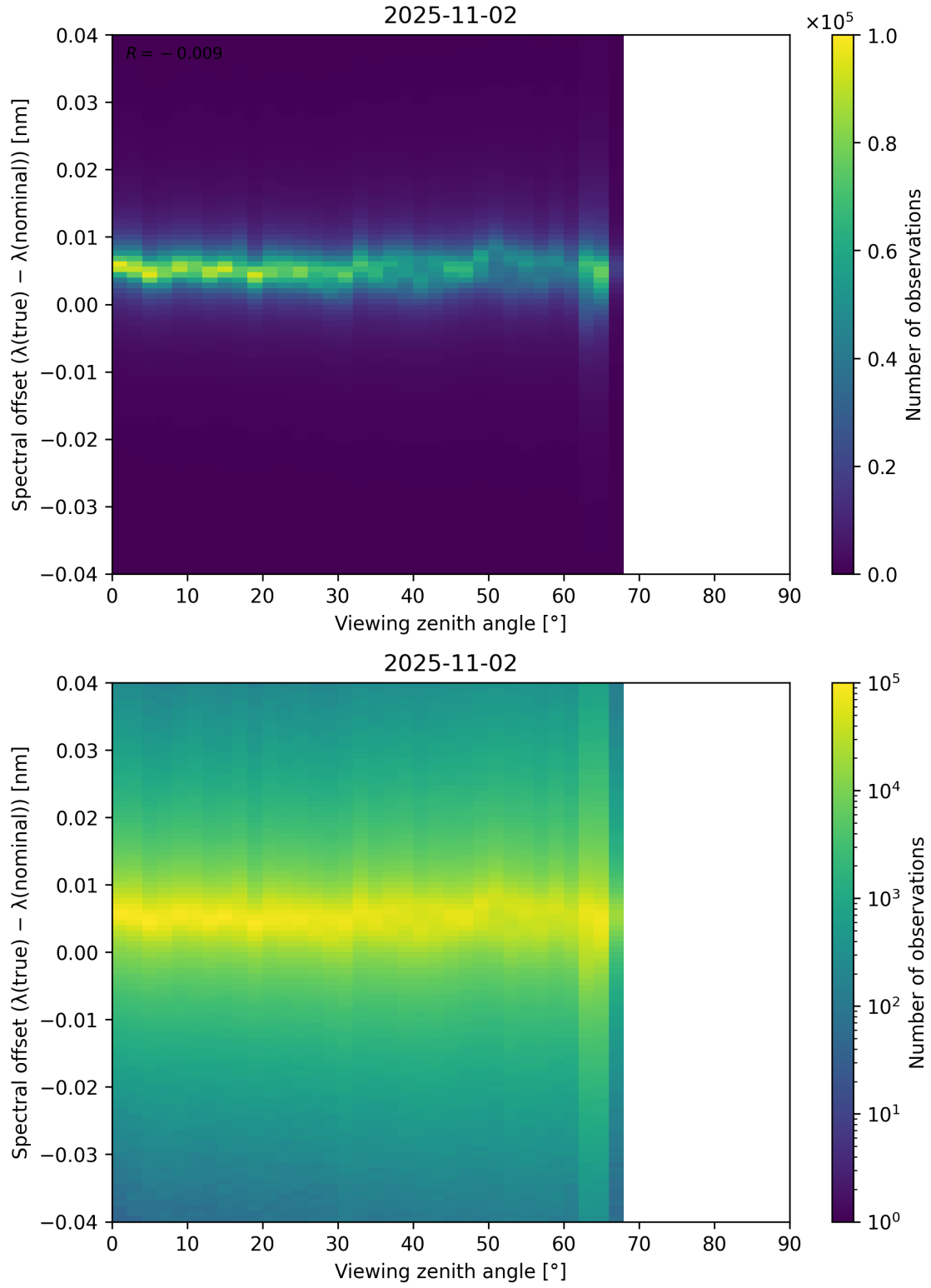
Figure 128: Scatter density plot of “Viewing zenith angle” against “Spectral offset ( \lambda_{\text{true}} - \lambda_{\text{nominal}} )” for 2025-11-02 to 2025-11-03.
