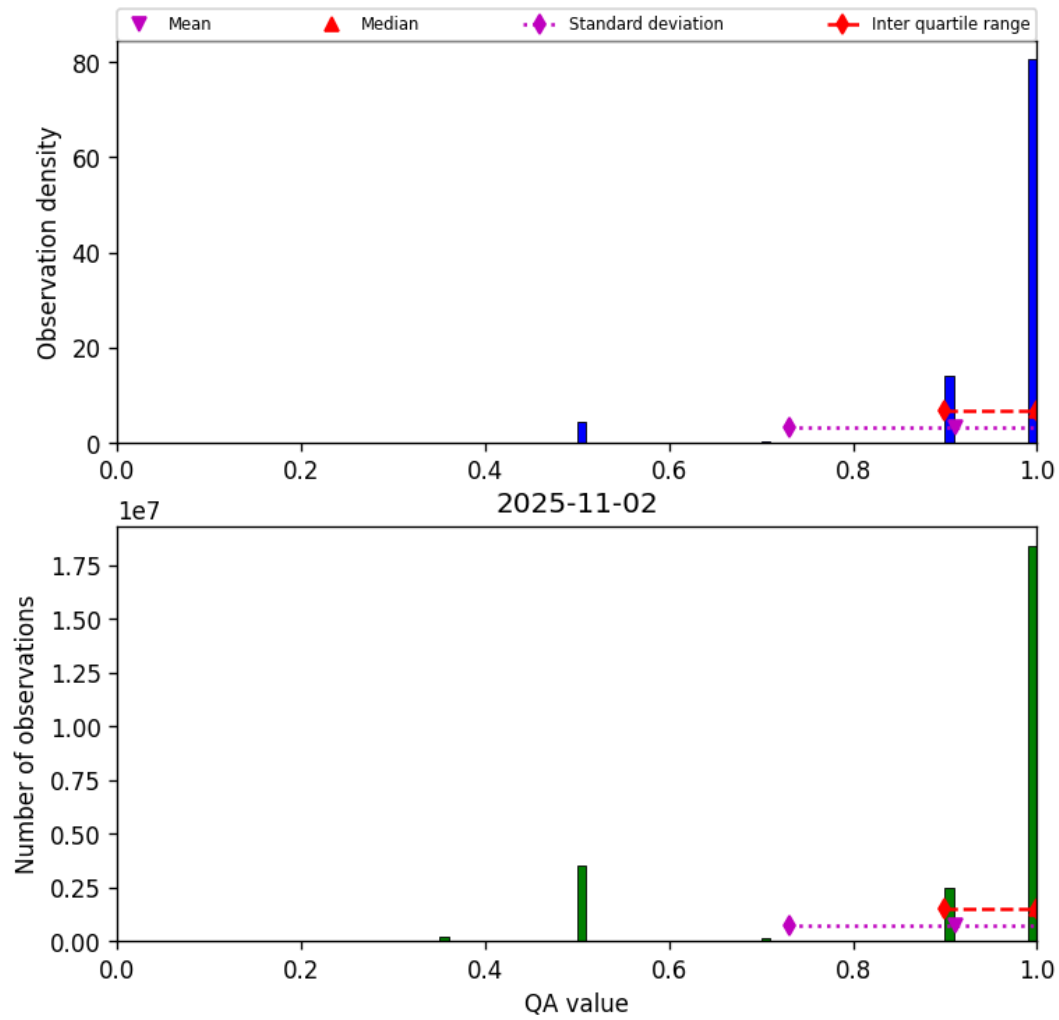
Figure 29: Histogram of “QA value” for 2025-11-02 to 2025-11-03
