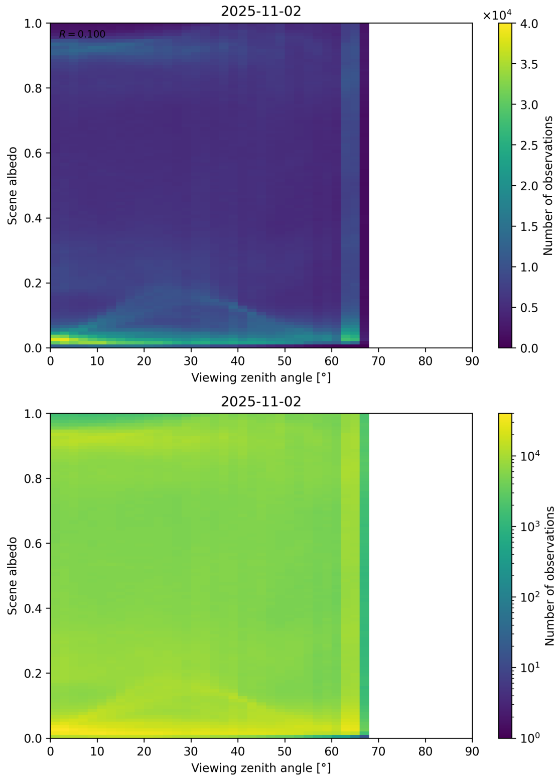
Figure 126: Scatter density plot of “Viewing zenith angle” against “Scene albedo” for 2025-11-02 to 2025-11-03.
