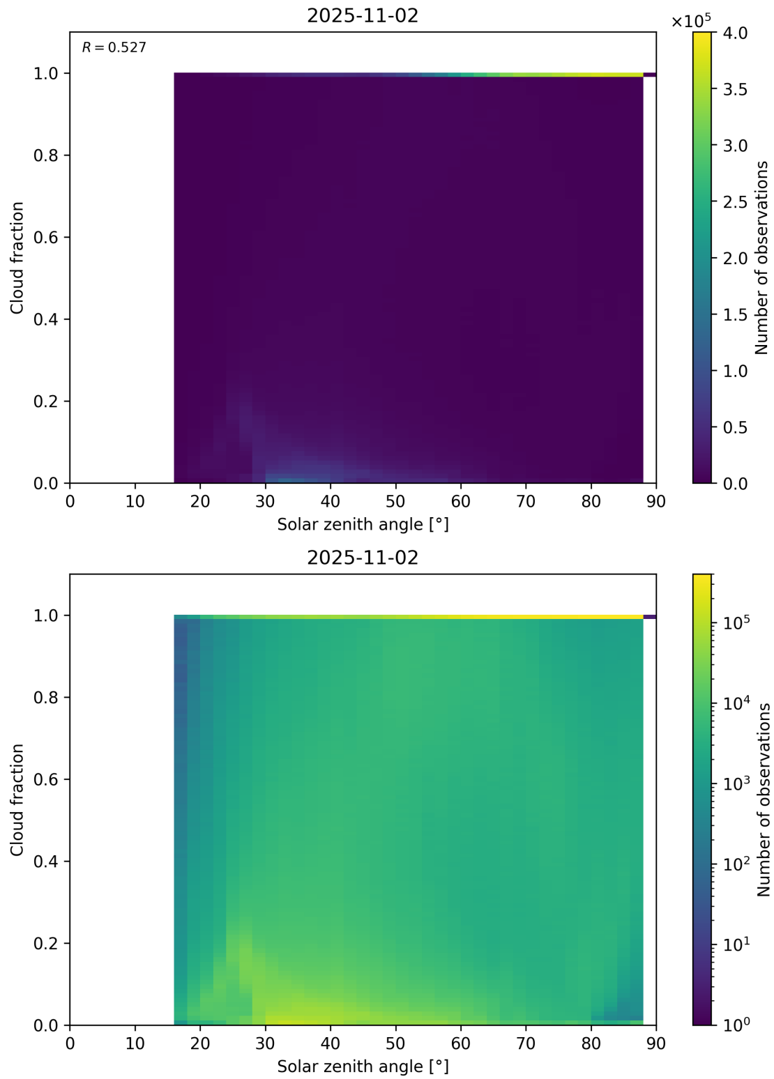
Figure 110: Scatter density plot of “Solar zenith angle” against “Cloud fraction” for 2025-11-02 to 2025-11-03.
