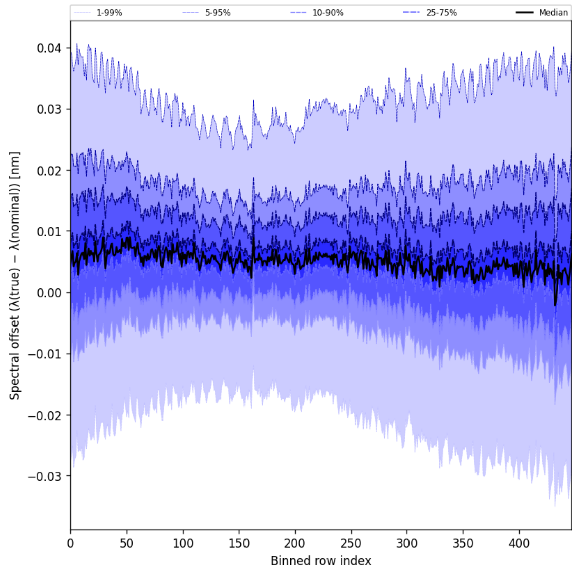
Figure 62: Along track statistics of “Spectral offset ( \lambda_{\text{true}} - \lambda_{\text{nominal}} )” for 2025-11-02 to 2025-11-03
