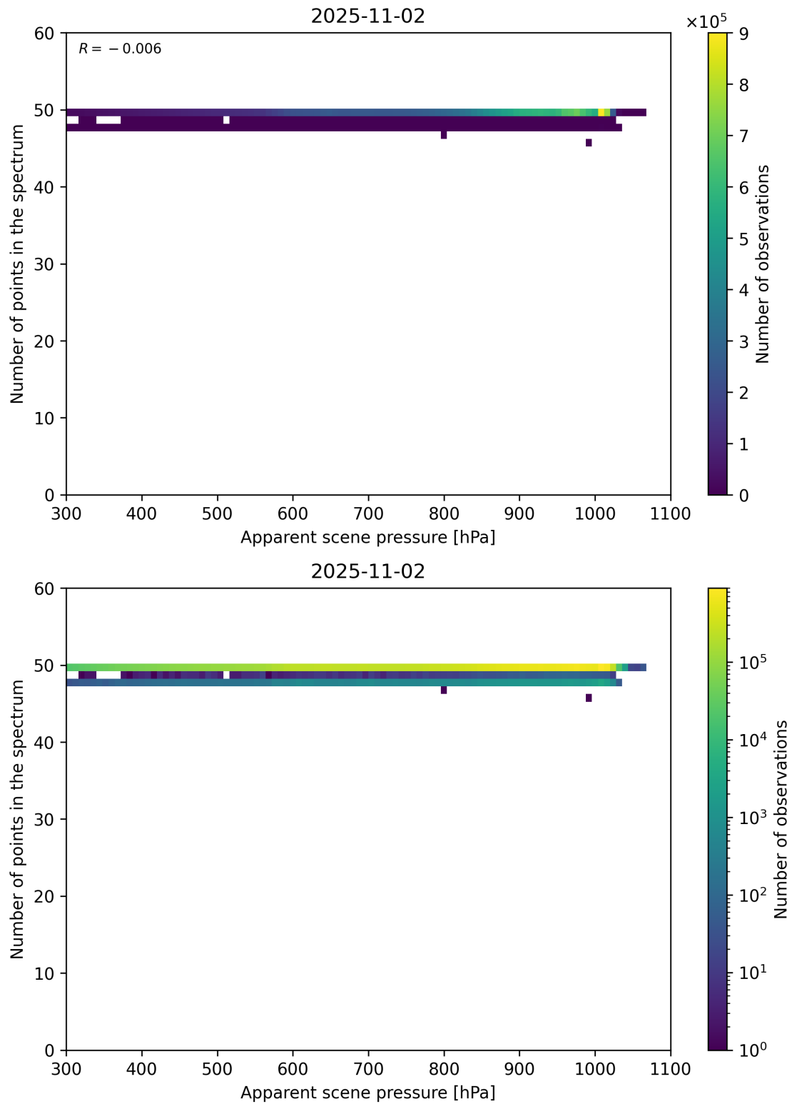
Figure 66: Scatter density plot of “Apparent scene pressure” against “Number of points in the spectrum” for 2025-11-02 to 2025-11-03.
