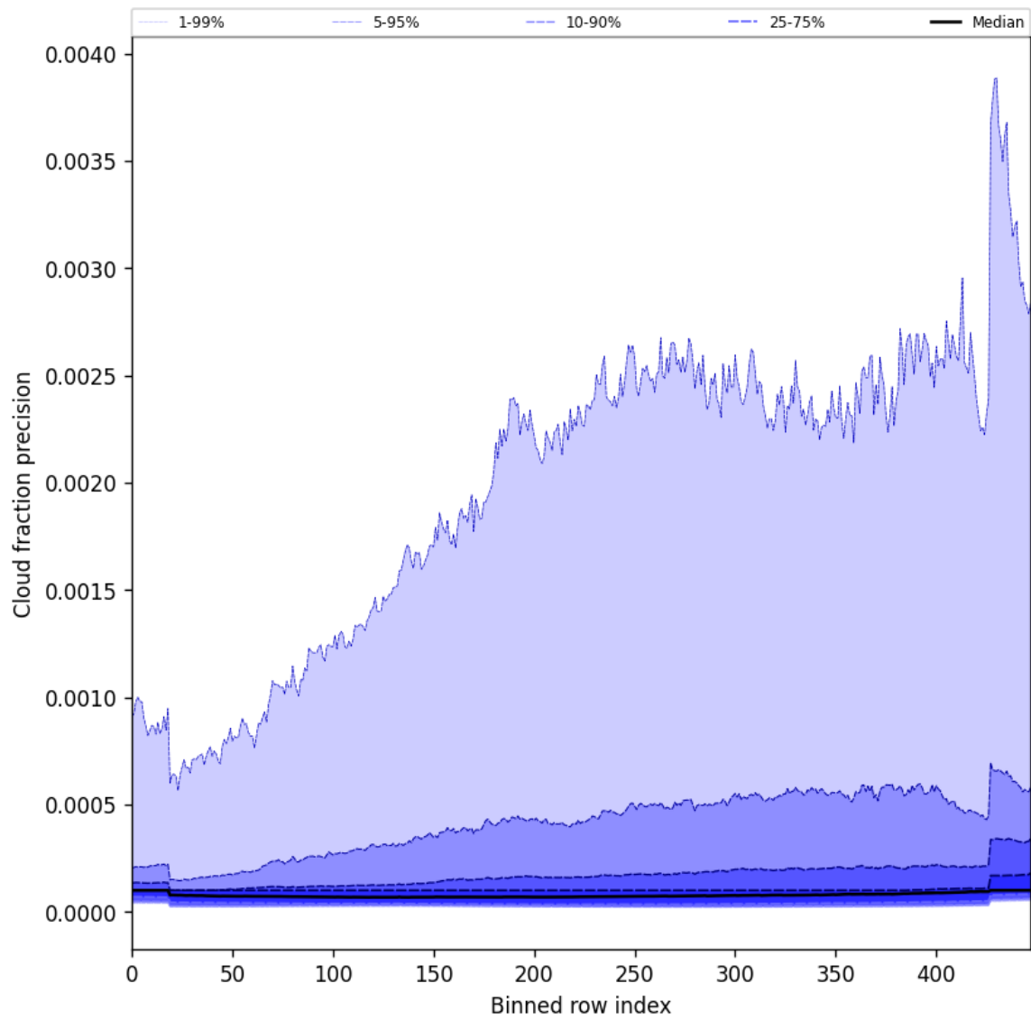
Figure 50: Along track statistics of “Cloud fraction precision” for 2025-11-02 to 2025-11-03
