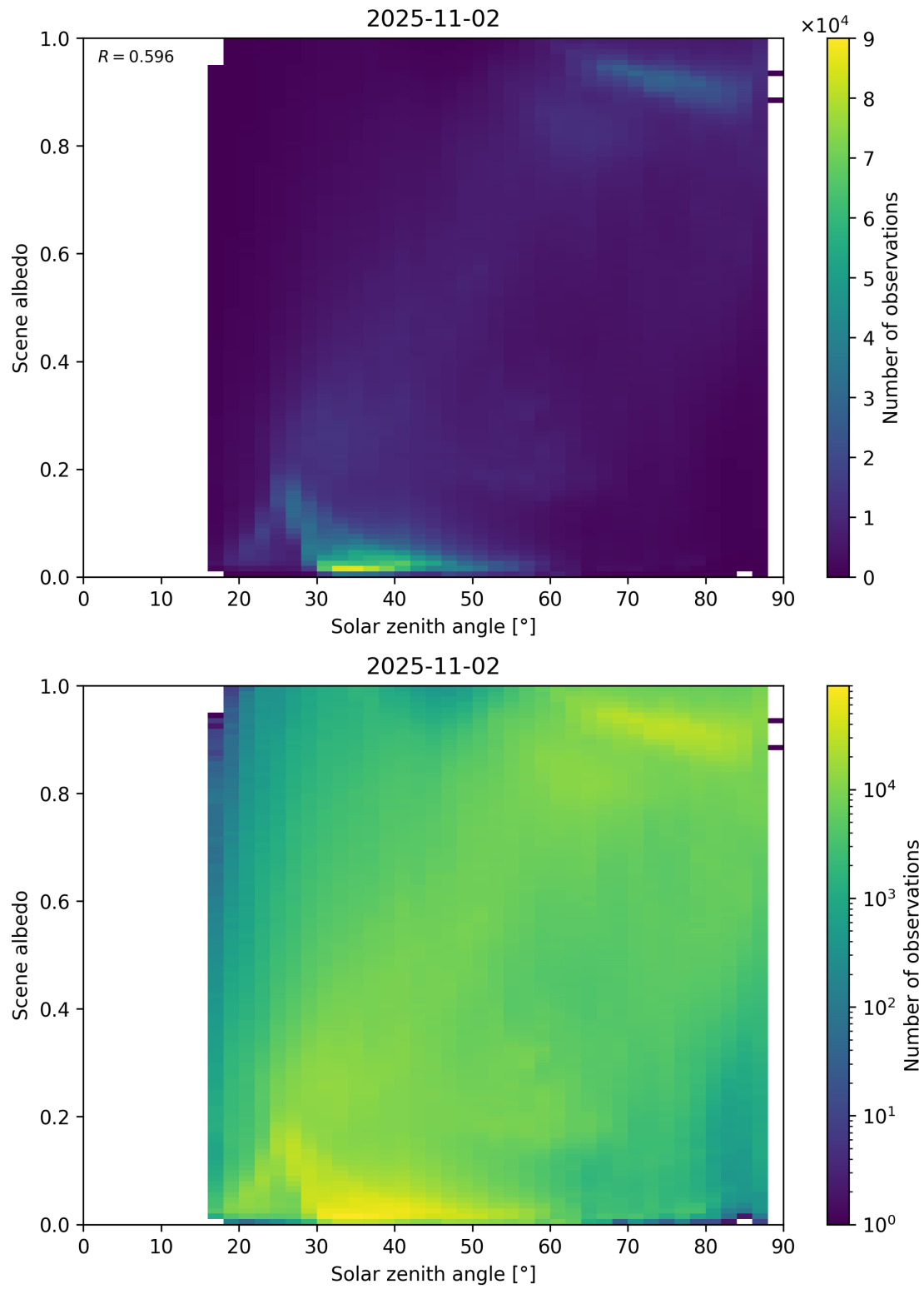
Figure 116: Scatter density plot of “Solar zenith angle” against “Scene albedo” for 2025-11-02 to 2025-11-03.
