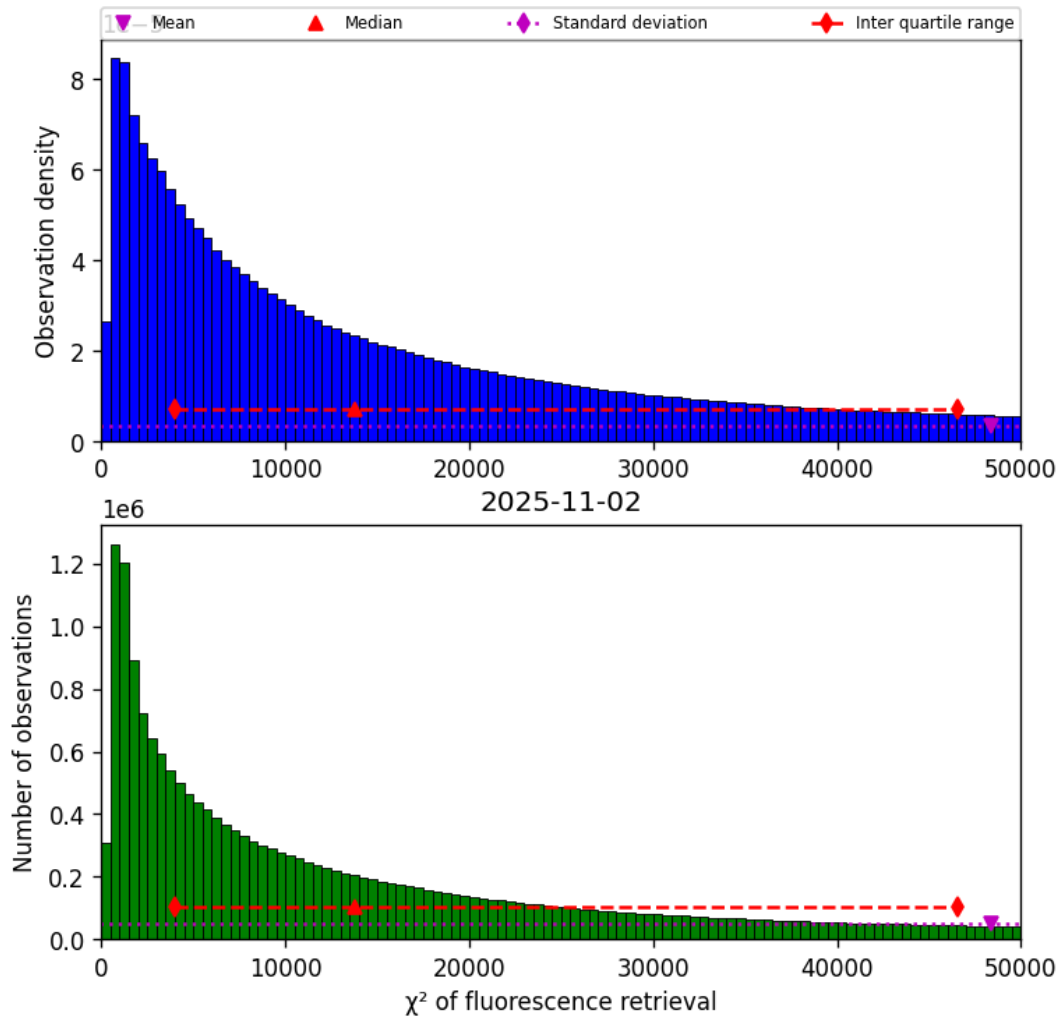
Figure 42: Histogram of “ \chi^2 of fluorescence retrieval” for 2025-11-02 to 2025-11-03
