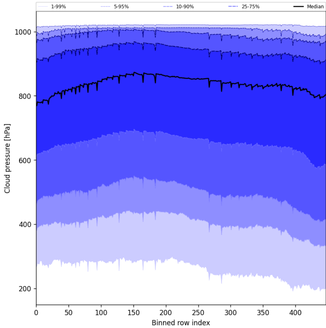
Figure 47: Along track statistics of “Cloud pressure” for 2025-11-02 to 2025-11-03
