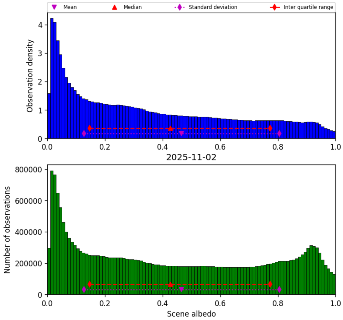
Figure 34: Histogram of “Scene albedo” for 2025-11-02 to 2025-11-03
