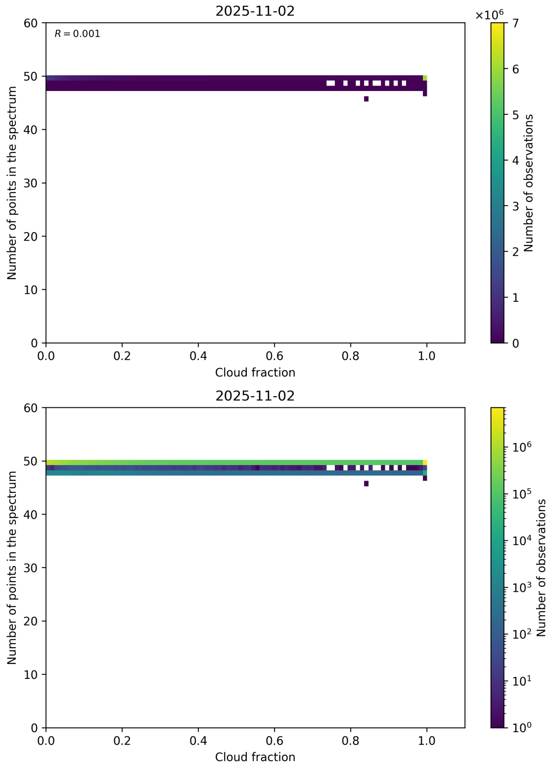
Figure 74: Scatter density plot of “Cloud fraction” against “Number of points in the spectrum” for 2025-11-02 to 2025-11-03.
