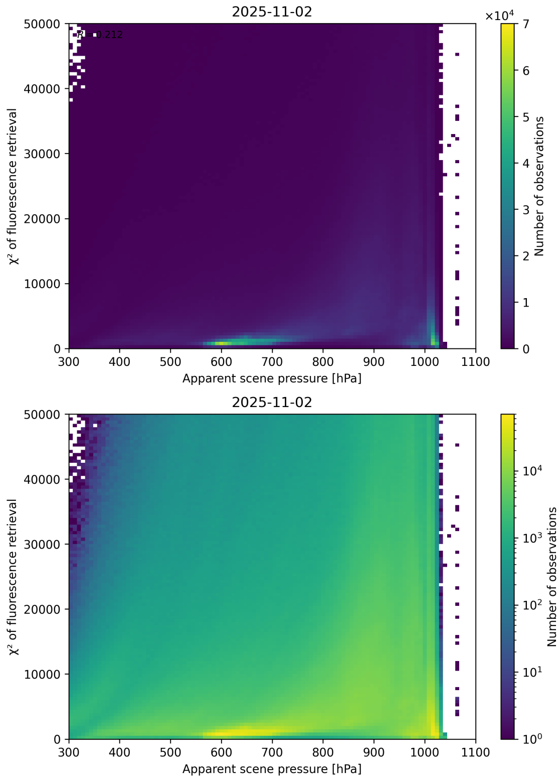
Figure 63: Scatter density plot of “Apparent scene pressure” against “ \chi^2 of fluorescence retrieval” for 2025-11-02 to 2025-11-03.
