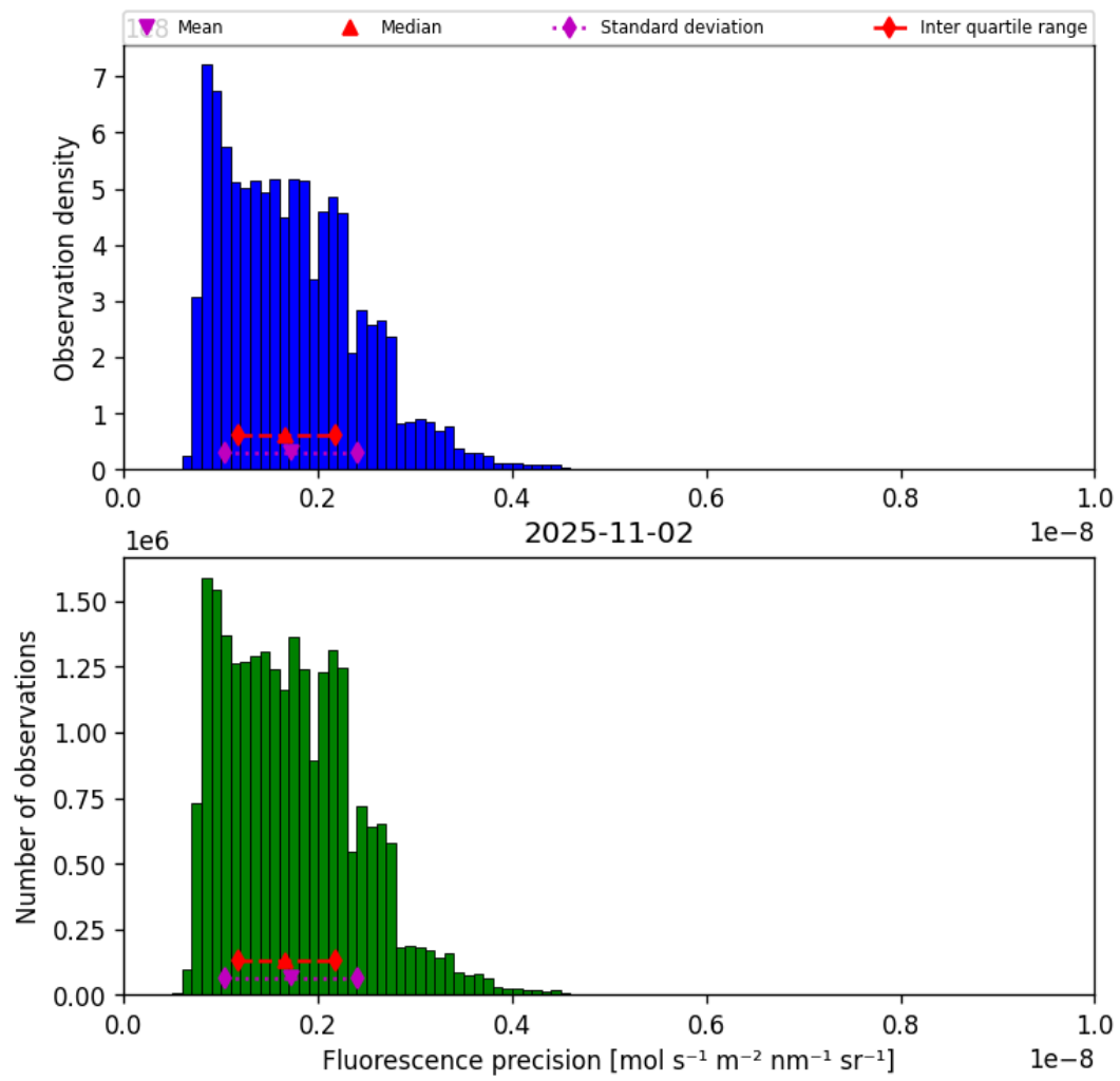
Figure 41: Histogram of “Fluorescence precision” for 2025-11-02 to 2025-11-03
