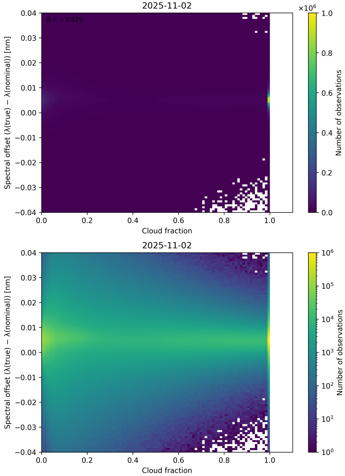
Figure 76: Scatter density plot of “Cloud fraction” against “Spectral offset ( \lambda_{\text{true}} - \lambda_{\text{nominal}} )” for 2025-11-02 to 2025-11-03.
