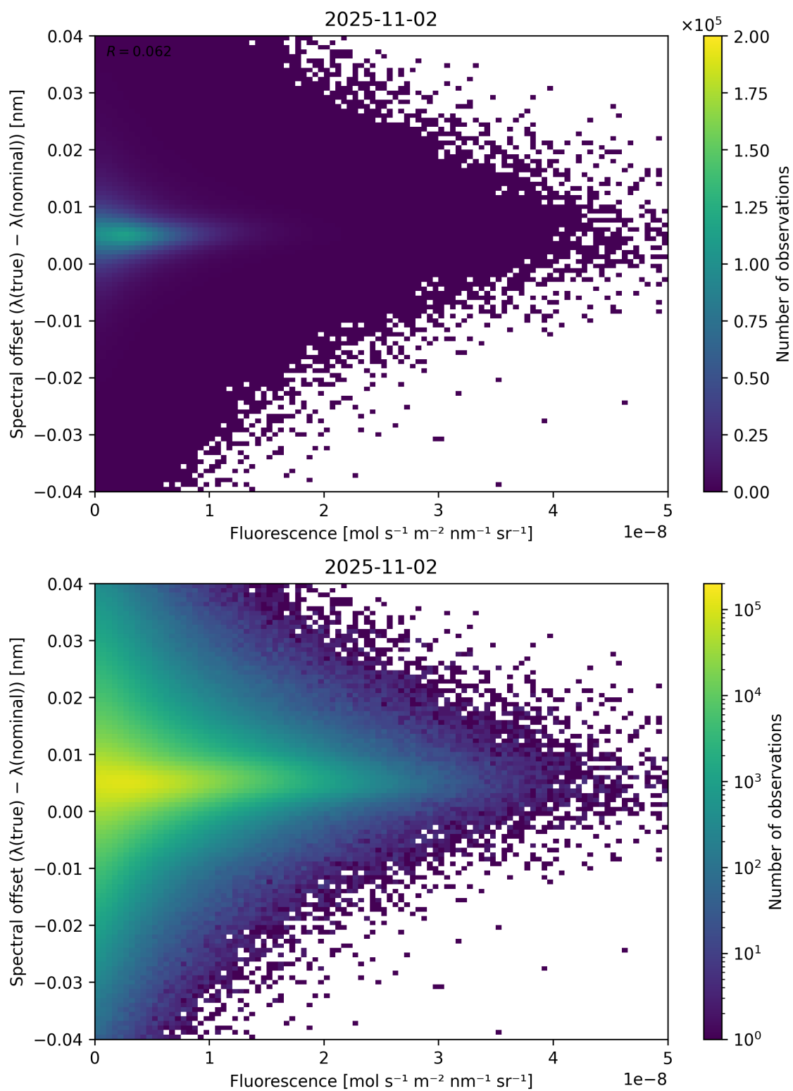
Figure 87: Scatter density plot of “Fluorescence” against “Spectral offset ( \lambda_{\text{true}} - \lambda_{\text{nominal}} )” for 2025-11-02 to 2025-11-03.
