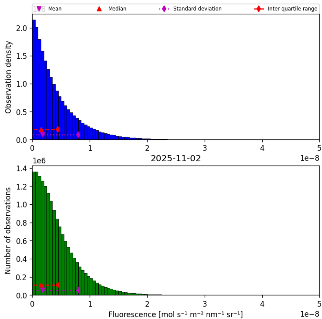
Figure 40: Histogram of “Fluorescence” for 2025-11-02 to 2025-11-03
