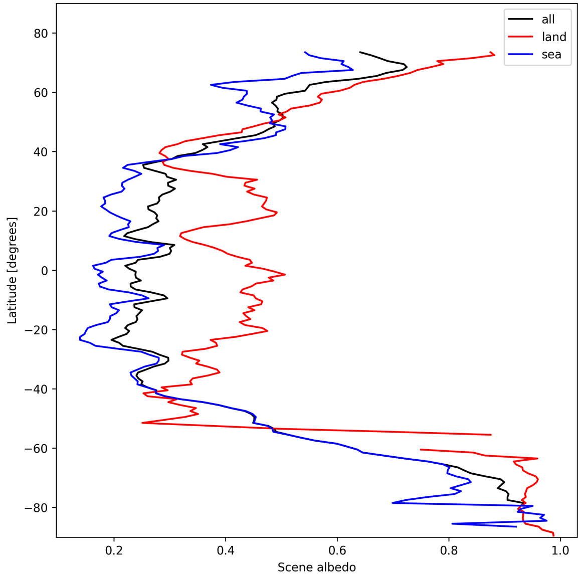
Figure 17: Zonal average of “Scene albedo” for 2025-11-02 to 2025-11-03.
