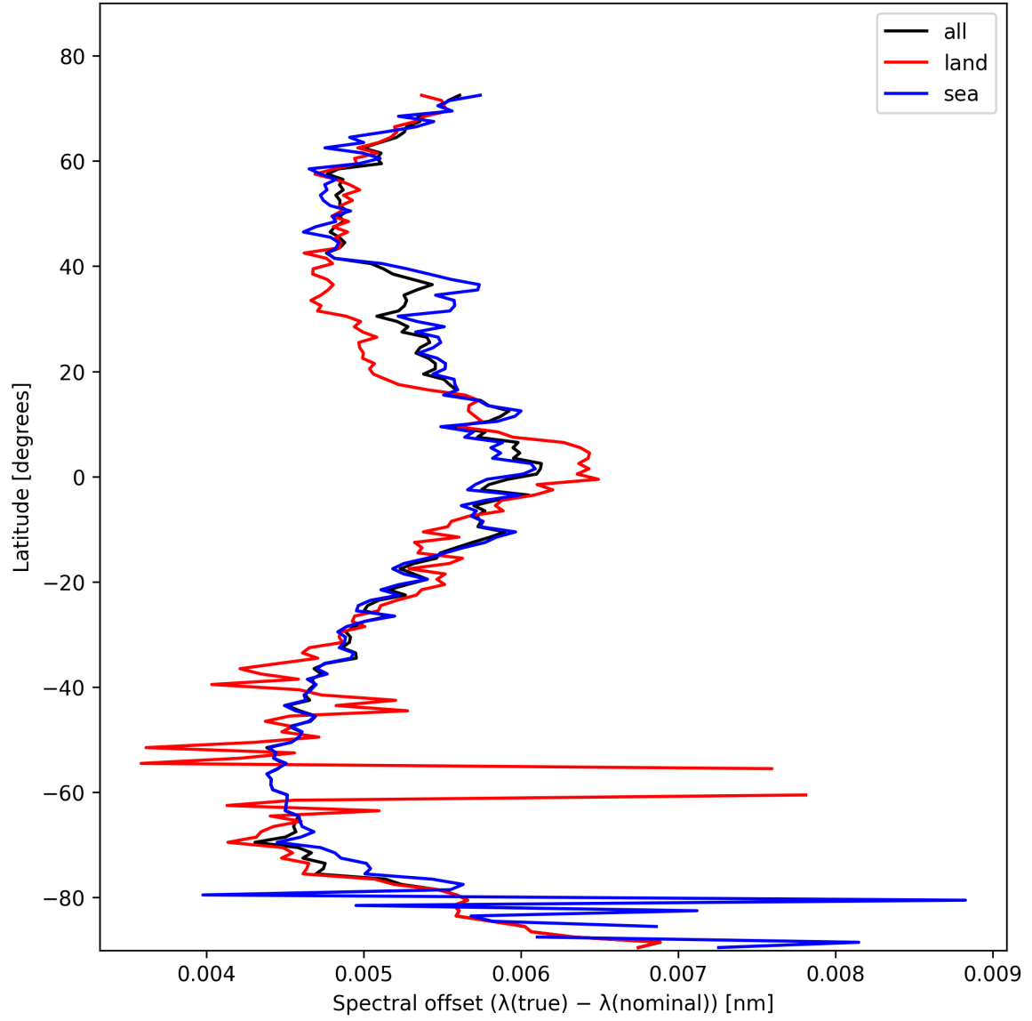
Figure 28: Zonal average of “Spectral offset ( \lambda_{\text{true}} - \lambda_{\text{nominal}} )” for 2025-11-02 to 2025-11-04.
