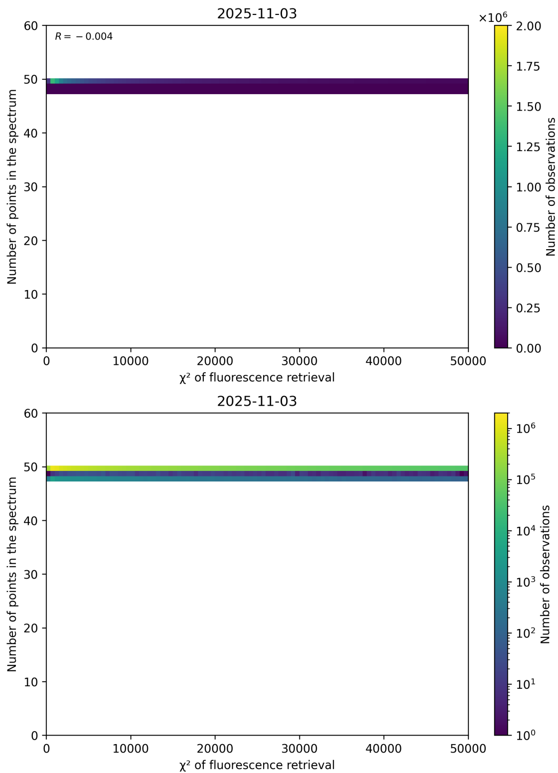
Figure 68: Scatter density plot of " \chi^2 of fluorescence retrieval" against "Number of points in the spectrum" for 2025-11-02 to 2025-11-04.
