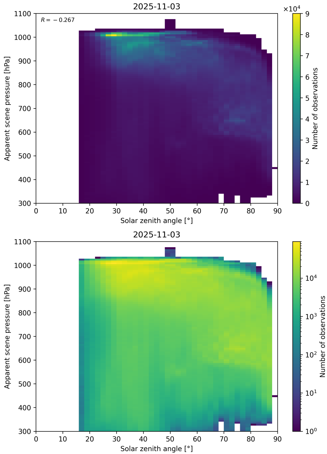
Figure 108: Scatter density plot of “Solar zenith angle” against “Apparent scene pressure” for 2025-11-02 to 2025-11-04.
