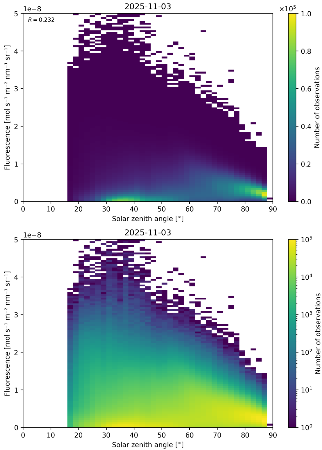
Figure 112: Scatter density plot of “Solar zenith angle” against “Fluorescence” for 2025-11-02 to 2025-11-04.
