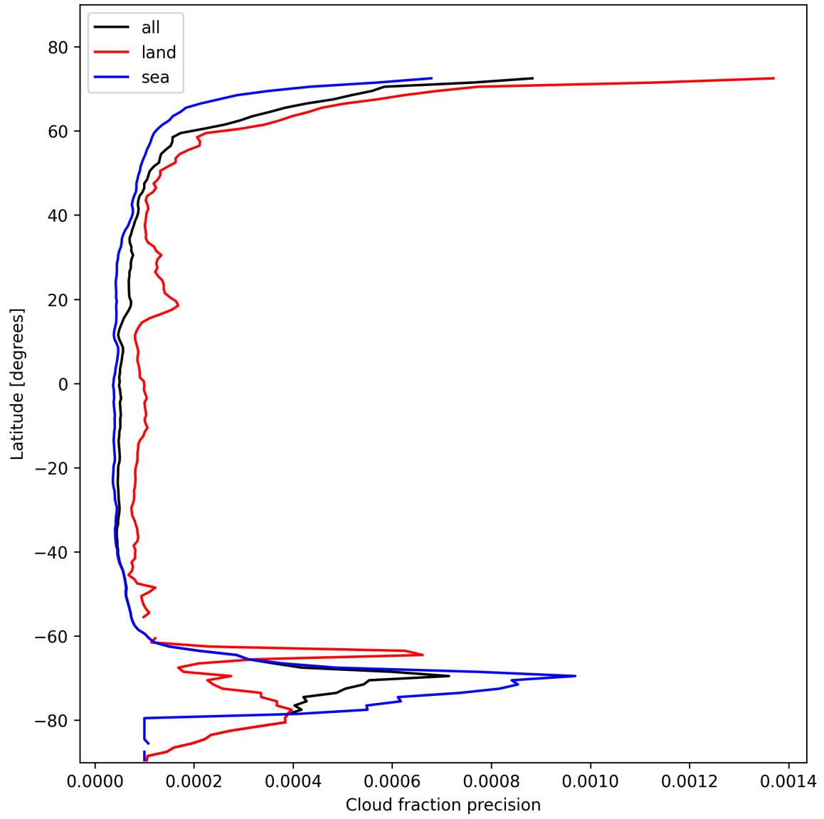
Figure 16: Zonal average of “Cloud fraction precision” for 2025-11-02 to 2025-11-04.
