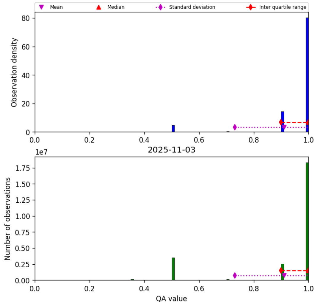
Figure 29: Histogram of “QA value” for 2025-11-02 to 2025-11-04
