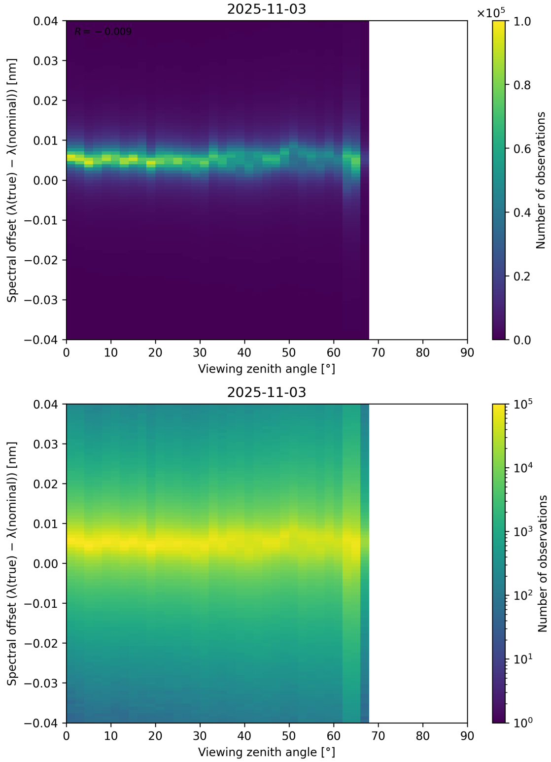
Figure 128: Scatter density plot of “Viewing zenith angle” against “Spectral offset ( \lambda_{\text{true}} - \lambda_{\text{nominal}} )” for 2025-11-02 to 2025-11-04.
