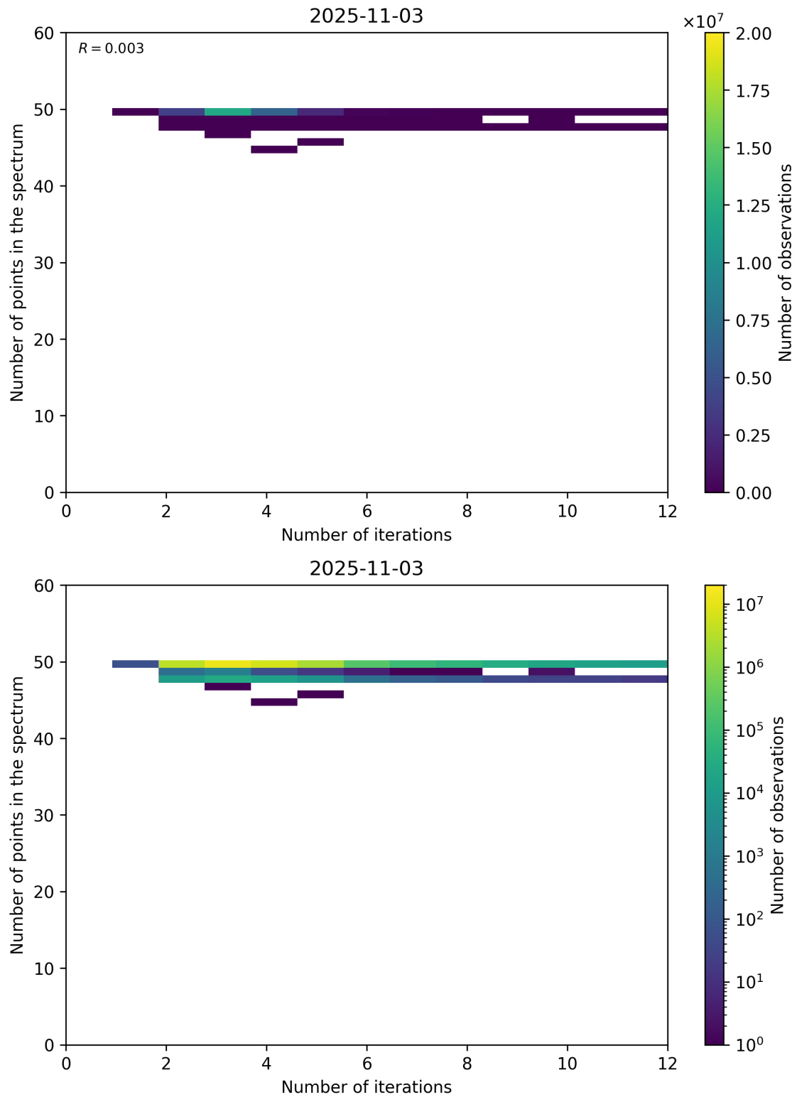
Figure 99: Scatter density plot of “Number of iterations” against “Number of points in the spectrum” for 2025-11-02 to 2025-11-04.
