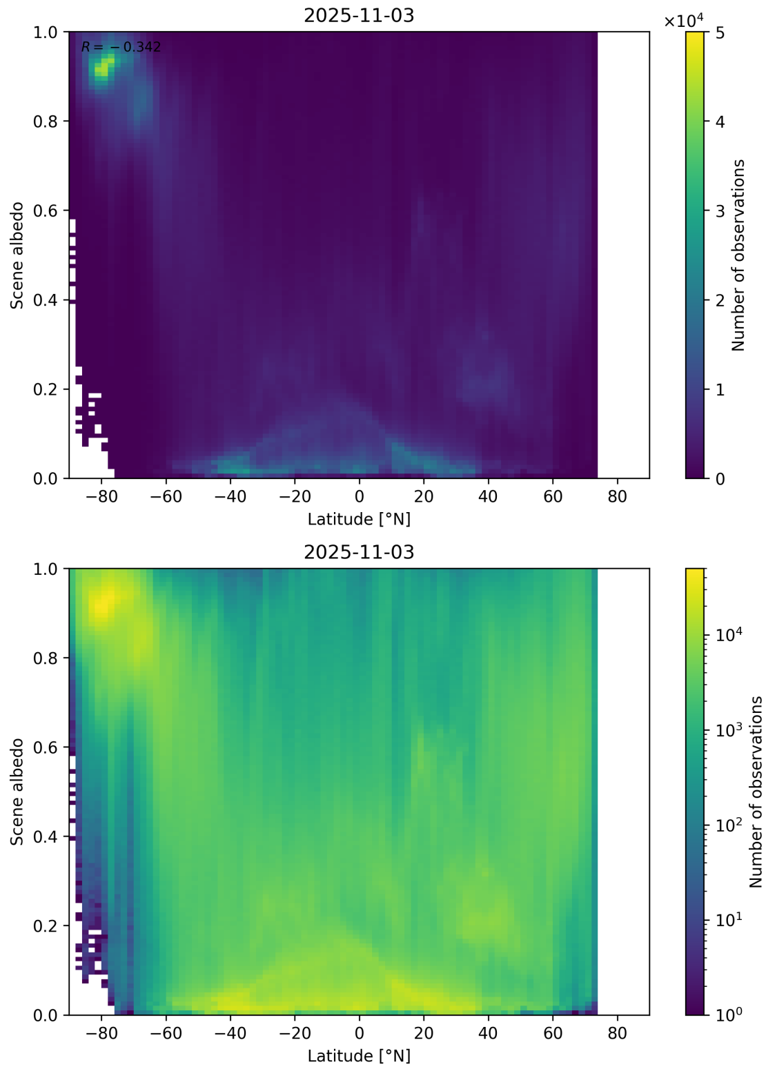
Figure 95: Scatter density plot of “Latitude” against “Scene albedo” for 2025-11-02 to 2025-11-04.
