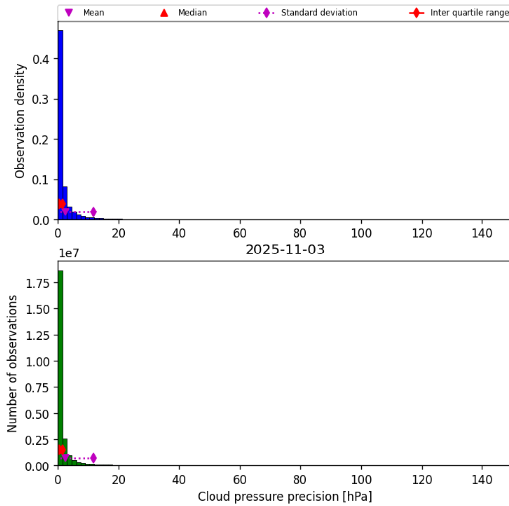
Figure 31: Histogram of “Cloud pressure precision” for 2025-11-02 to 2025-11-04
