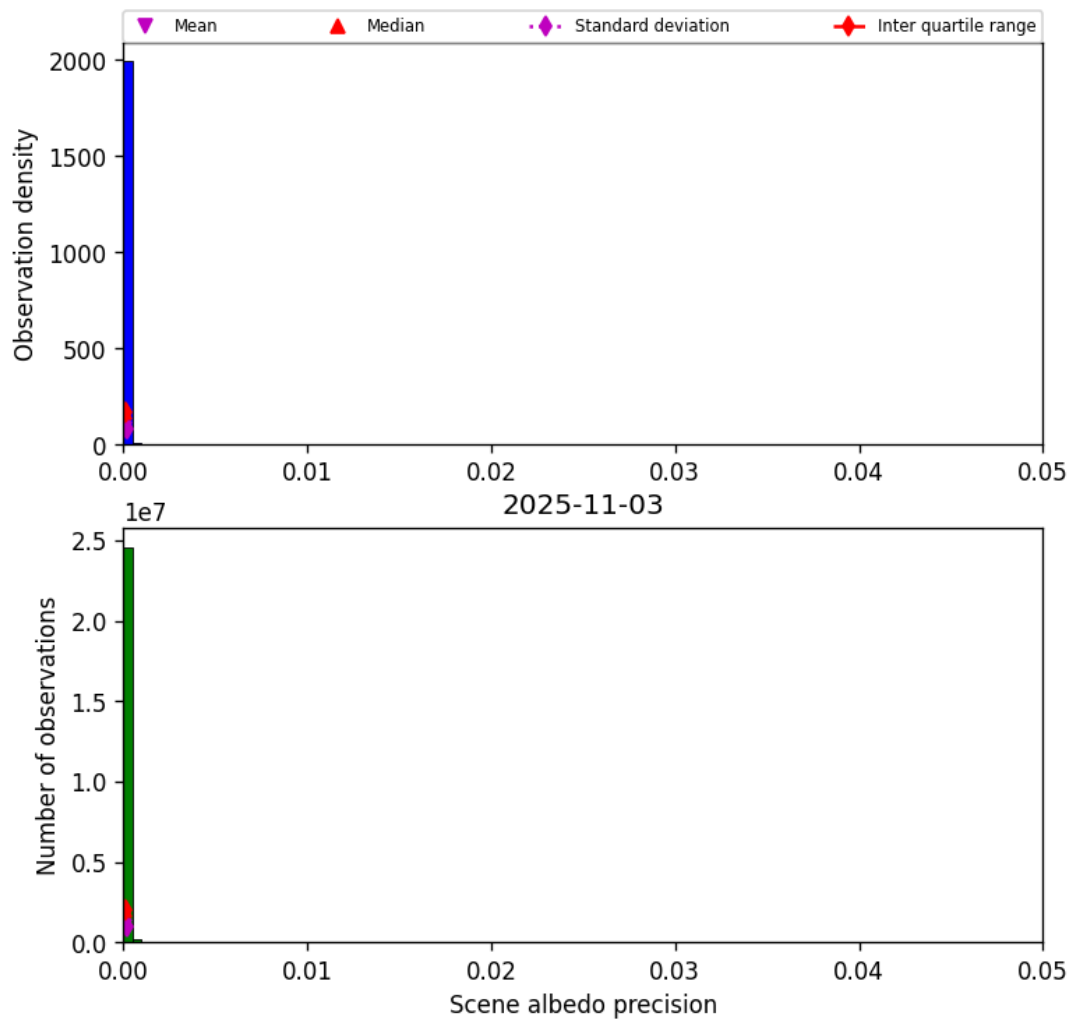
Figure 35: Histogram of “Scene albedo precision” for 2025-11-02 to 2025-11-04
