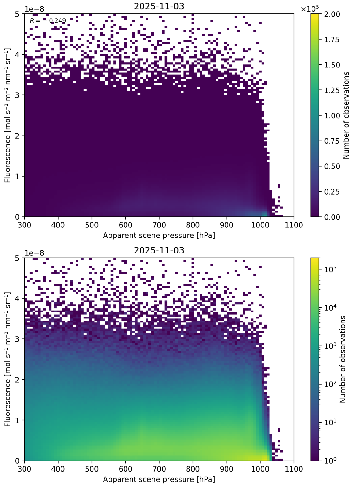
Figure 64: Scatter density plot of “Apparent scene pressure” against “Fluorescence” for 2025-11-02 to 2025-11-04.
