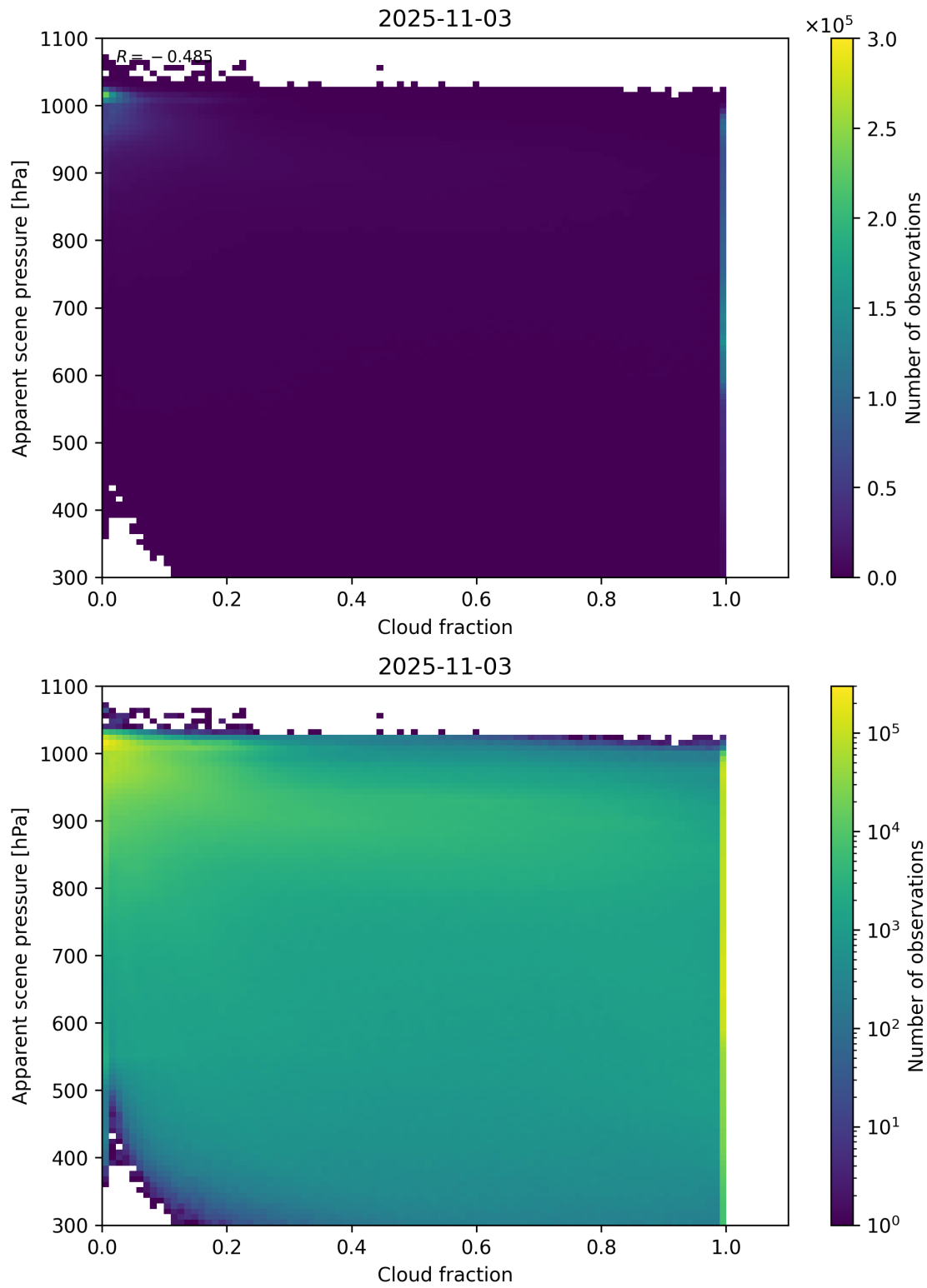
Figure 70: Scatter density plot of “Cloud fraction” against “Apparent scene pressure” for 2025-11-02 to 2025-11-04.
