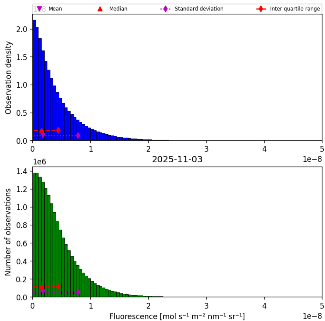
Figure 40: Histogram of “Fluorescence” for 2025-11-02 to 2025-11-04
