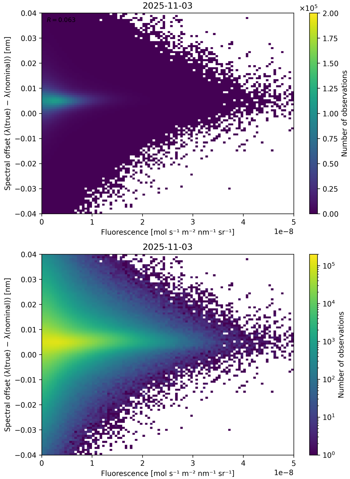
Figure 87: Scatter density plot of “Fluorescence” against “Spectral offset ( \lambda_{\text{true}} - \lambda_{\text{nominal}} )” for 2025-11-02 to 2025-11-04.
