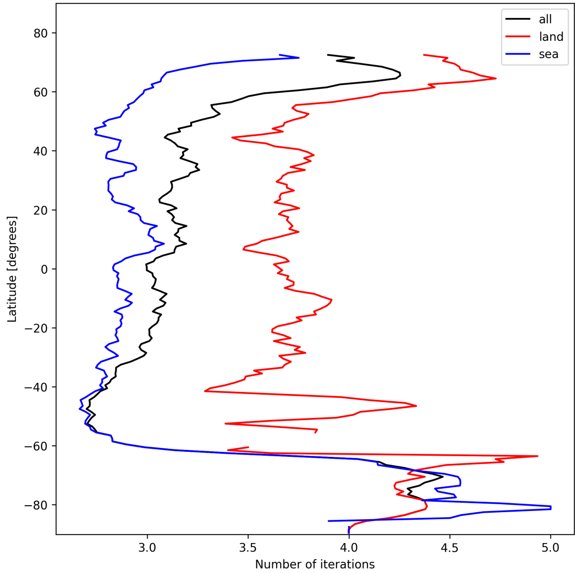
Figure 22: Zonal average of “Number of iterations” for 2025-11-02 to 2025-11-04.
