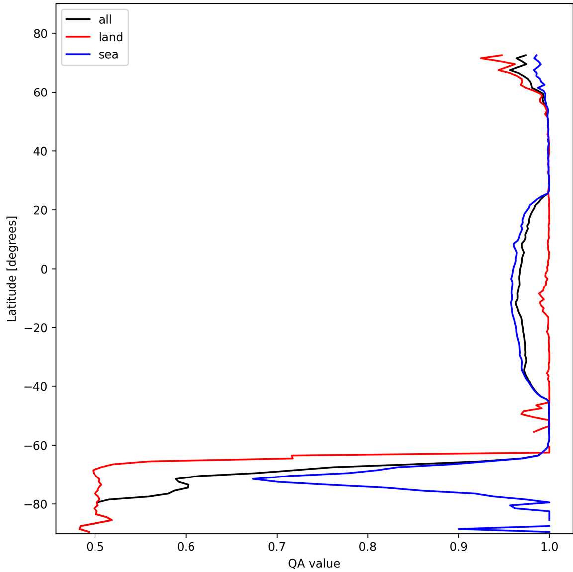
Figure 12: Zonal average of “QA value” for 2025-11-02 to 2025-11-04.
