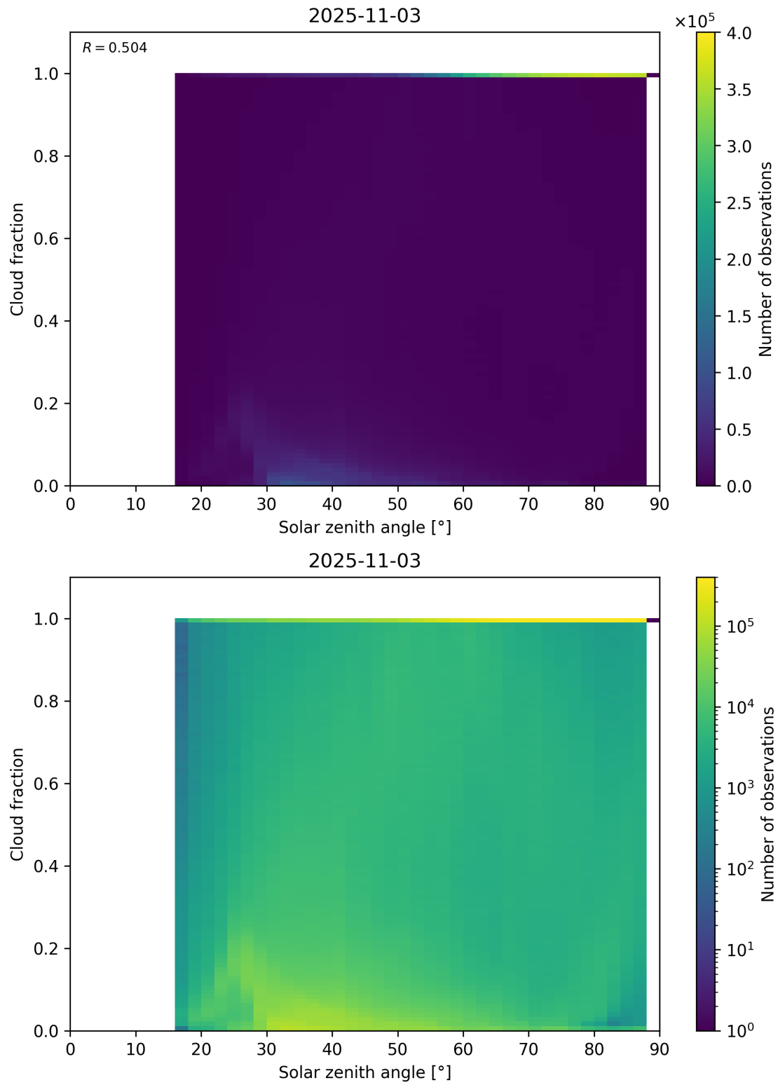
Figure 110: Scatter density plot of “Solar zenith angle” against “Cloud fraction” for 2025-11-02 to 2025-11-04.
