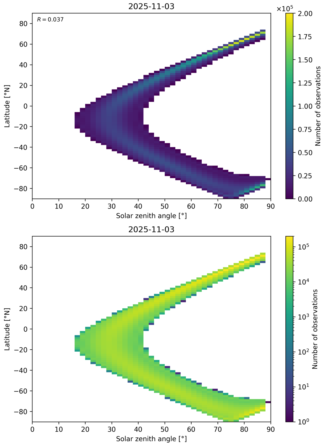
Figure 113: Scatter density plot of “Solar zenith angle” against “Latitude” for 2025-11-02 to 2025-11-04.
