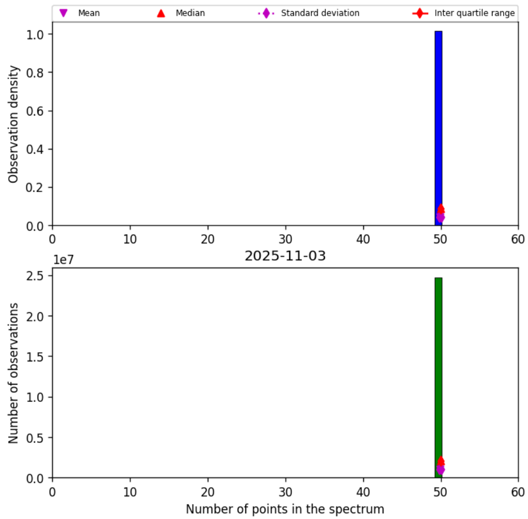
Figure 44: Histogram of "Number of points in the spectrum" for 2025-11-02 to 2025-11-04
