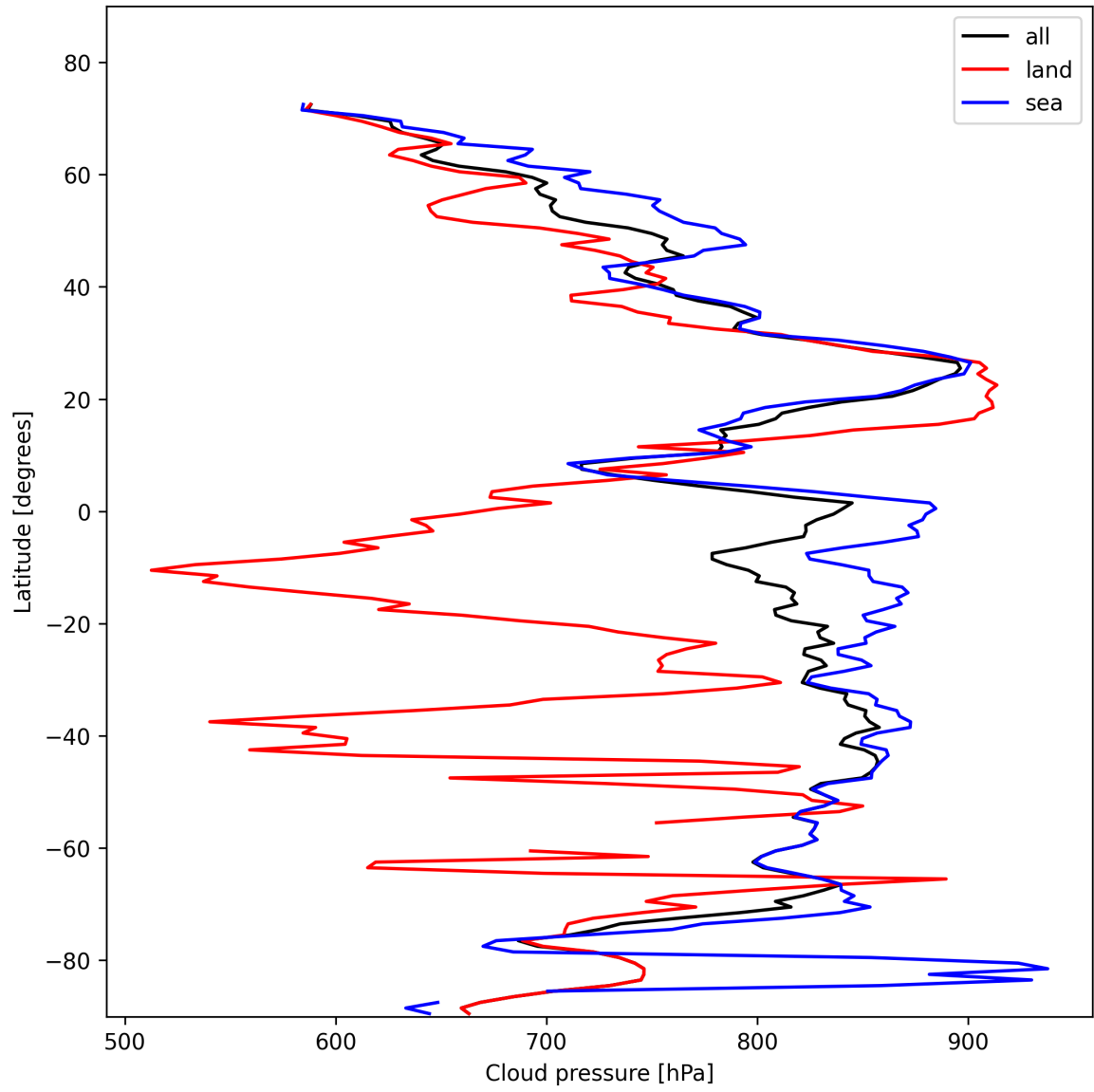
Figure 13: Zonal average of “Cloud pressure” for 2025-11-02 to 2025-11-04.
