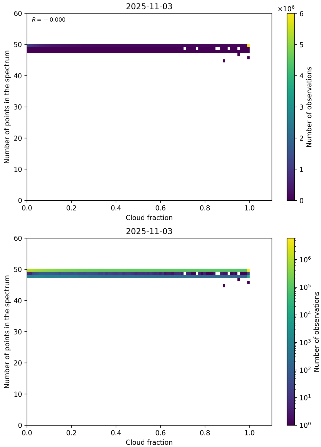
Figure 74: Scatter density plot of “Cloud fraction” against “Number of points in the spectrum” for 2025-11-02 to 2025-11-04.
