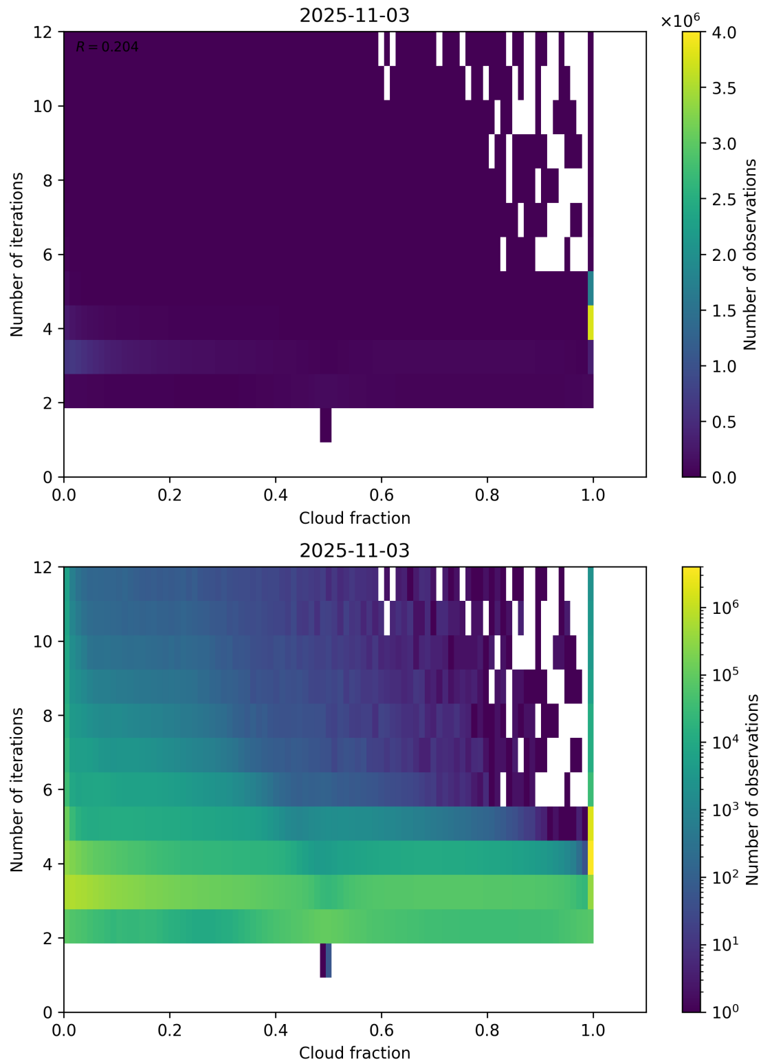
Figure 73: Scatter density plot of “Cloud fraction” against “Number of iterations” for 2025-11-02 to 2025-11-04.
