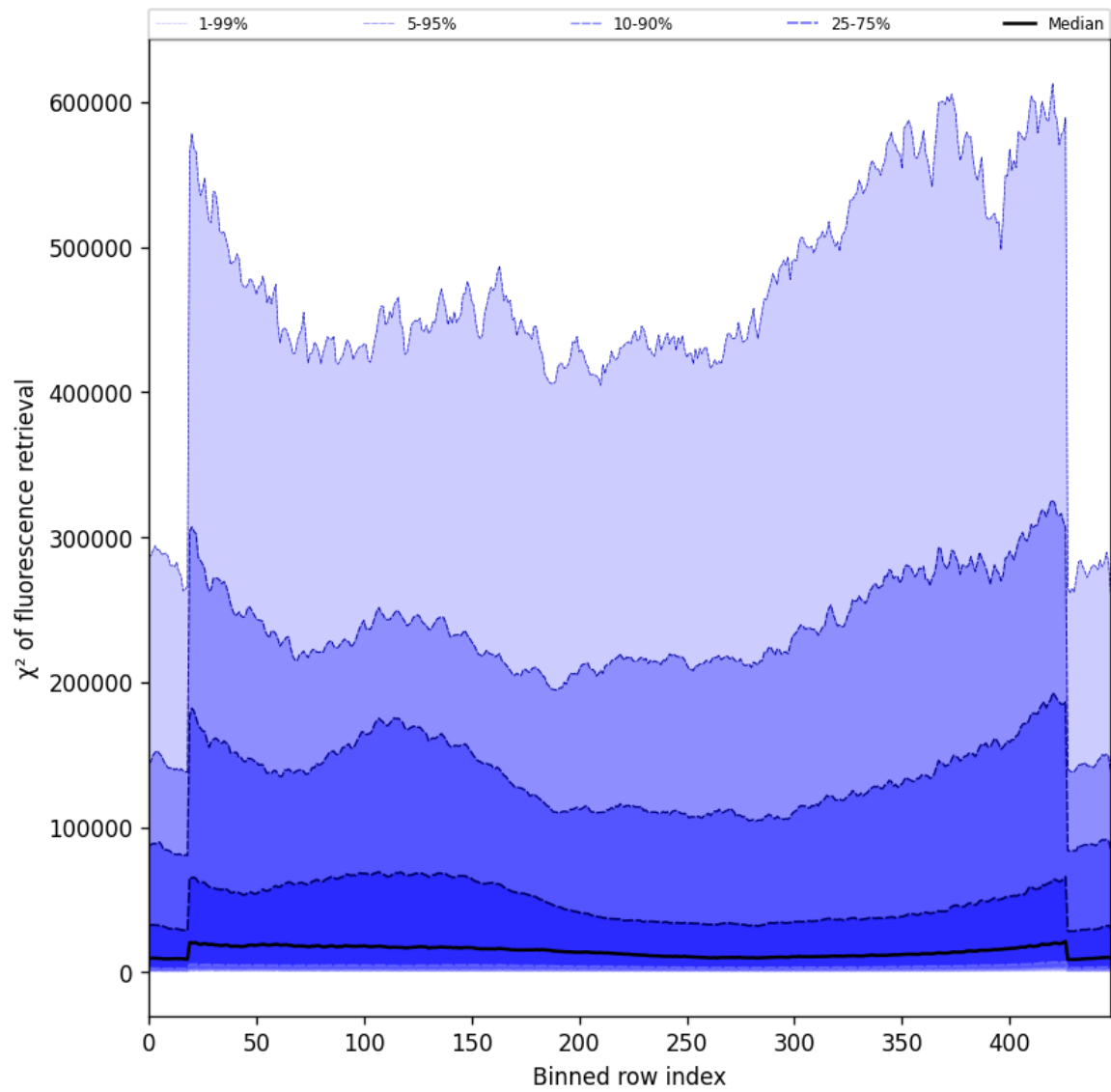
Figure 59: Along track statistics of “ \chi^2 of fluorescence retrieval” for 2025-11-02 to 2025-11-04
