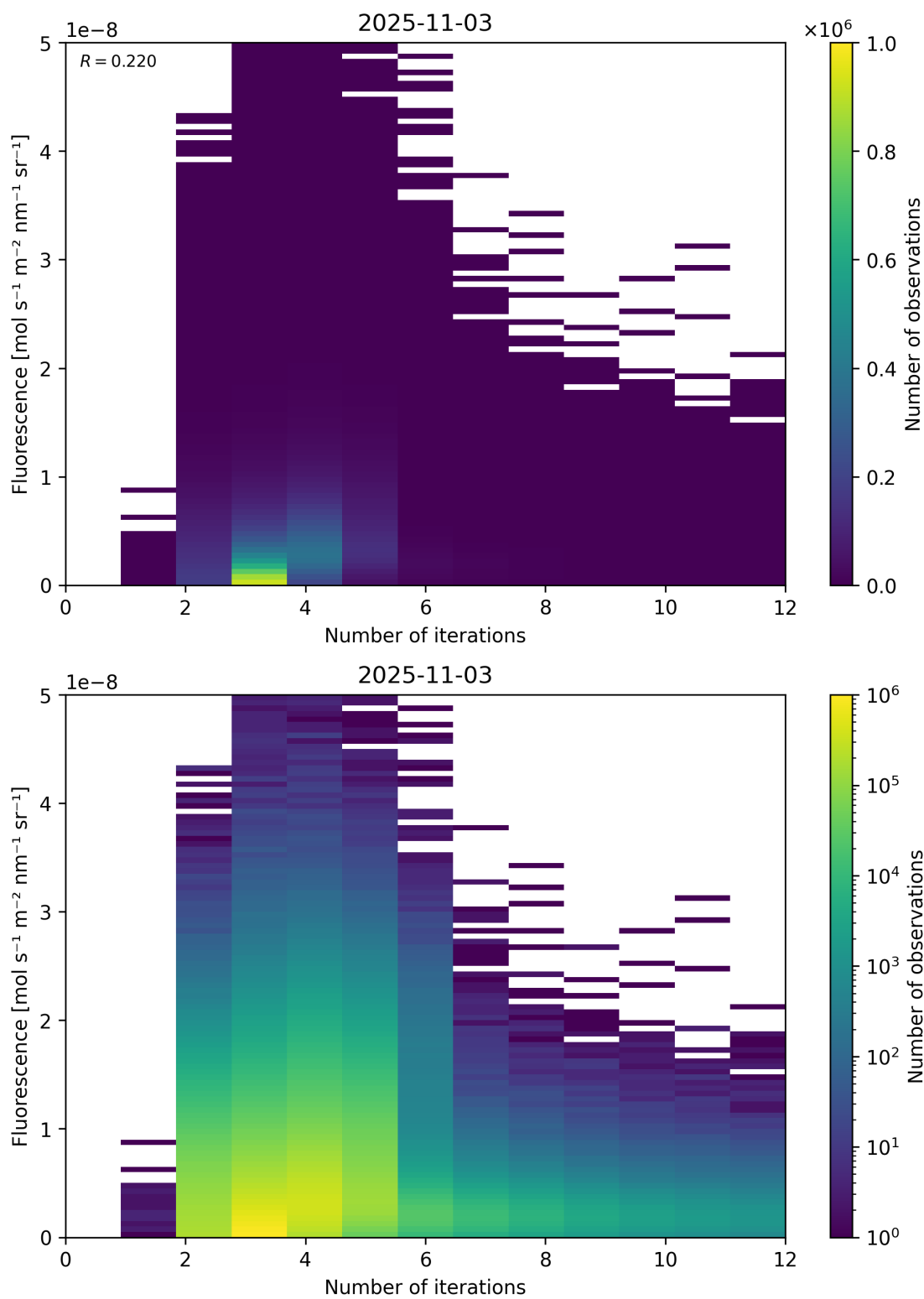
Figure 98: Scatter density plot of “Number of iterations” against “Fluorescence” for 2025-11-02 to 2025-11-04.
