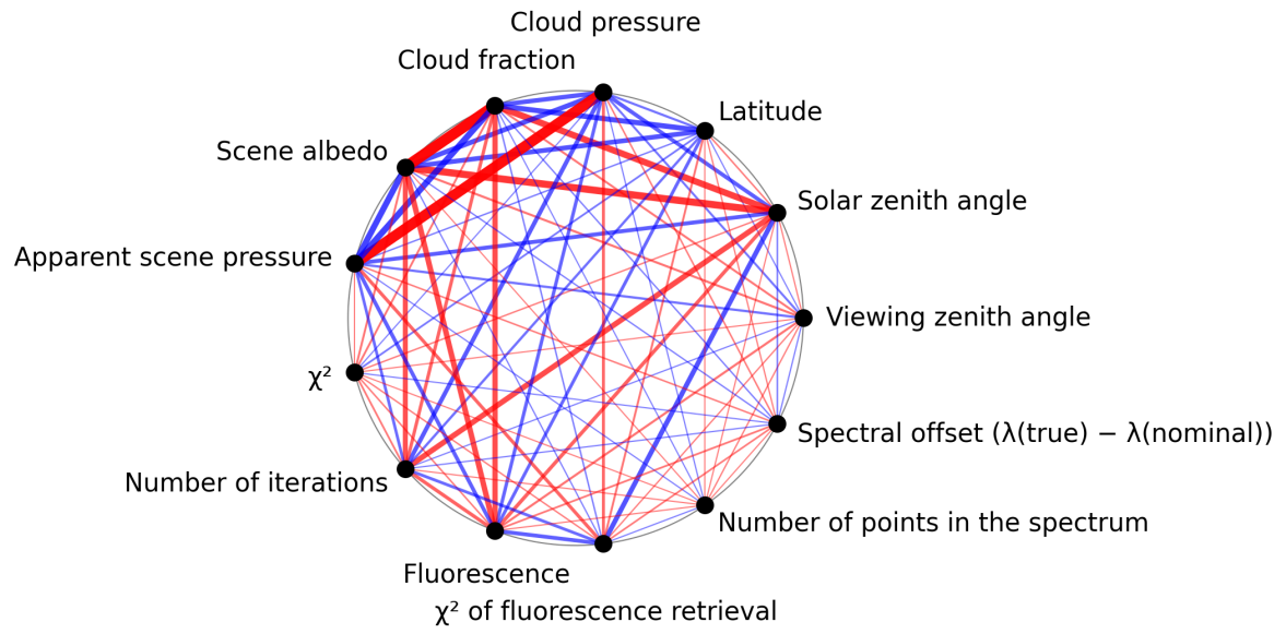
Figure 1: Map of correlation graph for 2025-11-02 to 2025-11-04.
