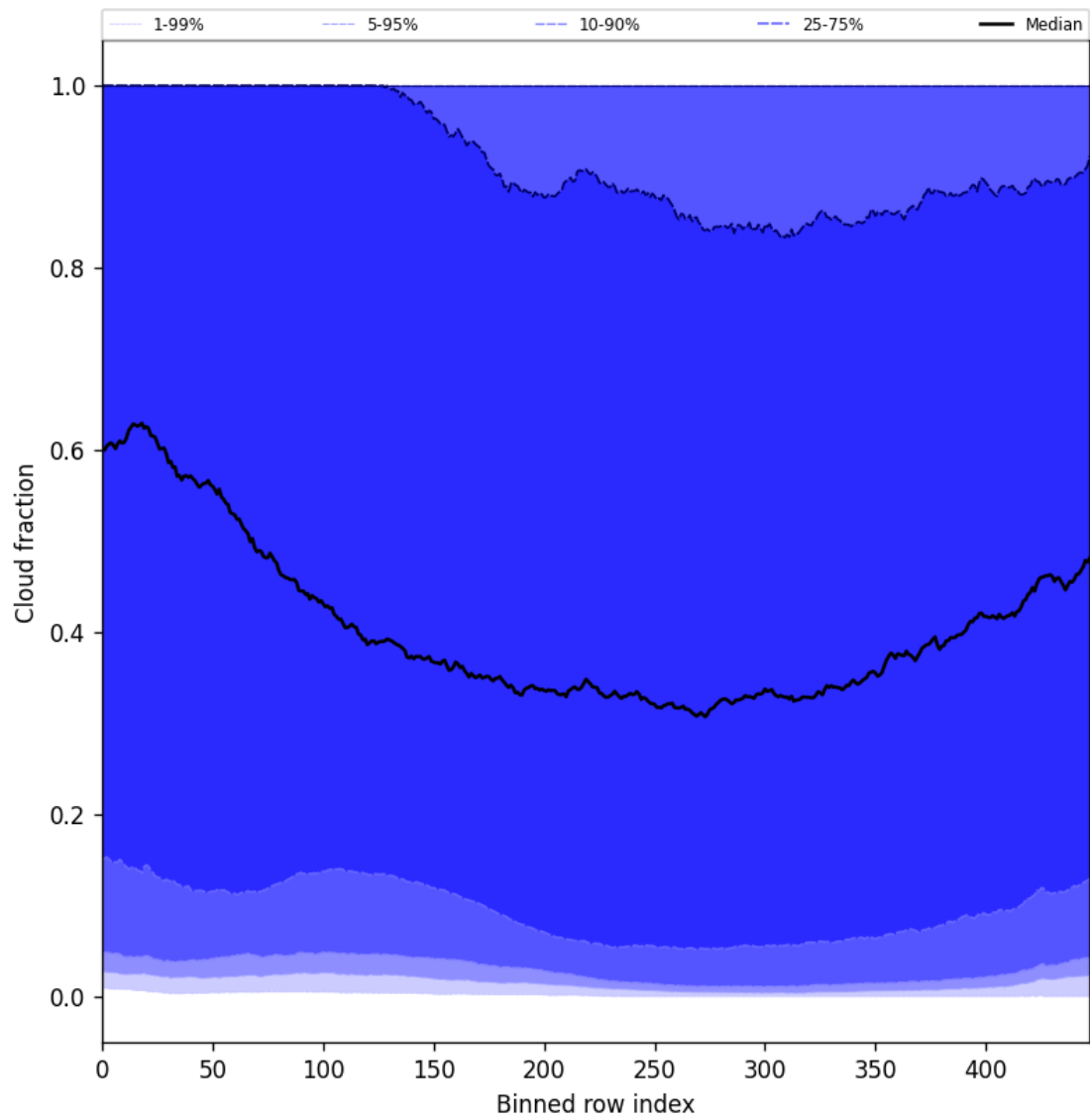
Figure 49: Along track statistics of “Cloud fraction” for 2025-11-02 to 2025-11-04
