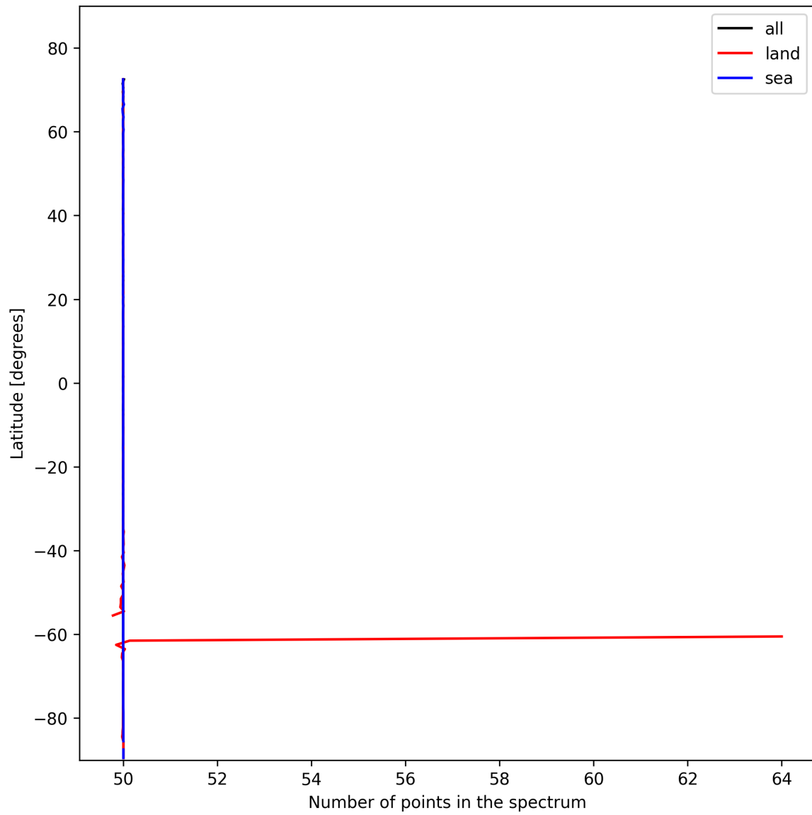
Figure 27: Zonal average of “Number of points in the spectrum” for 2025-11-02 to 2025-11-04.
