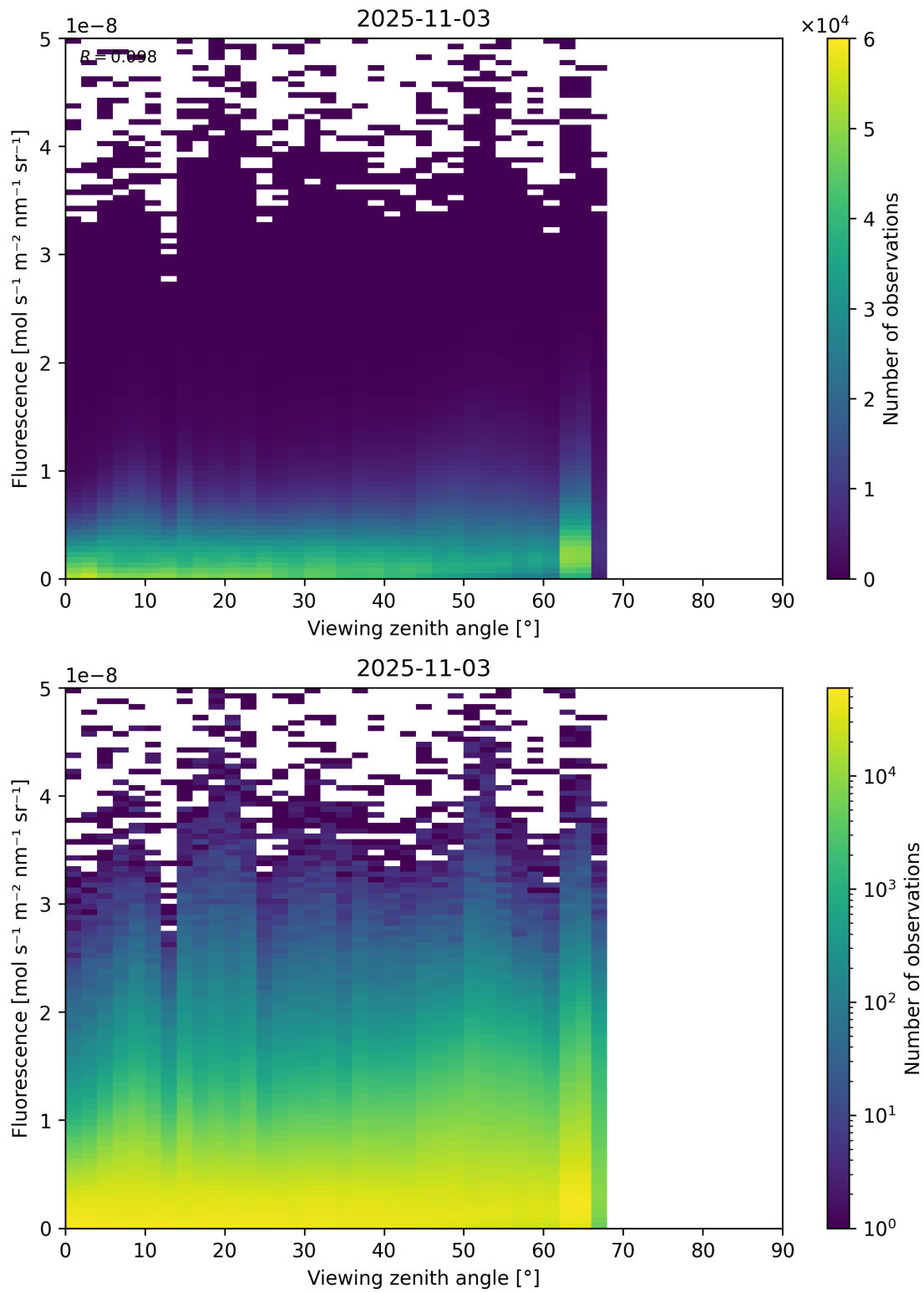
Figure 122: Scatter density plot of “Viewing zenith angle” against “Fluorescence” for 2025-11-02 to 2025-11-04.
