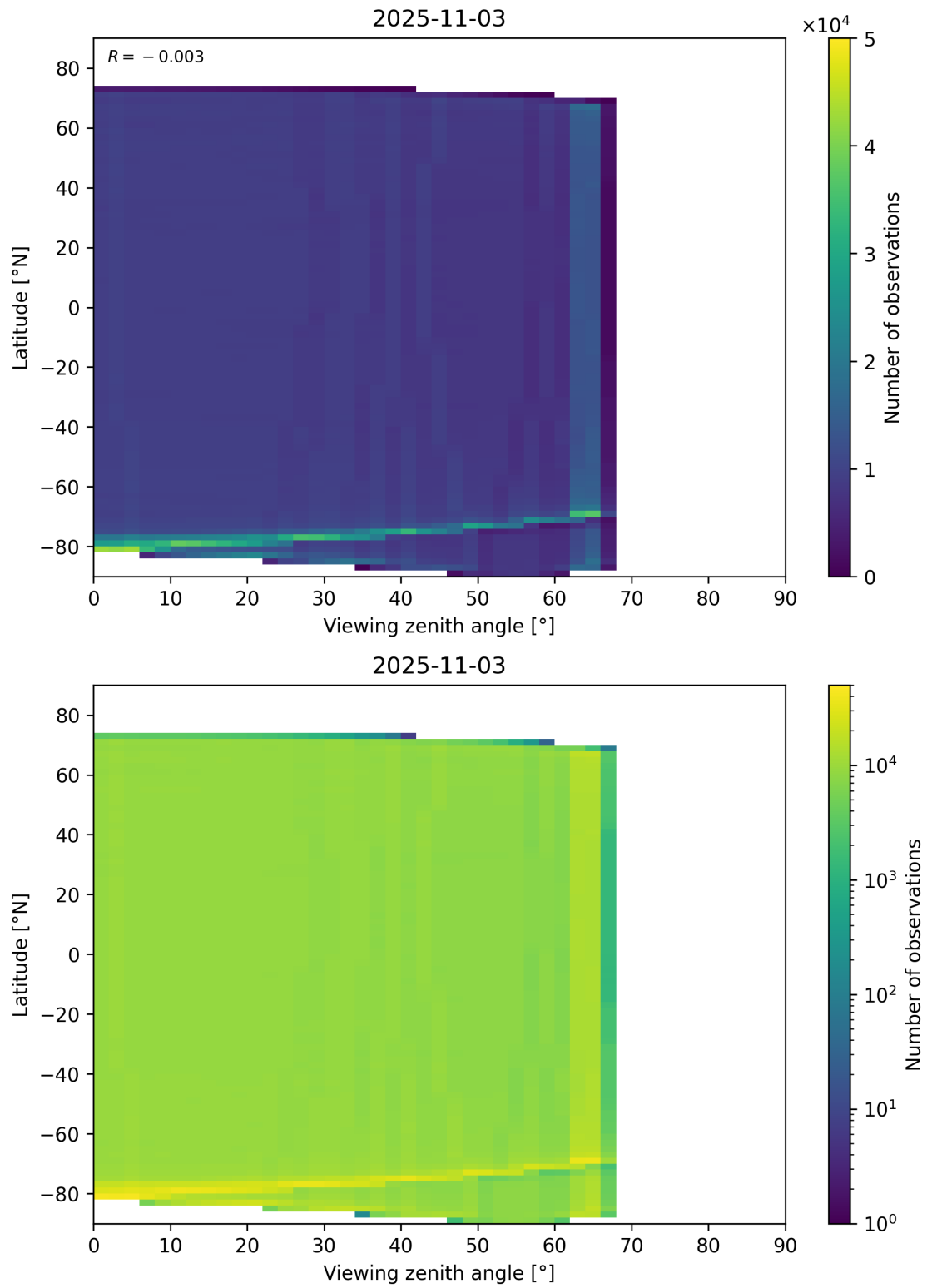
Figure 123: Scatter density plot of “Viewing zenith angle” against “Latitude” for 2025-11-02 to 2025-11-04.
