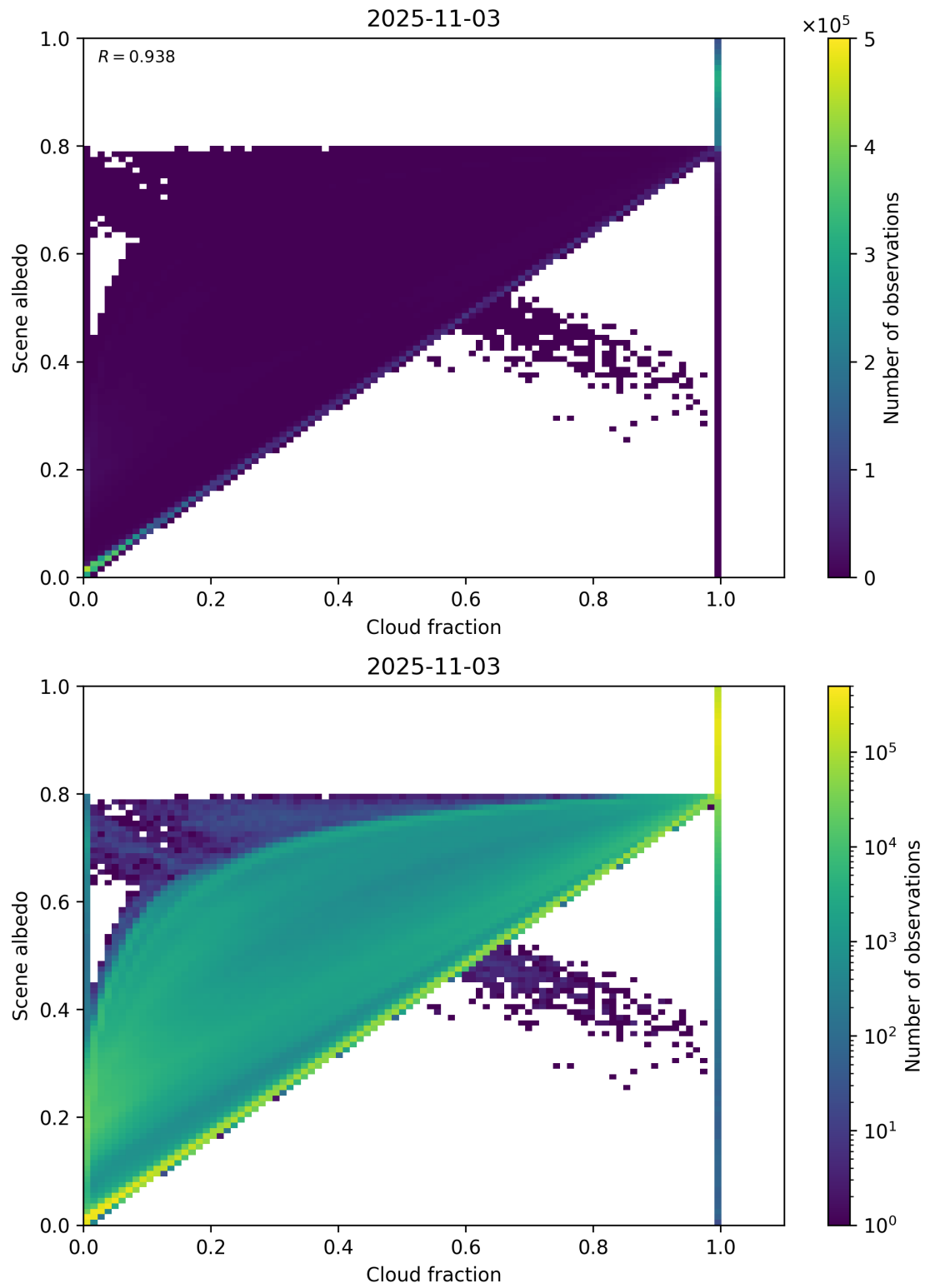
Figure 75: Scatter density plot of “Cloud fraction” against “Scene albedo” for 2025-11-02 to 2025-11-04.
