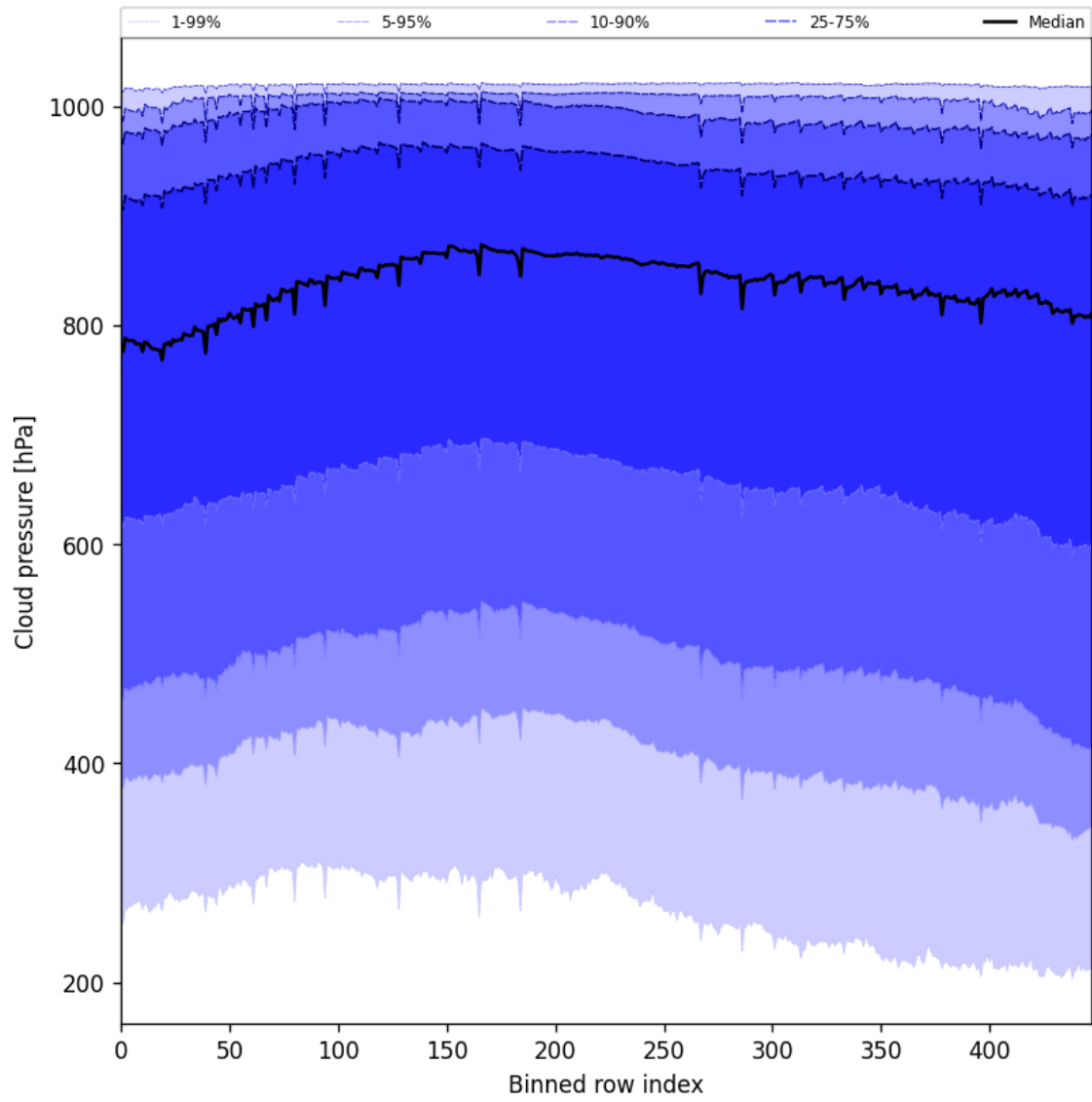
Figure 47: Along track statistics of “Cloud pressure” for 2025-11-02 to 2025-11-04
