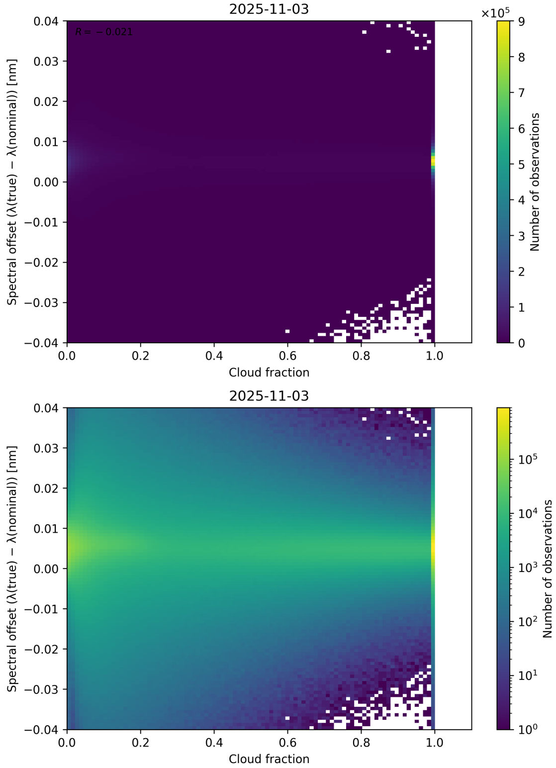
Figure 76: Scatter density plot of “Cloud fraction” against “Spectral offset ( \lambda_{\text{true}} - \lambda_{\text{nominal}} )” for 2025-11-02 to 2025-11-04.
