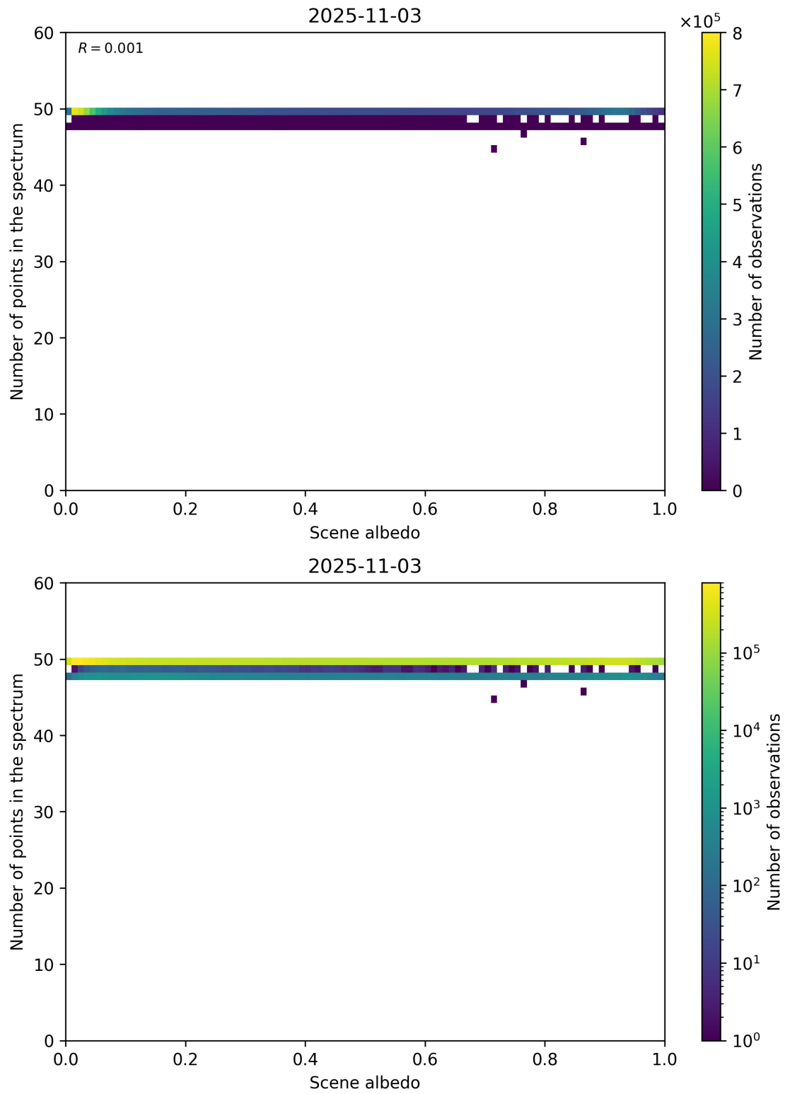
Figure 106: Scatter density plot of “Scene albedo” against “Number of points in the spectrum” for 2025-11-02 to 2025-11-04.
