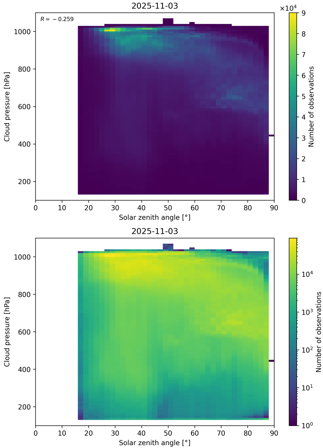
Figure 111: Scatter density plot of “Solar zenith angle” against “Cloud pressure” for 2025-11-02 to 2025-11-04.
