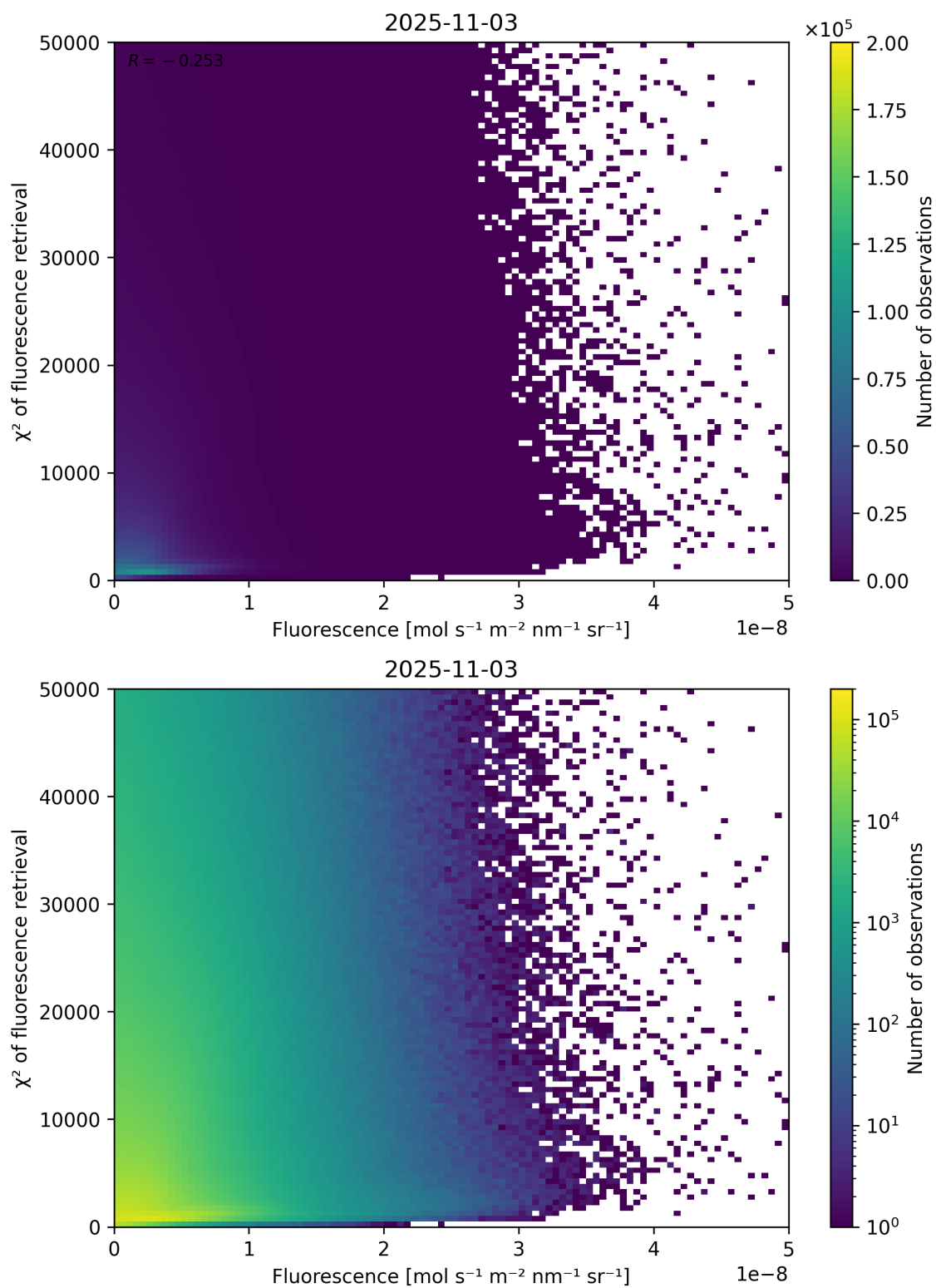
Figure 85: Scatter density plot of “Fluorescence” against “ \chi^2 of fluorescence retrieval” for 2025-11-02 to 2025-11-04.
