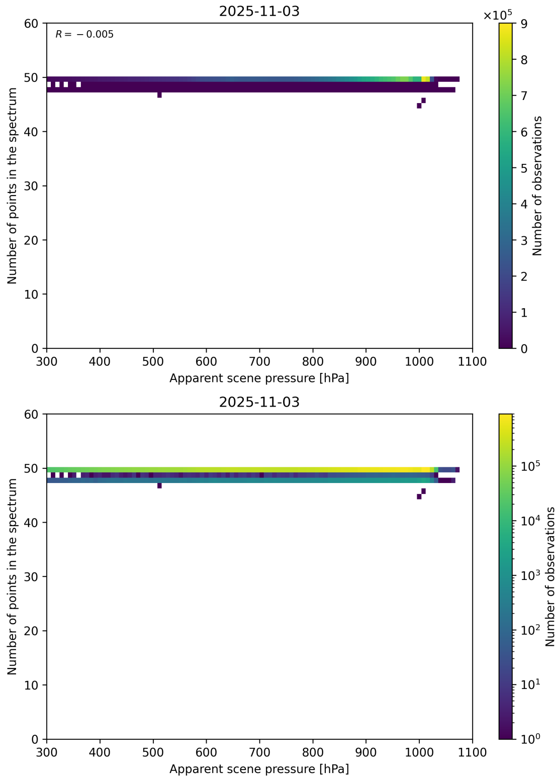
Figure 66: Scatter density plot of “Apparent scene pressure” against “Number of points in the spectrum” for 2025-11-02 to 2025-11-04.
