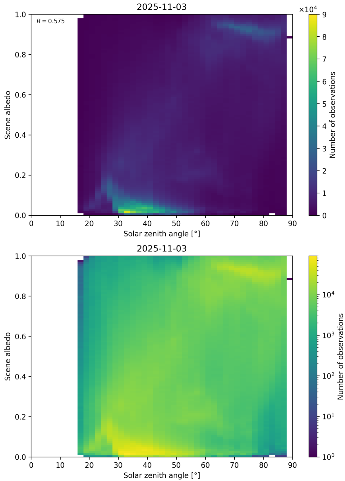
Figure 116: Scatter density plot of “Solar zenith angle” against “Scene albedo” for 2025-11-02 to 2025-11-04.
