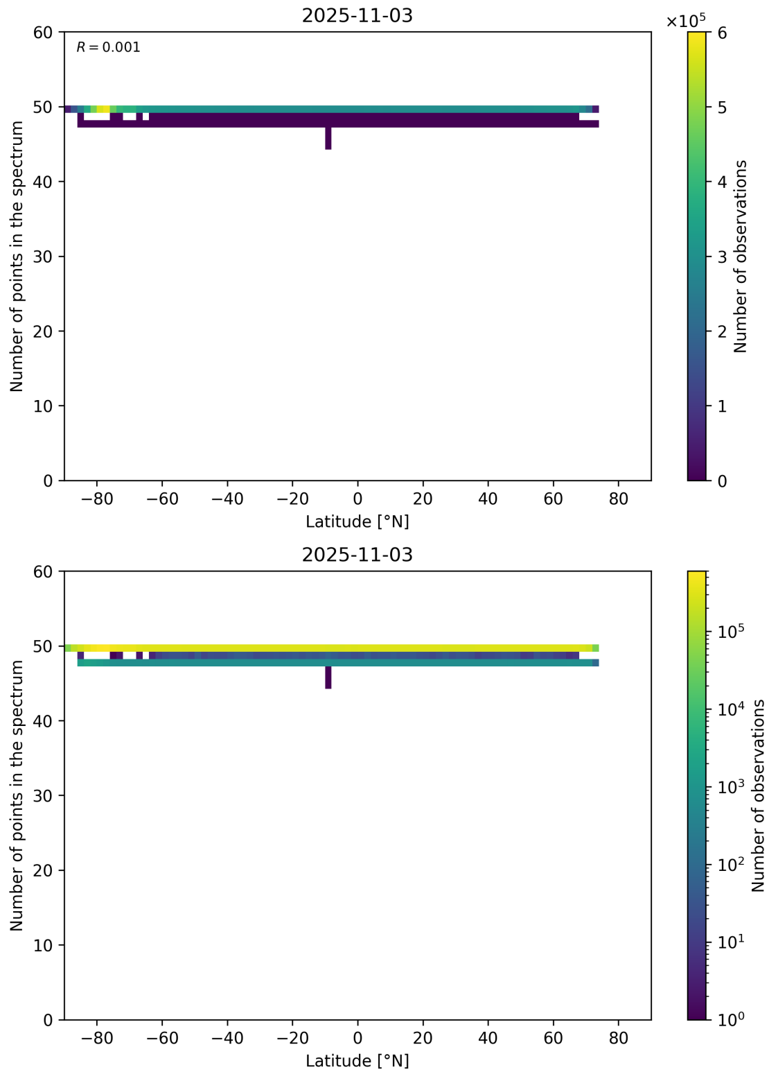
Figure 94: Scatter density plot of “Latitude” against “Number of points in the spectrum” for 2025-11-02 to 2025-11-04.
