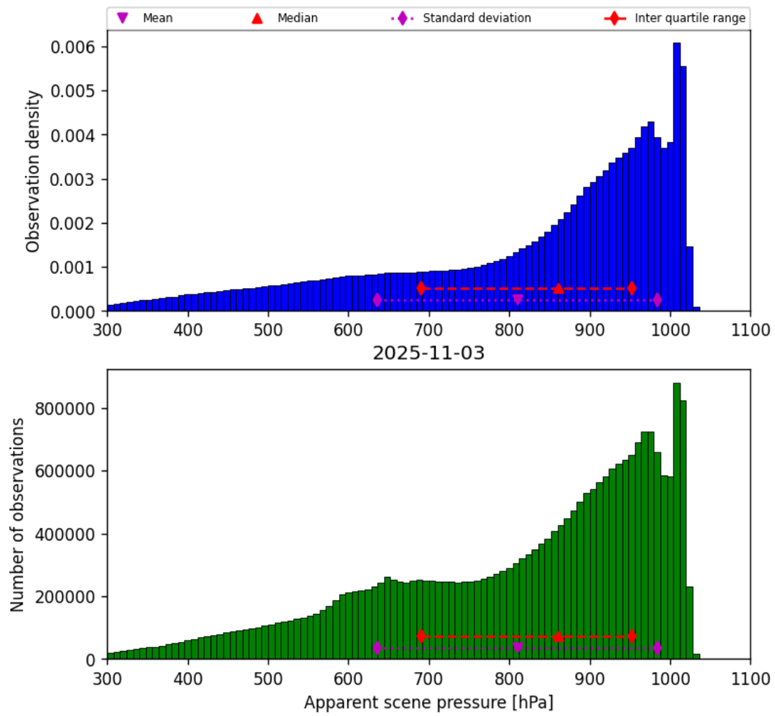
Figure 36: Histogram of “Apparent scene pressure” for 2025-11-02 to 2025-11-04
