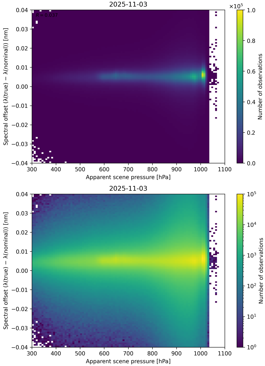
Figure 67: Scatter density plot of “Apparent scene pressure” against “Spectral offset ( \lambda_{\text{true}} - \lambda_{\text{nominal}} )” for 2025-11-02 to 2025-11-04.
