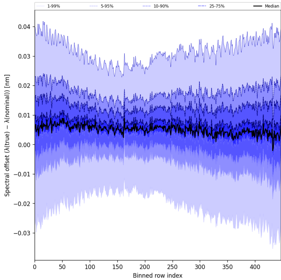
Figure 62: Along track statistics of “Spectral offset ( \lambda_{\text{true}} - \lambda_{\text{nominal}} )” for 2025-11-02 to 2025-11-04
