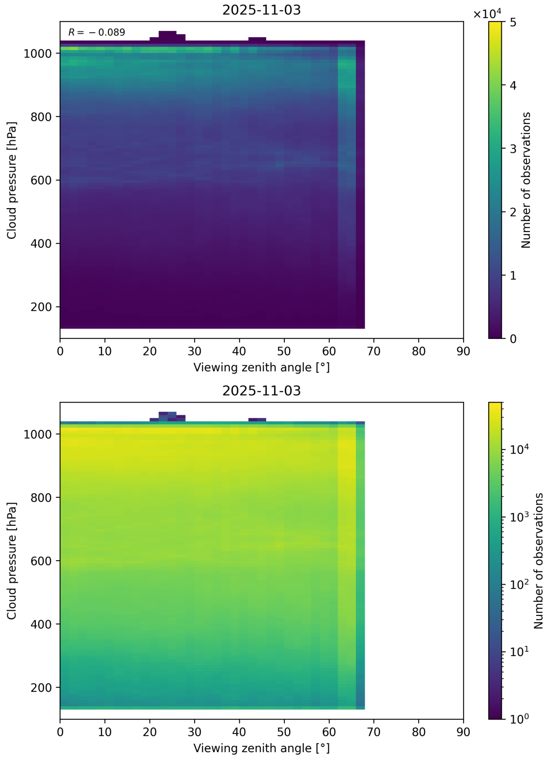
Figure 121: Scatter density plot of “Viewing zenith angle” against “Cloud pressure” for 2025-11-02 to 2025-11-04.
