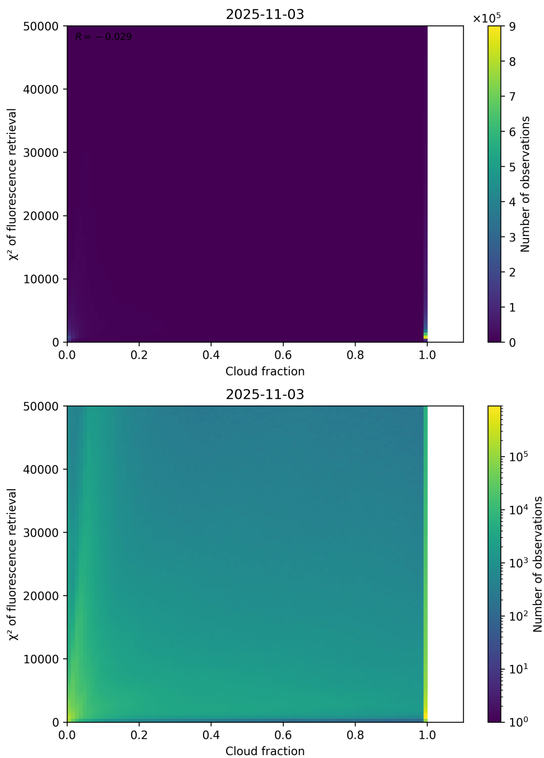
Figure 71: Scatter density plot of “Cloud fraction” against “ \chi^2 of fluorescence retrieval” for 2025-11-02 to 2025-11-04.
