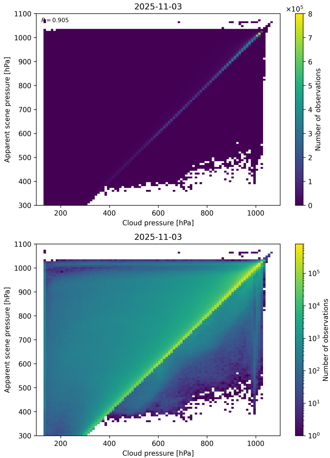
Figure 77: Scatter density plot of “Cloud pressure” against “Apparent scene pressure” for 2025-11-02 to 2025-11-04.
