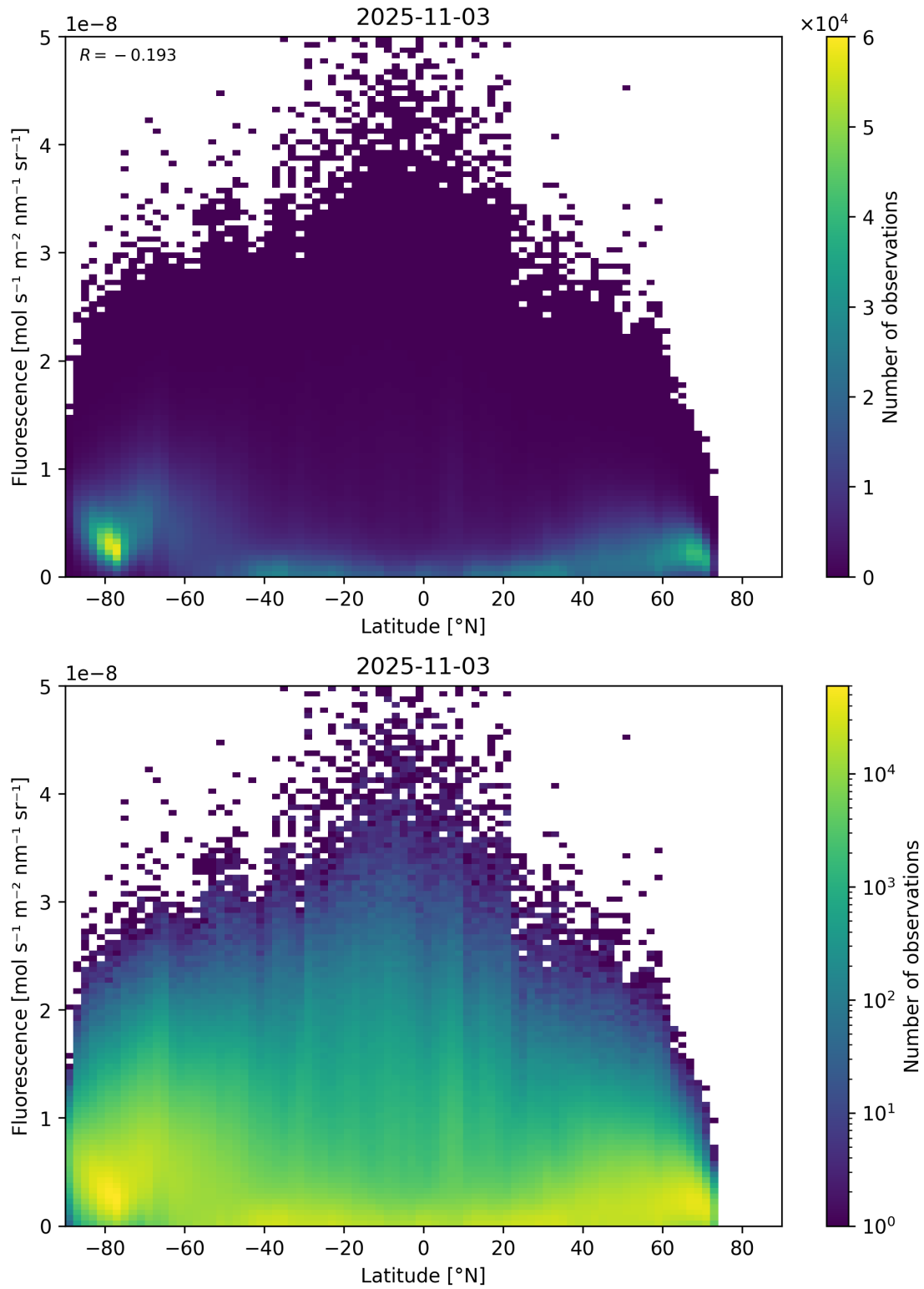
Figure 92: Scatter density plot of “Latitude” against “Fluorescence” for 2025-11-02 to 2025-11-04.
