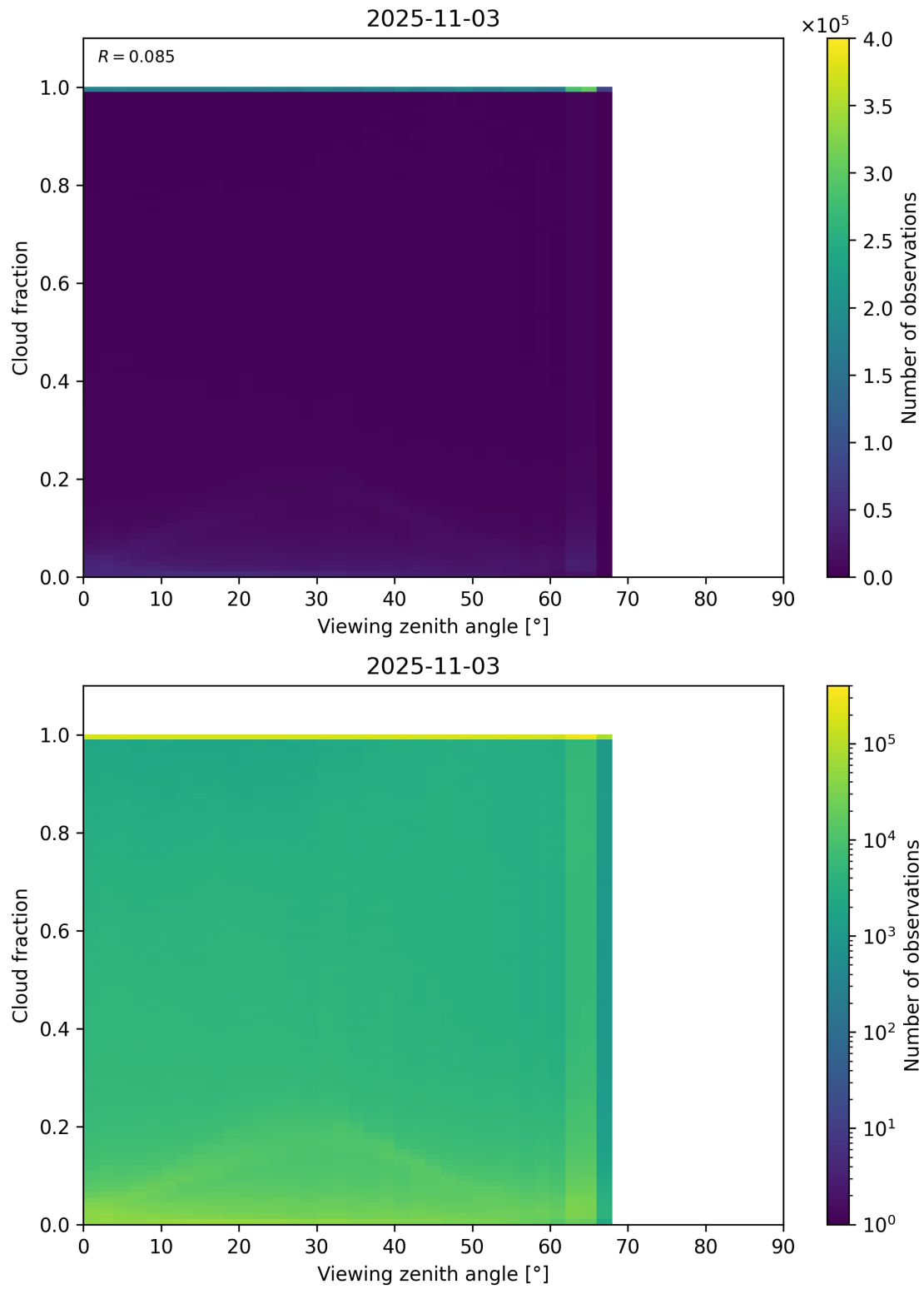
Figure 120: Scatter density plot of “Viewing zenith angle” against “Cloud fraction” for 2025-11-02 to 2025-11-04.
