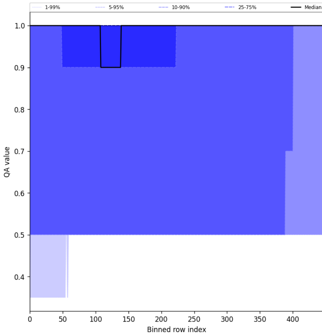
Figure 46: Along track statistics of “QA value” for 2025-11-02 to 2025-11-04
