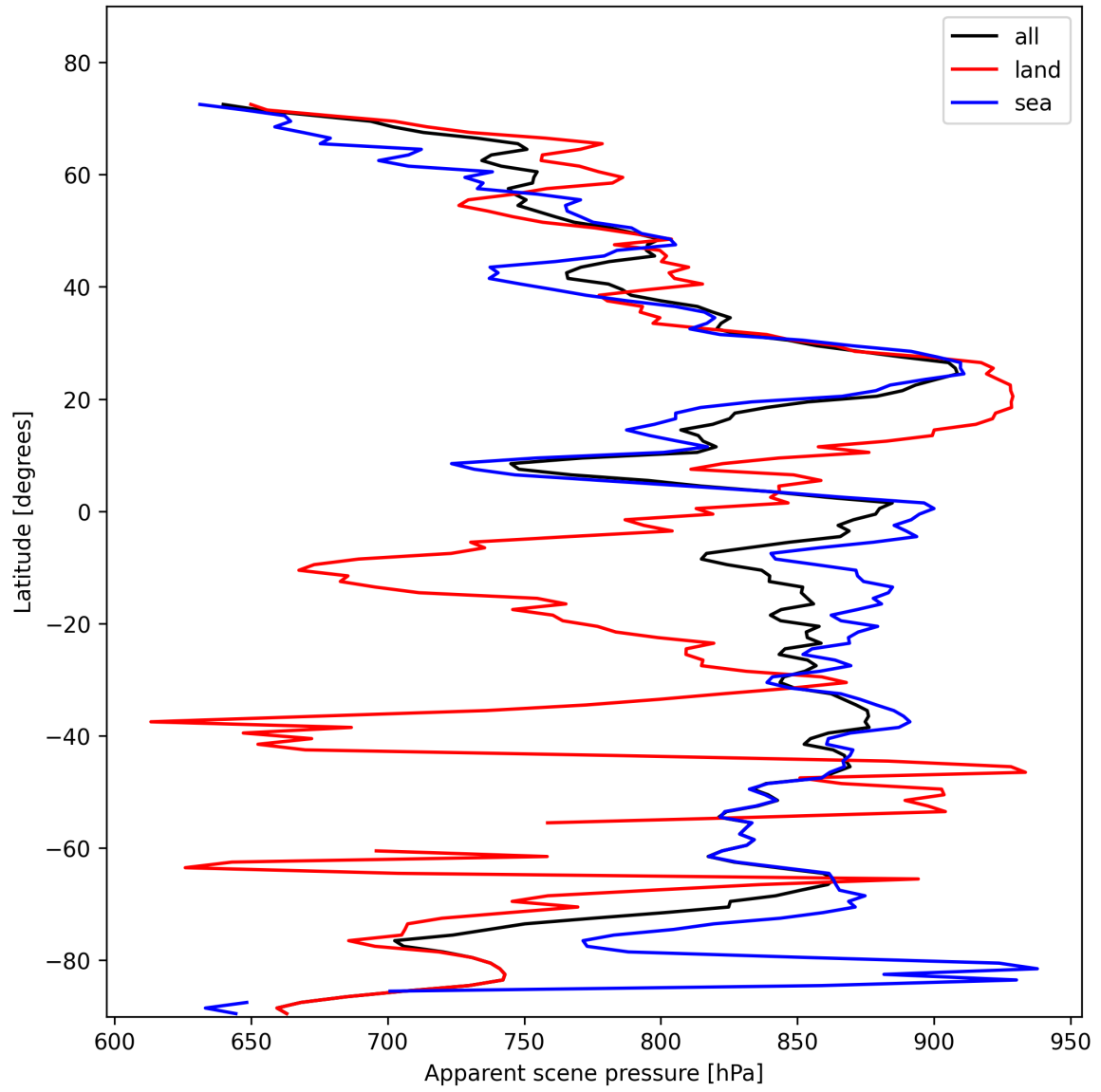
Figure 19: Zonal average of “Apparent scene pressure” for 2025-11-02 to 2025-11-04.
