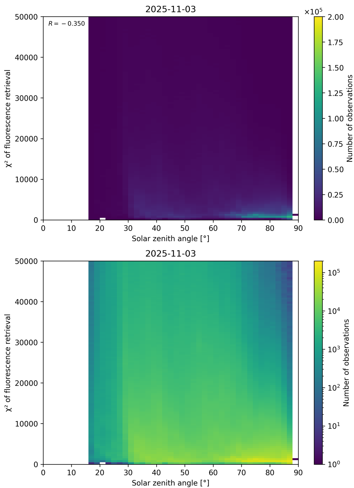
Figure 109: Scatter density plot of “Solar zenith angle” against “ \chi^2 of fluorescence retrieval” for 2025-11-02 to 2025-11-04.
