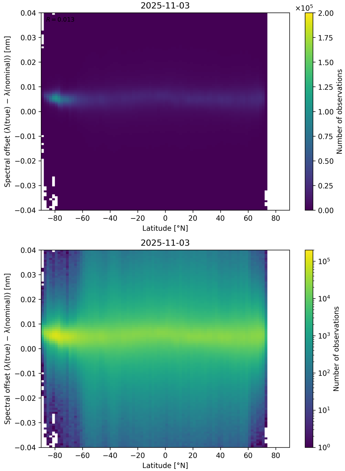
Figure 96: Scatter density plot of “Latitude” against “Spectral offset ( \lambda_{\text{true}} - \lambda_{\text{nominal}} )” for 2025-11-02 to 2025-11-04.
