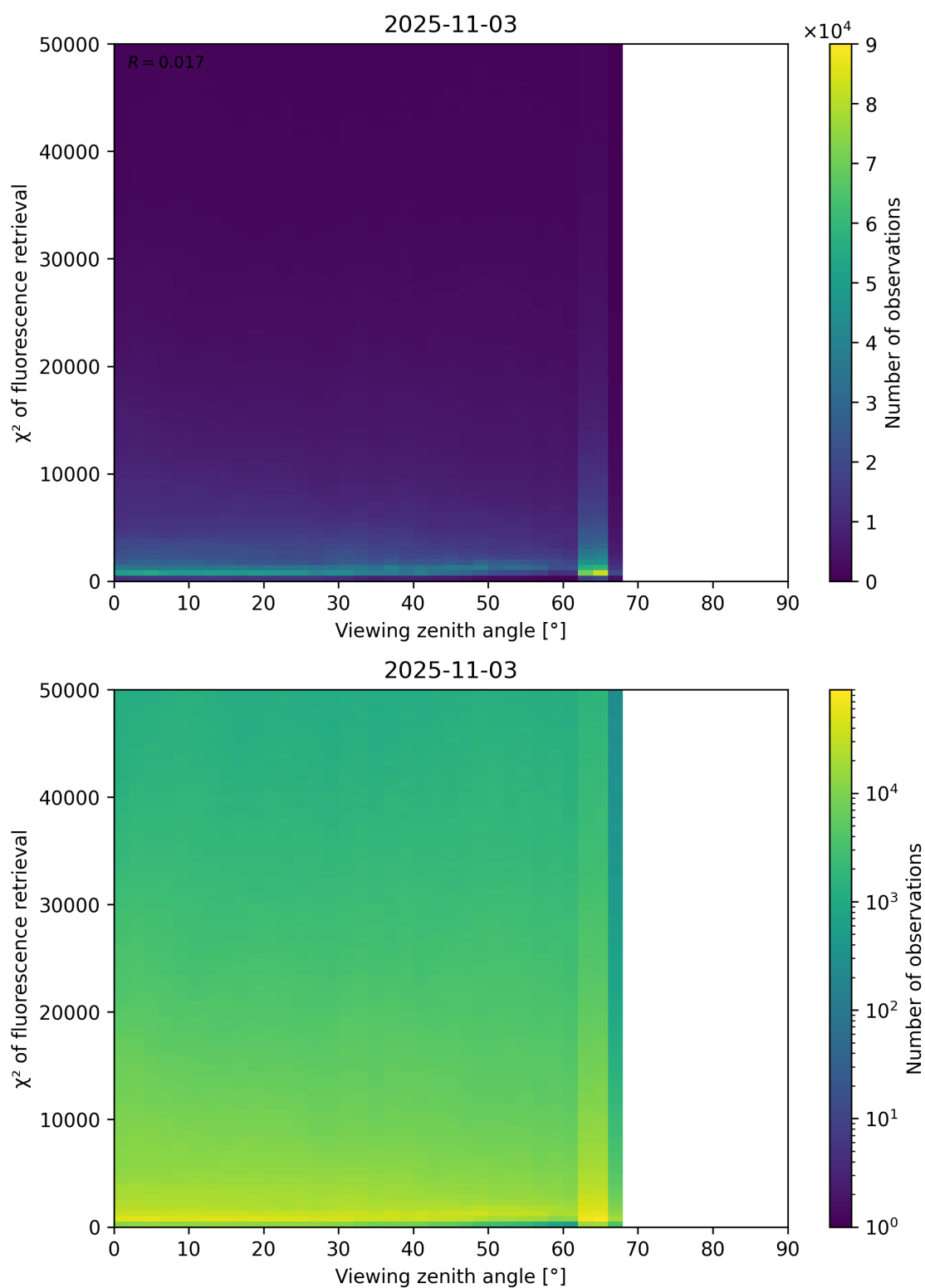
Figure 119: Scatter density plot of “Viewing zenith angle” against “ \chi^2 of fluorescence retrieval” for 2025-11-02 to 2025-11-04.
