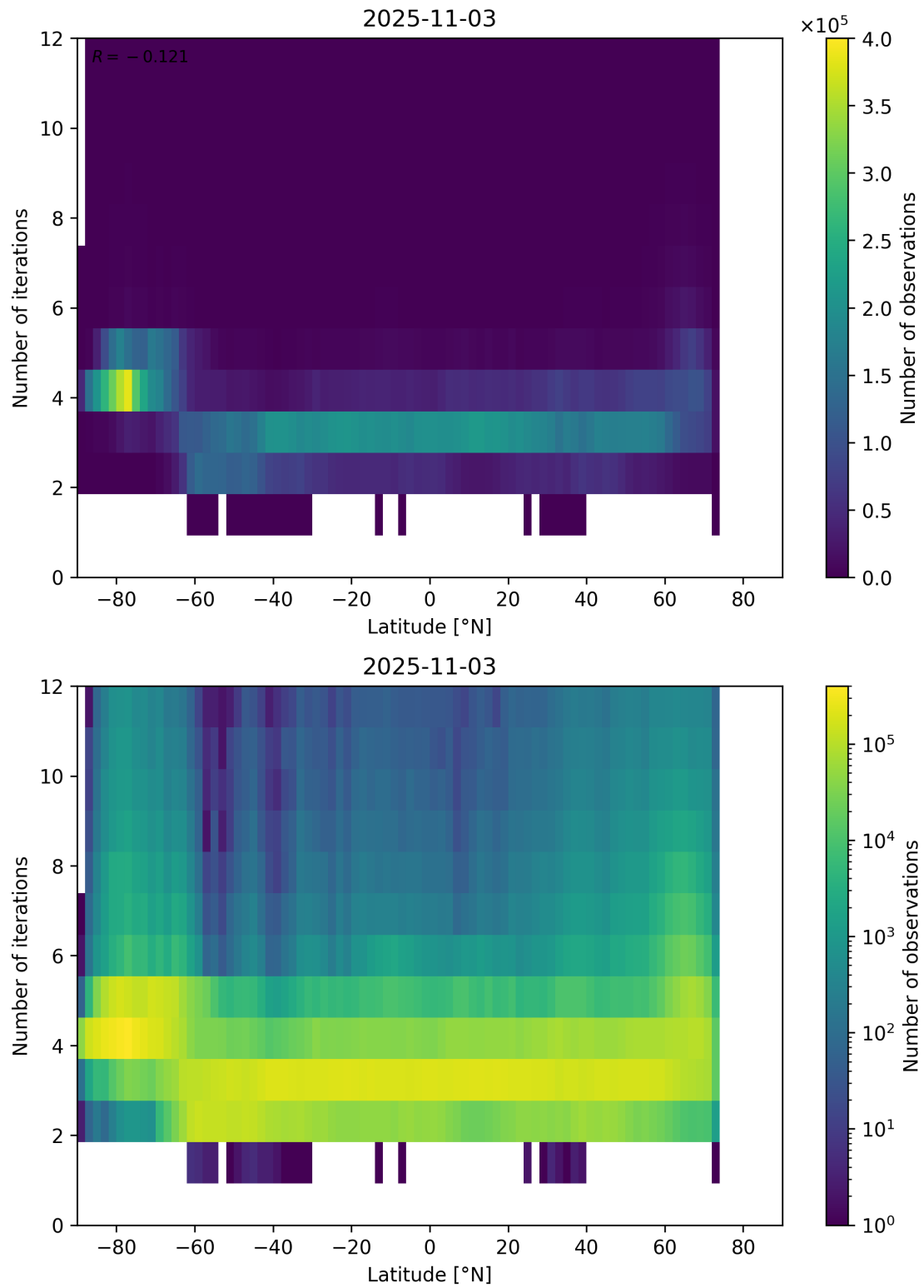
Figure 93: Scatter density plot of “Latitude” against “Number of iterations” for 2025-11-02 to 2025-11-04.
