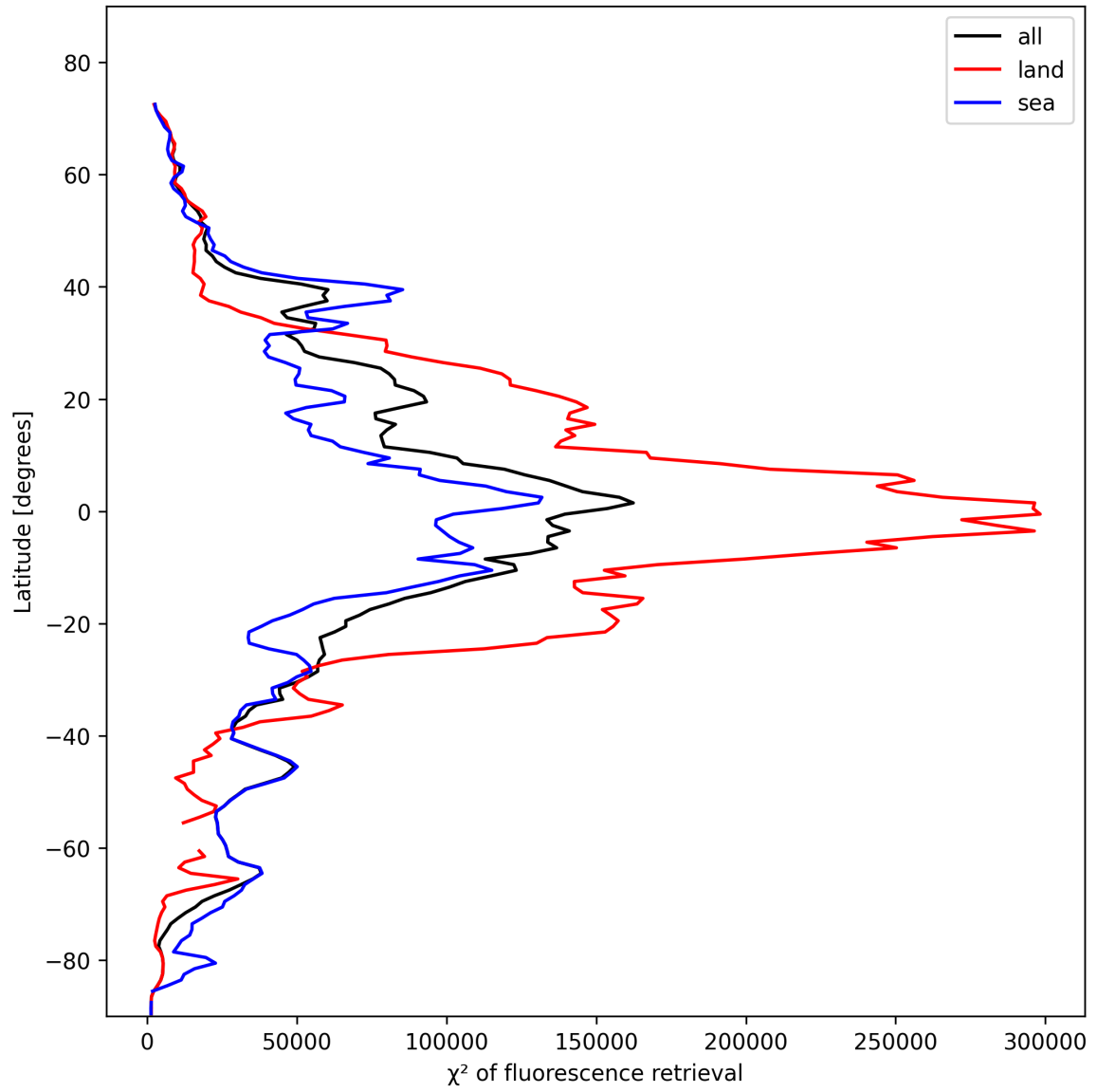
Figure 25: Zonal average of “ \chi^2 of fluorescence retrieval” for 2025-11-02 to 2025-11-04.
