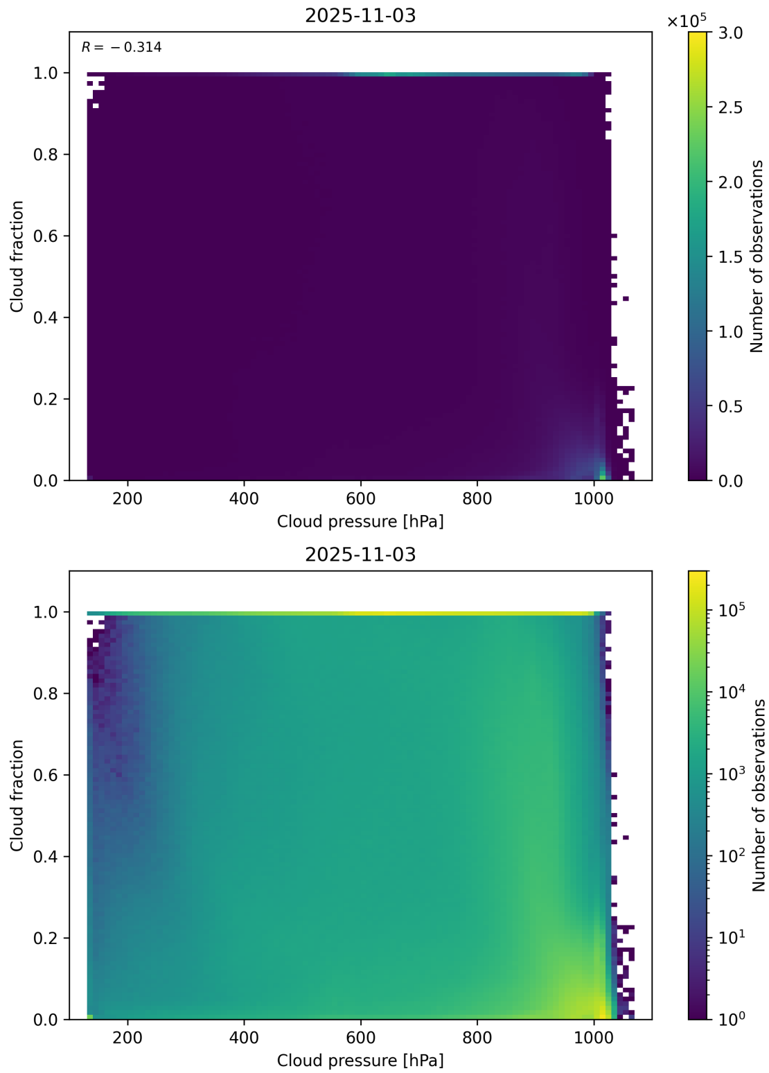
Figure 79: Scatter density plot of “Cloud pressure” against “Cloud fraction” for 2025-11-02 to 2025-11-04.
