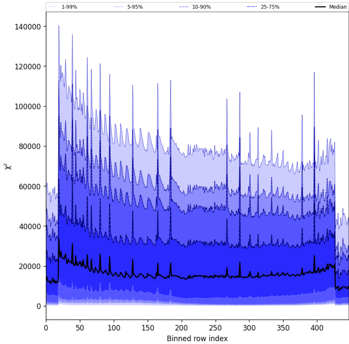
Figure 55: Along track statistics of “ \chi^2 ” for 2025-11-02 to 2025-11-04
