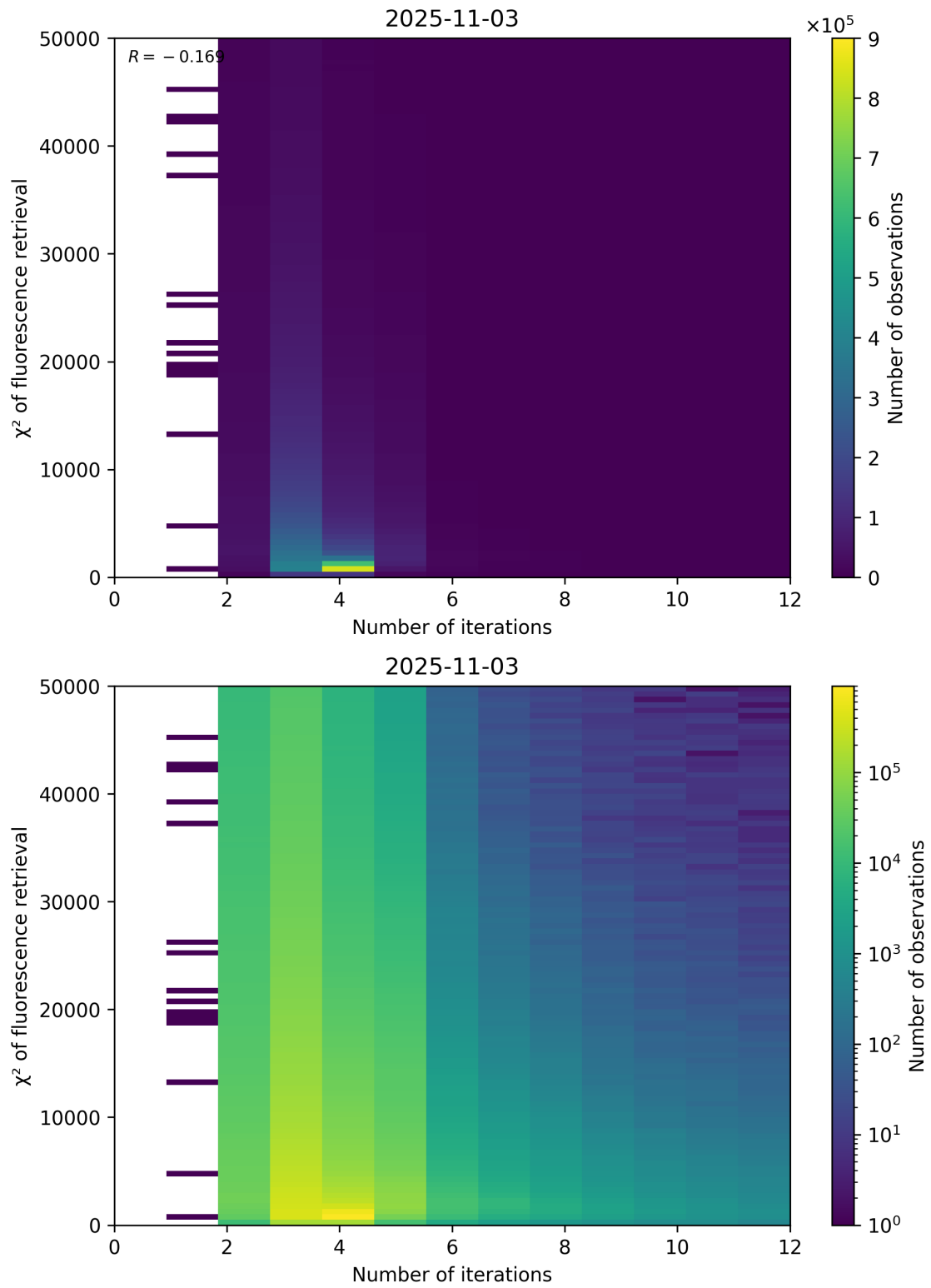
Figure 97: Scatter density plot of “Number of iterations” against “ \chi^2 of fluorescence retrieval” for 2025-11-02 to 2025-11-04.
