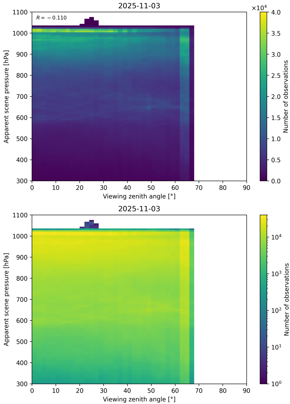
Figure 118: Scatter density plot of “Viewing zenith angle” against “Apparent scene pressure” for 2025-11-02 to 2025-11-04.
