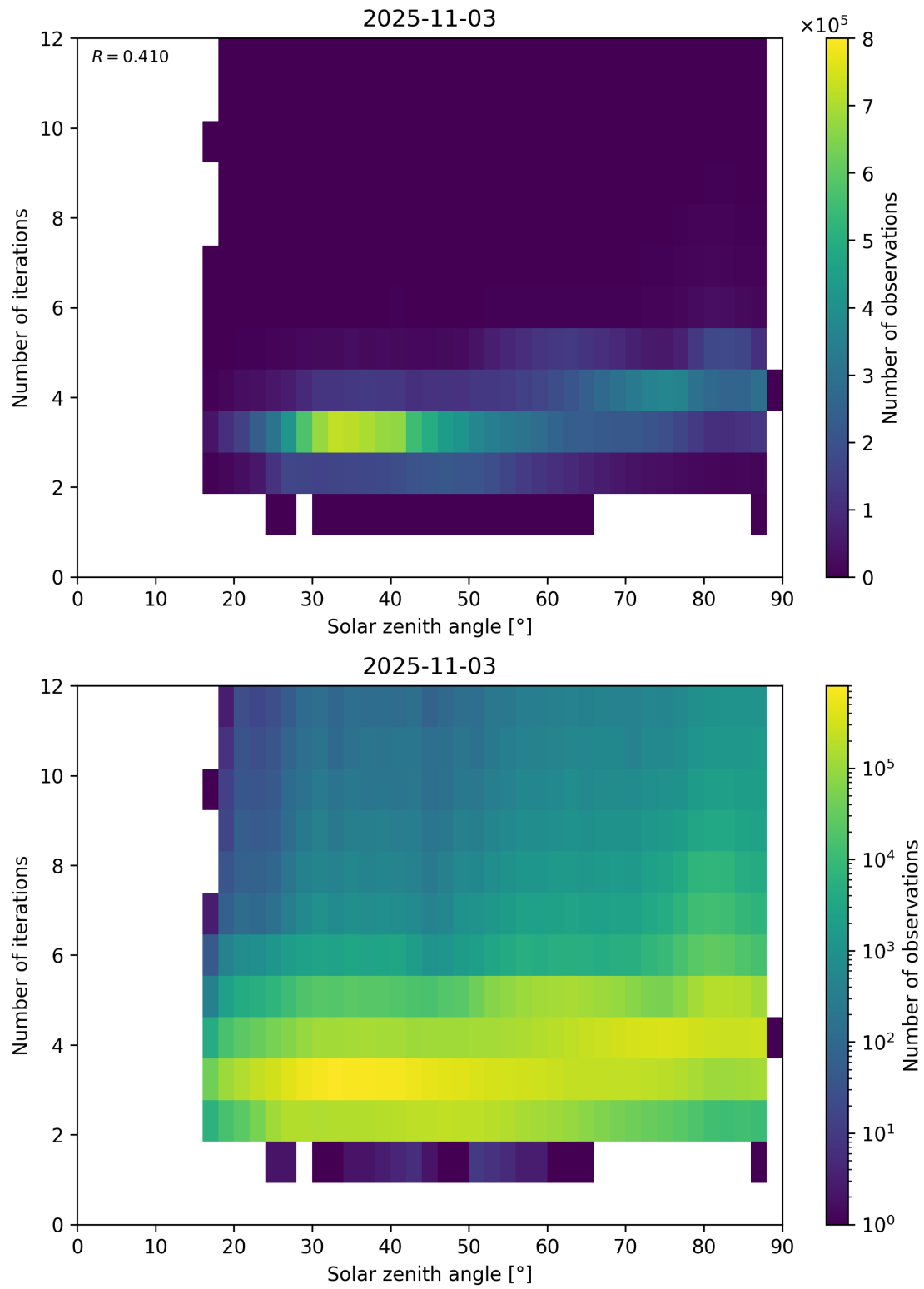
Figure 114: Scatter density plot of “Solar zenith angle” against “Number of iterations” for 2025-11-02 to 2025-11-04.
