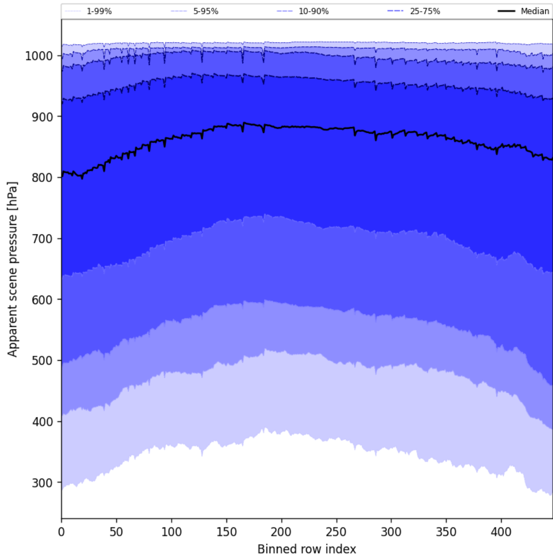
Figure 53: Along track statistics of “Apparent scene pressure” for 2025-11-02 to 2025-11-04
