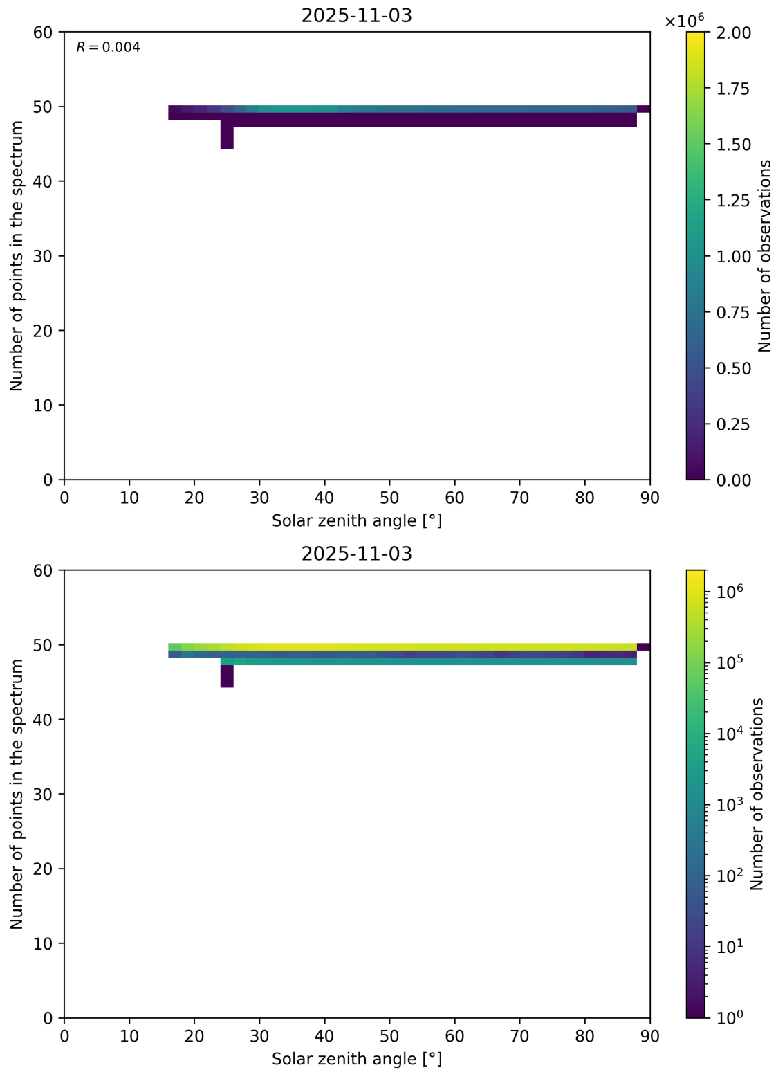
Figure 115: Scatter density plot of “Solar zenith angle” against “Number of points in the spectrum” for 2025-11-02 to 2025-11-04.
