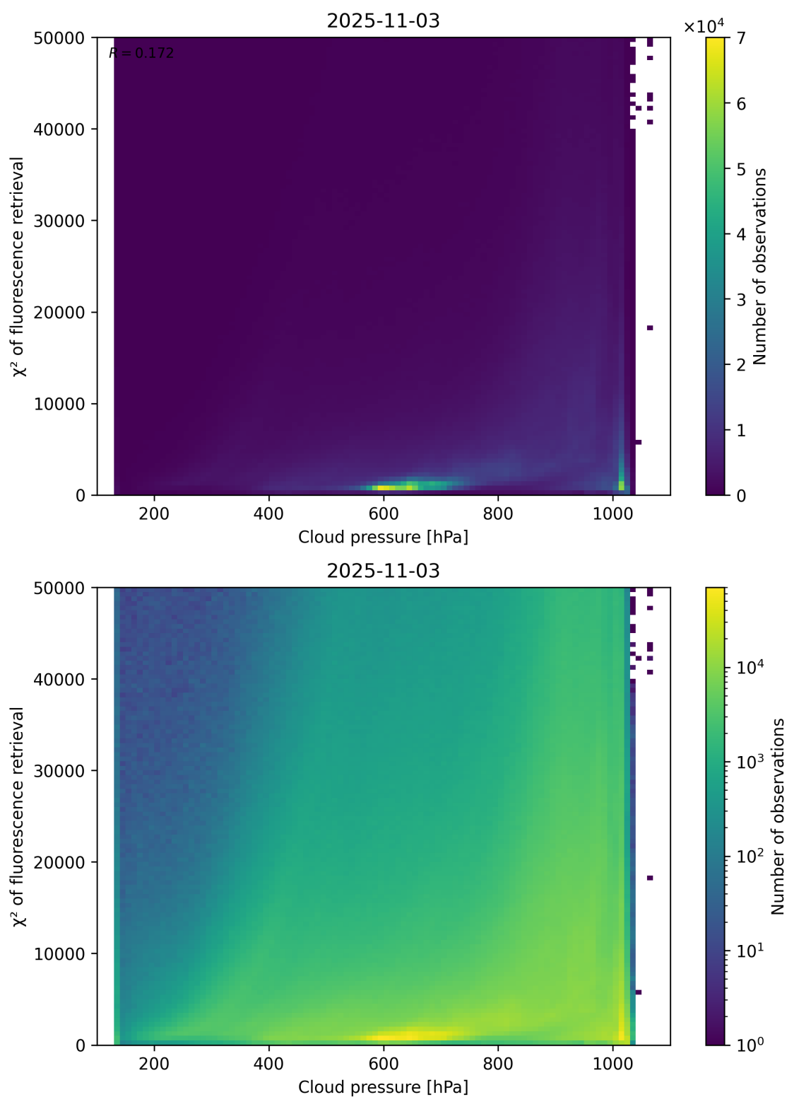
Figure 78: Scatter density plot of “Cloud pressure” against “ \chi^2 of fluorescence retrieval” for 2025-11-02 to 2025-11-04.
