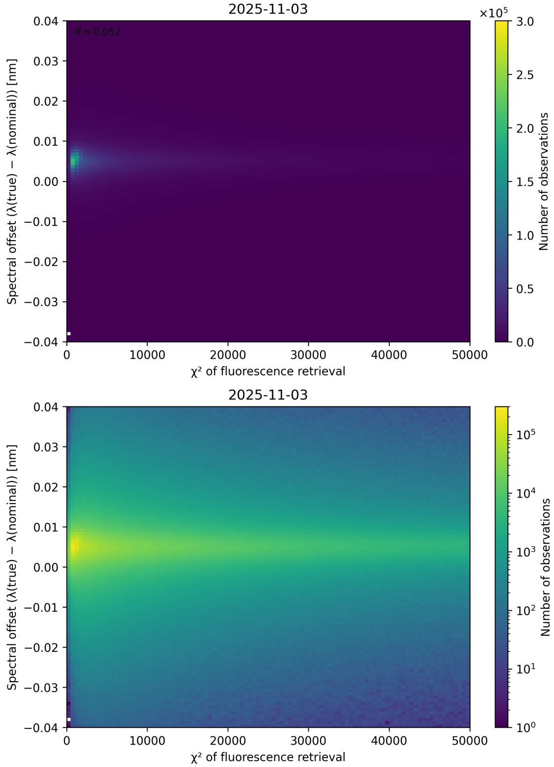
Figure 69: Scatter density plot of “ \chi^2 of fluorescence retrieval” against “Spectral offset ( \lambda_{\text{true}} - \lambda_{\text{nominal}} )” for 2025-11-02 to 2025-11-04.
