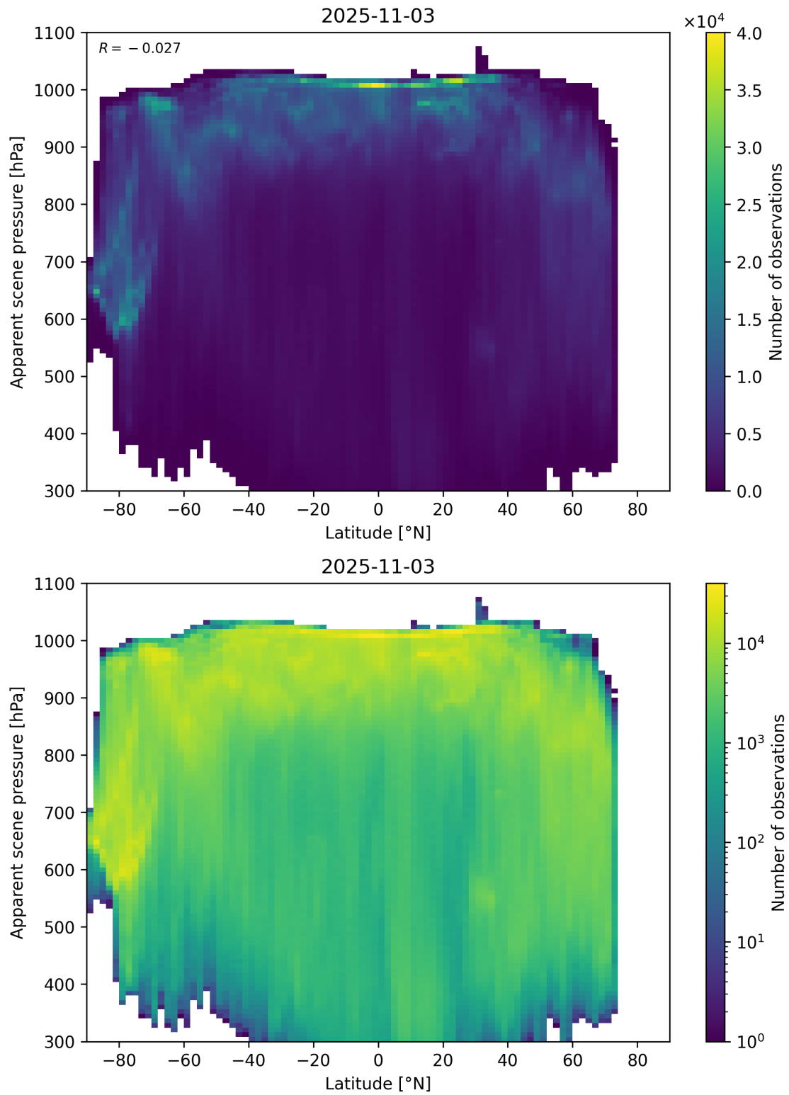
Figure 88: Scatter density plot of “Latitude” against “Apparent scene pressure” for 2025-11-02 to 2025-11-04.
