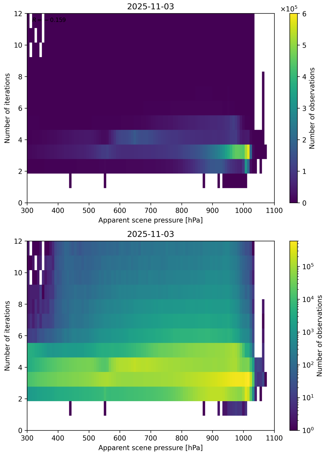
Figure 65: Scatter density plot of “Apparent scene pressure” against “Number of iterations” for 2025-11-02 to 2025-11-04.
