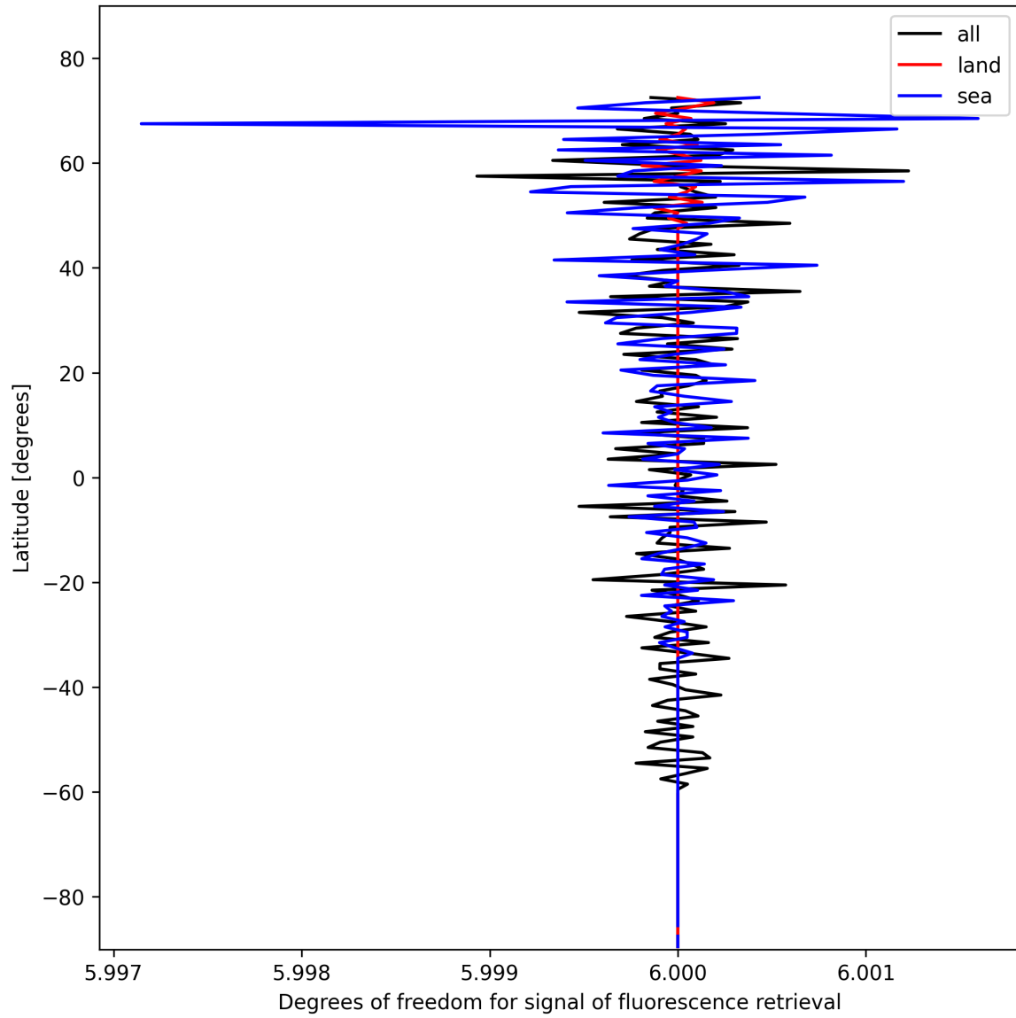
Figure 26: Zonal average of “Degrees of freedom for signal of fluorescence retrieval” for 2025-11-02 to 2025-11-04.
