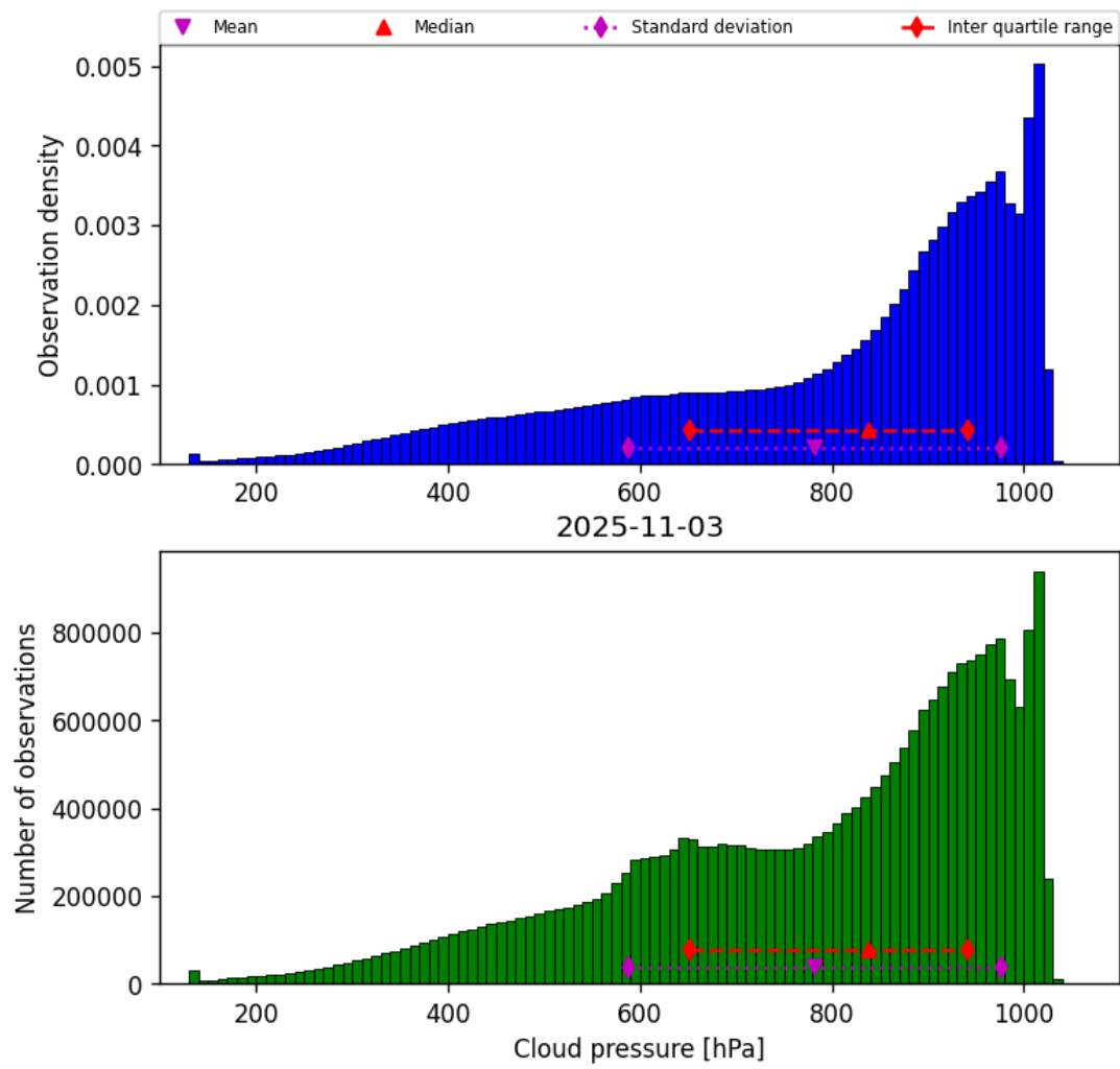
Figure 30: Histogram of “Cloud pressure” for 2025-11-02 to 2025-11-04
