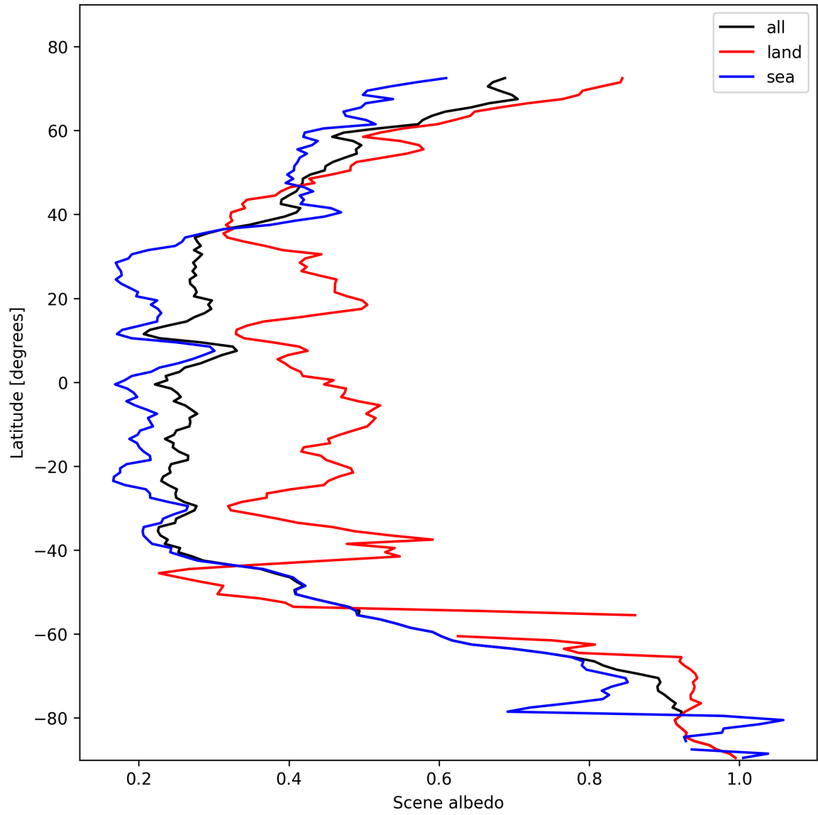
Figure 17: Zonal average of “Scene albedo” for 2025-11-02 to 2025-11-04.
