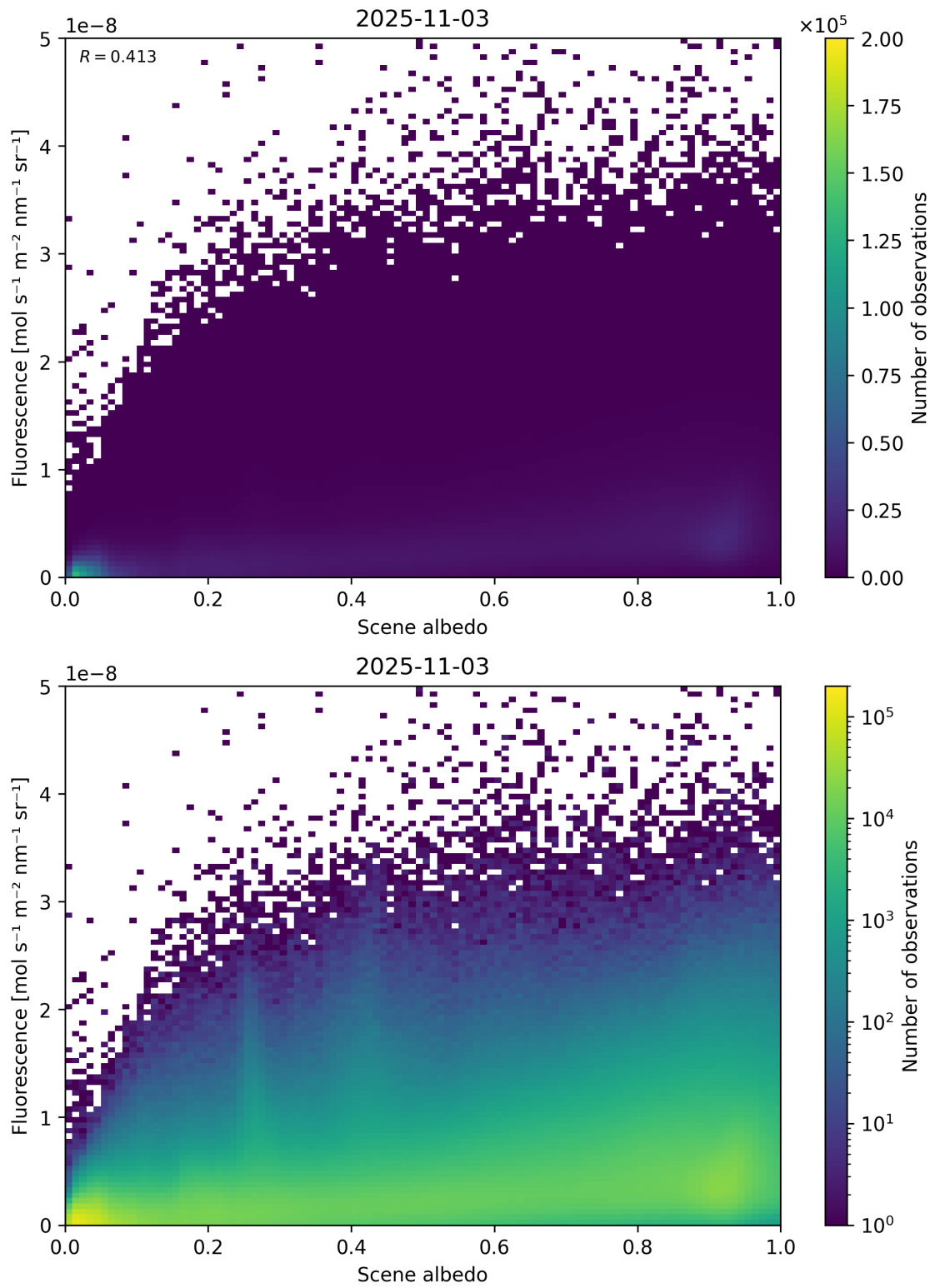
Figure 104: Scatter density plot of “Scene albedo” against “Fluorescence” for 2025-11-02 to 2025-11-04.
