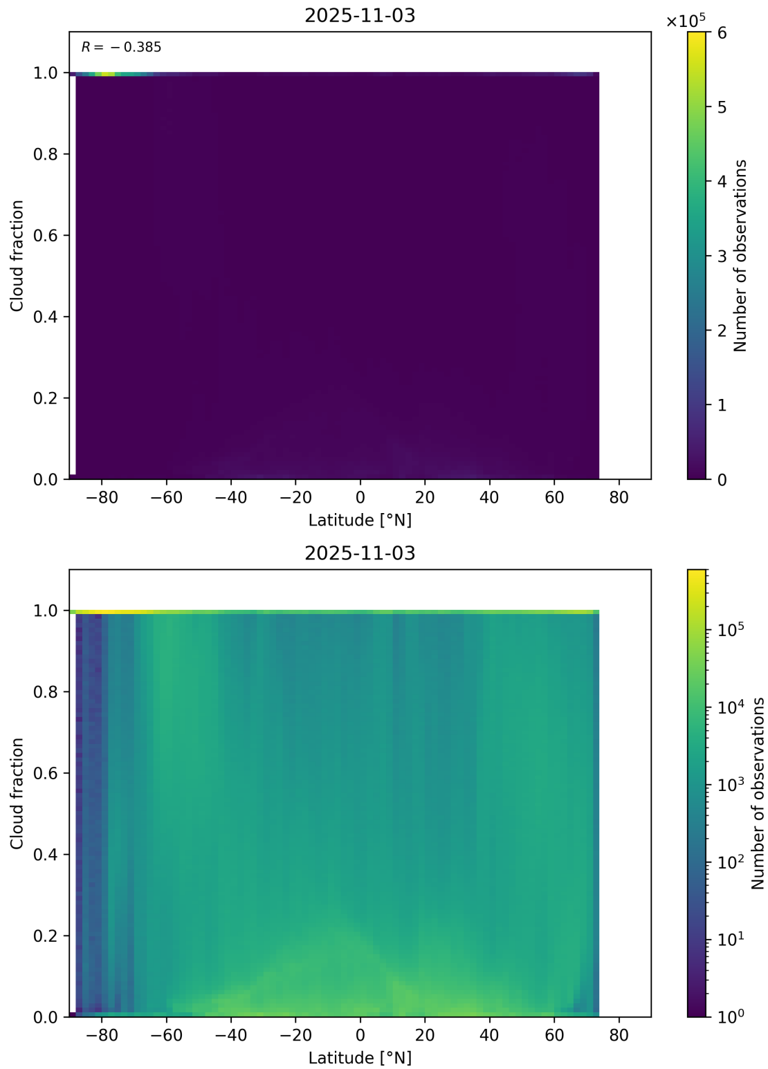
Figure 90: Scatter density plot of “Latitude” against “Cloud fraction” for 2025-11-02 to 2025-11-04.
