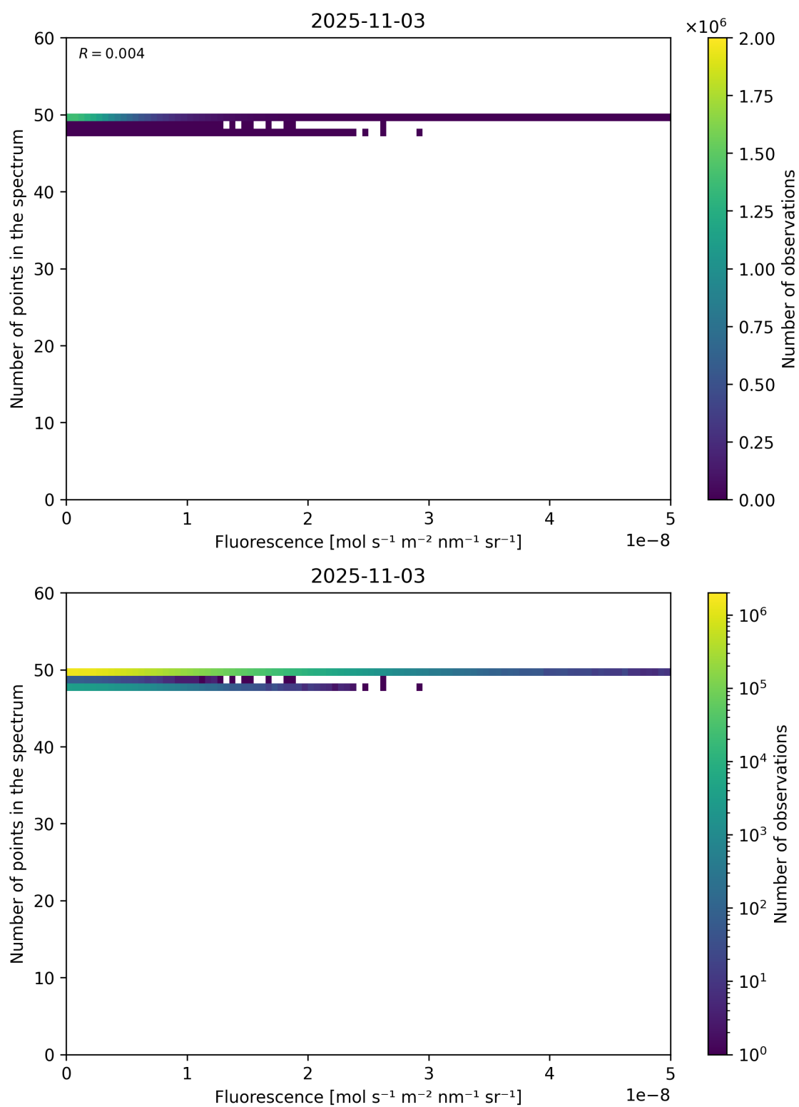
Figure 86: Scatter density plot of “Fluorescence” against “Number of points in the spectrum” for 2025-11-02 to 2025-11-04.
