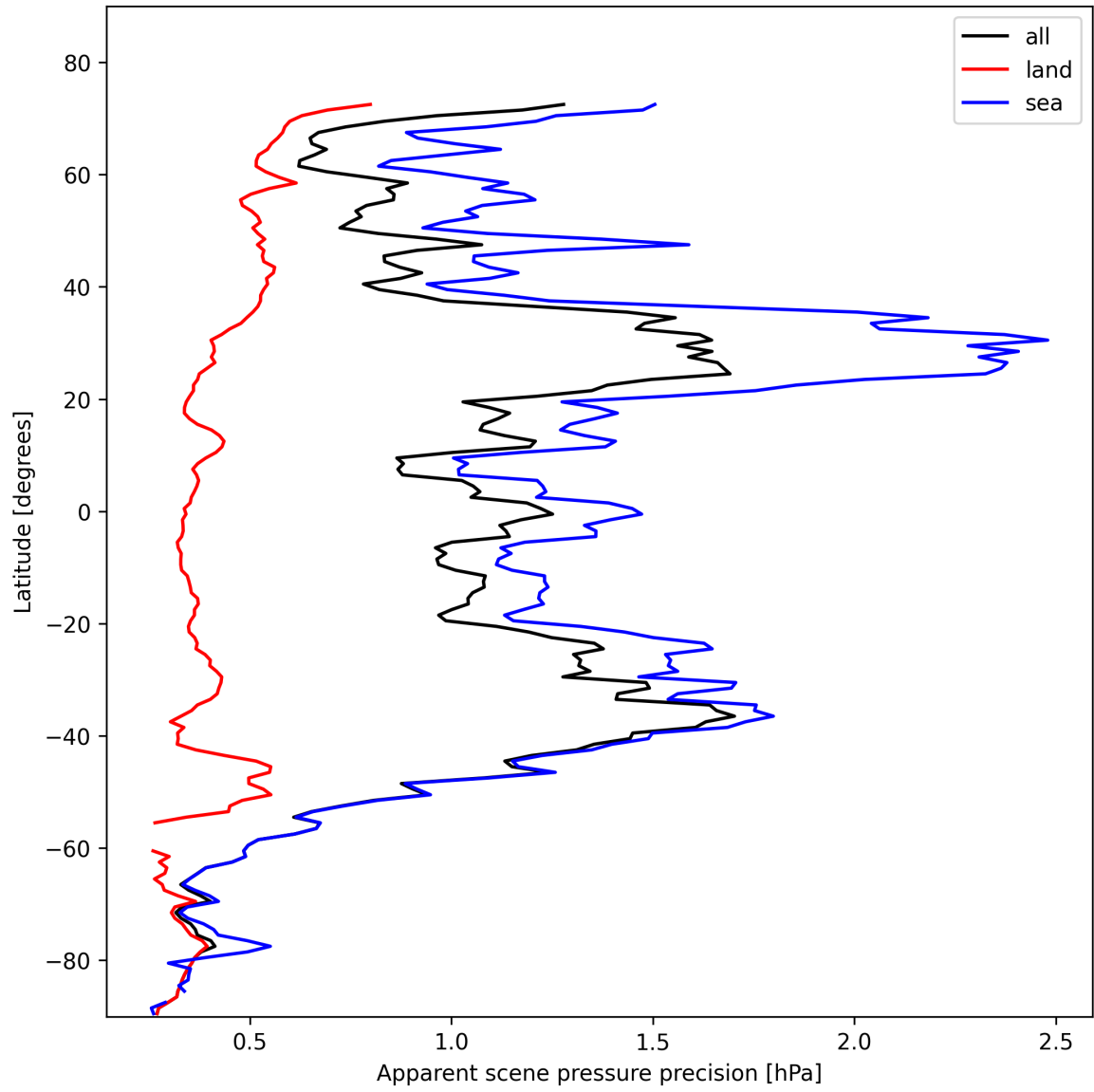
Figure 20: Zonal average of “Apparent scene pressure precision” for 2025-11-02 to 2025-11-04.
