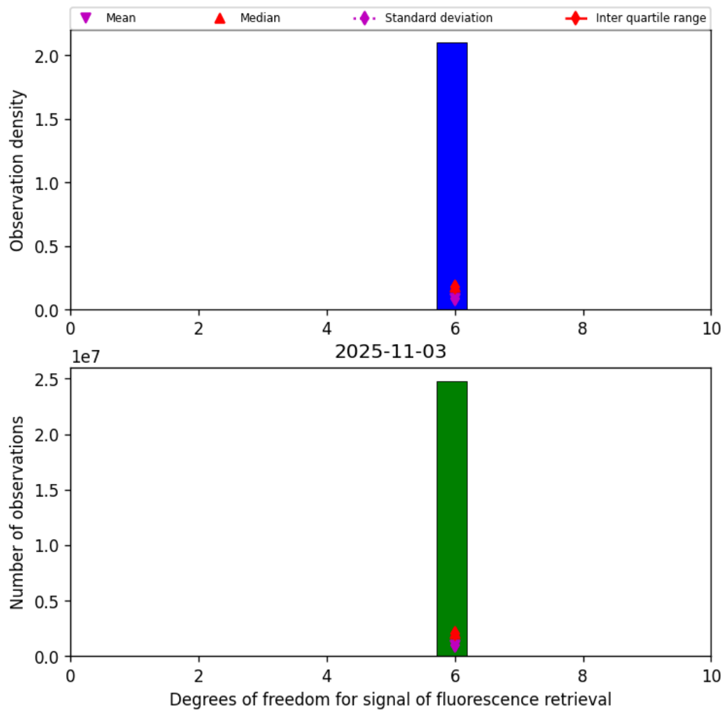
Figure 43: Histogram of "Degrees of freedom for signal of fluorescence retrieval" for 2025-11-02 to 2025-11-04
