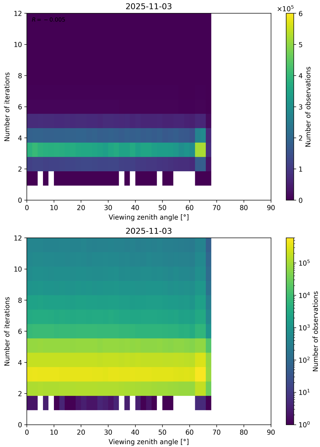
Figure 124: Scatter density plot of “Viewing zenith angle” against “Number of iterations” for 2025-11-02 to 2025-11-04.
