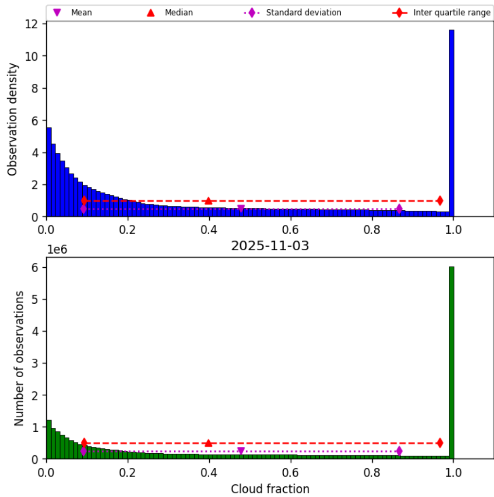
Figure 32: Histogram of “Cloud fraction” for 2025-11-02 to 2025-11-04
