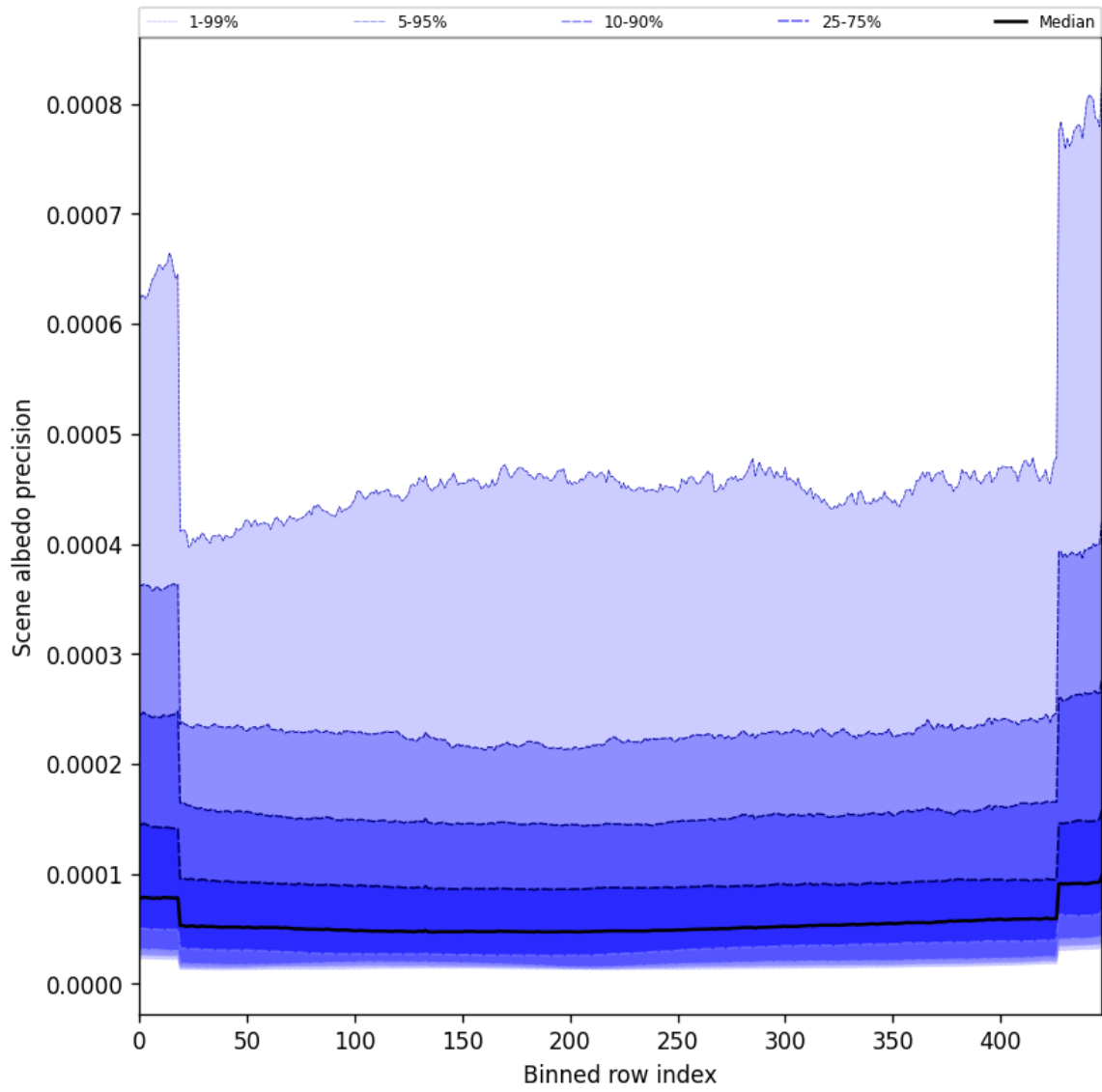
Figure 52: Along track statistics of “Scene albedo precision” for 2025-11-02 to 2025-11-04
