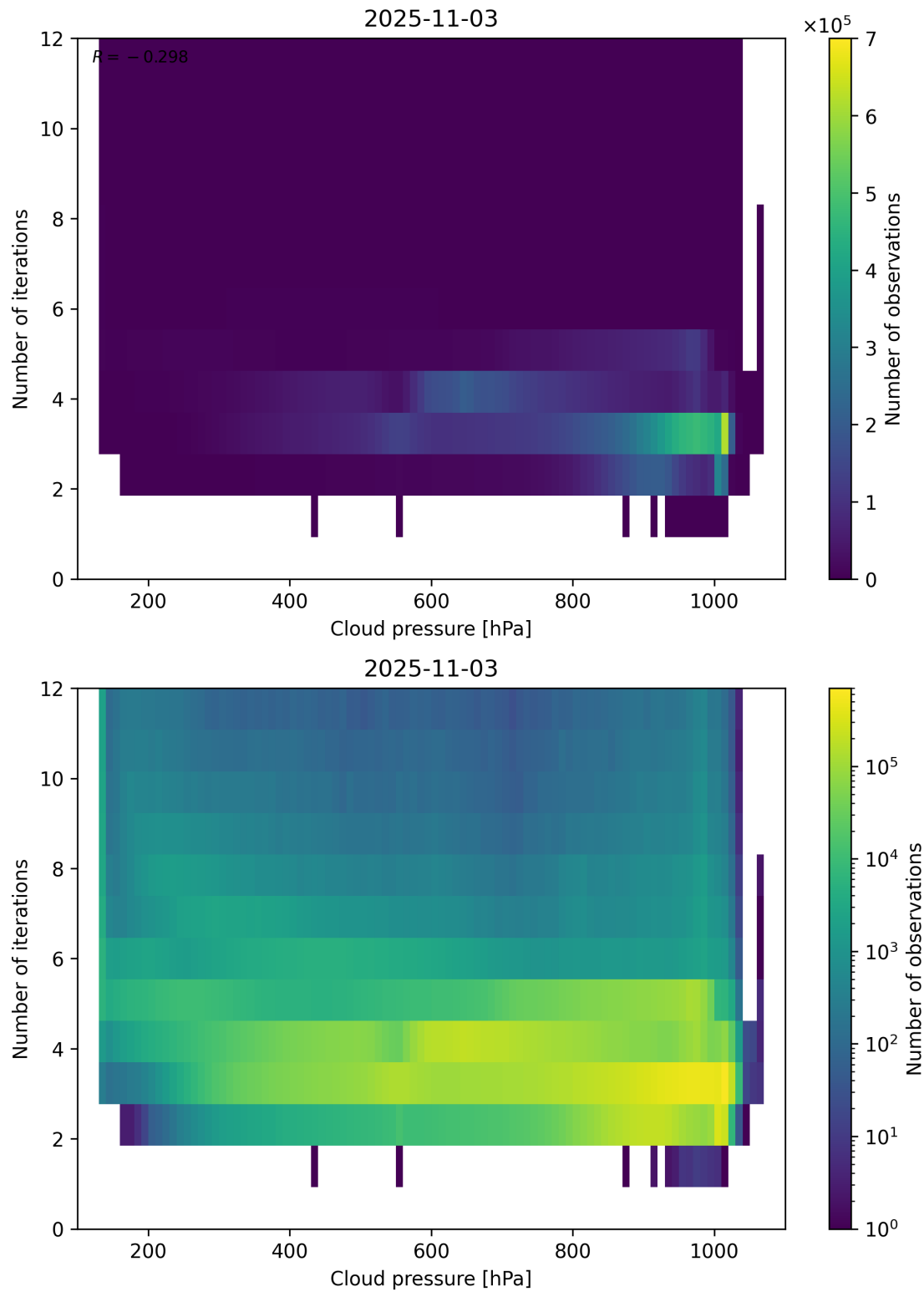
Figure 81: Scatter density plot of “Cloud pressure” against “Number of iterations” for 2025-11-02 to 2025-11-04.
