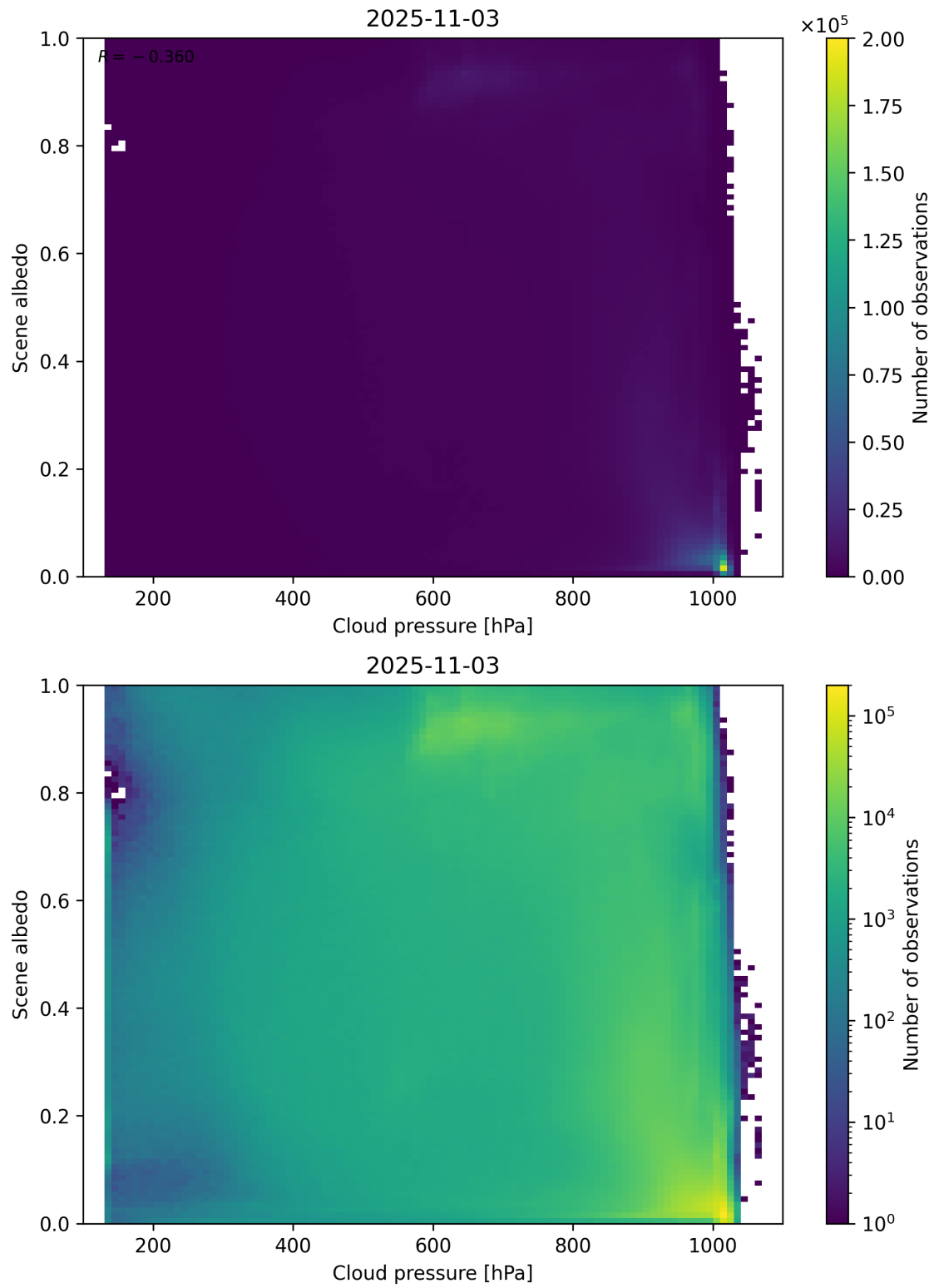
Figure 83: Scatter density plot of “Cloud pressure” against “Scene albedo” for 2025-11-02 to 2025-11-04.
