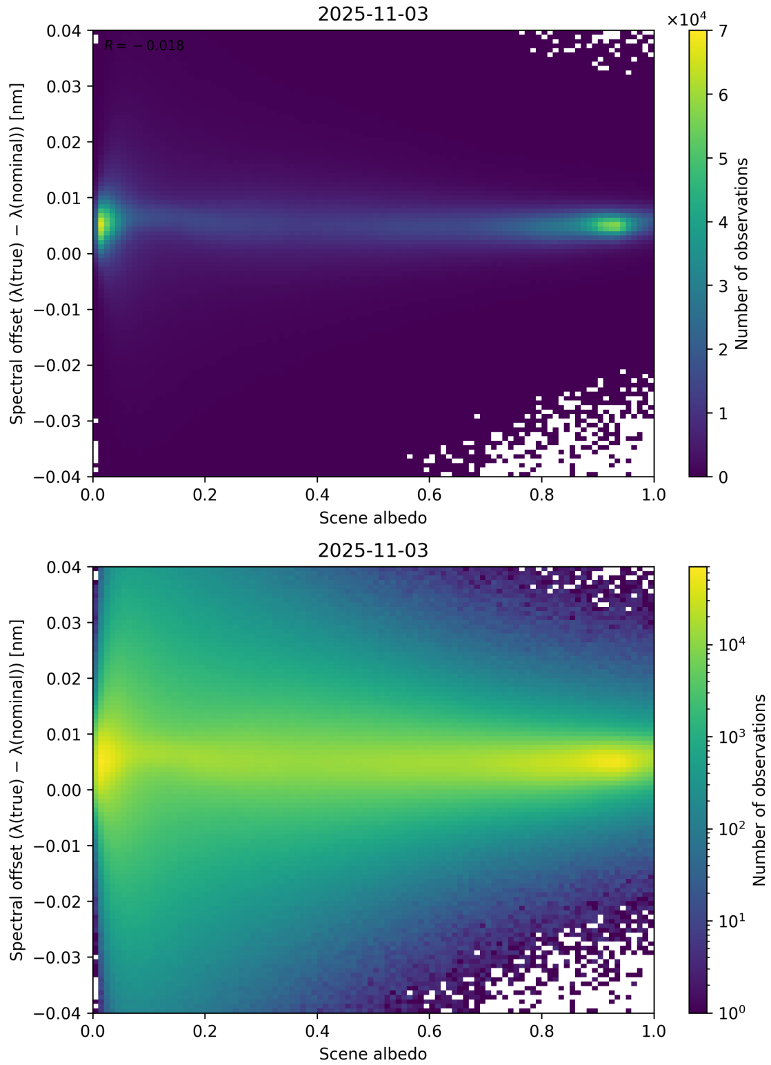
Figure 107: Scatter density plot of “Scene albedo” against “Spectral offset ( \lambda_{\text{true}} - \lambda_{\text{nominal}} )” for 2025-11-02 to 2025-11-04.
