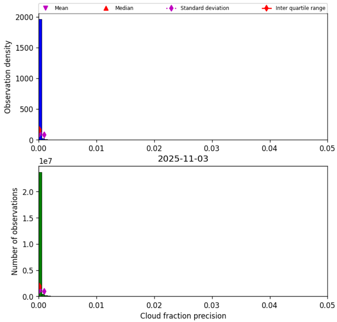
Figure 33: Histogram of “Cloud fraction precision” for 2025-11-02 to 2025-11-04
