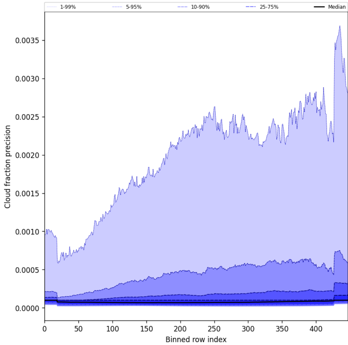
Figure 50: Along track statistics of “Cloud fraction precision” for 2025-11-02 to 2025-11-04
