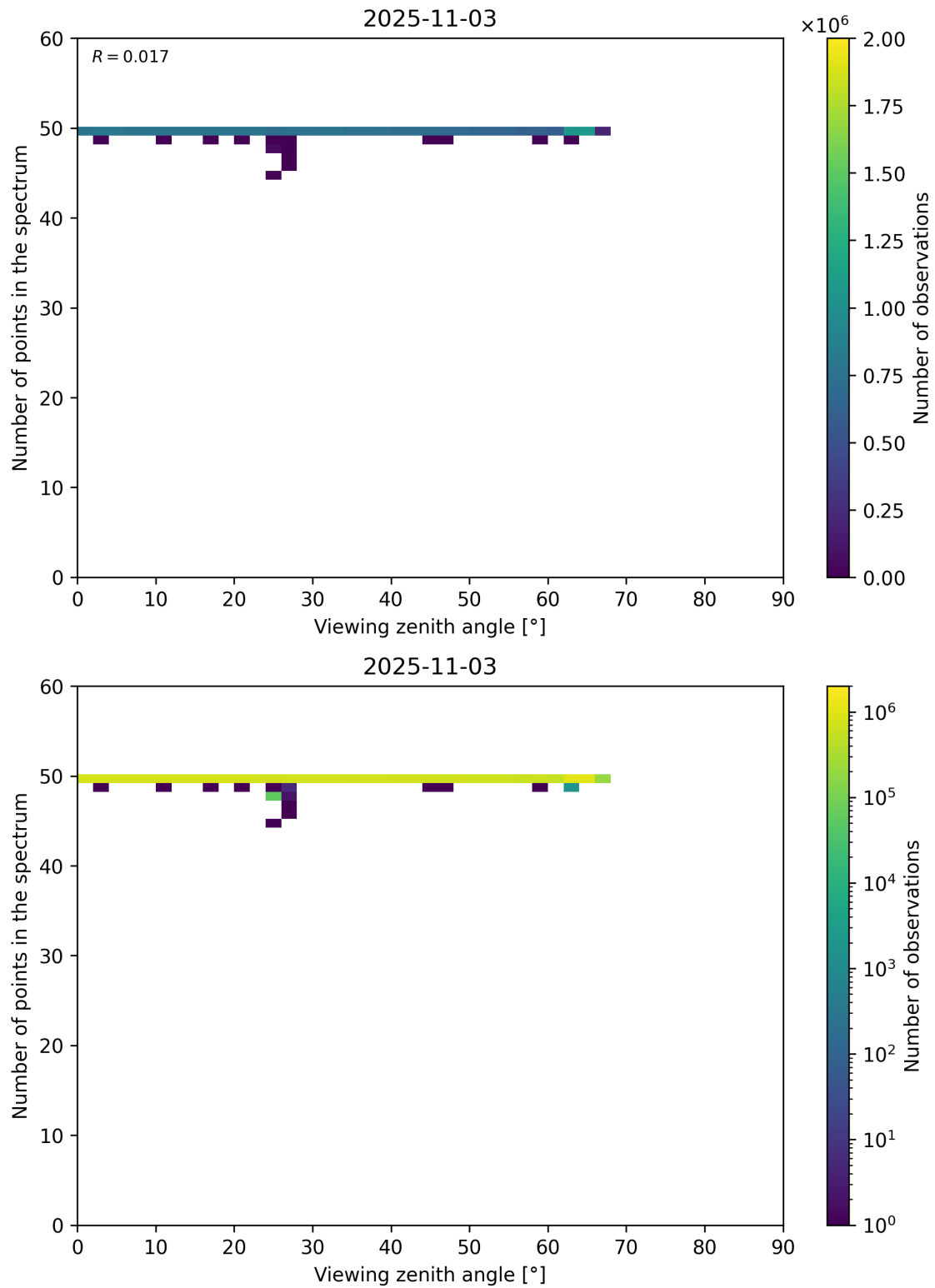
Figure 125: Scatter density plot of “Viewing zenith angle” against “Number of points in the spectrum” for 2025-11-02 to 2025-11-04.
