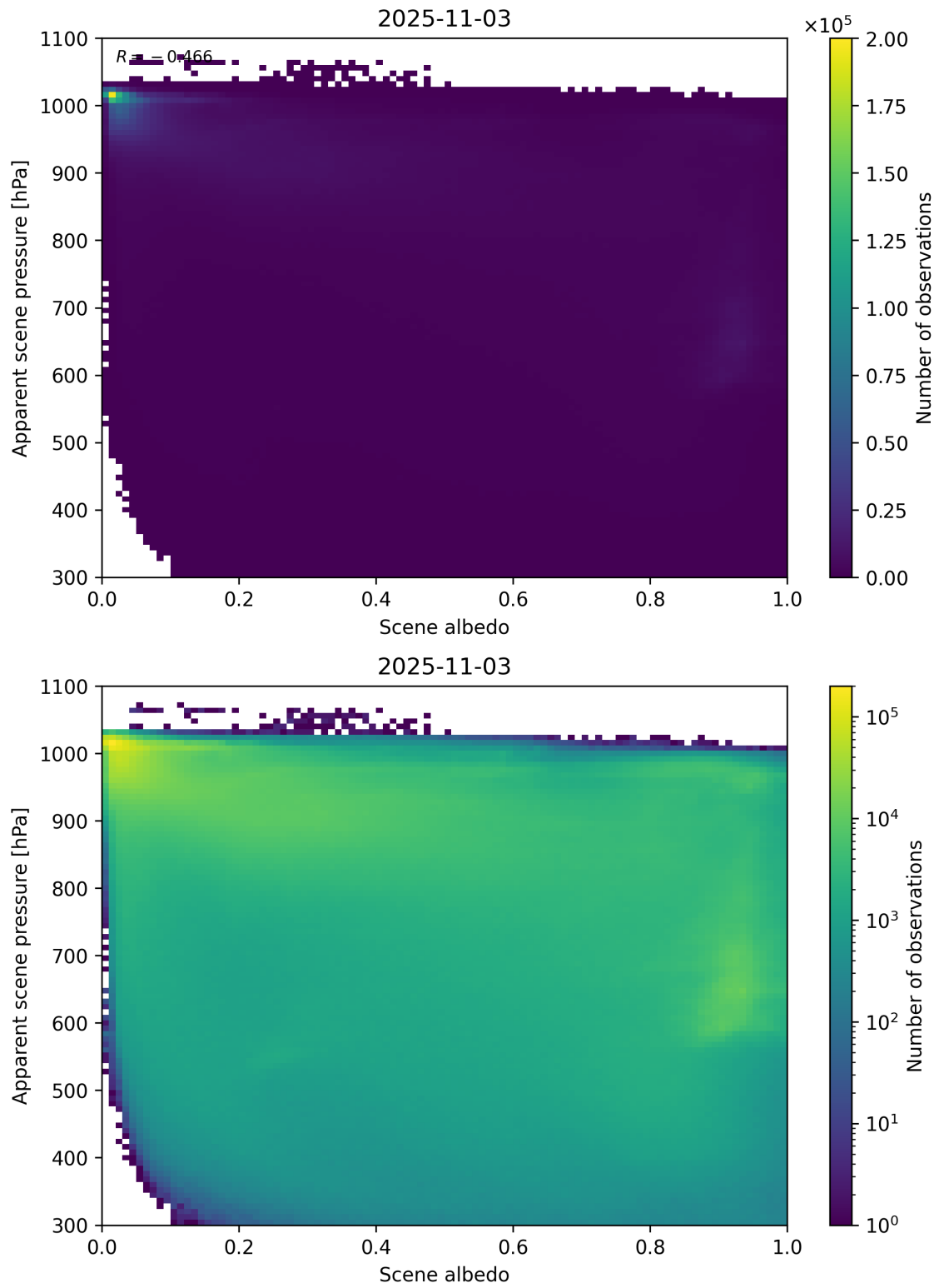
Figure 102: Scatter density plot of “Scene albedo” against “Apparent scene pressure” for 2025-11-02 to 2025-11-04.
