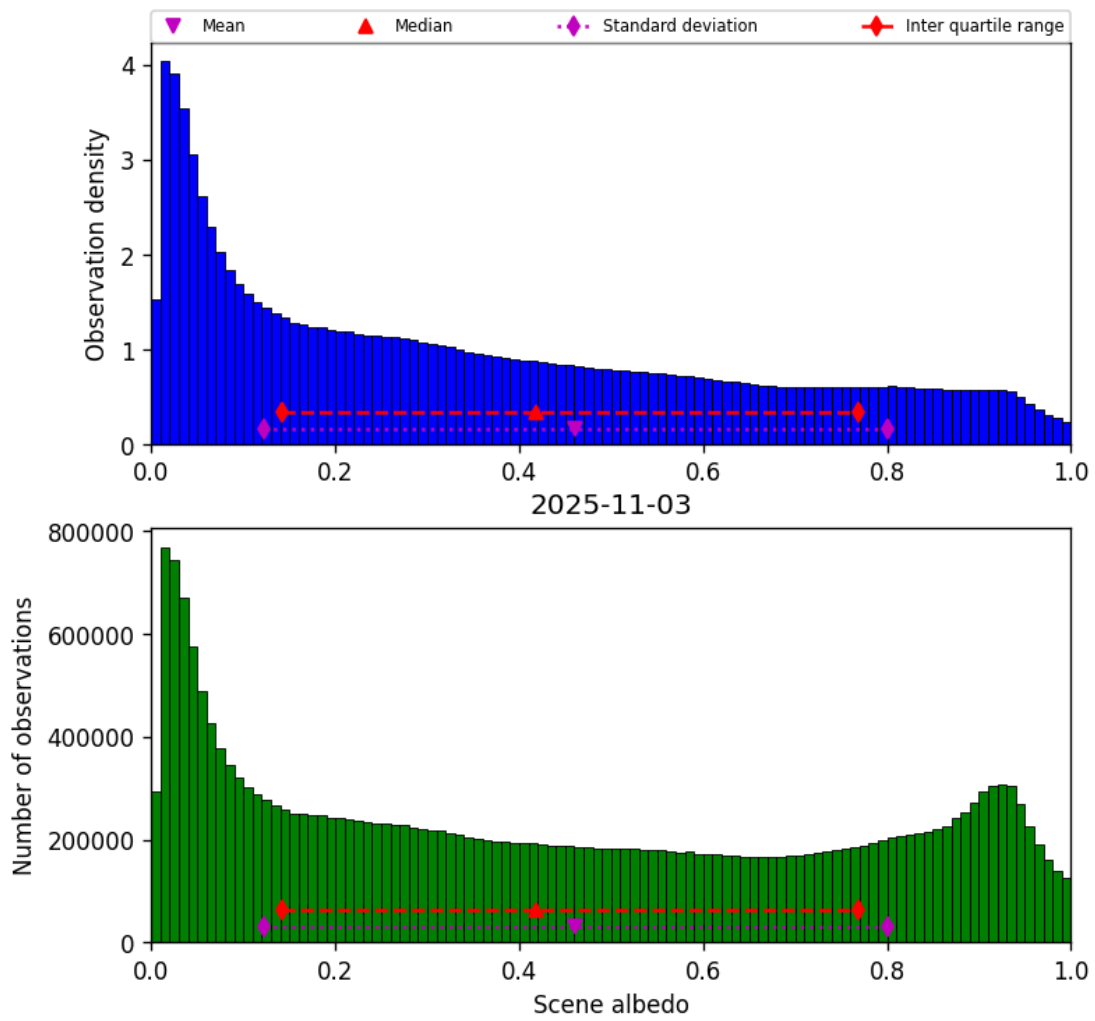
Figure 34: Histogram of “Scene albedo” for 2025-11-02 to 2025-11-04
