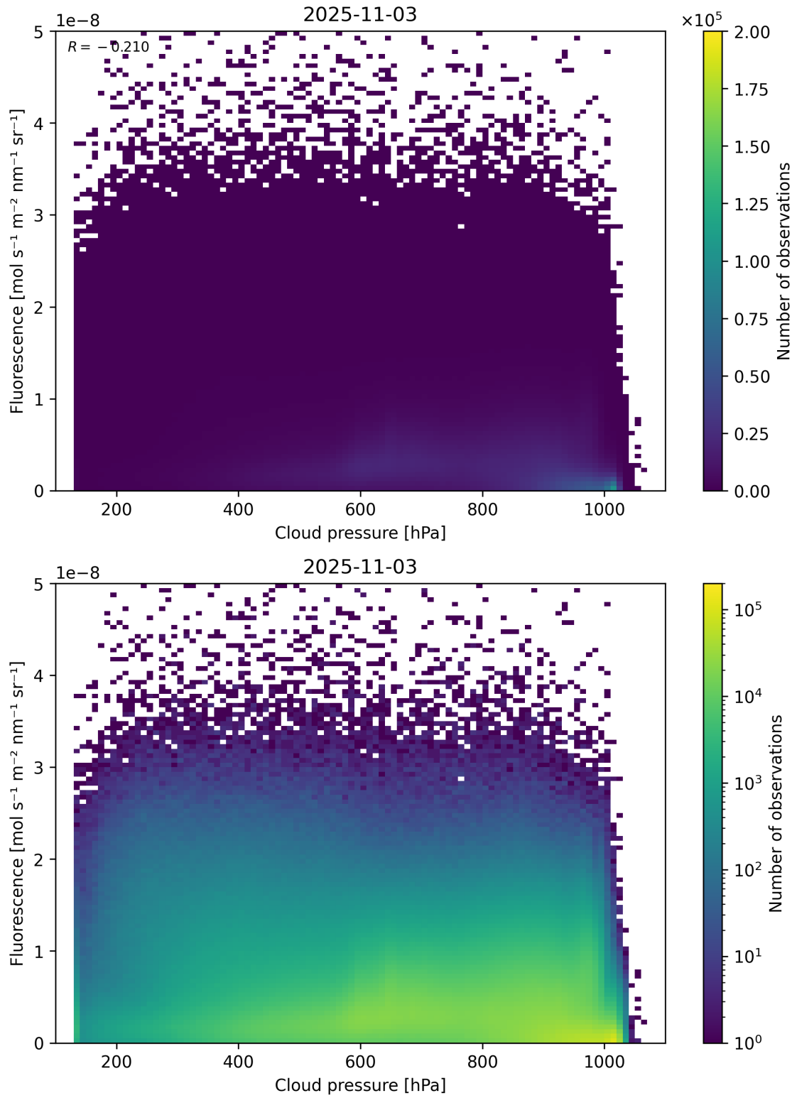
Figure 80: Scatter density plot of “Cloud pressure” against “Fluorescence” for 2025-11-02 to 2025-11-04.
