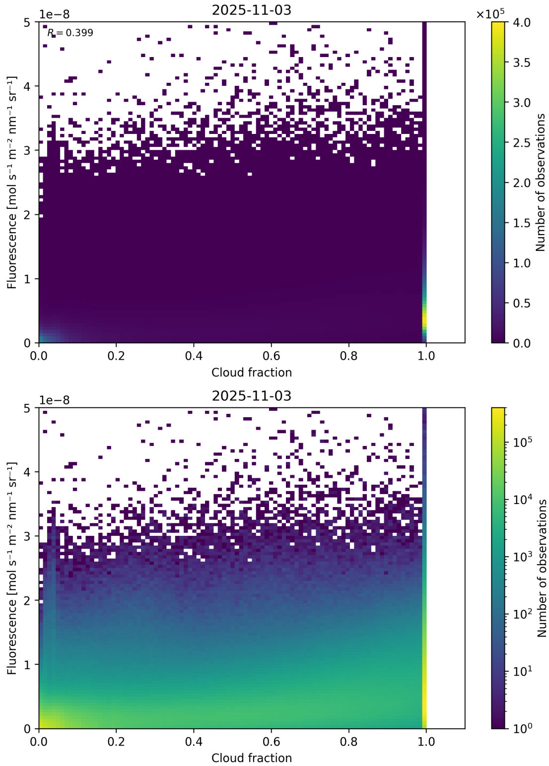
Figure 72: Scatter density plot of “Cloud fraction” against “Fluorescence” for 2025-11-02 to 2025-11-04.
