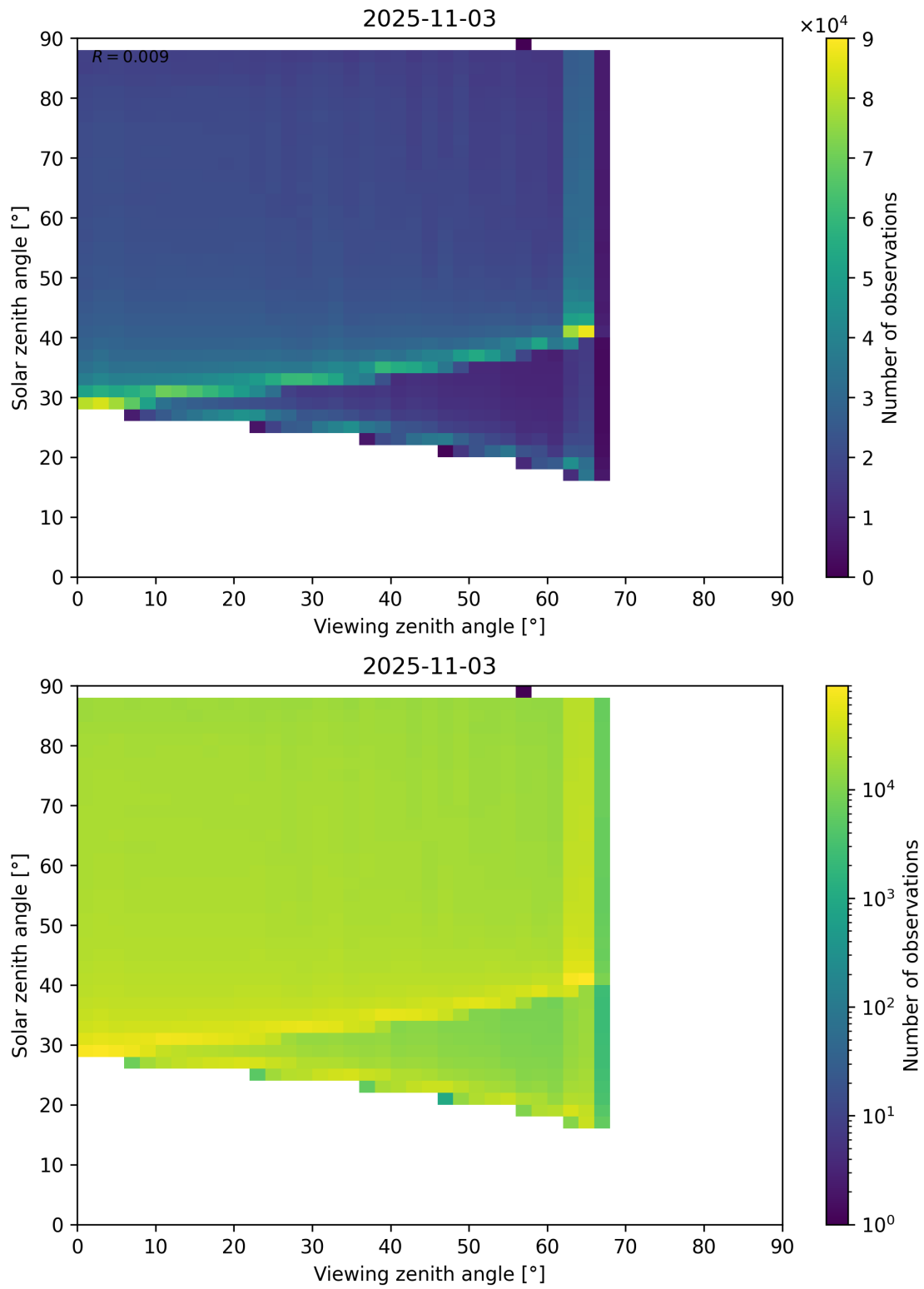
Figure 127: Scatter density plot of “Viewing zenith angle” against “Solar zenith angle” for 2025-11-02 to 2025-11-04.
