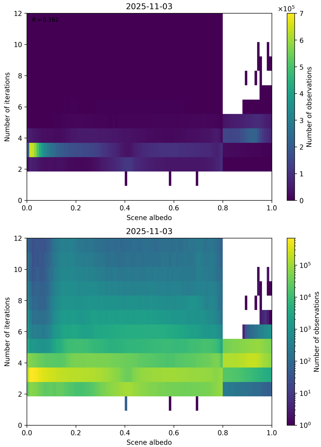
Figure 105: Scatter density plot of “Scene albedo” against “Number of iterations” for 2025-11-02 to 2025-11-04.
