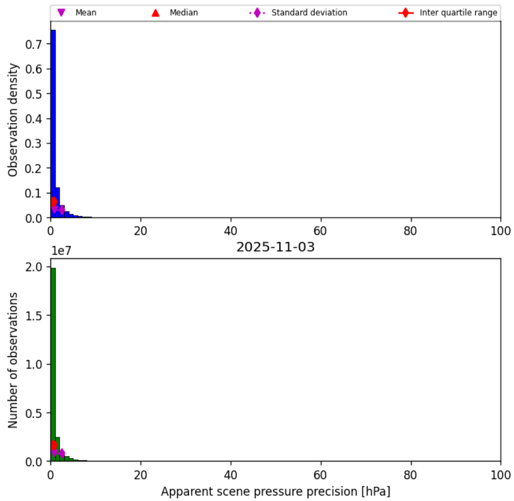
Figure 37: Histogram of “Apparent scene pressure precision” for 2025-11-02 to 2025-11-04
