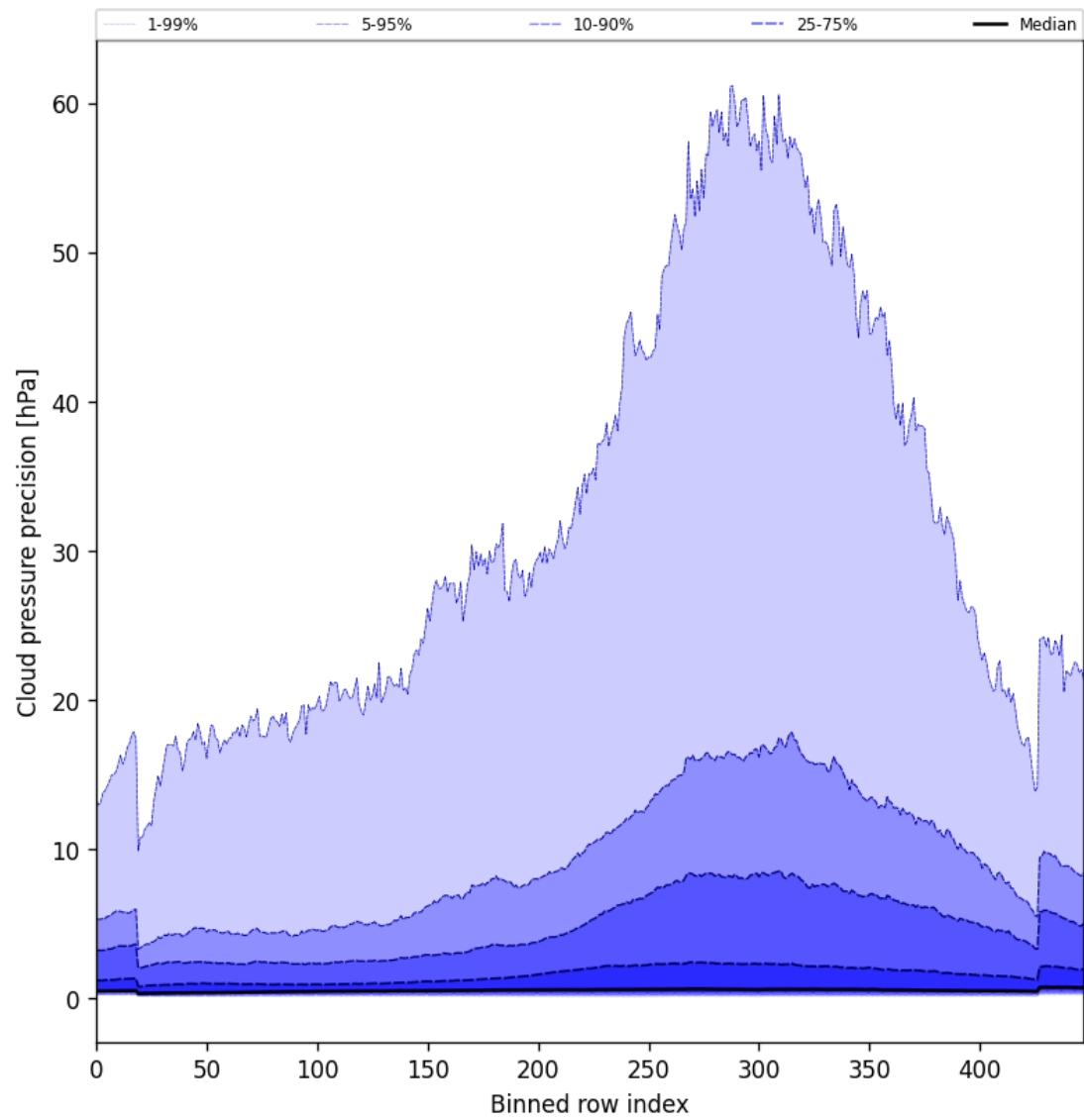
Figure 48: Along track statistics of “Cloud pressure precision” for 2025-11-02 to 2025-11-04
