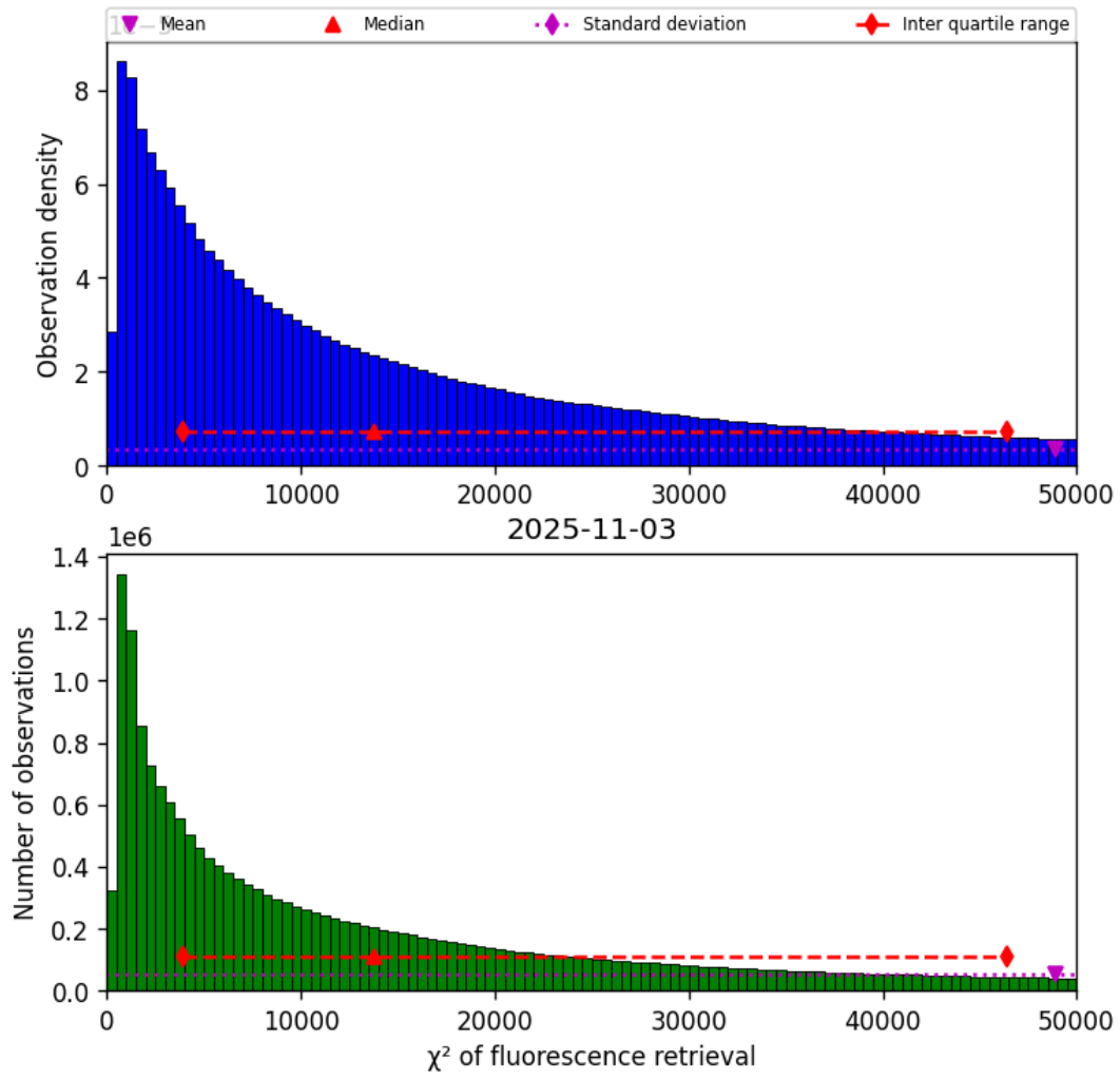
Figure 42: Histogram of “ \chi^2 of fluorescence retrieval” for 2025-11-02 to 2025-11-04
