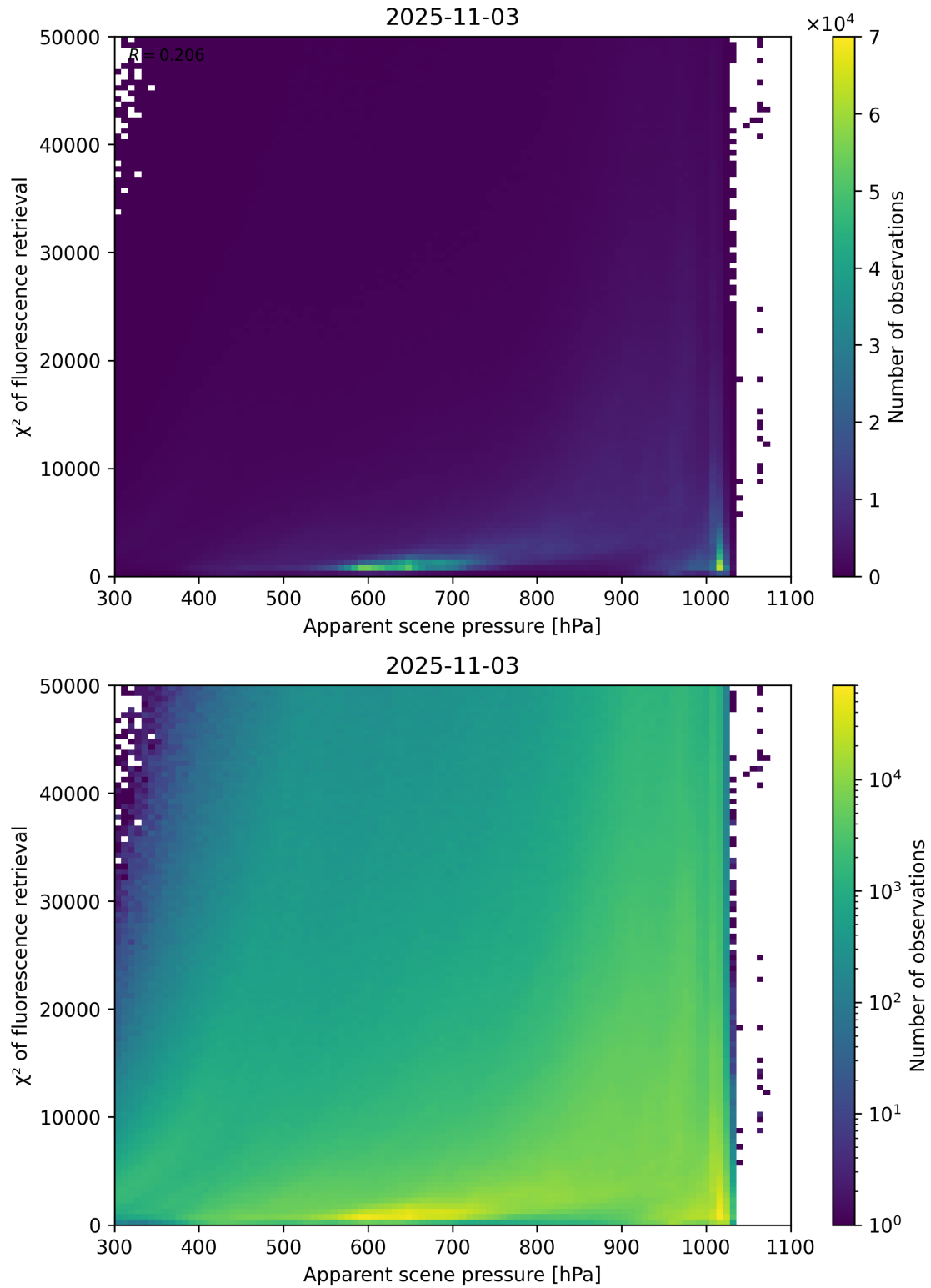
Figure 63: Scatter density plot of “Apparent scene pressure” against “ \chi^2 of fluorescence retrieval” for 2025-11-02 to 2025-11-04.
