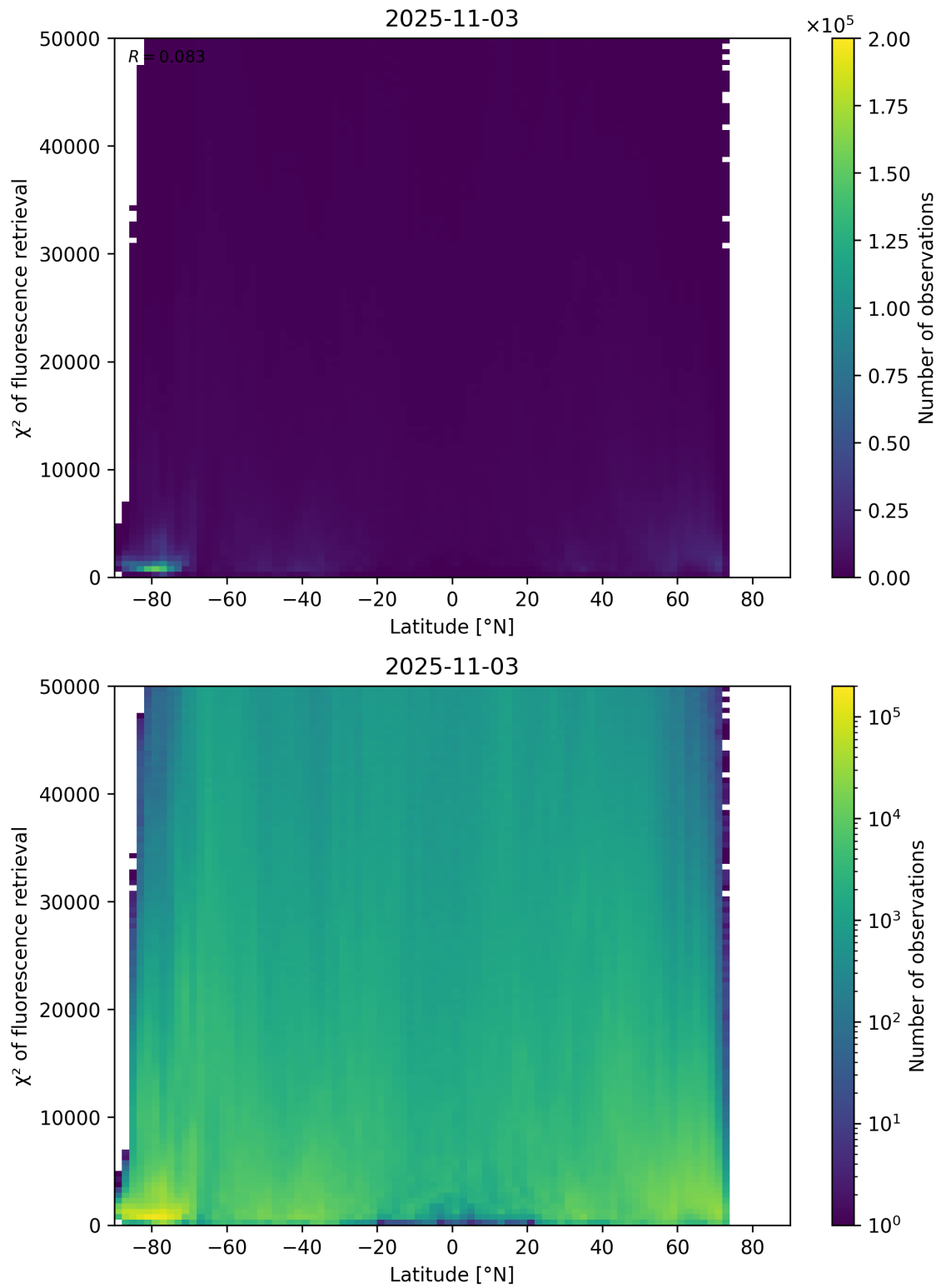
Figure 89: Scatter density plot of “Latitude” against “ \chi^2 of fluorescence retrieval” for 2025-11-02 to 2025-11-04.
