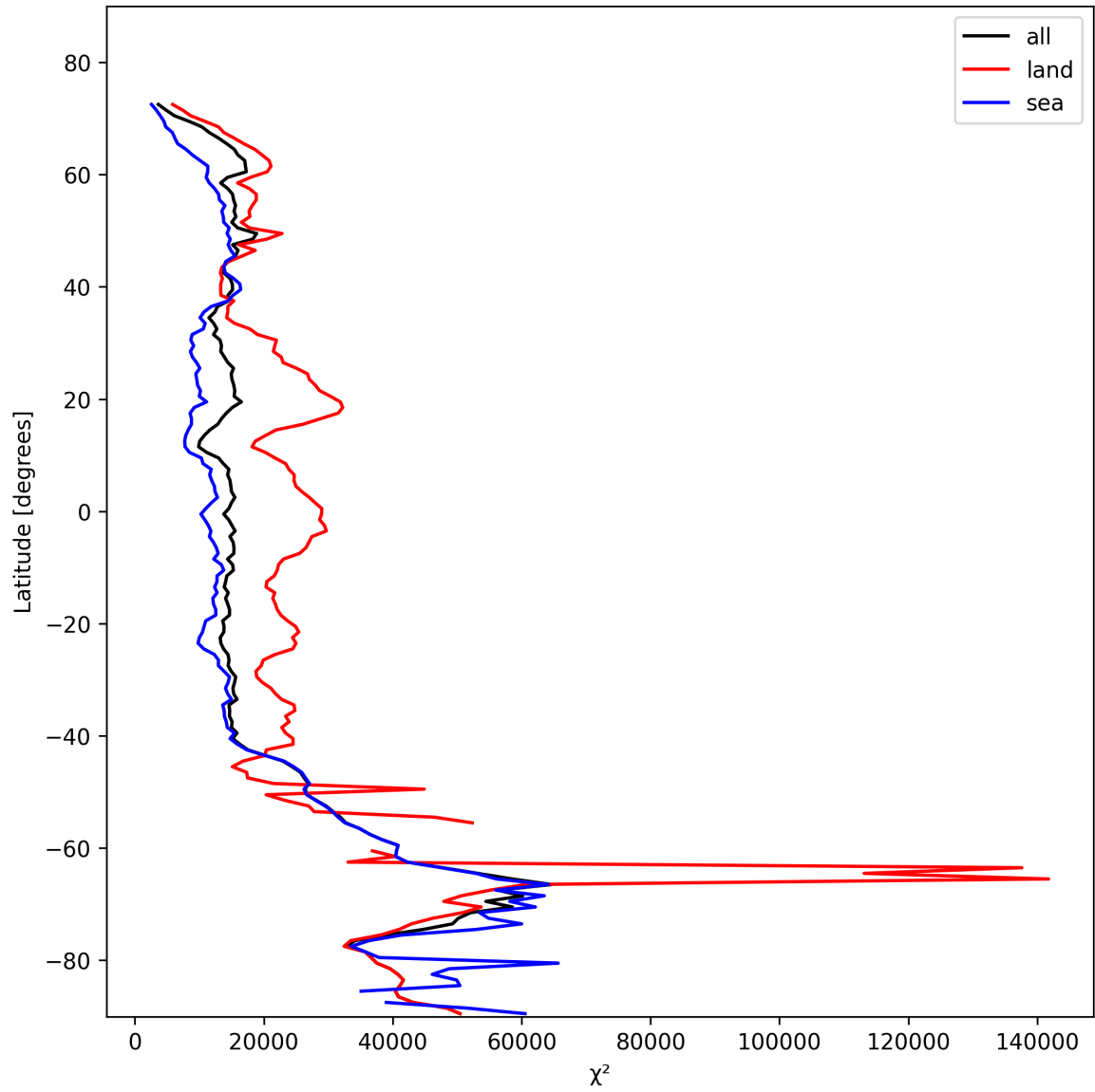
Figure 21: Zonal average of “ \chi^2 ” for 2025-11-02 to 2025-11-04.
