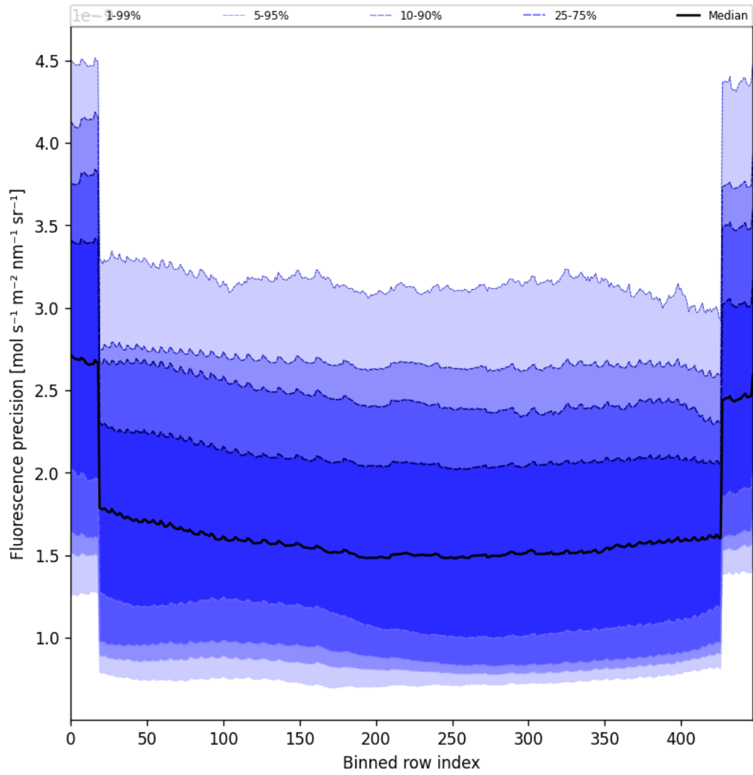
Figure 58: Along track statistics of “Fluorescence precision” for 2025-11-02 to 2025-11-04
