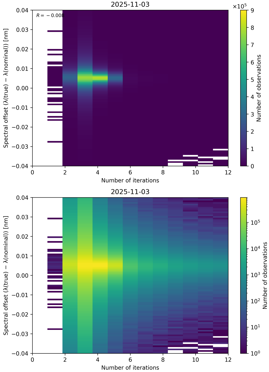
Figure 100: Scatter density plot of “Number of iterations” against “Spectral offset ( \lambda_{\text{true}} - \lambda_{\text{nominal}} )” for 2025-11-02 to 2025-11-04.
