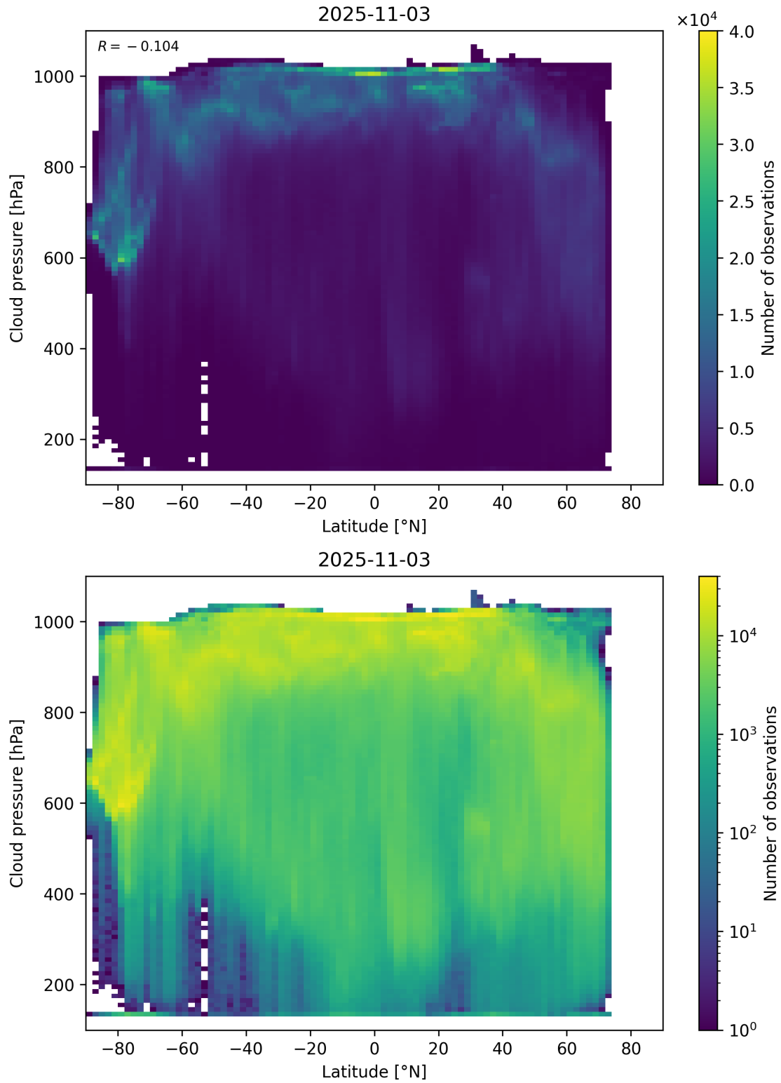
Figure 91: Scatter density plot of “Latitude” against “Cloud pressure” for 2025-11-02 to 2025-11-04.
