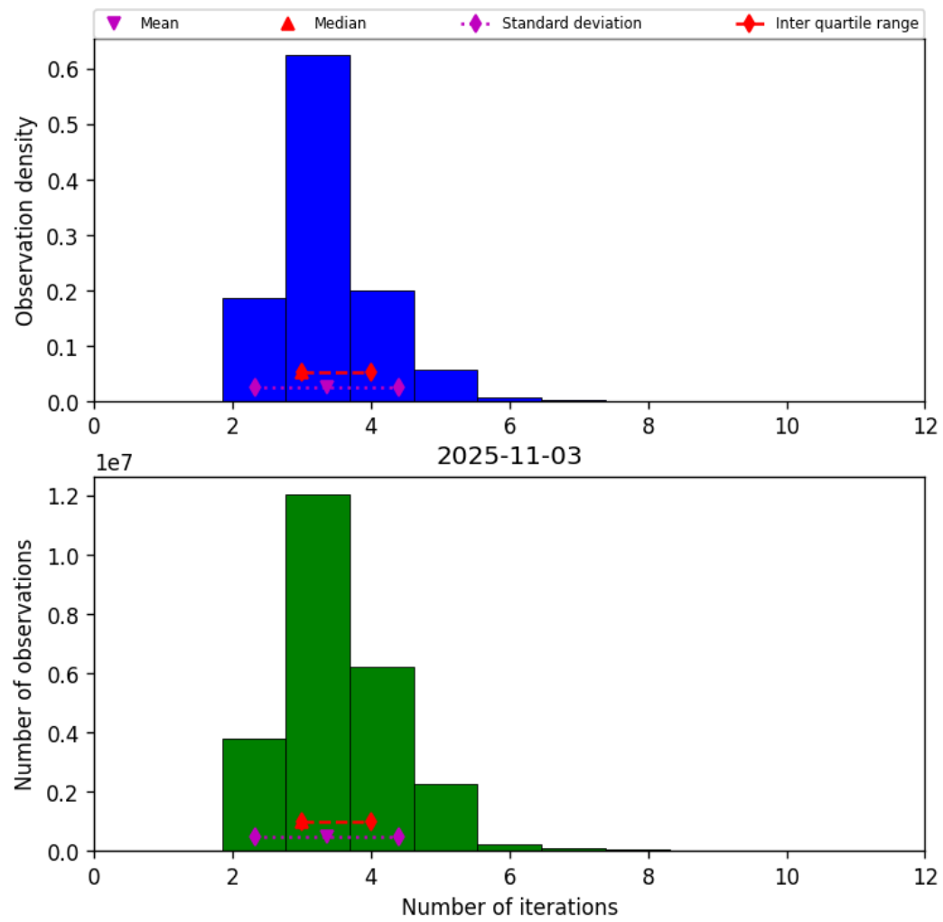
Figure 39: Histogram of “Number of iterations” for 2025-11-02 to 2025-11-04
