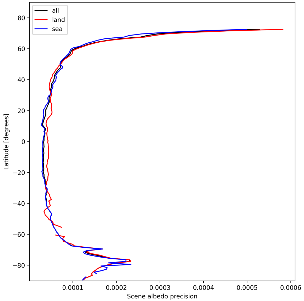
Figure 18: Zonal average of “Scene albedo precision” for 2025-11-02 to 2025-11-04.
