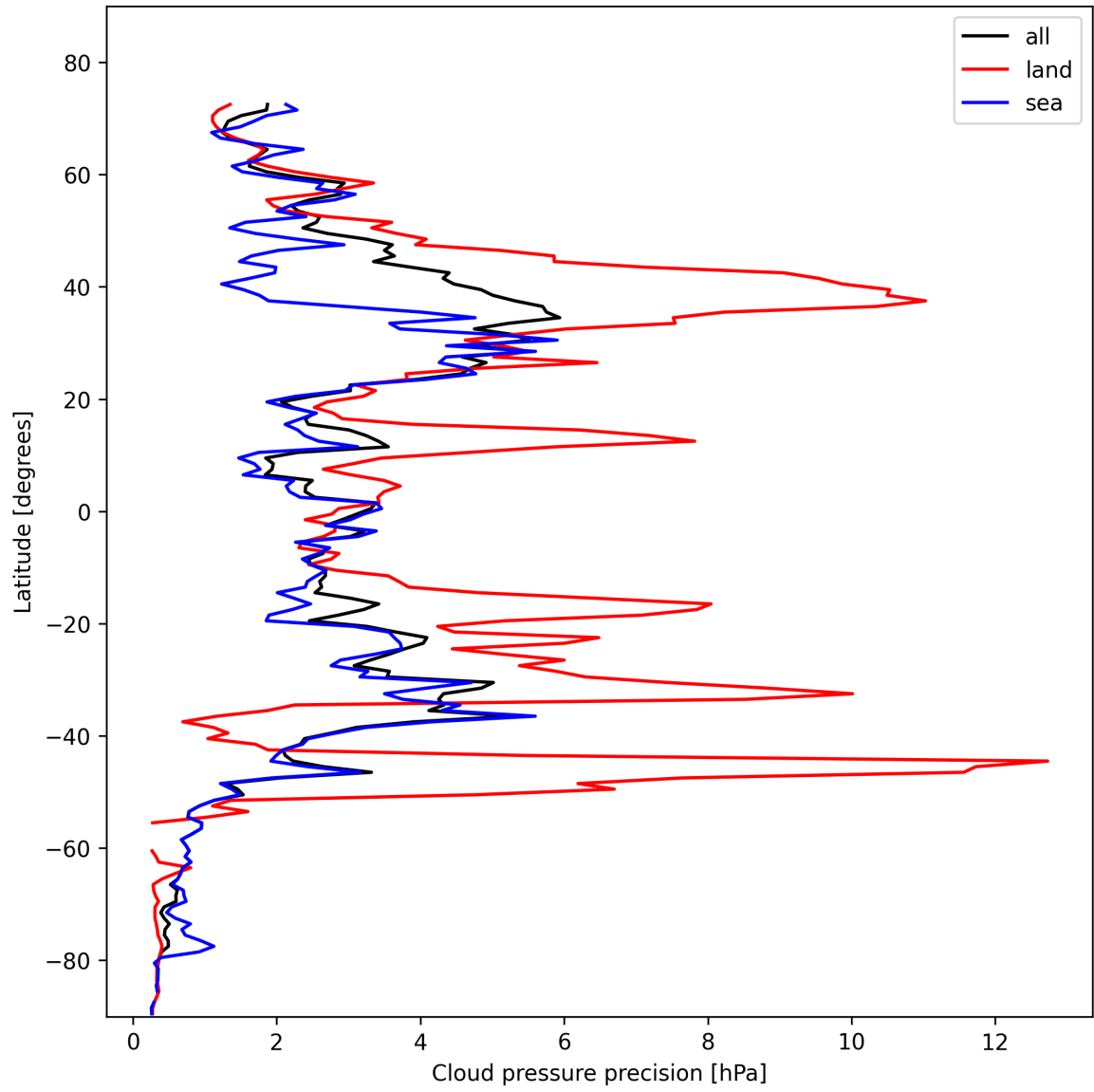
Figure 14: Zonal average of “Cloud pressure precision” for 2025-11-02 to 2025-11-04.
