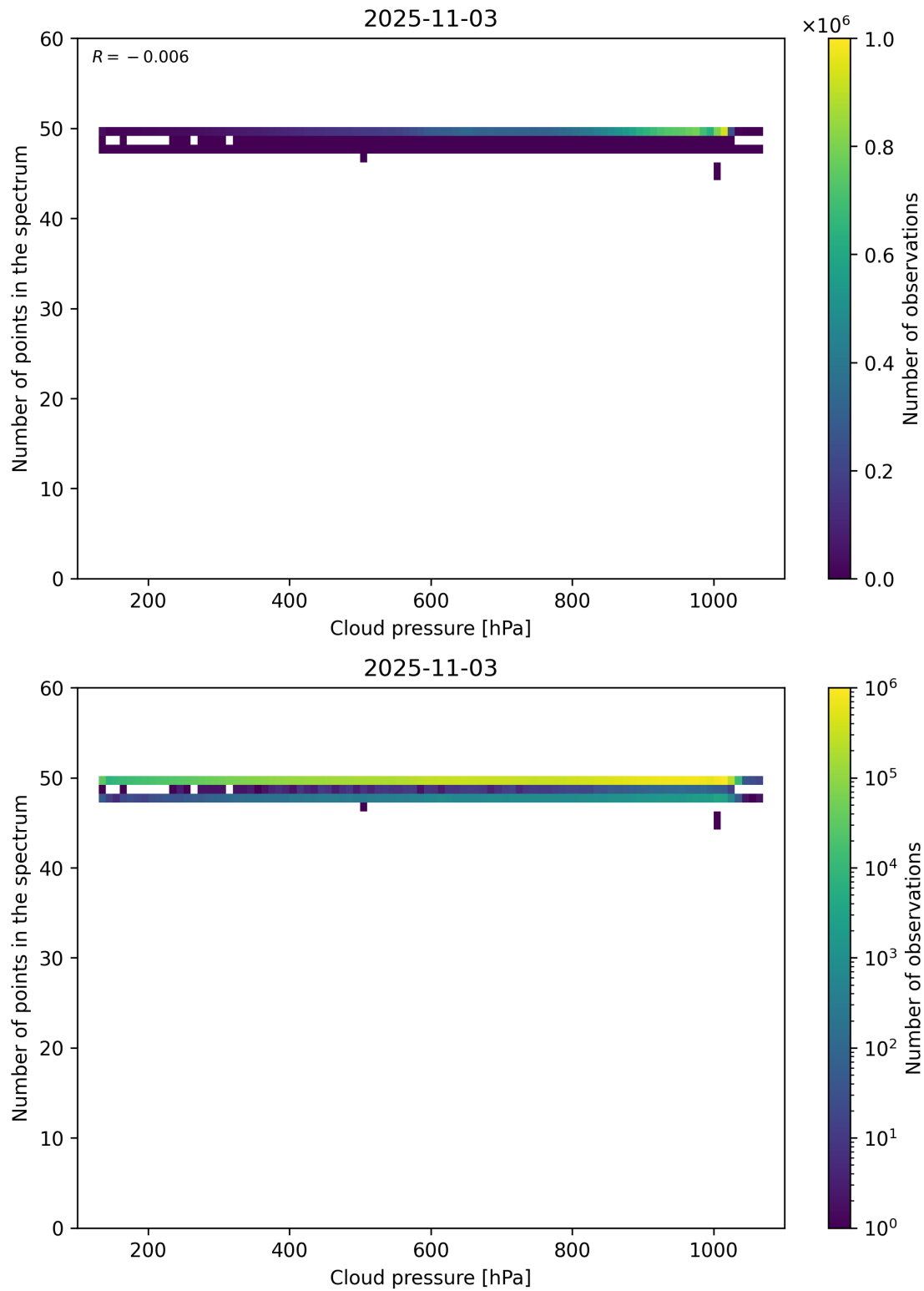
Figure 82: Scatter density plot of “Cloud pressure” against “Number of points in the spectrum” for 2025-11-02 to 2025-11-04.
