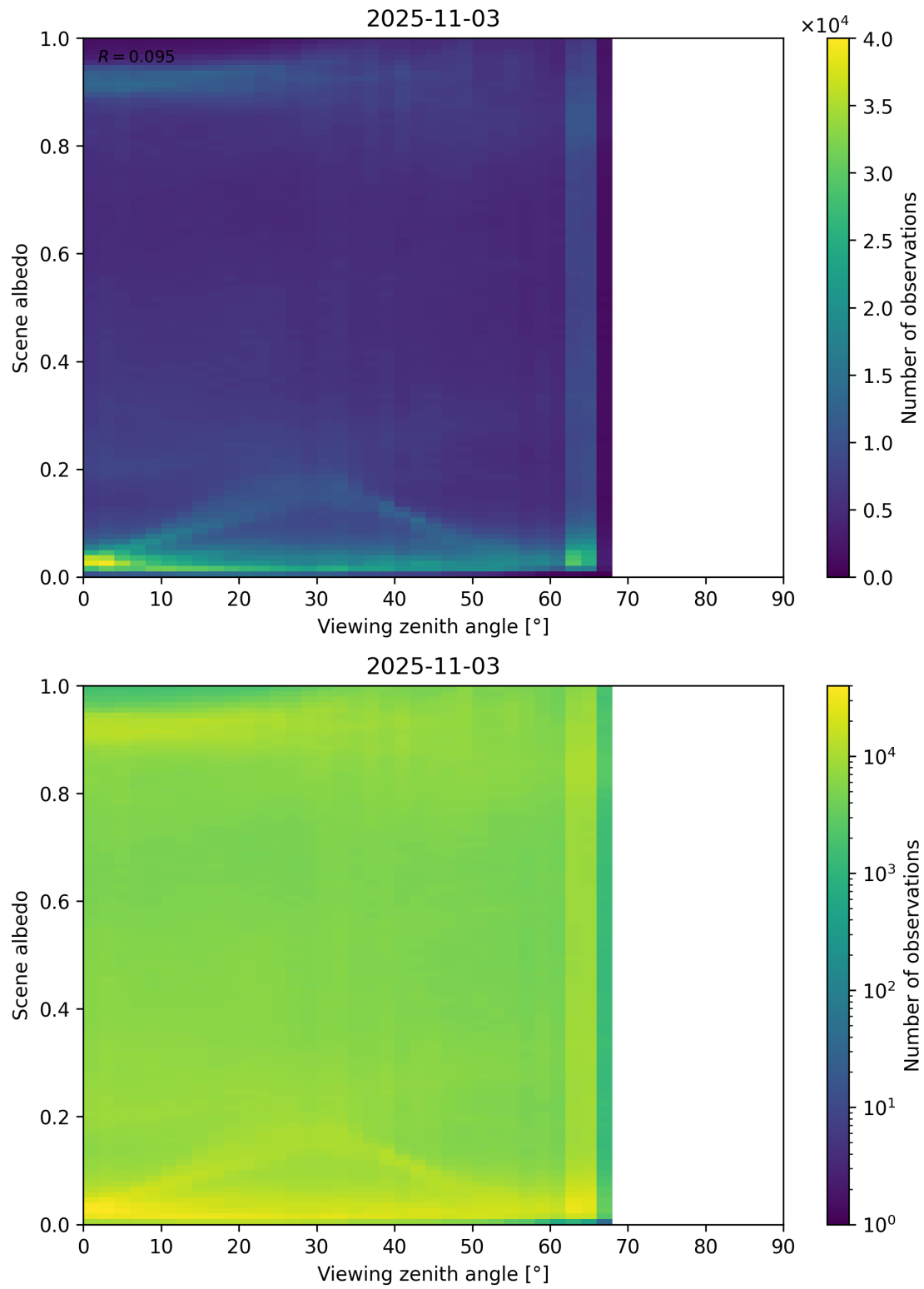
Figure 126: Scatter density plot of “Viewing zenith angle” against “Scene albedo” for 2025-11-02 to 2025-11-04.
