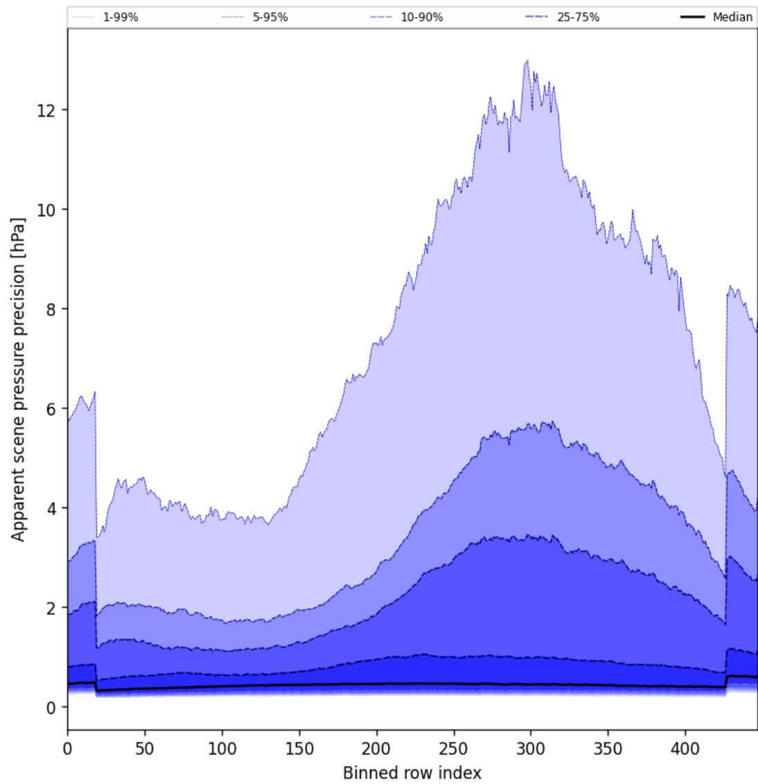
Figure 54: Along track statistics of “Apparent scene pressure precision” for 2025-11-02 to 2025-11-04
