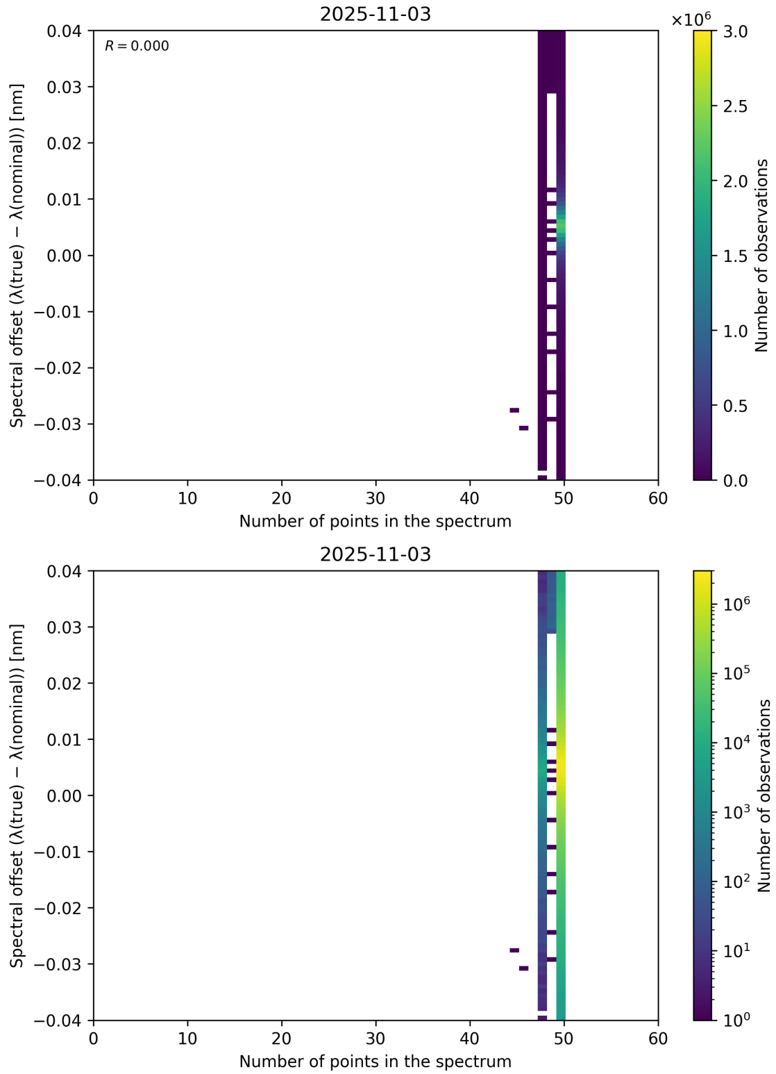
Figure 101: Scatter density plot of “Number of points in the spectrum” against “Spectral offset ( \lambda_{\text{true}} - \lambda_{\text{nominal}} )” for 2025-11-02 to 2025-11-04.
