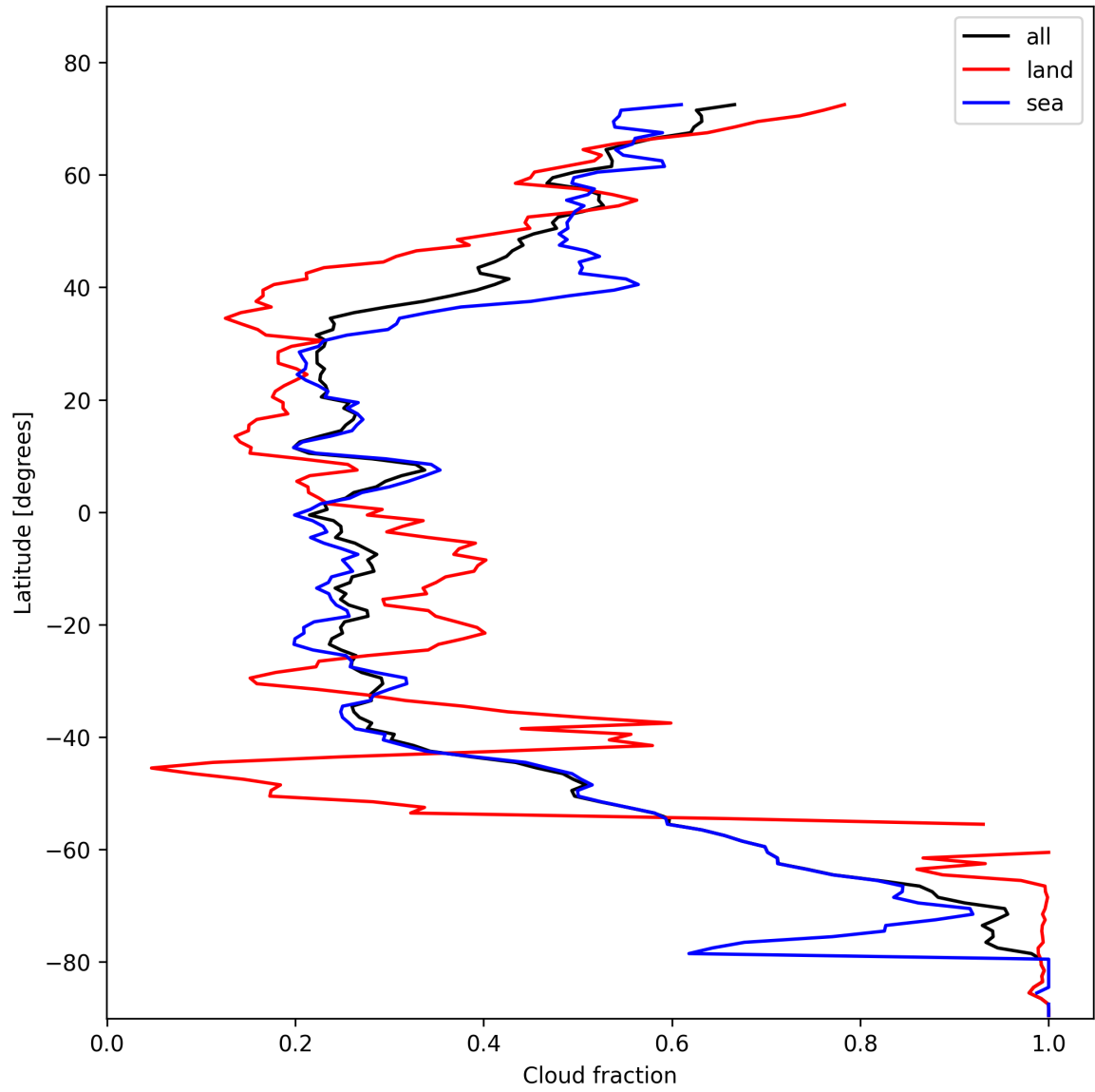
Figure 15: Zonal average of “Cloud fraction” for 2025-11-02 to 2025-11-04.
