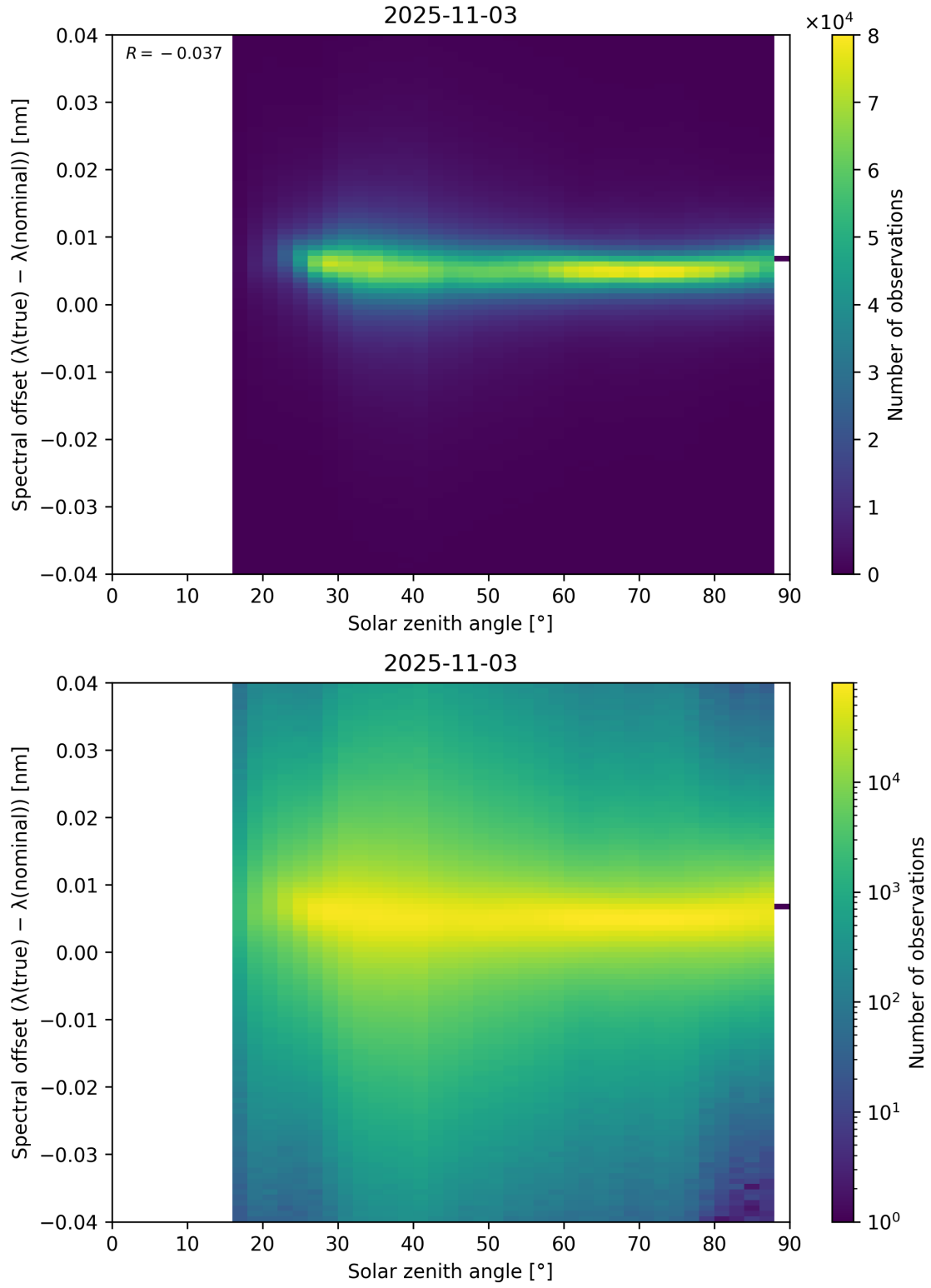
Figure 117: Scatter density plot of “Solar zenith angle” against “Spectral offset ( \lambda_{\text{true}} - \lambda_{\text{nominal}} )” for 2025-11-02 to 2025-11-04.
