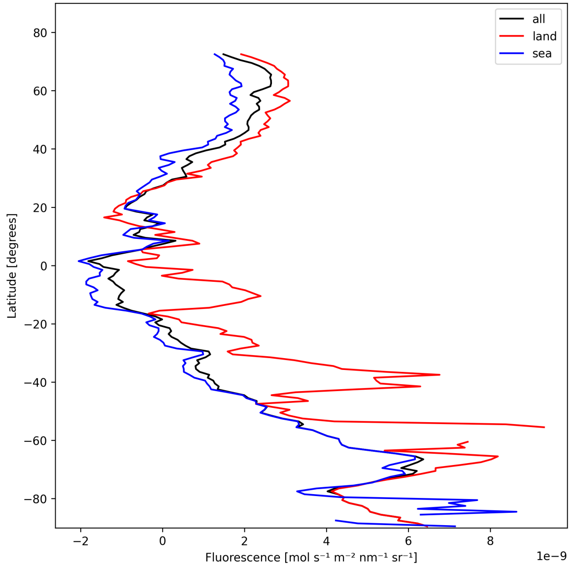
Figure 23: Zonal average of “Fluorescence” for 2025-11-02 to 2025-11-04.
