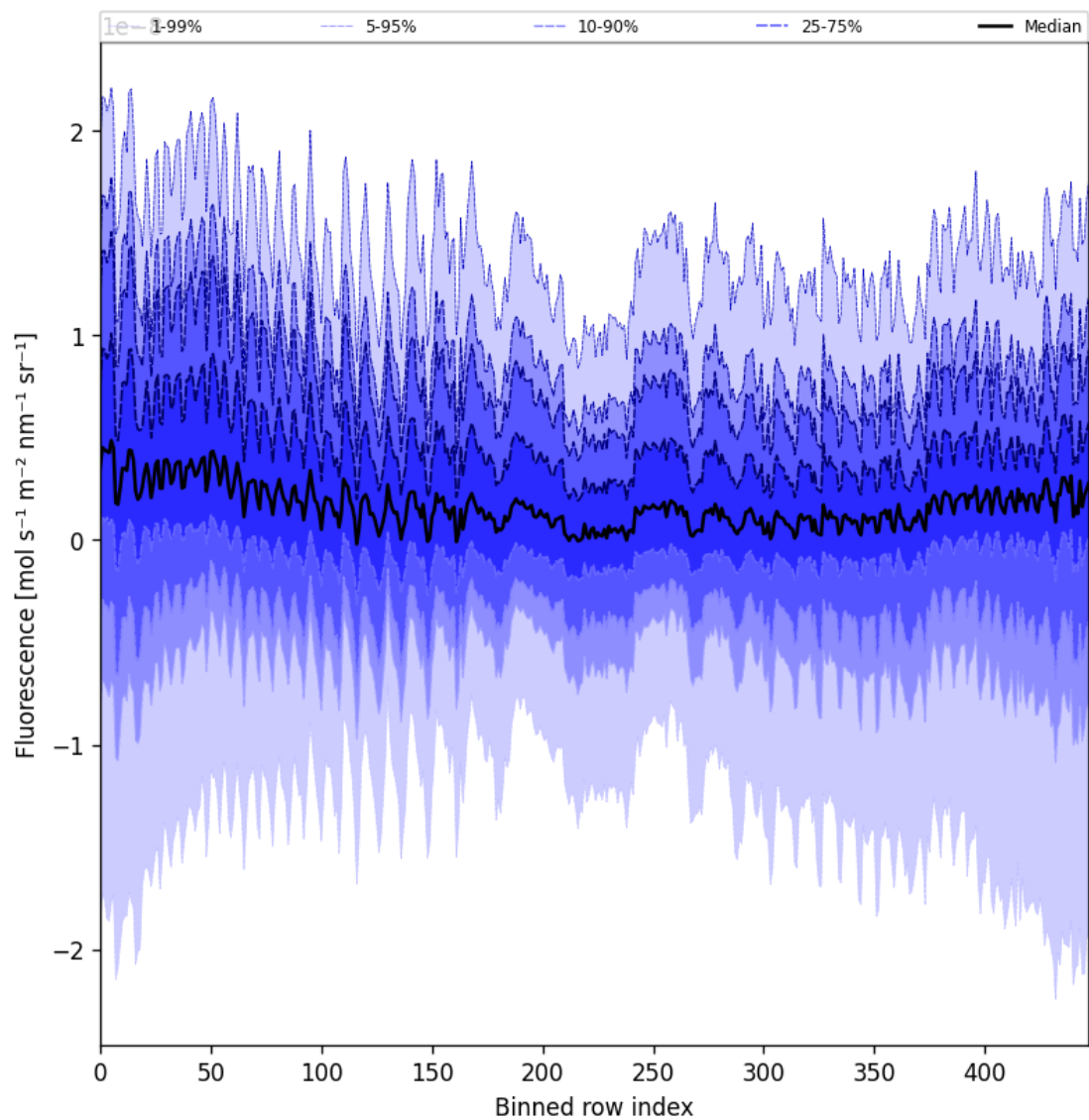
Figure 57: Along track statistics of “Fluorescence” for 2025-11-02 to 2025-11-04
