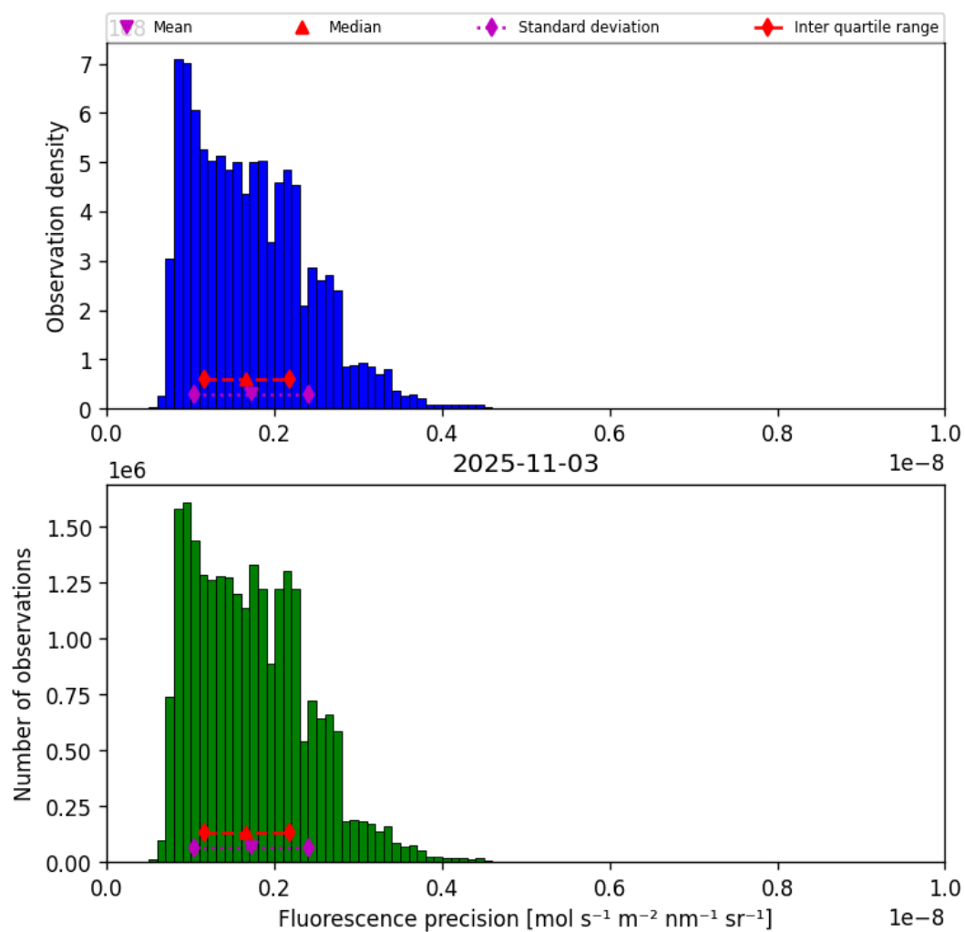
Figure 41: Histogram of “Fluorescence precision” for 2025-11-02 to 2025-11-04
