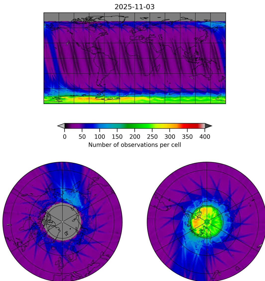
Figure 11: Map of the number of observations for 2025-11-02 to 2025-11-04
