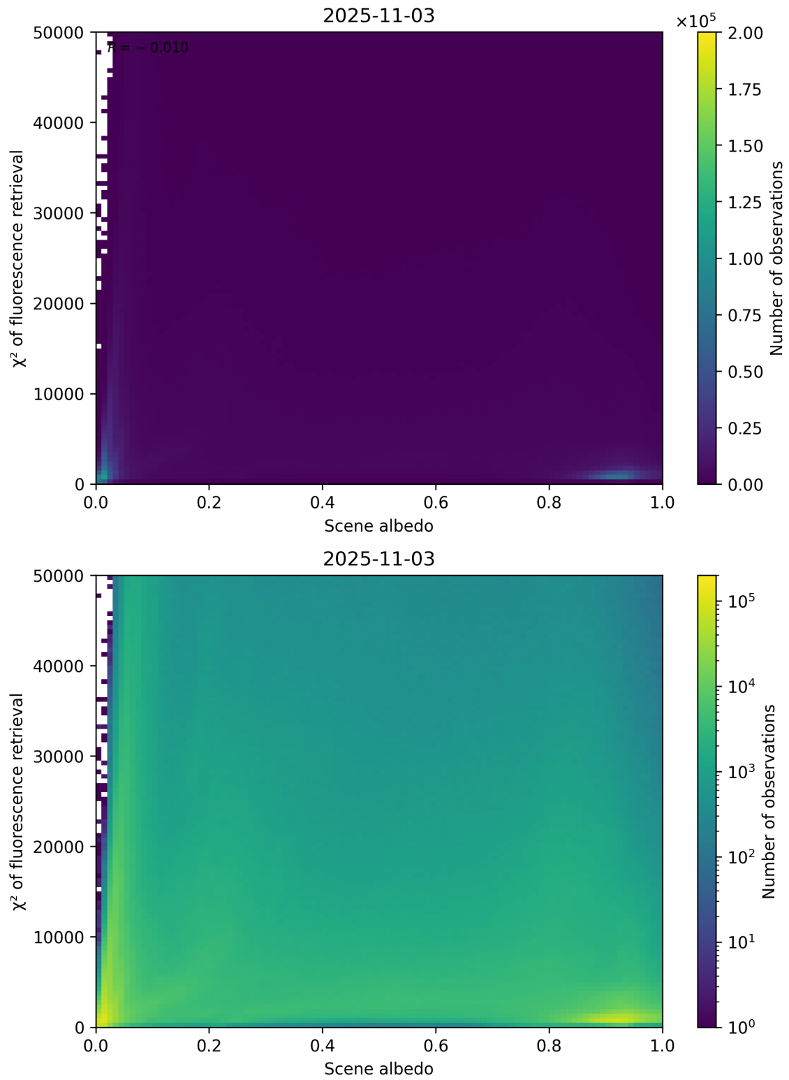
Figure 103: Scatter density plot of “Scene albedo” against “ \chi^2 of fluorescence retrieval” for 2025-11-02 to 2025-11-04.
