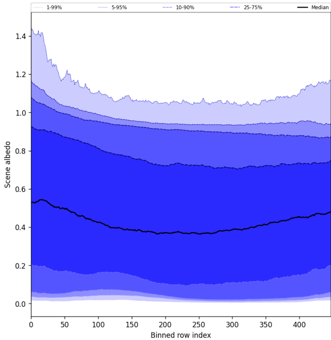
Figure 51: Along track statistics of “Scene albedo” for 2025-11-02 to 2025-11-04
