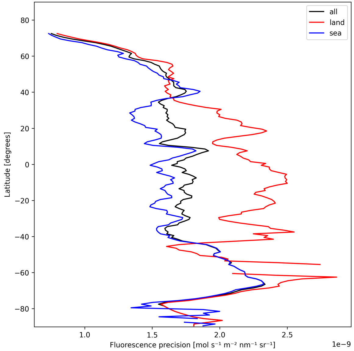
Figure 24: Zonal average of “Fluorescence precision” for 2025-11-02 to 2025-11-04.
