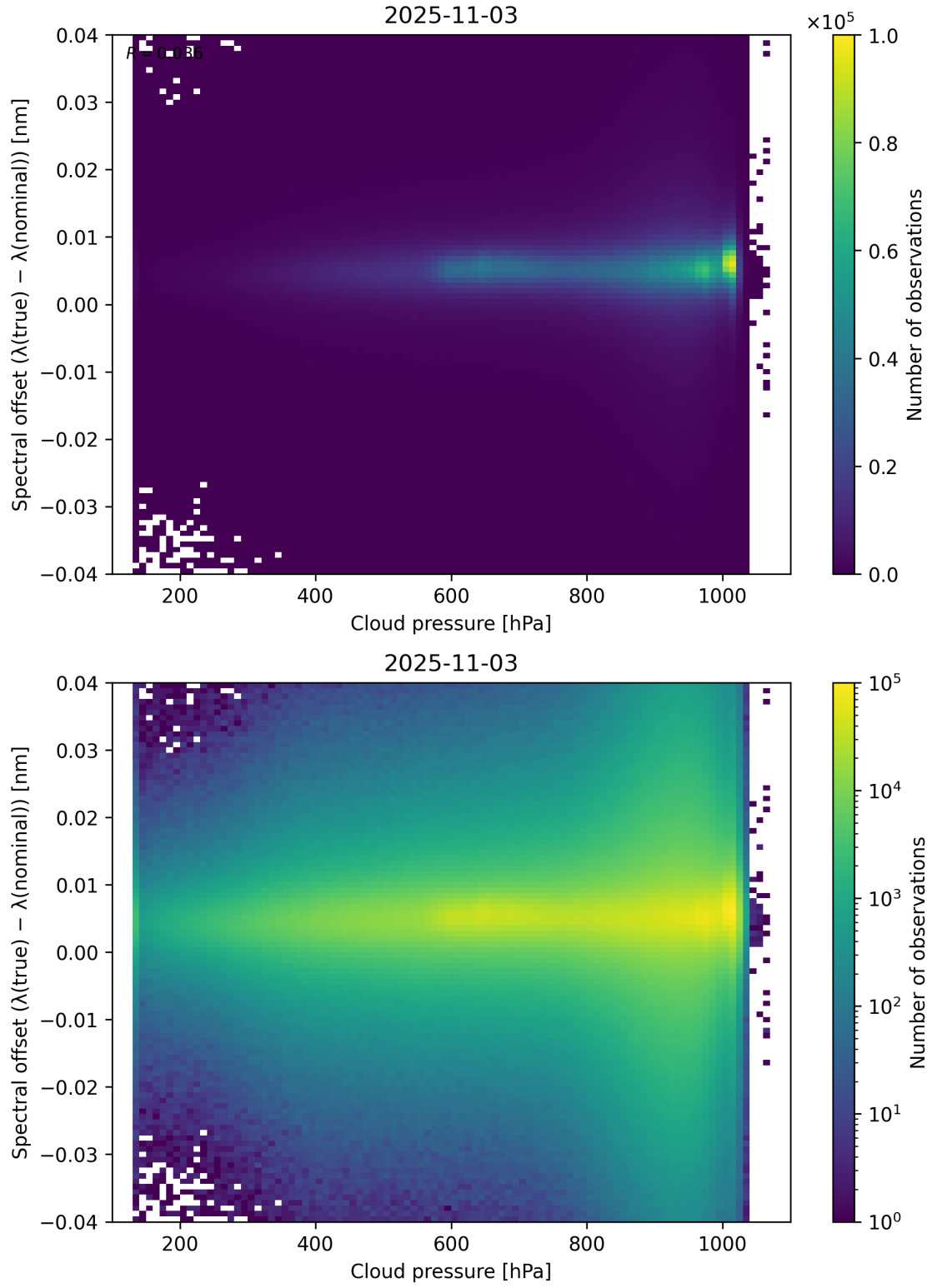
Figure 84: Scatter density plot of “Cloud pressure” against “Spectral offset ( \lambda_{\text{true}} - \lambda_{\text{nominal}} )” for 2025-11-02 to 2025-11-04.
