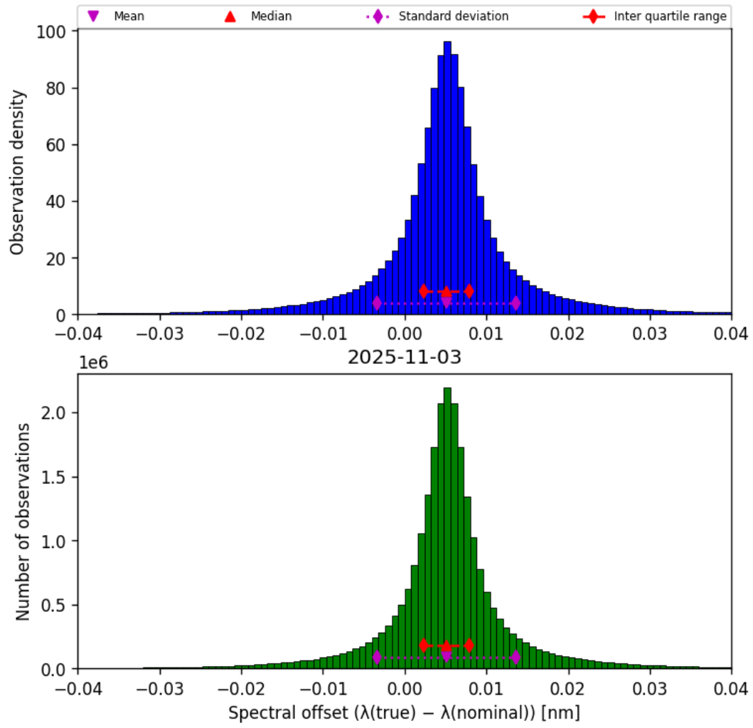
Figure 45: Histogram of “Spectral offset ( \lambda_{\text{true}} - \lambda_{\text{nominal}} )” for 2025-11-02 to 2025-11-04
