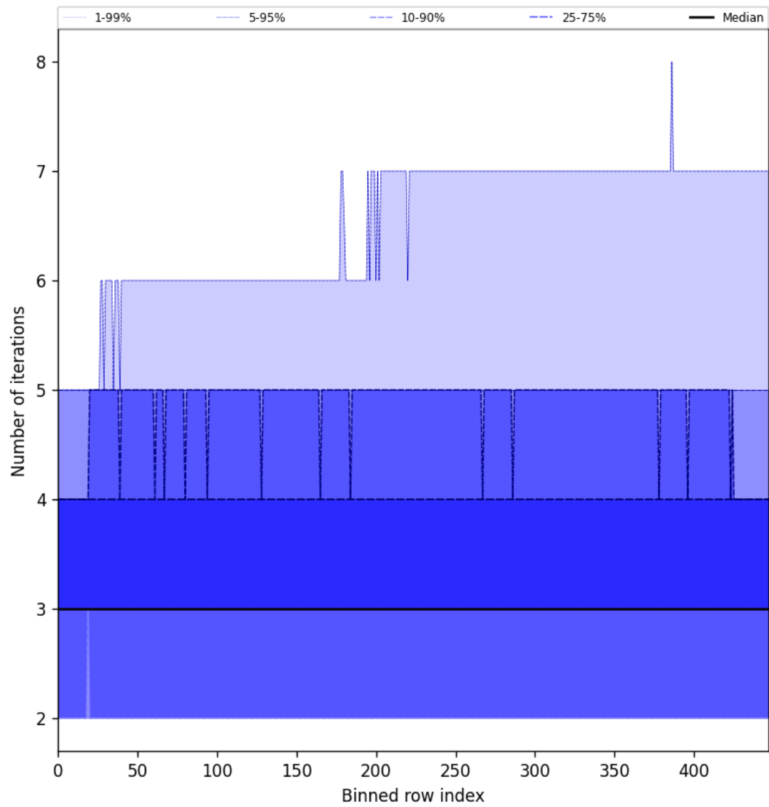
Figure 56: Along track statistics of “Number of iterations” for 2025-11-02 to 2025-11-04
