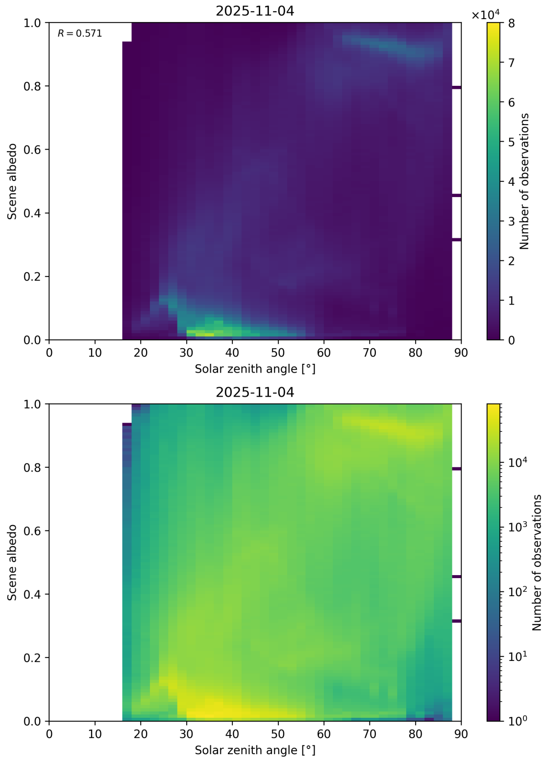
Figure 116: Scatter density plot of “Solar zenith angle” against “Scene albedo” for 2025-11-03 to 2025-11-05.
