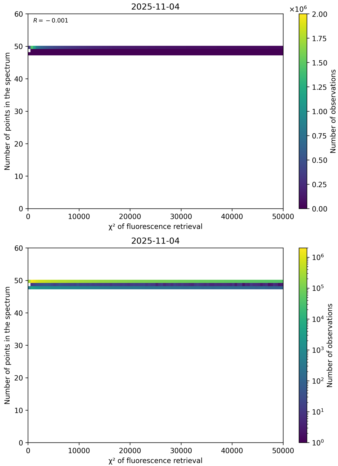
Figure 68: Scatter density plot of " \chi^2 of fluorescence retrieval" against "Number of points in the spectrum" for 2025-11-03 to 2025-11-05.
