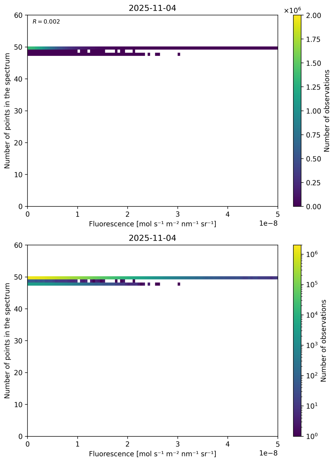
Figure 86: Scatter density plot of “Fluorescence” against “Number of points in the spectrum” for 2025-11-03 to 2025-11-05.
