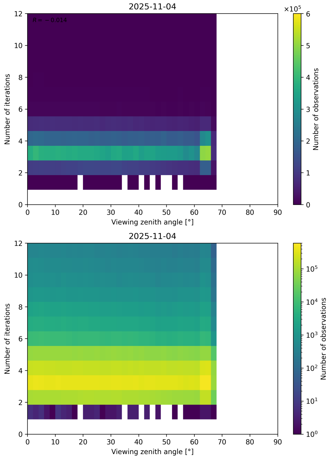
Figure 124: Scatter density plot of “Viewing zenith angle” against “Number of iterations” for 2025-11-03 to 2025-11-05.
