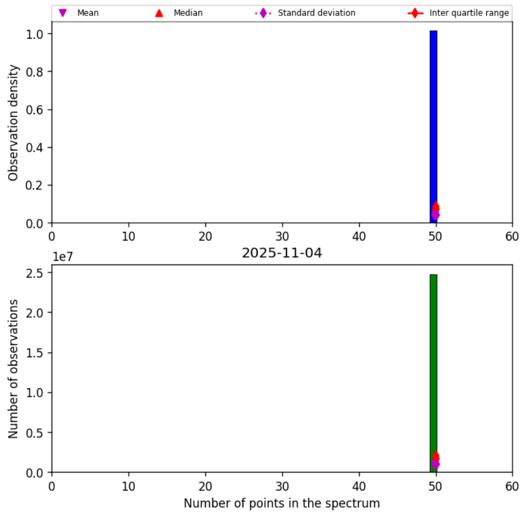
Figure 44: Histogram of “Number of points in the spectrum” for 2025-11-03 to 2025-11-05
