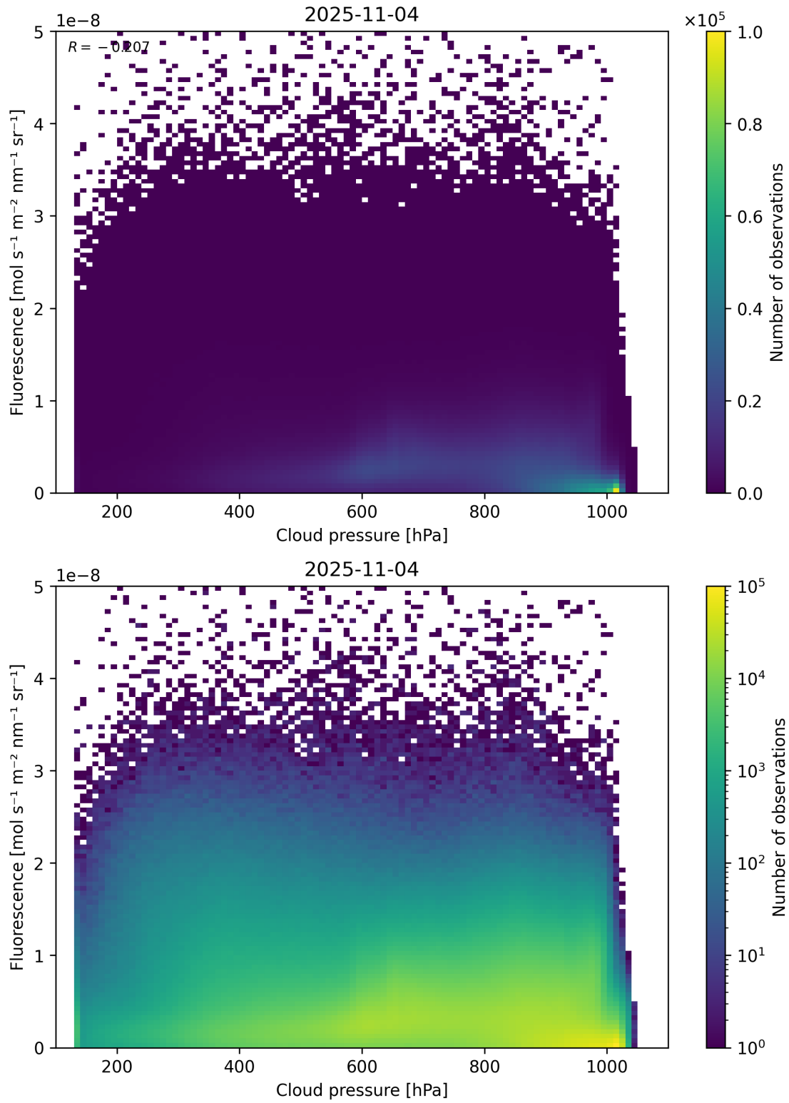
Figure 80: Scatter density plot of “Cloud pressure” against “Fluorescence” for 2025-11-03 to 2025-11-05.
