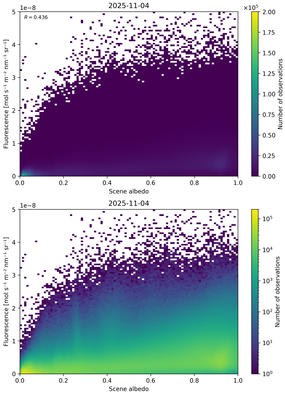
Figure 104: Scatter density plot of “Scene albedo” against “Fluorescence” for 2025-11-03 to 2025-11-05.
