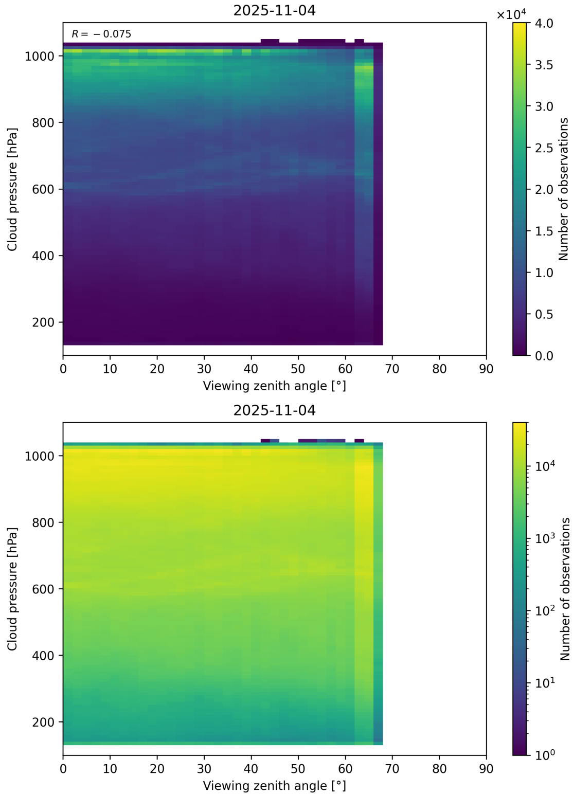
Figure 121: Scatter density plot of “Viewing zenith angle” against “Cloud pressure” for 2025-11-03 to 2025-11-05.
