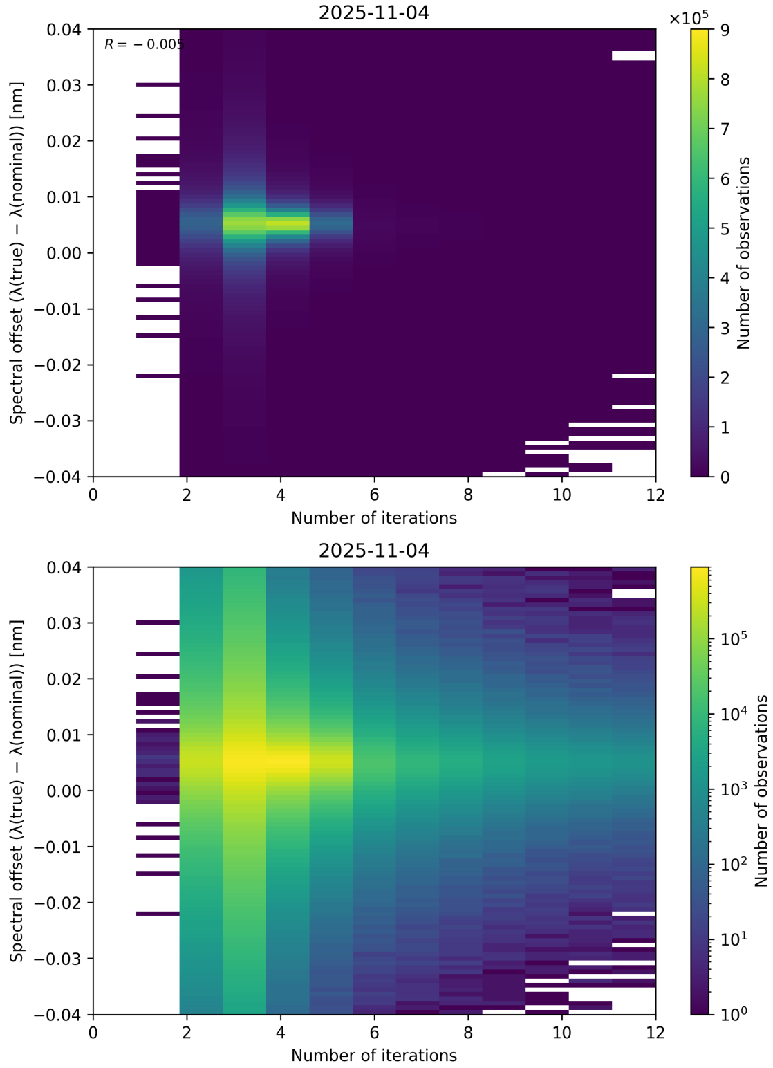
Figure 100: Scatter density plot of “Number of iterations” against “Spectral offset ( \lambda_{\text{true}} - \lambda_{\text{nominal}} )” for 2025-11-03 to 2025-11-05.
