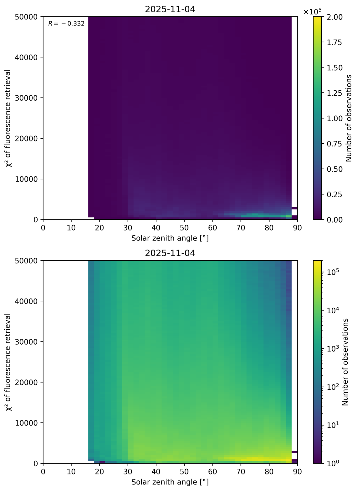
Figure 109: Scatter density plot of “Solar zenith angle” against “ \chi^2 of fluorescence retrieval” for 2025-11-03 to 2025-11-05.
