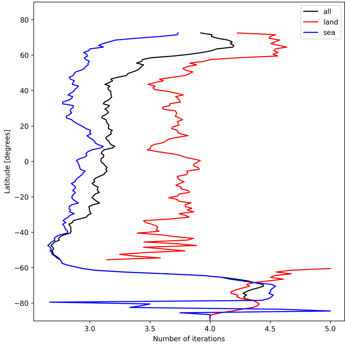
Figure 22: Zonal average of “Number of iterations” for 2025-11-03 to 2025-11-05.
