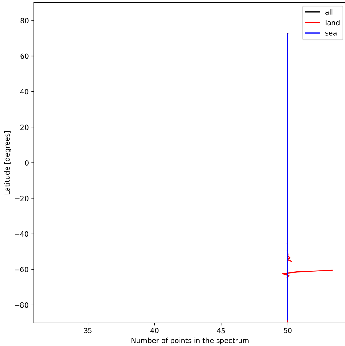
Figure 27: Zonal average of “Number of points in the spectrum” for 2025-11-03 to 2025-11-05.
