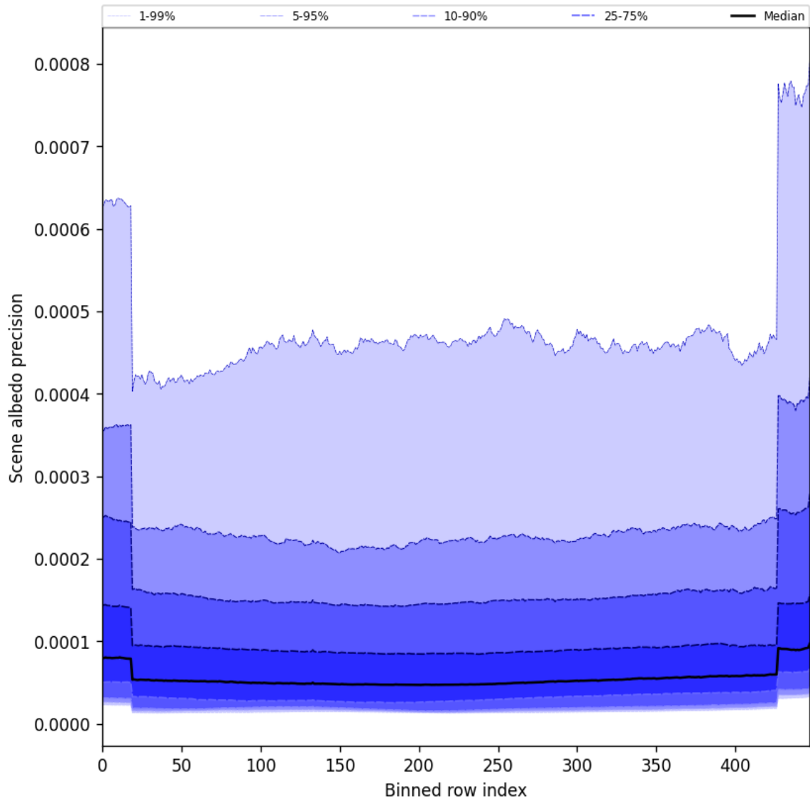
Figure 52: Along track statistics of “Scene albedo precision” for 2025-11-03 to 2025-11-05
