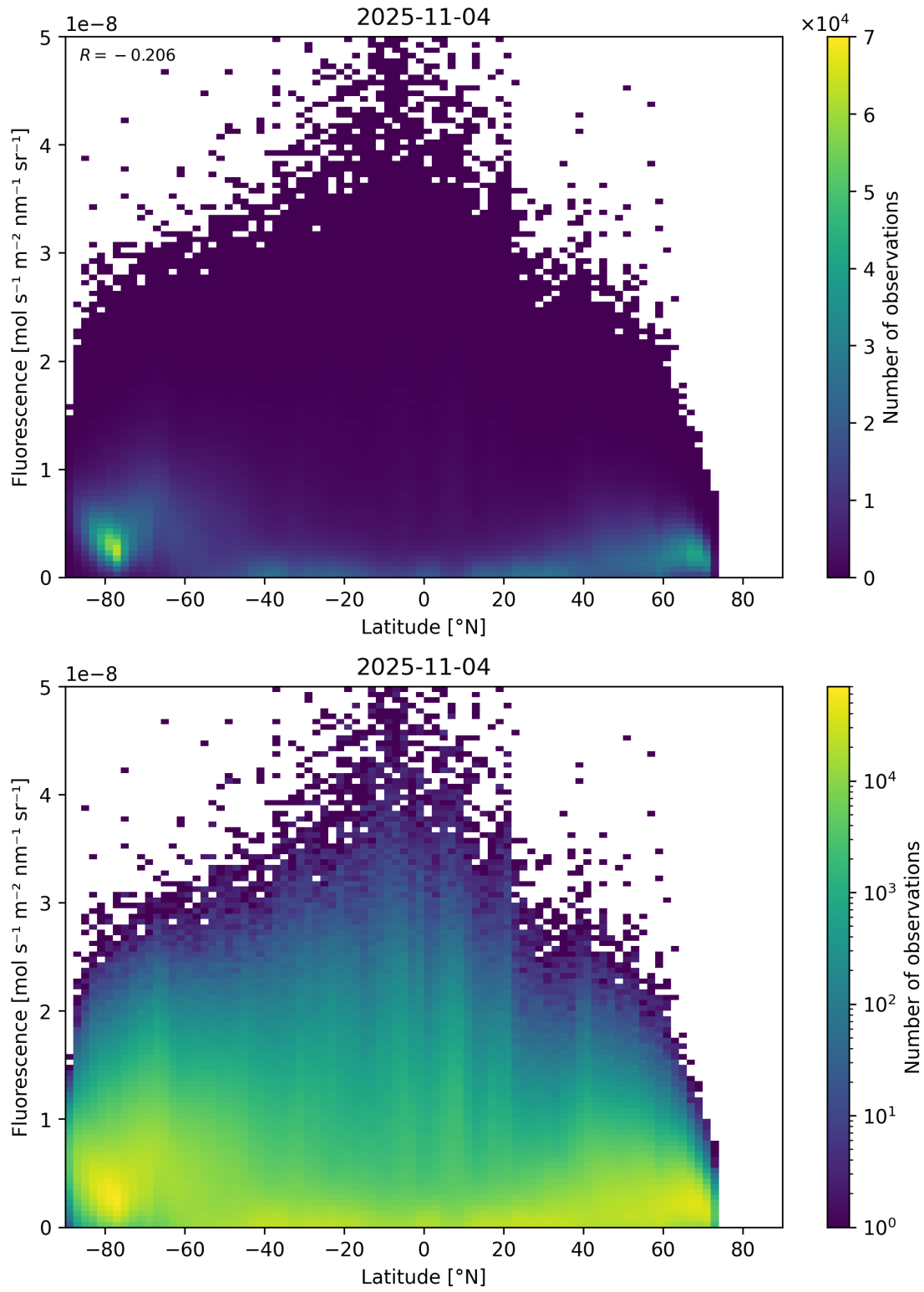
Figure 92: Scatter density plot of “Latitude” against “Fluorescence” for 2025-11-03 to 2025-11-05.
