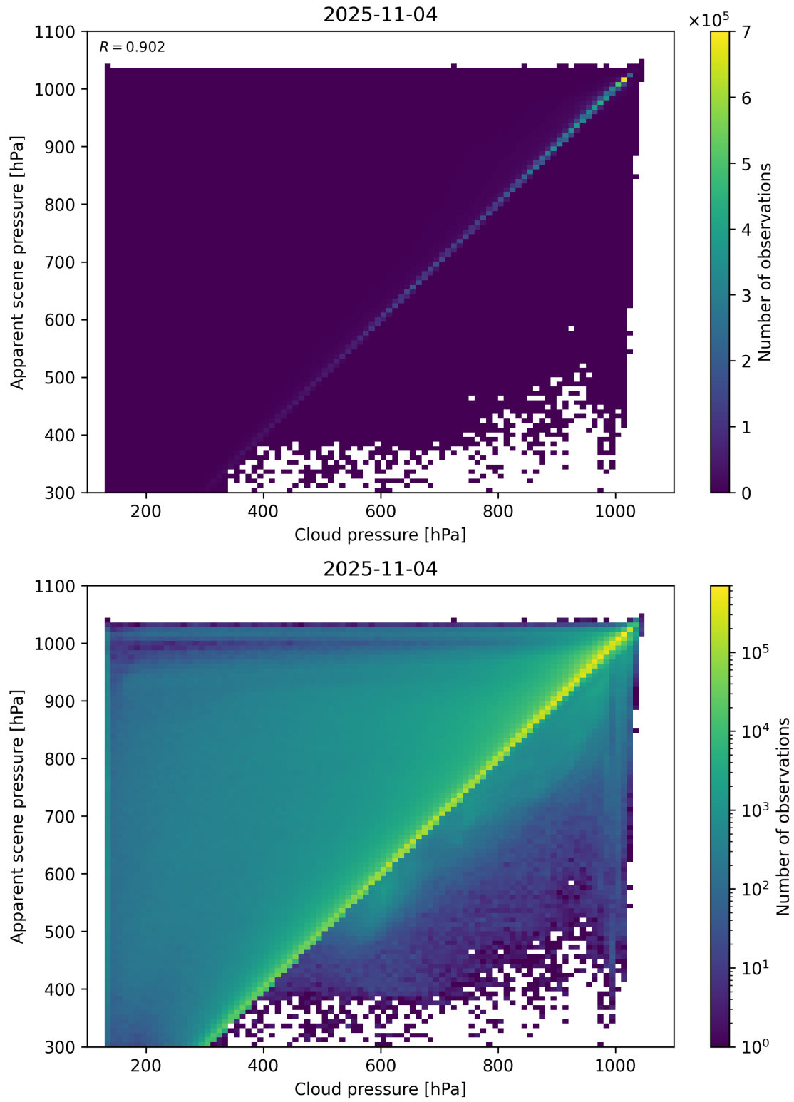
Figure 77: Scatter density plot of “Cloud pressure” against “Apparent scene pressure” for 2025-11-03 to 2025-11-05.
