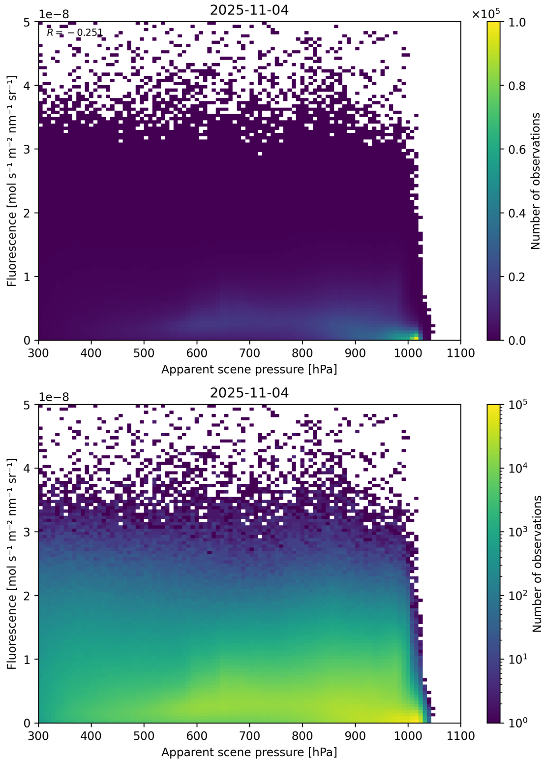
Figure 64: Scatter density plot of “Apparent scene pressure” against “Fluorescence” for 2025-11-03 to 2025-11-05.
