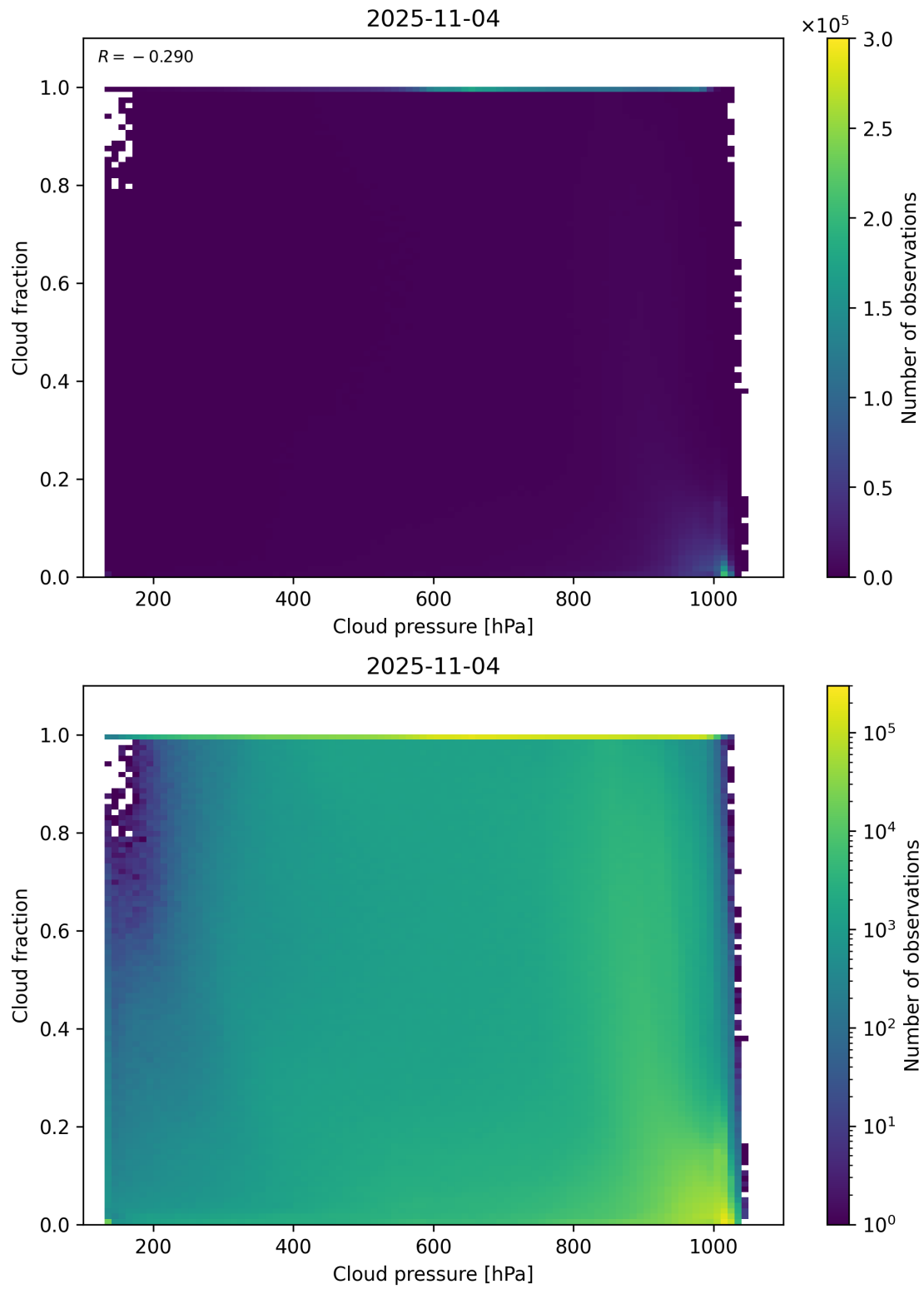
Figure 79: Scatter density plot of “Cloud pressure” against “Cloud fraction” for 2025-11-03 to 2025-11-05.
