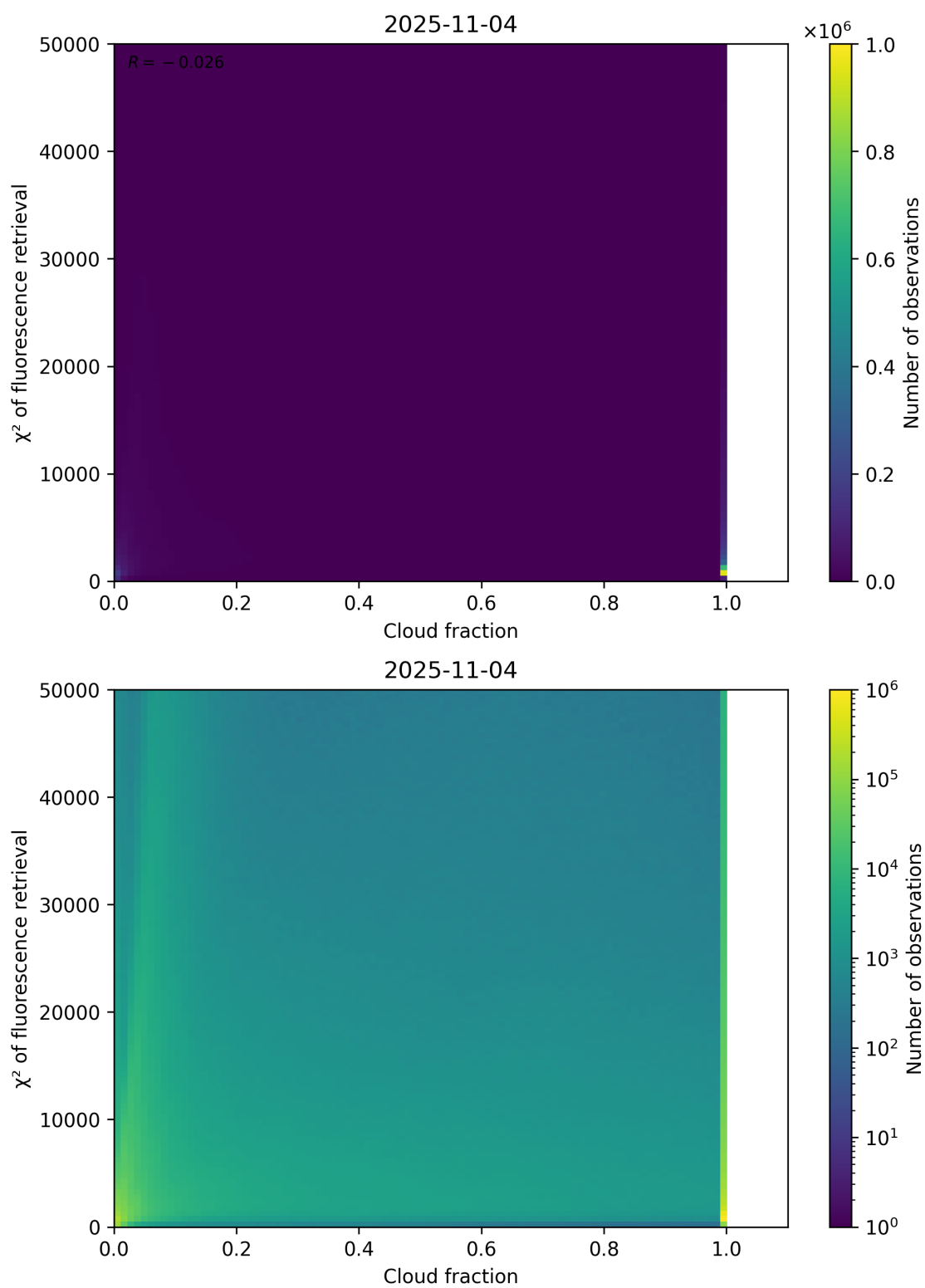
Figure 71: Scatter density plot of “Cloud fraction” against “ \chi^2 of fluorescence retrieval” for 2025-11-03 to 2025-11-05.
