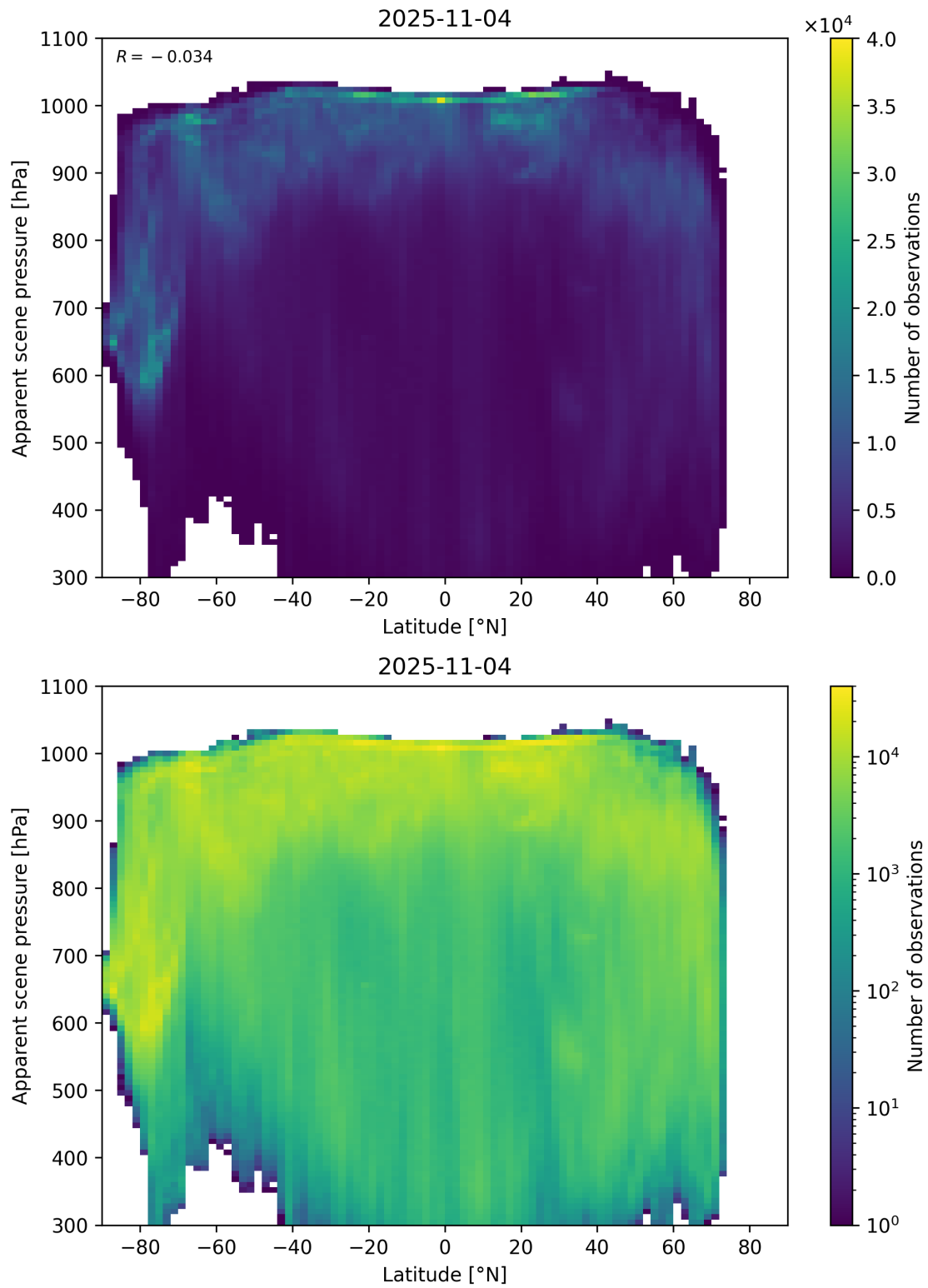
Figure 88: Scatter density plot of “Latitude” against “Apparent scene pressure” for 2025-11-03 to 2025-11-05.
