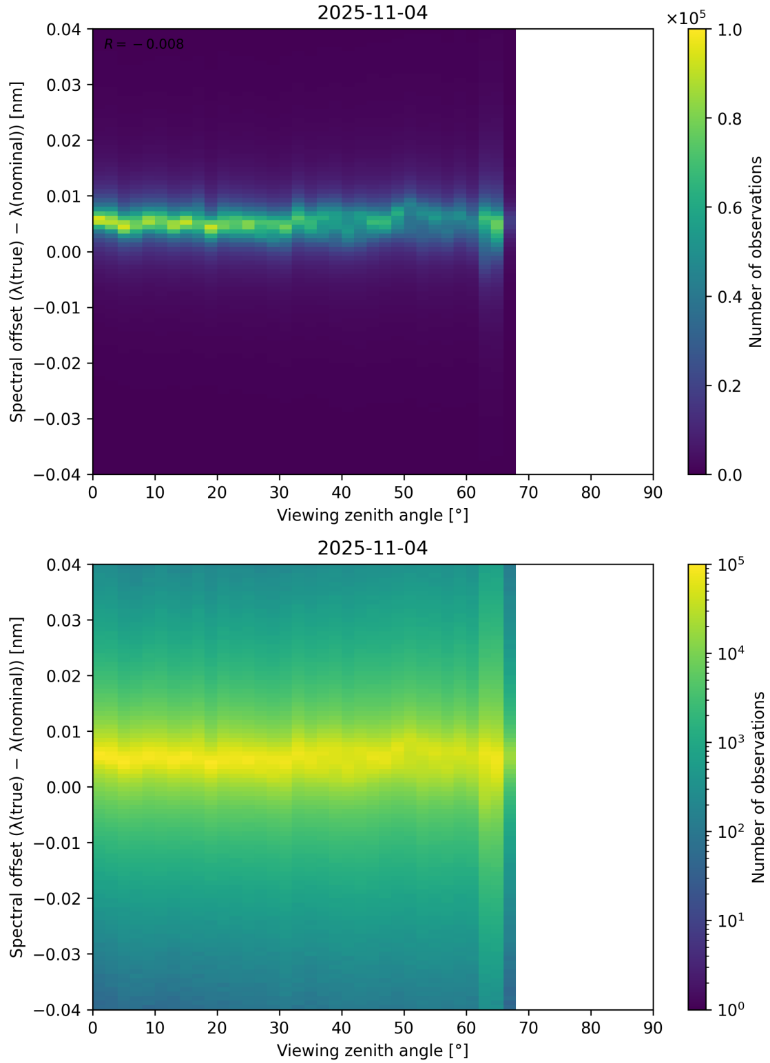
Figure 128: Scatter density plot of “Viewing zenith angle” against “Spectral offset ( \lambda_{\text{true}} - \lambda_{\text{nominal}} )” for 2025-11-03 to 2025-11-05.
