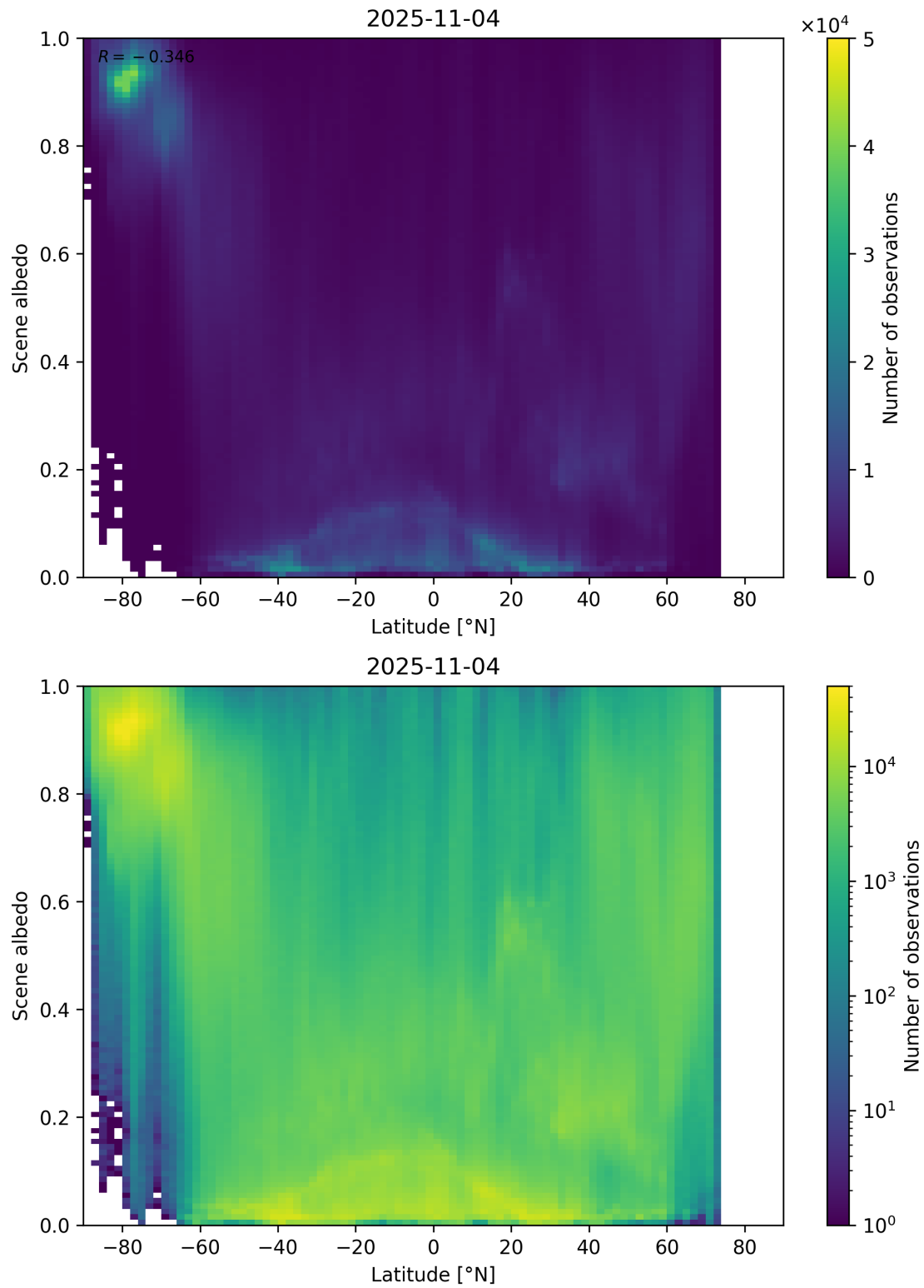
Figure 95: Scatter density plot of “Latitude” against “Scene albedo” for 2025-11-03 to 2025-11-05.
