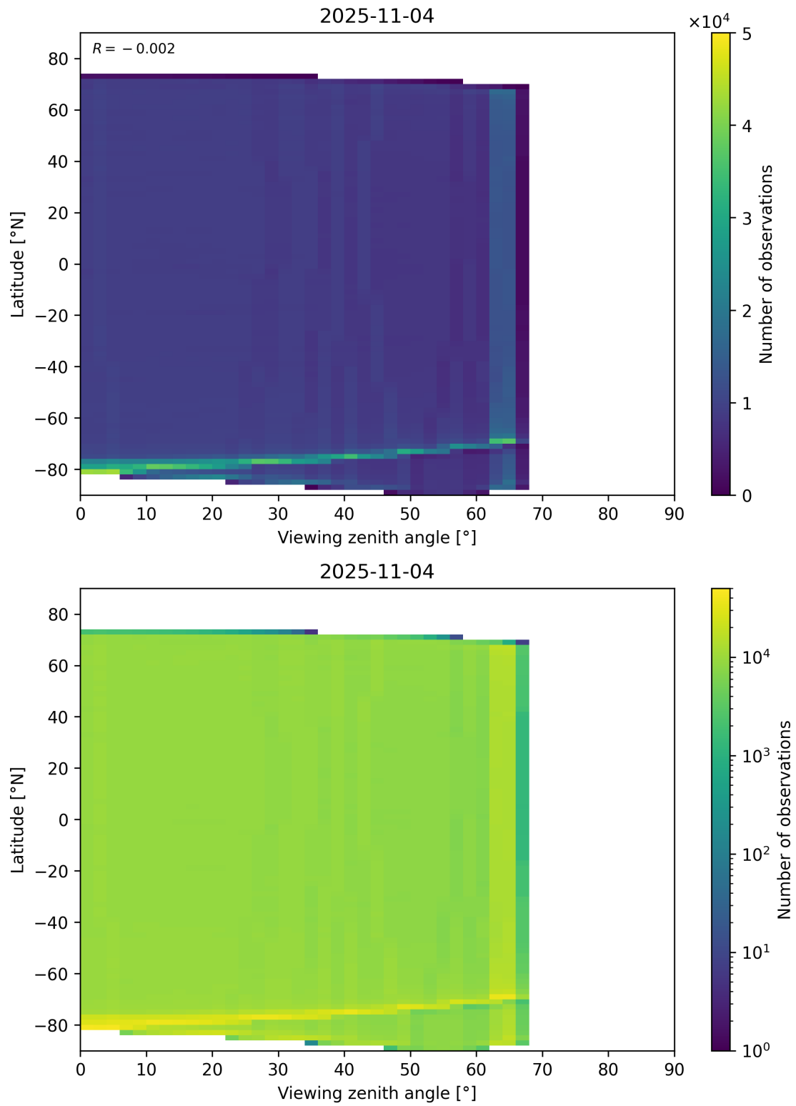
Figure 123: Scatter density plot of “Viewing zenith angle” against “Latitude” for 2025-11-03 to 2025-11-05.
