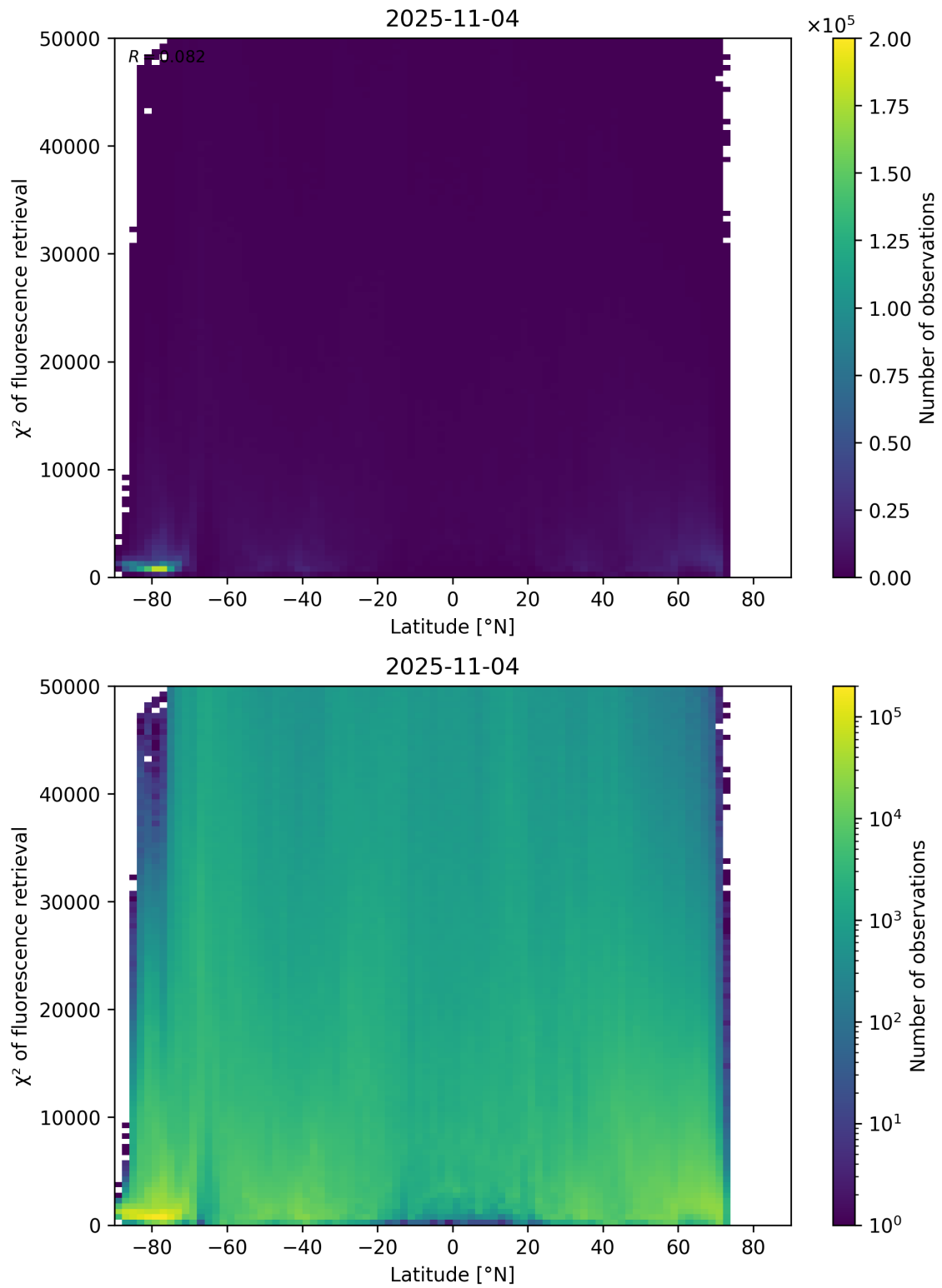
Figure 89: Scatter density plot of “Latitude” against “ \chi^2 of fluorescence retrieval” for 2025-11-03 to 2025-11-05.
