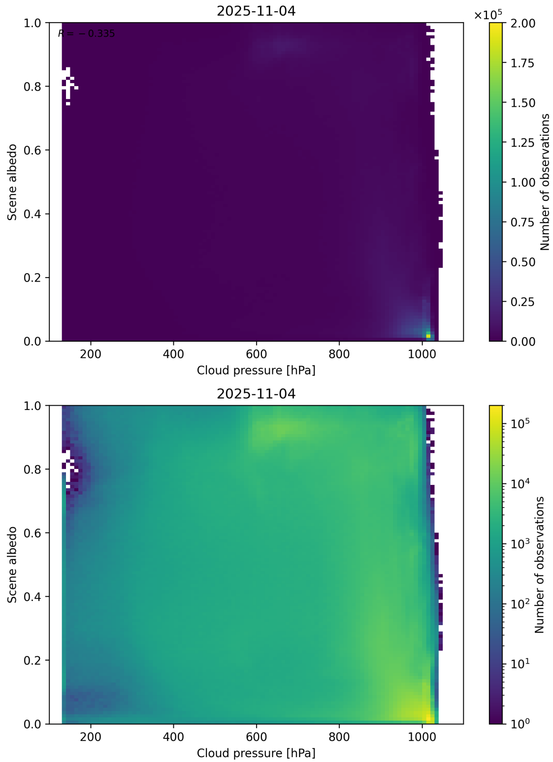
Figure 83: Scatter density plot of “Cloud pressure” against “Scene albedo” for 2025-11-03 to 2025-11-05.
