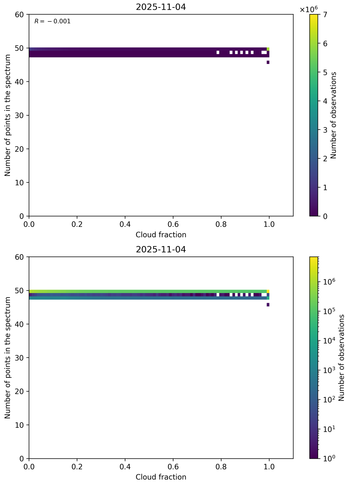
Figure 74: Scatter density plot of “Cloud fraction” against “Number of points in the spectrum” for 2025-11-03 to 2025-11-05.
