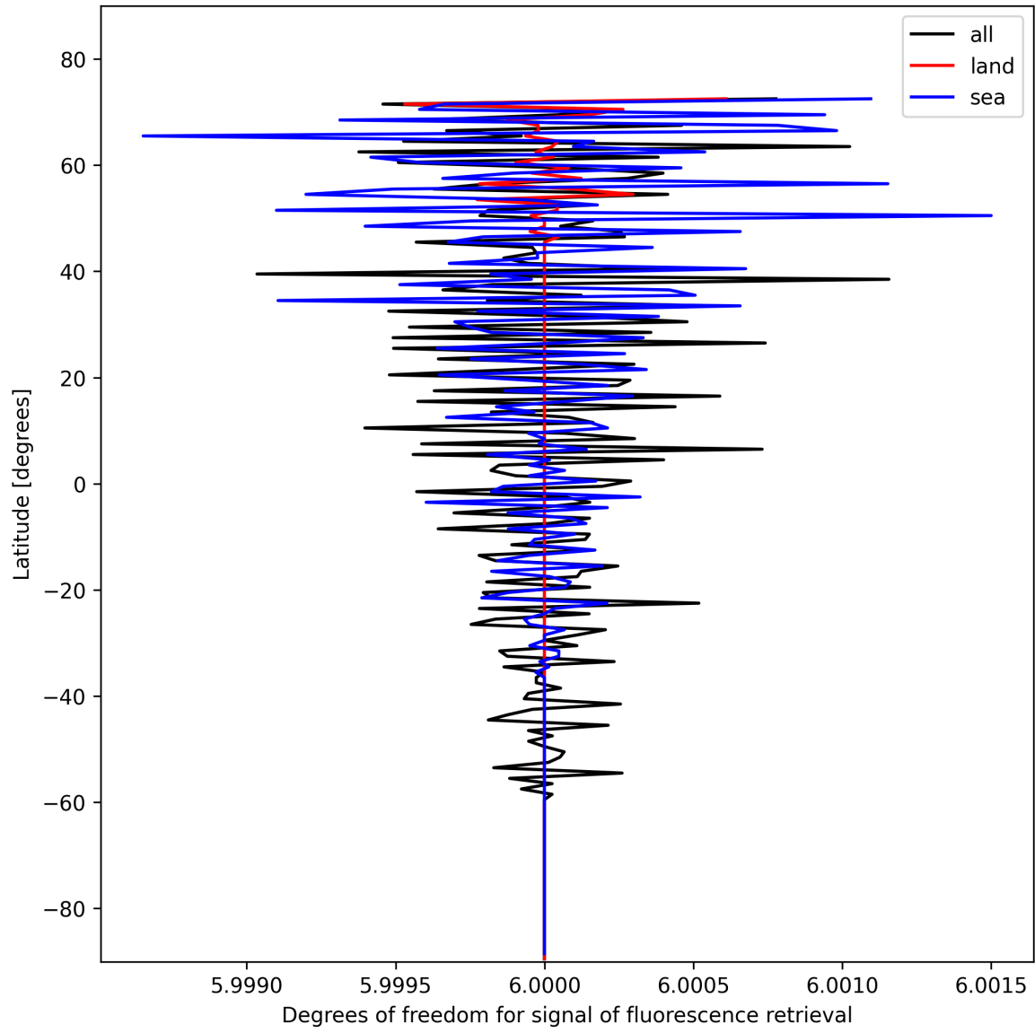
Figure 26: Zonal average of “Degrees of freedom for signal of fluorescence retrieval” for 2025-11-03 to 2025-11-05.
