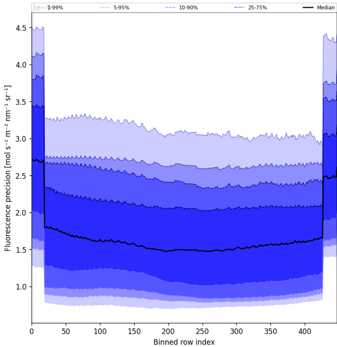
Figure 58: Along track statistics of “Fluorescence precision” for 2025-11-03 to 2025-11-05
