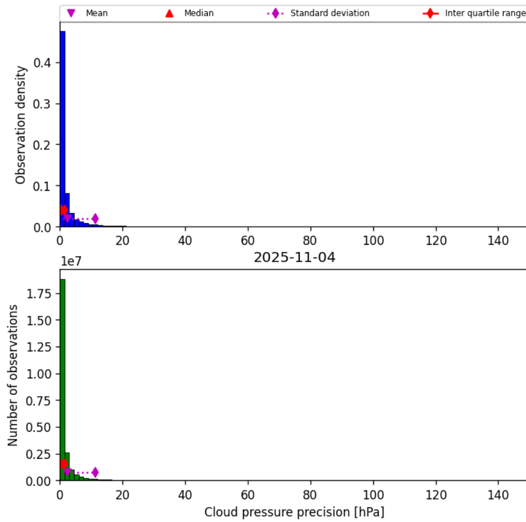
Figure 31: Histogram of “Cloud pressure precision” for 2025-11-03 to 2025-11-05
