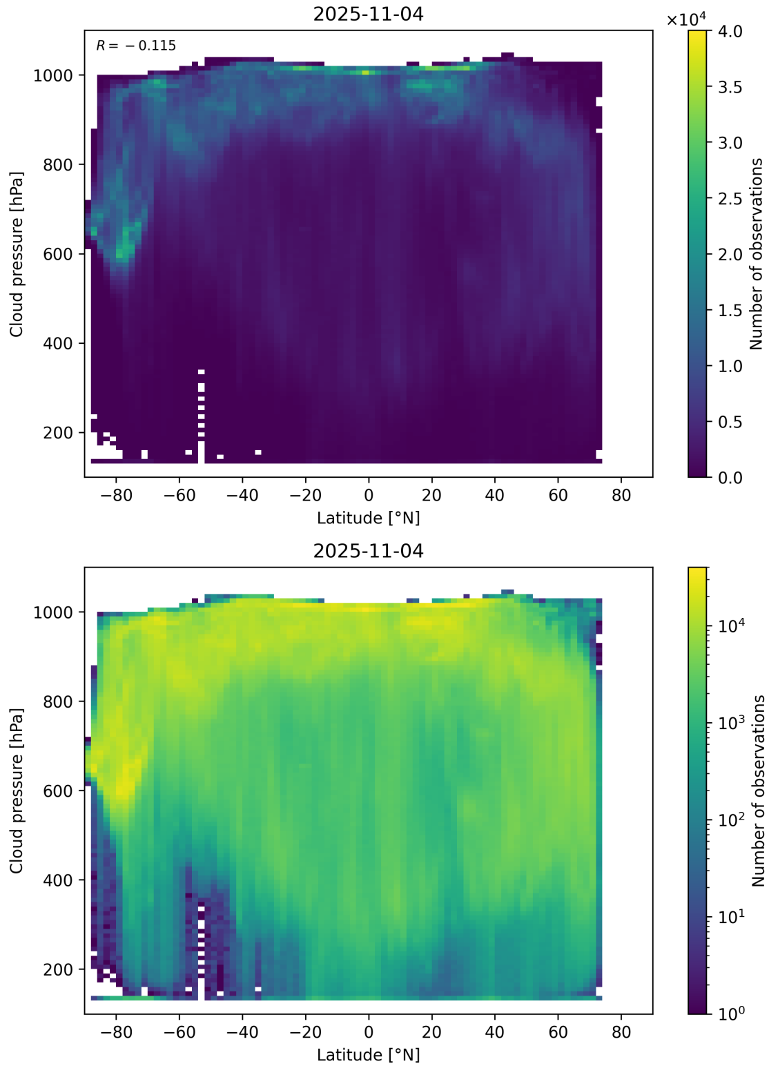
Figure 91: Scatter density plot of “Latitude” against “Cloud pressure” for 2025-11-03 to 2025-11-05.
