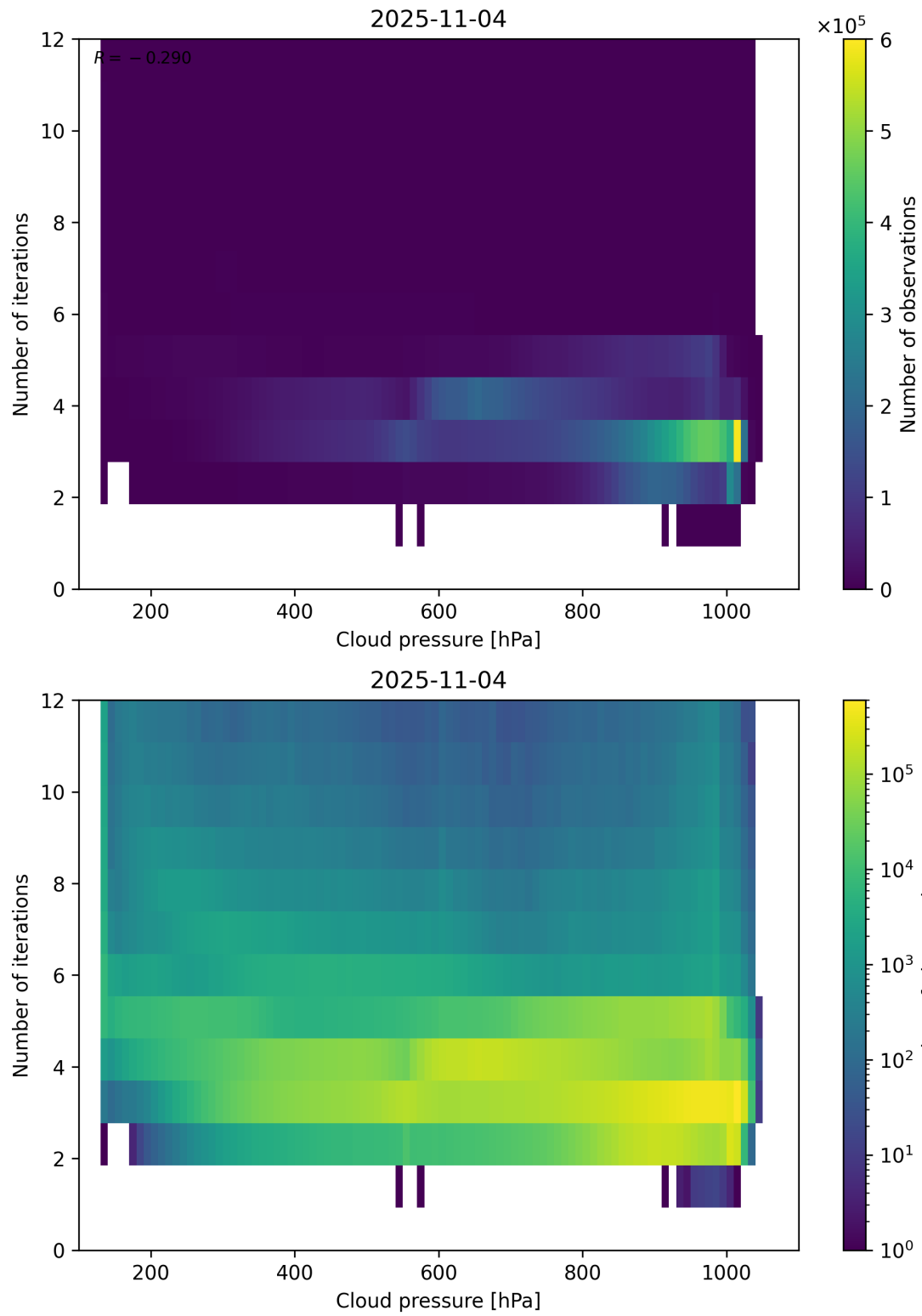
Figure 81: Scatter density plot of “Cloud pressure” against “Number of iterations” for 2025-11-03 to 2025-11-05.
