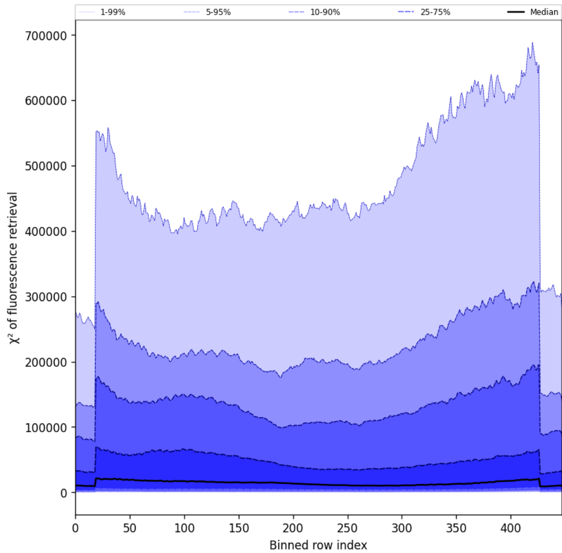
Figure 59: Along track statistics of “ \chi^2 of fluorescence retrieval” for 2025-11-03 to 2025-11-05
