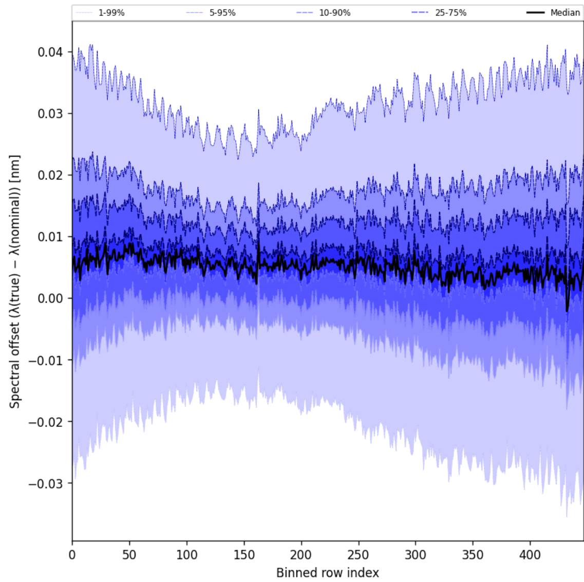
Figure 62: Along track statistics of “Spectral offset ( \lambda_{\text{true}} - \lambda_{\text{nominal}} )” for 2025-11-03 to 2025-11-05
