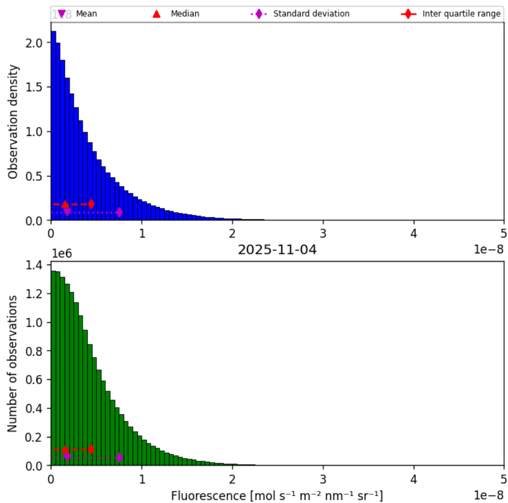
Figure 40: Histogram of “Fluorescence” for 2025-11-03 to 2025-11-05
