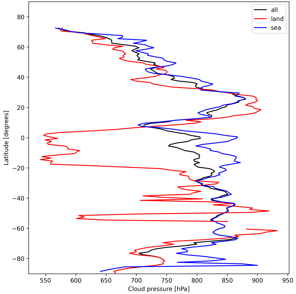
Figure 13: Zonal average of “Cloud pressure” for 2025-11-03 to 2025-11-05.
