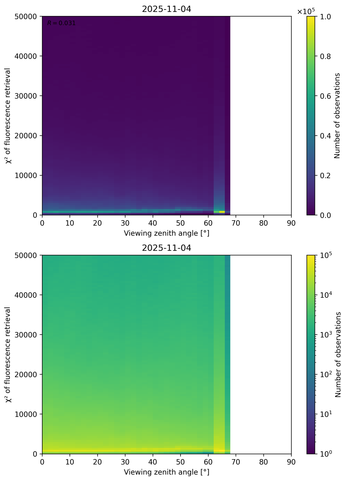
Figure 119: Scatter density plot of “Viewing zenith angle” against “ \chi^2 of fluorescence retrieval” for 2025-11-03 to 2025-11-05.
