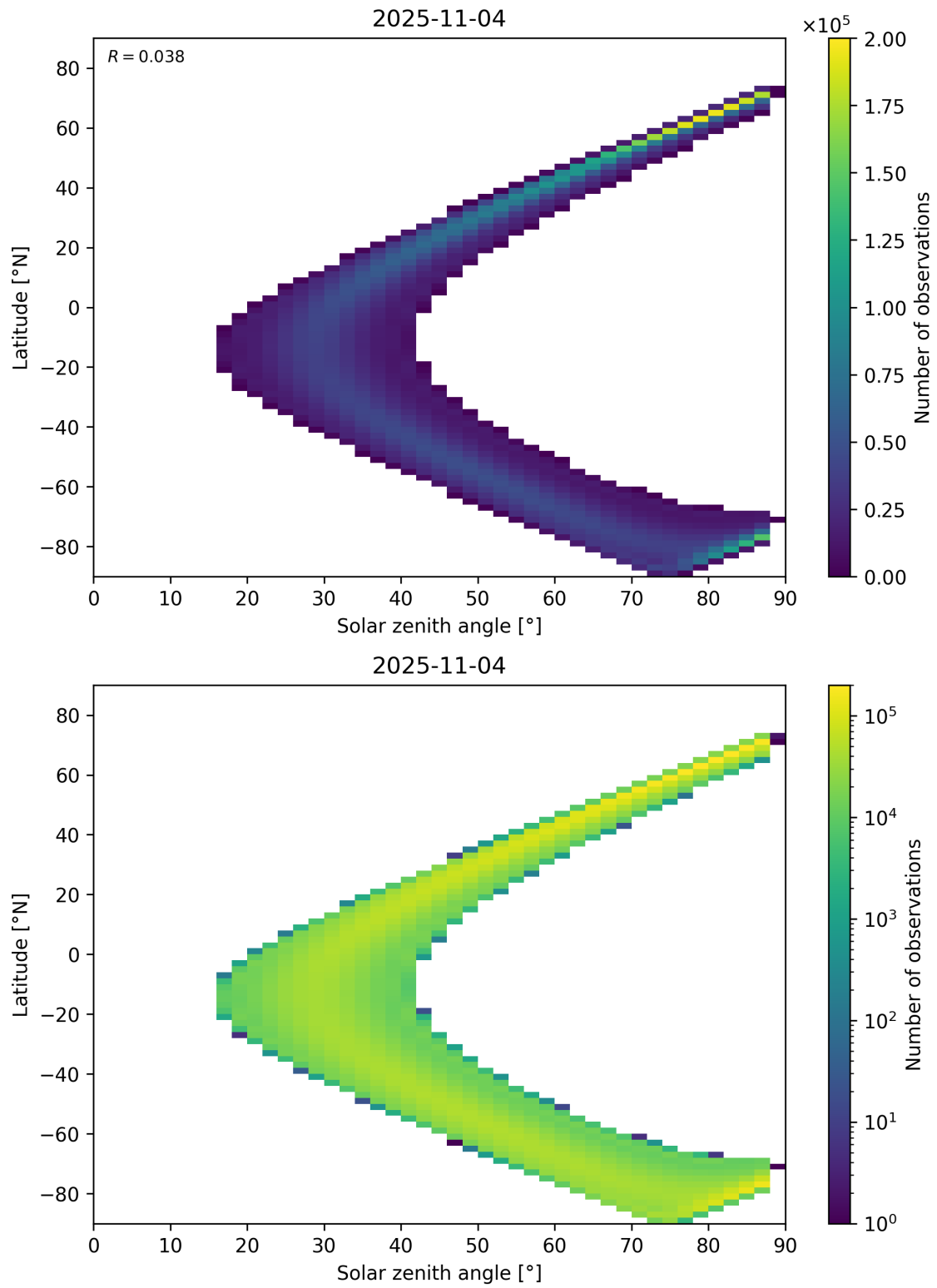
Figure 113: Scatter density plot of “Solar zenith angle” against “Latitude” for 2025-11-03 to 2025-11-05.
