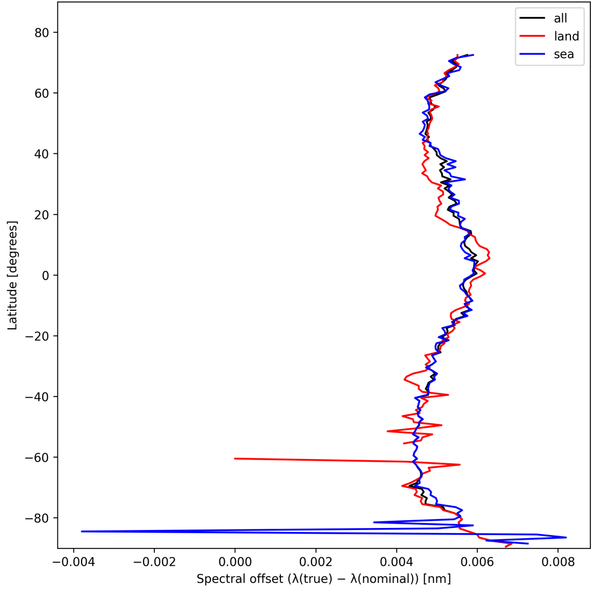
Figure 28: Zonal average of “Spectral offset ( \lambda_{\text{true}} - \lambda_{\text{nominal}} )” for 2025-11-03 to 2025-11-05.
