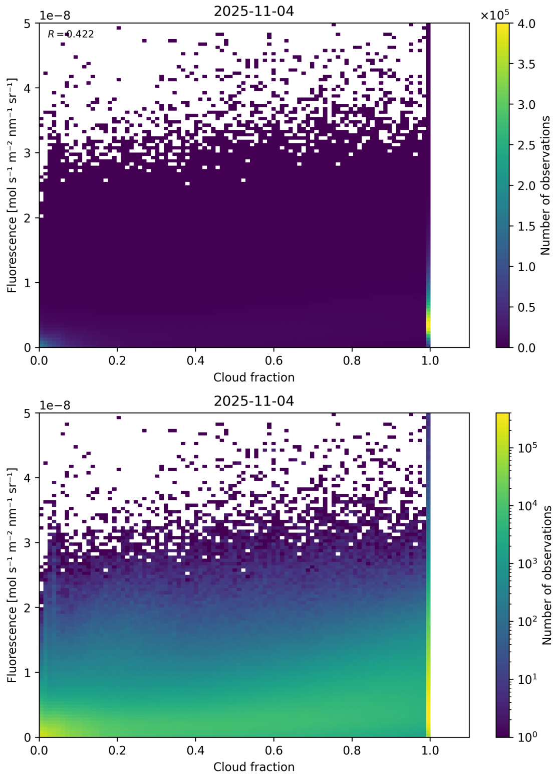
Figure 72: Scatter density plot of “Cloud fraction” against “Fluorescence” for 2025-11-03 to 2025-11-05.
