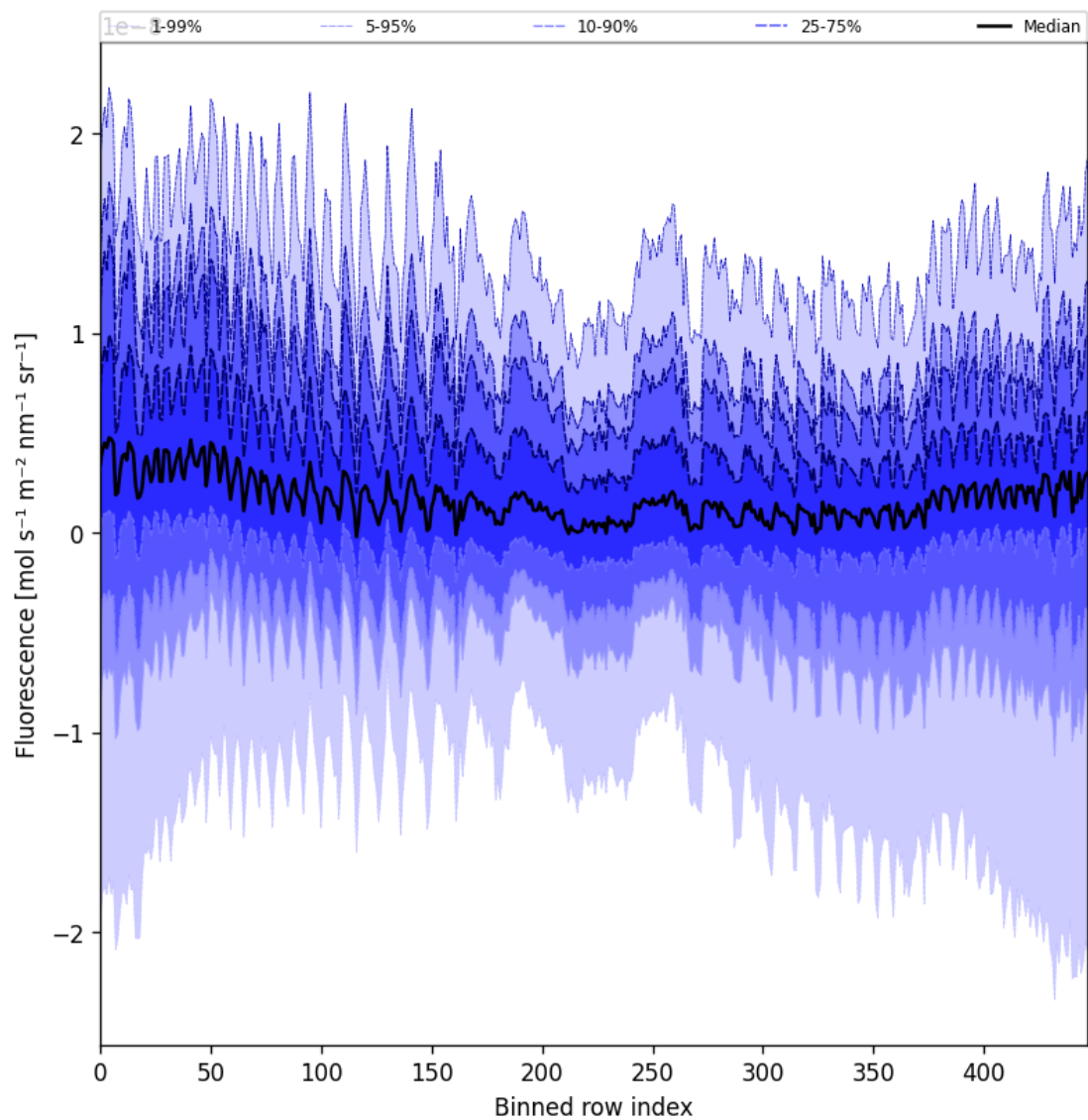
Figure 57: Along track statistics of “Fluorescence” for 2025-11-03 to 2025-11-05
