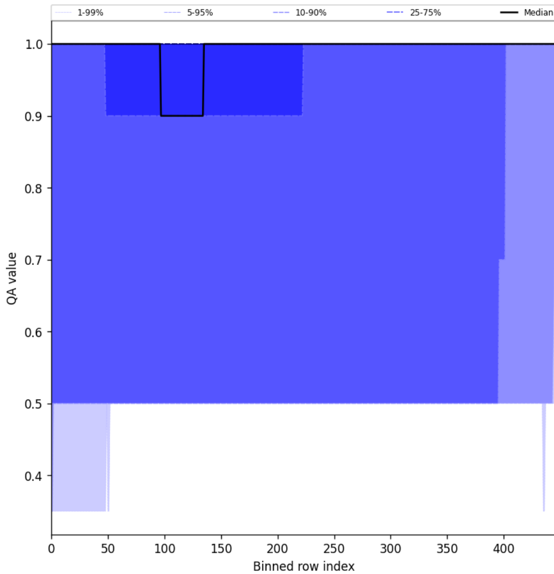
Figure 46: Along track statistics of “QA value” for 2025-11-03 to 2025-11-05
