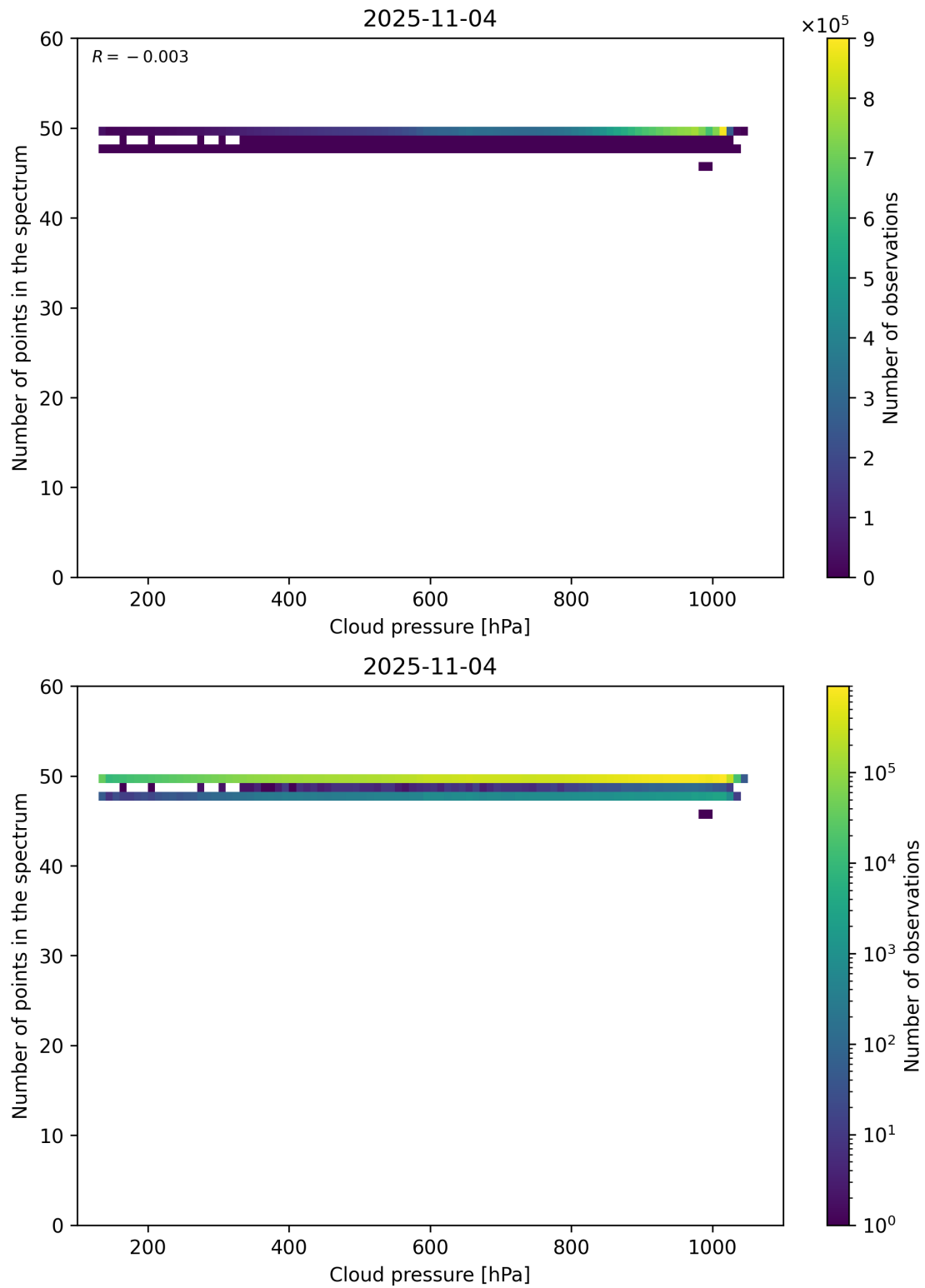
Figure 82: Scatter density plot of “Cloud pressure” against “Number of points in the spectrum” for 2025-11-03 to 2025-11-05.
