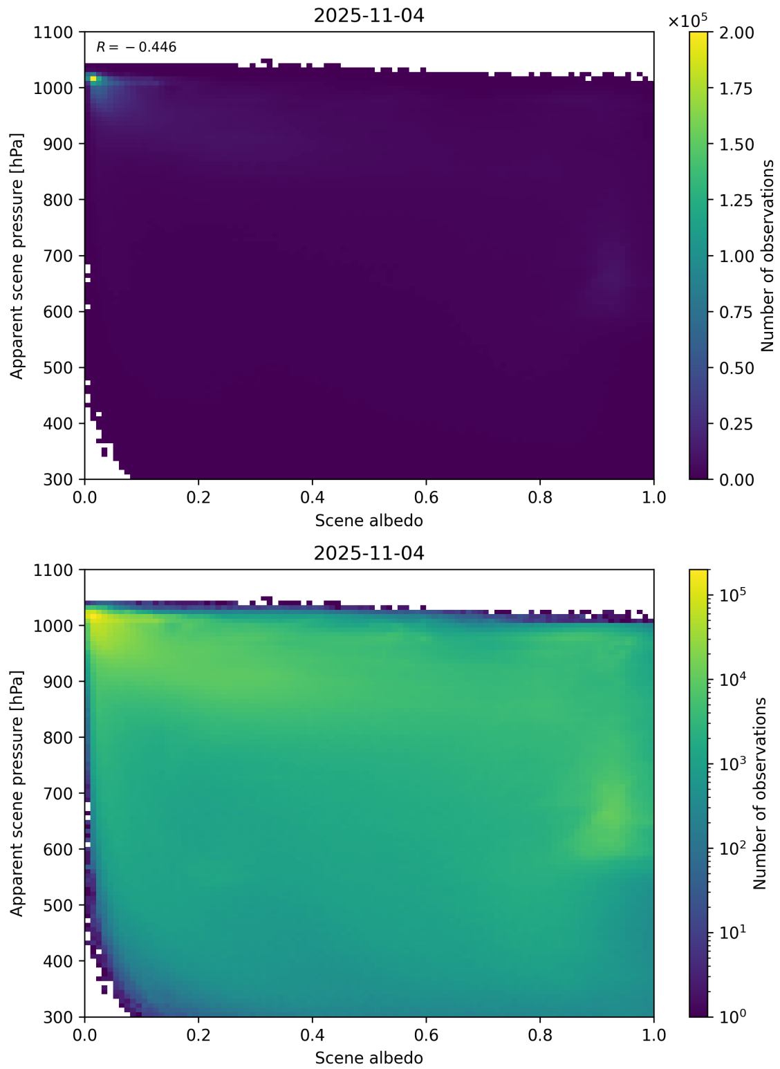
Figure 102: Scatter density plot of “Scene albedo” against “Apparent scene pressure” for 2025-11-03 to 2025-11-05.
