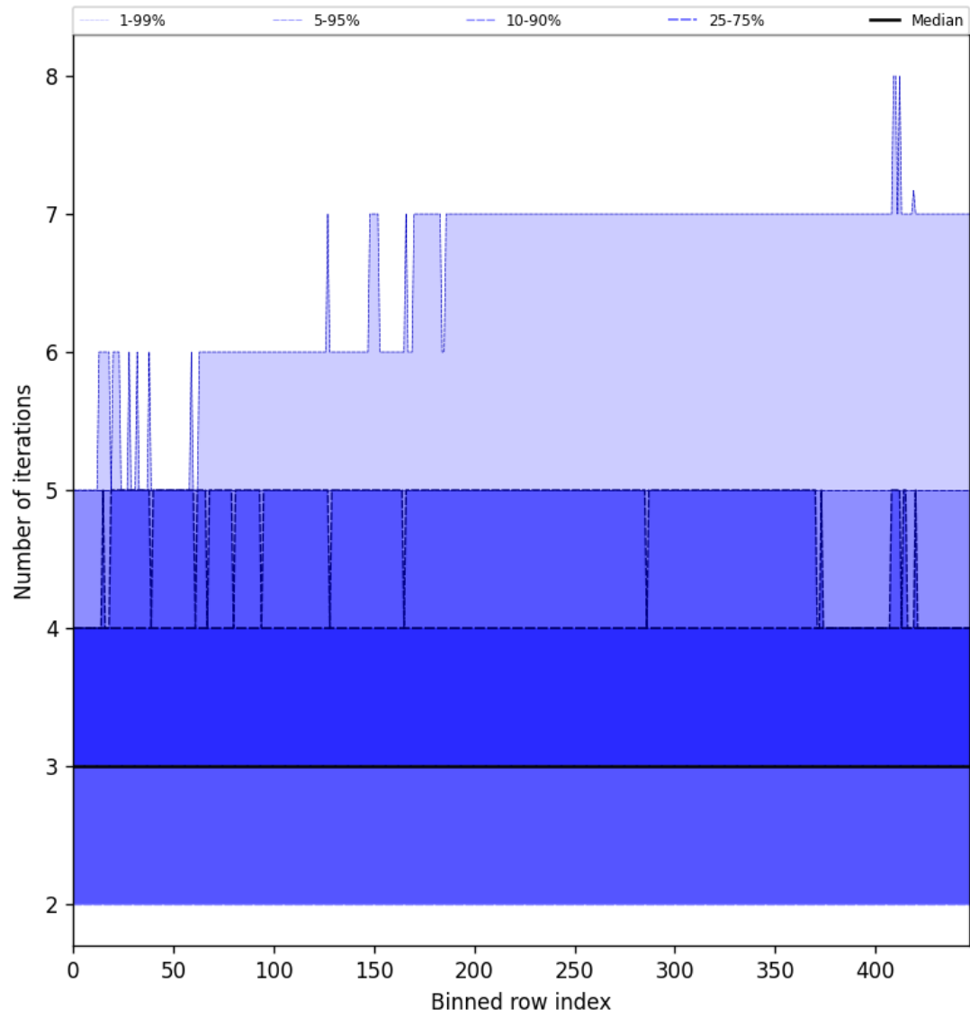
Figure 56: Along track statistics of “Number of iterations” for 2025-11-03 to 2025-11-05
