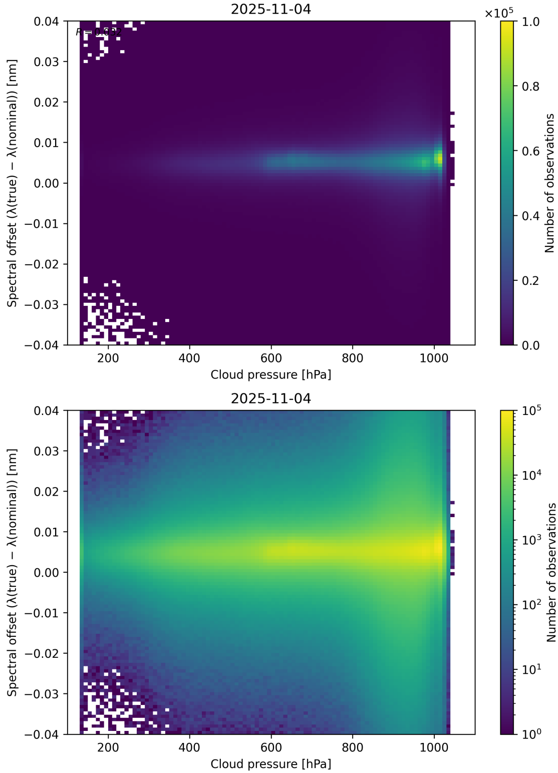
Figure 84: Scatter density plot of “Cloud pressure” against “Spectral offset ( \lambda_{\text{true}} - \lambda_{\text{nominal}} )” for 2025-11-03 to 2025-11-05.
