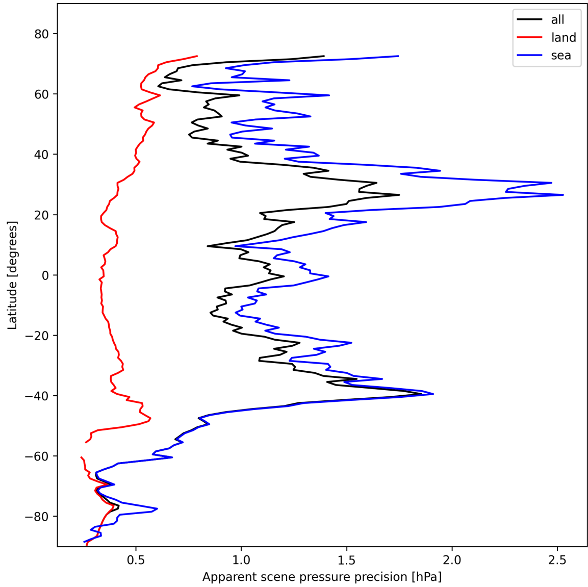
Figure 20: Zonal average of “Apparent scene pressure precision” for 2025-11-03 to 2025-11-05.
