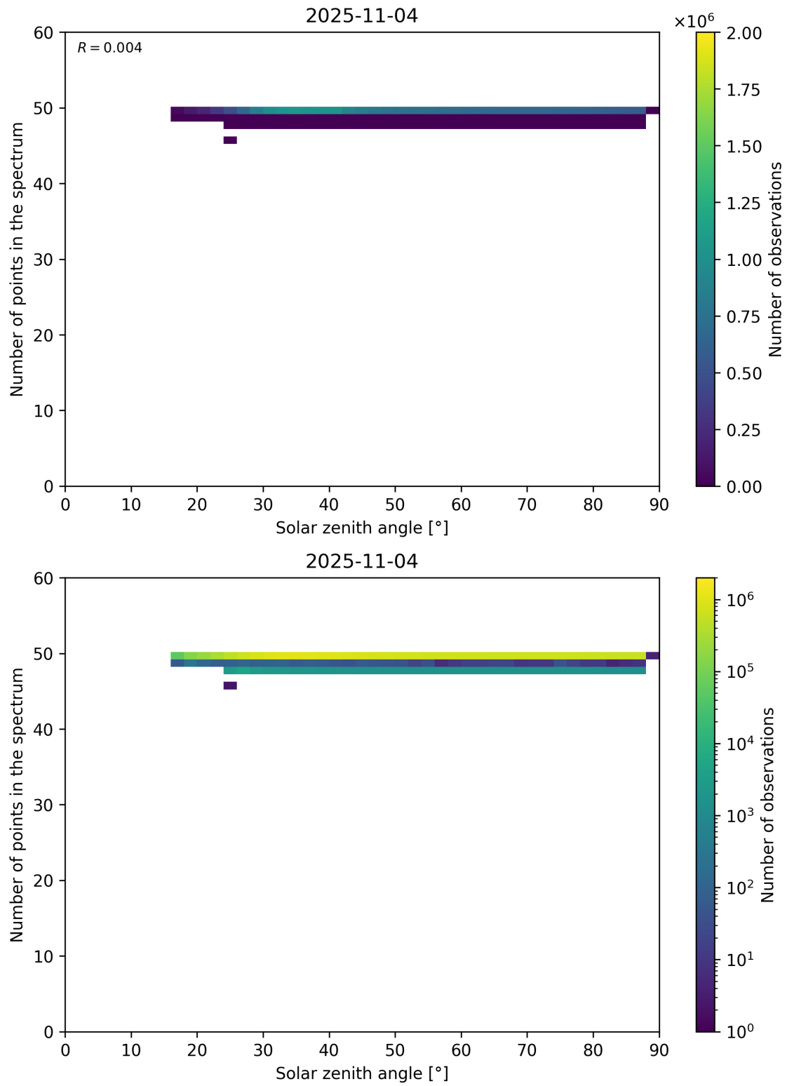
Figure 115: Scatter density plot of “Solar zenith angle” against “Number of points in the spectrum” for 2025-11-03 to 2025-11-05.
