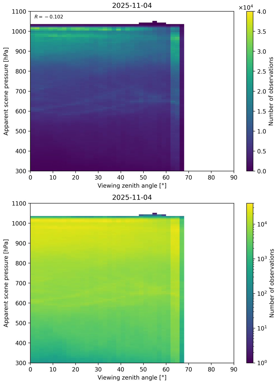
Figure 118: Scatter density plot of “Viewing zenith angle” against “Apparent scene pressure” for 2025-11-03 to 2025-11-05.
