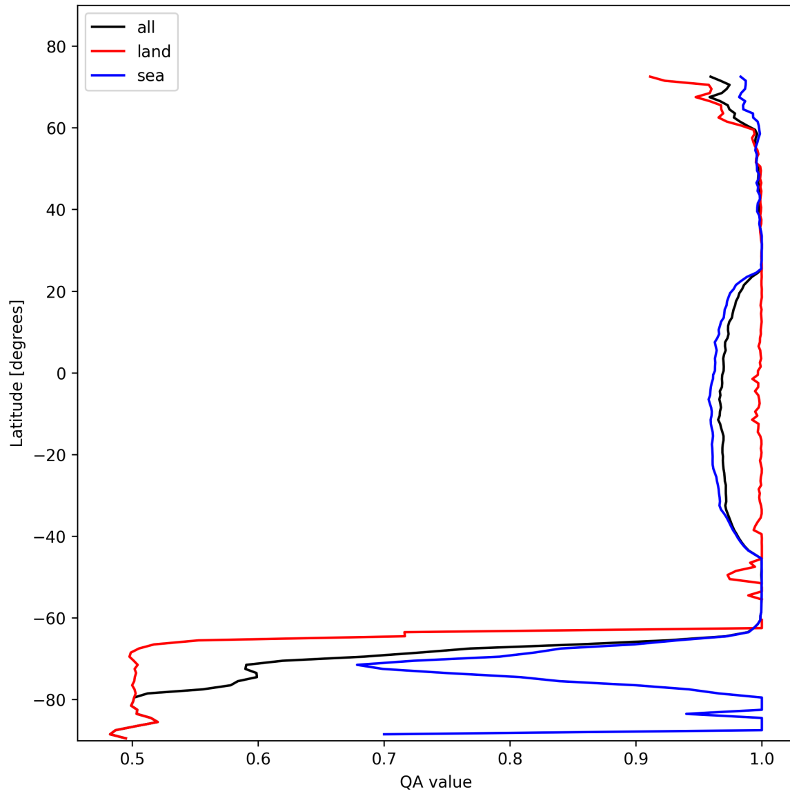
Figure 12: Zonal average of “QA value” for 2025-11-03 to 2025-11-05.
