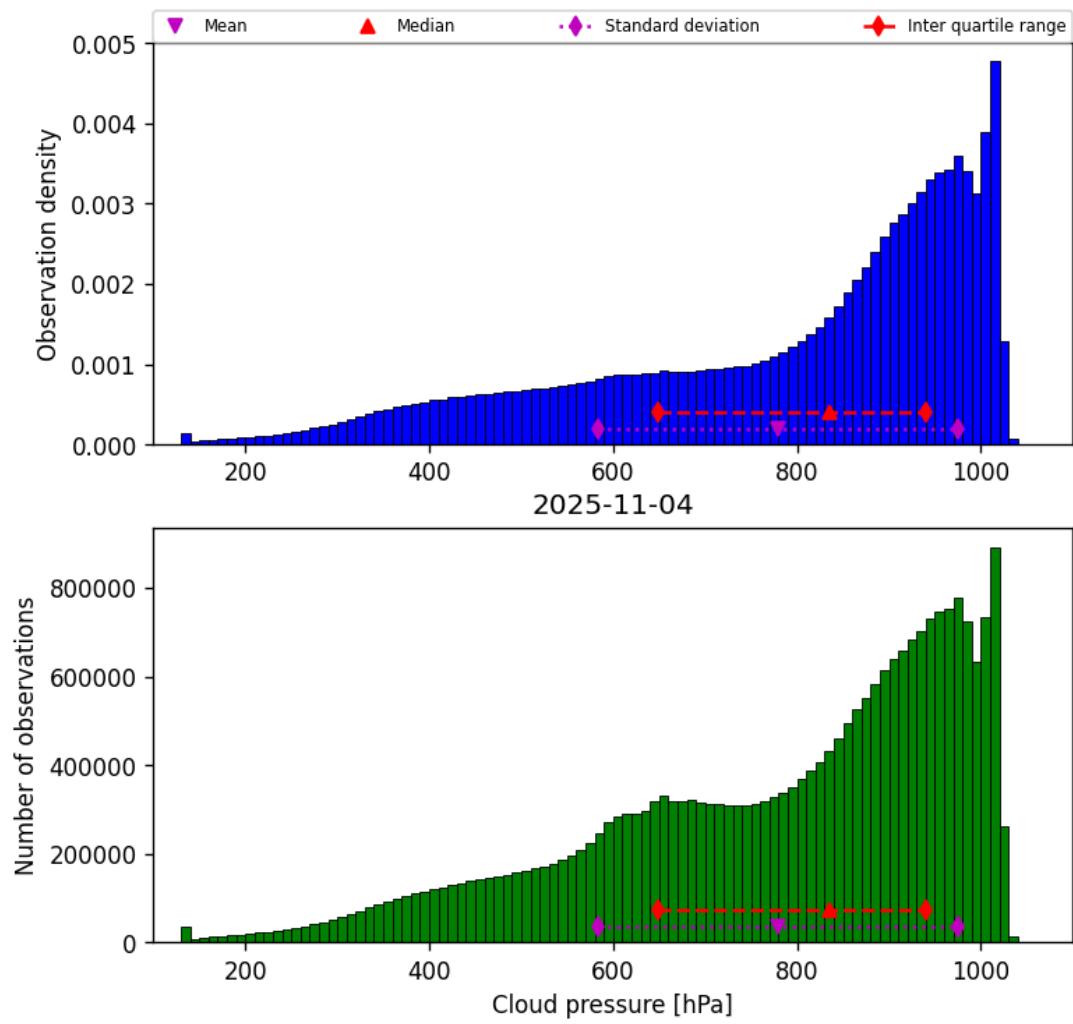
Figure 30: Histogram of “Cloud pressure” for 2025-11-03 to 2025-11-05
