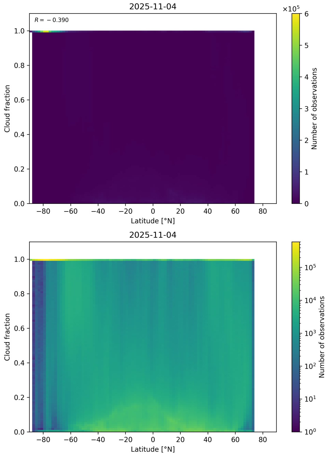
Figure 90: Scatter density plot of “Latitude” against “Cloud fraction” for 2025-11-03 to 2025-11-05.
