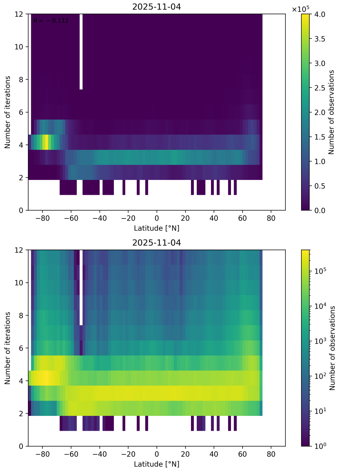
Figure 93: Scatter density plot of “Latitude” against “Number of iterations” for 2025-11-03 to 2025-11-05.
