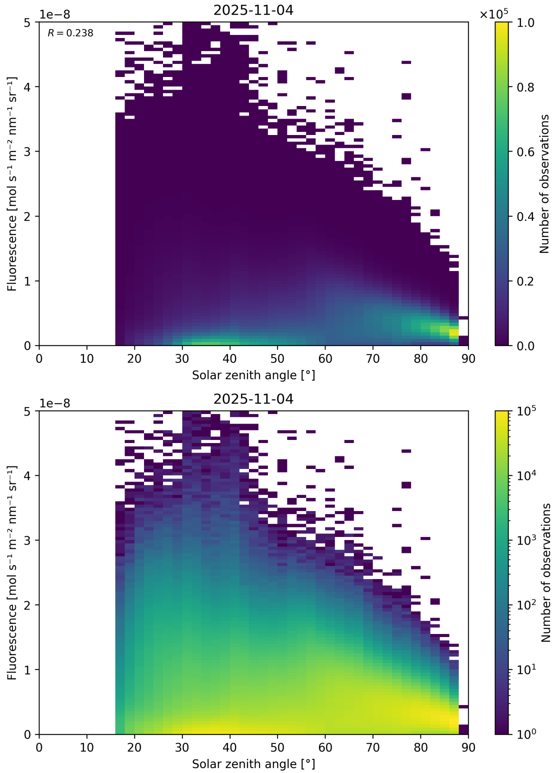
Figure 112: Scatter density plot of “Solar zenith angle” against “Fluorescence” for 2025-11-03 to 2025-11-05.
