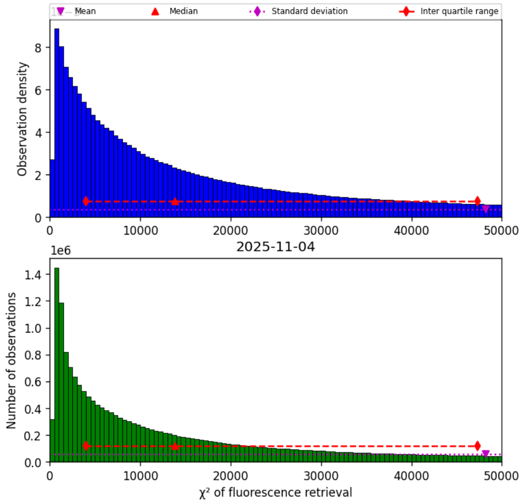
Figure 42: Histogram of “ \chi^2 of fluorescence retrieval” for 2025-11-03 to 2025-11-05
