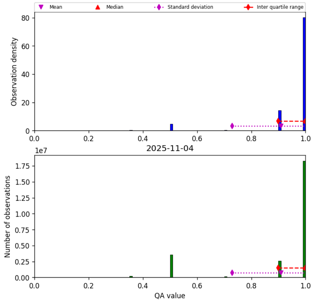
Figure 29: Histogram of “QA value” for 2025-11-03 to 2025-11-05
