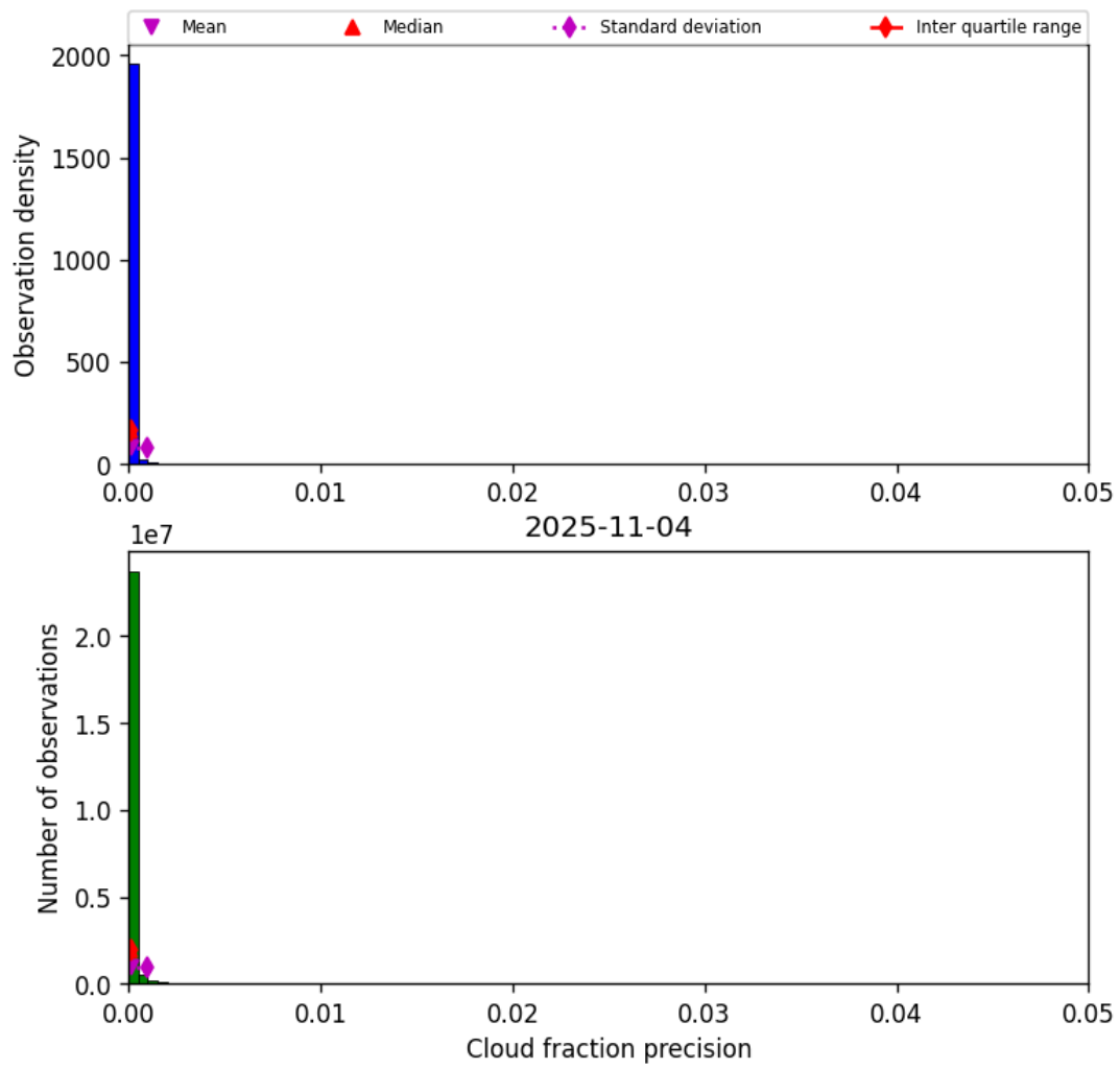
Figure 33: Histogram of “Cloud fraction precision” for 2025-11-03 to 2025-11-05
