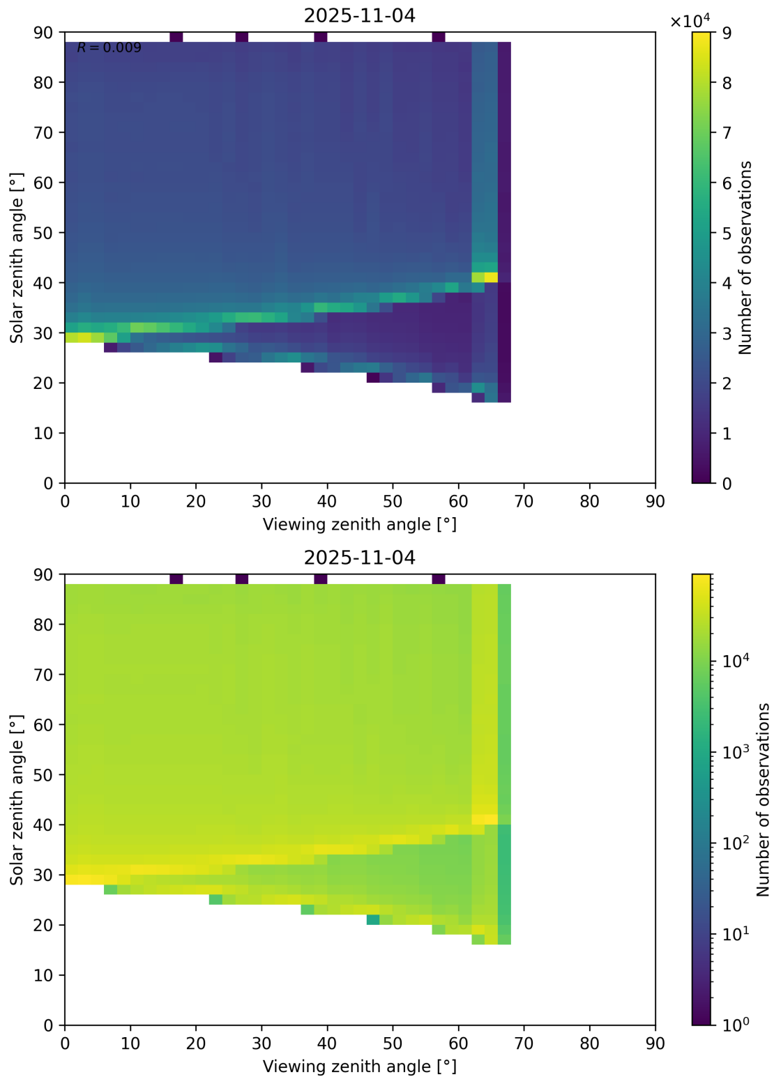
Figure 127: Scatter density plot of “Viewing zenith angle” against “Solar zenith angle” for 2025-11-03 to 2025-11-05.
