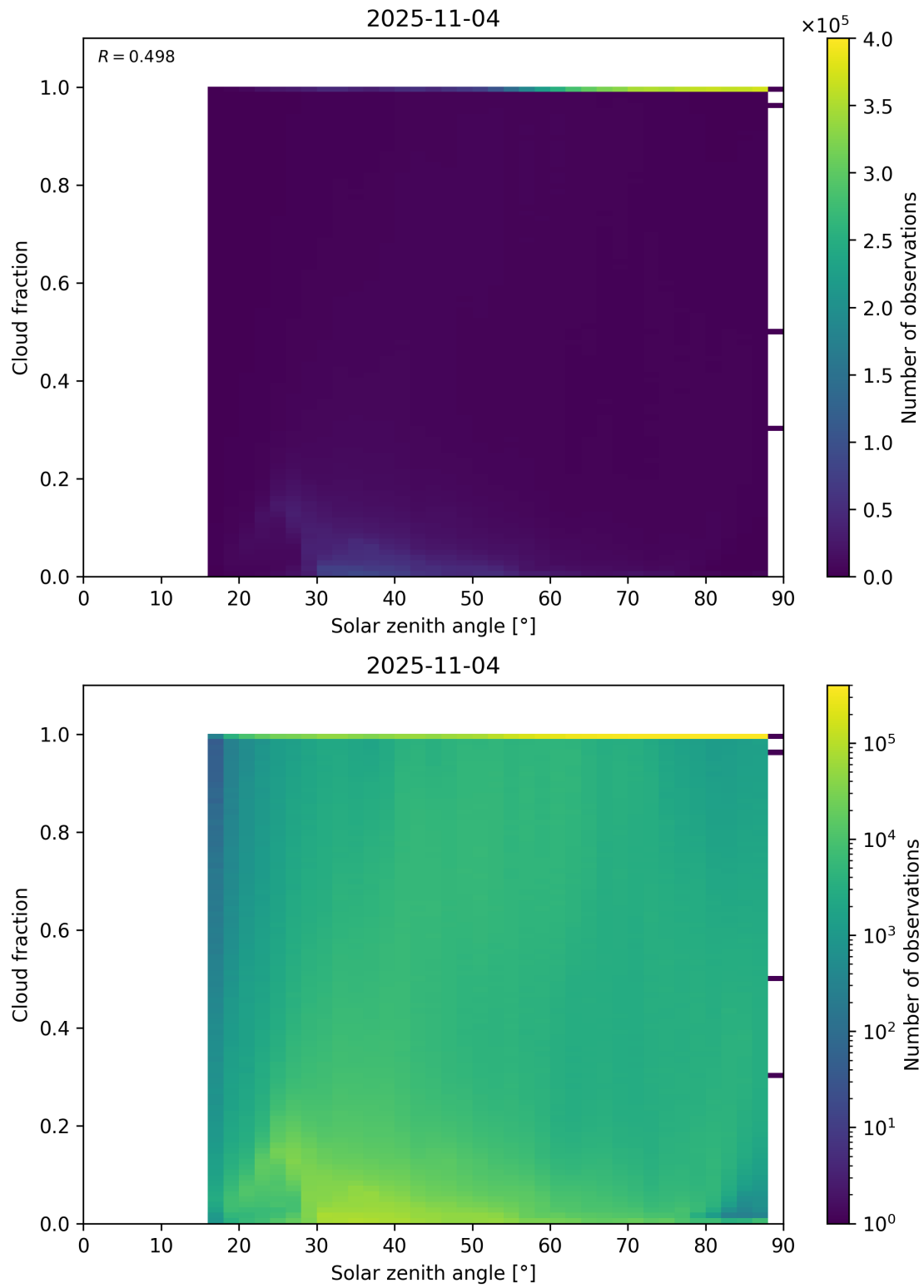
Figure 110: Scatter density plot of “Solar zenith angle” against “Cloud fraction” for 2025-11-03 to 2025-11-05.
