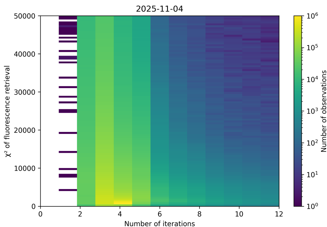
Figure 97: Scatter density plot of “Number of iterations” against “ \chi^2 of fluorescence retrieval” for 2025-11-03 to 2025-11-05.
