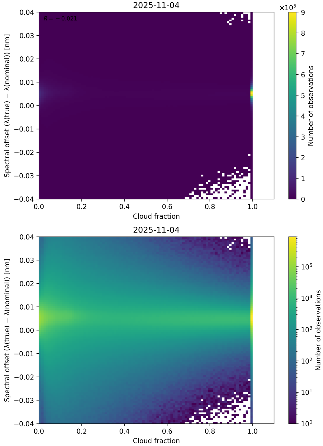
Figure 76: Scatter density plot of “Cloud fraction” against “Spectral offset ( \lambda_{\text{true}} - \lambda_{\text{nominal}} )” for 2025-11-03 to 2025-11-05.
