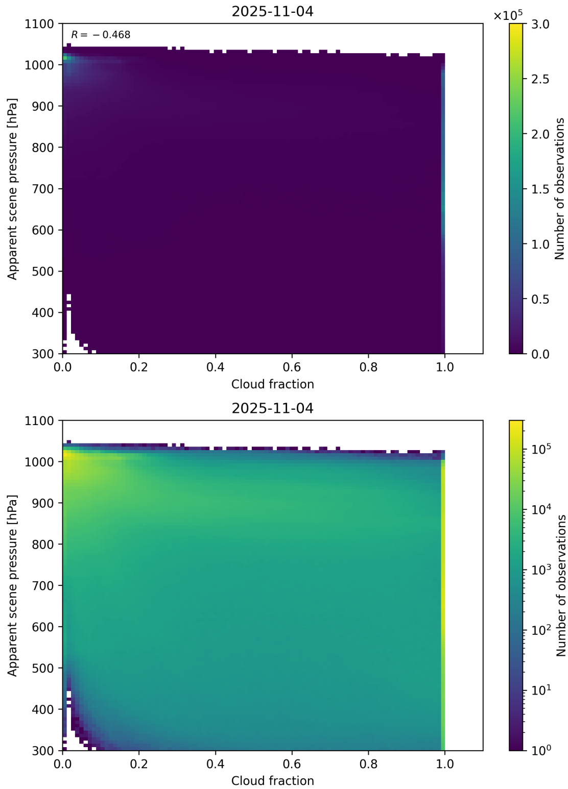
Figure 70: Scatter density plot of “Cloud fraction” against “Apparent scene pressure” for 2025-11-03 to 2025-11-05.
