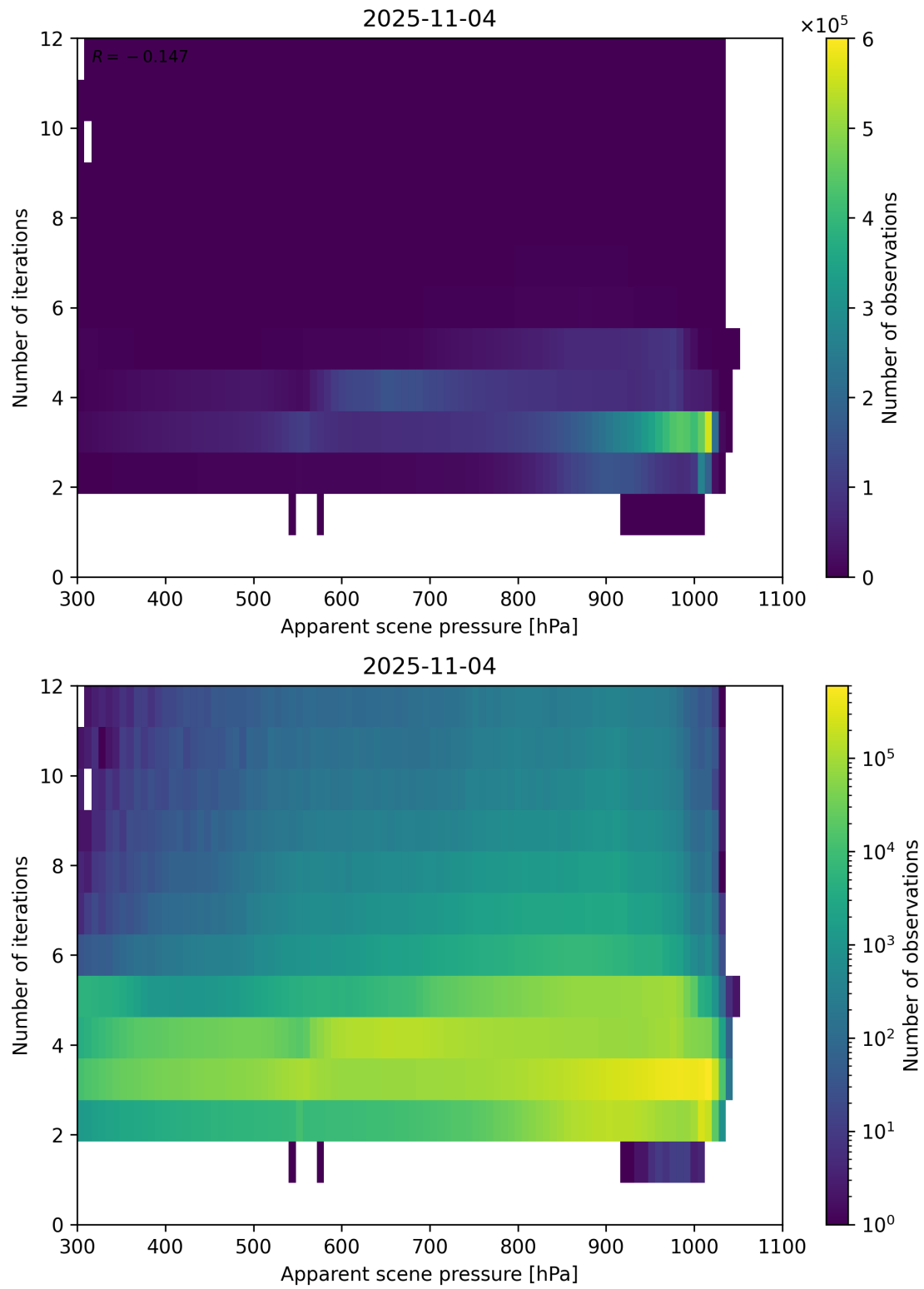
Figure 65: Scatter density plot of “Apparent scene pressure” against “Number of iterations” for 2025-11-03 to 2025-11-05.
