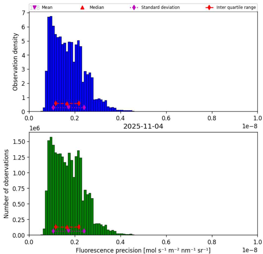
Figure 41: Histogram of “Fluorescence precision” for 2025-11-03 to 2025-11-05
