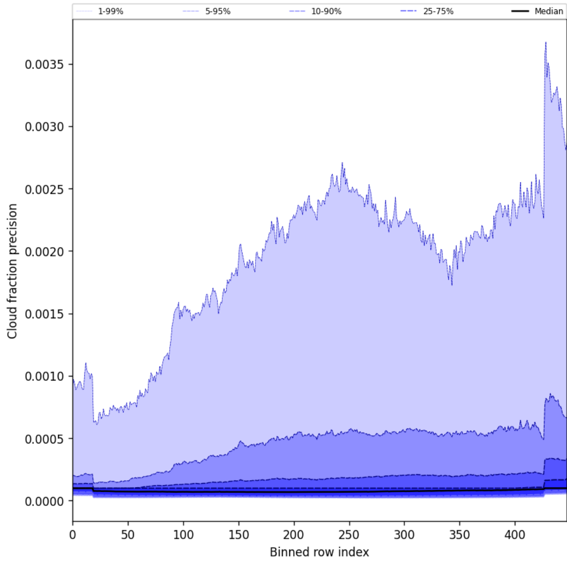
Figure 50: Along track statistics of “Cloud fraction precision” for 2025-11-03 to 2025-11-05
