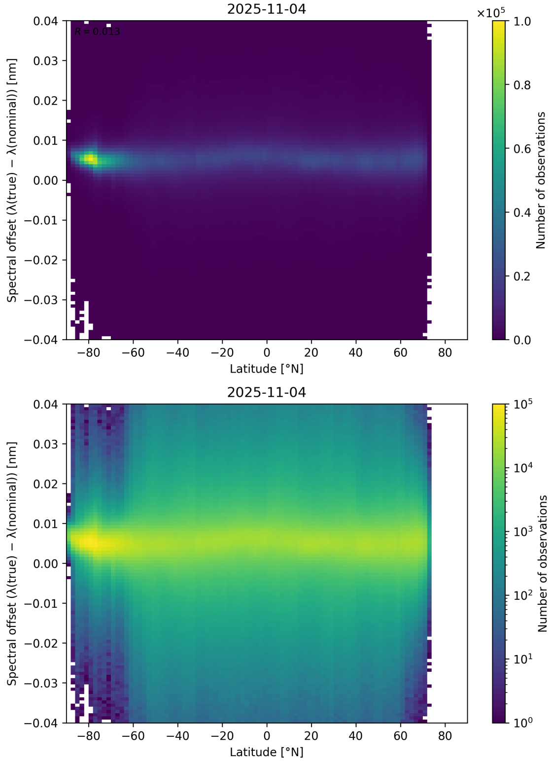
Figure 96: Scatter density plot of “Latitude” against “Spectral offset ( \lambda_{\text{true}} - \lambda_{\text{nominal}} )” for 2025-11-03 to 2025-11-05.
