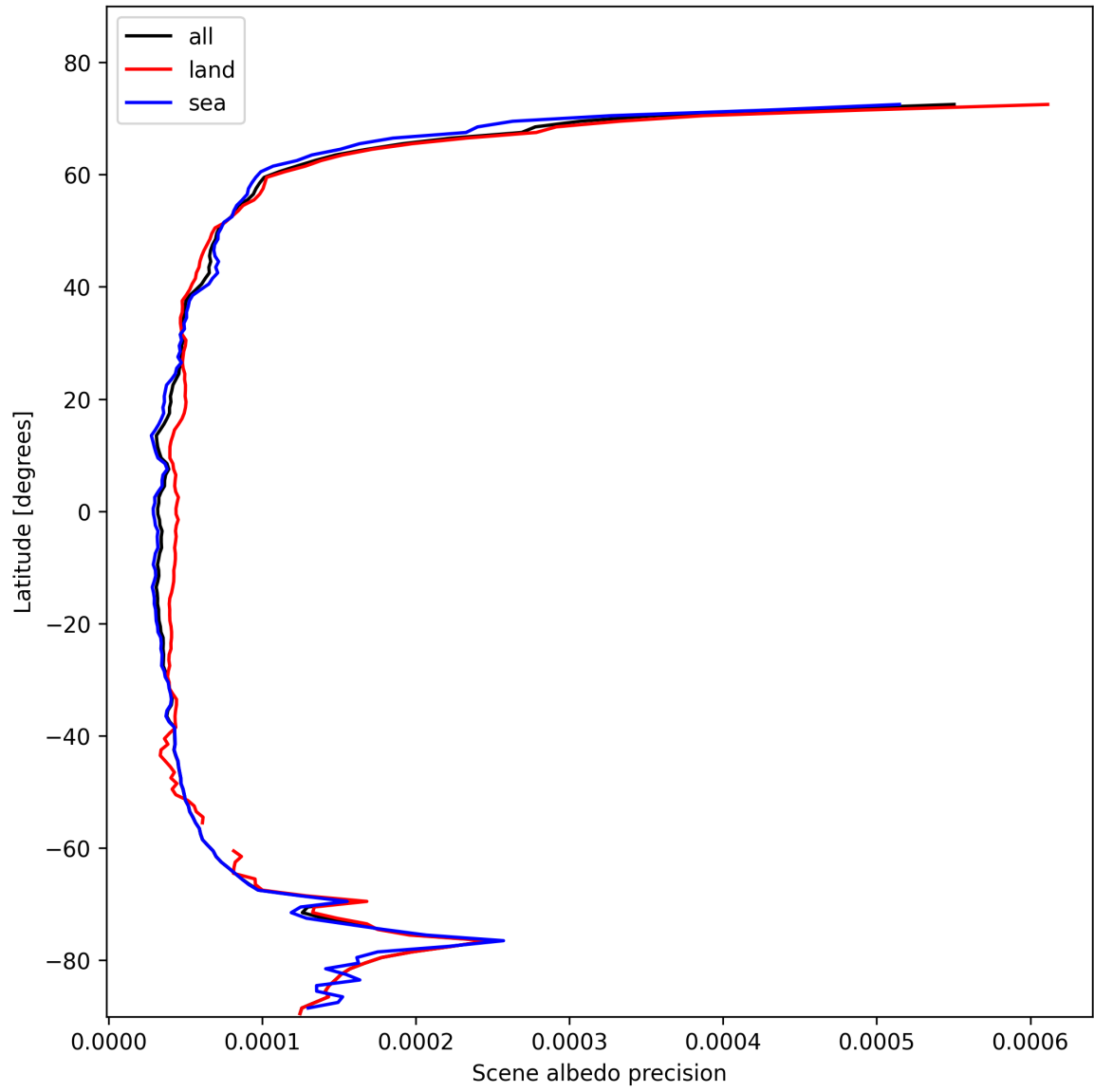
Figure 18: Zonal average of "Scene albedo precision" for 2025-11-03 to 2025-11-05.
