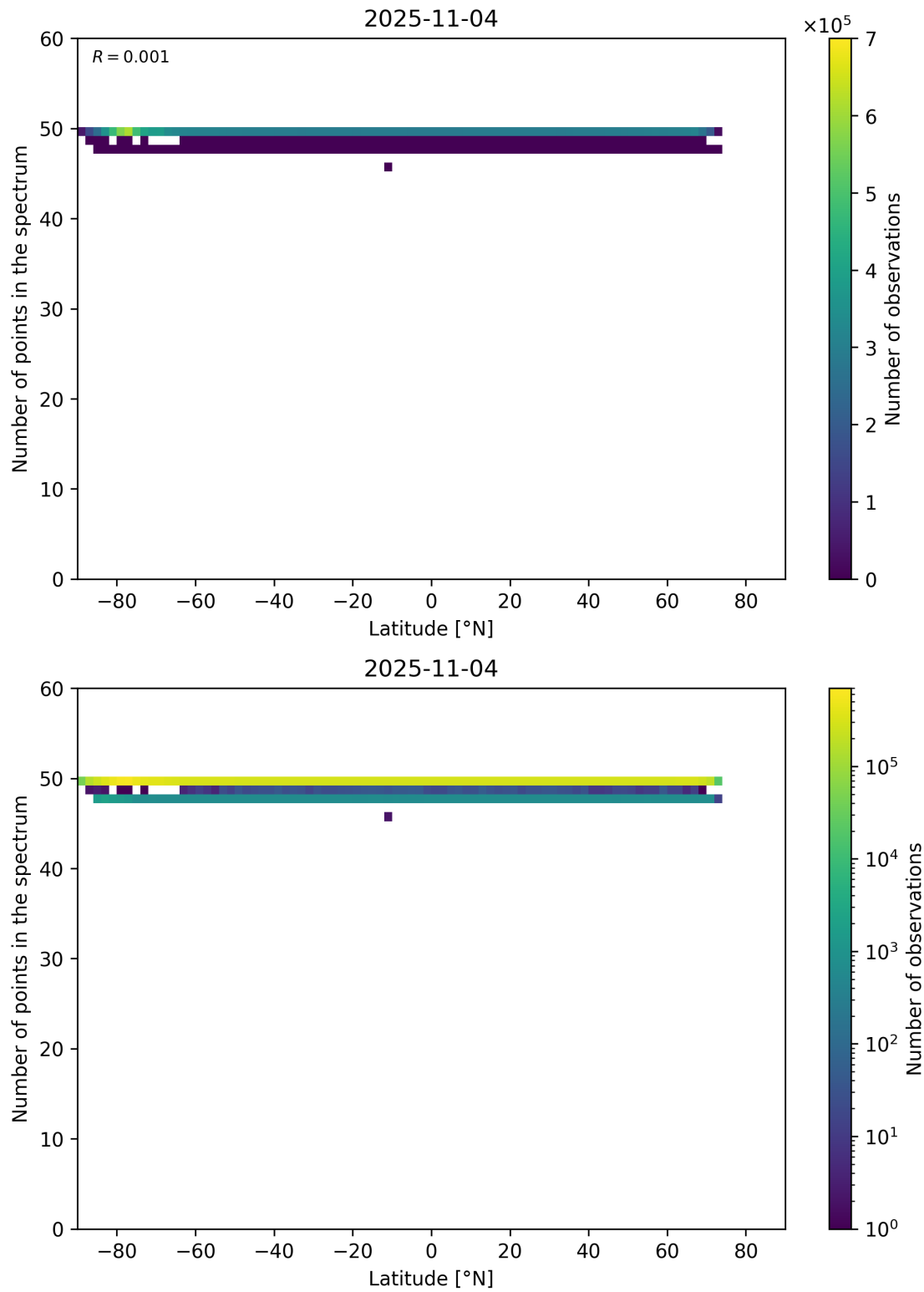
Figure 94: Scatter density plot of “Latitude” against “Number of points in the spectrum” for 2025-11-03 to 2025-11-05.
