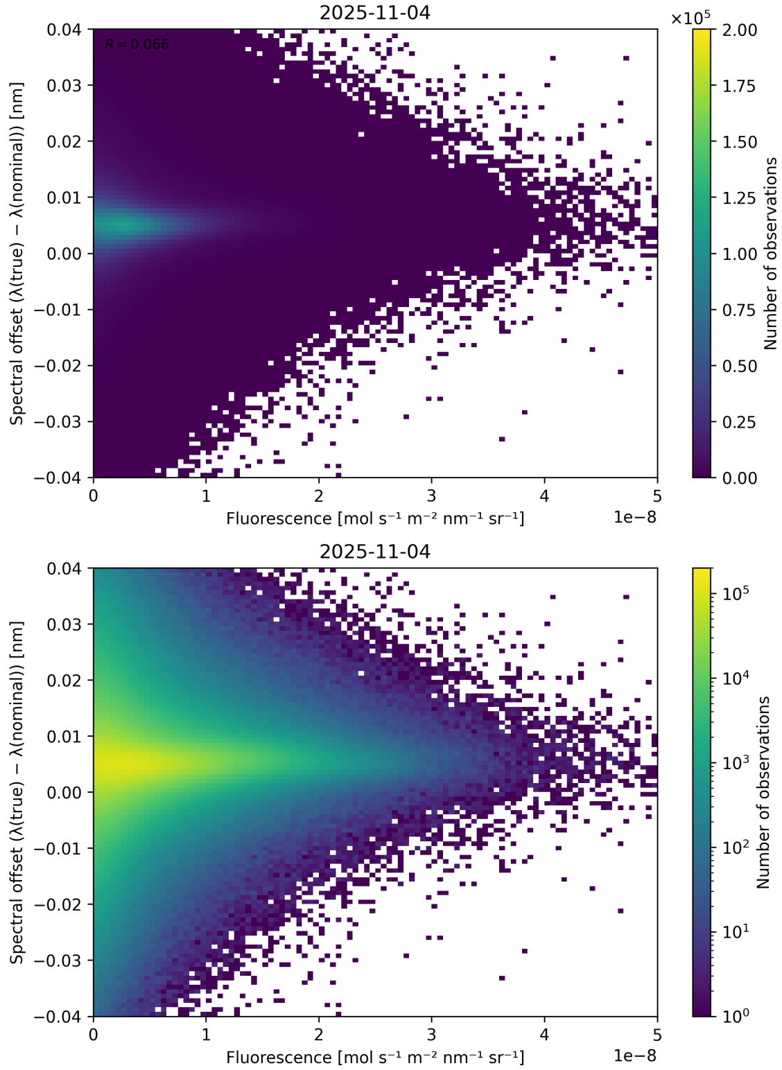
Figure 87: Scatter density plot of “Fluorescence” against “Spectral offset ( \lambda_{\text{true}} - \lambda_{\text{nominal}} )” for 2025-11-03 to 2025-11-05.
