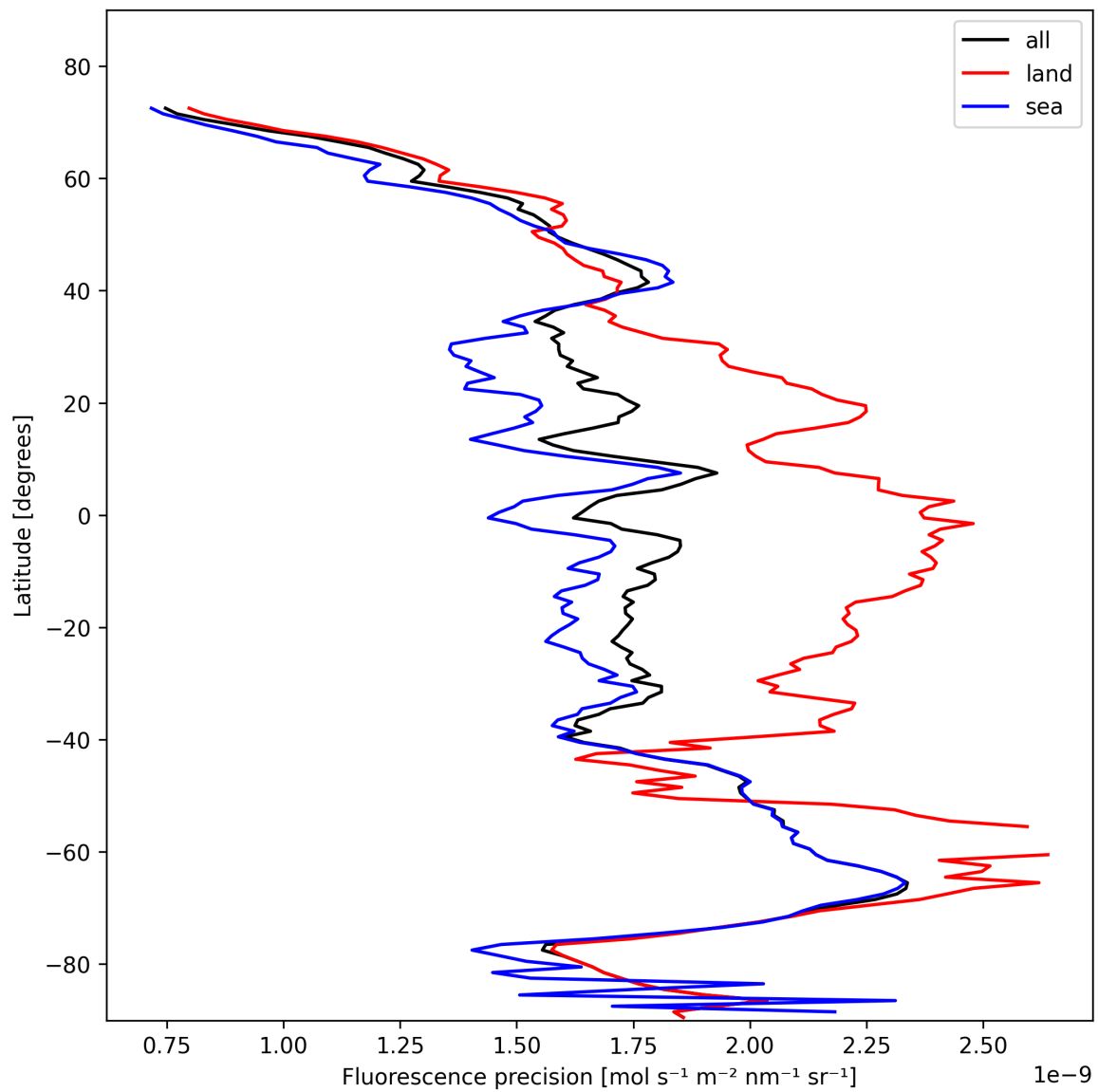
Figure 24: Zonal average of “Fluorescence precision” for 2025-11-03 to 2025-11-05.
