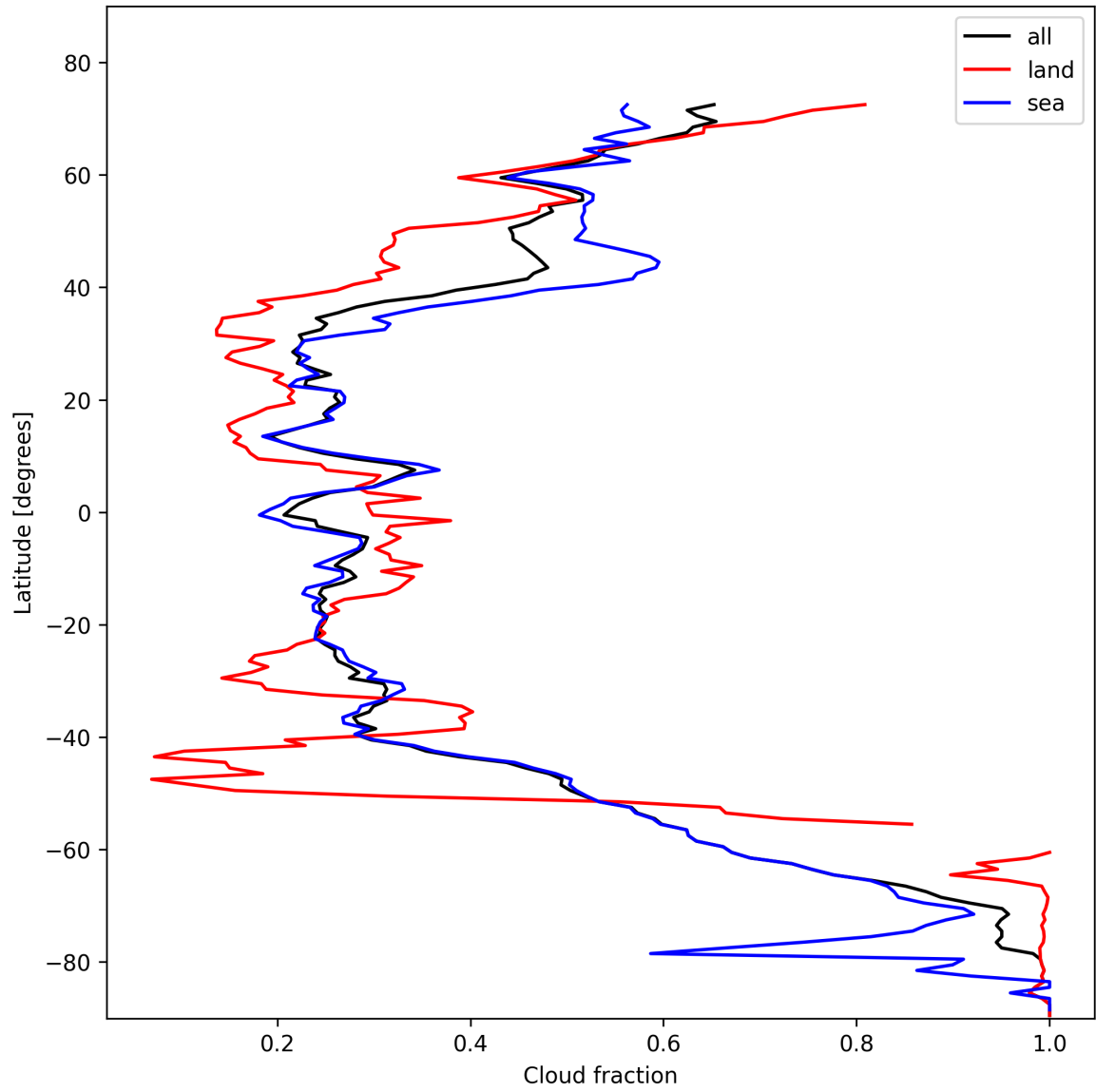
Figure 15: Zonal average of “Cloud fraction” for 2025-11-03 to 2025-11-05.
