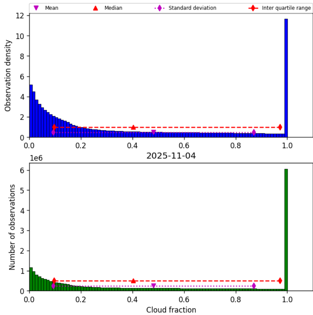
Figure 32: Histogram of “Cloud fraction” for 2025-11-03 to 2025-11-05
