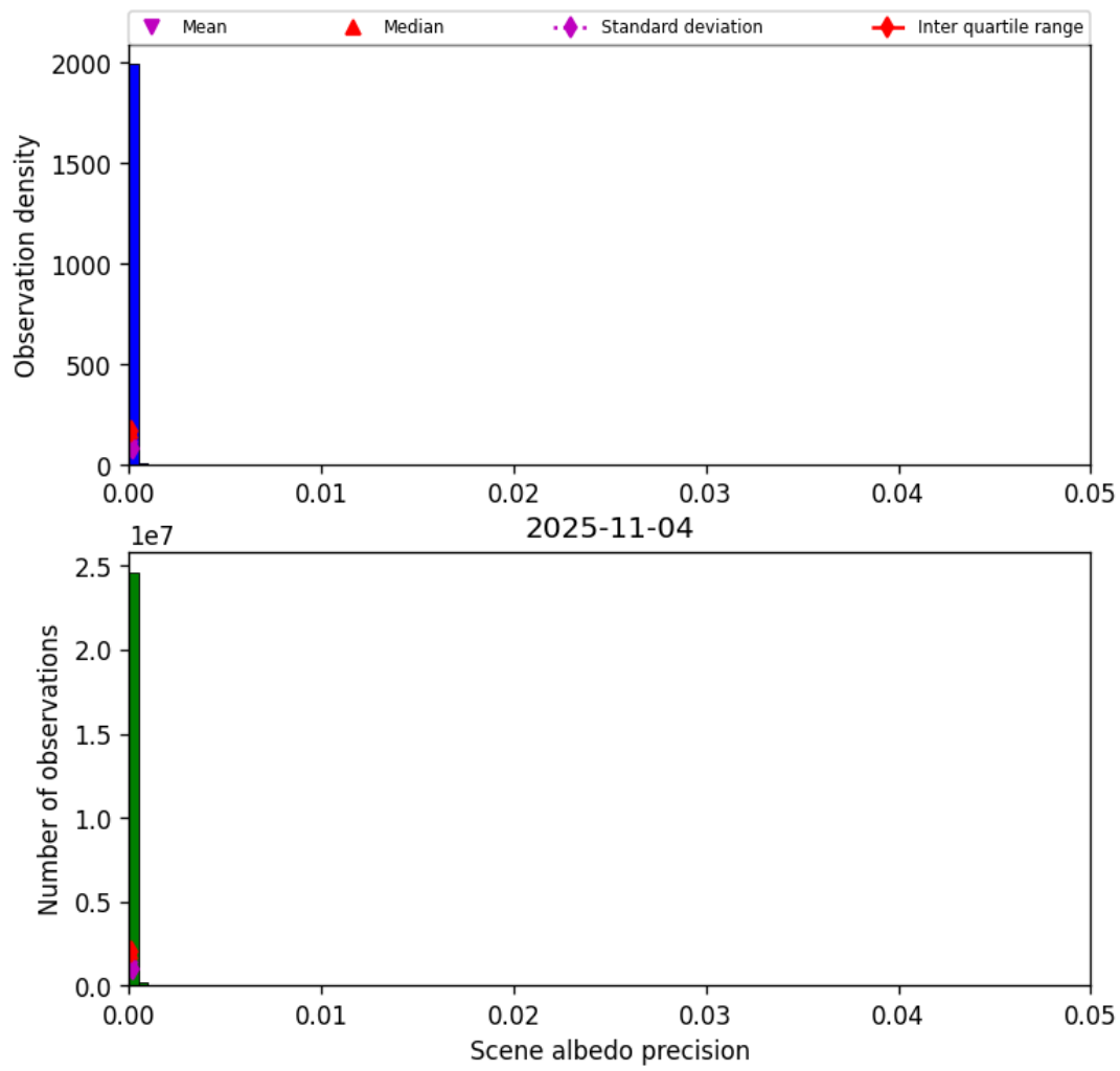
Figure 35: Histogram of “Scene albedo precision” for 2025-11-03 to 2025-11-05
