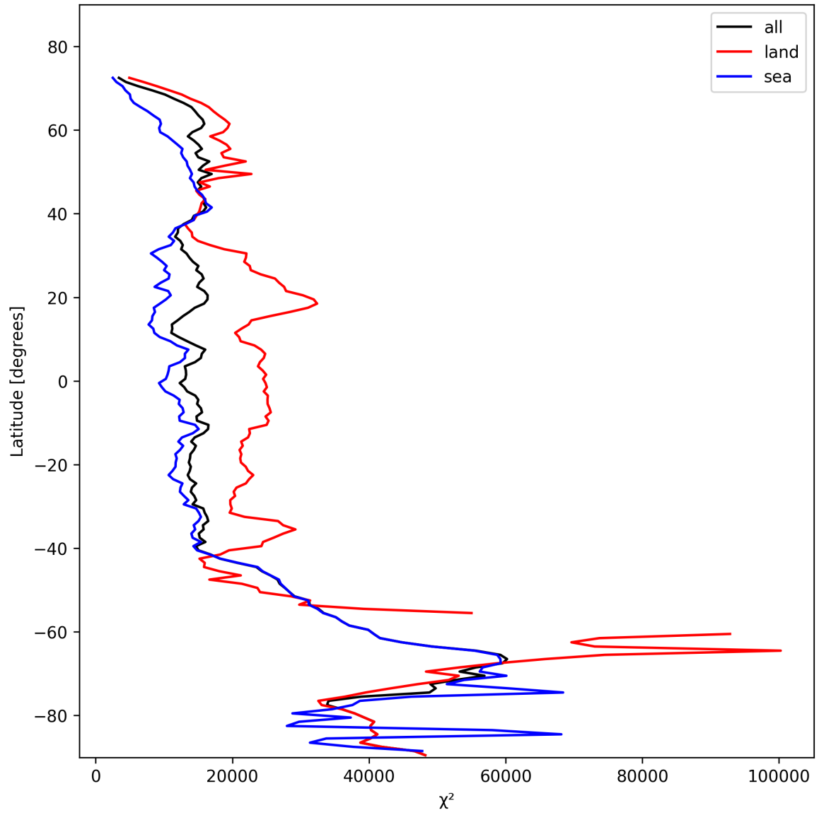
Figure 21: Zonal average of “ \chi^2 ” for 2025-11-03 to 2025-11-05.
