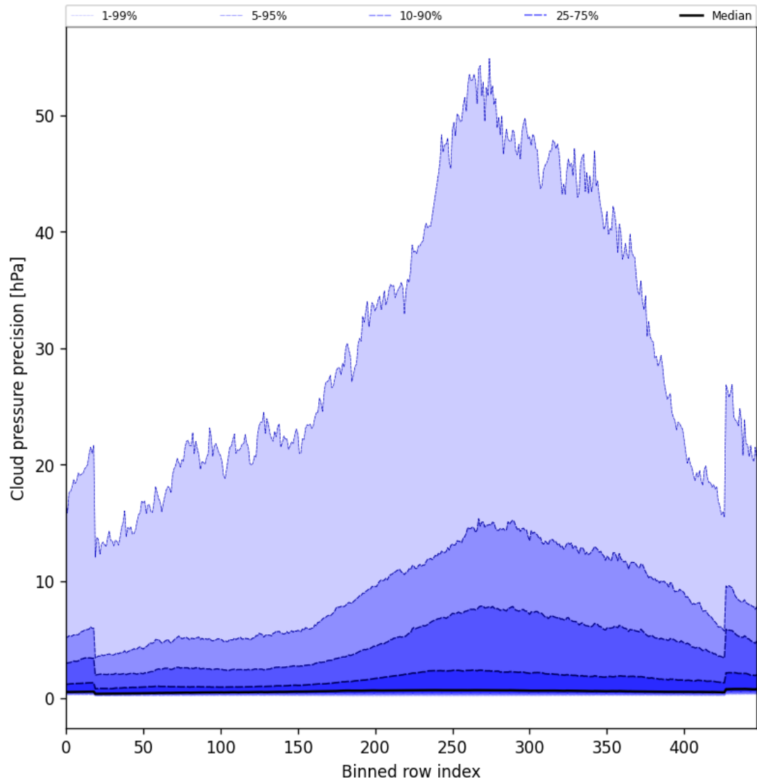
Figure 48: Along track statistics of “Cloud pressure precision” for 2025-11-03 to 2025-11-05
