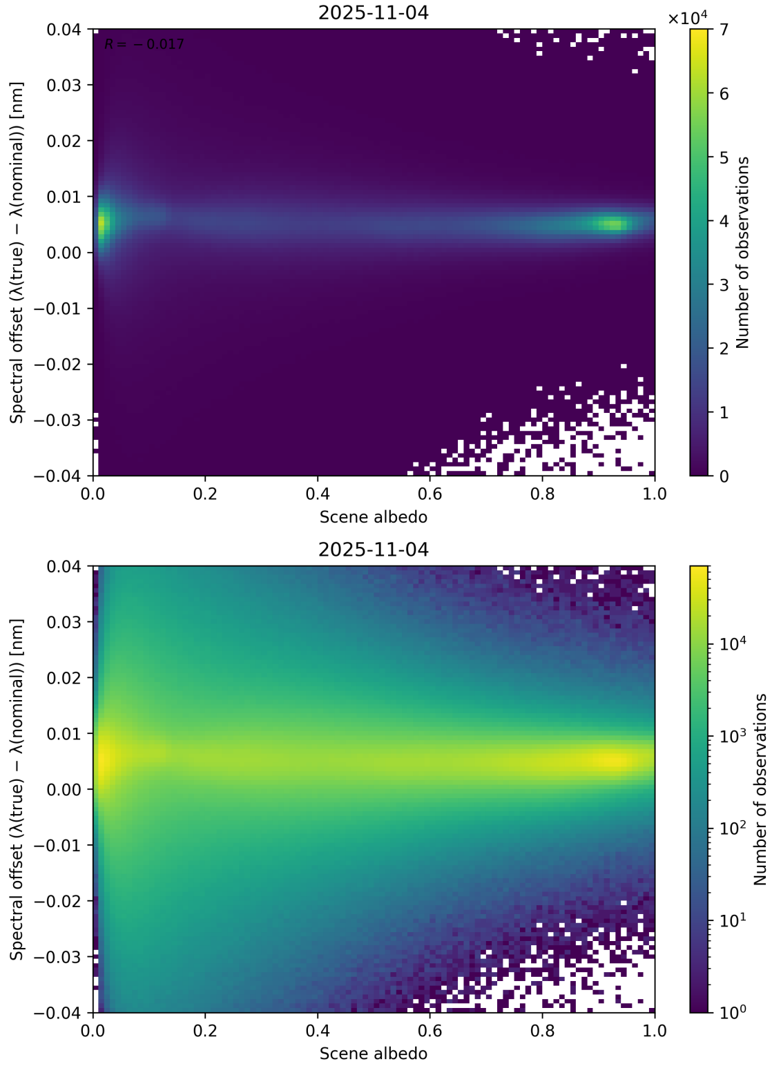
Figure 107: Scatter density plot of “Scene albedo” against “Spectral offset ( \lambda_{\text{true}} - \lambda_{\text{nominal}} )” for 2025-11-03 to 2025-11-05.
