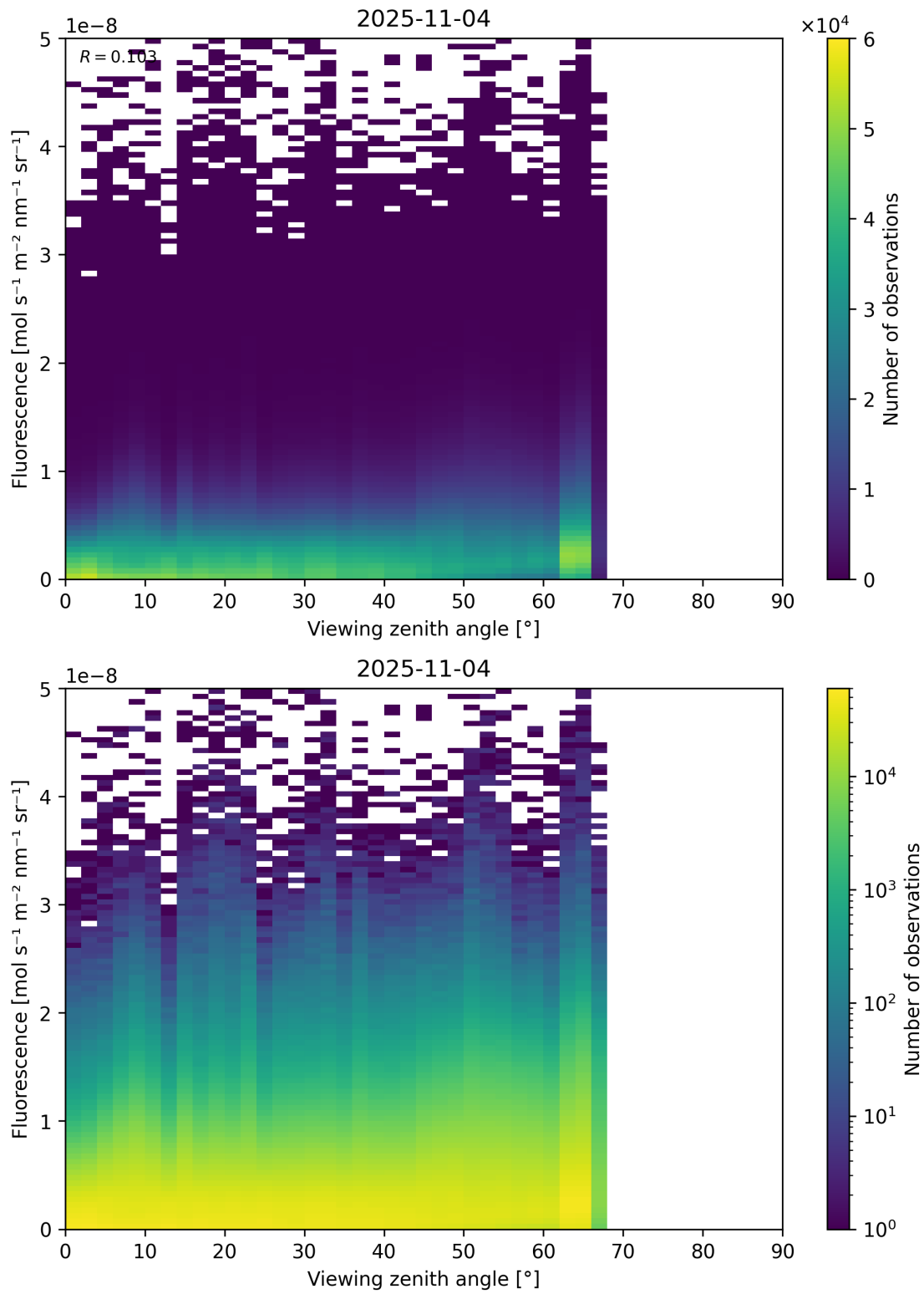
Figure 122: Scatter density plot of “Viewing zenith angle” against “Fluorescence” for 2025-11-03 to 2025-11-05.
