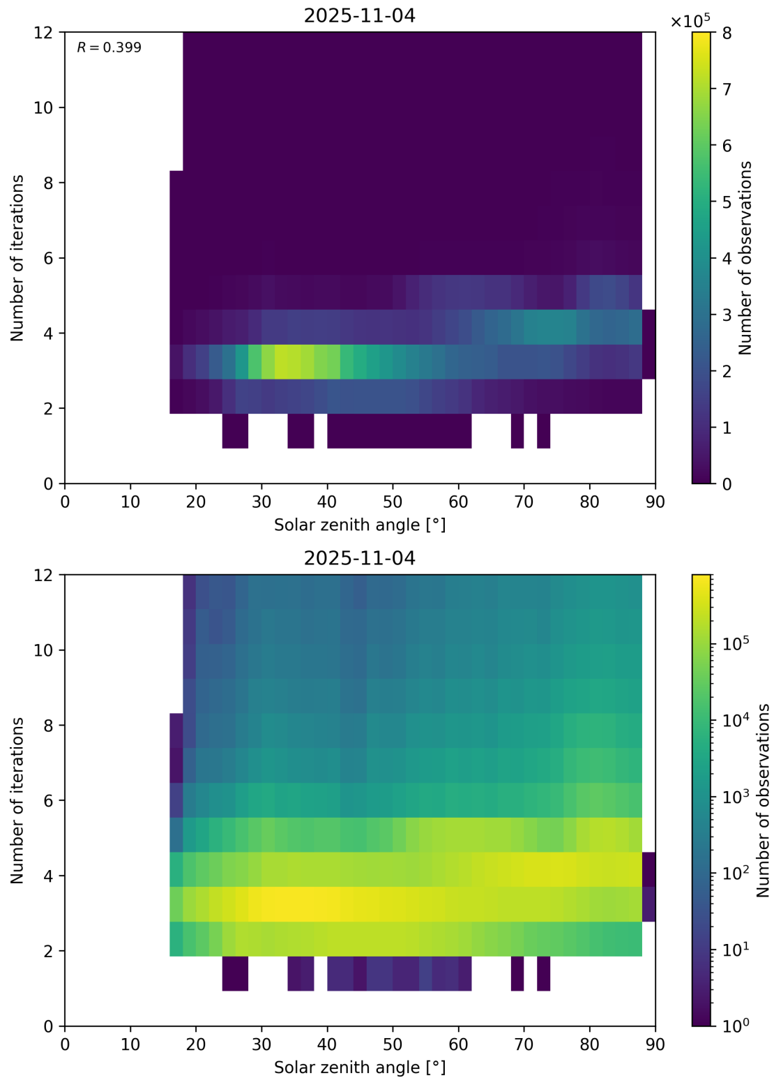
Figure 114: Scatter density plot of “Solar zenith angle” against “Number of iterations” for 2025-11-03 to 2025-11-05.
