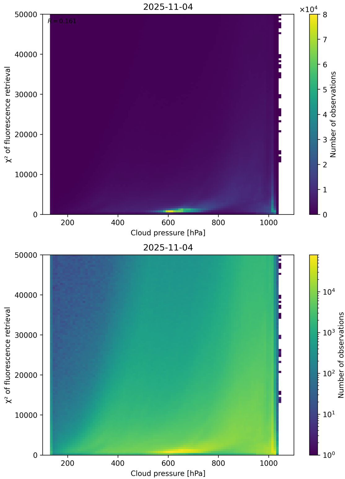
Figure 78: Scatter density plot of “Cloud pressure” against “ \chi^2 of fluorescence retrieval” for 2025-11-03 to 2025-11-05.
