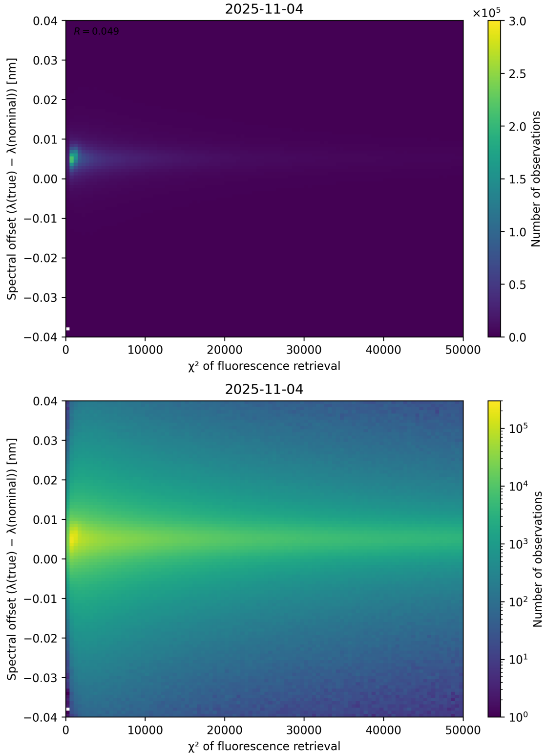
Figure 69: Scatter density plot of “ \chi^2 of fluorescence retrieval” against “Spectral offset ( \lambda_{\text{true}} - \lambda_{\text{nominal}} )” for 2025-11-03 to 2025-11-05.
