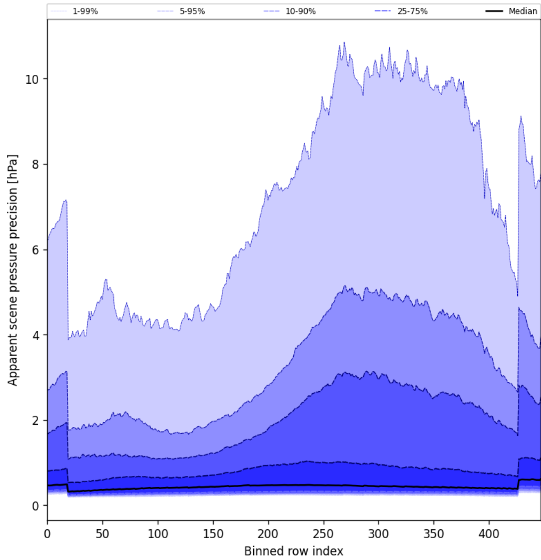
Figure 54: Along track statistics of “Apparent scene pressure precision” for 2025-11-03 to 2025-11-05
