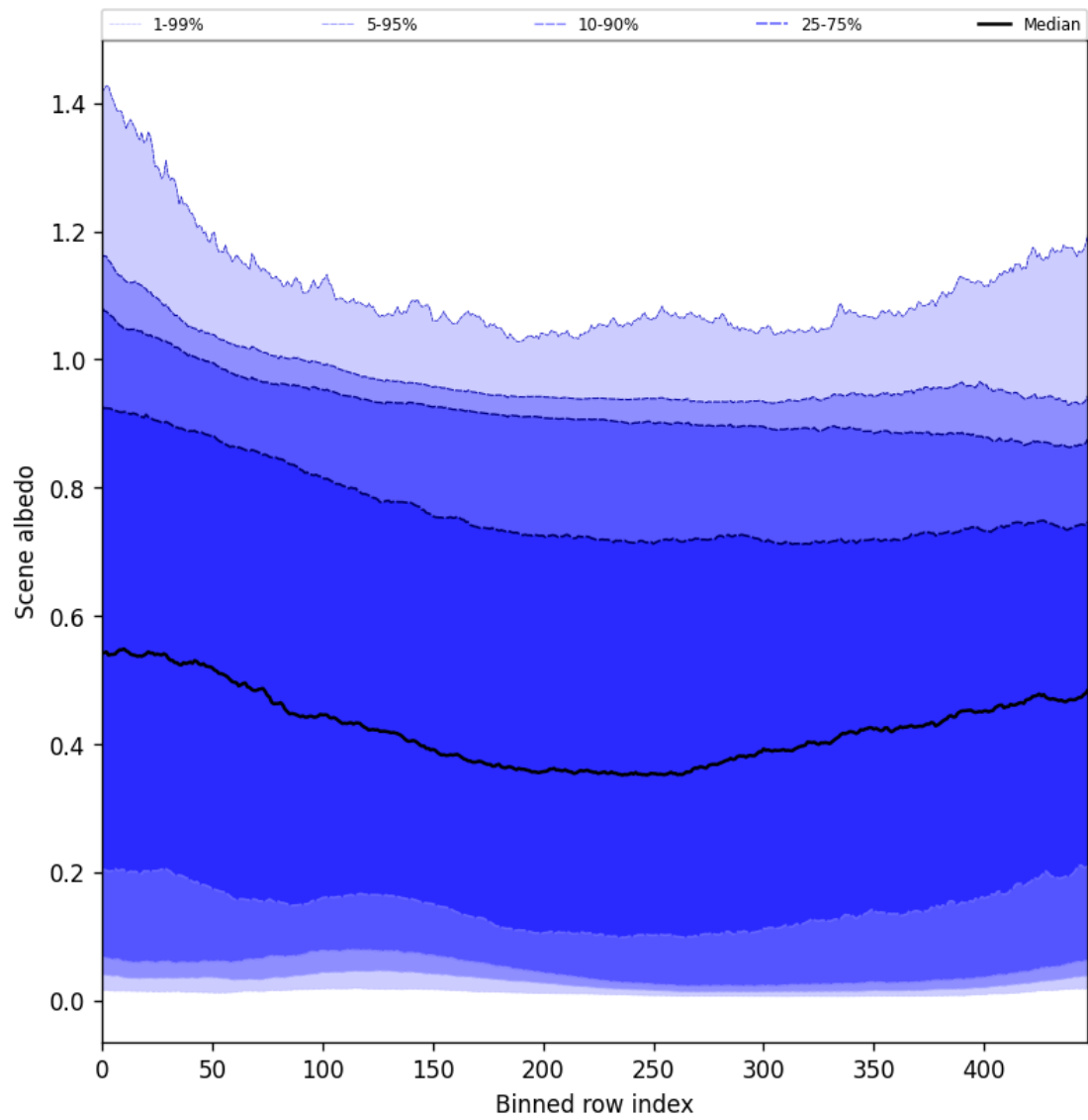
Figure 51: Along track statistics of “Scene albedo” for 2025-11-03 to 2025-11-05
