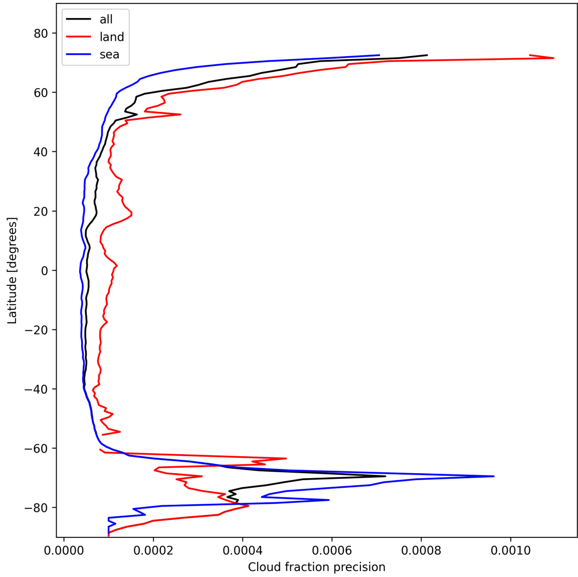
Figure 16: Zonal average of “Cloud fraction precision” for 2025-11-03 to 2025-11-05.
