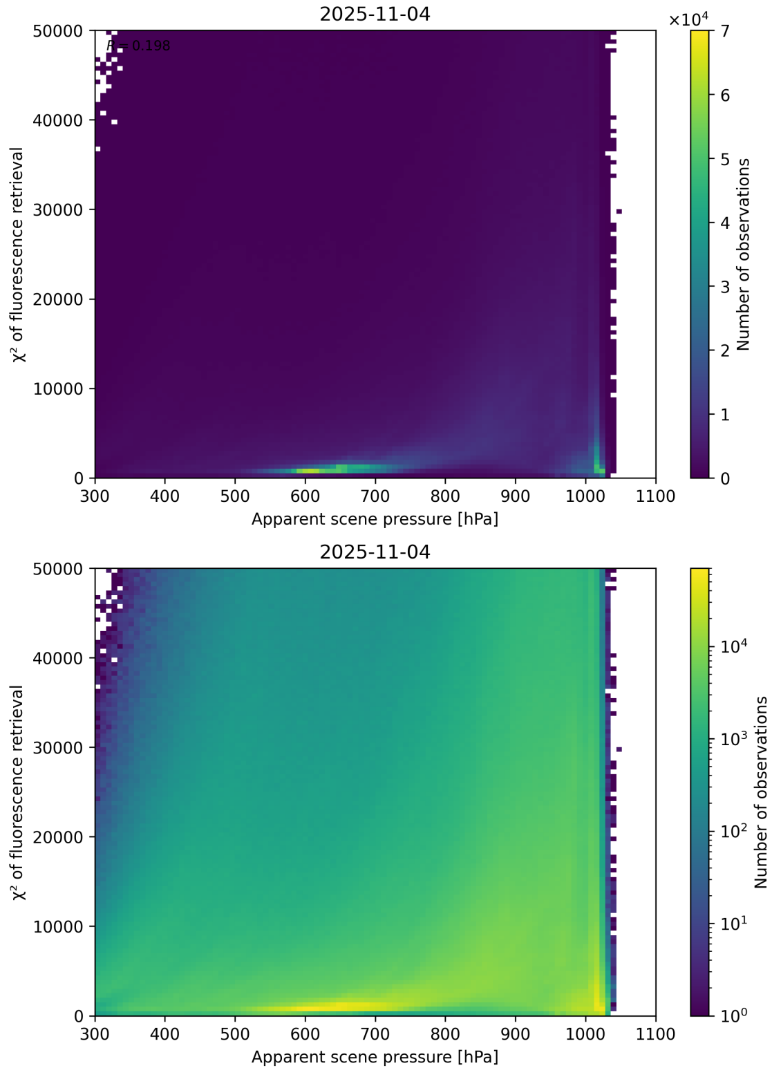
Figure 63: Scatter density plot of “Apparent scene pressure” against “ \chi^2 of fluorescence retrieval” for 2025-11-03 to 2025-11-05.
