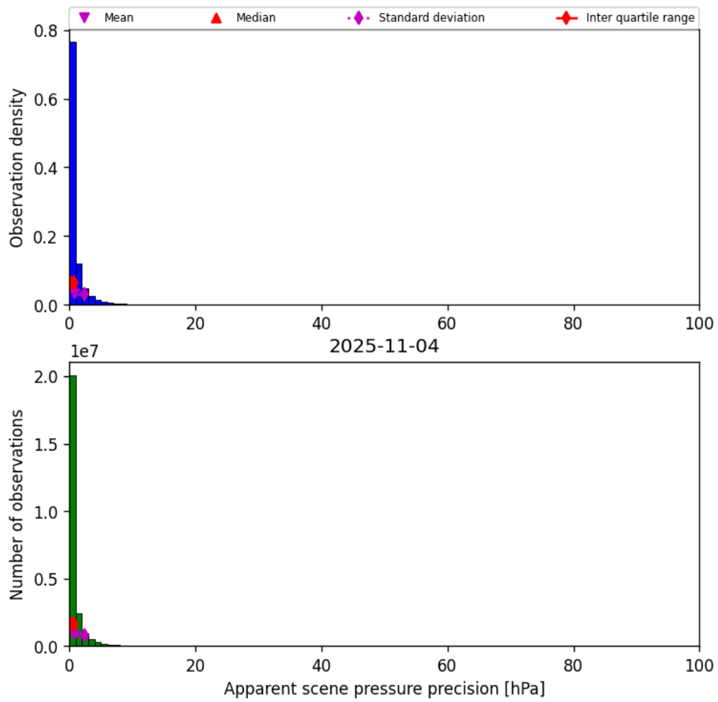
Figure 37: Histogram of “Apparent scene pressure precision” for 2025-11-03 to 2025-11-05
