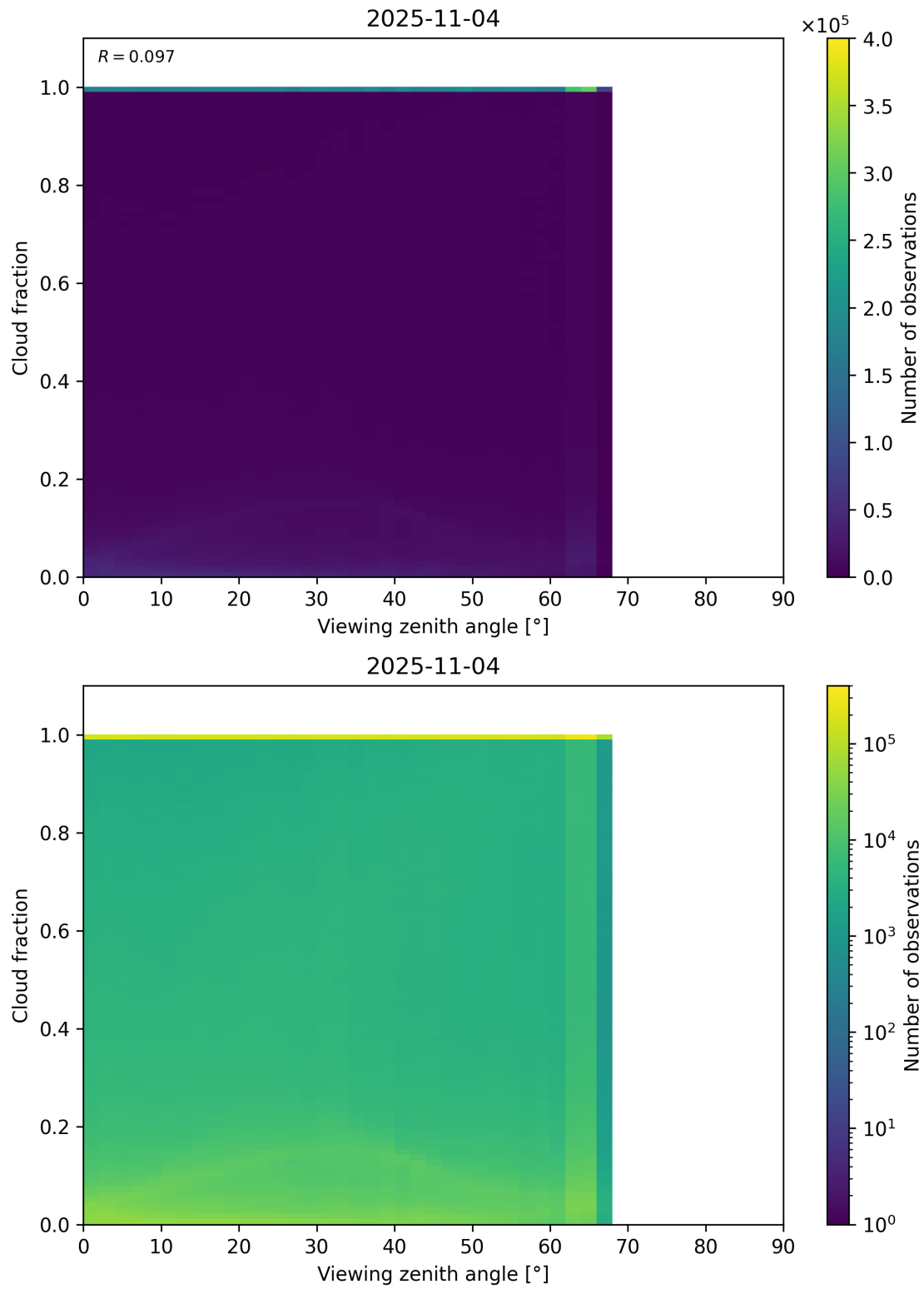
Figure 120: Scatter density plot of “Viewing zenith angle” against “Cloud fraction” for 2025-11-03 to 2025-11-05.
