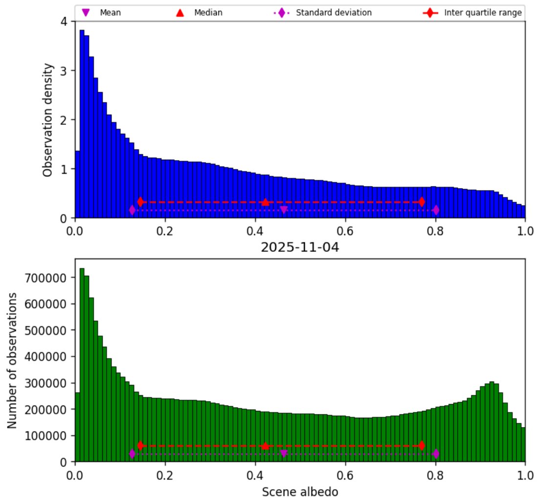
Figure 34: Histogram of “Scene albedo” for 2025-11-03 to 2025-11-05
