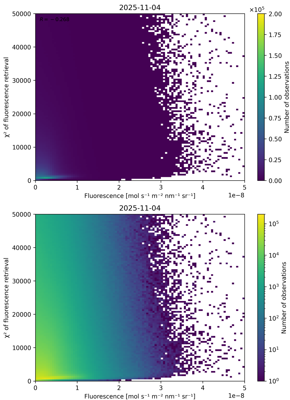
Figure 85: Scatter density plot of “Fluorescence” against “ \chi^2 of fluorescence retrieval” for 2025-11-03 to 2025-11-05.
