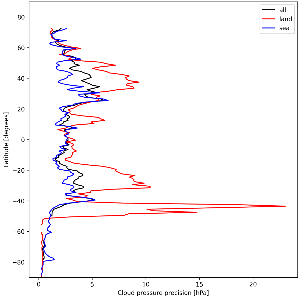
Figure 14: Zonal average of “Cloud pressure precision” for 2025-11-03 to 2025-11-05.
