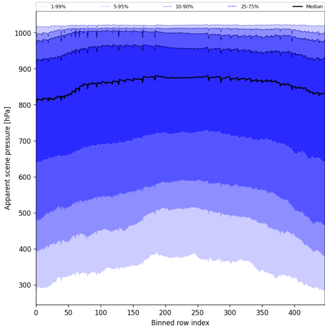
Figure 53: Along track statistics of “Apparent scene pressure” for 2025-11-03 to 2025-11-05
