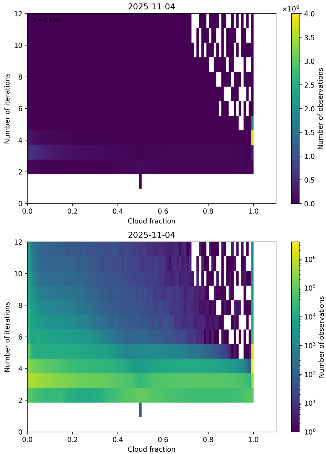
Figure 73: Scatter density plot of “Cloud fraction” against “Number of iterations” for 2025-11-03 to 2025-11-05.
