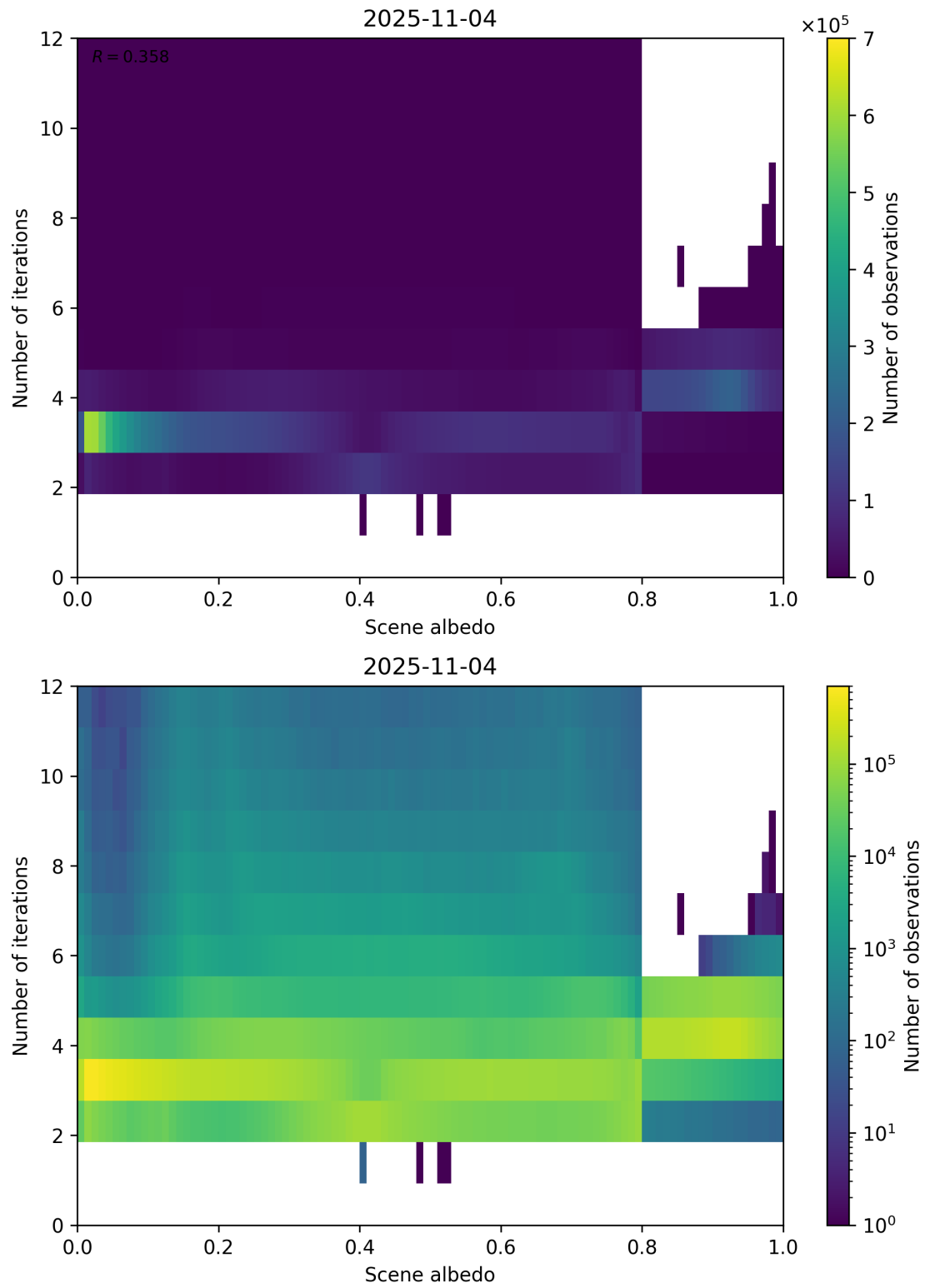
Figure 105: Scatter density plot of “Scene albedo” against “Number of iterations” for 2025-11-03 to 2025-11-05.
