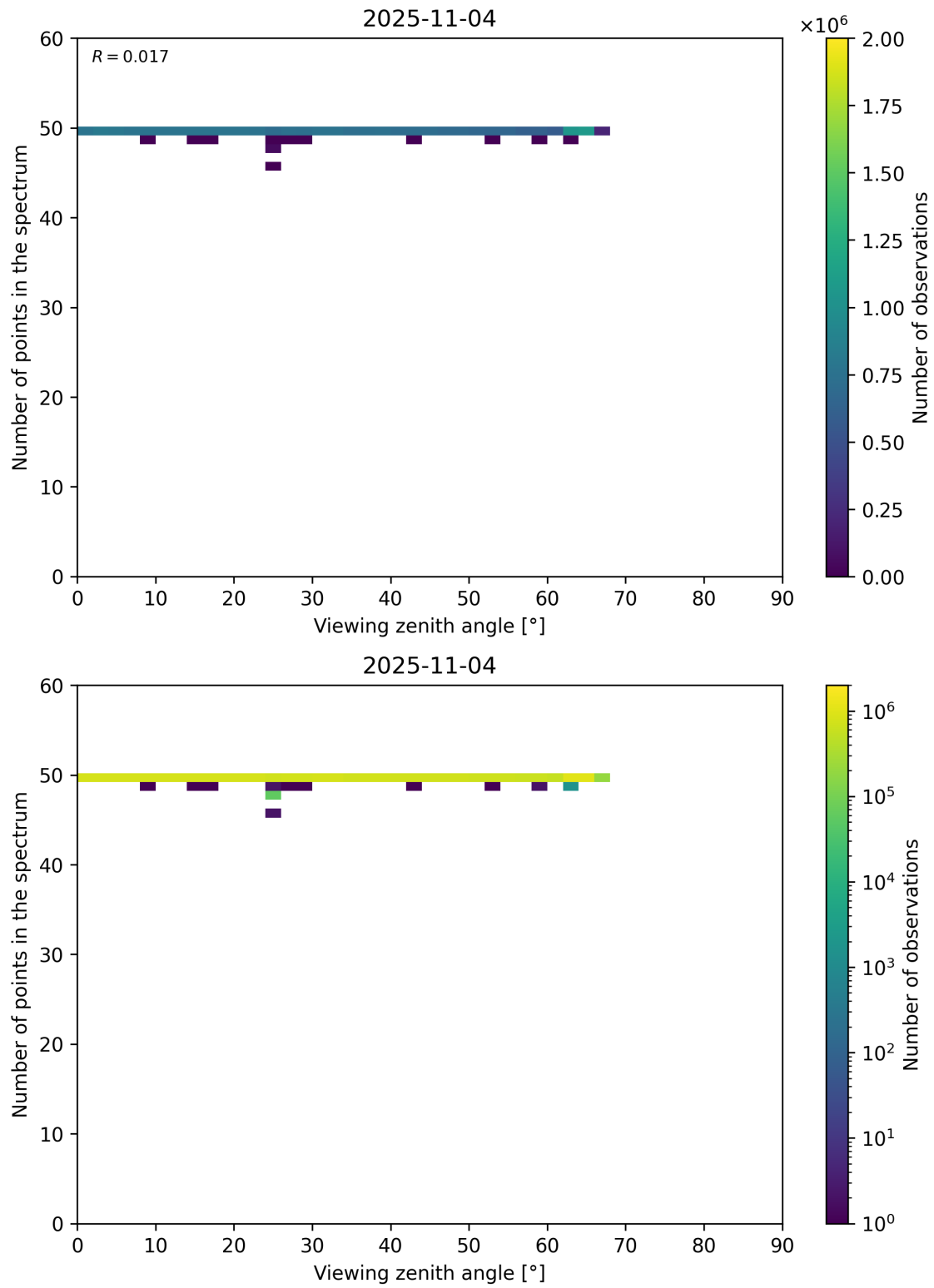
Figure 125: Scatter density plot of “Viewing zenith angle” against “Number of points in the spectrum” for 2025-11-03 to 2025-11-05.
