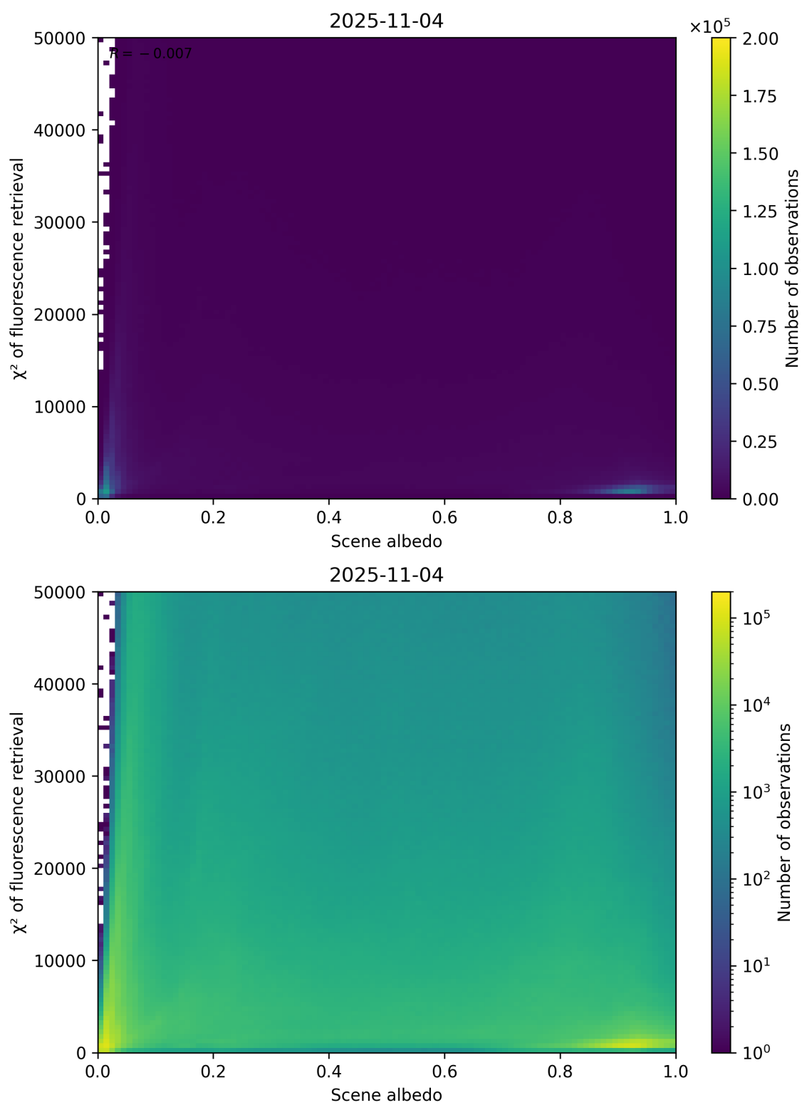
Figure 103: Scatter density plot of “Scene albedo” against “ \chi^2 of fluorescence retrieval” for 2025-11-03 to 2025-11-05.
