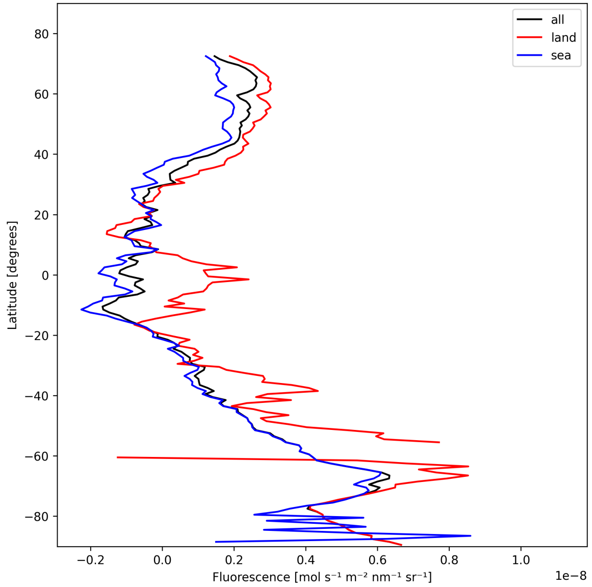
Figure 23: Zonal average of “Fluorescence” for 2025-11-03 to 2025-11-05.
