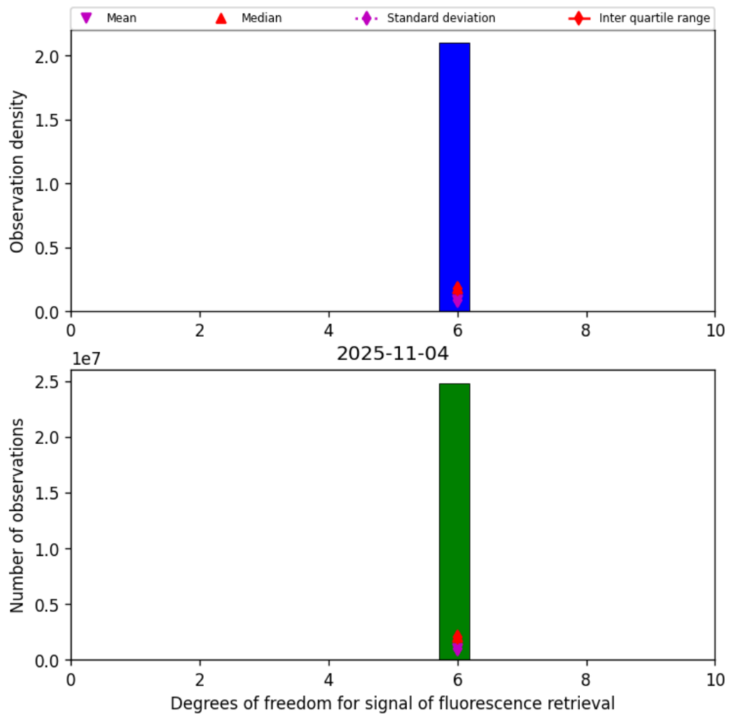
Figure 43: Histogram of "Degrees of freedom for signal of fluorescence retrieval" for 2025-11-03 to 2025-11-05
