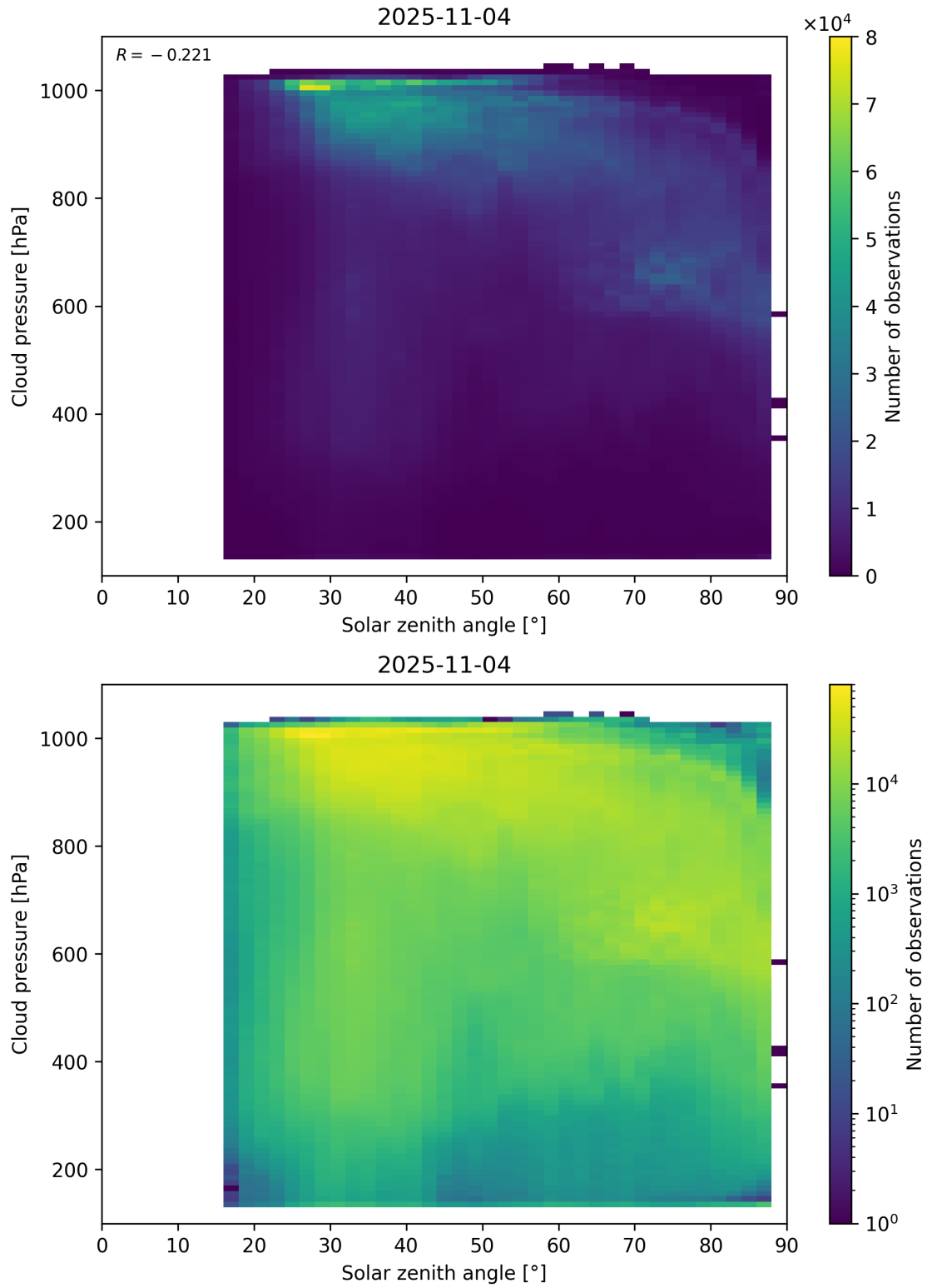
Figure 111: Scatter density plot of “Solar zenith angle” against “Cloud pressure” for 2025-11-03 to 2025-11-05.
