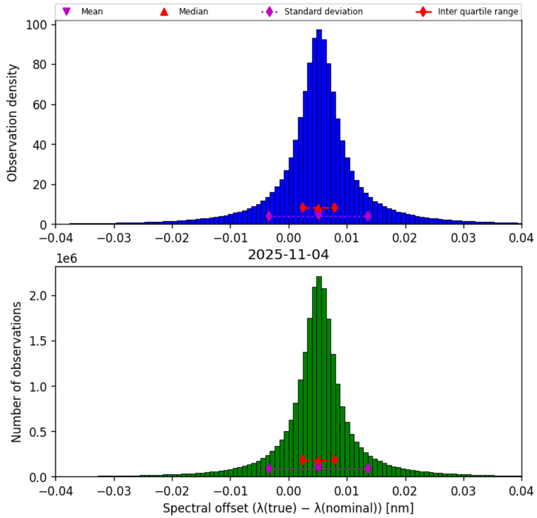
Figure 45: Histogram of “Spectral offset ( \lambda_{\text{true}} - \lambda_{\text{nominal}} )” for 2025-11-03 to 2025-11-05
