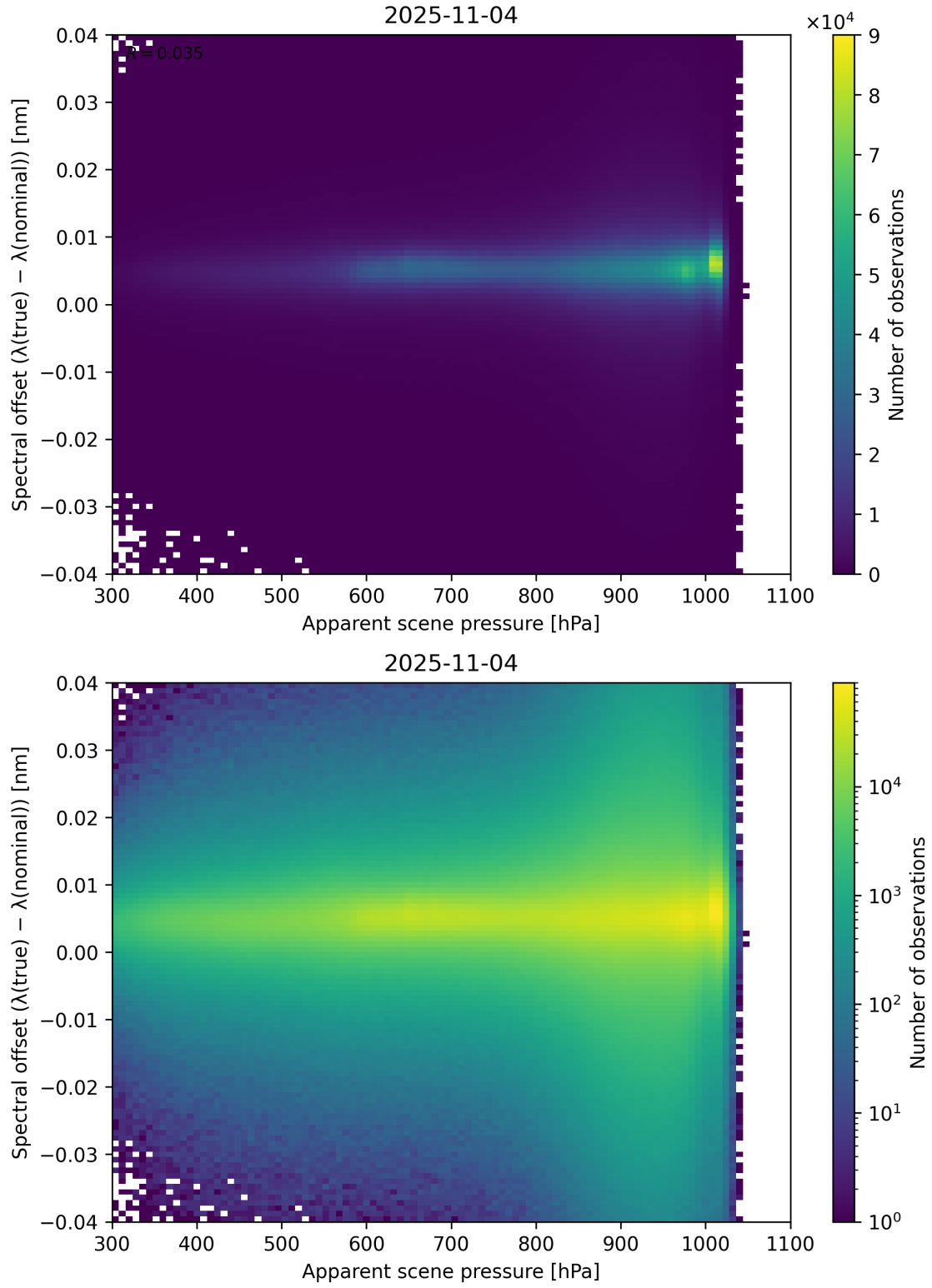
Figure 67: Scatter density plot of “Apparent scene pressure” against “Spectral offset ( \lambda_{\text{true}} - \lambda_{\text{nominal}} )” for 2025-11-03 to 2025-11-05.
