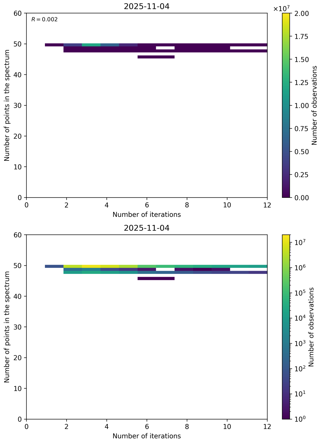
Figure 99: Scatter density plot of “Number of iterations” against “Number of points in the spectrum” for 2025-11-03 to 2025-11-05.
