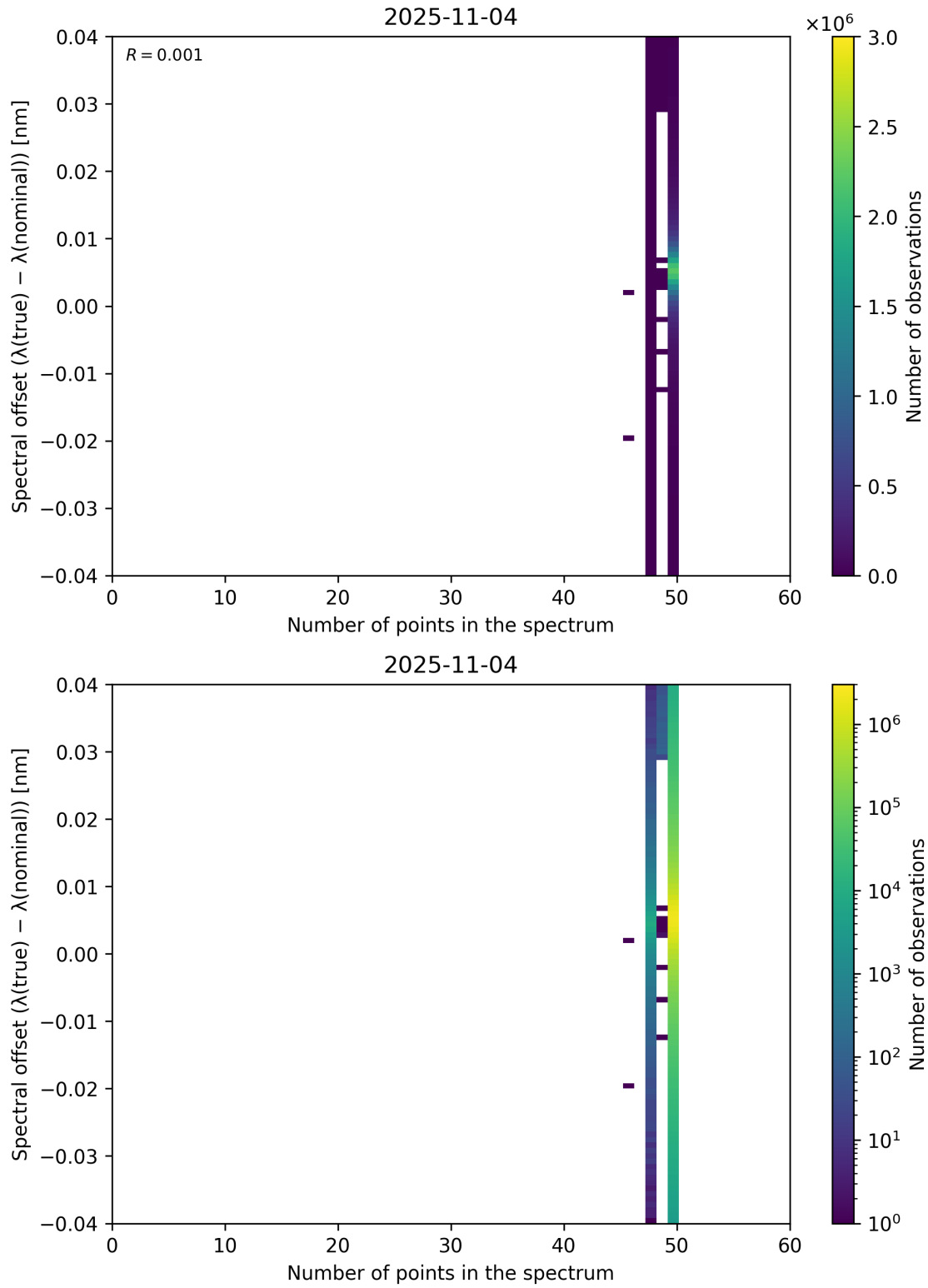
Figure 101: Scatter density plot of “Number of points in the spectrum” against “Spectral offset ( \lambda_{\text{true}} - \lambda_{\text{nominal}} )” for 2025-11-03 to 2025-11-05.
