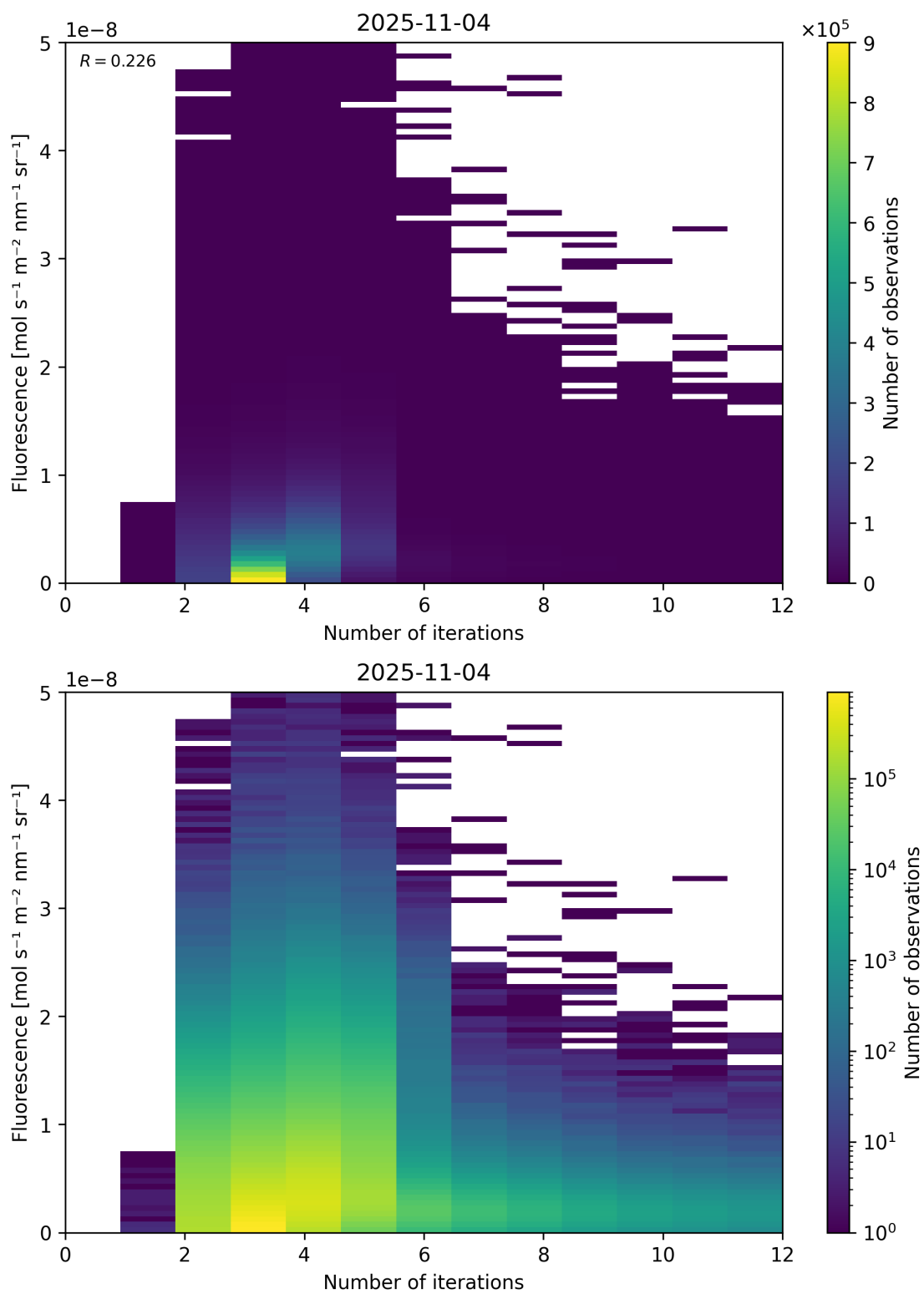
Figure 98: Scatter density plot of “Number of iterations” against “Fluorescence” for 2025-11-03 to 2025-11-05.
