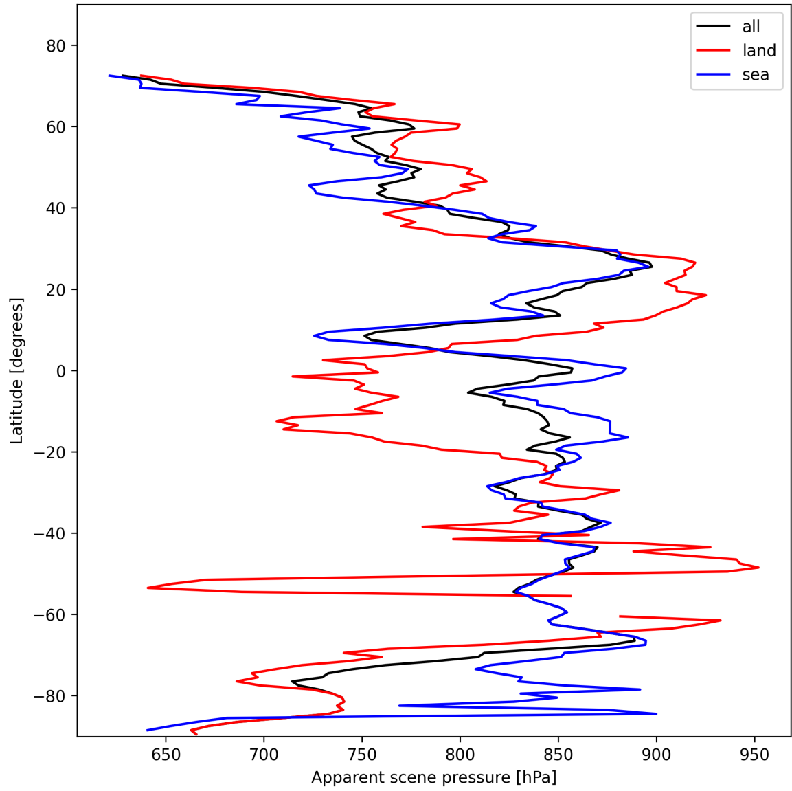
Figure 19: Zonal average of “Apparent scene pressure” for 2025-11-03 to 2025-11-05.
