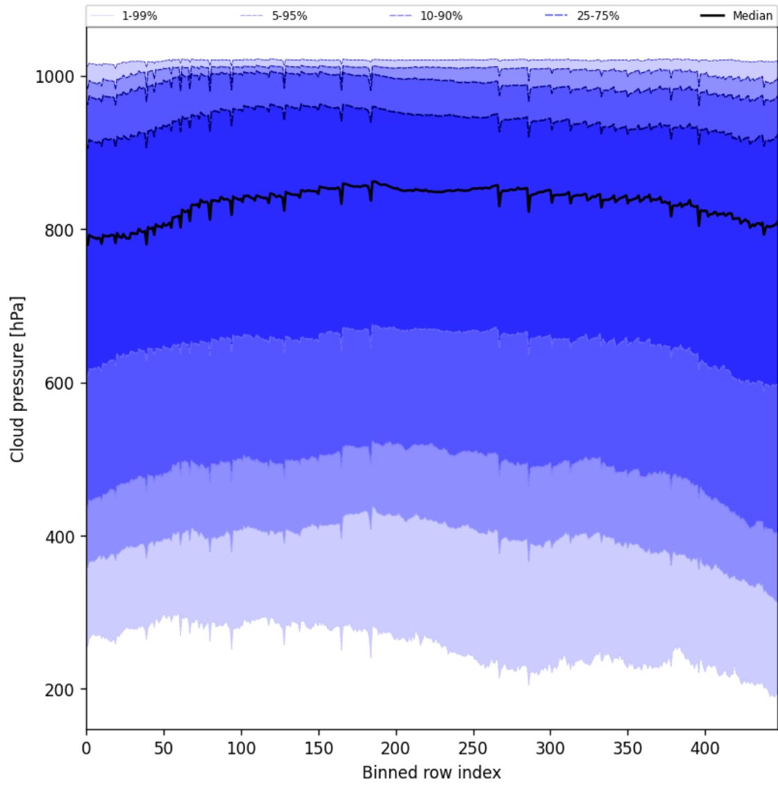
Figure 47: Along track statistics of “Cloud pressure” for 2025-11-03 to 2025-11-05
