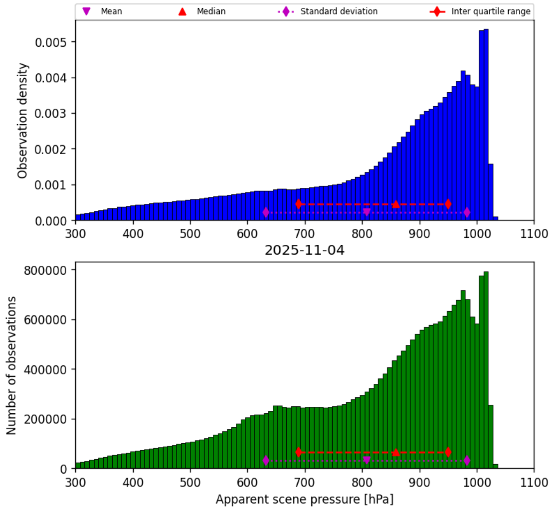
Figure 36: Histogram of “Apparent scene pressure” for 2025-11-03 to 2025-11-05
