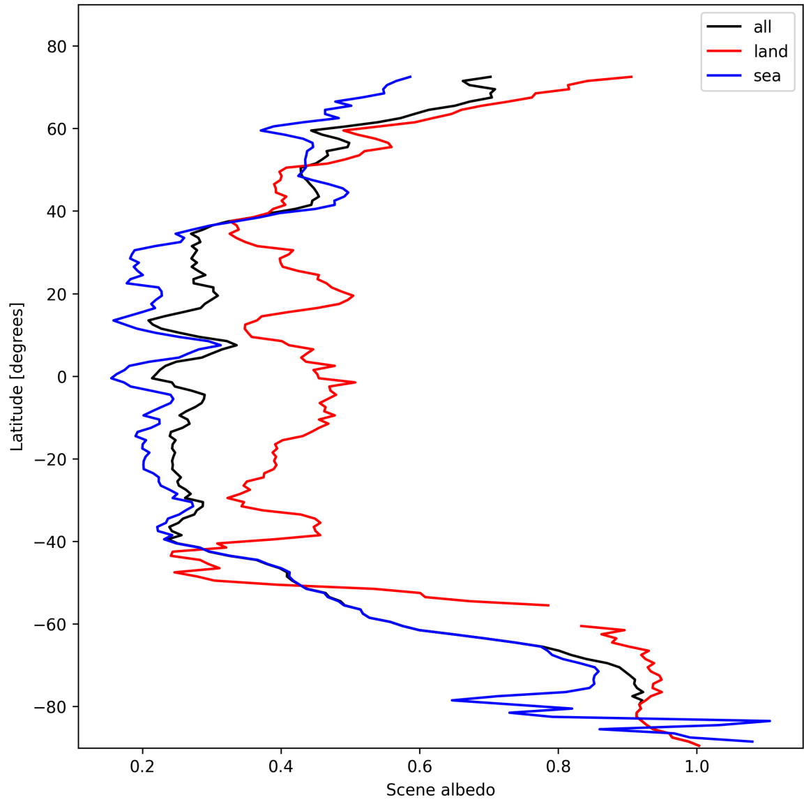
Figure 17: Zonal average of “Scene albedo” for 2025-11-03 to 2025-11-05.
