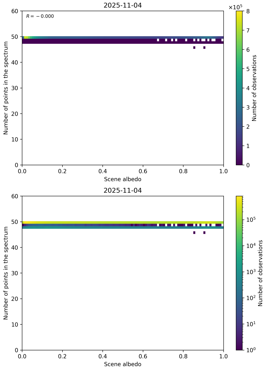
Figure 106: Scatter density plot of “Scene albedo” against “Number of points in the spectrum” for 2025-11-03 to 2025-11-05.
