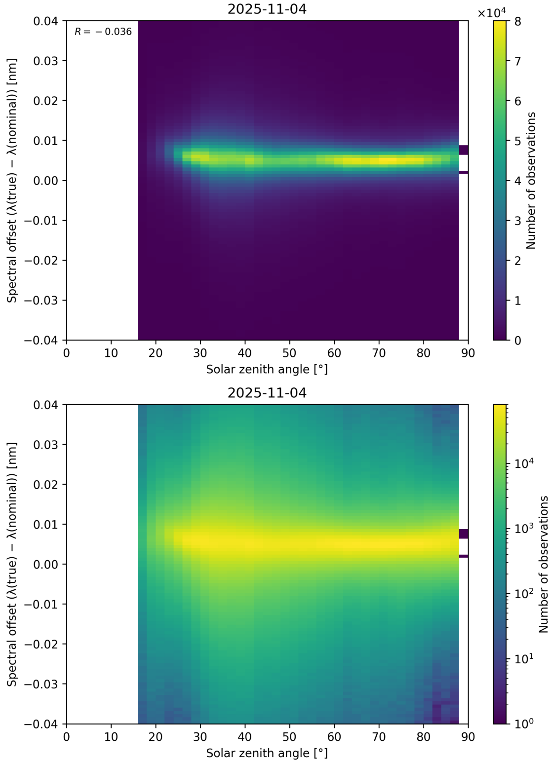
Figure 117: Scatter density plot of “Solar zenith angle” against “Spectral offset ( \lambda_{\text{true}} - \lambda_{\text{nominal}} )” for 2025-11-03 to 2025-11-05.
