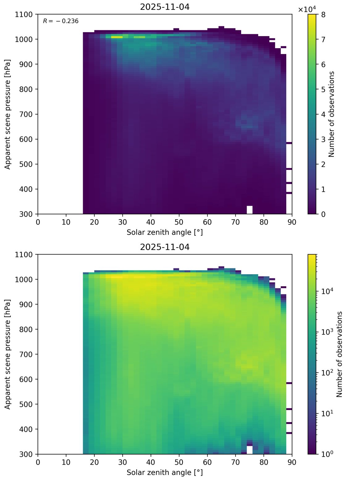
Figure 108: Scatter density plot of “Solar zenith angle” against “Apparent scene pressure” for 2025-11-03 to 2025-11-05.
