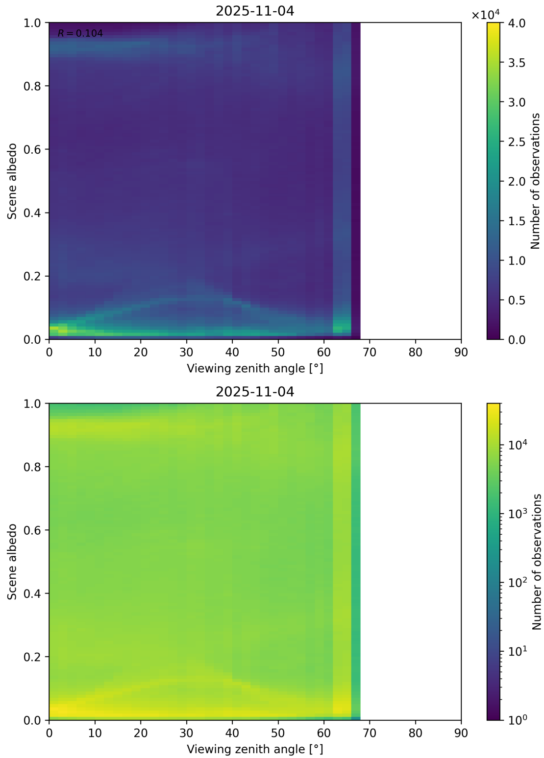
Figure 126: Scatter density plot of “Viewing zenith angle” against “Scene albedo” for 2025-11-03 to 2025-11-05.
