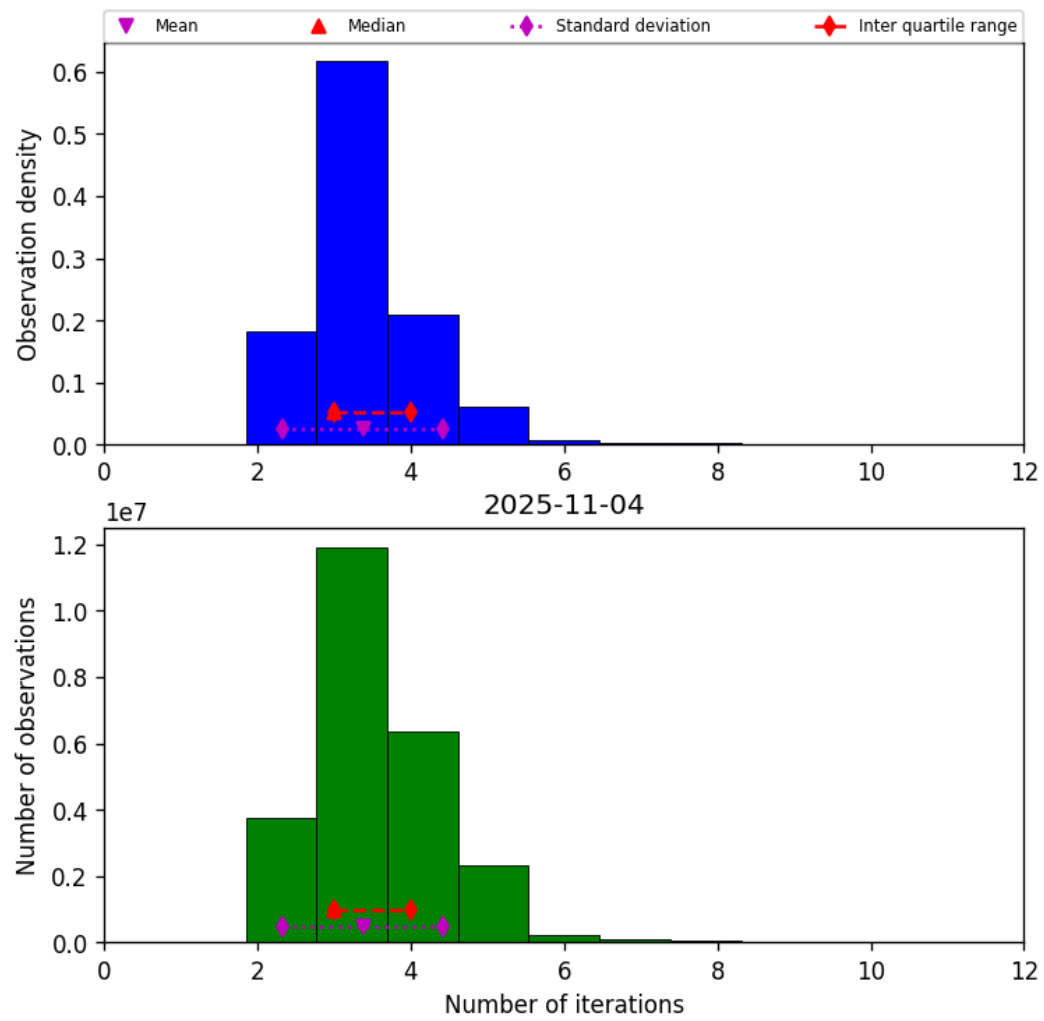
Figure 39: Histogram of “Number of iterations” for 2025-11-03 to 2025-11-05
