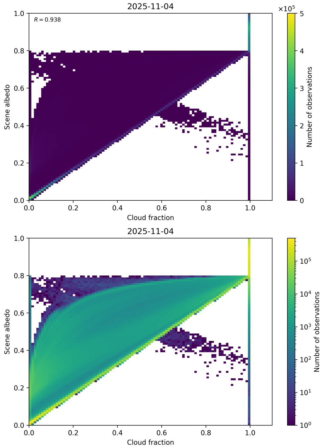
Figure 75: Scatter density plot of “Cloud fraction” against “Scene albedo” for 2025-11-03 to 2025-11-05.
