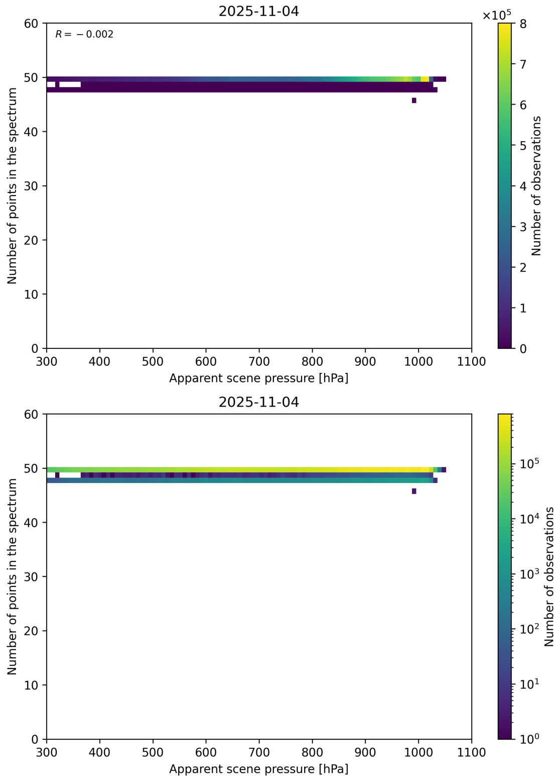
Figure 66: Scatter density plot of “Apparent scene pressure” against “Number of points in the spectrum” for 2025-11-03 to 2025-11-05.
