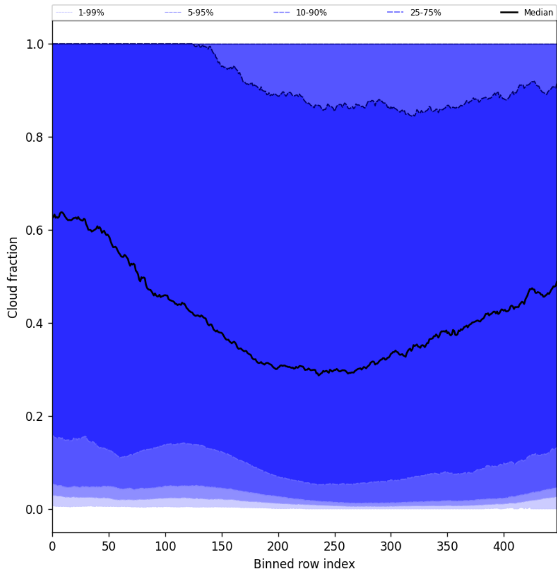
Figure 49: Along track statistics of “Cloud fraction” for 2025-11-03 to 2025-11-05
