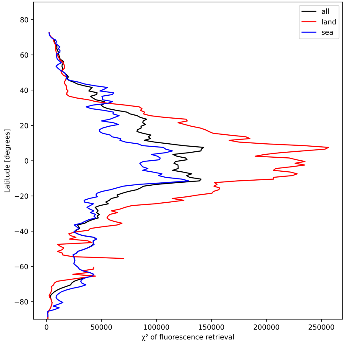
Figure 25: Zonal average of “ \chi^2 of fluorescence retrieval” for 2025-11-03 to 2025-11-05.
