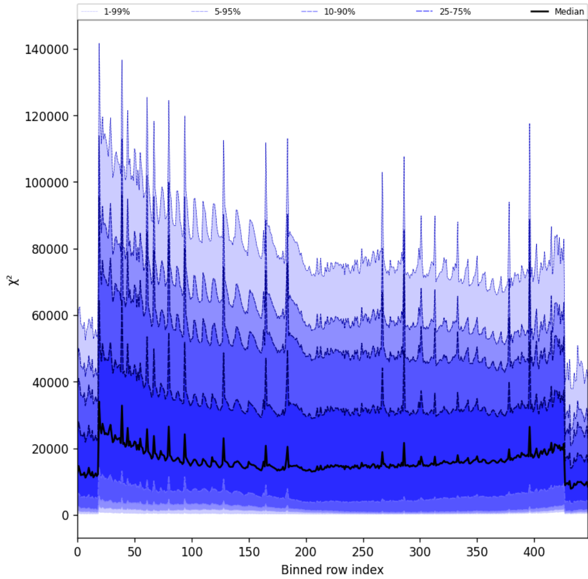
Figure 55: Along track statistics of “ \chi^2 ” for 2025-11-03 to 2025-11-05
