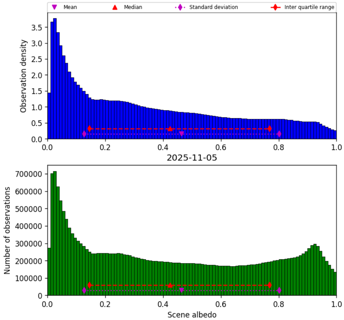
Figure 34: Histogram of “Scene albedo” for 2025-11-04 to 2025-11-06
