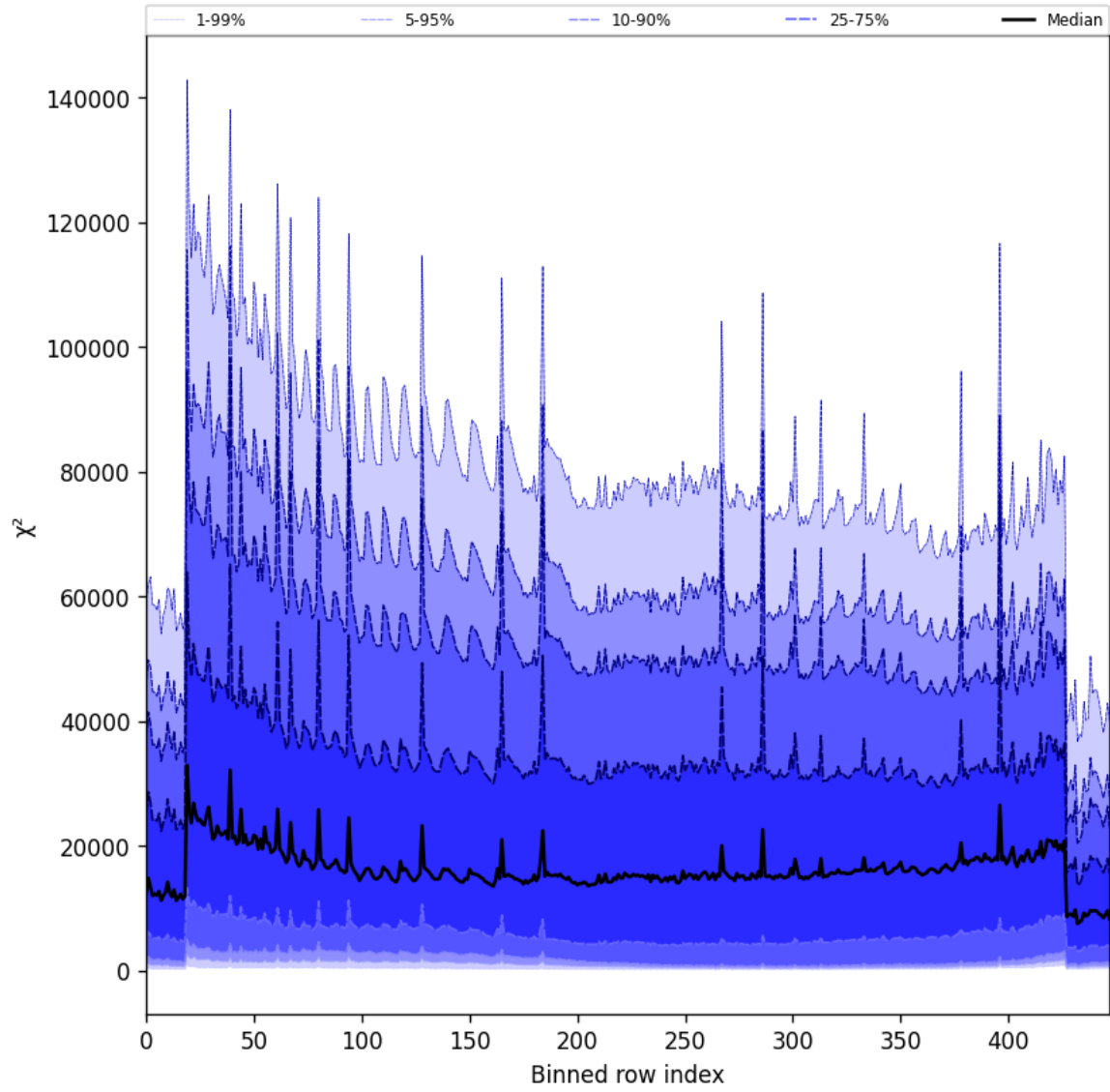
Figure 55: Along track statistics of “ \chi^2 ” for 2025-11-04 to 2025-11-06
