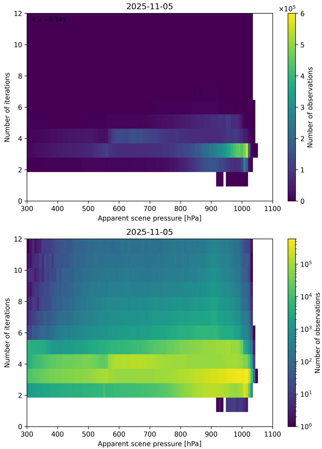
Figure 65: Scatter density plot of “Apparent scene pressure” against “Number of iterations” for 2025-11-04 to 2025-11-06.
