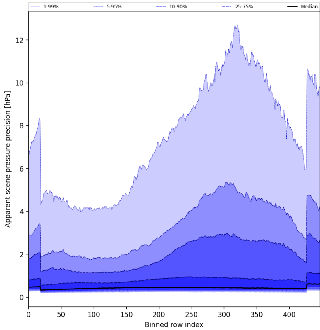
Figure 54: Along track statistics of “Apparent scene pressure precision” for 2025-11-04 to 2025-11-06
