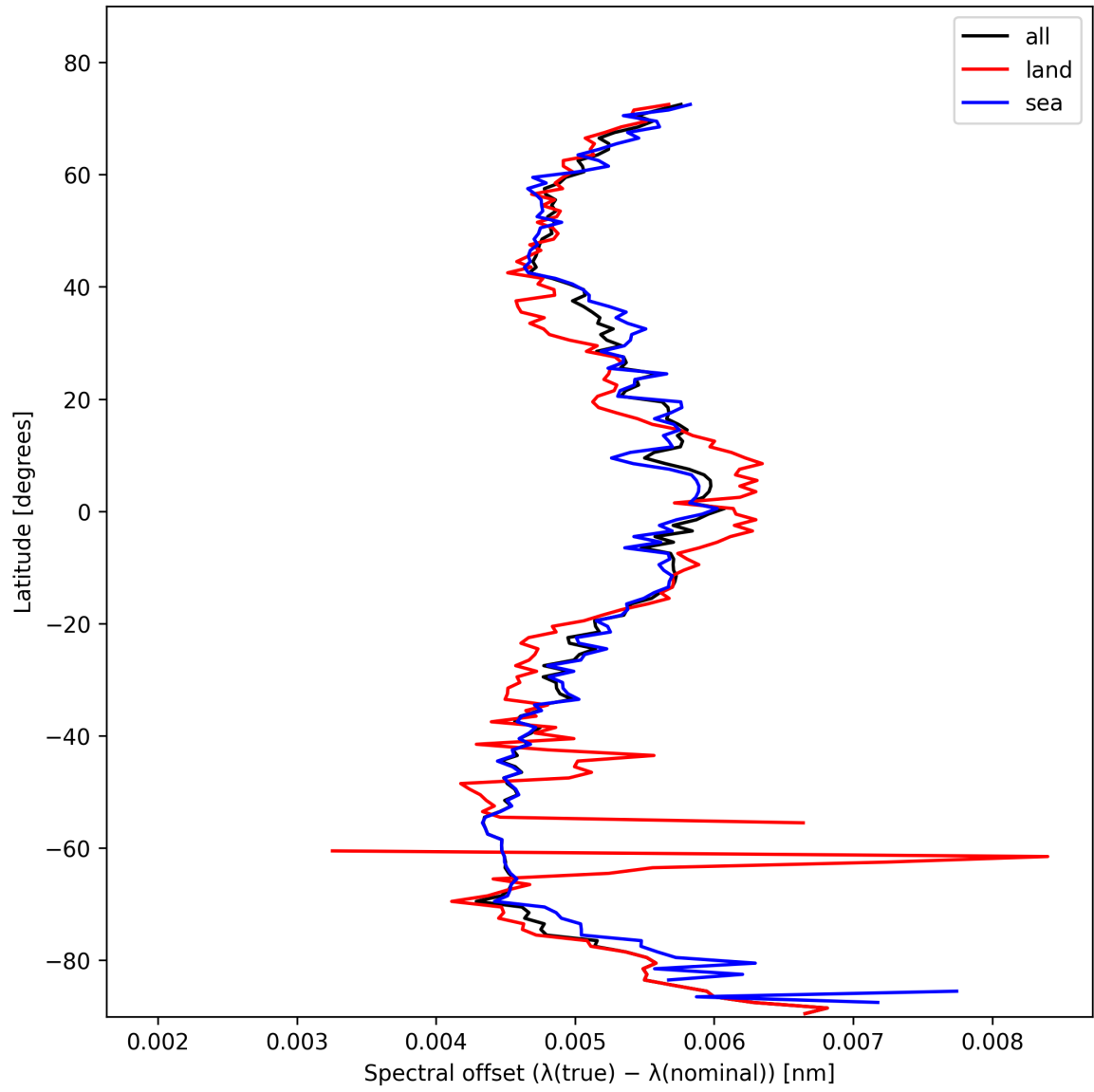
Figure 28: Zonal average of “Spectral offset ( \lambda_{\text{true}} - \lambda_{\text{nominal}} )” for 2025-11-04 to 2025-11-06.
