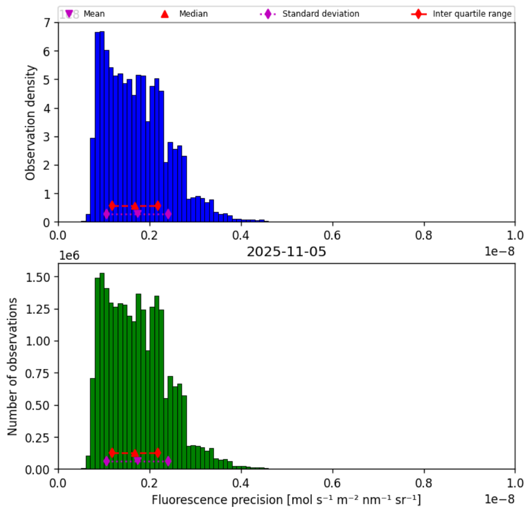
Figure 41: Histogram of “Fluorescence precision” for 2025-11-04 to 2025-11-06
