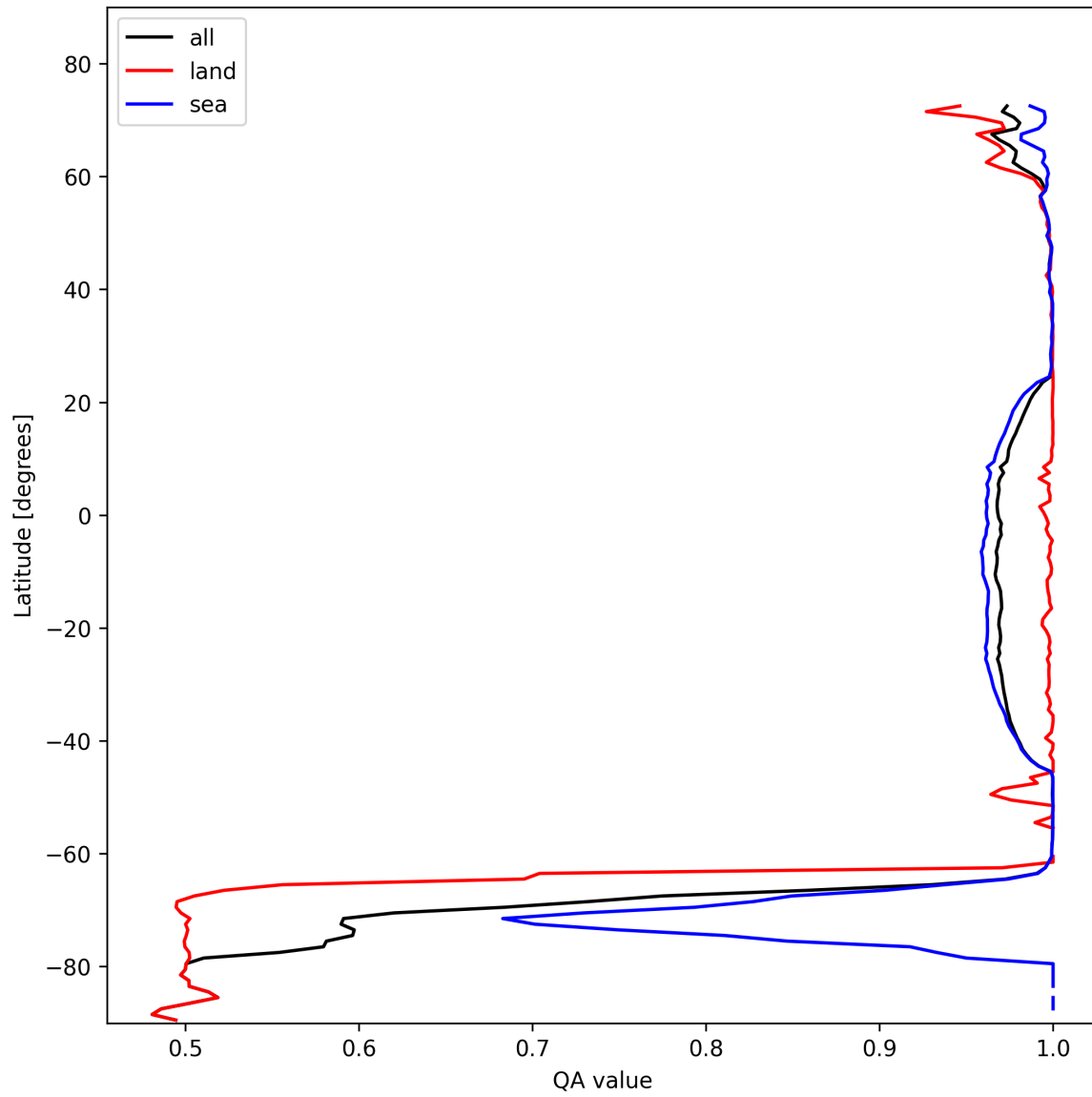
Figure 12: Zonal average of “QA value” for 2025-11-04 to 2025-11-06.
