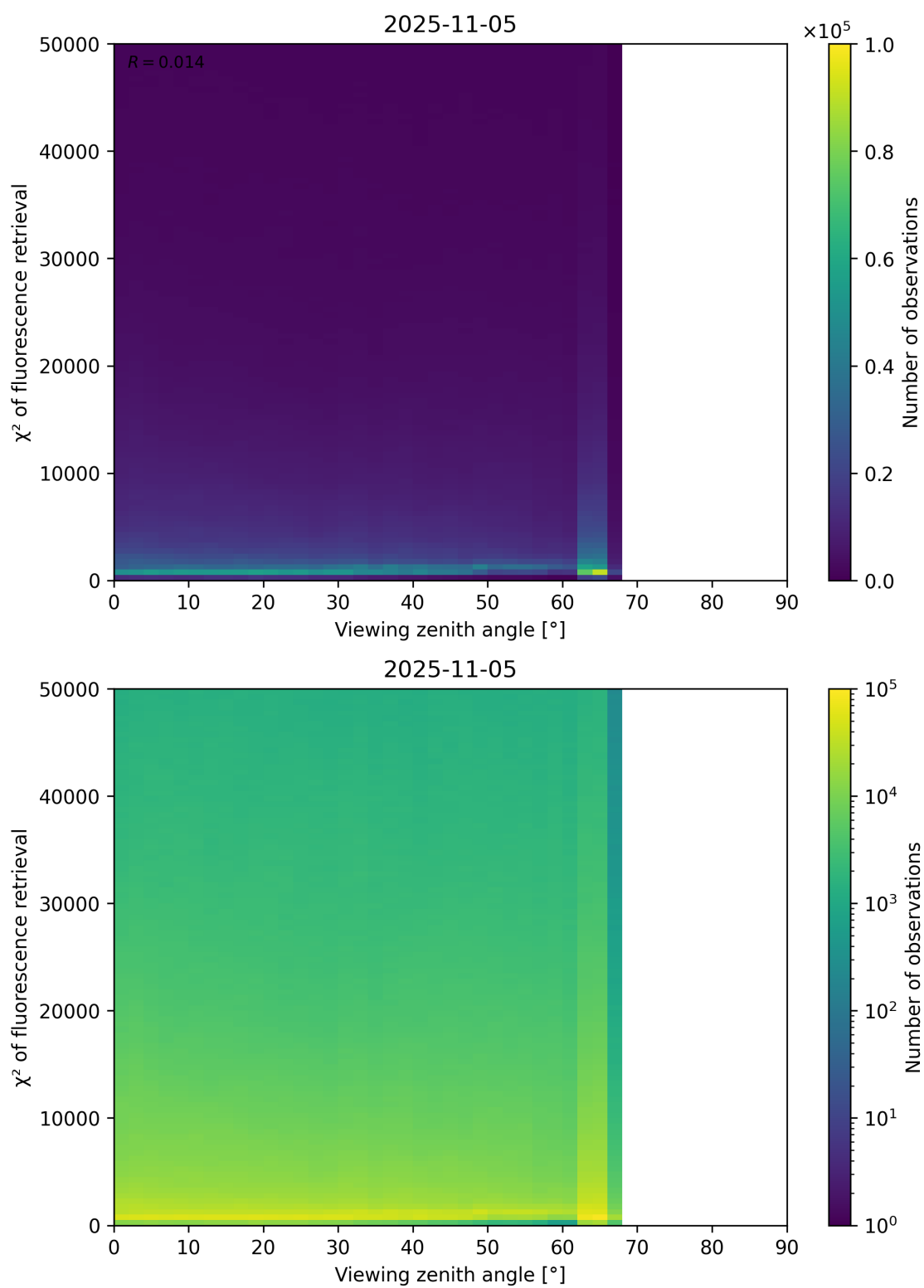
Figure 119: Scatter density plot of “Viewing zenith angle” against “ \chi^2 of fluorescence retrieval” for 2025-11-04 to 2025-11-06.
