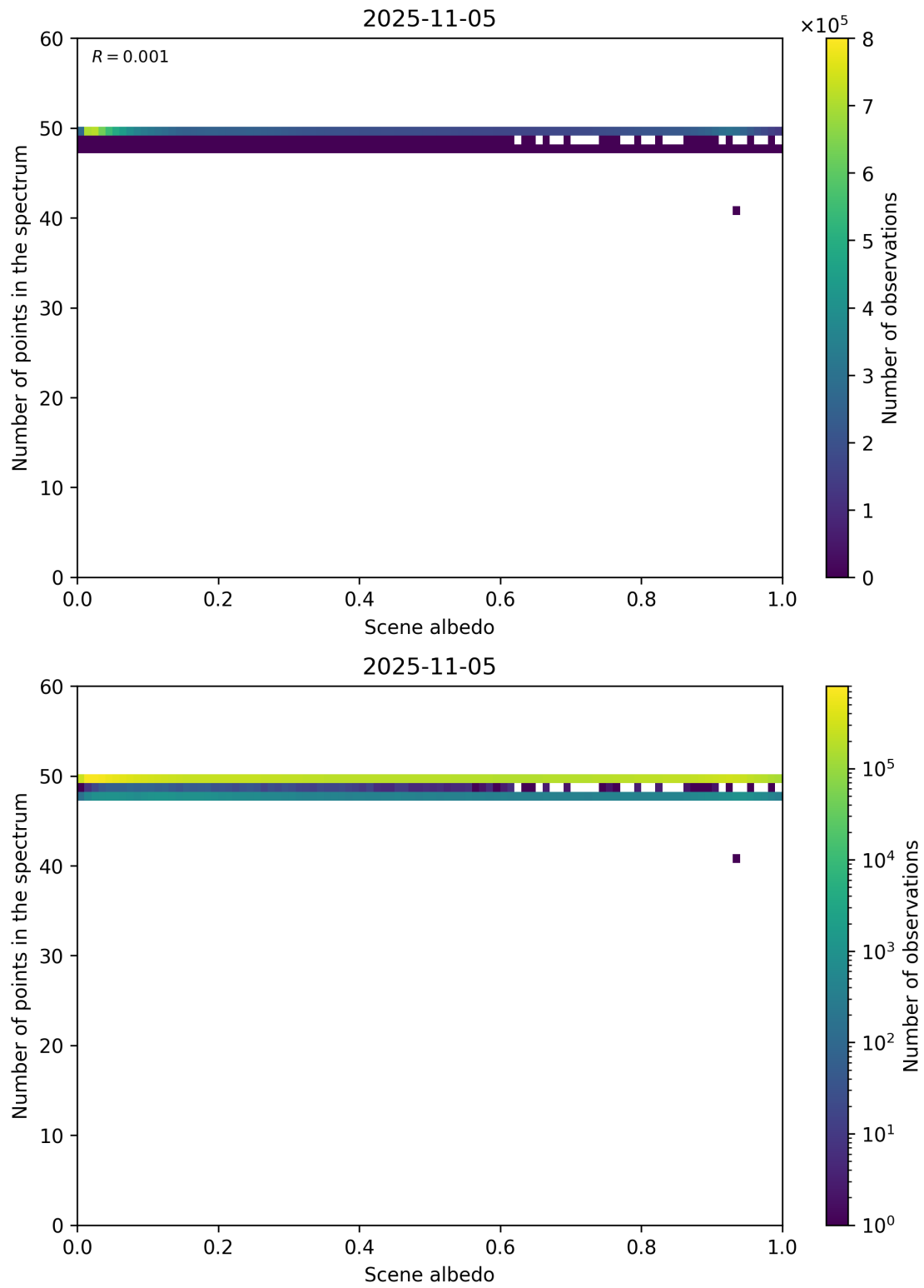
Figure 106: Scatter density plot of “Scene albedo” against “Number of points in the spectrum” for 2025-11-04 to 2025-11-06.
