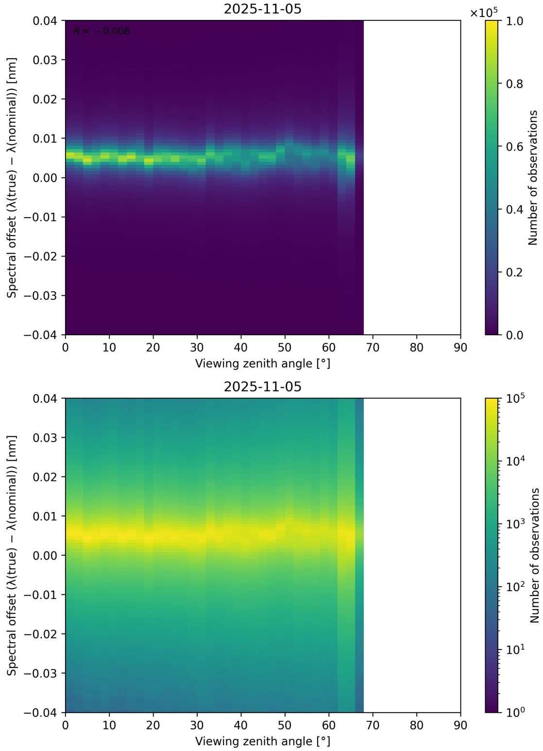
Figure 128: Scatter density plot of “Viewing zenith angle” against “Spectral offset ( \lambda_{\text{true}} - \lambda_{\text{nominal}} )” for 2025-11-04 to 2025-11-06.
