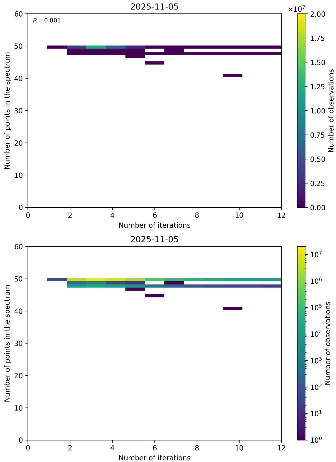
Figure 99: Scatter density plot of “Number of iterations” against “Number of points in the spectrum” for 2025-11-04 to 2025-11-06.
