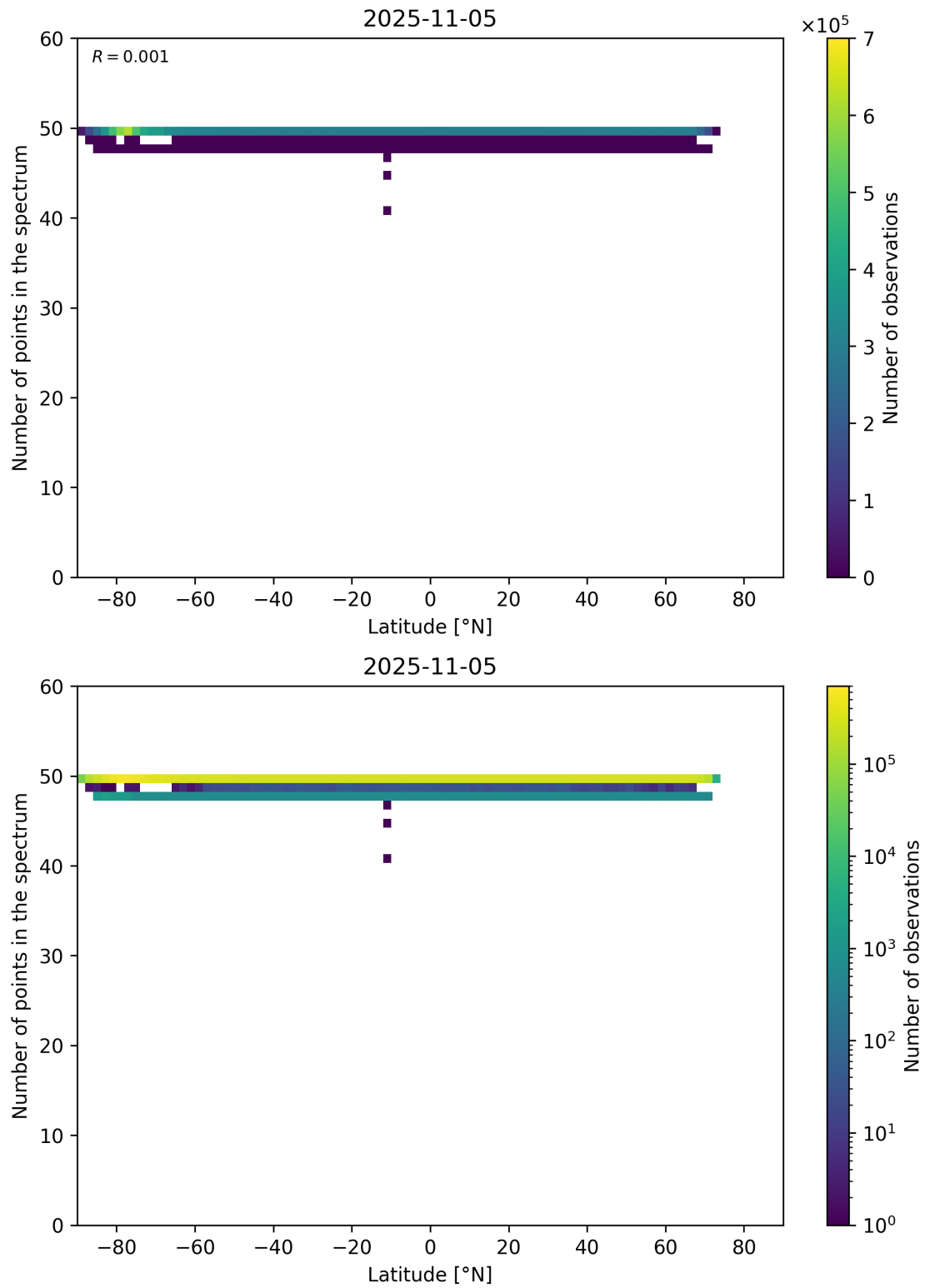
Figure 94: Scatter density plot of “Latitude” against “Number of points in the spectrum” for 2025-11-04 to 2025-11-06.
