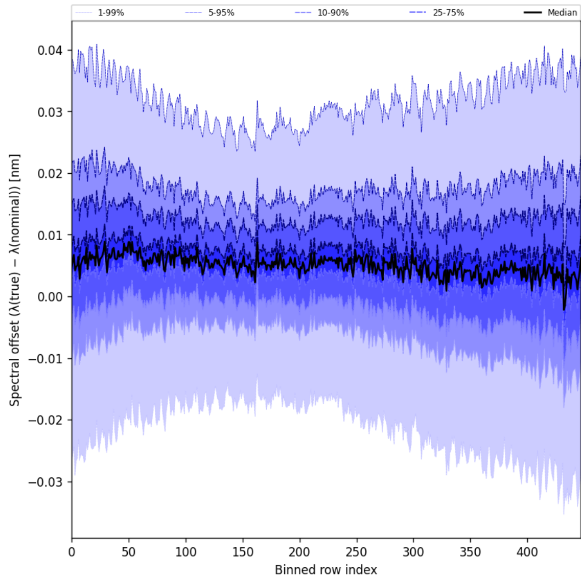
Figure 62: Along track statistics of “Spectral offset ( \lambda_{\text{true}} - \lambda_{\text{nominal}} )” for 2025-11-04 to 2025-11-06
