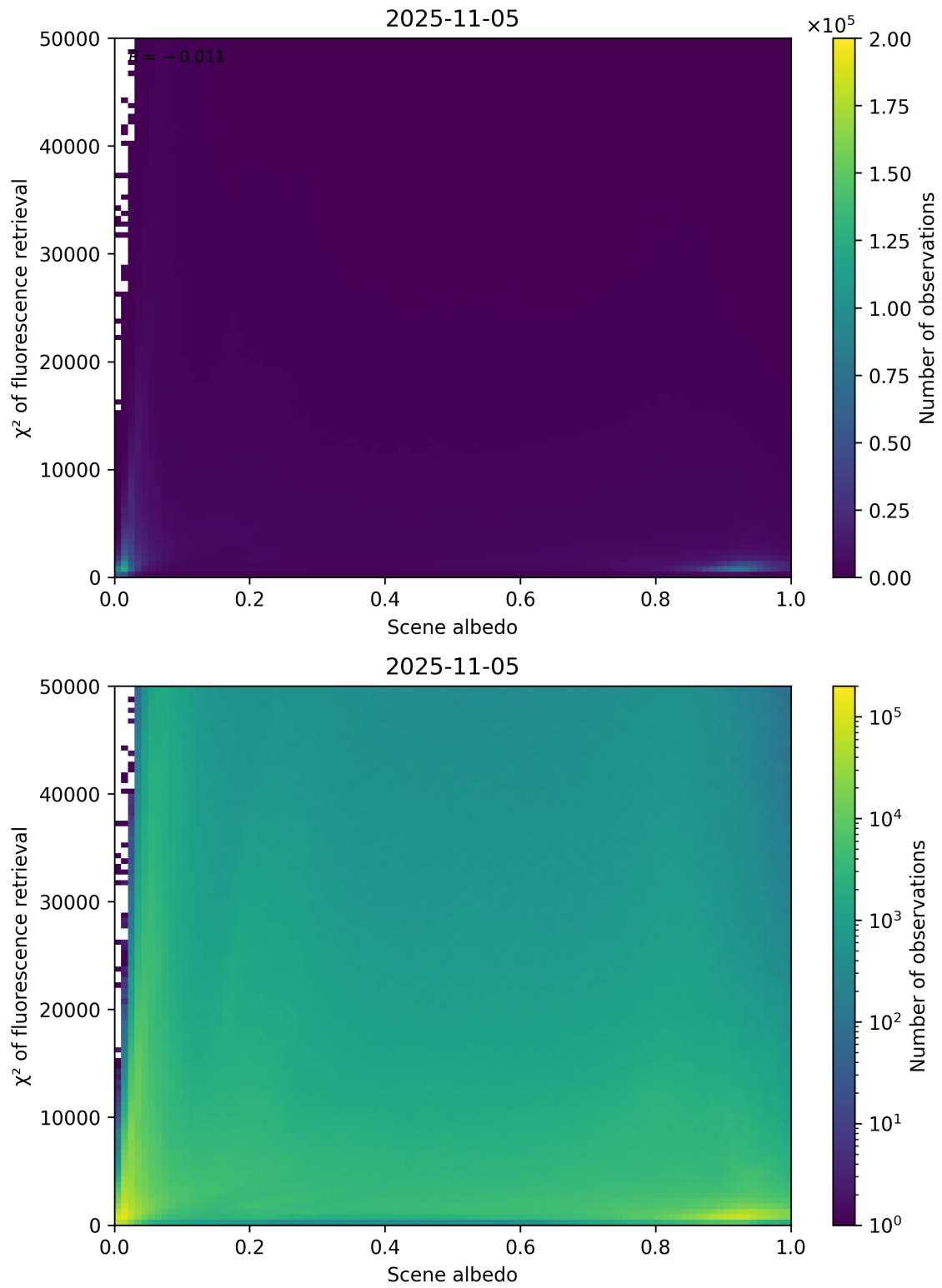
Figure 103: Scatter density plot of “Scene albedo” against “ \chi^2 of fluorescence retrieval” for 2025-11-04 to 2025-11-06.
