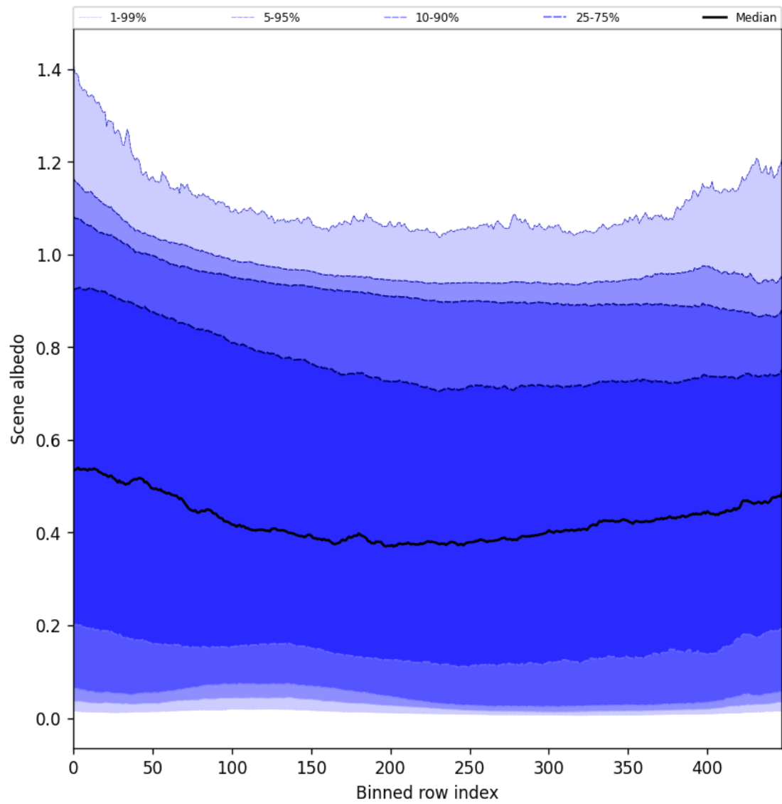
Figure 51: Along track statistics of “Scene albedo” for 2025-11-04 to 2025-11-06
