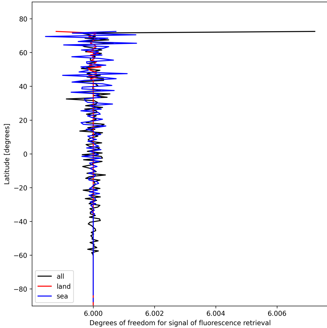
Figure 26: Zonal average of “Degrees of freedom for signal of fluorescence retrieval” for 2025-11-04 to 2025-11-06.
