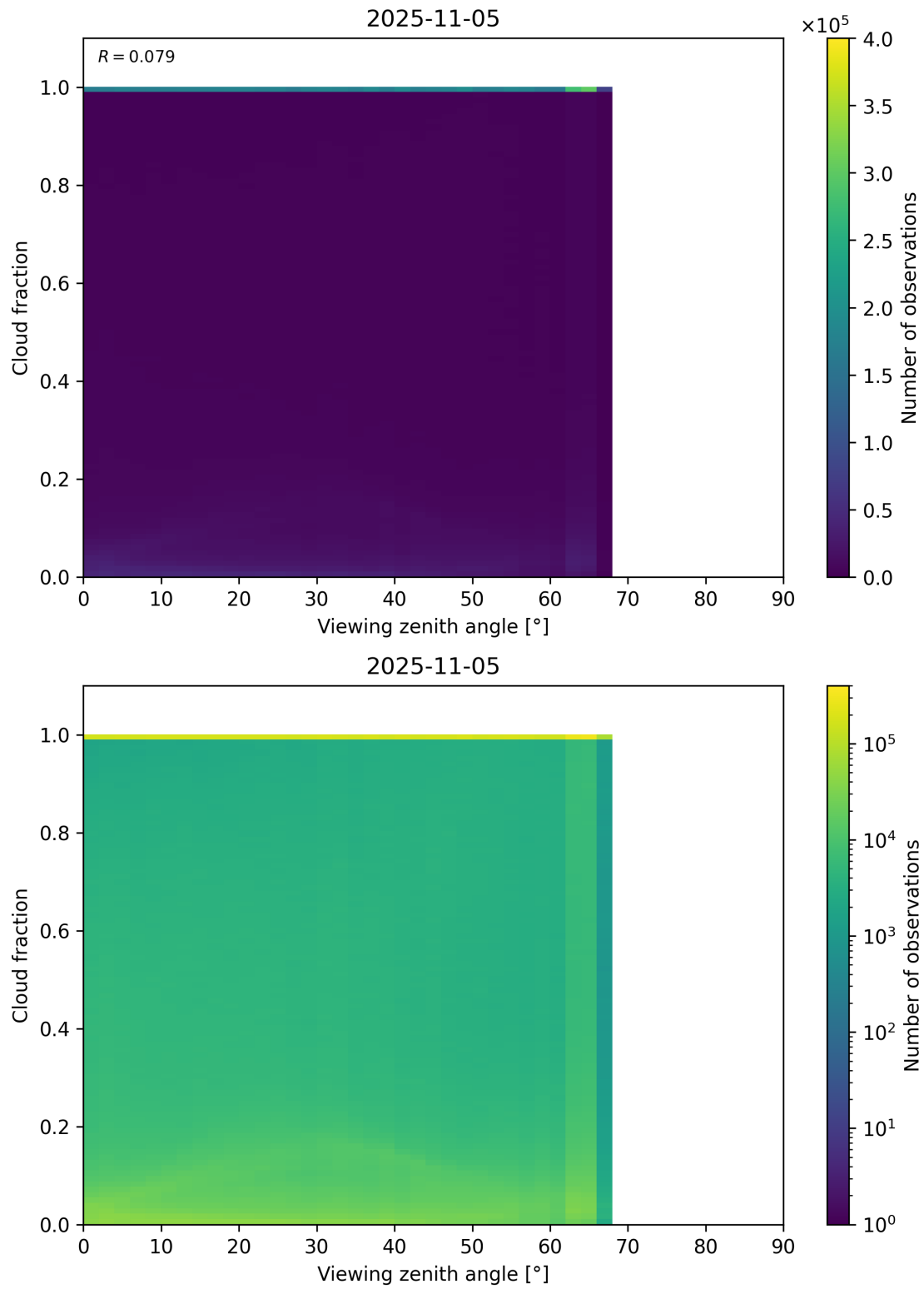
Figure 120: Scatter density plot of “Viewing zenith angle” against “Cloud fraction” for 2025-11-04 to 2025-11-06.
