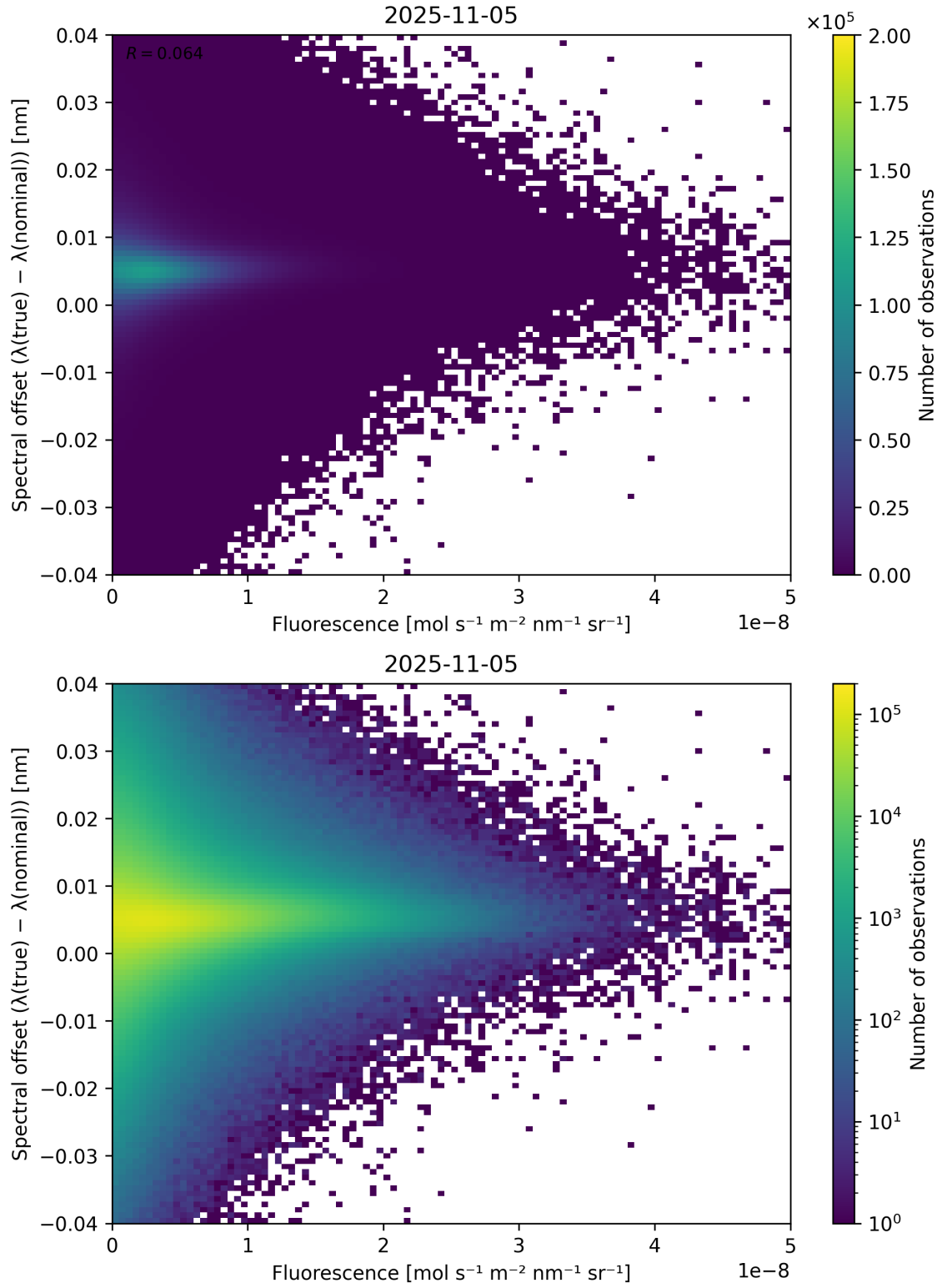
Figure 87: Scatter density plot of “Fluorescence” against “Spectral offset ( \lambda_{\text{true}} - \lambda_{\text{nominal}} )” for 2025-11-04 to 2025-11-06.
