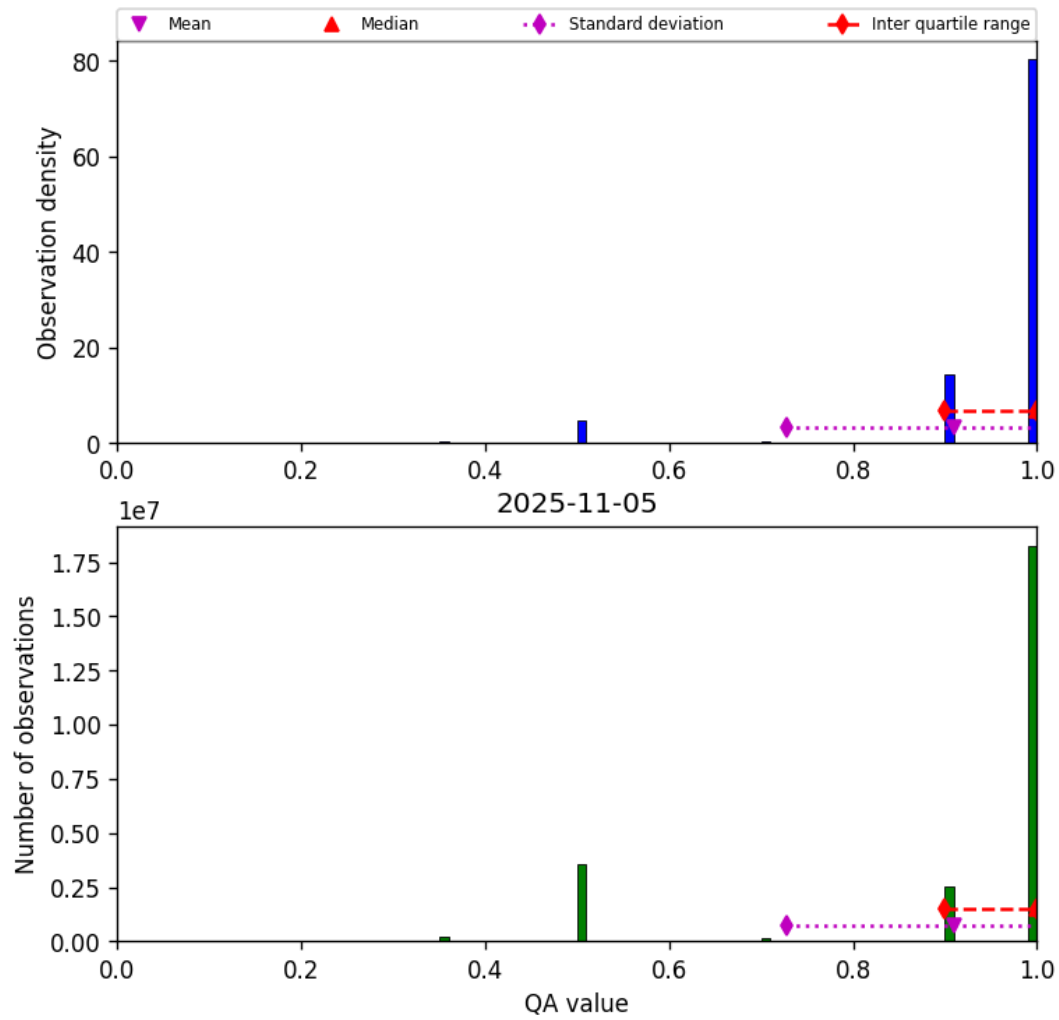
Figure 29: Histogram of “QA value” for 2025-11-04 to 2025-11-06
