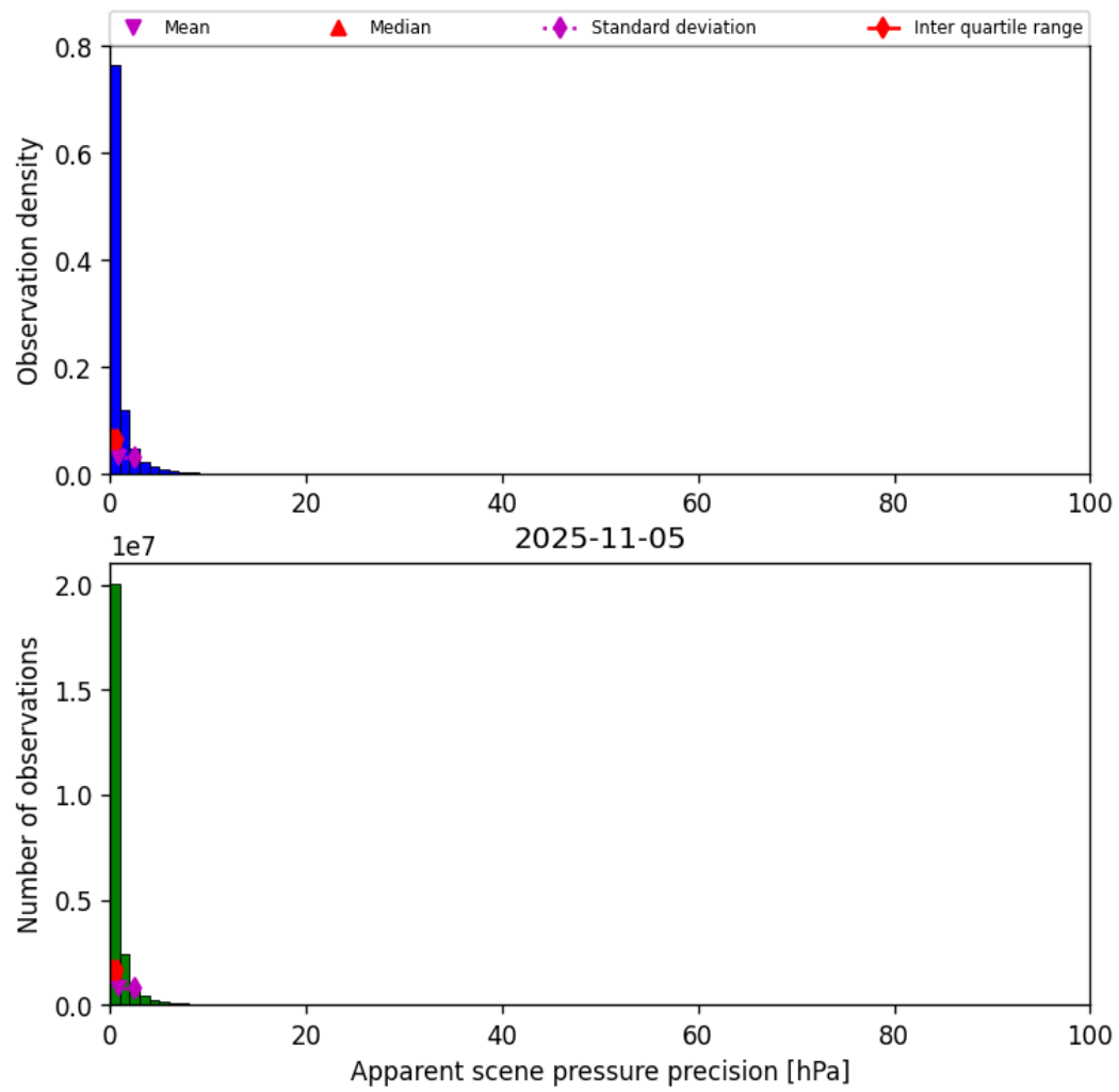
Figure 37: Histogram of “Apparent scene pressure precision” for 2025-11-04 to 2025-11-06
