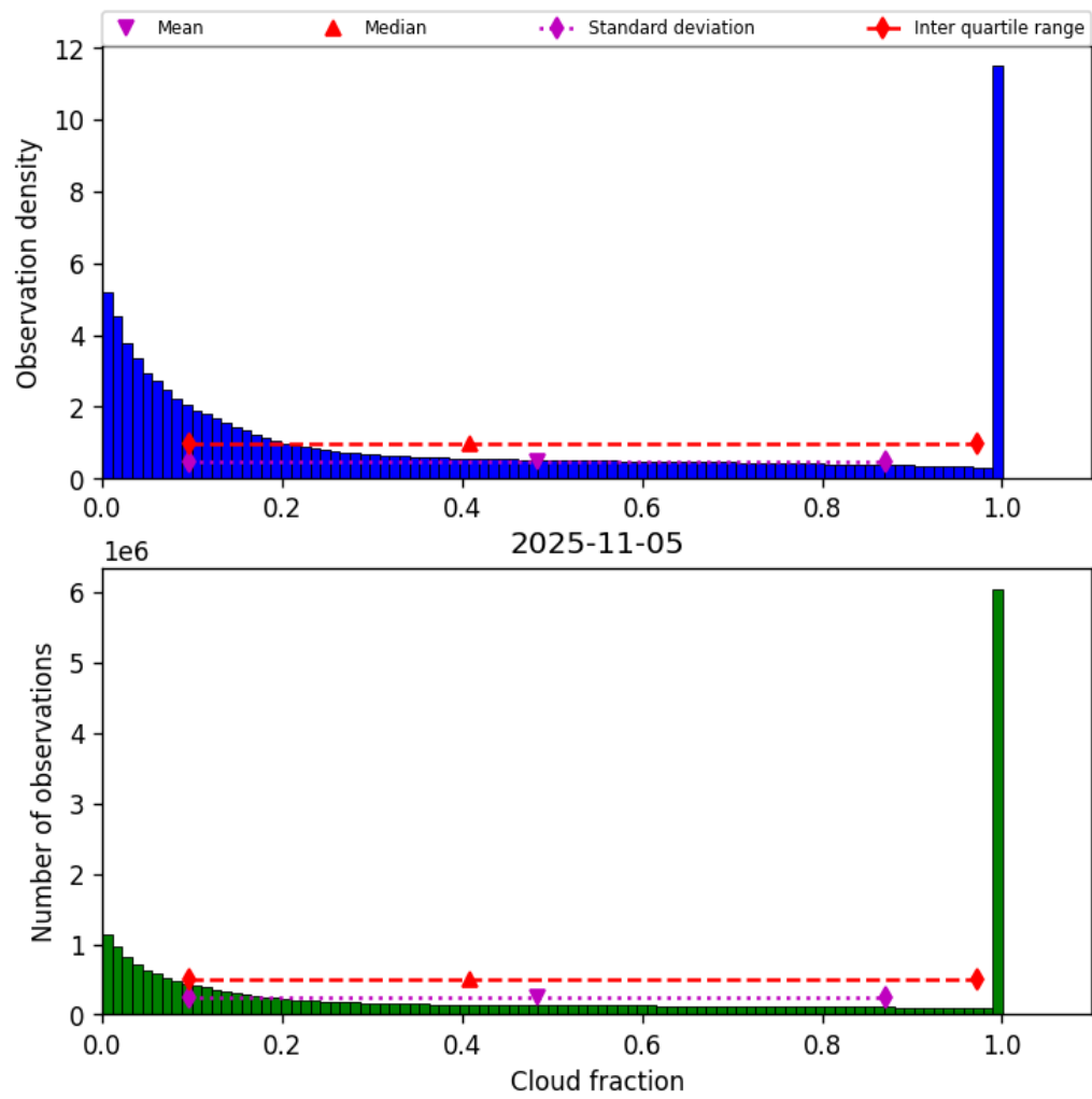
Figure 32: Histogram of “Cloud fraction” for 2025-11-04 to 2025-11-06
