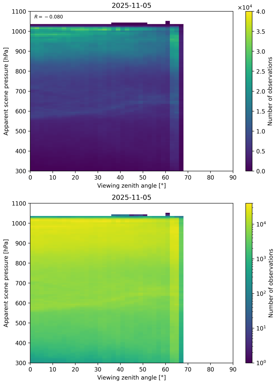
Figure 118: Scatter density plot of “Viewing zenith angle” against “Apparent scene pressure” for 2025-11-04 to 2025-11-06.
