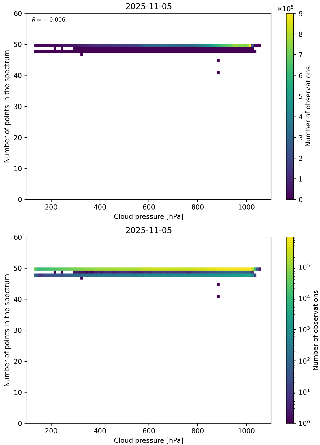
Figure 82: Scatter density plot of “Cloud pressure” against “Number of points in the spectrum” for 2025-11-04 to 2025-11-06.
