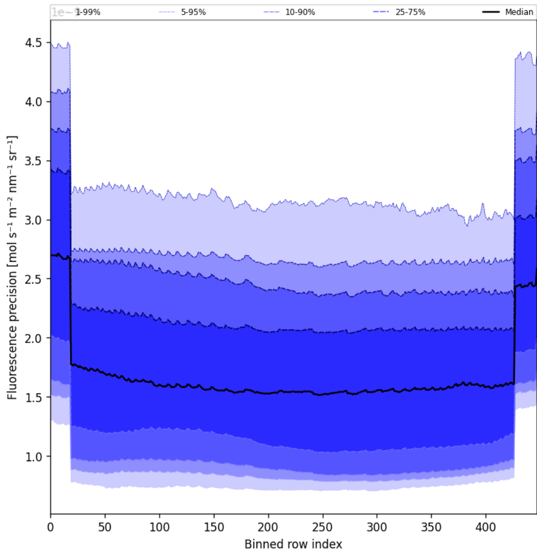
Figure 58: Along track statistics of “Fluorescence precision” for 2025-11-04 to 2025-11-06
