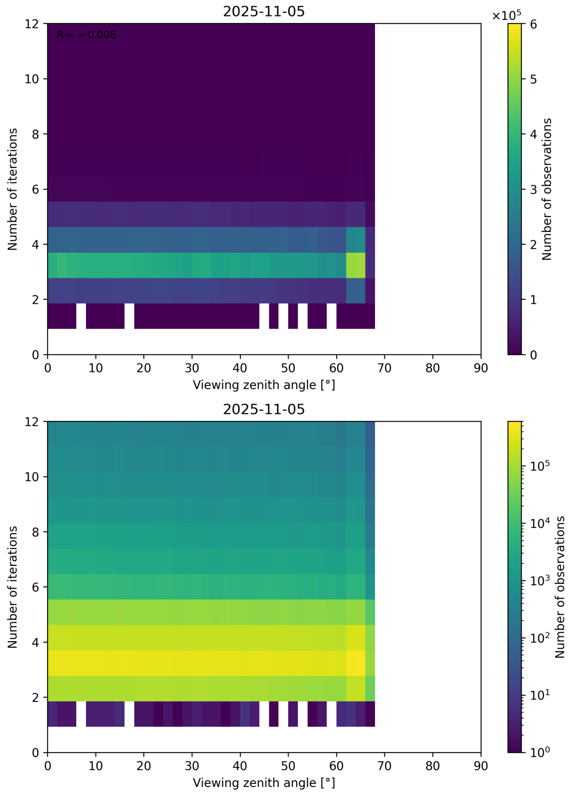
Figure 124: Scatter density plot of “Viewing zenith angle” against “Number of iterations” for 2025-11-04 to 2025-11-06.
