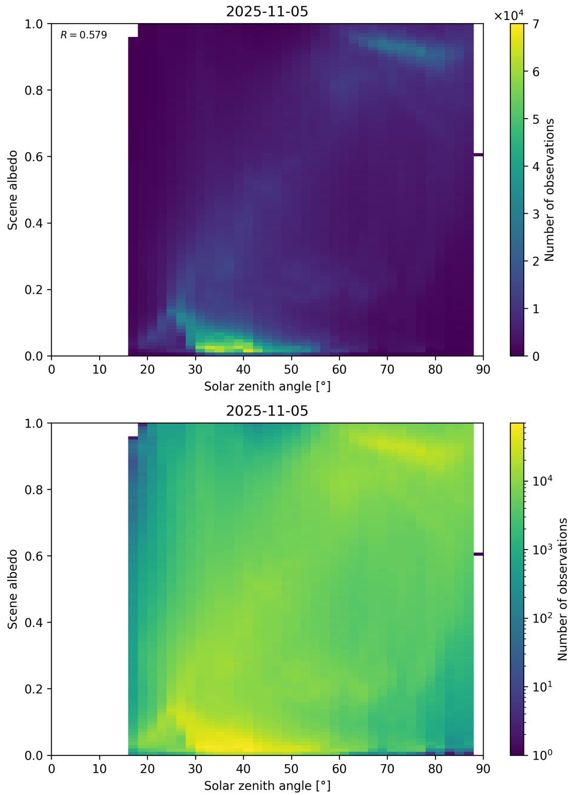
Figure 116: Scatter density plot of “Solar zenith angle” against “Scene albedo” for 2025-11-04 to 2025-11-06.
