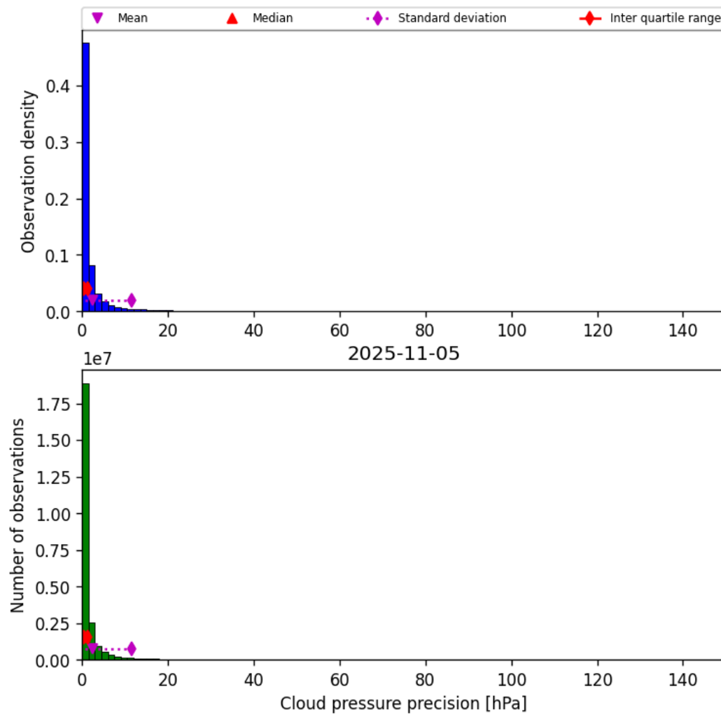
Figure 31: Histogram of “Cloud pressure precision” for 2025-11-04 to 2025-11-06
