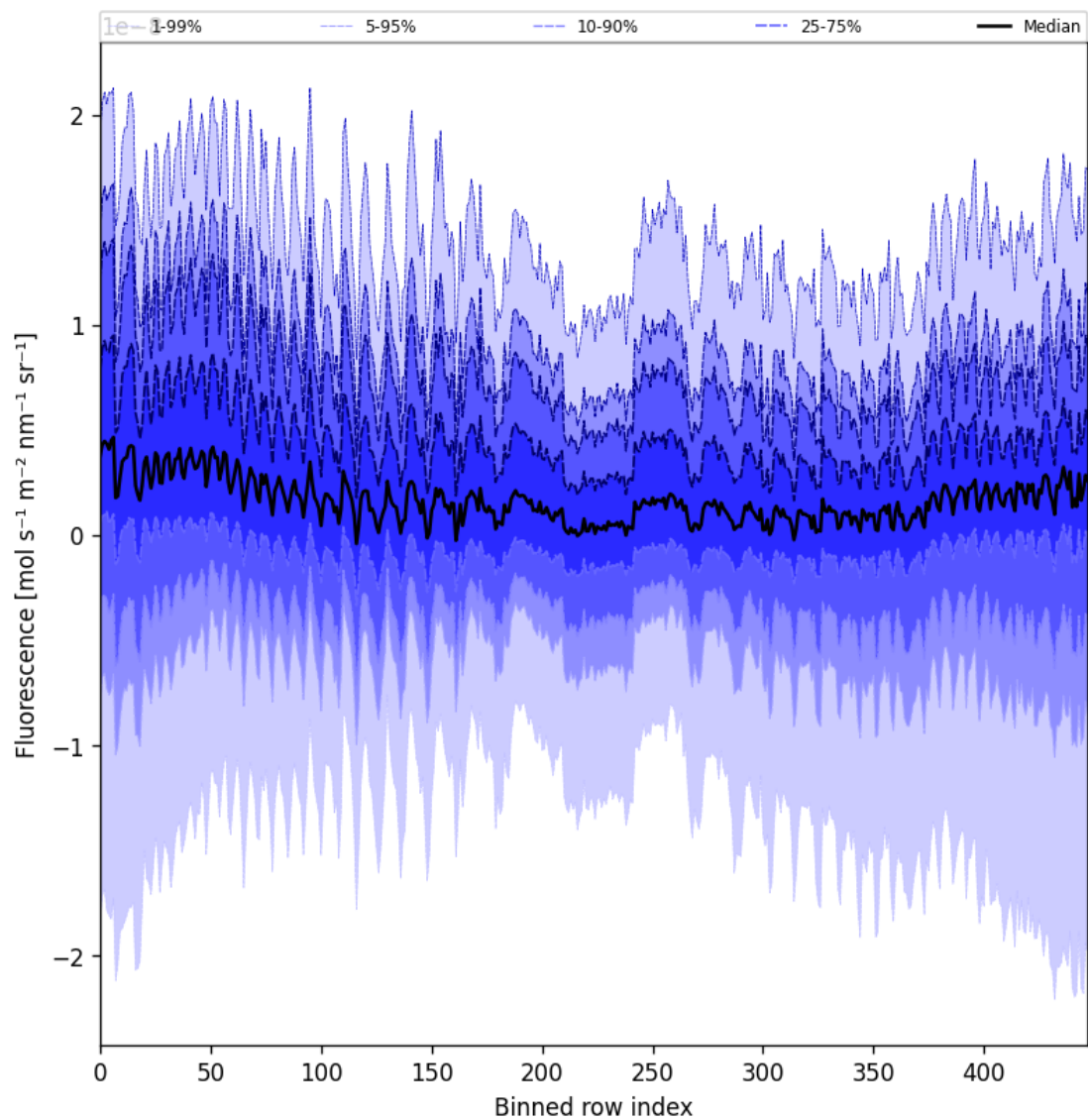
Figure 57: Along track statistics of “Fluorescence” for 2025-11-04 to 2025-11-06
