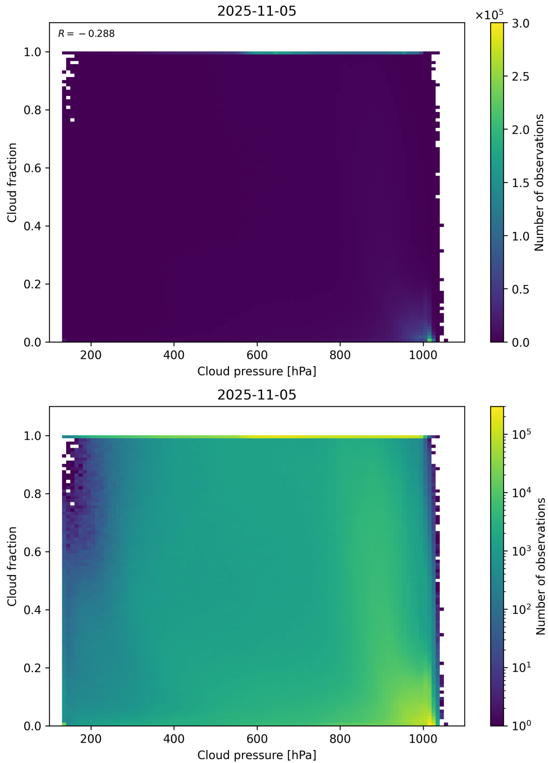
Figure 79: Scatter density plot of “Cloud pressure” against “Cloud fraction” for 2025-11-04 to 2025-11-06.
