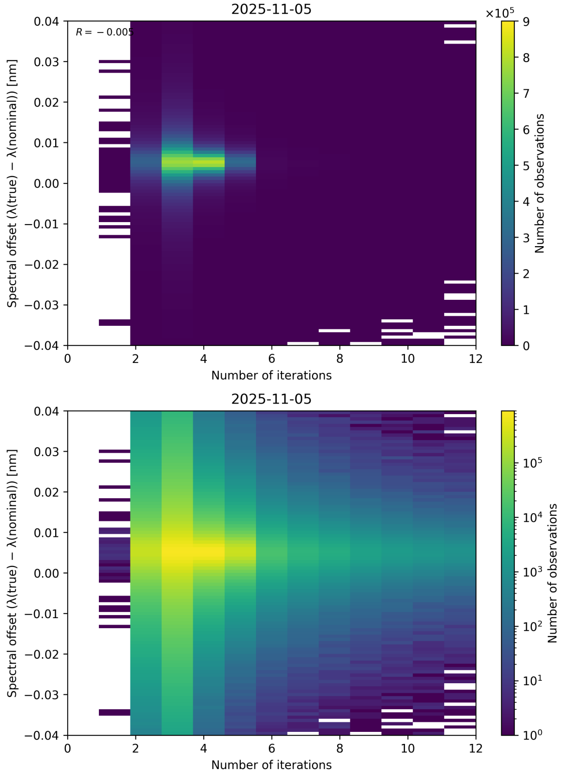
Figure 100: Scatter density plot of “Number of iterations” against “Spectral offset ( \lambda_{\text{true}} - \lambda_{\text{nominal}} )” for 2025-11-04 to 2025-11-06.
