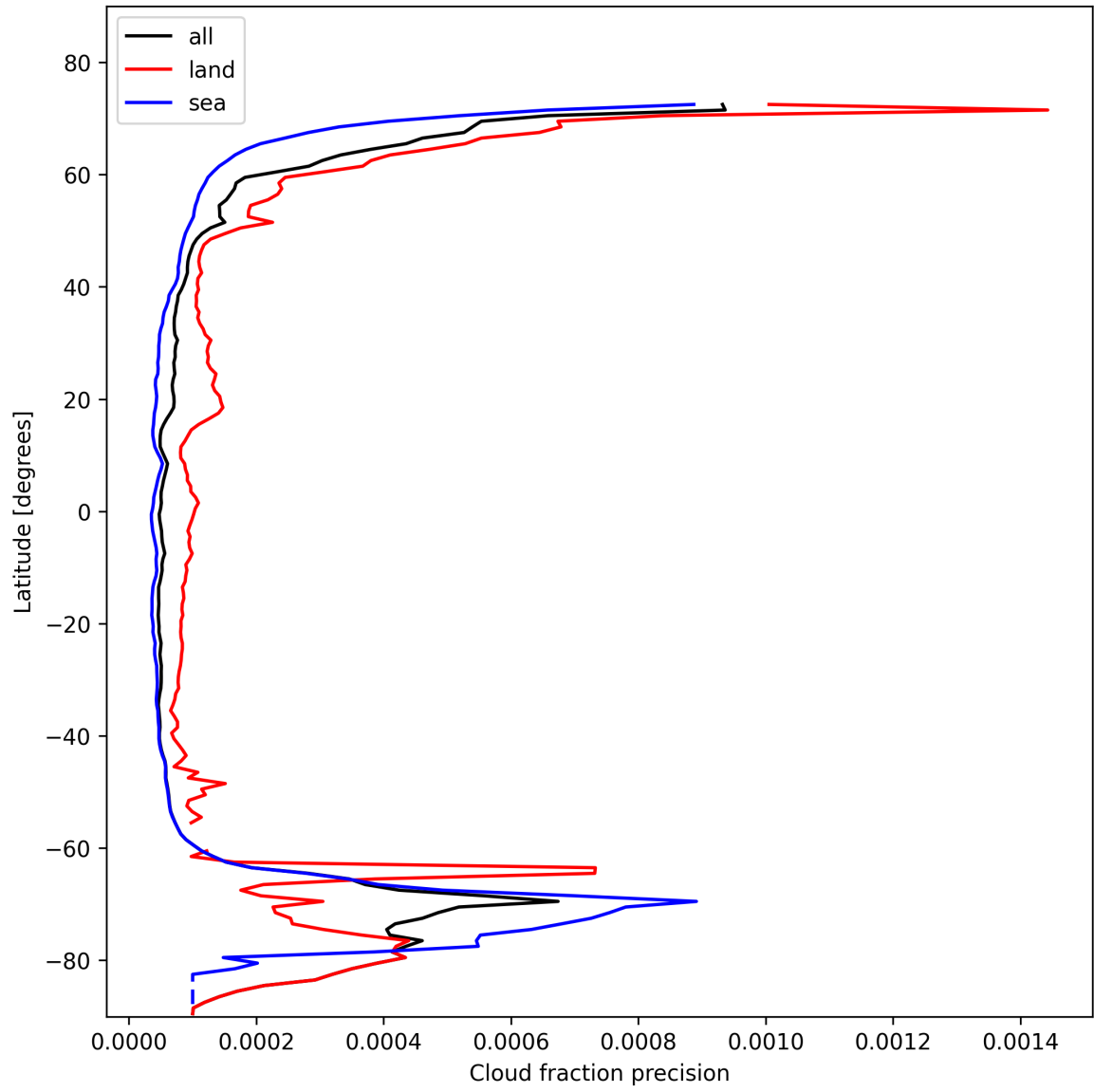
Figure 16: Zonal average of “Cloud fraction precision” for 2025-11-04 to 2025-11-06.
