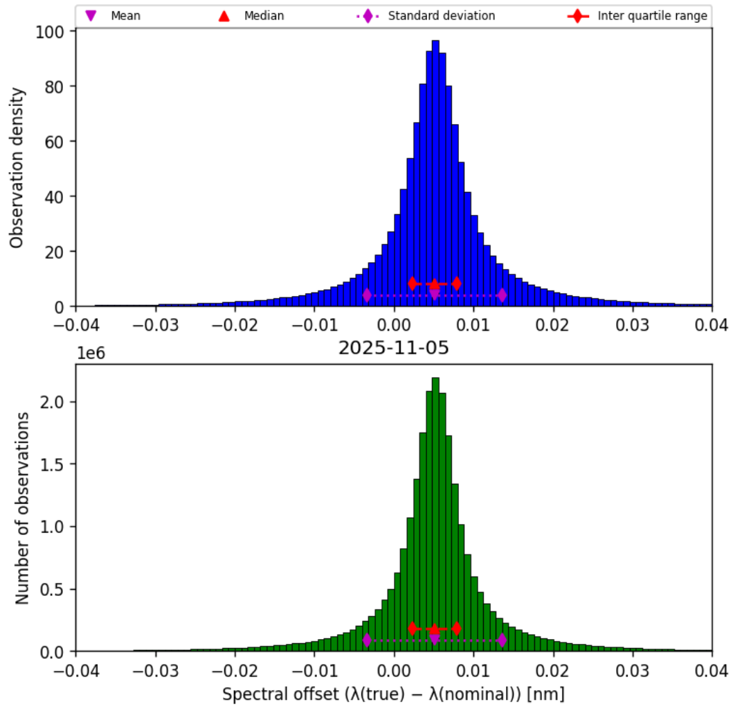
Figure 45: Histogram of “Spectral offset ( \lambda_{\text{true}} - \lambda_{\text{nominal}} )” for 2025-11-04 to 2025-11-06
