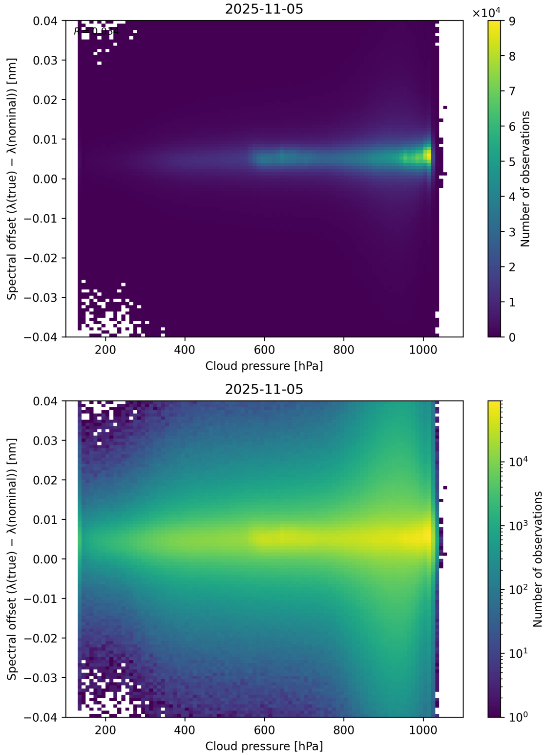
Figure 84: Scatter density plot of “Cloud pressure” against “Spectral offset ( \lambda_{\text{true}} - \lambda_{\text{nominal}} )” for 2025-11-04 to 2025-11-06.
