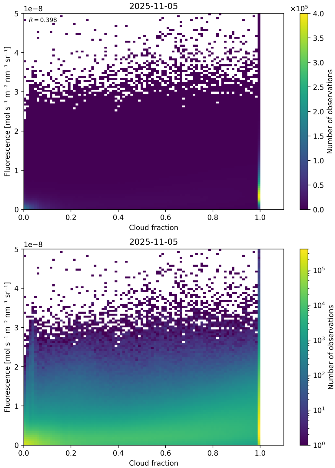
Figure 72: Scatter density plot of “Cloud fraction” against “Fluorescence” for 2025-11-04 to 2025-11-06.
