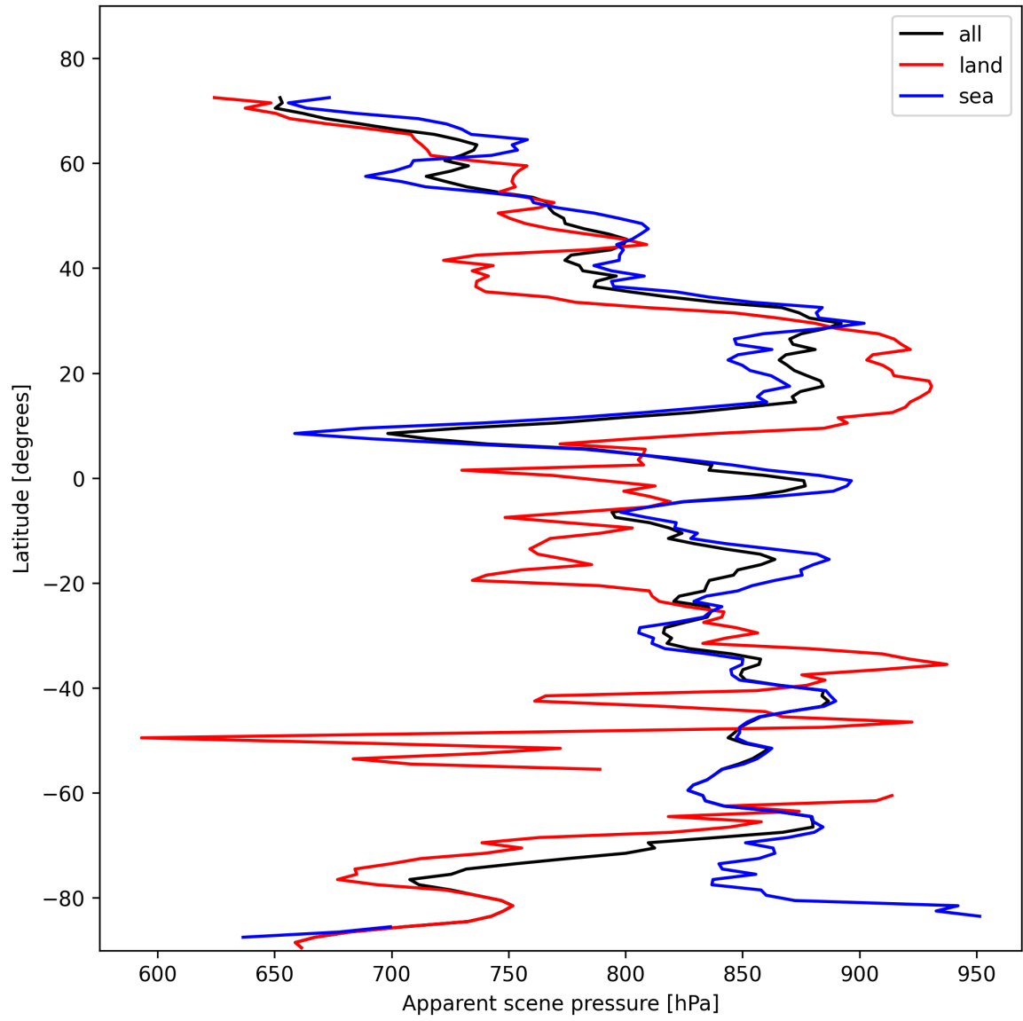
Figure 19: Zonal average of “Apparent scene pressure” for 2025-11-04 to 2025-11-06.
