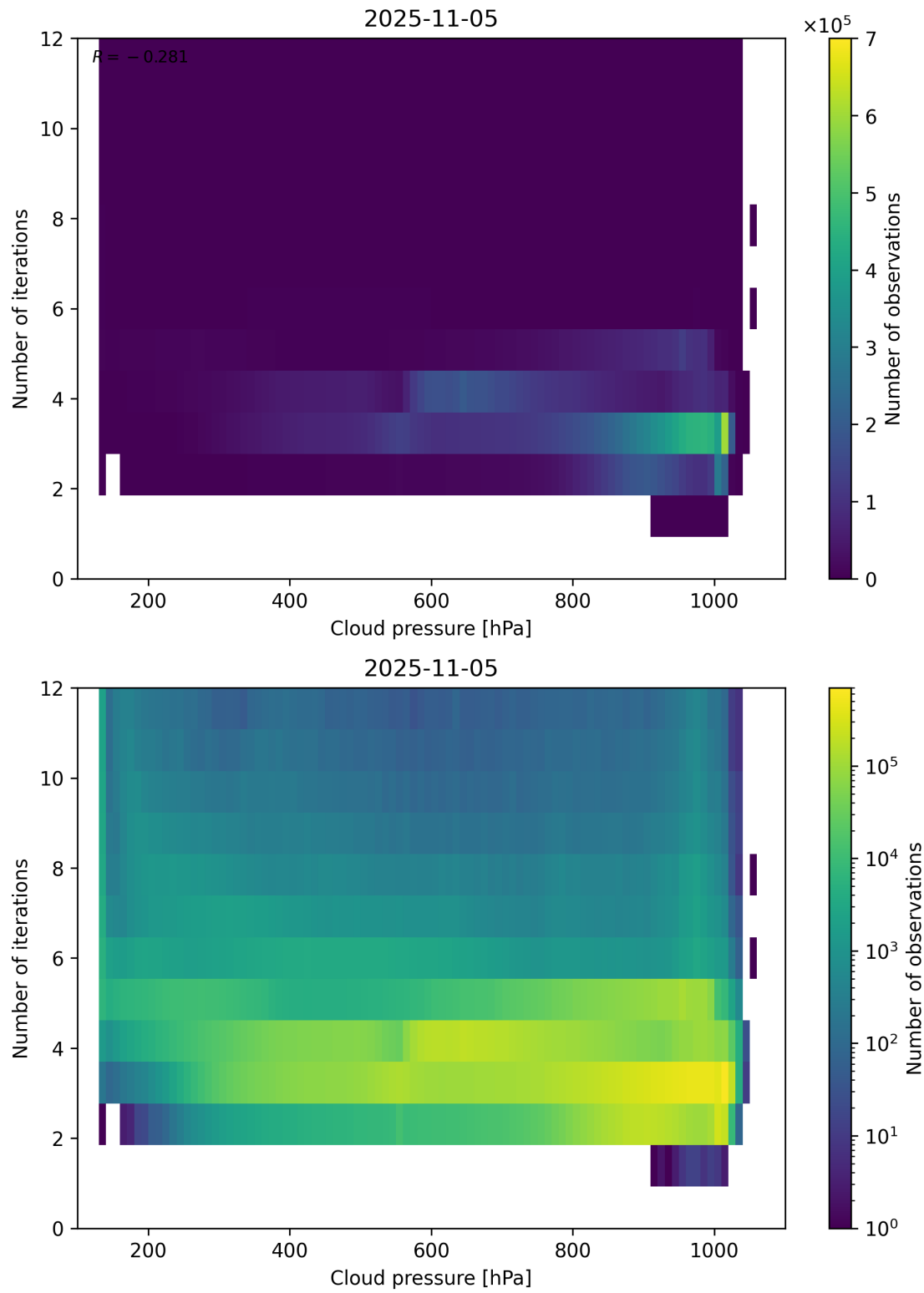
Figure 81: Scatter density plot of “Cloud pressure” against “Number of iterations” for 2025-11-04 to 2025-11-06.
