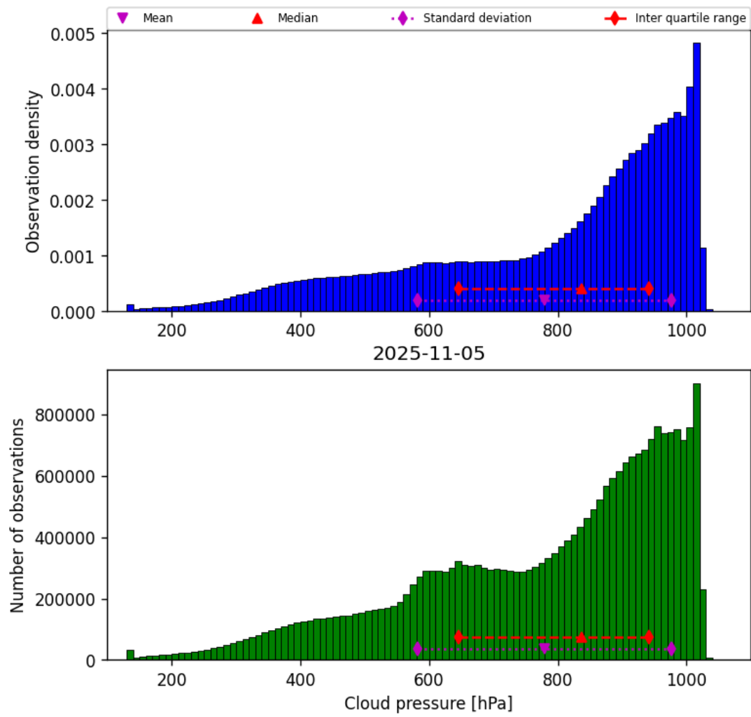
Figure 30: Histogram of “Cloud pressure” for 2025-11-04 to 2025-11-06
