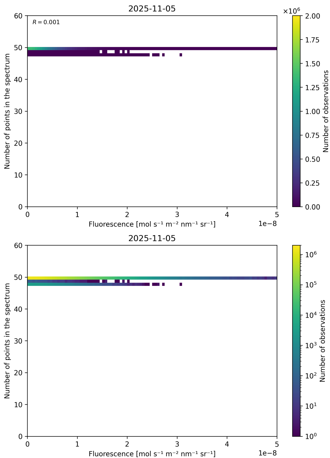
Figure 86: Scatter density plot of “Fluorescence” against “Number of points in the spectrum” for 2025-11-04 to 2025-11-06.
