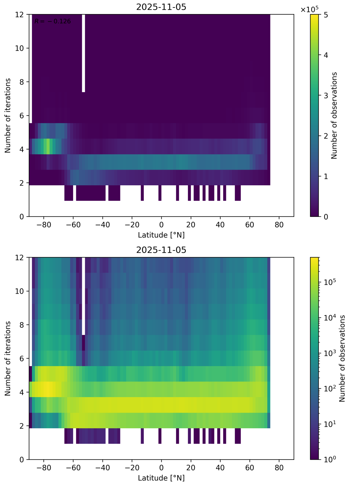
Figure 93: Scatter density plot of “Latitude” against “Number of iterations” for 2025-11-04 to 2025-11-06.
