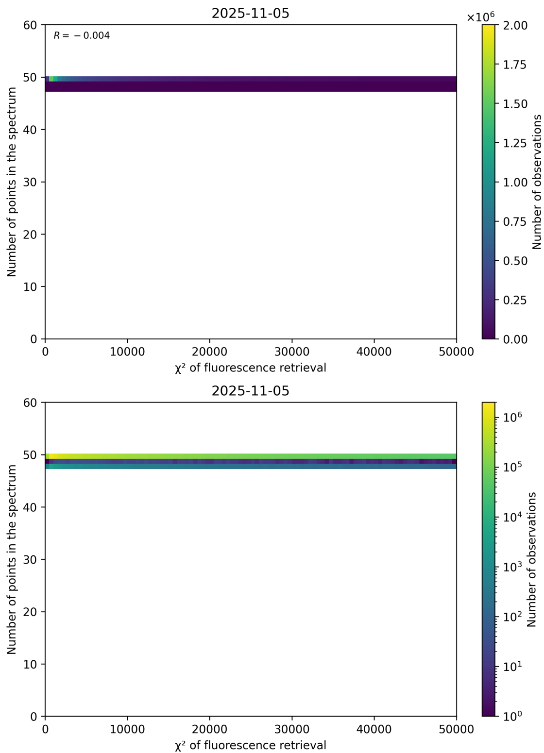
Figure 68: Scatter density plot of “ \chi^2 of fluorescence retrieval” against “Number of points in the spectrum” for 2025-11-04 to 2025-11-06.
