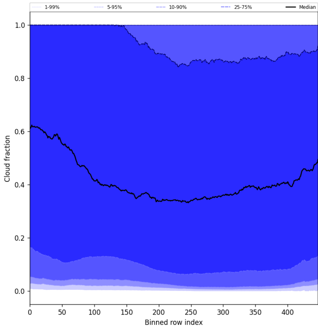
Figure 49: Along track statistics of “Cloud fraction” for 2025-11-04 to 2025-11-06
