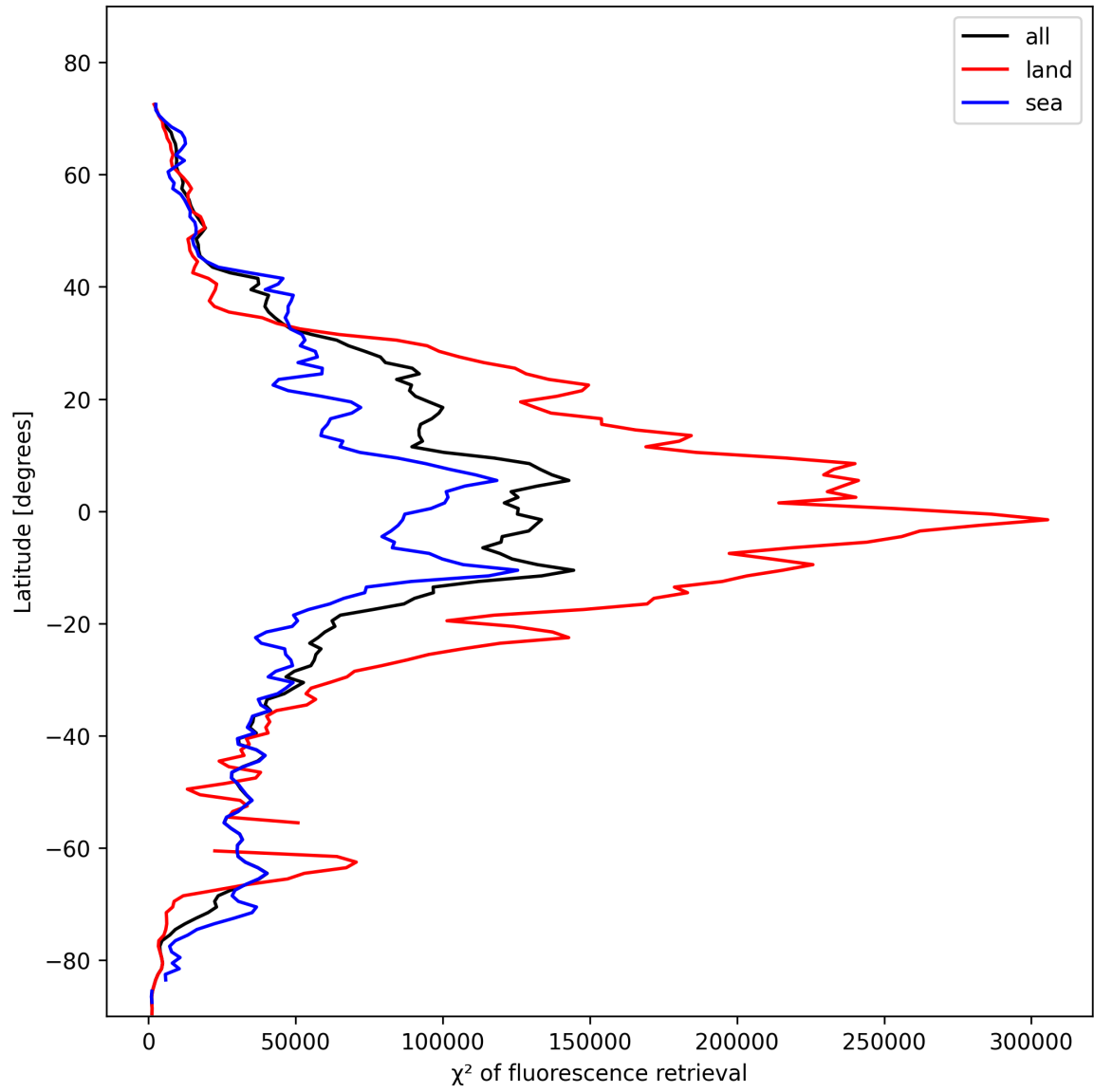
Figure 25: Zonal average of “ \chi^2 of fluorescence retrieval” for 2025-11-04 to 2025-11-06.
