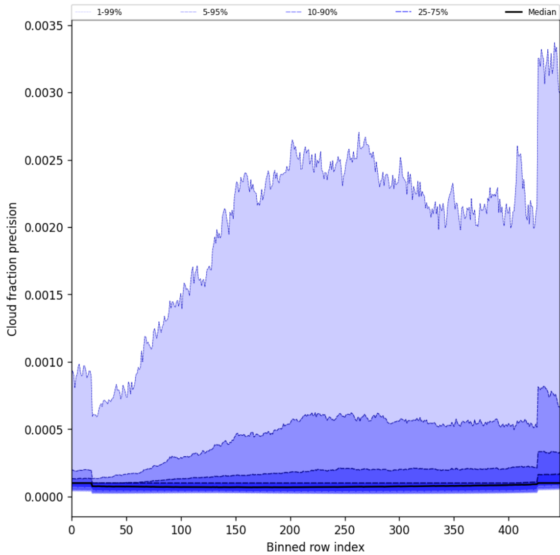
Figure 50: Along track statistics of “Cloud fraction precision” for 2025-11-04 to 2025-11-06
