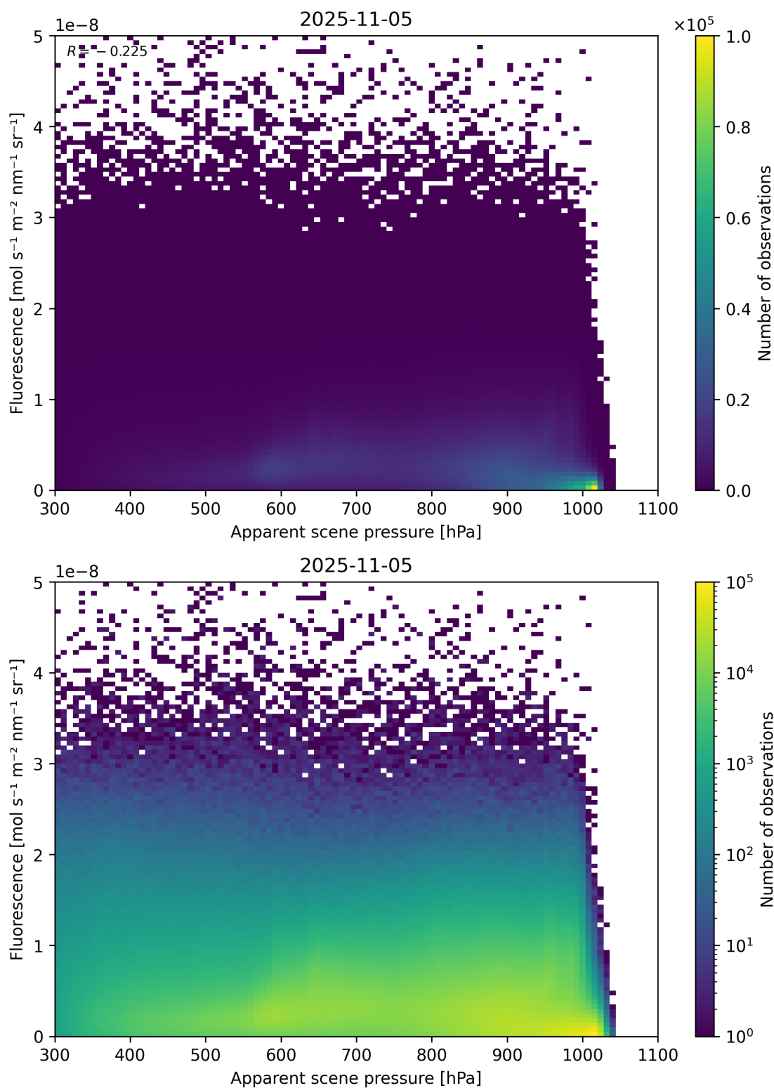
Figure 64: Scatter density plot of “Apparent scene pressure” against “Fluorescence” for 2025-11-04 to 2025-11-06.
