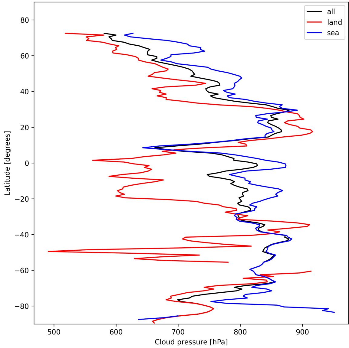
Figure 13: Zonal average of “Cloud pressure” for 2025-11-04 to 2025-11-06.
