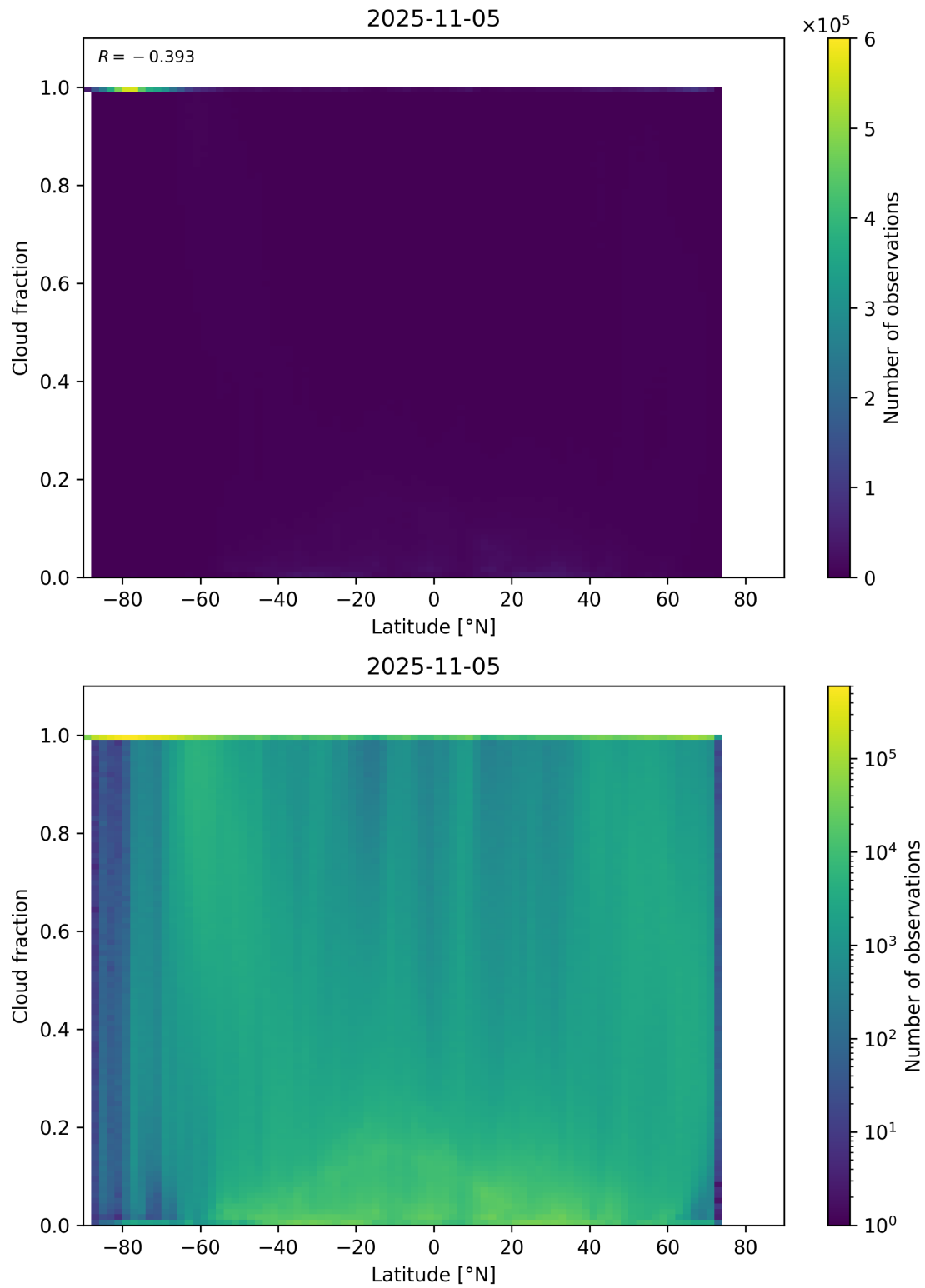
Figure 90: Scatter density plot of “Latitude” against “Cloud fraction” for 2025-11-04 to 2025-11-06.
