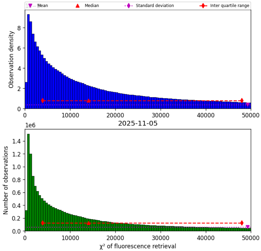
Figure 42: Histogram of “ \chi^2 of fluorescence retrieval” for 2025-11-04 to 2025-11-06
