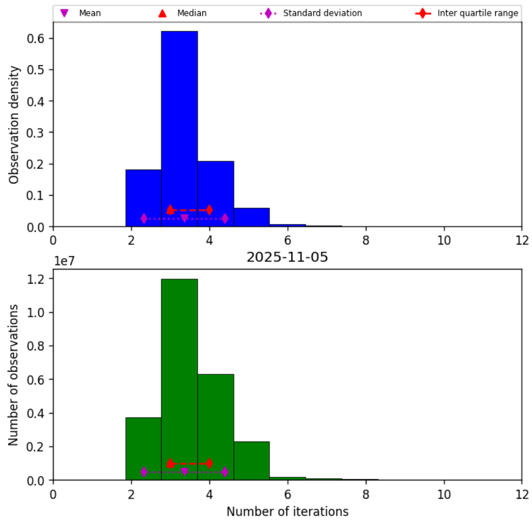
Figure 39: Histogram of “Number of iterations” for 2025-11-04 to 2025-11-06
