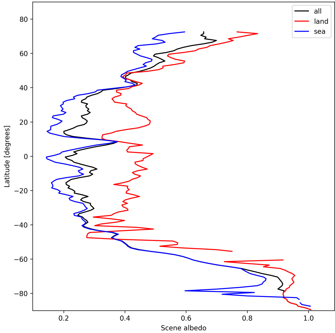
Figure 17: Zonal average of “Scene albedo” for 2025-11-04 to 2025-11-06.
