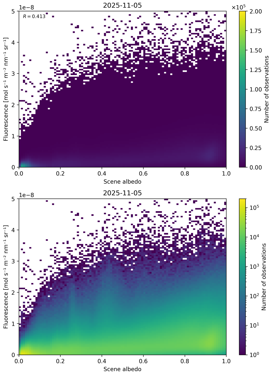
Figure 104: Scatter density plot of “Scene albedo” against “Fluorescence” for 2025-11-04 to 2025-11-06.
