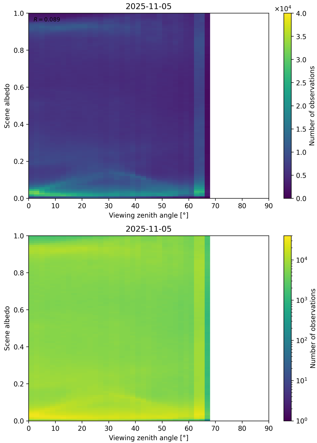
Figure 126: Scatter density plot of “Viewing zenith angle” against “Scene albedo” for 2025-11-04 to 2025-11-06.
