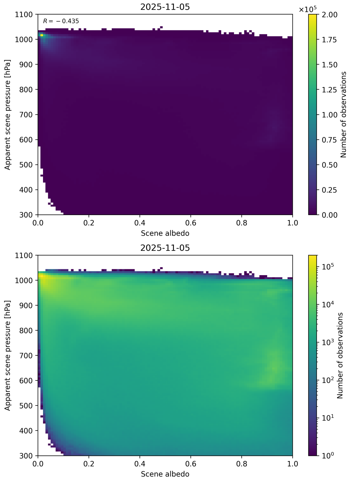
Figure 102: Scatter density plot of “Scene albedo” against “Apparent scene pressure” for 2025-11-04 to 2025-11-06.
