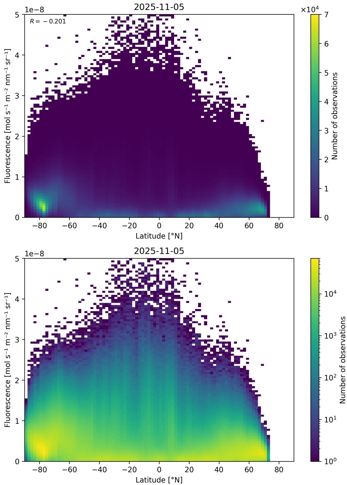
Figure 92: Scatter density plot of “Latitude” against “Fluorescence” for 2025-11-04 to 2025-11-06.
