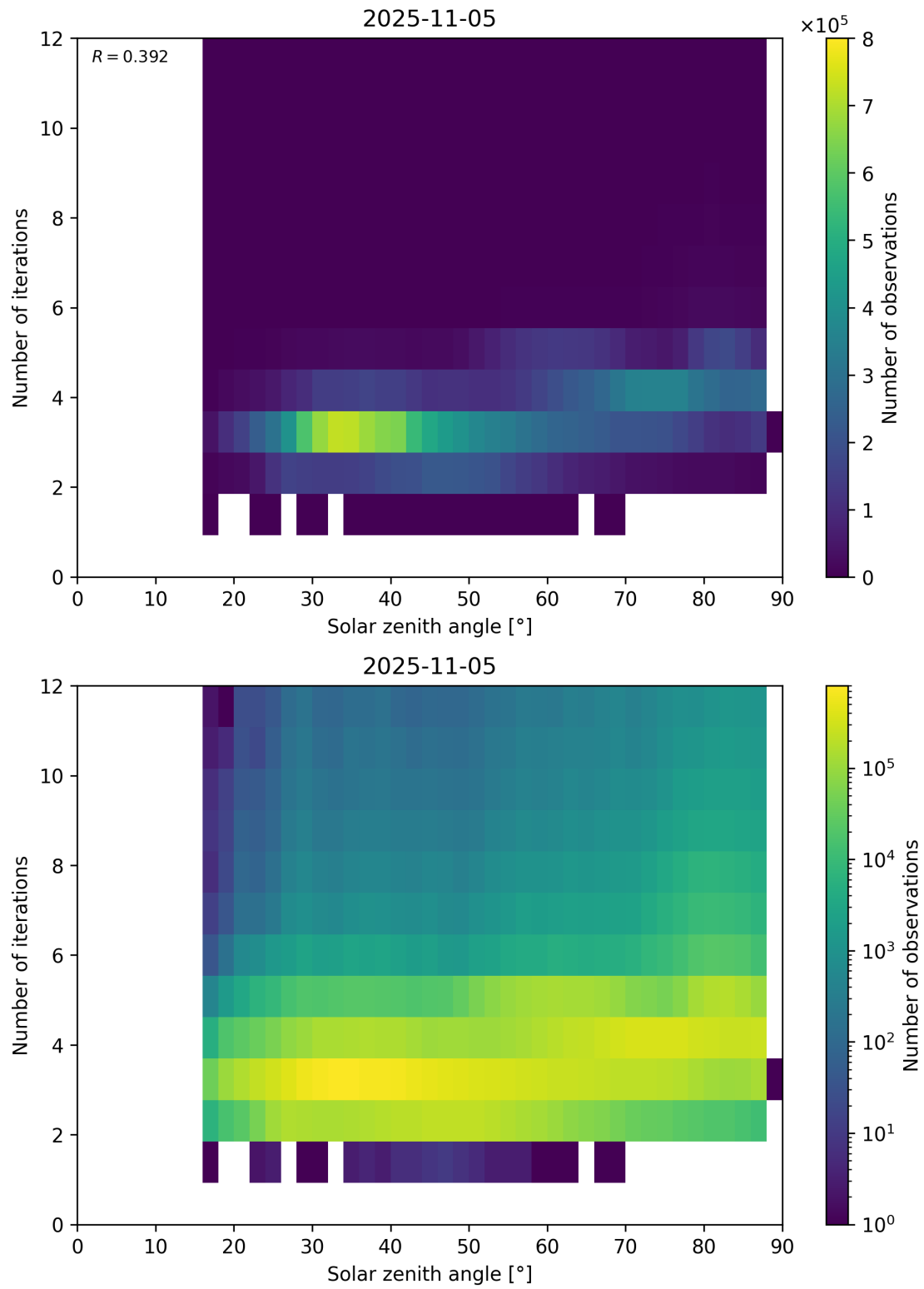
Figure 114: Scatter density plot of “Solar zenith angle” against “Number of iterations” for 2025-11-04 to 2025-11-06.
