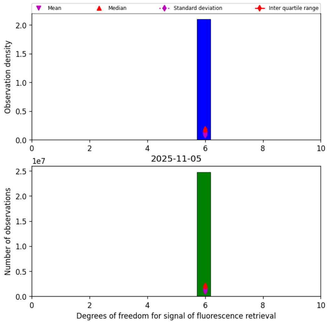
Figure 43: Histogram of “Degrees of freedom for signal of fluorescence retrieval” for 2025-11-04 to 2025-11-06
