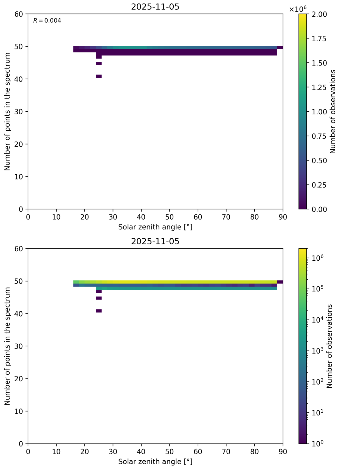
Figure 115: Scatter density plot of “Solar zenith angle” against “Number of points in the spectrum” for 2025-11-04 to 2025-11-06.
