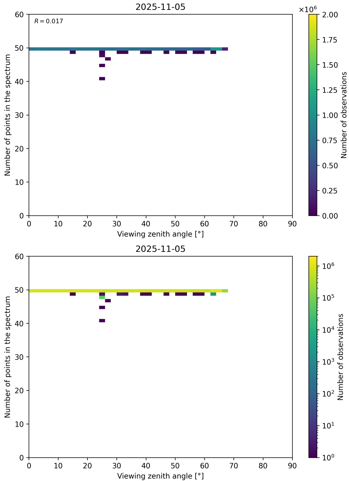
Figure 125: Scatter density plot of “Viewing zenith angle” against “Number of points in the spectrum” for 2025-11-04 to 2025-11-06.
