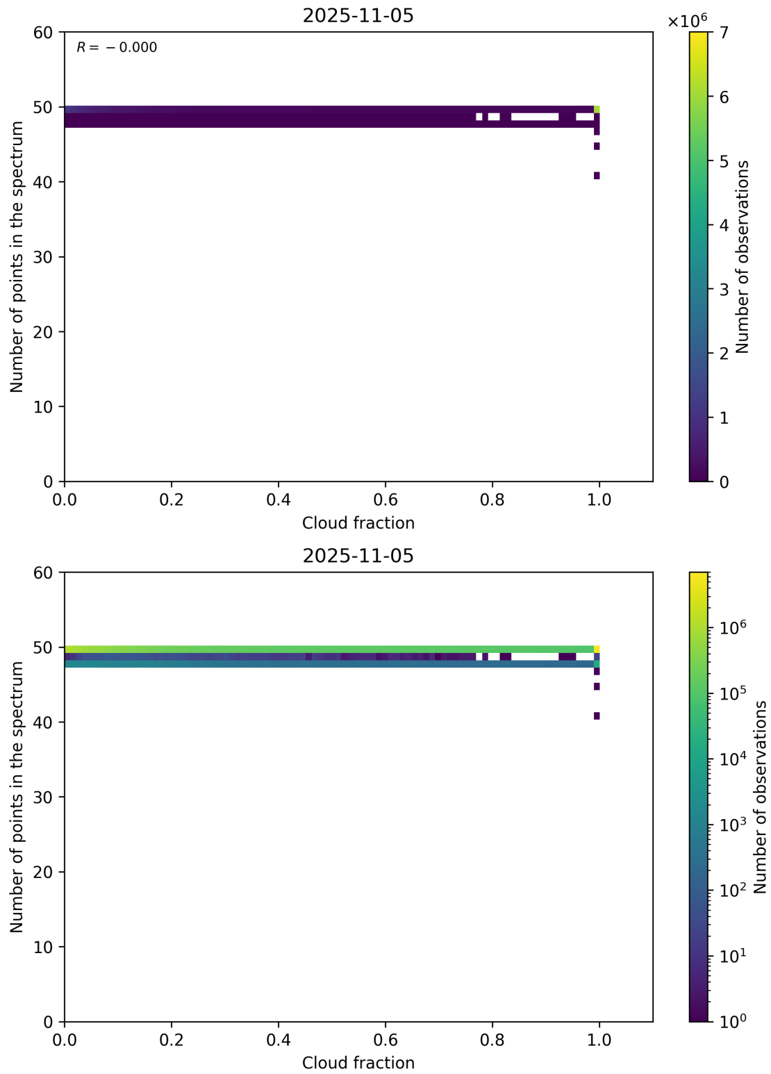
Figure 74: Scatter density plot of “Cloud fraction” against “Number of points in the spectrum” for 2025-11-04 to 2025-11-06.
