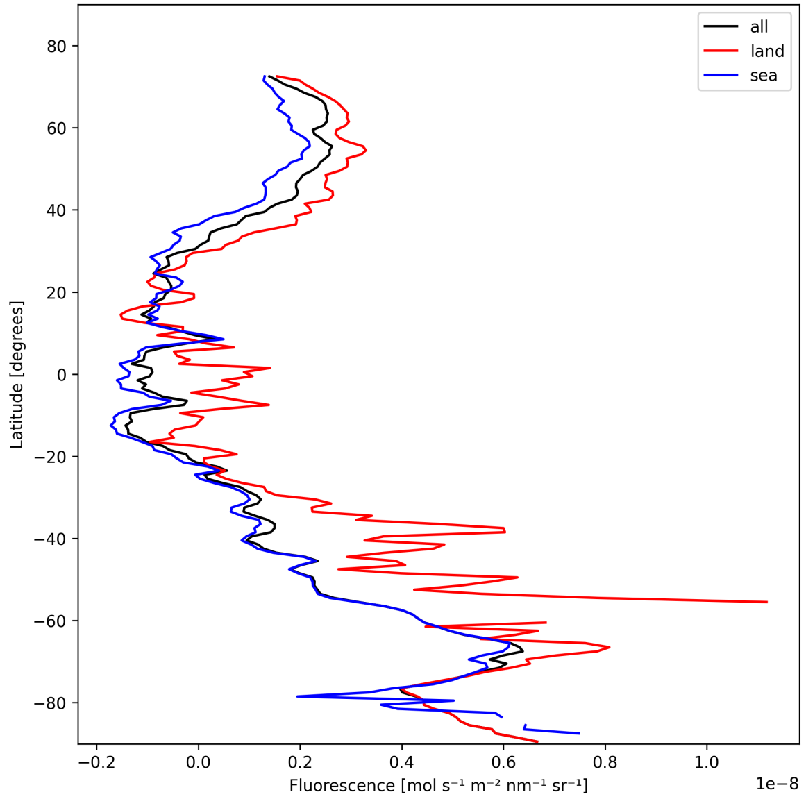
Figure 23: Zonal average of “Fluorescence” for 2025-11-04 to 2025-11-06.
