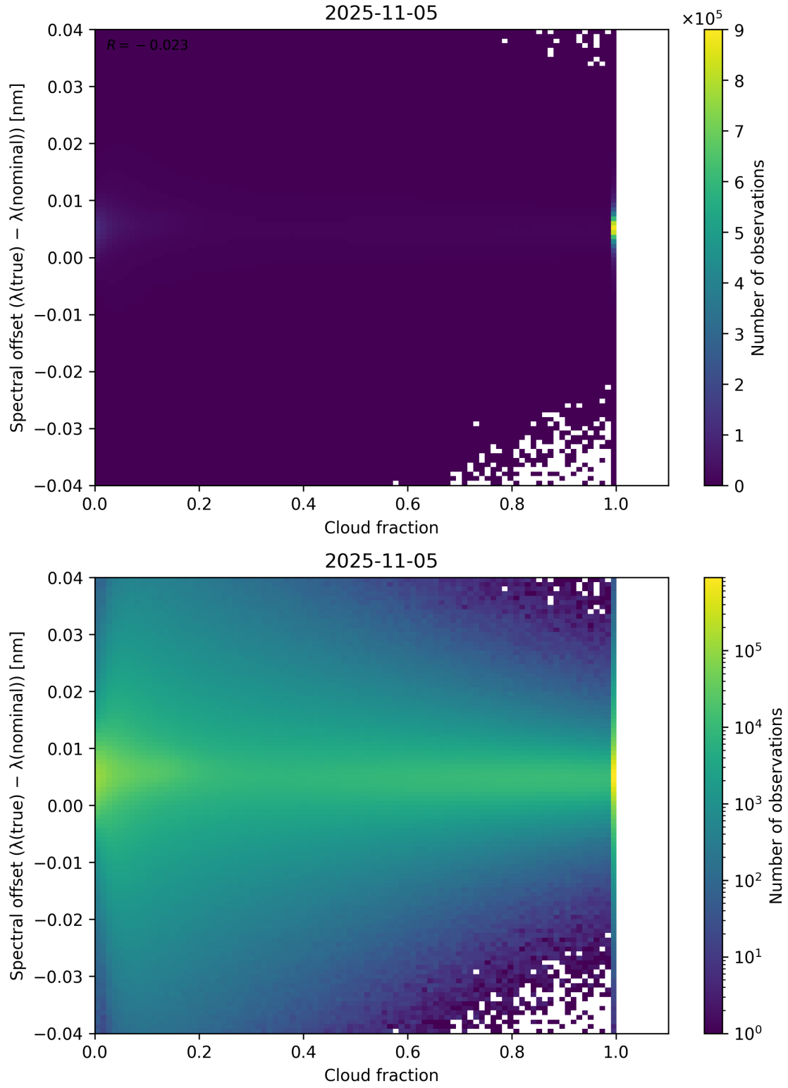
Figure 76: Scatter density plot of “Cloud fraction” against “Spectral offset ( \lambda_{\text{true}} - \lambda_{\text{nominal}} )” for 2025-11-04 to 2025-11-06.
