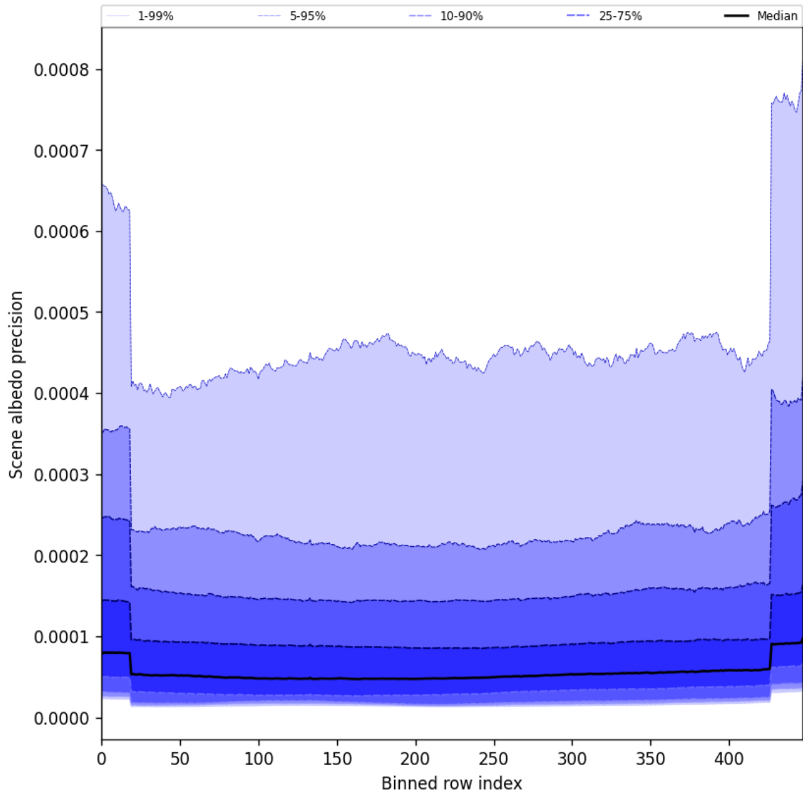
Figure 52: Along track statistics of “Scene albedo precision” for 2025-11-04 to 2025-11-06
