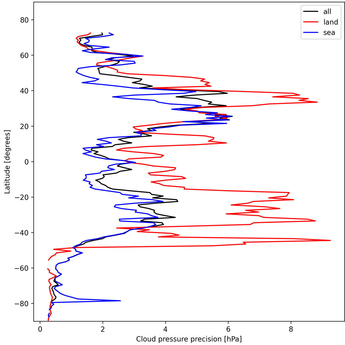
Figure 14: Zonal average of “Cloud pressure precision” for 2025-11-04 to 2025-11-06.
