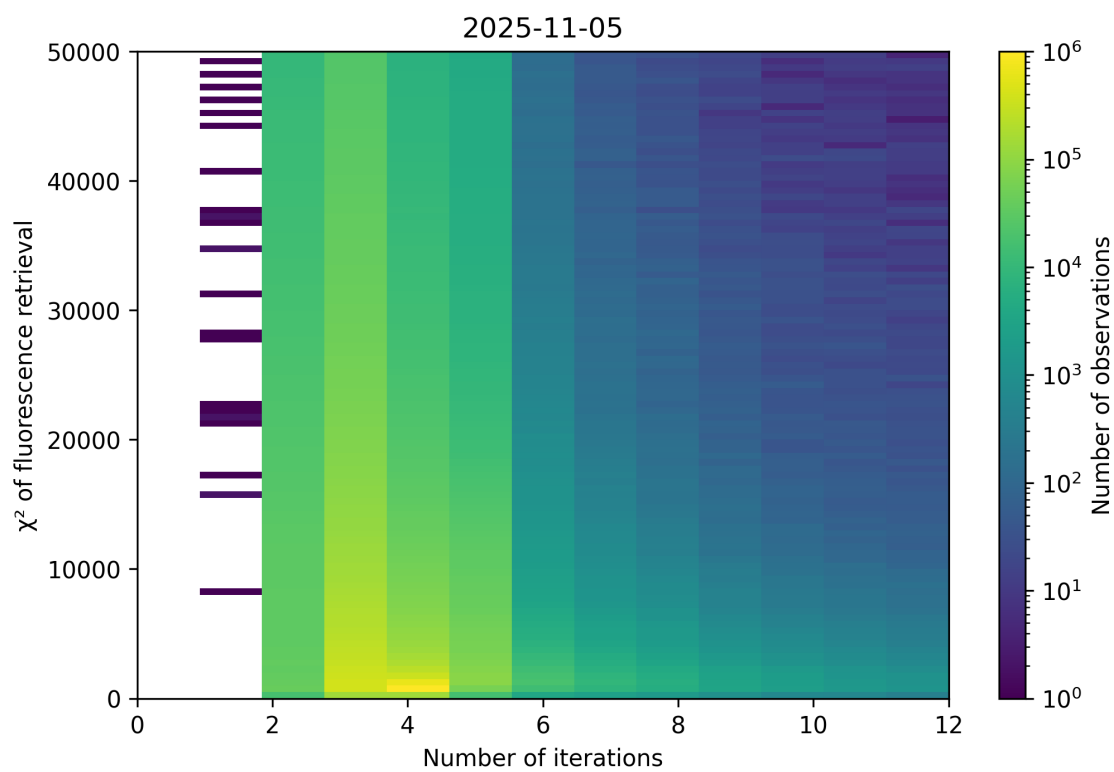
Figure 97: Scatter density plot of “Number of iterations” against “ \chi^2 of fluorescence retrieval” for 2025-11-04 to 2025-11-06.
