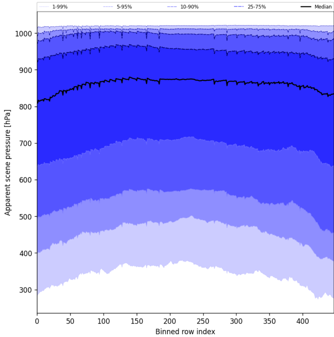
Figure 53: Along track statistics of “Apparent scene pressure” for 2025-11-04 to 2025-11-06
