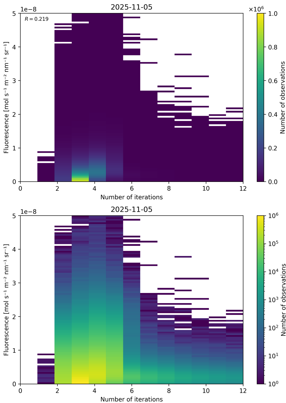
Figure 98: Scatter density plot of “Number of iterations” against “Fluorescence” for 2025-11-04 to 2025-11-06.
