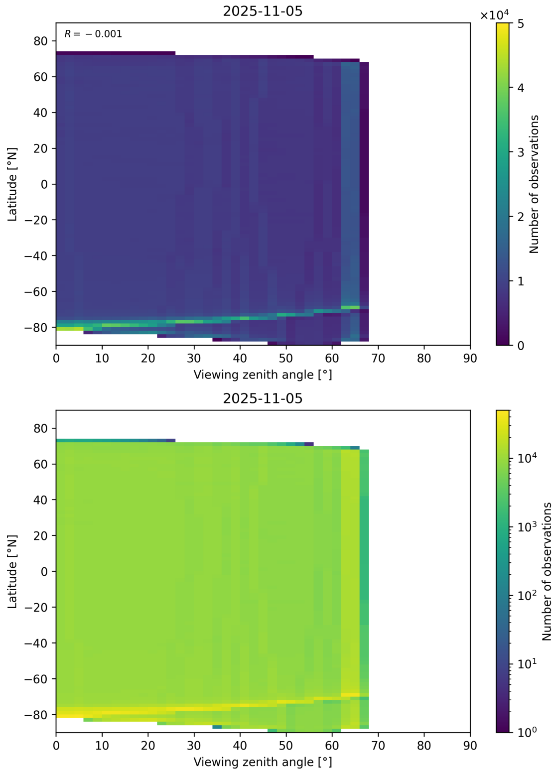
Figure 123: Scatter density plot of “Viewing zenith angle” against “Latitude” for 2025-11-04 to 2025-11-06.
