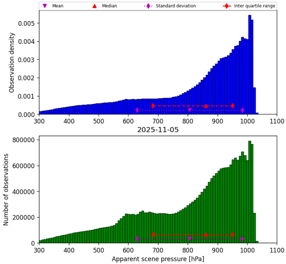
Figure 36: Histogram of “Apparent scene pressure” for 2025-11-04 to 2025-11-06
