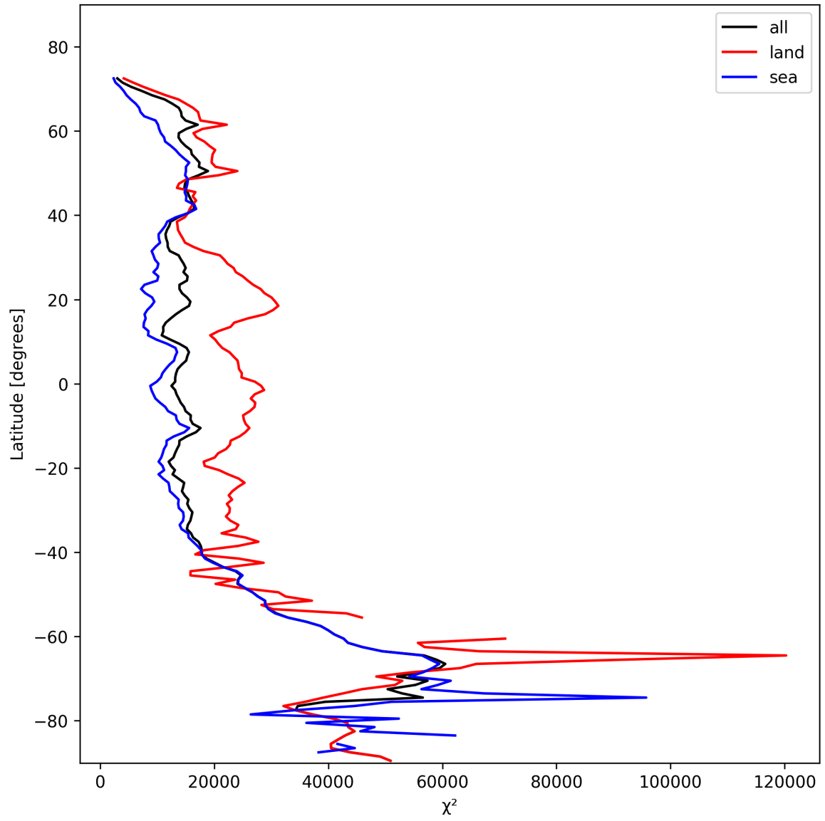
Figure 21: Zonal average of “ \chi^2 ” for 2025-11-04 to 2025-11-06.
