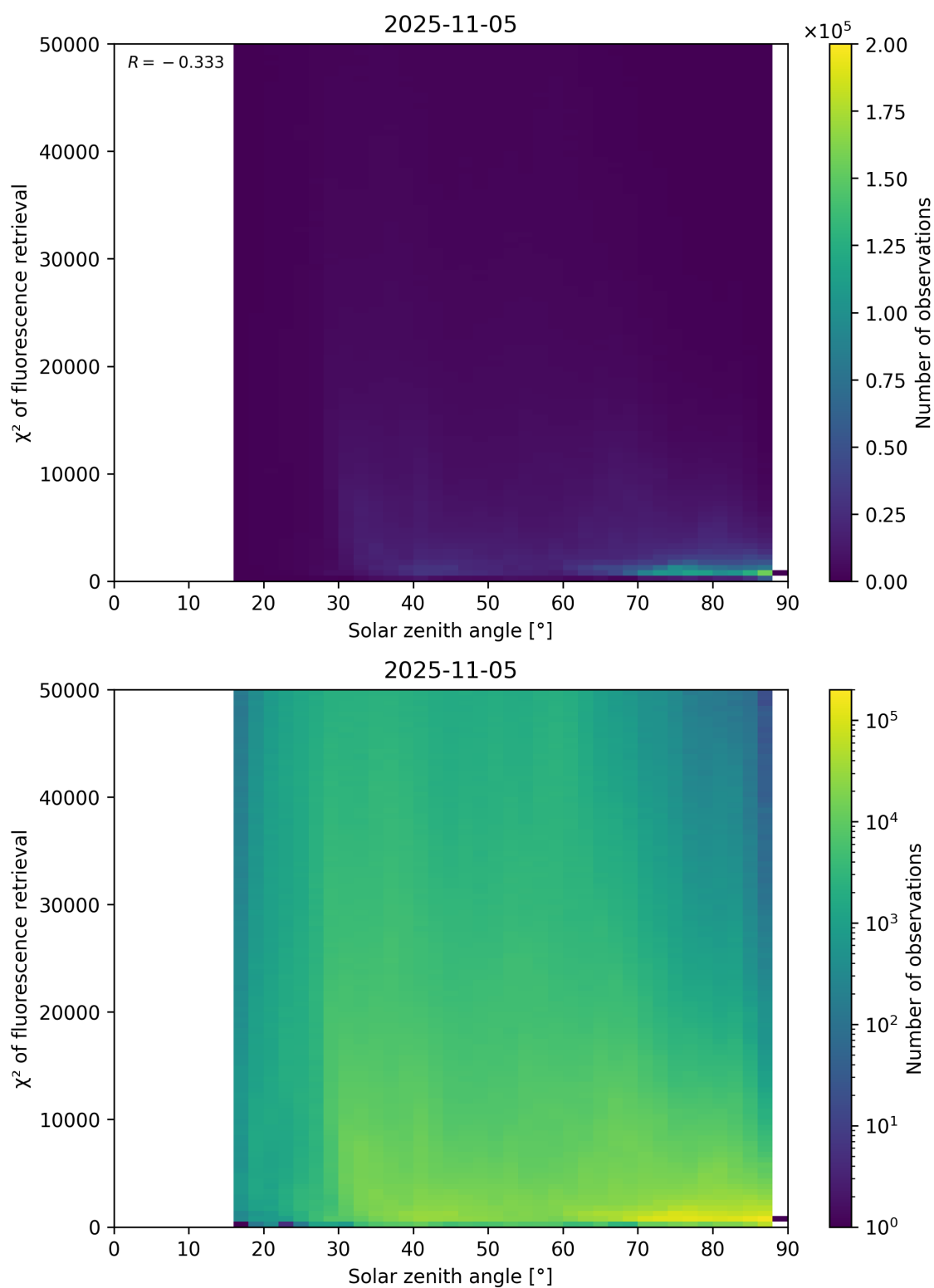
Figure 109: Scatter density plot of “Solar zenith angle” against “ \chi^2 of fluorescence retrieval” for 2025-11-04 to 2025-11-06.
