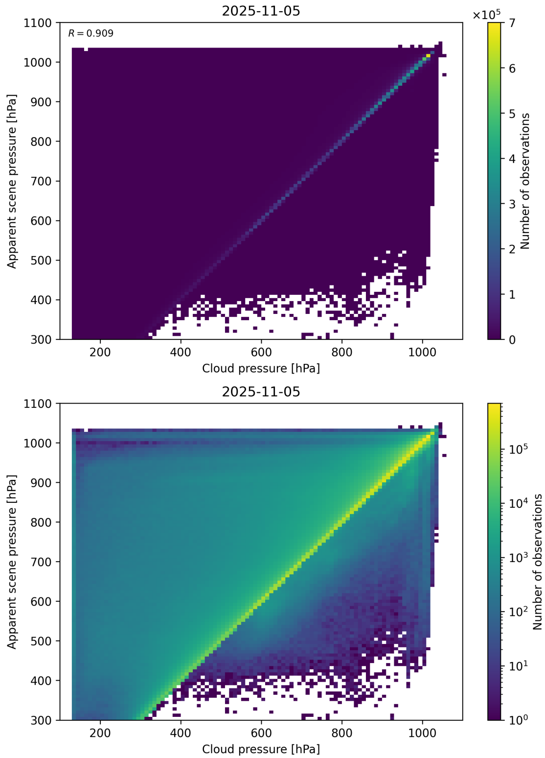
Figure 77: Scatter density plot of “Cloud pressure” against “Apparent scene pressure” for 2025-11-04 to 2025-11-06.
