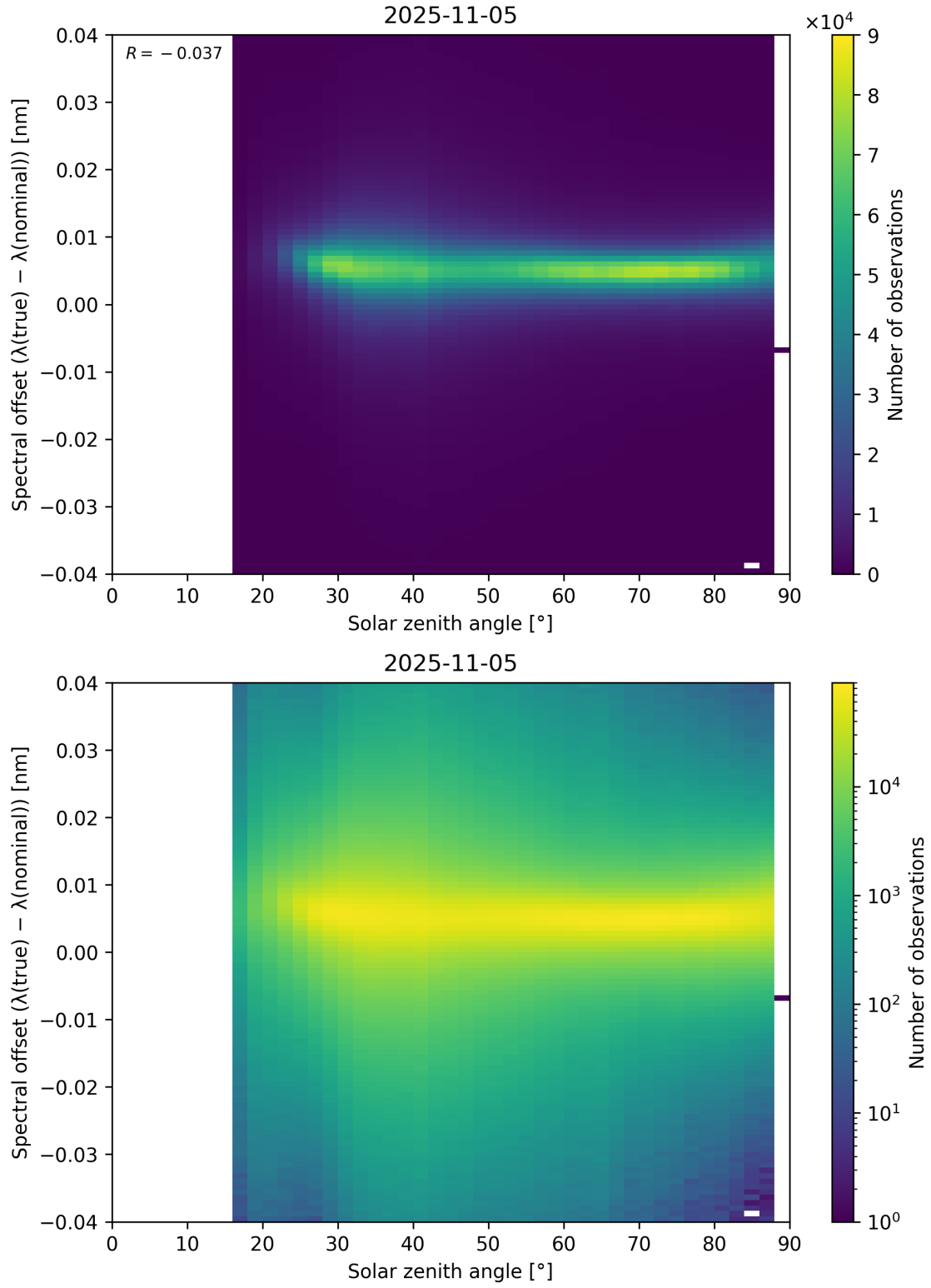
Figure 117: Scatter density plot of “Solar zenith angle” against “Spectral offset ( \lambda_{\text{true}} - \lambda_{\text{nominal}} )” for 2025-11-04 to 2025-11-06.
