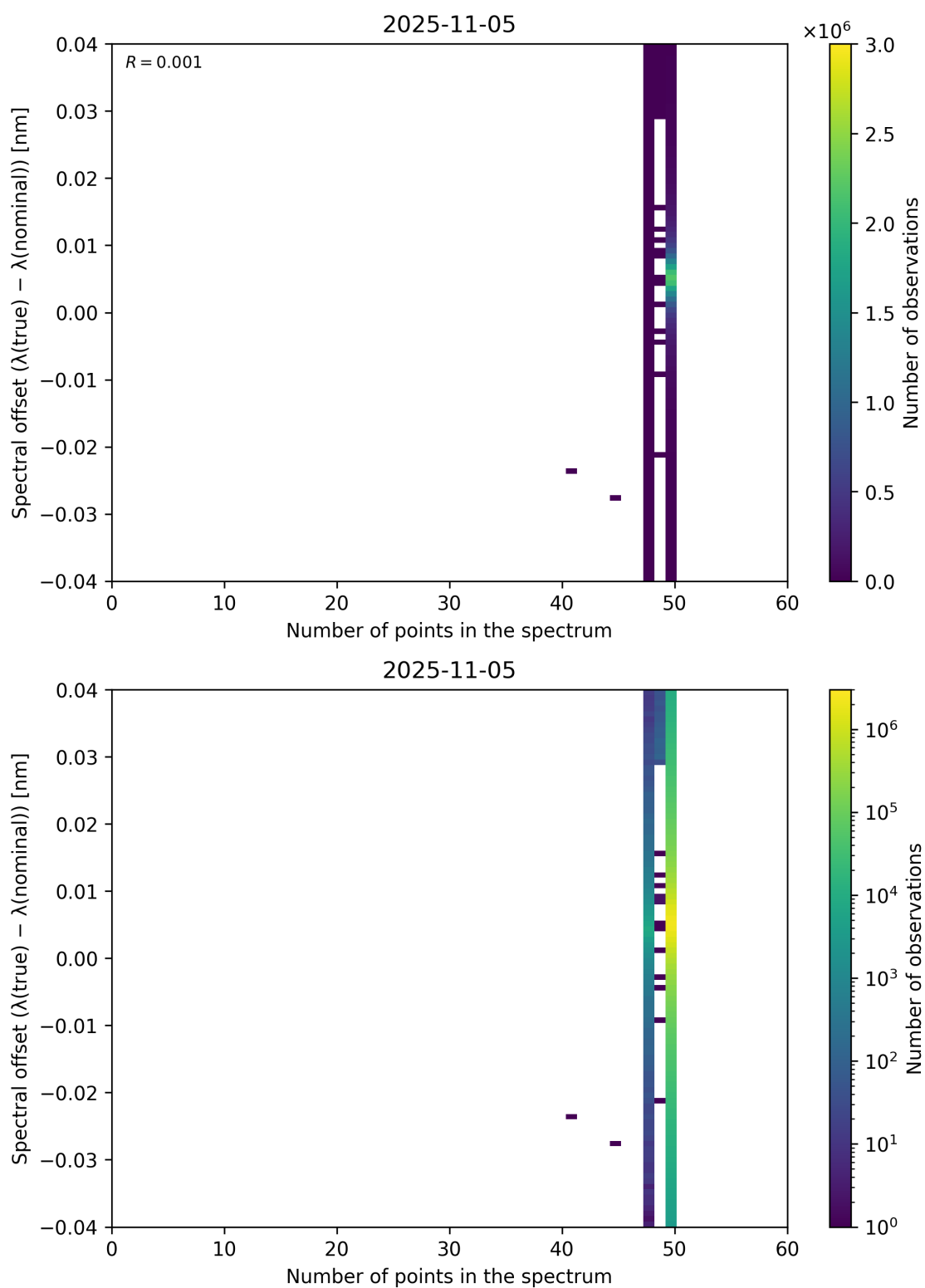
Figure 101: Scatter density plot of “Number of points in the spectrum” against “Spectral offset ( \lambda_{\text{true}} - \lambda_{\text{nominal}} )” for 2025-11-04 to 2025-11-06.
