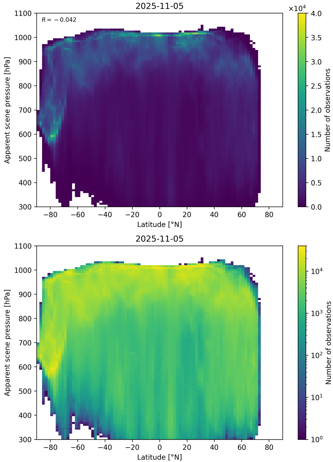
Figure 88: Scatter density plot of “Latitude” against “Apparent scene pressure” for 2025-11-04 to 2025-11-06.
