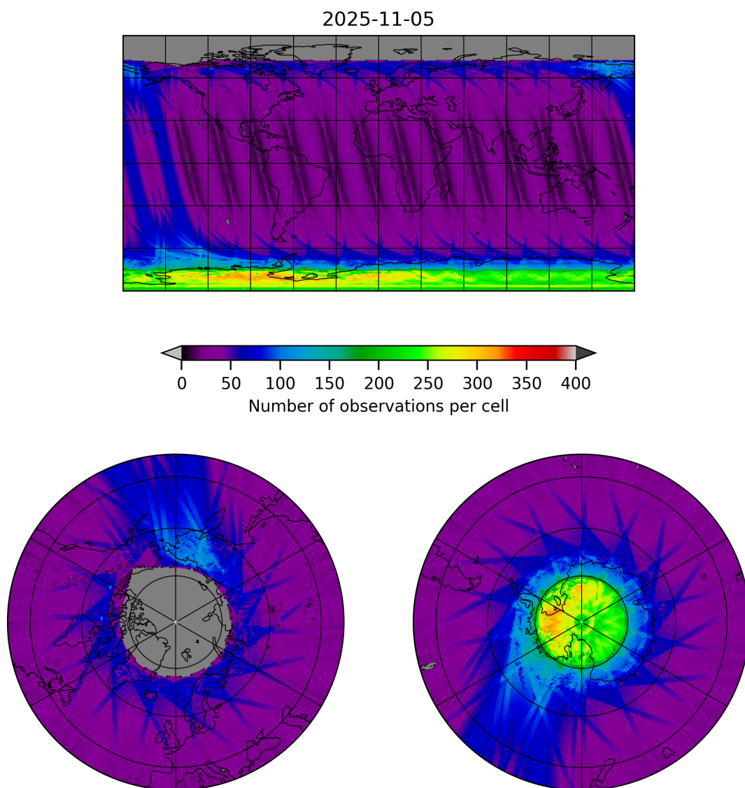
Figure 11: Map of the number of observations for 2025-11-04 to 2025-11-06
