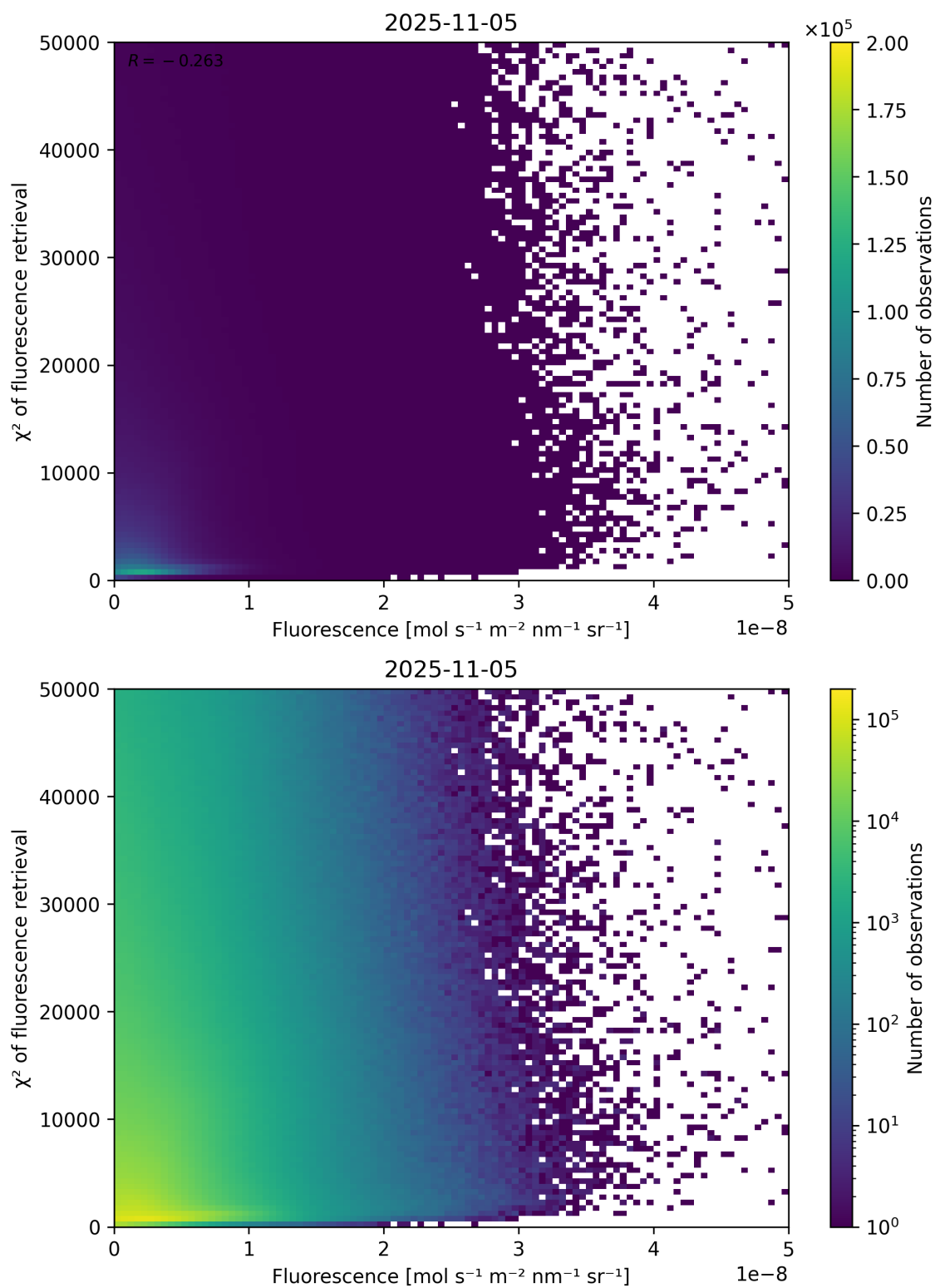
Figure 85: Scatter density plot of “Fluorescence” against “ \chi^2 of fluorescence retrieval” for 2025-11-04 to 2025-11-06.
