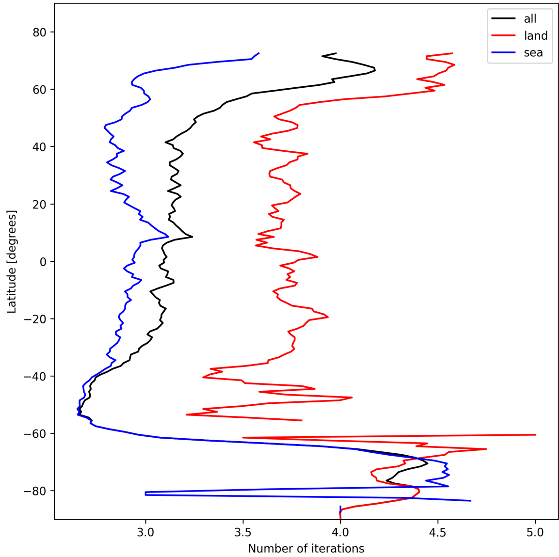
Figure 22: Zonal average of “Number of iterations” for 2025-11-04 to 2025-11-06.
