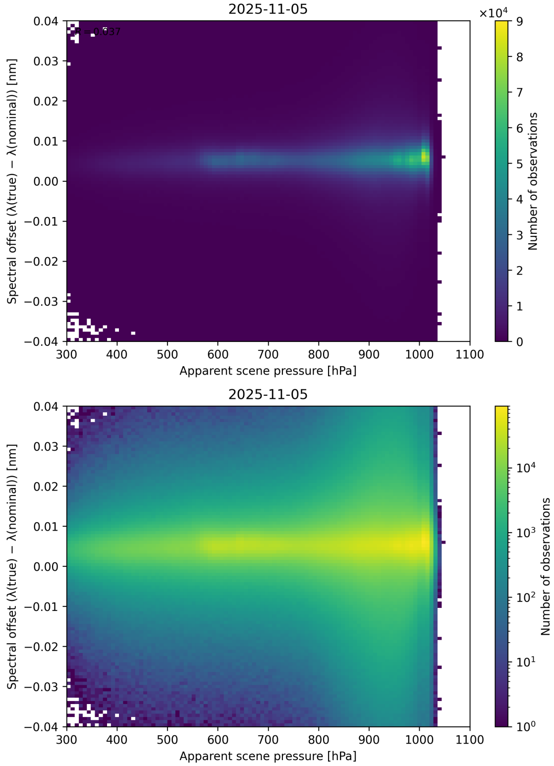
Figure 67: Scatter density plot of “Apparent scene pressure” against “Spectral offset ( \lambda_{\text{true}} - \lambda_{\text{nominal}} )” for 2025-11-04 to 2025-11-06.
