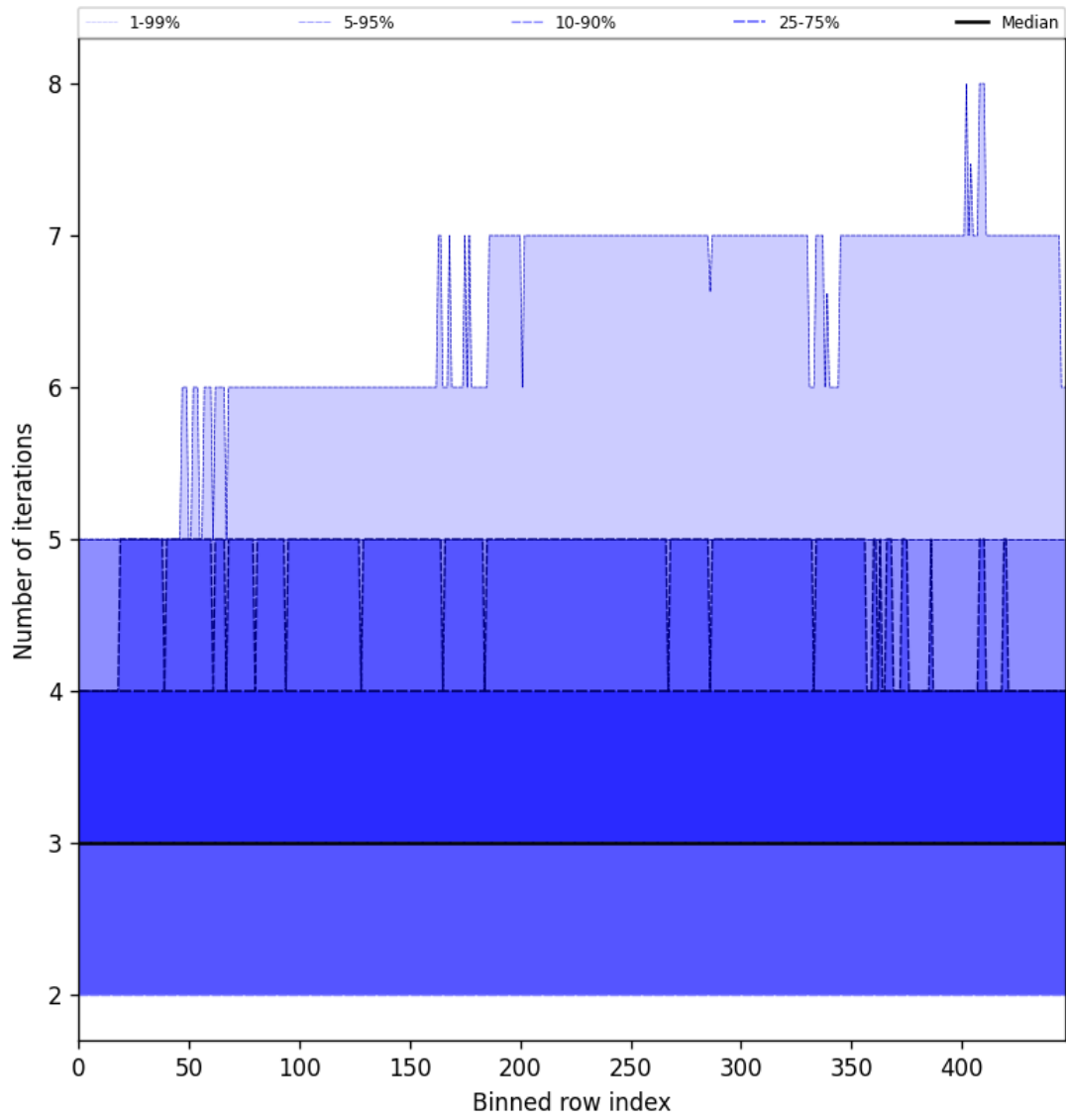
Figure 56: Along track statistics of “Number of iterations” for 2025-11-04 to 2025-11-06
