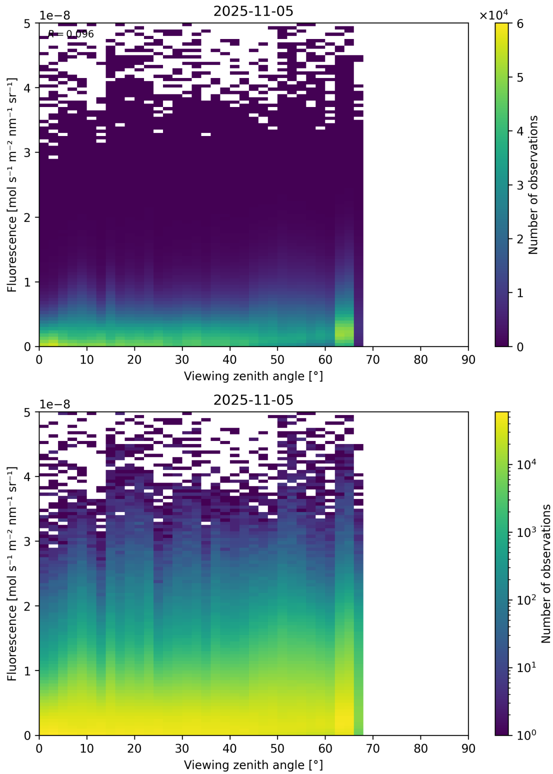
Figure 122: Scatter density plot of “Viewing zenith angle” against “Fluorescence” for 2025-11-04 to 2025-11-06.
