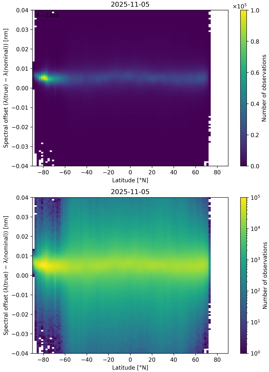
Figure 96: Scatter density plot of “Latitude” against “Spectral offset ( \lambda_{\text{true}} - \lambda_{\text{nominal}} )” for 2025-11-04 to 2025-11-06.
