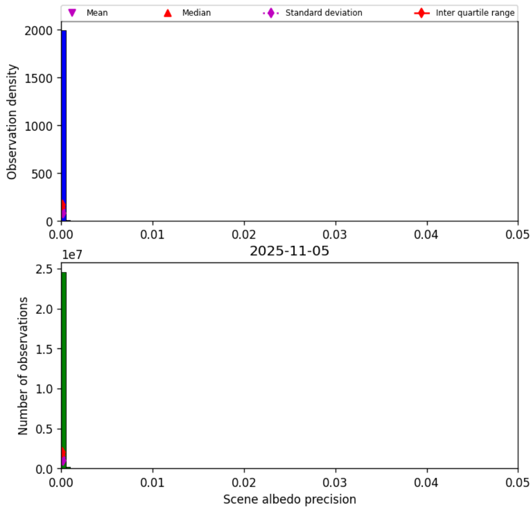
Figure 35: Histogram of “Scene albedo precision” for 2025-11-04 to 2025-11-06
