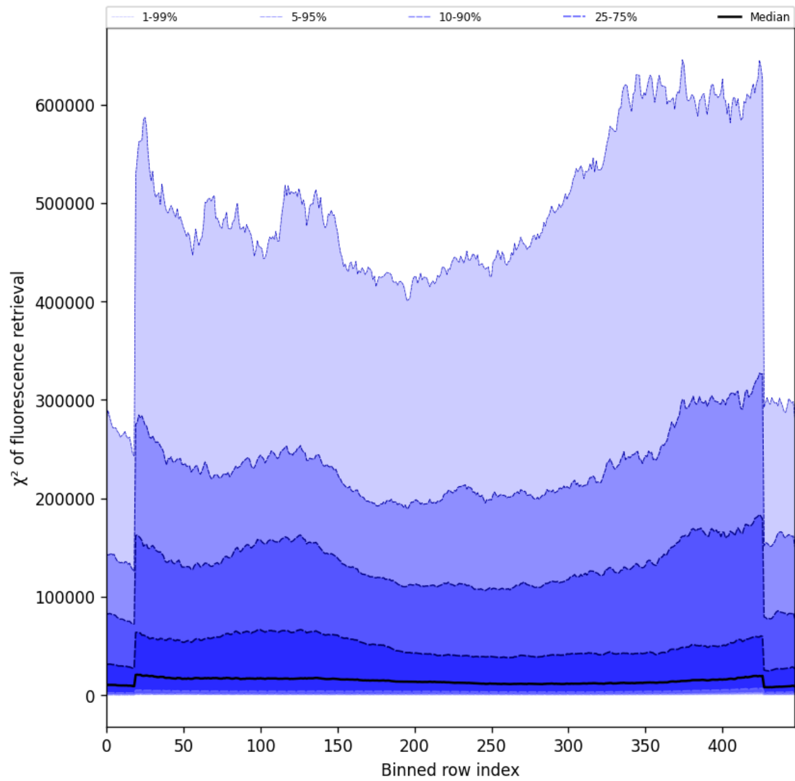
Figure 59: Along track statistics of “ \chi^2 of fluorescence retrieval” for 2025-11-04 to 2025-11-06
