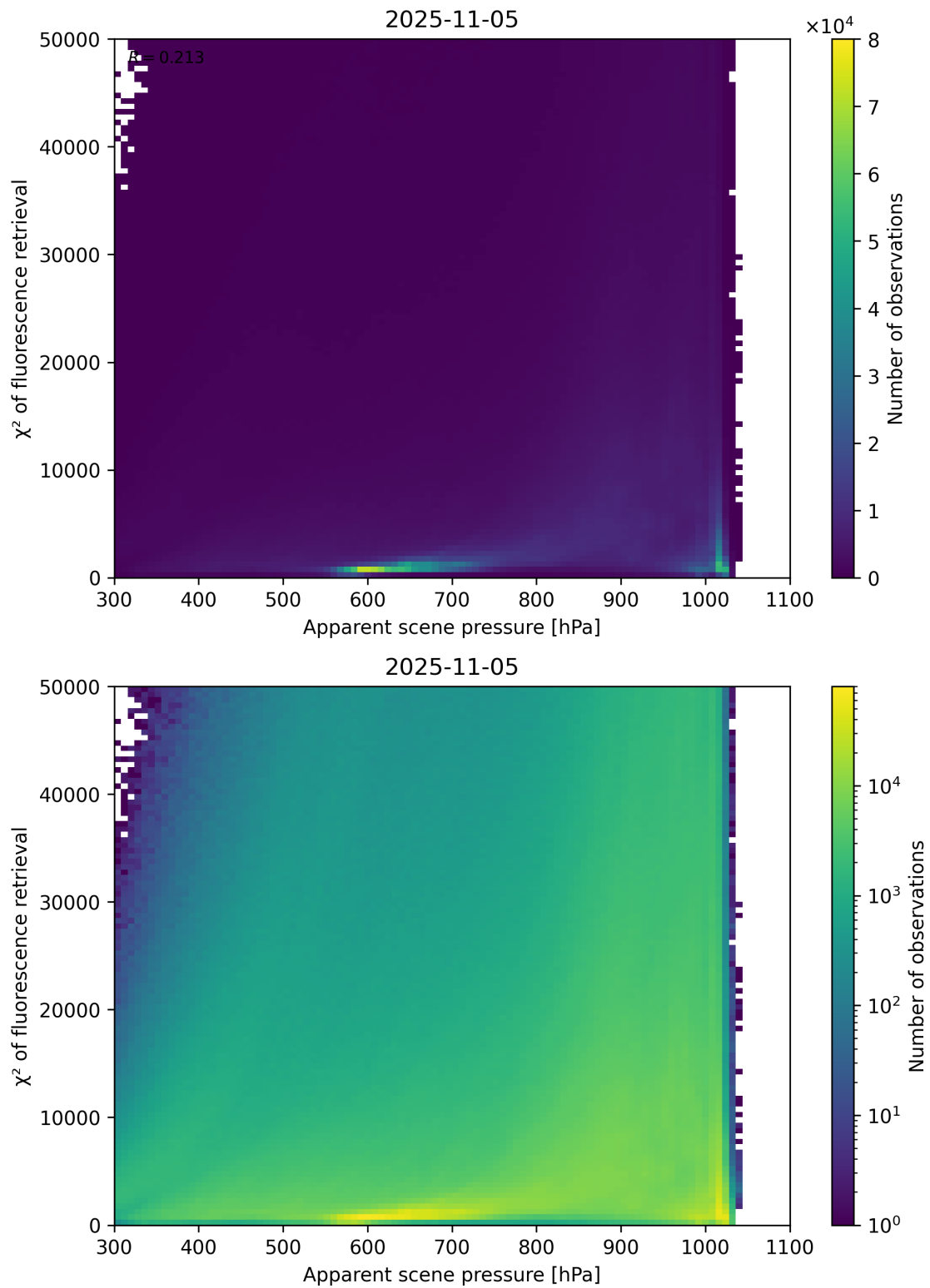
Figure 63: Scatter density plot of “Apparent scene pressure” against “ \chi^2 of fluorescence retrieval” for 2025-11-04 to 2025-11-06.
