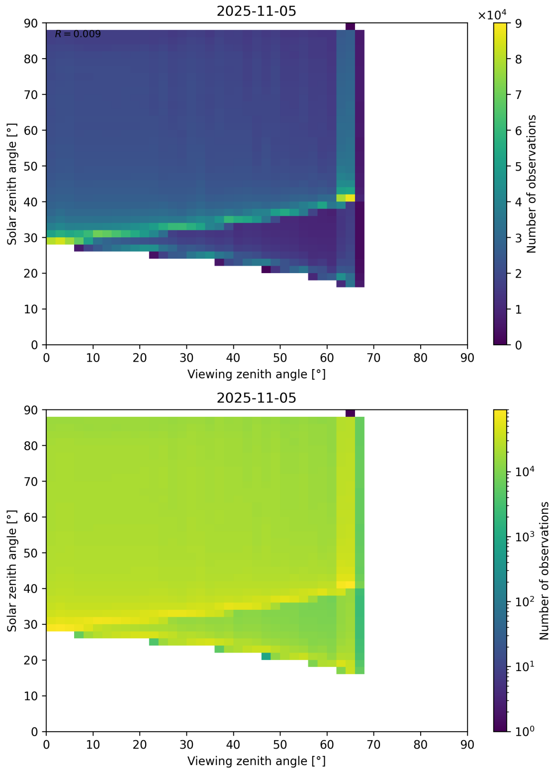
Figure 127: Scatter density plot of “Viewing zenith angle” against “Solar zenith angle” for 2025-11-04 to 2025-11-06.
