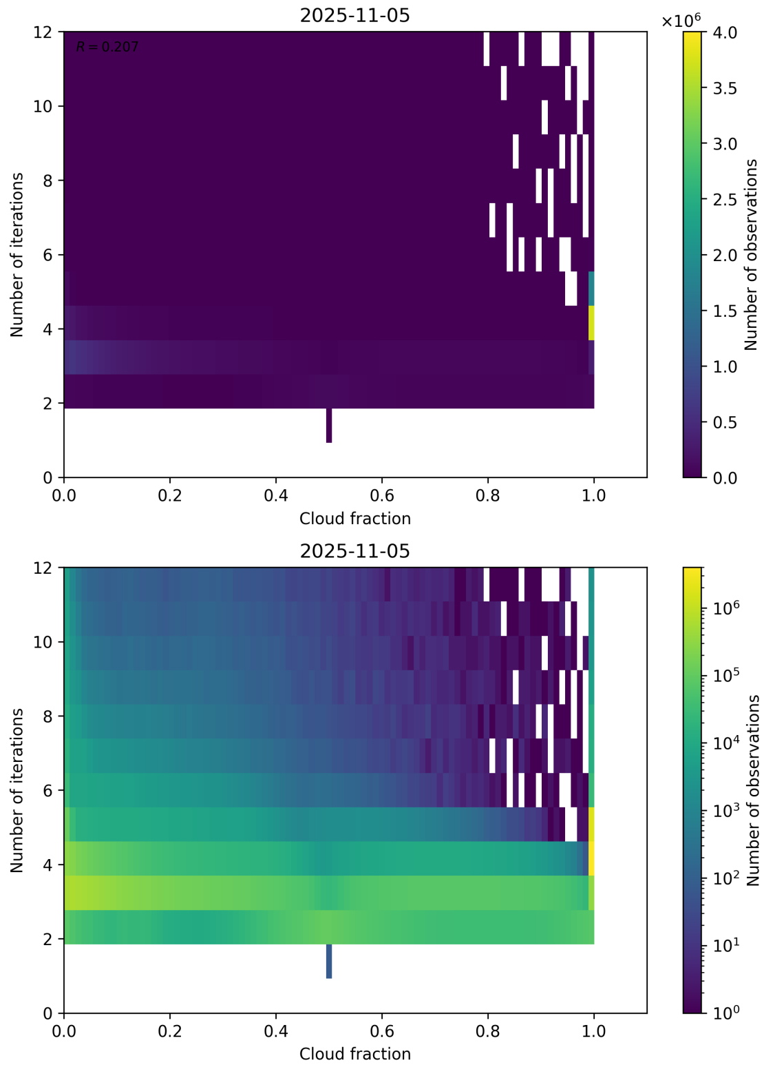
Figure 73: Scatter density plot of “Cloud fraction” against “Number of iterations” for 2025-11-04 to 2025-11-06.
