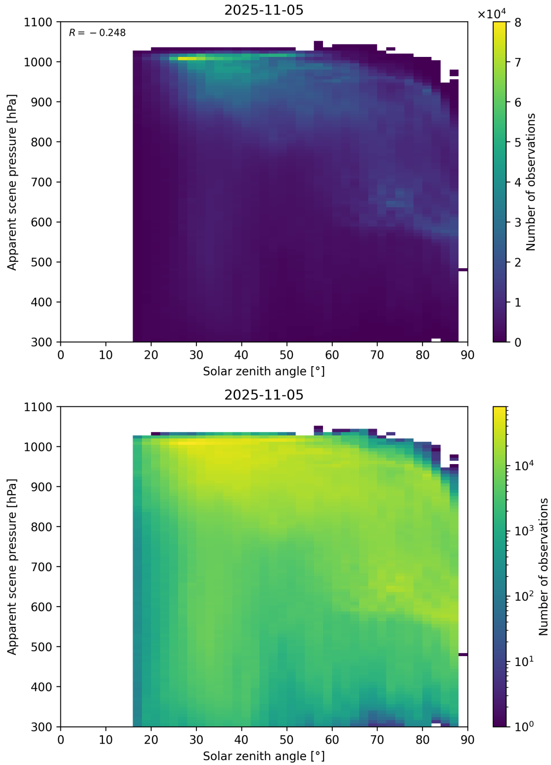
Figure 108: Scatter density plot of “Solar zenith angle” against “Apparent scene pressure” for 2025-11-04 to 2025-11-06.
