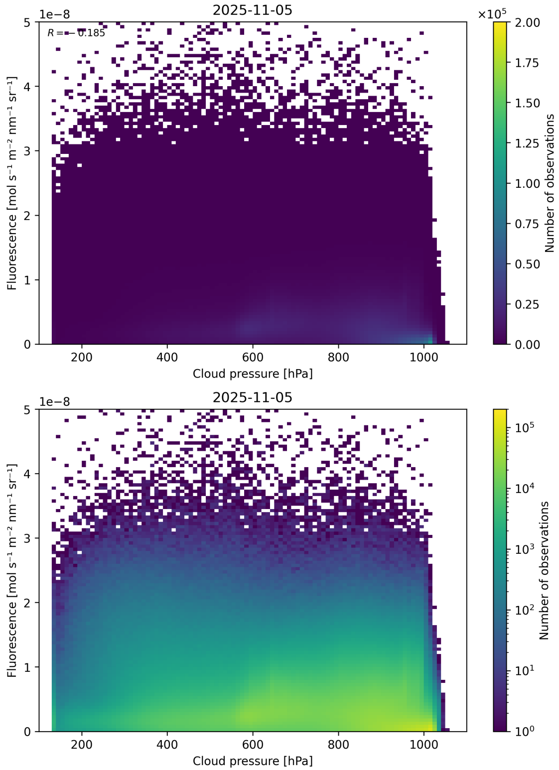
Figure 80: Scatter density plot of “Cloud pressure” against “Fluorescence” for 2025-11-04 to 2025-11-06.
