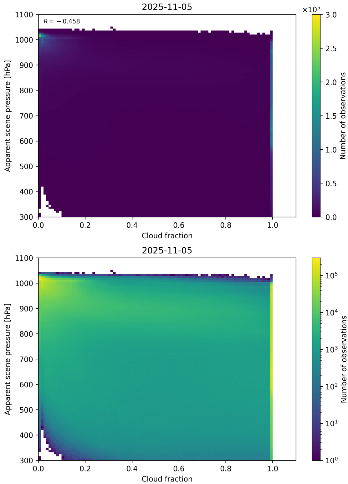
Figure 70: Scatter density plot of “Cloud fraction” against “Apparent scene pressure” for 2025-11-04 to 2025-11-06.
