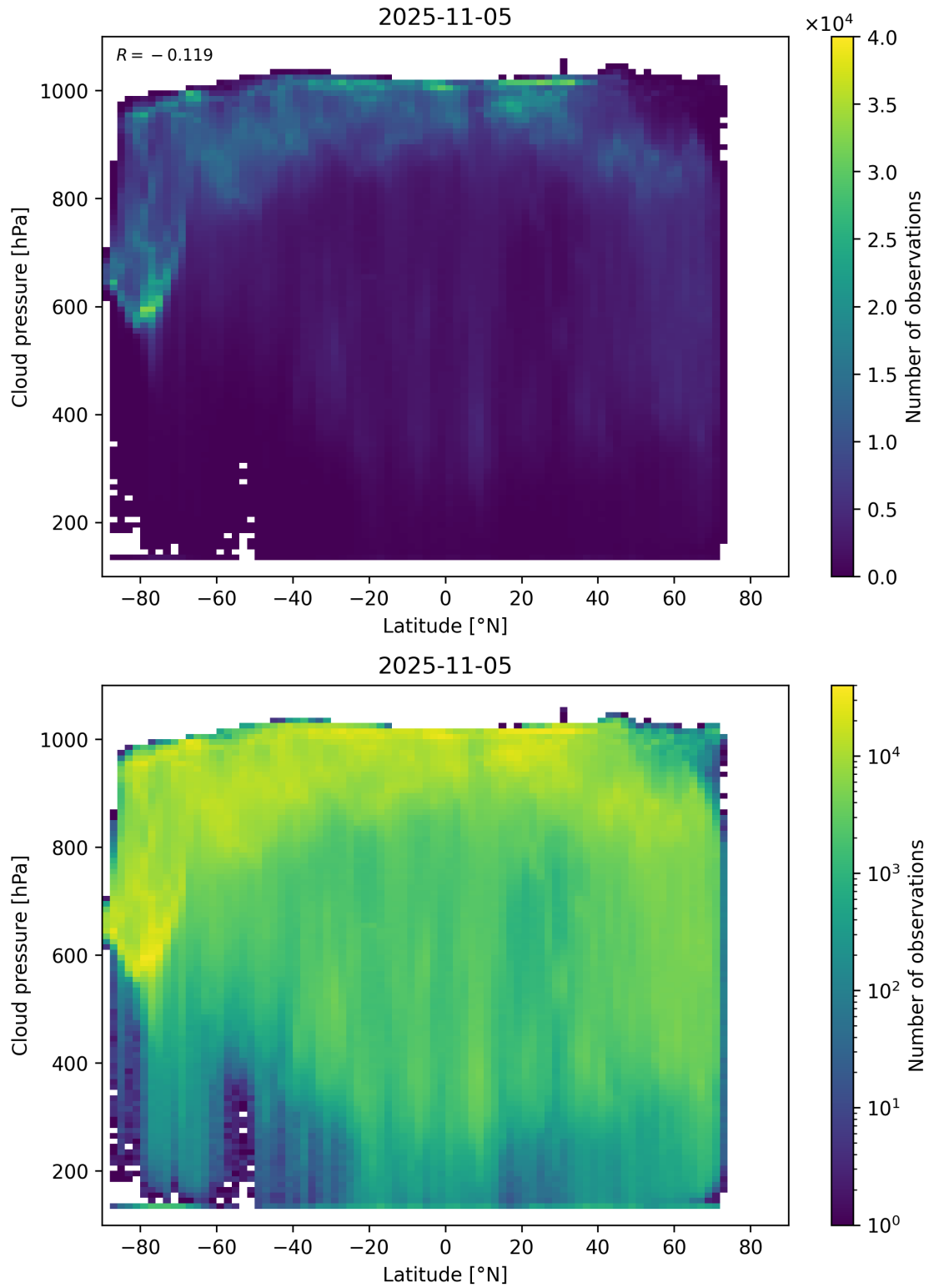
Figure 91: Scatter density plot of “Latitude” against “Cloud pressure” for 2025-11-04 to 2025-11-06.
