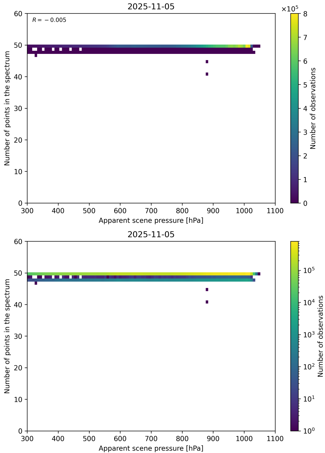
Figure 66: Scatter density plot of “Apparent scene pressure” against “Number of points in the spectrum” for 2025-11-04 to 2025-11-06.
