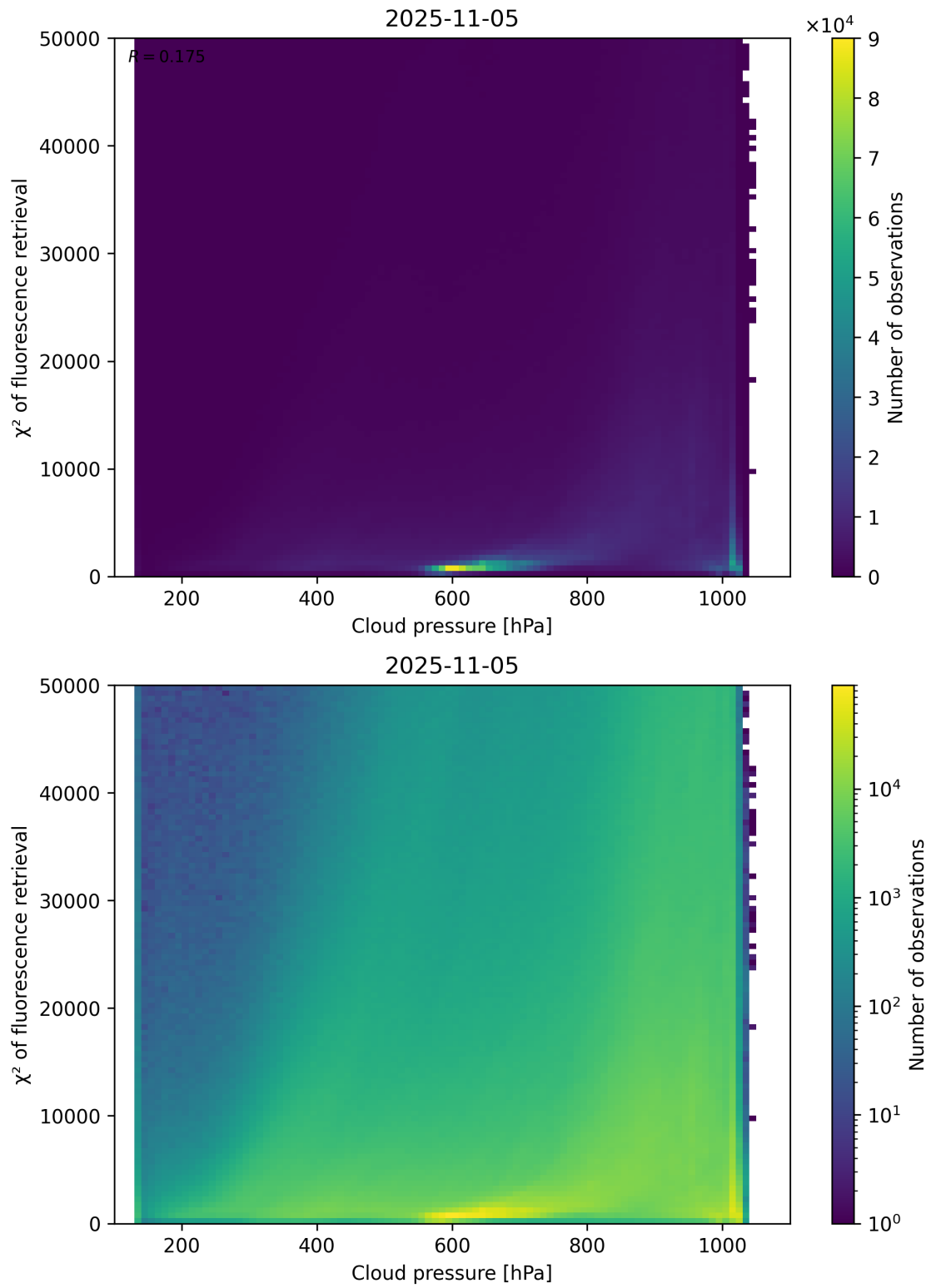
Figure 78: Scatter density plot of “Cloud pressure” against “ \chi^2 of fluorescence retrieval” for 2025-11-04 to 2025-11-06.
