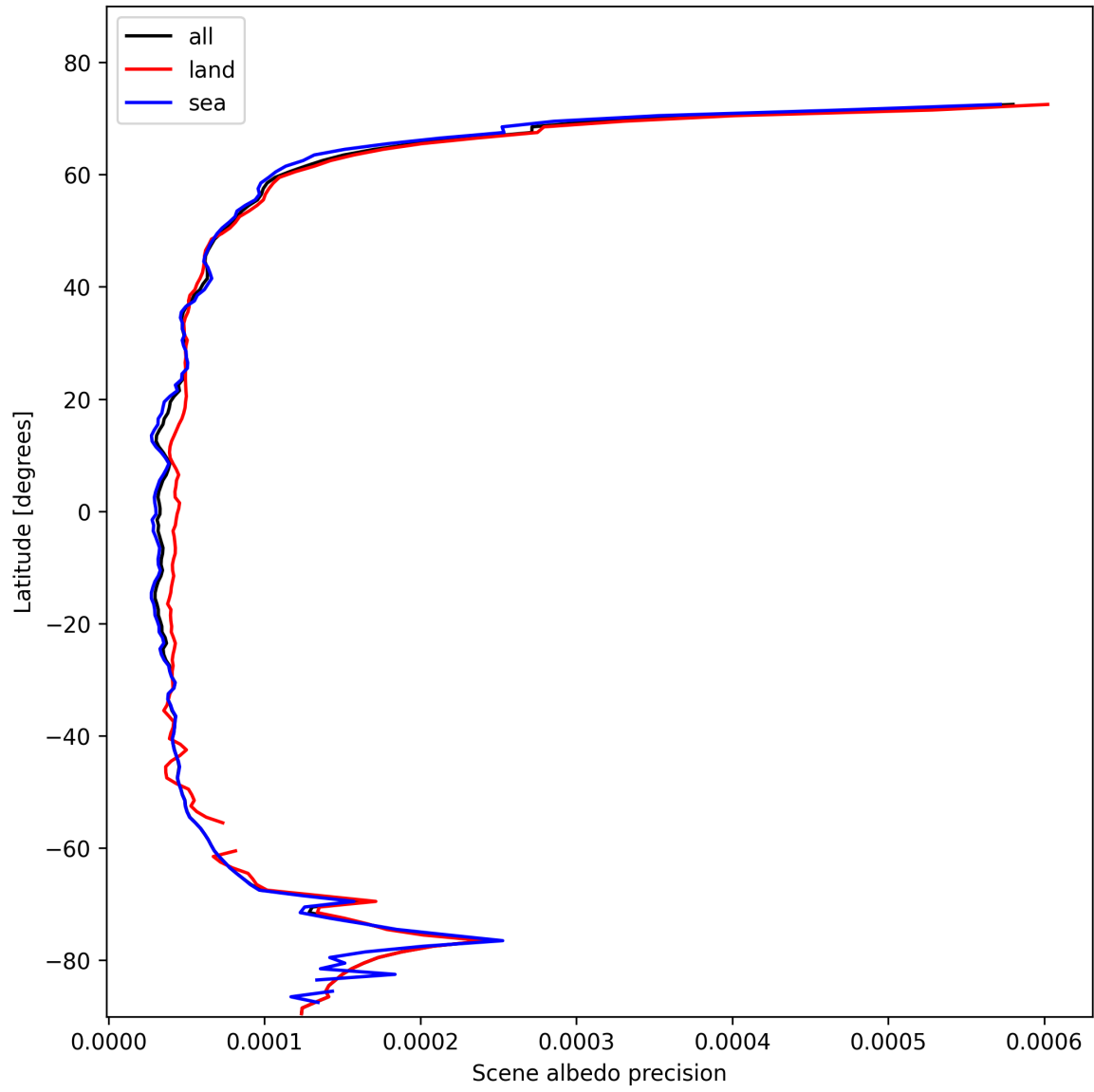
Figure 18: Zonal average of “Scene albedo precision” for 2025-11-04 to 2025-11-06.
