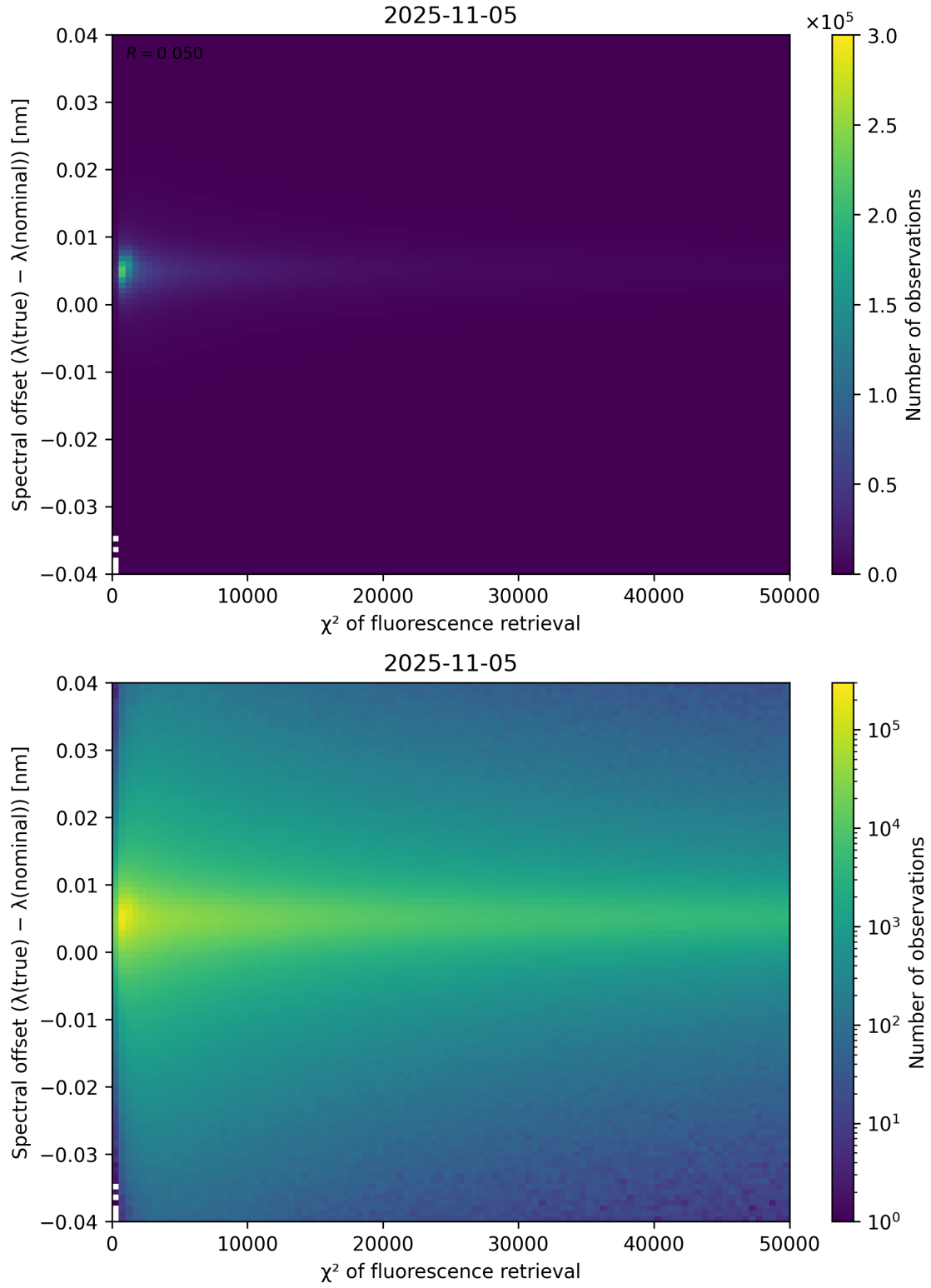
Figure 69: Scatter density plot of “ \chi^2 of fluorescence retrieval” against “Spectral offset ( \lambda_{\text{true}} - \lambda_{\text{nominal}} )” for 2025-11-04 to 2025-11-06.
