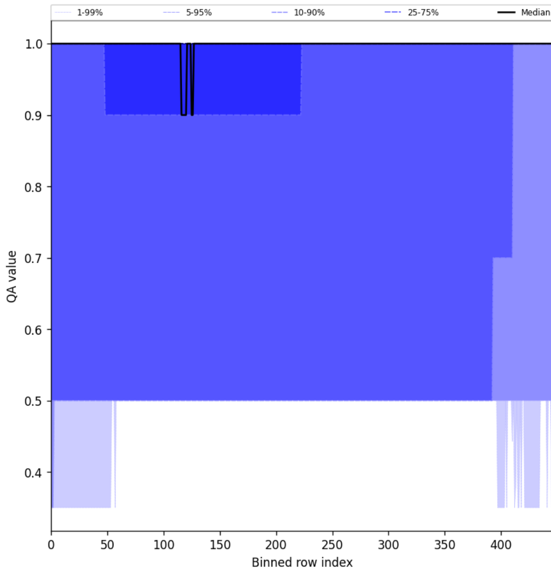
Figure 46: Along track statistics of “QA value” for 2025-11-04 to 2025-11-06
