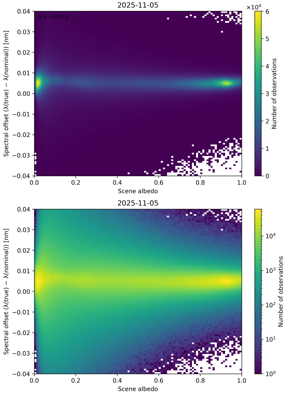
Figure 107: Scatter density plot of “Scene albedo” against “Spectral offset ( \lambda_{\text{true}} - \lambda_{\text{nominal}} )” for 2025-11-04 to 2025-11-06.
