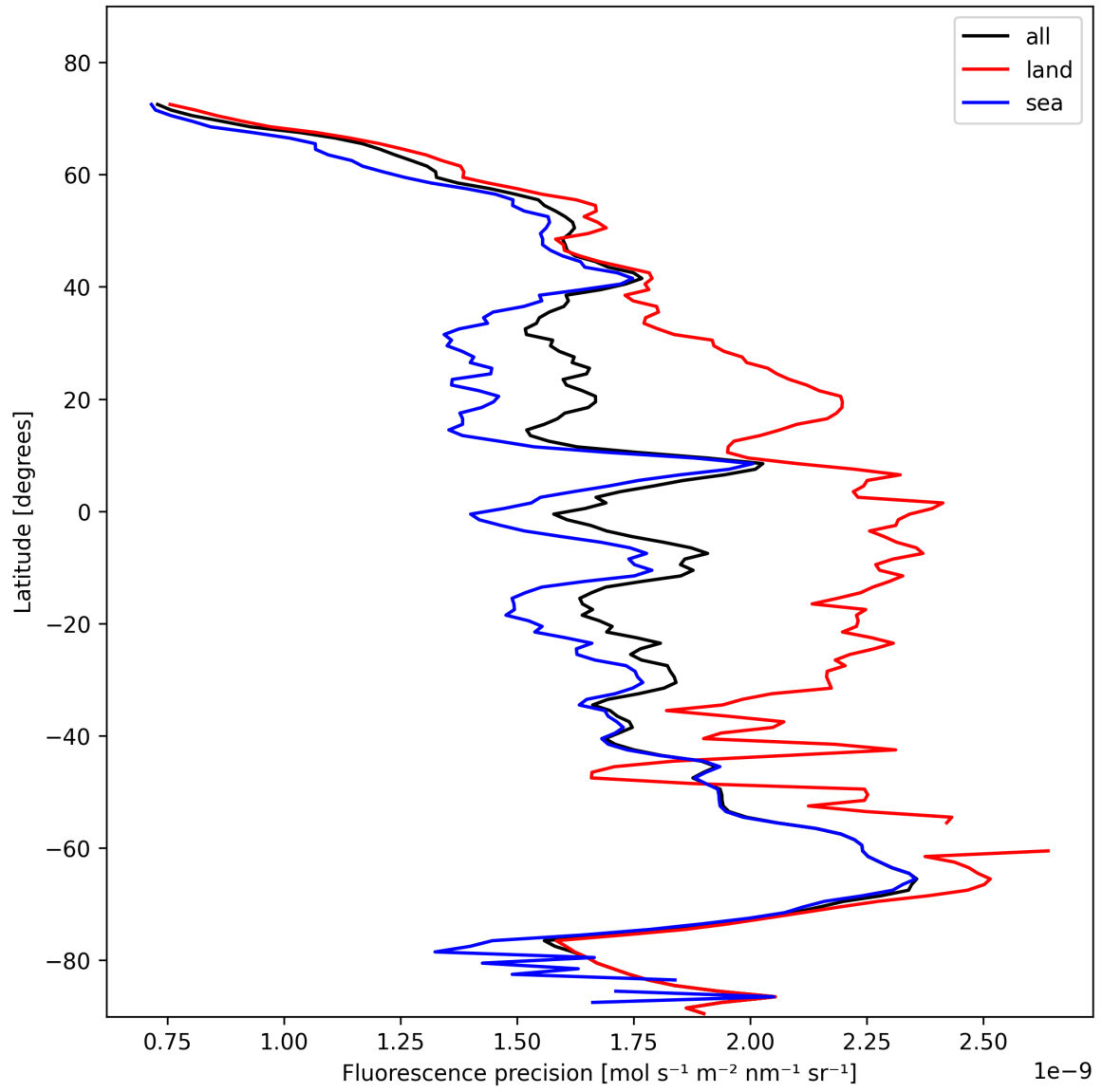
Figure 24: Zonal average of “Fluorescence precision” for 2025-11-04 to 2025-11-06.
