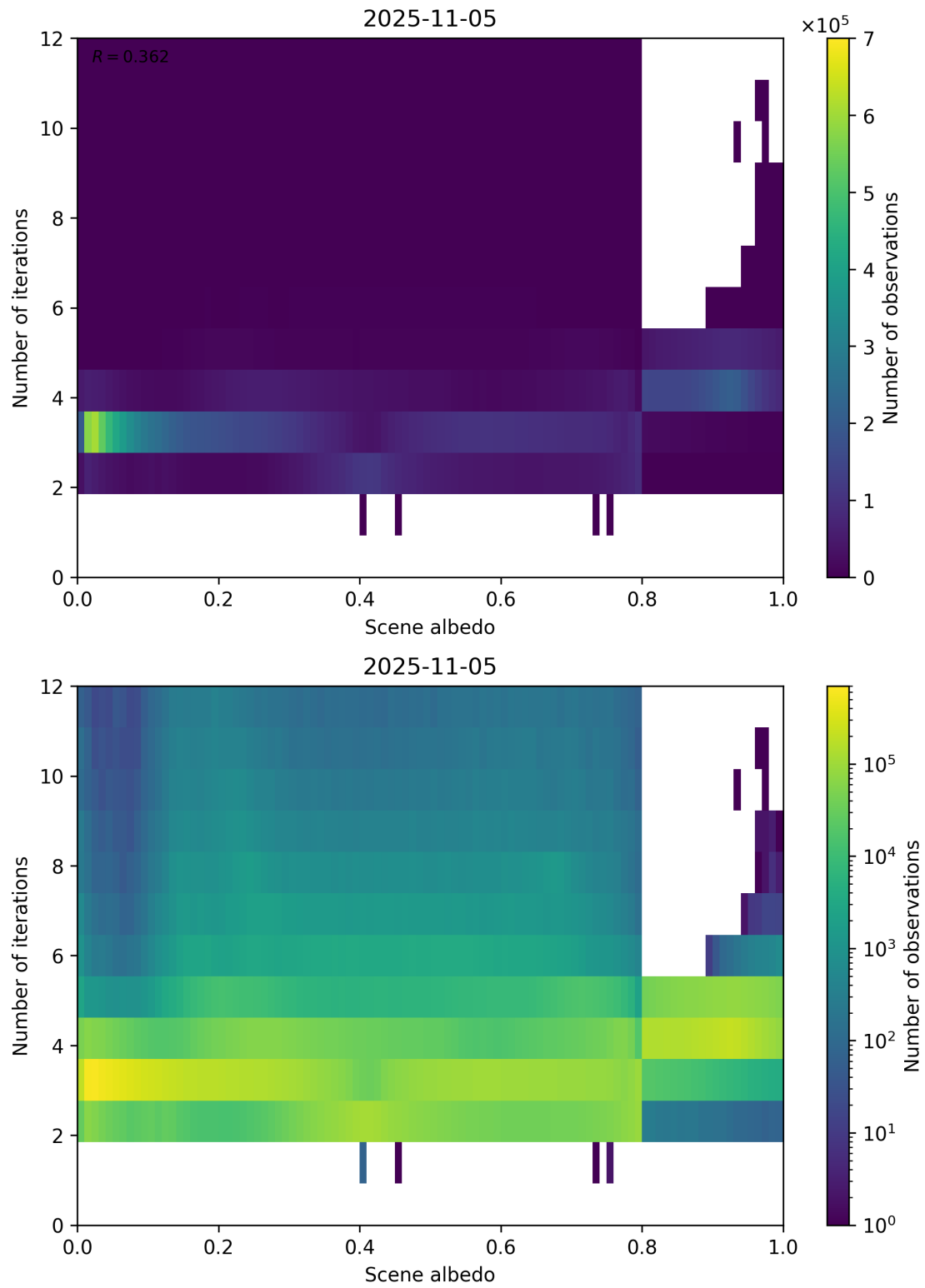
Figure 105: Scatter density plot of “Scene albedo” against “Number of iterations” for 2025-11-04 to 2025-11-06.
