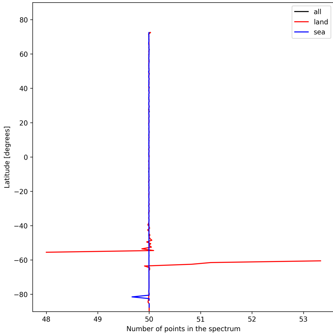
Figure 27: Zonal average of “Number of points in the spectrum” for 2025-11-04 to 2025-11-06.
