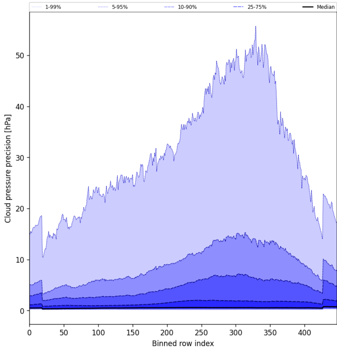
Figure 48: Along track statistics of “Cloud pressure precision” for 2025-11-04 to 2025-11-06
