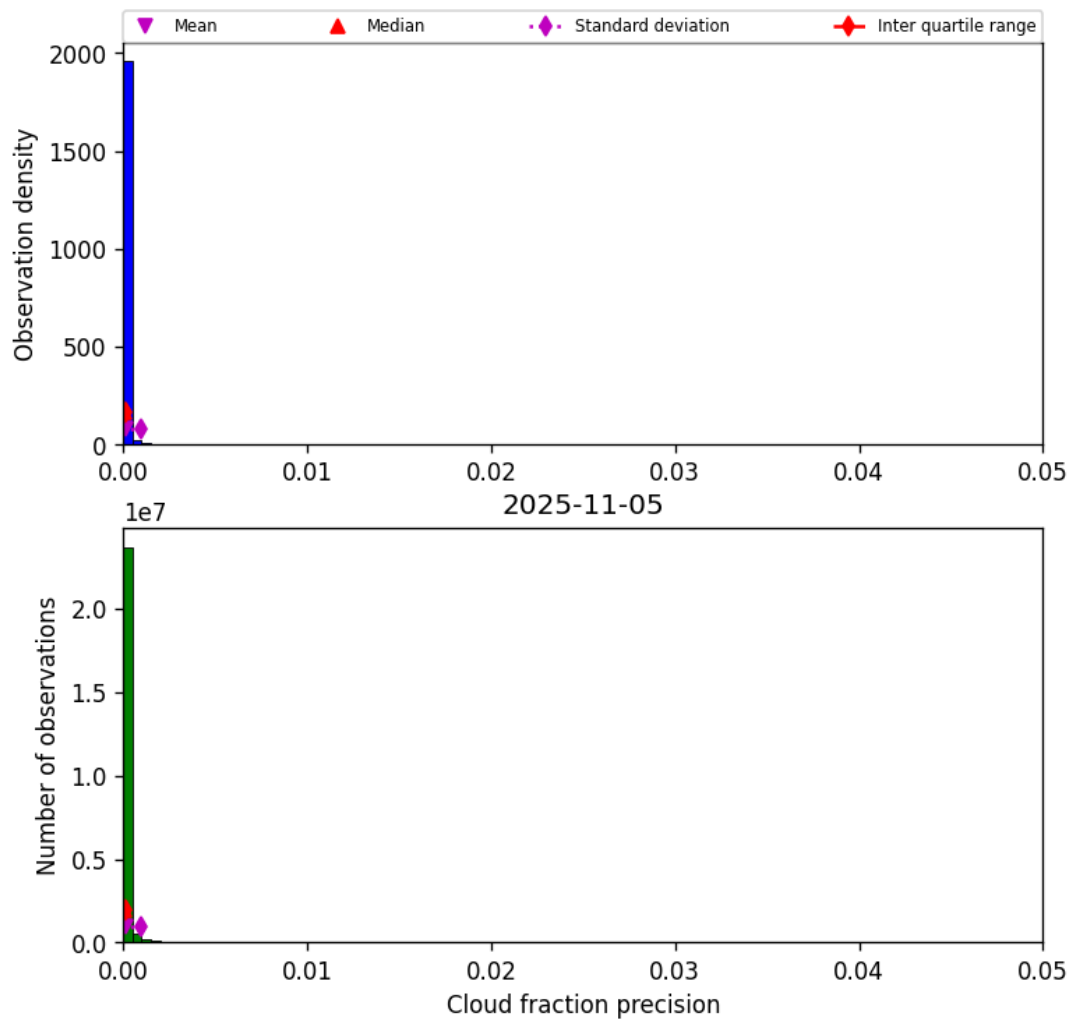
Figure 33: Histogram of “Cloud fraction precision” for 2025-11-04 to 2025-11-06
