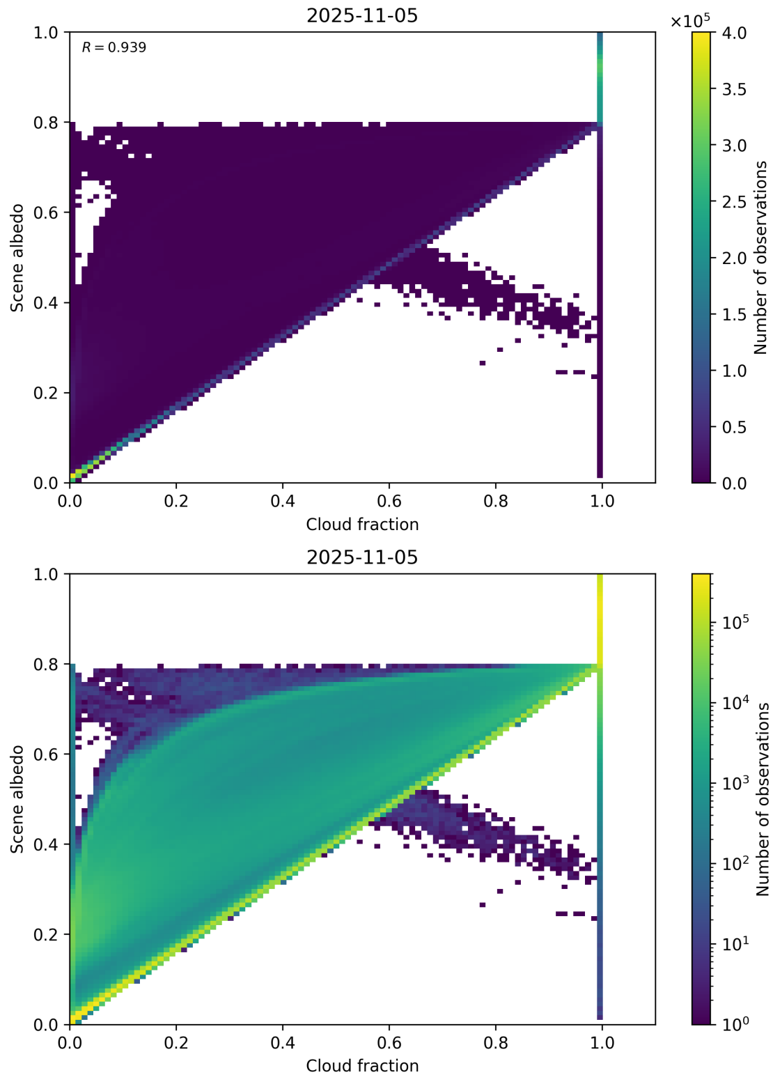
Figure 75: Scatter density plot of “Cloud fraction” against “Scene albedo” for 2025-11-04 to 2025-11-06.
