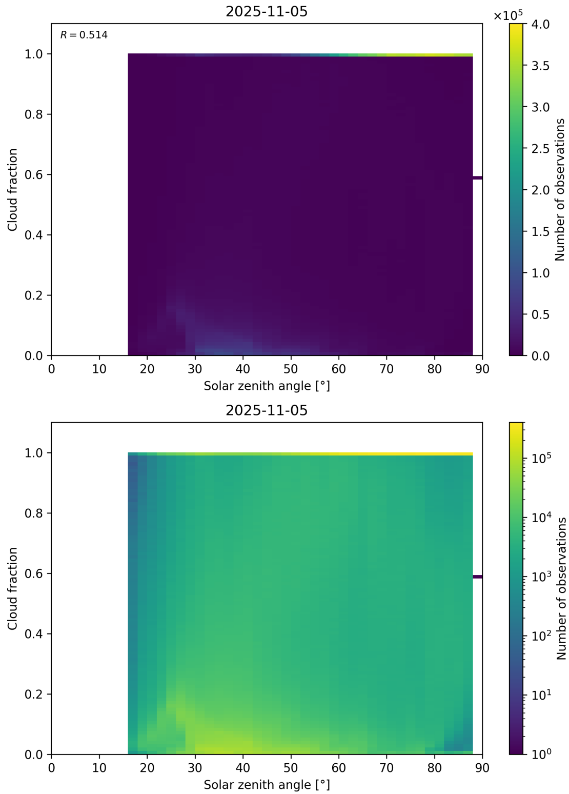
Figure 110: Scatter density plot of “Solar zenith angle” against “Cloud fraction” for 2025-11-04 to 2025-11-06.
