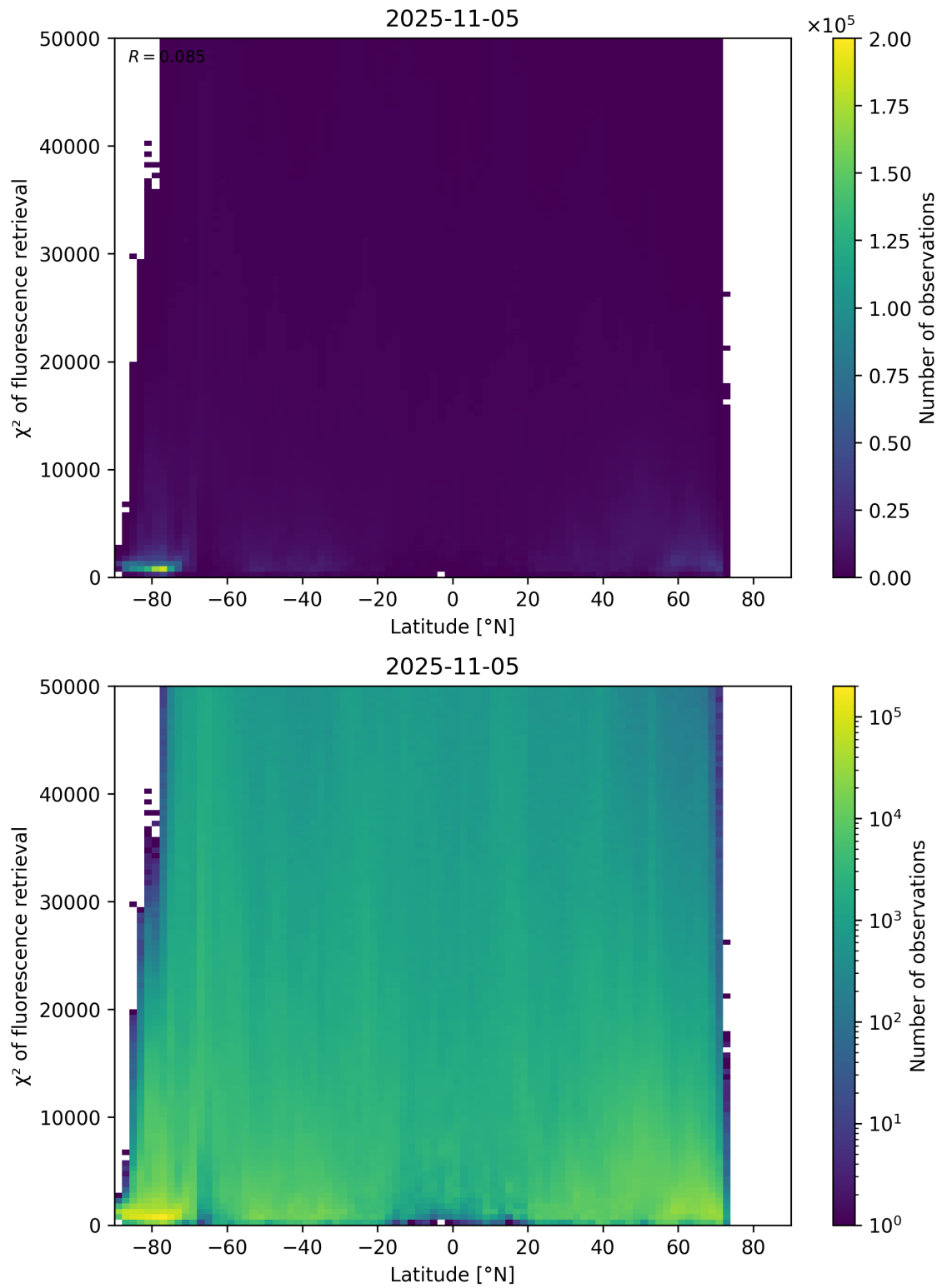
Figure 89: Scatter density plot of “Latitude” against “ \chi^2 of fluorescence retrieval” for 2025-11-04 to 2025-11-06.
