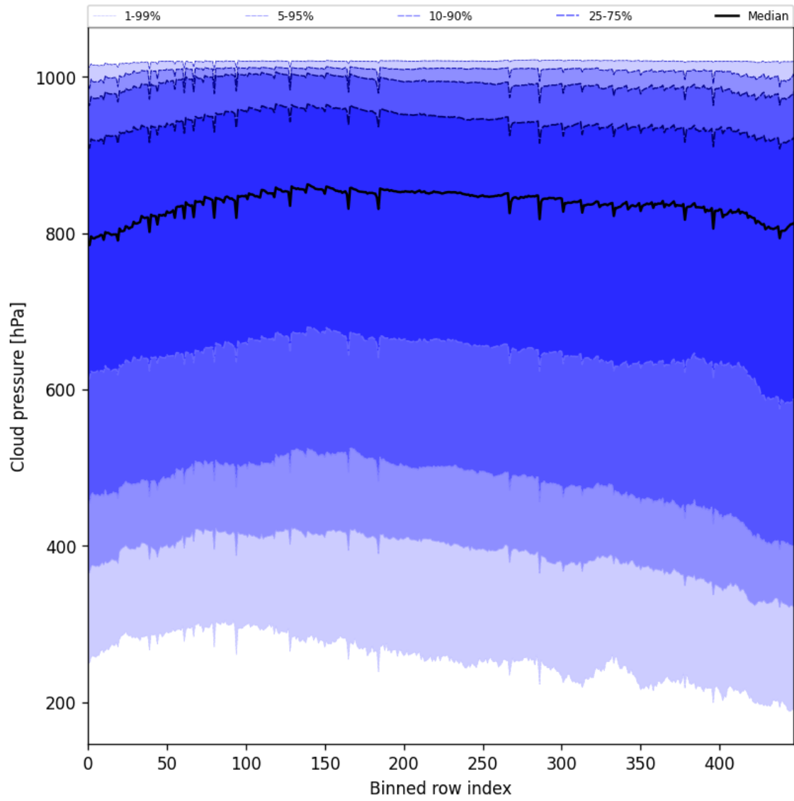
Figure 47: Along track statistics of “Cloud pressure” for 2025-11-04 to 2025-11-06
