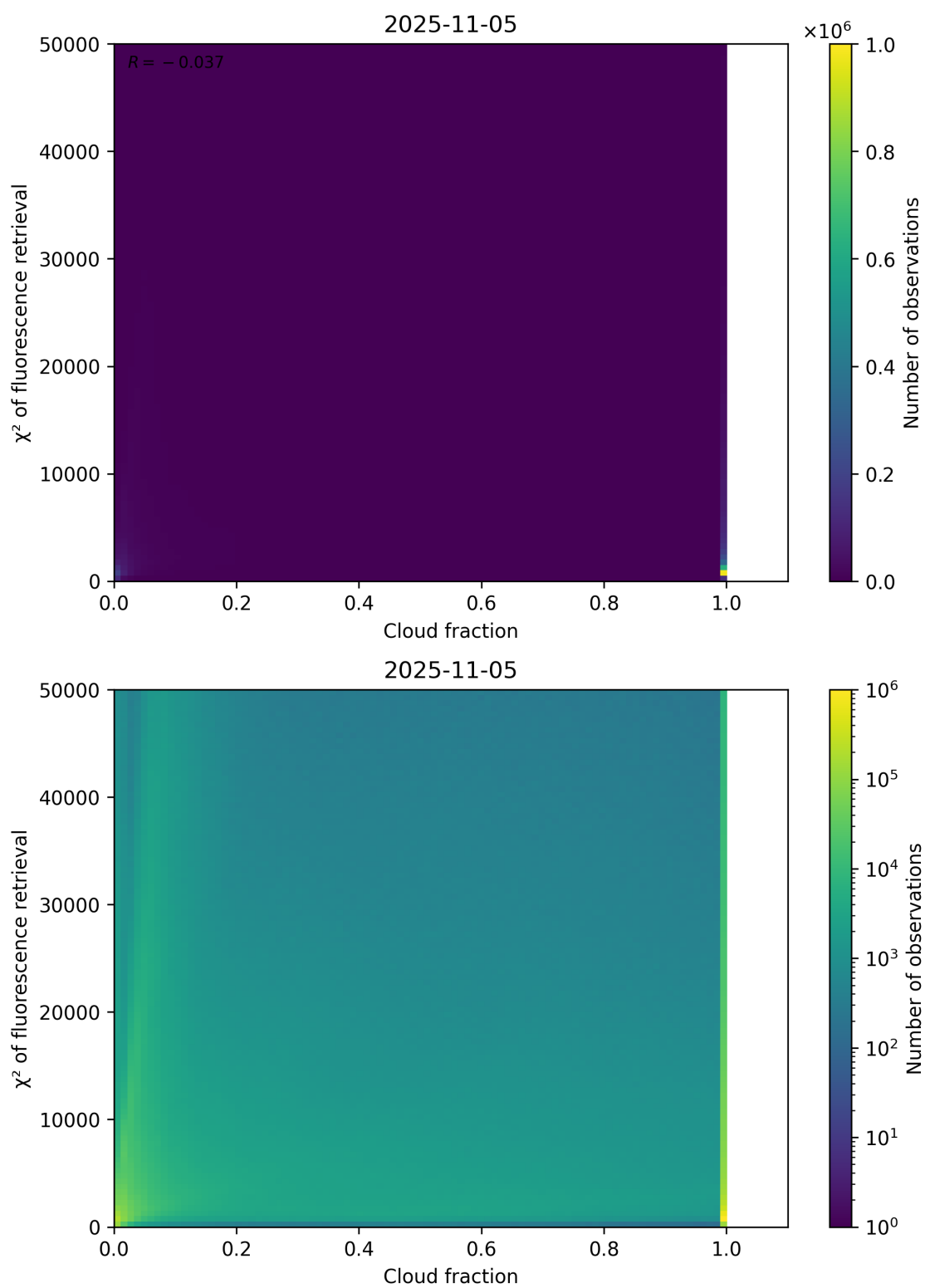
Figure 71: Scatter density plot of “Cloud fraction” against “ \chi^2 of fluorescence retrieval” for 2025-11-04 to 2025-11-06.
