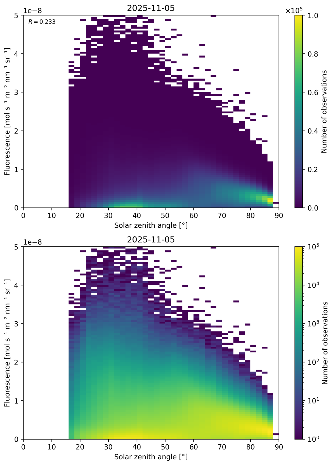
Figure 112: Scatter density plot of “Solar zenith angle” against “Fluorescence” for 2025-11-04 to 2025-11-06.
