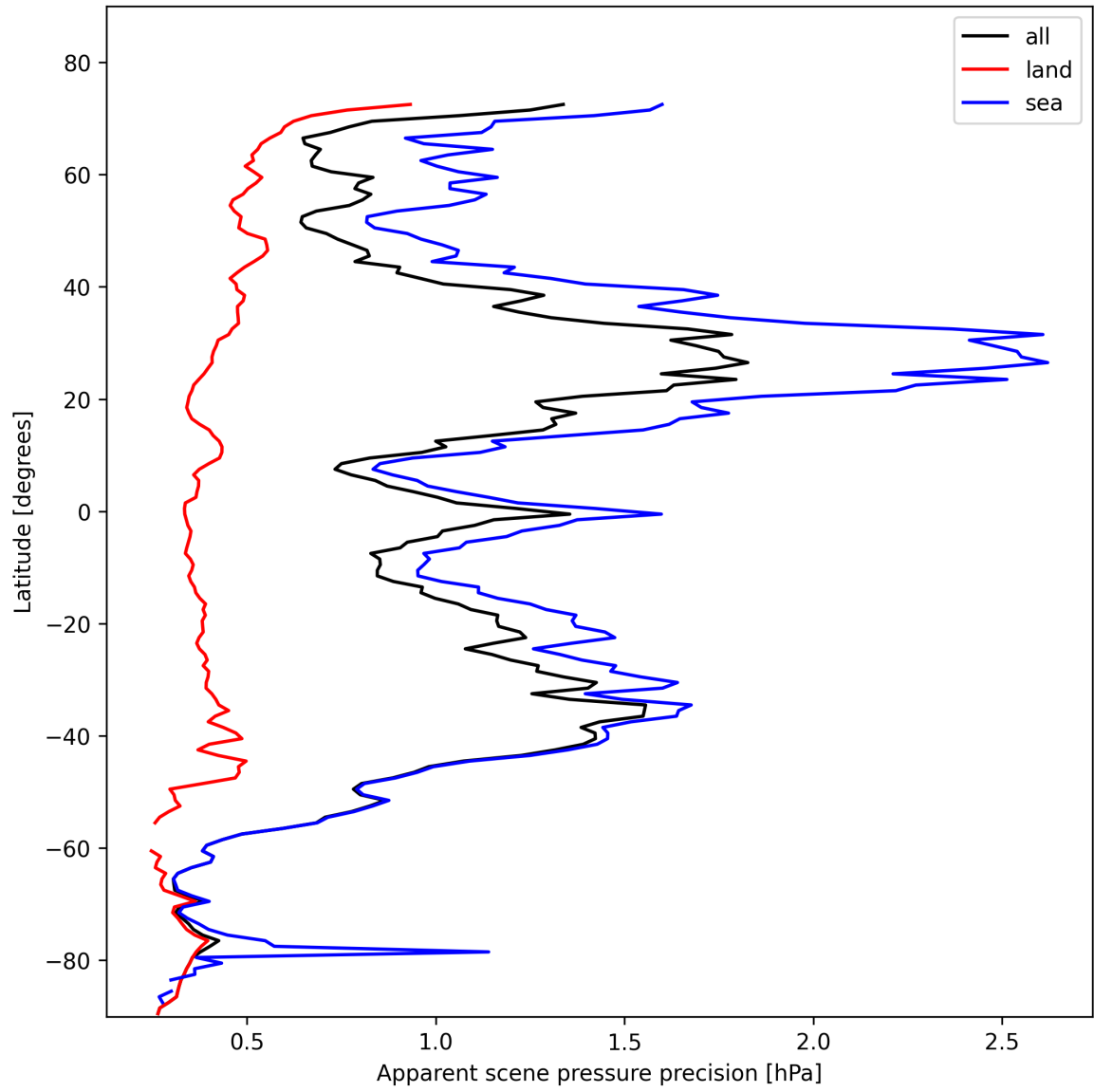
Figure 20: Zonal average of “Apparent scene pressure precision” for 2025-11-04 to 2025-11-06.
