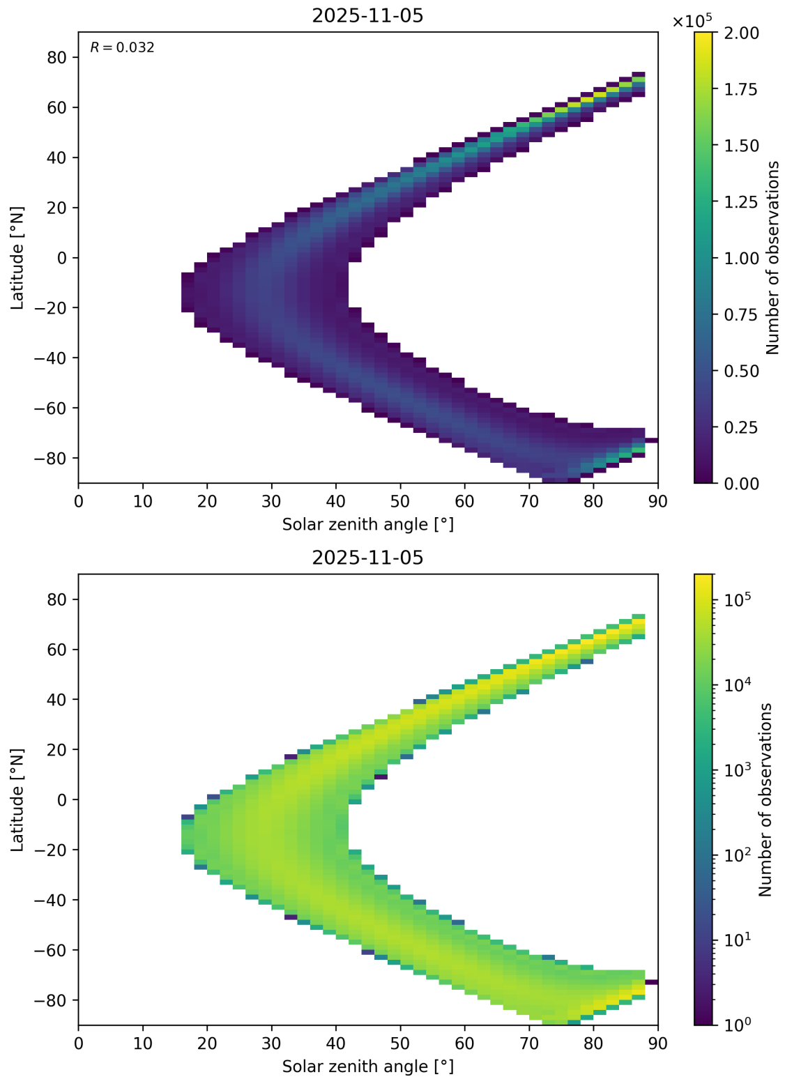
Figure 113: Scatter density plot of “Solar zenith angle” against “Latitude” for 2025-11-04 to 2025-11-06.
