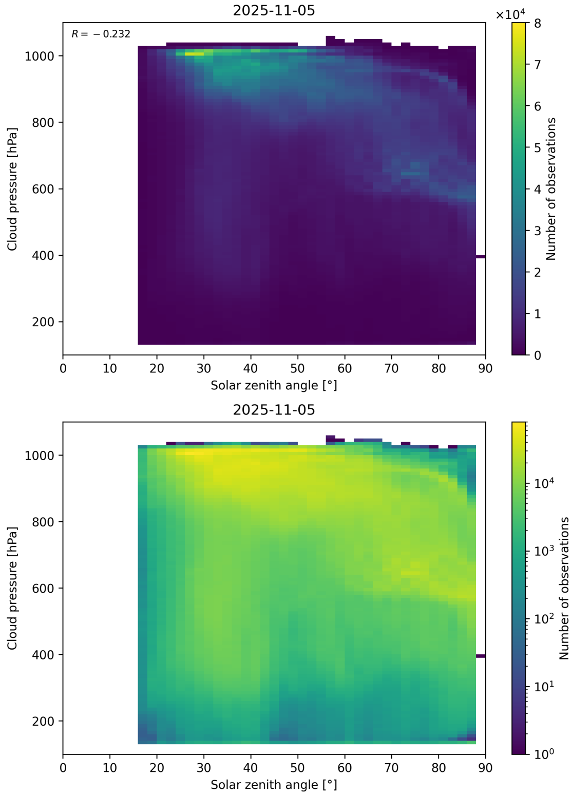
Figure 111: Scatter density plot of “Solar zenith angle” against “Cloud pressure” for 2025-11-04 to 2025-11-06.
