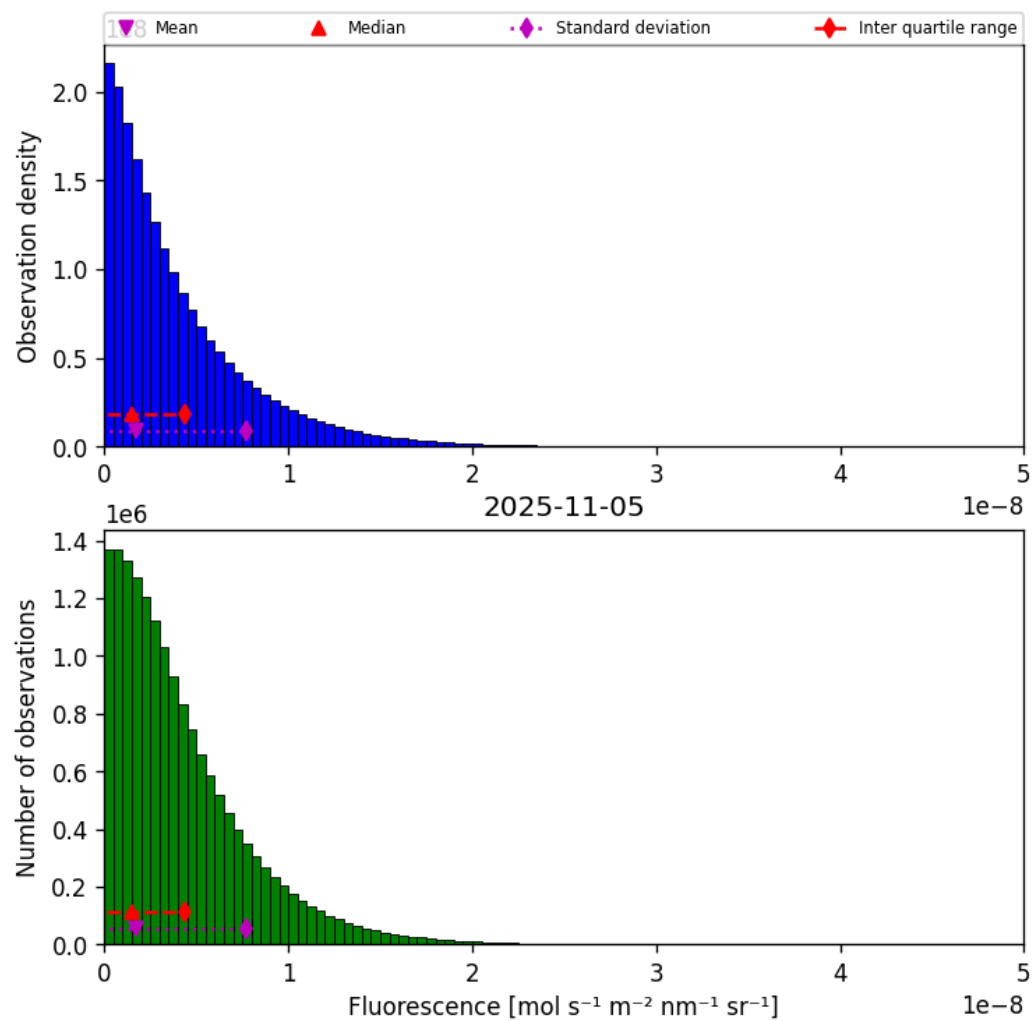
Figure 40: Histogram of “Fluorescence” for 2025-11-04 to 2025-11-06
