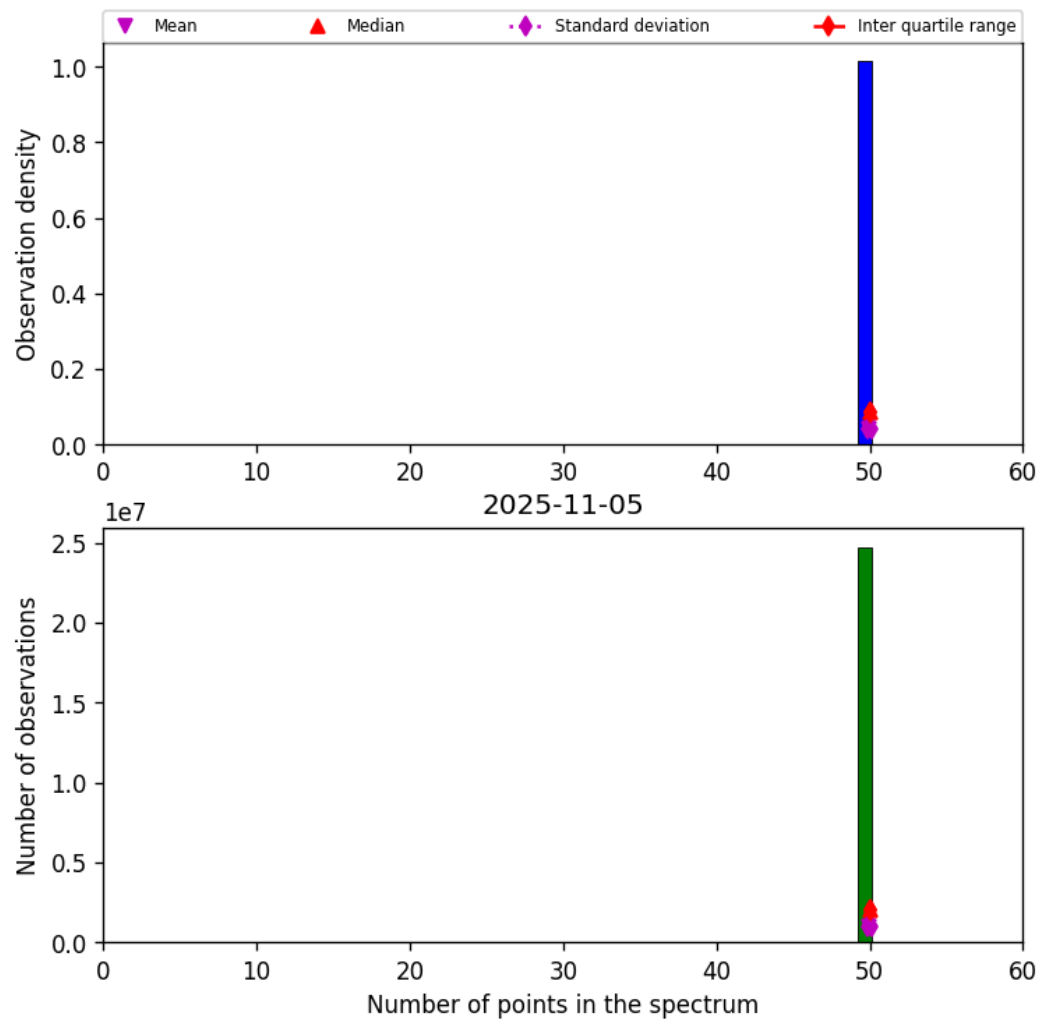
Figure 44: Histogram of "Number of points in the spectrum" for 2025-11-04 to 2025-11-06
