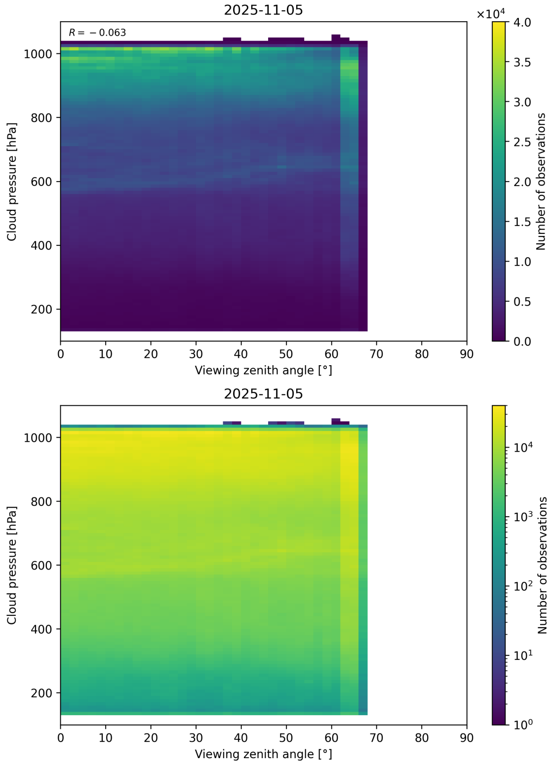
Figure 121: Scatter density plot of “Viewing zenith angle” against “Cloud pressure” for 2025-11-04 to 2025-11-06.
