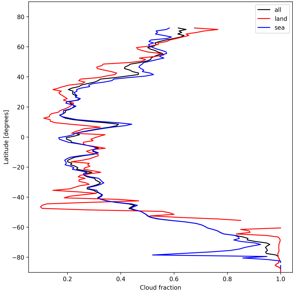
Figure 15: Zonal average of “Cloud fraction” for 2025-11-04 to 2025-11-06.
