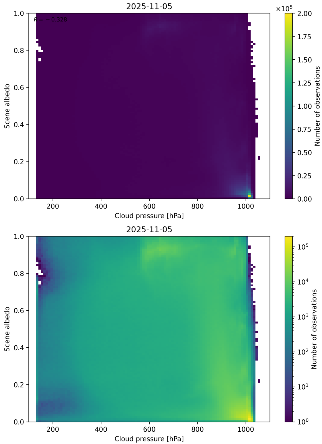
Figure 83: Scatter density plot of “Cloud pressure” against “Scene albedo” for 2025-11-04 to 2025-11-06.
