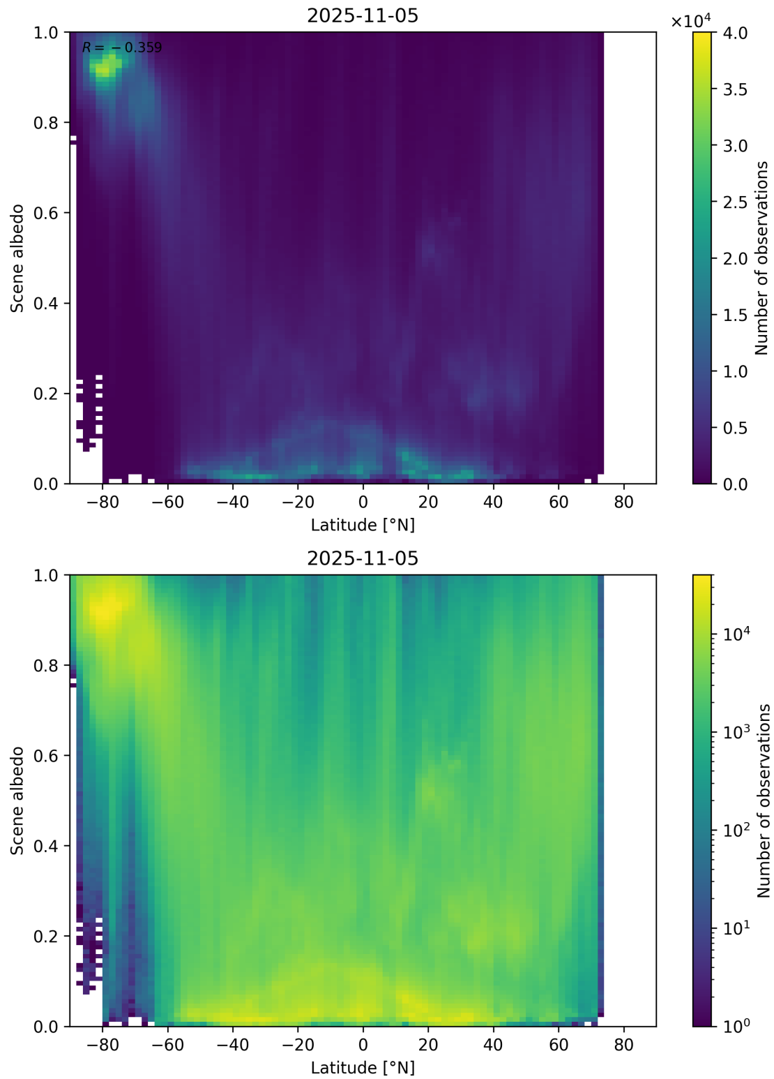
Figure 95: Scatter density plot of “Latitude” against “Scene albedo” for 2025-11-04 to 2025-11-06.
