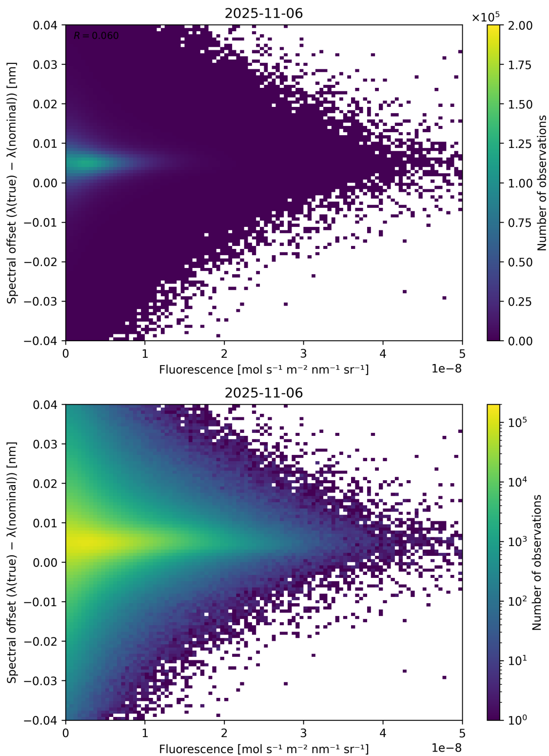
Figure 87: Scatter density plot of “Fluorescence” against “Spectral offset ( \lambda_{\text{true}} - \lambda_{\text{nominal}} )” for 2025-11-05 to 2025-11-07.
