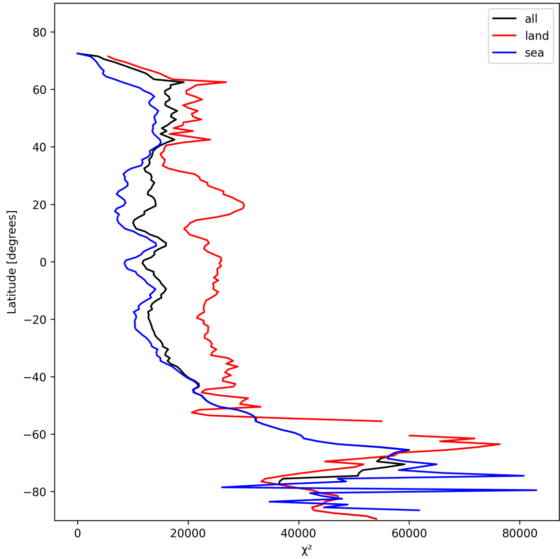
Figure 21: Zonal average of “ \chi^2 ” for 2025-11-05 to 2025-11-07.
