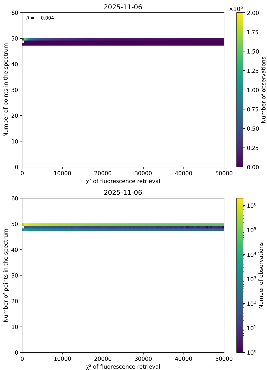
Figure 68: Scatter density plot of " \chi^2 of fluorescence retrieval" against "Number of points in the spectrum" for 2025-11-05 to 2025-11-07.
