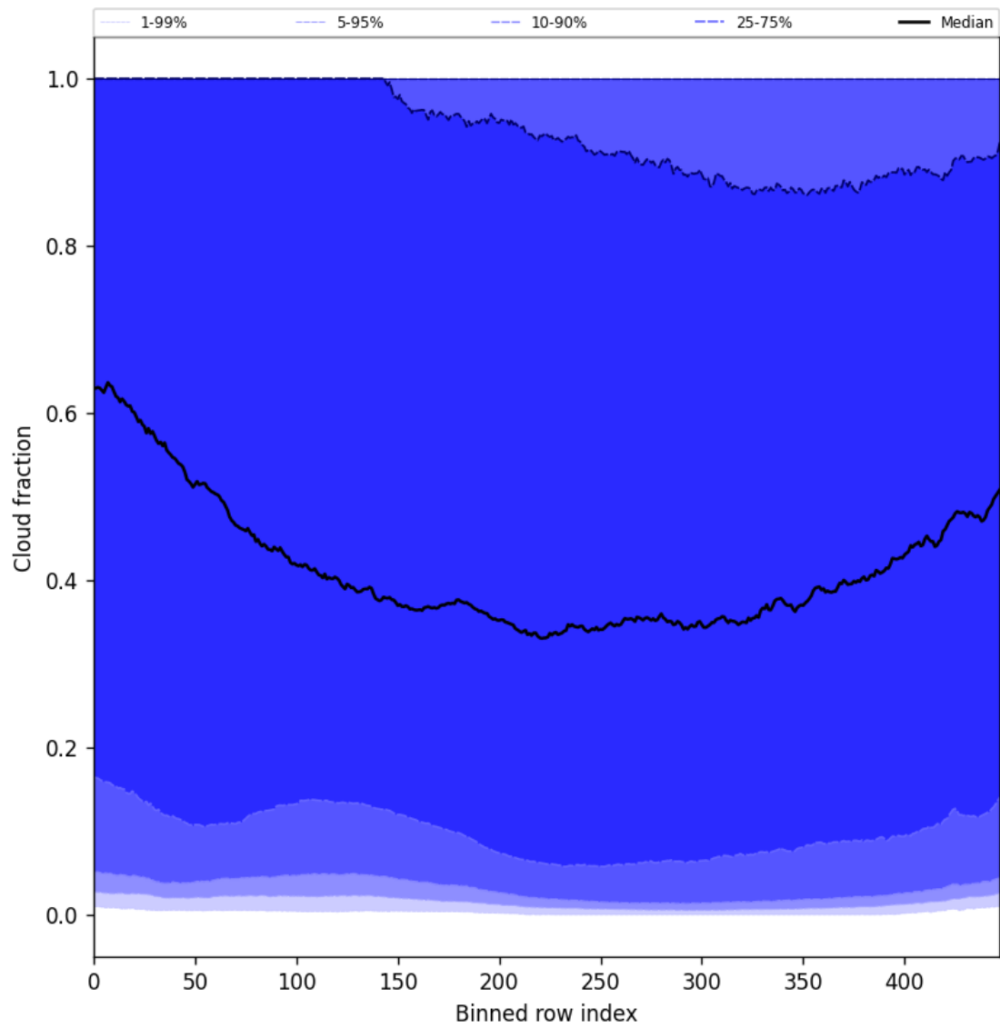
Figure 49: Along track statistics of “Cloud fraction” for 2025-11-05 to 2025-11-07
