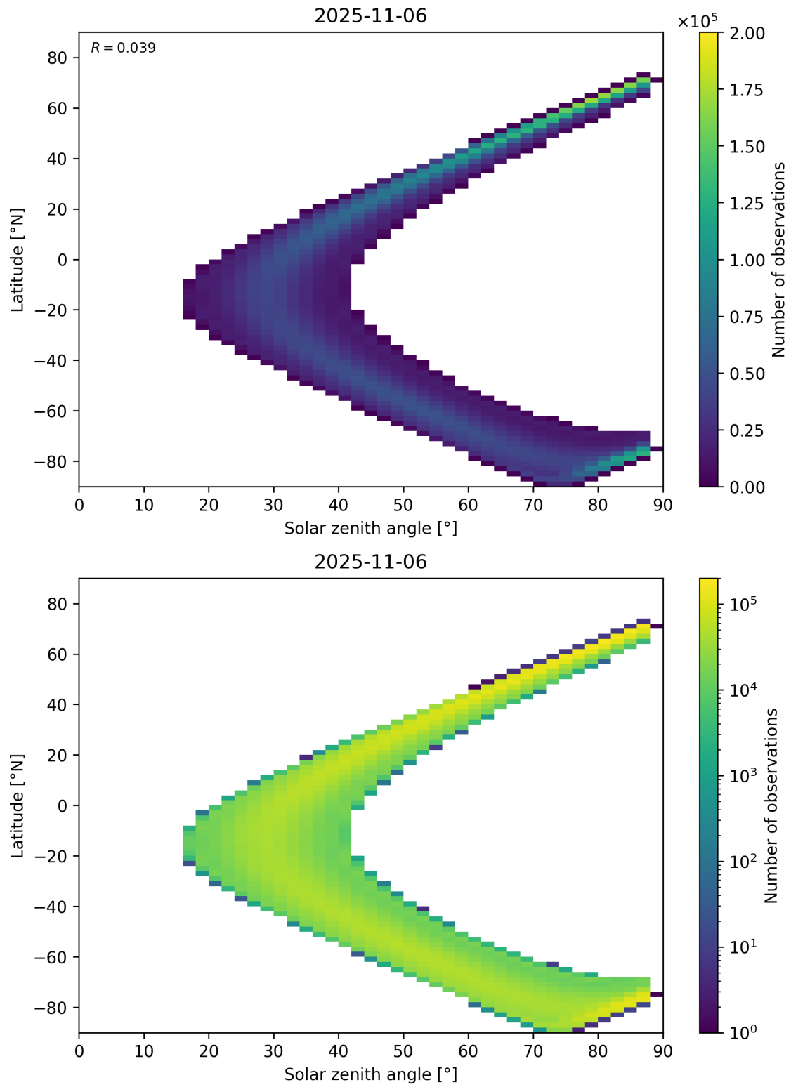
Figure 113: Scatter density plot of “Solar zenith angle” against “Latitude” for 2025-11-05 to 2025-11-07.
