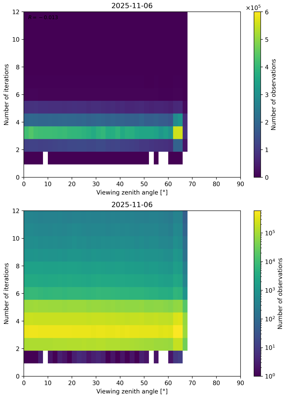
Figure 124: Scatter density plot of “Viewing zenith angle” against “Number of iterations” for 2025-11-05 to 2025-11-07.
