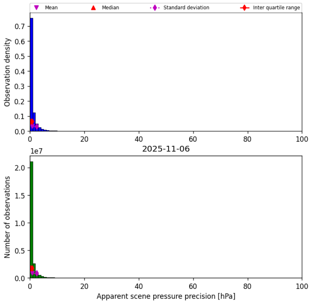
Figure 37: Histogram of “Apparent scene pressure precision” for 2025-11-05 to 2025-11-07
