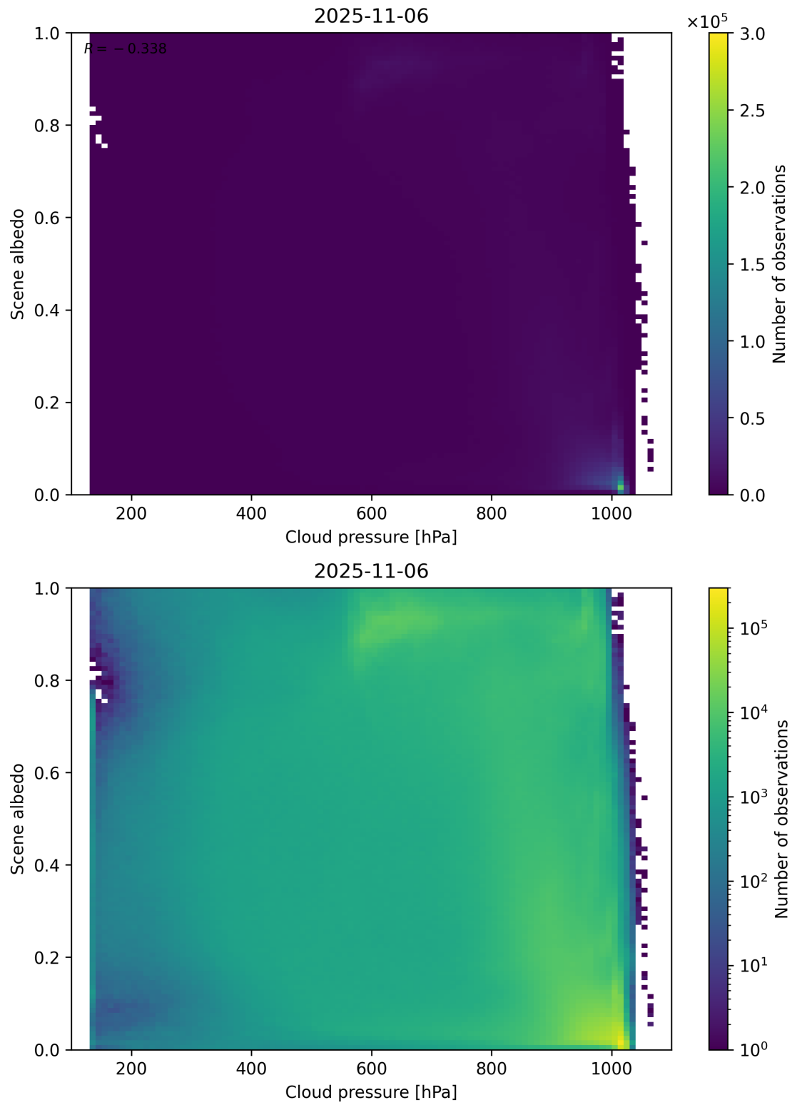
Figure 83: Scatter density plot of “Cloud pressure” against “Scene albedo” for 2025-11-05 to 2025-11-07.
