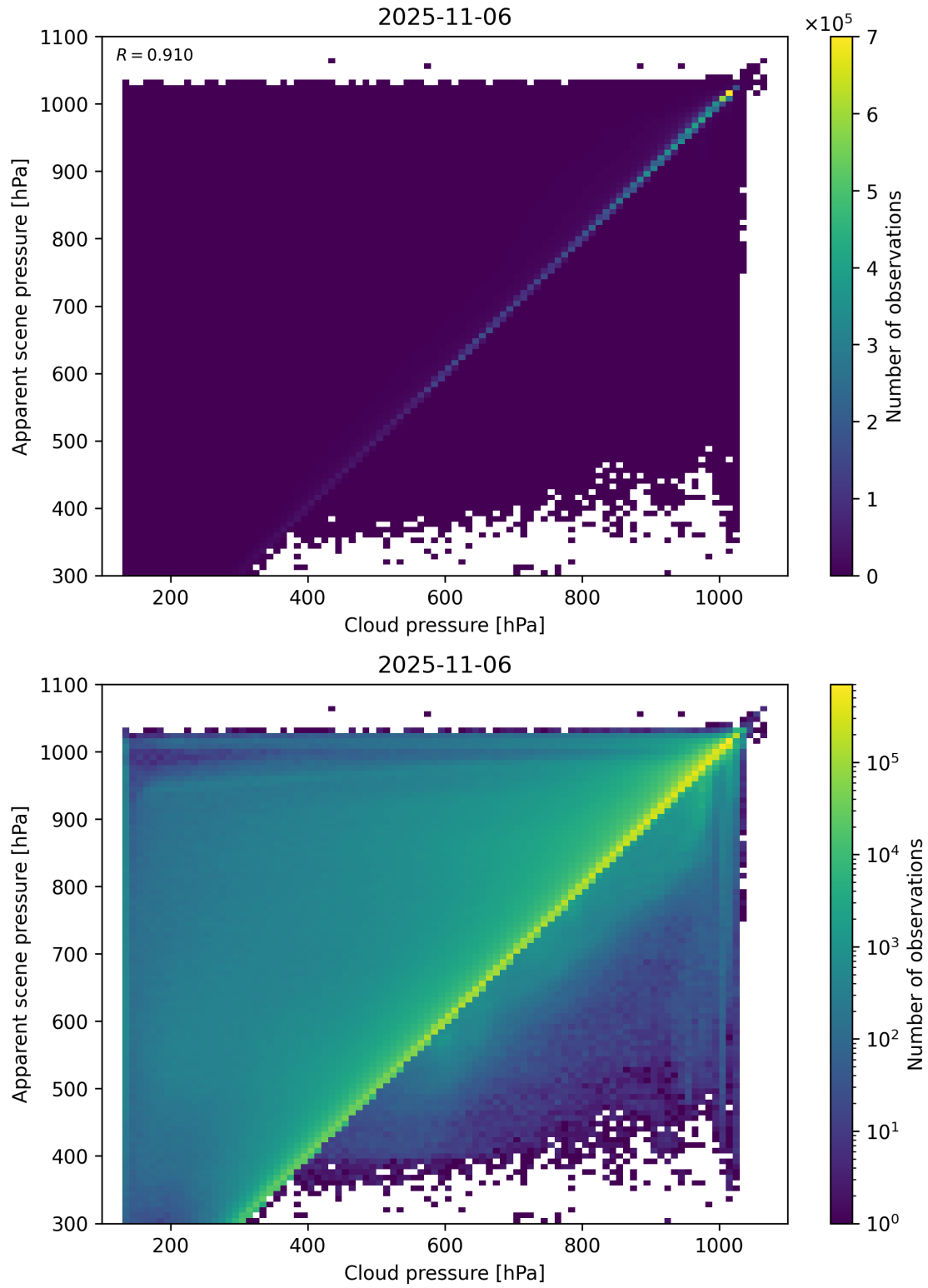
Figure 77: Scatter density plot of “Cloud pressure” against “Apparent scene pressure” for 2025-11-05 to 2025-11-07.
