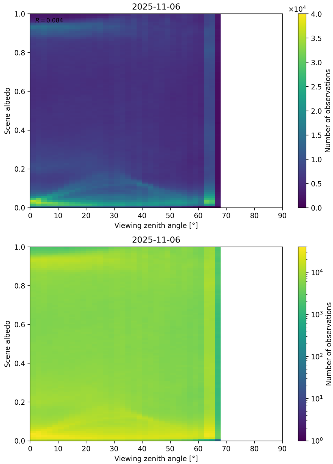
Figure 126: Scatter density plot of “Viewing zenith angle” against “Scene albedo” for 2025-11-05 to 2025-11-07.
