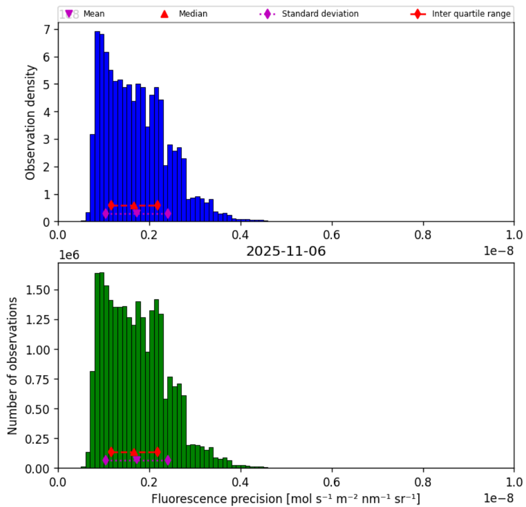
Figure 41: Histogram of “Fluorescence precision” for 2025-11-05 to 2025-11-07
