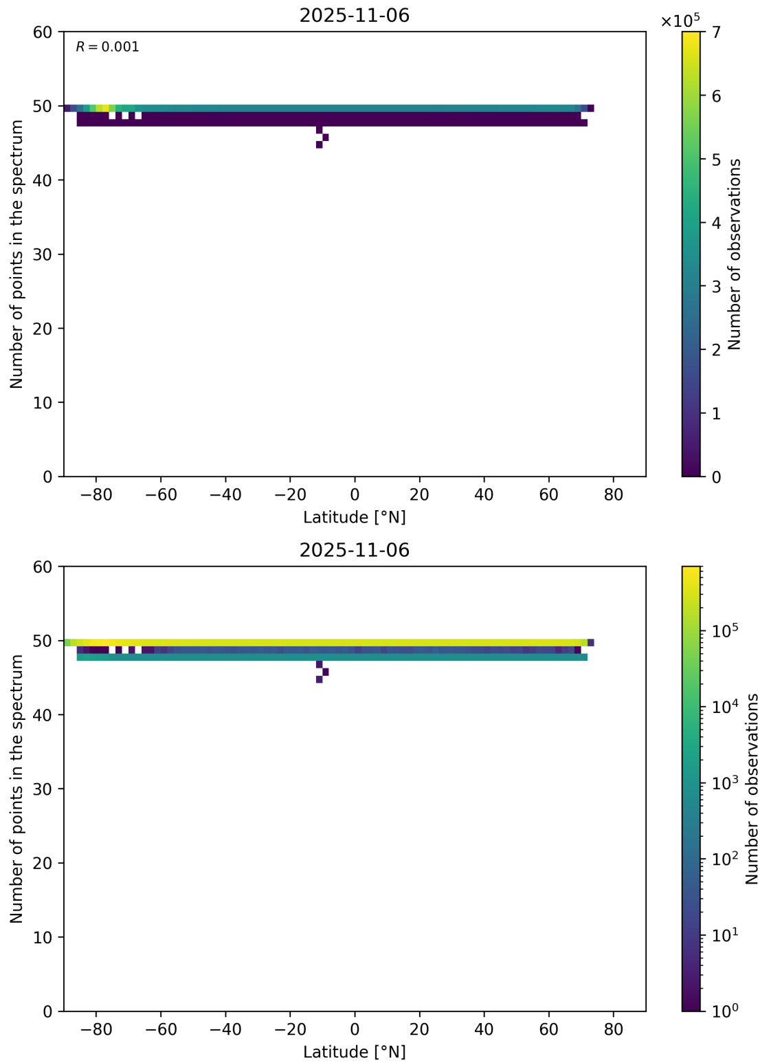
Figure 94: Scatter density plot of “Latitude” against “Number of points in the spectrum” for 2025-11-05 to 2025-11-07.
