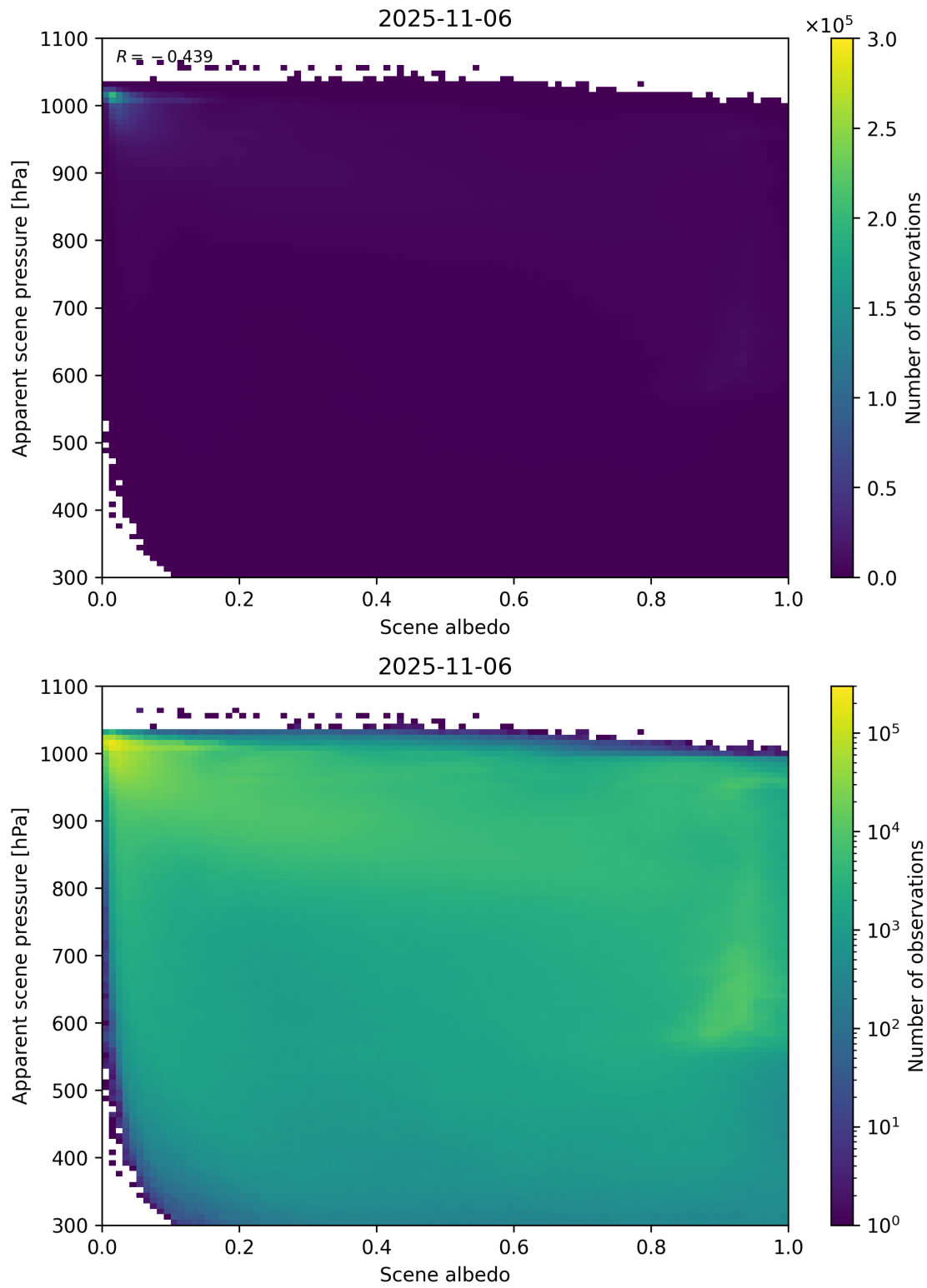
Figure 102: Scatter density plot of “Scene albedo” against “Apparent scene pressure” for 2025-11-05 to 2025-11-07.
