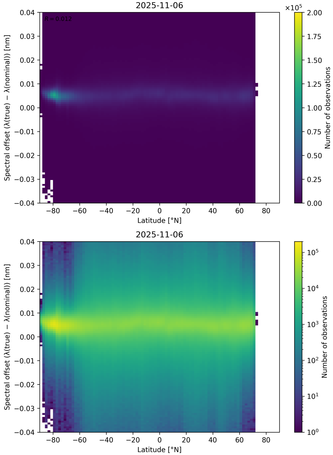
Figure 96: Scatter density plot of “Latitude” against “Spectral offset ( \lambda_{\text{true}} - \lambda_{\text{nominal}} )” for 2025-11-05 to 2025-11-07.
