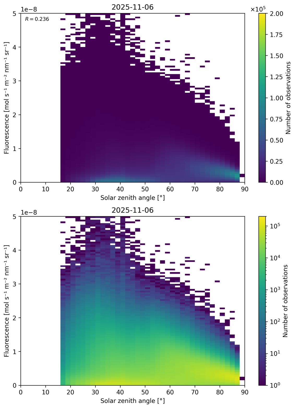
Figure 112: Scatter density plot of “Solar zenith angle” against “Fluorescence” for 2025-11-05 to 2025-11-07.
