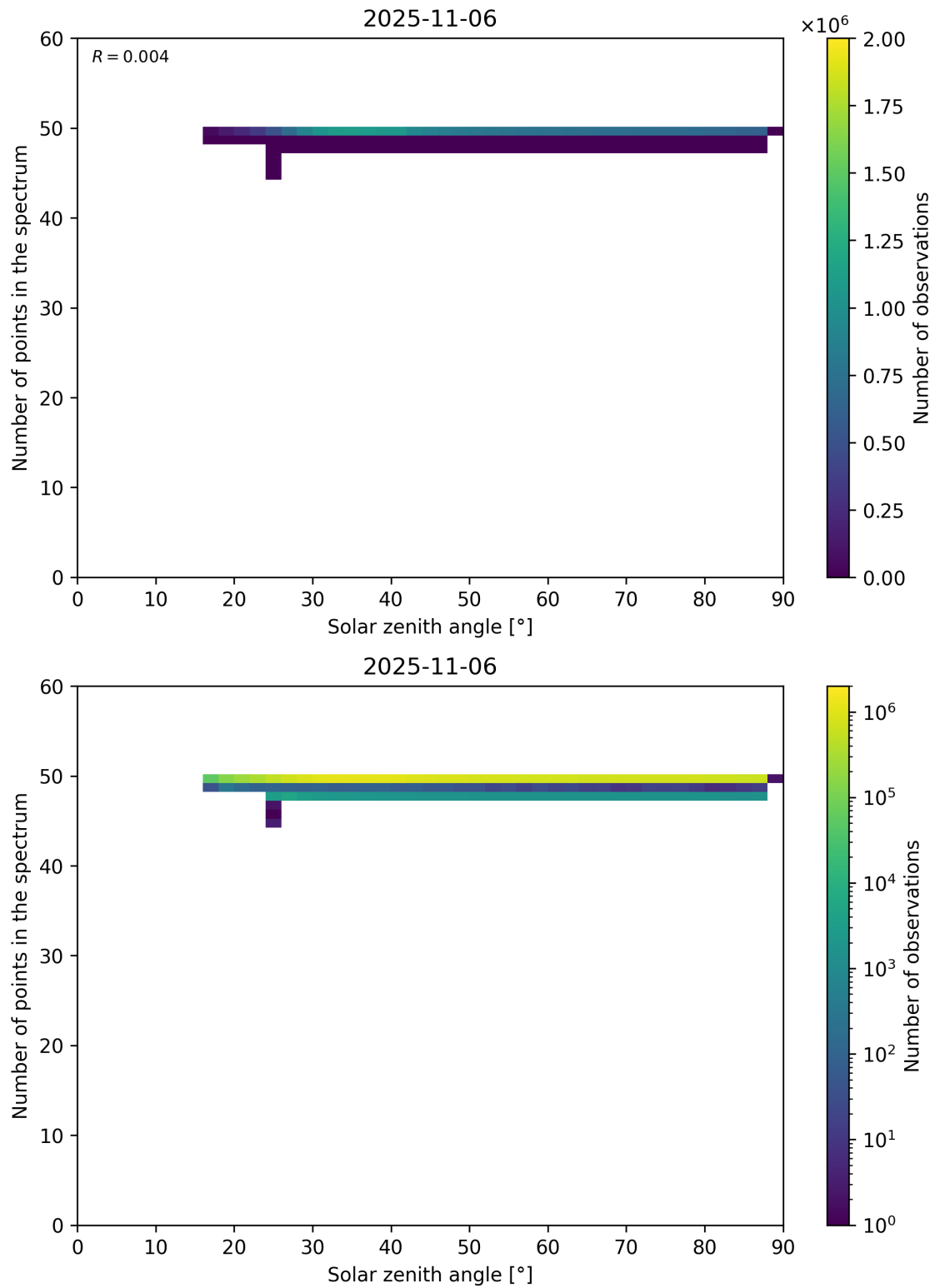
Figure 115: Scatter density plot of “Solar zenith angle” against “Number of points in the spectrum” for 2025-11-05 to 2025-11-07.
