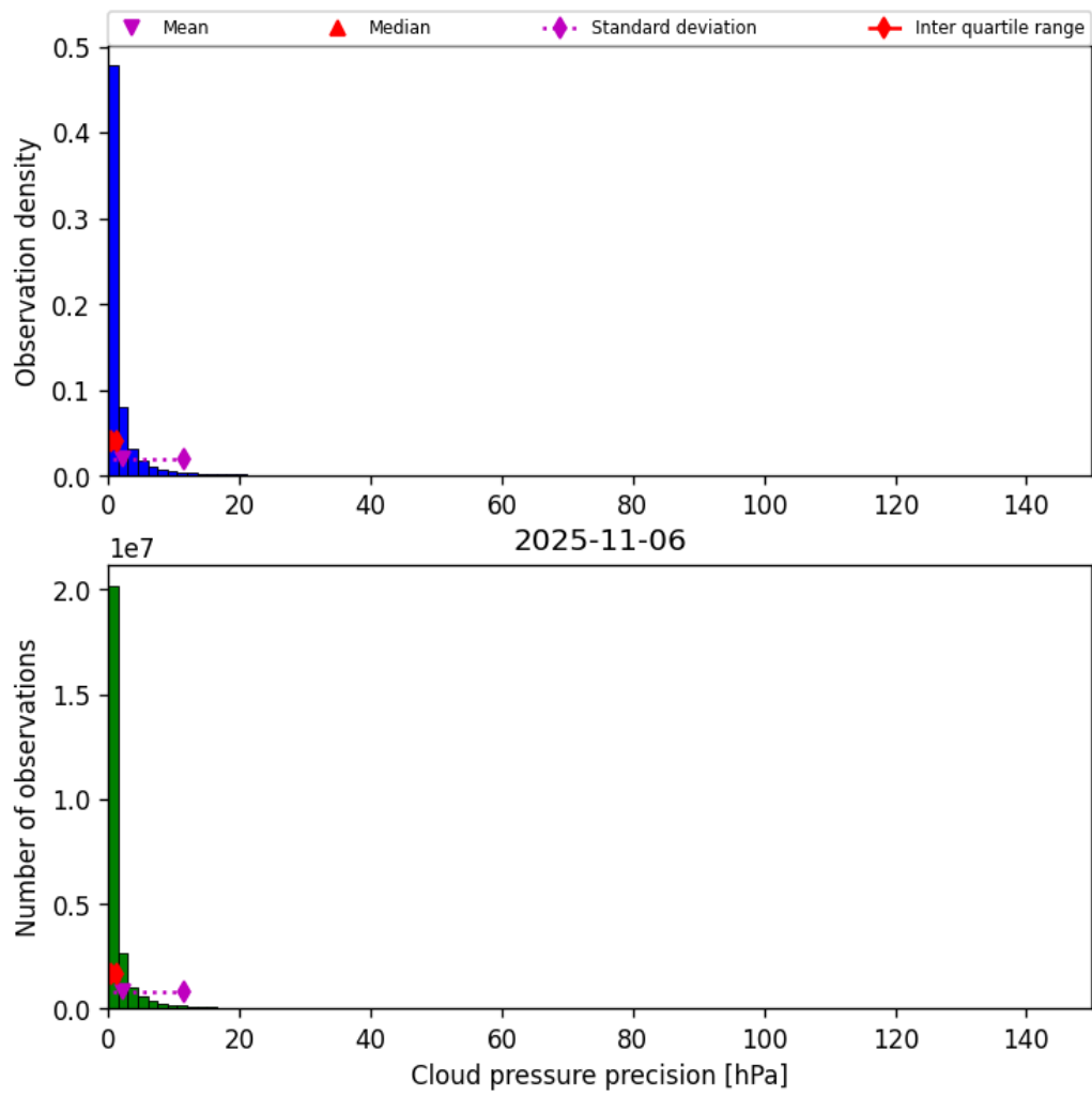
Figure 31: Histogram of “Cloud pressure precision” for 2025-11-05 to 2025-11-07
