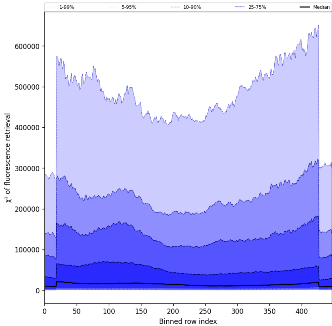
Figure 59: Along track statistics of “ \chi^2 of fluorescence retrieval” for 2025-11-05 to 2025-11-07
