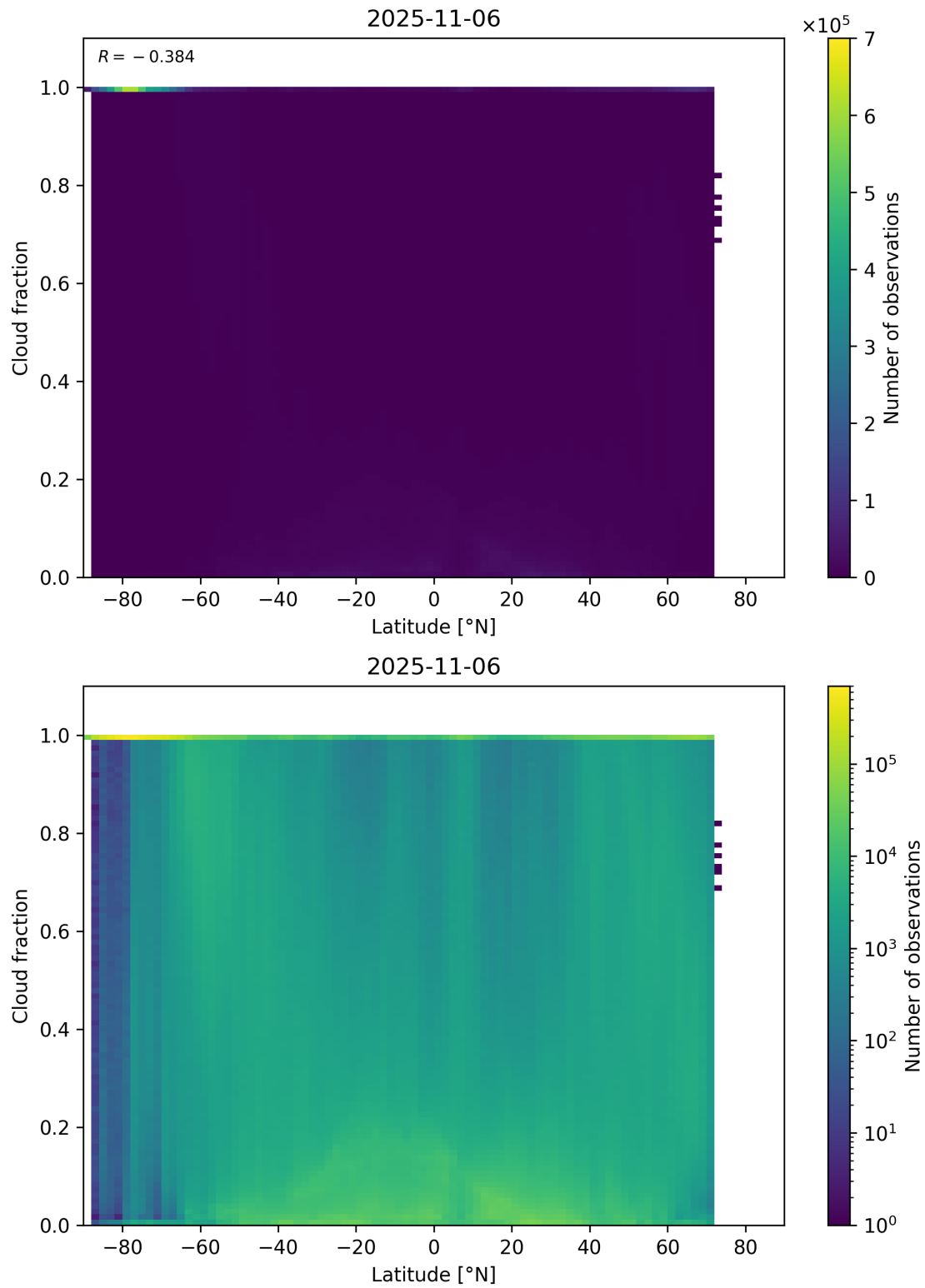
Figure 90: Scatter density plot of “Latitude” against “Cloud fraction” for 2025-11-05 to 2025-11-07.
