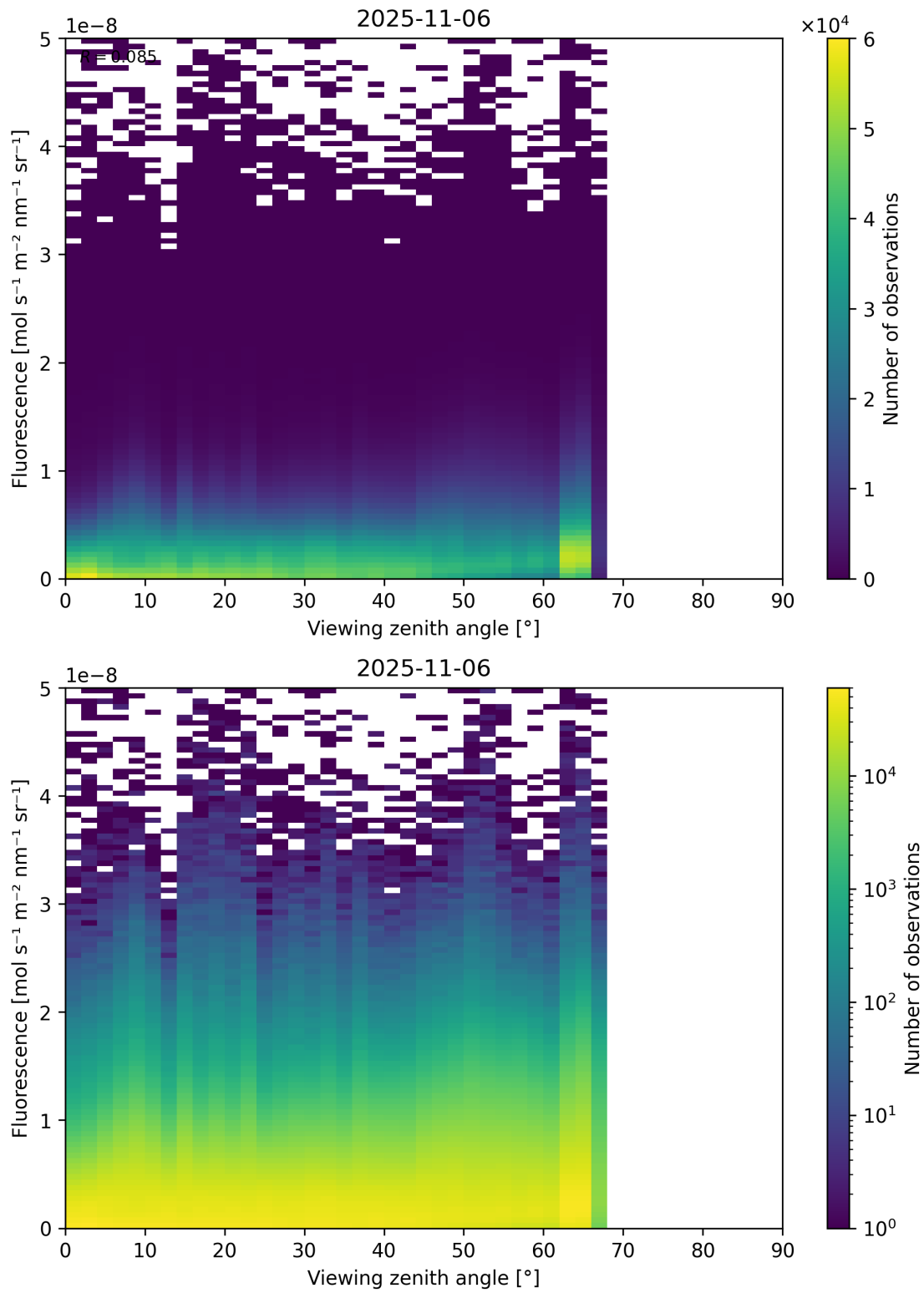
Figure 122: Scatter density plot of “Viewing zenith angle” against “Fluorescence” for 2025-11-05 to 2025-11-07.
