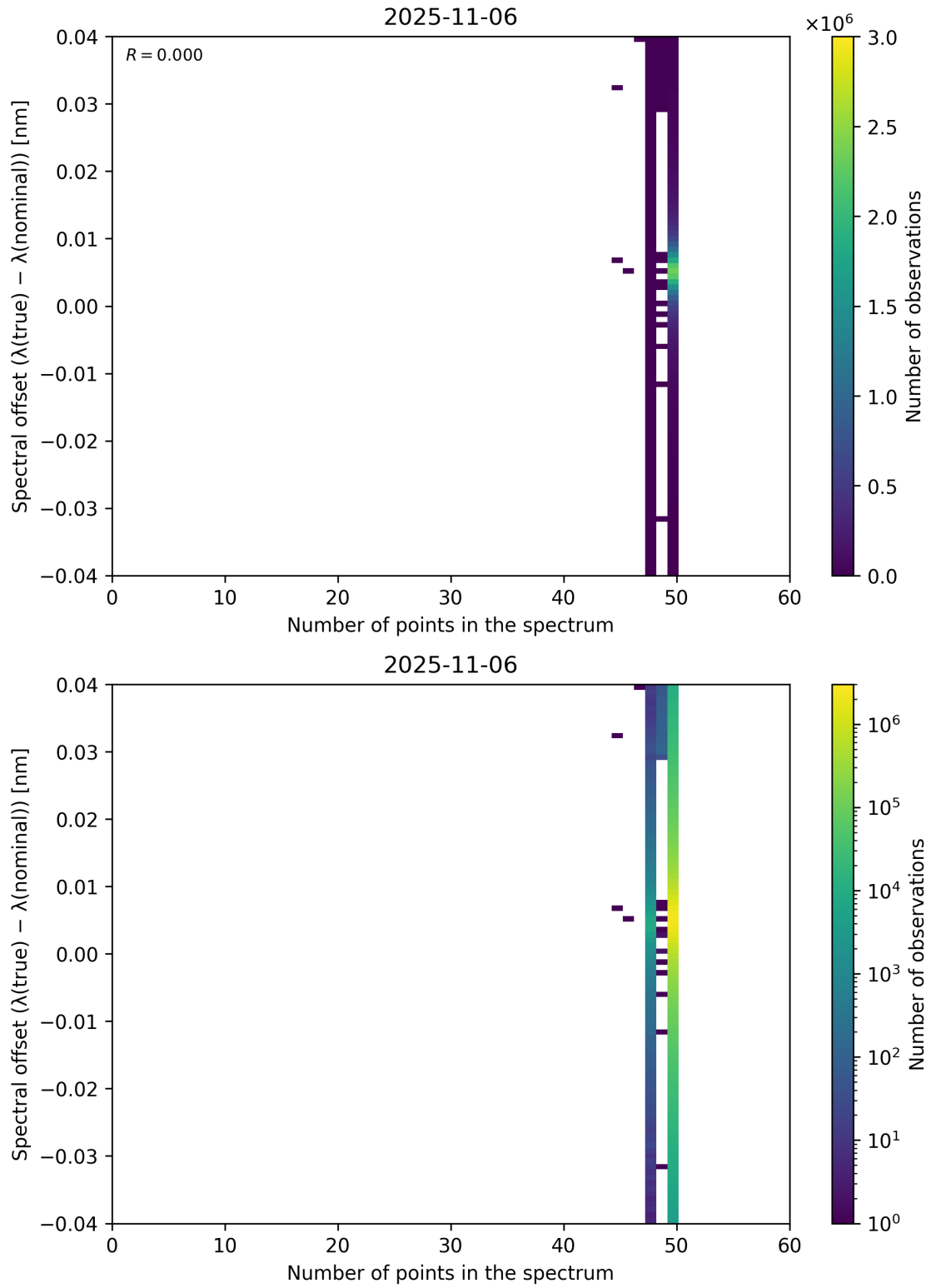
Figure 101: Scatter density plot of “Number of points in the spectrum” against “Spectral offset ( \lambda_{\text{true}} - \lambda_{\text{nominal}} )” for 2025-11-05 to 2025-11-07.
