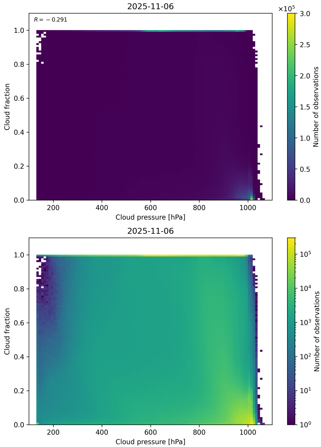
Figure 79: Scatter density plot of “Cloud pressure” against “Cloud fraction” for 2025-11-05 to 2025-11-07.
