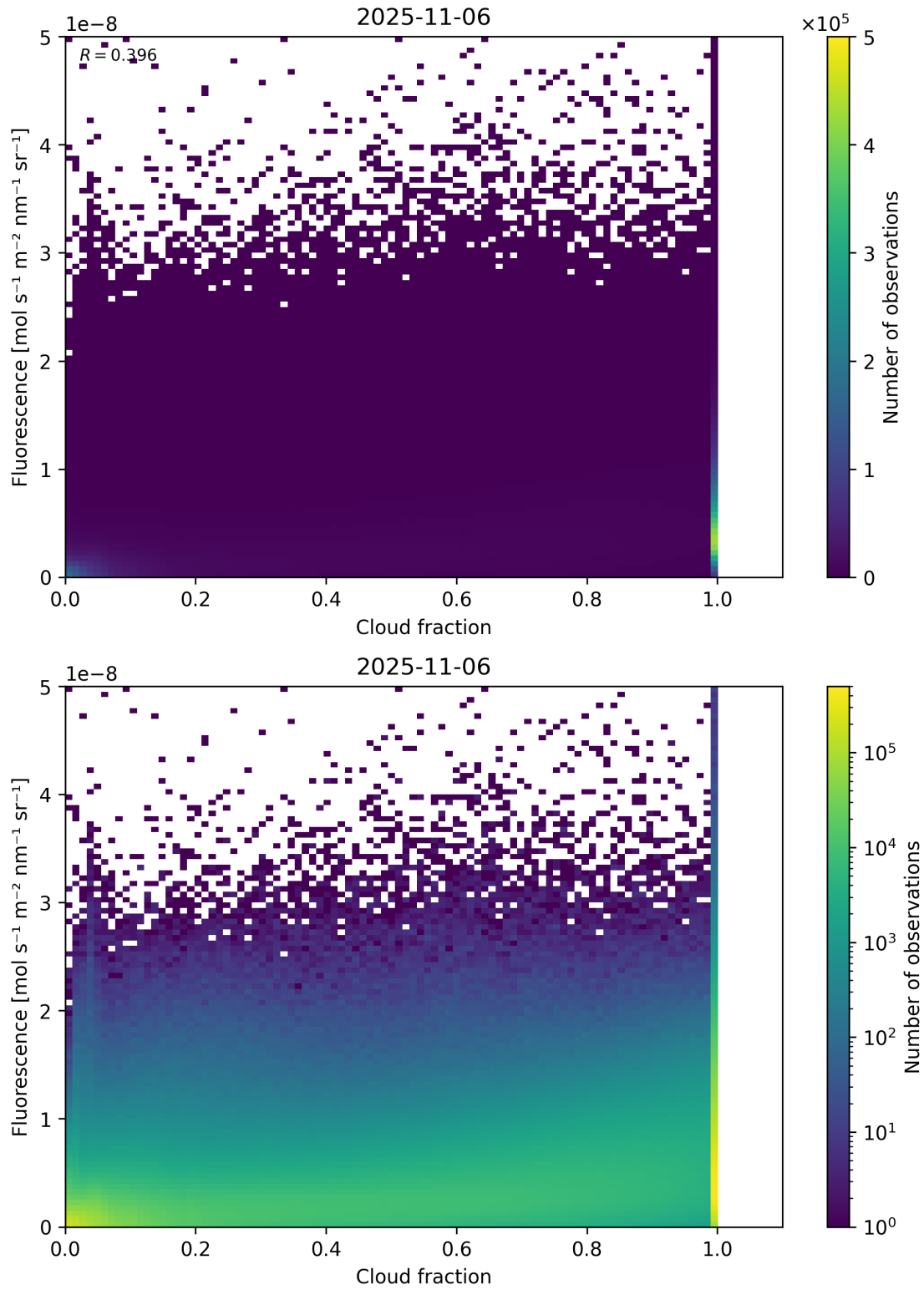
Figure 72: Scatter density plot of “Cloud fraction” against “Fluorescence” for 2025-11-05 to 2025-11-07.
