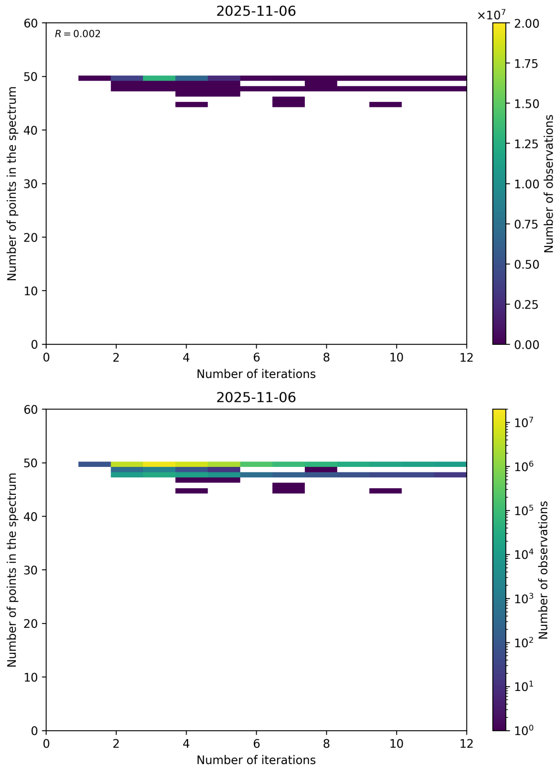
Figure 99: Scatter density plot of “Number of iterations” against “Number of points in the spectrum” for 2025-11-05 to 2025-11-07.
