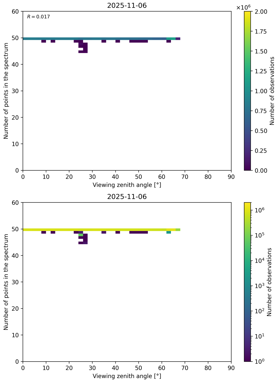
Figure 125: Scatter density plot of “Viewing zenith angle” against “Number of points in the spectrum” for 2025-11-05 to 2025-11-07.
