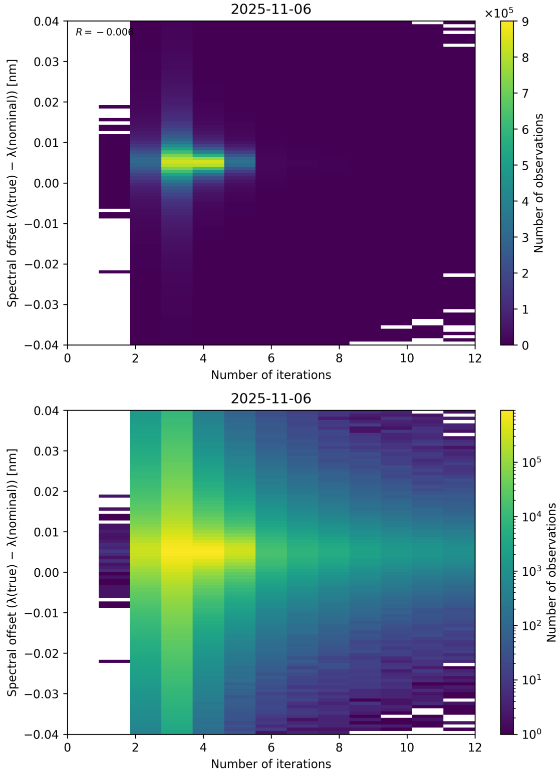
Figure 100: Scatter density plot of “Number of iterations” against “Spectral offset ( \lambda_{\text{true}} - \lambda_{\text{nominal}} )” for 2025-11-05 to 2025-11-07.
