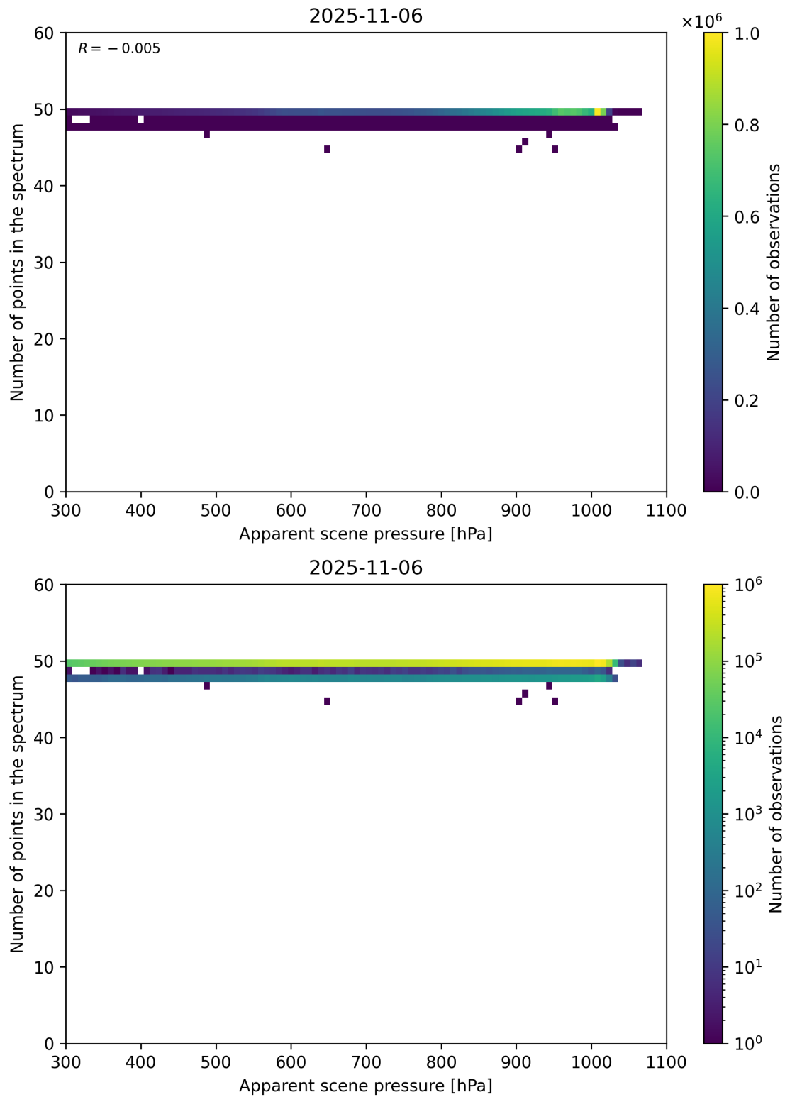
Figure 66: Scatter density plot of “Apparent scene pressure” against “Number of points in the spectrum” for 2025-11-05 to 2025-11-07.
