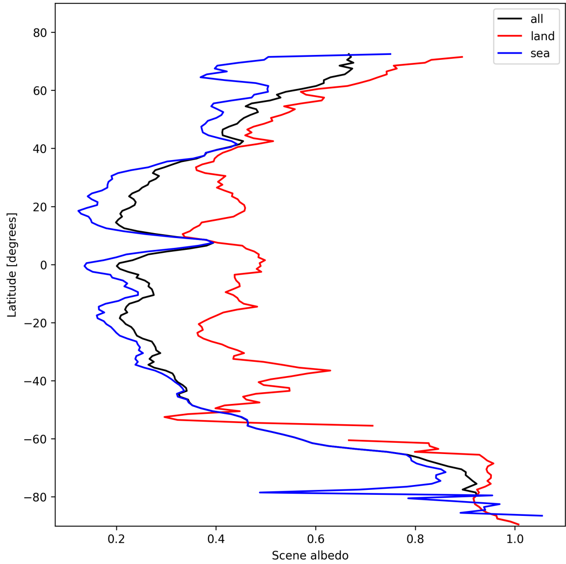
Figure 17: Zonal average of “Scene albedo” for 2025-11-05 to 2025-11-07.
