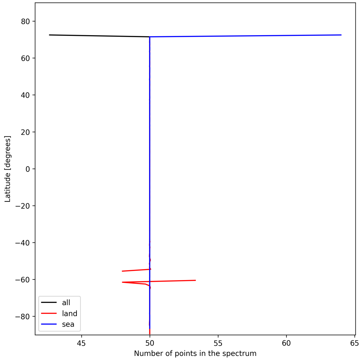
Figure 27: Zonal average of “Number of points in the spectrum” for 2025-11-05 to 2025-11-07.
