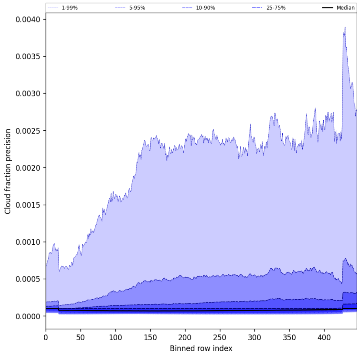
Figure 50: Along track statistics of “Cloud fraction precision” for 2025-11-05 to 2025-11-07
