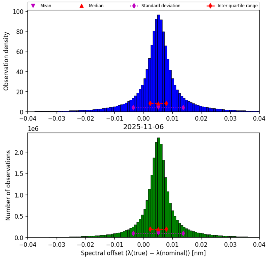
Figure 45: Histogram of “Spectral offset ( \lambda_{\text{true}} - \lambda_{\text{nominal}} )” for 2025-11-05 to 2025-11-07
