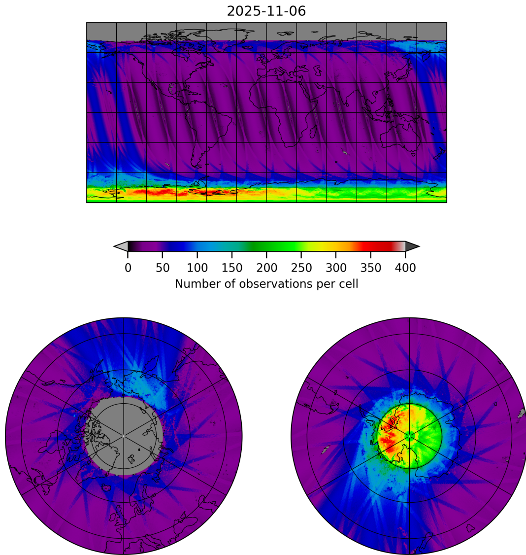
Figure 11: Map of the number of observations for 2025-11-05 to 2025-11-07
