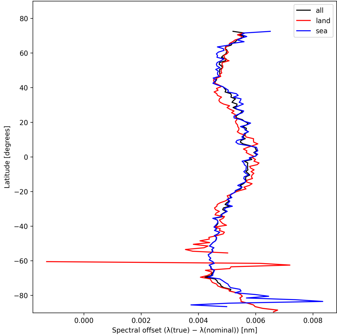
Figure 28: Zonal average of “Spectral offset ( \lambda_{\text{true}} - \lambda_{\text{nominal}} )” for 2025-11-05 to 2025-11-07.
