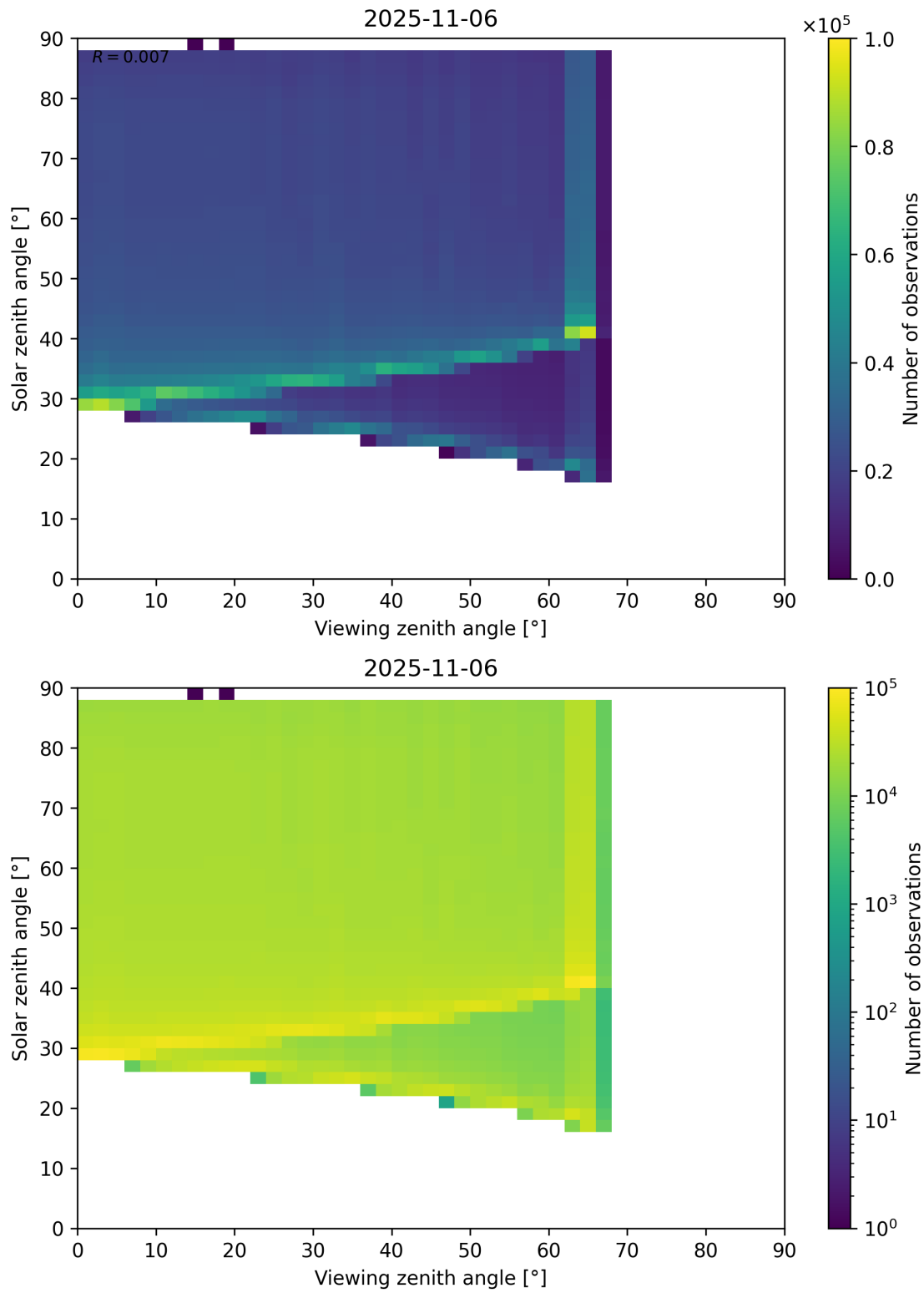
Figure 127: Scatter density plot of “Viewing zenith angle” against “Solar zenith angle” for 2025-11-05 to 2025-11-07.
