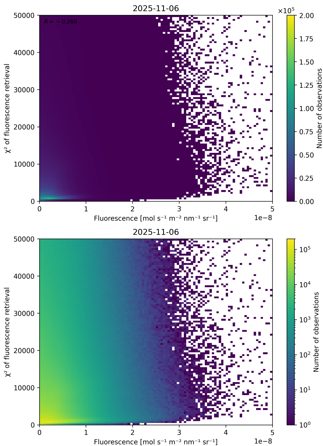
Figure 85: Scatter density plot of “Fluorescence” against “ \chi^2 of fluorescence retrieval” for 2025-11-05 to 2025-11-07.
