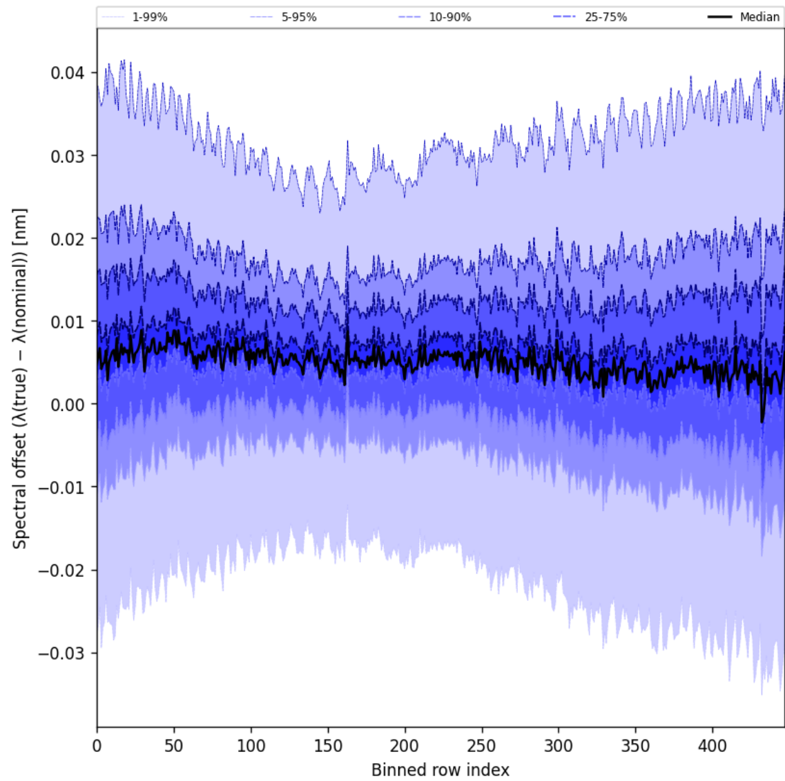
Figure 62: Along track statistics of “Spectral offset ( \lambda_{\text{true}} - \lambda_{\text{nominal}} )” for 2025-11-05 to 2025-11-07
