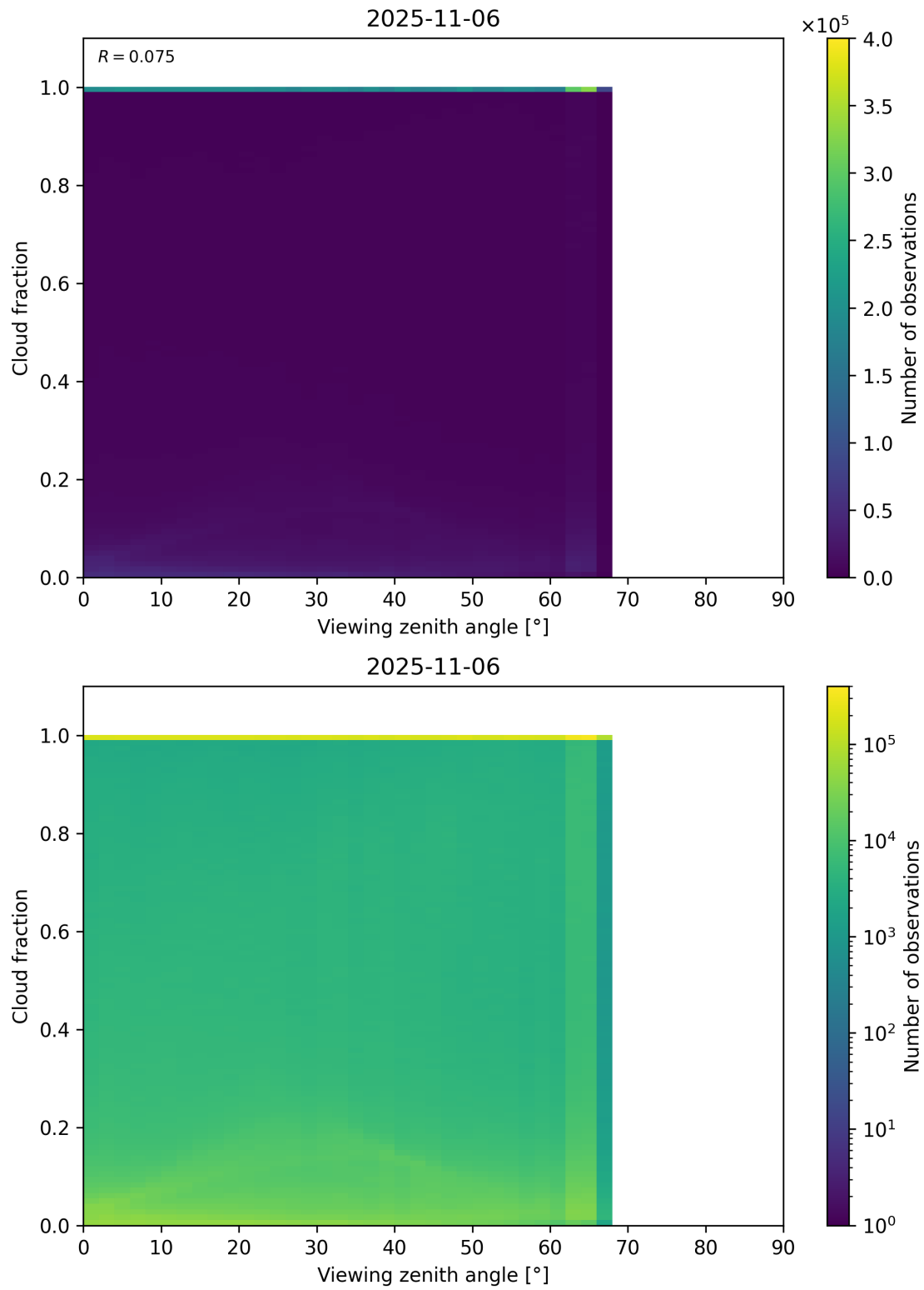
Figure 120: Scatter density plot of “Viewing zenith angle” against “Cloud fraction” for 2025-11-05 to 2025-11-07.
