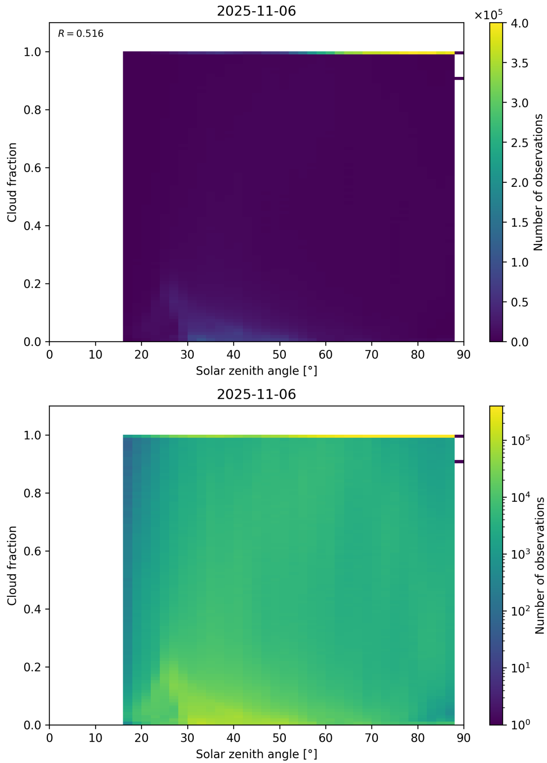
Figure 110: Scatter density plot of “Solar zenith angle” against “Cloud fraction” for 2025-11-05 to 2025-11-07.
