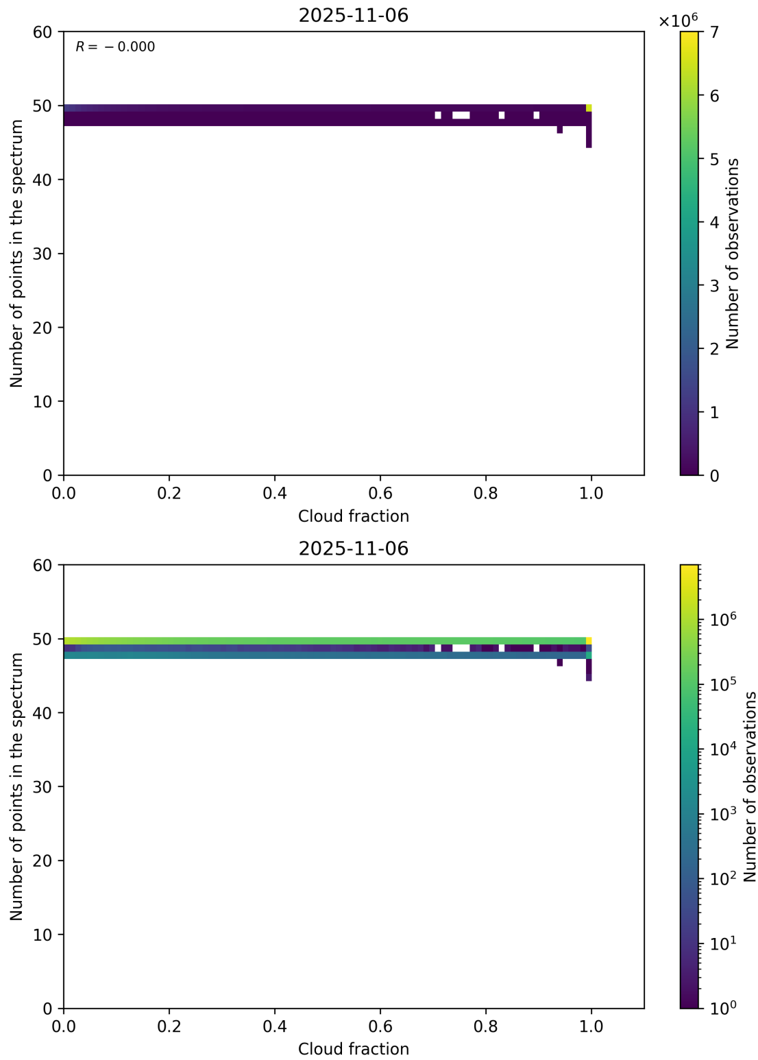
Figure 74: Scatter density plot of “Cloud fraction” against “Number of points in the spectrum” for 2025-11-05 to 2025-11-07.
