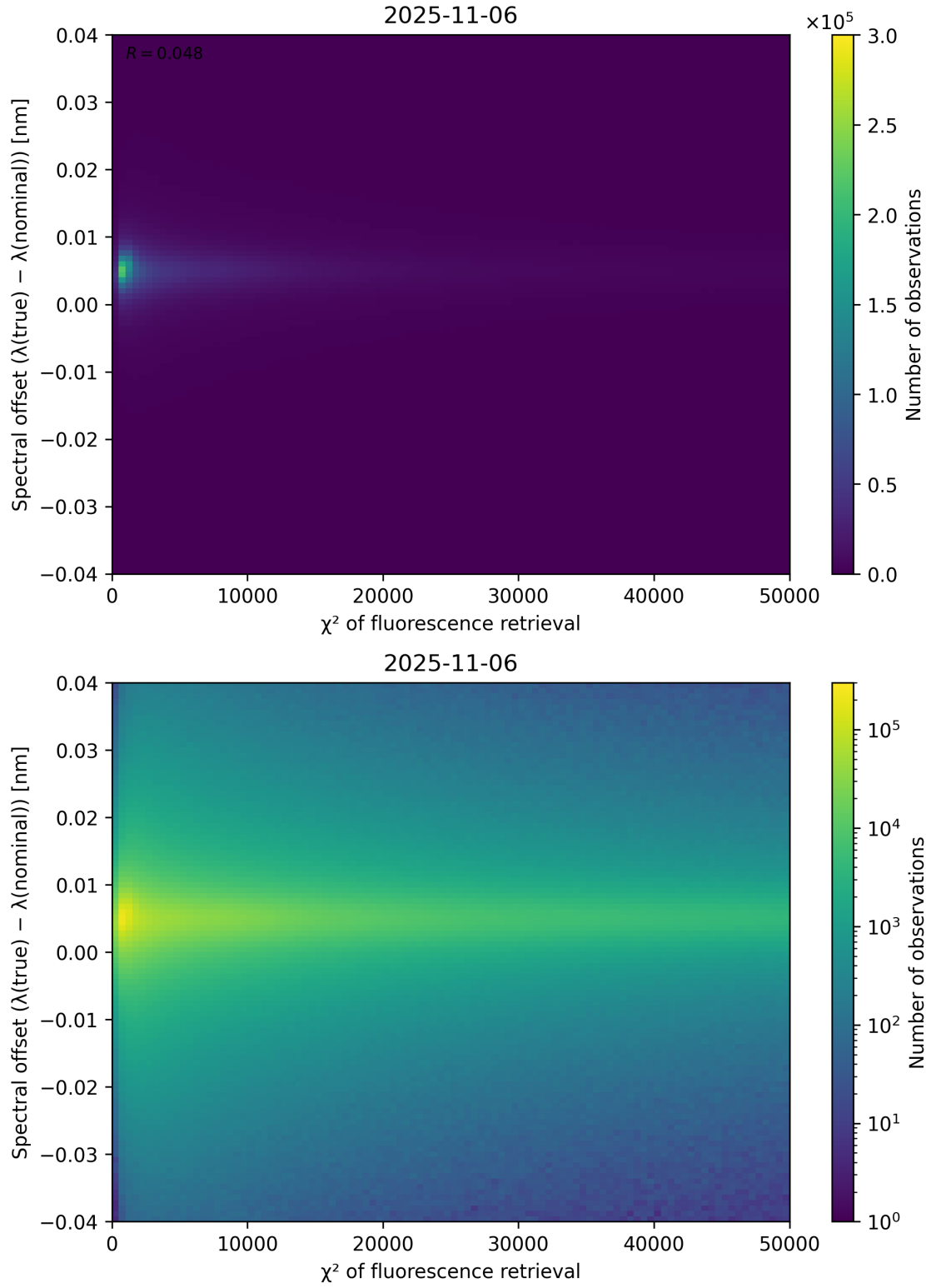
Figure 69: Scatter density plot of “ \chi^2 of fluorescence retrieval” against “Spectral offset ( \lambda_{\text{true}} - \lambda_{\text{nominal}} )” for 2025-11-05 to 2025-11-07.
