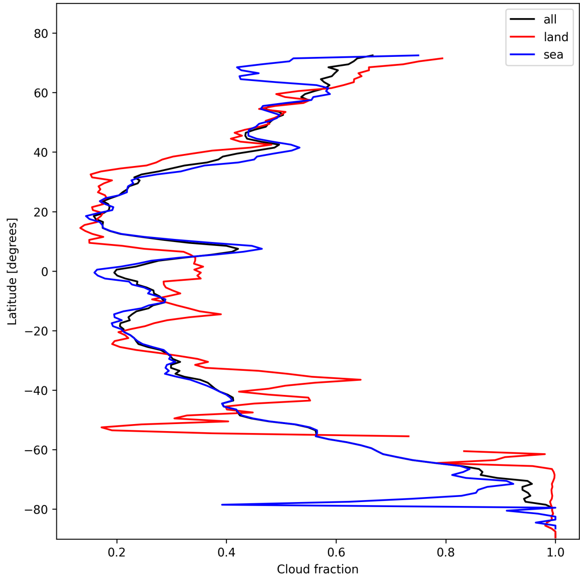
Figure 15: Zonal average of “Cloud fraction” for 2025-11-05 to 2025-11-07.
