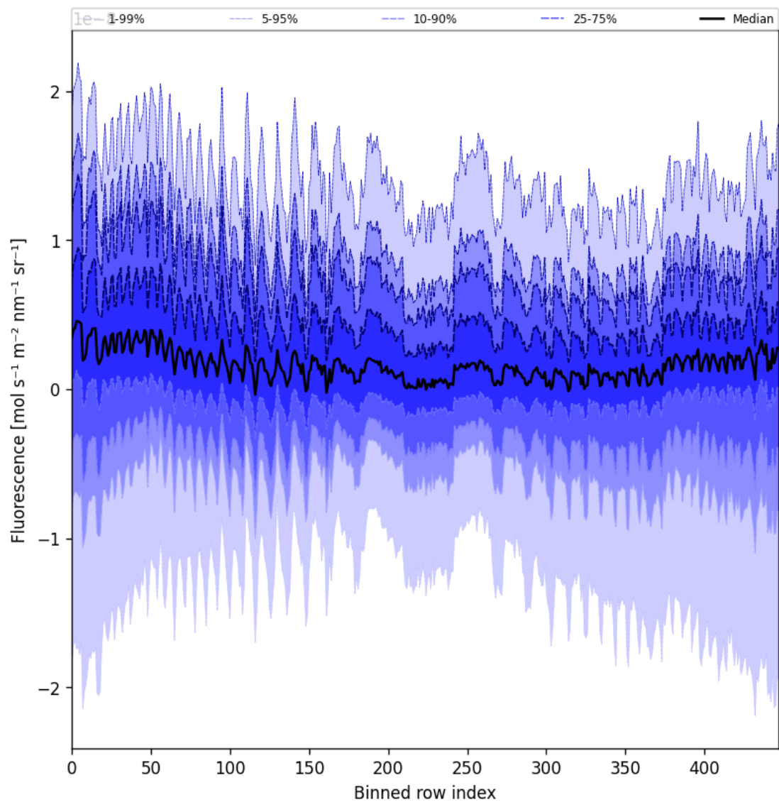
Figure 57: Along track statistics of “Fluorescence” for 2025-11-05 to 2025-11-07
