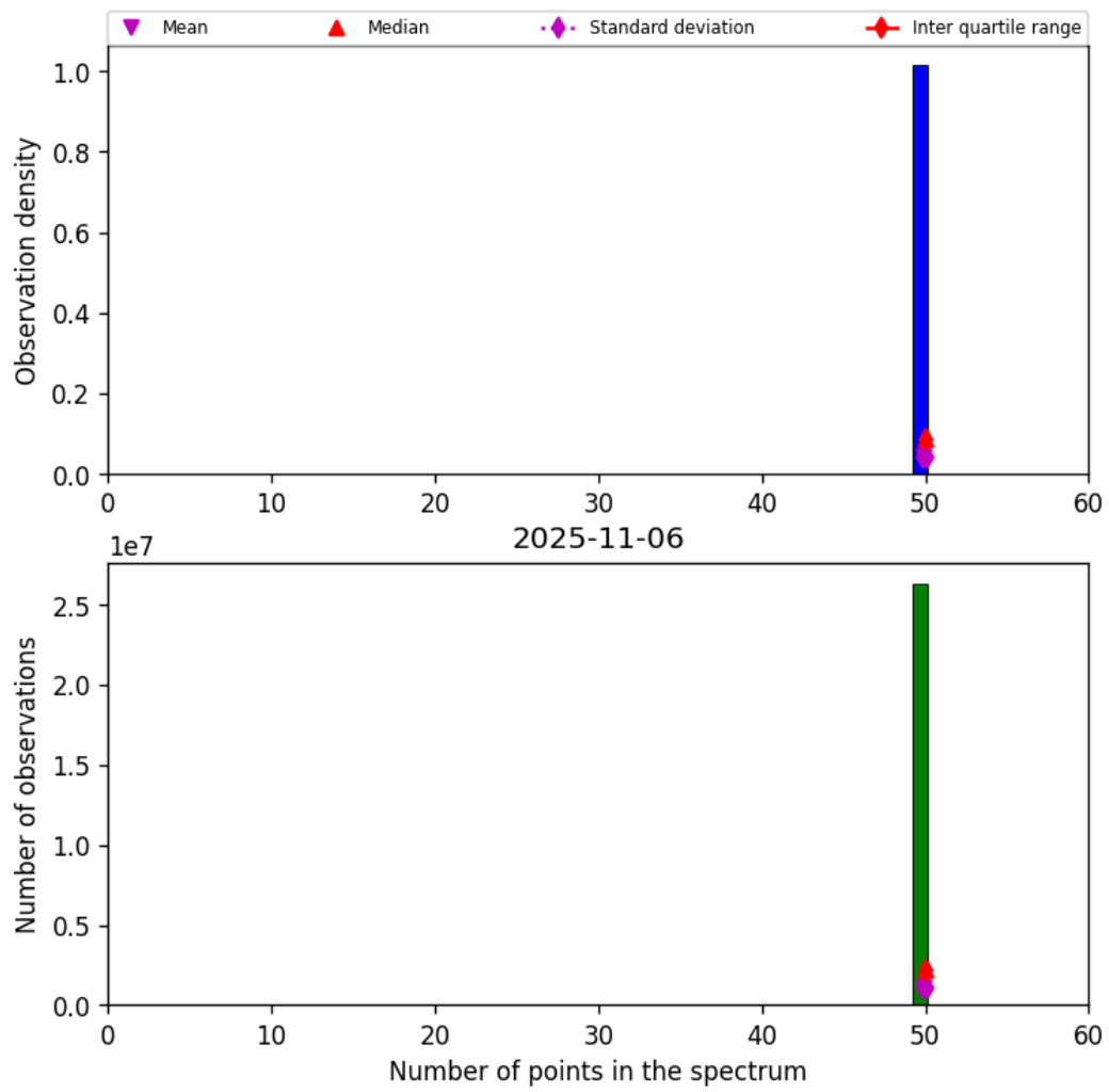
Figure 44: Histogram of "Number of points in the spectrum" for 2025-11-05 to 2025-11-07
