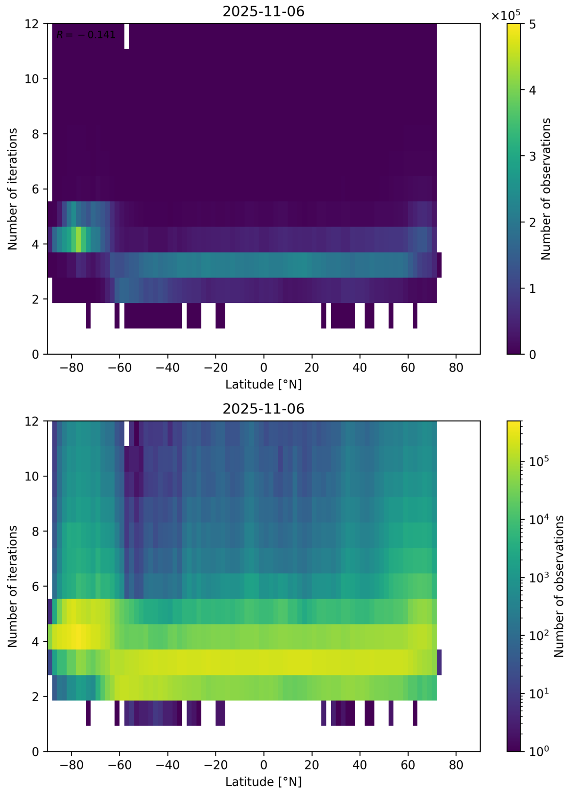
Figure 93: Scatter density plot of “Latitude” against “Number of iterations” for 2025-11-05 to 2025-11-07.
