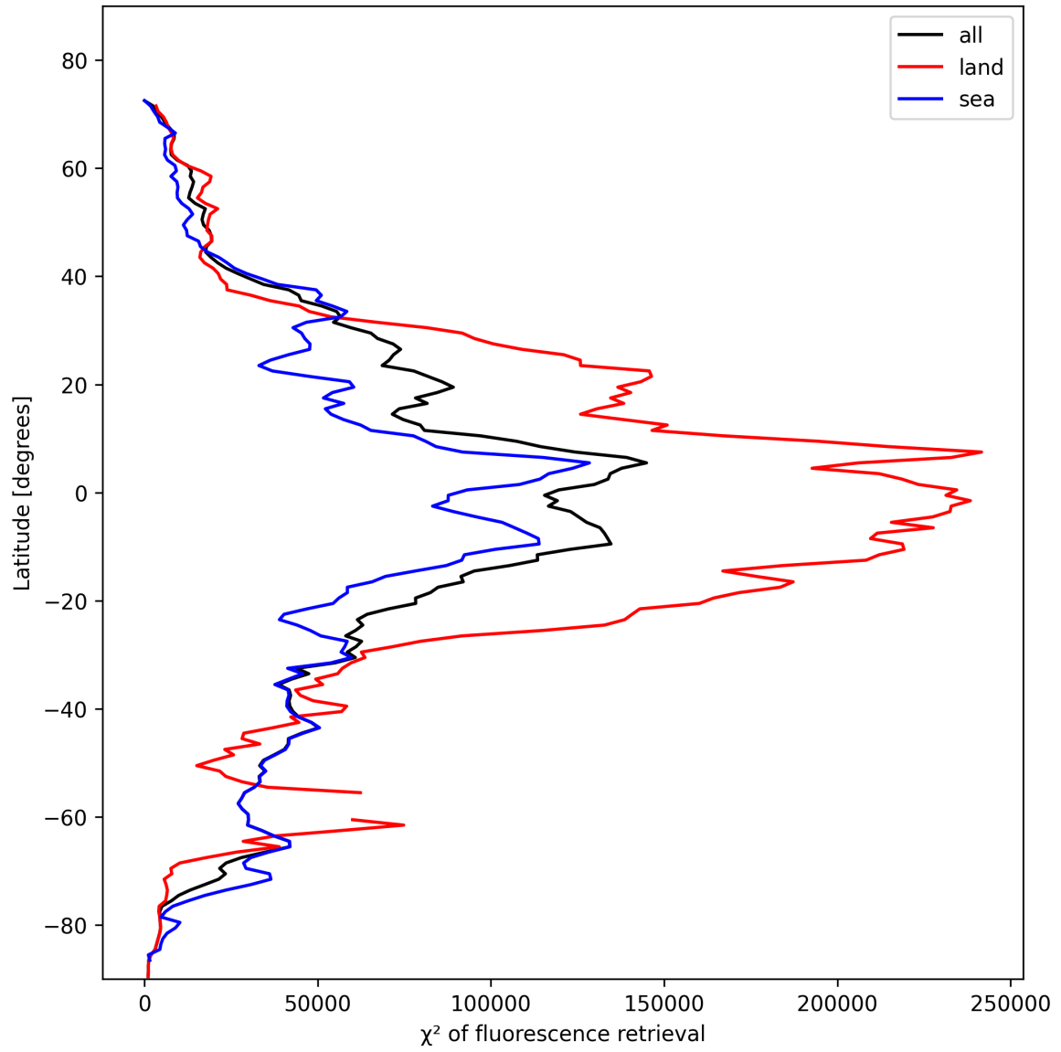
Figure 25: Zonal average of “ \chi^2 of fluorescence retrieval” for 2025-11-05 to 2025-11-07.
