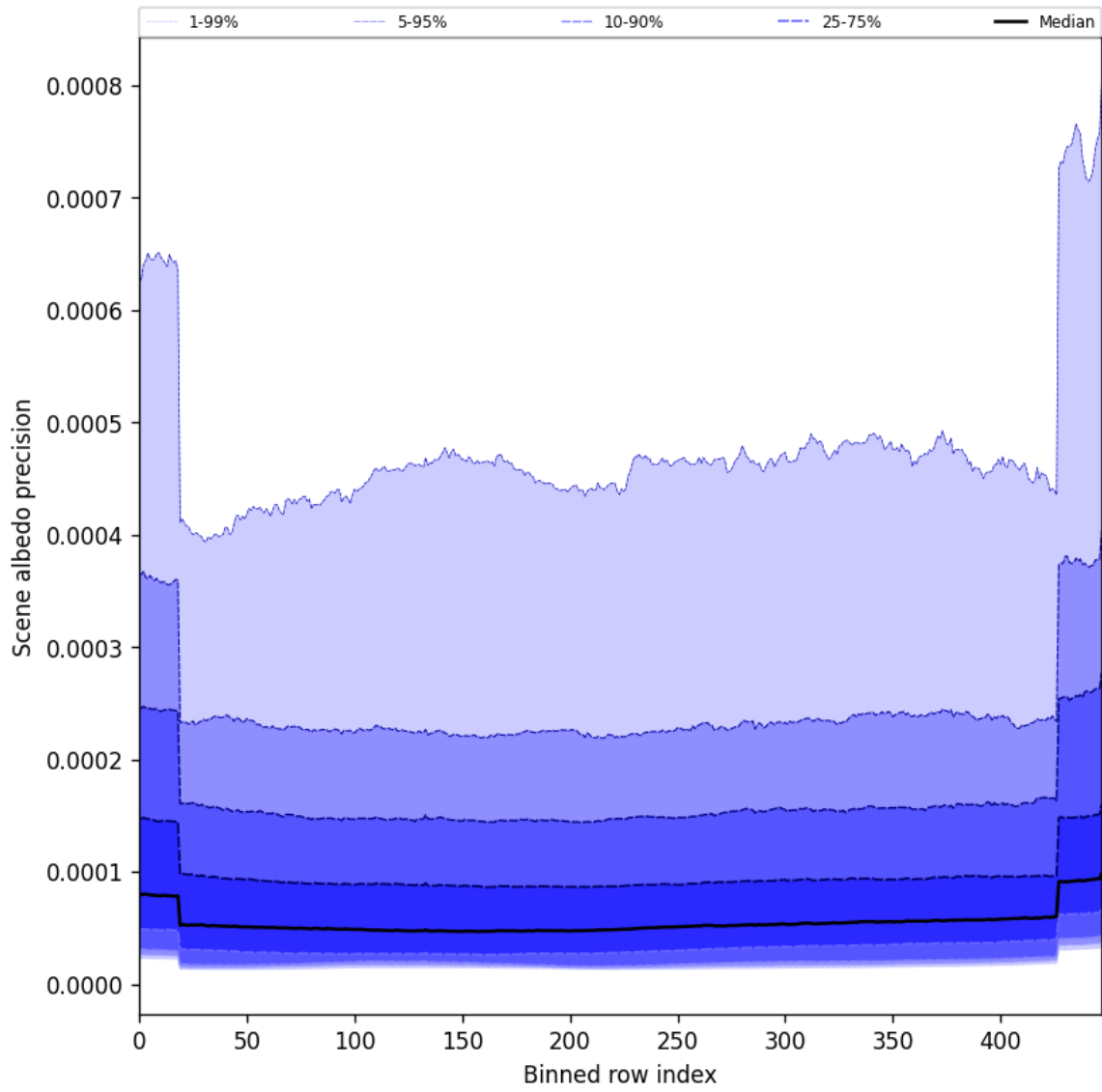
Figure 52: Along track statistics of “Scene albedo precision” for 2025-11-05 to 2025-11-07
