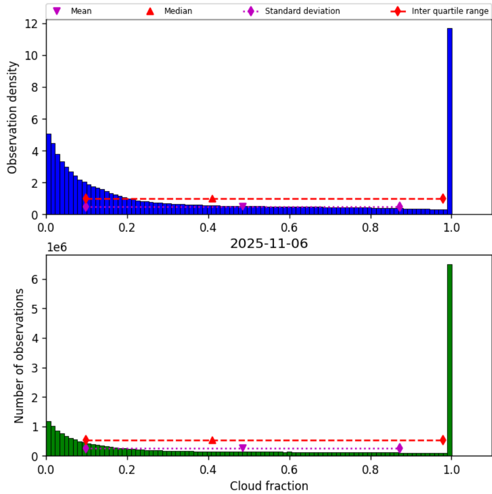
Figure 32: Histogram of “Cloud fraction” for 2025-11-05 to 2025-11-07
