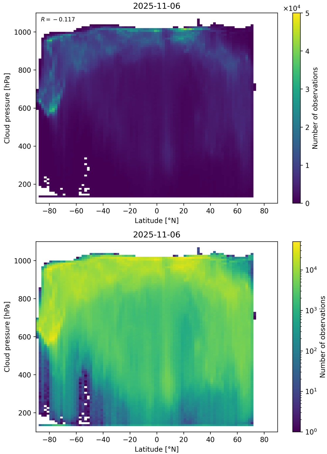
Figure 91: Scatter density plot of “Latitude” against “Cloud pressure” for 2025-11-05 to 2025-11-07.
