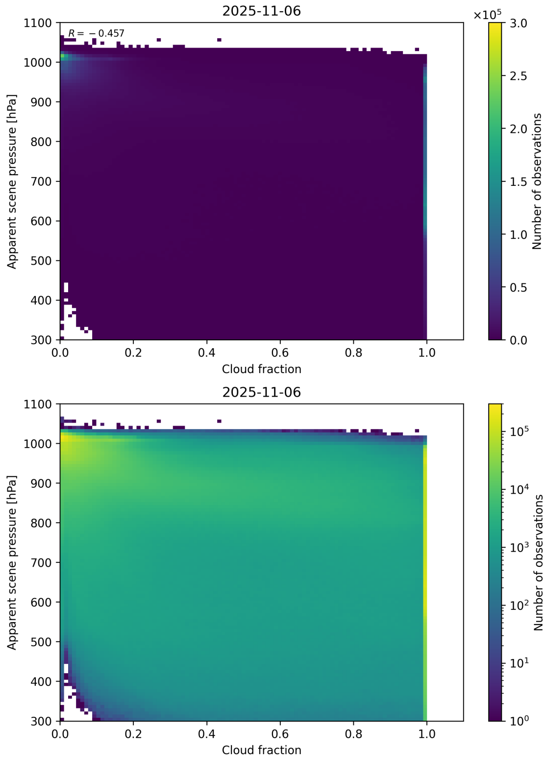
Figure 70: Scatter density plot of “Cloud fraction” against “Apparent scene pressure” for 2025-11-05 to 2025-11-07.
