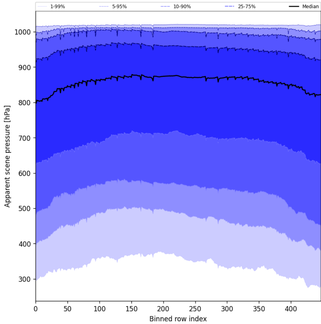
Figure 53: Along track statistics of “Apparent scene pressure” for 2025-11-05 to 2025-11-07
