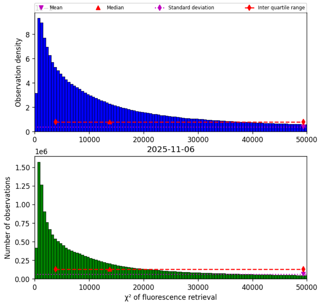
Figure 42: Histogram of “ \chi^2 of fluorescence retrieval” for 2025-11-05 to 2025-11-07
