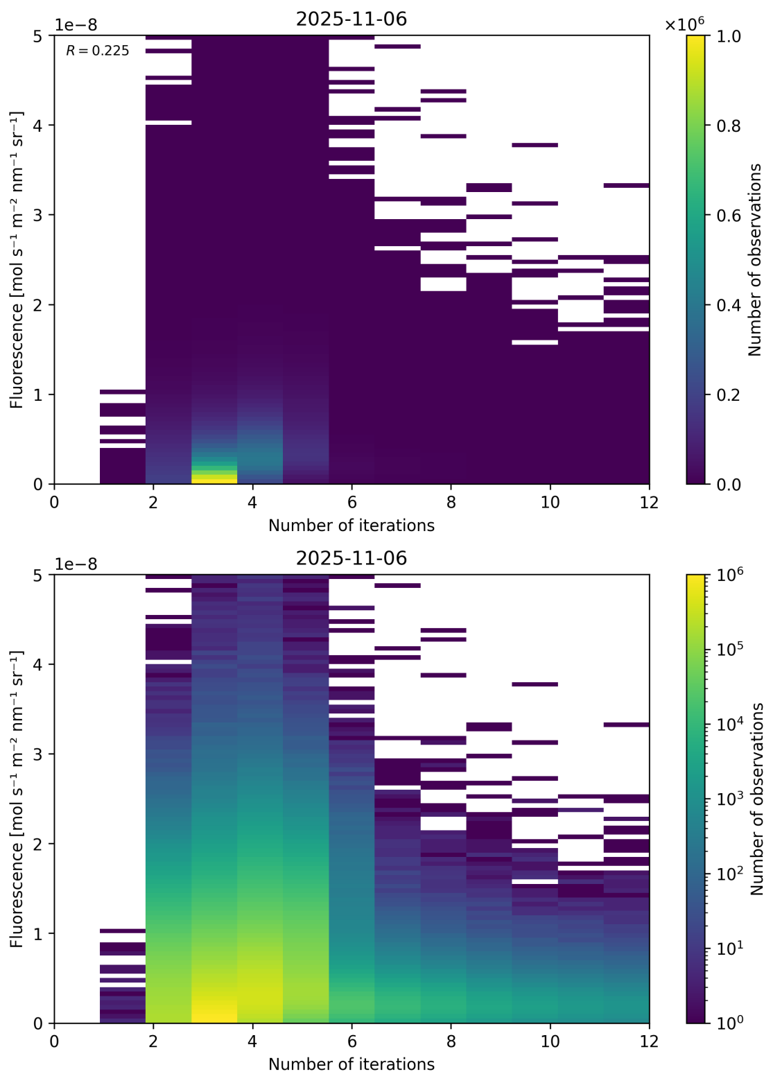
Figure 98: Scatter density plot of "Number of iterations" against "Fluorescence" for 2025-11-05 to 2025-11-07.
