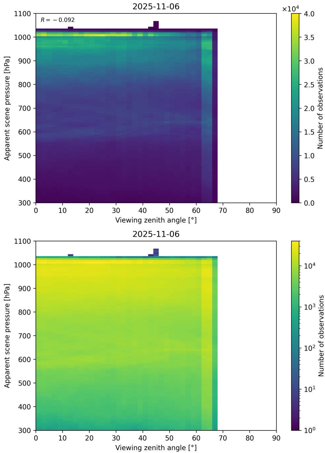
Figure 118: Scatter density plot of “Viewing zenith angle” against “Apparent scene pressure” for 2025-11-05 to 2025-11-07.
