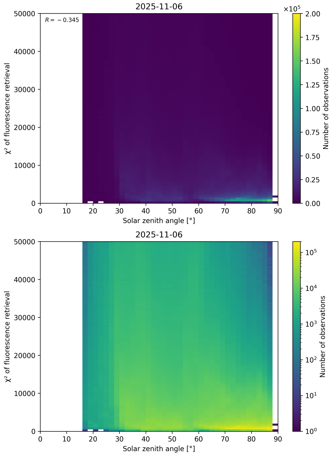
Figure 109: Scatter density plot of “Solar zenith angle” against “ \chi^2 of fluorescence retrieval” for 2025-11-05 to 2025-11-07.
