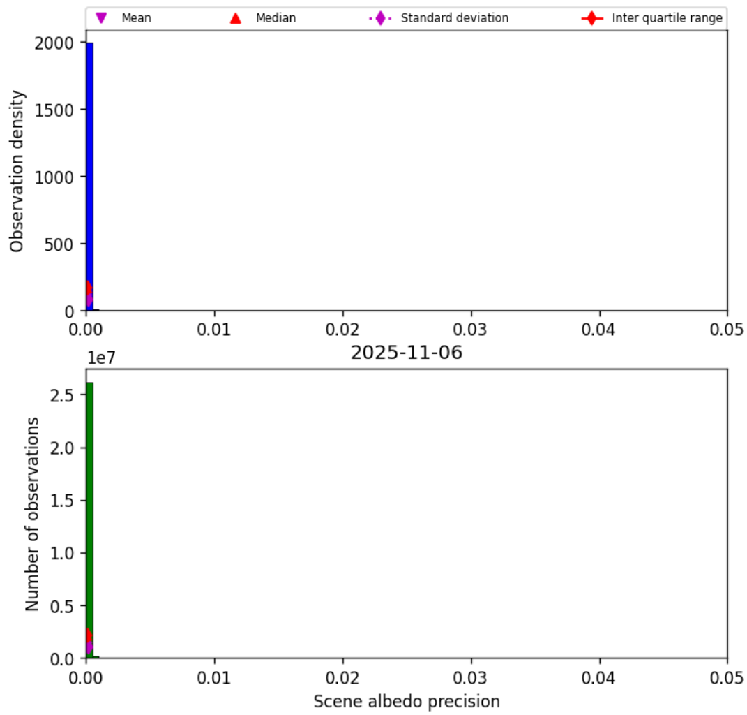
Figure 35: Histogram of “Scene albedo precision” for 2025-11-05 to 2025-11-07
