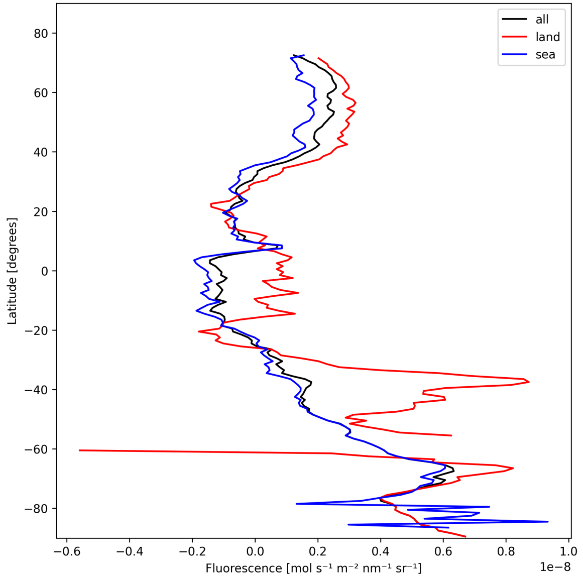
Figure 23: Zonal average of “Fluorescence” for 2025-11-05 to 2025-11-07.
