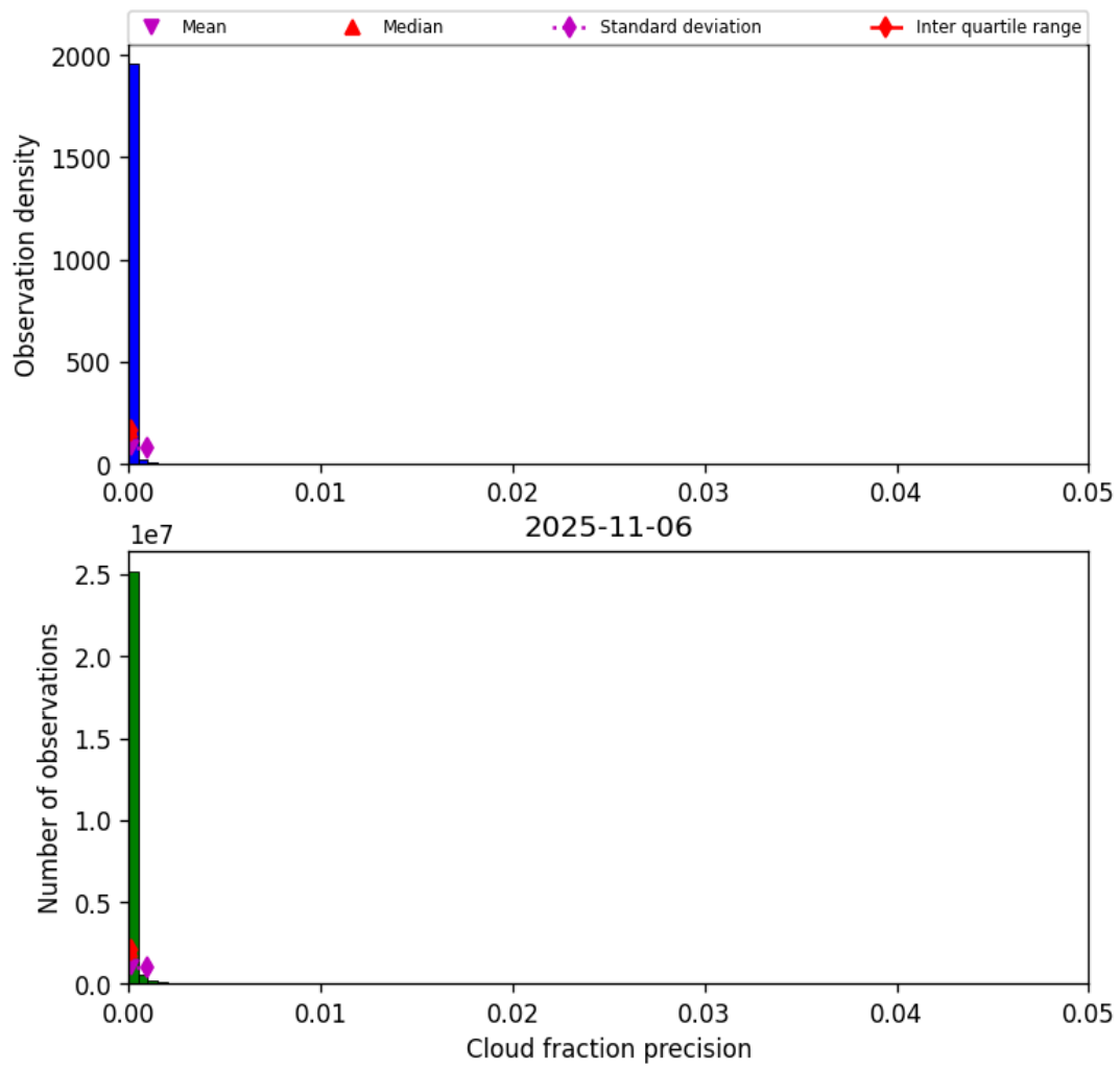
Figure 33: Histogram of “Cloud fraction precision” for 2025-11-05 to 2025-11-07
