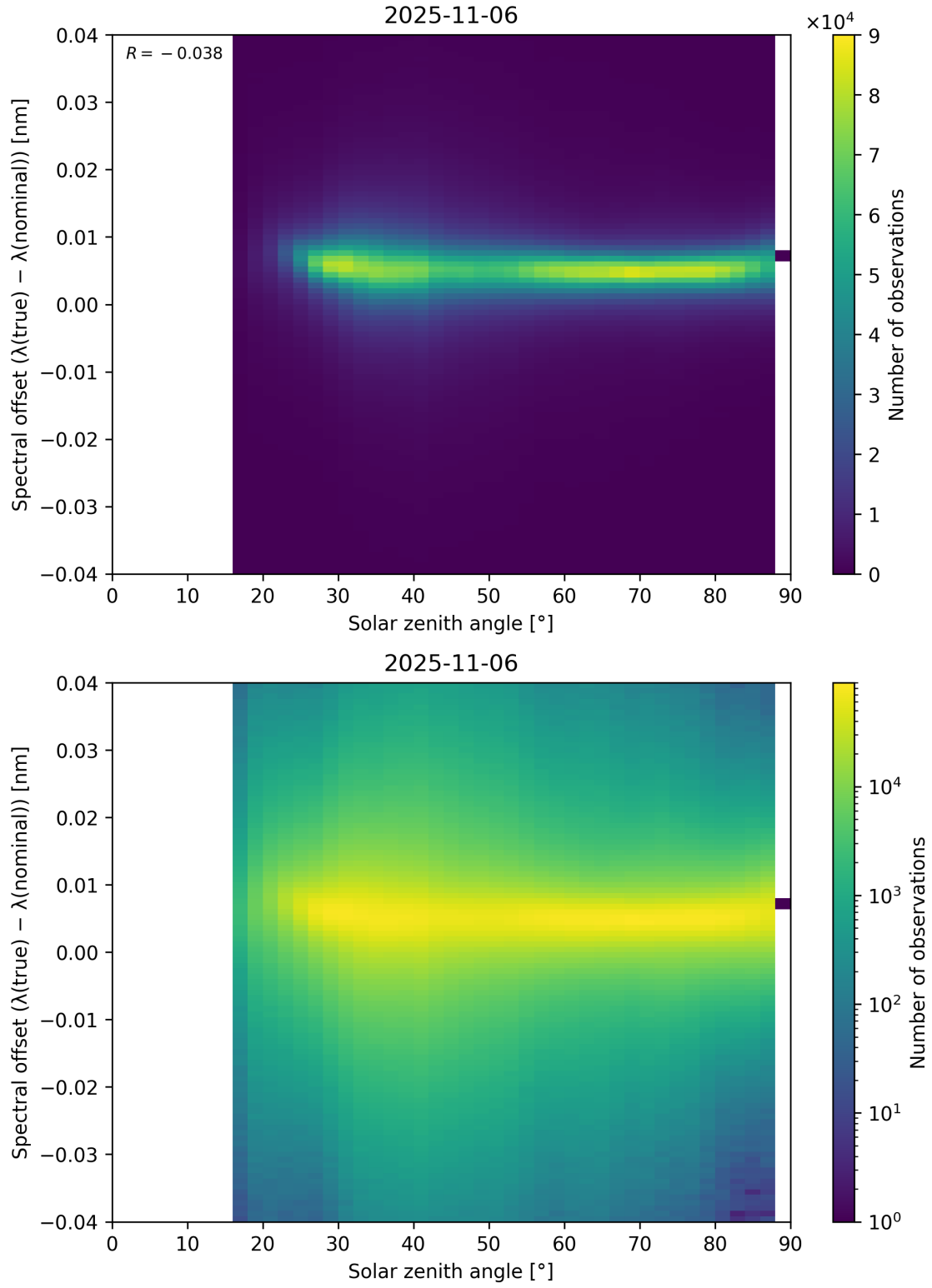
Figure 117: Scatter density plot of “Solar zenith angle” against “Spectral offset ( \lambda_{\text{true}} - \lambda_{\text{nominal}} )” for 2025-11-05 to 2025-11-07.
