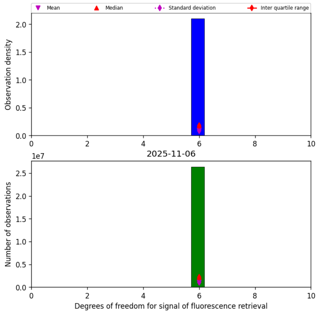
Figure 43: Histogram of "Degrees of freedom for signal of fluorescence retrieval" for 2025-11-05 to 2025-11-07
