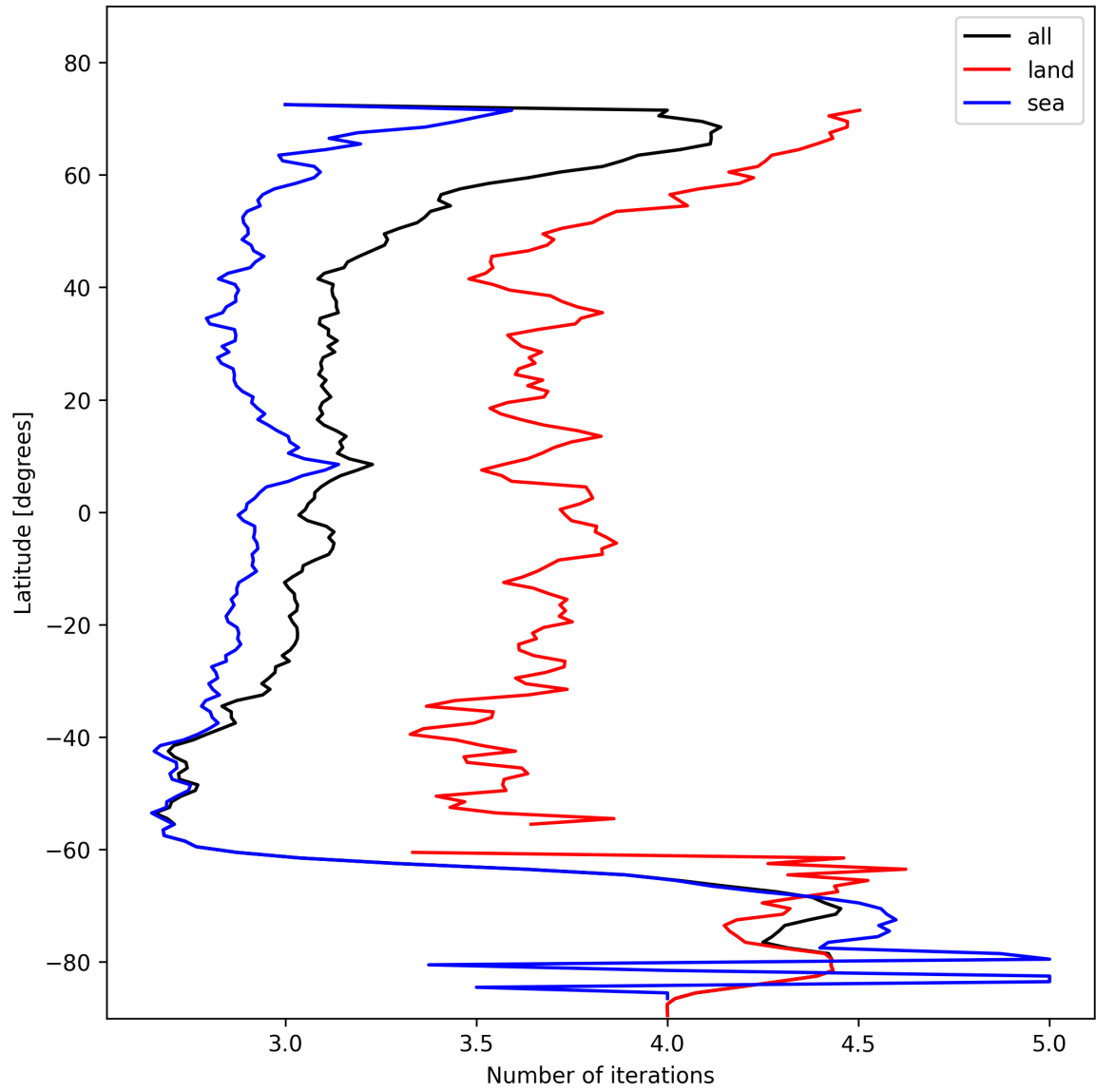
Figure 22: Zonal average of “Number of iterations” for 2025-11-05 to 2025-11-07.
