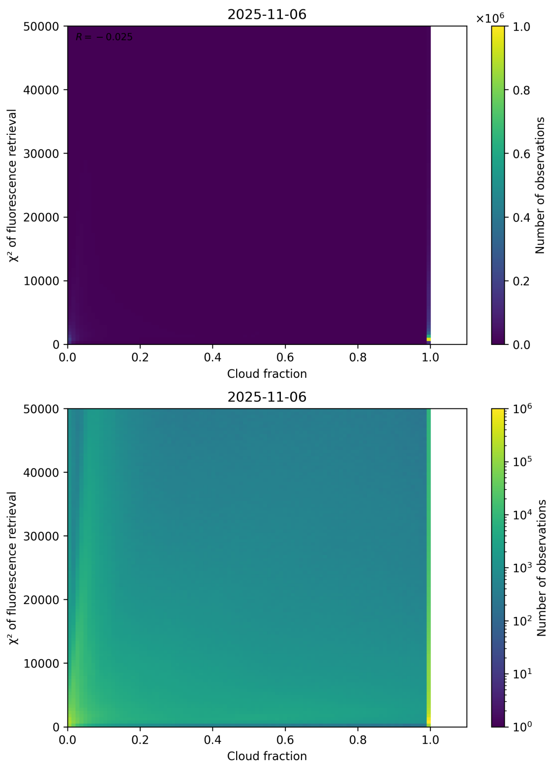
Figure 71: Scatter density plot of “Cloud fraction” against “ \chi^2 of fluorescence retrieval” for 2025-11-05 to 2025-11-07.
