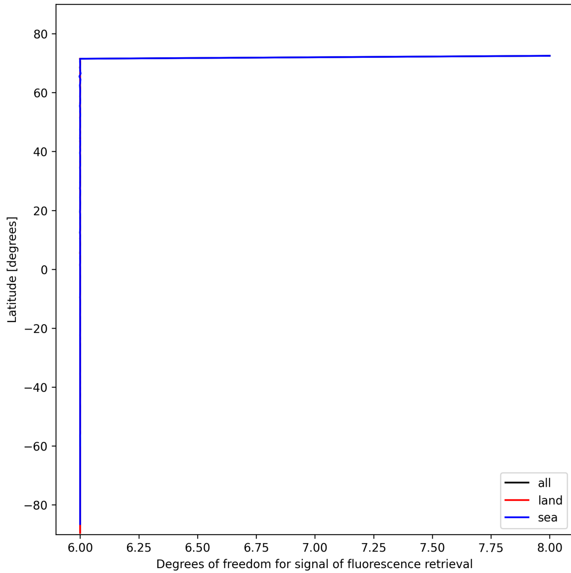
Figure 26: Zonal average of “Degrees of freedom for signal of fluorescence retrieval” for 2025-11-05 to 2025-11-07.
