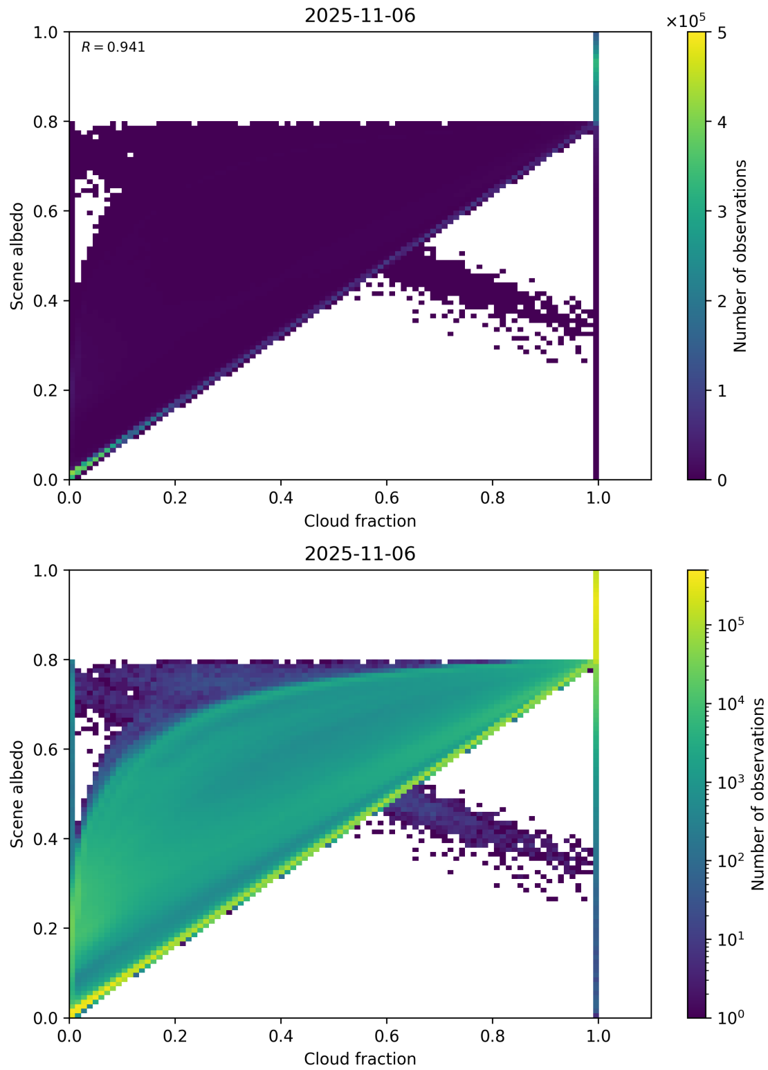
Figure 75: Scatter density plot of “Cloud fraction” against “Scene albedo” for 2025-11-05 to 2025-11-07.
