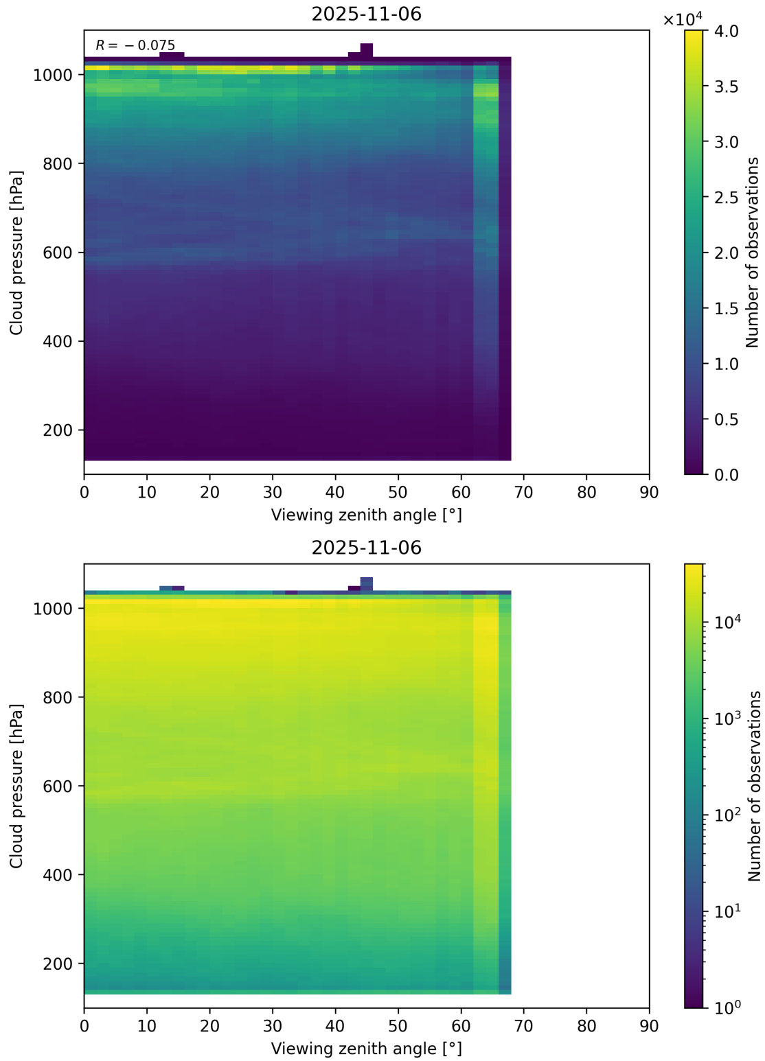
Figure 121: Scatter density plot of “Viewing zenith angle” against “Cloud pressure” for 2025-11-05 to 2025-11-07.
