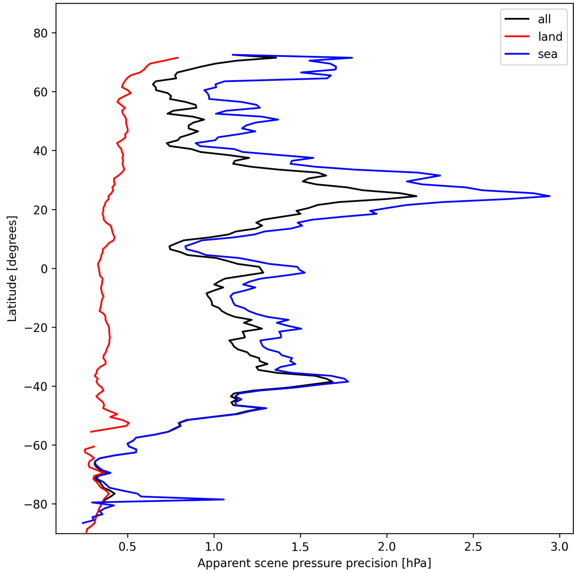
Figure 20: Zonal average of “Apparent scene pressure precision” for 2025-11-05 to 2025-11-07.
