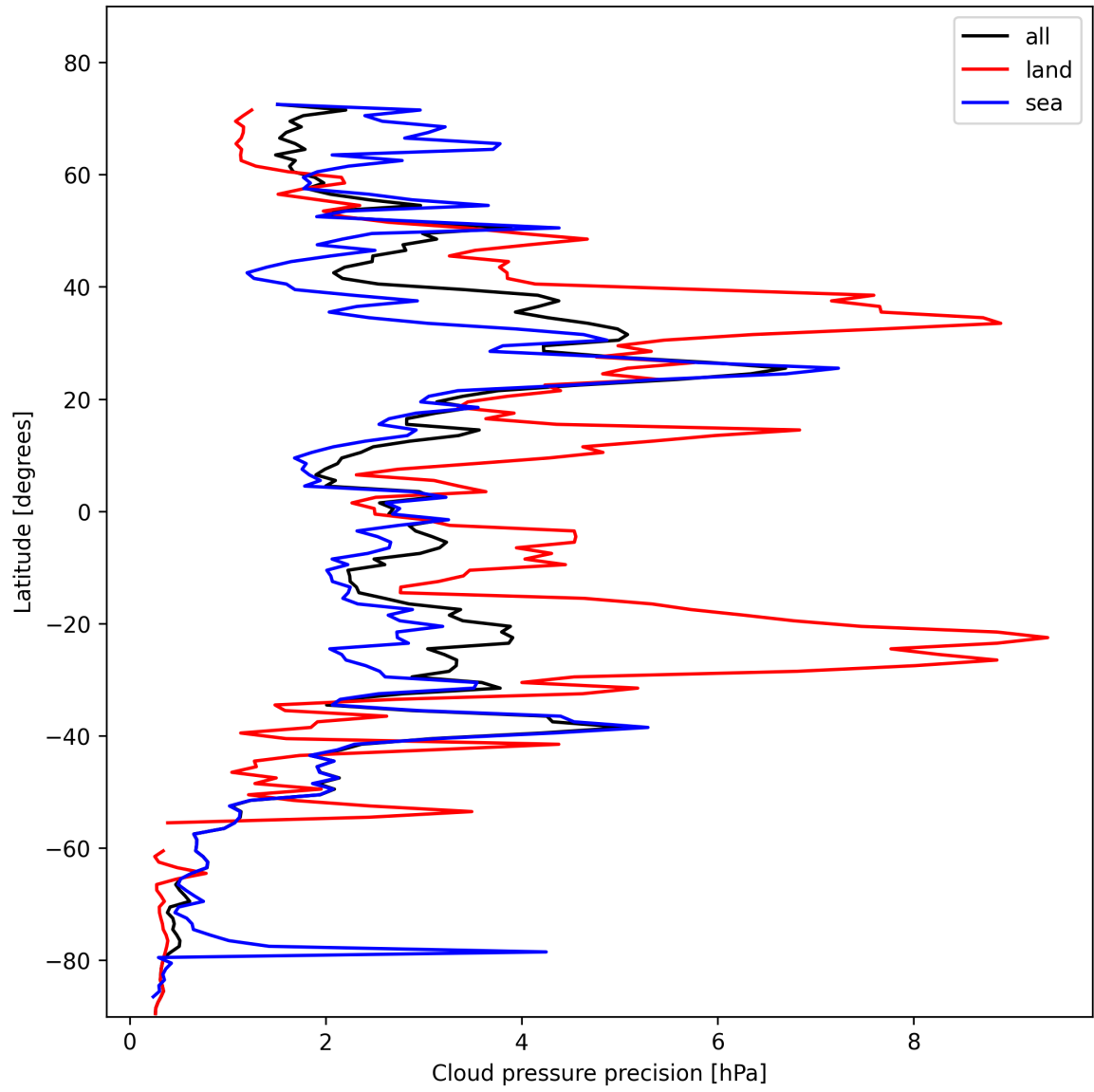
Figure 14: Zonal average of "Cloud pressure precision" for 2025-11-05 to 2025-11-07.
