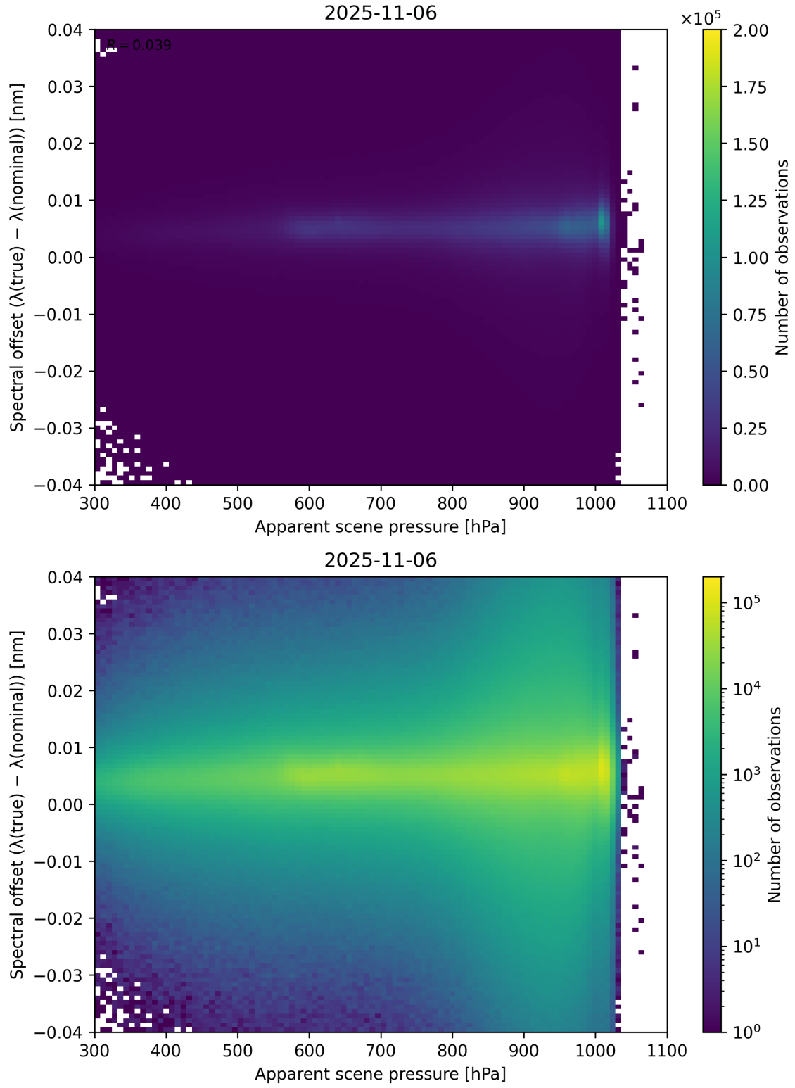
Figure 67: Scatter density plot of “Apparent scene pressure” against “Spectral offset ( \lambda_{\text{true}} - \lambda_{\text{nominal}} )” for 2025-11-05 to 2025-11-07.
