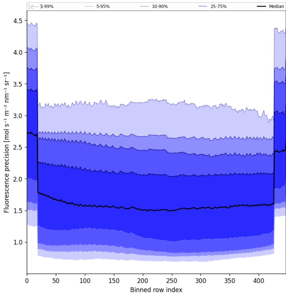
Figure 58: Along track statistics of “Fluorescence precision” for 2025-11-05 to 2025-11-07
