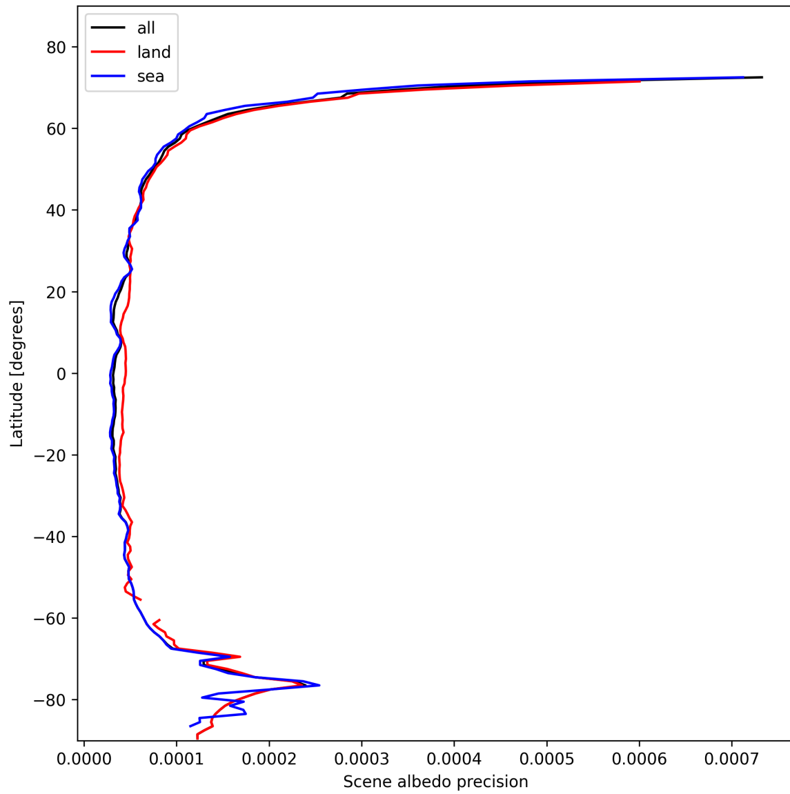
Figure 18: Zonal average of “Scene albedo precision” for 2025-11-05 to 2025-11-07.
