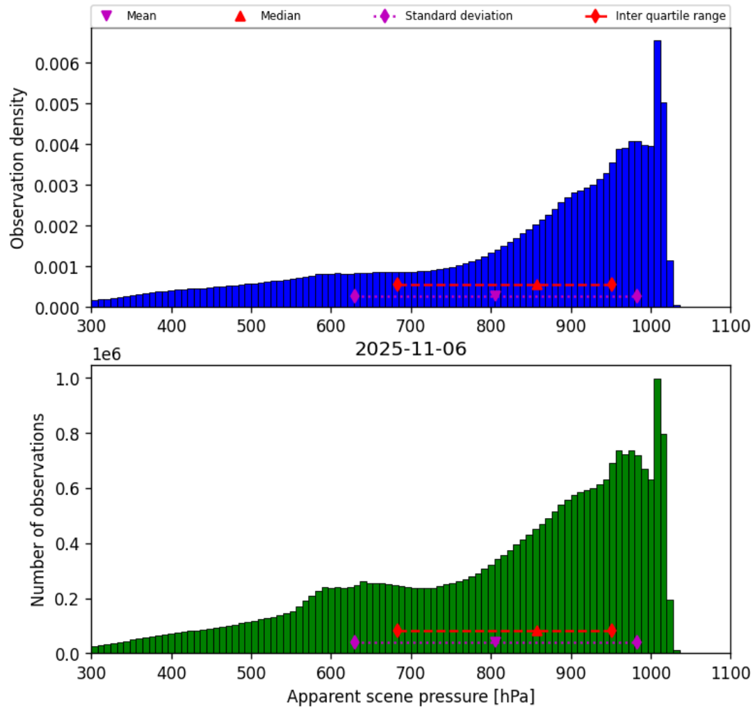
Figure 36: Histogram of “Apparent scene pressure” for 2025-11-05 to 2025-11-07
