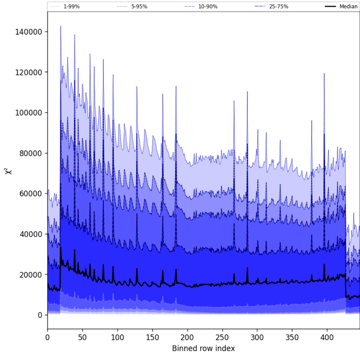
Figure 55: Along track statistics of “ \chi^2 ” for 2025-11-05 to 2025-11-07
