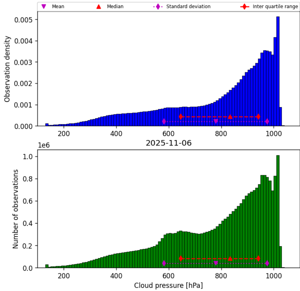
Figure 30: Histogram of “Cloud pressure” for 2025-11-05 to 2025-11-07
