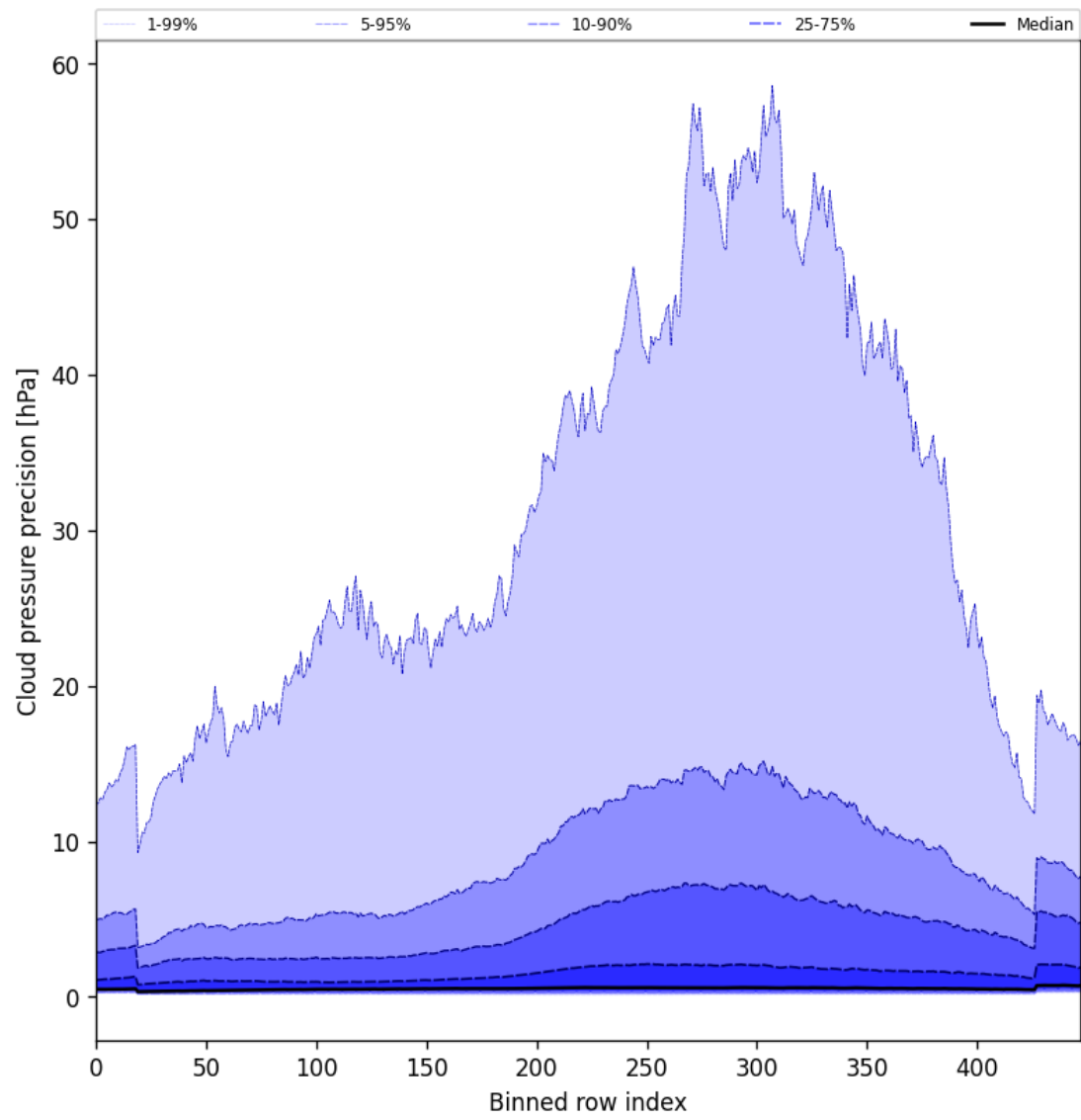
Figure 48: Along track statistics of “Cloud pressure precision” for 2025-11-05 to 2025-11-07
