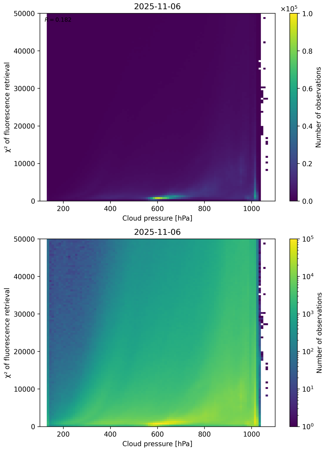
Figure 78: Scatter density plot of “Cloud pressure” against “ \chi^2 of fluorescence retrieval” for 2025-11-05 to 2025-11-07.
