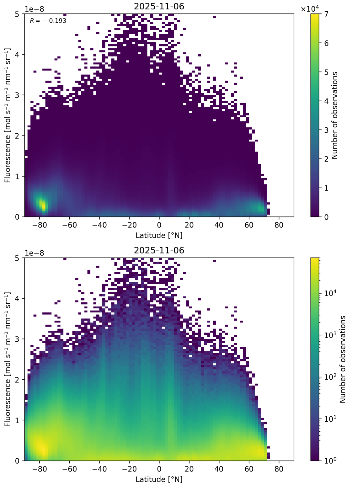
Figure 92: Scatter density plot of “Latitude” against “Fluorescence” for 2025-11-05 to 2025-11-07.
