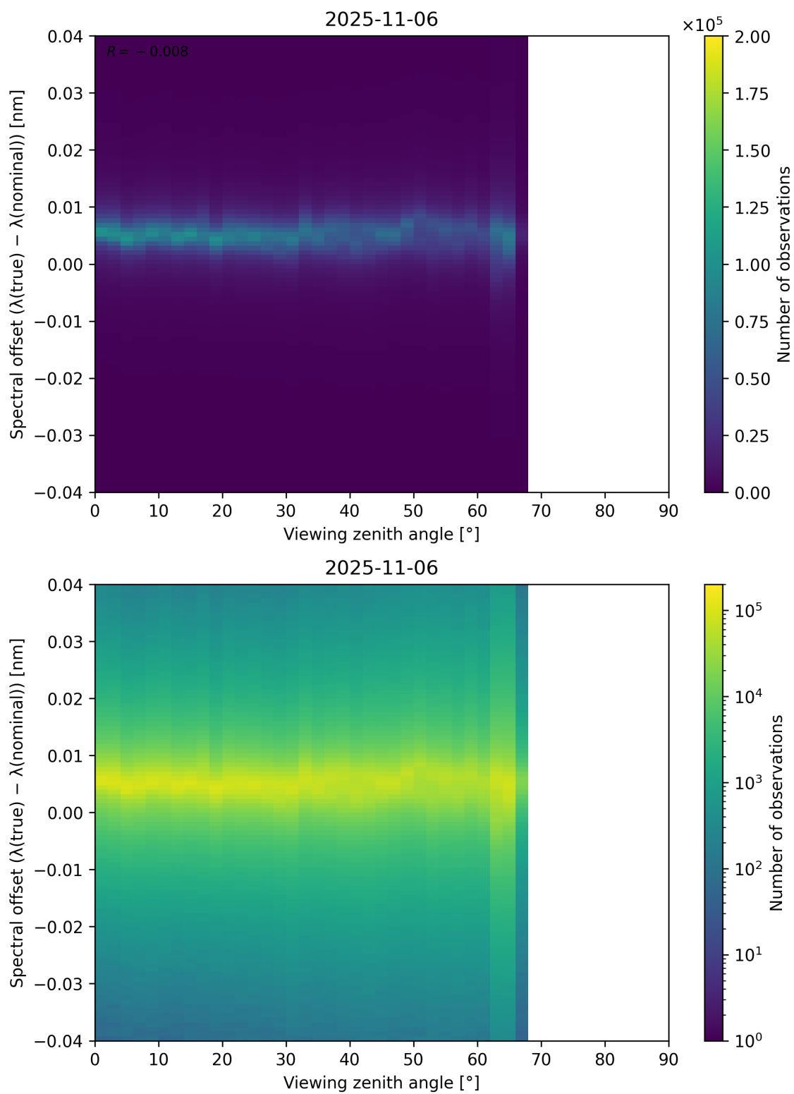
Figure 128: Scatter density plot of “Viewing zenith angle” against “Spectral offset ( \lambda_{\text{true}} - \lambda_{\text{nominal}} )” for 2025-11-05 to 2025-11-07.
