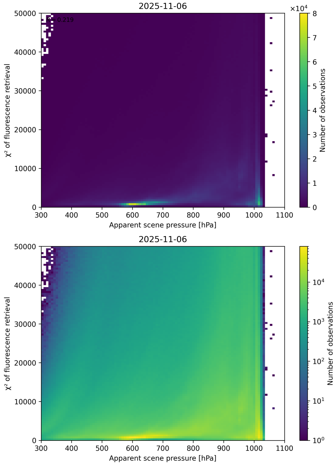
Figure 63: Scatter density plot of “Apparent scene pressure” against “ \chi^2 of fluorescence retrieval” for 2025-11-05 to 2025-11-07.
