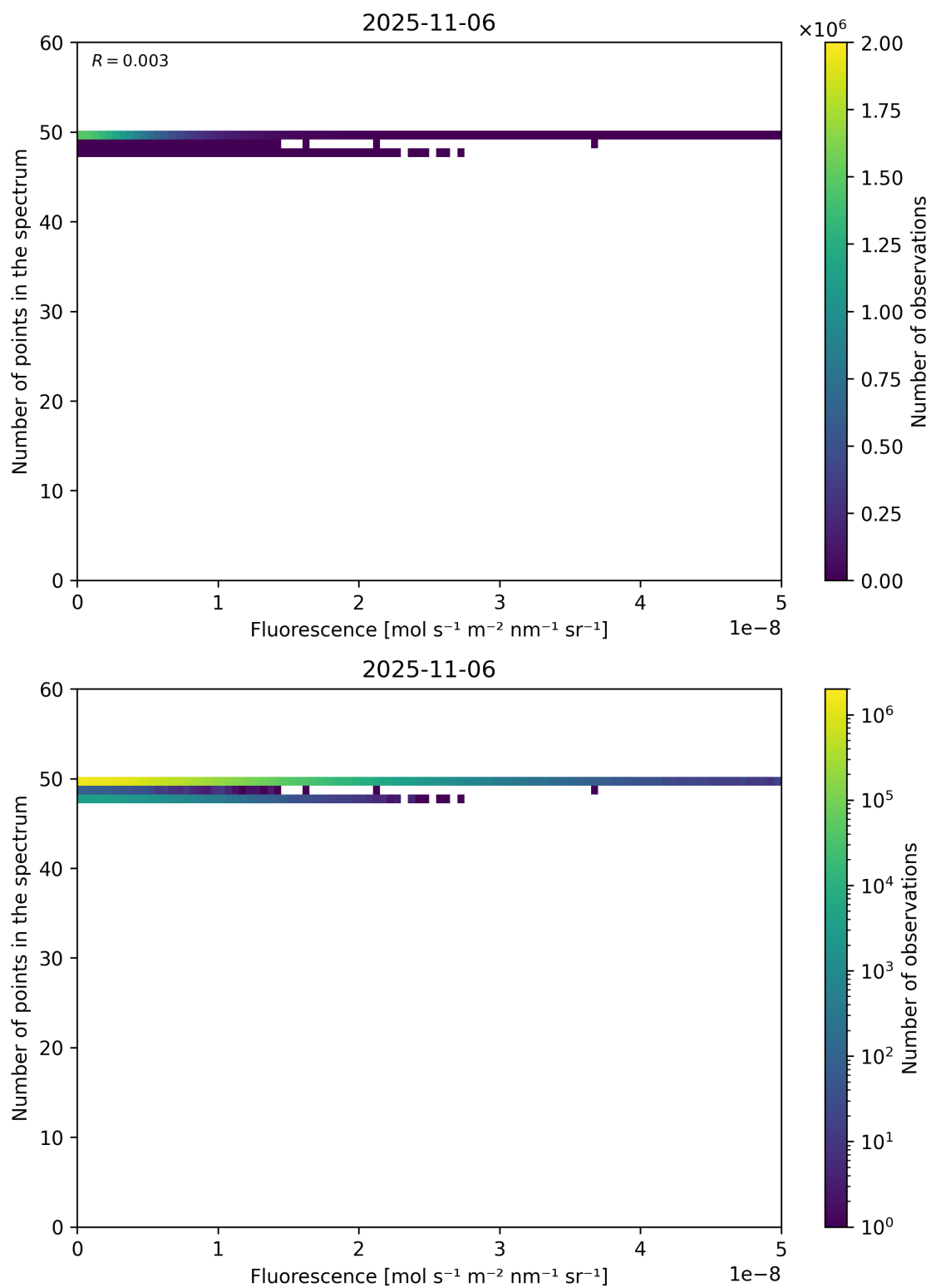
Figure 86: Scatter density plot of “Fluorescence” against “Number of points in the spectrum” for 2025-11-05 to 2025-11-07.
