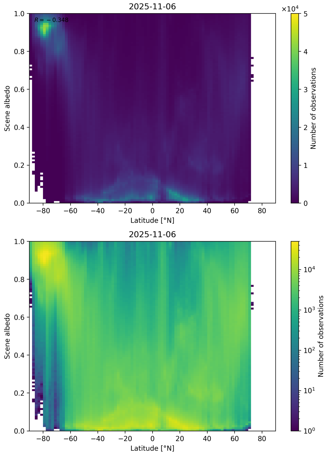
Figure 95: Scatter density plot of “Latitude” against “Scene albedo” for 2025-11-05 to 2025-11-07.
