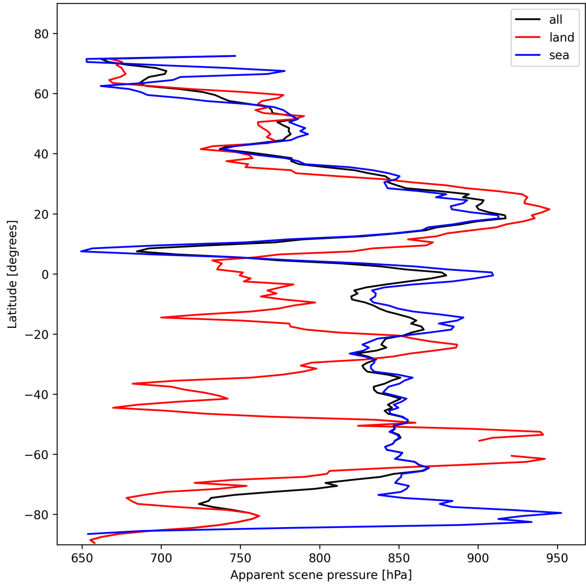
Figure 19: Zonal average of “Apparent scene pressure” for 2025-11-05 to 2025-11-07.
