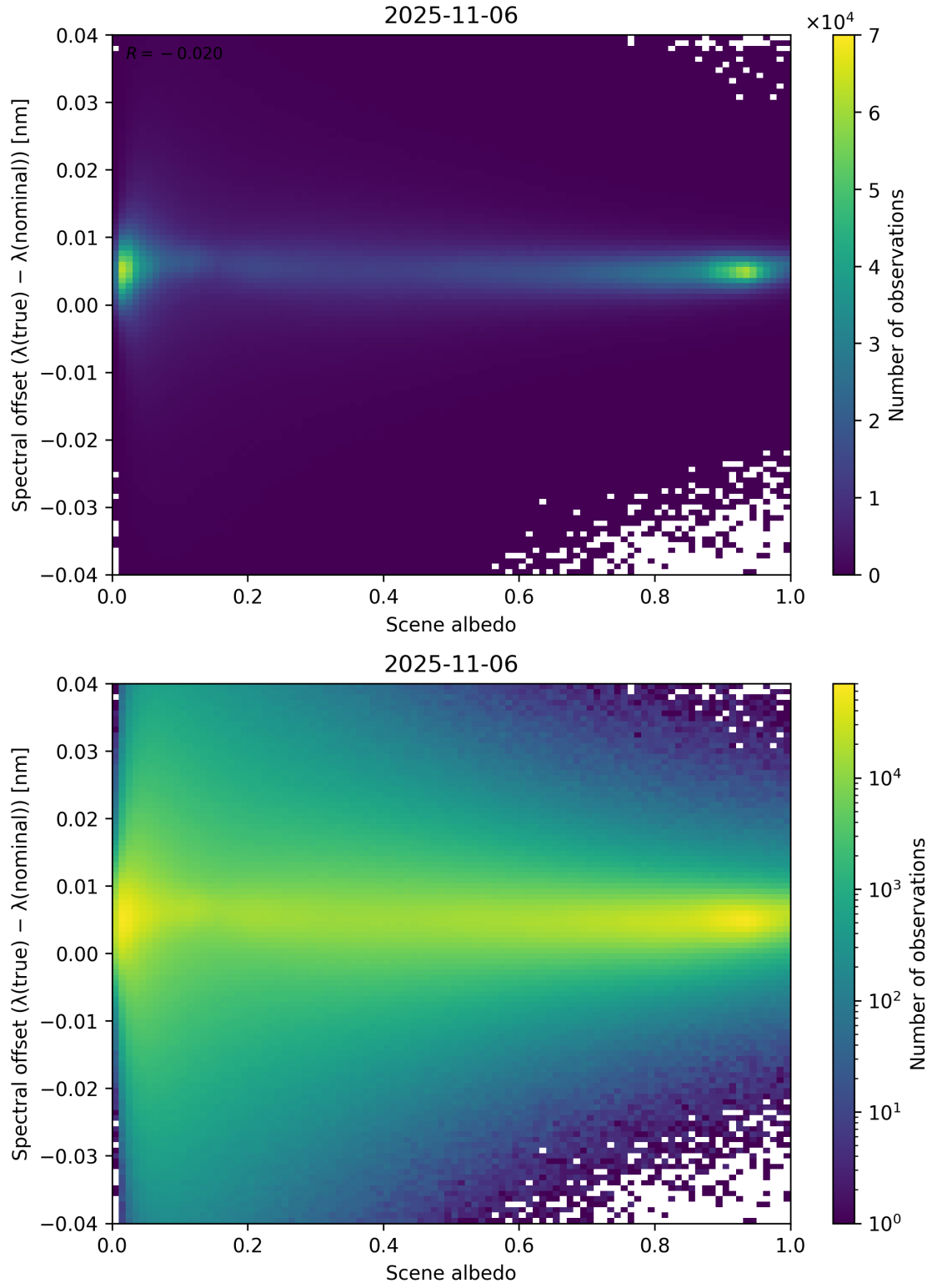
Figure 107: Scatter density plot of “Scene albedo” against “Spectral offset ( \lambda_{\text{true}} - \lambda_{\text{nominal}} )” for 2025-11-05 to 2025-11-07.
