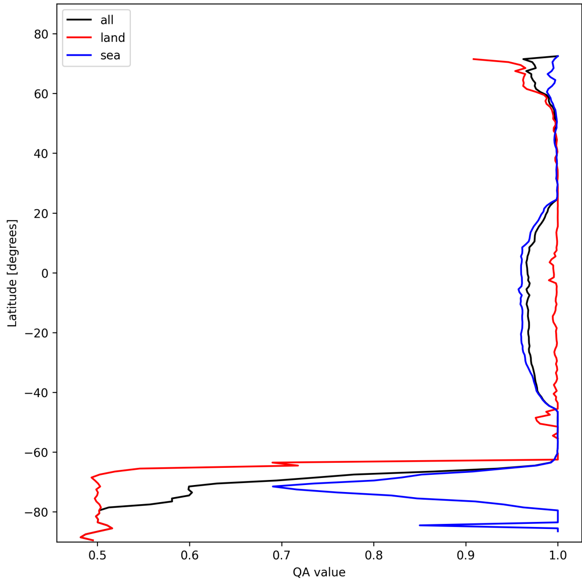
Figure 12: Zonal average of “QA value” for 2025-11-05 to 2025-11-07.
