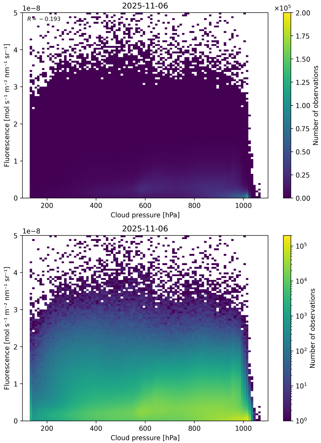
Figure 80: Scatter density plot of “Cloud pressure” against “Fluorescence” for 2025-11-05 to 2025-11-07.
