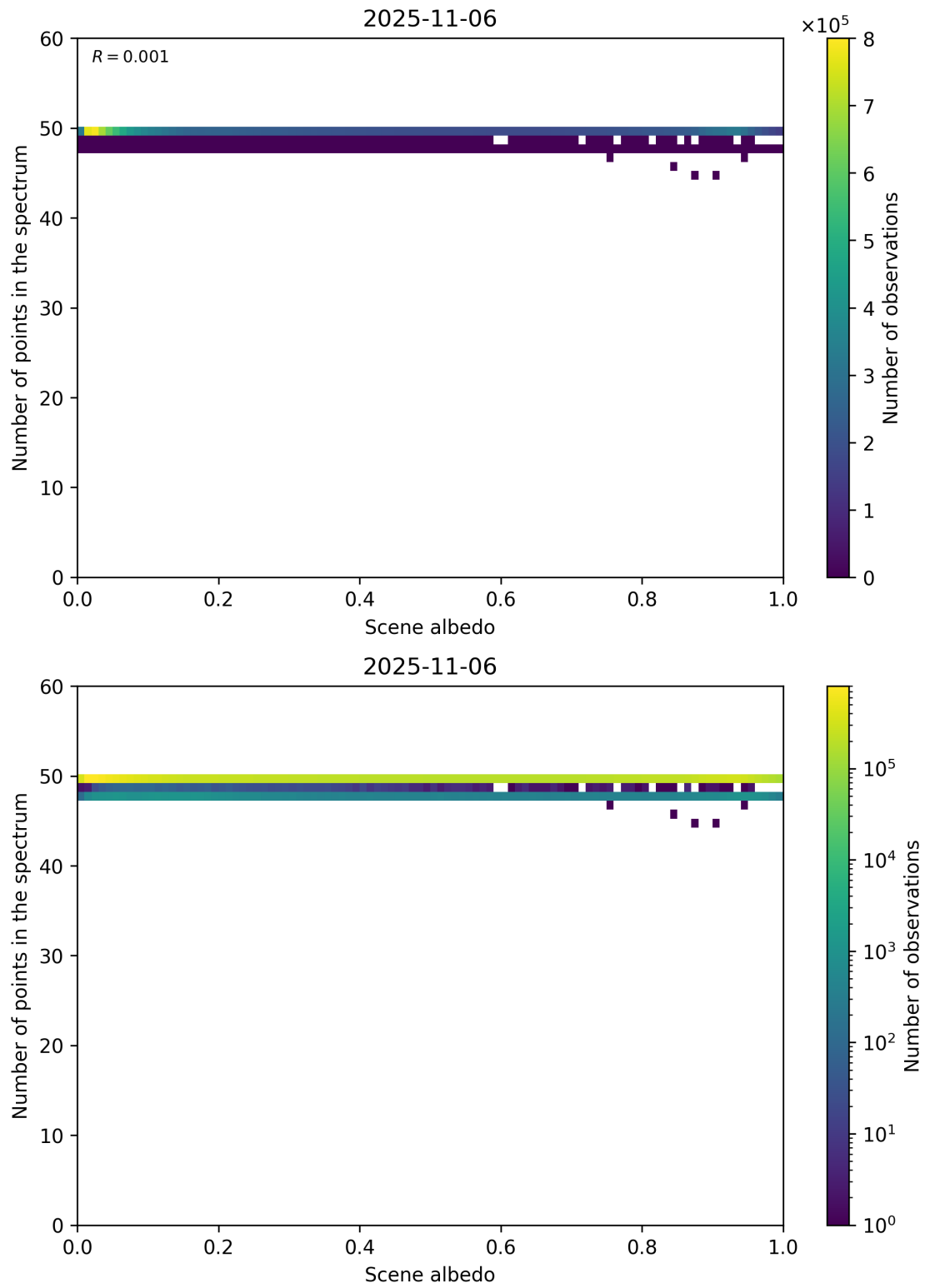
Figure 106: Scatter density plot of “Scene albedo” against “Number of points in the spectrum” for 2025-11-05 to 2025-11-07.
