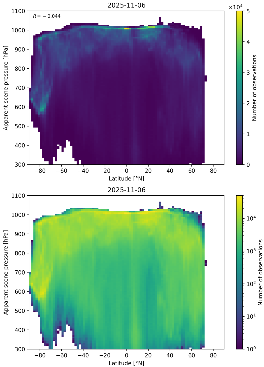
Figure 88: Scatter density plot of “Latitude” against “Apparent scene pressure” for 2025-11-05 to 2025-11-07.
