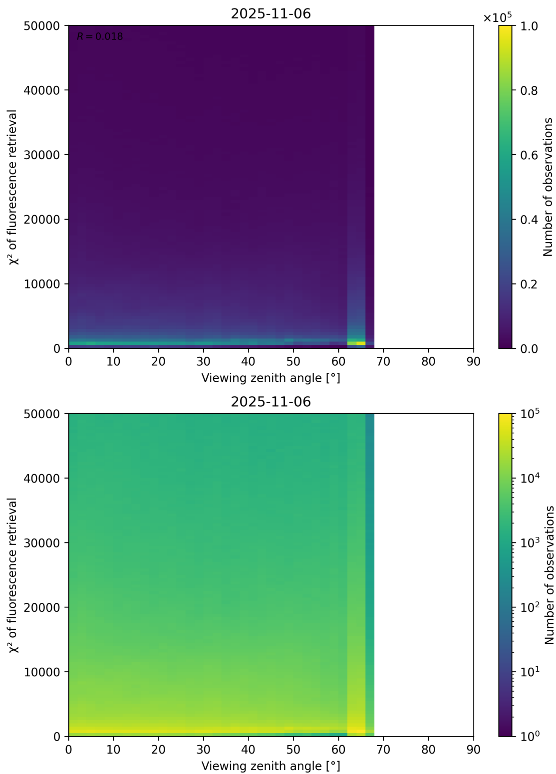
Figure 119: Scatter density plot of “Viewing zenith angle” against “ \chi^2 of fluorescence retrieval” for 2025-11-05 to 2025-11-07.
