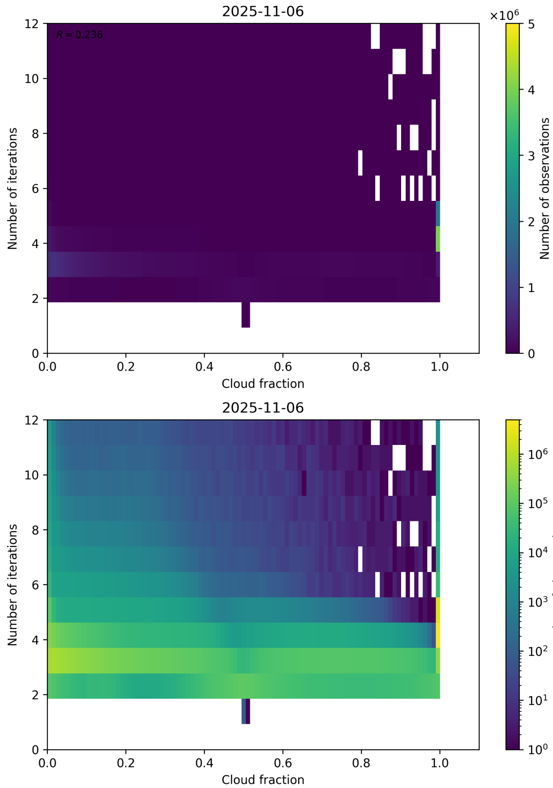
Figure 73: Scatter density plot of “Cloud fraction” against “Number of iterations” for 2025-11-05 to 2025-11-07.
