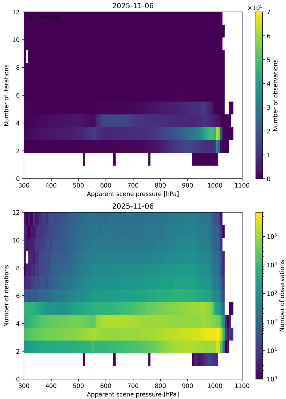
Figure 65: Scatter density plot of “Apparent scene pressure” against “Number of iterations” for 2025-11-05 to 2025-11-07.
