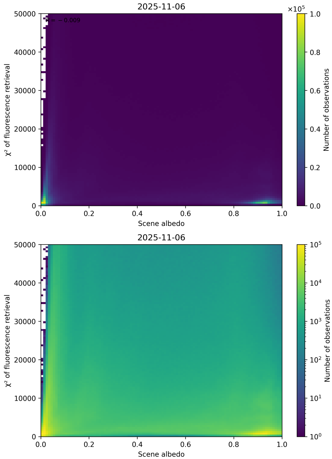
Figure 103: Scatter density plot of “Scene albedo” against “ \chi^2 of fluorescence retrieval” for 2025-11-05 to 2025-11-07.
