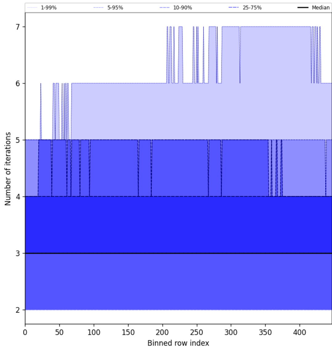
Figure 56: Along track statistics of “Number of iterations” for 2025-11-05 to 2025-11-07
