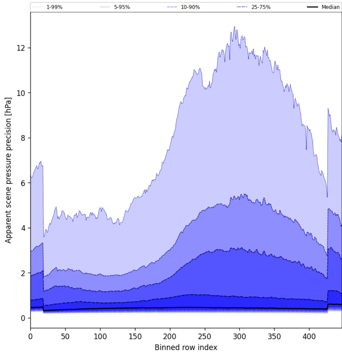
Figure 54: Along track statistics of “Apparent scene pressure precision” for 2025-11-05 to 2025-11-07
