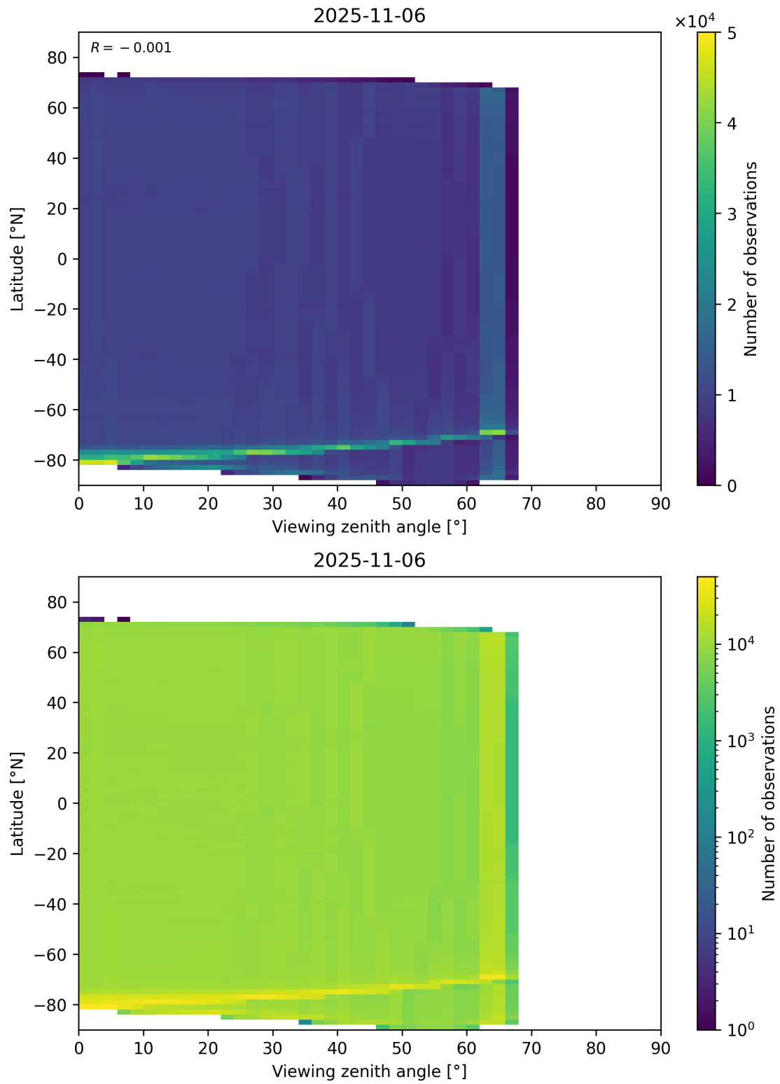
Figure 123: Scatter density plot of “Viewing zenith angle” against “Latitude” for 2025-11-05 to 2025-11-07.
