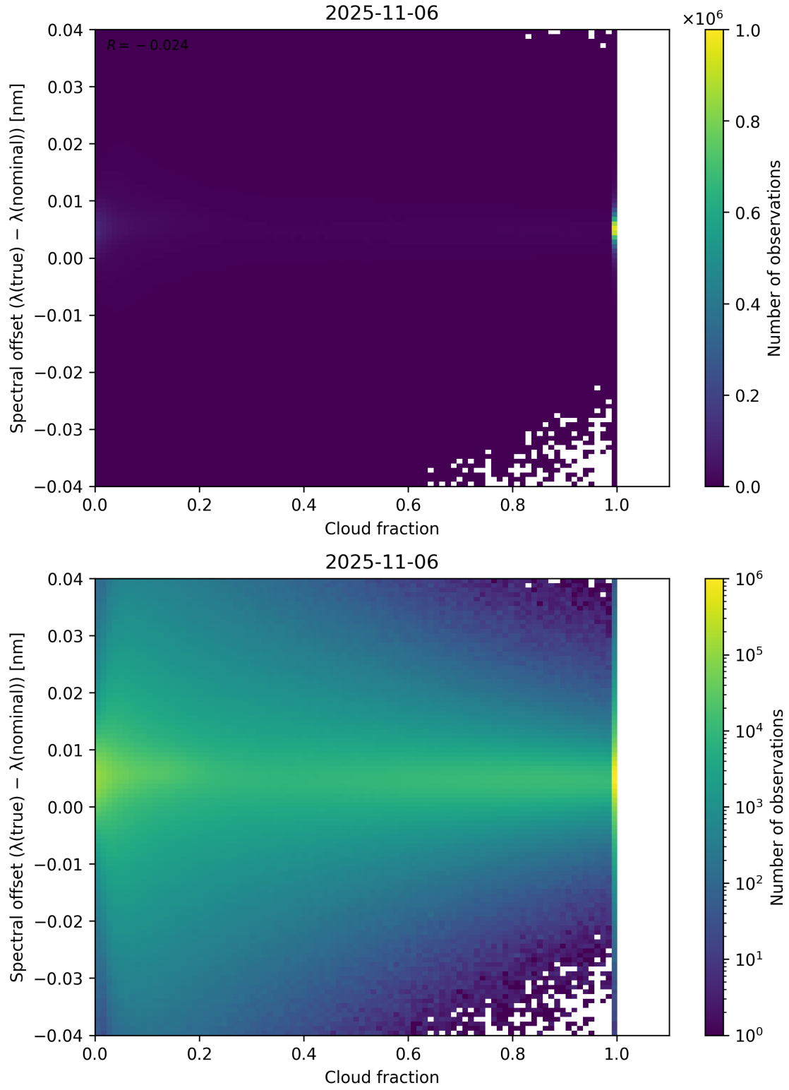
Figure 76: Scatter density plot of “Cloud fraction” against “Spectral offset ( \lambda_{\text{true}} - \lambda_{\text{nominal}} )” for 2025-11-05 to 2025-11-07.
