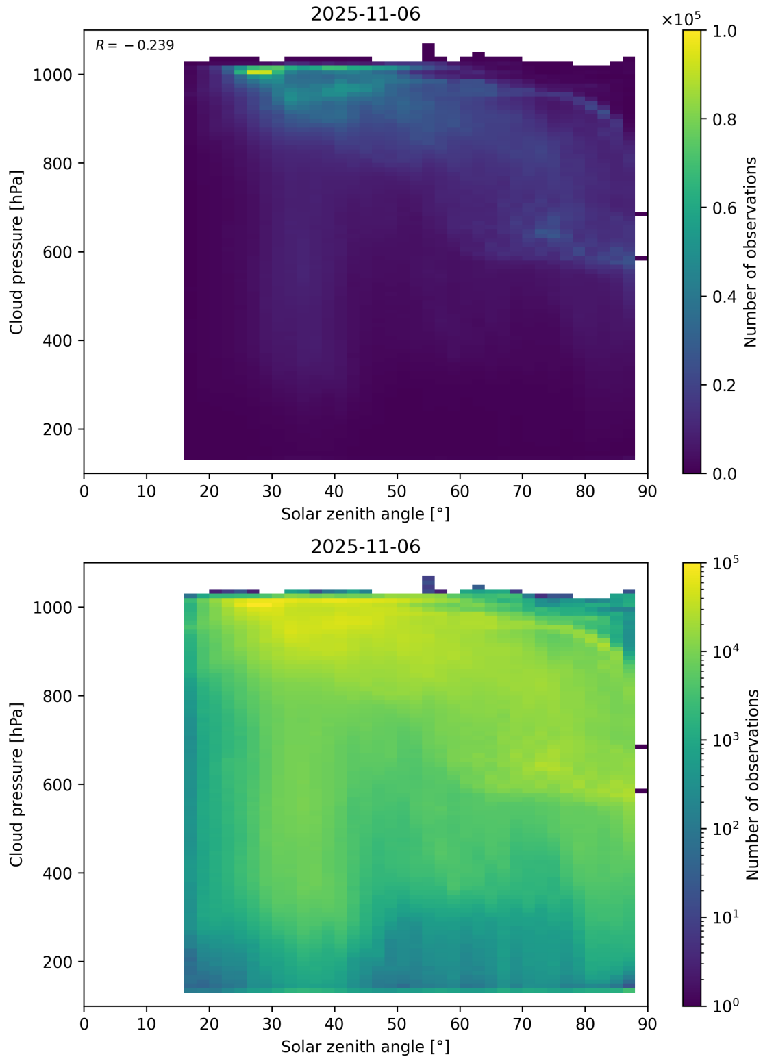
Figure 111: Scatter density plot of “Solar zenith angle” against “Cloud pressure” for 2025-11-05 to 2025-11-07.
