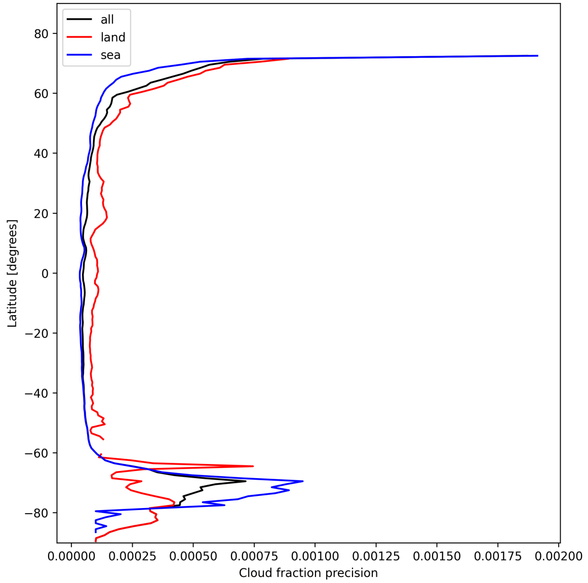
Figure 16: Zonal average of “Cloud fraction precision” for 2025-11-05 to 2025-11-07.
