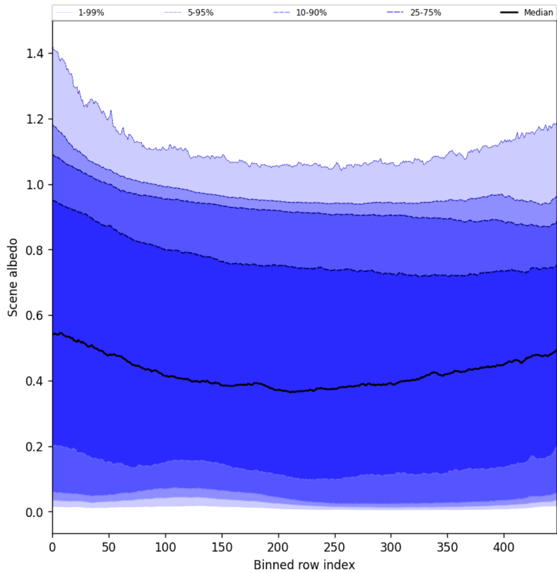
Figure 51: Along track statistics of “Scene albedo” for 2025-11-05 to 2025-11-07
