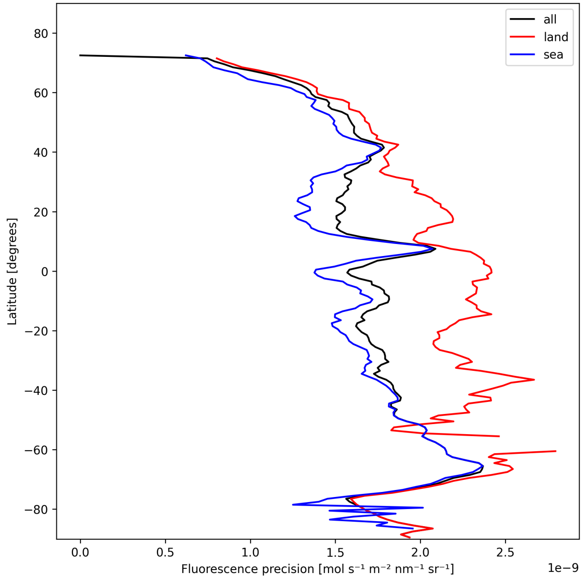
Figure 24: Zonal average of “Fluorescence precision” for 2025-11-05 to 2025-11-07.
