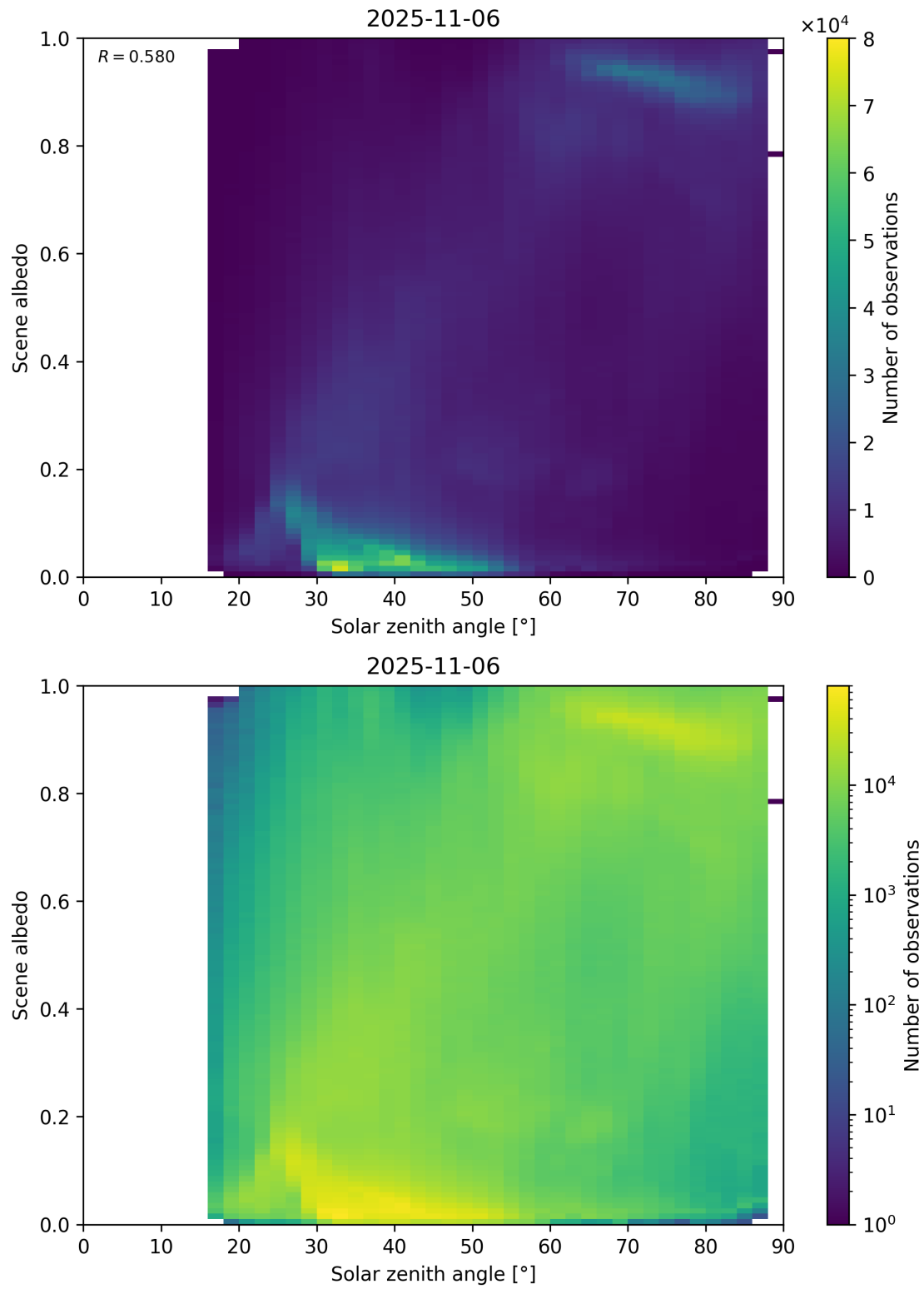
Figure 116: Scatter density plot of “Solar zenith angle” against “Scene albedo” for 2025-11-05 to 2025-11-07.
