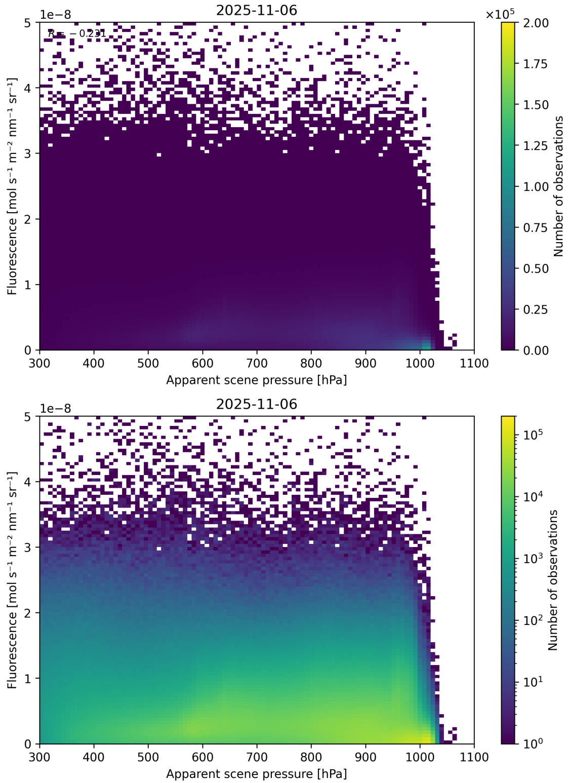
Figure 64: Scatter density plot of “Apparent scene pressure” against “Fluorescence” for 2025-11-05 to 2025-11-07.
