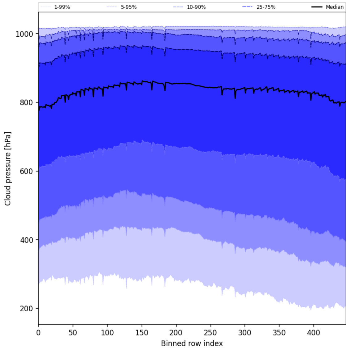
Figure 47: Along track statistics of “Cloud pressure” for 2025-11-05 to 2025-11-07
