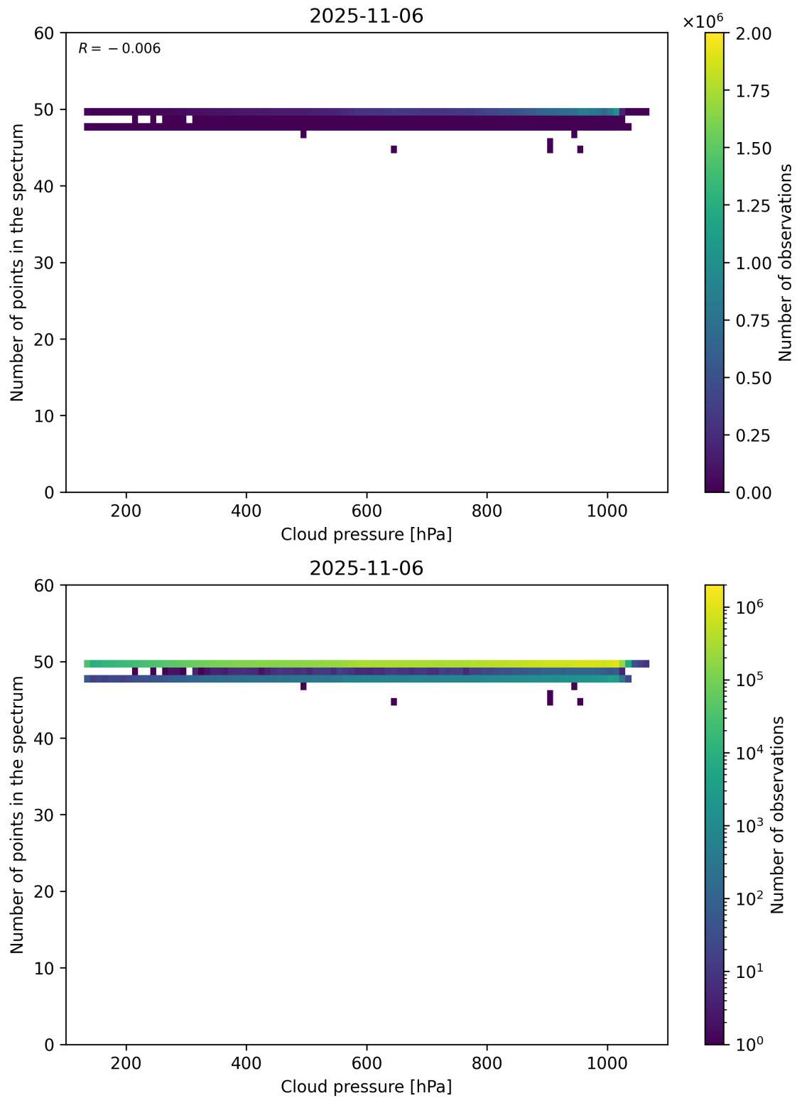
Figure 82: Scatter density plot of “Cloud pressure” against “Number of points in the spectrum” for 2025-11-05 to 2025-11-07.
