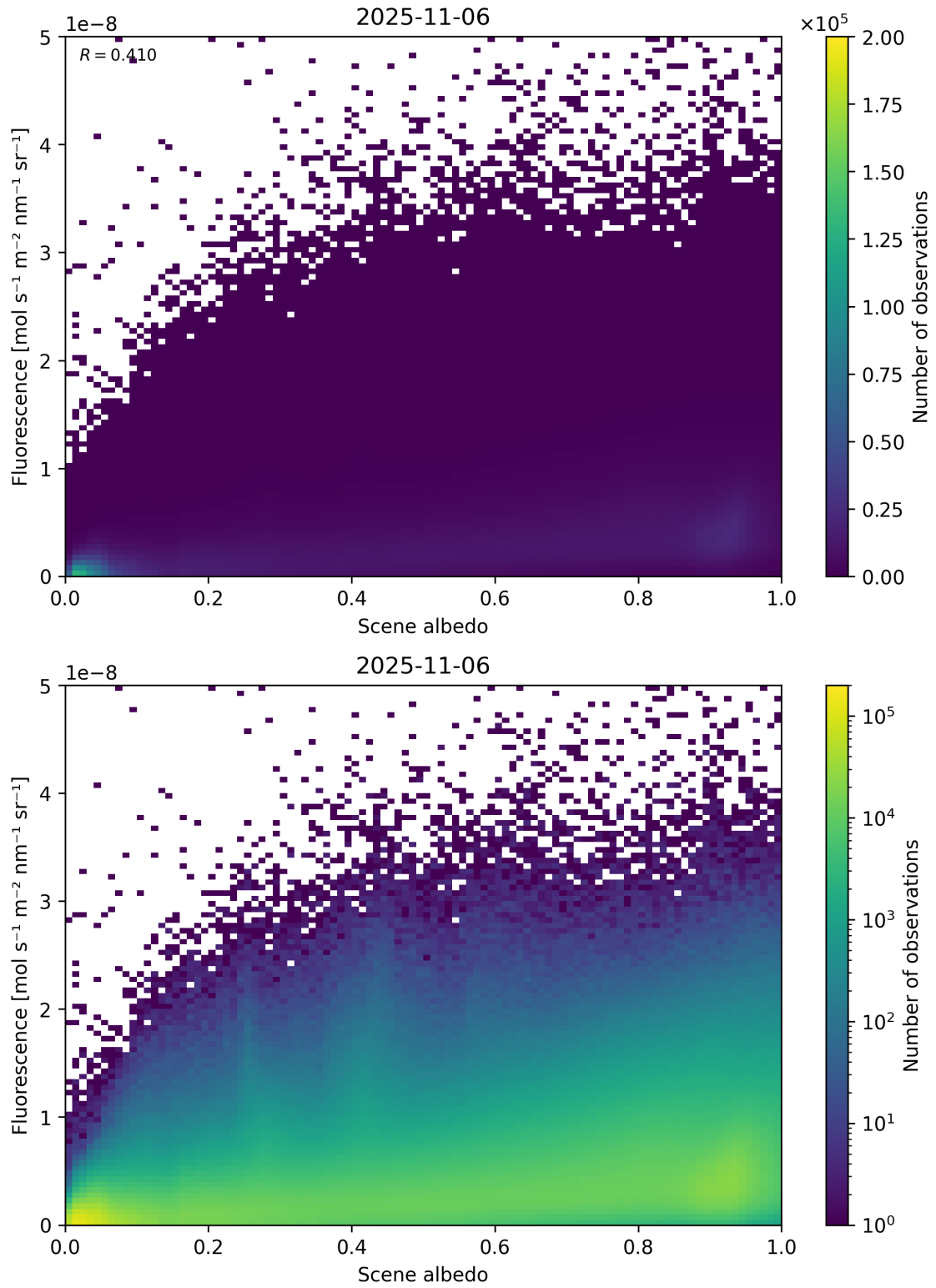
Figure 104: Scatter density plot of “Scene albedo” against “Fluorescence” for 2025-11-05 to 2025-11-07.
