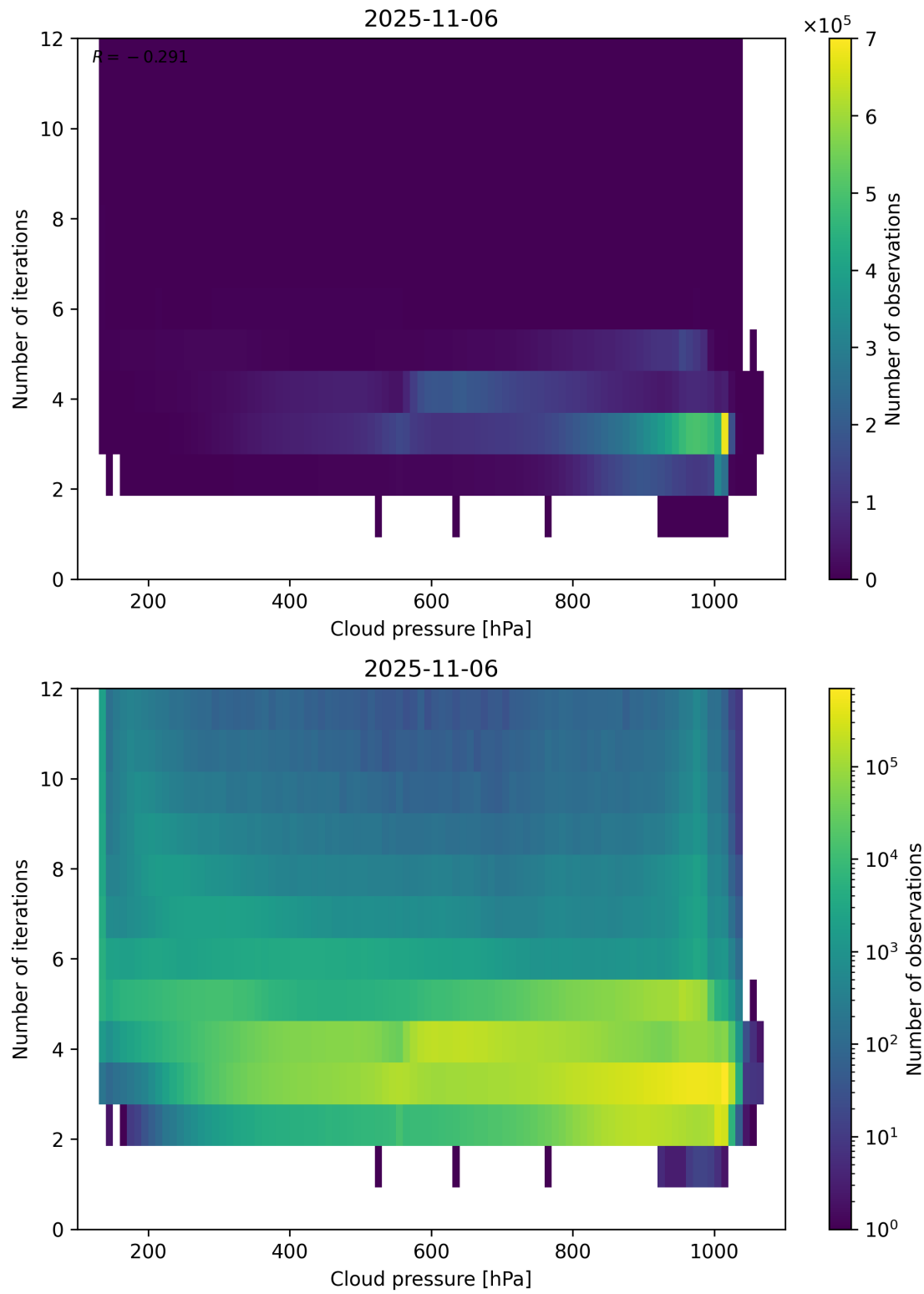
Figure 81: Scatter density plot of “Cloud pressure” against “Number of iterations” for 2025-11-05 to 2025-11-07.
