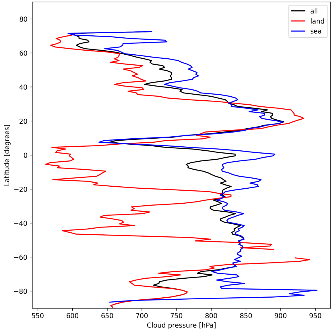
Figure 13: Zonal average of “Cloud pressure” for 2025-11-05 to 2025-11-07.
