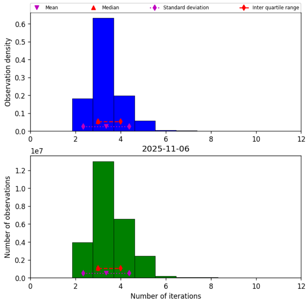
Figure 39: Histogram of “Number of iterations” for 2025-11-05 to 2025-11-07
