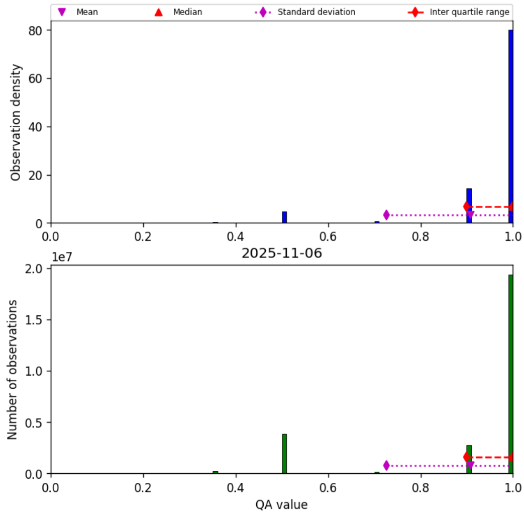
Figure 29: Histogram of “QA value” for 2025-11-05 to 2025-11-07
