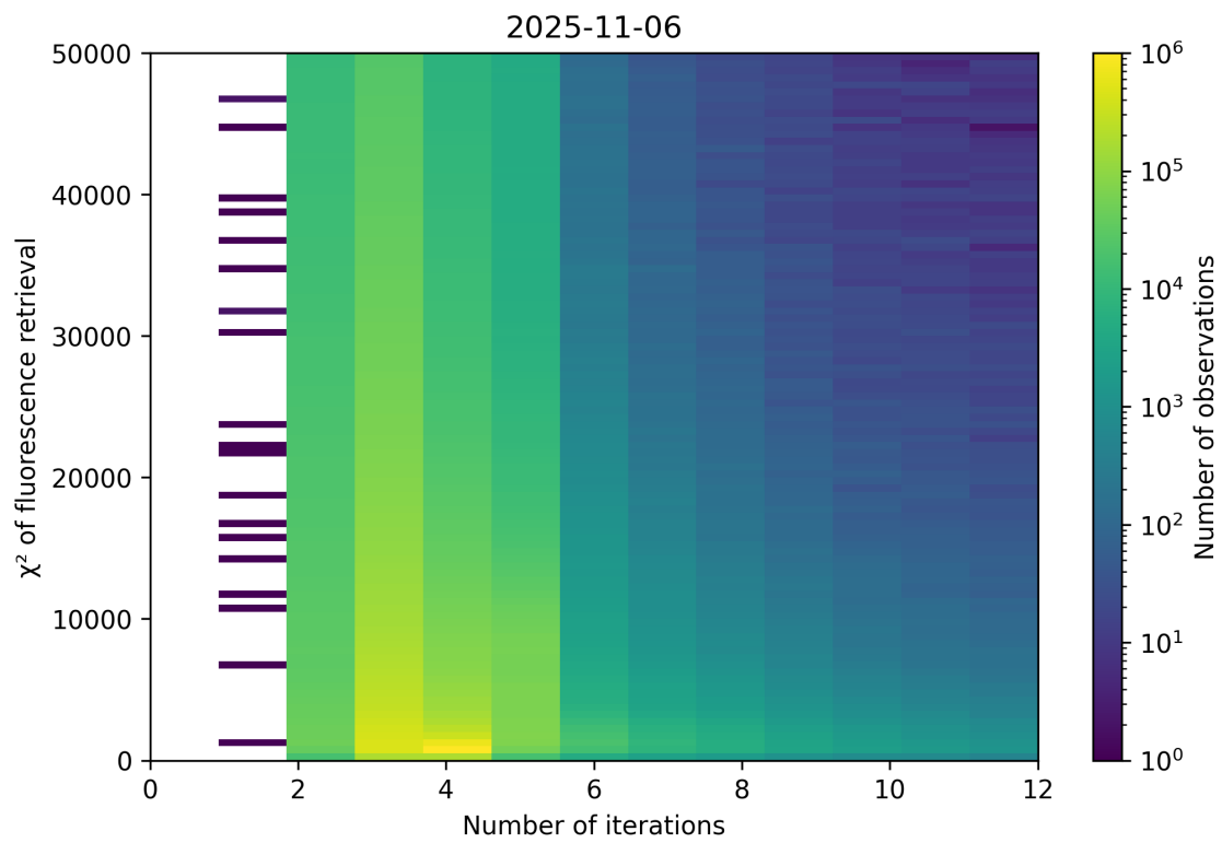
Figure 97: Scatter density plot of “Number of iterations” against “ \chi^2 of fluorescence retrieval” for 2025-11-05 to 2025-11-07.
