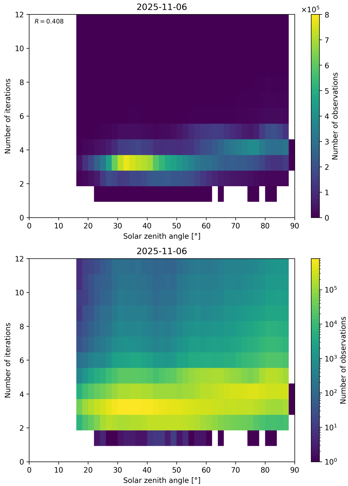
Figure 114: Scatter density plot of “Solar zenith angle” against “Number of iterations” for 2025-11-05 to 2025-11-07.
