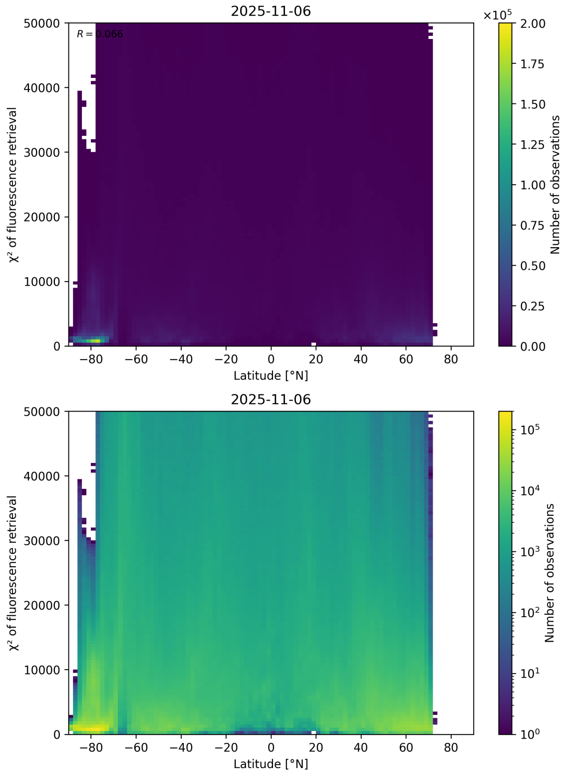
Figure 89: Scatter density plot of “Latitude” against “ \chi^2 of fluorescence retrieval” for 2025-11-05 to 2025-11-07.
