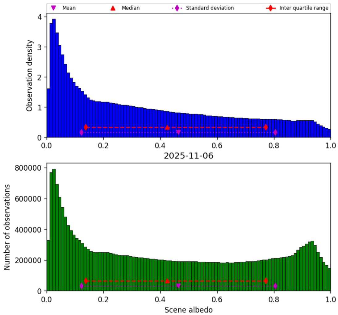
Figure 34: Histogram of “Scene albedo” for 2025-11-05 to 2025-11-07
