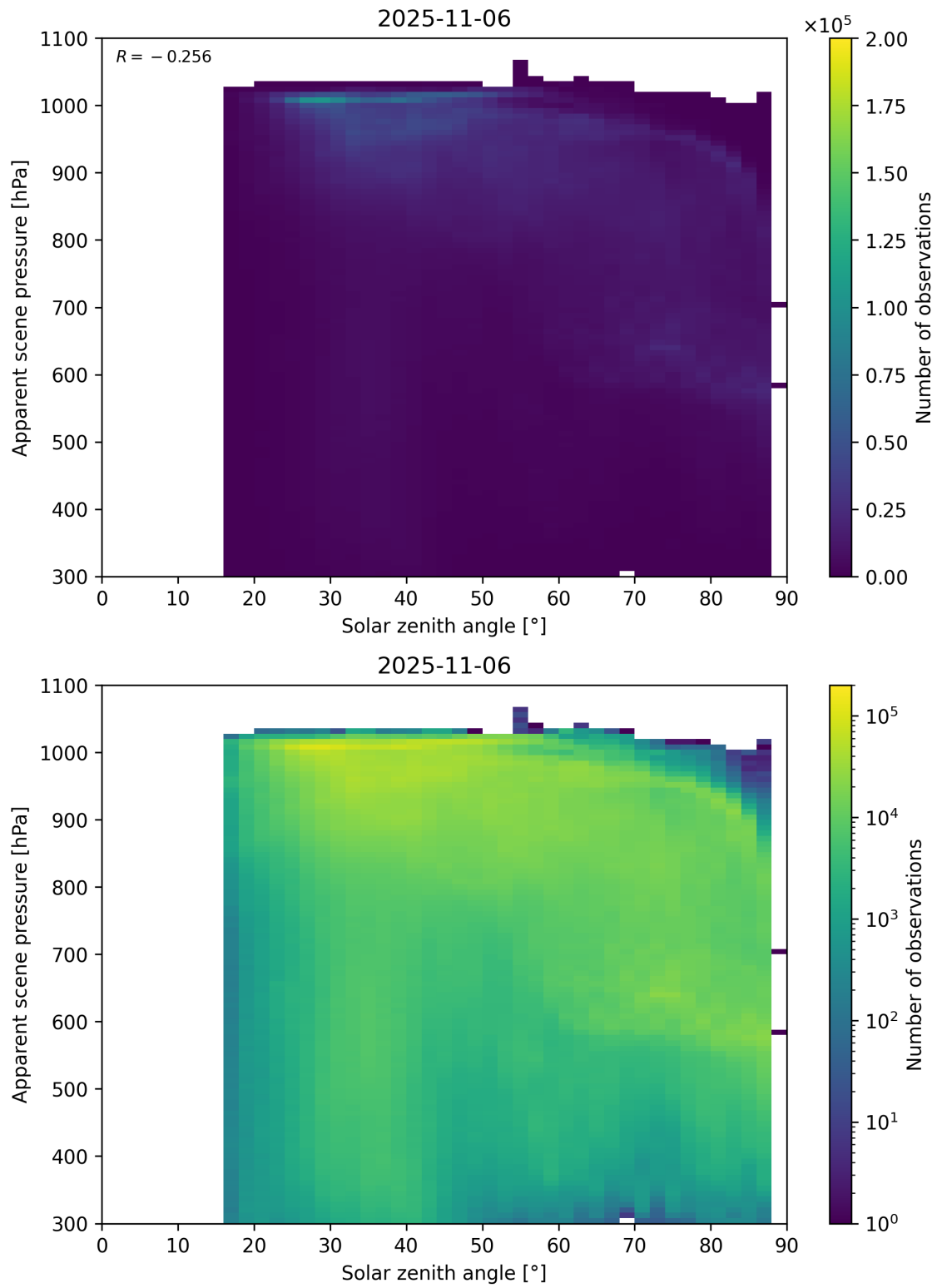
Figure 108: Scatter density plot of “Solar zenith angle” against “Apparent scene pressure” for 2025-11-05 to 2025-11-07.
