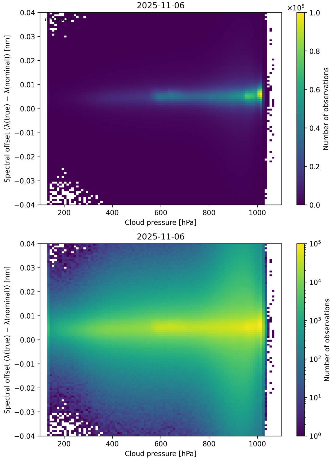
Figure 84: Scatter density plot of “Cloud pressure” against “Spectral offset ( \lambda_{\text{true}} - \lambda_{\text{nominal}} )” for 2025-11-05 to 2025-11-07.
