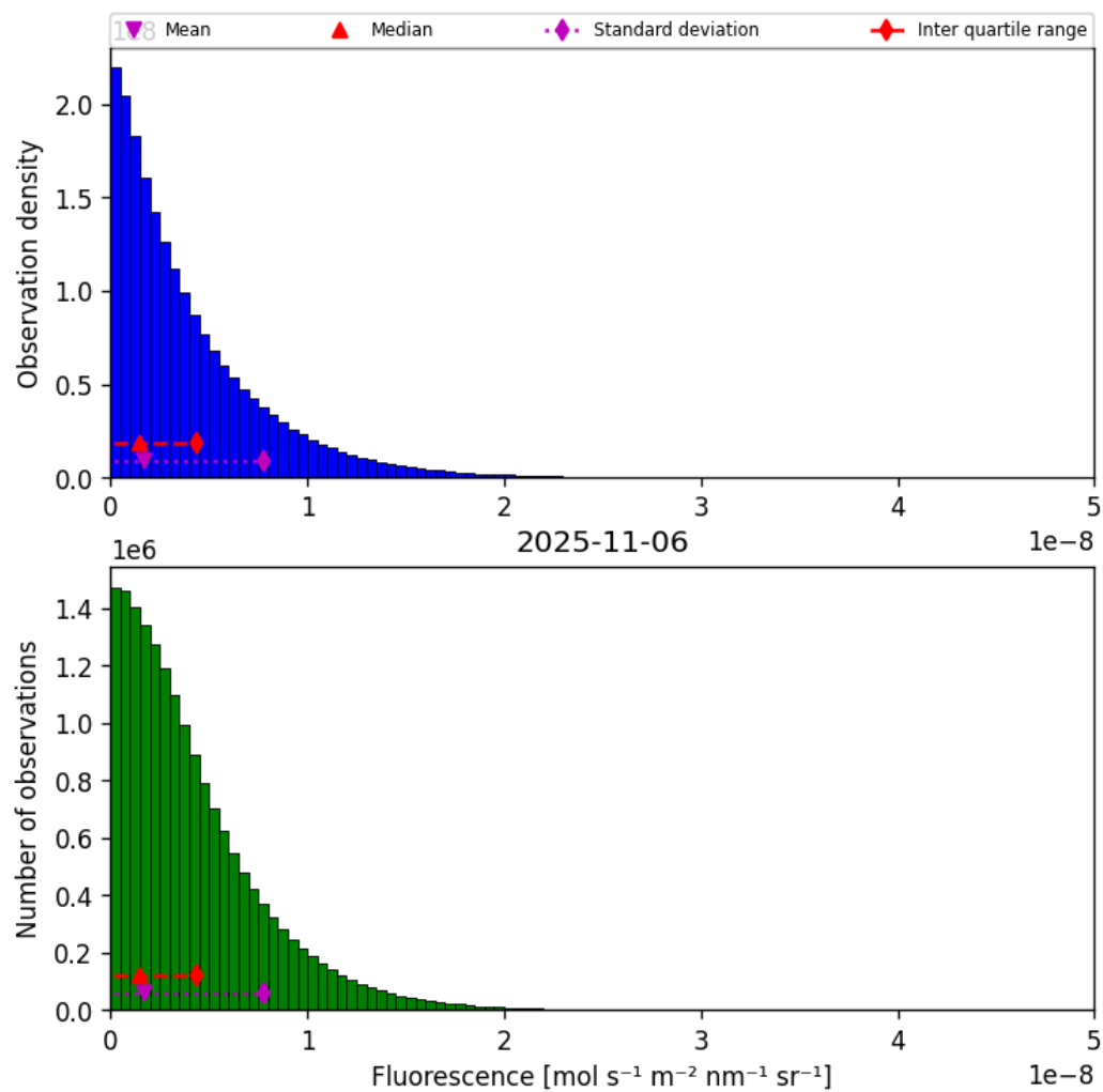
Figure 40: Histogram of “Fluorescence” for 2025-11-05 to 2025-11-07
