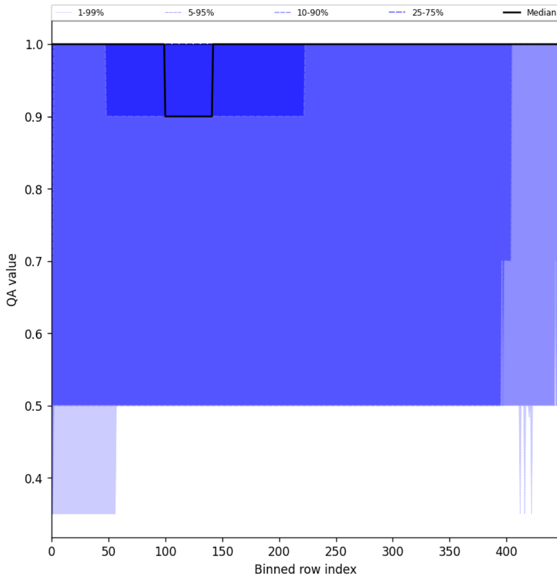
Figure 46: Along track statistics of “QA value” for 2025-11-05 to 2025-11-07
