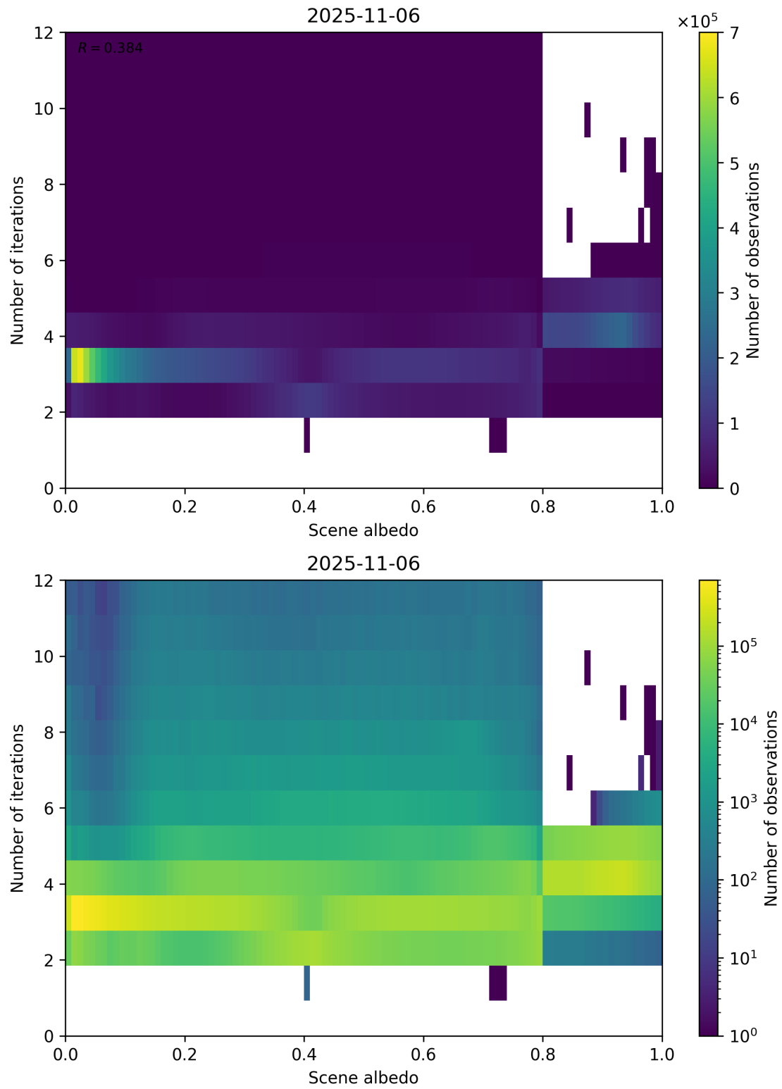
Figure 105: Scatter density plot of “Scene albedo” against “Number of iterations” for 2025-11-05 to 2025-11-07.
