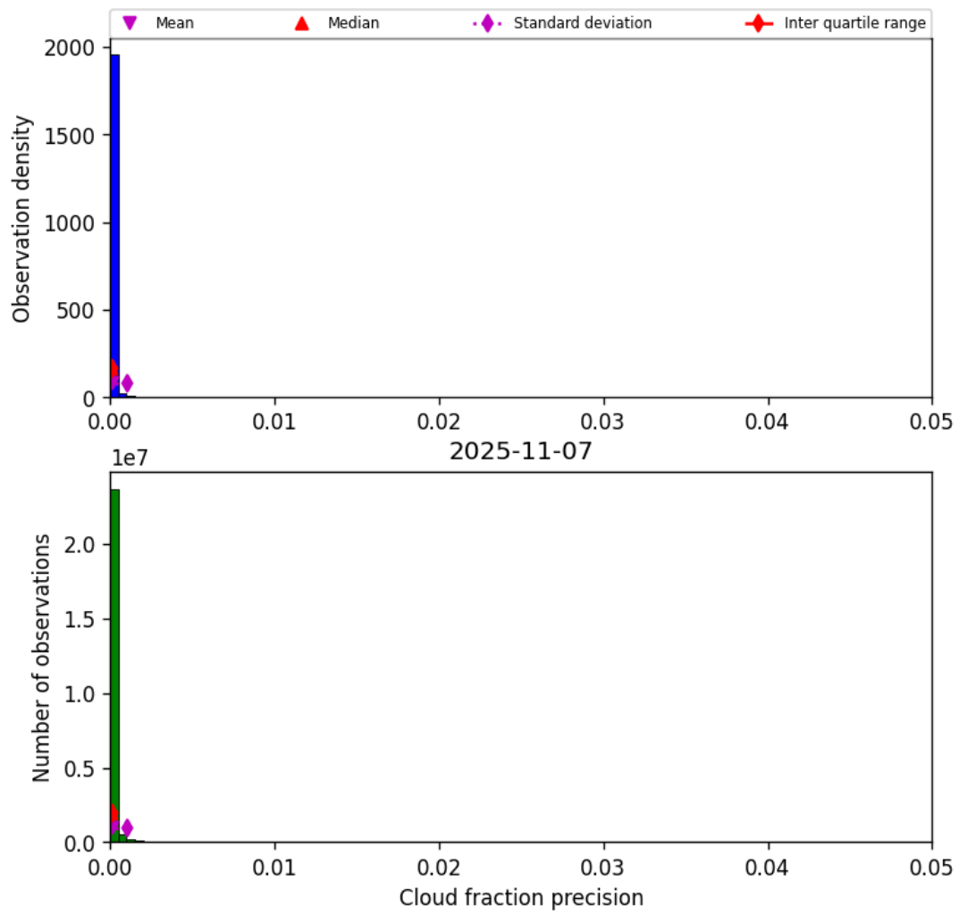
Figure 33: Histogram of “Cloud fraction precision” for 2025-11-07 to 2025-11-08
