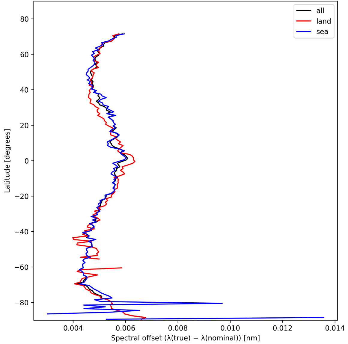
Figure 28: Zonal average of “Spectral offset ( \lambda_{\text{true}} - \lambda_{\text{nominal}} )” for 2025-11-07 to 2025-11-08.
