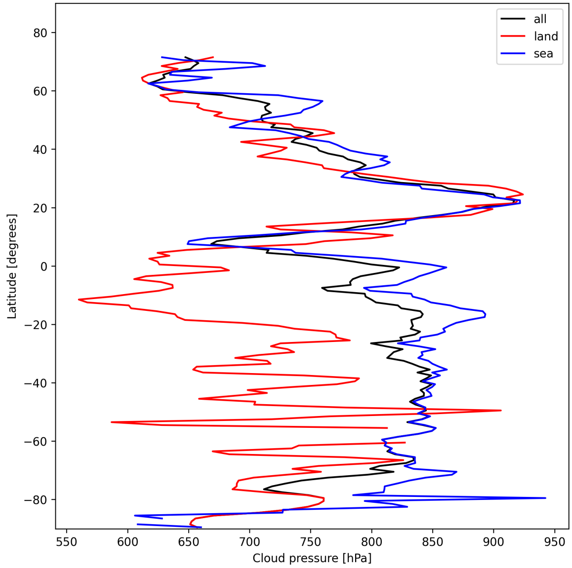
Figure 13: Zonal average of “Cloud pressure” for 2025-11-07 to 2025-11-08.
