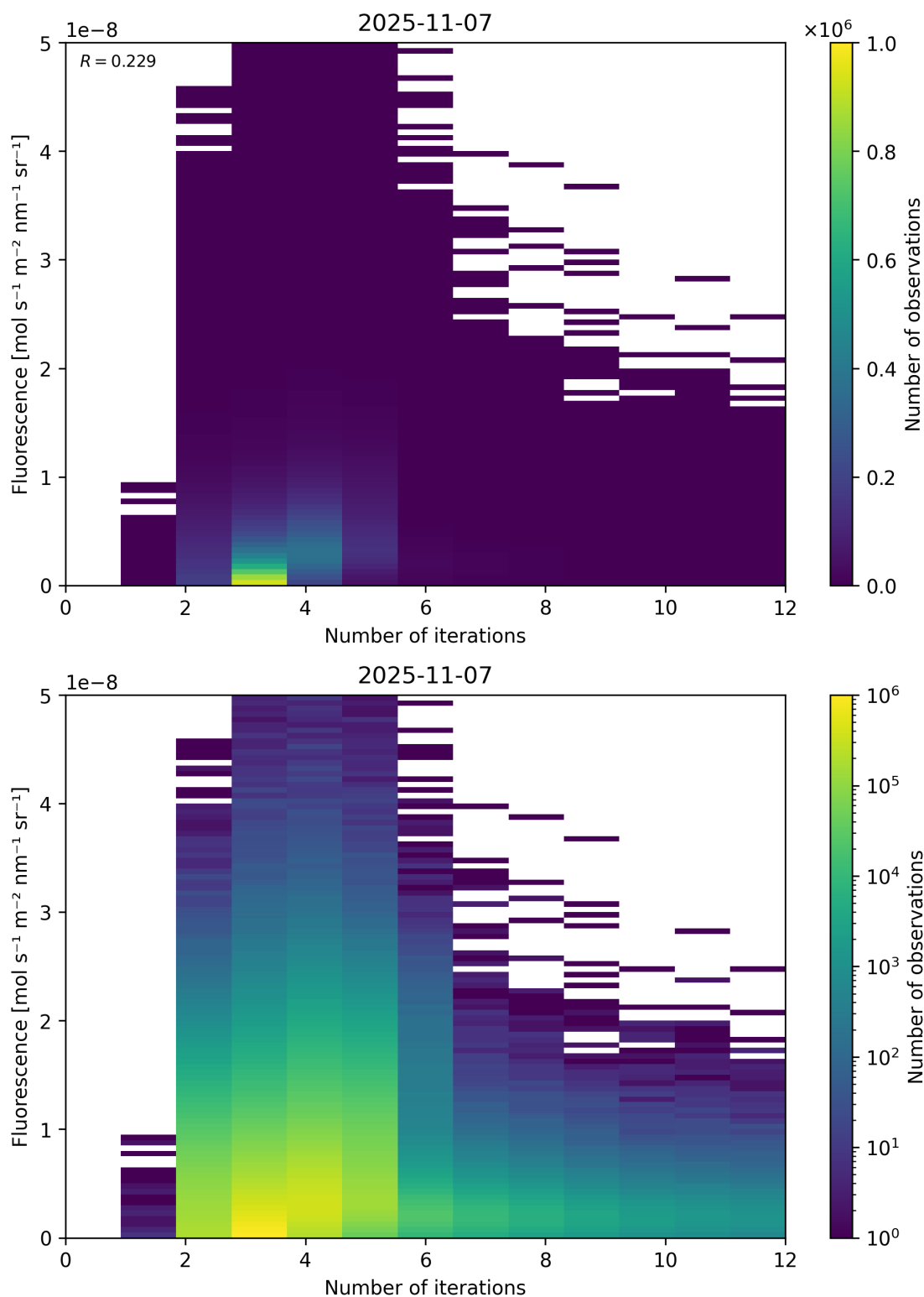
Figure 98: Scatter density plot of “Number of iterations” against “Fluorescence” for 2025-11-07 to 2025-11-08.
