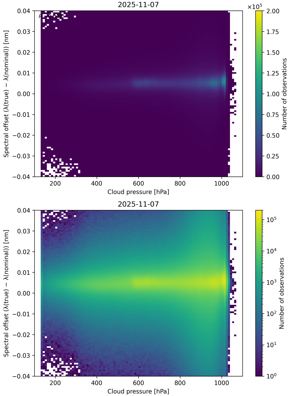
Figure 84: Scatter density plot of “Cloud pressure” against “Spectral offset ( \lambda_{\text{true}} - \lambda_{\text{nominal}} )” for 2025-11-07 to 2025-11-08.
