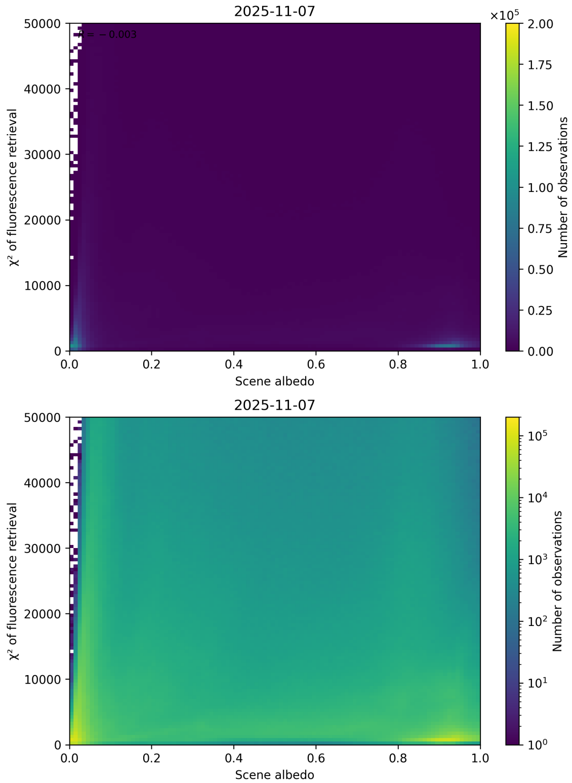
Figure 103: Scatter density plot of “Scene albedo” against “ \chi^2 of fluorescence retrieval” for 2025-11-07 to 2025-11-08.
