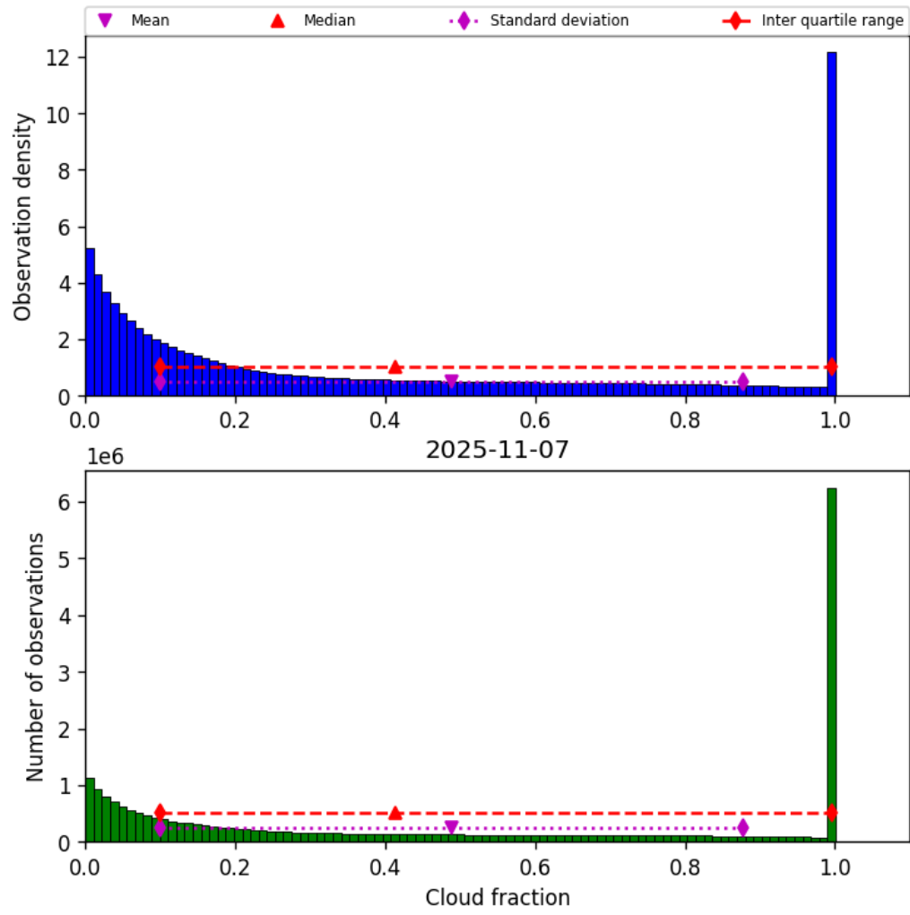
Figure 32: Histogram of “Cloud fraction” for 2025-11-07 to 2025-11-08
