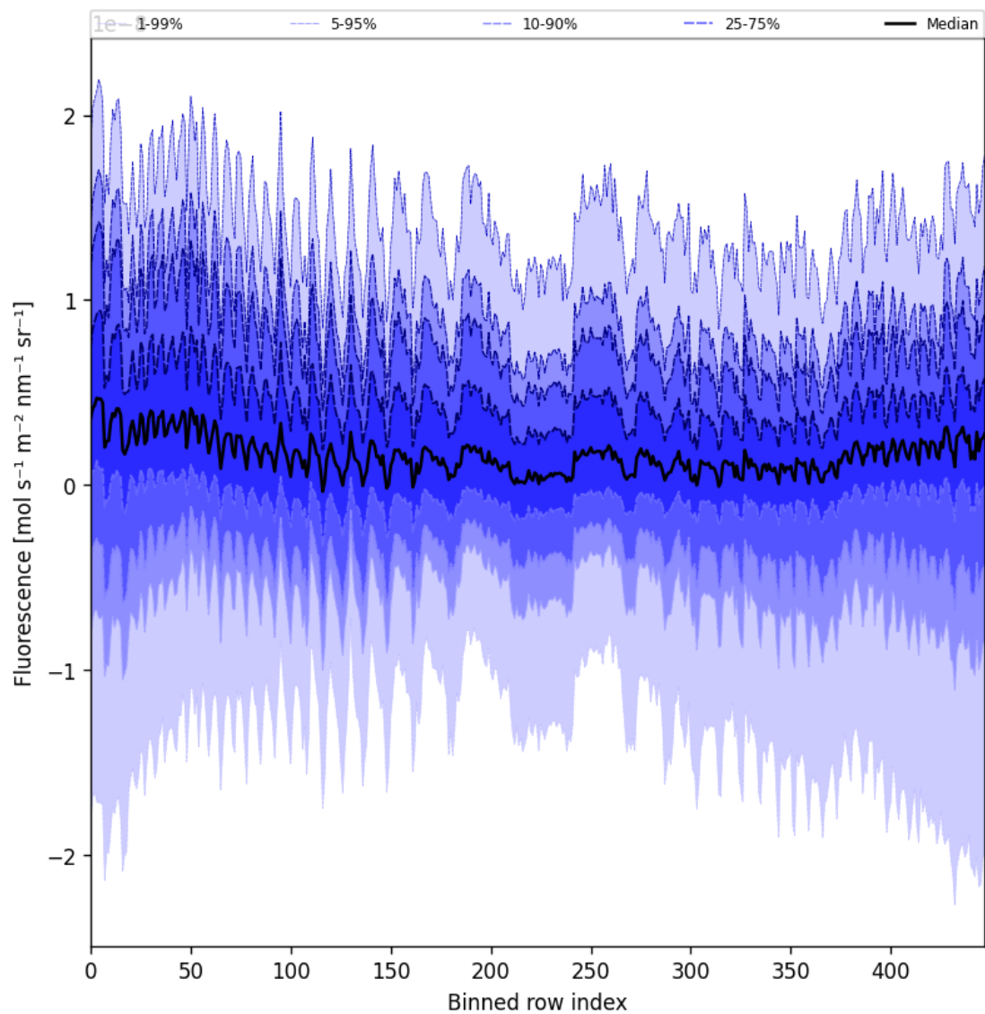
Figure 57: Along track statistics of “Fluorescence” for 2025-11-07 to 2025-11-08
