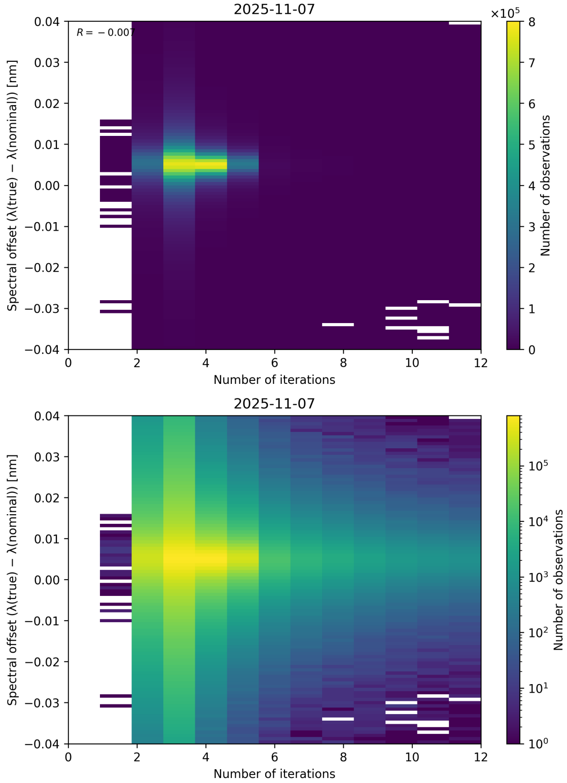
Figure 100: Scatter density plot of “Number of iterations” against “Spectral offset ( \lambda_{\text{true}} - \lambda_{\text{nominal}} )” for 2025-11-07 to 2025-11-08.
