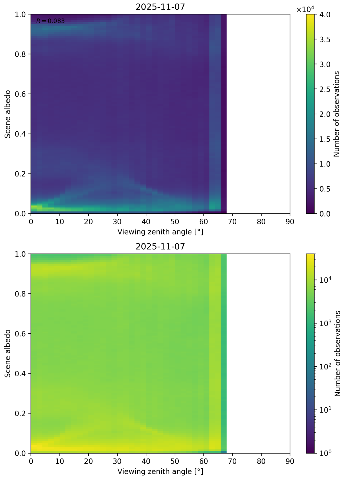
Figure 126: Scatter density plot of “Viewing zenith angle” against “Scene albedo” for 2025-11-07 to 2025-11-08.
