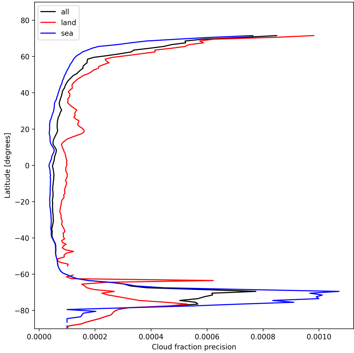
Figure 16: Zonal average of “Cloud fraction precision” for 2025-11-07 to 2025-11-08.
