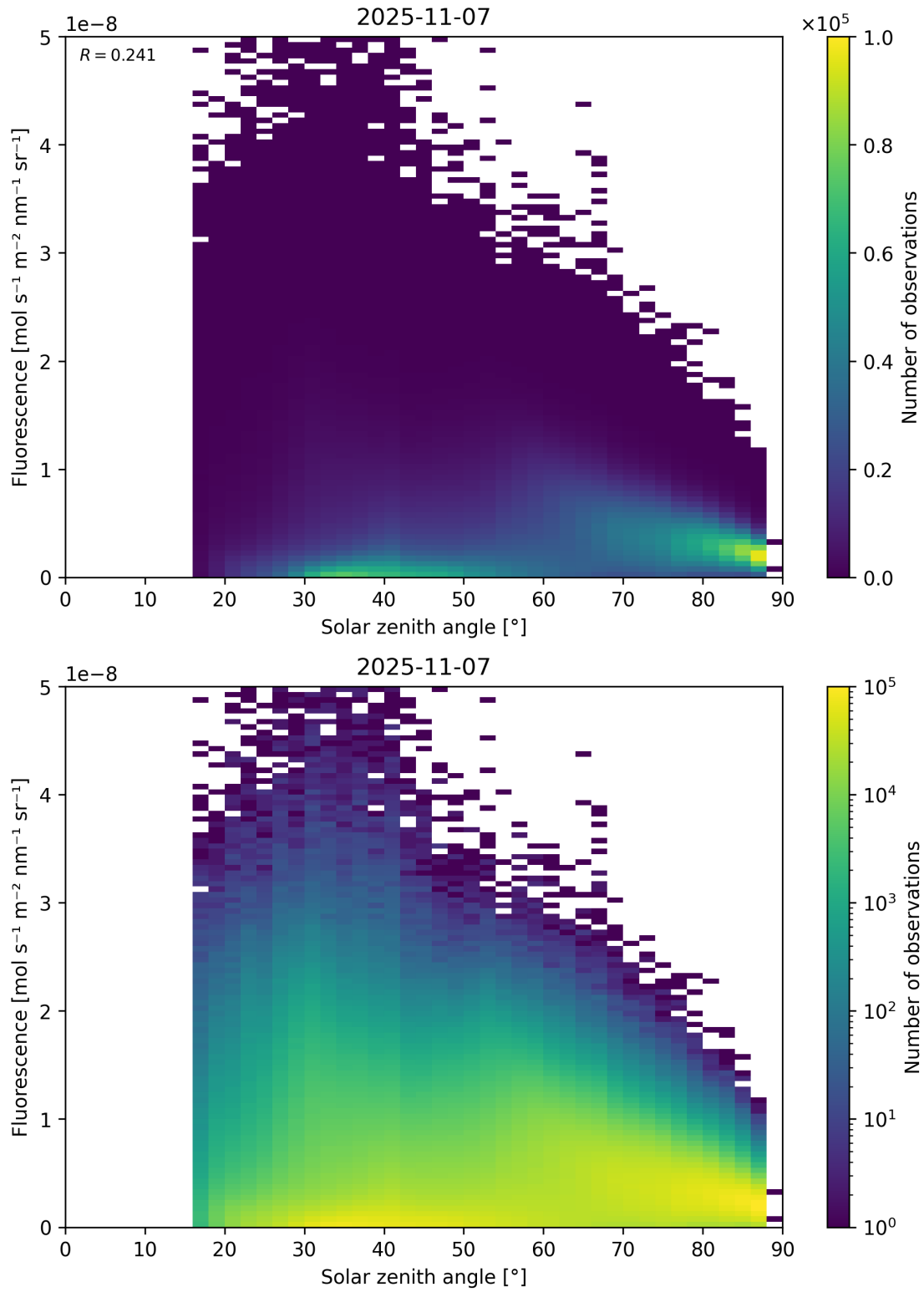
Figure 112: Scatter density plot of “Solar zenith angle” against “Fluorescence” for 2025-11-07 to 2025-11-08.
