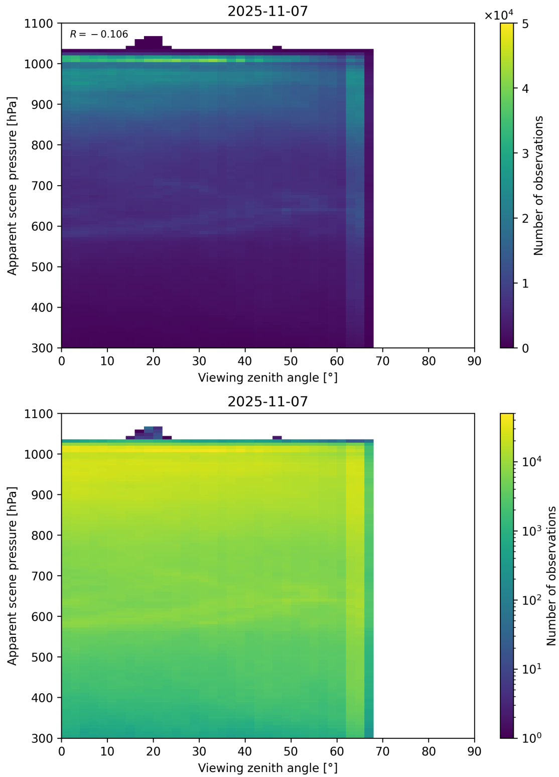
Figure 118: Scatter density plot of “Viewing zenith angle” against “Apparent scene pressure” for 2025-11-07 to 2025-11-08.
