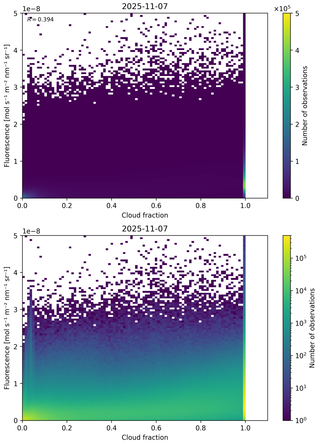
Figure 72: Scatter density plot of “Cloud fraction” against “Fluorescence” for 2025-11-07 to 2025-11-08.
