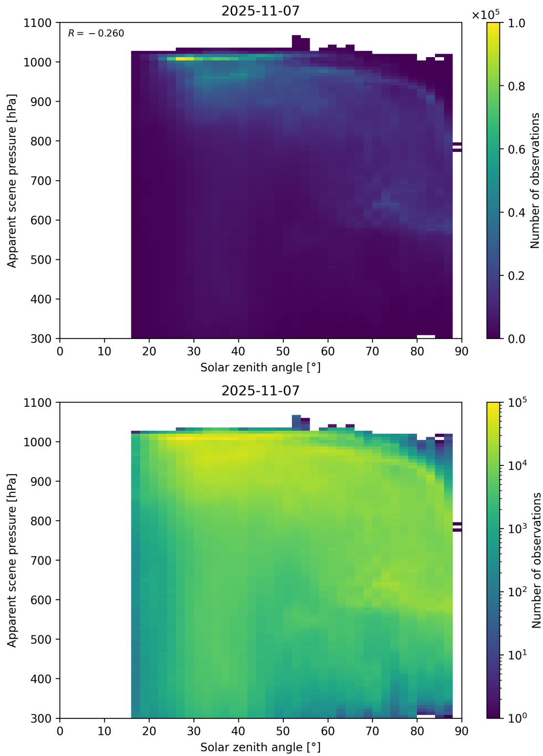
Figure 108: Scatter density plot of “Solar zenith angle” against “Apparent scene pressure” for 2025-11-07 to 2025-11-08.
