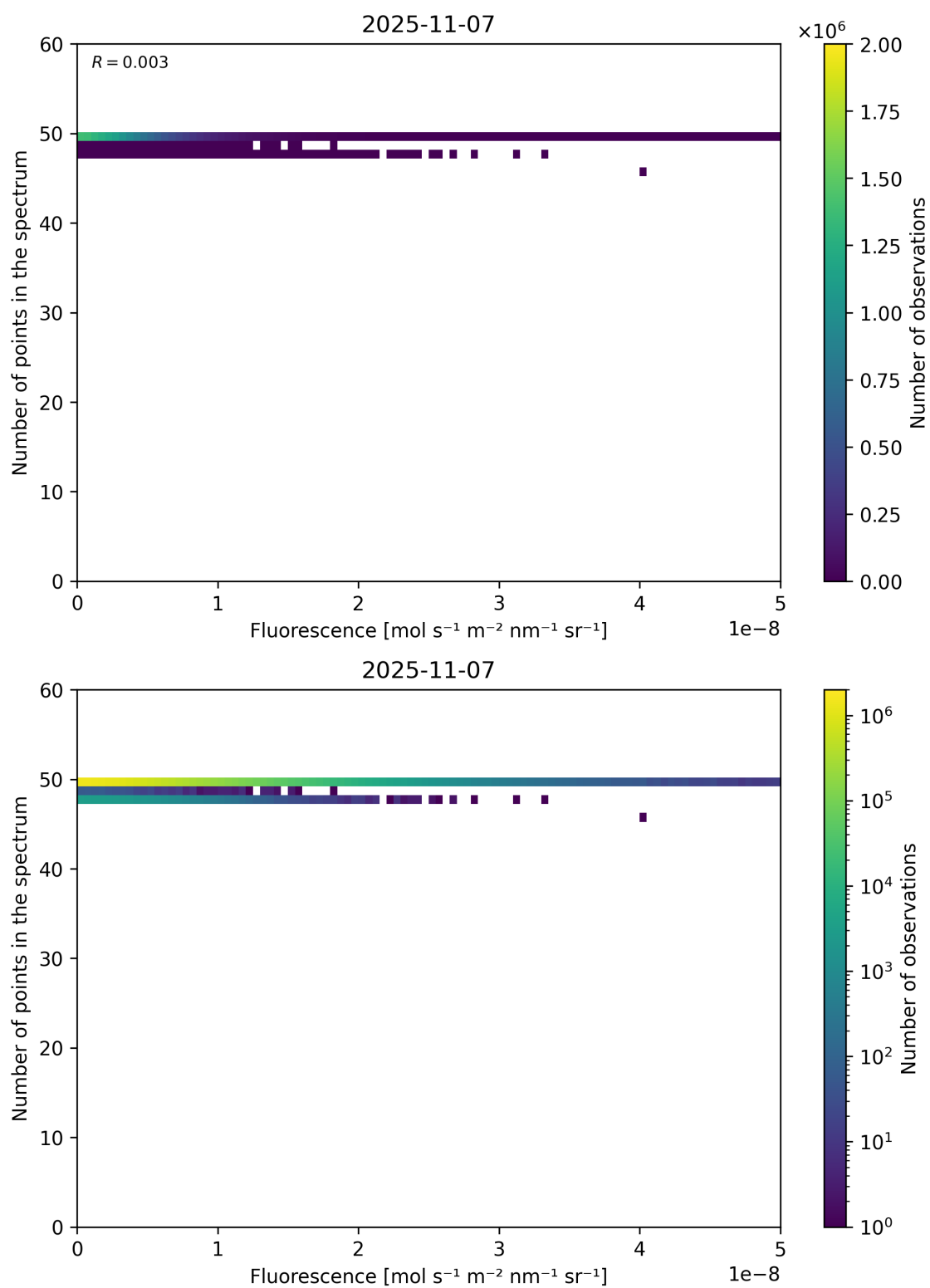
Figure 86: Scatter density plot of “Fluorescence” against “Number of points in the spectrum” for 2025-11-07 to 2025-11-08.
