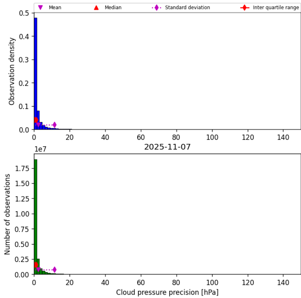
Figure 31: Histogram of “Cloud pressure precision” for 2025-11-07 to 2025-11-08
