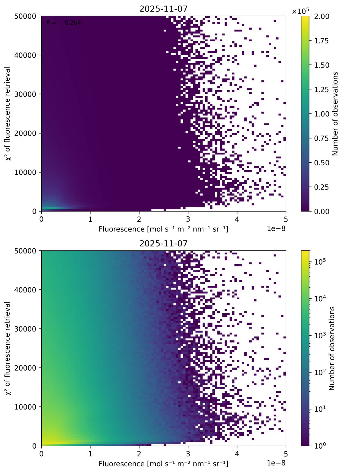
Figure 85: Scatter density plot of “Fluorescence” against “ \chi^2 of fluorescence retrieval” for 2025-11-07 to 2025-11-08.
