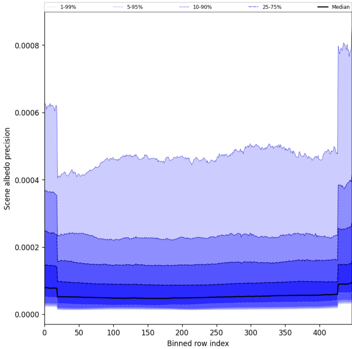
Figure 52: Along track statistics of “Scene albedo precision” for 2025-11-07 to 2025-11-08
