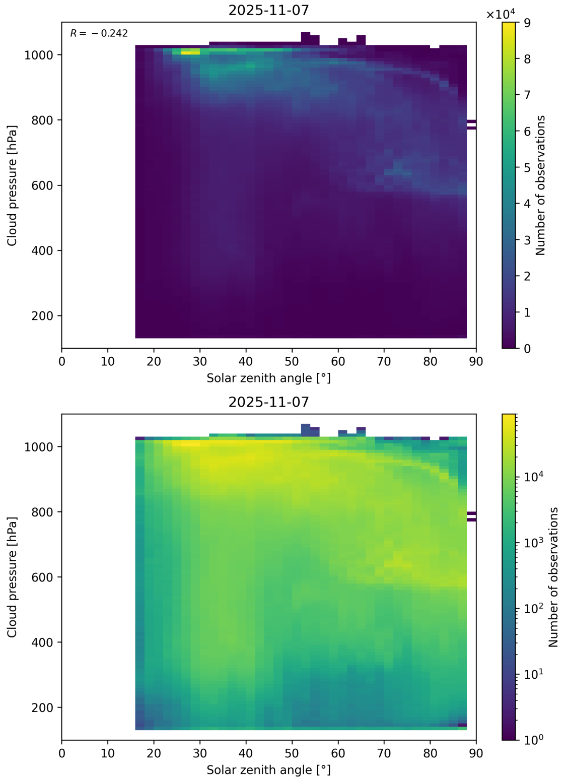
Figure 111: Scatter density plot of “Solar zenith angle” against “Cloud pressure” for 2025-11-07 to 2025-11-08.
