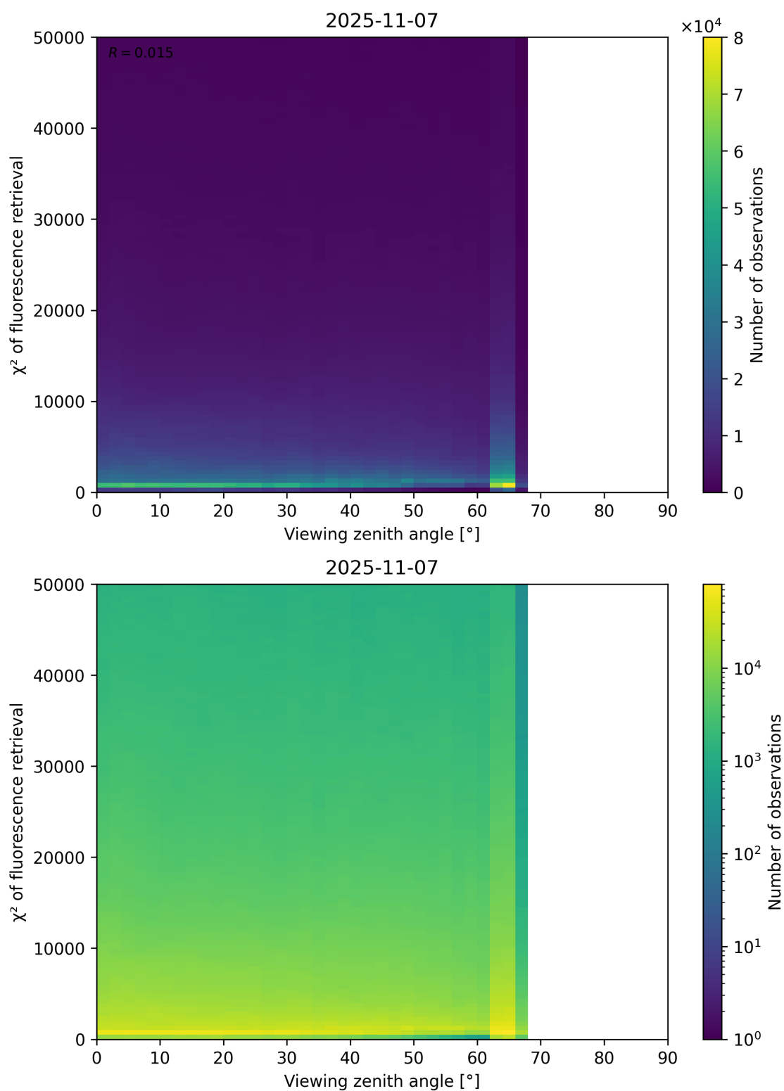
Figure 119: Scatter density plot of “Viewing zenith angle” against “ \chi^2 of fluorescence retrieval” for 2025-11-07 to 2025-11-08.
