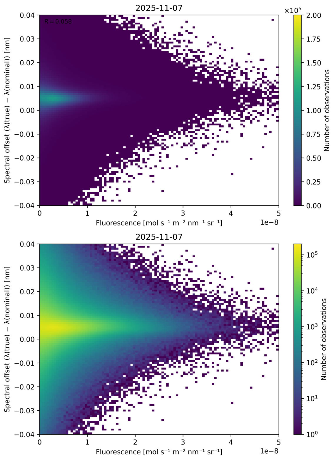
Figure 87: Scatter density plot of “Fluorescence” against “Spectral offset ( \lambda_{\text{true}} - \lambda_{\text{nominal}} )” for 2025-11-07 to 2025-11-08.
