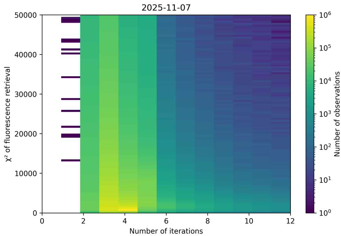
Figure 97: Scatter density plot of “Number of iterations” against “ \chi^2 of fluorescence retrieval” for 2025-11-07 to 2025-11-08.
