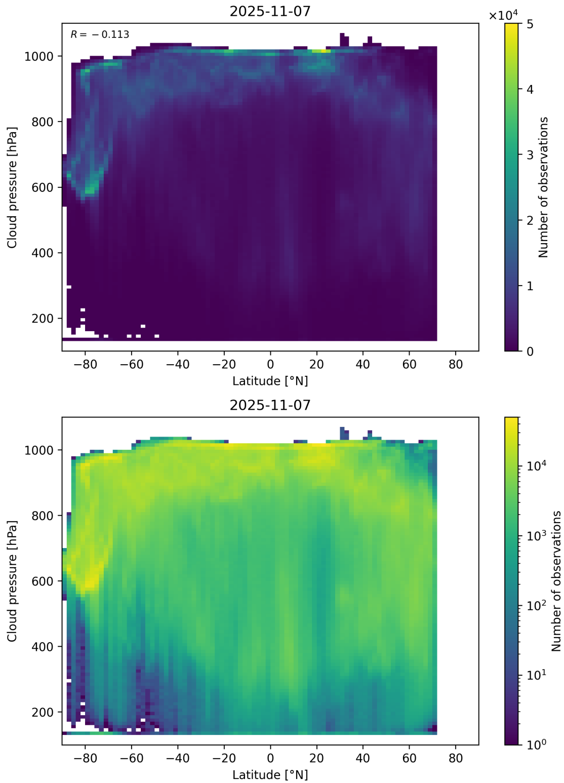
Figure 91: Scatter density plot of “Latitude” against “Cloud pressure” for 2025-11-07 to 2025-11-08.
