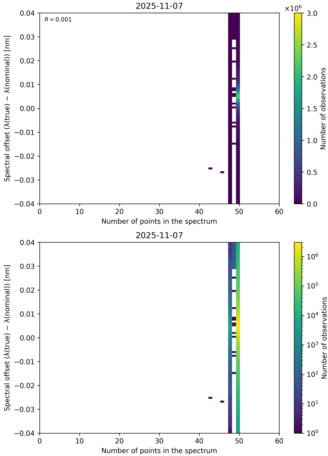
Figure 101: Scatter density plot of “Number of points in the spectrum” against “Spectral offset ( \lambda_{\text{true}} - \lambda_{\text{nominal}} )” for 2025-11-07 to 2025-11-08.
