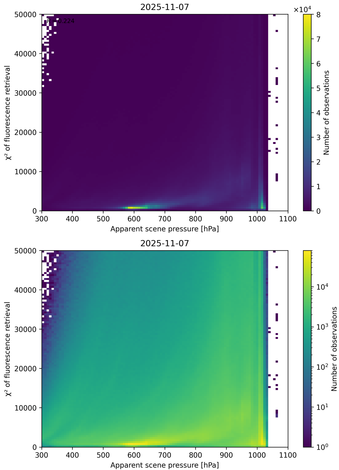
Figure 63: Scatter density plot of “Apparent scene pressure” against “ \chi^2 of fluorescence retrieval” for 2025-11-07 to 2025-11-08.
