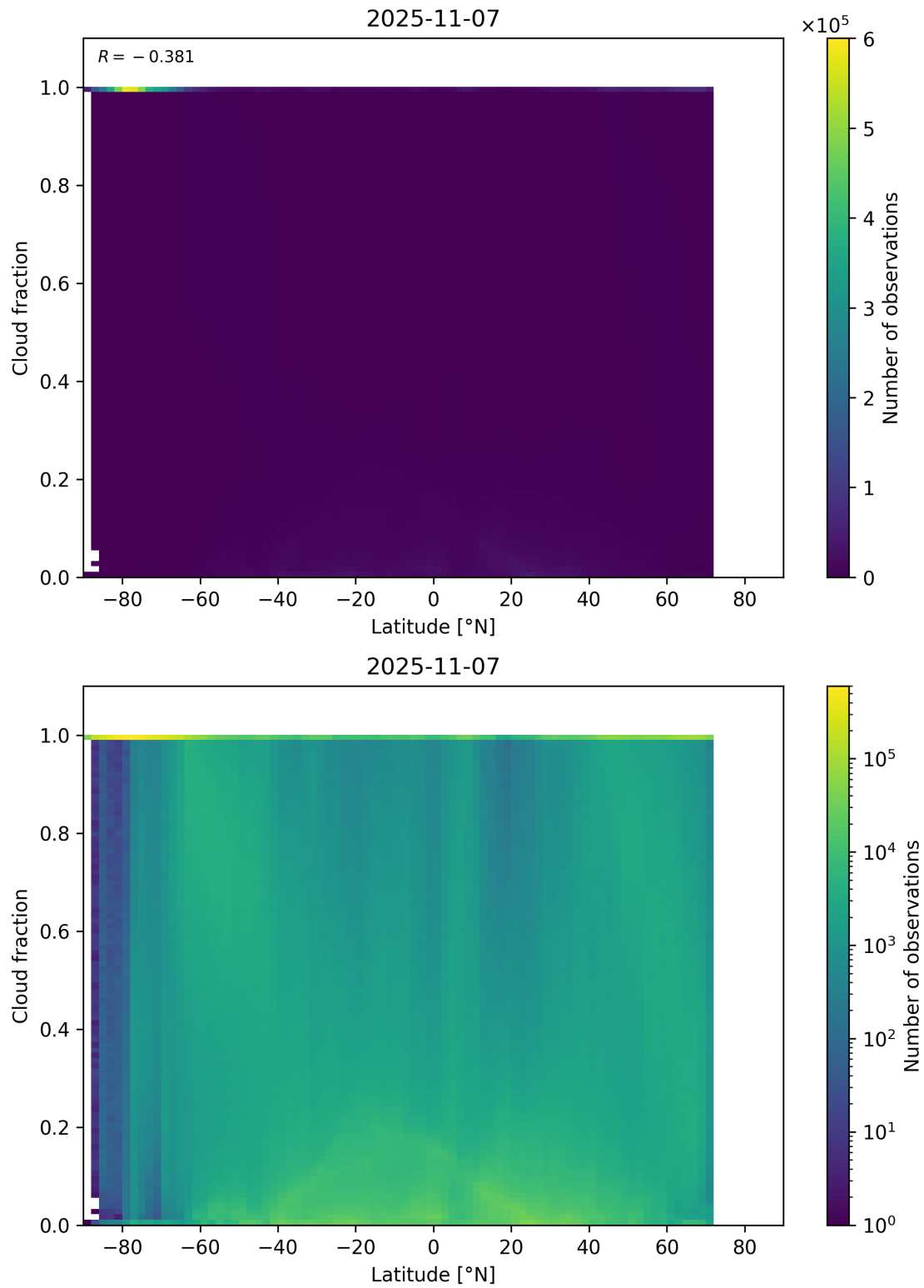
Figure 90: Scatter density plot of “Latitude” against “Cloud fraction” for 2025-11-07 to 2025-11-08.
