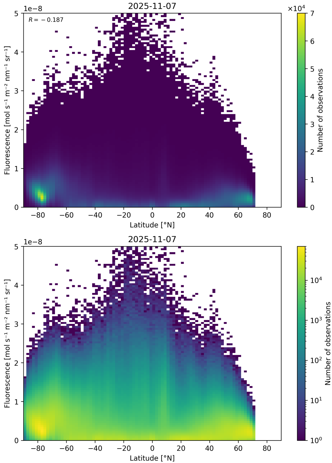
Figure 92: Scatter density plot of “Latitude” against “Fluorescence” for 2025-11-07 to 2025-11-08.
