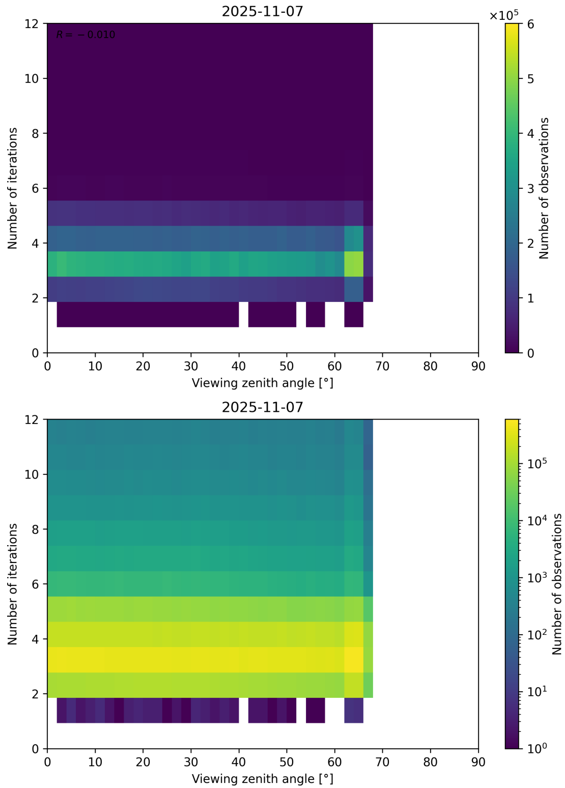
Figure 124: Scatter density plot of “Viewing zenith angle” against “Number of iterations” for 2025-11-07 to 2025-11-08.
