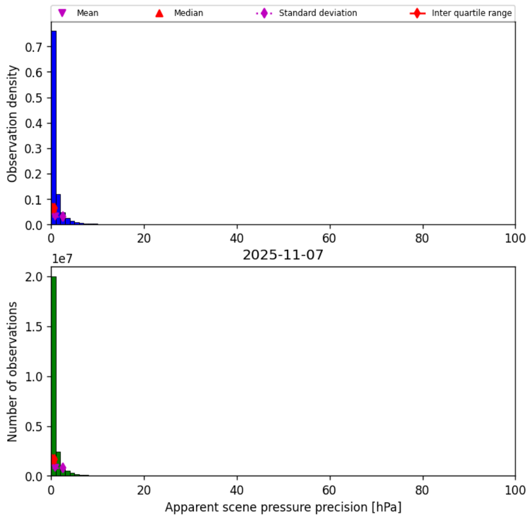
Figure 37: Histogram of “Apparent scene pressure precision” for 2025-11-07 to 2025-11-08
