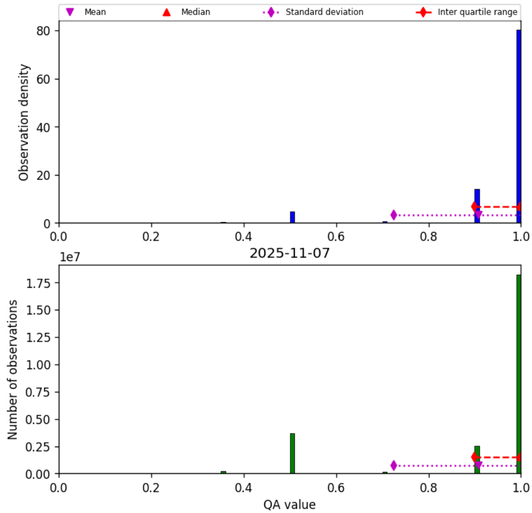
Figure 29: Histogram of “QA value” for 2025-11-07 to 2025-11-08
