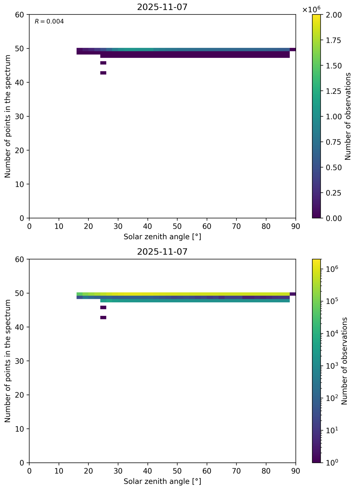
Figure 115: Scatter density plot of “Solar zenith angle” against “Number of points in the spectrum” for 2025-11-07 to 2025-11-08.
