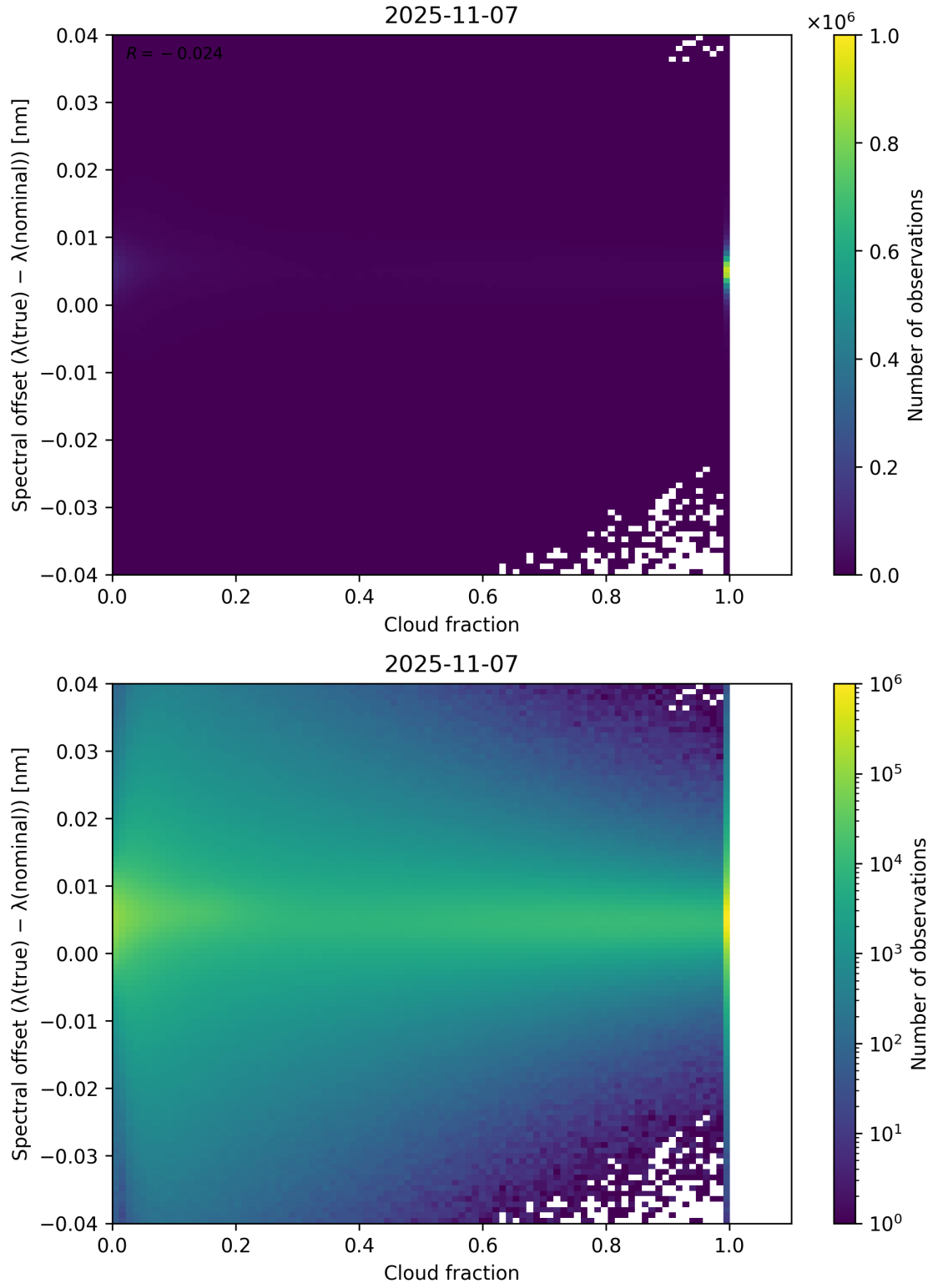
Figure 76: Scatter density plot of “Cloud fraction” against “Spectral offset ( \lambda_{\text{true}} - \lambda_{\text{nominal}} )” for 2025-11-07 to 2025-11-08.
