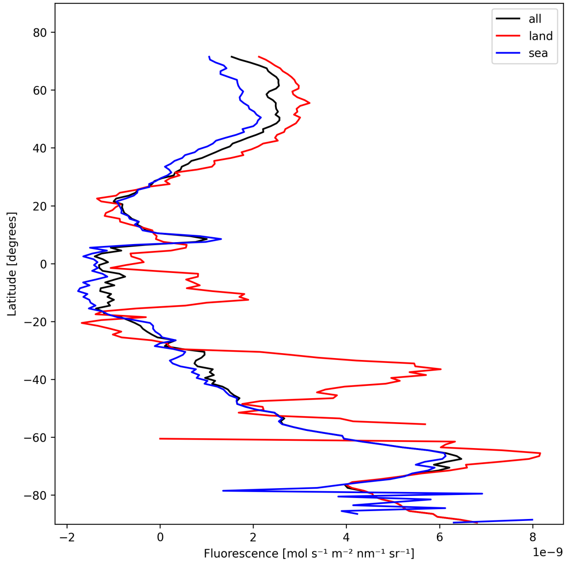
Figure 23: Zonal average of “Fluorescence” for 2025-11-07 to 2025-11-08.
