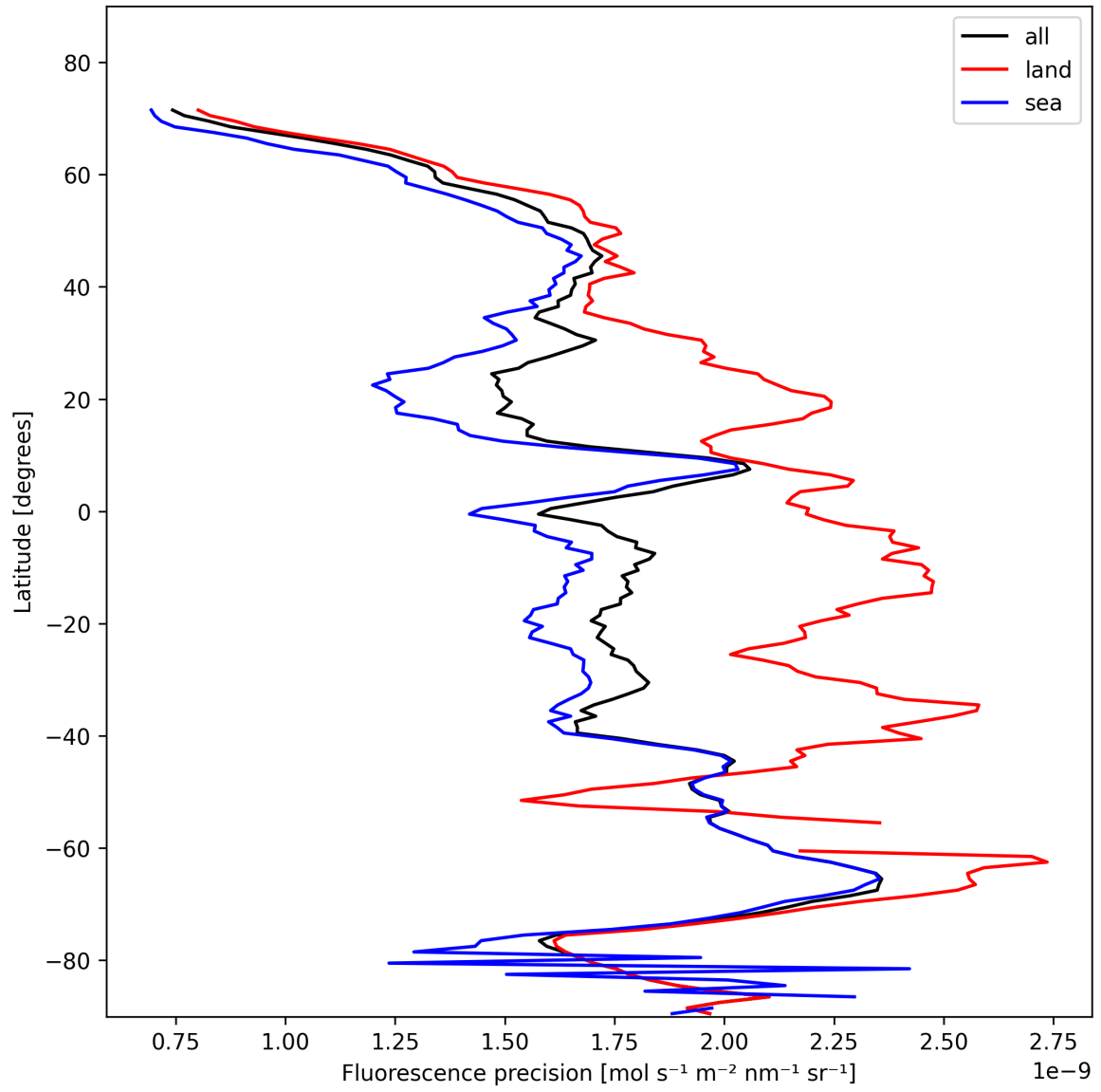
Figure 24: Zonal average of “Fluorescence precision” for 2025-11-07 to 2025-11-08.
