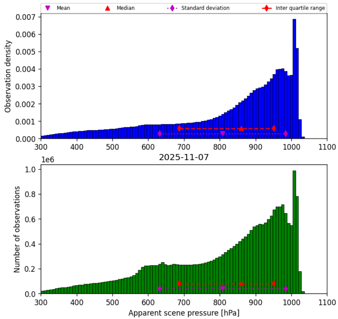
Figure 36: Histogram of “Apparent scene pressure” for 2025-11-07 to 2025-11-08
