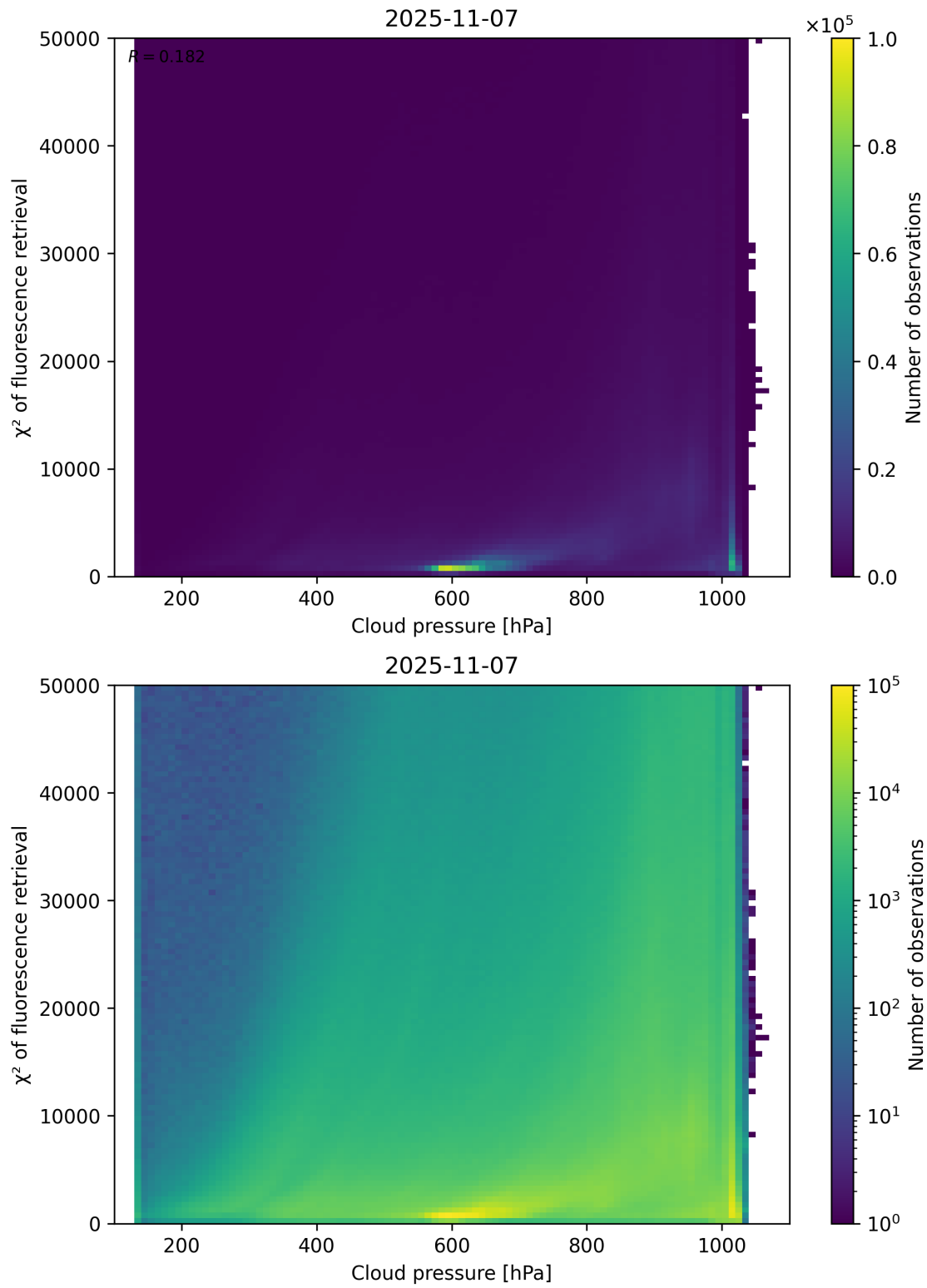
Figure 78: Scatter density plot of “Cloud pressure” against “ \chi^2 of fluorescence retrieval” for 2025-11-07 to 2025-11-08.
