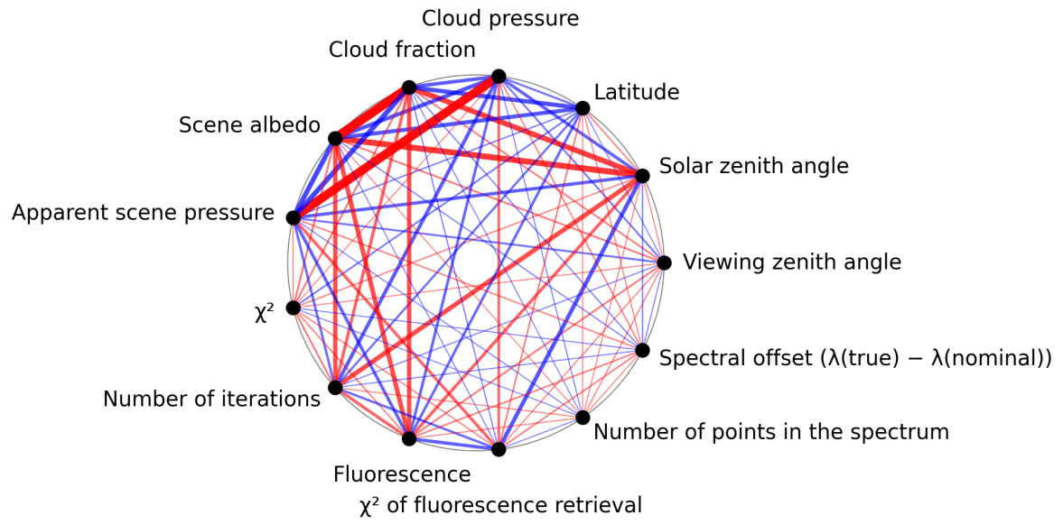
Figure 1: Map of correlation graph for 2025-11-07 to 2025-11-08.
