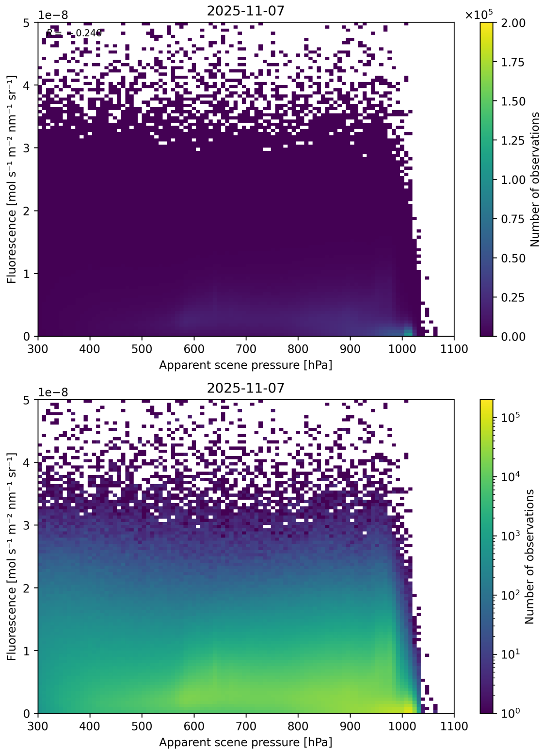
Figure 64: Scatter density plot of “Apparent scene pressure” against “Fluorescence” for 2025-11-07 to 2025-11-08.
