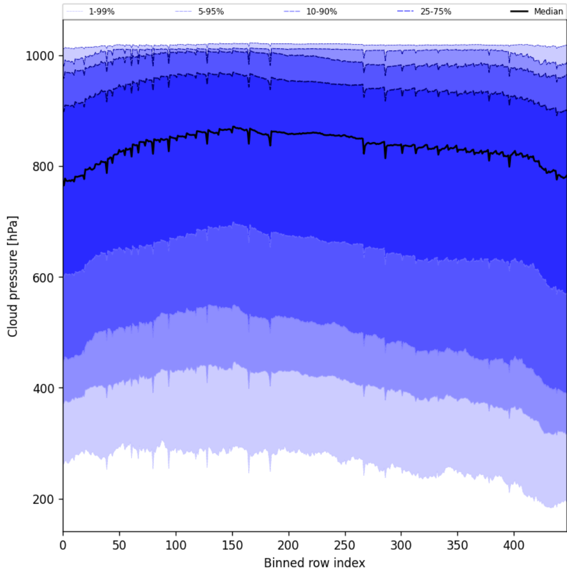
Figure 47: Along track statistics of “Cloud pressure” for 2025-11-07 to 2025-11-08
