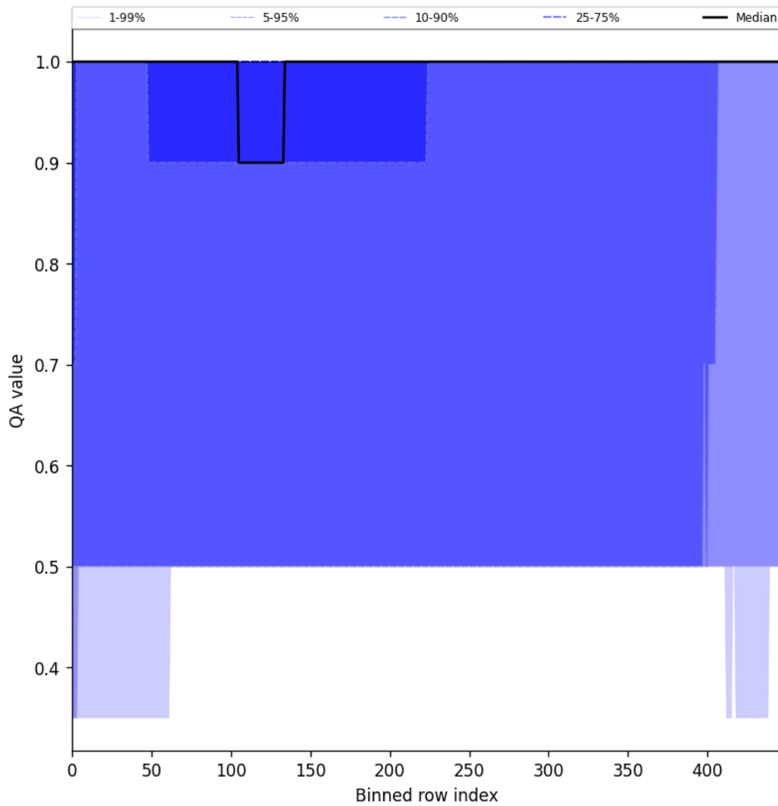
Figure 46: Along track statistics of “QA value” for 2025-11-07 to 2025-11-08
