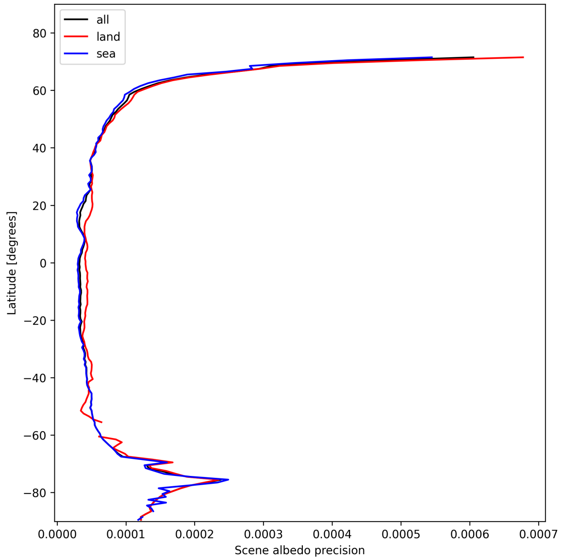
Figure 18: Zonal average of “Scene albedo precision” for 2025-11-07 to 2025-11-08.
