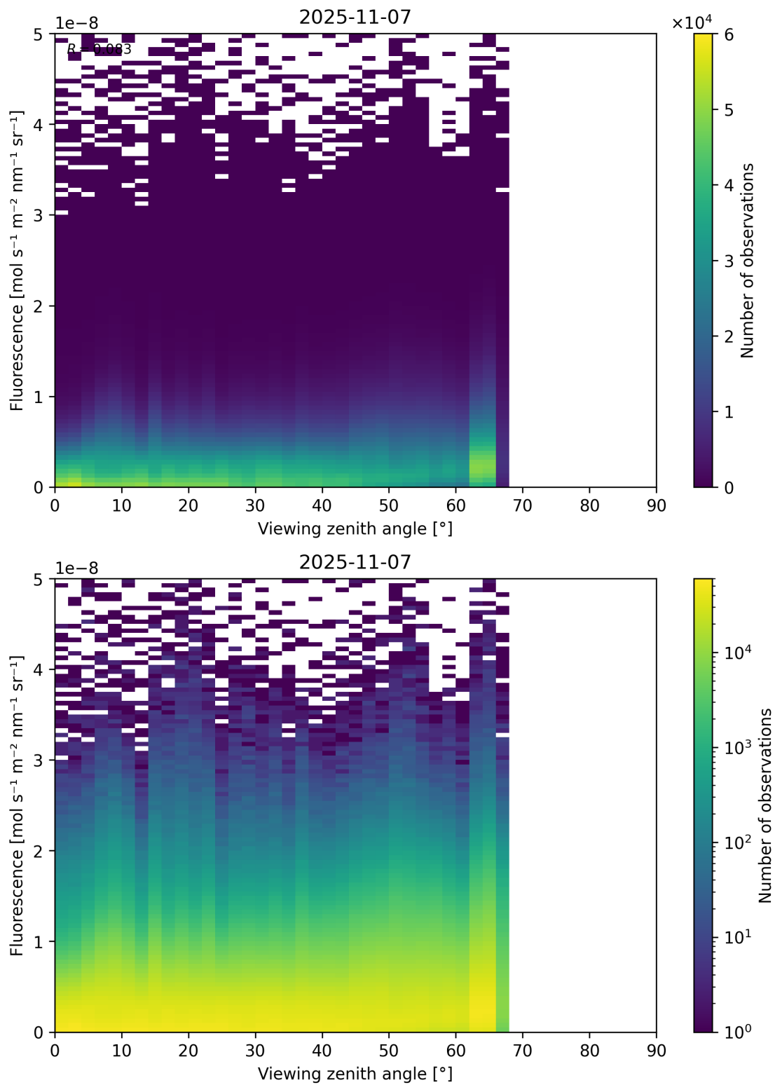
Figure 122: Scatter density plot of “Viewing zenith angle” against “Fluorescence” for 2025-11-07 to 2025-11-08.
