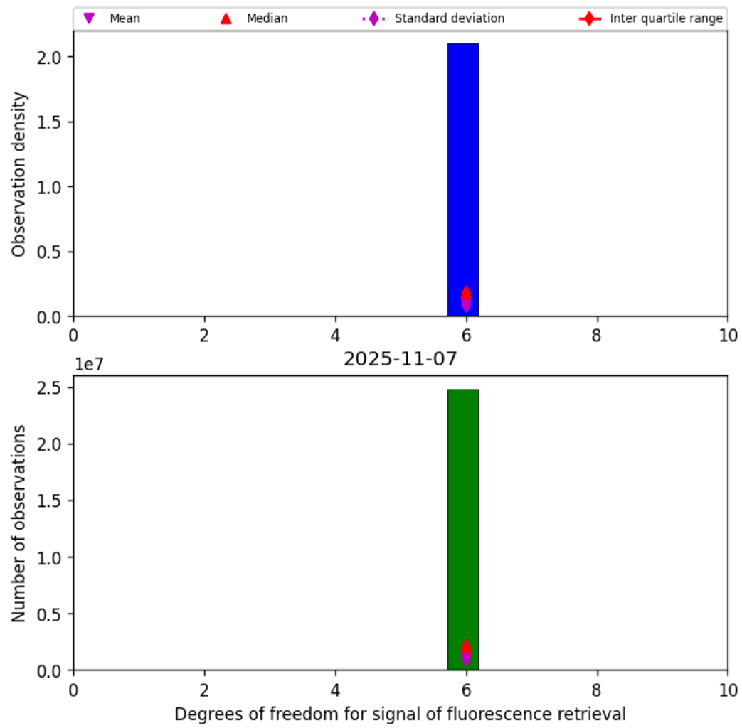
Figure 43: Histogram of “Degrees of freedom for signal of fluorescence retrieval” for 2025-11-07 to 2025-11-08
