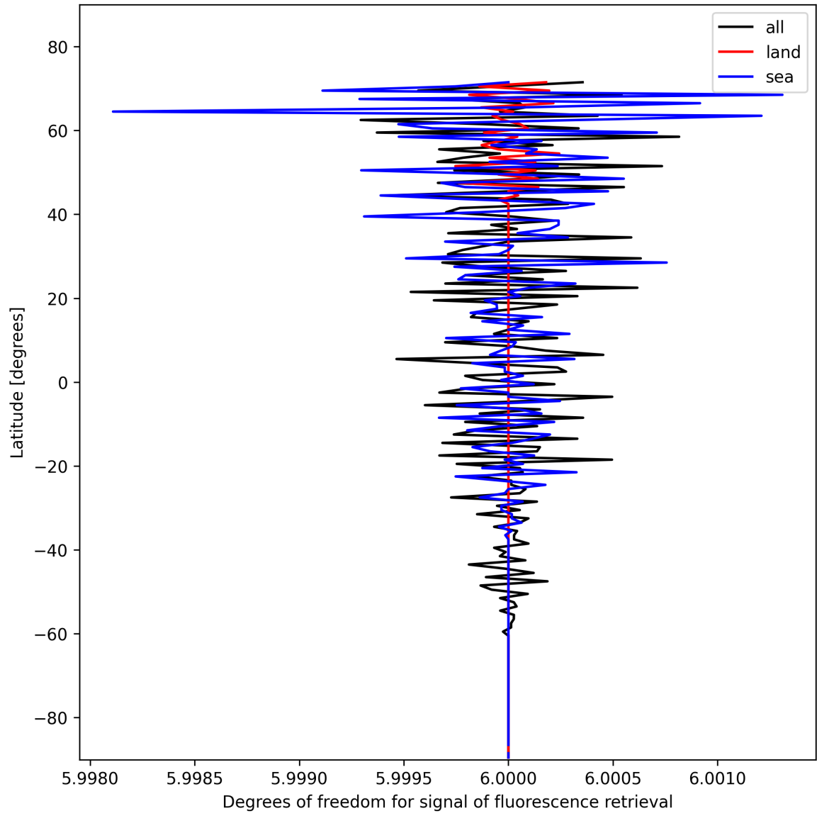
Figure 26: Zonal average of “Degrees of freedom for signal of fluorescence retrieval” for 2025-11-07 to 2025-11-08.
