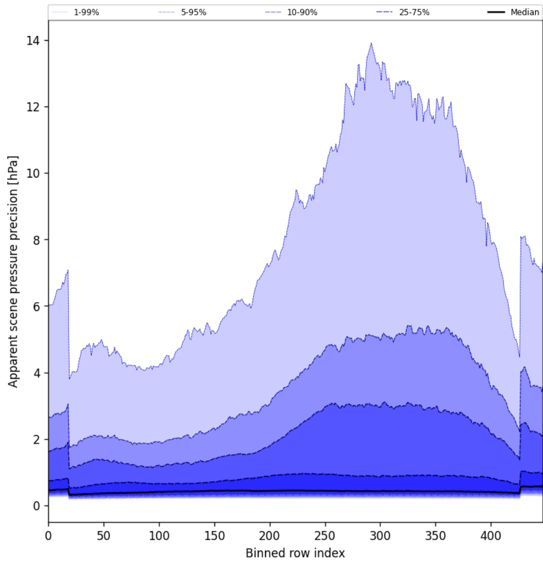
Figure 54: Along track statistics of “Apparent scene pressure precision” for 2025-11-07 to 2025-11-08
