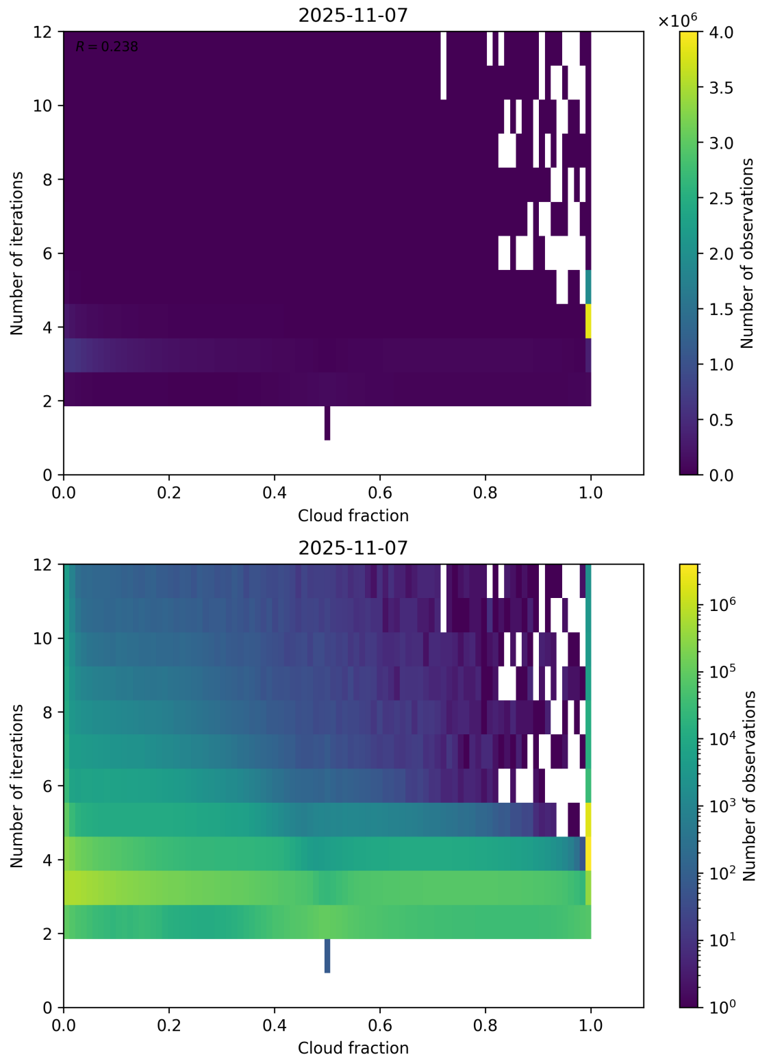
Figure 73: Scatter density plot of “Cloud fraction” against “Number of iterations” for 2025-11-07 to 2025-11-08.
