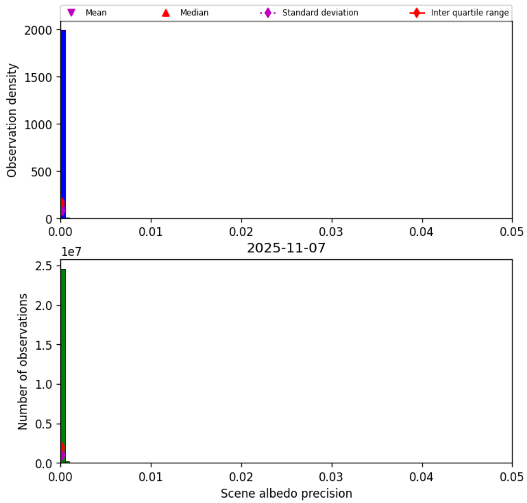
Figure 35: Histogram of “Scene albedo precision” for 2025-11-07 to 2025-11-08
