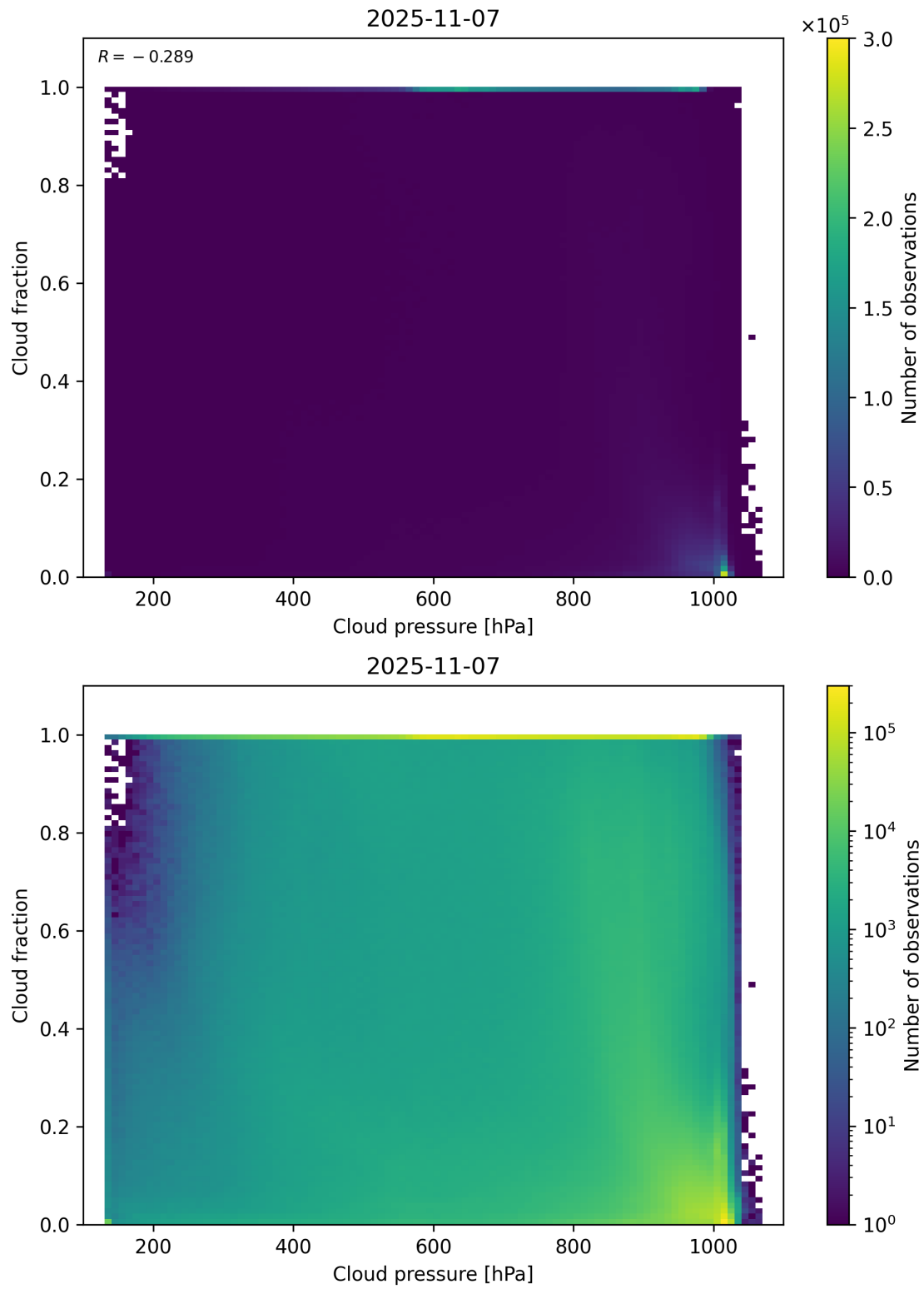
Figure 79: Scatter density plot of “Cloud pressure” against “Cloud fraction” for 2025-11-07 to 2025-11-08.
