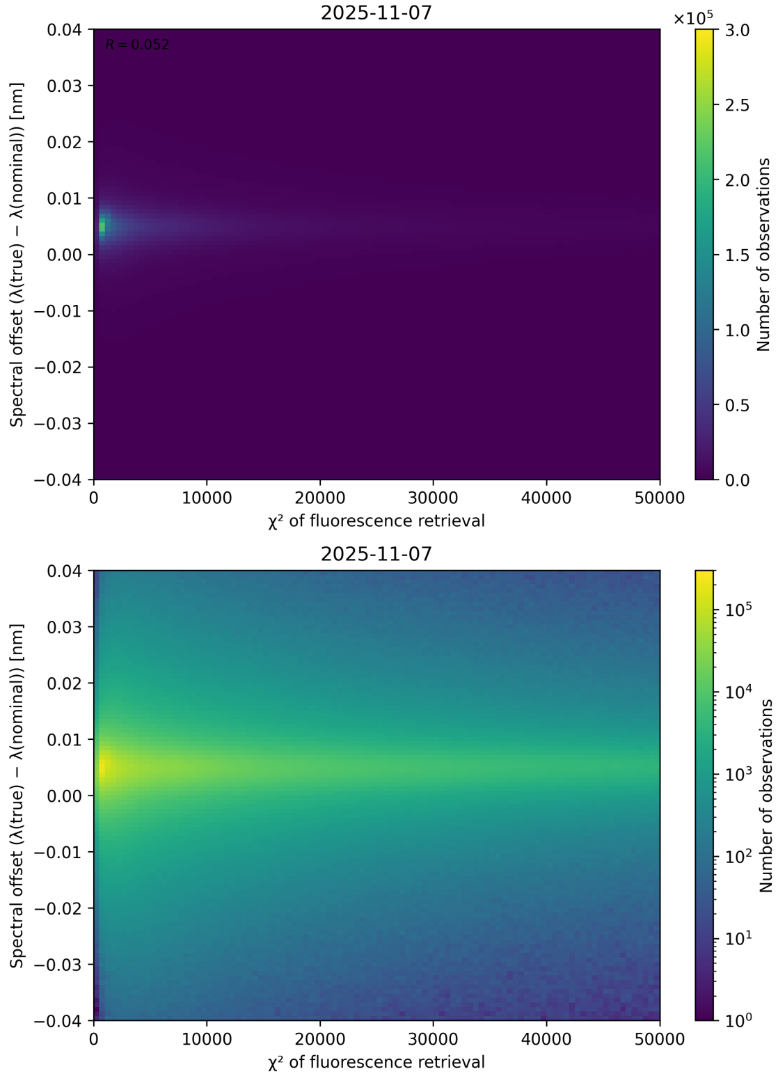
Figure 69: Scatter density plot of “ \chi^2 of fluorescence retrieval” against “Spectral offset ( \lambda_{\text{true}} - \lambda_{\text{nominal}} )” for 2025-11-07 to 2025-11-08.
