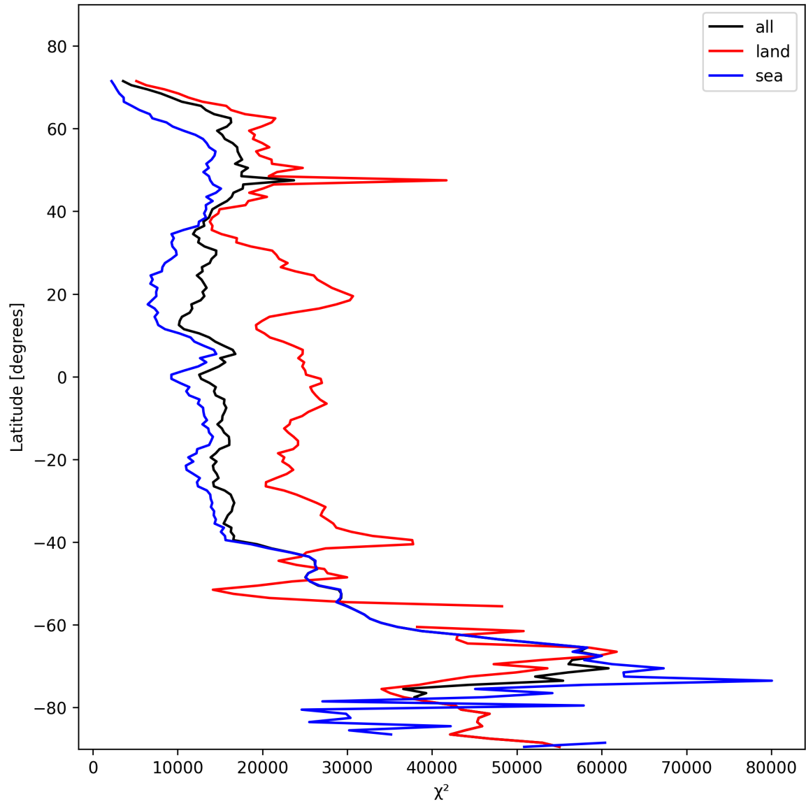
Figure 21: Zonal average of “ \chi^2 ” for 2025-11-07 to 2025-11-08.
