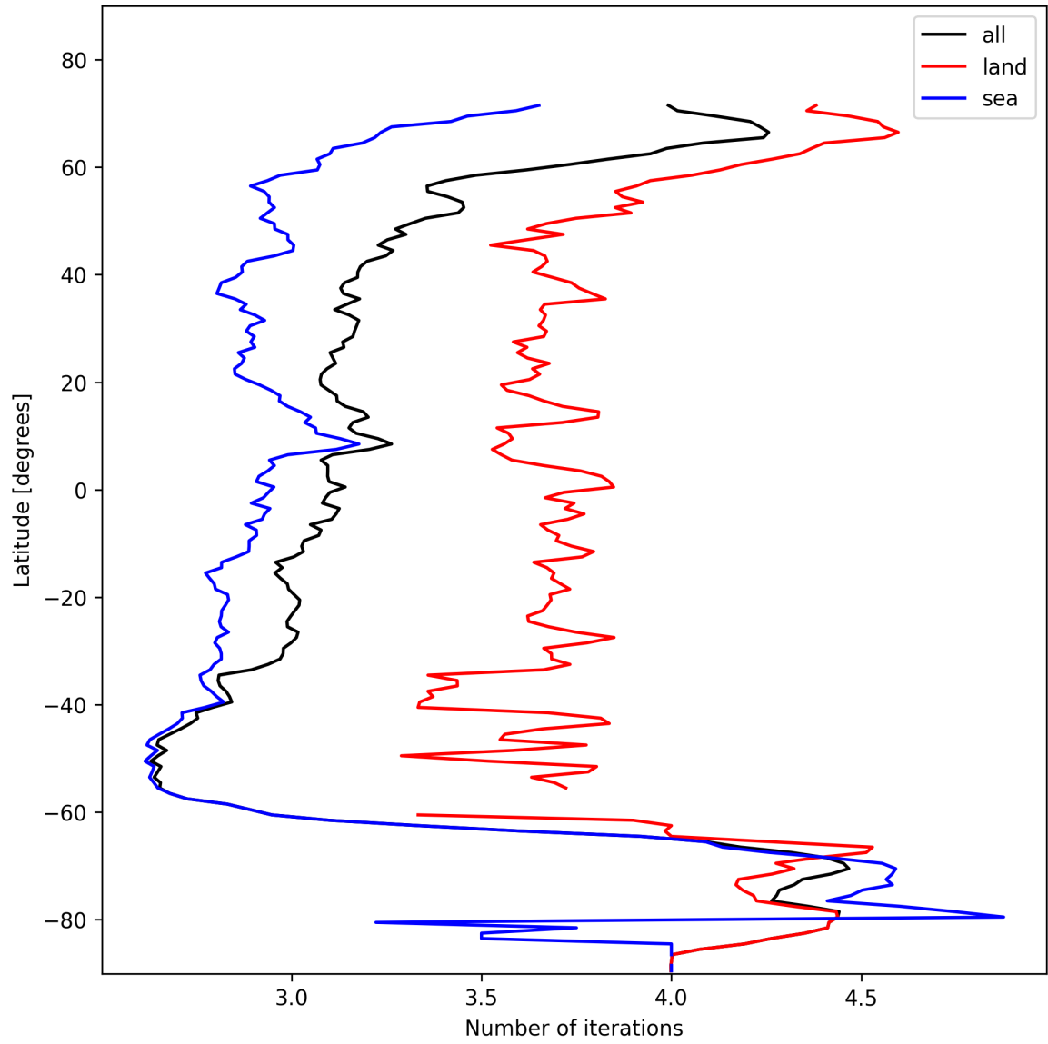
Figure 22: Zonal average of “Number of iterations” for 2025-11-07 to 2025-11-08.
