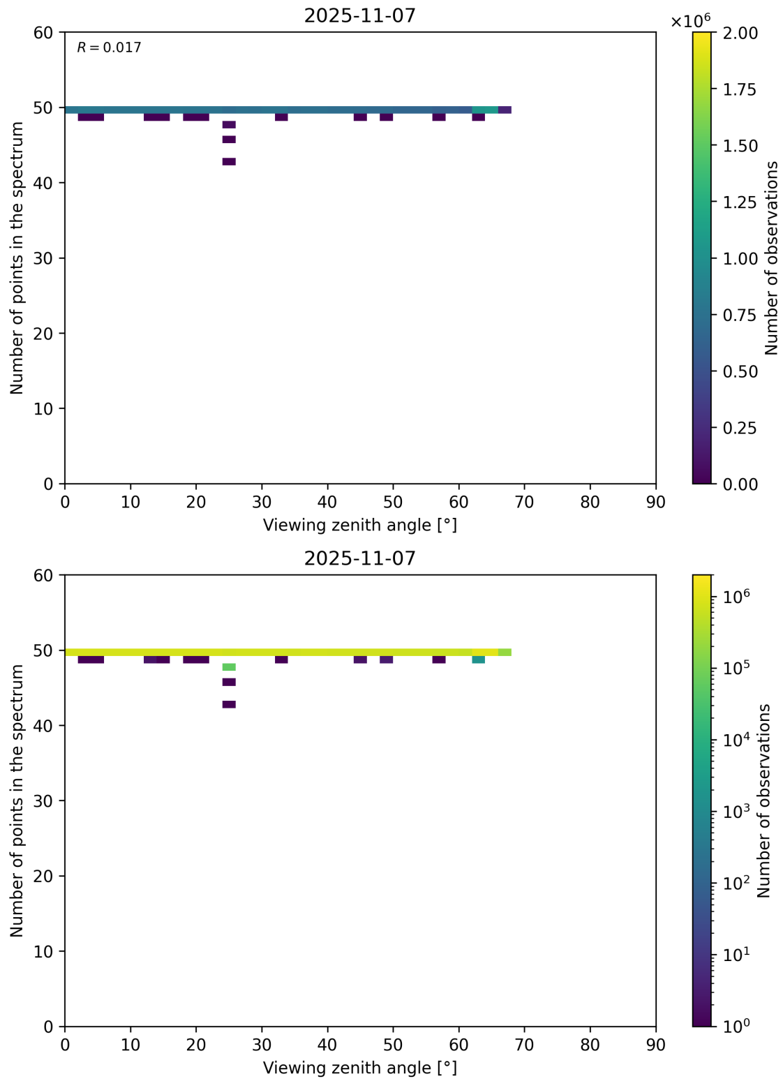
Figure 125: Scatter density plot of “Viewing zenith angle” against “Number of points in the spectrum” for 2025-11-07 to 2025-11-08.
