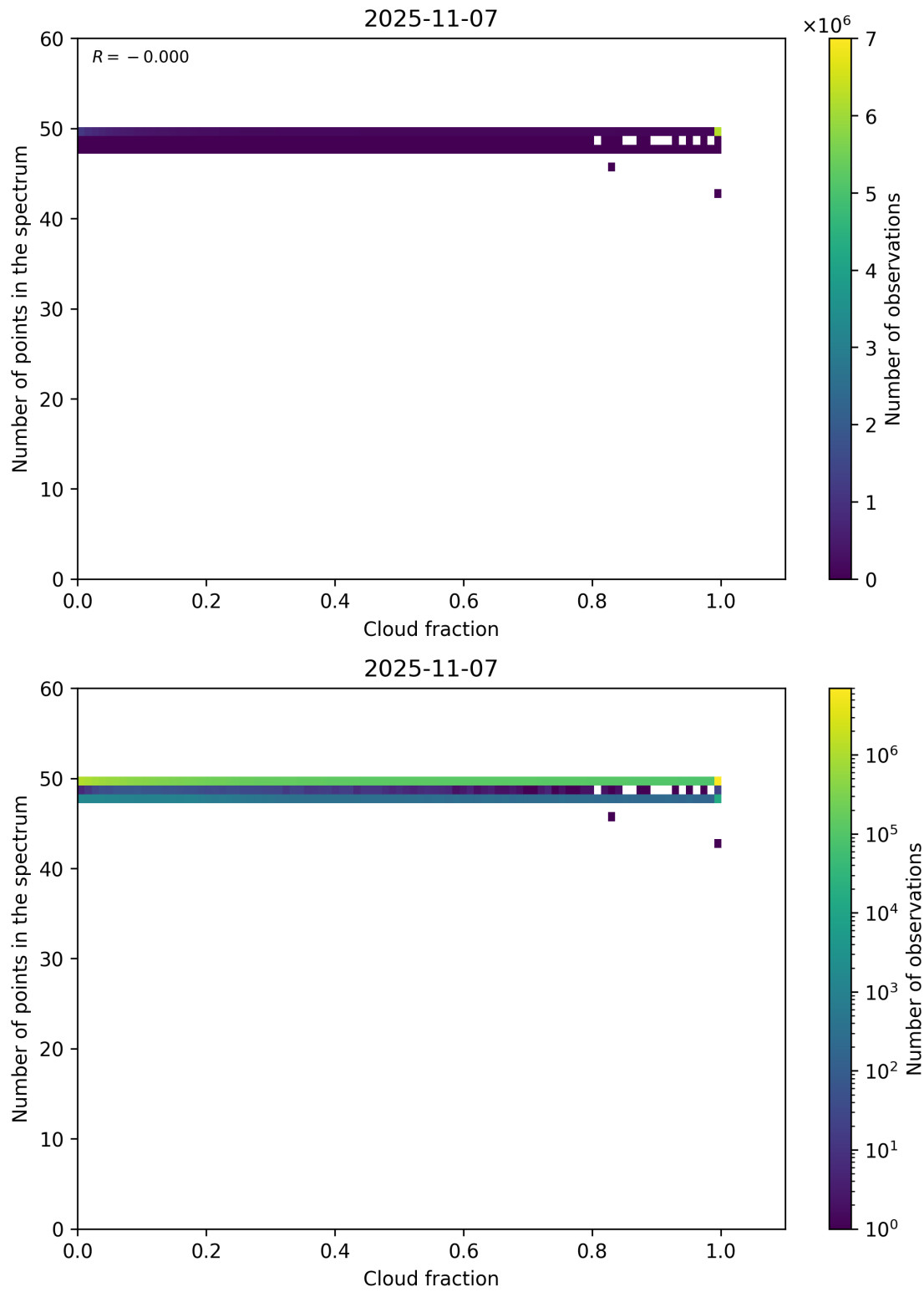
Figure 74: Scatter density plot of “Cloud fraction” against “Number of points in the spectrum” for 2025-11-07 to 2025-11-08.
