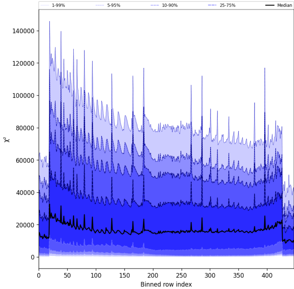
Figure 55: Along track statistics of “ \chi^2 ” for 2025-11-07 to 2025-11-08
