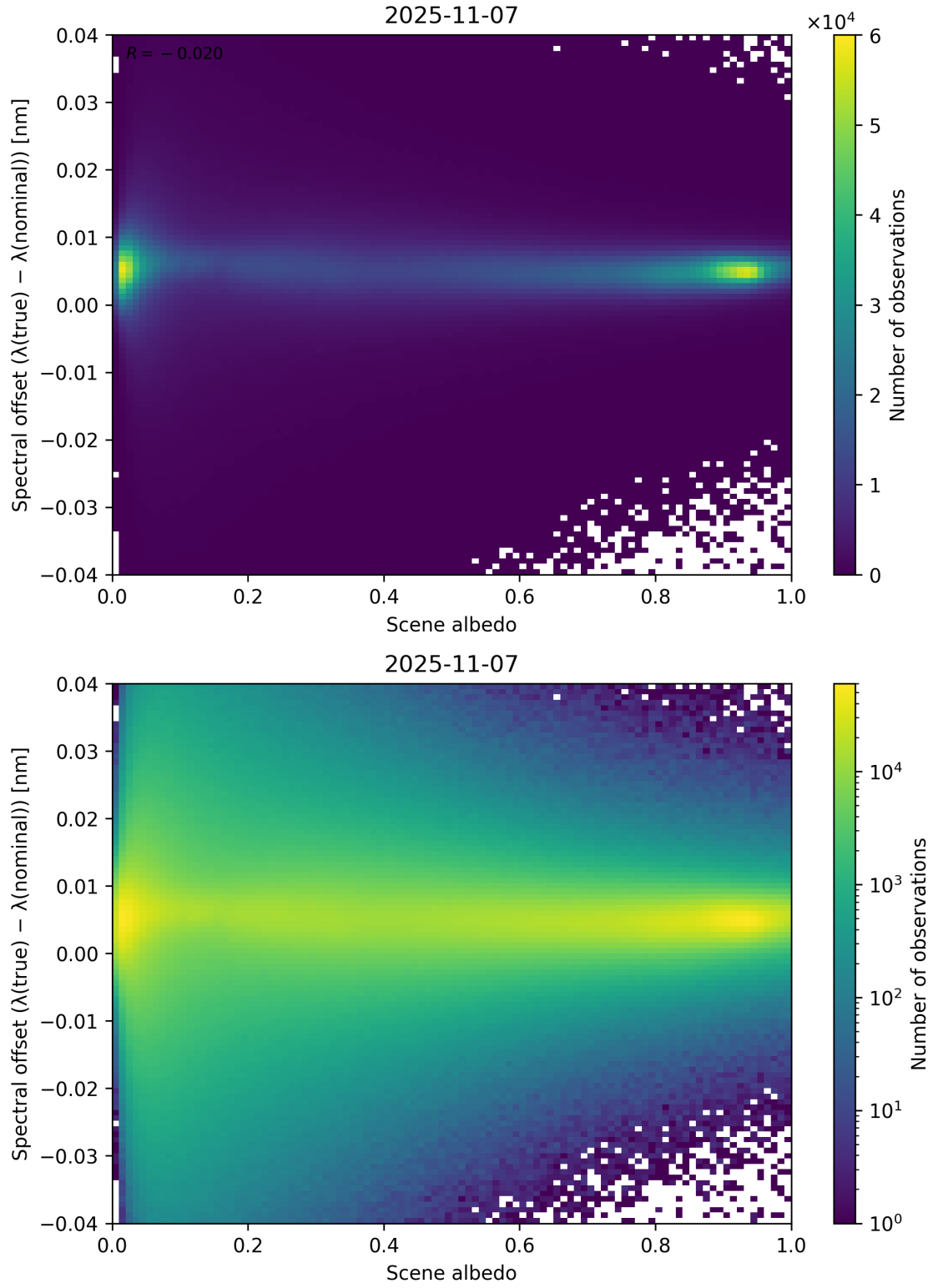
Figure 107: Scatter density plot of “Scene albedo” against “Spectral offset ( \lambda_{\text{true}} - \lambda_{\text{nominal}} )” for 2025-11-07 to 2025-11-08.
