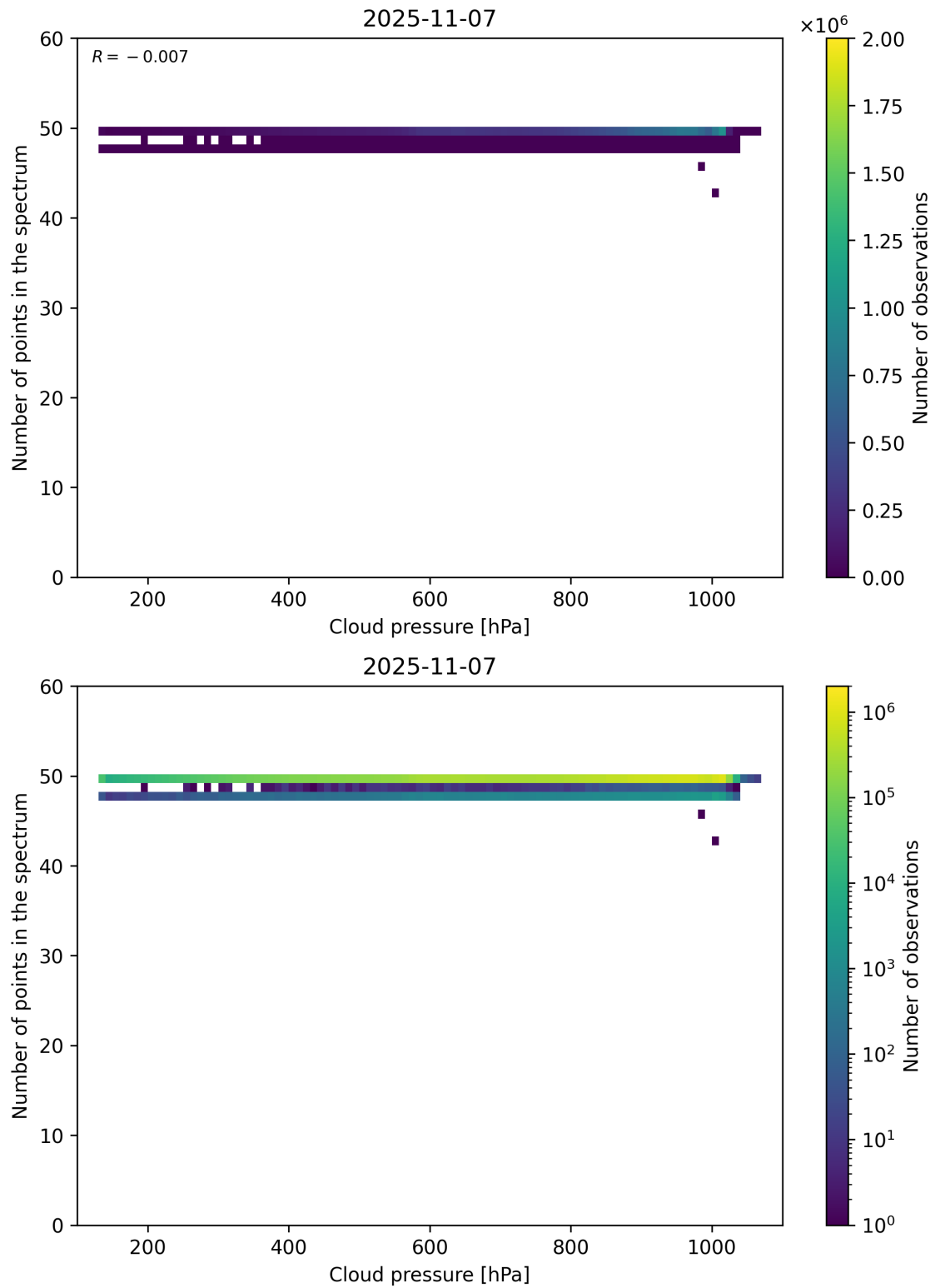
Figure 82: Scatter density plot of “Cloud pressure” against “Number of points in the spectrum” for 2025-11-07 to 2025-11-08.
