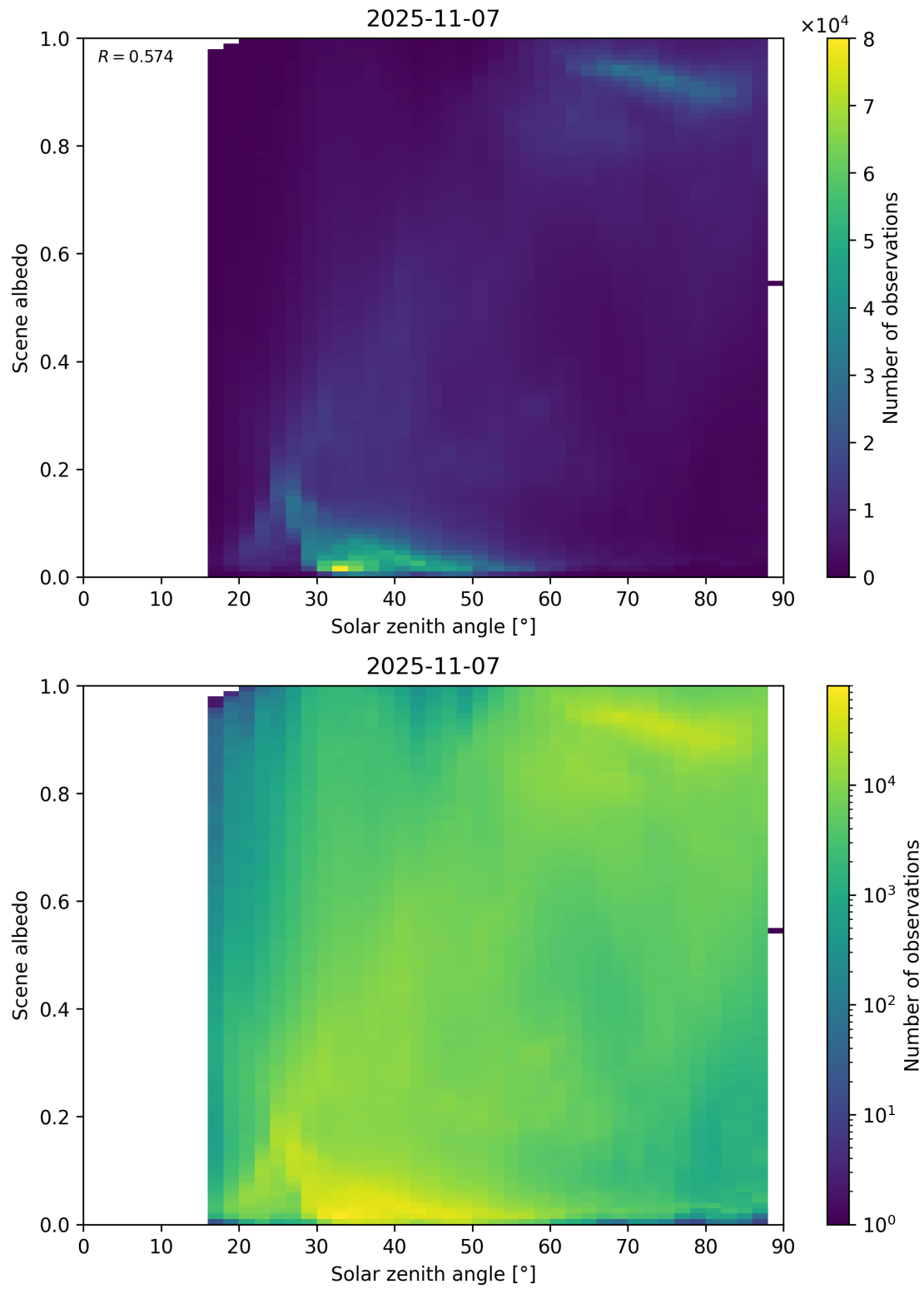
Figure 116: Scatter density plot of “Solar zenith angle” against “Scene albedo” for 2025-11-07 to 2025-11-08.
