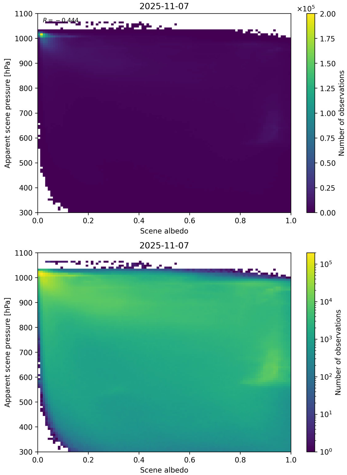
Figure 102: Scatter density plot of “Scene albedo” against “Apparent scene pressure” for 2025-11-07 to 2025-11-08.
