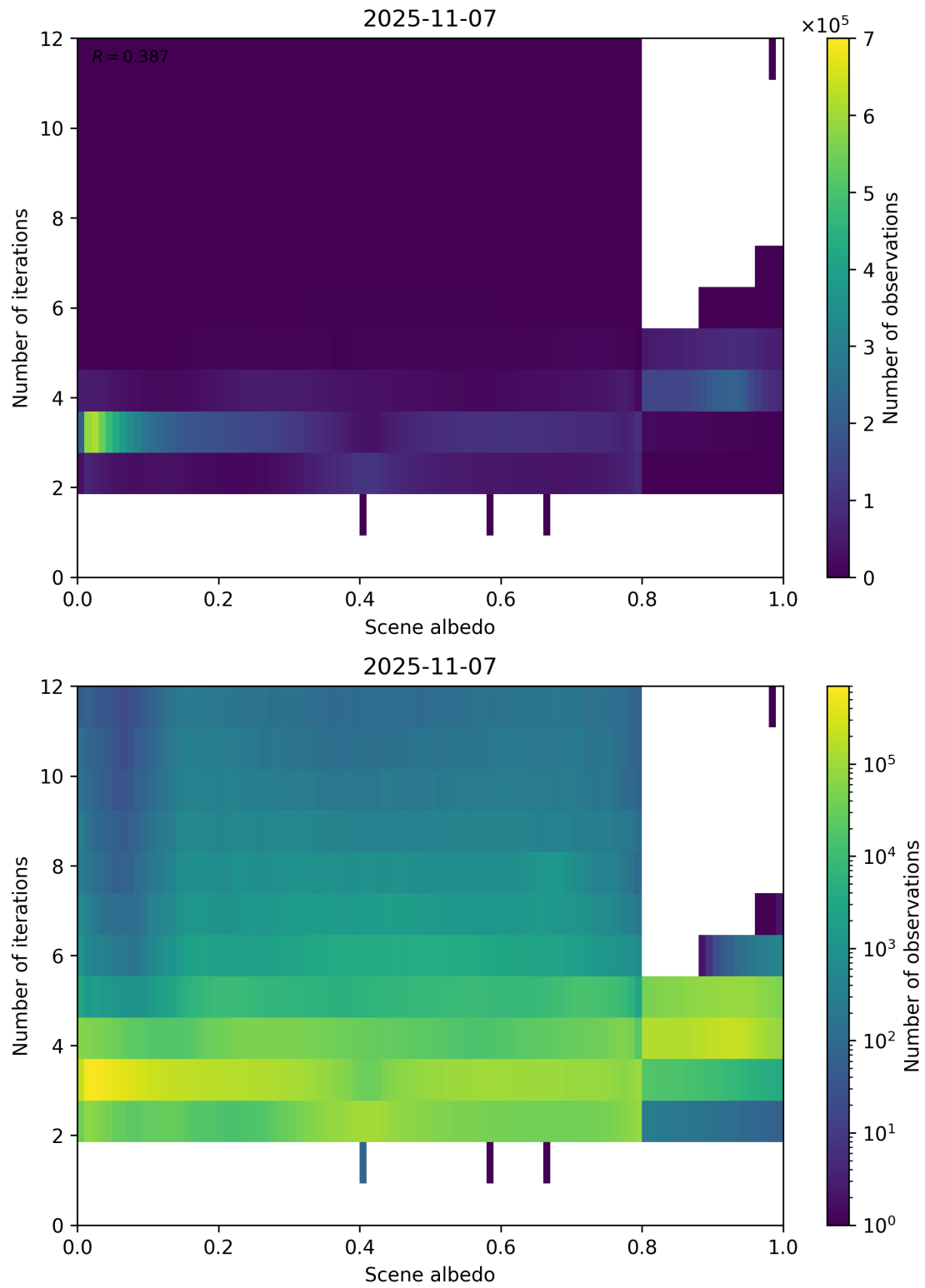
Figure 105: Scatter density plot of “Scene albedo” against “Number of iterations” for 2025-11-07 to 2025-11-08.
