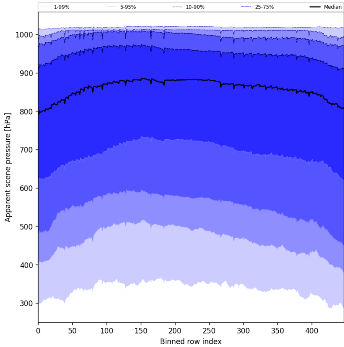
Figure 53: Along track statistics of “Apparent scene pressure” for 2025-11-07 to 2025-11-08
