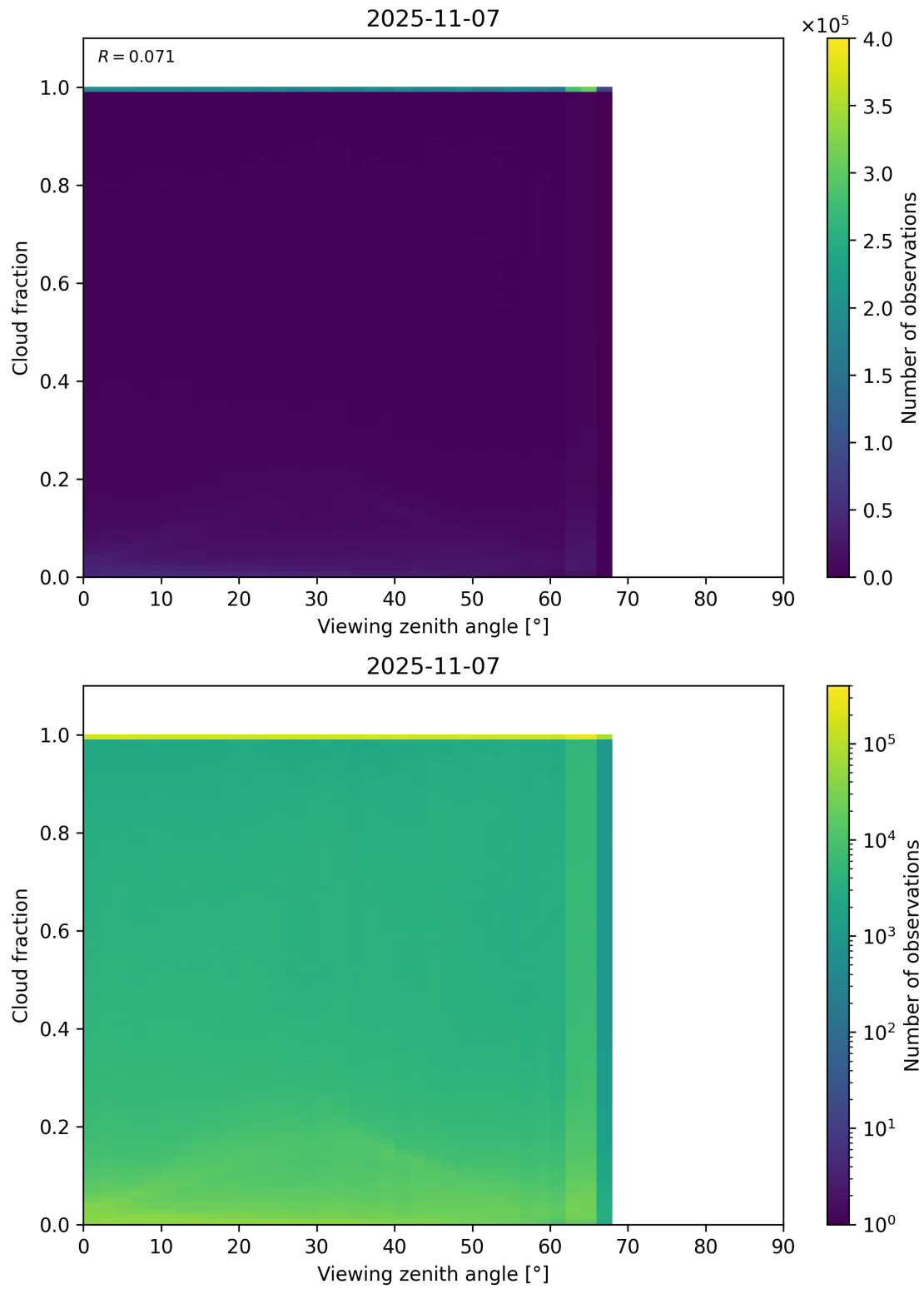
Figure 120: Scatter density plot of “Viewing zenith angle” against “Cloud fraction” for 2025-11-07 to 2025-11-08.
