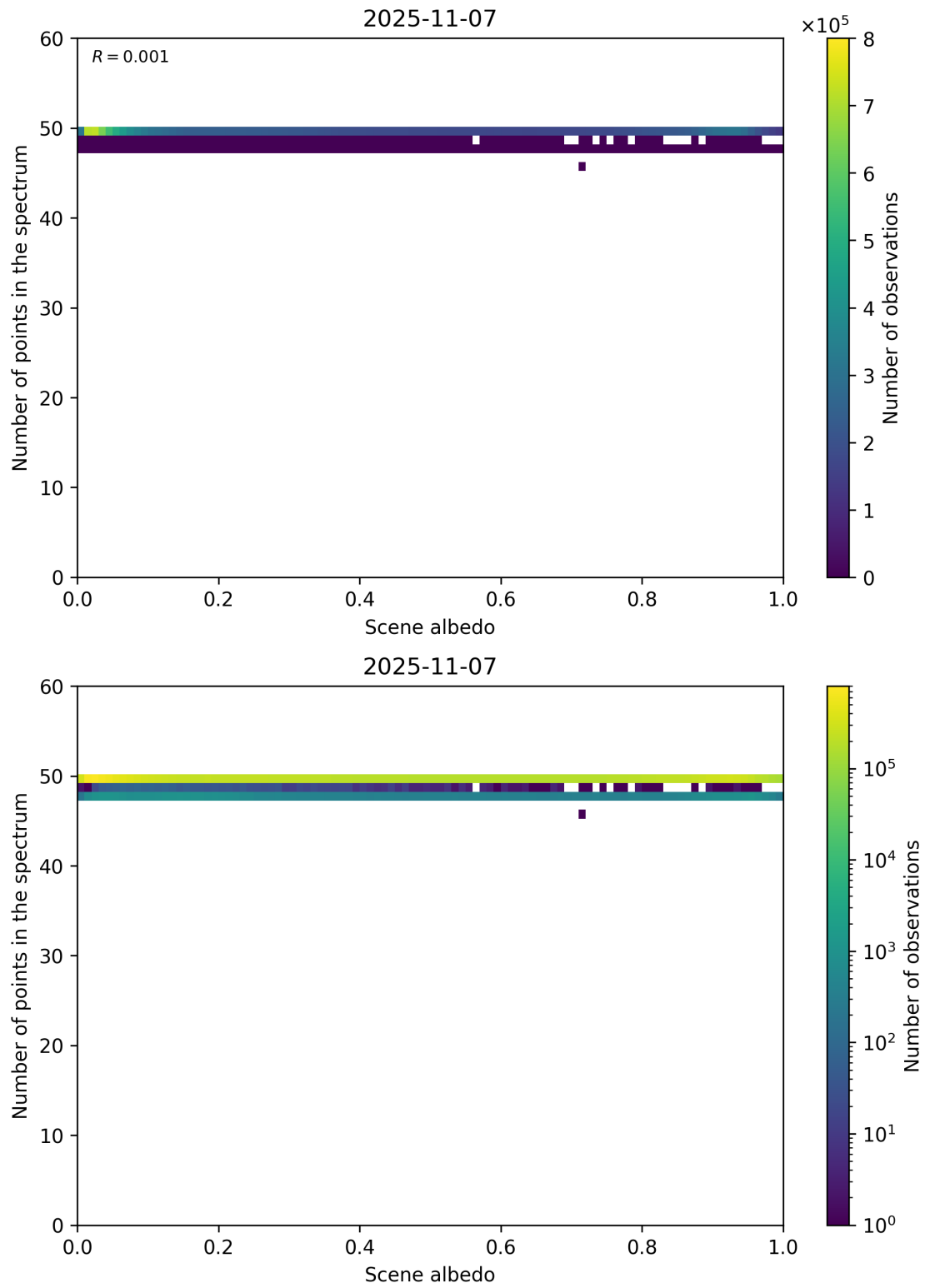
Figure 106: Scatter density plot of “Scene albedo” against “Number of points in the spectrum” for 2025-11-07 to 2025-11-08.
