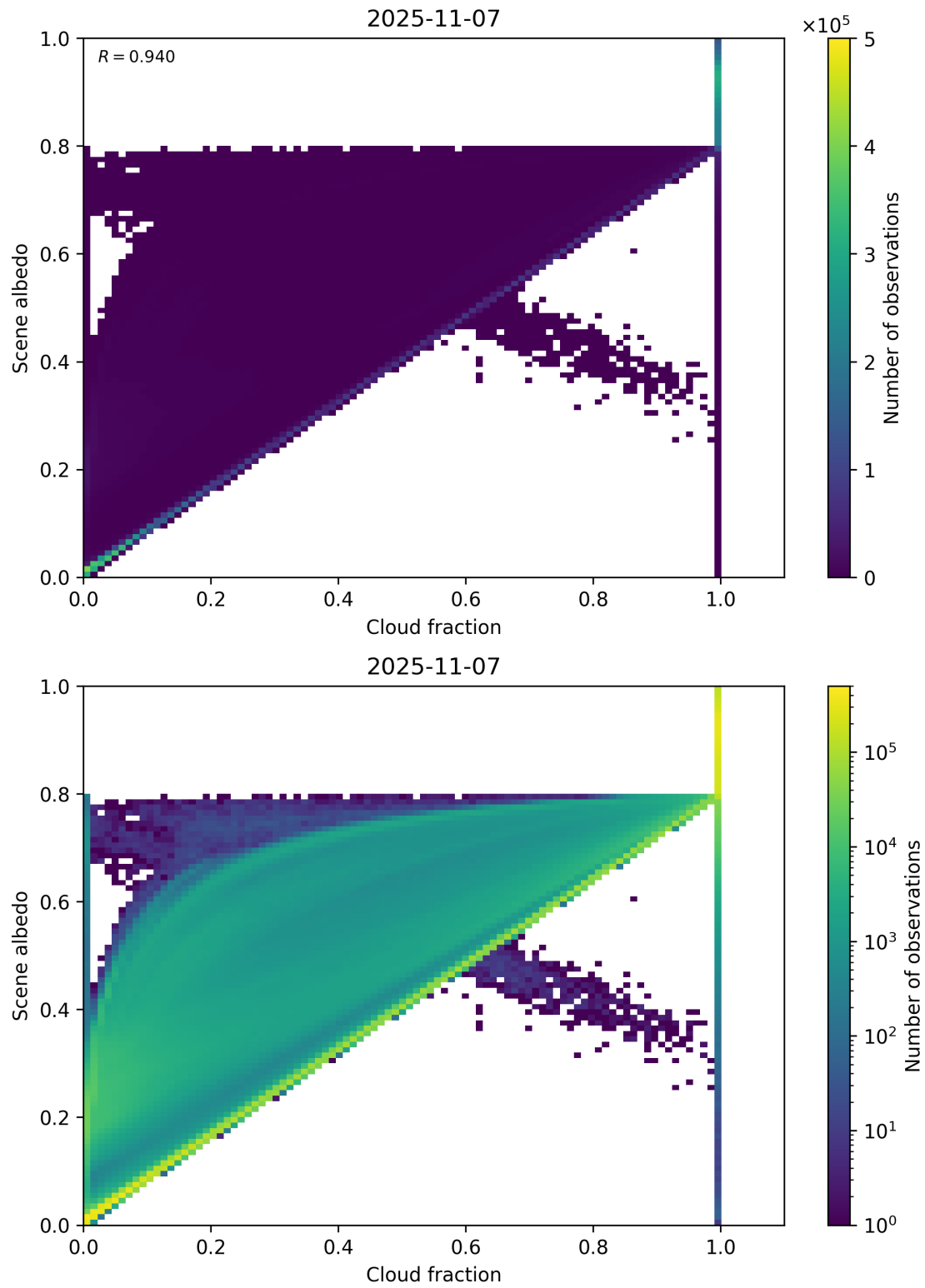
Figure 75: Scatter density plot of “Cloud fraction” against “Scene albedo” for 2025-11-07 to 2025-11-08.
