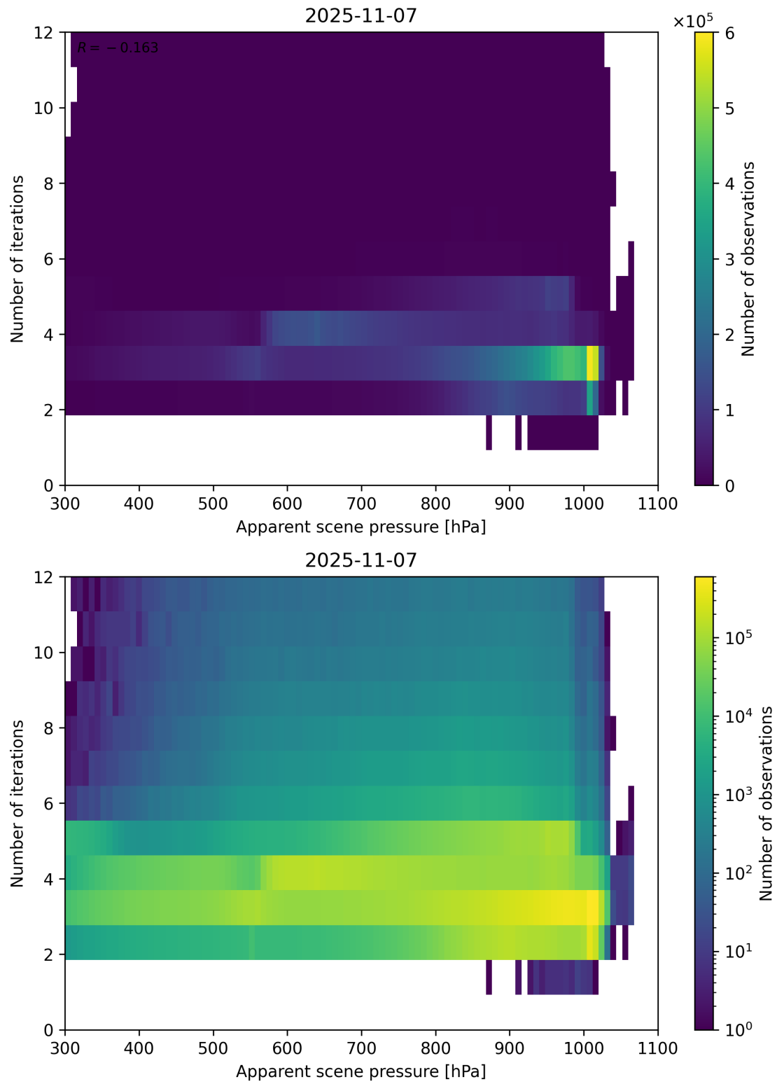
Figure 65: Scatter density plot of “Apparent scene pressure” against “Number of iterations” for 2025-11-07 to 2025-11-08.
