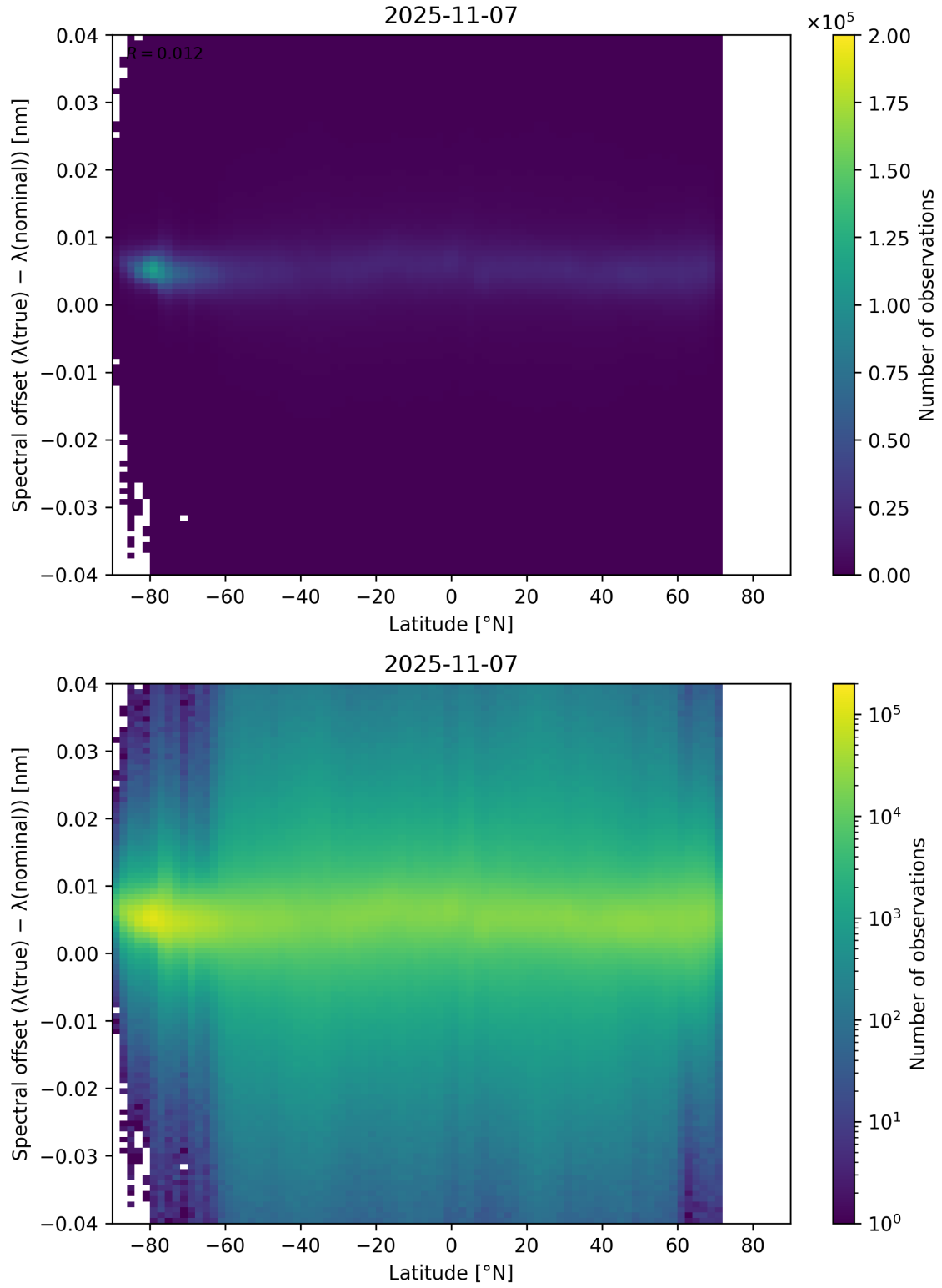
Figure 96: Scatter density plot of “Latitude” against “Spectral offset ( \lambda_{\text{true}} - \lambda_{\text{nominal}} )” for 2025-11-07 to 2025-11-08.
