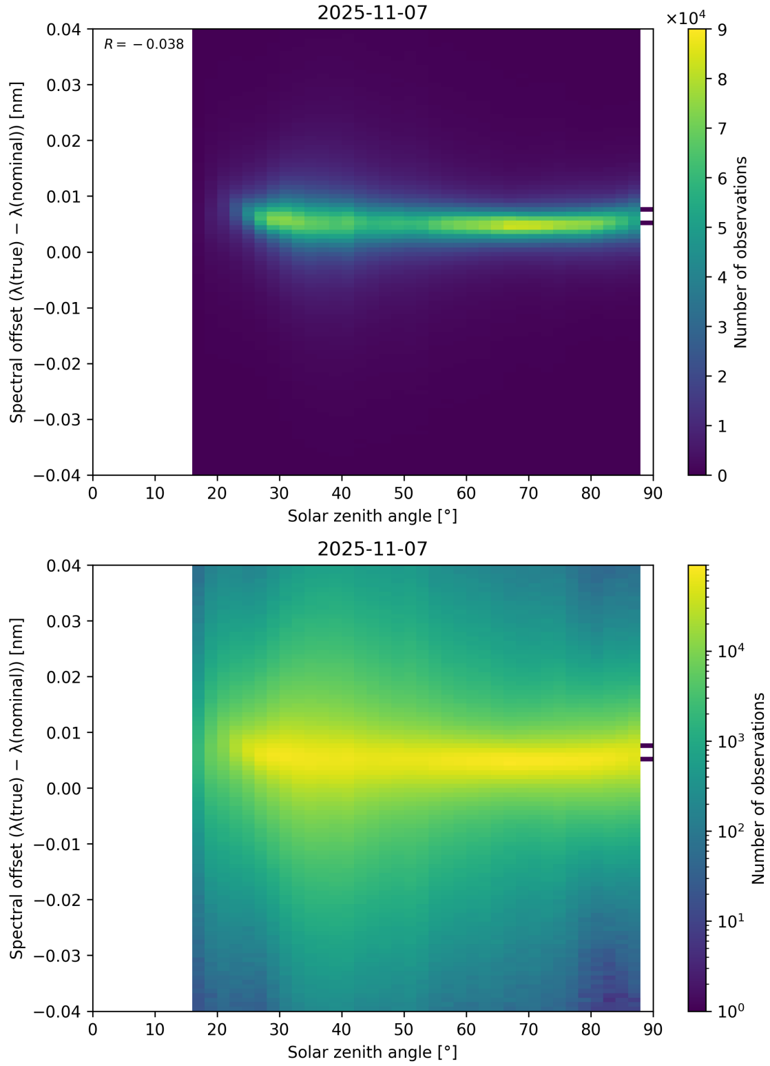
Figure 117: Scatter density plot of “Solar zenith angle” against “Spectral offset ( \lambda_{\text{true}} - \lambda_{\text{nominal}} )” for 2025-11-07 to 2025-11-08.
