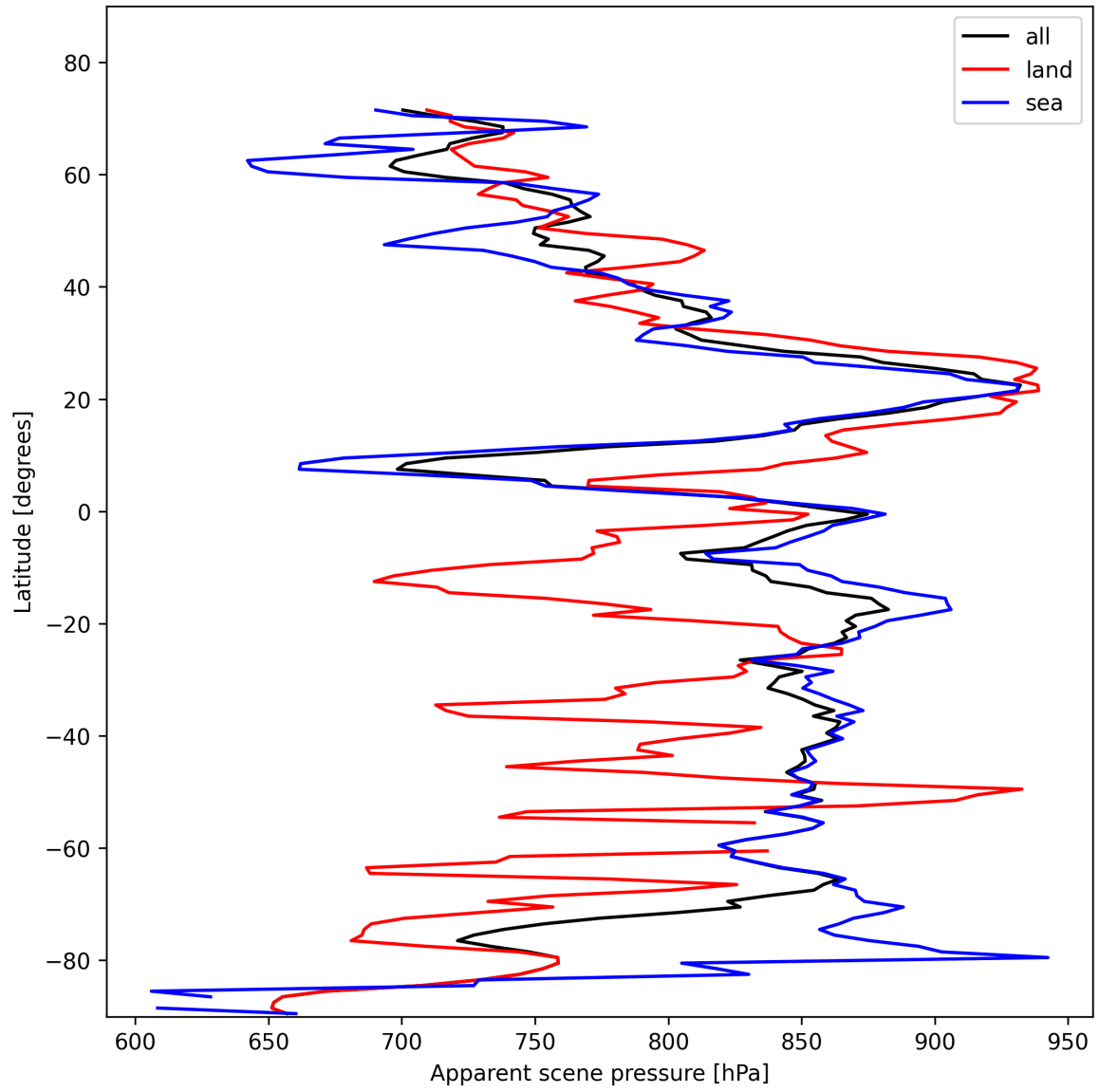
Figure 19: Zonal average of “Apparent scene pressure” for 2025-11-07 to 2025-11-08.
