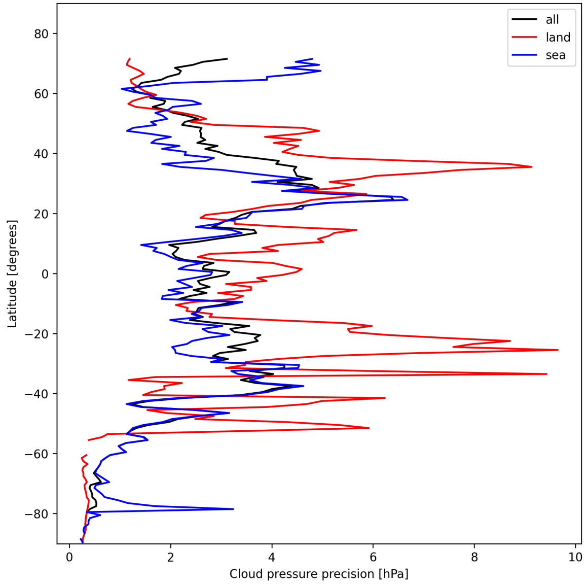
Figure 14: Zonal average of “Cloud pressure precision” for 2025-11-07 to 2025-11-08.
