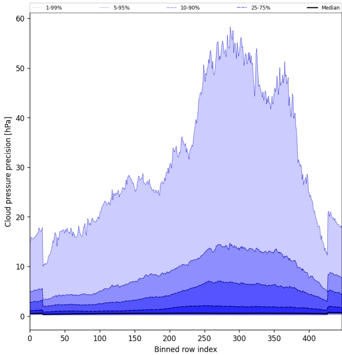
Figure 48: Along track statistics of “Cloud pressure precision” for 2025-11-07 to 2025-11-08
