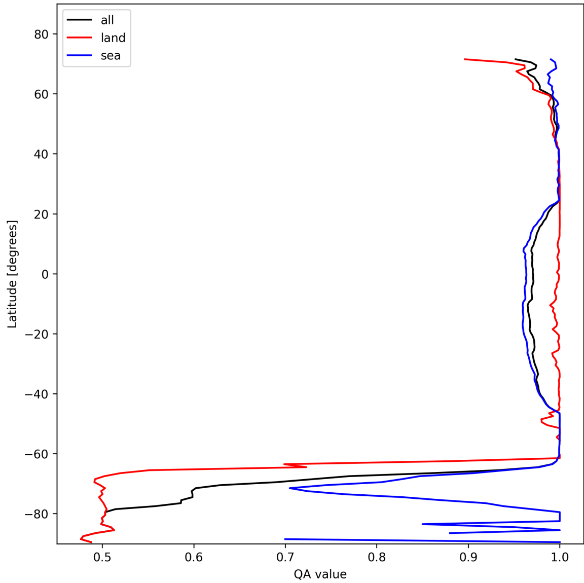
Figure 12: Zonal average of “QA value” for 2025-11-07 to 2025-11-08.
