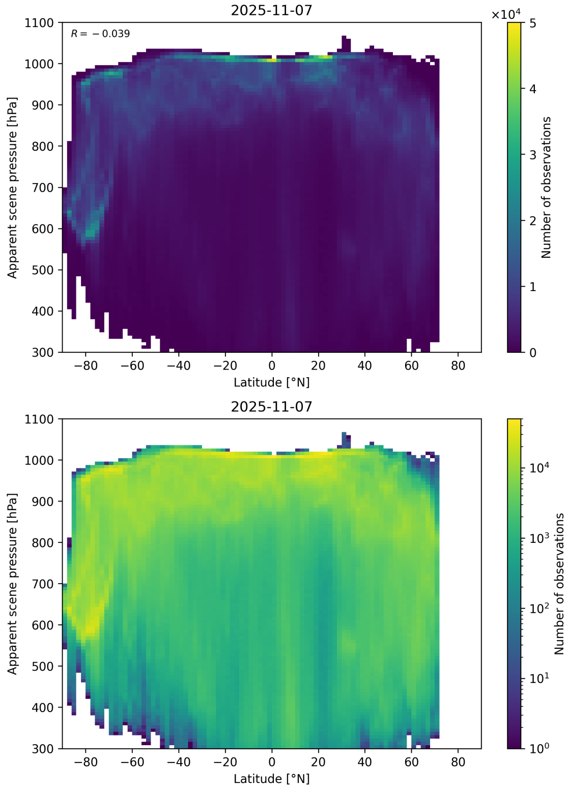
Figure 88: Scatter density plot of “Latitude” against “Apparent scene pressure” for 2025-11-07 to 2025-11-08.
