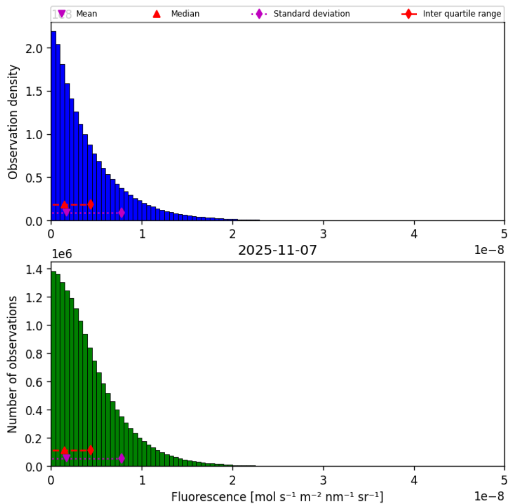
Figure 40: Histogram of “Fluorescence” for 2025-11-07 to 2025-11-08
