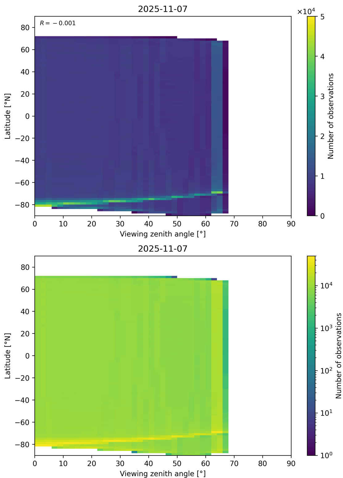
Figure 123: Scatter density plot of “Viewing zenith angle” against “Latitude” for 2025-11-07 to 2025-11-08.
