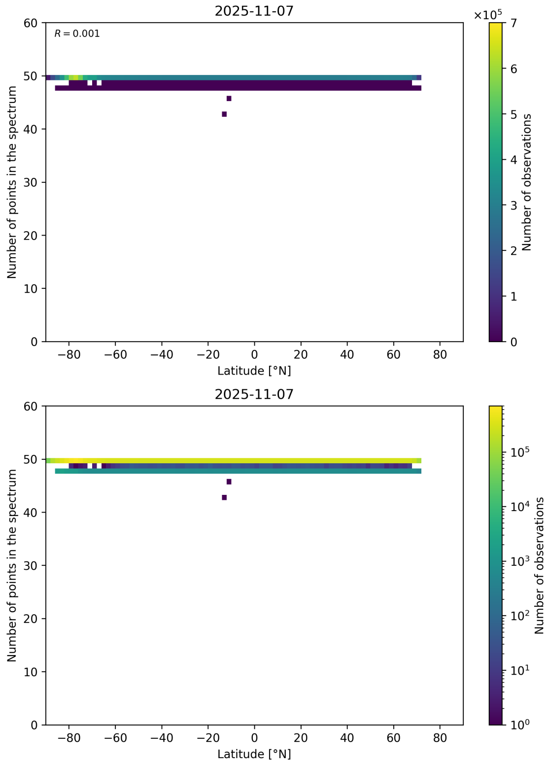
Figure 94: Scatter density plot of “Latitude” against “Number of points in the spectrum” for 2025-11-07 to 2025-11-08.
