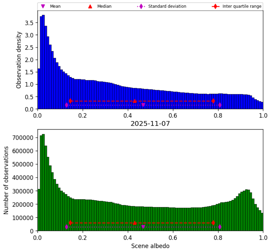
Figure 34: Histogram of “Scene albedo” for 2025-11-07 to 2025-11-08
