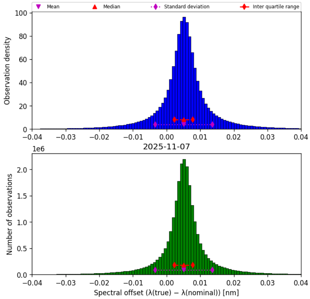
Figure 45: Histogram of “Spectral offset ( \lambda_{\text{true}} - \lambda_{\text{nominal}} )” for 2025-11-07 to 2025-11-08
