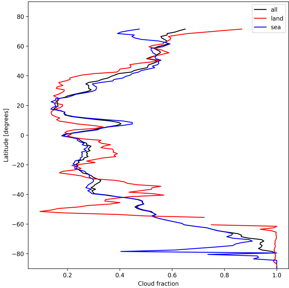
Figure 15: Zonal average of “Cloud fraction” for 2025-11-07 to 2025-11-08.
