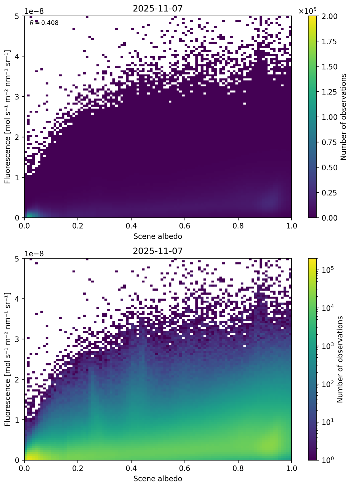
Figure 104: Scatter density plot of “Scene albedo” against “Fluorescence” for 2025-11-07 to 2025-11-08.
