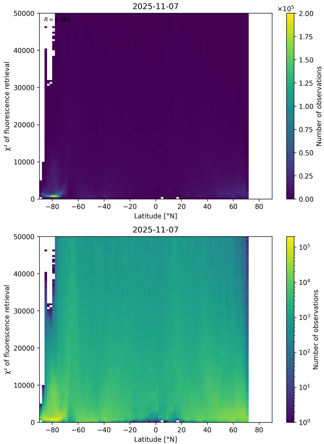
Figure 89: Scatter density plot of “Latitude” against “ \chi^2 of fluorescence retrieval” for 2025-11-07 to 2025-11-08.
