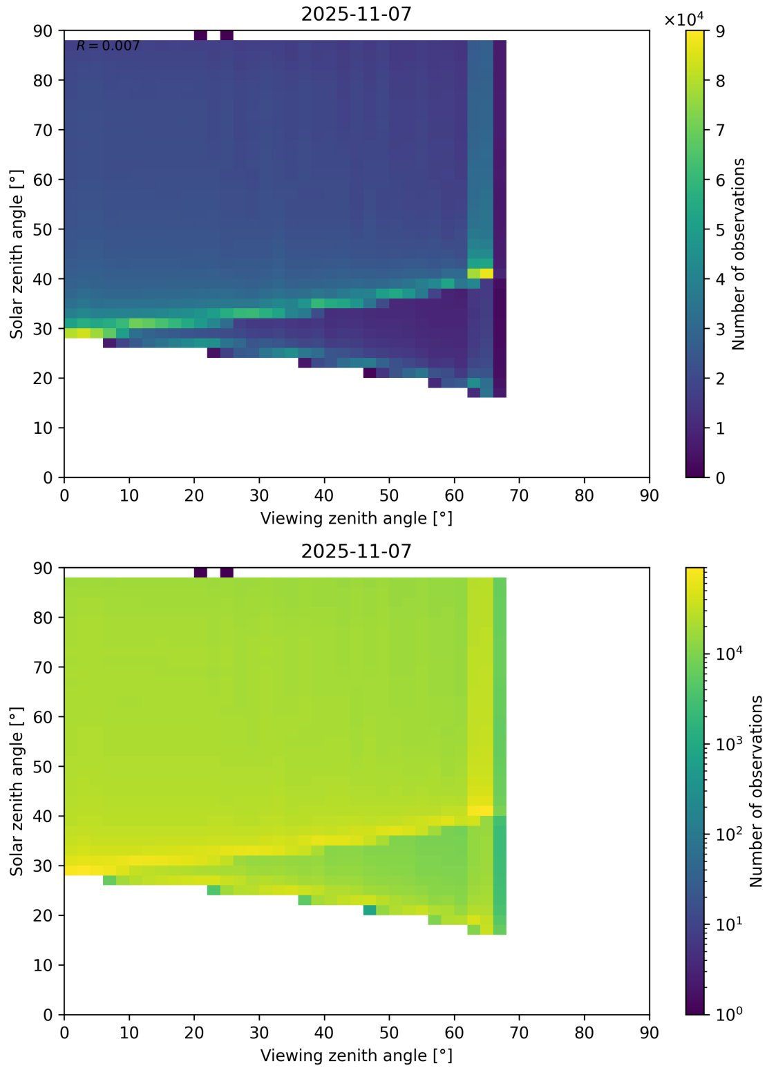
Figure 127: Scatter density plot of “Viewing zenith angle” against “Solar zenith angle” for 2025-11-07 to 2025-11-08.
