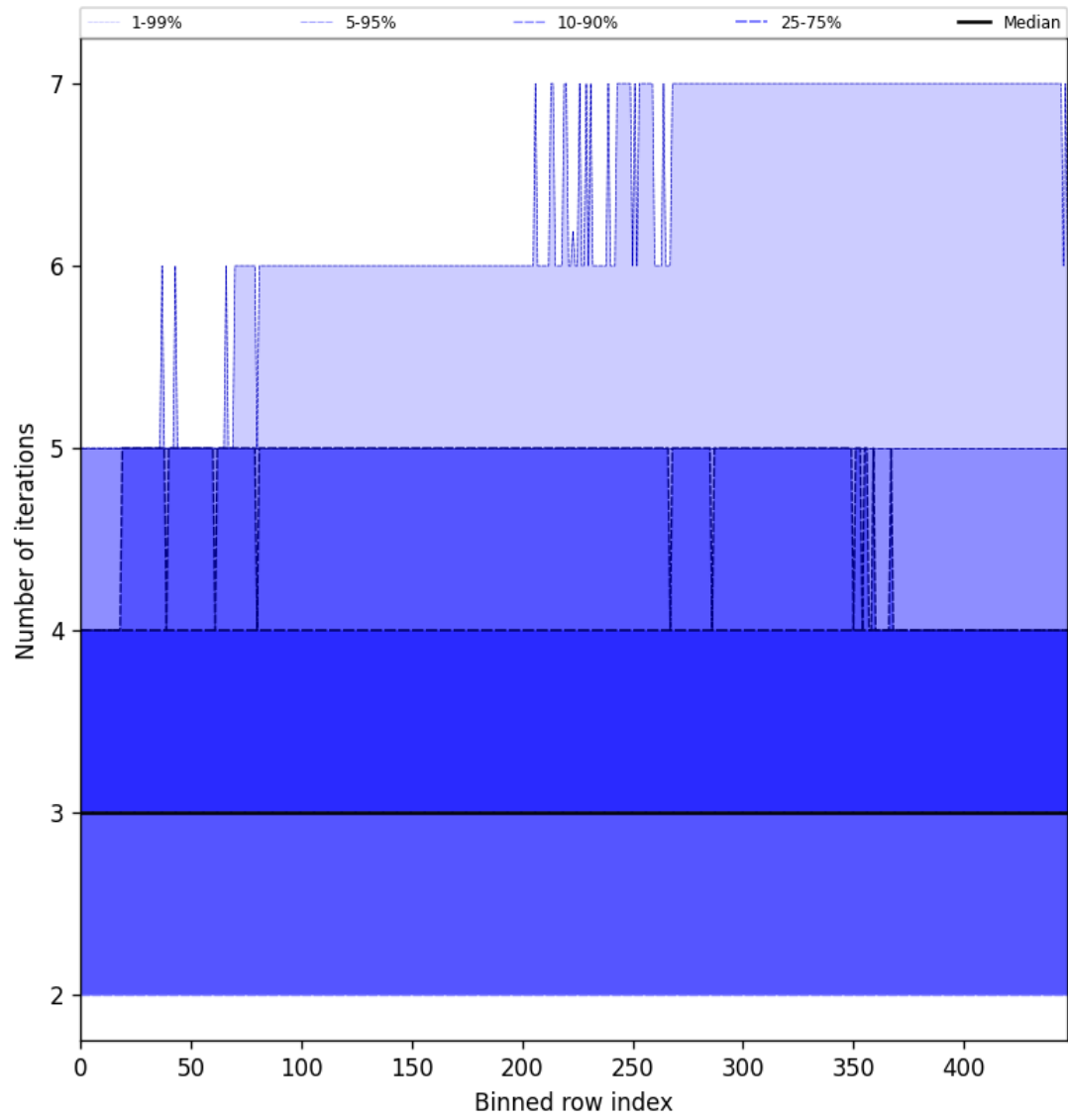
Figure 56: Along track statistics of “Number of iterations” for 2025-11-07 to 2025-11-08
