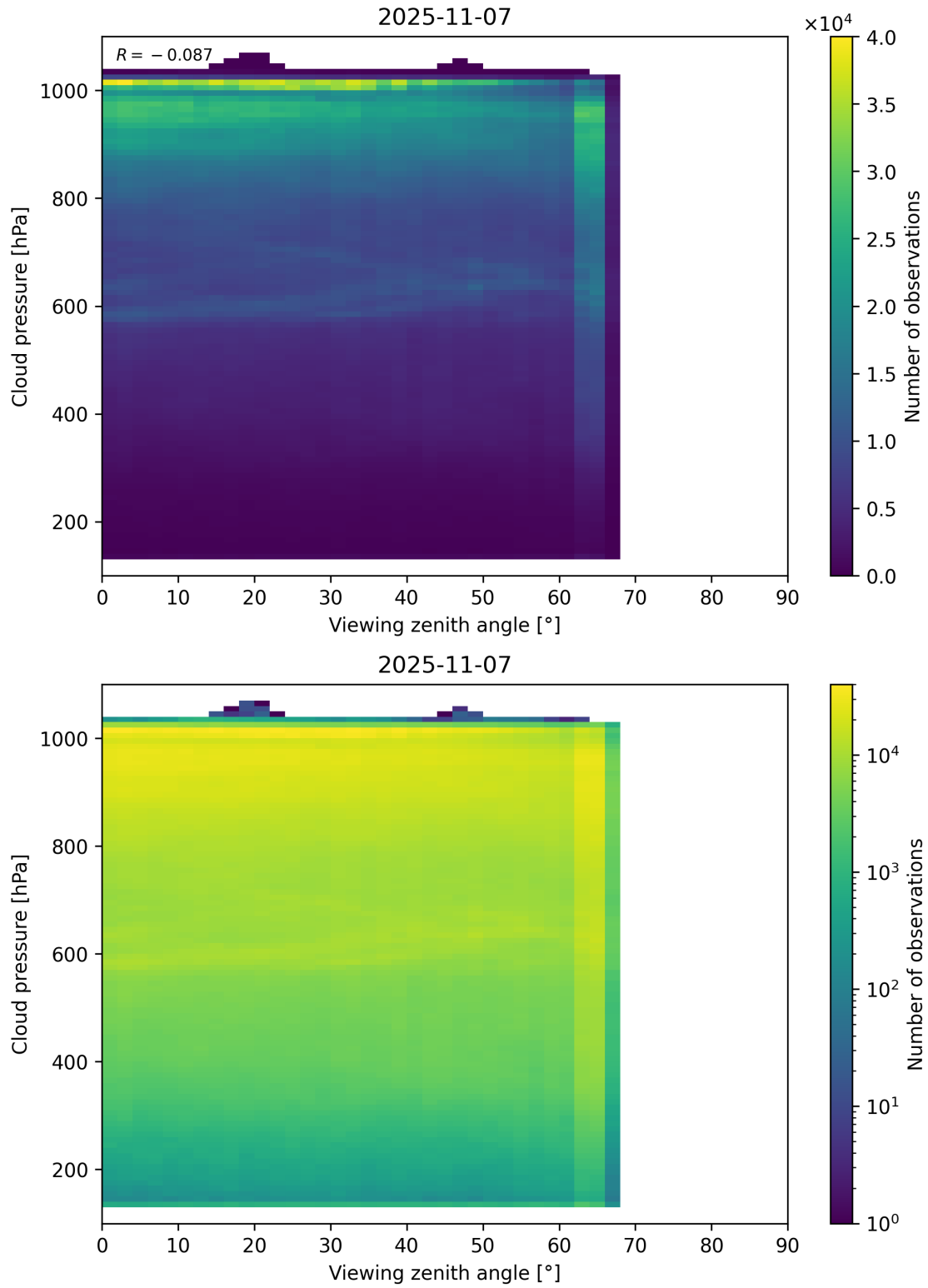
Figure 121: Scatter density plot of “Viewing zenith angle” against “Cloud pressure” for 2025-11-07 to 2025-11-08.
