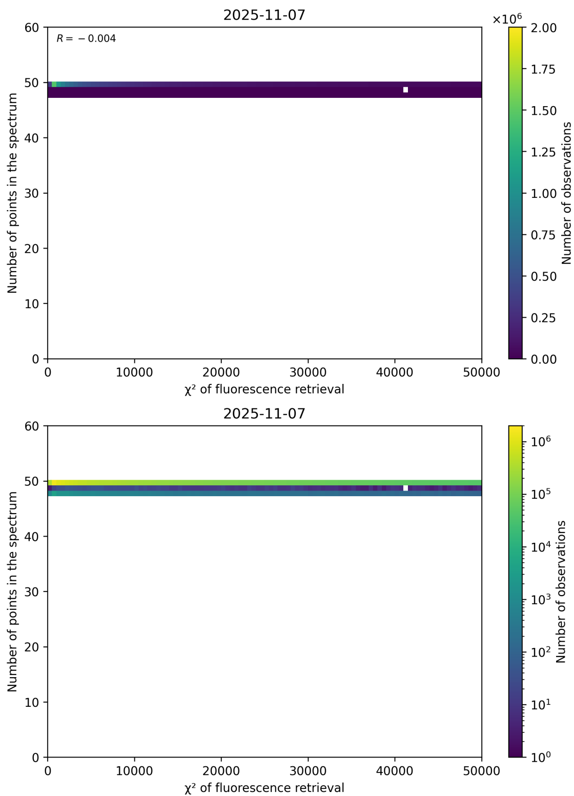
Figure 68: Scatter density plot of “ \chi^2 of fluorescence retrieval” against “Number of points in the spectrum” for 2025-11-07 to 2025-11-08.
