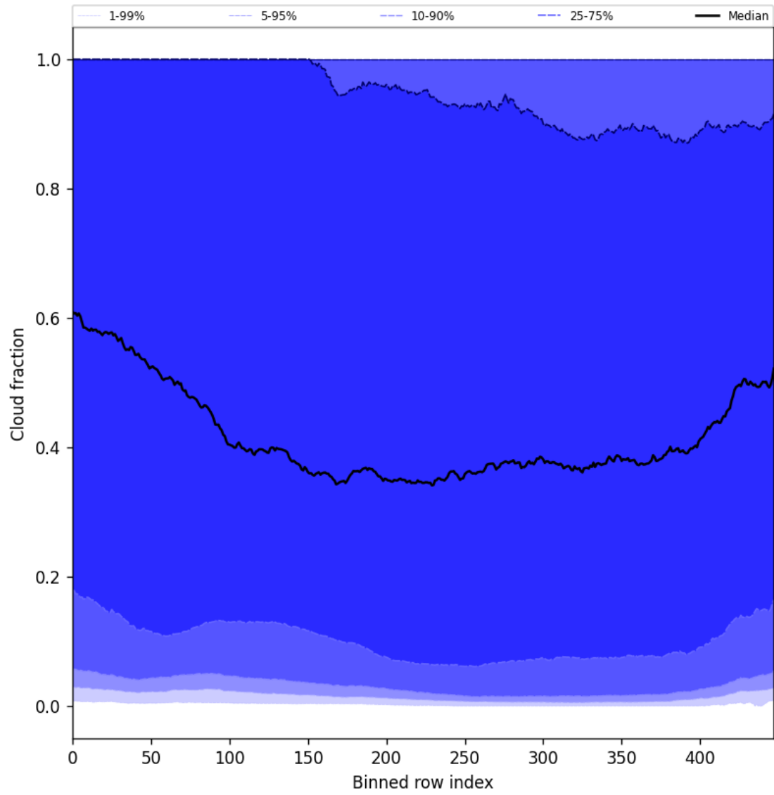
Figure 49: Along track statistics of “Cloud fraction” for 2025-11-07 to 2025-11-08
