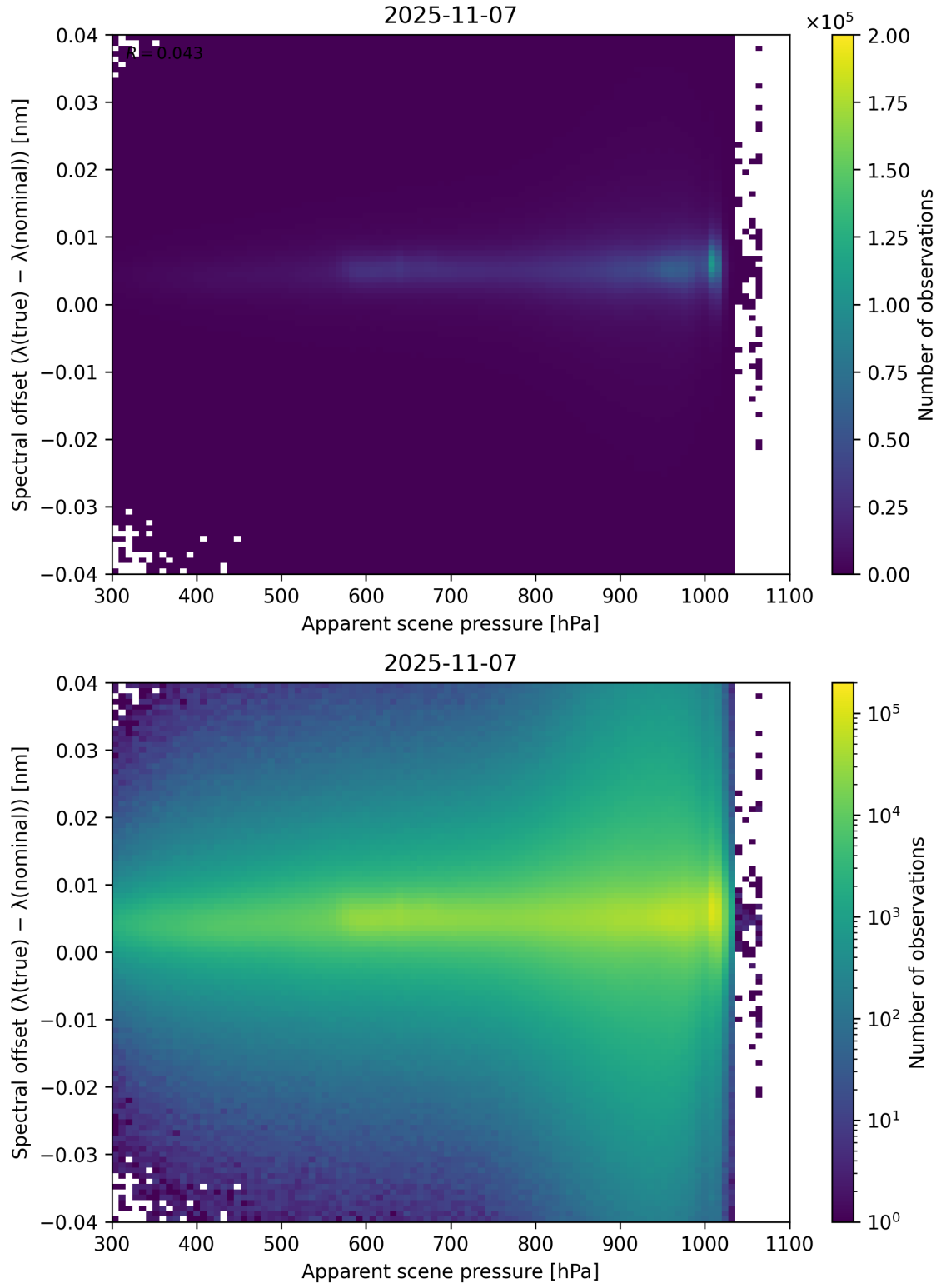
Figure 67: Scatter density plot of “Apparent scene pressure” against “Spectral offset ( \lambda_{\text{true}} - \lambda_{\text{nominal}} )” for 2025-11-07 to 2025-11-08.
