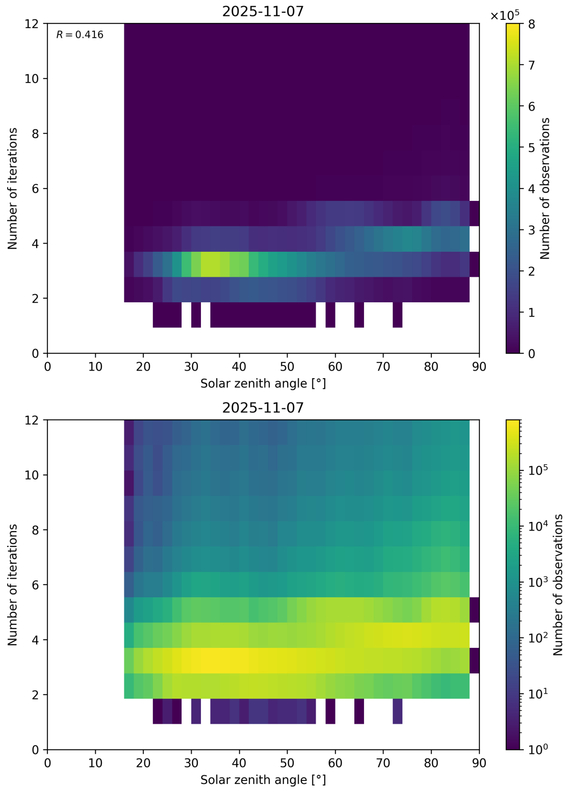
Figure 114: Scatter density plot of “Solar zenith angle” against “Number of iterations” for 2025-11-07 to 2025-11-08.
