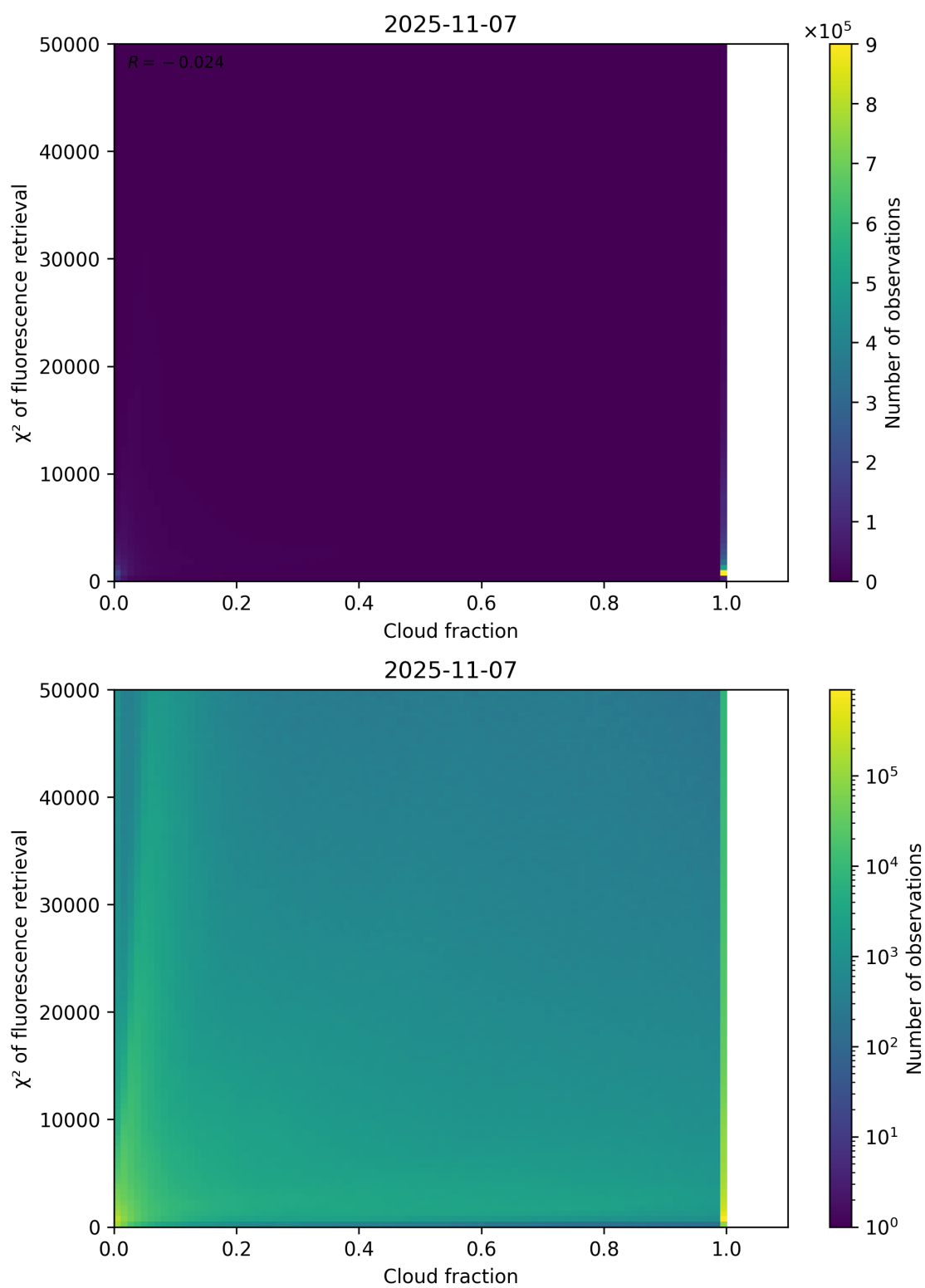
Figure 71: Scatter density plot of “Cloud fraction” against “ \chi^2 of fluorescence retrieval” for 2025-11-07 to 2025-11-08.
