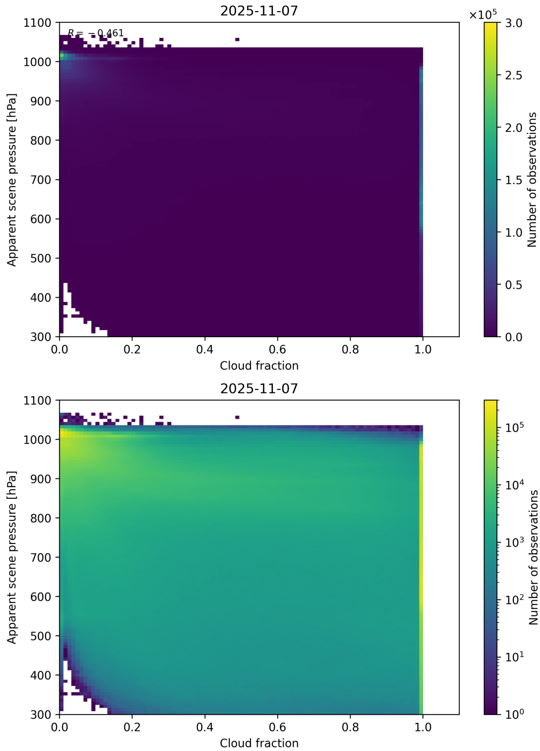
Figure 70: Scatter density plot of “Cloud fraction” against “Apparent scene pressure” for 2025-11-07 to 2025-11-08.
