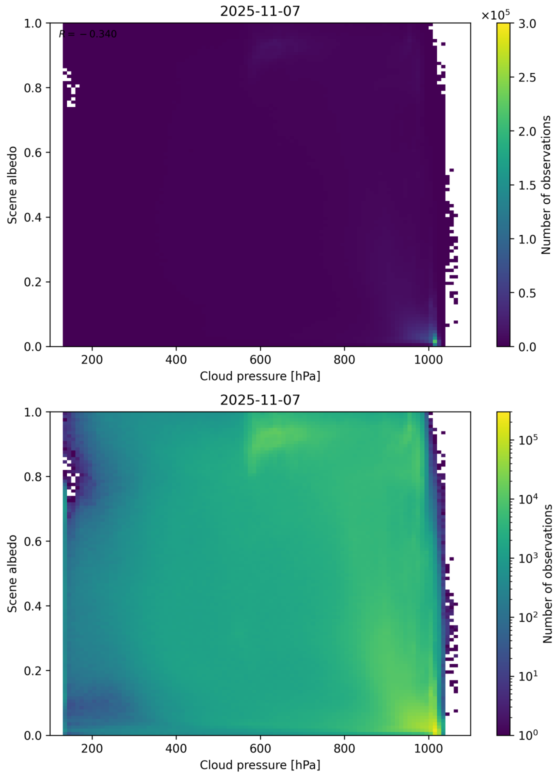
Figure 83: Scatter density plot of “Cloud pressure” against “Scene albedo” for 2025-11-07 to 2025-11-08.
