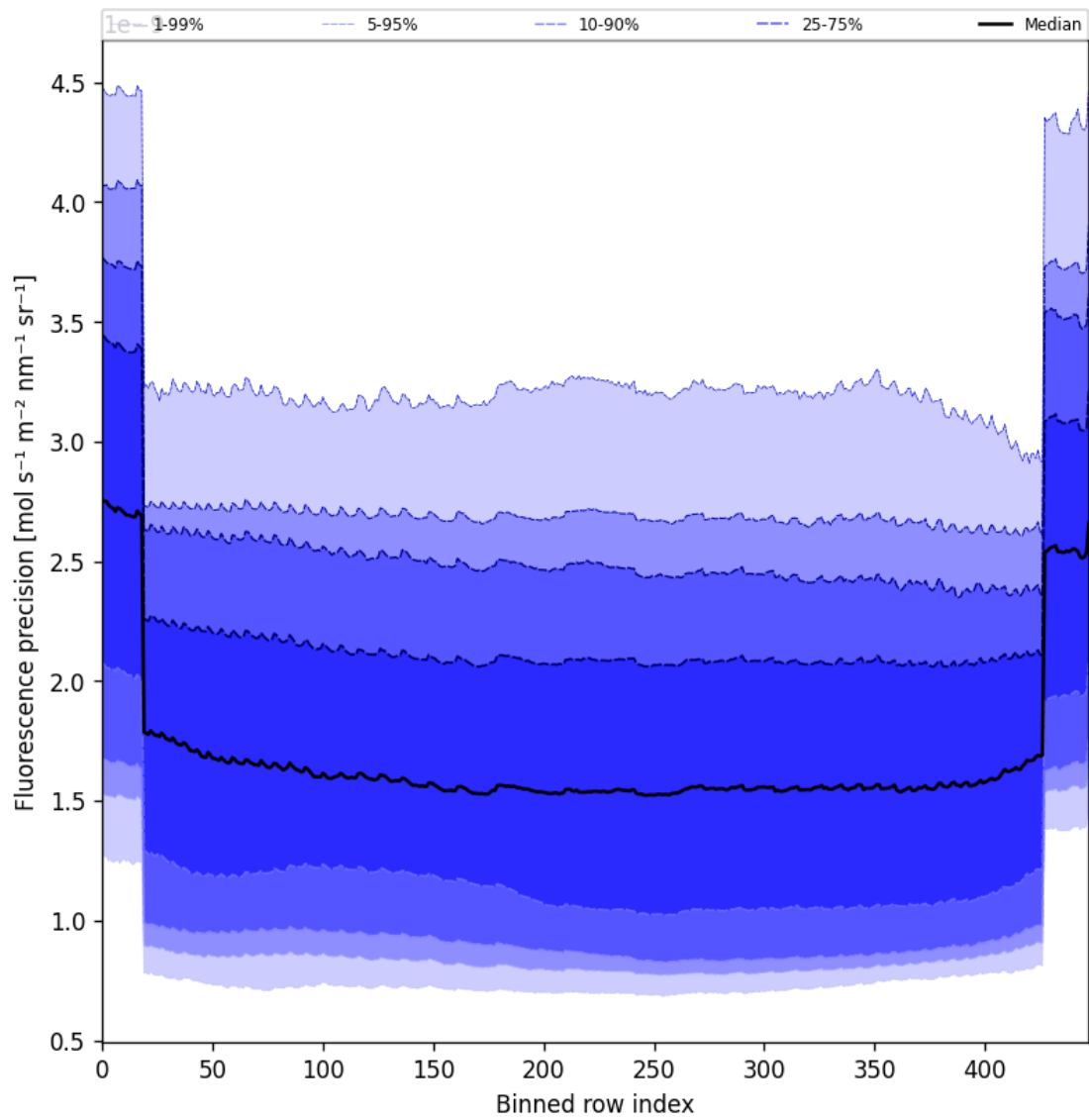
Figure 58: Along track statistics of “Fluorescence precision” for 2025-11-07 to 2025-11-08
