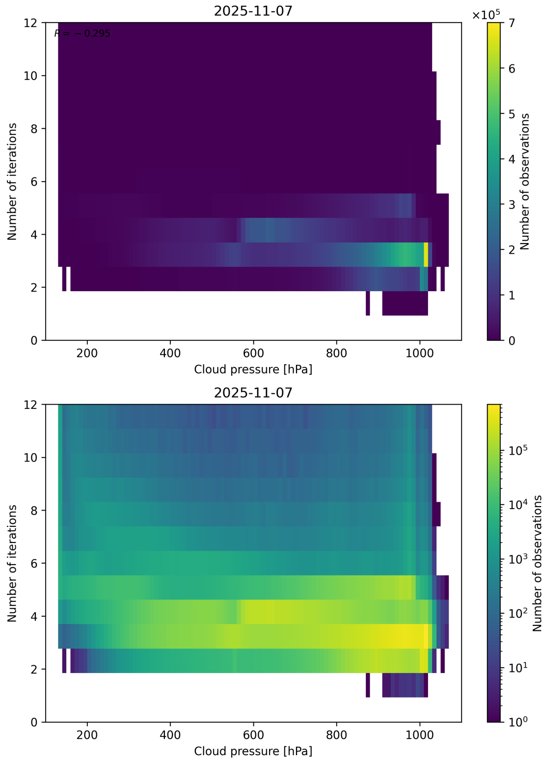
Figure 81: Scatter density plot of “Cloud pressure” against “Number of iterations” for 2025-11-07 to 2025-11-08.
