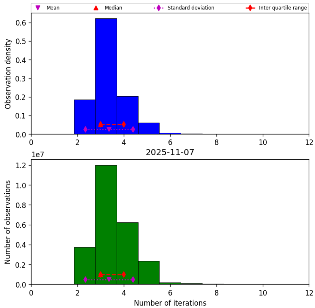
Figure 39: Histogram of “Number of iterations” for 2025-11-07 to 2025-11-08
