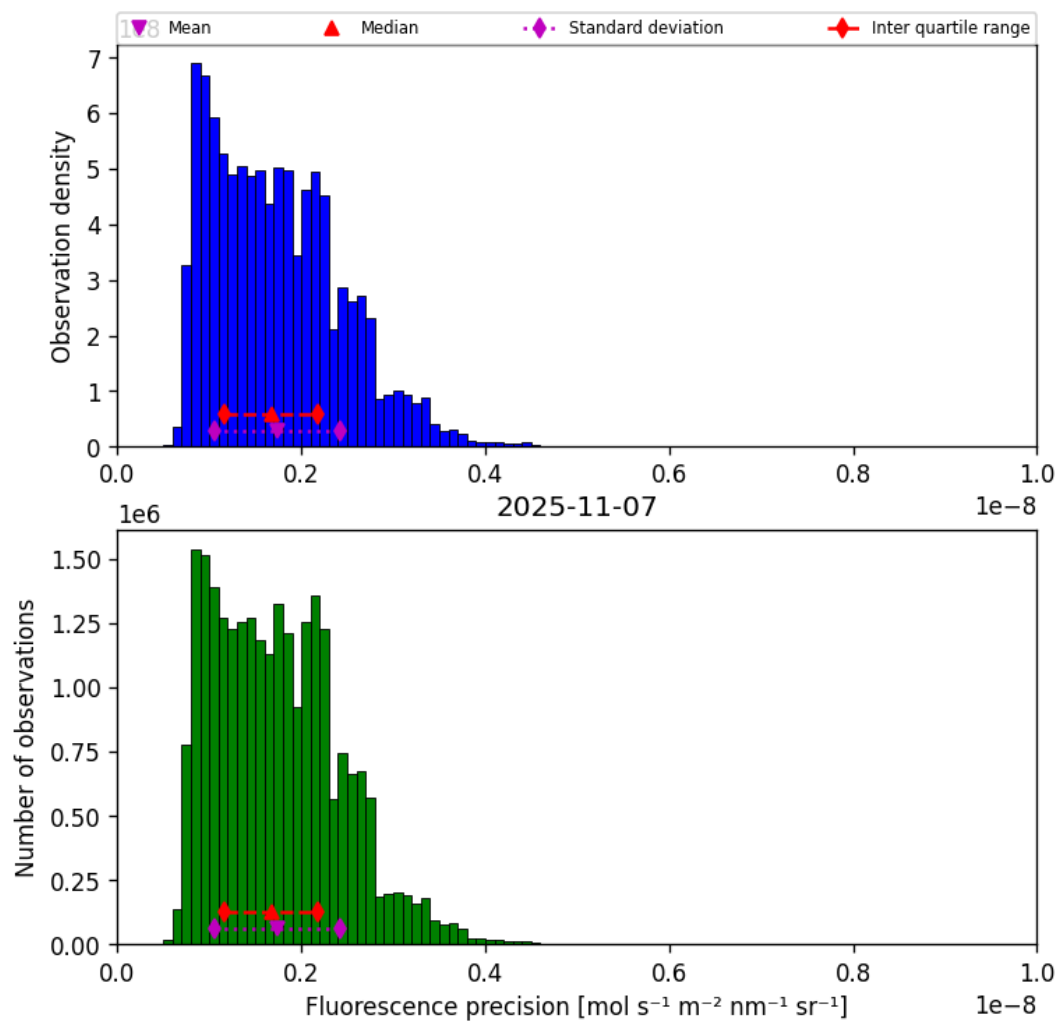
Figure 41: Histogram of “Fluorescence precision” for 2025-11-07 to 2025-11-08
