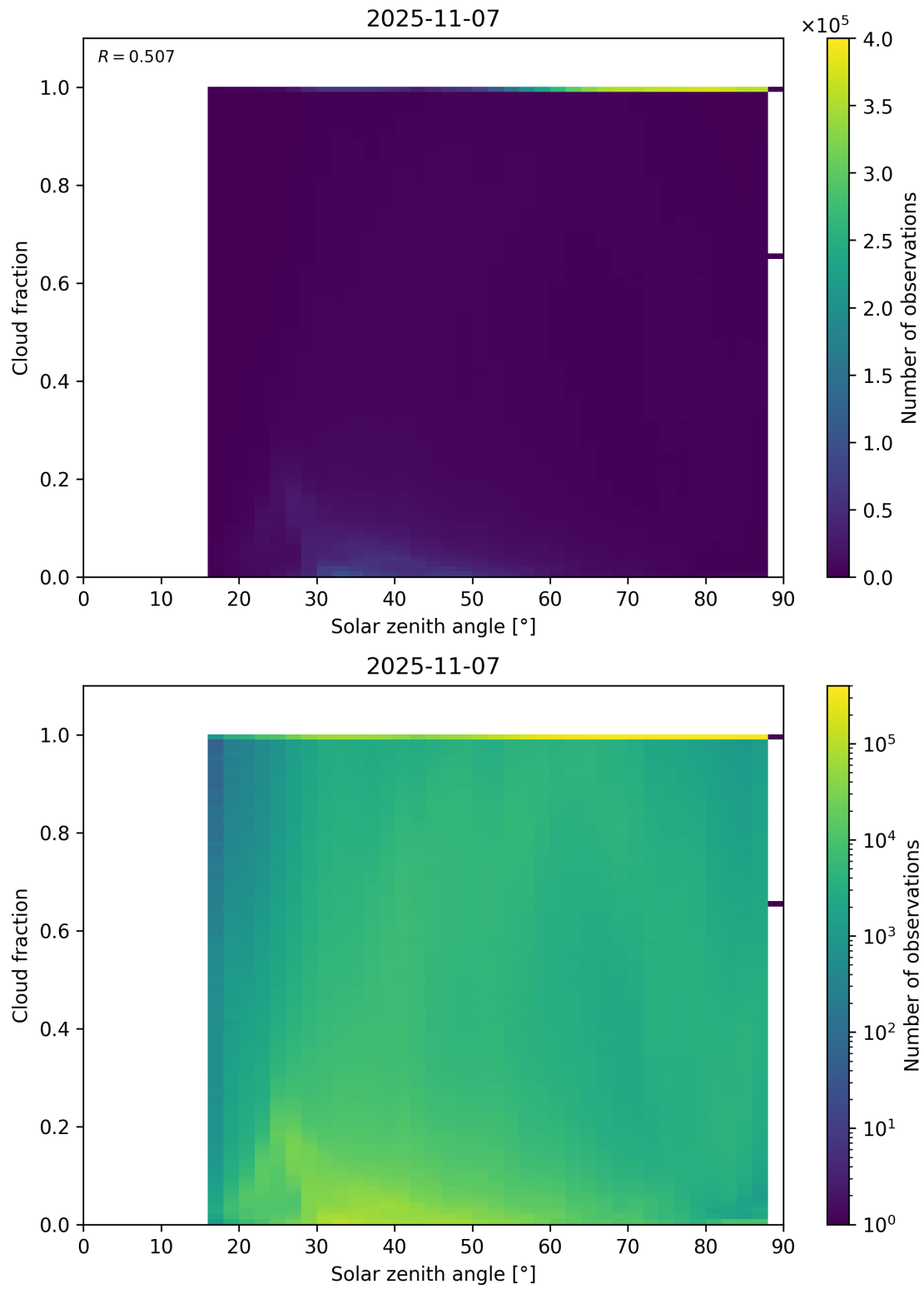
Figure 110: Scatter density plot of “Solar zenith angle” against “Cloud fraction” for 2025-11-07 to 2025-11-08.
