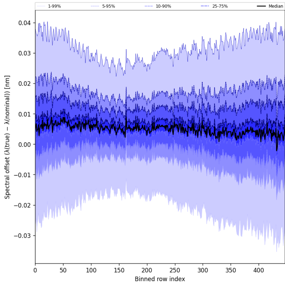
Figure 62: Along track statistics of “Spectral offset ( \lambda_{\text{true}} - \lambda_{\text{nominal}} )” for 2025-11-07 to 2025-11-08
