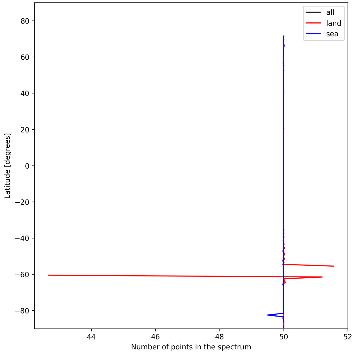
Figure 27: Zonal average of “Number of points in the spectrum” for 2025-11-07 to 2025-11-08.
