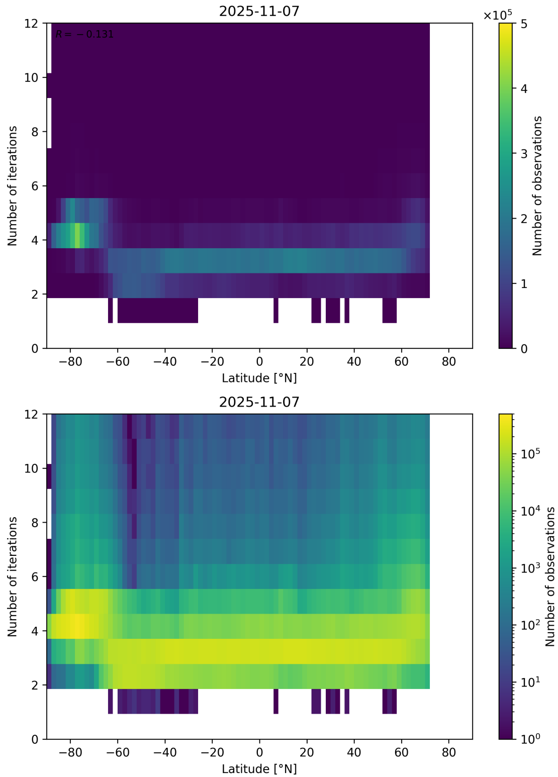
Figure 93: Scatter density plot of “Latitude” against “Number of iterations” for 2025-11-07 to 2025-11-08.
