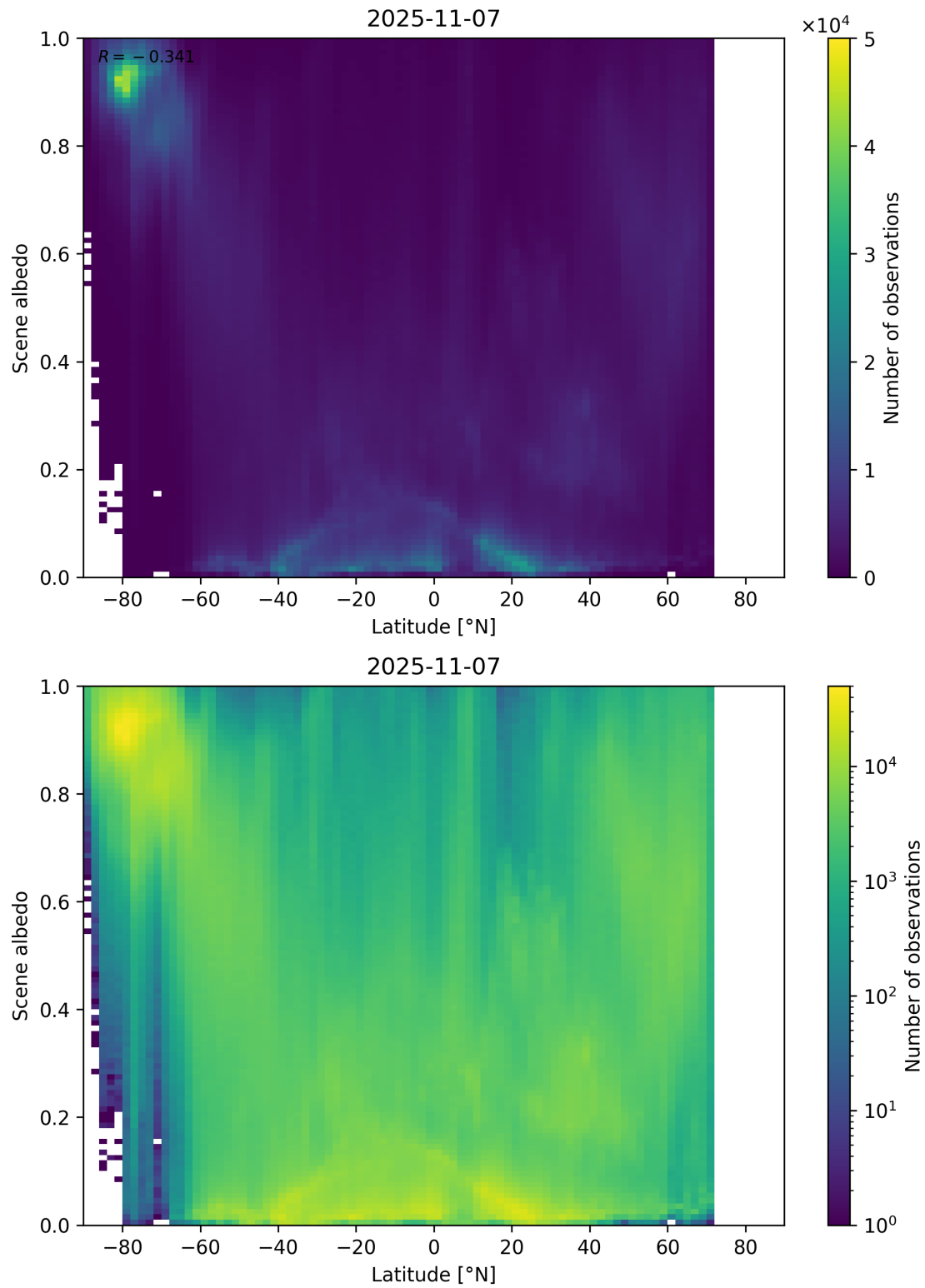
Figure 95: Scatter density plot of “Latitude” against “Scene albedo” for 2025-11-07 to 2025-11-08.
