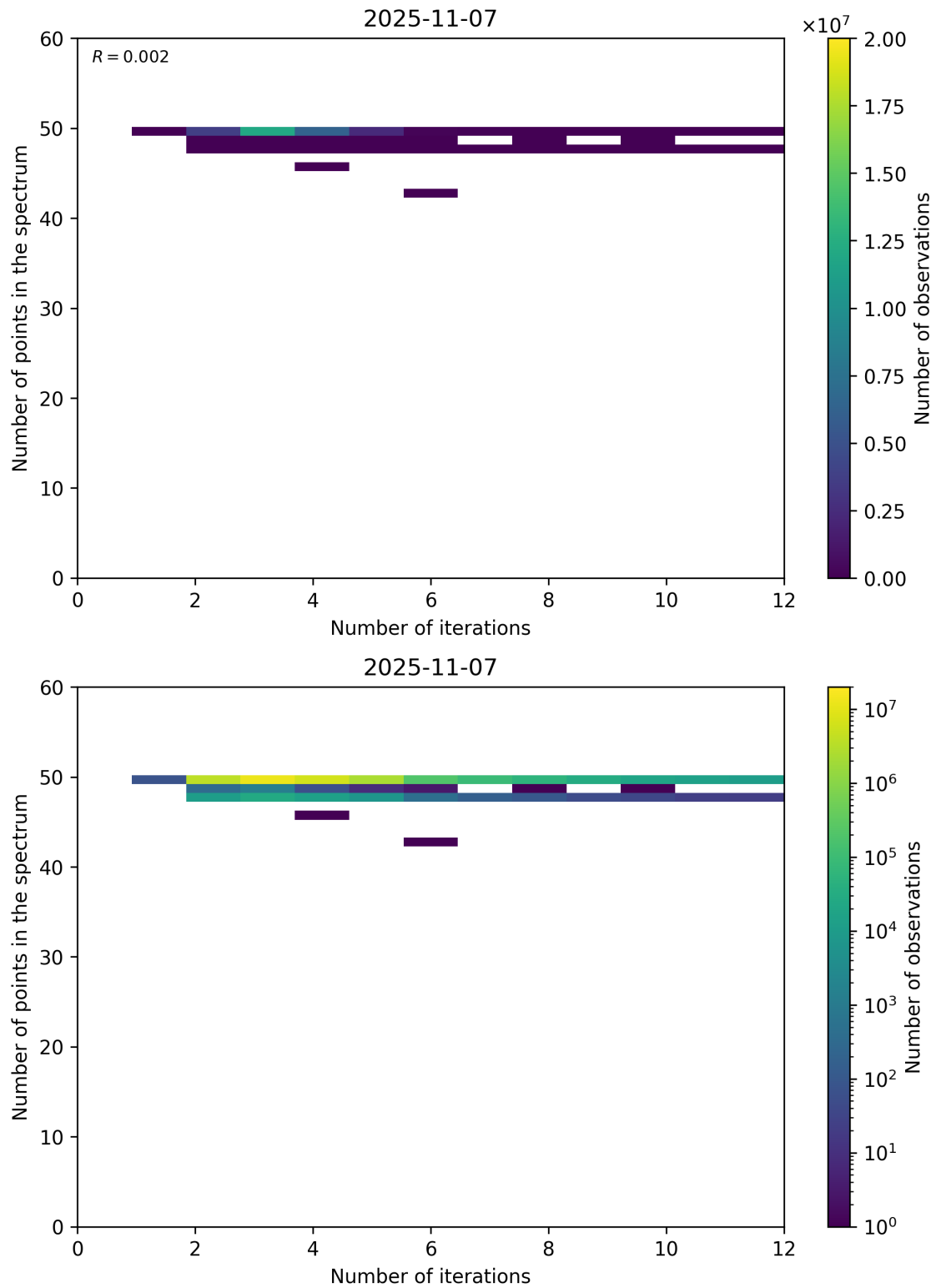
Figure 99: Scatter density plot of “Number of iterations” against “Number of points in the spectrum” for 2025-11-07 to 2025-11-08.
