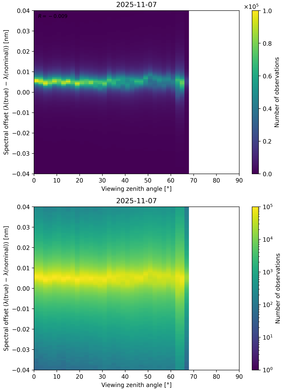
Figure 128: Scatter density plot of “Viewing zenith angle” against “Spectral offset ( \lambda_{\text{true}} - \lambda_{\text{nominal}} )” for 2025-11-07 to 2025-11-08.
