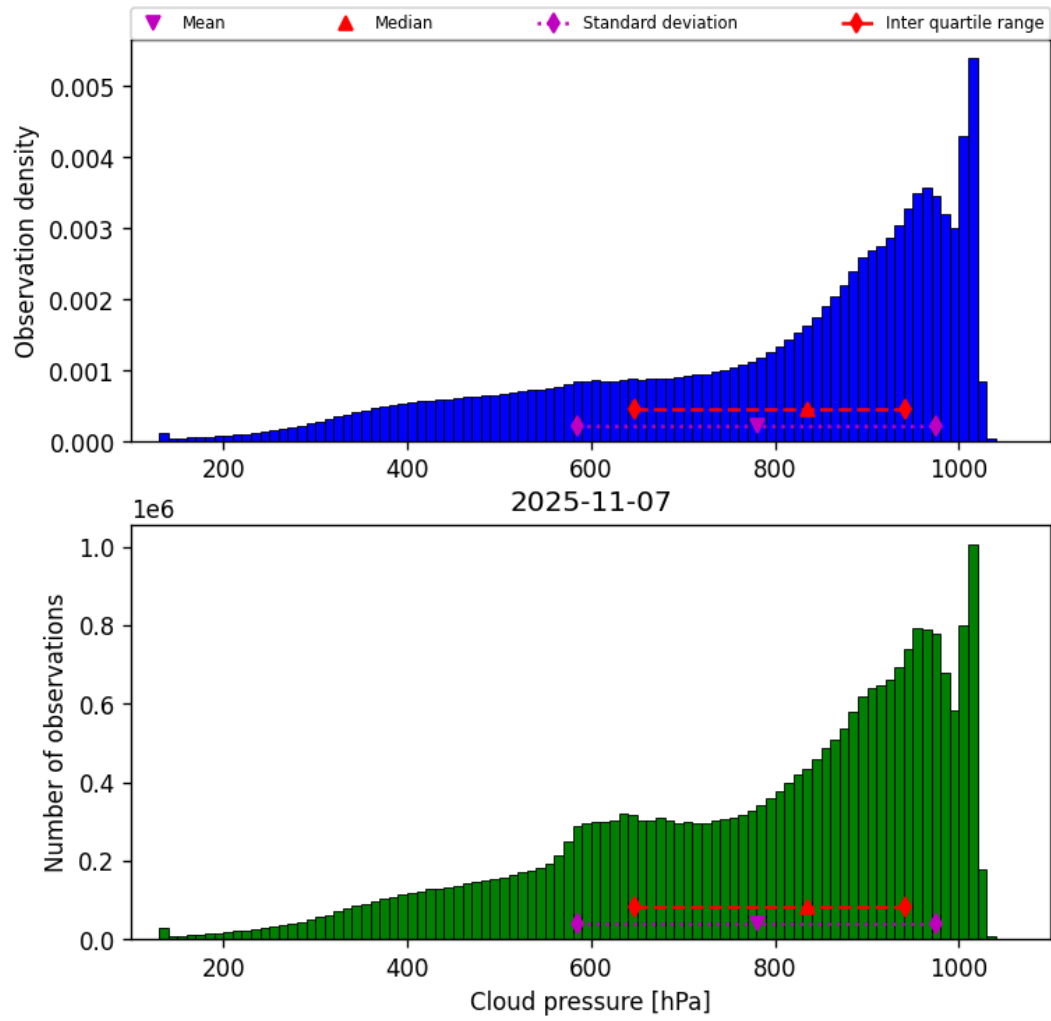
Figure 30: Histogram of “Cloud pressure” for 2025-11-07 to 2025-11-08
