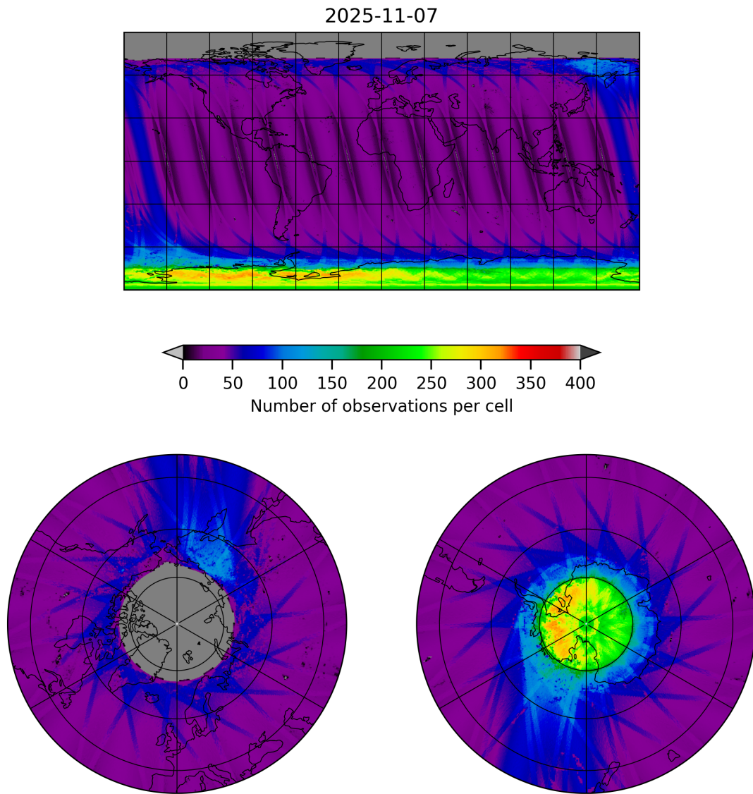
Figure 11: Map of the number of observations for 2025-11-07 to 2025-11-08
