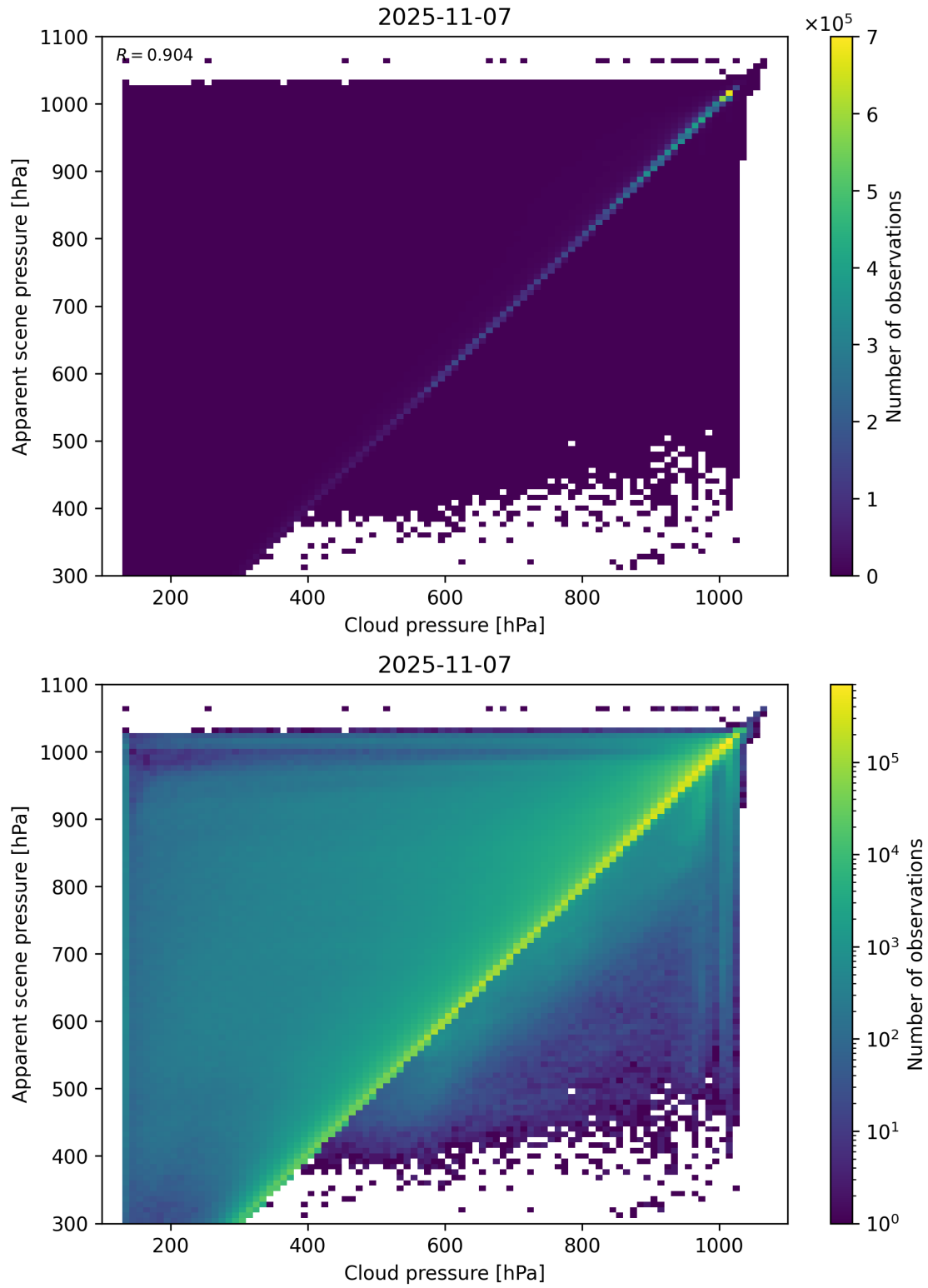
Figure 77: Scatter density plot of “Cloud pressure” against “Apparent scene pressure” for 2025-11-07 to 2025-11-08.
