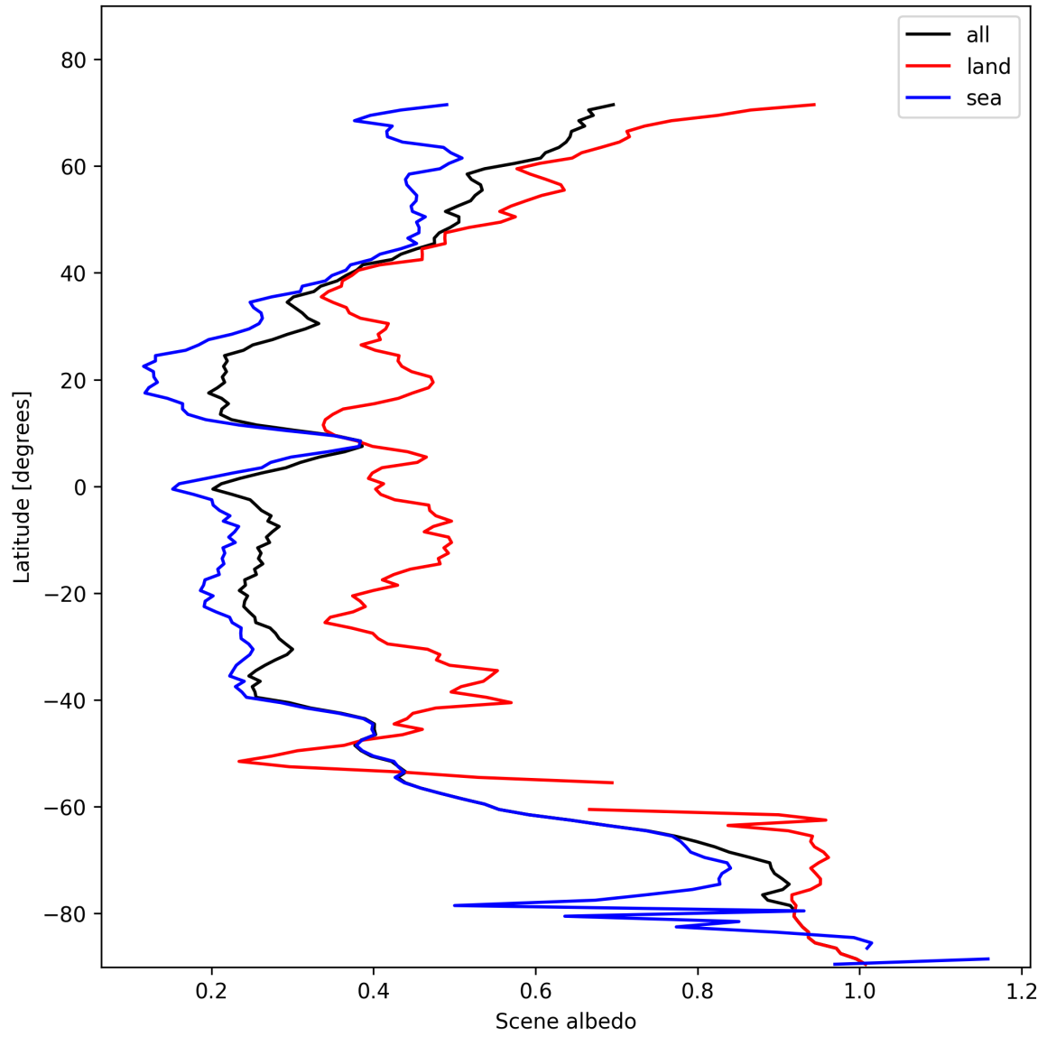
Figure 17: Zonal average of “Scene albedo” for 2025-11-07 to 2025-11-08.
