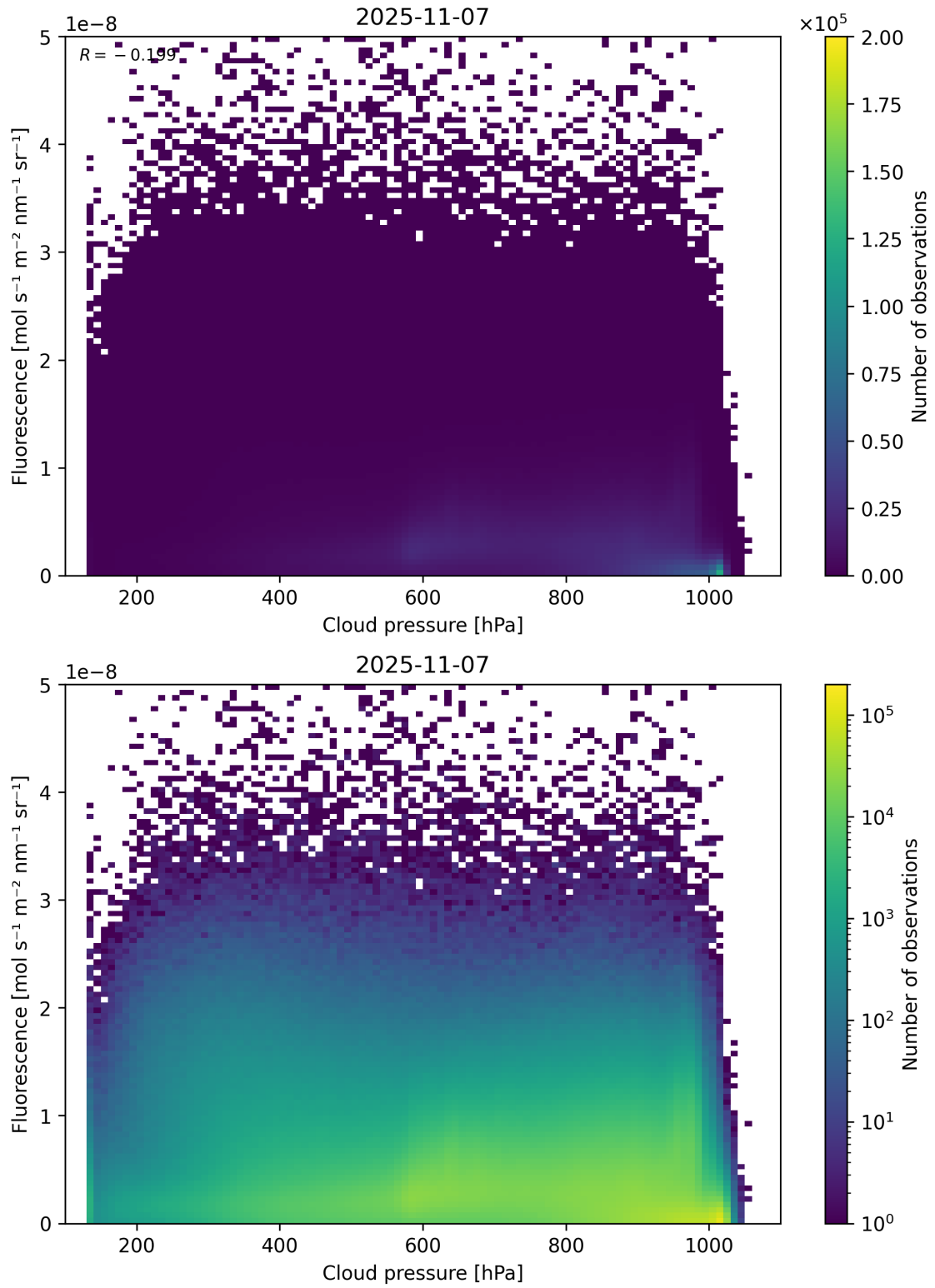
Figure 80: Scatter density plot of “Cloud pressure” against “Fluorescence” for 2025-11-07 to 2025-11-08.
