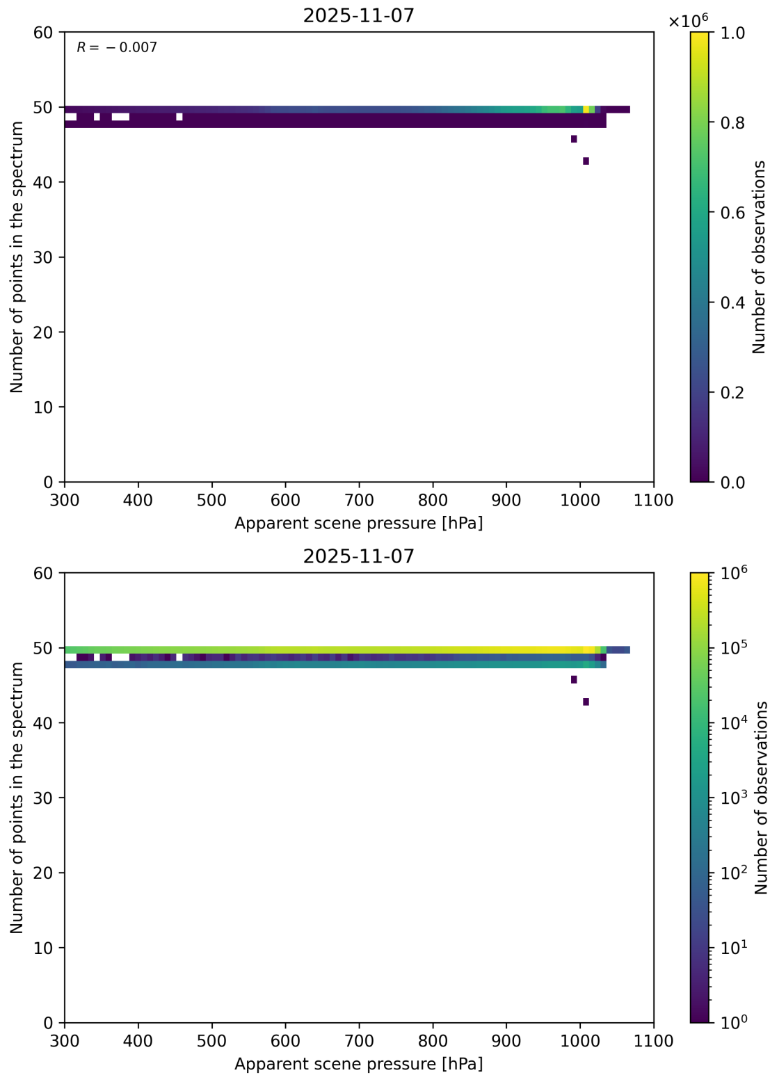
Figure 66: Scatter density plot of “Apparent scene pressure” against “Number of points in the spectrum” for 2025-11-07 to 2025-11-08.
