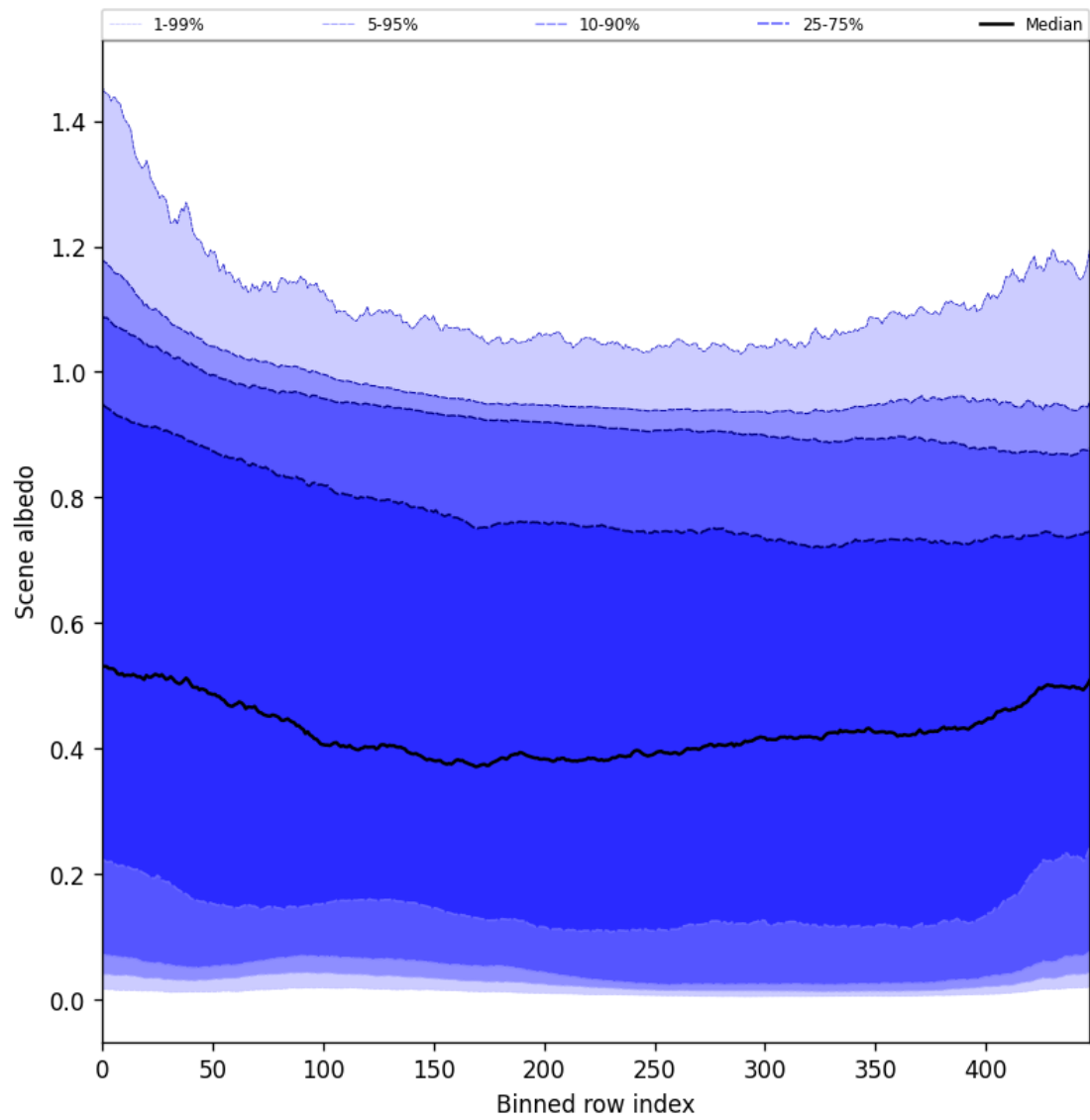
Figure 51: Along track statistics of “Scene albedo” for 2025-11-07 to 2025-11-08
