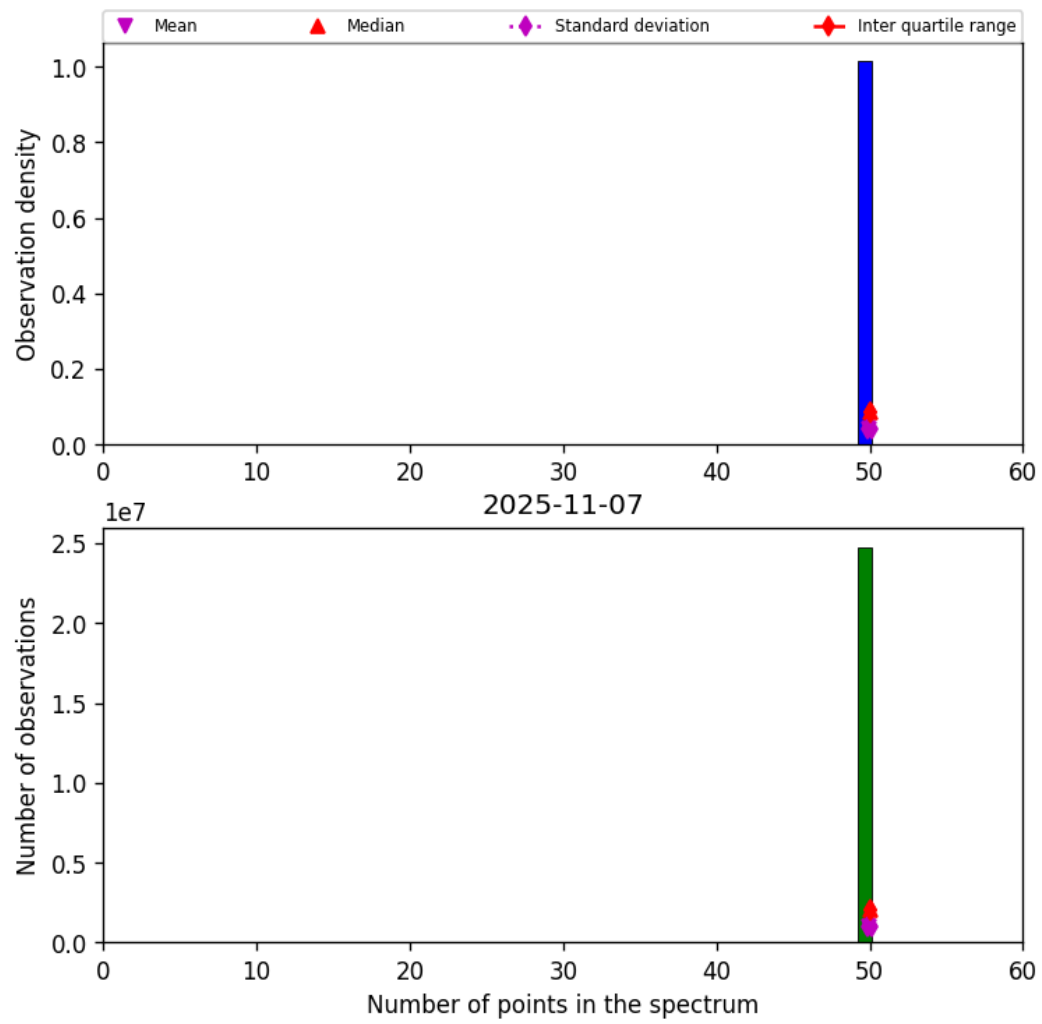
Figure 44: Histogram of “Number of points in the spectrum” for 2025-11-07 to 2025-11-08
