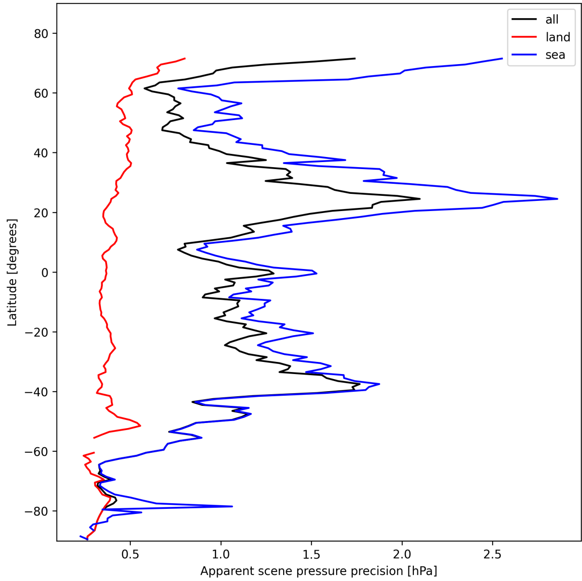
Figure 20: Zonal average of “Apparent scene pressure precision” for 2025-11-07 to 2025-11-08.
