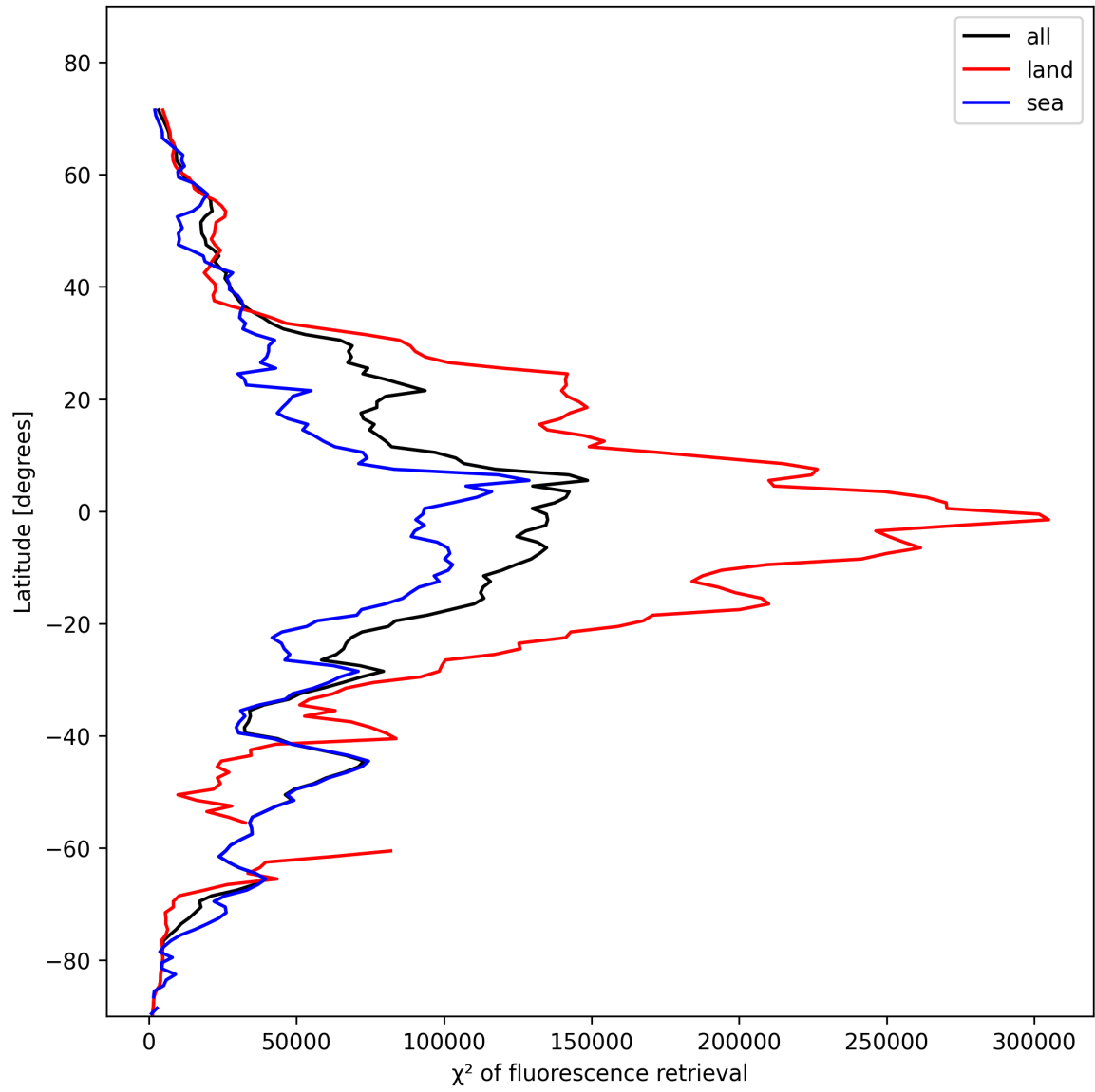
Figure 25: Zonal average of “ \chi^2 of fluorescence retrieval” for 2025-11-07 to 2025-11-08.
