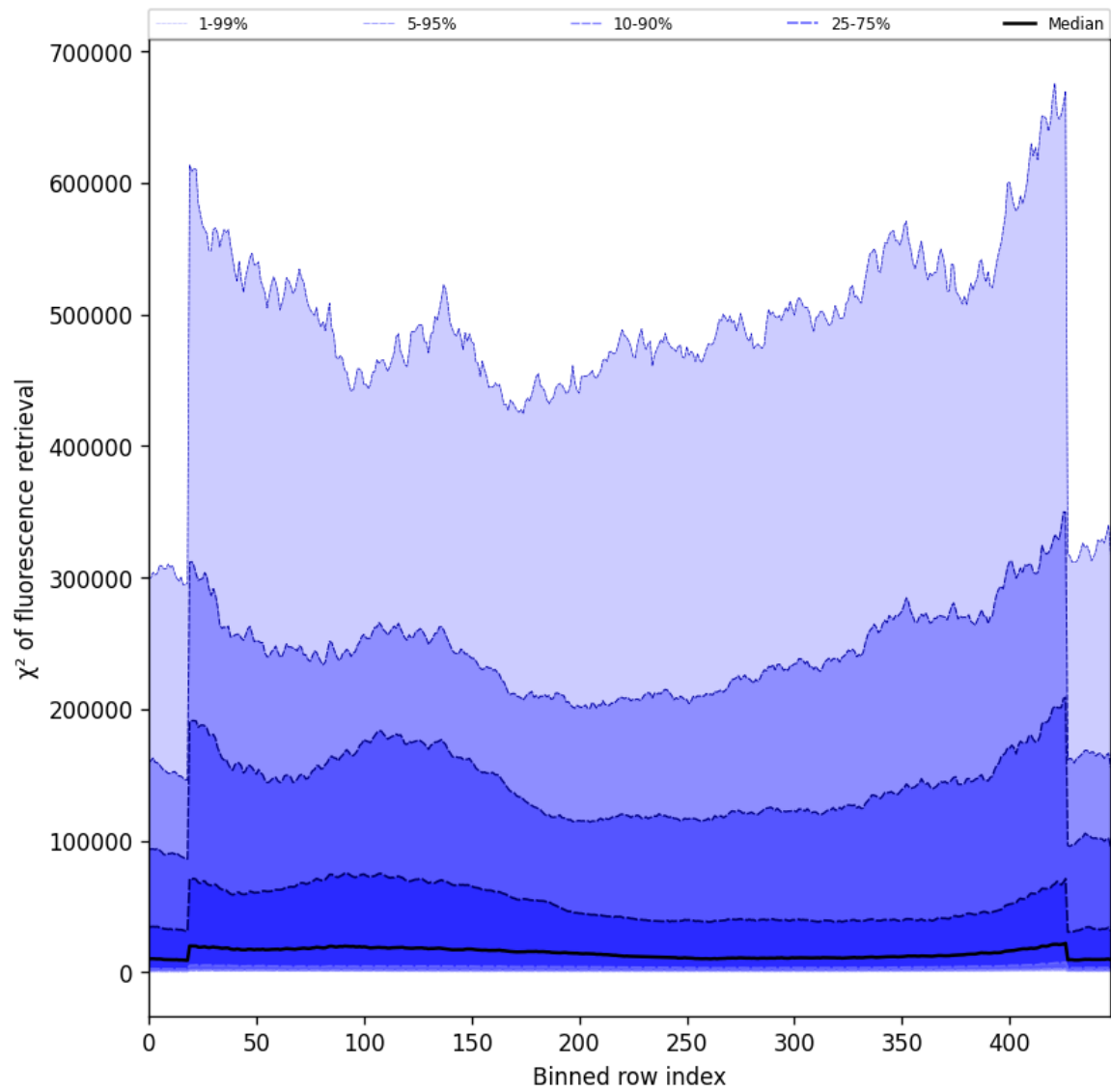
Figure 59: Along track statistics of “ \chi^2 of fluorescence retrieval” for 2025-11-07 to 2025-11-08
