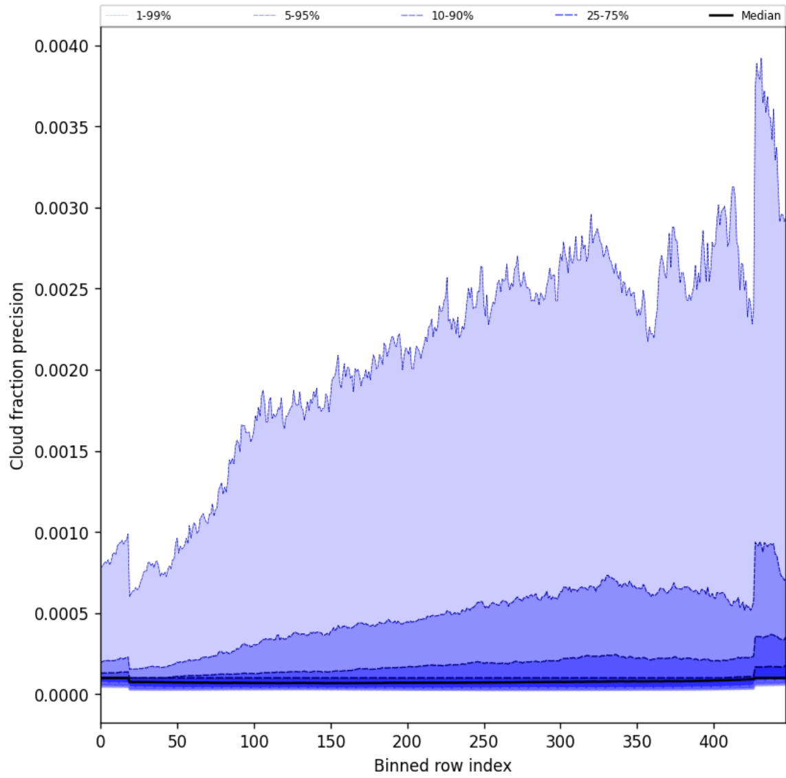
Figure 50: Along track statistics of “Cloud fraction precision” for 2025-11-07 to 2025-11-08
