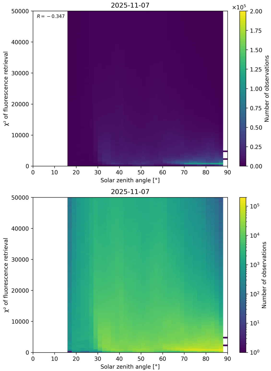
Figure 109: Scatter density plot of “Solar zenith angle” against “ \chi^2 of fluorescence retrieval” for 2025-11-07 to 2025-11-08.
