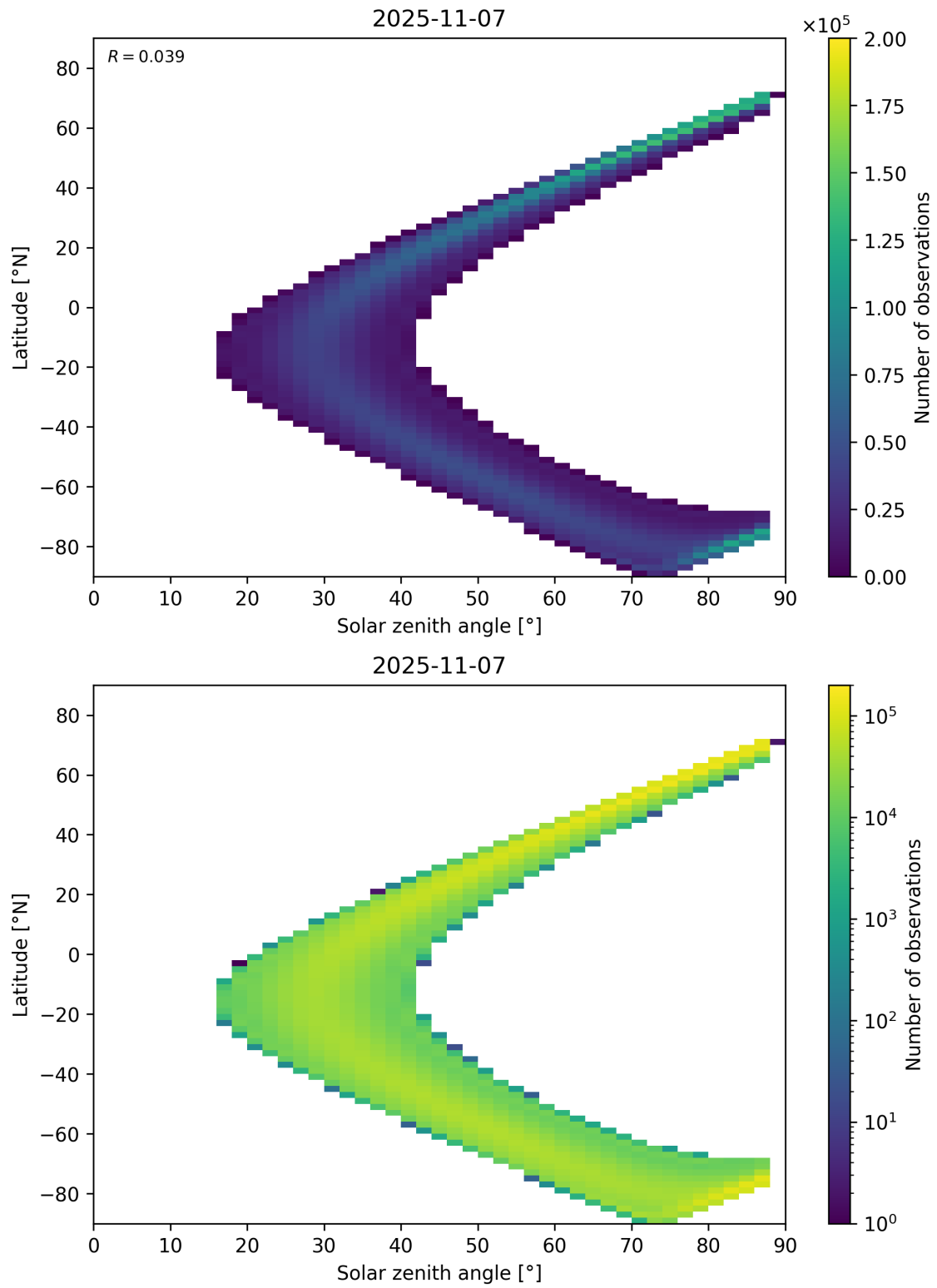
Figure 113: Scatter density plot of “Solar zenith angle” against “Latitude” for 2025-11-07 to 2025-11-08.
