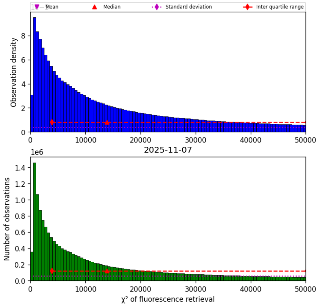
Figure 42: Histogram of “ \chi^2 of fluorescence retrieval” for 2025-11-07 to 2025-11-08
