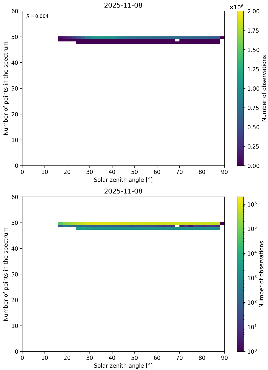
Figure 115: Scatter density plot of “Solar zenith angle” against “Number of points in the spectrum” for 2025-11-07 to 2025-11-09.
