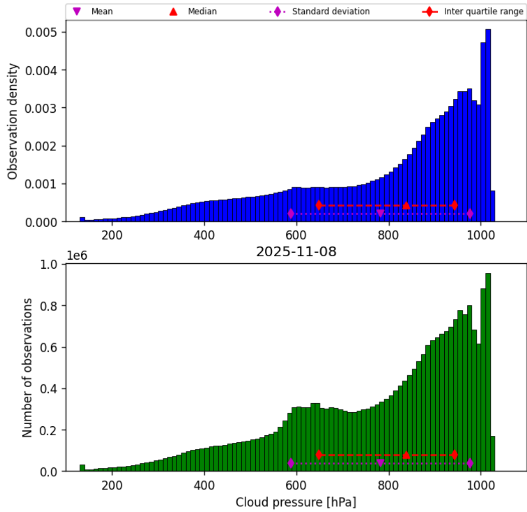
Figure 30: Histogram of “Cloud pressure” for 2025-11-07 to 2025-11-09
