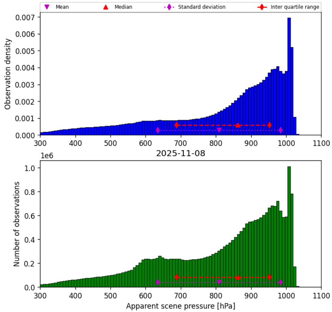
Figure 36: Histogram of “Apparent scene pressure” for 2025-11-07 to 2025-11-09
