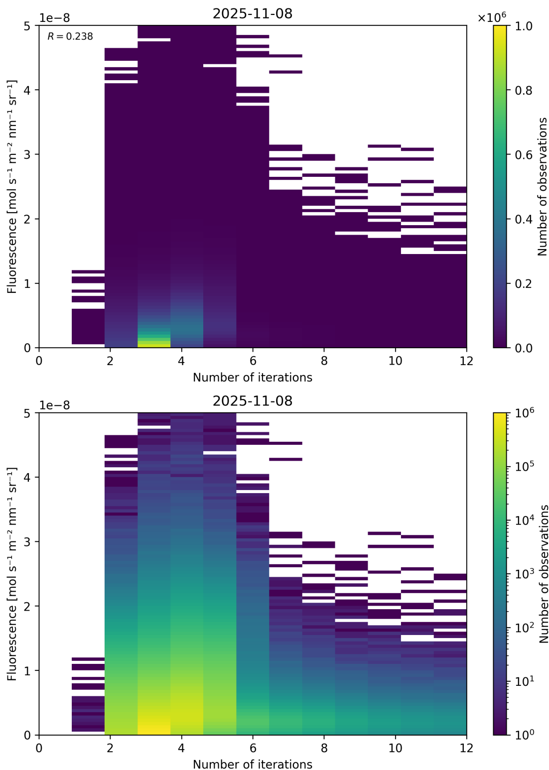
Figure 98: Scatter density plot of “Number of iterations” against “Fluorescence” for 2025-11-07 to 2025-11-09.
