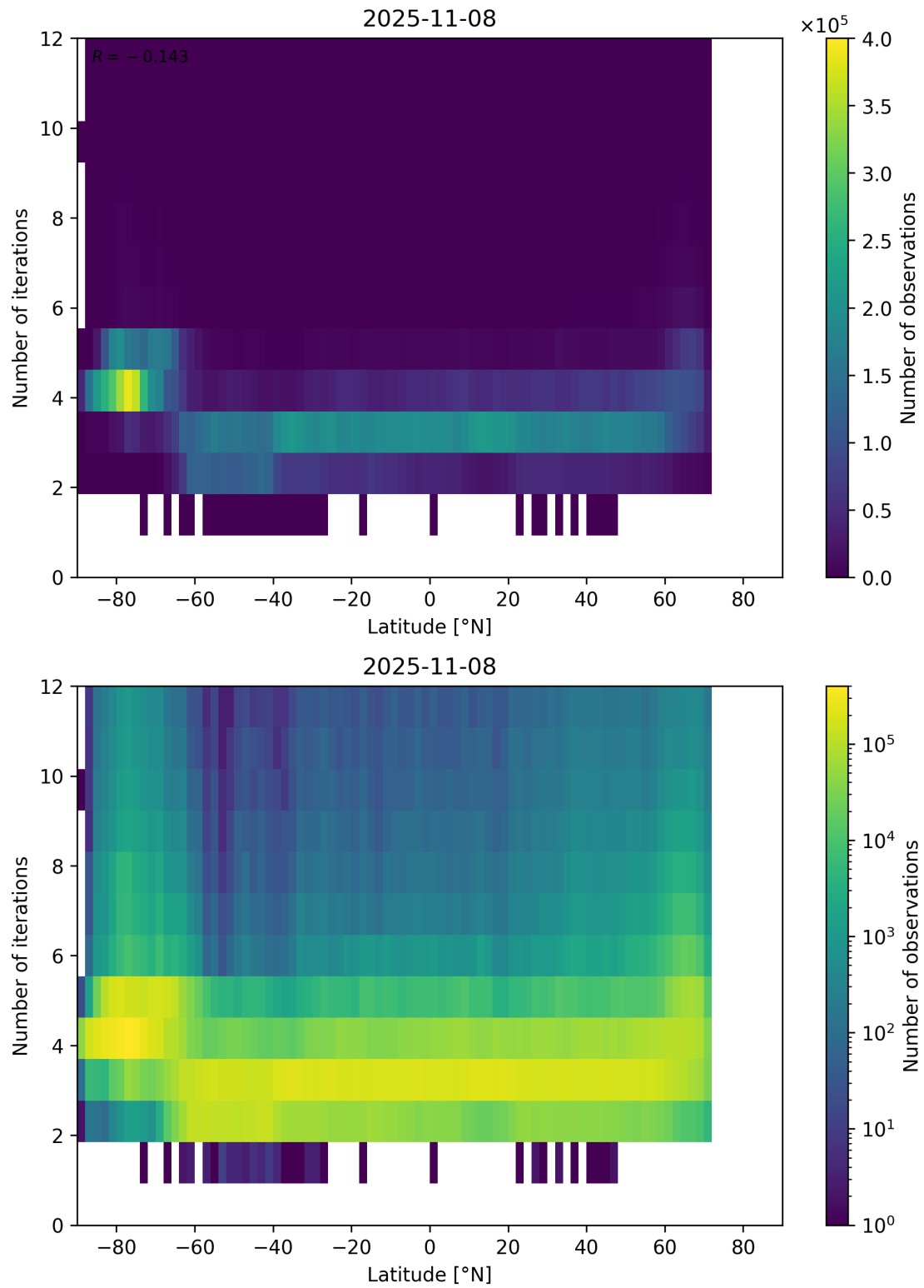
Figure 93: Scatter density plot of “Latitude” against “Number of iterations” for 2025-11-07 to 2025-11-09.
