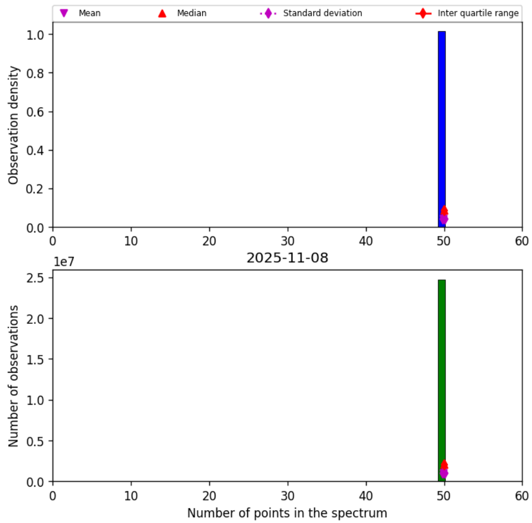
Figure 44: Histogram of “Number of points in the spectrum” for 2025-11-07 to 2025-11-09
