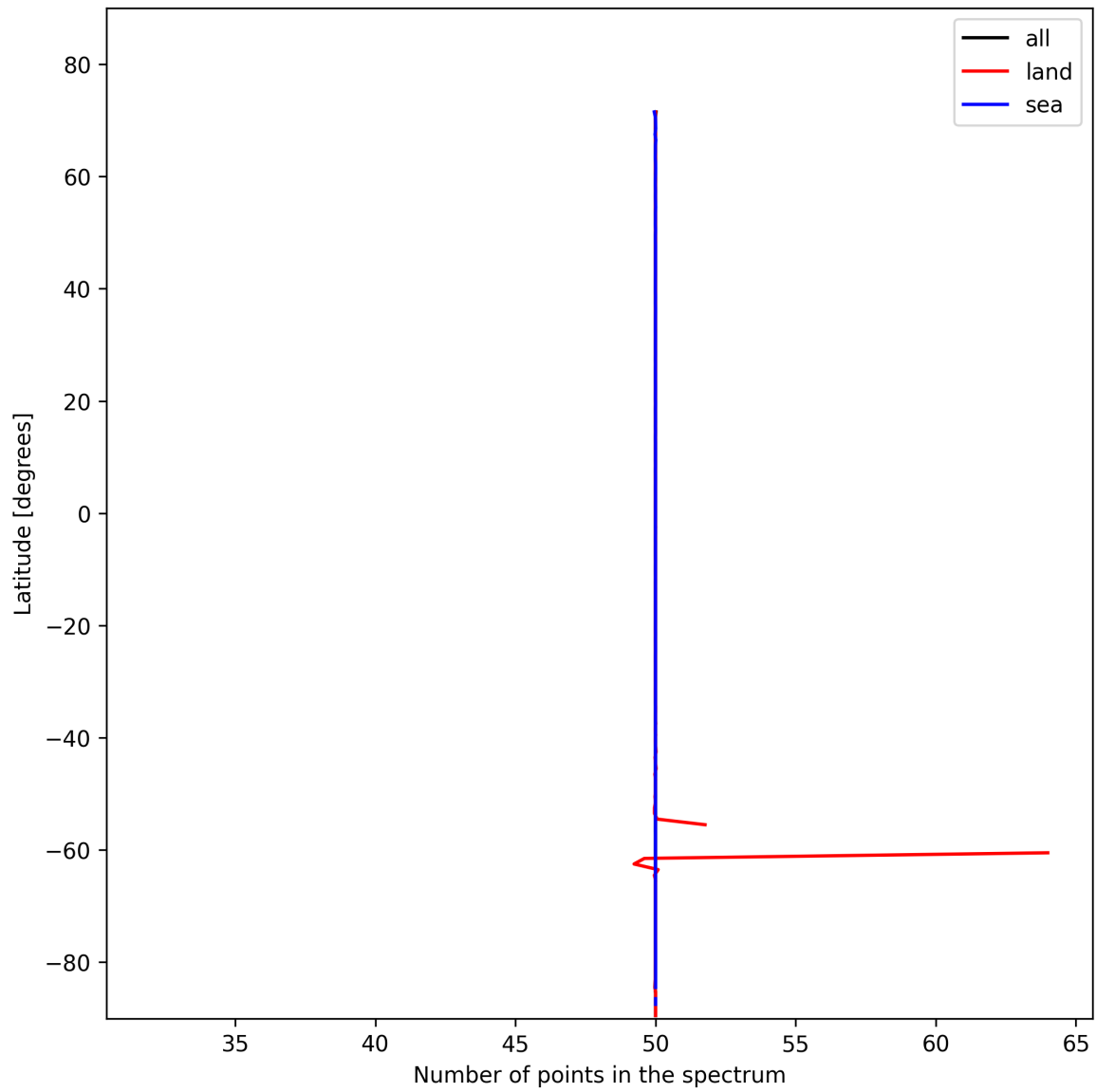
Figure 27: Zonal average of “Number of points in the spectrum” for 2025-11-07 to 2025-11-09.
