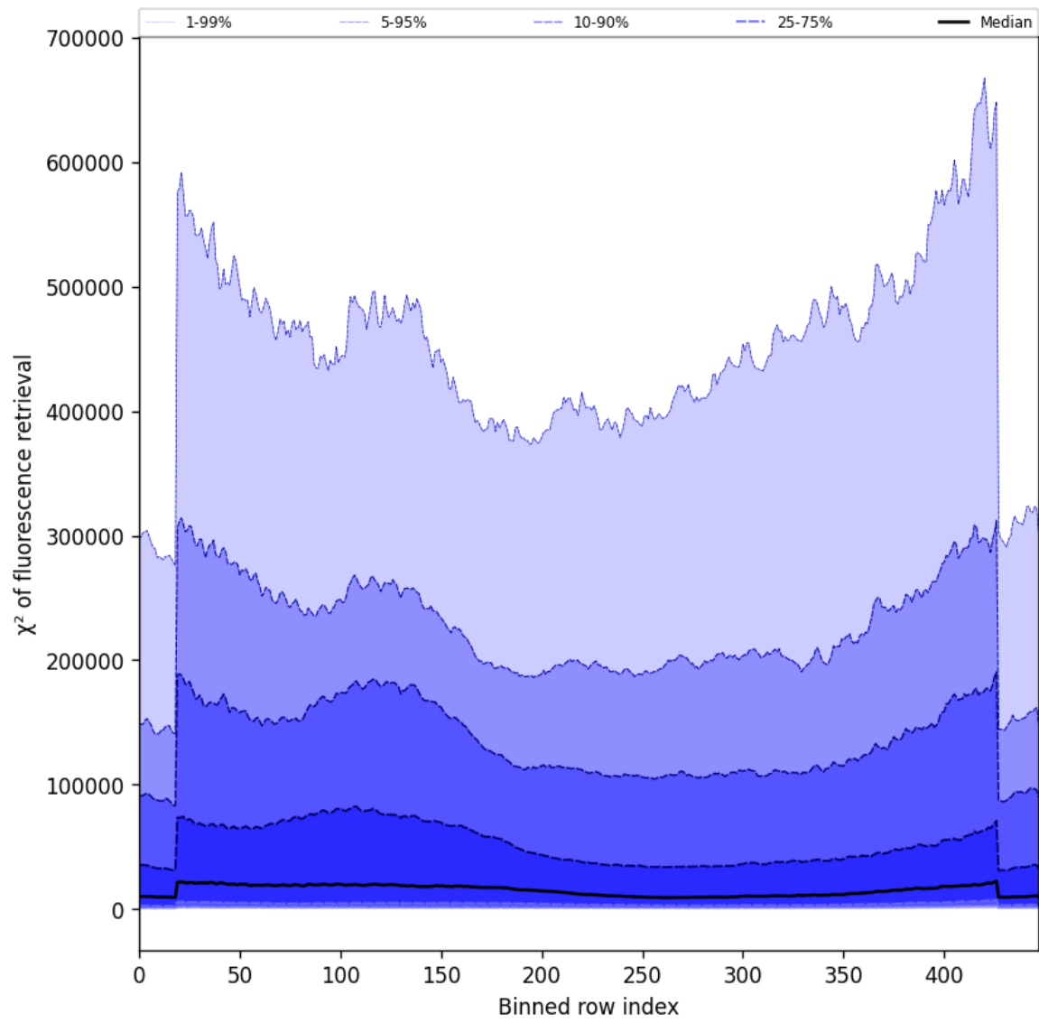
Figure 59: Along track statistics of “ \chi^2 of fluorescence retrieval” for 2025-11-07 to 2025-11-09
