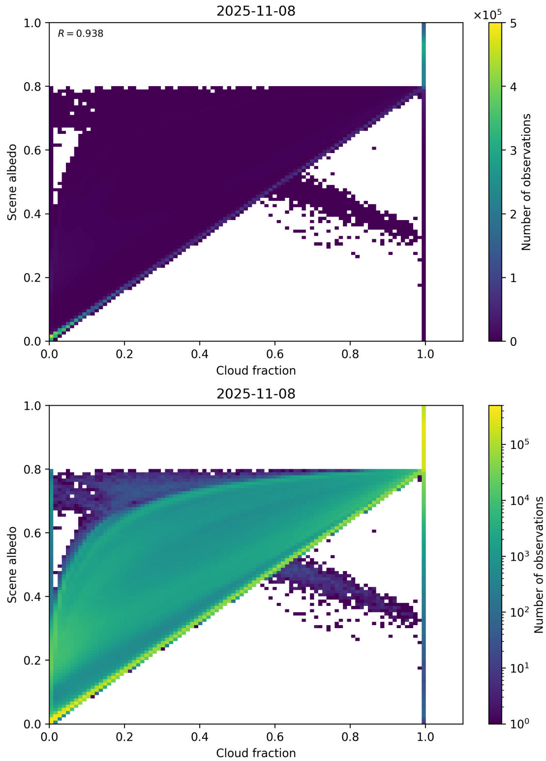
Figure 75: Scatter density plot of “Cloud fraction” against “Scene albedo” for 2025-11-07 to 2025-11-09.
