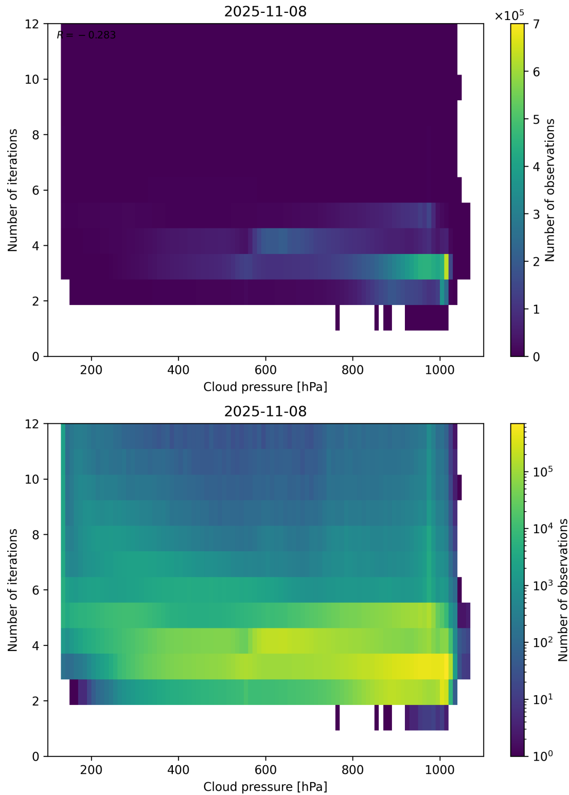
Figure 81: Scatter density plot of “Cloud pressure” against “Number of iterations” for 2025-11-07 to 2025-11-09.
