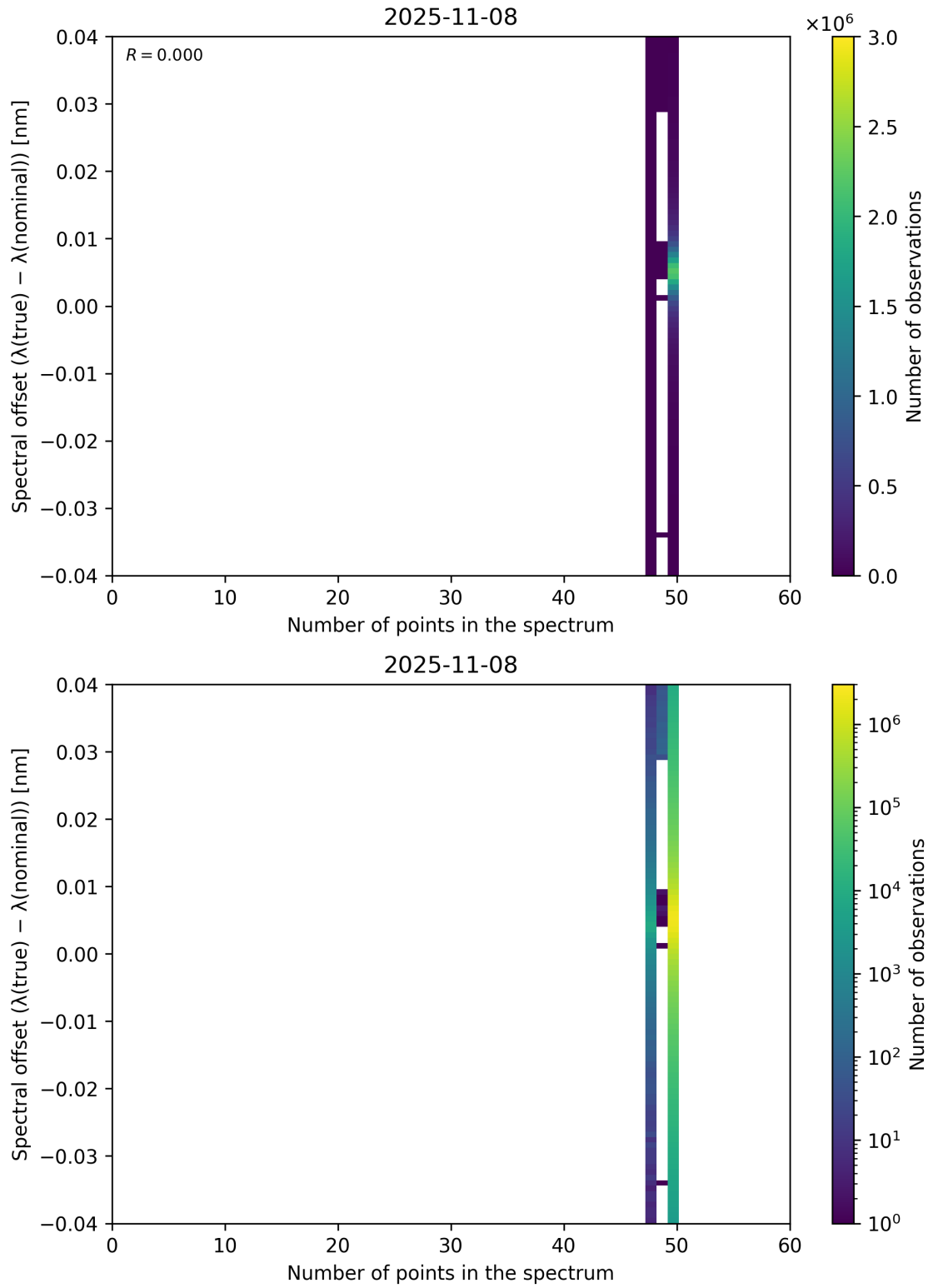
Figure 101: Scatter density plot of “Number of points in the spectrum” against “Spectral offset ( \lambda_{\text{true}} - \lambda_{\text{nominal}} )” for 2025-11-07 to 2025-11-09.
