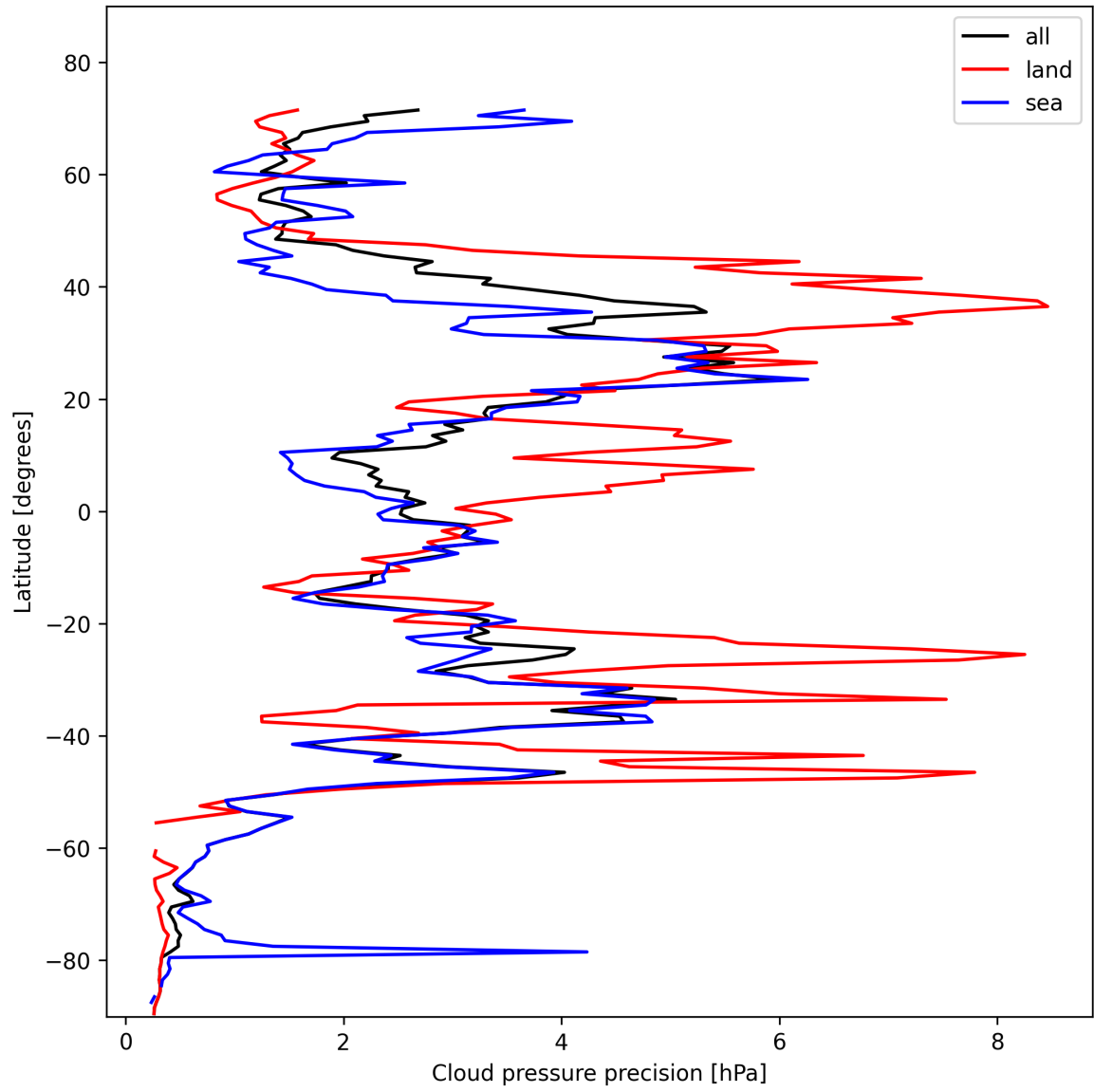
Figure 14: Zonal average of “Cloud pressure precision” for 2025-11-07 to 2025-11-09.
