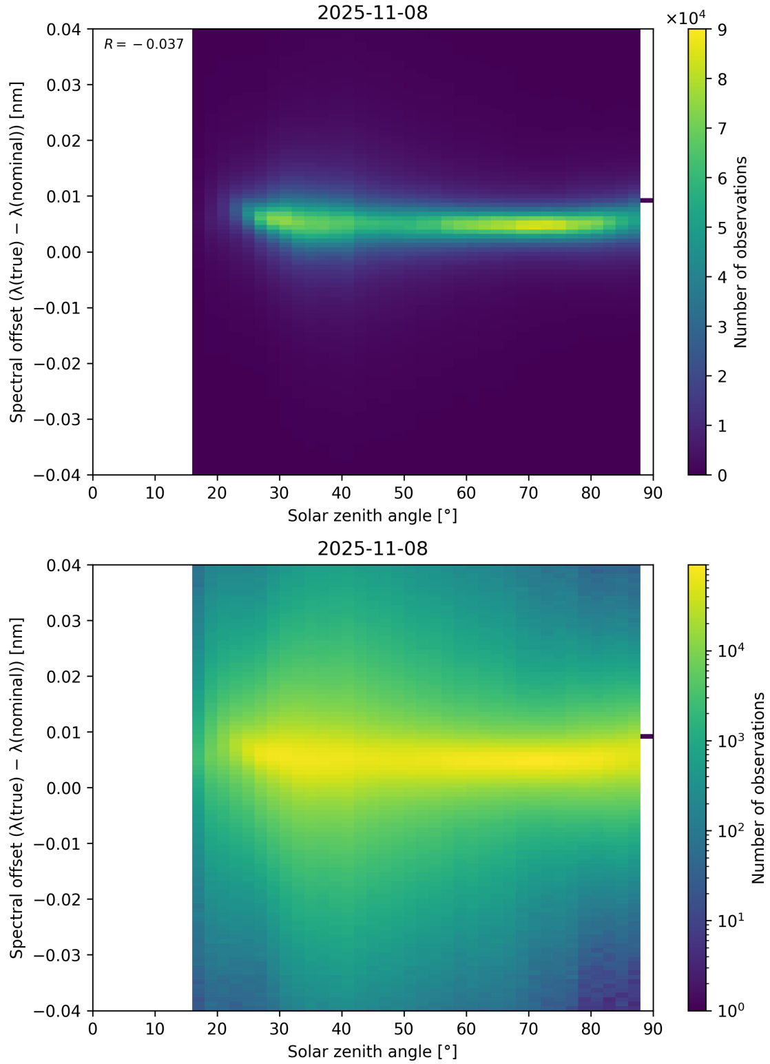
Figure 117: Scatter density plot of “Solar zenith angle” against “Spectral offset ( \lambda_{\text{true}} - \lambda_{\text{nominal}} )” for 2025-11-07 to 2025-11-09.
