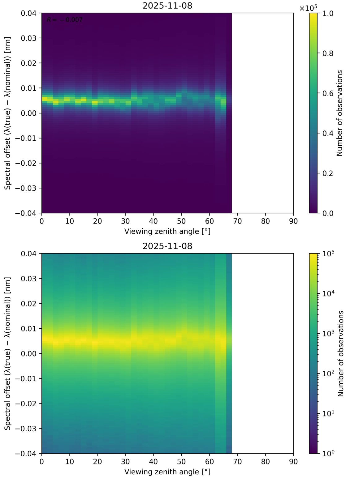
Figure 128: Scatter density plot of “Viewing zenith angle” against “Spectral offset ( \lambda_{\text{true}} - \lambda_{\text{nominal}} )” for 2025-11-07 to 2025-11-09.
