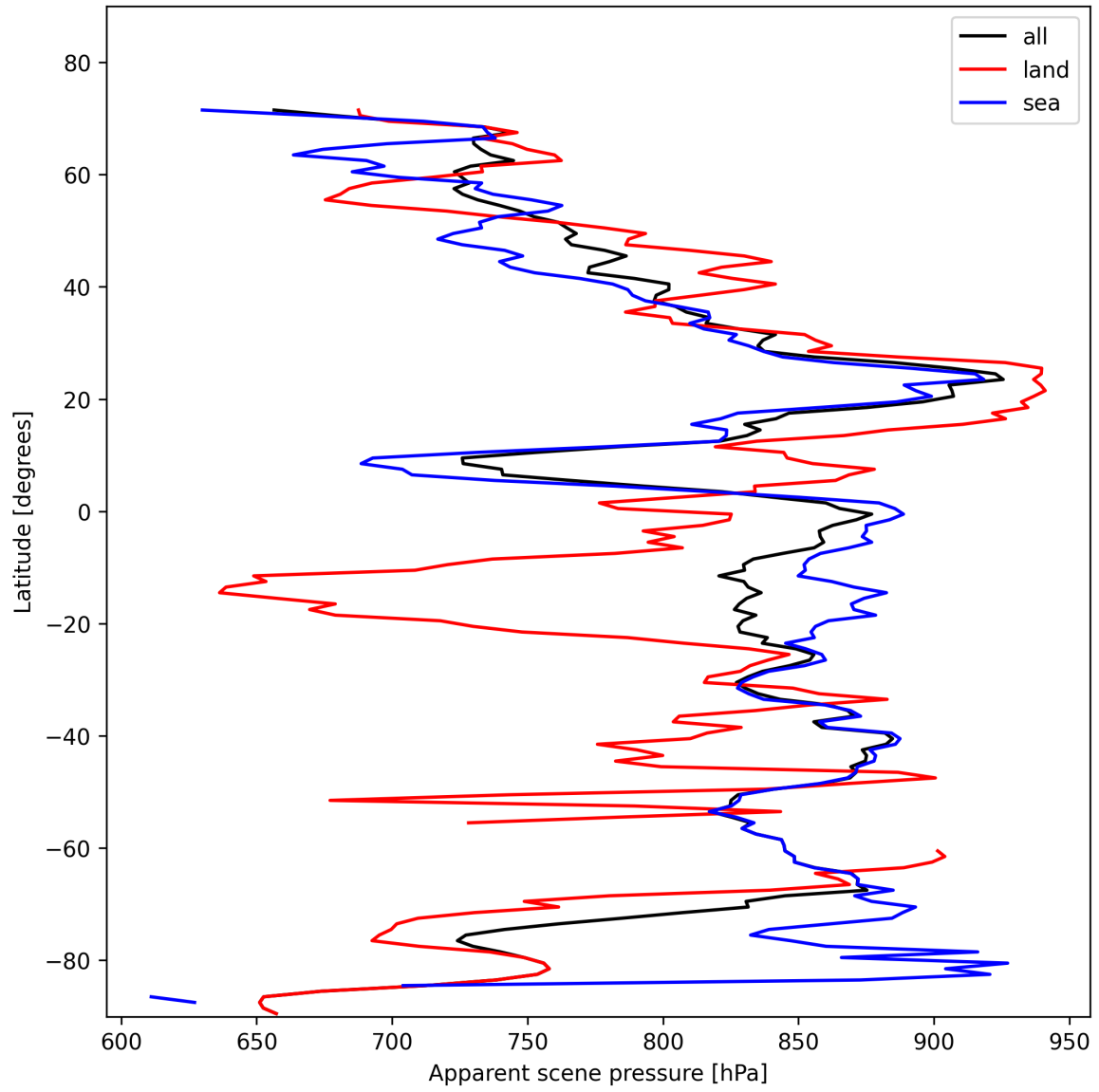
Figure 19: Zonal average of “Apparent scene pressure” for 2025-11-07 to 2025-11-09.
