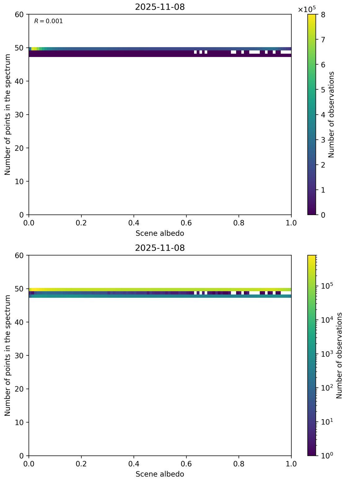
Figure 106: Scatter density plot of “Scene albedo” against “Number of points in the spectrum” for 2025-11-07 to 2025-11-09.
