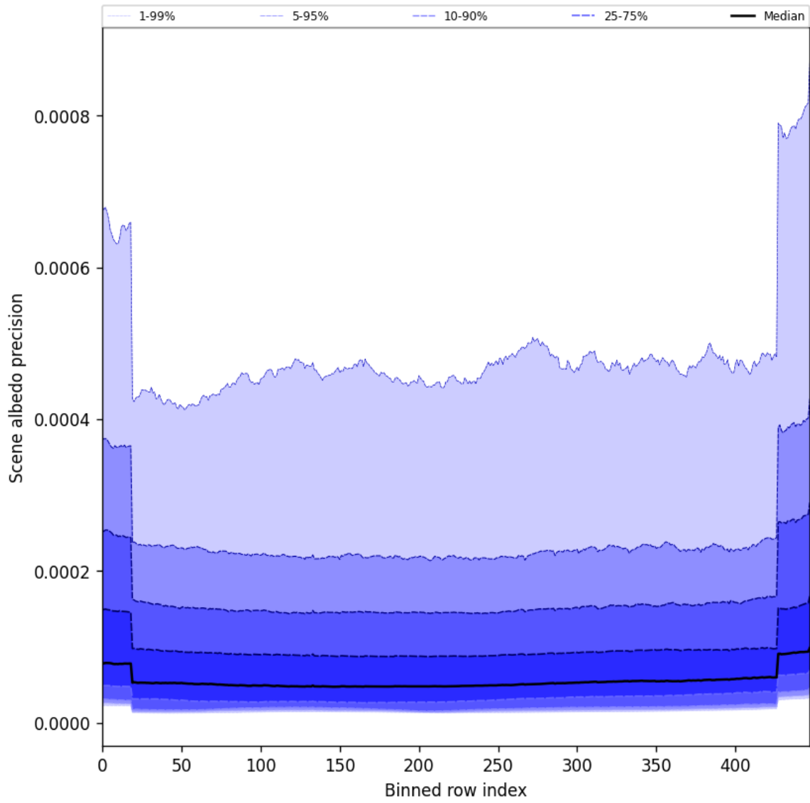
Figure 52: Along track statistics of “Scene albedo precision” for 2025-11-07 to 2025-11-09
