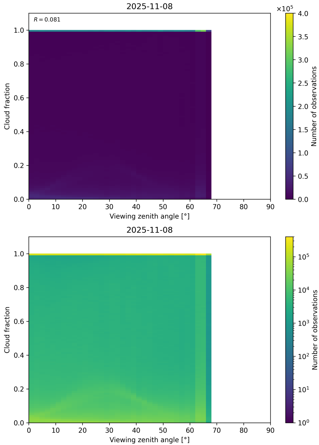
Figure 120: Scatter density plot of “Viewing zenith angle” against “Cloud fraction” for 2025-11-07 to 2025-11-09.
