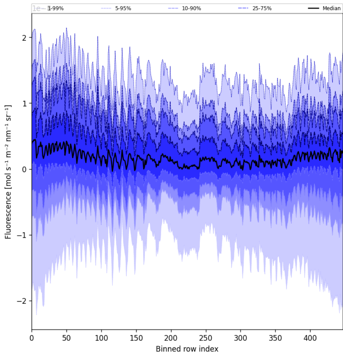
Figure 57: Along track statistics of “Fluorescence” for 2025-11-07 to 2025-11-09
