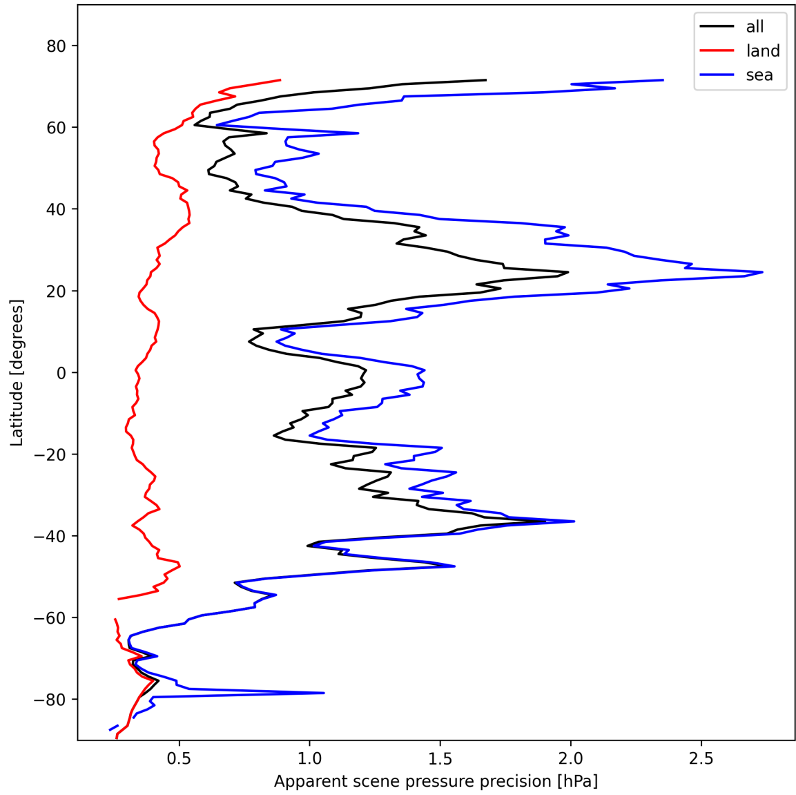
Figure 20: Zonal average of “Apparent scene pressure precision” for 2025-11-07 to 2025-11-09.
