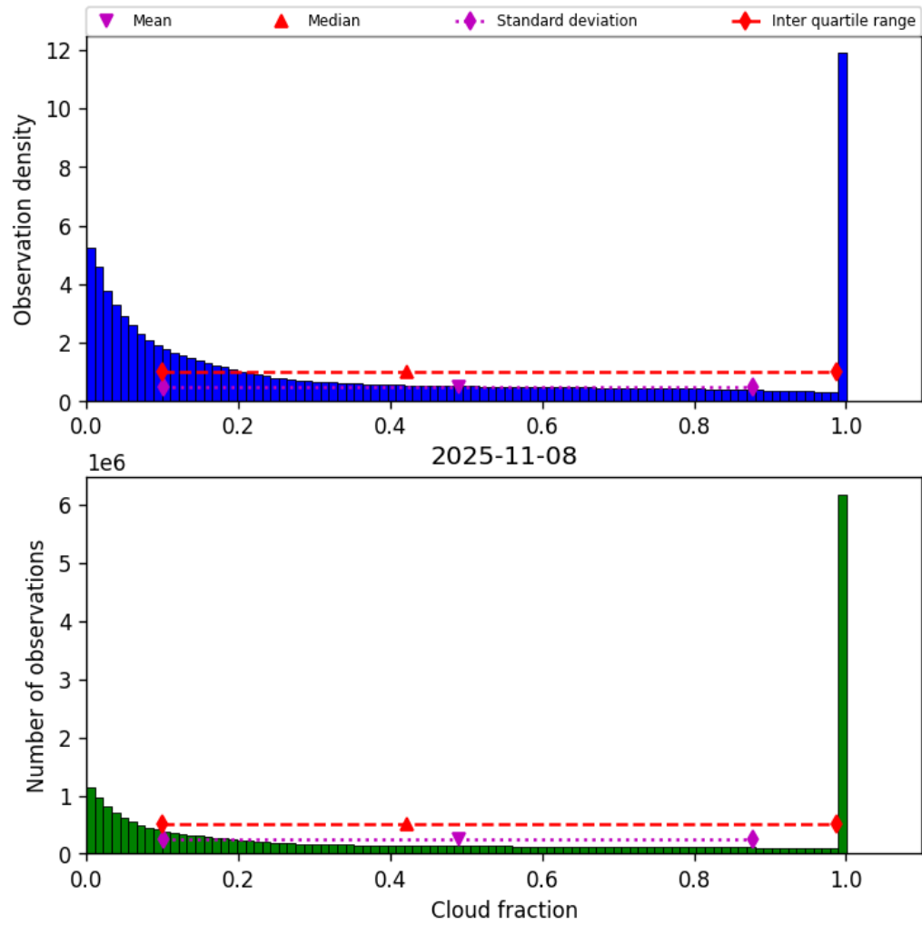
Figure 32: Histogram of “Cloud fraction” for 2025-11-07 to 2025-11-09
