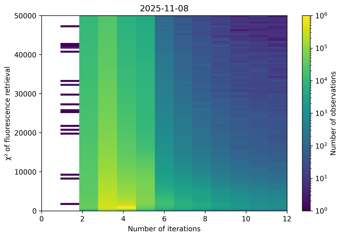
Figure 97: Scatter density plot of “Number of iterations” against “ \chi^2 of fluorescence retrieval” for 2025-11-07 to 2025-11-09.
