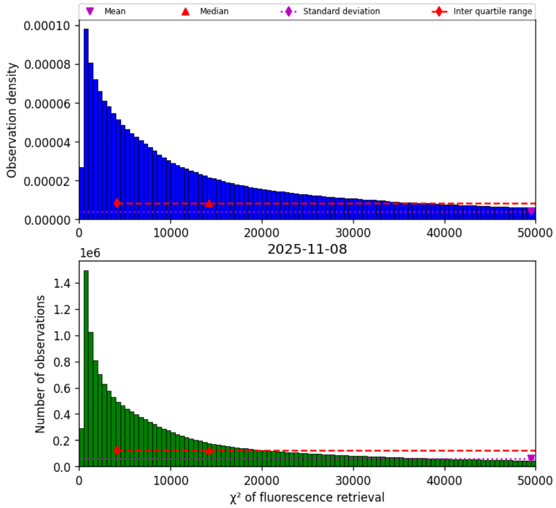
Figure 42: Histogram of “ \chi^2 of fluorescence retrieval” for 2025-11-07 to 2025-11-09
