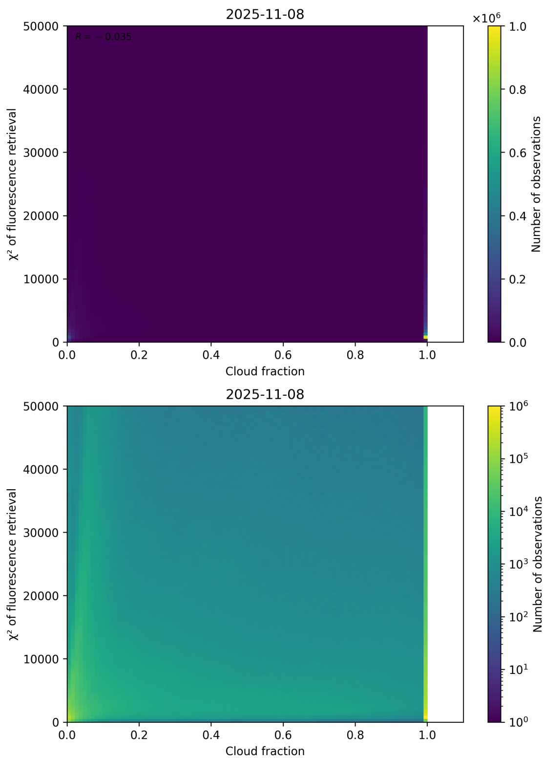
Figure 71: Scatter density plot of “Cloud fraction” against “ \chi^2 of fluorescence retrieval” for 2025-11-07 to 2025-11-09.
