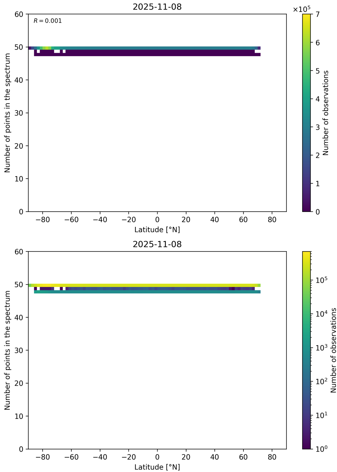
Figure 94: Scatter density plot of “Latitude” against “Number of points in the spectrum” for 2025-11-07 to 2025-11-09.
