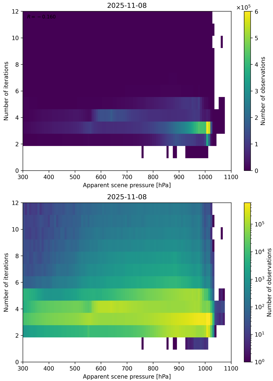
Figure 65: Scatter density plot of “Apparent scene pressure” against “Number of iterations” for 2025-11-07 to 2025-11-09.
