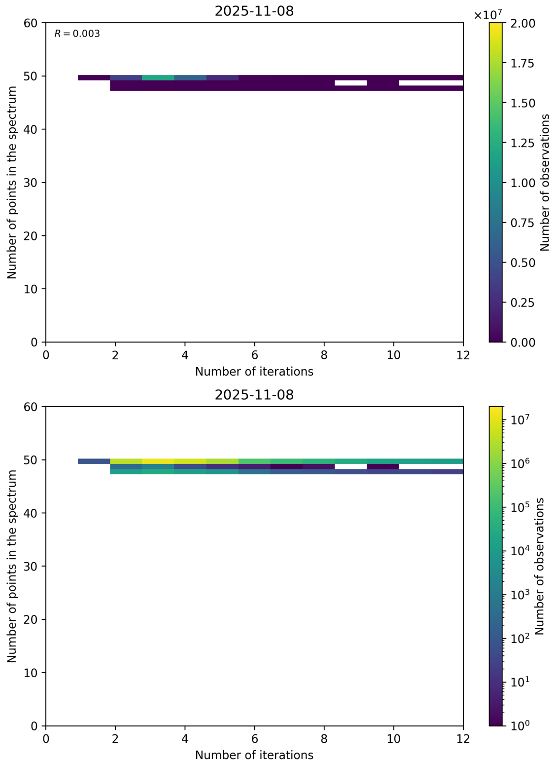
Figure 99: Scatter density plot of “Number of iterations” against “Number of points in the spectrum” for 2025-11-07 to 2025-11-09.
