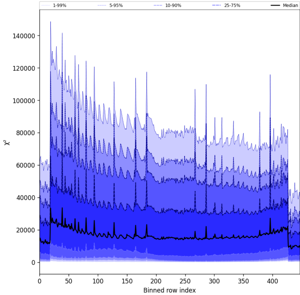
Figure 55: Along track statistics of “ \chi^2 ” for 2025-11-07 to 2025-11-09
