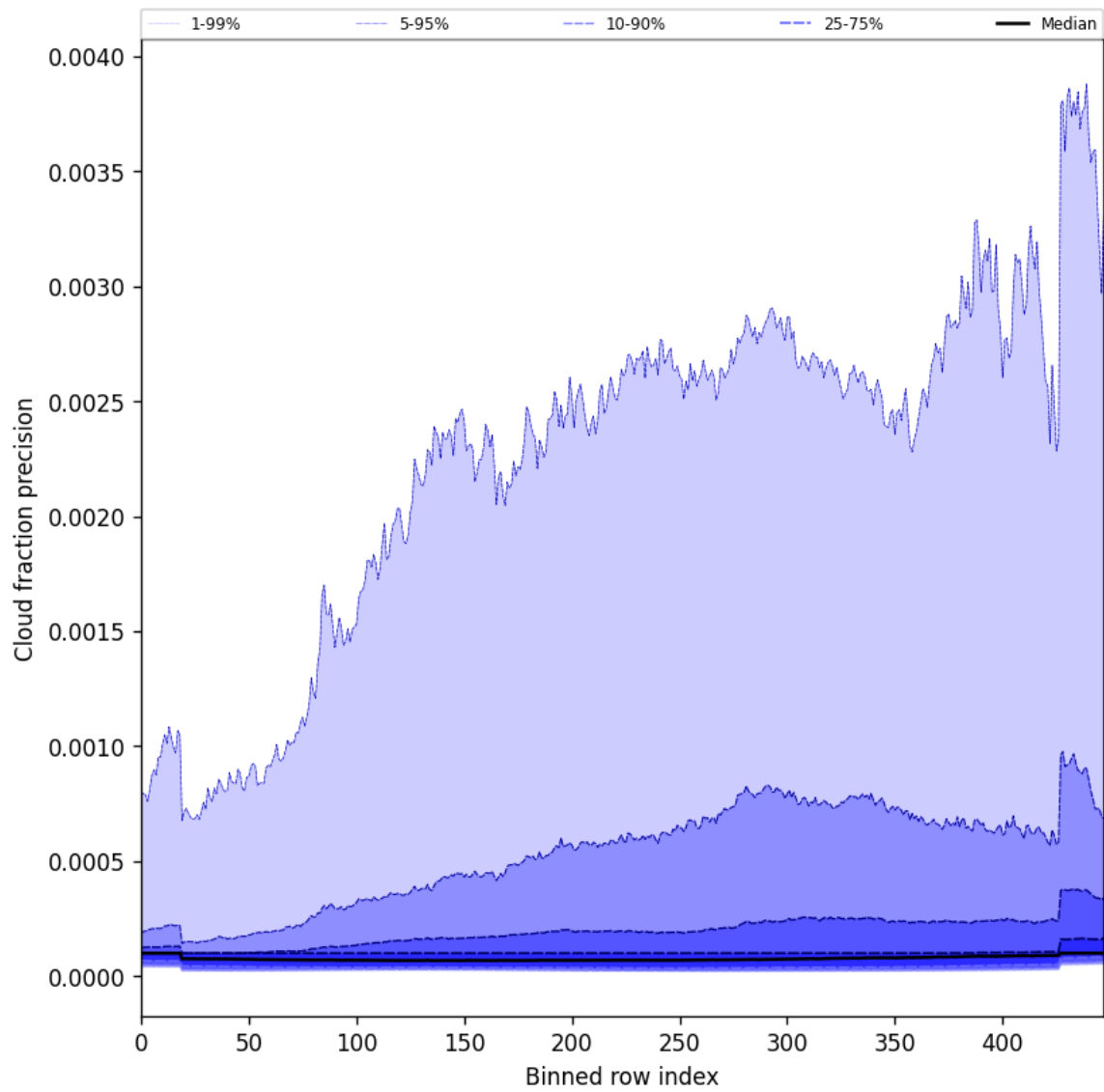
Figure 50: Along track statistics of “Cloud fraction precision” for 2025-11-07 to 2025-11-09
