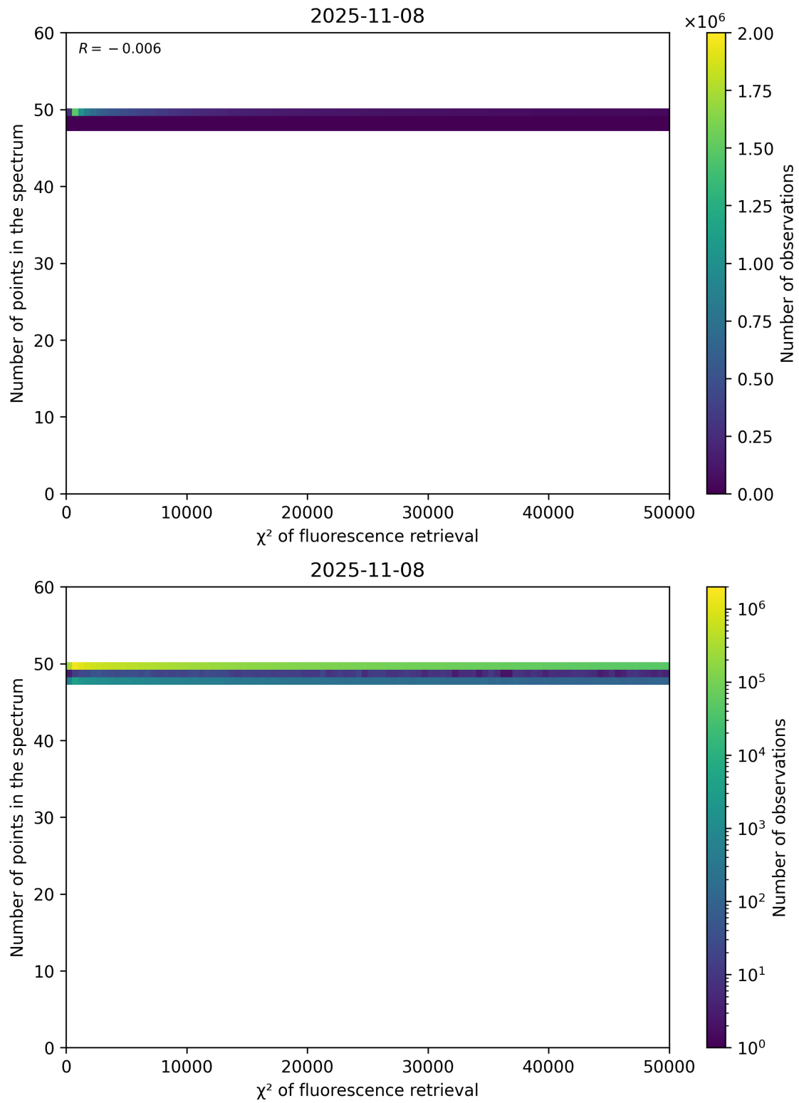
Figure 68: Scatter density plot of “ \chi^2 of fluorescence retrieval” against “Number of points in the spectrum” for 2025-11-07 to 2025-11-09.
