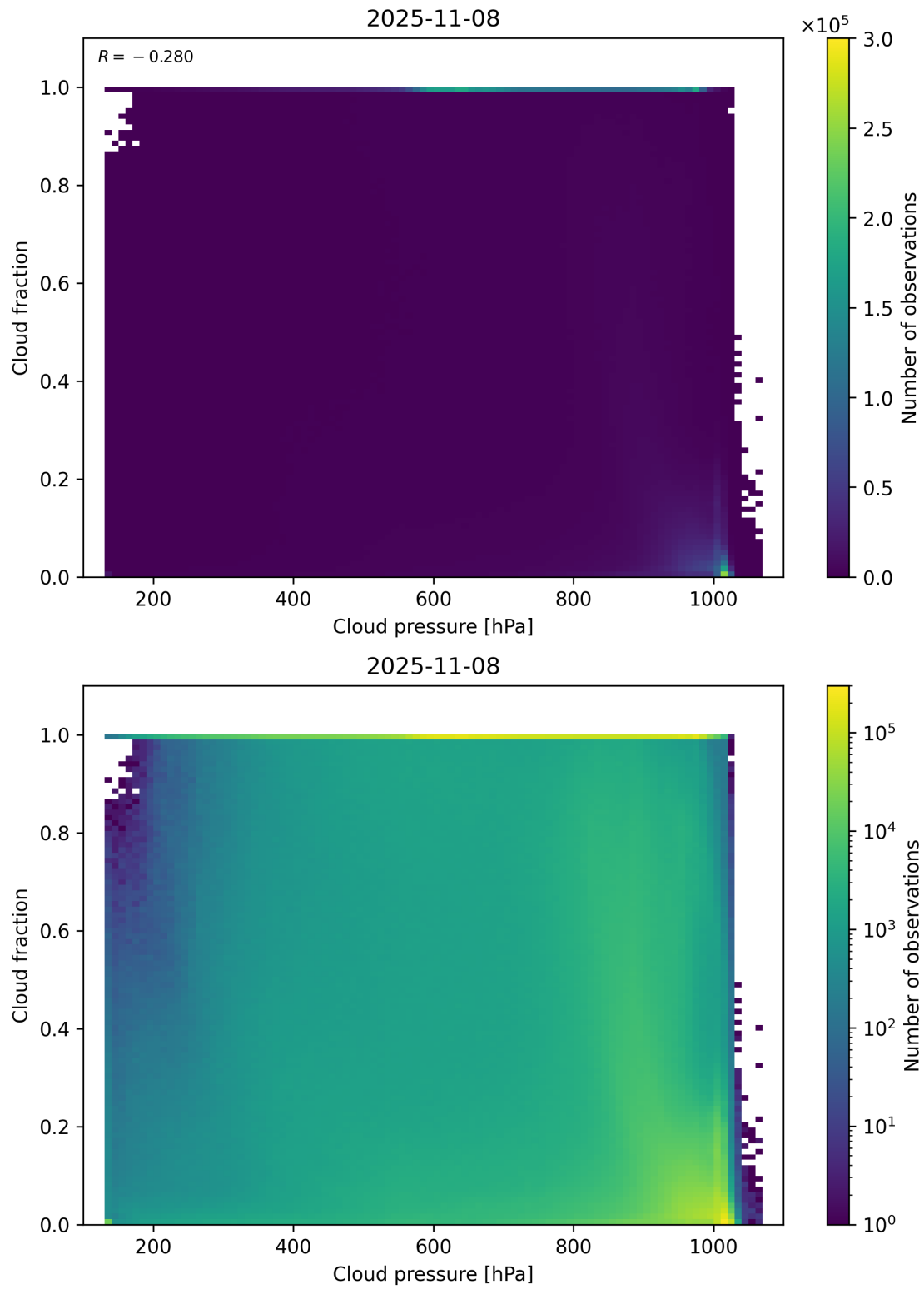
Figure 79: Scatter density plot of “Cloud pressure” against “Cloud fraction” for 2025-11-07 to 2025-11-09.
