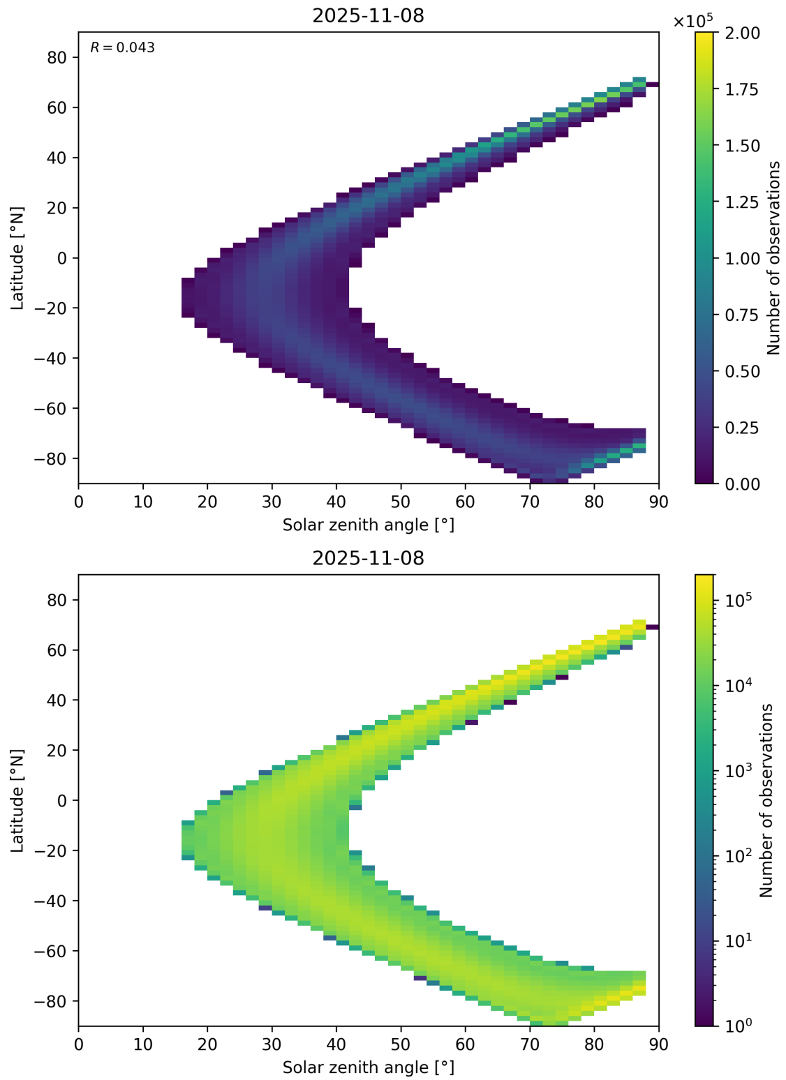
Figure 113: Scatter density plot of “Solar zenith angle” against “Latitude” for 2025-11-07 to 2025-11-09.
