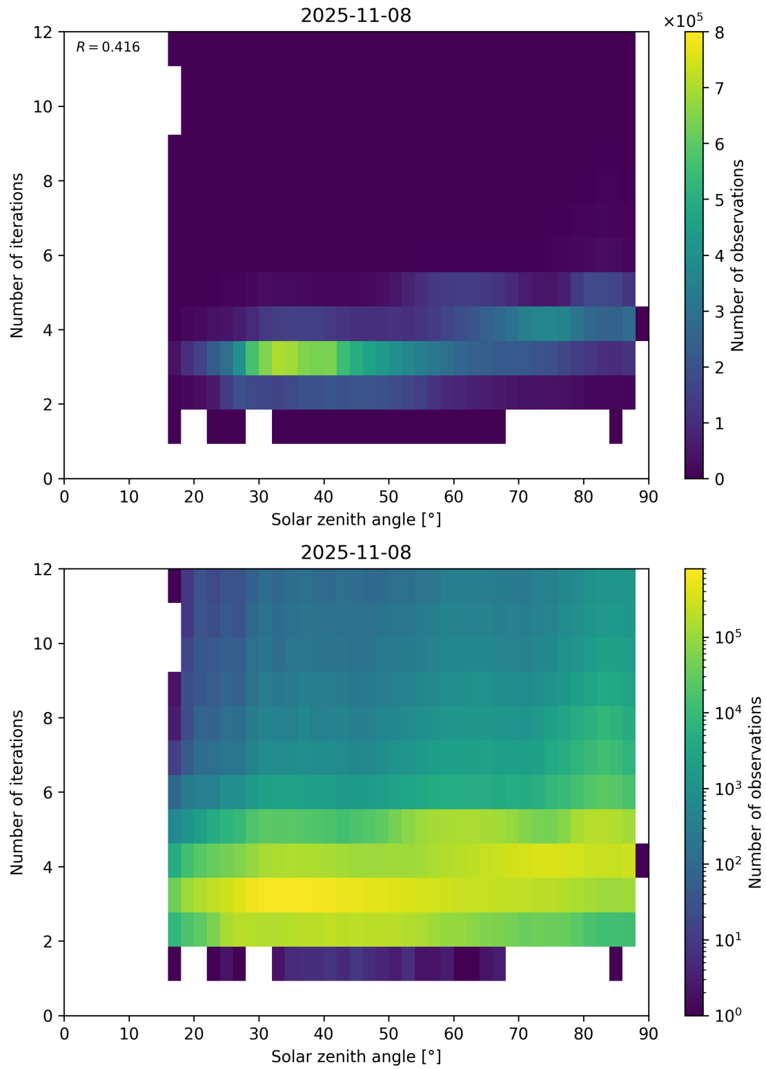
Figure 114: Scatter density plot of “Solar zenith angle” against “Number of iterations” for 2025-11-07 to 2025-11-09.
