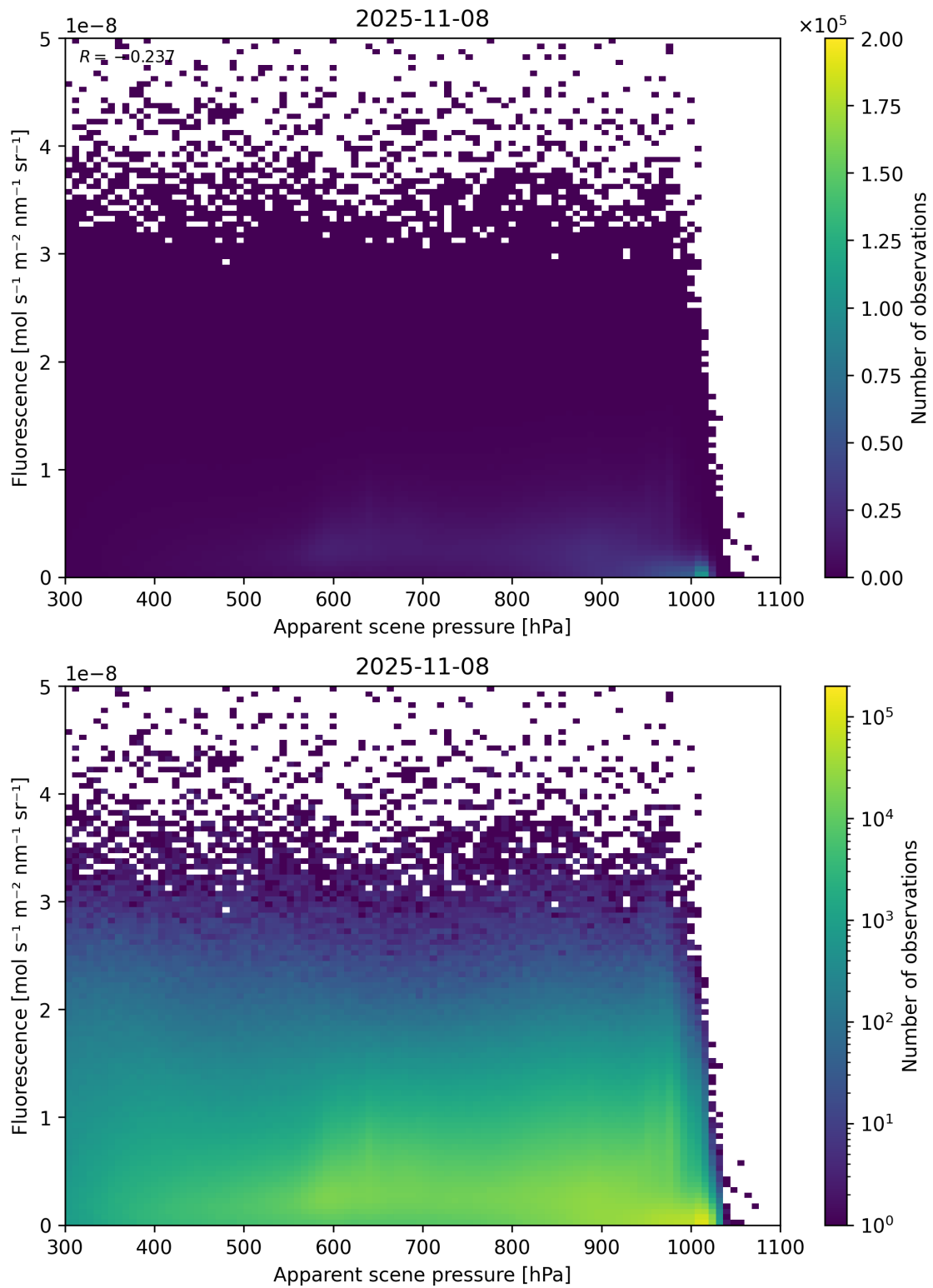
Figure 64: Scatter density plot of “Apparent scene pressure” against “Fluorescence” for 2025-11-07 to 2025-11-09.
