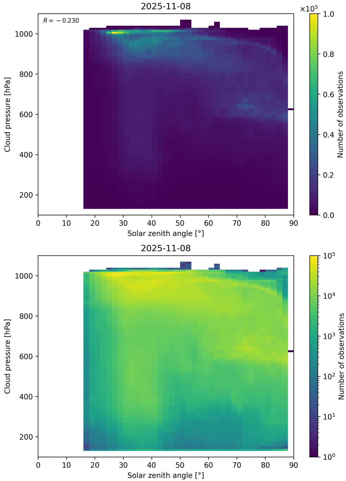
Figure 111: Scatter density plot of “Solar zenith angle” against “Cloud pressure” for 2025-11-07 to 2025-11-09.
