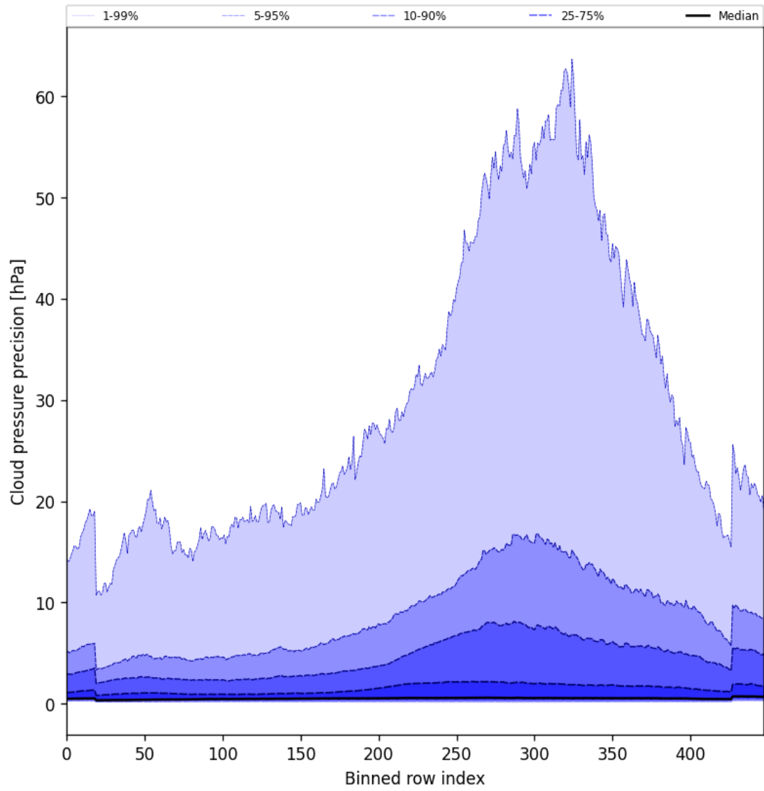
Figure 48: Along track statistics of “Cloud pressure precision” for 2025-11-07 to 2025-11-09
