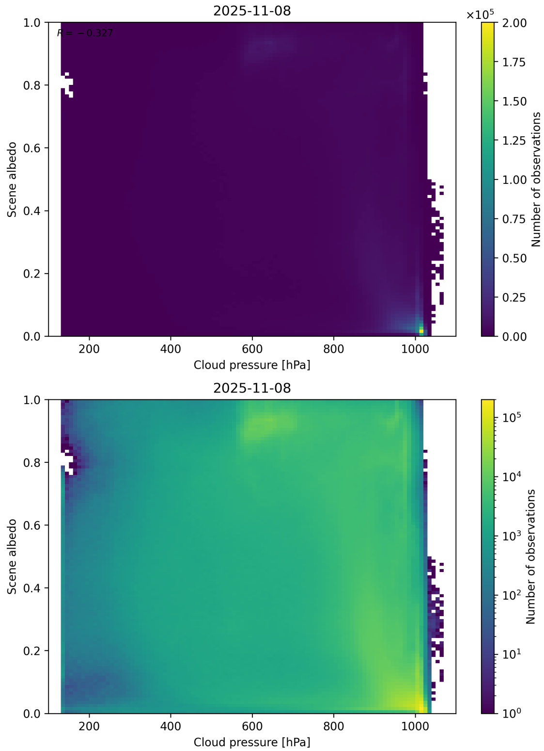
Figure 83: Scatter density plot of “Cloud pressure” against “Scene albedo” for 2025-11-07 to 2025-11-09.
