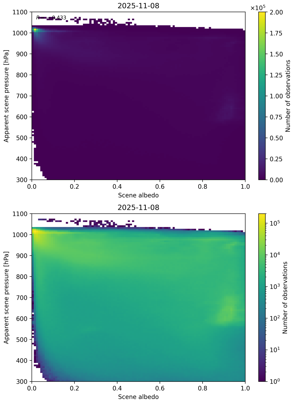
Figure 102: Scatter density plot of “Scene albedo” against “Apparent scene pressure” for 2025-11-07 to 2025-11-09.
