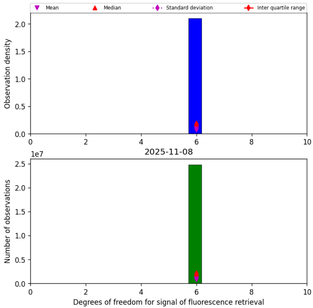
Figure 43: Histogram of “Degrees of freedom for signal of fluorescence retrieval” for 2025-11-07 to 2025-11-09
