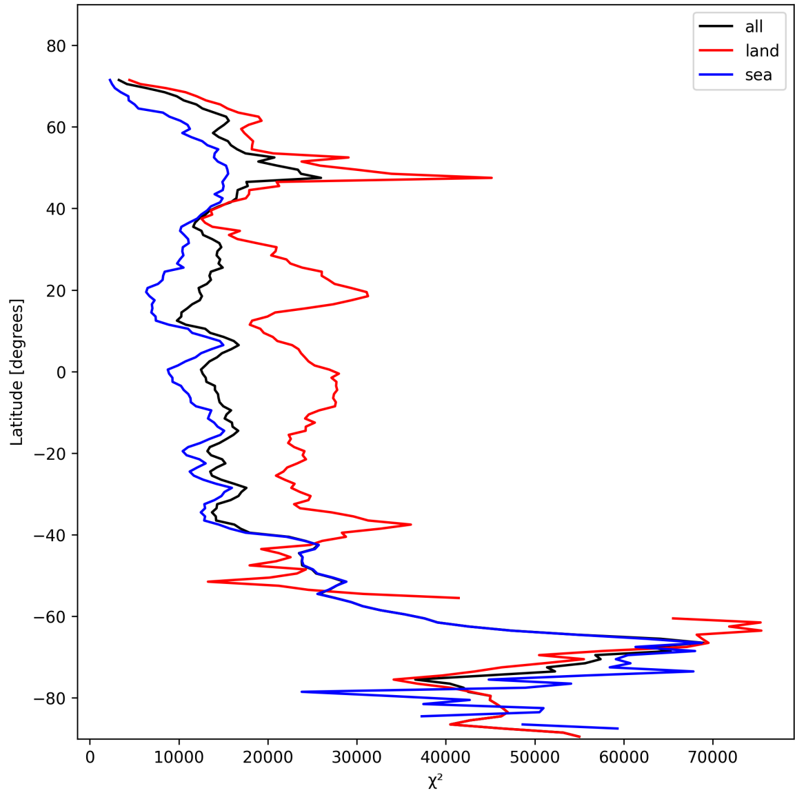
Figure 21: Zonal average of “ \chi^2 ” for 2025-11-07 to 2025-11-09.
