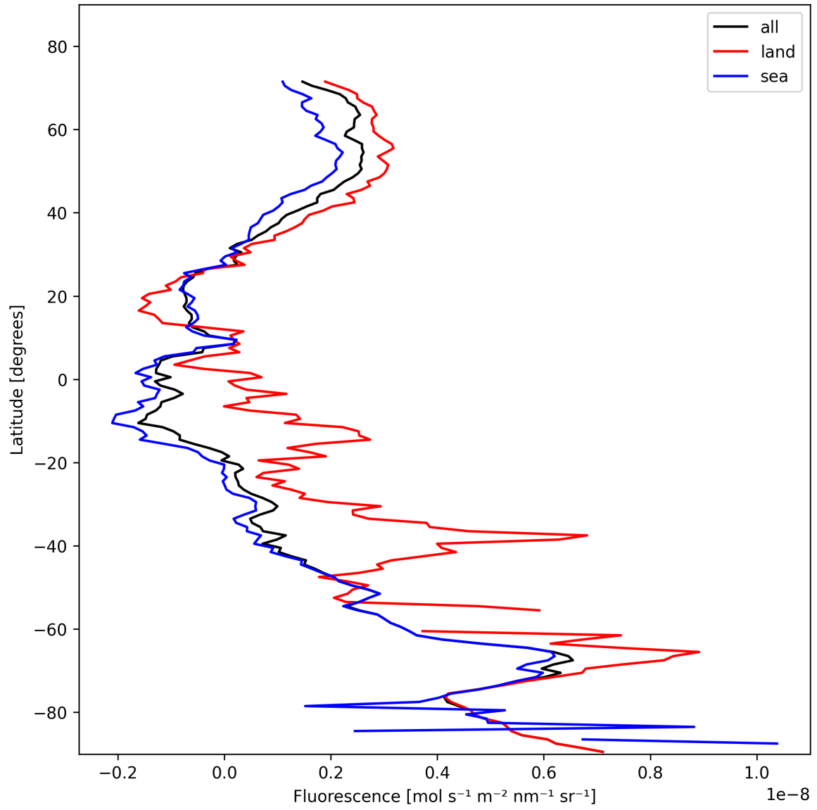
Figure 23: Zonal average of “Fluorescence” for 2025-11-07 to 2025-11-09.
