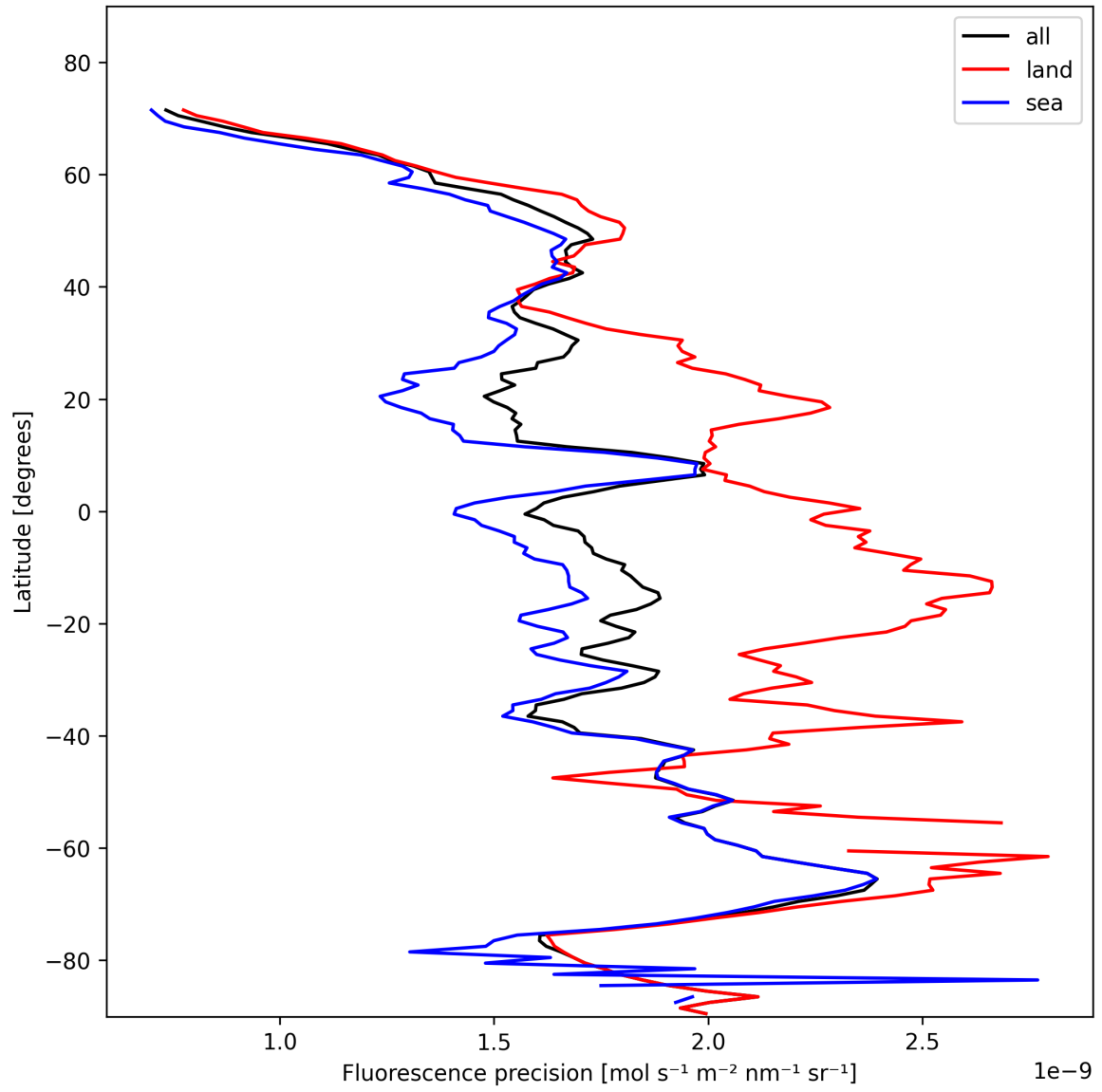
Figure 24: Zonal average of “Fluorescence precision” for 2025-11-07 to 2025-11-09.
