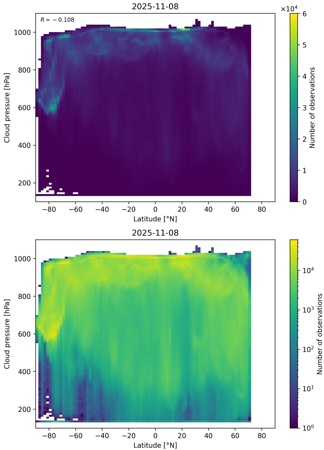
Figure 91: Scatter density plot of “Latitude” against “Cloud pressure” for 2025-11-07 to 2025-11-09.
