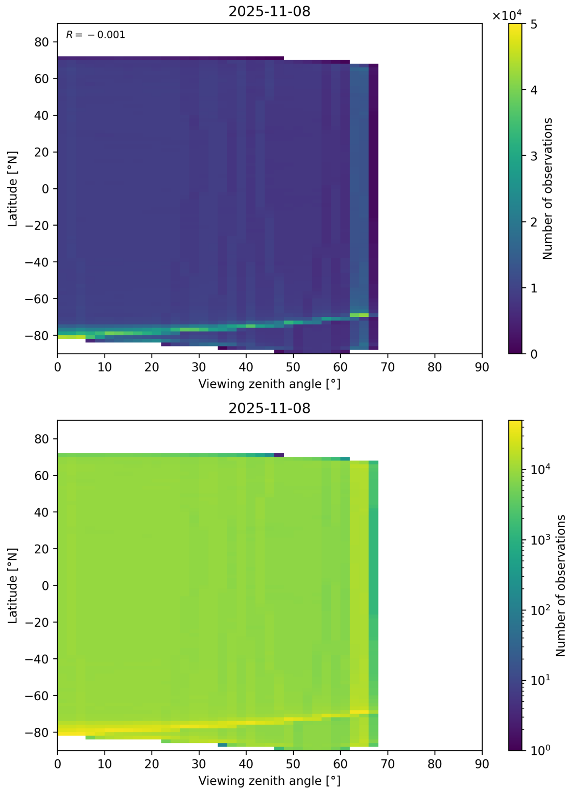
Figure 123: Scatter density plot of “Viewing zenith angle” against “Latitude” for 2025-11-07 to 2025-11-09.
