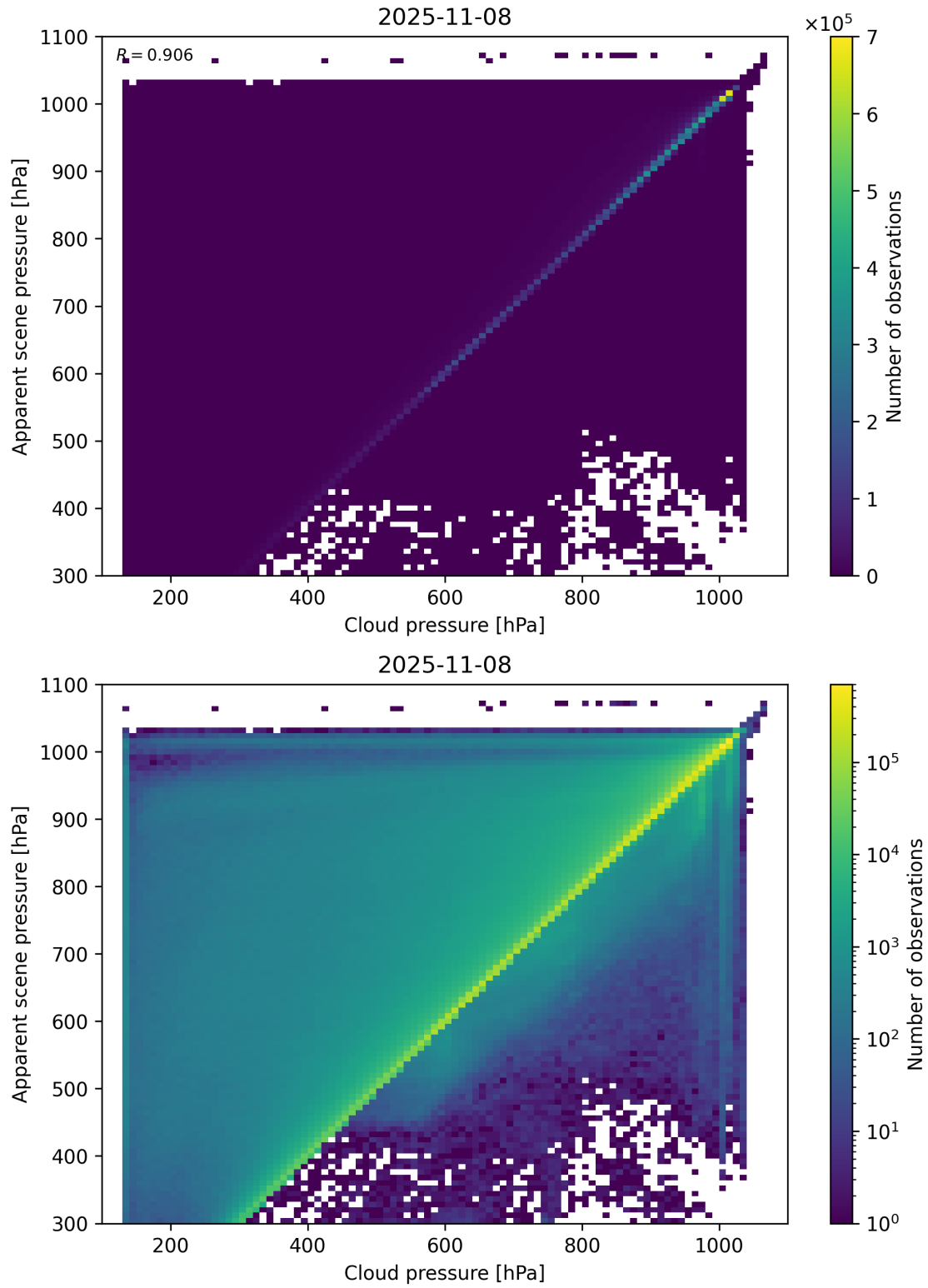
Figure 77: Scatter density plot of “Cloud pressure” against “Apparent scene pressure” for 2025-11-07 to 2025-11-09.
