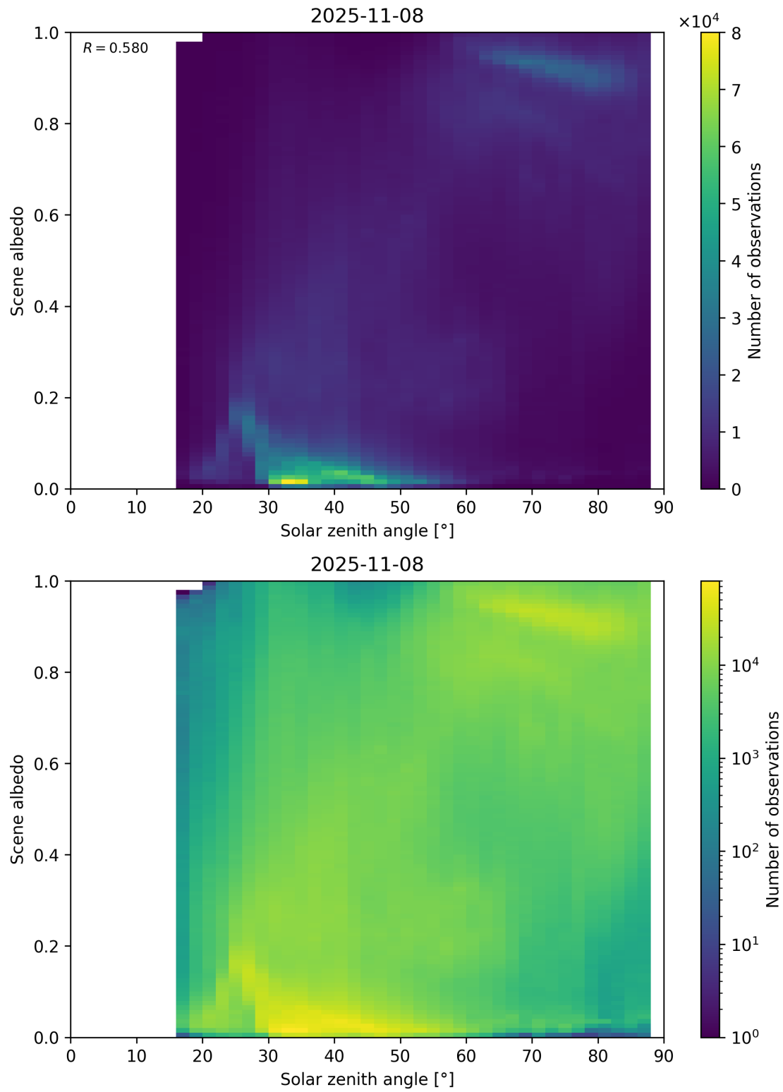
Figure 116: Scatter density plot of “Solar zenith angle” against “Scene albedo” for 2025-11-07 to 2025-11-09.
