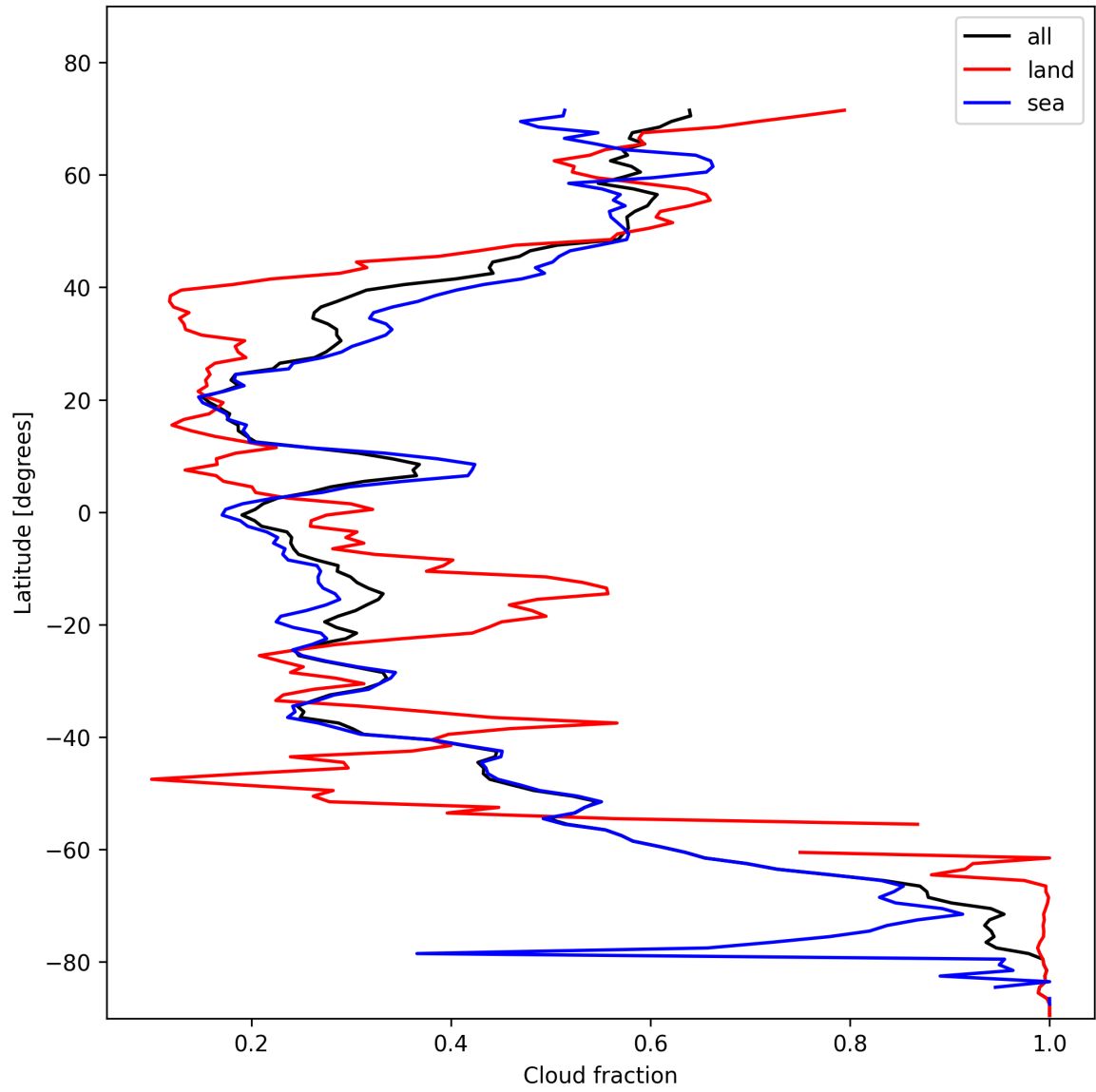
Figure 15: Zonal average of “Cloud fraction” for 2025-11-07 to 2025-11-09.
