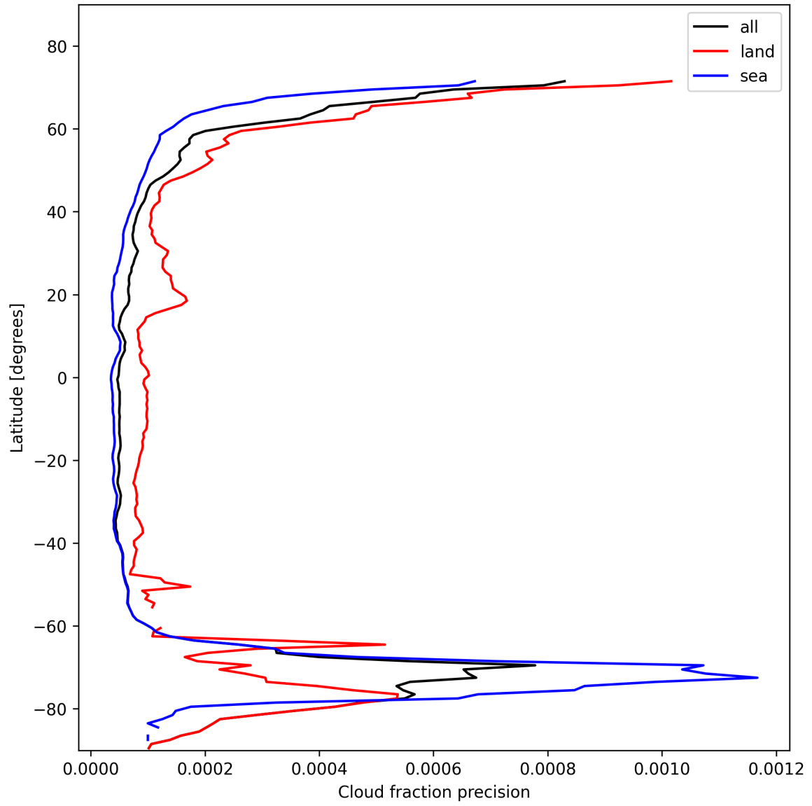
Figure 16: Zonal average of “Cloud fraction precision” for 2025-11-07 to 2025-11-09.
