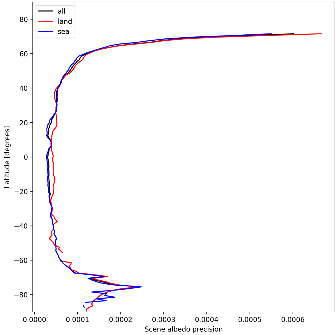
Figure 18: Zonal average of “Scene albedo precision” for 2025-11-07 to 2025-11-09.
