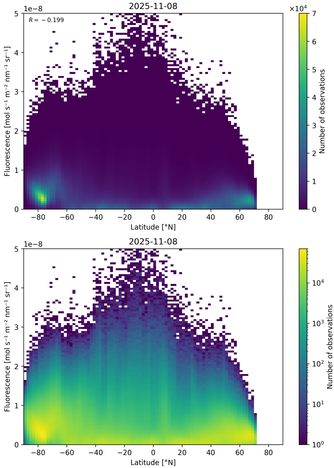
Figure 92: Scatter density plot of “Latitude” against “Fluorescence” for 2025-11-07 to 2025-11-09.
