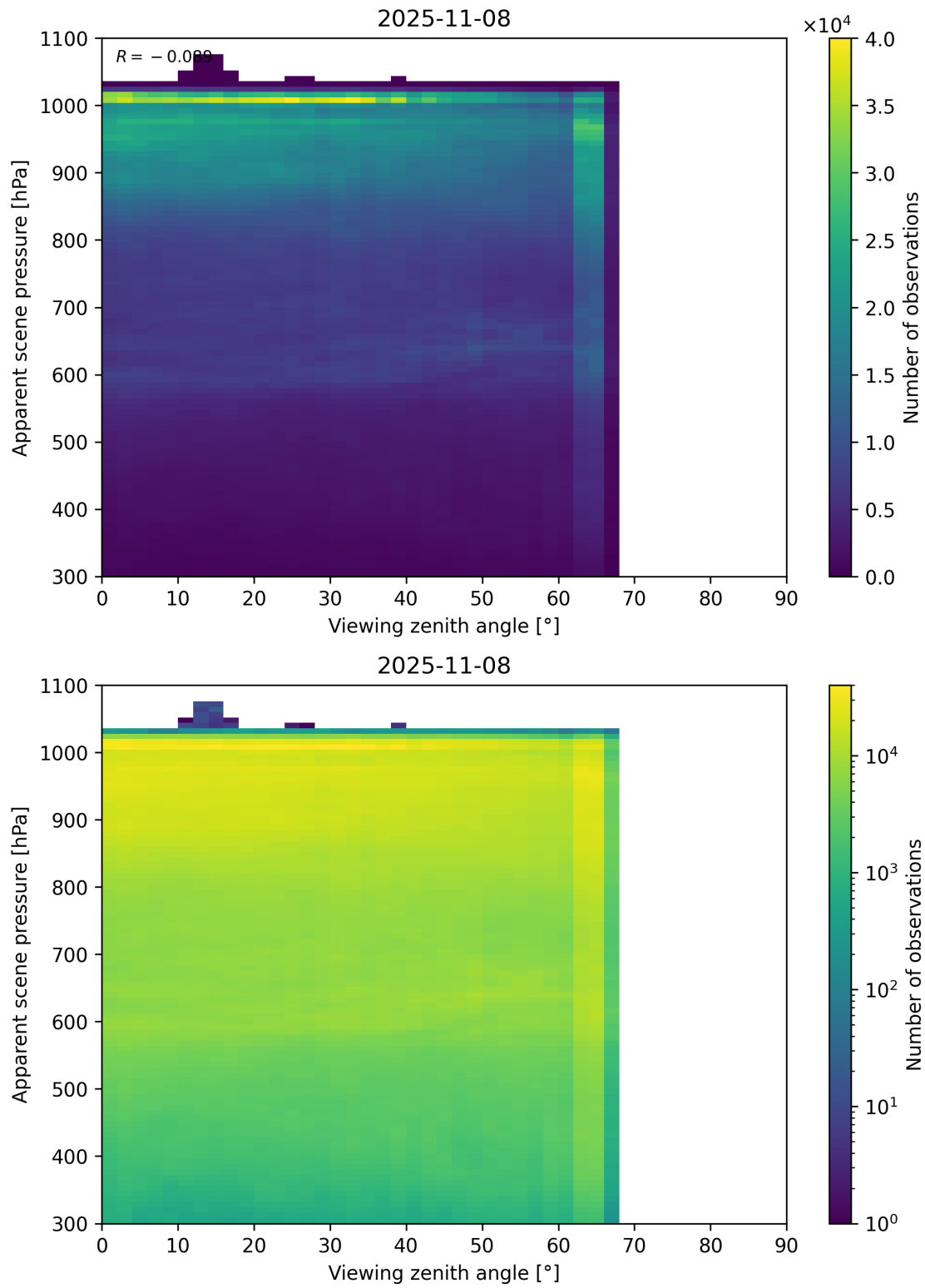
Figure 118: Scatter density plot of “Viewing zenith angle” against “Apparent scene pressure” for 2025-11-07 to 2025-11-09.
