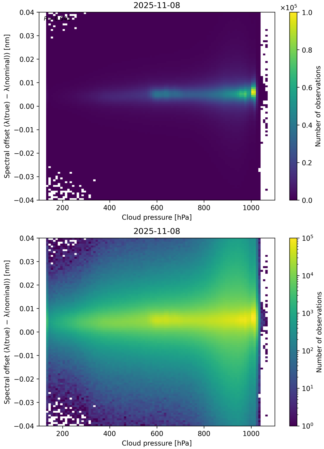
Figure 84: Scatter density plot of “Cloud pressure” against “Spectral offset ( \lambda_{\text{true}} - \lambda_{\text{nominal}} )” for 2025-11-07 to 2025-11-09.
