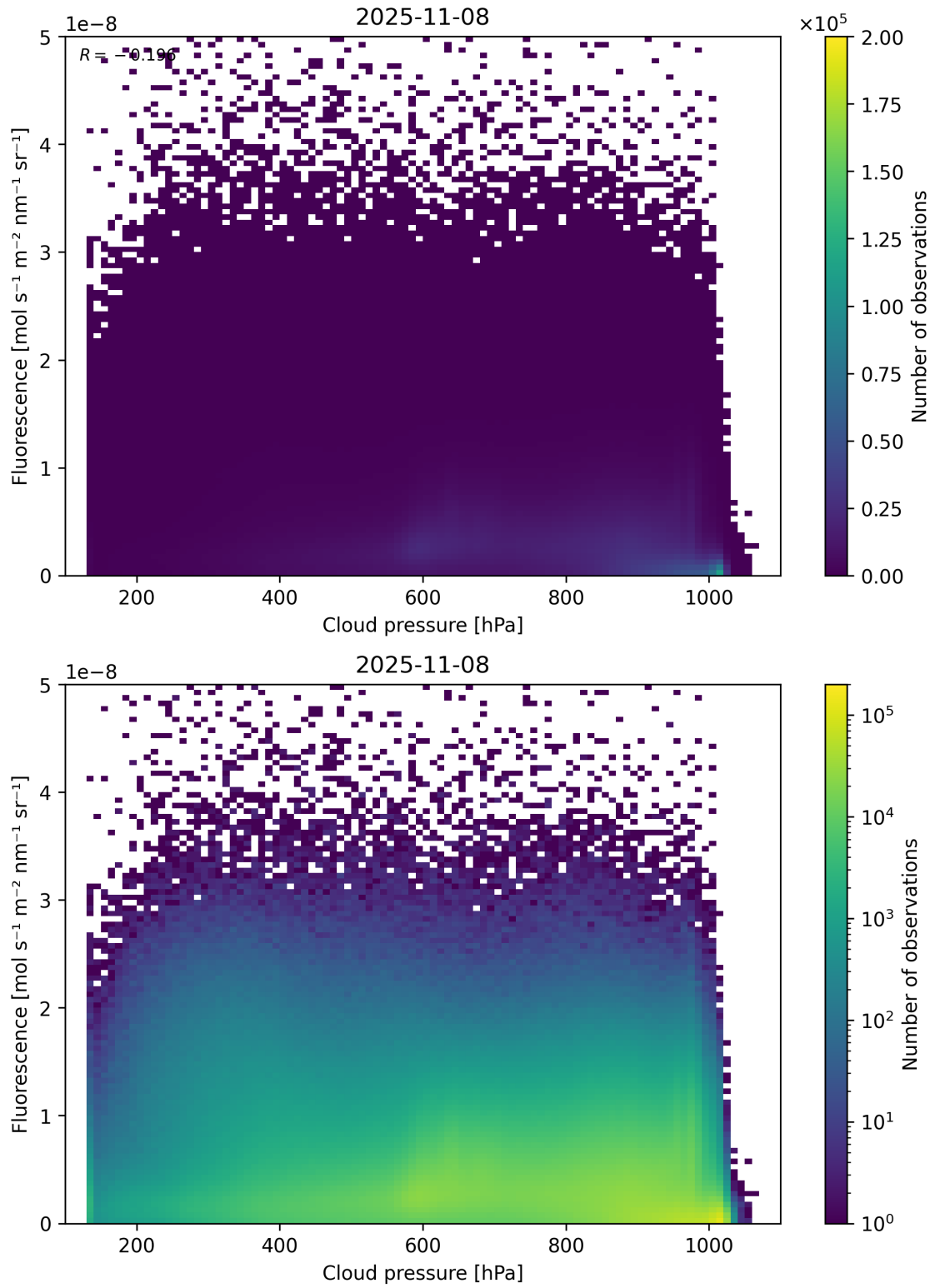
Figure 80: Scatter density plot of “Cloud pressure” against “Fluorescence” for 2025-11-07 to 2025-11-09.
