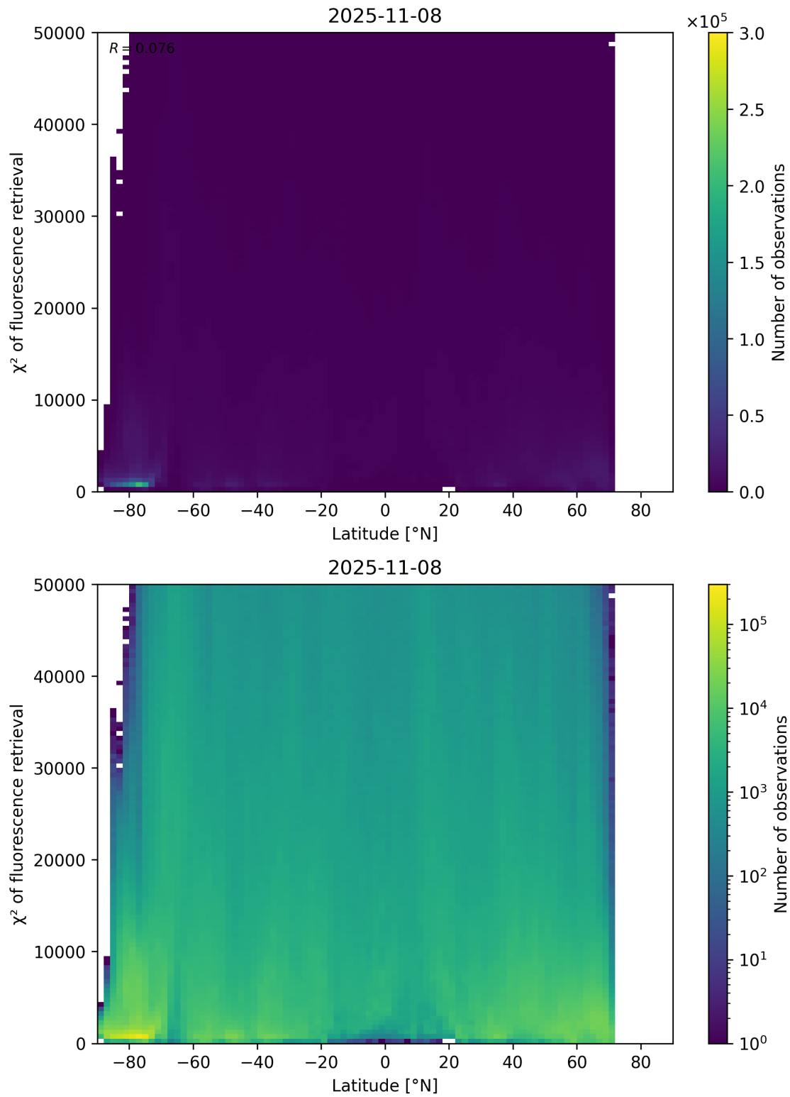
Figure 89: Scatter density plot of “Latitude” against “ \chi^2 of fluorescence retrieval” for 2025-11-07 to 2025-11-09.
