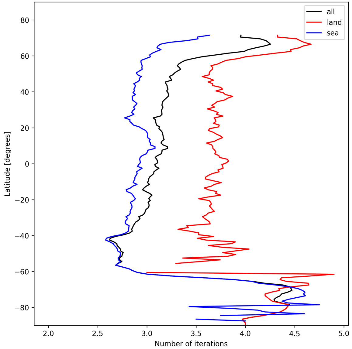
Figure 22: Zonal average of “Number of iterations” for 2025-11-07 to 2025-11-09.
