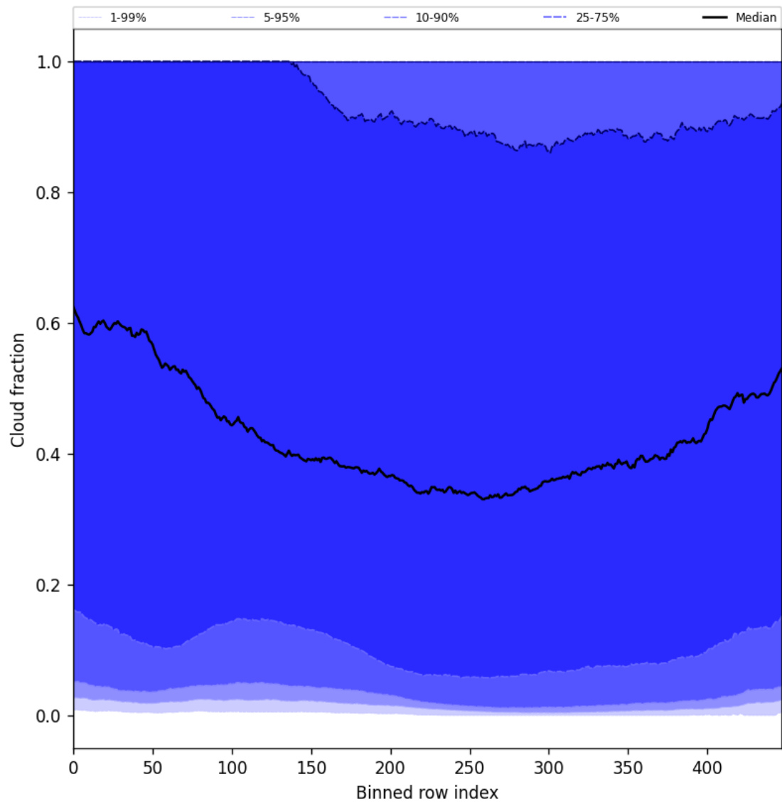
Figure 49: Along track statistics of “Cloud fraction” for 2025-11-07 to 2025-11-09
