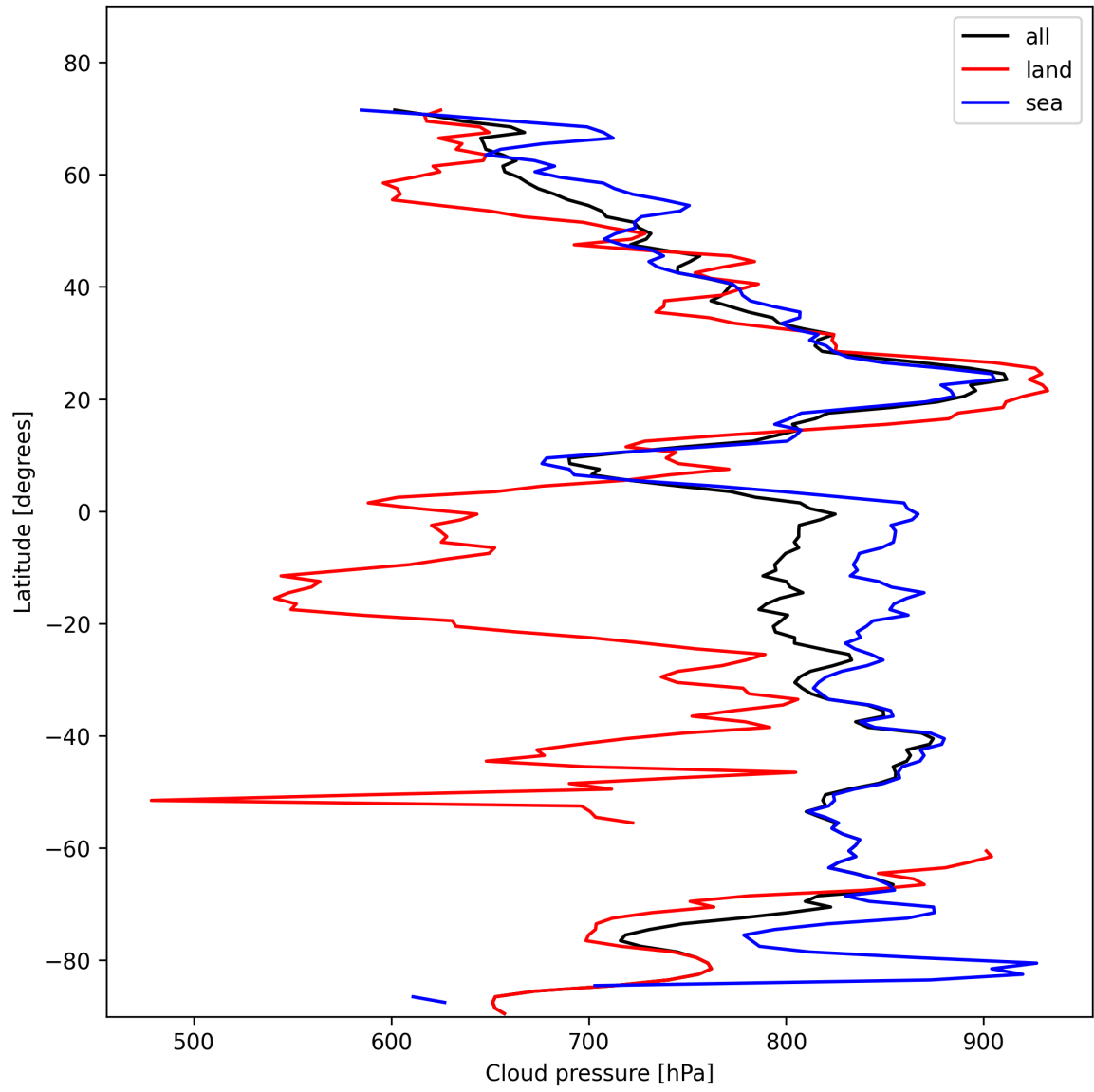
Figure 13: Zonal average of “Cloud pressure” for 2025-11-07 to 2025-11-09.
