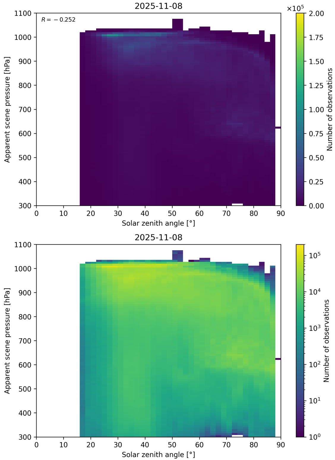
Figure 108: Scatter density plot of “Solar zenith angle” against “Apparent scene pressure” for 2025-11-07 to 2025-11-09.
