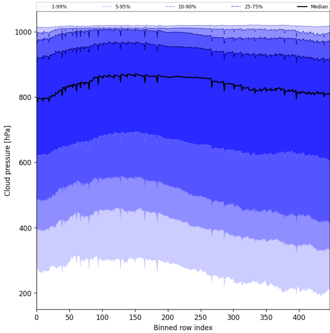
Figure 47: Along track statistics of “Cloud pressure” for 2025-11-07 to 2025-11-09
