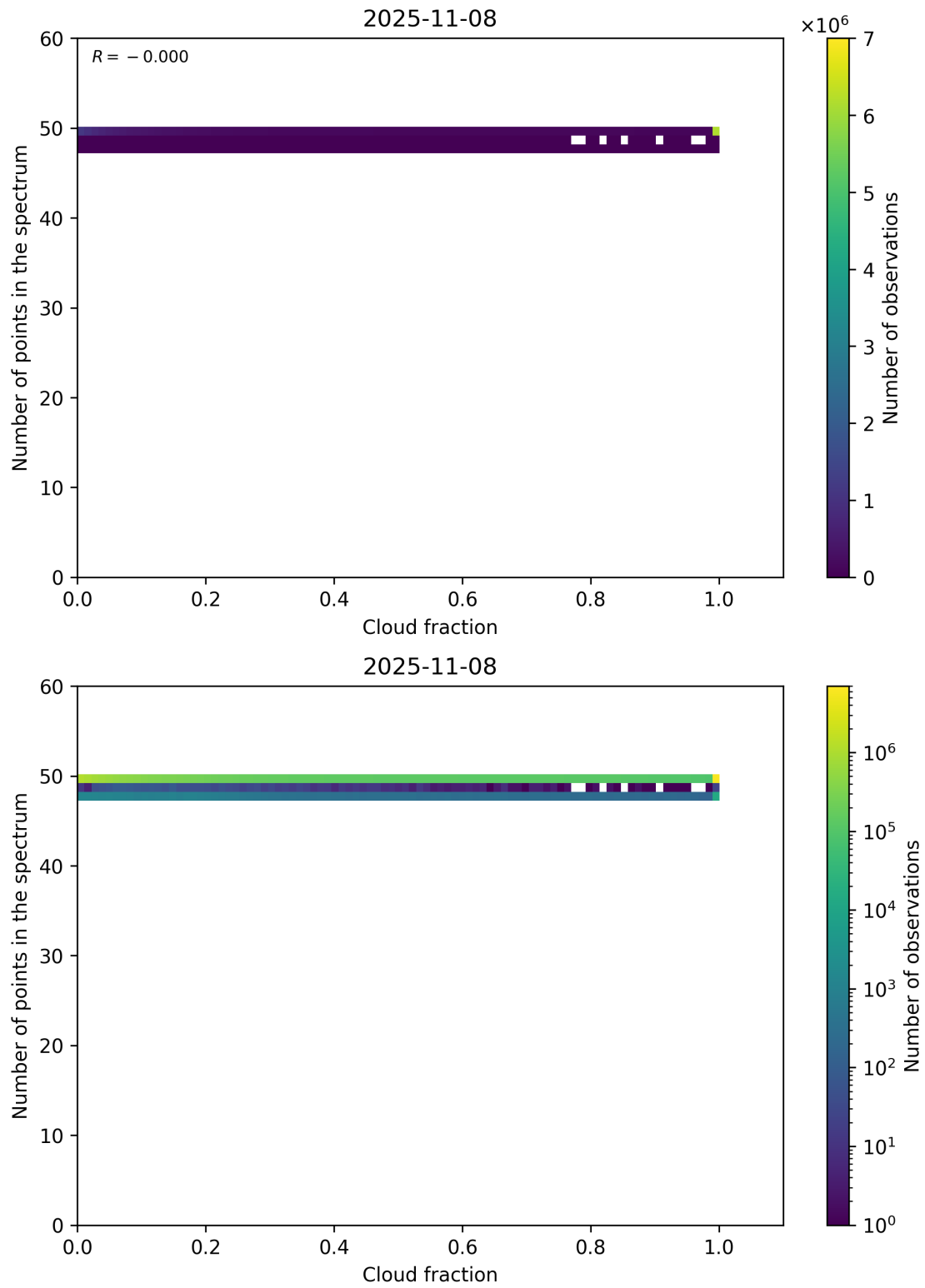
Figure 74: Scatter density plot of “Cloud fraction” against “Number of points in the spectrum” for 2025-11-07 to 2025-11-09.
