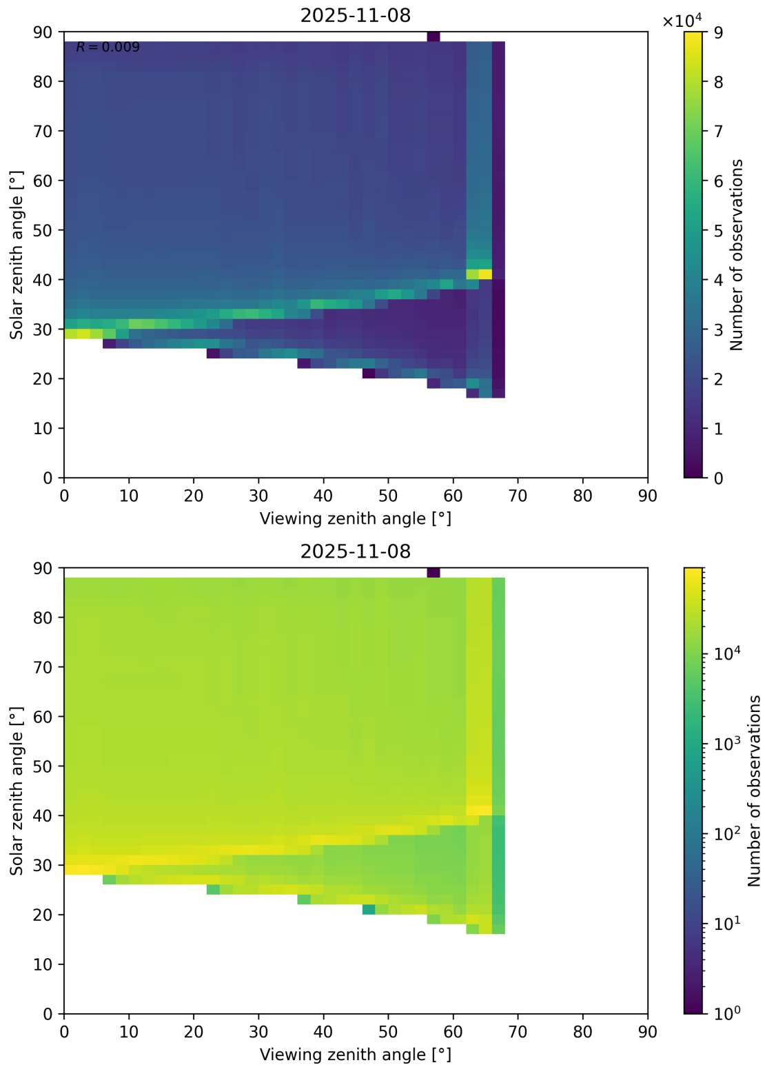
Figure 127: Scatter density plot of “Viewing zenith angle” against “Solar zenith angle” for 2025-11-07 to 2025-11-09.
