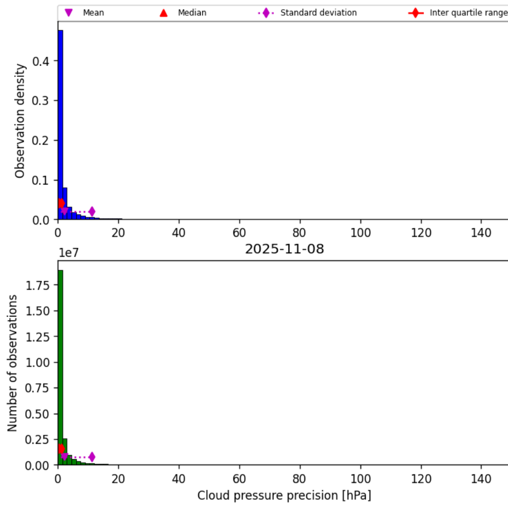
Figure 31: Histogram of “Cloud pressure precision” for 2025-11-07 to 2025-11-09
