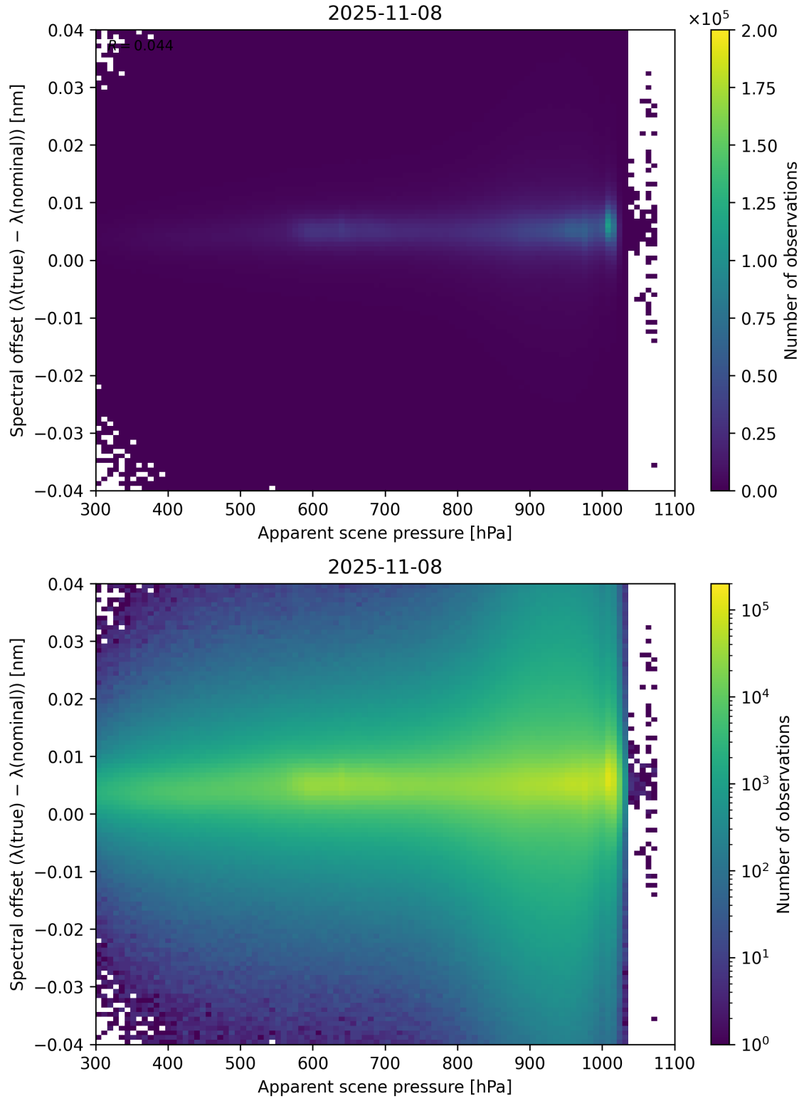
Figure 67: Scatter density plot of “Apparent scene pressure” against “Spectral offset ( \lambda_{\text{true}} - \lambda_{\text{nominal}} )” for 2025-11-07 to 2025-11-09.
