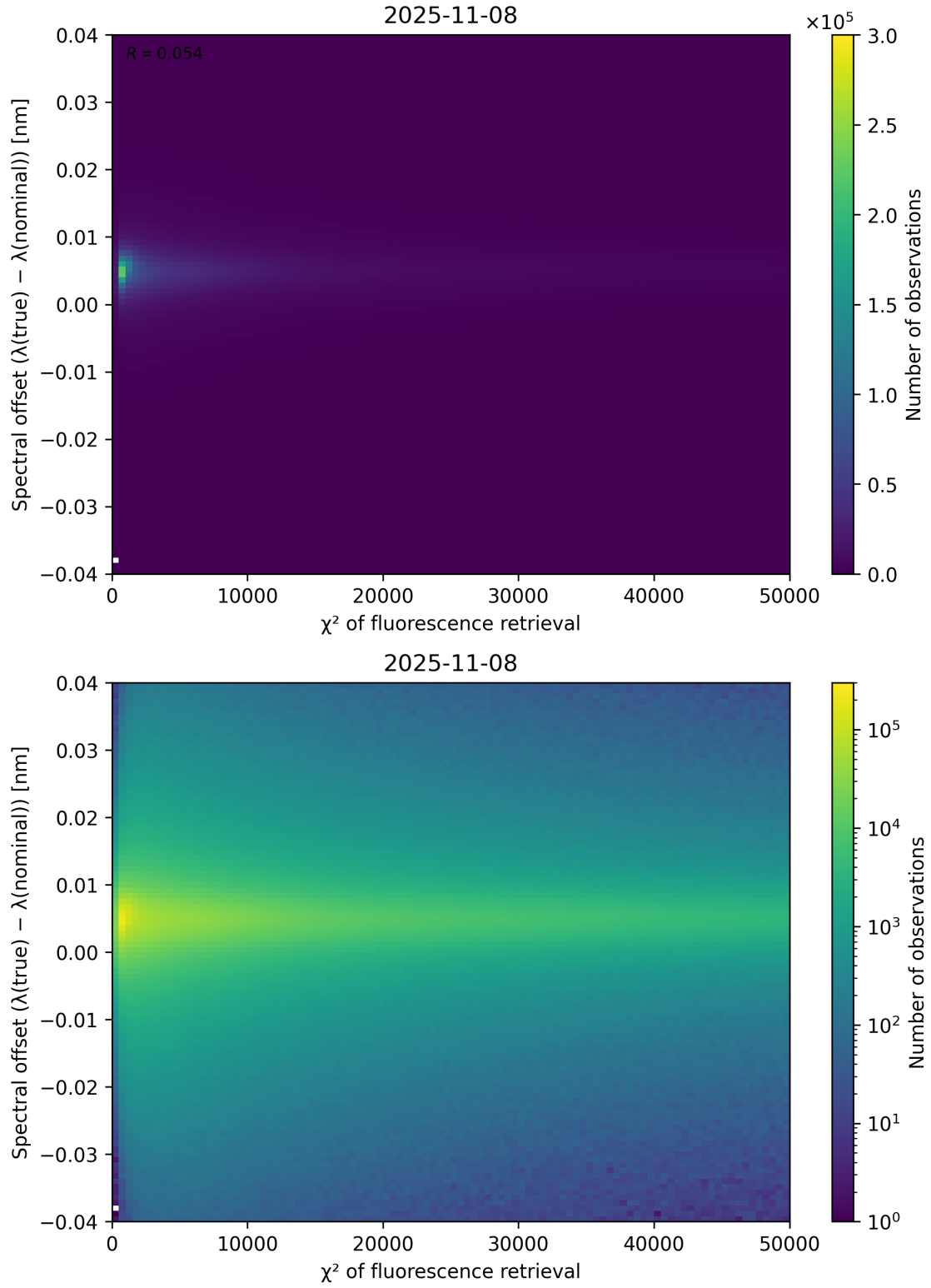
Figure 69: Scatter density plot of “ \chi^2 of fluorescence retrieval” against “Spectral offset ( \lambda_{\text{true}} - \lambda_{\text{nominal}} )” for 2025-11-07 to 2025-11-09.
