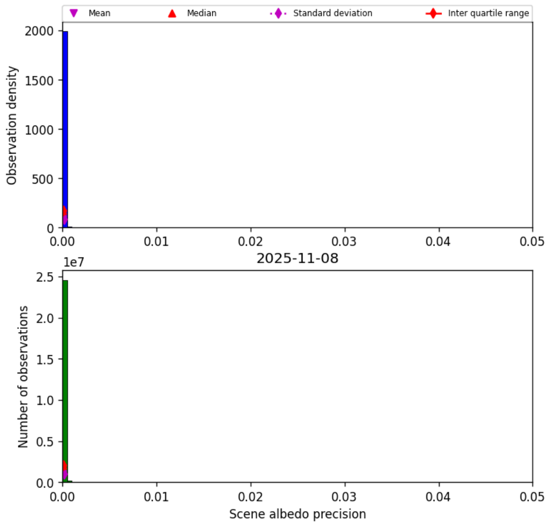
Figure 35: Histogram of “Scene albedo precision” for 2025-11-07 to 2025-11-09
