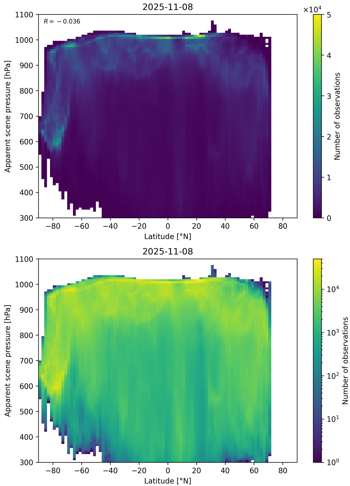
Figure 88: Scatter density plot of “Latitude” against “Apparent scene pressure” for 2025-11-07 to 2025-11-09.
