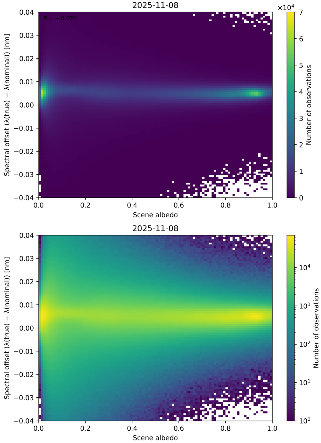
Figure 107: Scatter density plot of “Scene albedo” against “Spectral offset ( \lambda_{\text{true}} - \lambda_{\text{nominal}} )” for 2025-11-07 to 2025-11-09.
