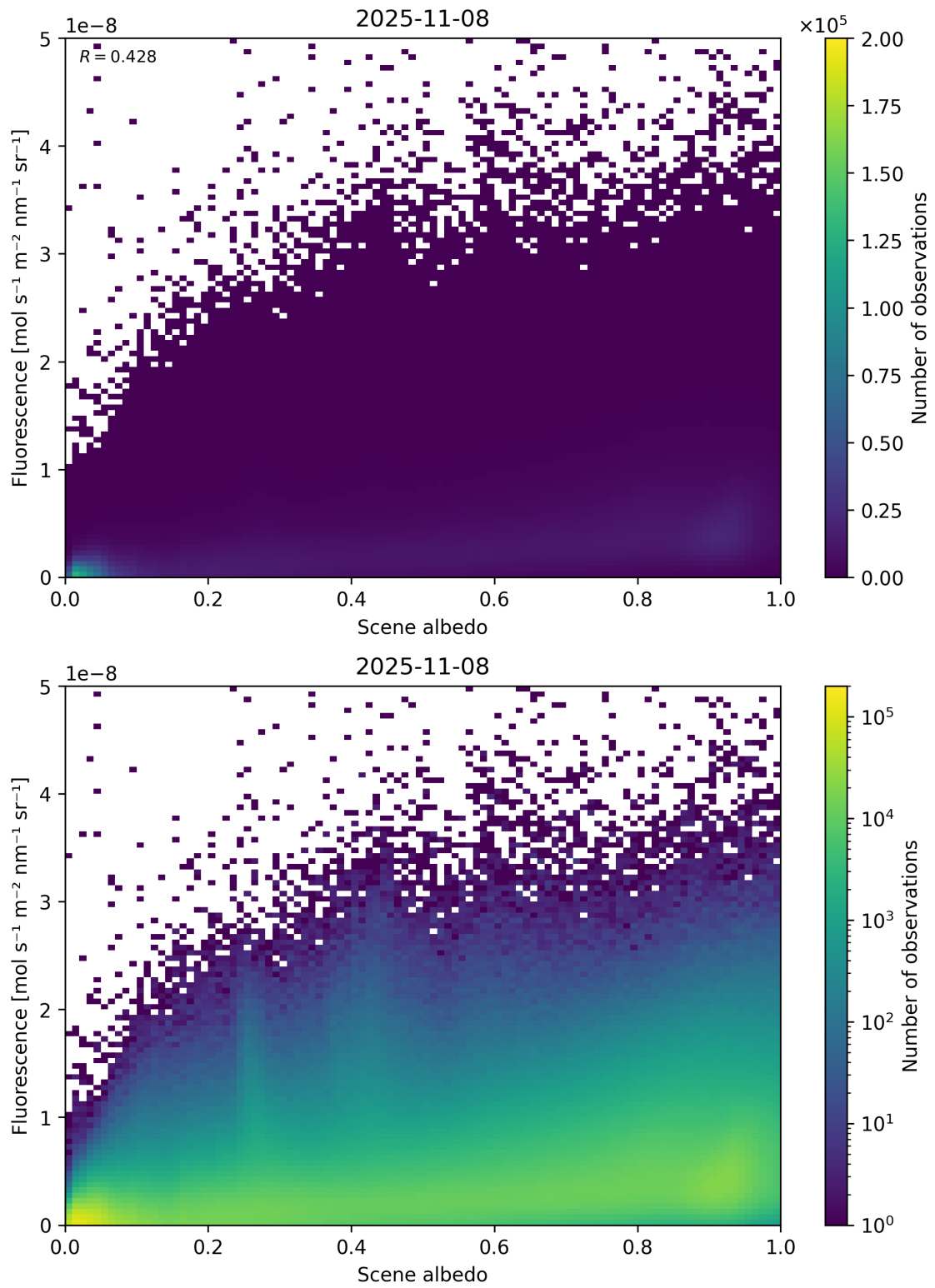
Figure 104: Scatter density plot of “Scene albedo” against “Fluorescence” for 2025-11-07 to 2025-11-09.
