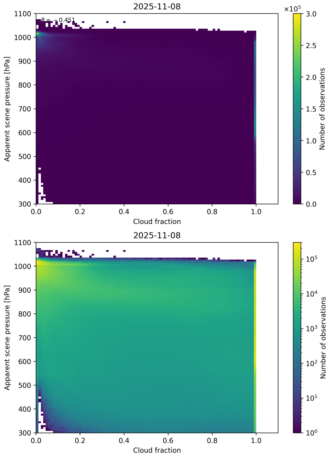
Figure 70: Scatter density plot of “Cloud fraction” against “Apparent scene pressure” for 2025-11-07 to 2025-11-09.
