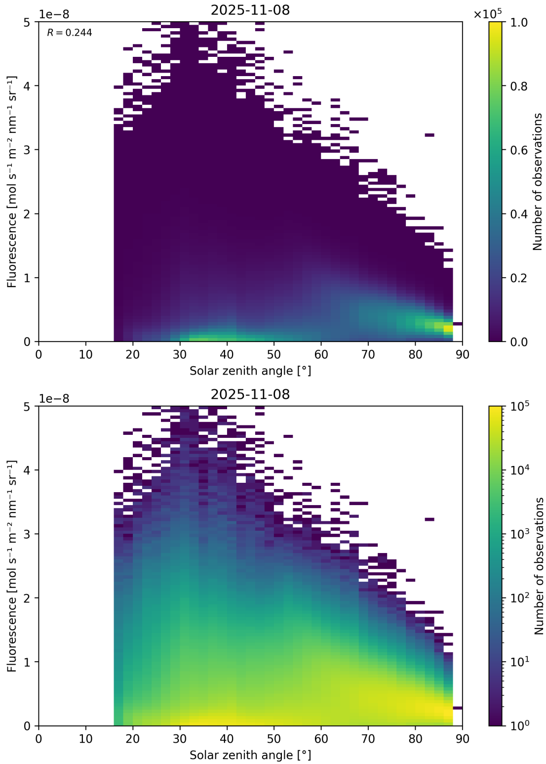
Figure 112: Scatter density plot of “Solar zenith angle” against “Fluorescence” for 2025-11-07 to 2025-11-09.
