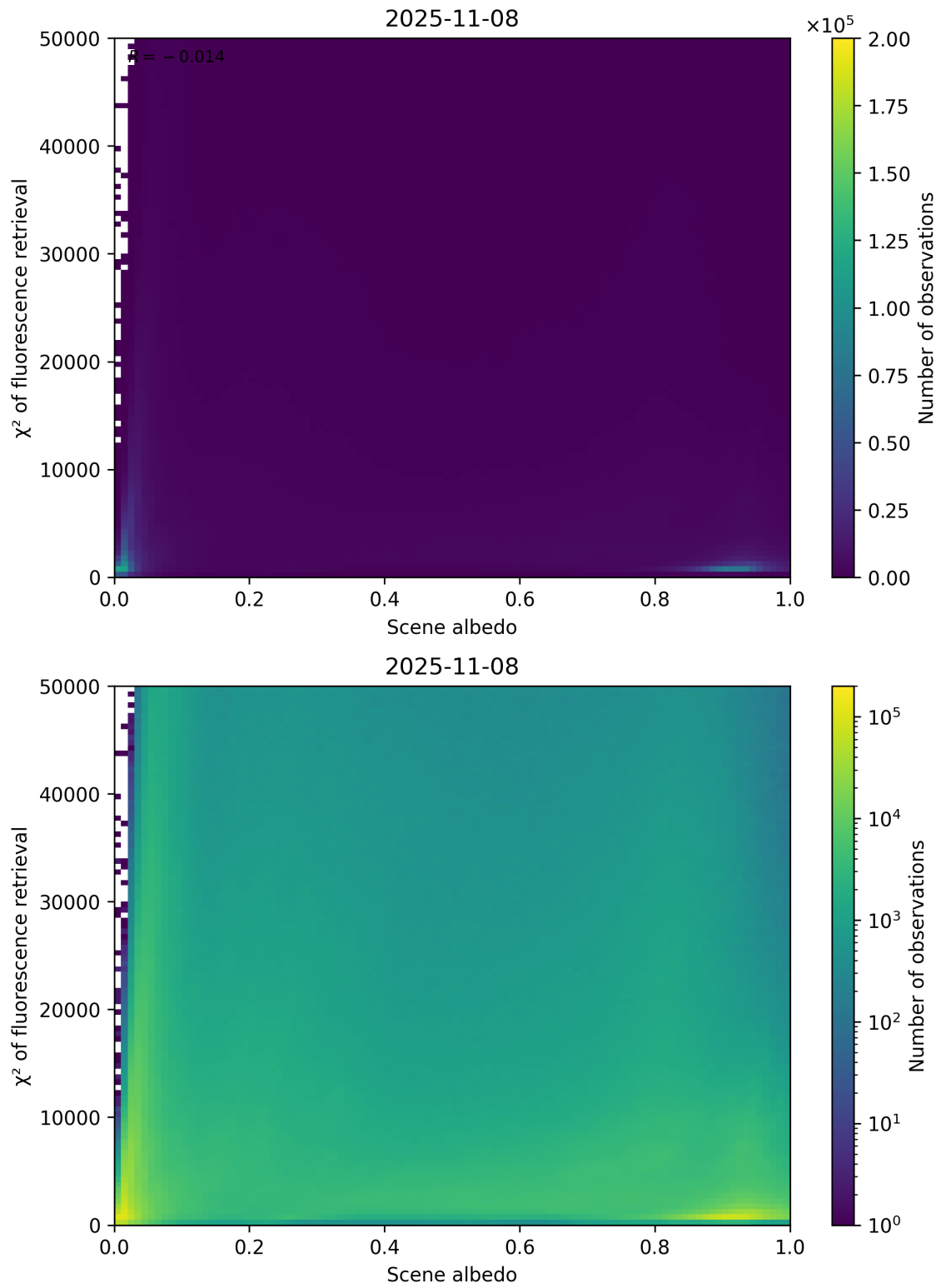
Figure 103: Scatter density plot of “Scene albedo” against “ \chi^2 of fluorescence retrieval” for 2025-11-07 to 2025-11-09.
