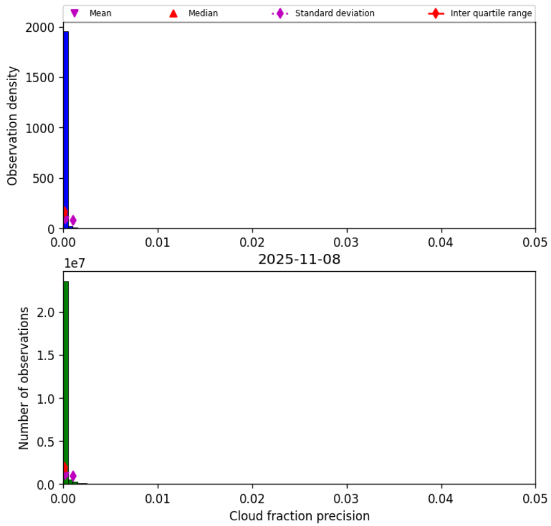
Figure 33: Histogram of “Cloud fraction precision” for 2025-11-07 to 2025-11-09
