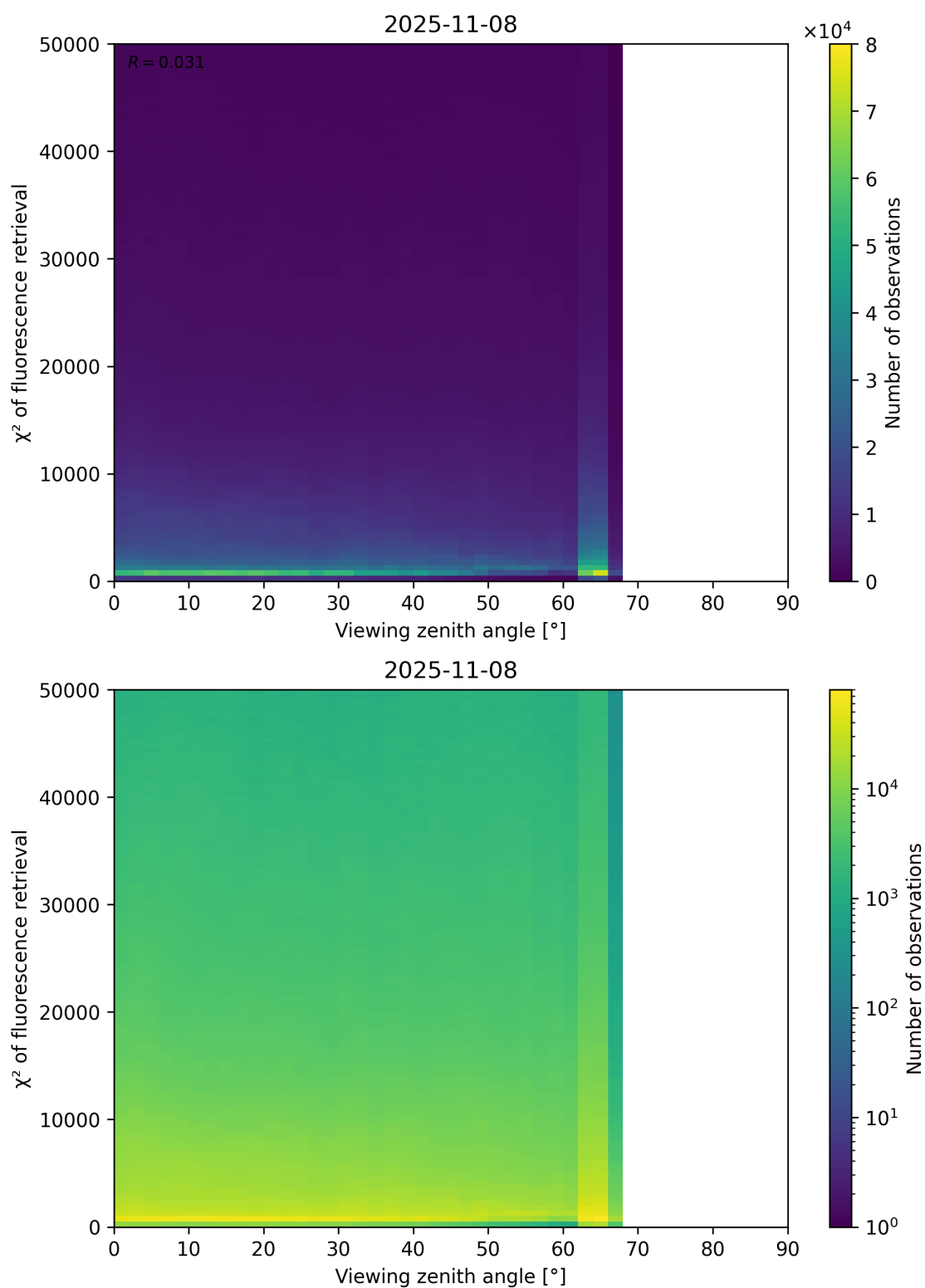
Figure 119: Scatter density plot of “Viewing zenith angle” against “ \chi^2 of fluorescence retrieval” for 2025-11-07 to 2025-11-09.
