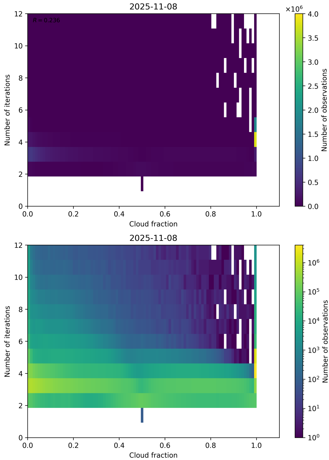
Figure 73: Scatter density plot of “Cloud fraction” against “Number of iterations” for 2025-11-07 to 2025-11-09.
