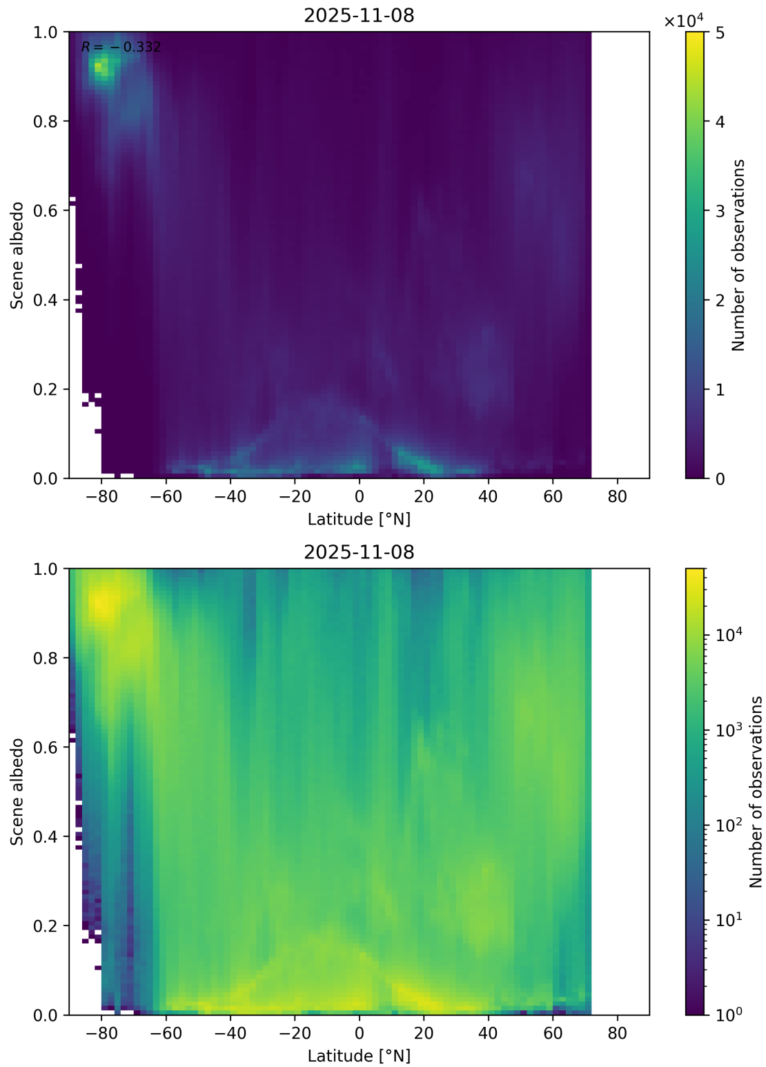
Figure 95: Scatter density plot of “Latitude” against “Scene albedo” for 2025-11-07 to 2025-11-09.
