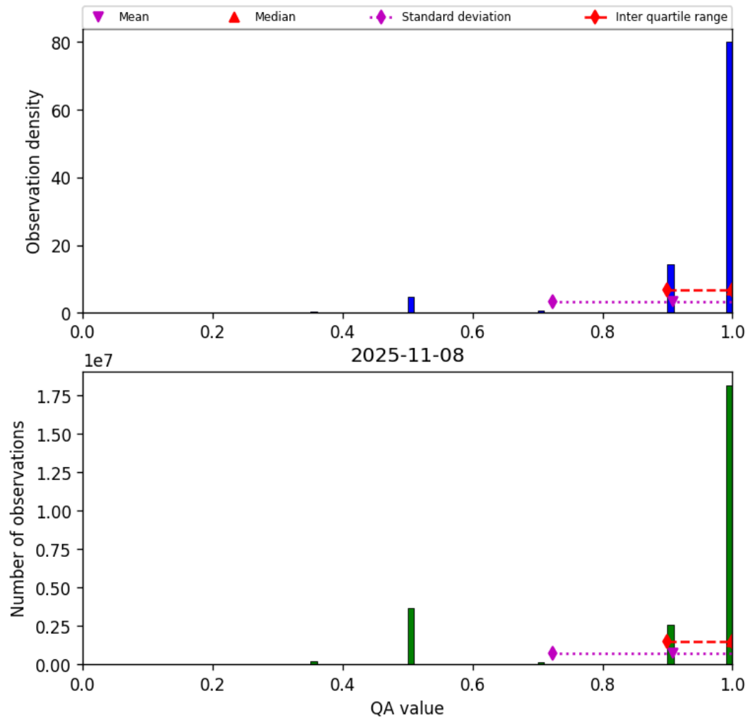
Figure 29: Histogram of “QA value” for 2025-11-07 to 2025-11-09
