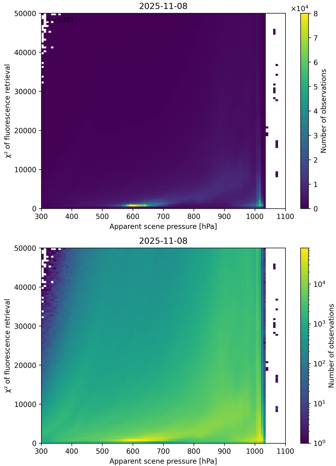
Figure 63: Scatter density plot of “Apparent scene pressure” against “ \chi^2 of fluorescence retrieval” for 2025-11-07 to 2025-11-09.
