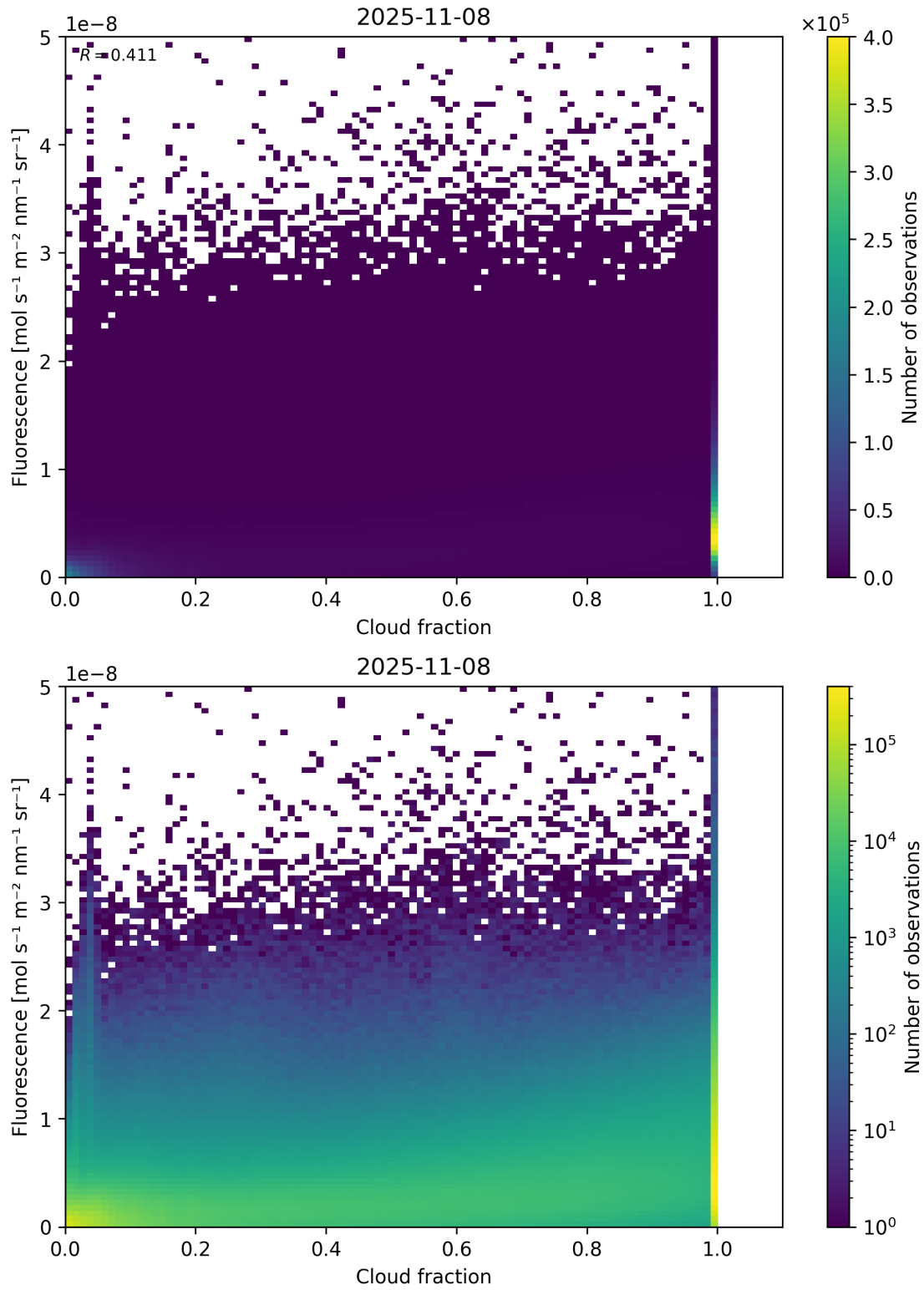
Figure 72: Scatter density plot of “Cloud fraction” against “Fluorescence” for 2025-11-07 to 2025-11-09.
