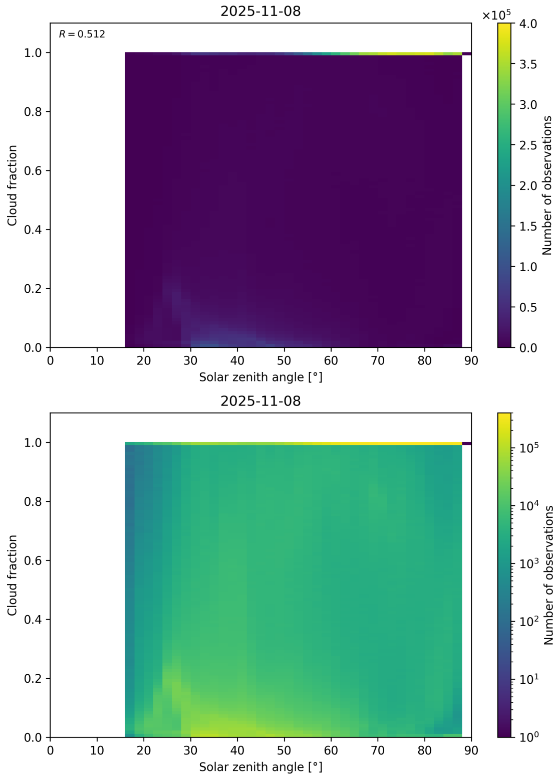
Figure 110: Scatter density plot of “Solar zenith angle” against “Cloud fraction” for 2025-11-07 to 2025-11-09.
