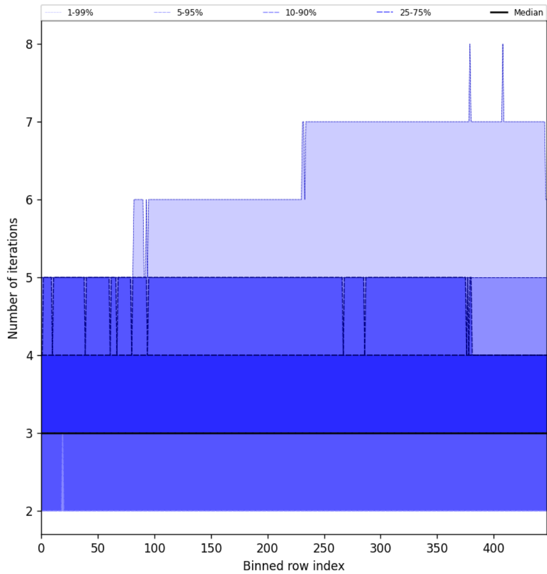
Figure 56: Along track statistics of “Number of iterations” for 2025-11-07 to 2025-11-09
