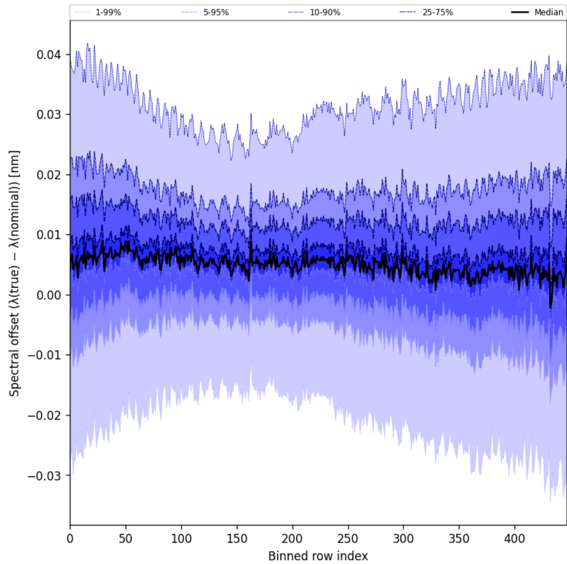
Figure 62: Along track statistics of “Spectral offset ( \lambda_{\text{true}} - \lambda_{\text{nominal}} )” for 2025-11-07 to 2025-11-09
