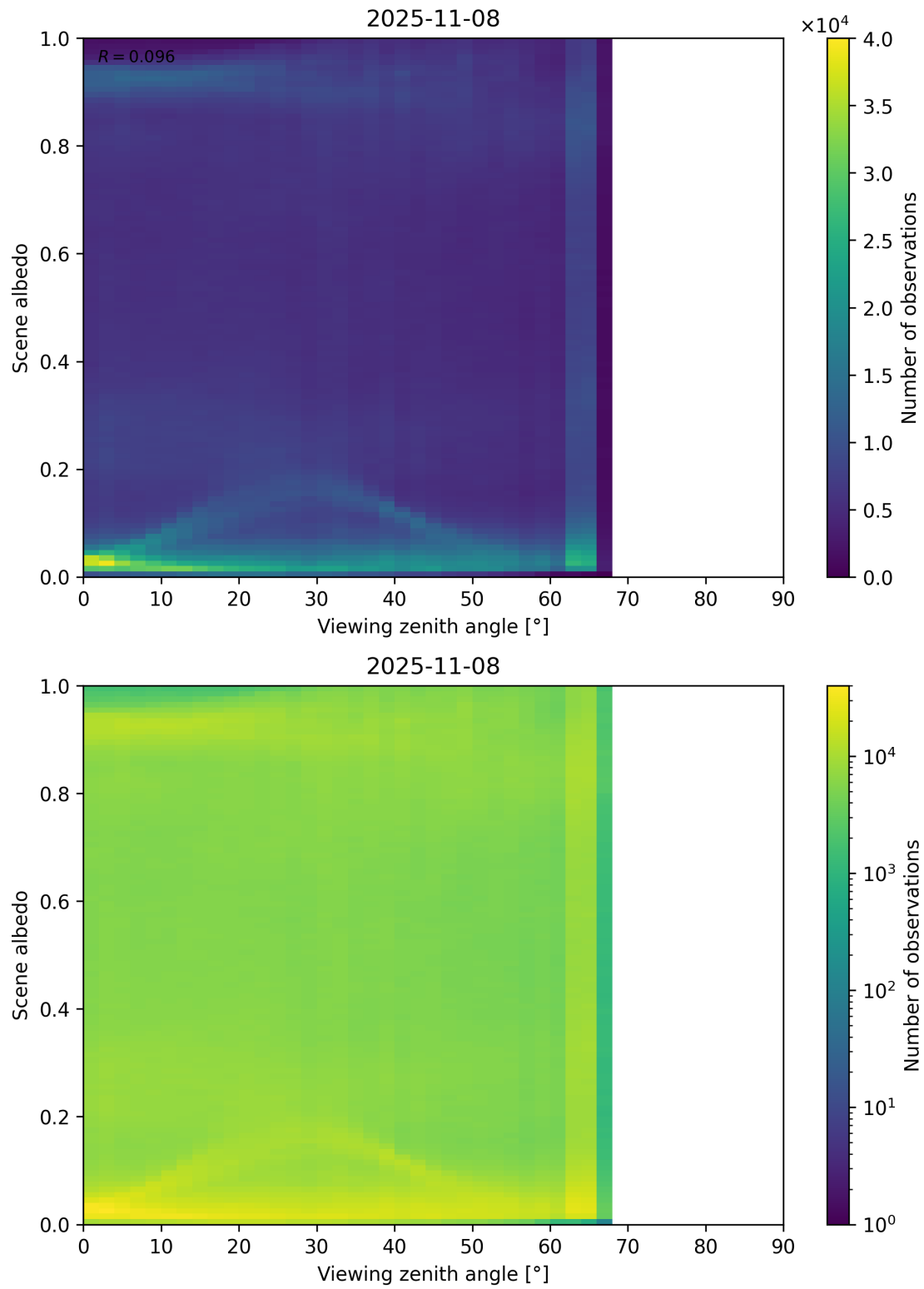
Figure 126: Scatter density plot of “Viewing zenith angle” against “Scene albedo” for 2025-11-07 to 2025-11-09.
