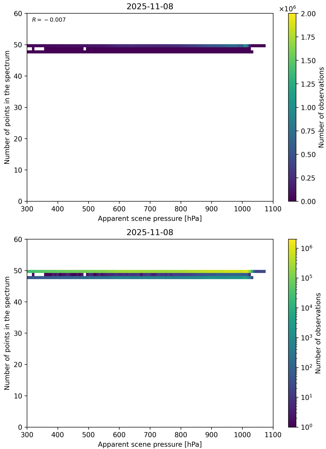
Figure 66: Scatter density plot of “Apparent scene pressure” against “Number of points in the spectrum” for 2025-11-07 to 2025-11-09.
