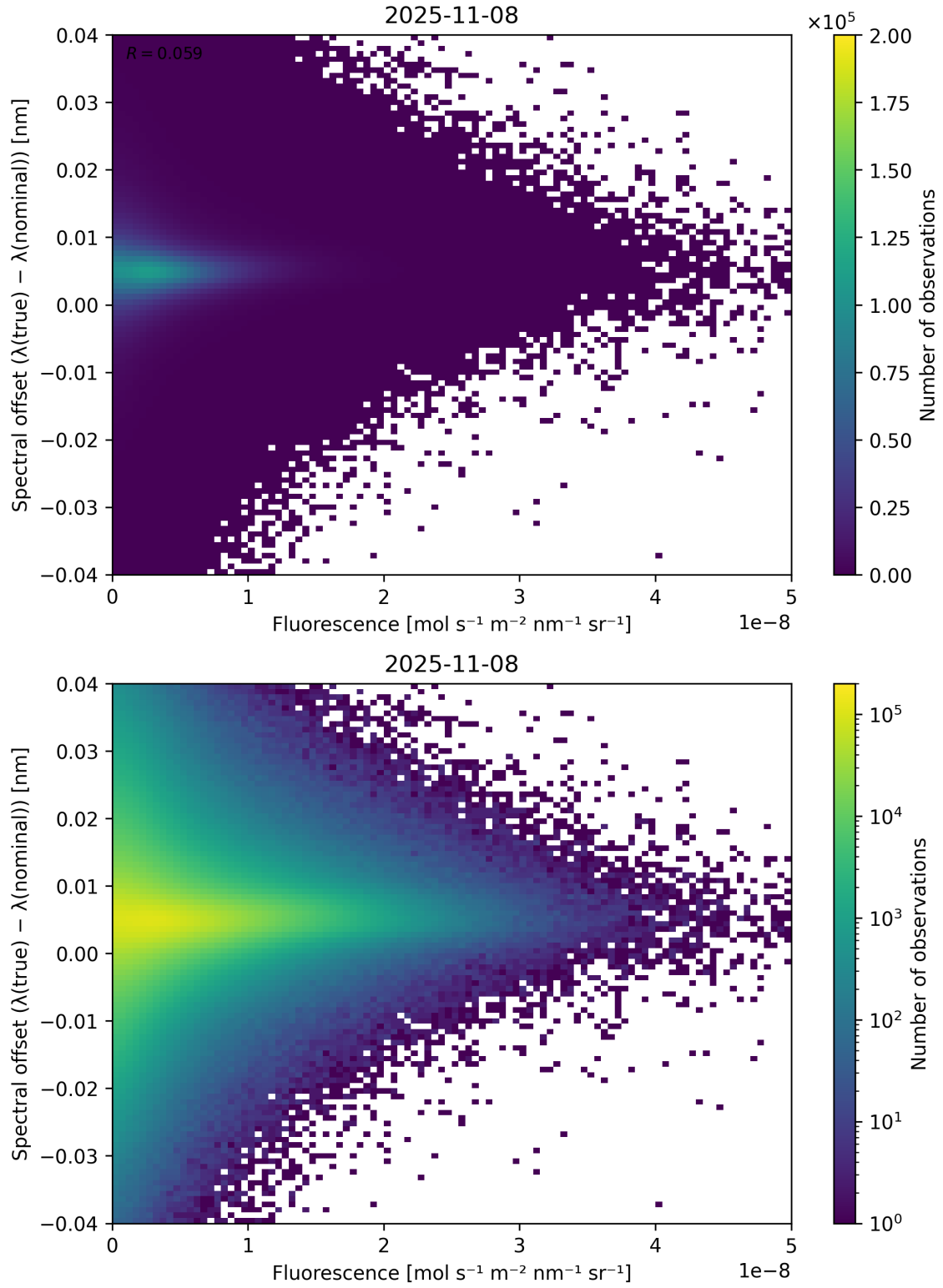
Figure 87: Scatter density plot of “Fluorescence” against “Spectral offset ( \lambda_{\text{true}} - \lambda_{\text{nominal}} )” for 2025-11-07 to 2025-11-09.
