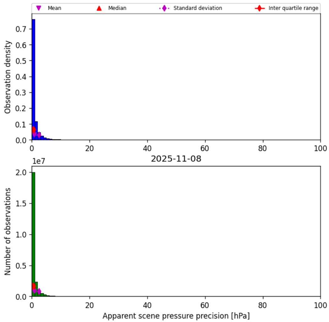
Figure 37: Histogram of “Apparent scene pressure precision” for 2025-11-07 to 2025-11-09
