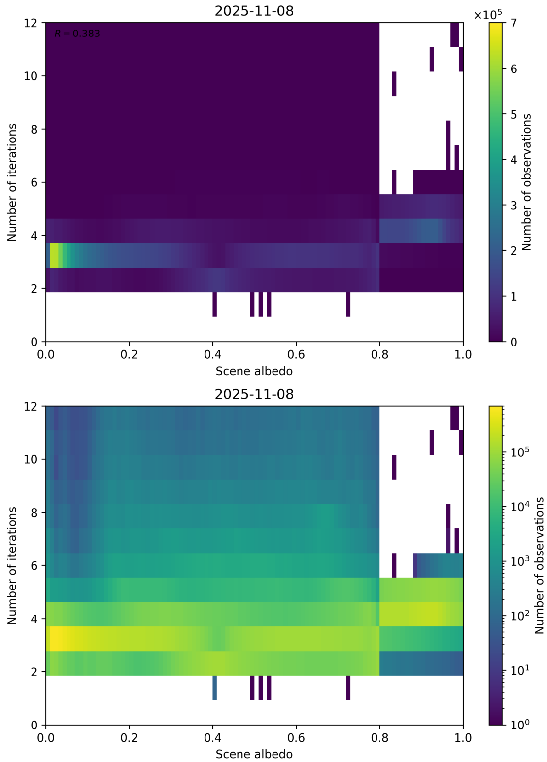
Figure 105: Scatter density plot of “Scene albedo” against “Number of iterations” for 2025-11-07 to 2025-11-09.
