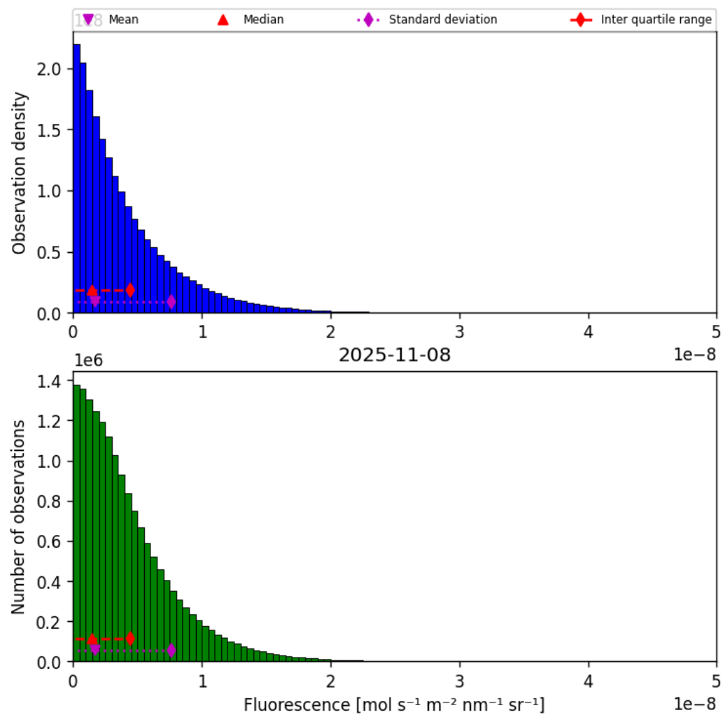
Figure 40: Histogram of “Fluorescence” for 2025-11-07 to 2025-11-09
