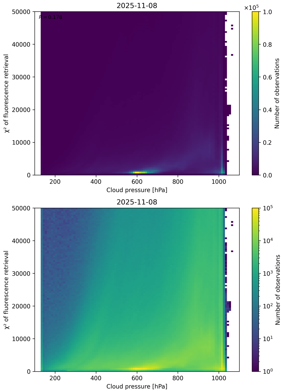
Figure 78: Scatter density plot of “Cloud pressure” against “ \chi^2 of fluorescence retrieval” for 2025-11-07 to 2025-11-09.
