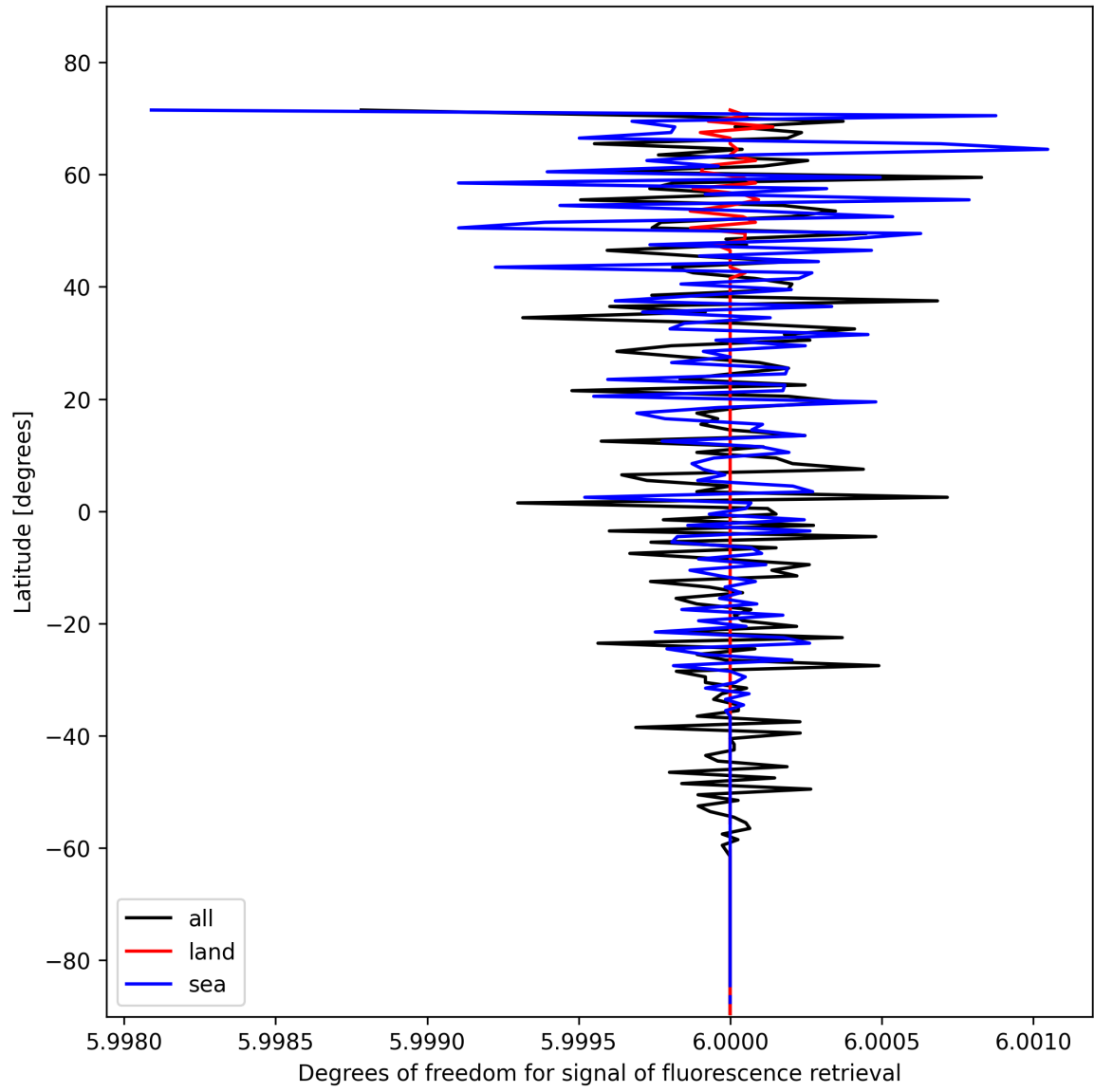
Figure 26: Zonal average of “Degrees of freedom for signal of fluorescence retrieval” for 2025-11-07 to 2025-11-09.
