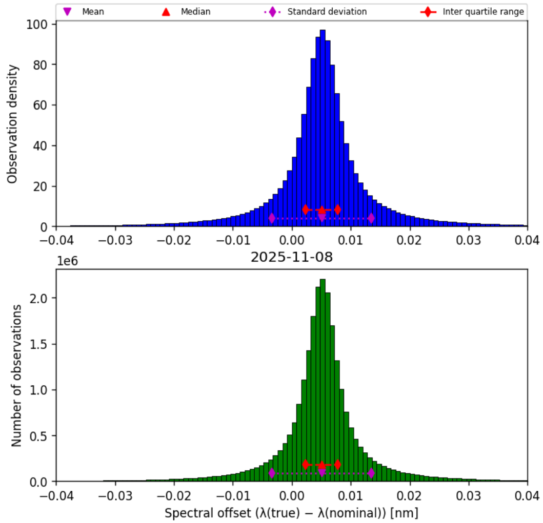
Figure 45: Histogram of “Spectral offset ( \lambda_{\text{true}} - \lambda_{\text{nominal}} )” for 2025-11-07 to 2025-11-09
