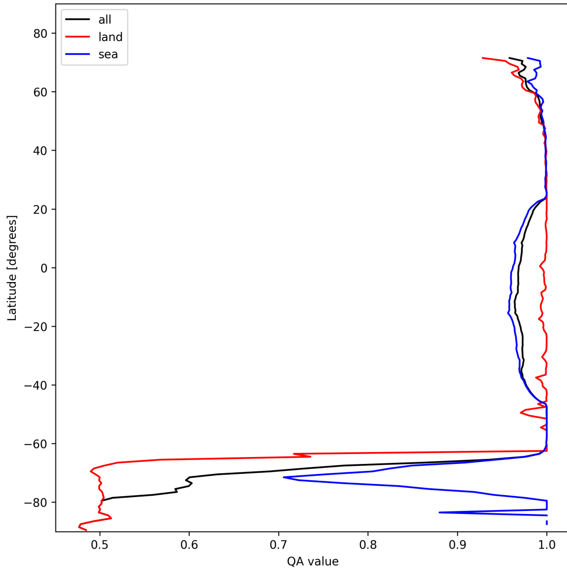
Figure 12: Zonal average of “QA value” for 2025-11-07 to 2025-11-09.
