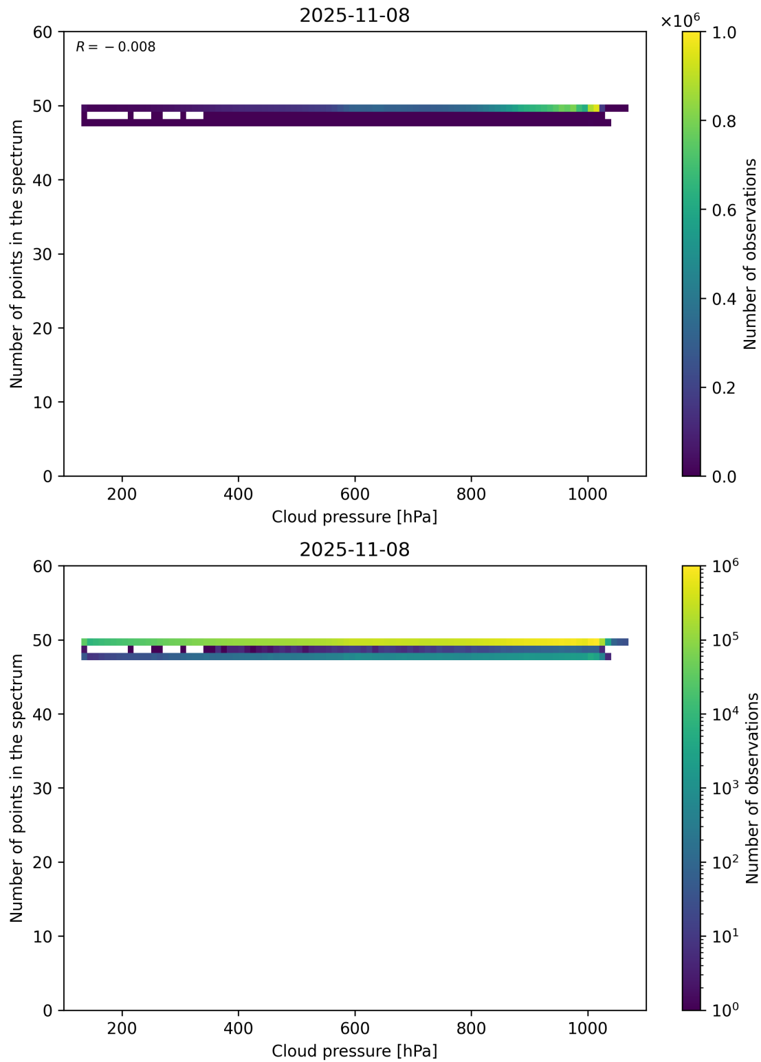
Figure 82: Scatter density plot of “Cloud pressure” against “Number of points in the spectrum” for 2025-11-07 to 2025-11-09.
