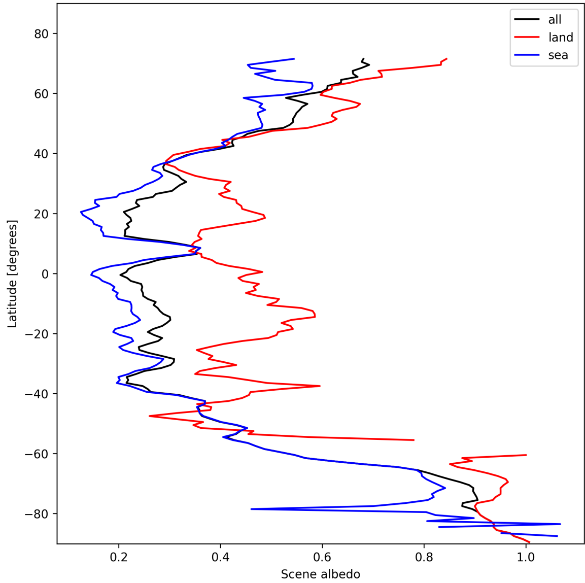
Figure 17: Zonal average of “Scene albedo” for 2025-11-07 to 2025-11-09.
