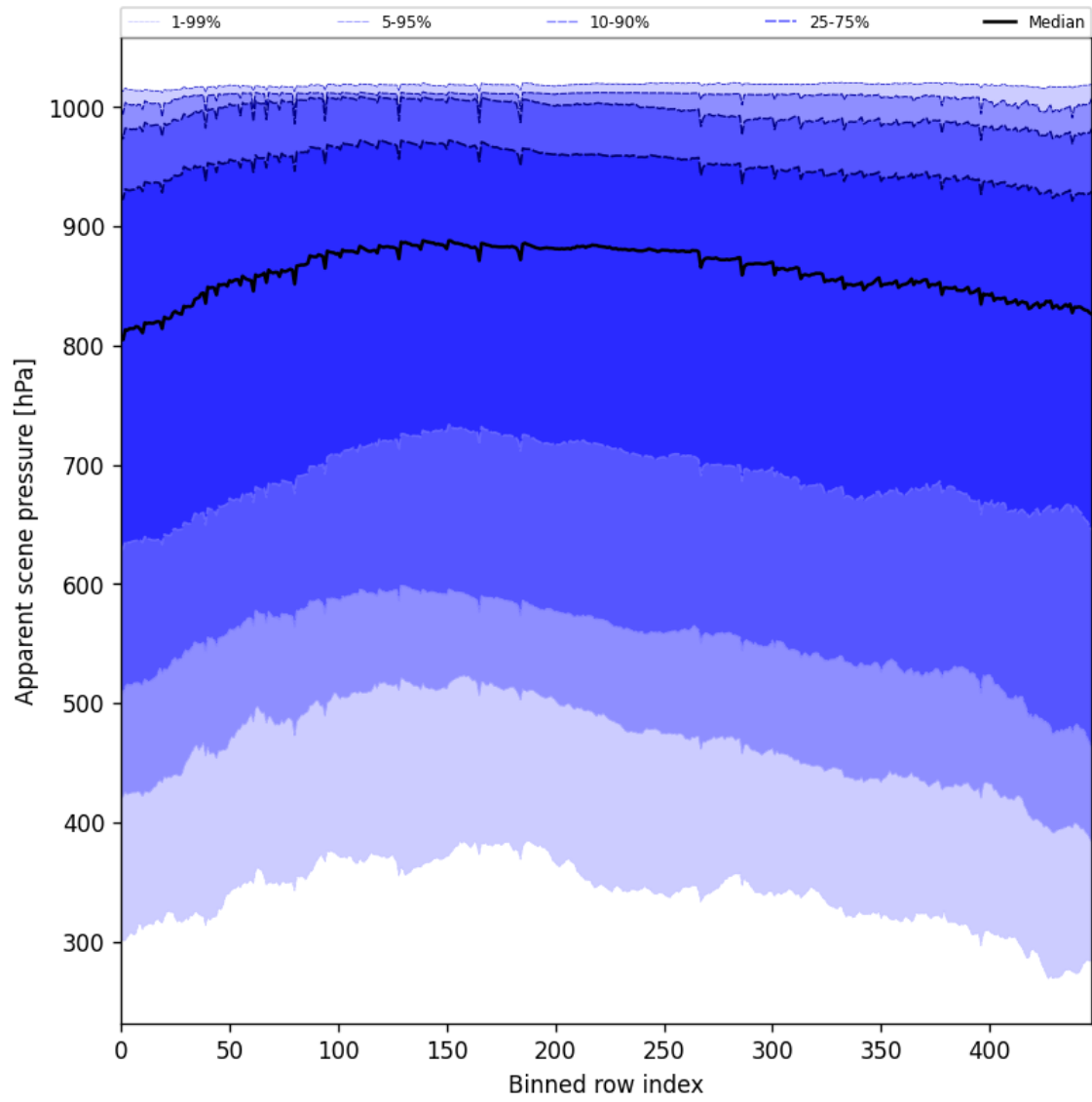
Figure 53: Along track statistics of “Apparent scene pressure” for 2025-11-07 to 2025-11-09
