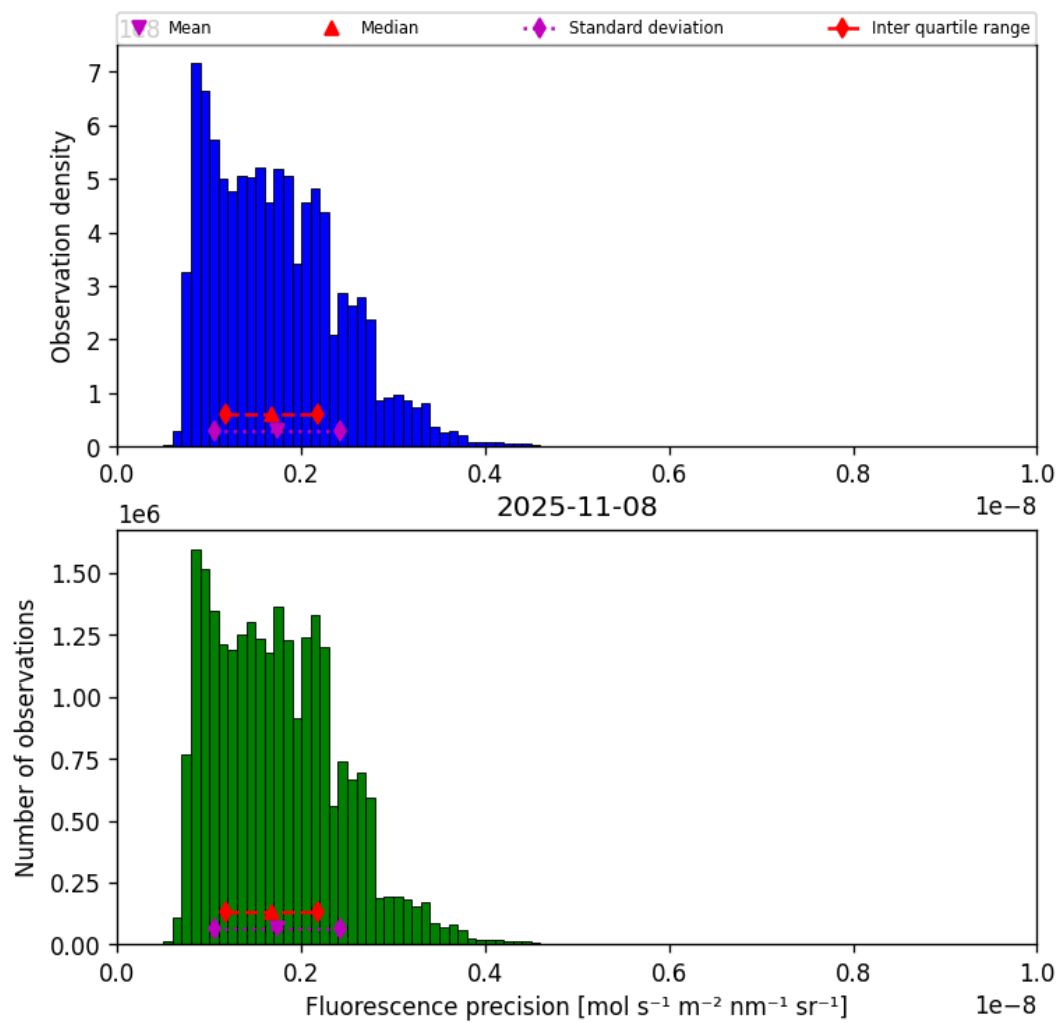
Figure 41: Histogram of “Fluorescence precision” for 2025-11-07 to 2025-11-09
