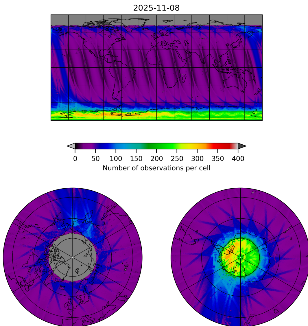
Figure 11: Map of the number of observations for 2025-11-07 to 2025-11-09
