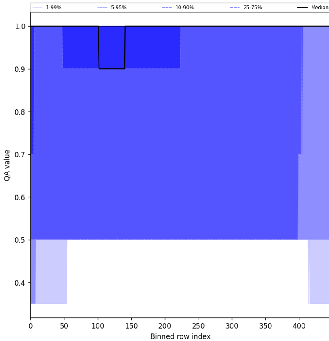
Figure 46: Along track statistics of “QA value” for 2025-11-07 to 2025-11-09
