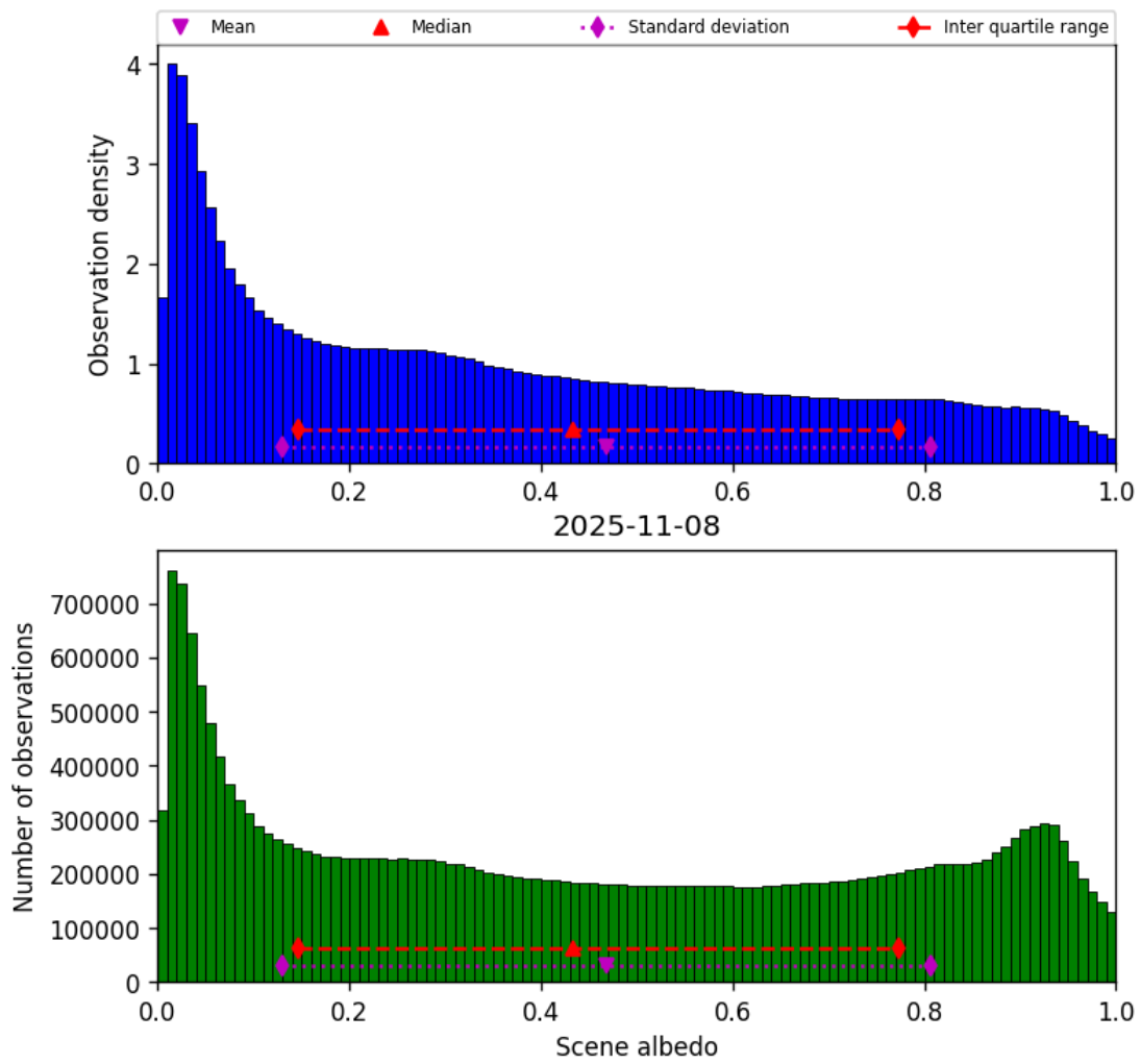
Figure 34: Histogram of “Scene albedo” for 2025-11-07 to 2025-11-09
