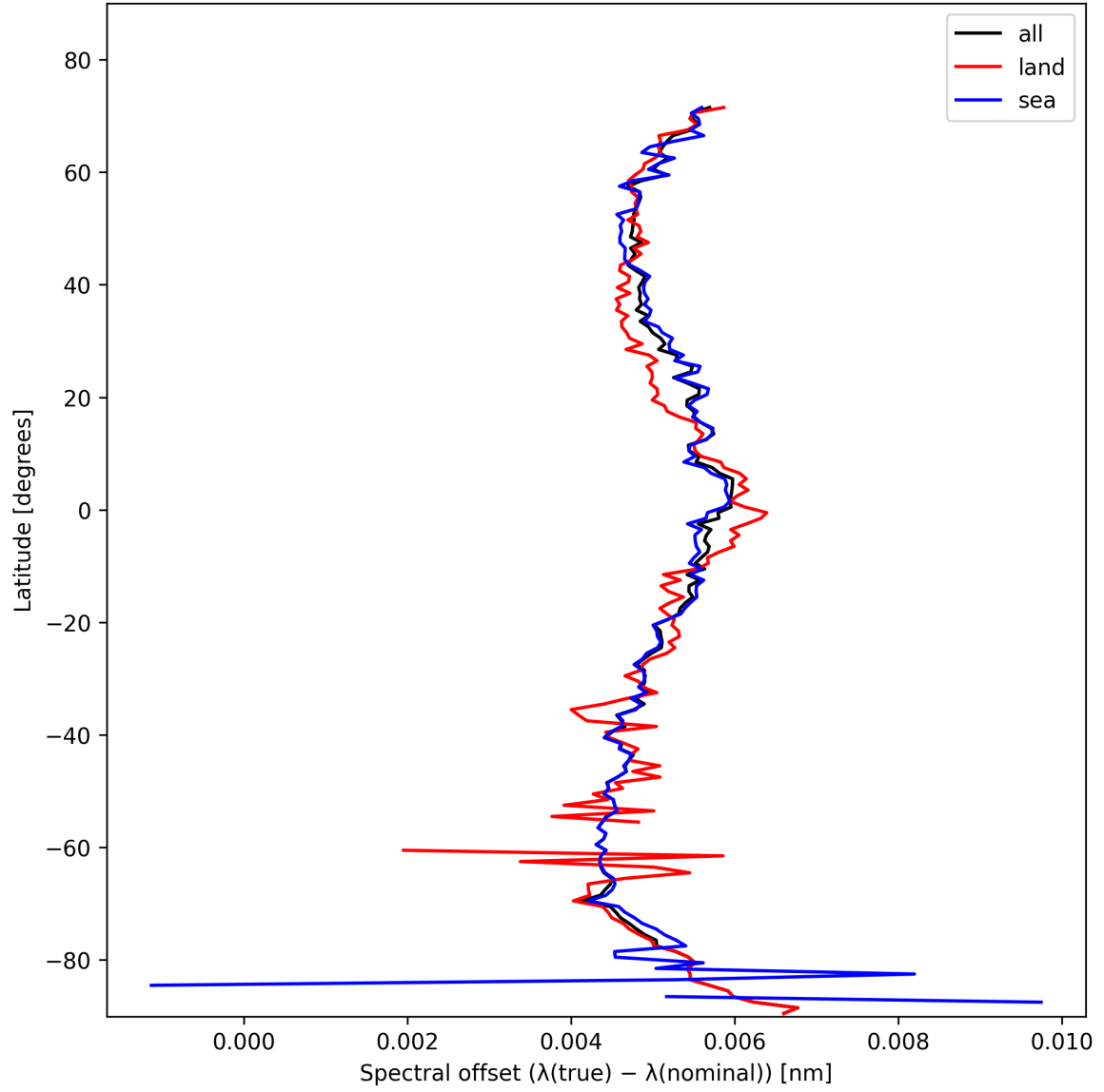
Figure 28: Zonal average of “Spectral offset ( \lambda_{\text{true}} - \lambda_{\text{nominal}} )” for 2025-11-07 to 2025-11-09.
