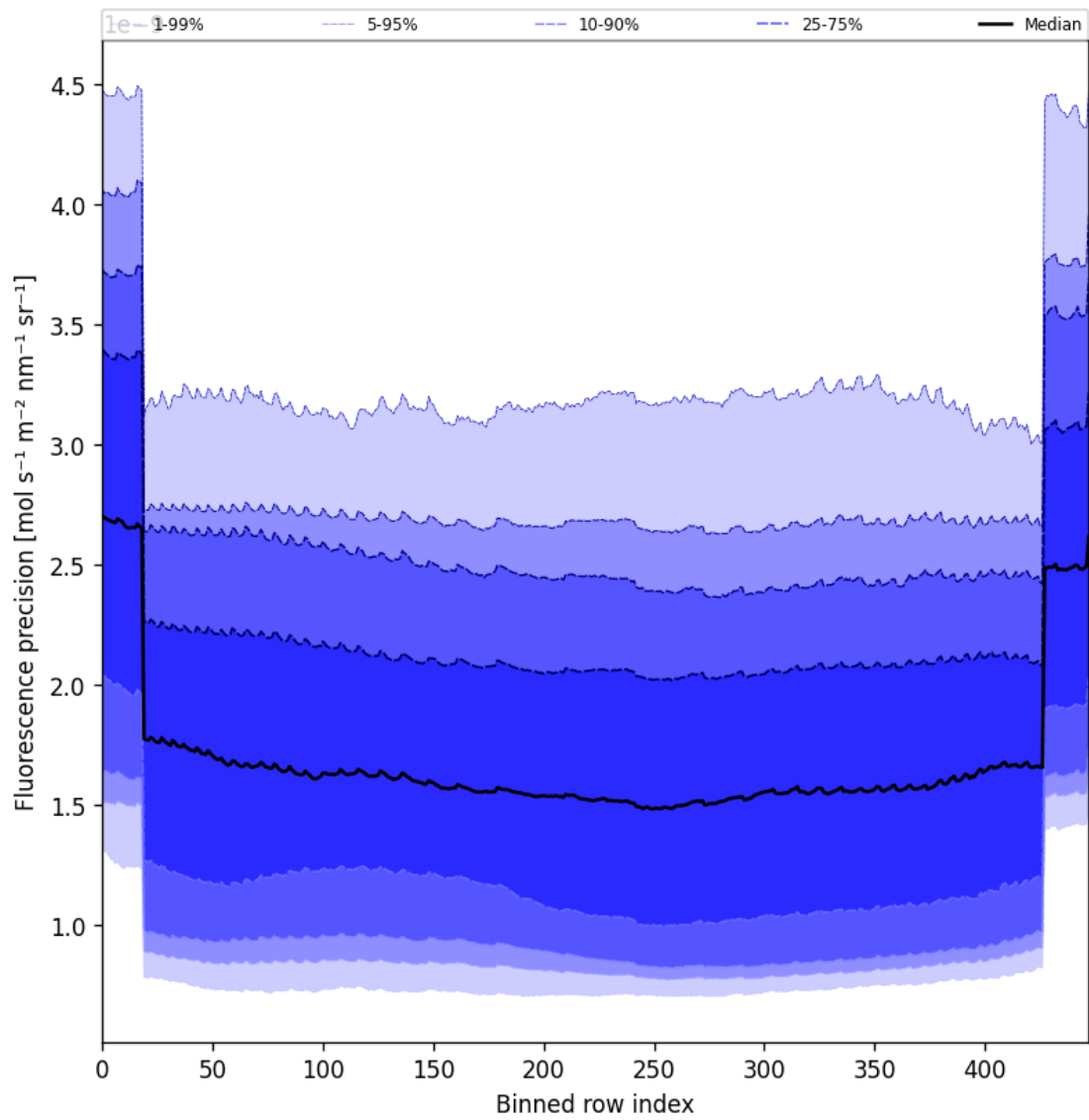
Figure 58: Along track statistics of “Fluorescence precision” for 2025-11-07 to 2025-11-09
