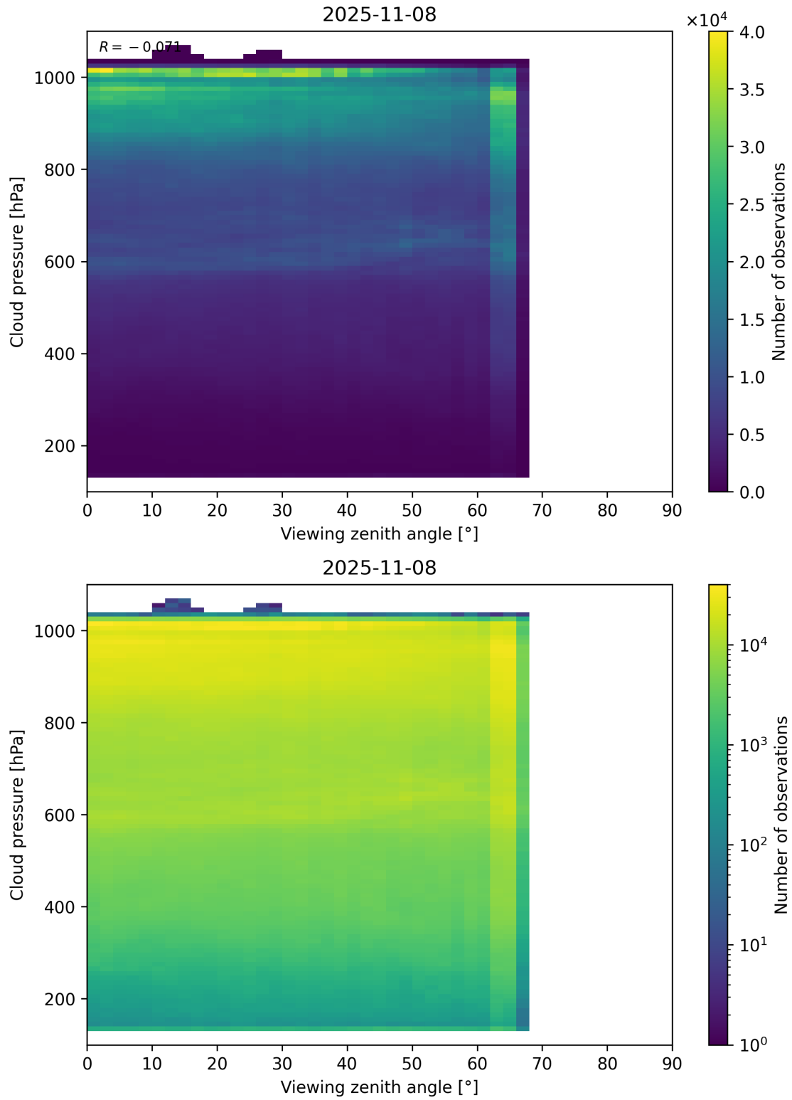
Figure 121: Scatter density plot of “Viewing zenith angle” against “Cloud pressure” for 2025-11-07 to 2025-11-09.
