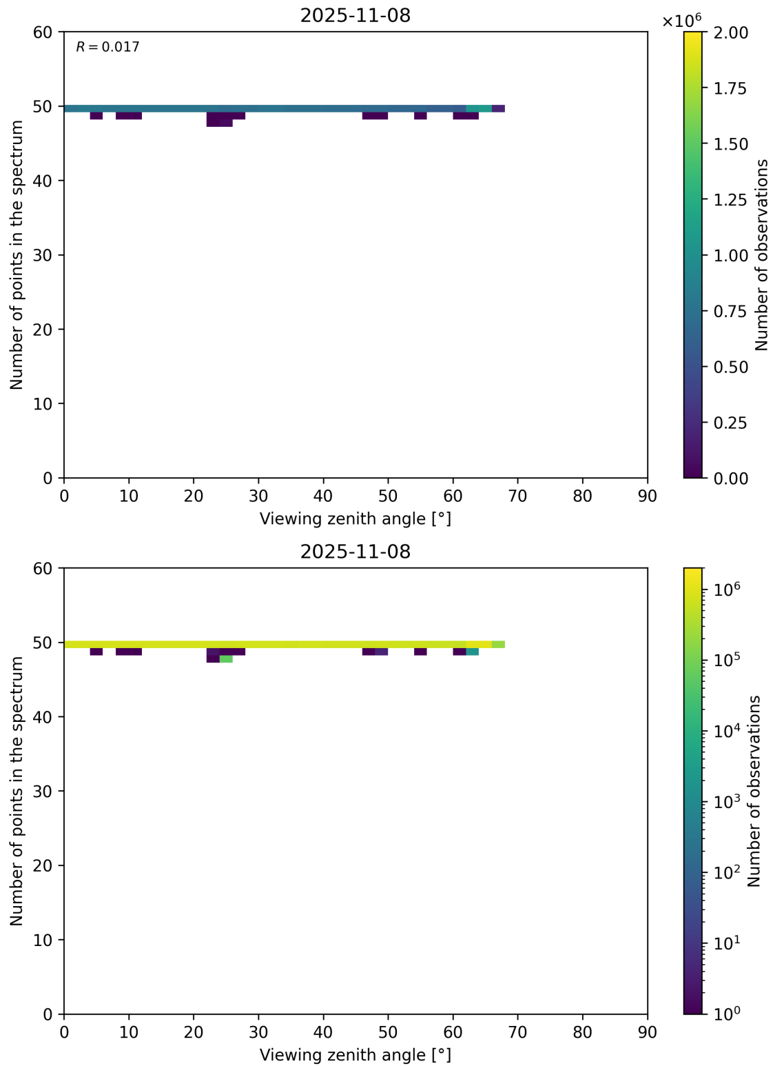
Figure 125: Scatter density plot of “Viewing zenith angle” against “Number of points in the spectrum” for 2025-11-07 to 2025-11-09.
