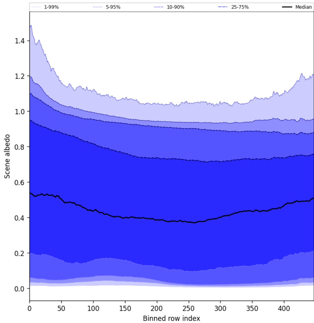
Figure 51: Along track statistics of “Scene albedo” for 2025-11-07 to 2025-11-09
