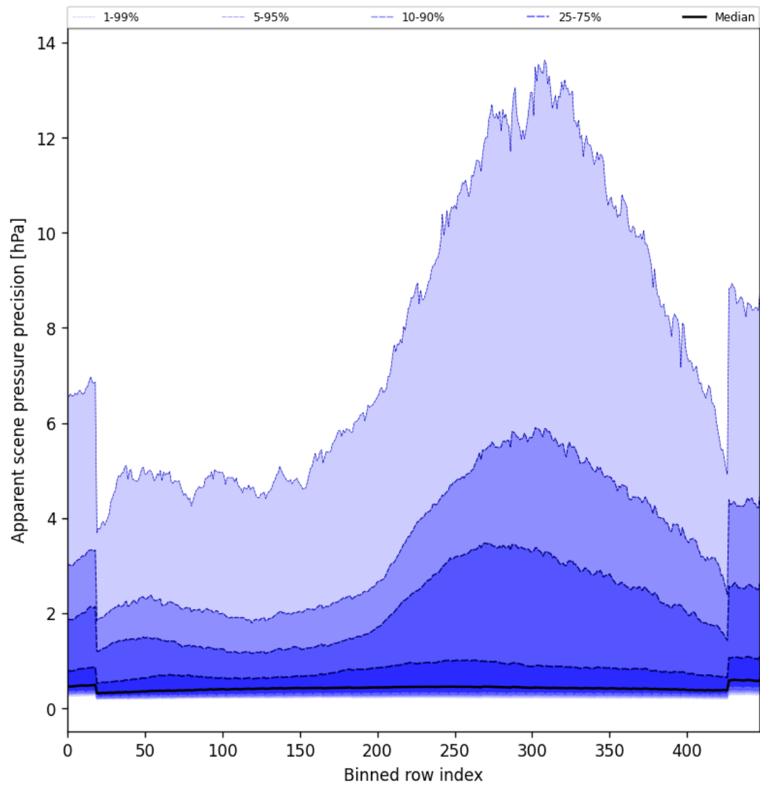
Figure 54: Along track statistics of “Apparent scene pressure precision” for 2025-11-07 to 2025-11-09
