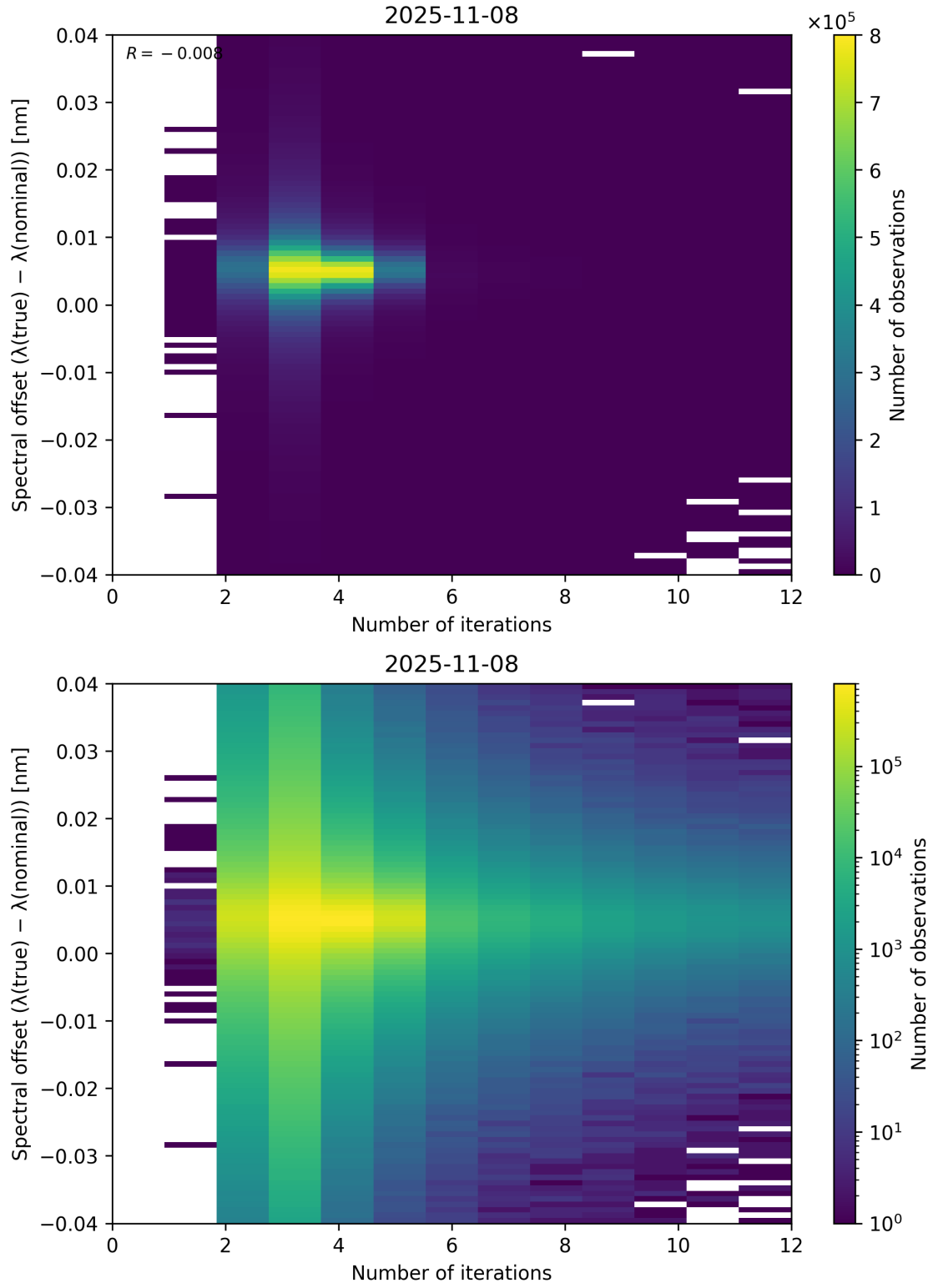
Figure 100: Scatter density plot of “Number of iterations” against “Spectral offset ( \lambda_{\text{true}} - \lambda_{\text{nominal}} )” for 2025-11-07 to 2025-11-09.
