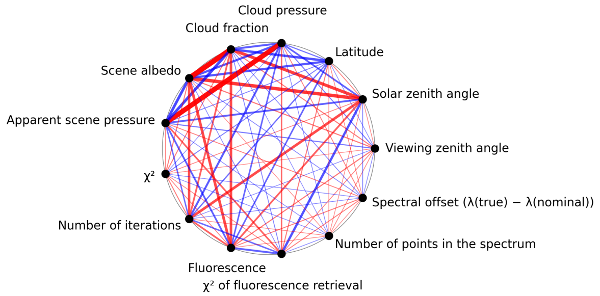
Figure 1: Map of correlation graph for 2025-11-07 to 2025-11-09.
