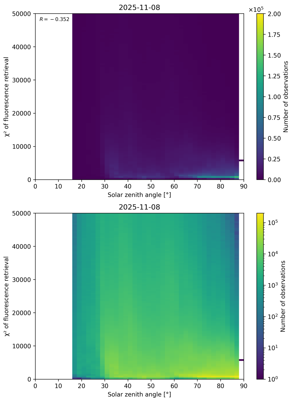
Figure 109: Scatter density plot of “Solar zenith angle” against “ \chi^2 of fluorescence retrieval” for 2025-11-07 to 2025-11-09.
