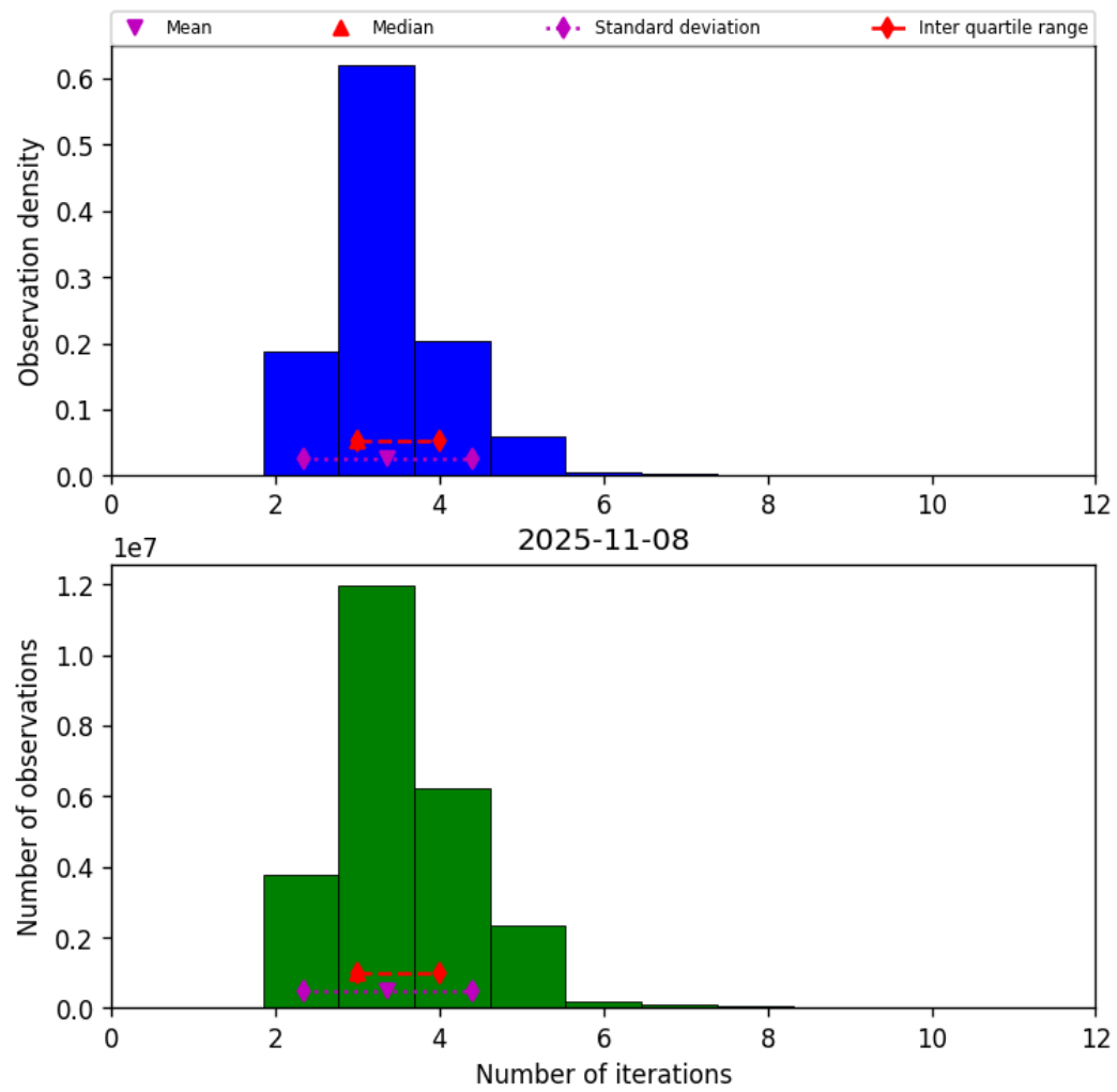
Figure 39: Histogram of “Number of iterations” for 2025-11-07 to 2025-11-09
