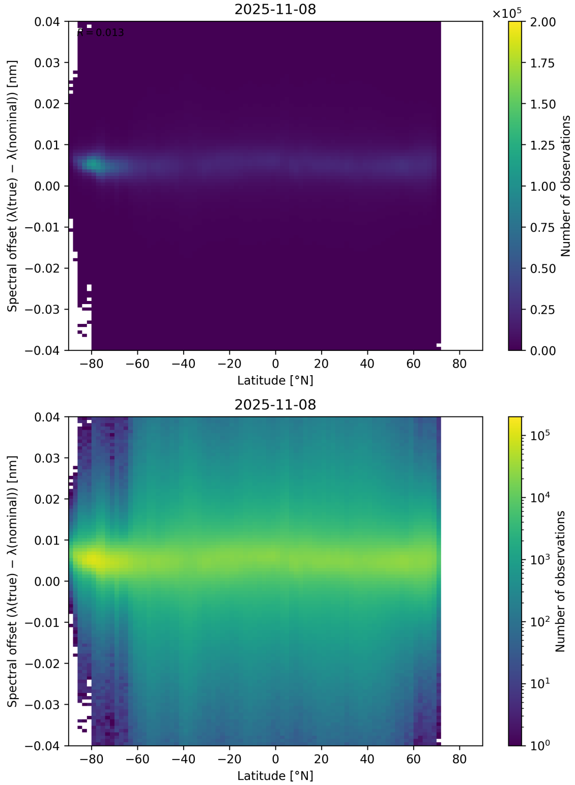
Figure 96: Scatter density plot of “Latitude” against “Spectral offset ( \lambda_{\text{true}} - \lambda_{\text{nominal}} )” for 2025-11-07 to 2025-11-09.
