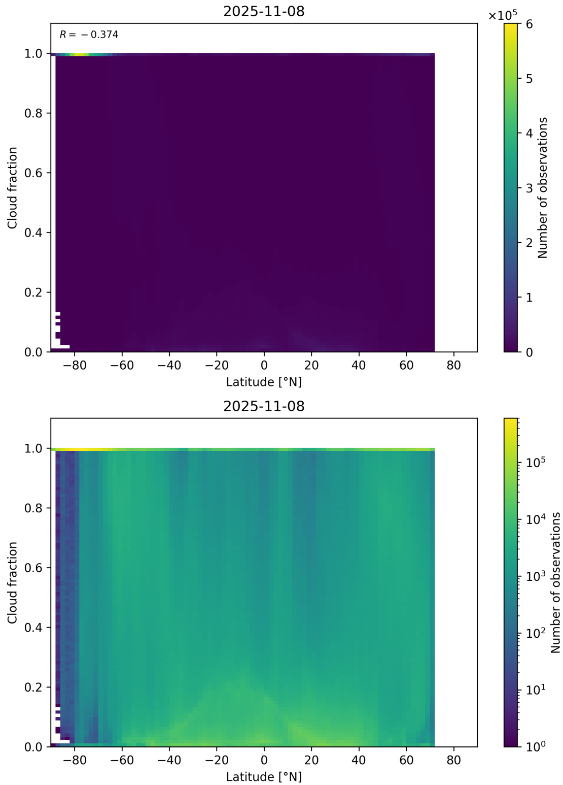
Figure 90: Scatter density plot of “Latitude” against “Cloud fraction” for 2025-11-07 to 2025-11-09.
