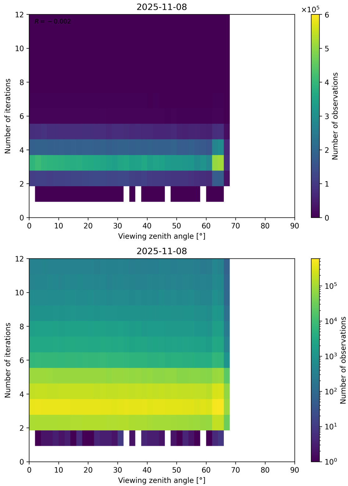
Figure 124: Scatter density plot of “Viewing zenith angle” against “Number of iterations” for 2025-11-07 to 2025-11-09.
