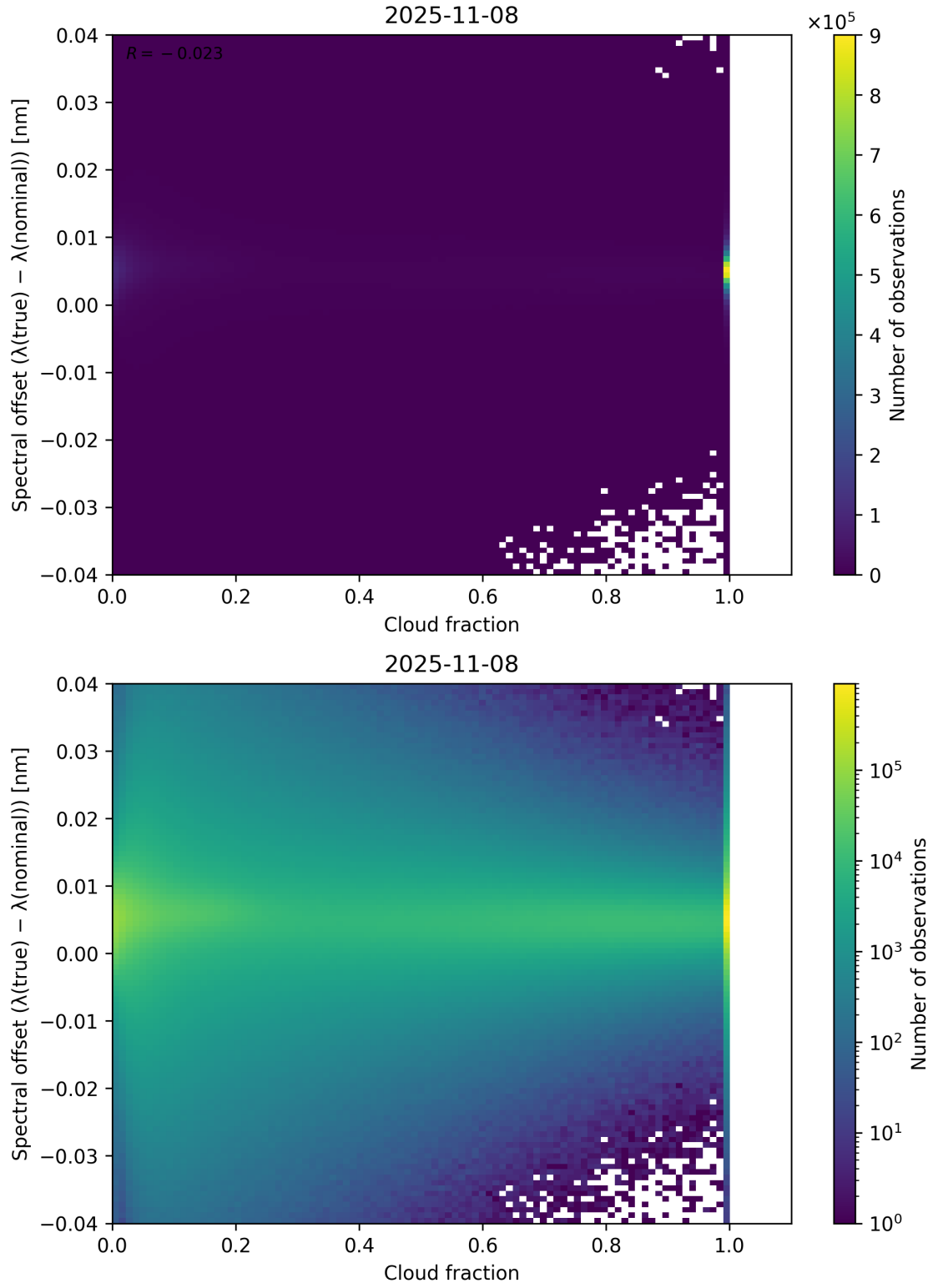
Figure 76: Scatter density plot of “Cloud fraction” against “Spectral offset ( \lambda_{\text{true}} - \lambda_{\text{nominal}} )” for 2025-11-07 to 2025-11-09.
