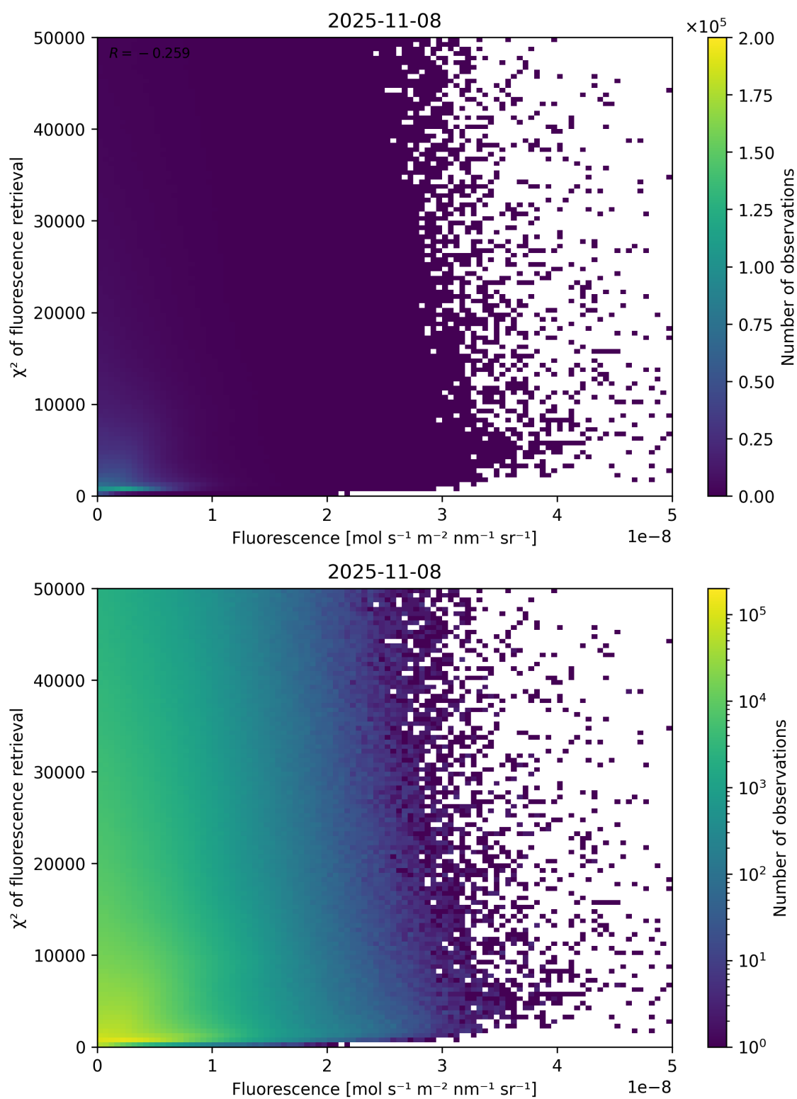
Figure 85: Scatter density plot of “Fluorescence” against “ \chi^2 of fluorescence retrieval” for 2025-11-07 to 2025-11-09.
