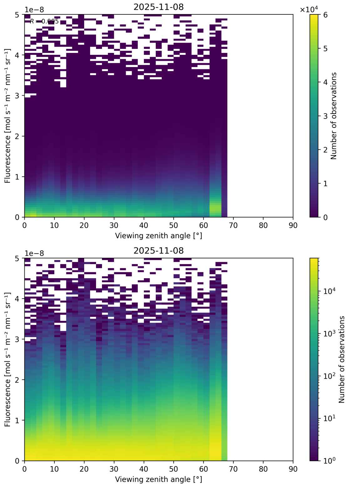
Figure 122: Scatter density plot of “Viewing zenith angle” against “Fluorescence” for 2025-11-07 to 2025-11-09.
