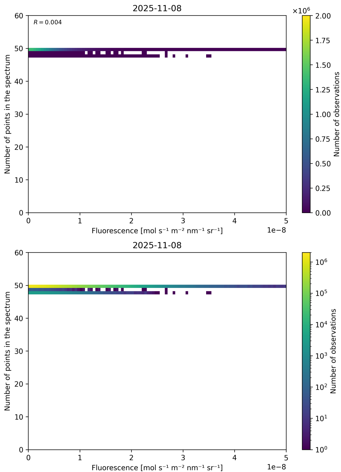
Figure 86: Scatter density plot of “Fluorescence” against “Number of points in the spectrum” for 2025-11-07 to 2025-11-09.
