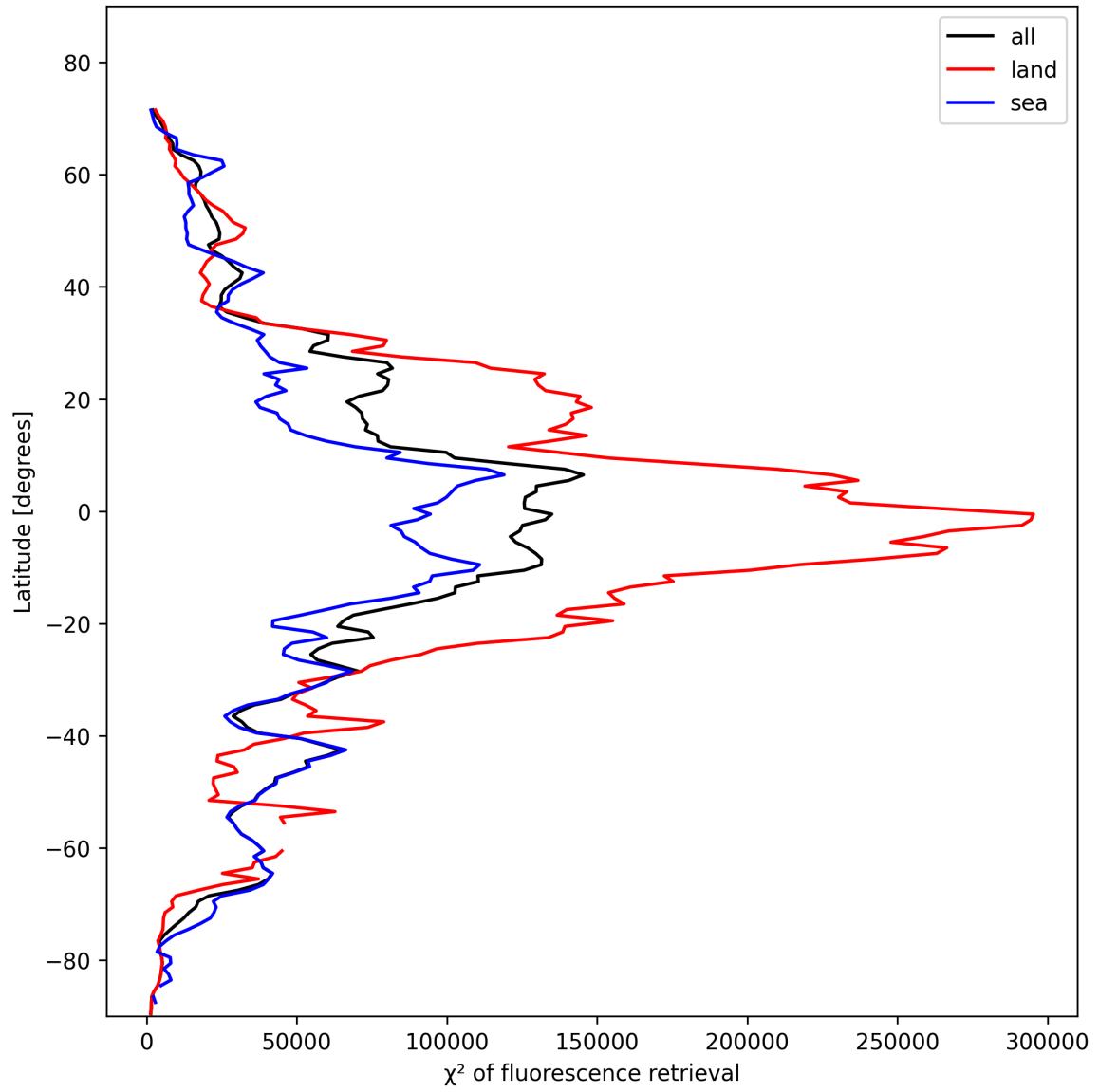
Figure 25: Zonal average of “ \chi^2 of fluorescence retrieval” for 2025-11-07 to 2025-11-09.
