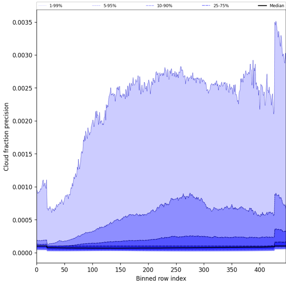
Figure 50: Along track statistics of “Cloud fraction precision” for 2025-11-08 to 2025-11-10
