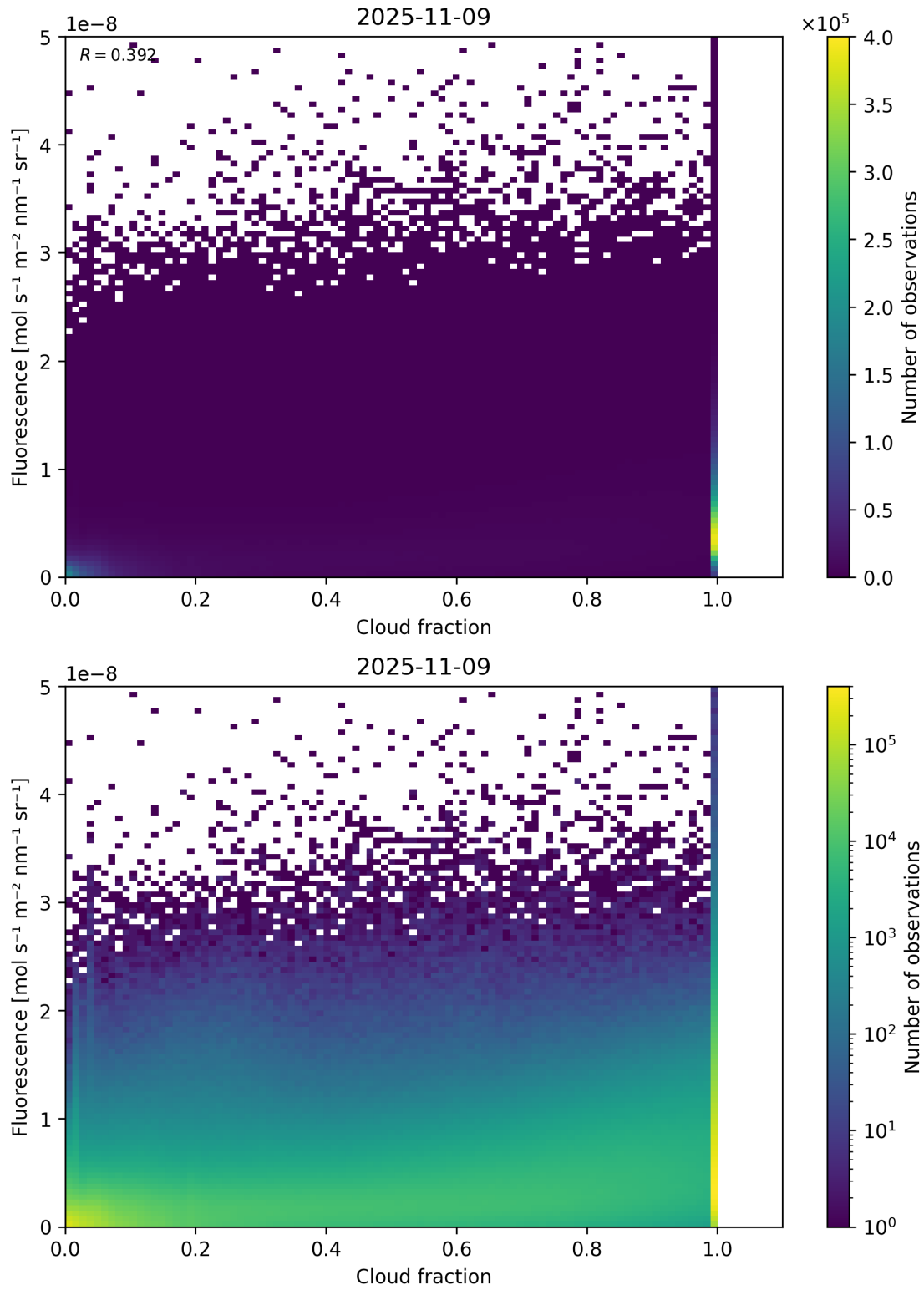
Figure 72: Scatter density plot of “Cloud fraction” against “Fluorescence” for 2025-11-08 to 2025-11-10.
