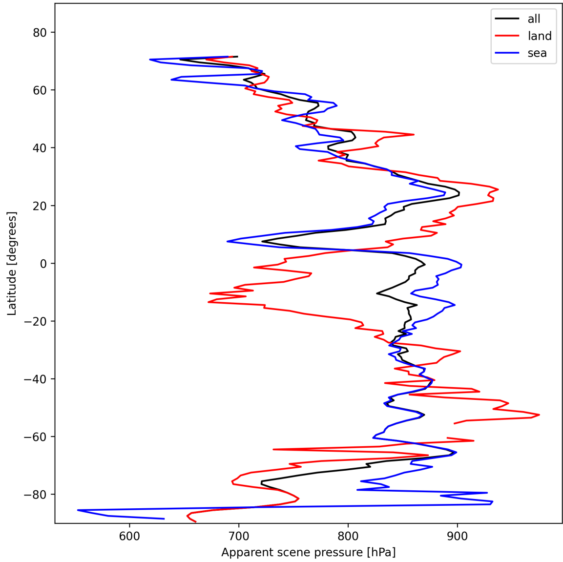
Figure 19: Zonal average of “Apparent scene pressure” for 2025-11-08 to 2025-11-10.
