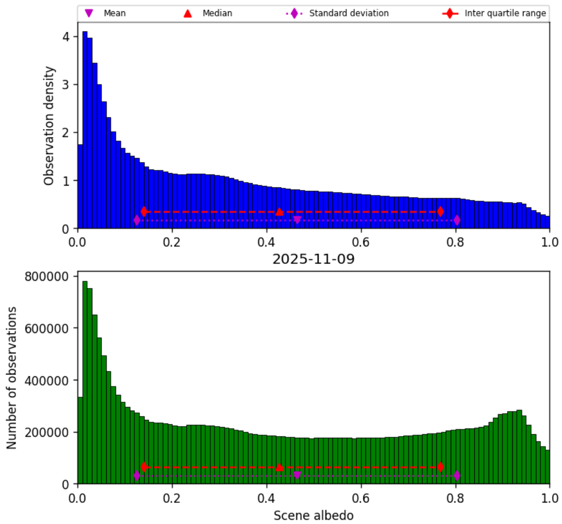
Figure 34: Histogram of “Scene albedo” for 2025-11-08 to 2025-11-10
