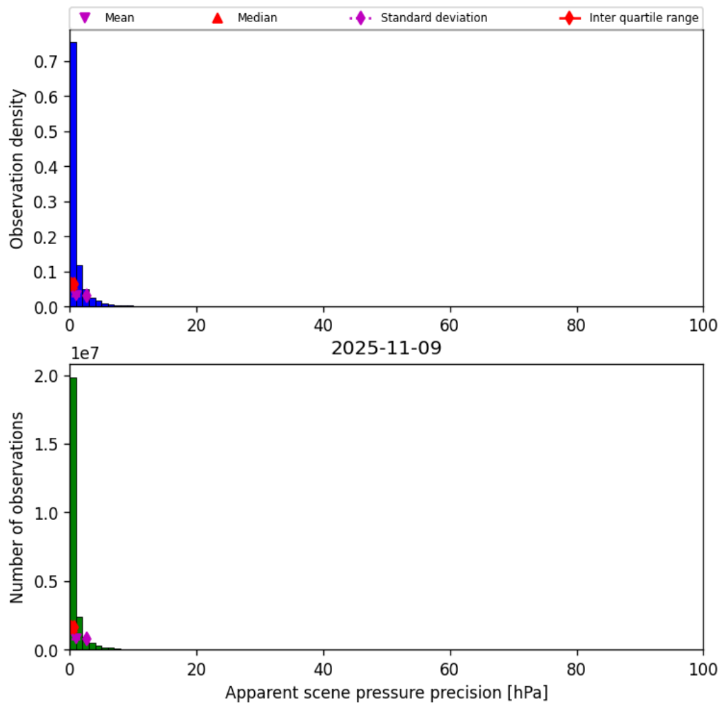
Figure 37: Histogram of “Apparent scene pressure precision” for 2025-11-08 to 2025-11-10
