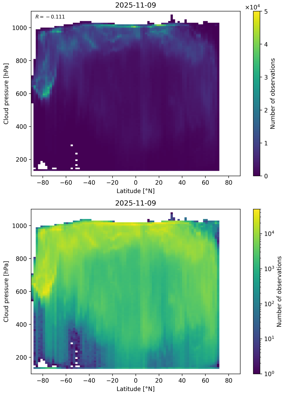
Figure 91: Scatter density plot of “Latitude” against “Cloud pressure” for 2025-11-08 to 2025-11-10.
