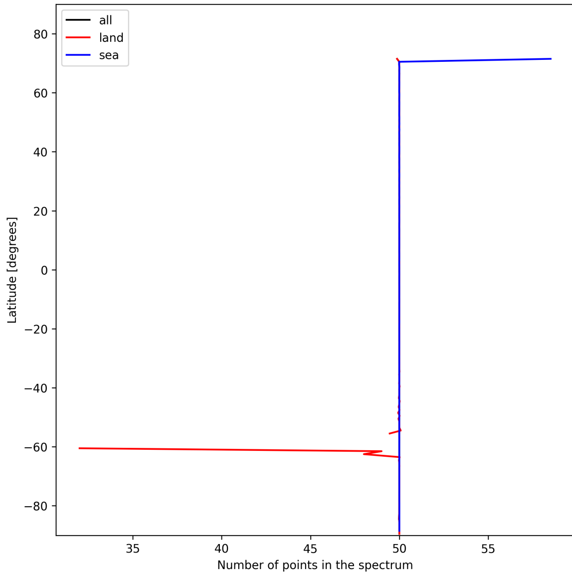
Figure 27: Zonal average of “Number of points in the spectrum” for 2025-11-08 to 2025-11-10.
