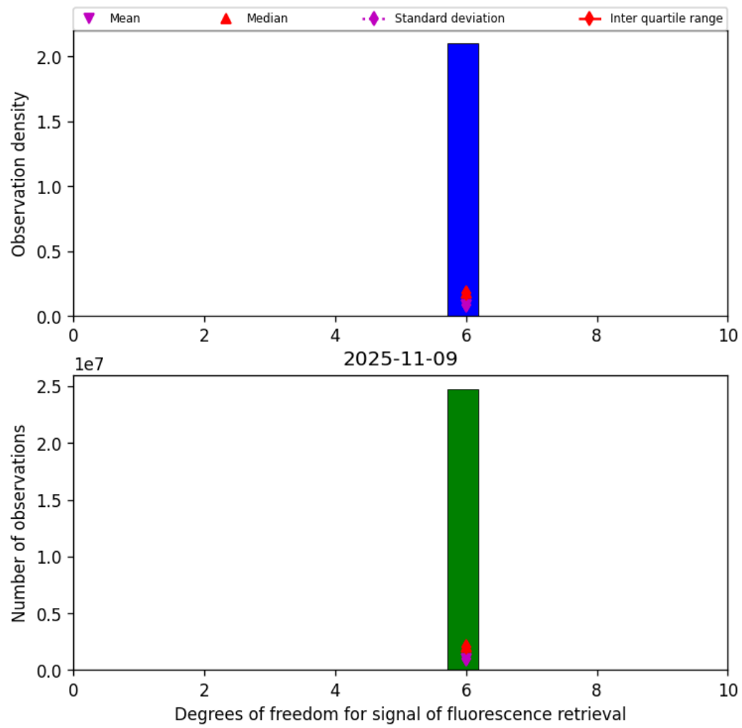
Figure 43: Histogram of “Degrees of freedom for signal of fluorescence retrieval” for 2025-11-08 to 2025-11-10
