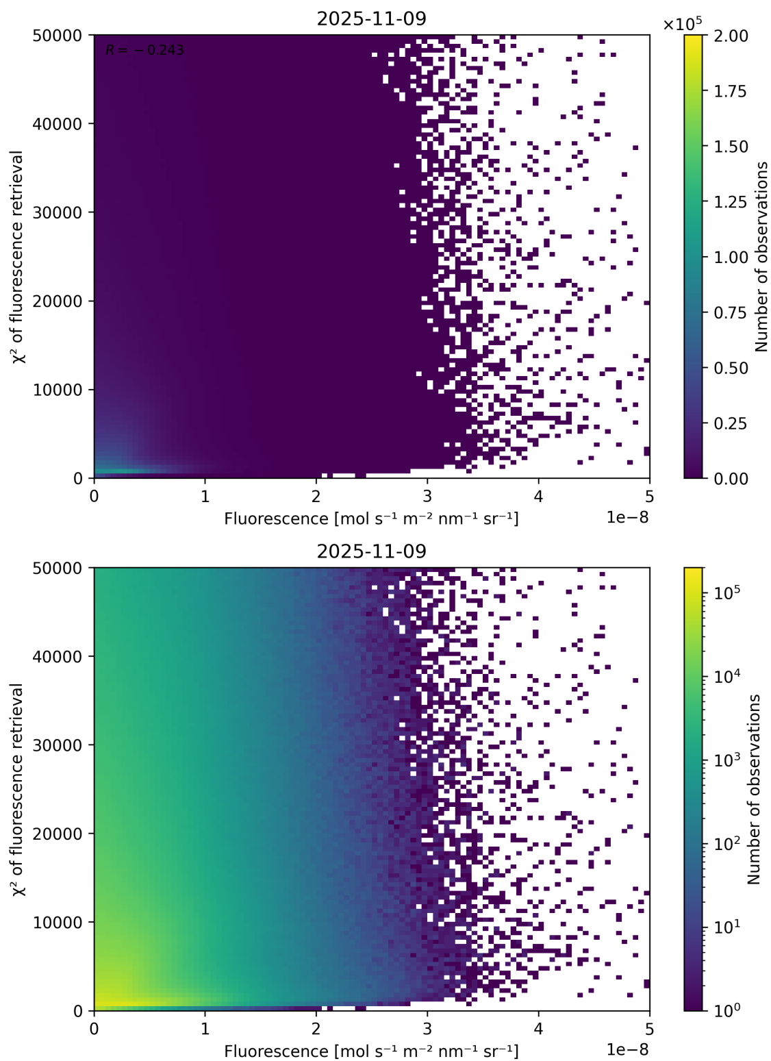
Figure 85: Scatter density plot of “Fluorescence” against “ \chi^2 of fluorescence retrieval” for 2025-11-08 to 2025-11-10.
