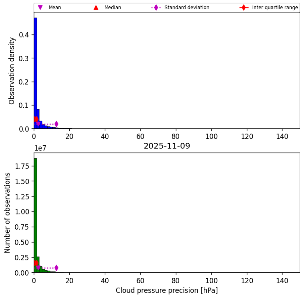
Figure 31: Histogram of “Cloud pressure precision” for 2025-11-08 to 2025-11-10
