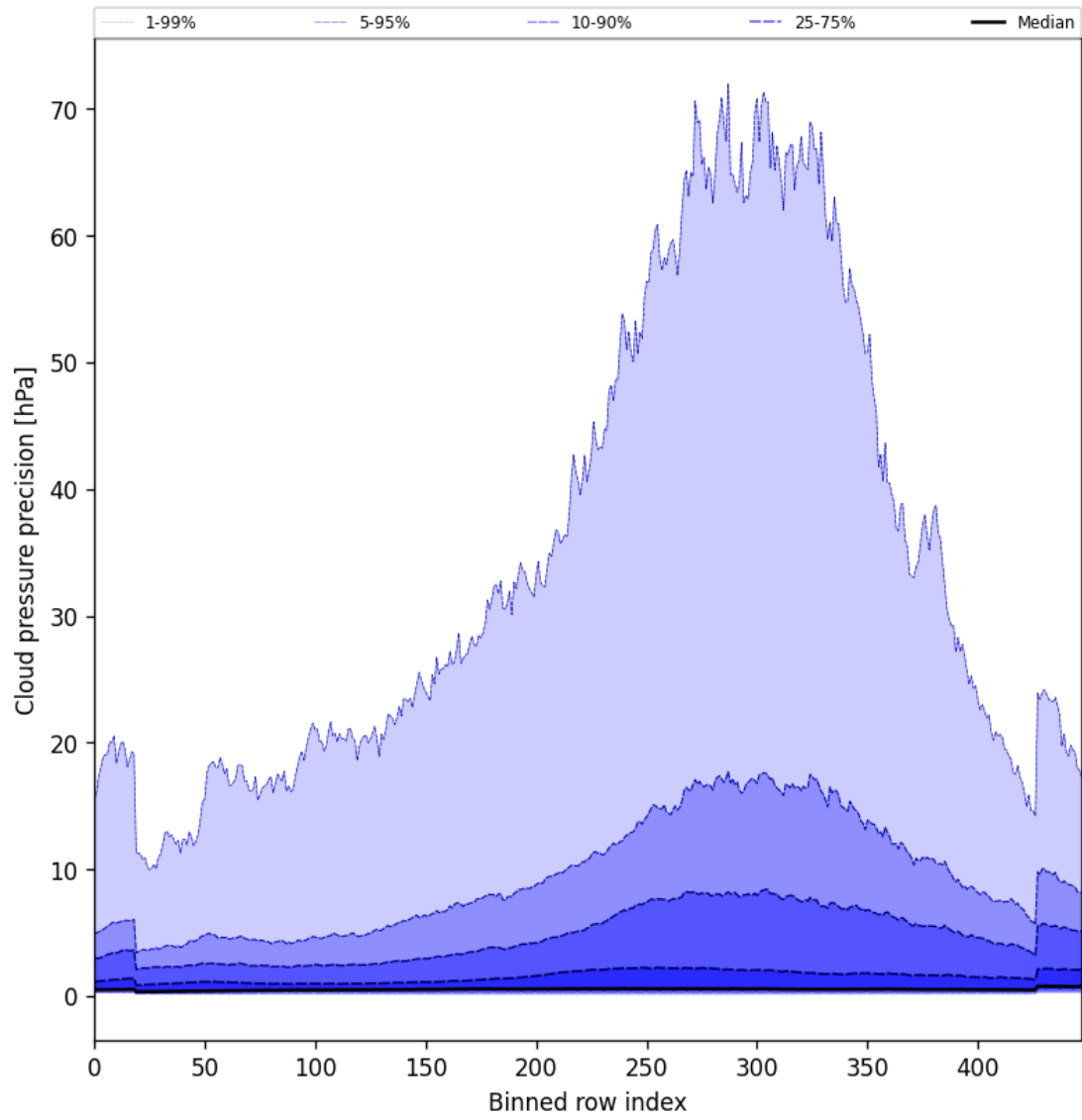
Figure 48: Along track statistics of “Cloud pressure precision” for 2025-11-08 to 2025-11-10
