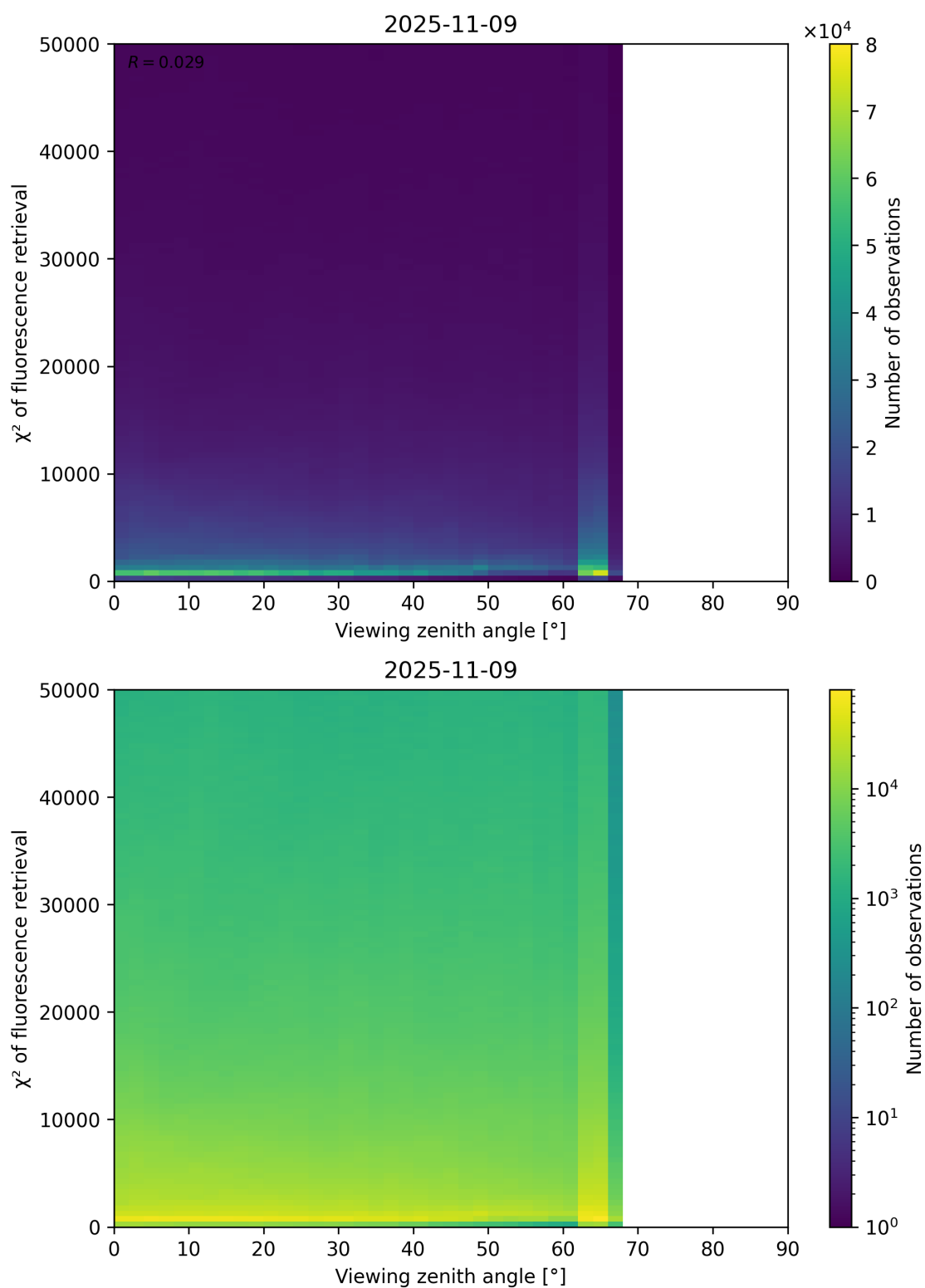
Figure 119: Scatter density plot of “Viewing zenith angle” against “ \chi^2 of fluorescence retrieval” for 2025-11-08 to 2025-11-10.
