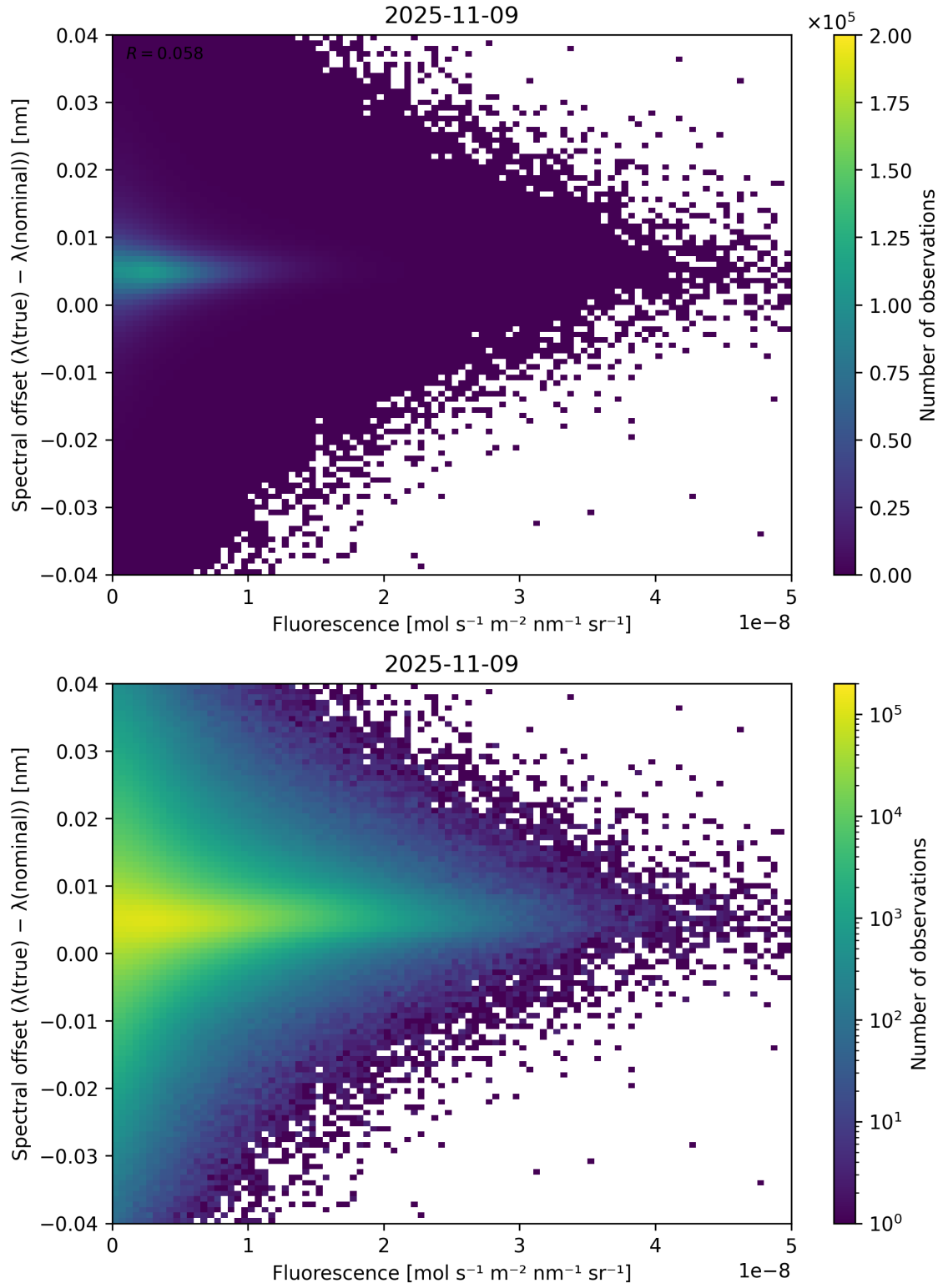
Figure 87: Scatter density plot of “Fluorescence” against “Spectral offset ( \lambda_{\text{true}} - \lambda_{\text{nominal}} )” for 2025-11-08 to 2025-11-10.
