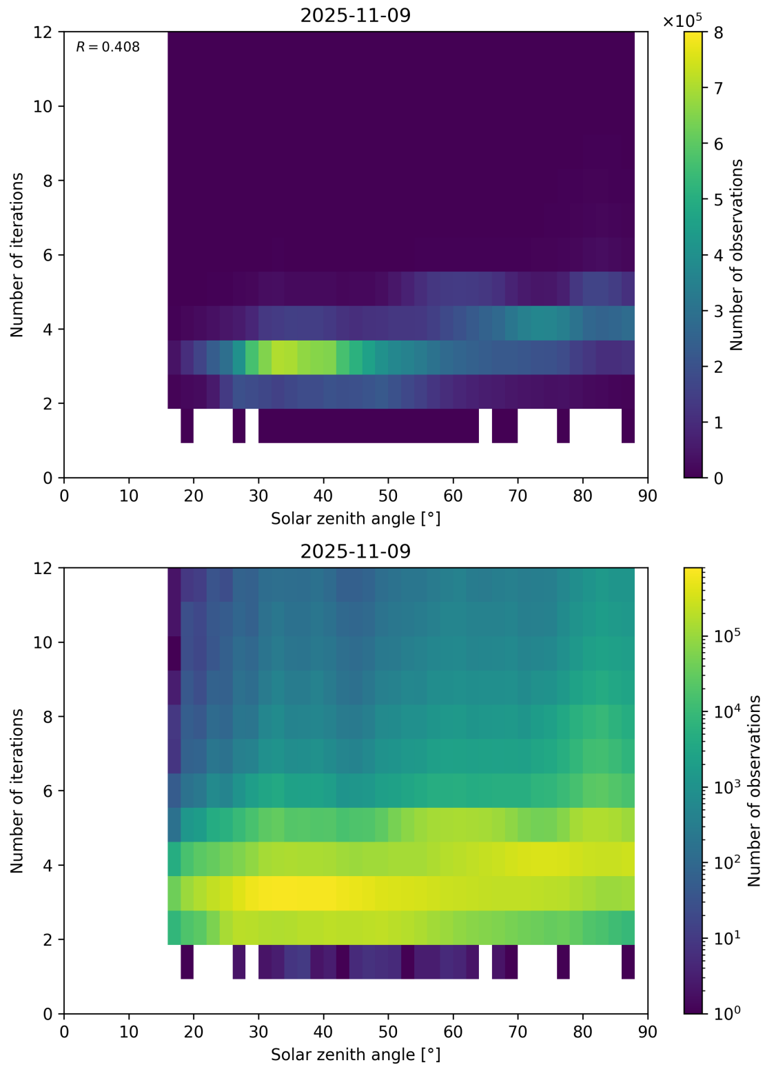
Figure 114: Scatter density plot of “Solar zenith angle” against “Number of iterations” for 2025-11-08 to 2025-11-10.
