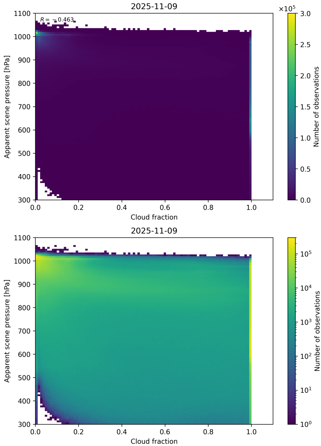
Figure 70: Scatter density plot of “Cloud fraction” against “Apparent scene pressure” for 2025-11-08 to 2025-11-10.
