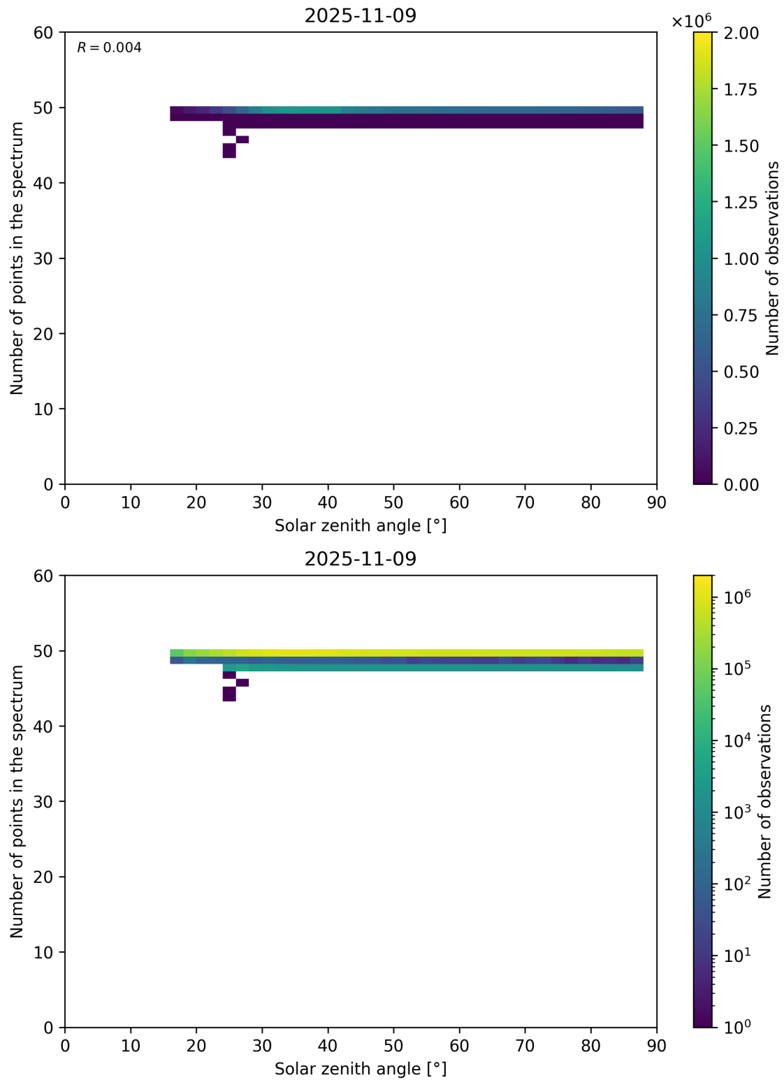
Figure 115: Scatter density plot of “Solar zenith angle” against “Number of points in the spectrum” for 2025-11-08 to 2025-11-10.
