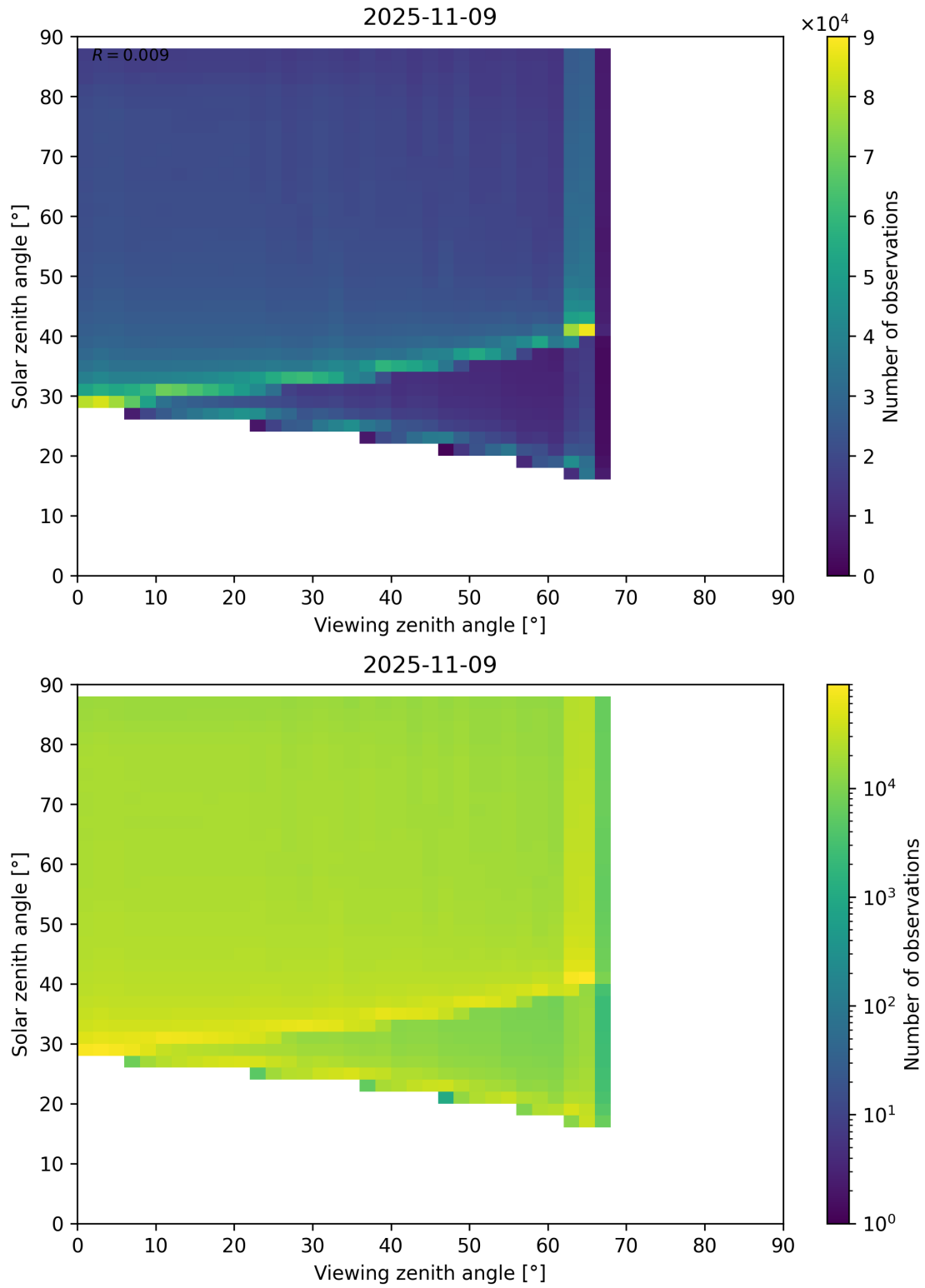
Figure 127: Scatter density plot of “Viewing zenith angle” against “Solar zenith angle” for 2025-11-08 to 2025-11-10.
