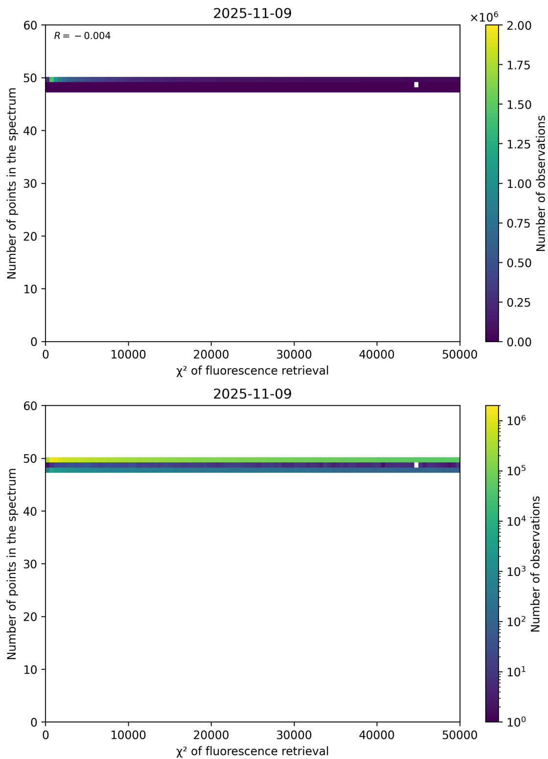
Figure 68: Scatter density plot of " \chi^2 of fluorescence retrieval" against "Number of points in the spectrum" for 2025-11-08 to 2025-11-10.
