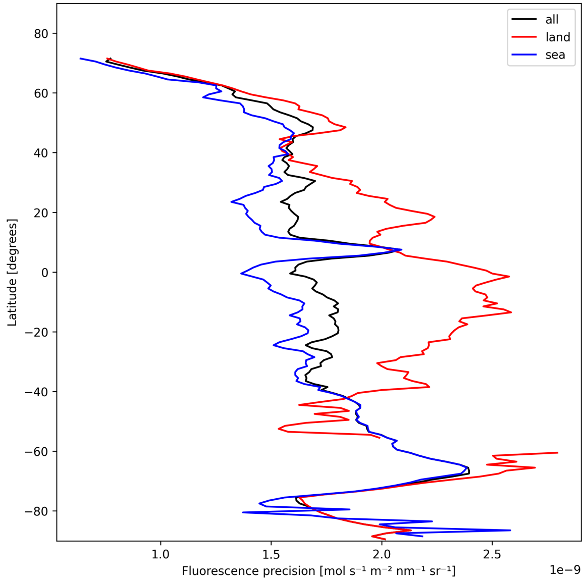
Figure 24: Zonal average of “Fluorescence precision” for 2025-11-08 to 2025-11-10.
