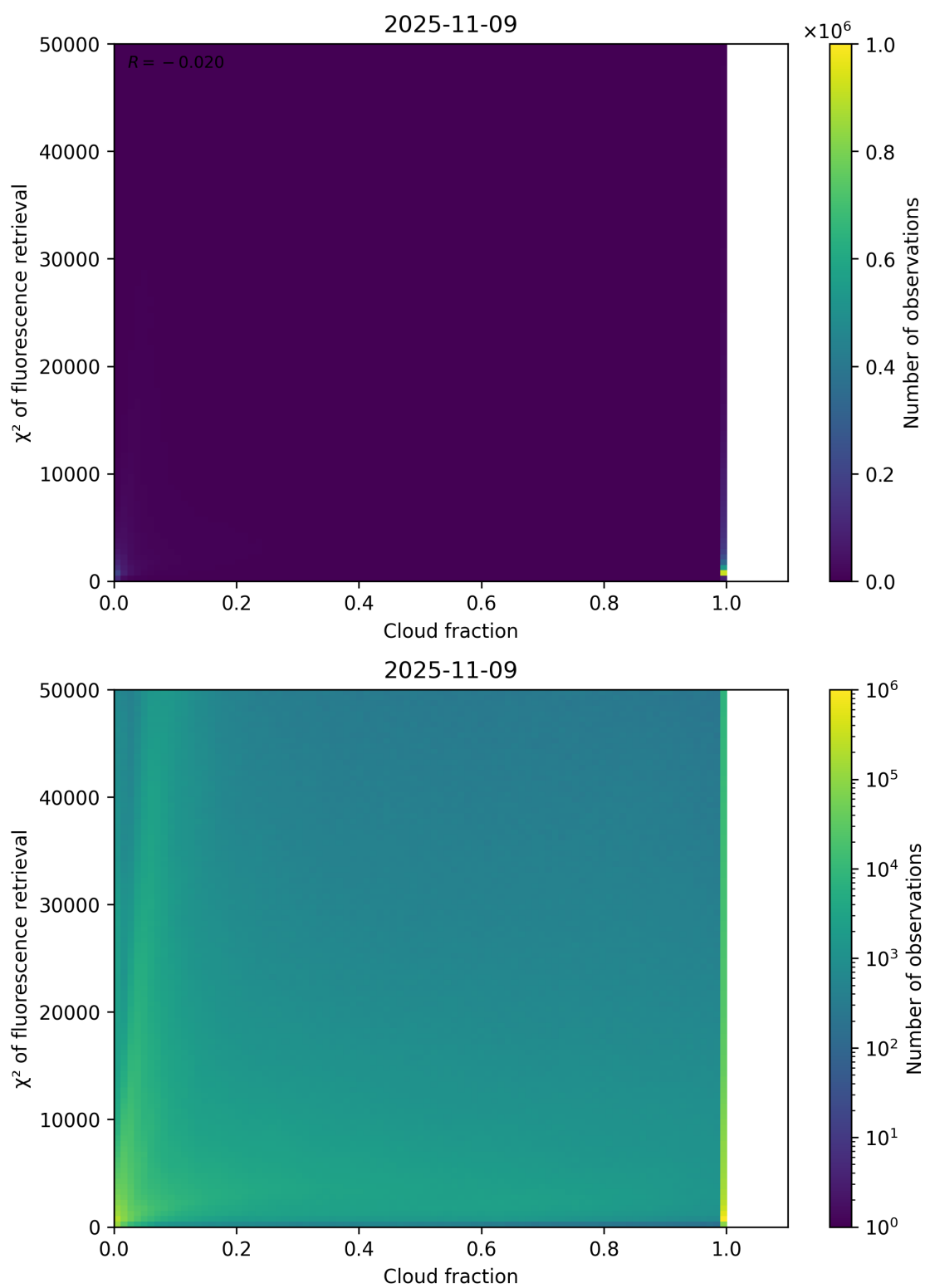
Figure 71: Scatter density plot of “Cloud fraction” against “ \chi^2 of fluorescence retrieval” for 2025-11-08 to 2025-11-10.
