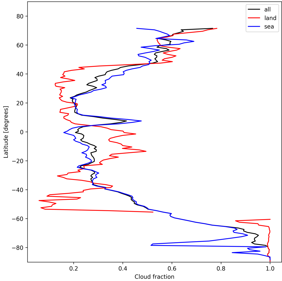
Figure 15: Zonal average of “Cloud fraction” for 2025-11-08 to 2025-11-10.
