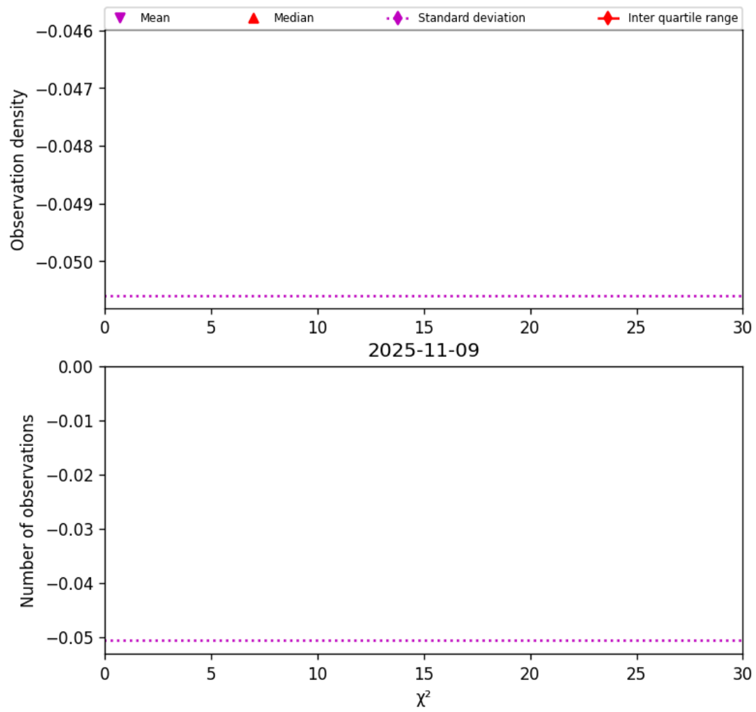
Figure 38: Histogram of “ \chi^2 ” for 2025-11-08 to 2025-11-10
