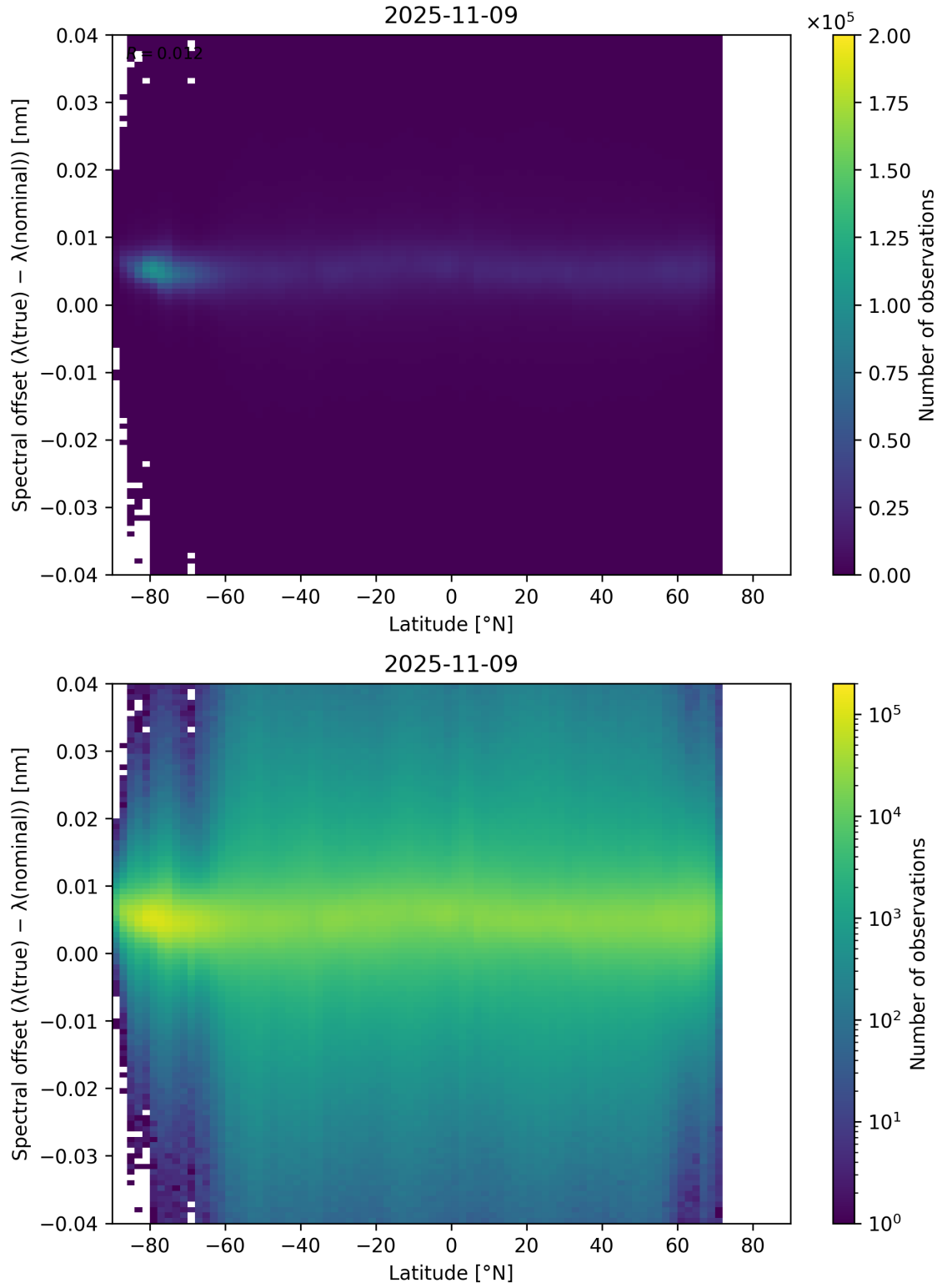
Figure 96: Scatter density plot of “Latitude” against “Spectral offset ( \lambda_{\text{true}} - \lambda_{\text{nominal}} )” for 2025-11-08 to 2025-11-10.
