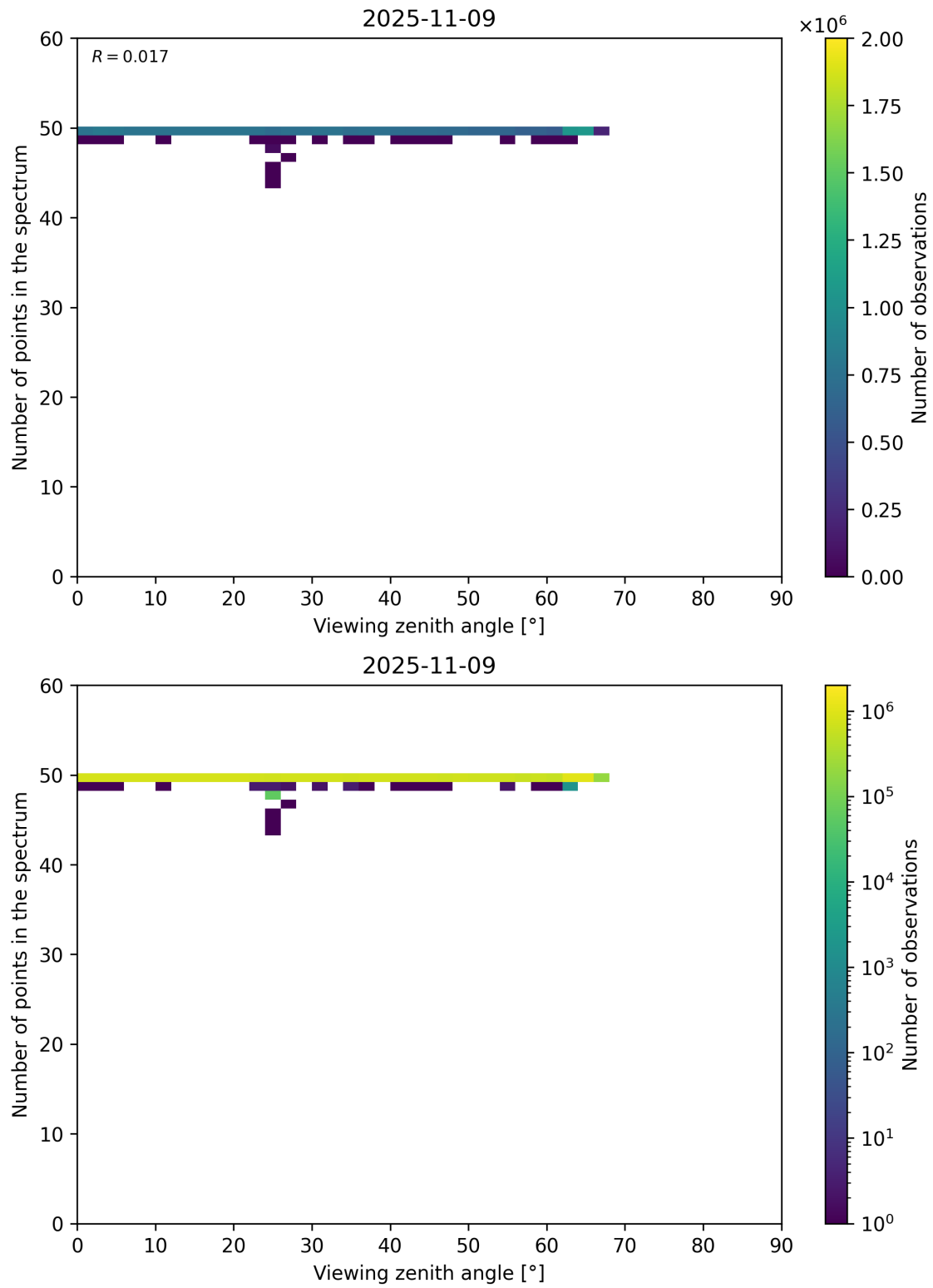
Figure 125: Scatter density plot of “Viewing zenith angle” against “Number of points in the spectrum” for 2025-11-08 to 2025-11-10.
