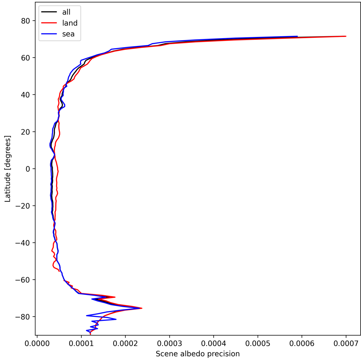
Figure 18: Zonal average of “Scene albedo precision” for 2025-11-08 to 2025-11-10.
