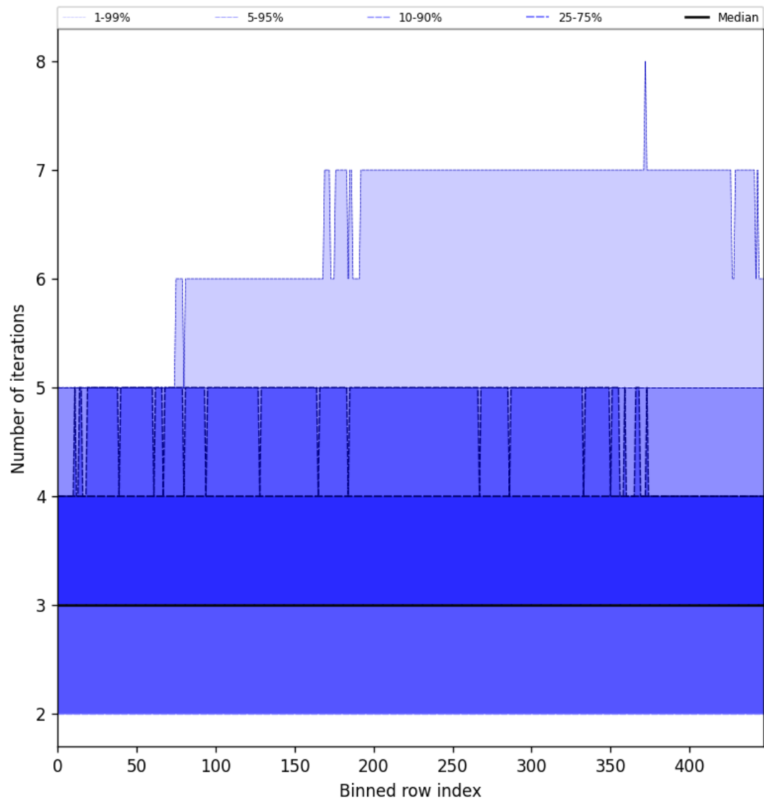
Figure 56: Along track statistics of “Number of iterations” for 2025-11-08 to 2025-11-10
