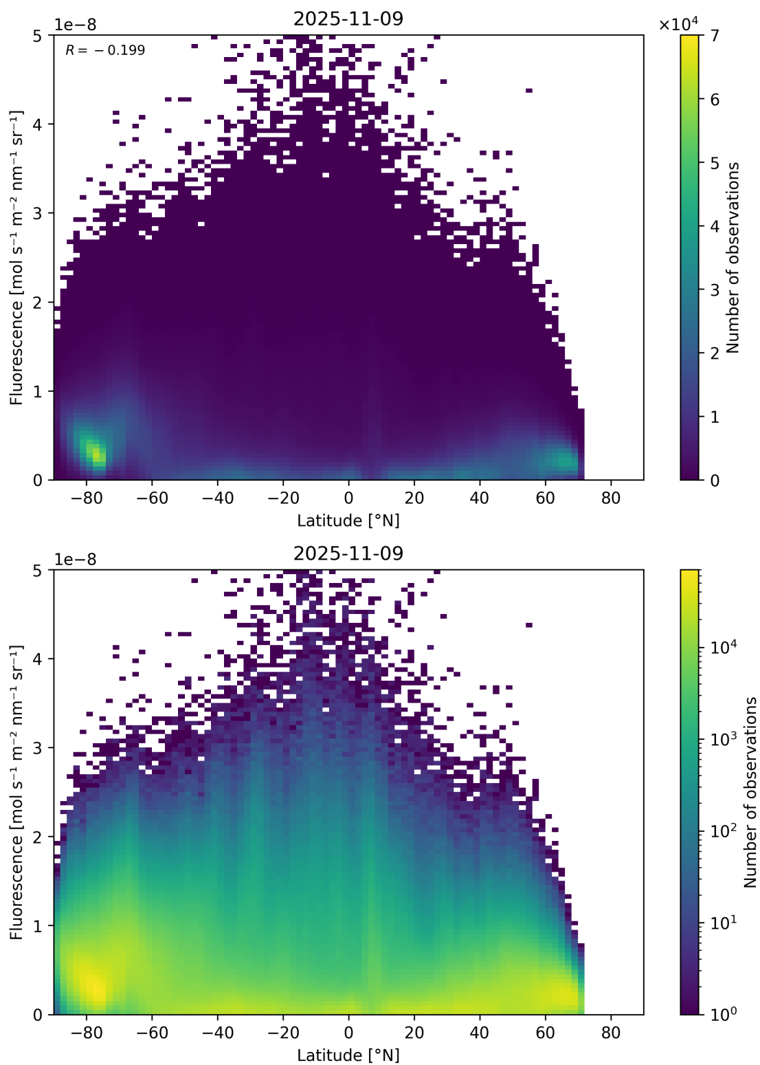
Figure 92: Scatter density plot of “Latitude” against “Fluorescence” for 2025-11-08 to 2025-11-10.
