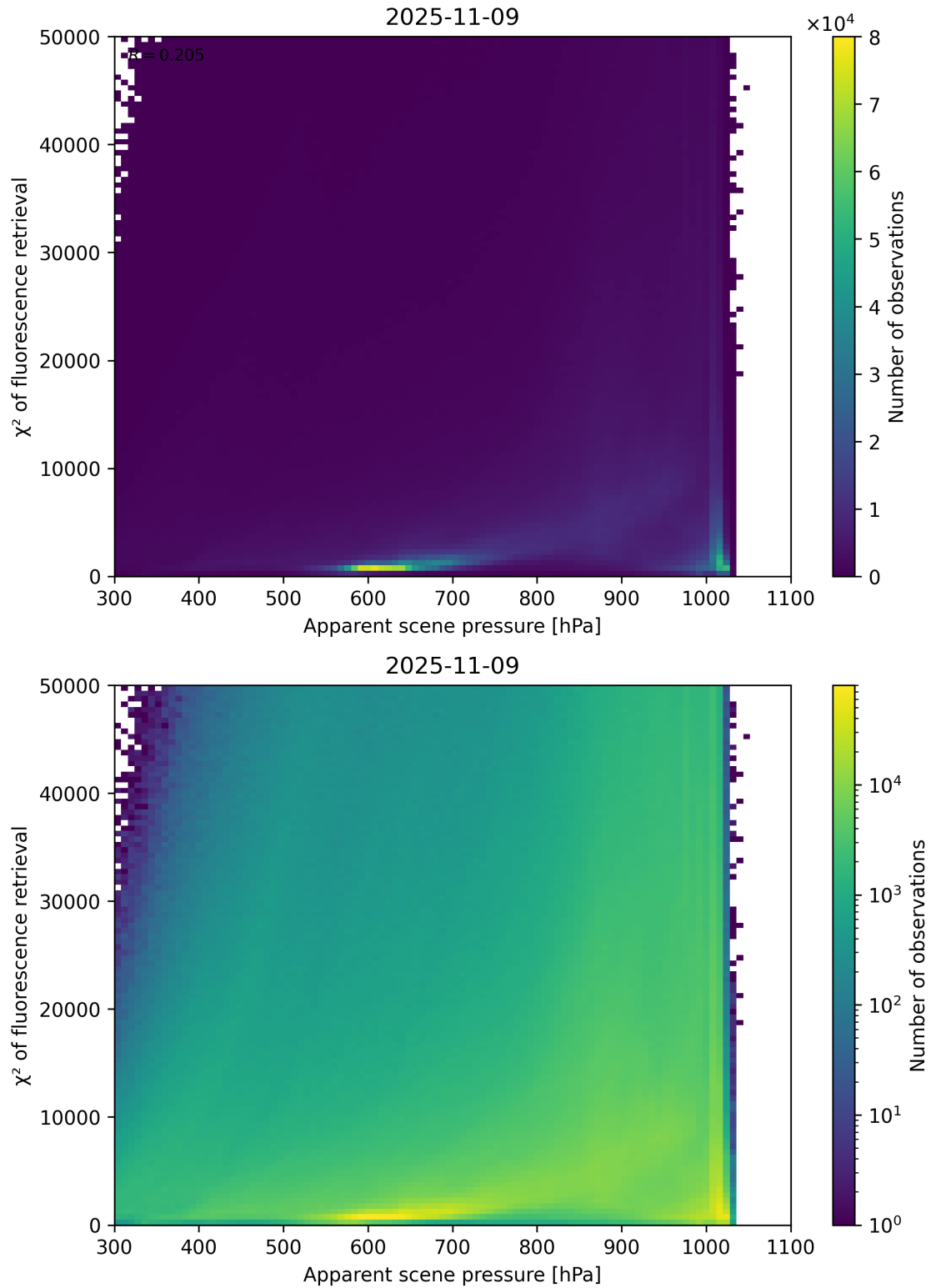
Figure 63: Scatter density plot of “Apparent scene pressure” against “ \chi^2 of fluorescence retrieval” for 2025-11-08 to 2025-11-10.
