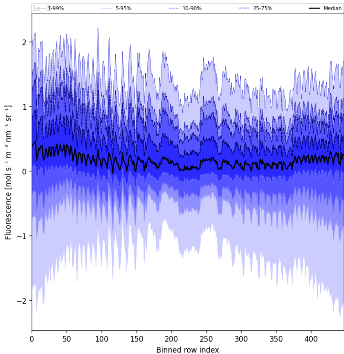
Figure 57: Along track statistics of “Fluorescence” for 2025-11-08 to 2025-11-10
