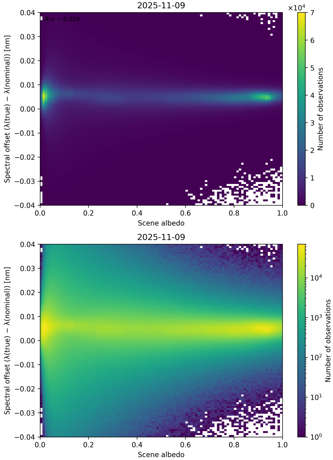
Figure 107: Scatter density plot of “Scene albedo” against “Spectral offset ( \lambda_{\text{true}} - \lambda_{\text{nominal}} )” for 2025-11-08 to 2025-11-10.
