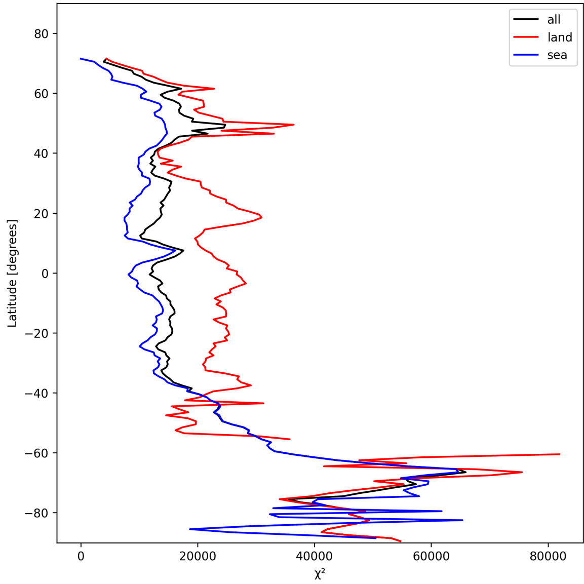
Figure 21: Zonal average of “ \chi^2 ” for 2025-11-08 to 2025-11-10.
