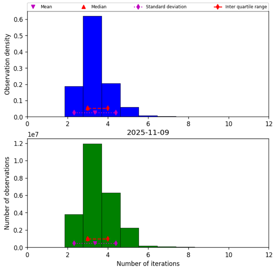
Figure 39: Histogram of “Number of iterations” for 2025-11-08 to 2025-11-10
