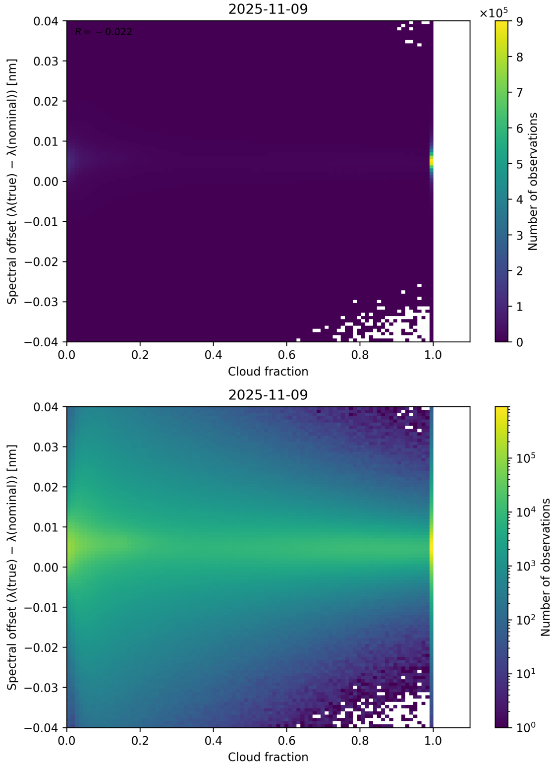
Figure 76: Scatter density plot of “Cloud fraction” against “Spectral offset ( \lambda_{\text{true}} - \lambda_{\text{nominal}} )” for 2025-11-08 to 2025-11-10.
