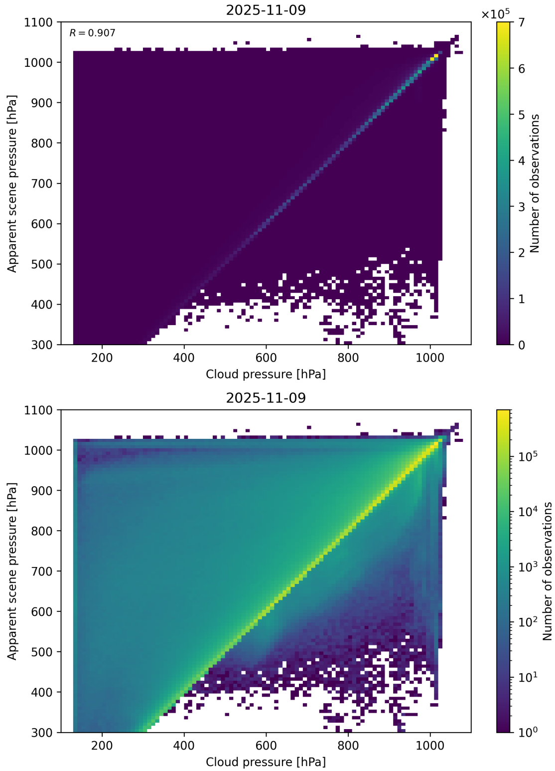
Figure 77: Scatter density plot of “Cloud pressure” against “Apparent scene pressure” for 2025-11-08 to 2025-11-10.
