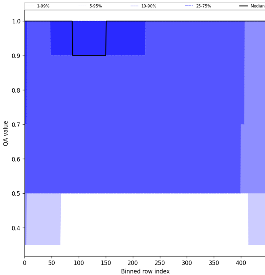
Figure 46: Along track statistics of “QA value” for 2025-11-08 to 2025-11-10
