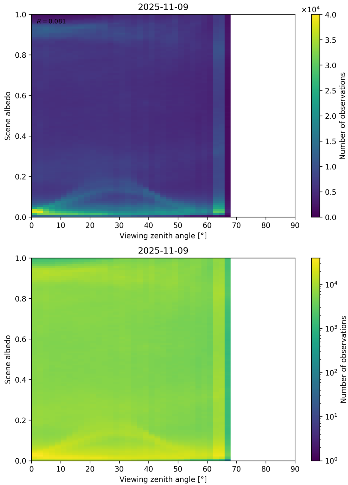
Figure 126: Scatter density plot of “Viewing zenith angle” against “Scene albedo” for 2025-11-08 to 2025-11-10.
