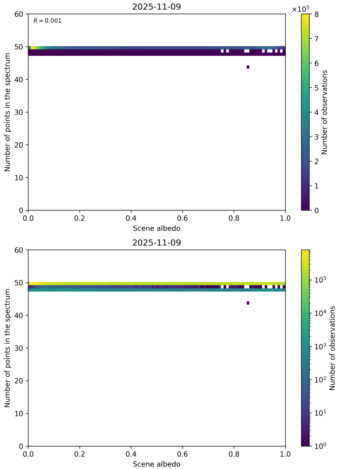
Figure 106: Scatter density plot of “Scene albedo” against “Number of points in the spectrum” for 2025-11-08 to 2025-11-10.
