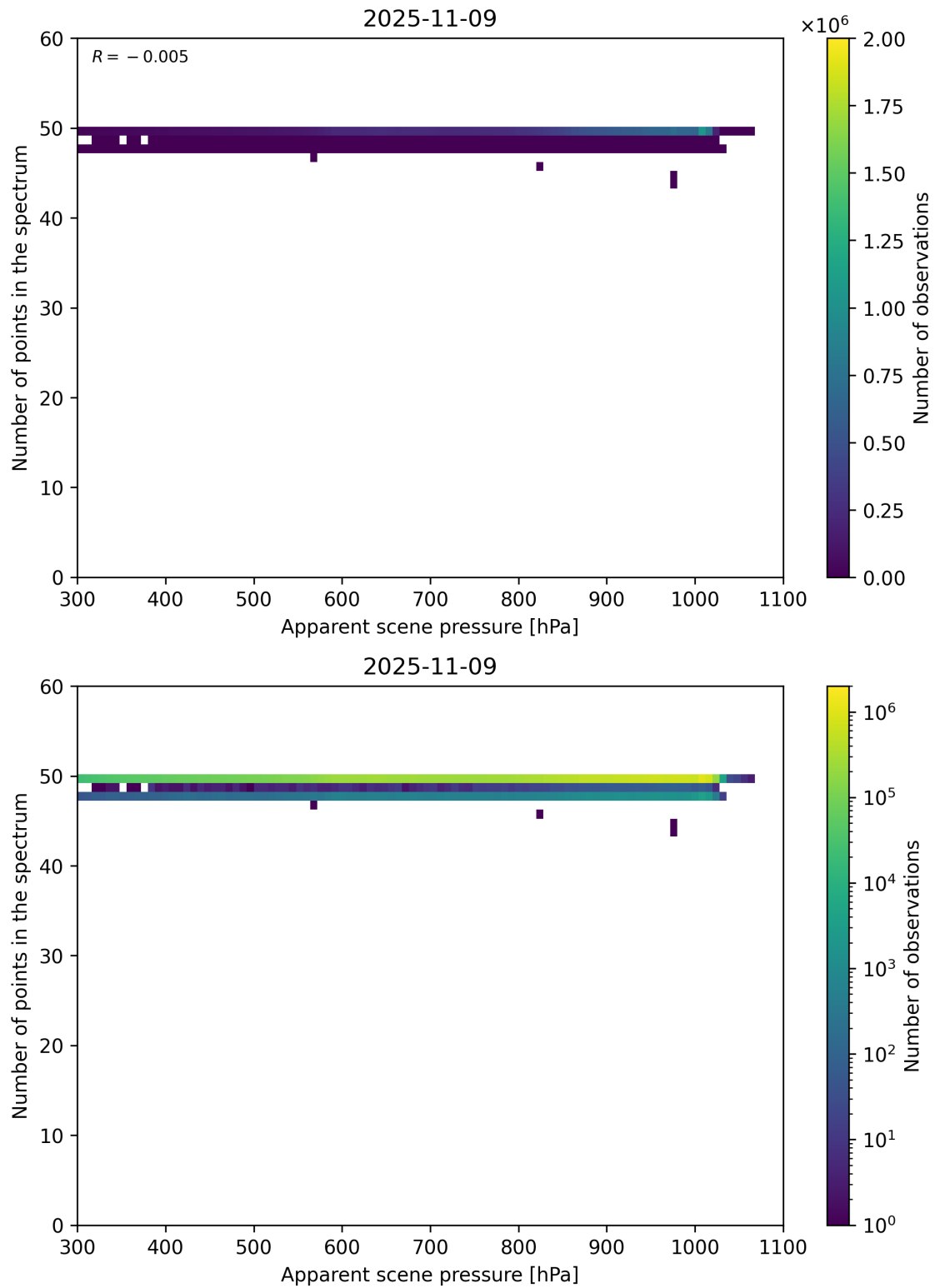
Figure 66: Scatter density plot of “Apparent scene pressure” against “Number of points in the spectrum” for 2025-11-08 to 2025-11-10.
