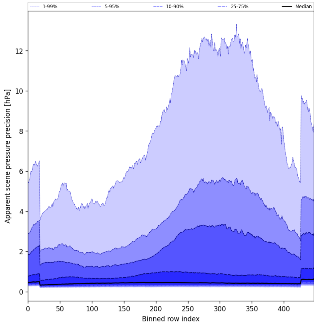
Figure 54: Along track statistics of “Apparent scene pressure precision” for 2025-11-08 to 2025-11-10
