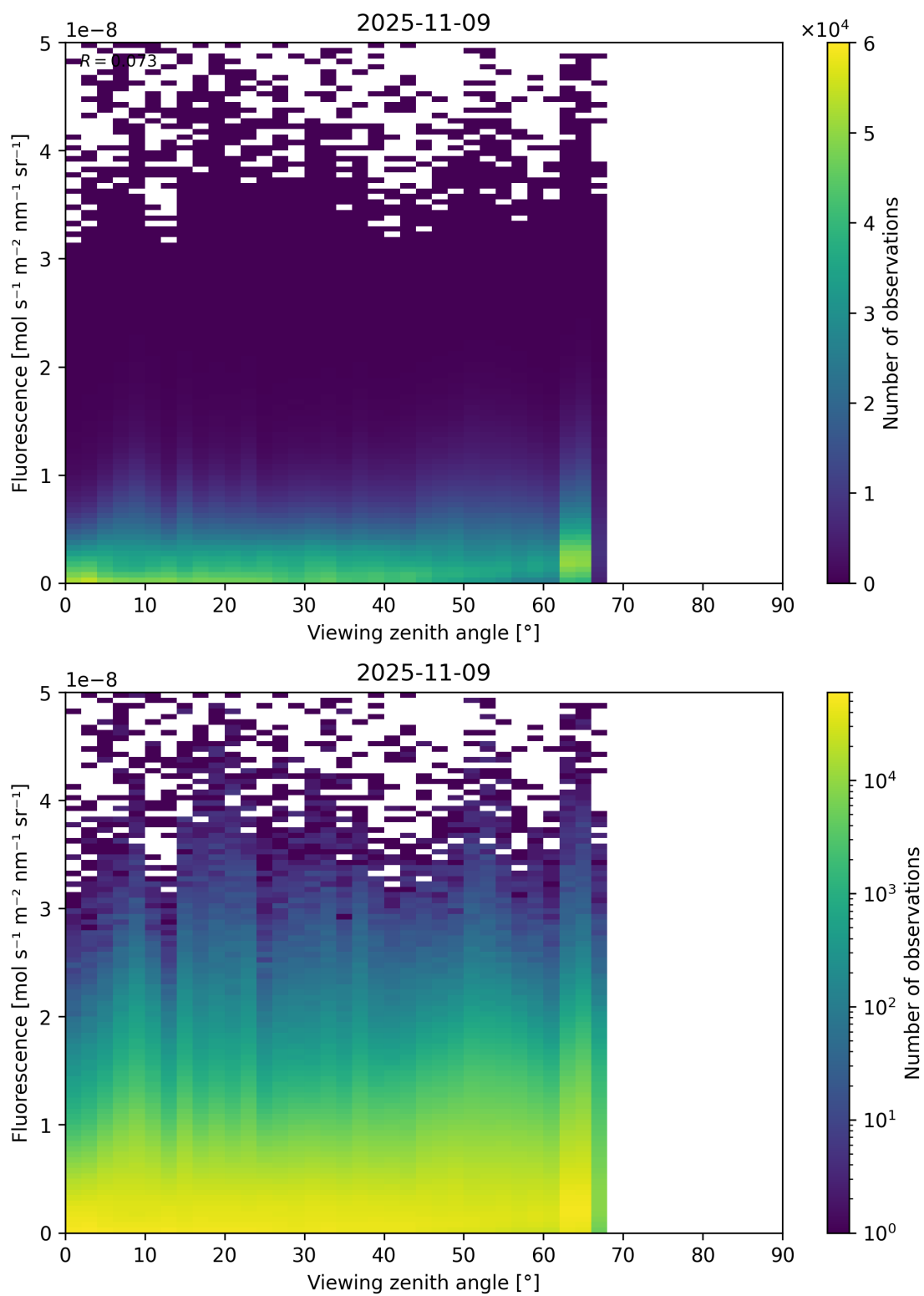
Figure 122: Scatter density plot of “Viewing zenith angle” against “Fluorescence” for 2025-11-08 to 2025-11-10.
