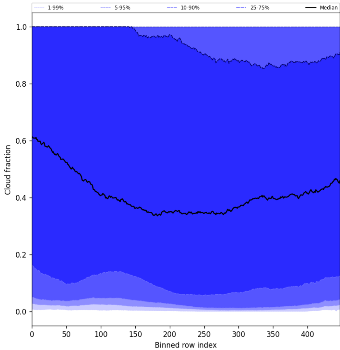
Figure 49: Along track statistics of “Cloud fraction” for 2025-11-08 to 2025-11-10
