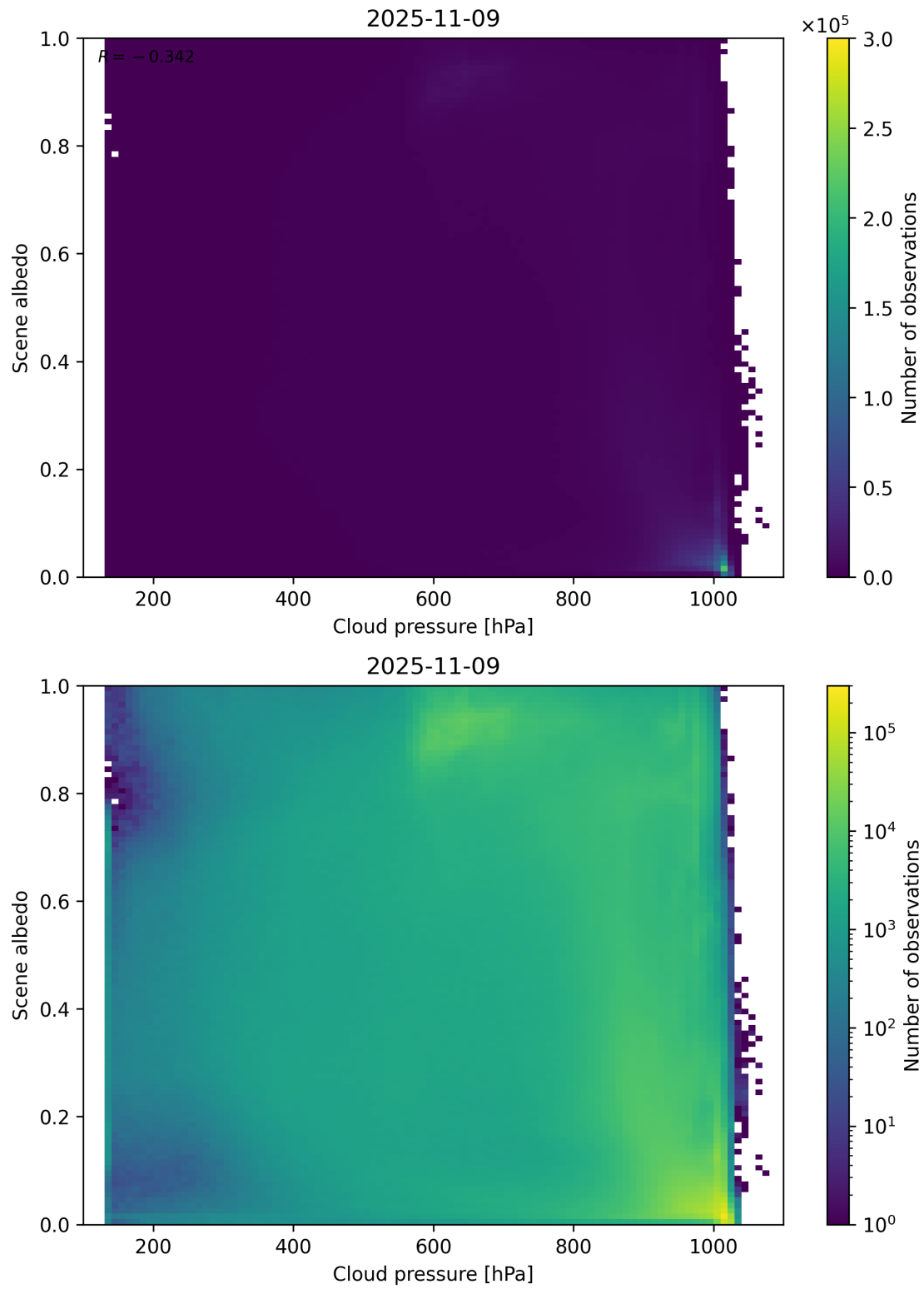
Figure 83: Scatter density plot of “Cloud pressure” against “Scene albedo” for 2025-11-08 to 2025-11-10.
