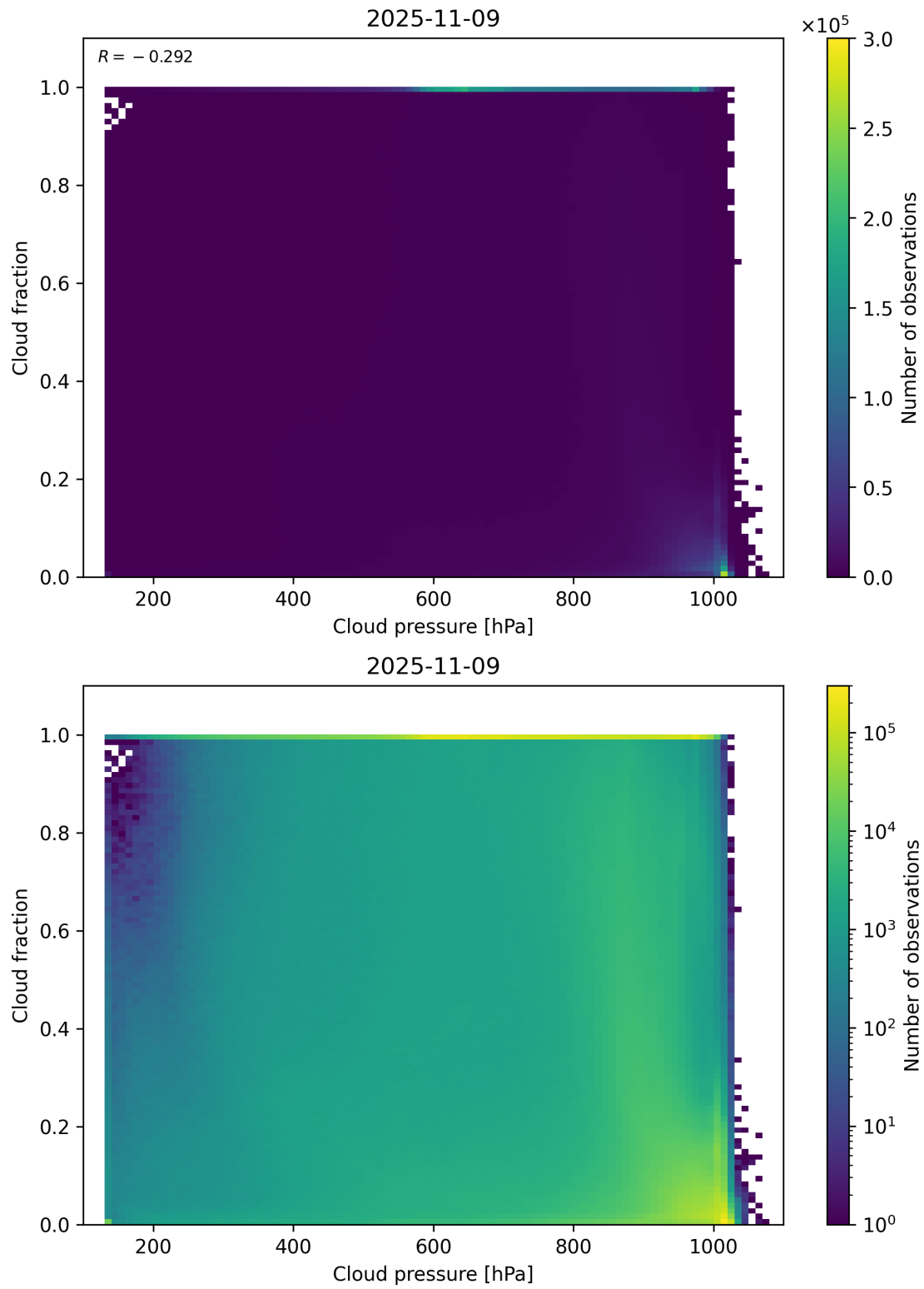
Figure 79: Scatter density plot of “Cloud pressure” against “Cloud fraction” for 2025-11-08 to 2025-11-10.
