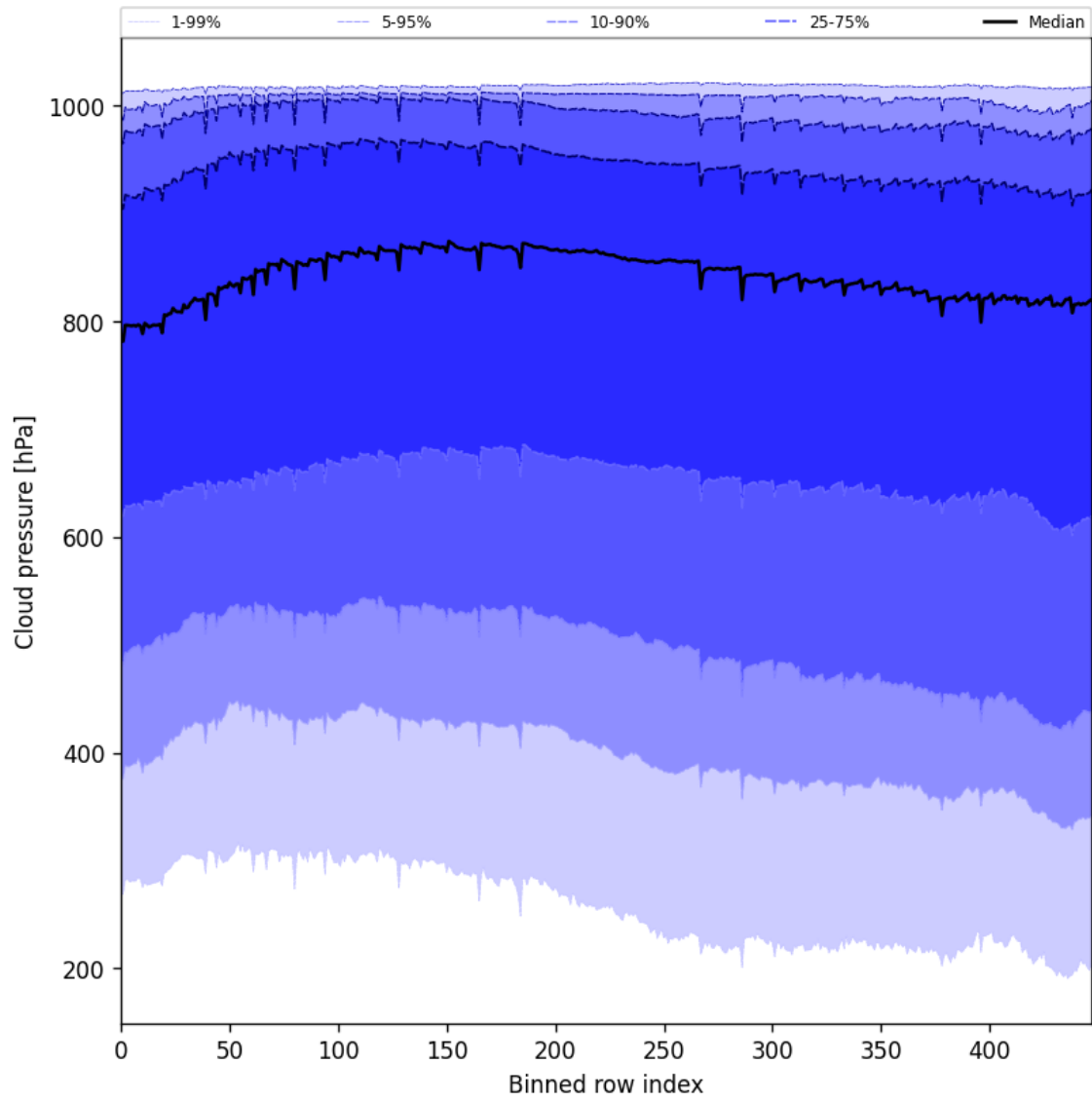
Figure 47: Along track statistics of “Cloud pressure” for 2025-11-08 to 2025-11-10
