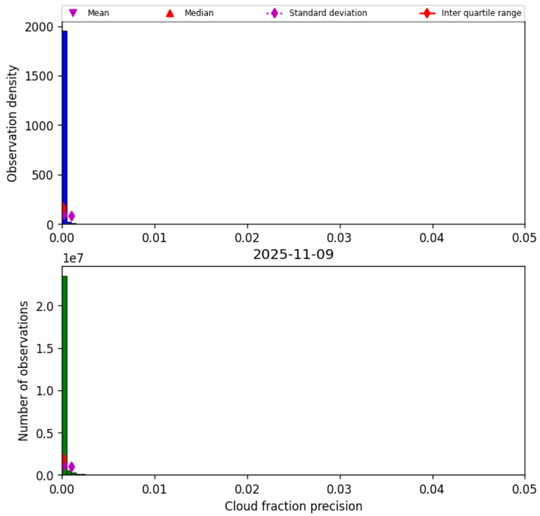
Figure 33: Histogram of “Cloud fraction precision” for 2025-11-08 to 2025-11-10
