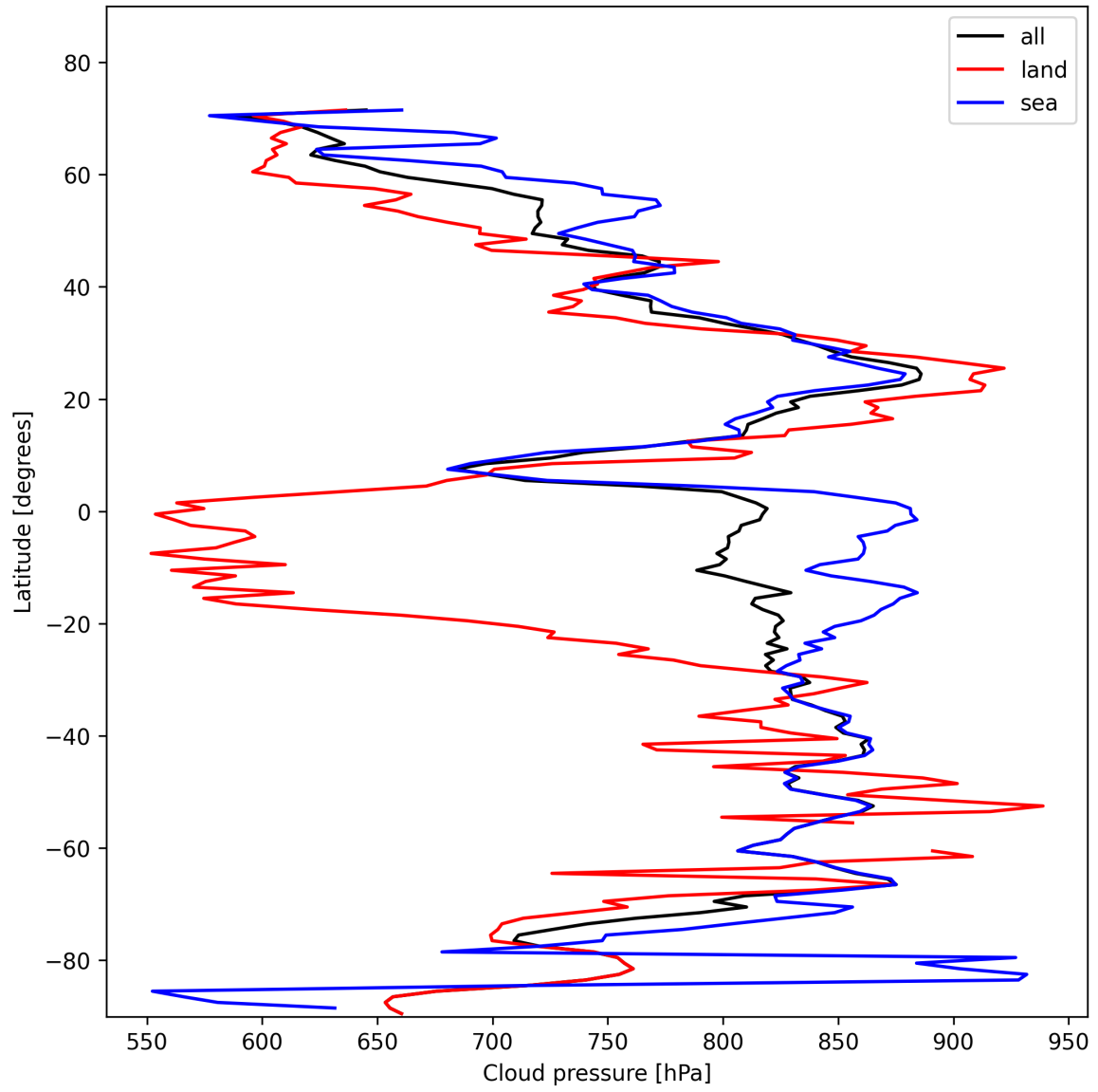
Figure 13: Zonal average of “Cloud pressure” for 2025-11-08 to 2025-11-10.
