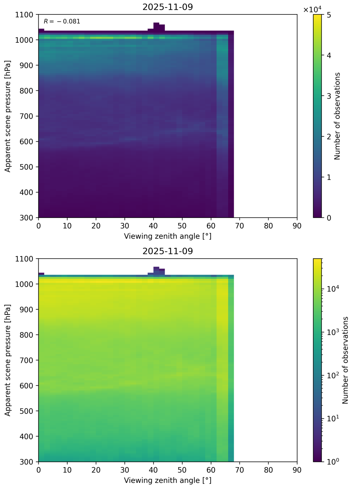
Figure 118: Scatter density plot of “Viewing zenith angle” against “Apparent scene pressure” for 2025-11-08 to 2025-11-10.
