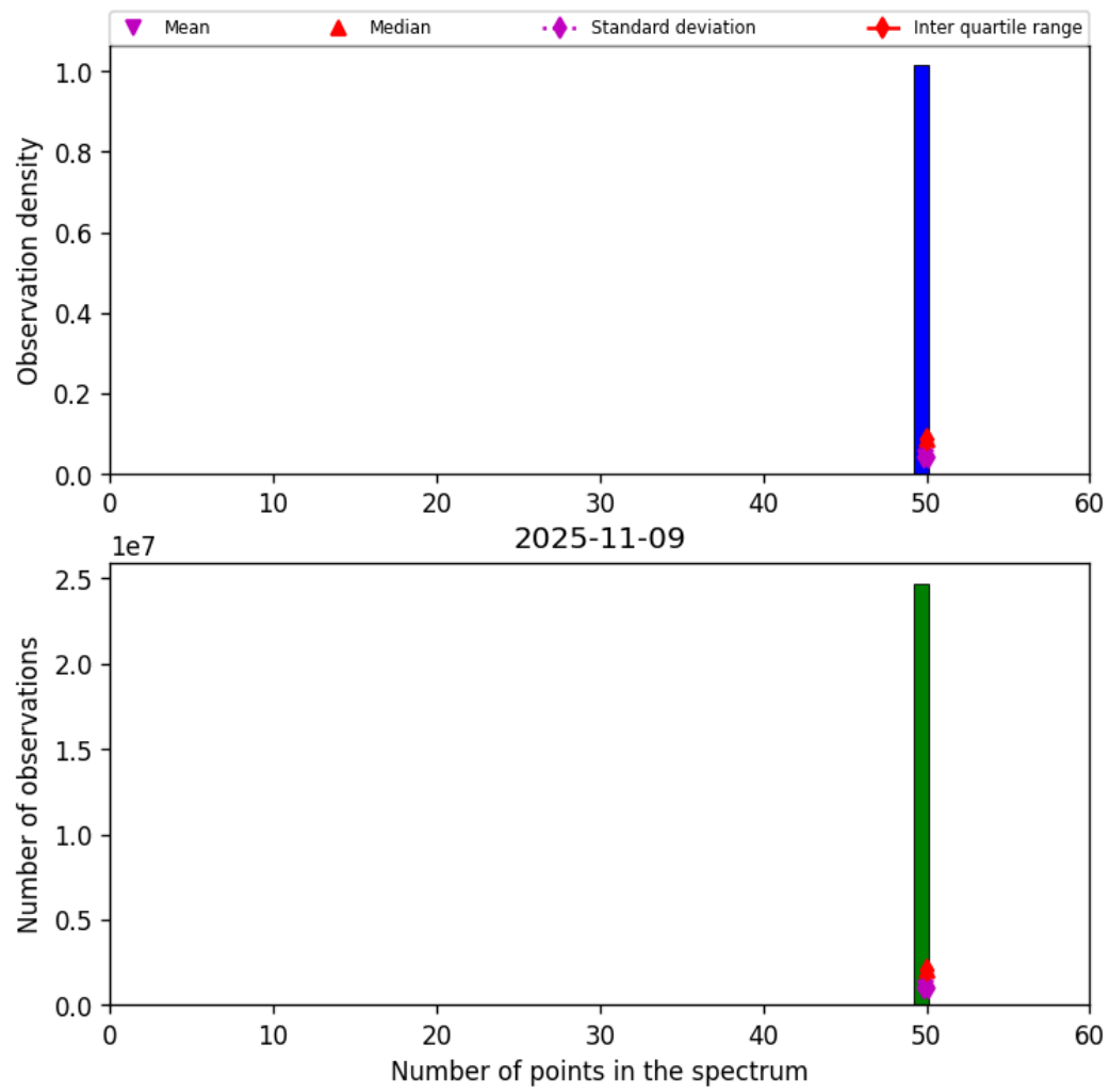
Figure 44: Histogram of "Number of points in the spectrum" for 2025-11-08 to 2025-11-10
