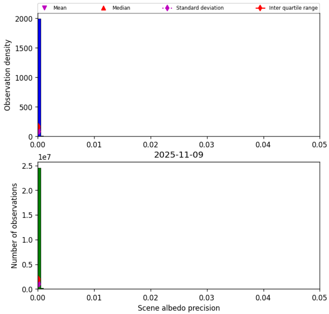
Figure 35: Histogram of “Scene albedo precision” for 2025-11-08 to 2025-11-10
