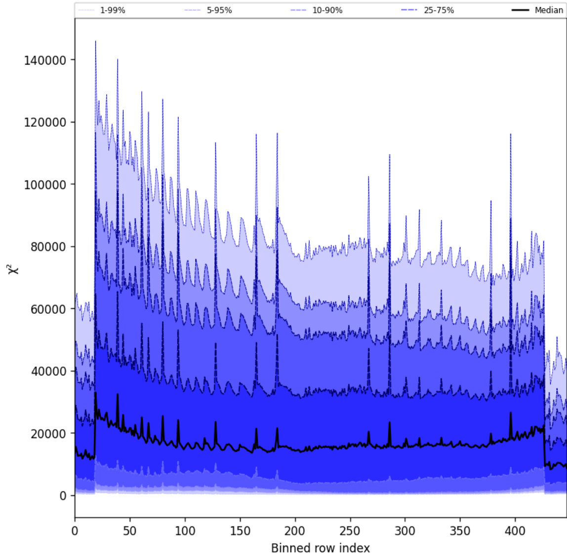
Figure 55: Along track statistics of “ \chi^2 ” for 2025-11-08 to 2025-11-10
