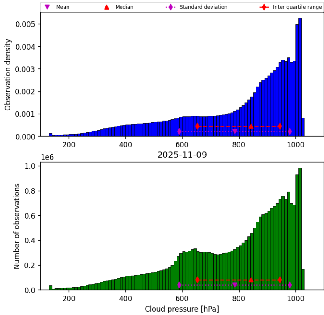
Figure 30: Histogram of “Cloud pressure” for 2025-11-08 to 2025-11-10
