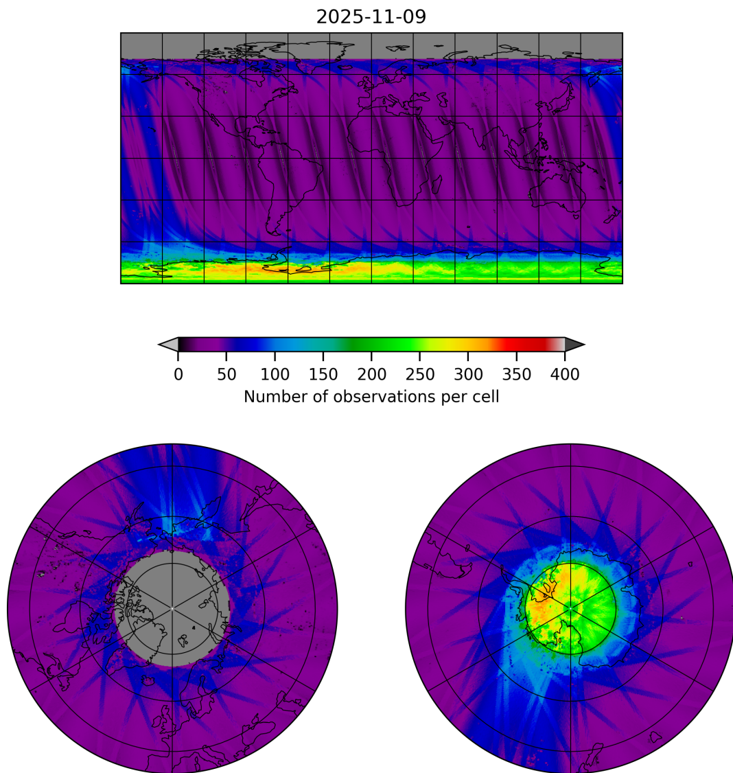
Figure 11: Map of the number of observations for 2025-11-08 to 2025-11-10
