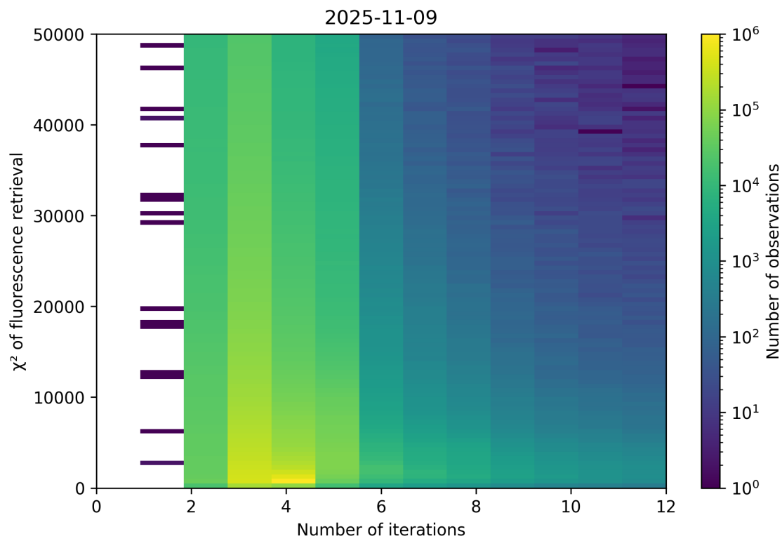
Figure 97: Scatter density plot of “Number of iterations” against “ \chi^2 of fluorescence retrieval” for 2025-11-08 to 2025-11-10.
