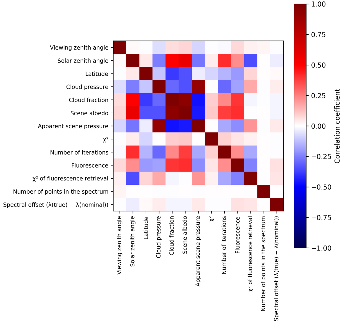
Figure 2: Map of correlation matrix for 2025-11-08 to 2025-11-10.
