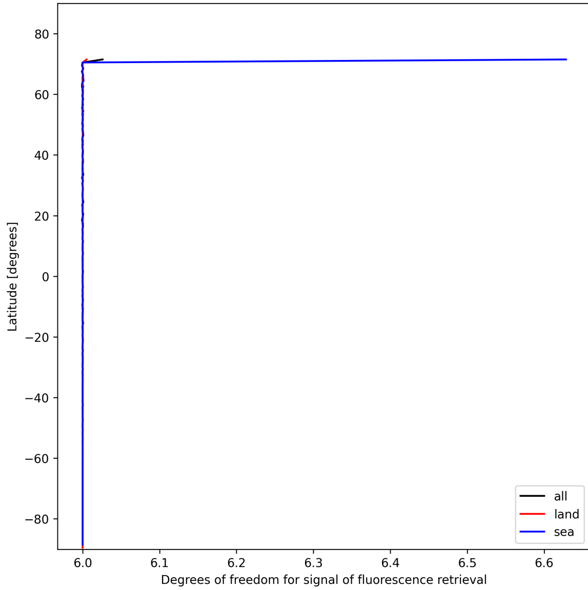
Figure 26: Zonal average of “Degrees of freedom for signal of fluorescence retrieval” for 2025-11-08 to 2025-11-10.
