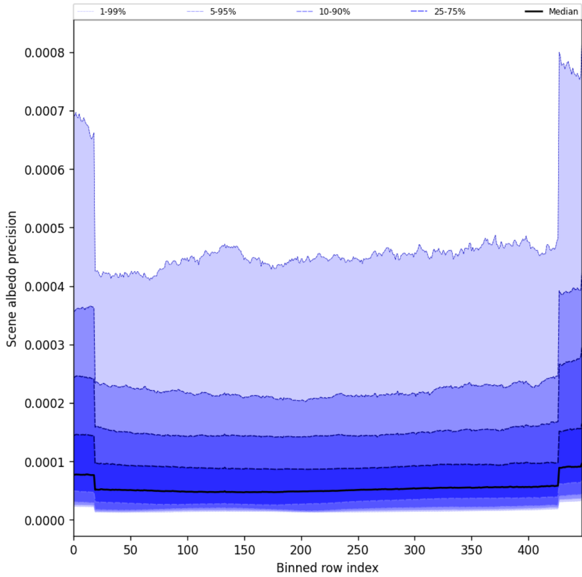
Figure 52: Along track statistics of “Scene albedo precision” for 2025-11-08 to 2025-11-10
