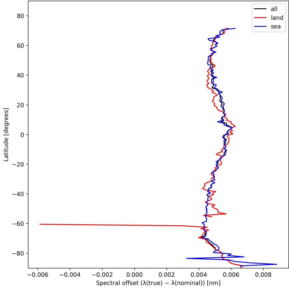
Figure 28: Zonal average of “Spectral offset ( \lambda_{\text{true}} - \lambda_{\text{nominal}} )” for 2025-11-08 to 2025-11-10.
