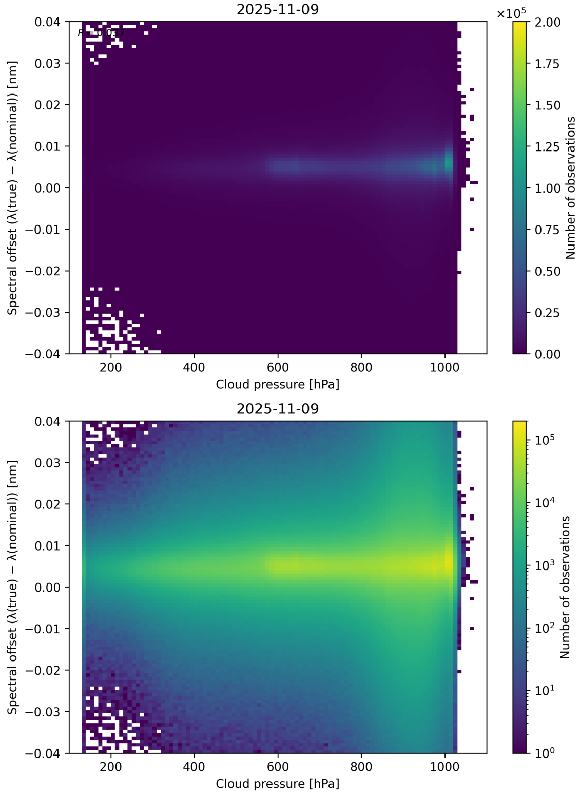
Figure 84: Scatter density plot of “Cloud pressure” against “Spectral offset ( \lambda_{\text{true}} - \lambda_{\text{nominal}} )” for 2025-11-08 to 2025-11-10.
