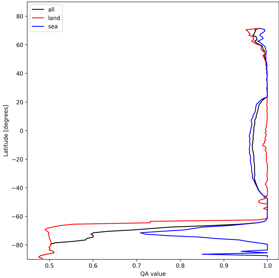
Figure 12: Zonal average of “QA value” for 2025-11-08 to 2025-11-10.
