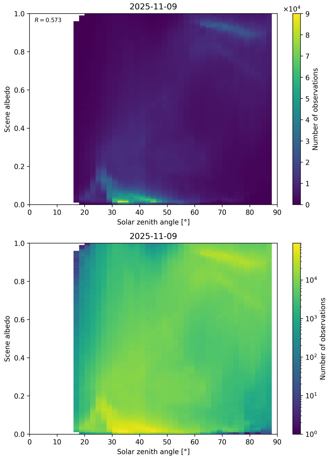
Figure 116: Scatter density plot of “Solar zenith angle” against “Scene albedo” for 2025-11-08 to 2025-11-10.
