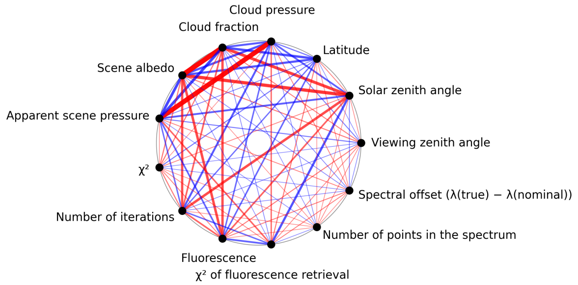
Figure 1: Map of correlation graph for 2025-11-08 to 2025-11-10.
