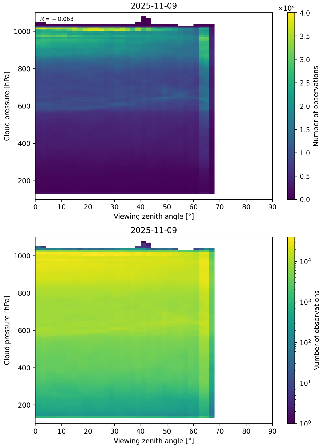
Figure 121: Scatter density plot of “Viewing zenith angle” against “Cloud pressure” for 2025-11-08 to 2025-11-10.
