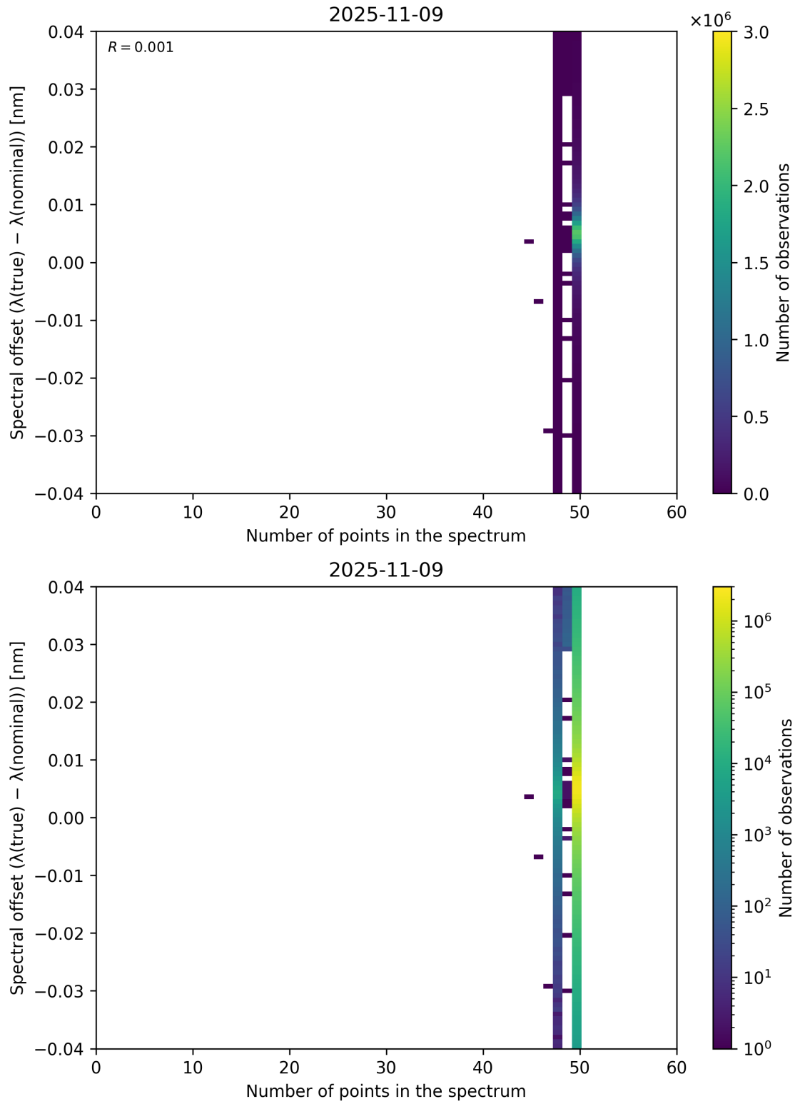
Figure 101: Scatter density plot of “Number of points in the spectrum” against “Spectral offset ( \lambda_{\text{true}} - \lambda_{\text{nominal}} )” for 2025-11-08 to 2025-11-10.
