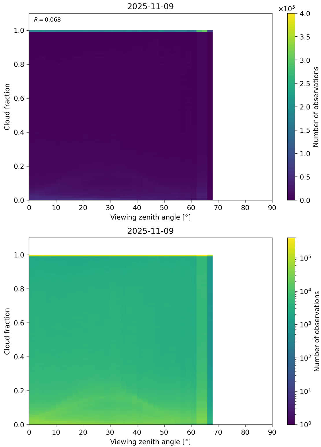
Figure 120: Scatter density plot of “Viewing zenith angle” against “Cloud fraction” for 2025-11-08 to 2025-11-10.
