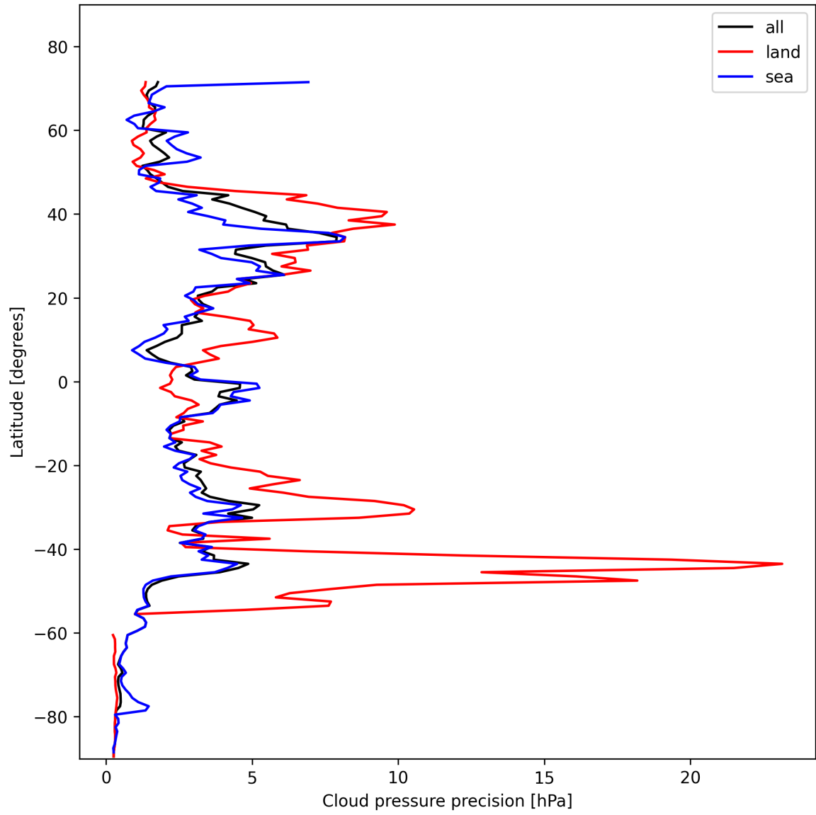
Figure 14: Zonal average of “Cloud pressure precision” for 2025-11-08 to 2025-11-10.
