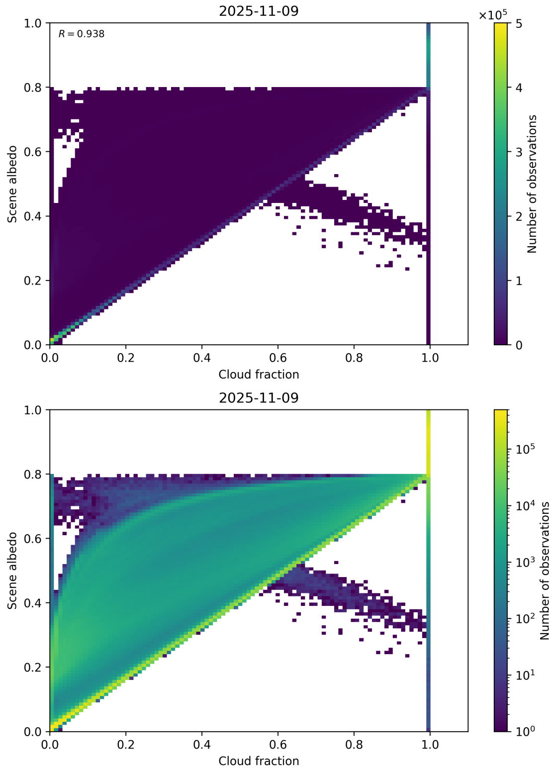
Figure 75: Scatter density plot of “Cloud fraction” against “Scene albedo” for 2025-11-08 to 2025-11-10.
