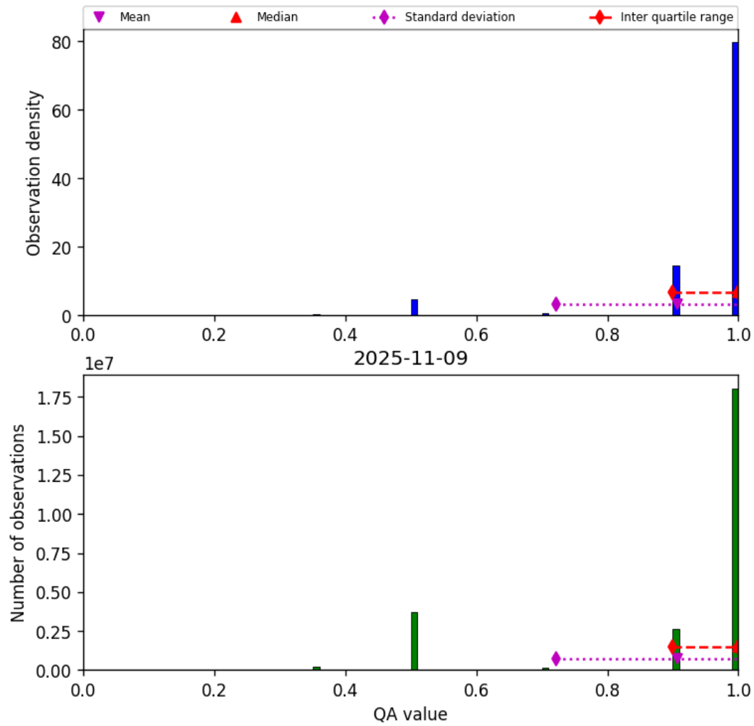
Figure 29: Histogram of “QA value” for 2025-11-08 to 2025-11-10
