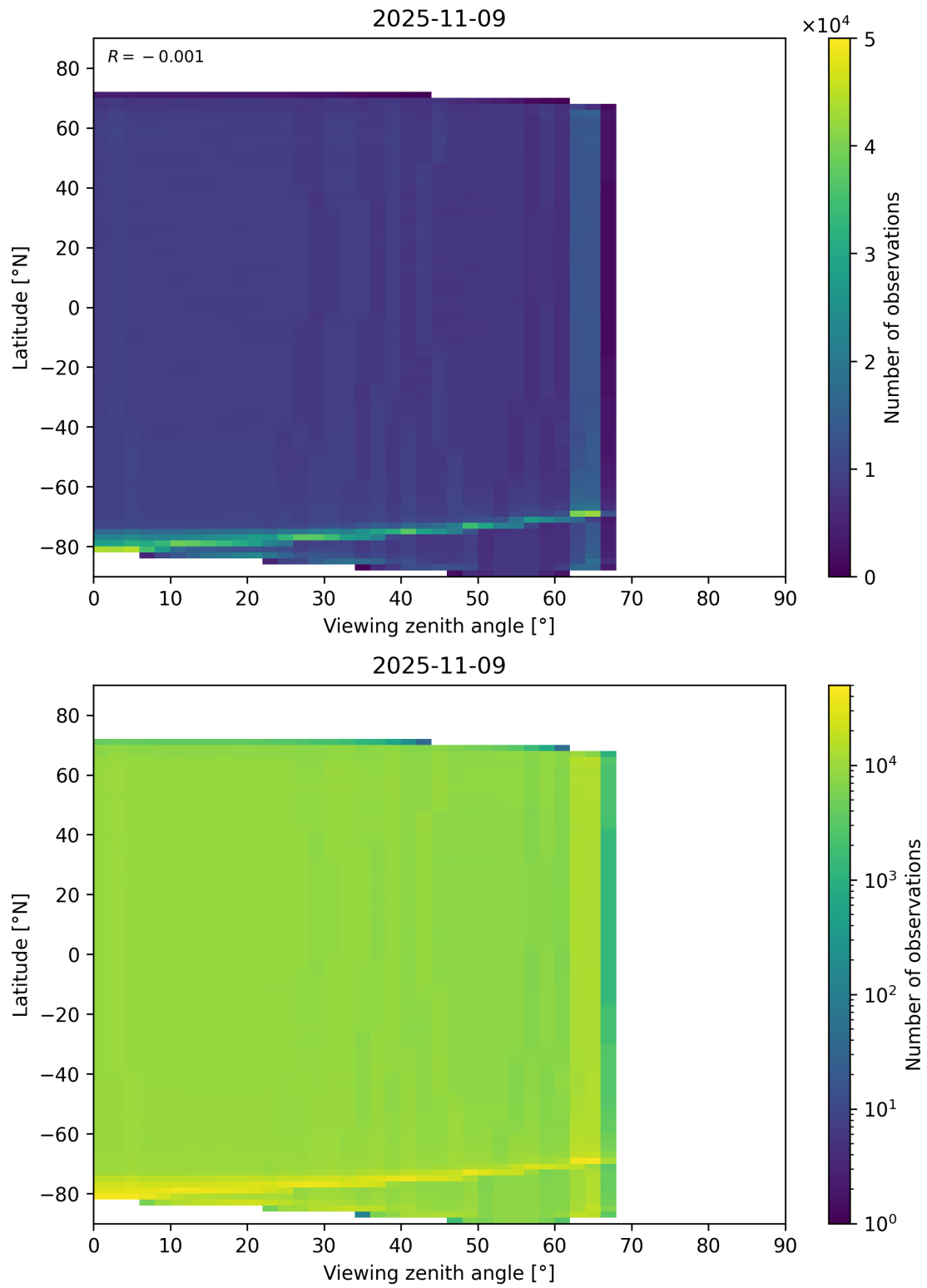
Figure 123: Scatter density plot of “Viewing zenith angle” against “Latitude” for 2025-11-08 to 2025-11-10.
