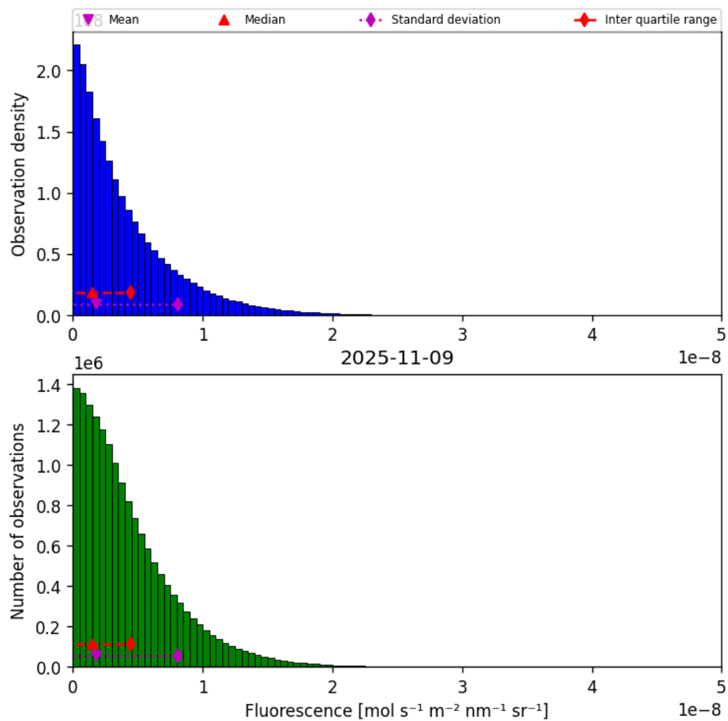
Figure 40: Histogram of “Fluorescence” for 2025-11-08 to 2025-11-10
