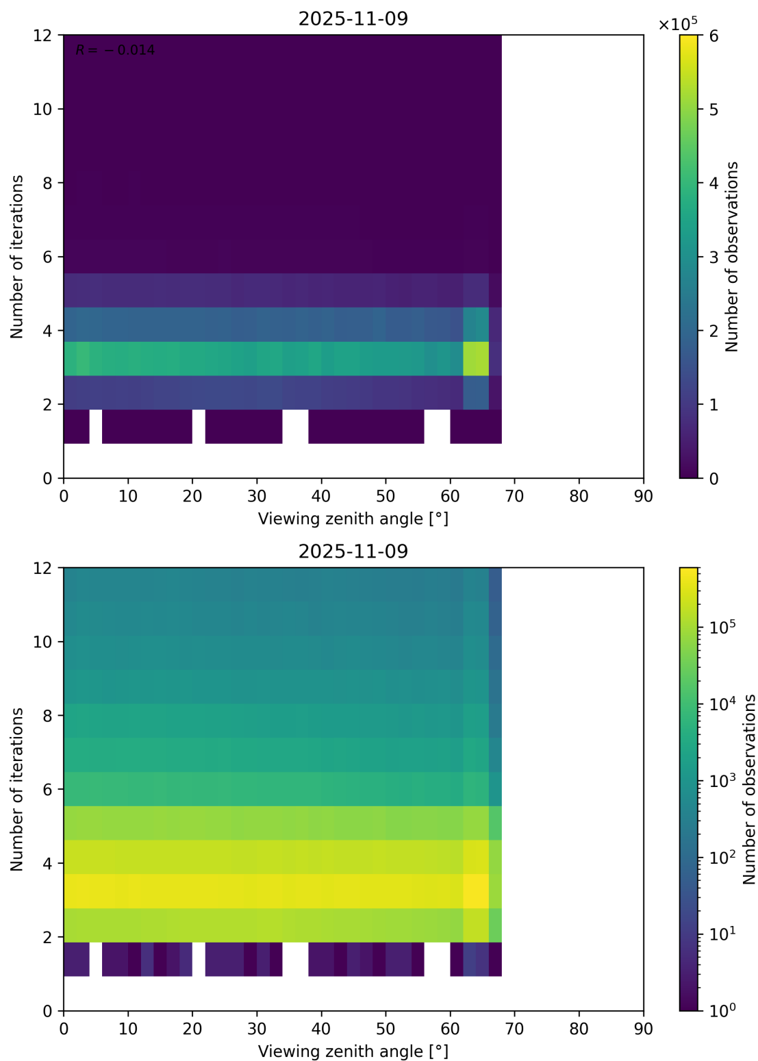
Figure 124: Scatter density plot of “Viewing zenith angle” against “Number of iterations” for 2025-11-08 to 2025-11-10.
