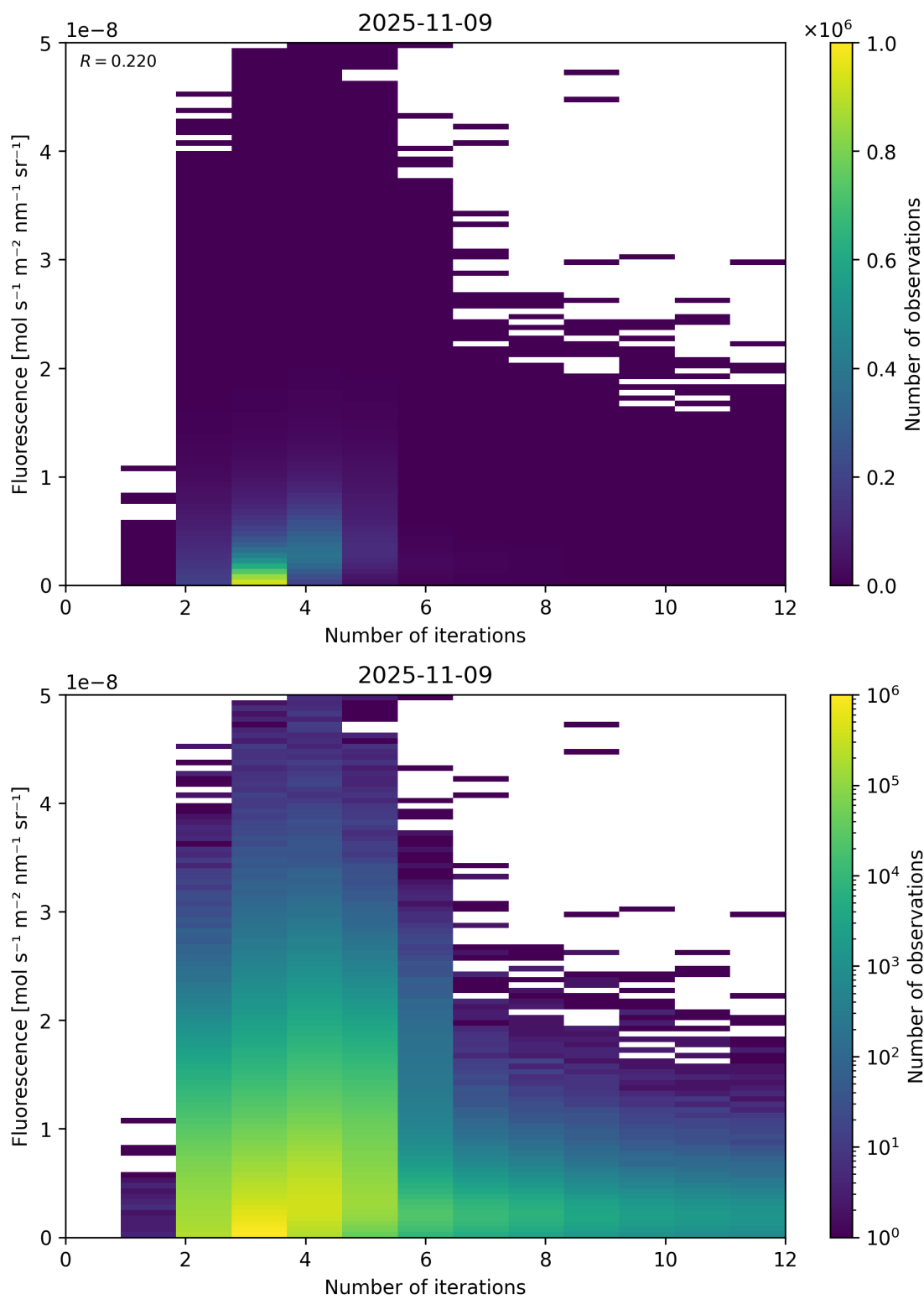
Figure 98: Scatter density plot of “Number of iterations” against “Fluorescence” for 2025-11-08 to 2025-11-10.
