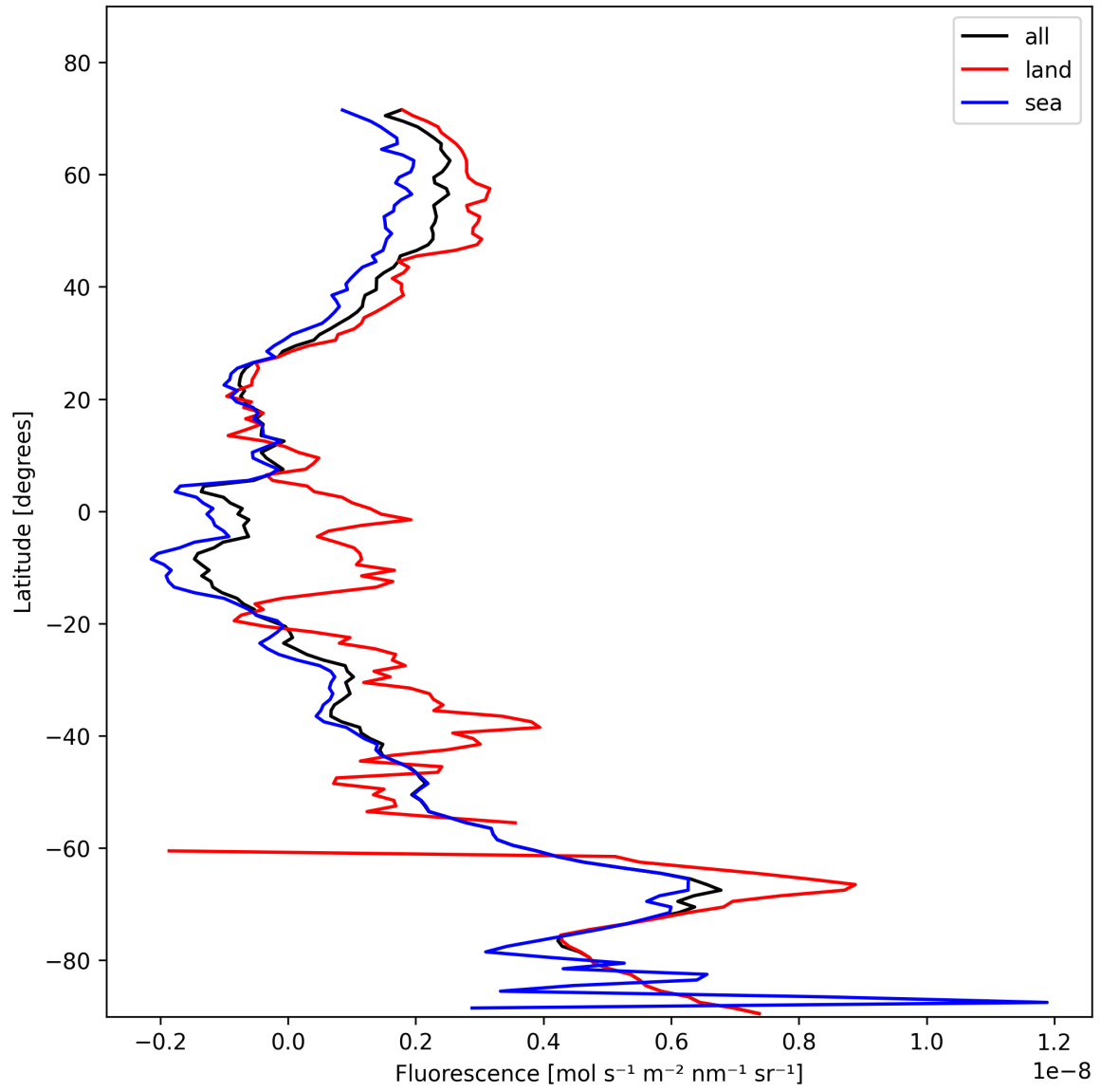
Figure 23: Zonal average of “Fluorescence” for 2025-11-08 to 2025-11-10.
