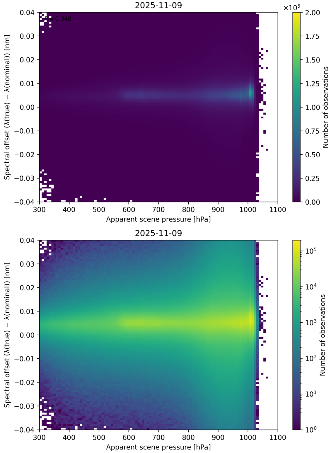
Figure 67: Scatter density plot of “Apparent scene pressure” against “Spectral offset ( \lambda_{\text{true}} - \lambda_{\text{nominal}} )” for 2025-11-08 to 2025-11-10.
