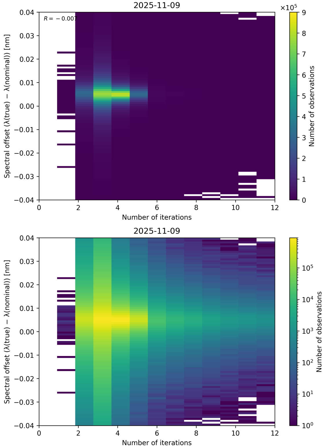
Figure 100: Scatter density plot of “Number of iterations” against “Spectral offset ( \lambda_{\text{true}} - \lambda_{\text{nominal}} )” for 2025-11-08 to 2025-11-10.
