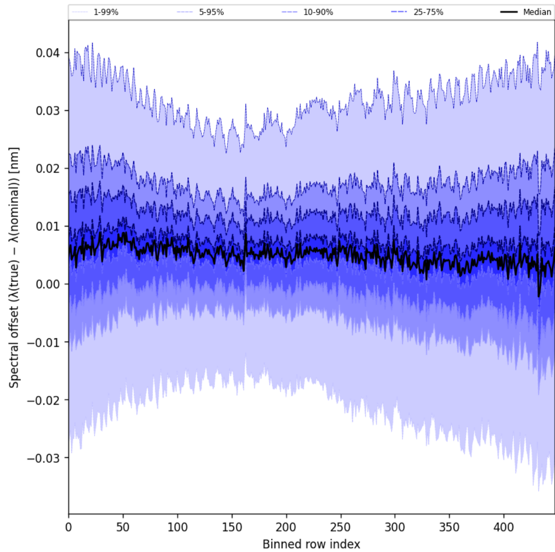
Figure 62: Along track statistics of “Spectral offset ( \lambda_{\text{true}} - \lambda_{\text{nominal}} )” for 2025-11-08 to 2025-11-10
