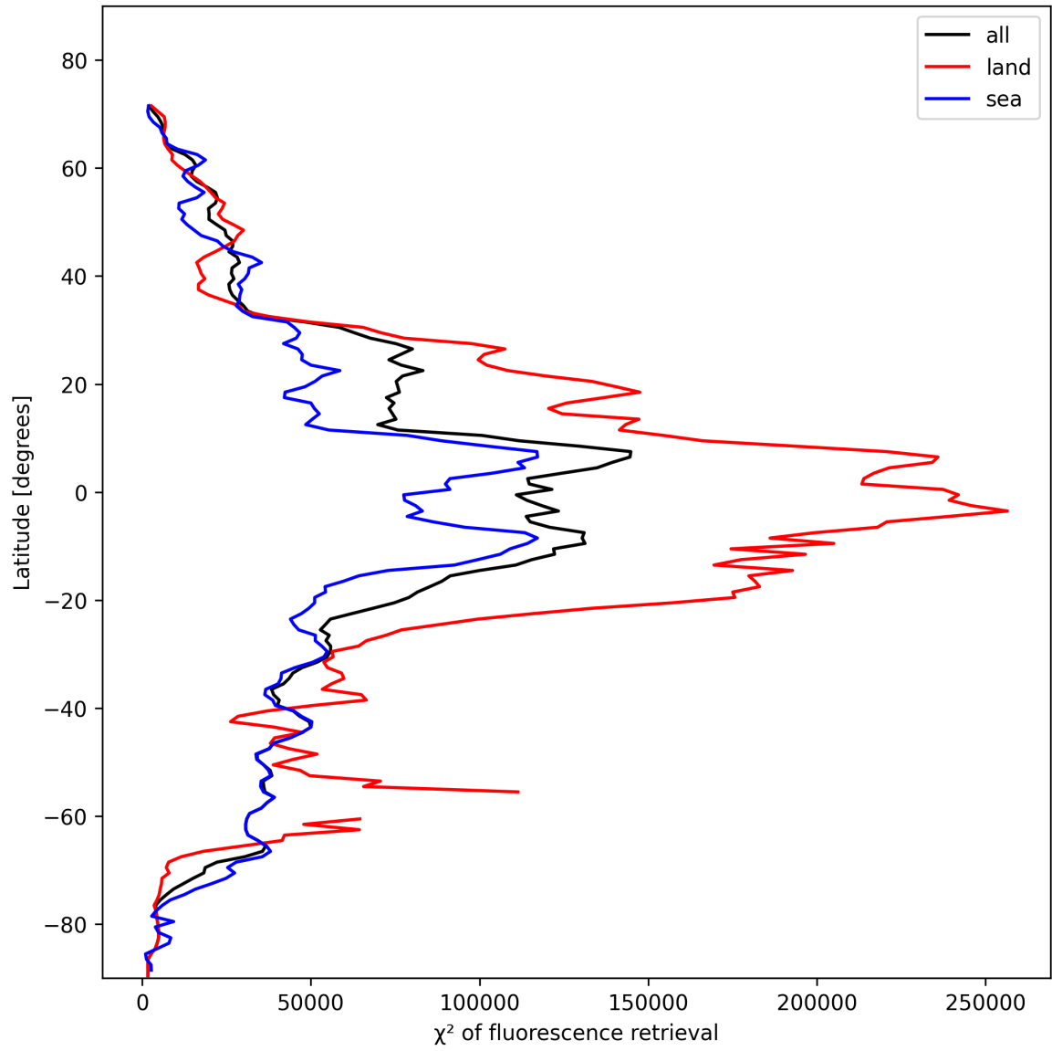
Figure 25: Zonal average of “ \chi^2 of fluorescence retrieval” for 2025-11-08 to 2025-11-10.
