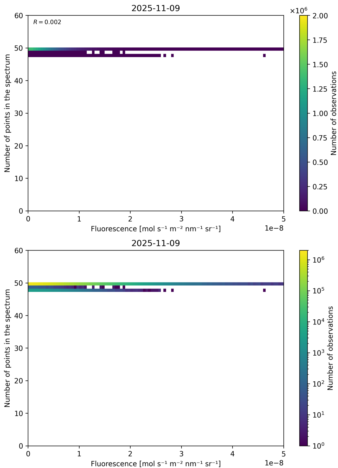
Figure 86: Scatter density plot of “Fluorescence” against “Number of points in the spectrum” for 2025-11-08 to 2025-11-10.
