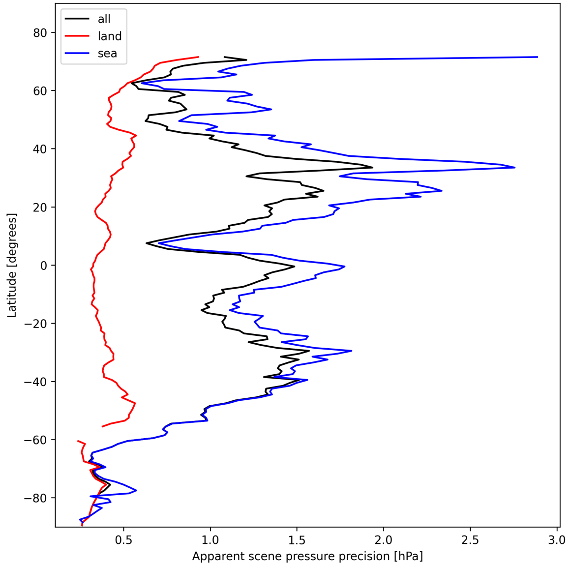
Figure 20: Zonal average of “Apparent scene pressure precision” for 2025-11-08 to 2025-11-10.
