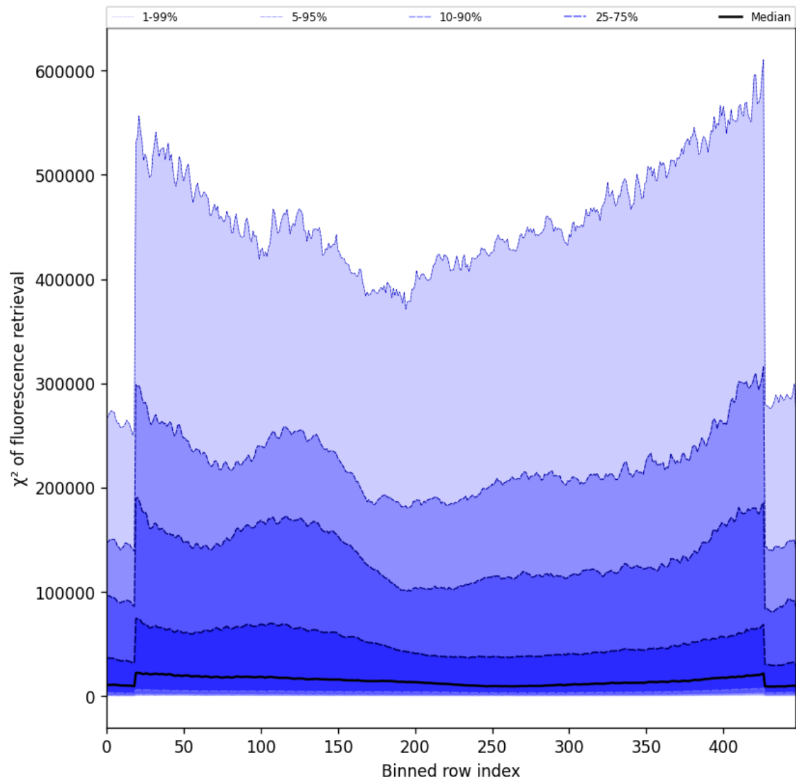
Figure 59: Along track statistics of “ \chi^2 of fluorescence retrieval” for 2025-11-08 to 2025-11-10
