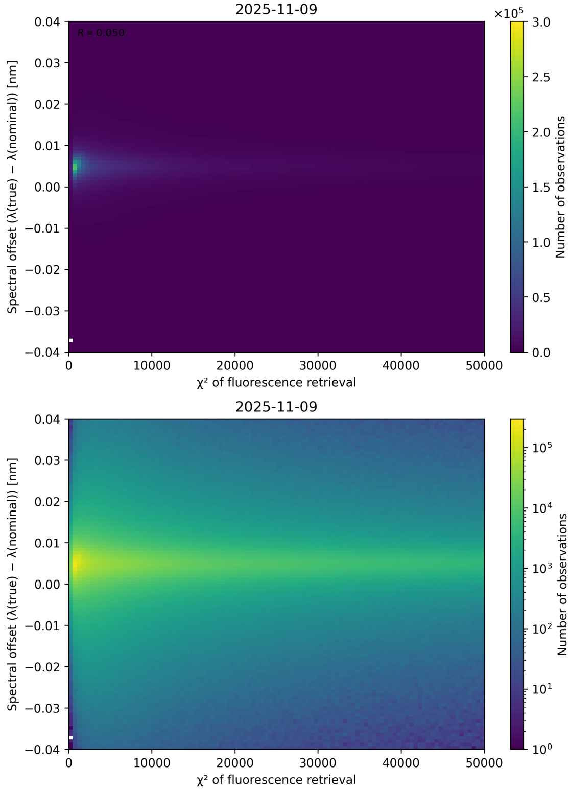
Figure 69: Scatter density plot of “ \chi^2 of fluorescence retrieval” against “Spectral offset ( \lambda_{\text{true}} - \lambda_{\text{nominal}} )” for 2025-11-08 to 2025-11-10.
