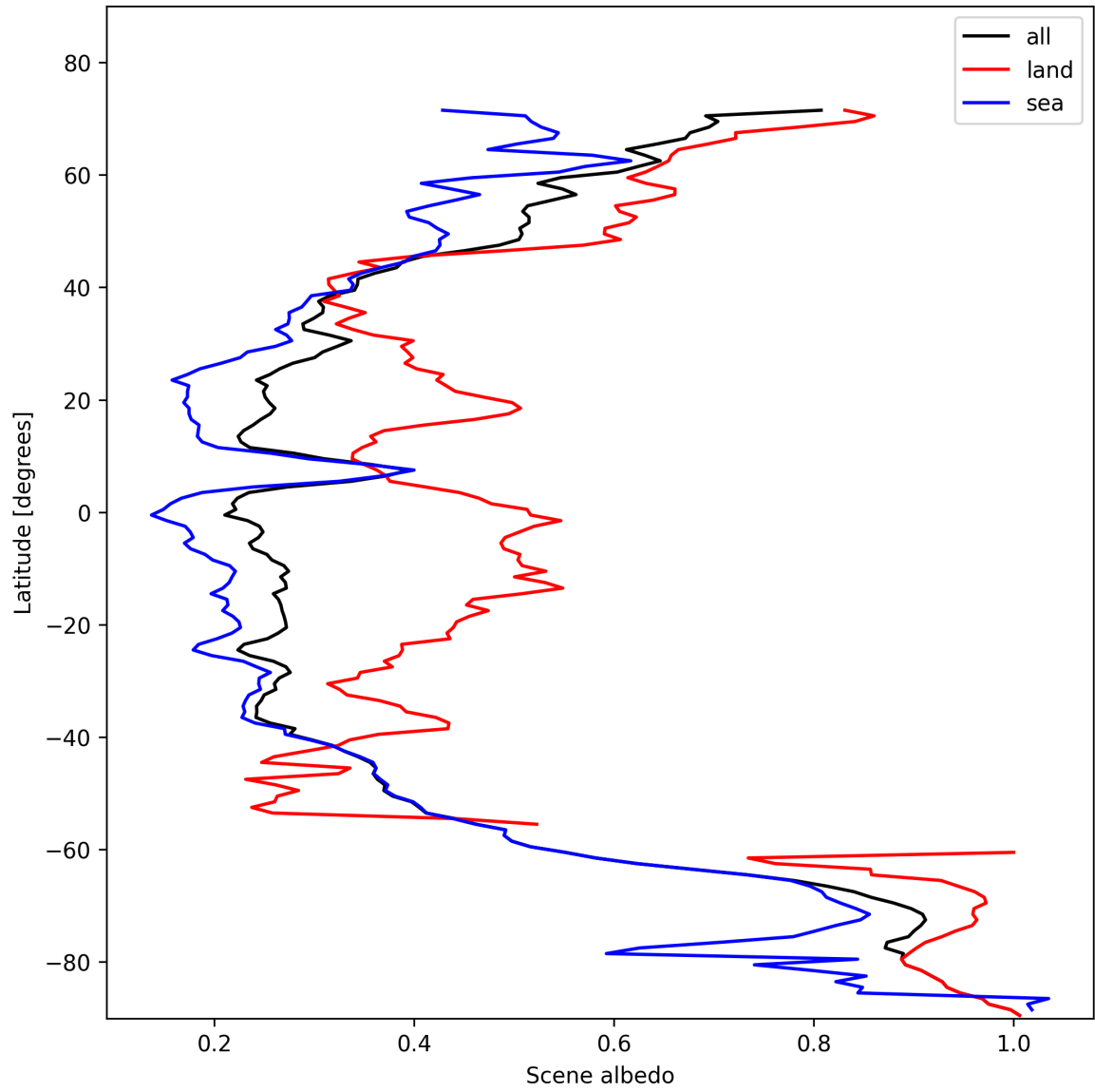
Figure 17: Zonal average of “Scene albedo” for 2025-11-08 to 2025-11-10.
