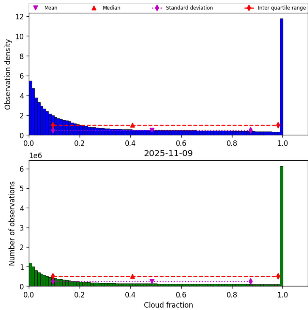
Figure 32: Histogram of “Cloud fraction” for 2025-11-08 to 2025-11-10
