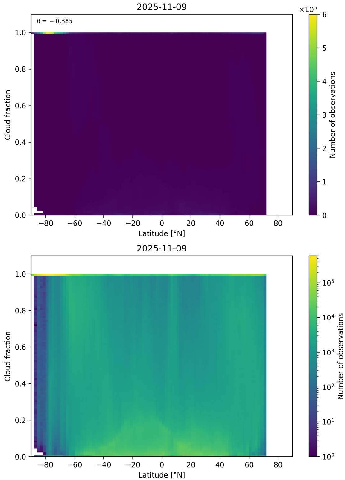
Figure 90: Scatter density plot of “Latitude” against “Cloud fraction” for 2025-11-08 to 2025-11-10.
