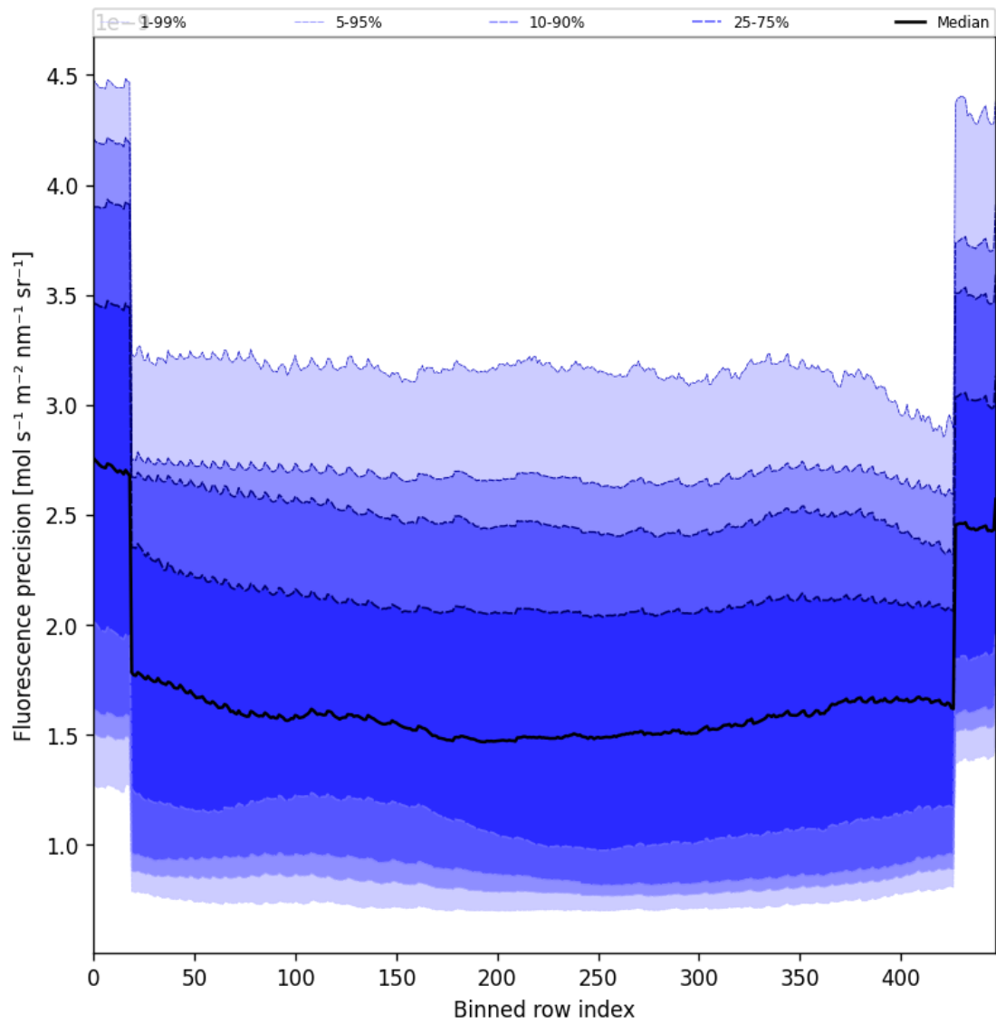
Figure 58: Along track statistics of “Fluorescence precision” for 2025-11-09 to 2025-11-11
