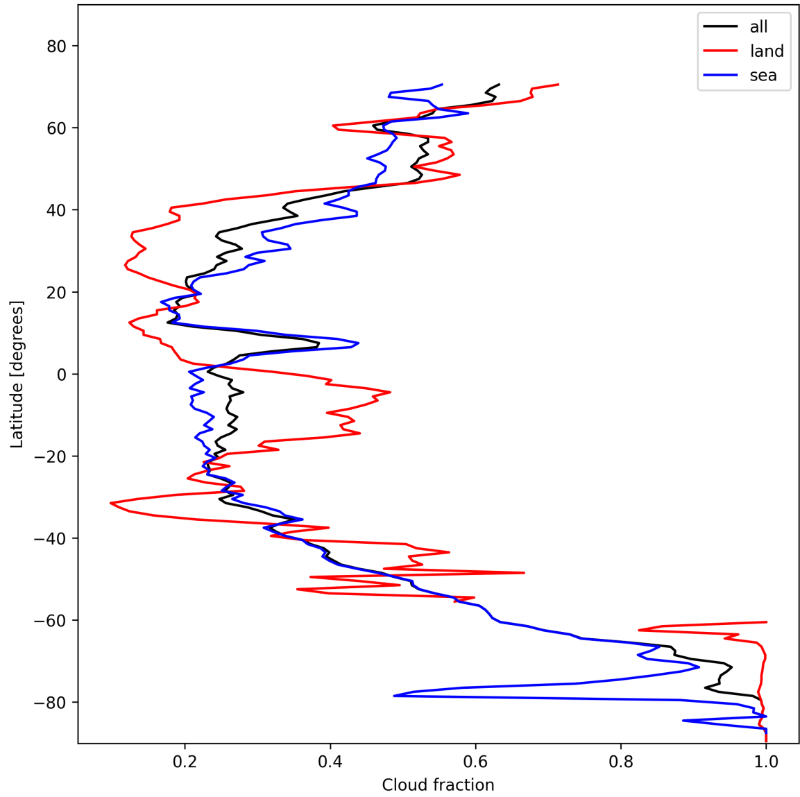
Figure 15: Zonal average of “Cloud fraction” for 2025-11-09 to 2025-11-11.
