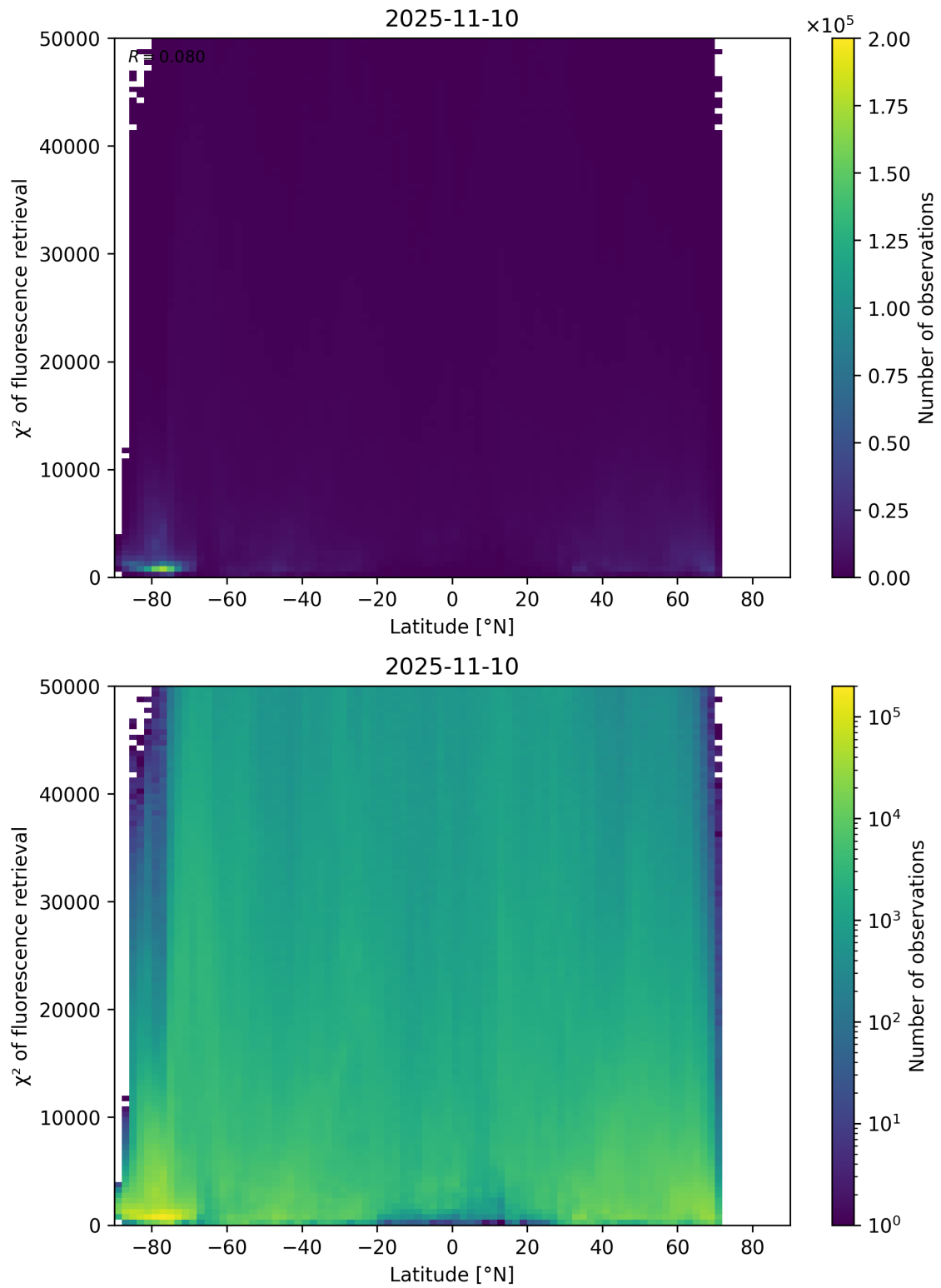
Figure 89: Scatter density plot of “Latitude” against “ \chi^2 of fluorescence retrieval” for 2025-11-09 to 2025-11-11.
