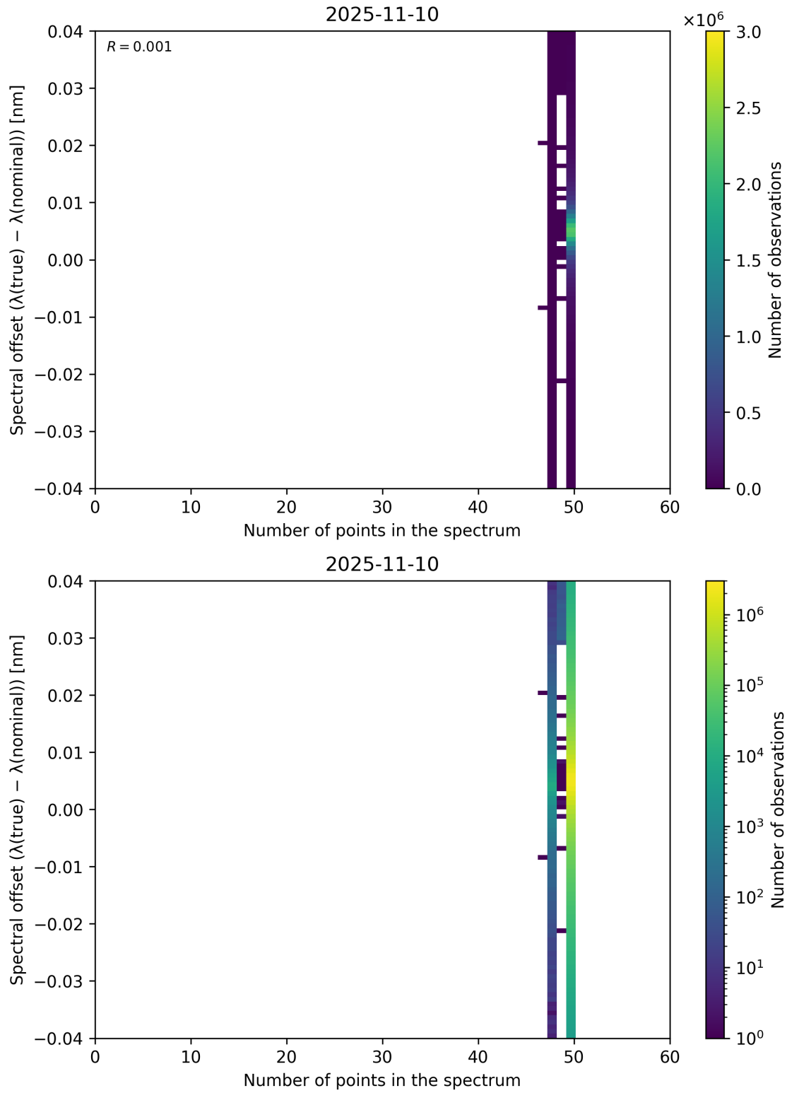
Figure 101: Scatter density plot of “Number of points in the spectrum” against “Spectral offset ( \lambda_{\text{true}} - \lambda_{\text{nominal}} )” for 2025-11-09 to 2025-11-11.
