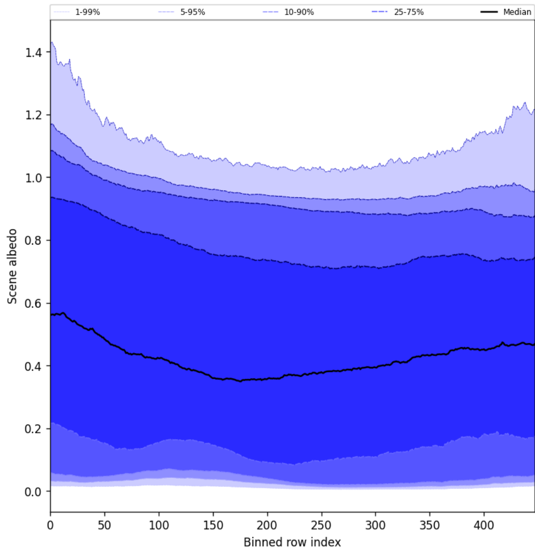
Figure 51: Along track statistics of “Scene albedo” for 2025-11-09 to 2025-11-11
