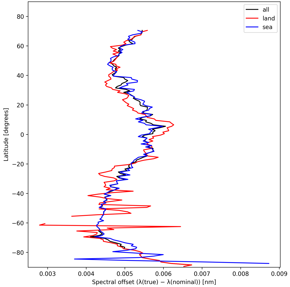
Figure 28: Zonal average of “Spectral offset ( \lambda_{\text{true}} - \lambda_{\text{nominal}} )” for 2025-11-09 to 2025-11-11.
