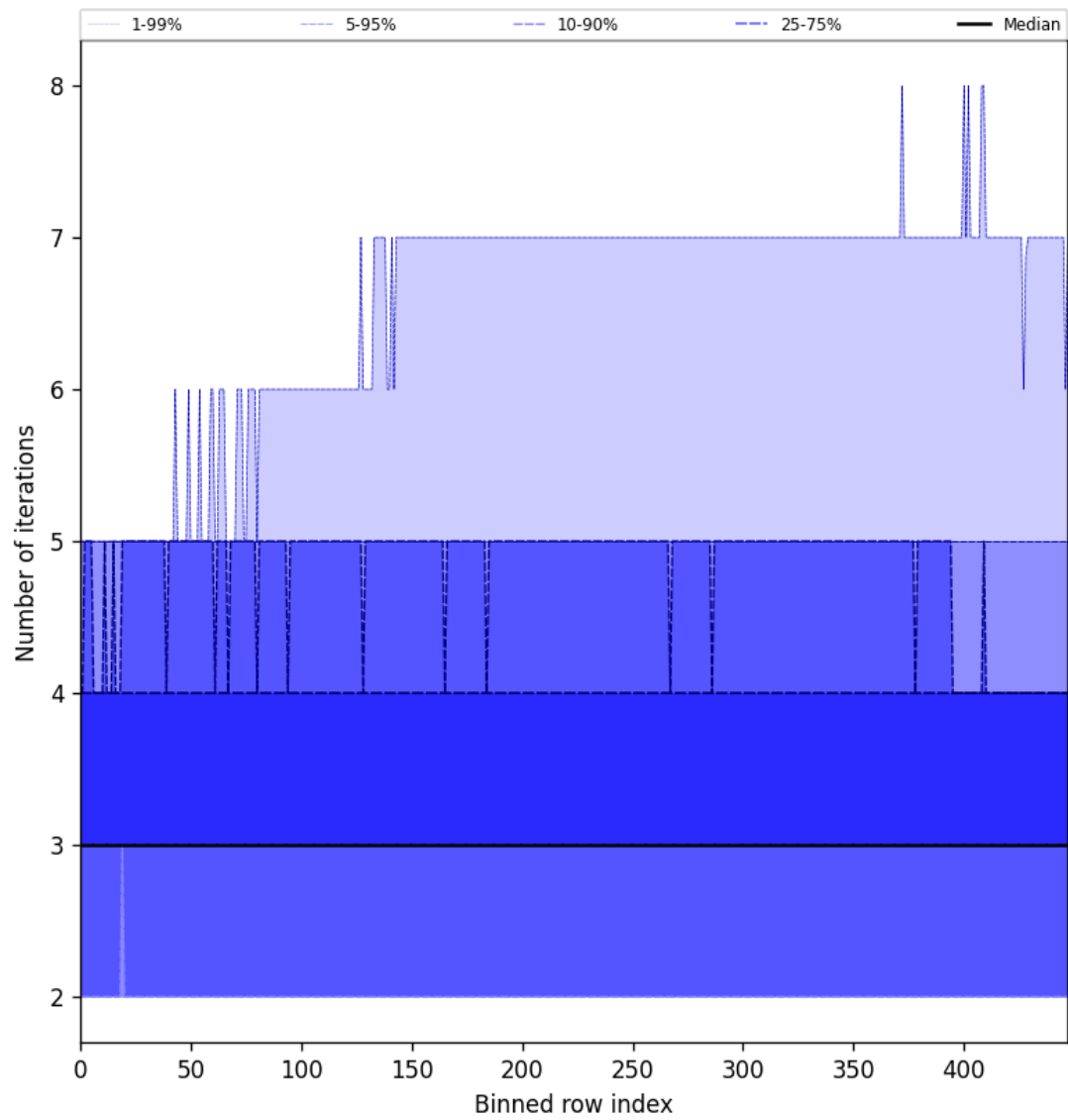
Figure 56: Along track statistics of “Number of iterations” for 2025-11-09 to 2025-11-11
