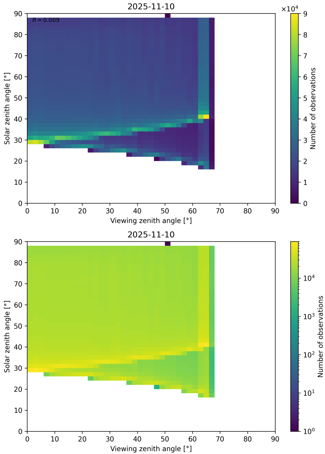
Figure 127: Scatter density plot of “Viewing zenith angle” against “Solar zenith angle” for 2025-11-09 to 2025-11-11.
