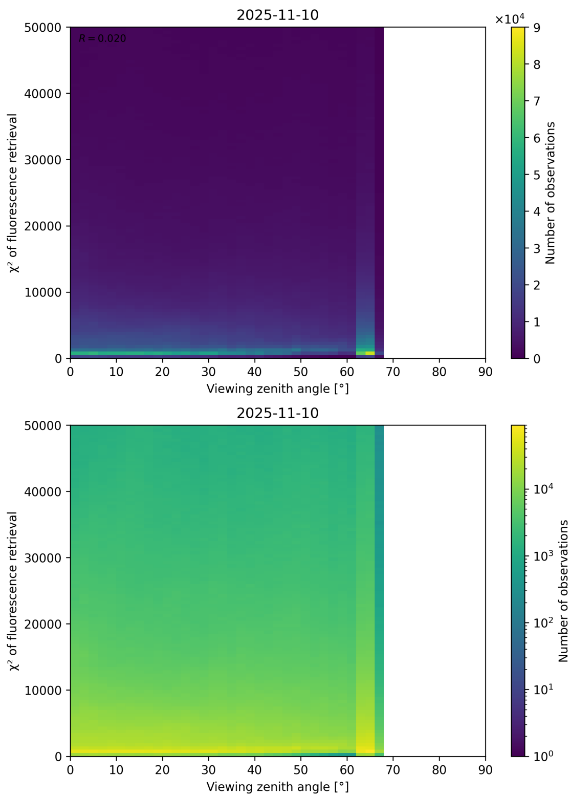
Figure 119: Scatter density plot of “Viewing zenith angle” against “ \chi^2 of fluorescence retrieval” for 2025-11-09 to 2025-11-11.
