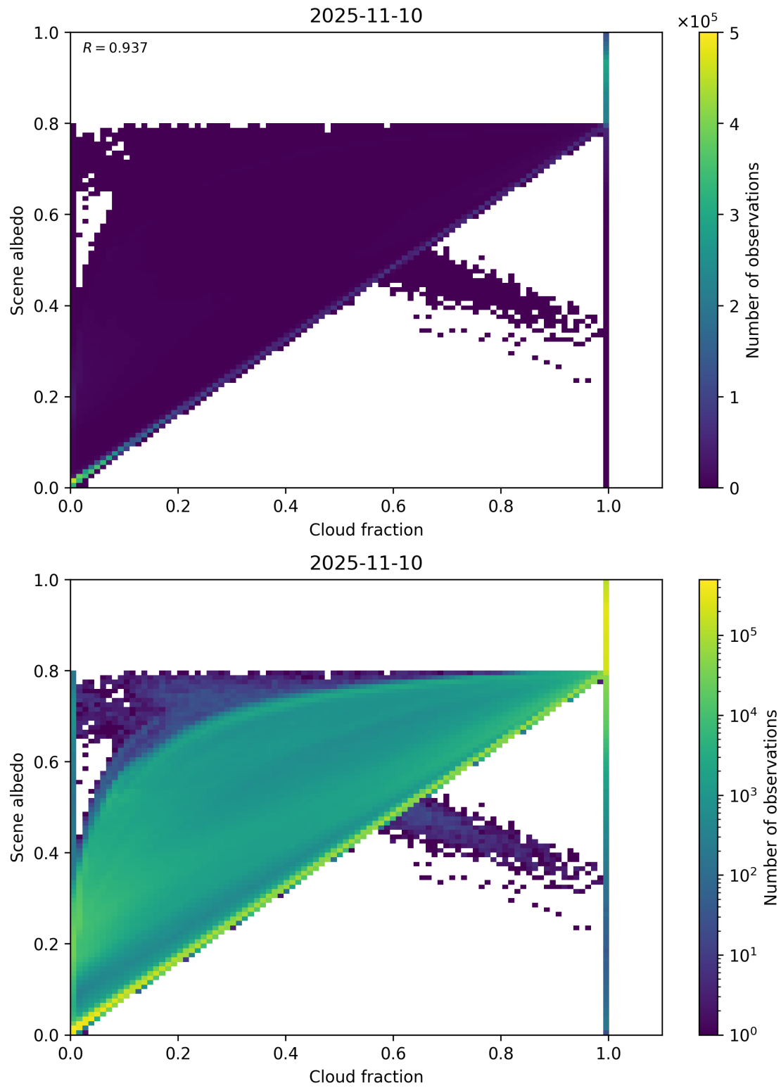
Figure 75: Scatter density plot of “Cloud fraction” against “Scene albedo” for 2025-11-09 to 2025-11-11.
