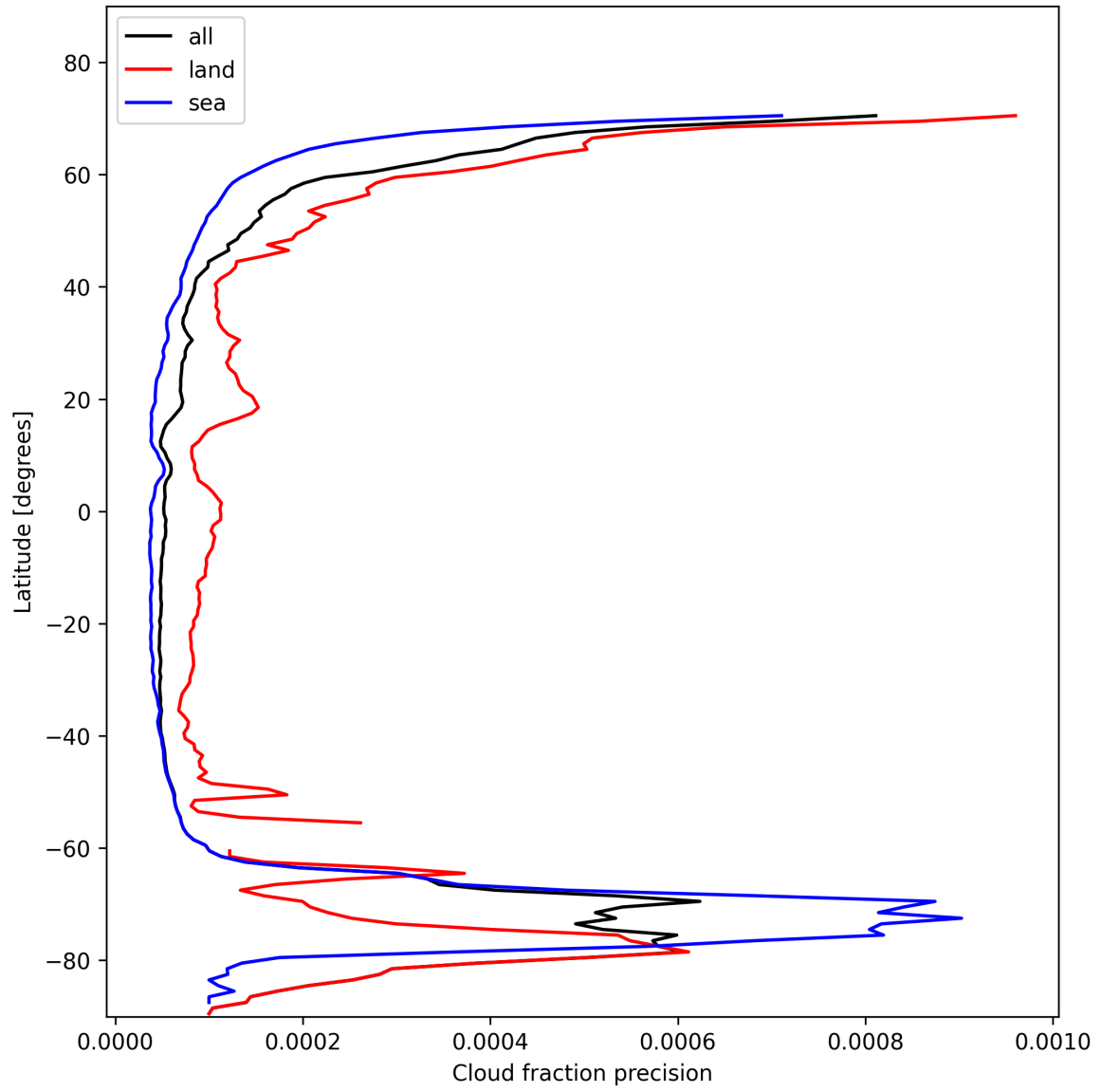
Figure 16: Zonal average of “Cloud fraction precision” for 2025-11-09 to 2025-11-11.
