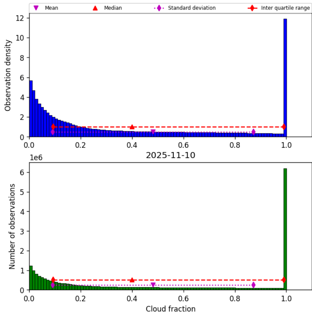
Figure 32: Histogram of “Cloud fraction” for 2025-11-09 to 2025-11-11
