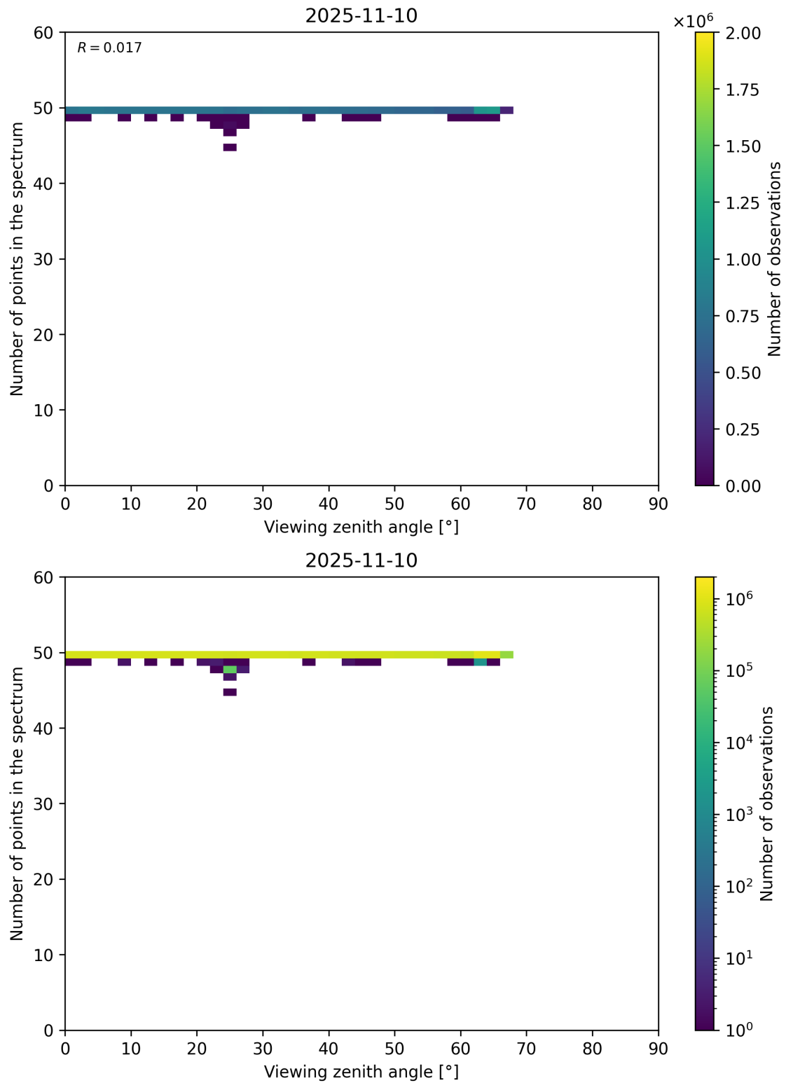
Figure 125: Scatter density plot of “Viewing zenith angle” against “Number of points in the spectrum” for 2025-11-09 to 2025-11-11.
