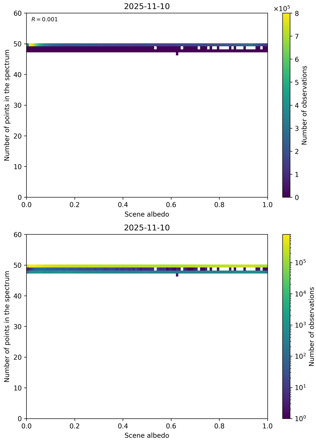
Figure 106: Scatter density plot of “Scene albedo” against “Number of points in the spectrum” for 2025-11-09 to 2025-11-11.
