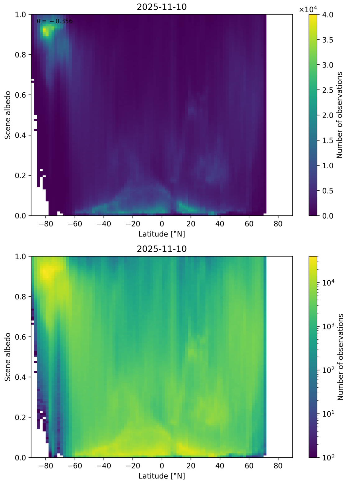
Figure 95: Scatter density plot of “Latitude” against “Scene albedo” for 2025-11-09 to 2025-11-11.
