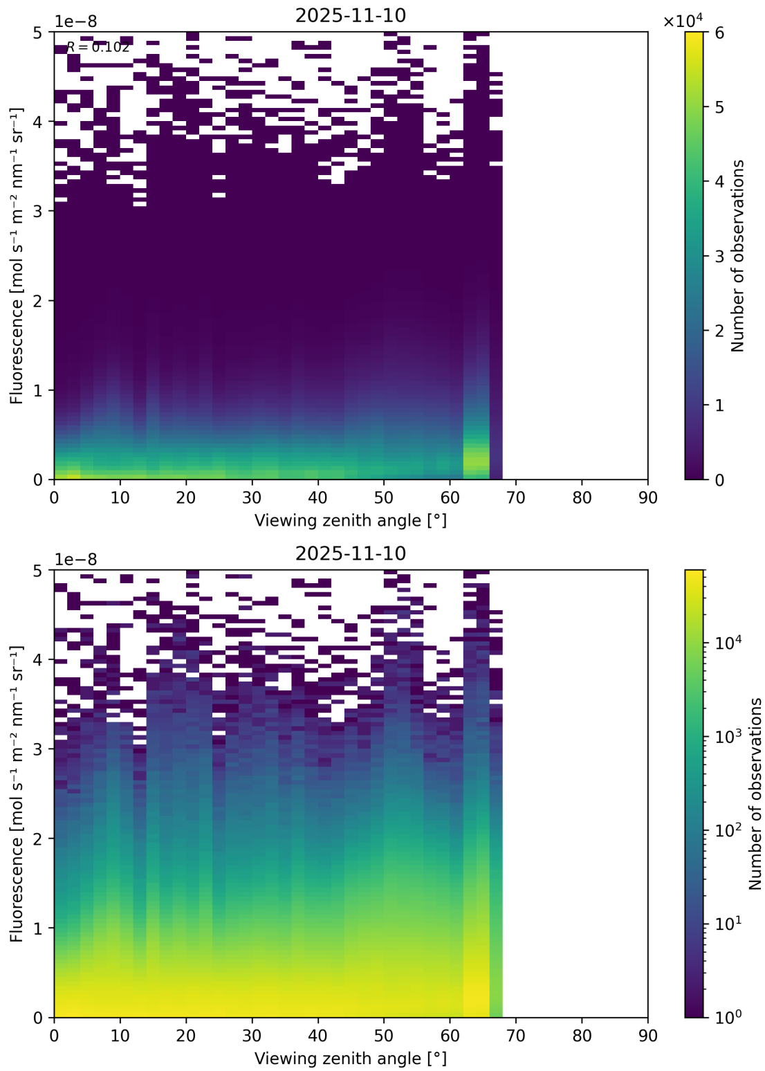
Figure 122: Scatter density plot of “Viewing zenith angle” against “Fluorescence” for 2025-11-09 to 2025-11-11.
