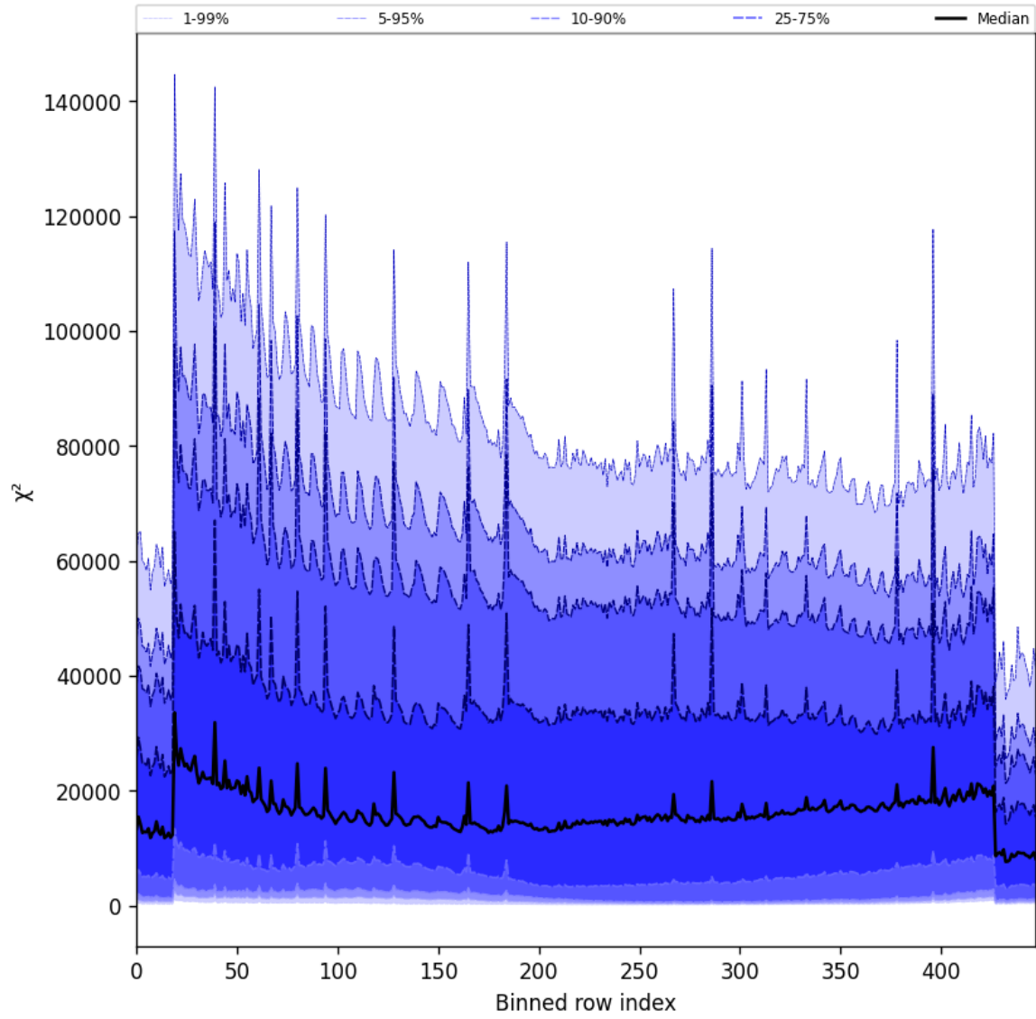
Figure 55: Along track statistics of “ \chi^2 ” for 2025-11-09 to 2025-11-11
