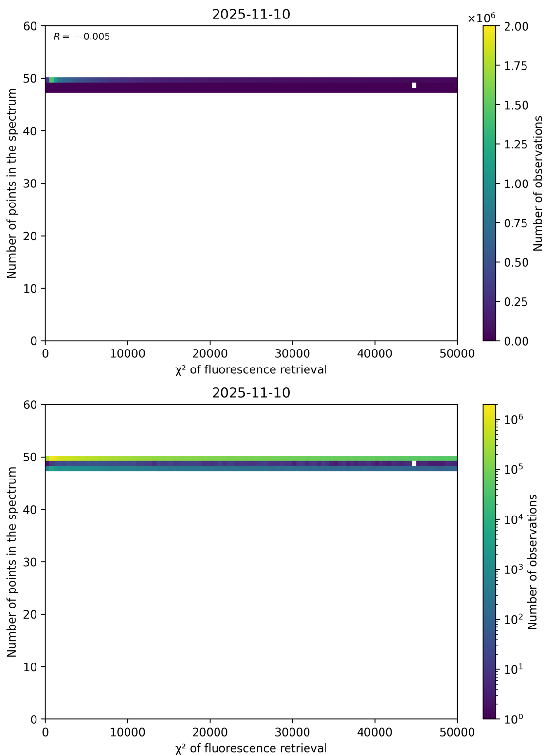
Figure 68: Scatter density plot of " \chi^2 of fluorescence retrieval" against "Number of points in the spectrum" for 2025-11-09 to 2025-11-11.
