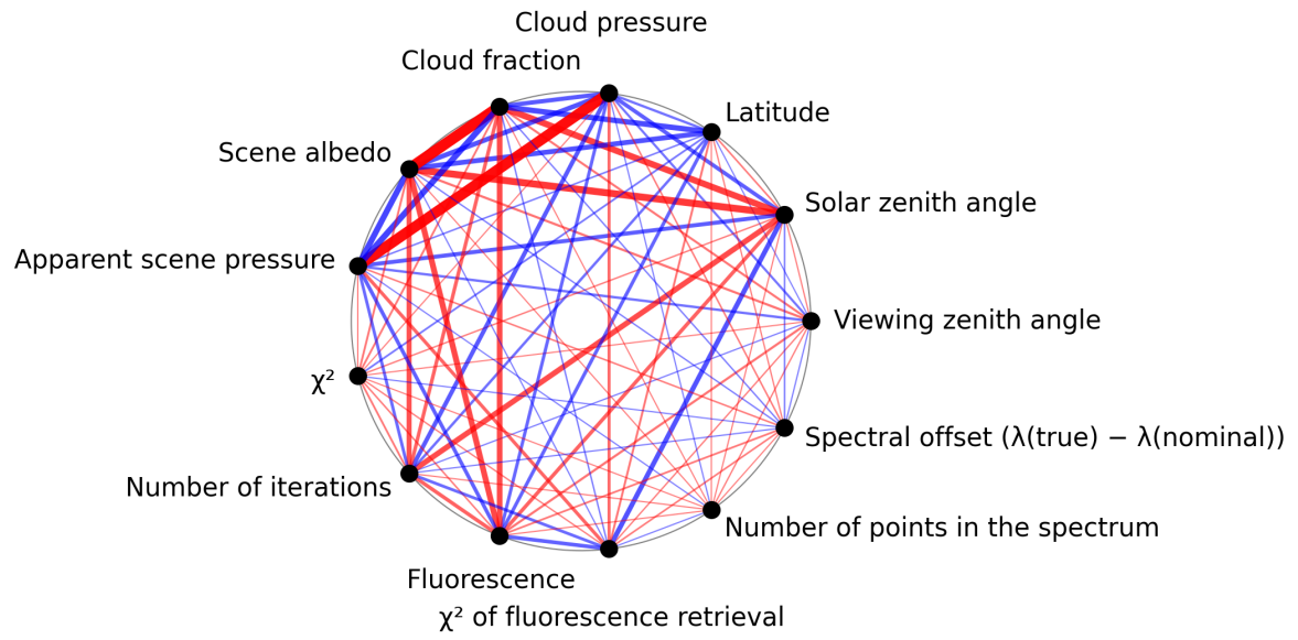
Figure 1: Map of correlation graph for 2025-11-09 to 2025-11-11.
