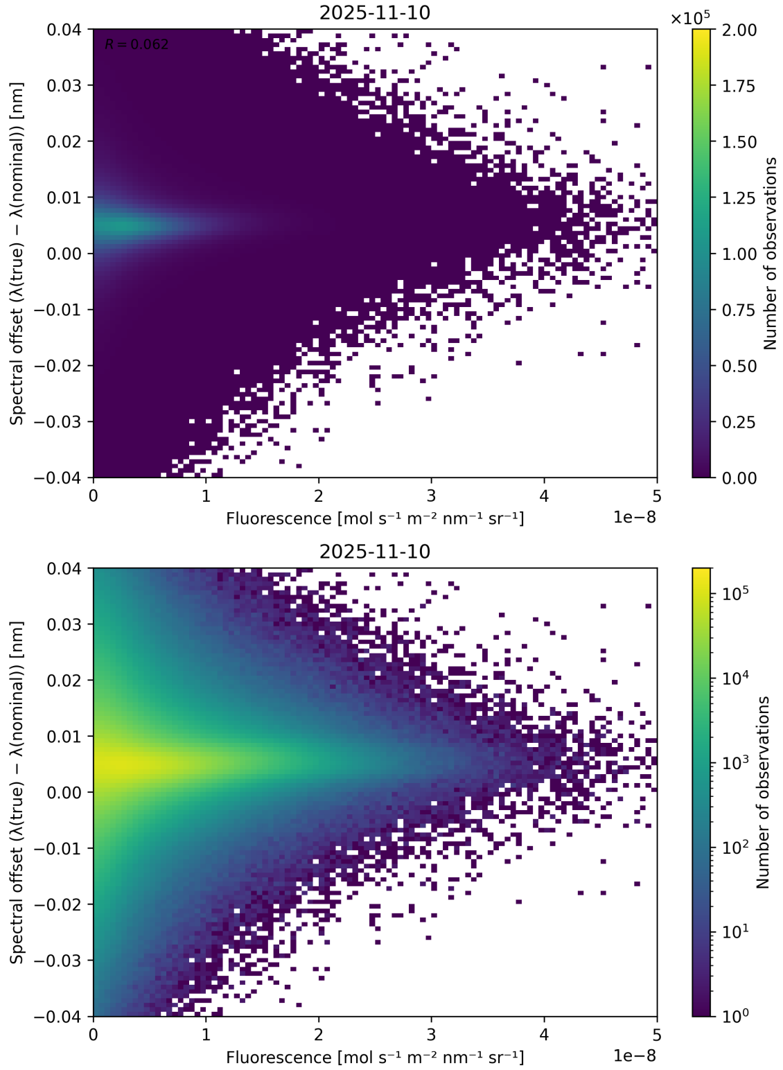
Figure 87: Scatter density plot of “Fluorescence” against “Spectral offset ( \lambda_{\text{true}} - \lambda_{\text{nominal}} )” for 2025-11-09 to 2025-11-11.
