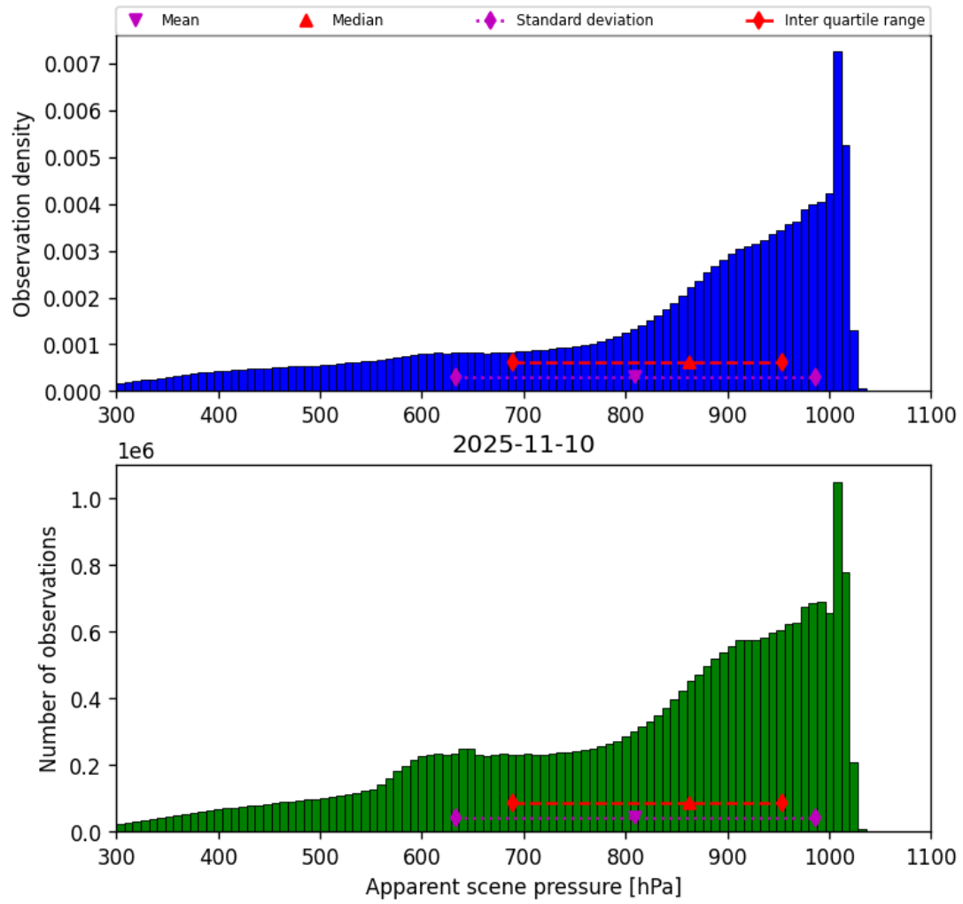
Figure 36: Histogram of “Apparent scene pressure” for 2025-11-09 to 2025-11-11
