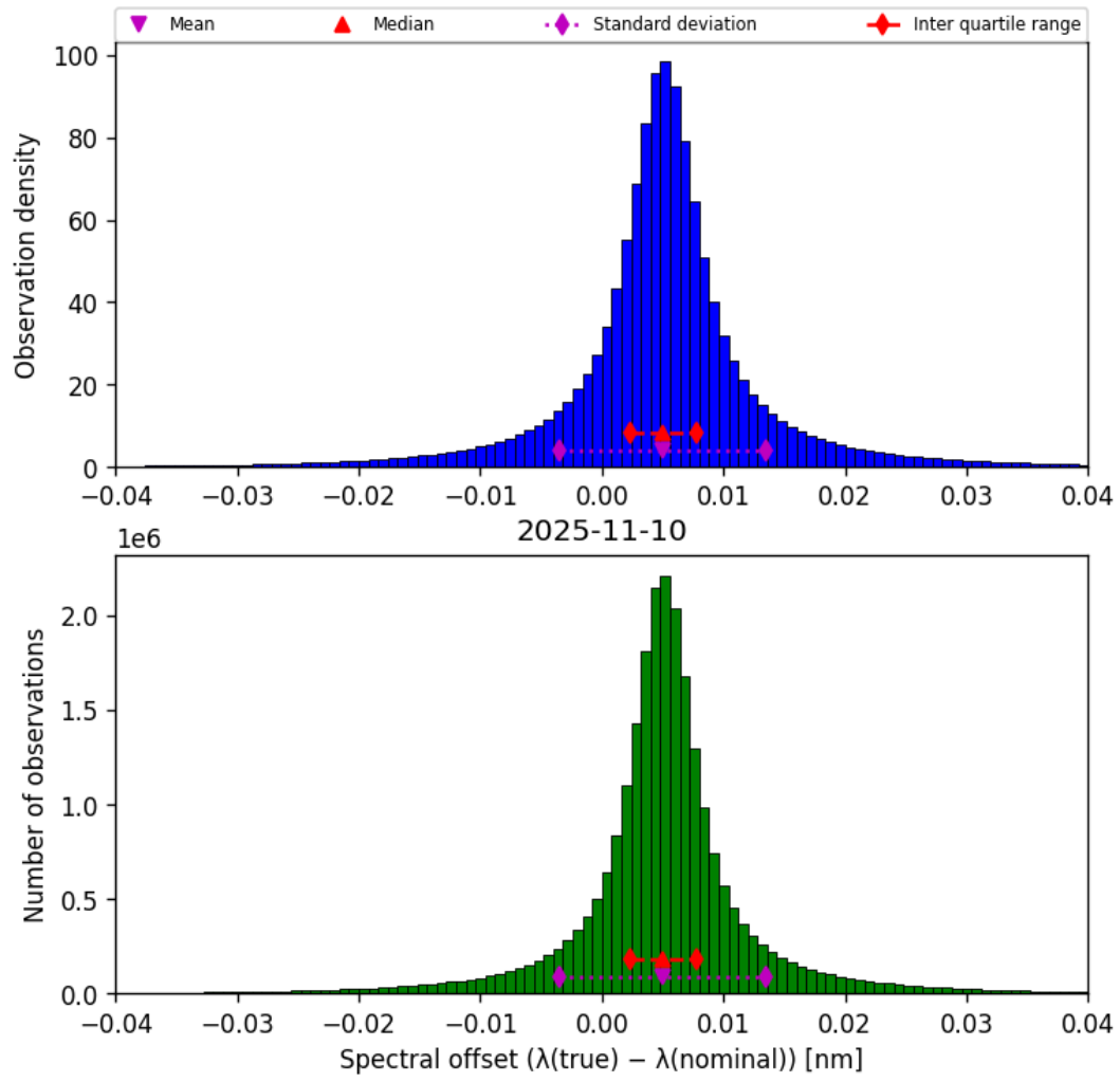
Figure 45: Histogram of “Spectral offset ( \lambda_{\text{true}} - \lambda_{\text{nominal}} )” for 2025-11-09 to 2025-11-11
