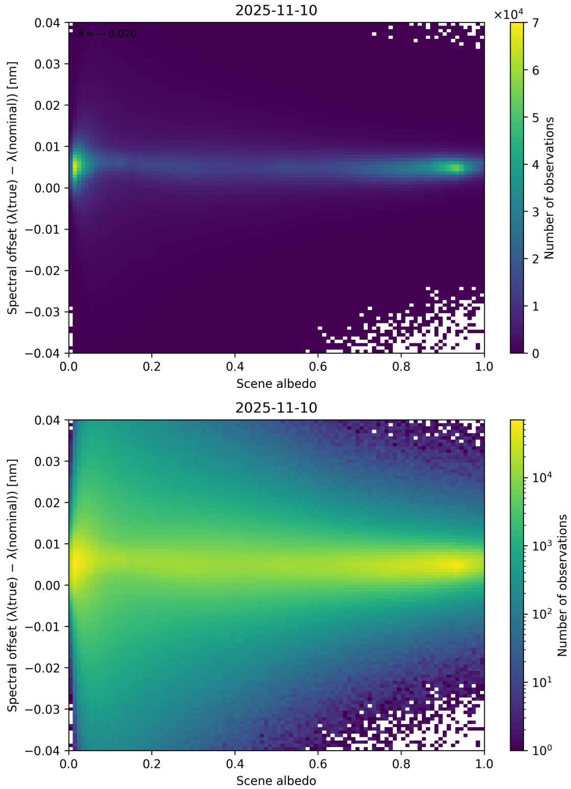
Figure 107: Scatter density plot of “Scene albedo” against “Spectral offset ( \lambda_{\text{true}} - \lambda_{\text{nominal}} )” for 2025-11-09 to 2025-11-11.
