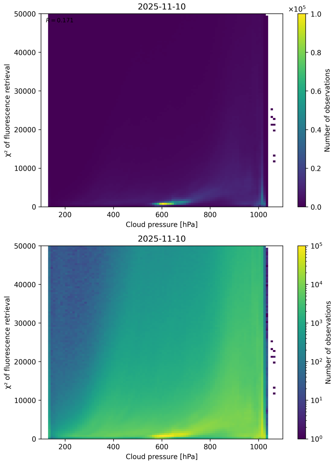
Figure 78: Scatter density plot of “Cloud pressure” against “ \chi^2 of fluorescence retrieval” for 2025-11-09 to 2025-11-11.
