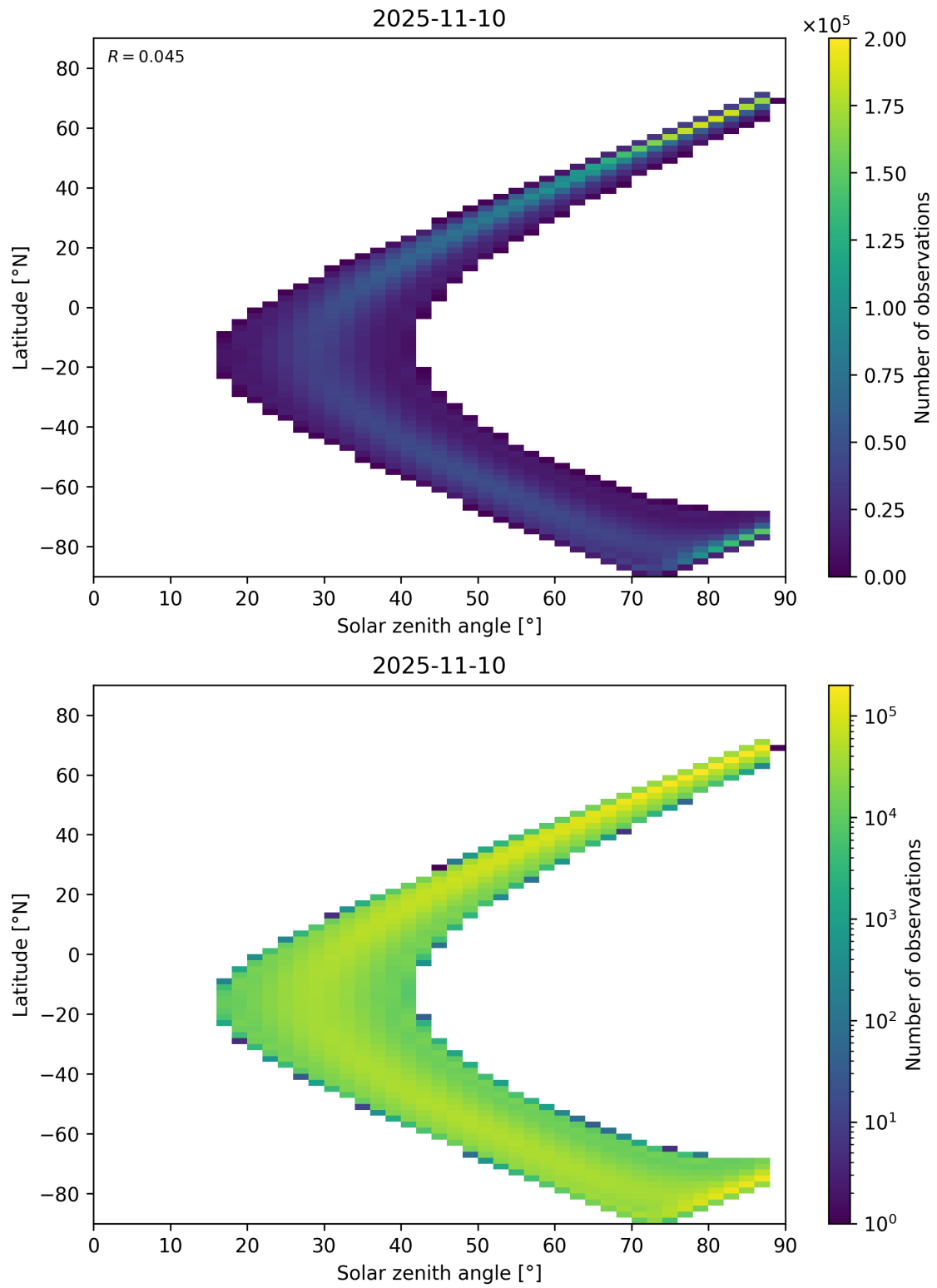
Figure 113: Scatter density plot of “Solar zenith angle” against “Latitude” for 2025-11-09 to 2025-11-11.
