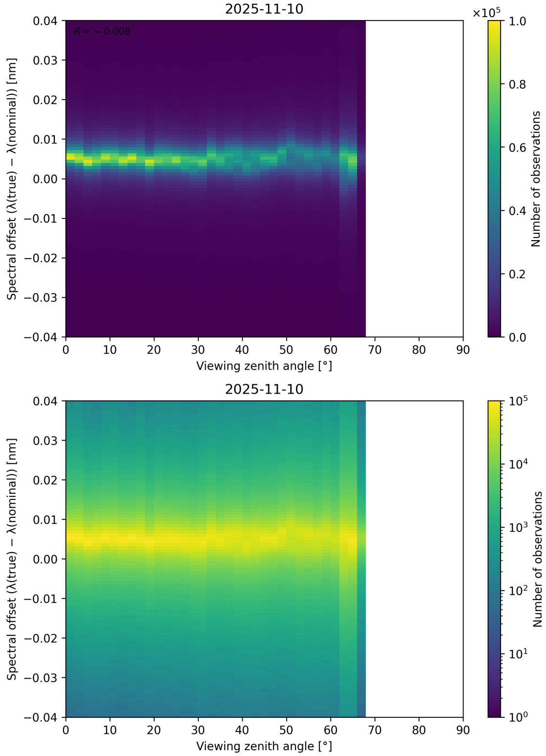
Figure 128: Scatter density plot of “Viewing zenith angle” against “Spectral offset ( \lambda_{\text{true}} - \lambda_{\text{nominal}} )” for 2025-11-09 to 2025-11-11.
