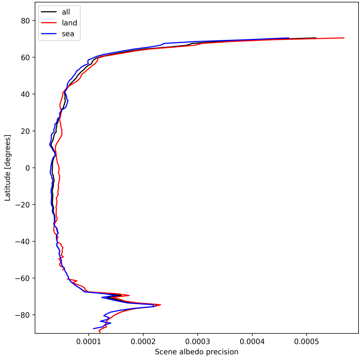
Figure 18: Zonal average of “Scene albedo precision” for 2025-11-09 to 2025-11-11.
