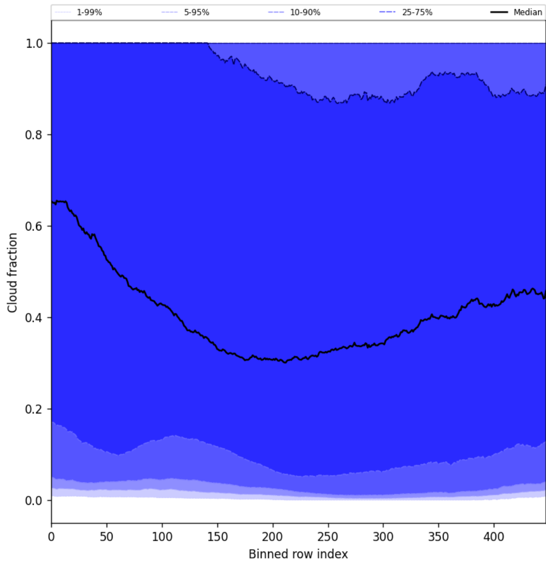
Figure 49: Along track statistics of “Cloud fraction” for 2025-11-09 to 2025-11-11
