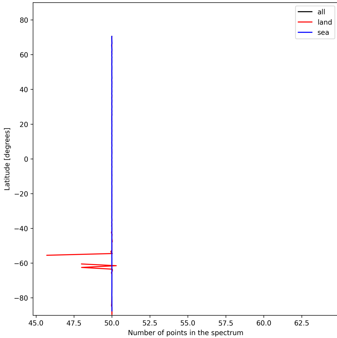
Figure 27: Zonal average of “Number of points in the spectrum” for 2025-11-09 to 2025-11-11.
