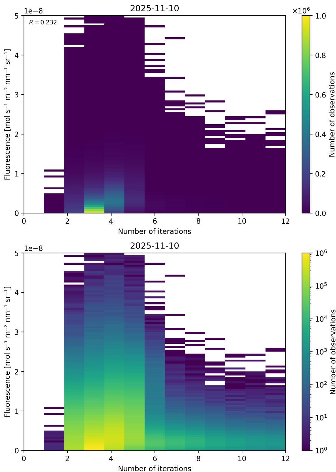
Figure 98: Scatter density plot of “Number of iterations” against “Fluorescence” for 2025-11-09 to 2025-11-11.
