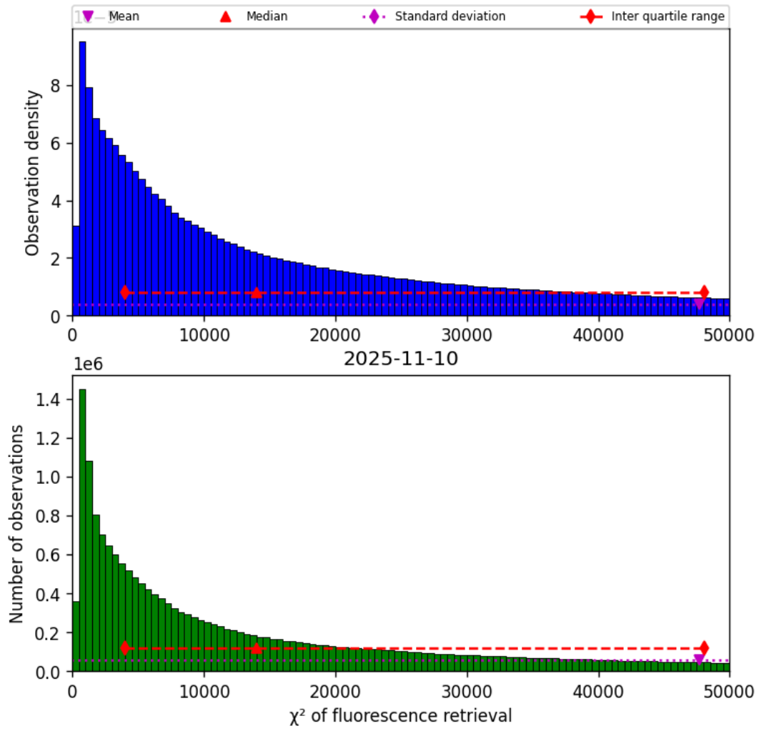
Figure 42: Histogram of “ \chi^2 of fluorescence retrieval” for 2025-11-09 to 2025-11-11
