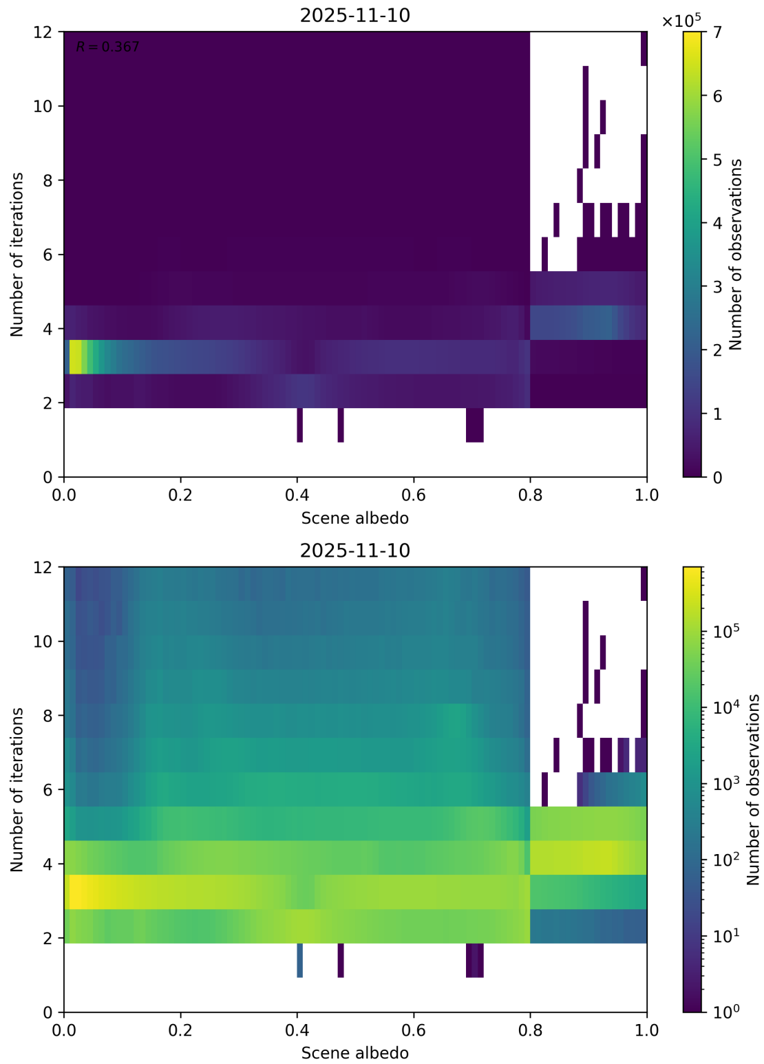
Figure 105: Scatter density plot of “Scene albedo” against “Number of iterations” for 2025-11-09 to 2025-11-11.
