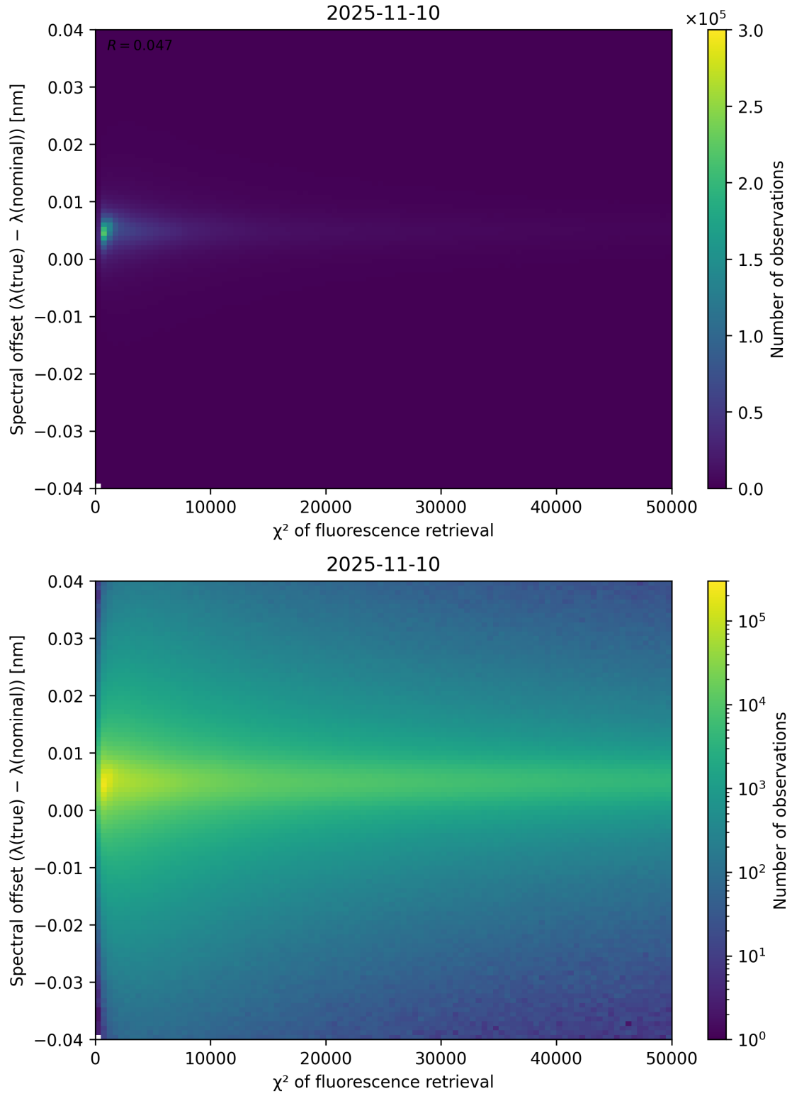
Figure 69: Scatter density plot of “ \chi^2 of fluorescence retrieval” against “Spectral offset ( \lambda_{\text{true}} - \lambda_{\text{nominal}} )” for 2025-11-09 to 2025-11-11.
