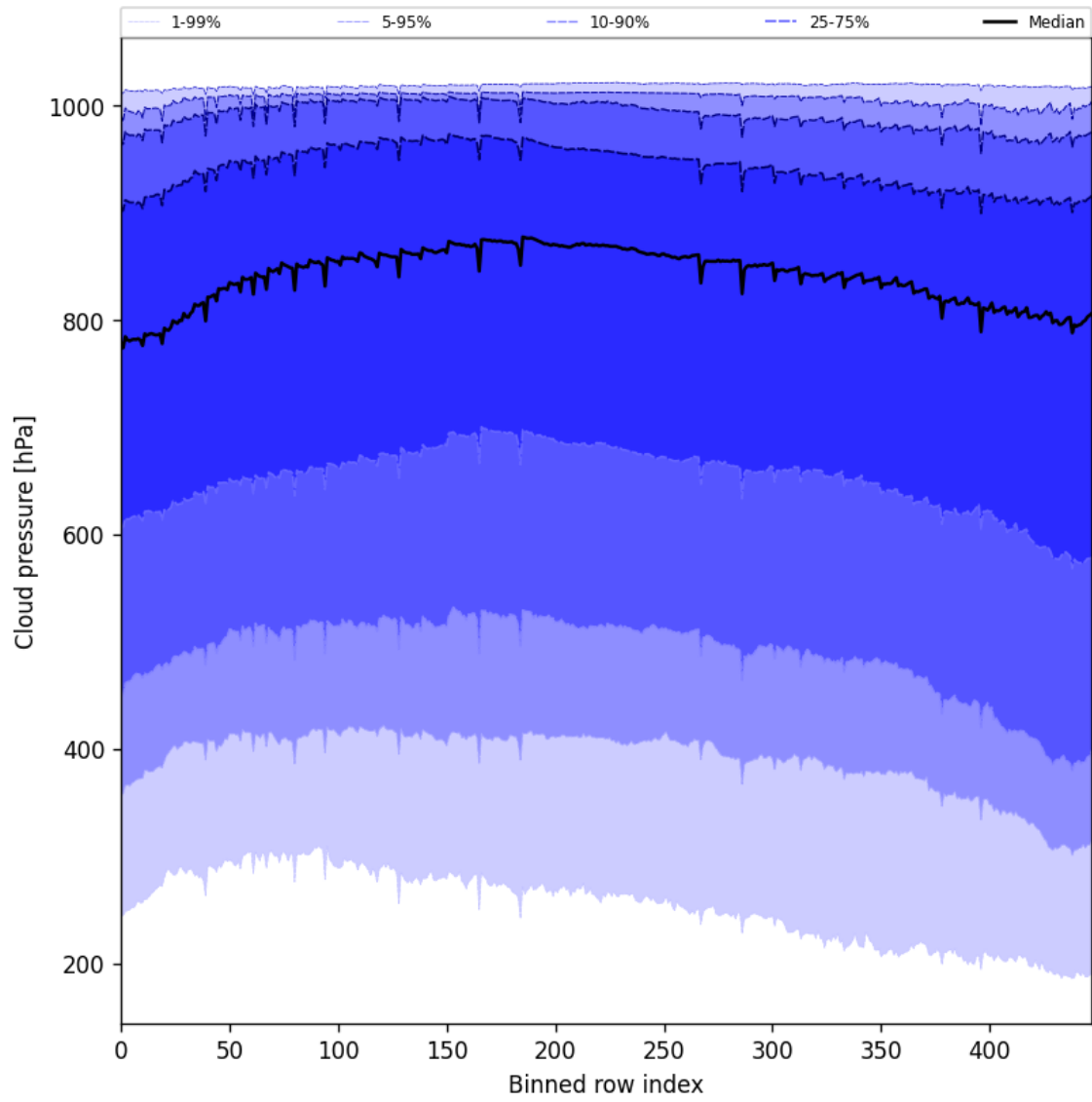
Figure 47: Along track statistics of “Cloud pressure” for 2025-11-09 to 2025-11-11
