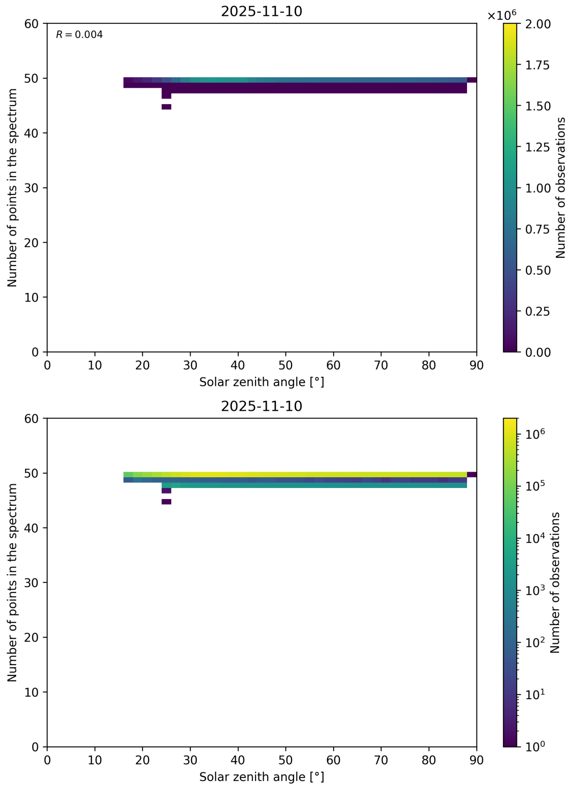
Figure 115: Scatter density plot of “Solar zenith angle” against “Number of points in the spectrum” for 2025-11-09 to 2025-11-11.
