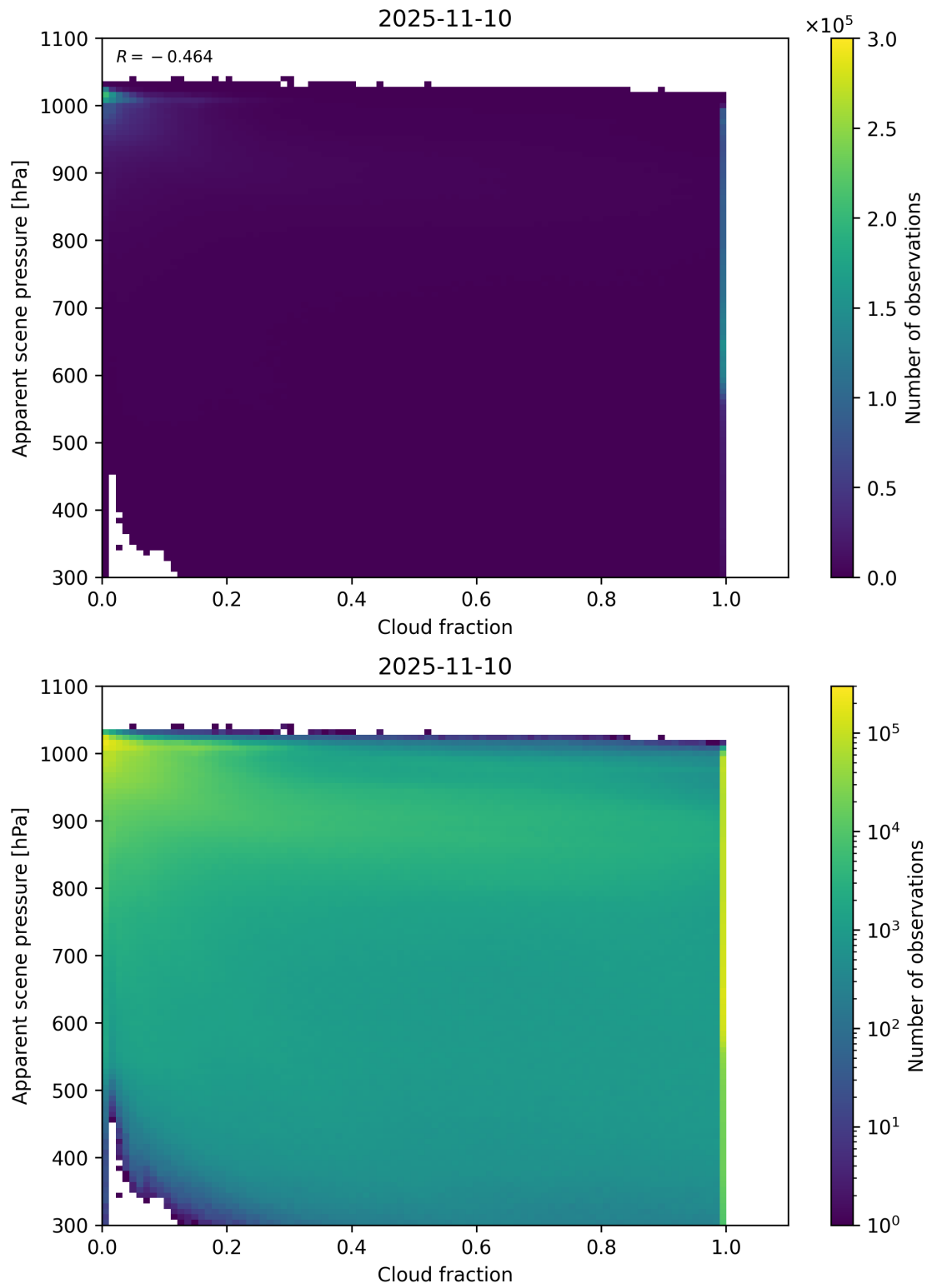
Figure 70: Scatter density plot of “Cloud fraction” against “Apparent scene pressure” for 2025-11-09 to 2025-11-11.
