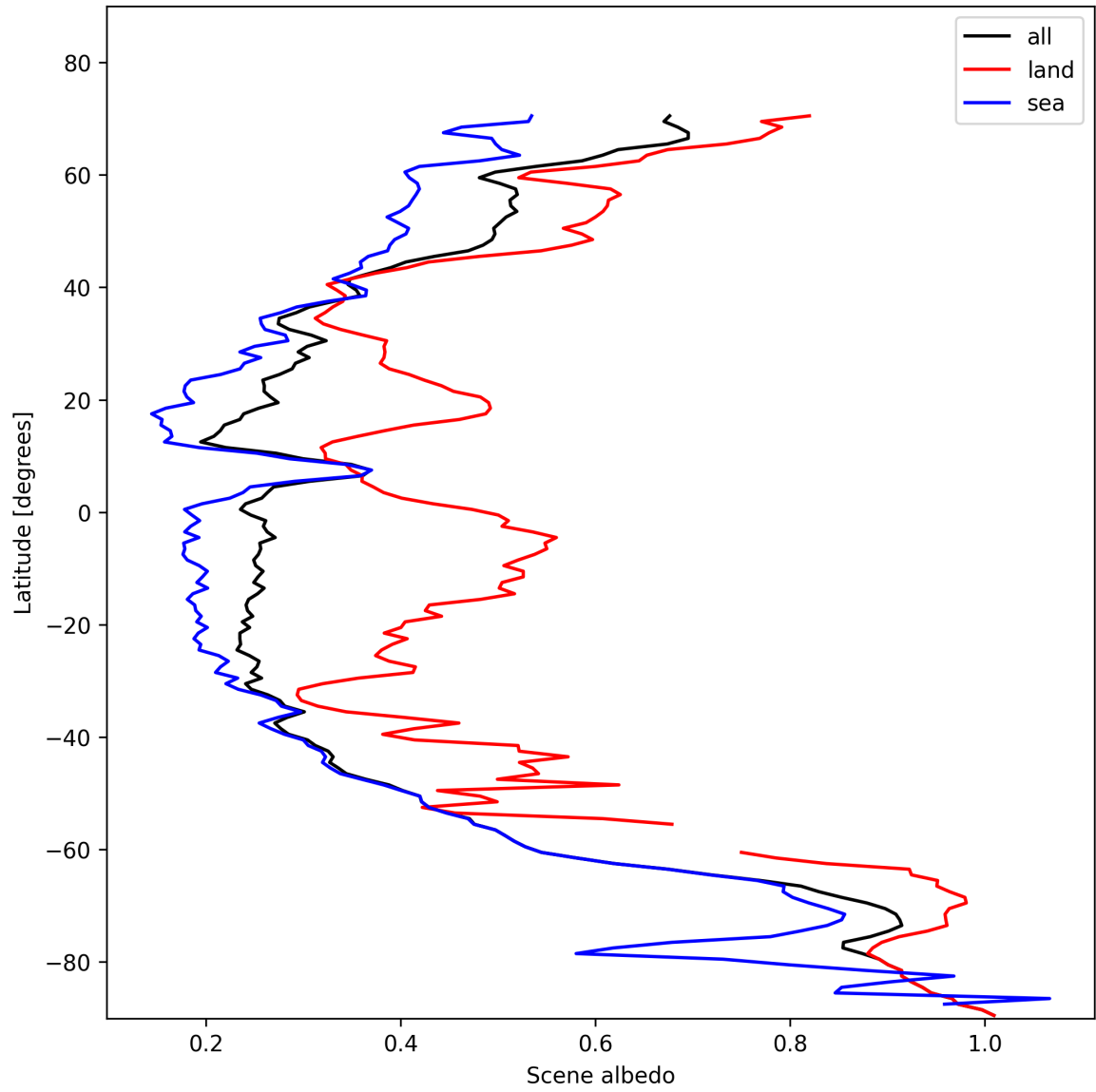
Figure 17: Zonal average of “Scene albedo” for 2025-11-09 to 2025-11-11.
