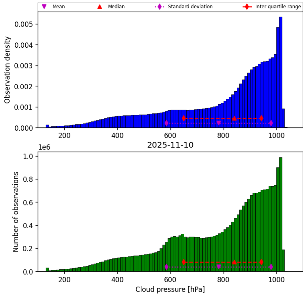
Figure 30: Histogram of “Cloud pressure” for 2025-11-09 to 2025-11-11
