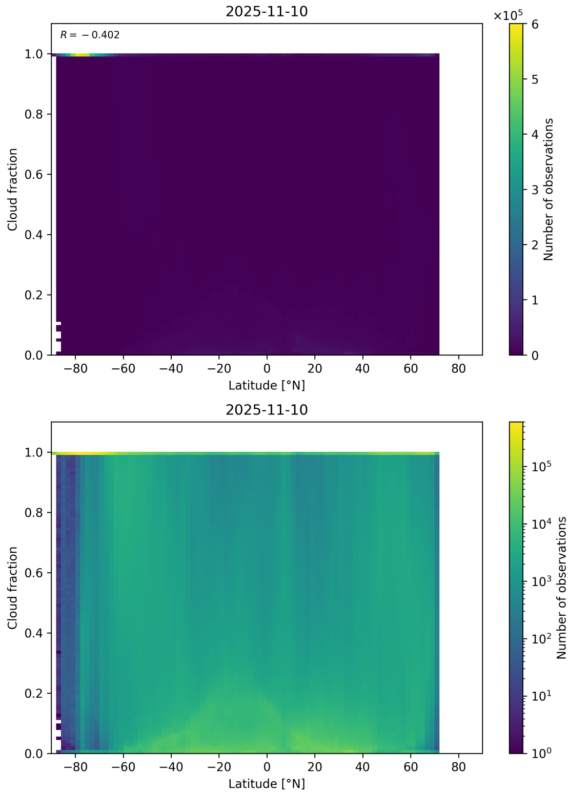
Figure 90: Scatter density plot of “Latitude” against “Cloud fraction” for 2025-11-09 to 2025-11-11.
