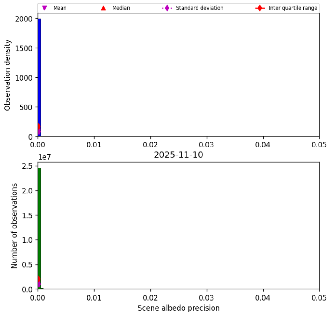
Figure 35: Histogram of “Scene albedo precision” for 2025-11-09 to 2025-11-11
