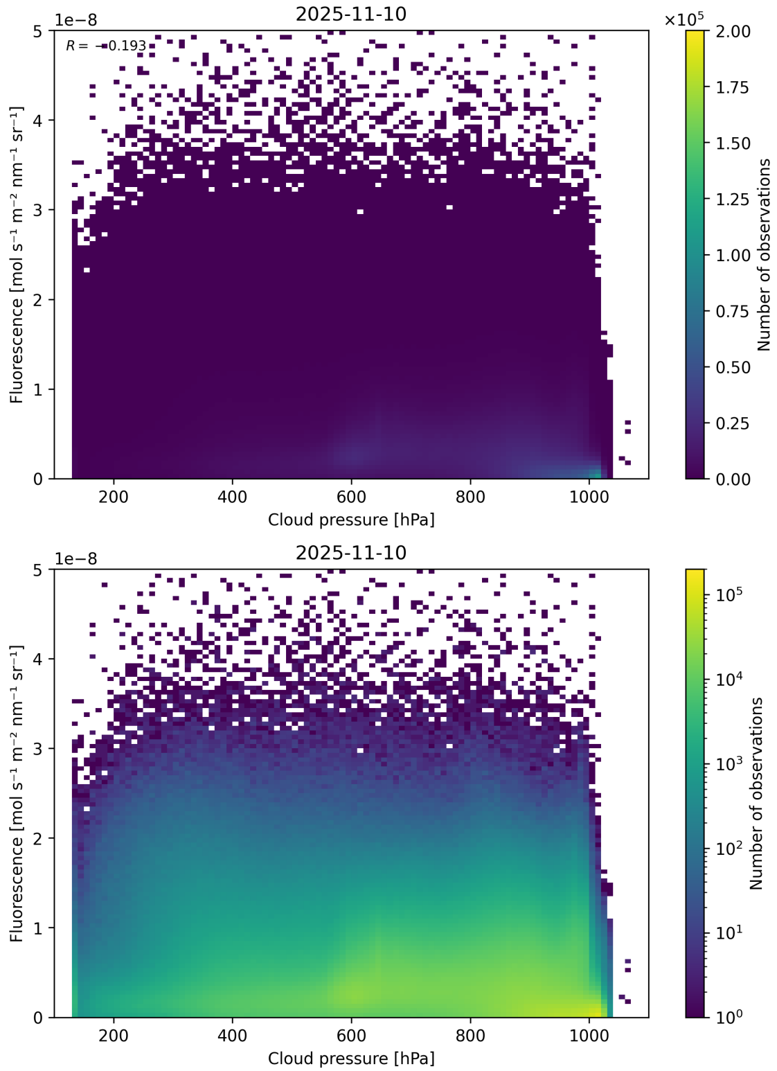
Figure 80: Scatter density plot of “Cloud pressure” against “Fluorescence” for 2025-11-09 to 2025-11-11.
