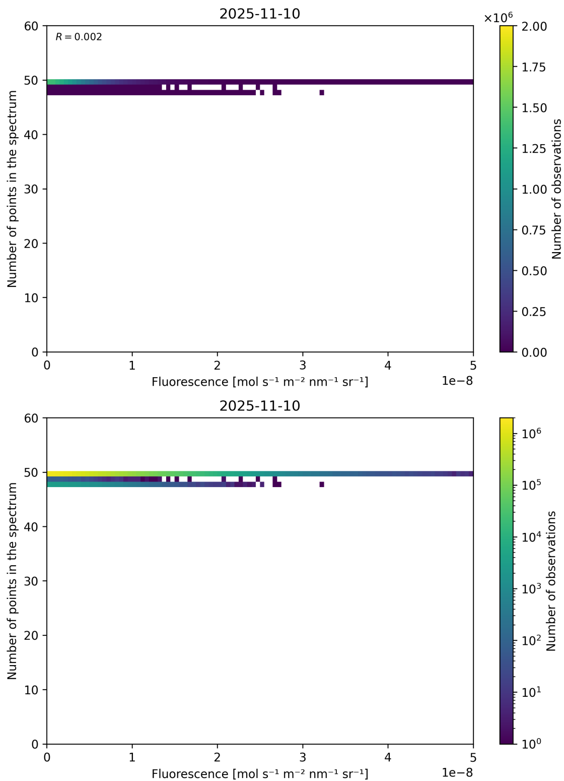
Figure 86: Scatter density plot of “Fluorescence” against “Number of points in the spectrum” for 2025-11-09 to 2025-11-11.
