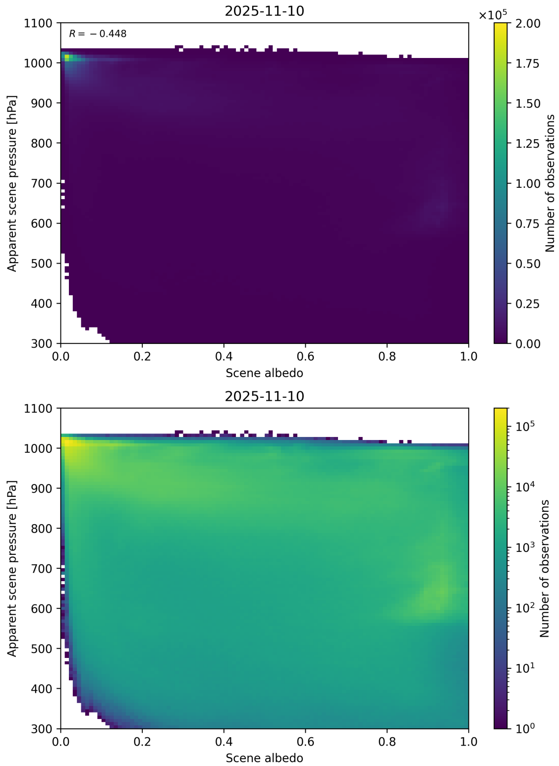
Figure 102: Scatter density plot of “Scene albedo” against “Apparent scene pressure” for 2025-11-09 to 2025-11-11.
