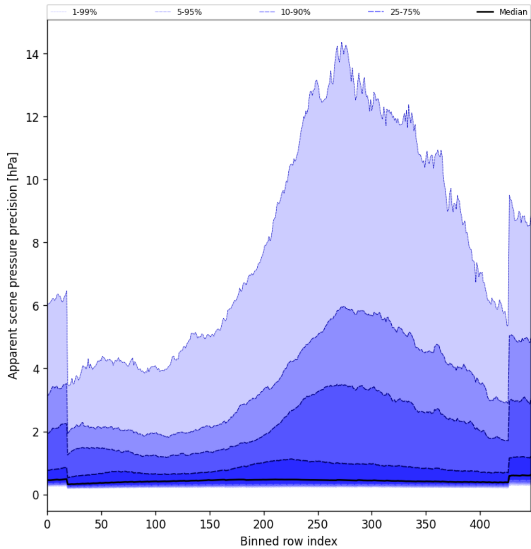
Figure 54: Along track statistics of “Apparent scene pressure precision” for 2025-11-09 to 2025-11-11
