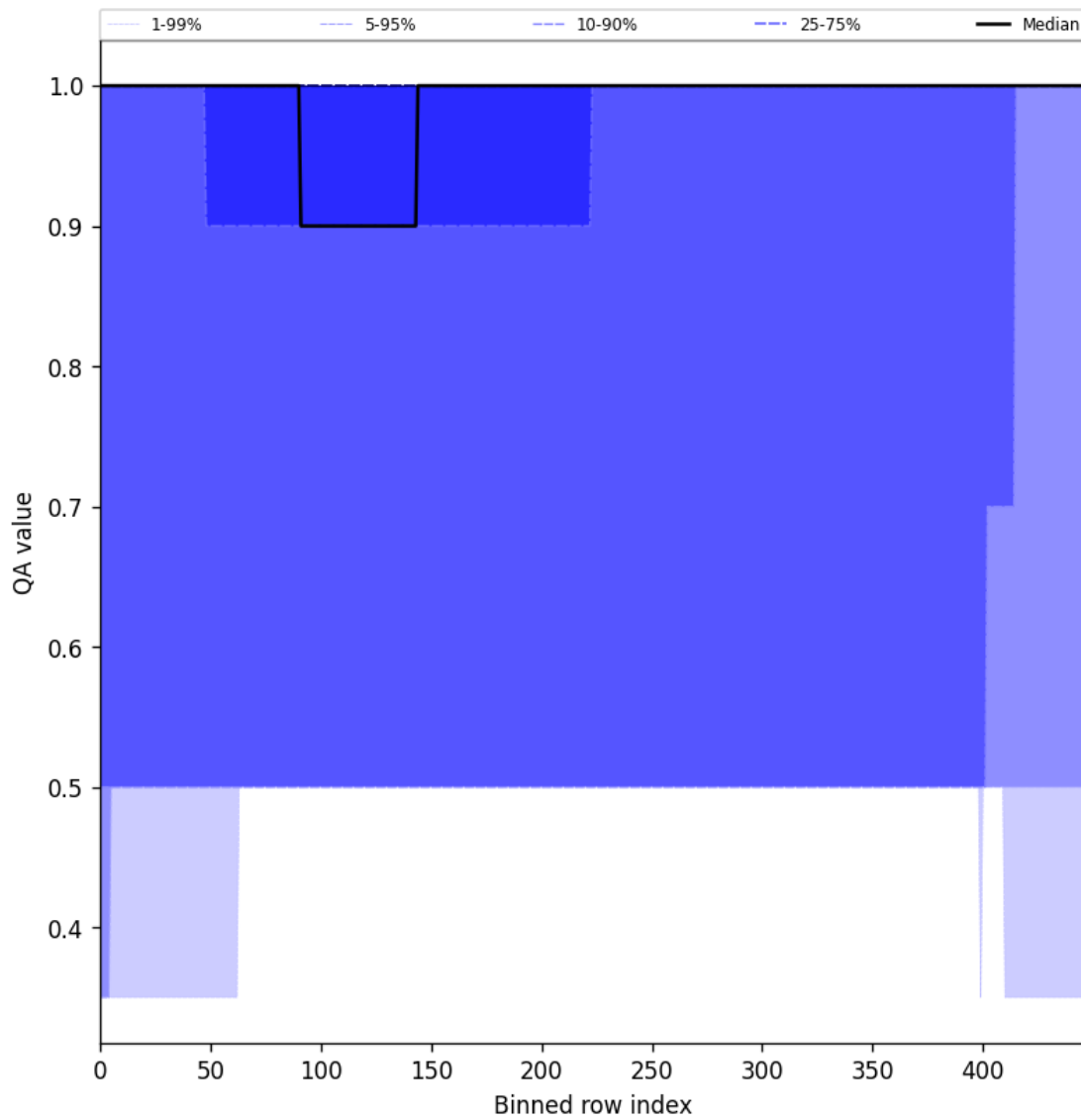
Figure 46: Along track statistics of “QA value” for 2025-11-09 to 2025-11-11
