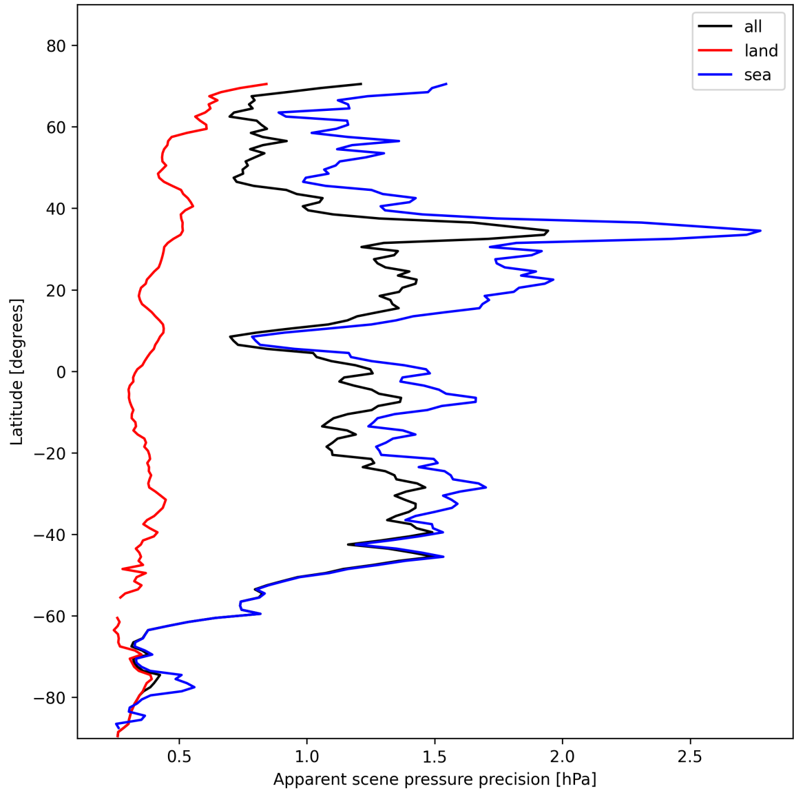
Figure 20: Zonal average of “Apparent scene pressure precision” for 2025-11-09 to 2025-11-11.
