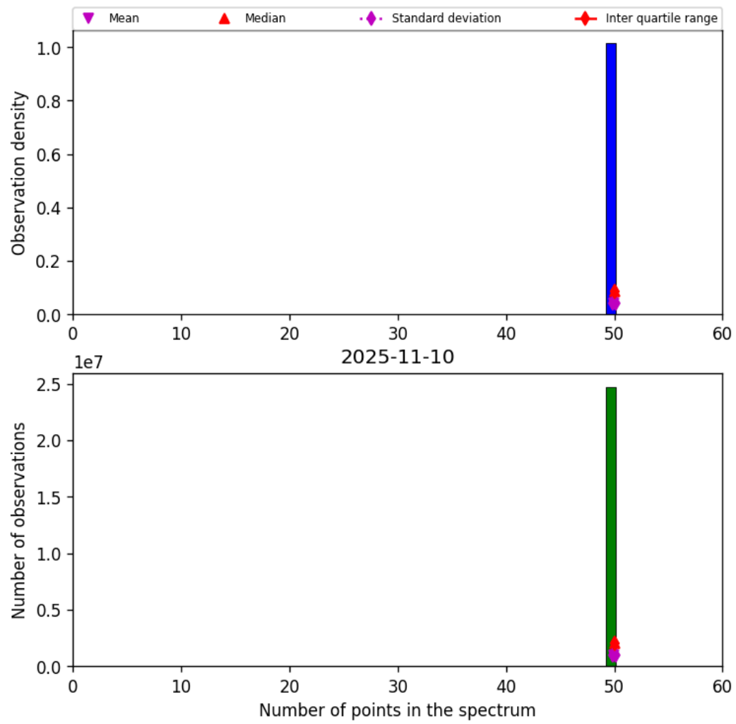
Figure 44: Histogram of "Number of points in the spectrum" for 2025-11-09 to 2025-11-11
