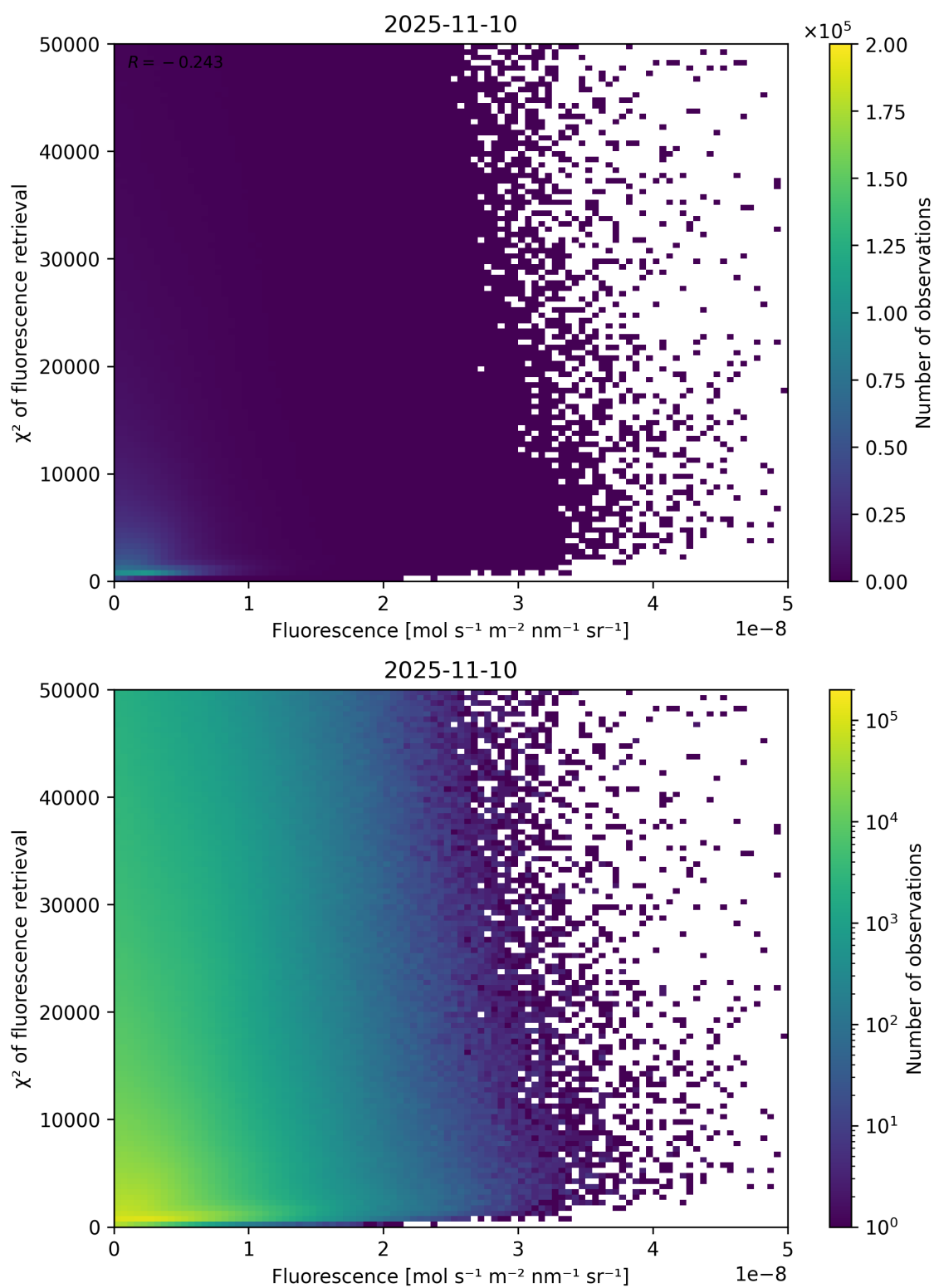
Figure 85: Scatter density plot of “Fluorescence” against “ \chi^2 of fluorescence retrieval” for 2025-11-09 to 2025-11-11.
