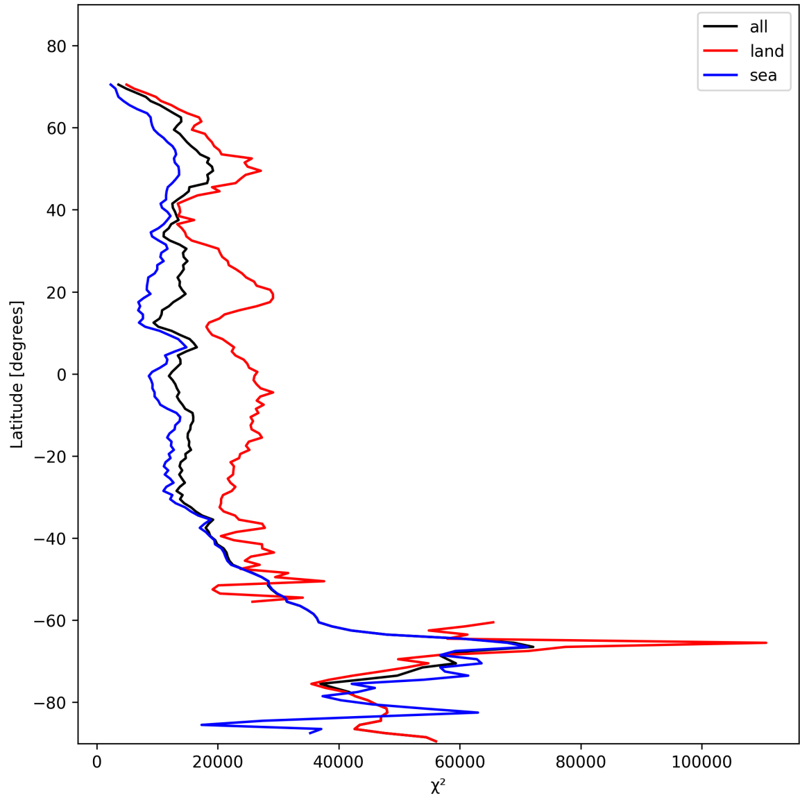
Figure 21: Zonal average of “ \chi^2 ” for 2025-11-09 to 2025-11-11.
