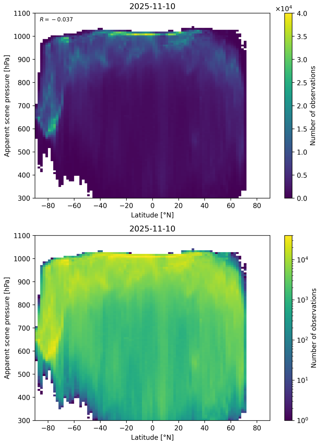
Figure 88: Scatter density plot of “Latitude” against “Apparent scene pressure” for 2025-11-09 to 2025-11-11.
