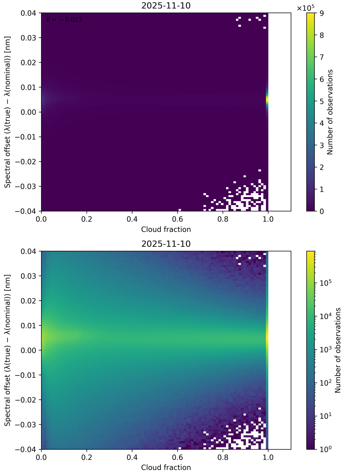
Figure 76: Scatter density plot of “Cloud fraction” against “Spectral offset ( \lambda_{\text{true}} - \lambda_{\text{nominal}} )” for 2025-11-09 to 2025-11-11.
