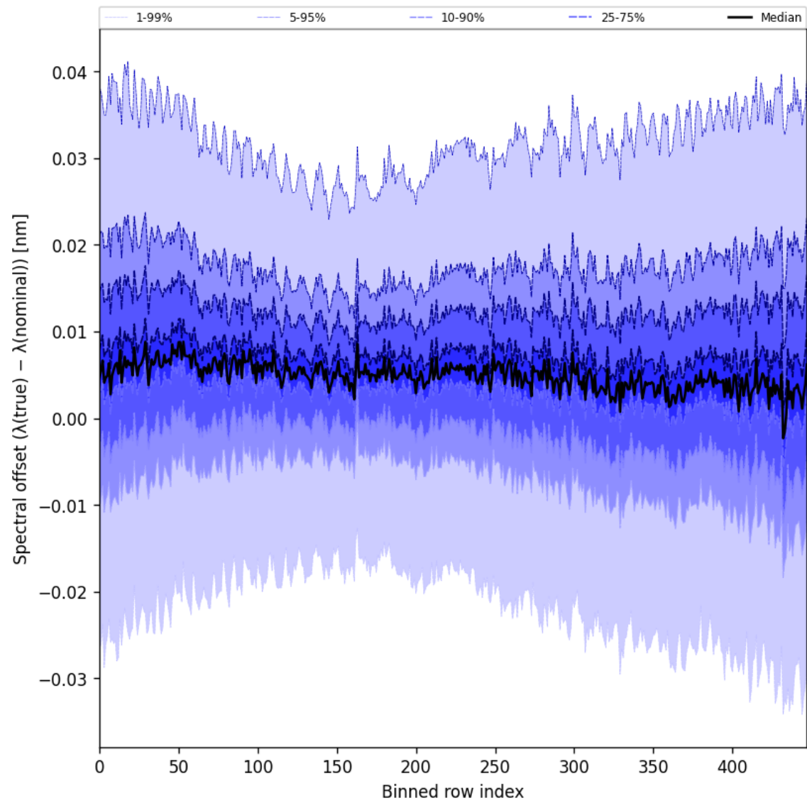
Figure 62: Along track statistics of “Spectral offset ( \lambda_{\text{true}} - \lambda_{\text{nominal}} )” for 2025-11-09 to 2025-11-11
