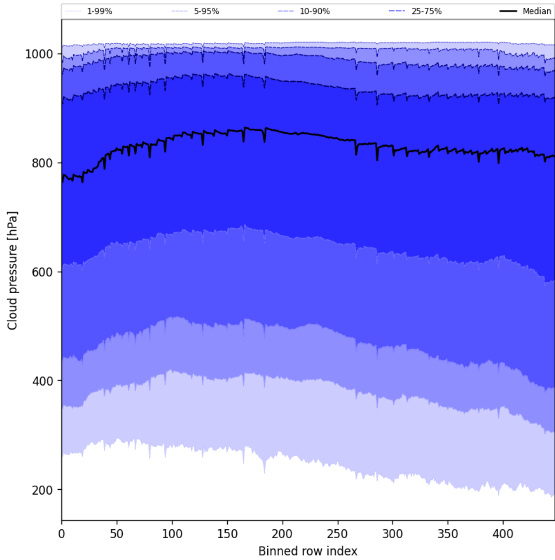
Figure 47: Along track statistics of “Cloud pressure” for 2025-11-12 to 2025-11-13
