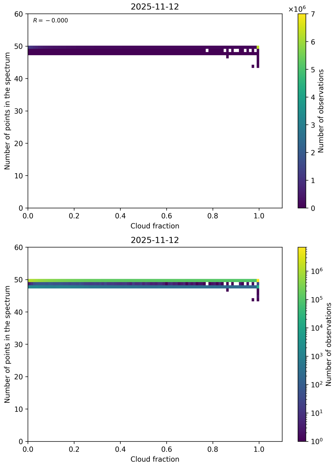
Figure 74: Scatter density plot of “Cloud fraction” against “Number of points in the spectrum” for 2025-11-12 to 2025-11-13.
