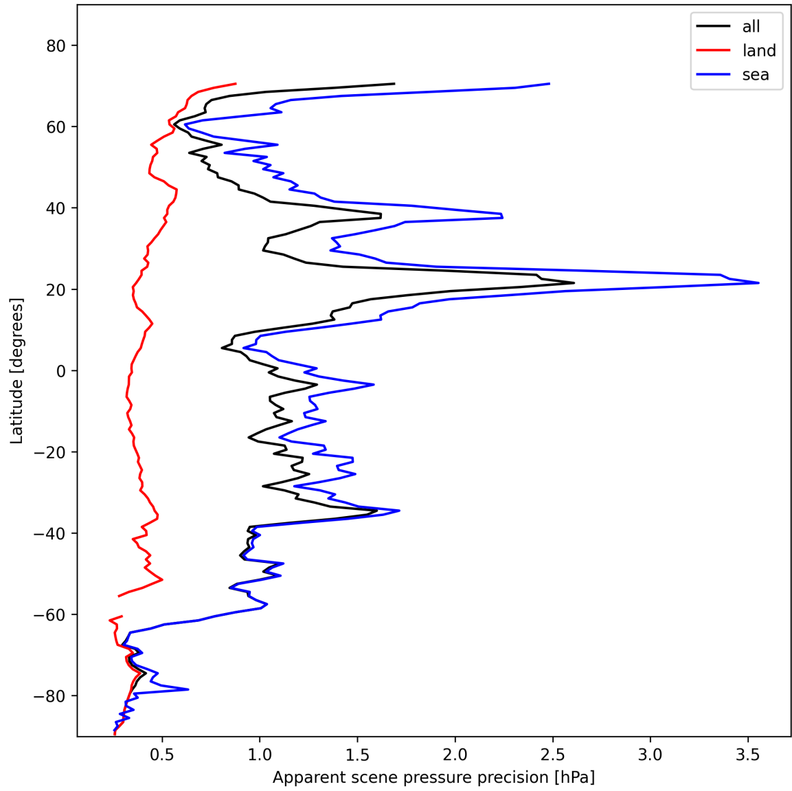
Figure 20: Zonal average of “Apparent scene pressure precision” for 2025-11-12 to 2025-11-13.
