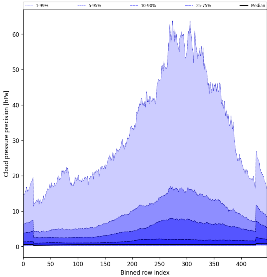
Figure 48: Along track statistics of “Cloud pressure precision” for 2025-11-12 to 2025-11-13
