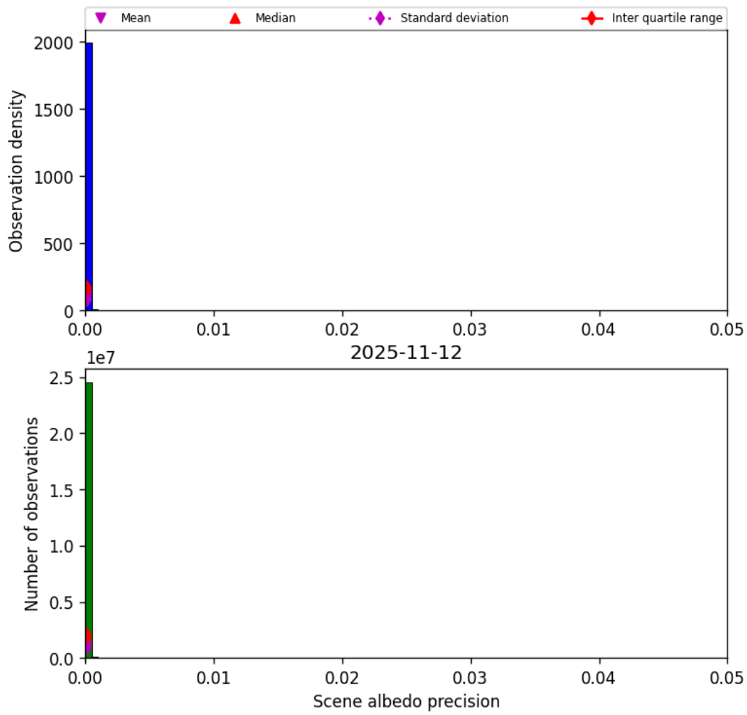
Figure 35: Histogram of “Scene albedo precision” for 2025-11-12 to 2025-11-13
