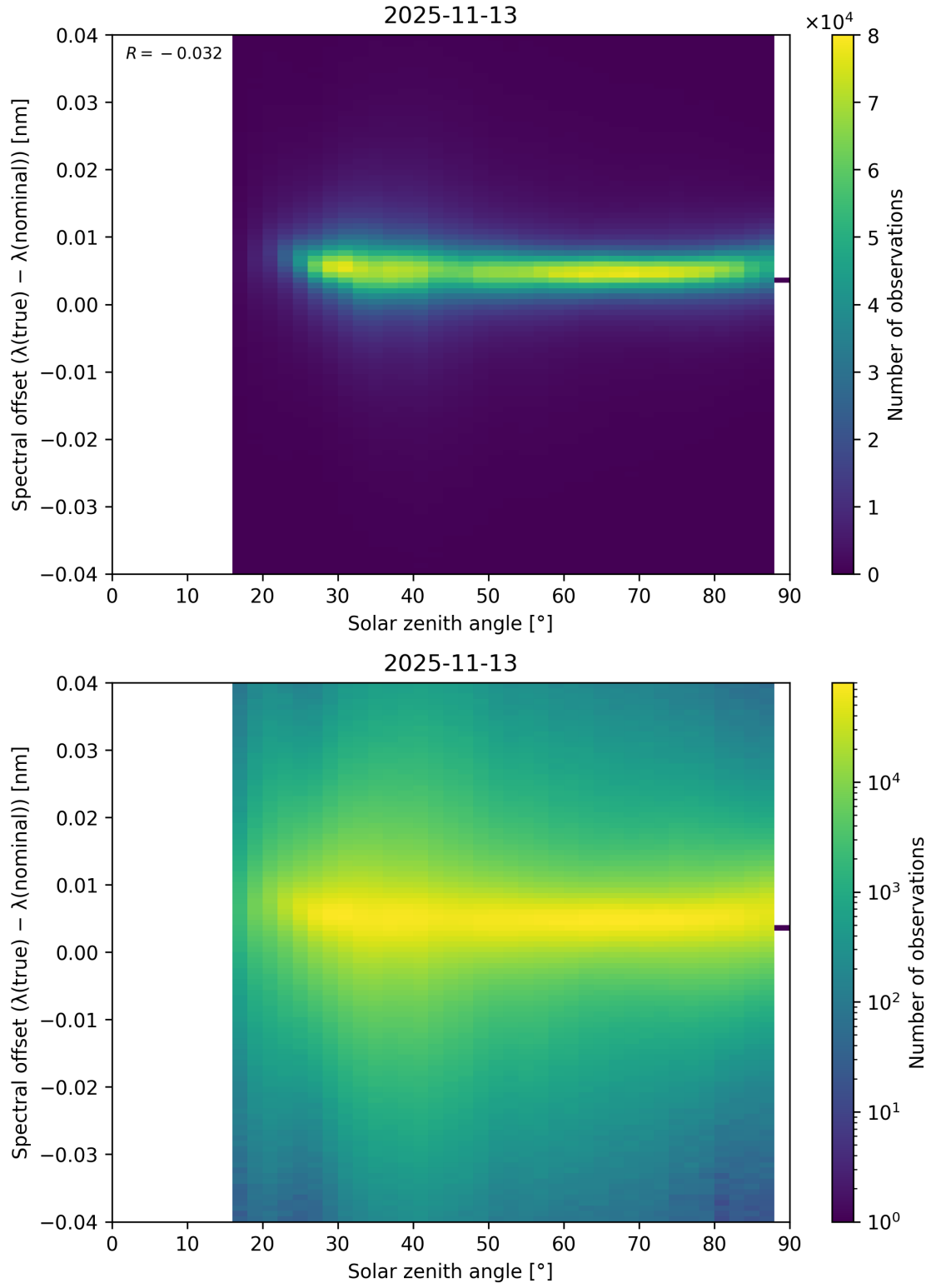
Figure 117: Scatter density plot of “Solar zenith angle” against “Spectral offset ( \lambda_{\text{true}} - \lambda_{\text{nominal}} )” for 2025-11-12 to 2025-11-14.
