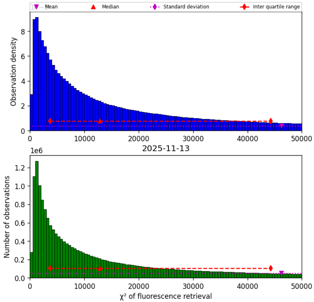
Figure 42: Histogram of “ \chi^2 of fluorescence retrieval” for 2025-11-12 to 2025-11-14
