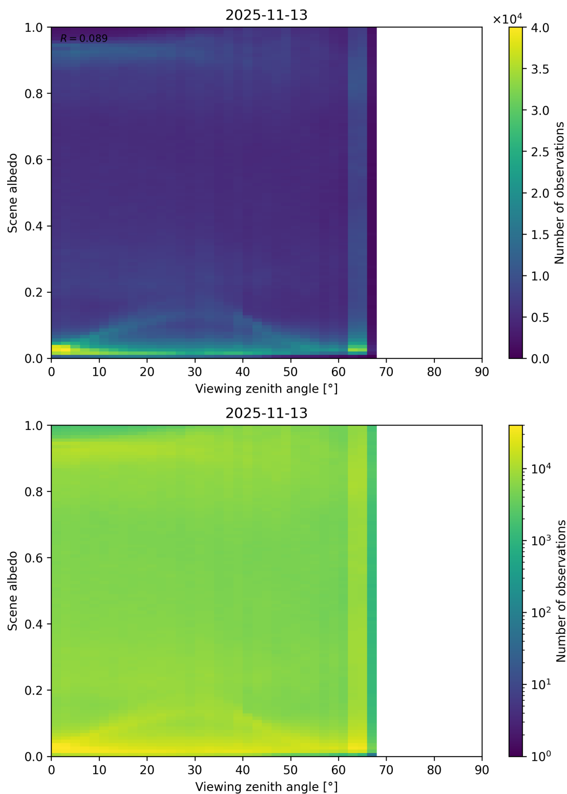
Figure 126: Scatter density plot of “Viewing zenith angle” against “Scene albedo” for 2025-11-12 to 2025-11-14.
