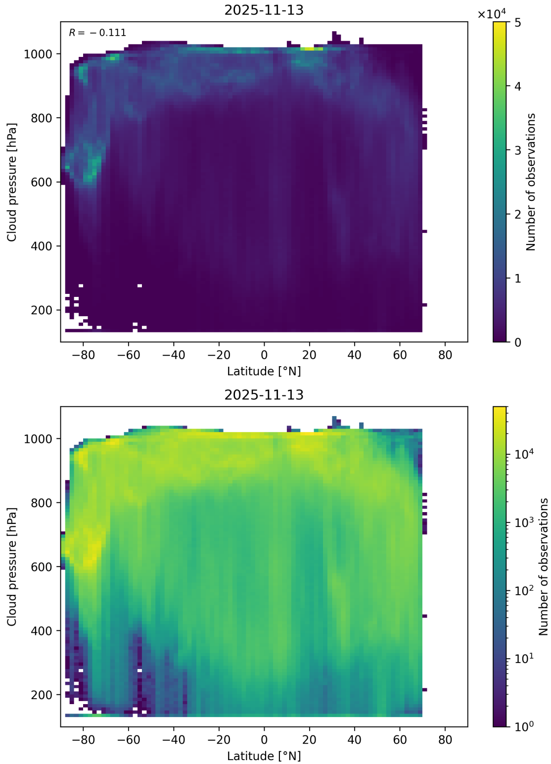
Figure 91: Scatter density plot of “Latitude” against “Cloud pressure” for 2025-11-12 to 2025-11-14.
