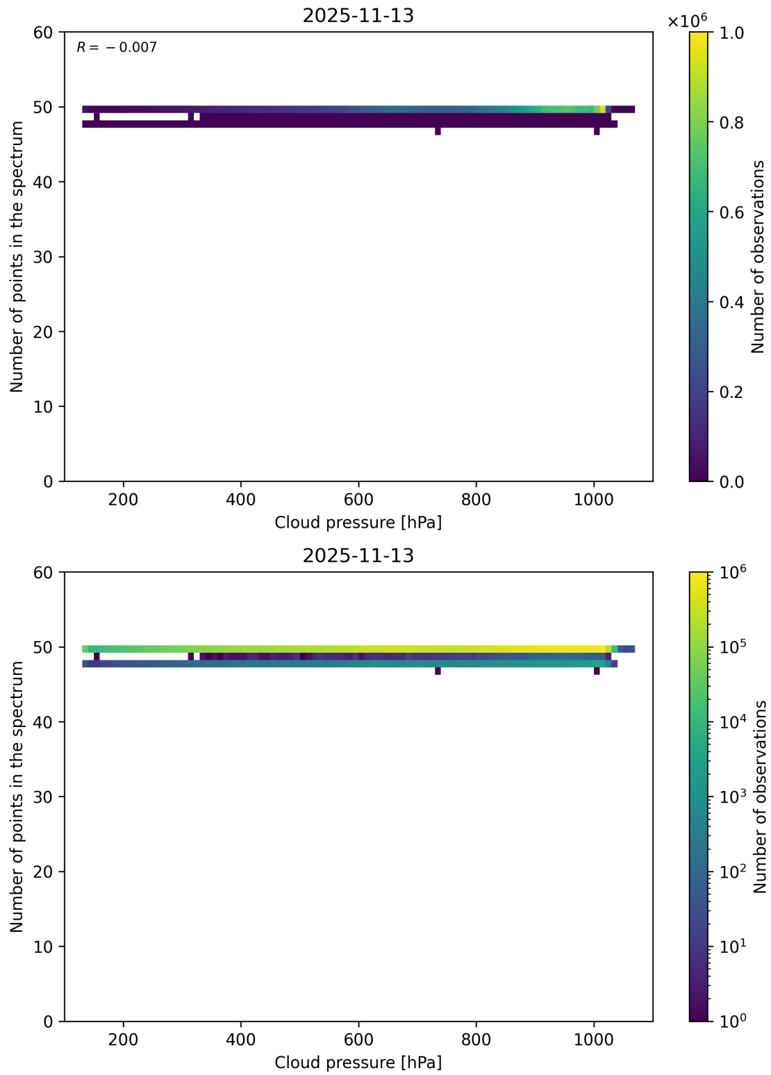
Figure 82: Scatter density plot of “Cloud pressure” against “Number of points in the spectrum” for 2025-11-12 to 2025-11-14.
