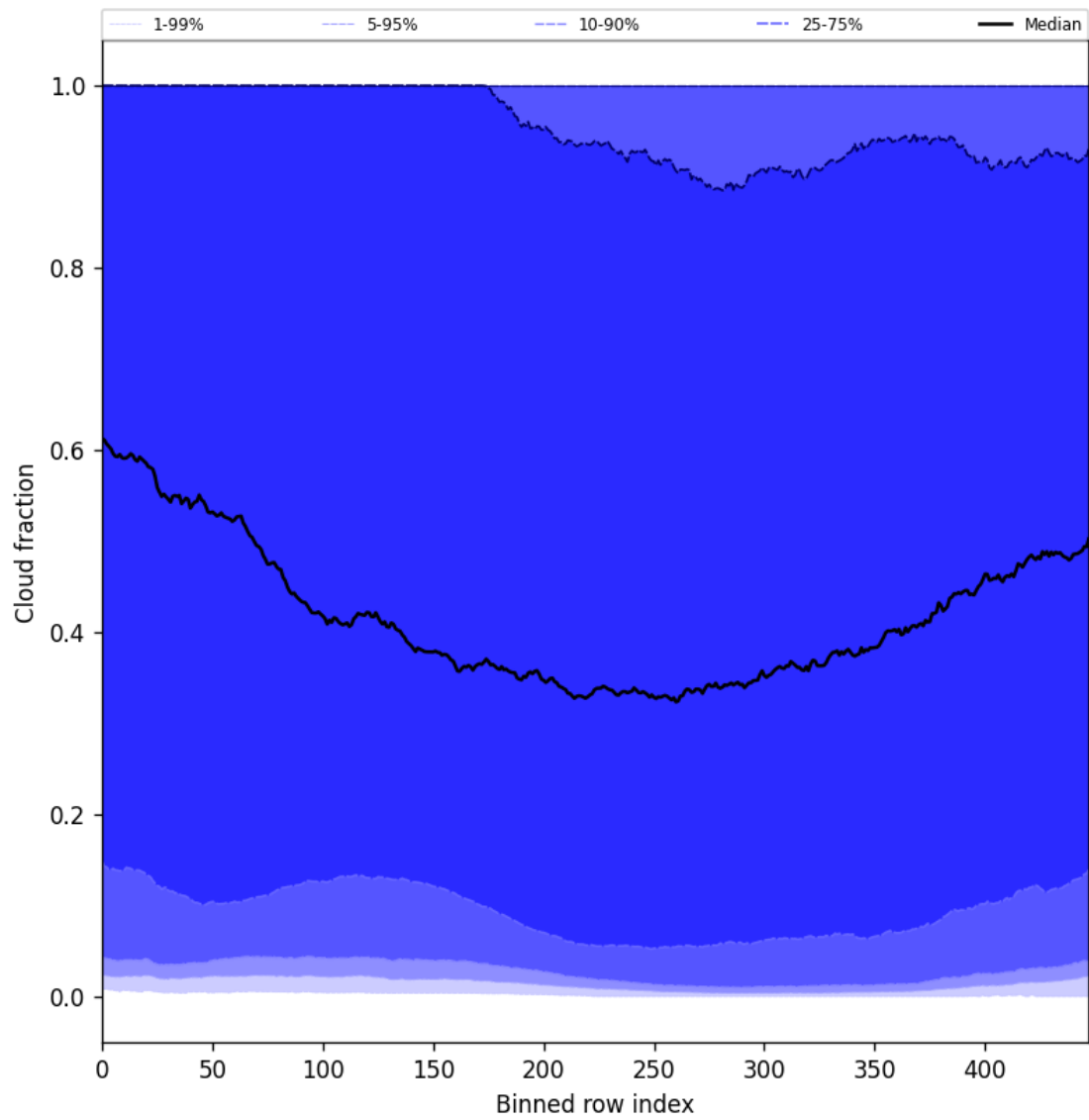
Figure 49: Along track statistics of “Cloud fraction” for 2025-11-12 to 2025-11-14
