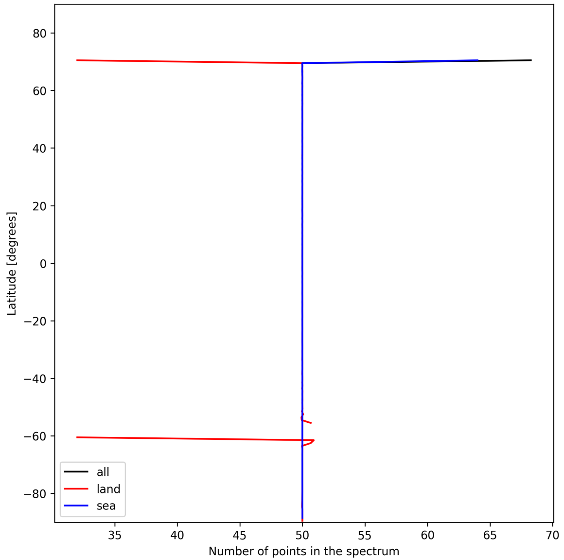
Figure 27: Zonal average of “Number of points in the spectrum” for 2025-11-12 to 2025-11-14.
