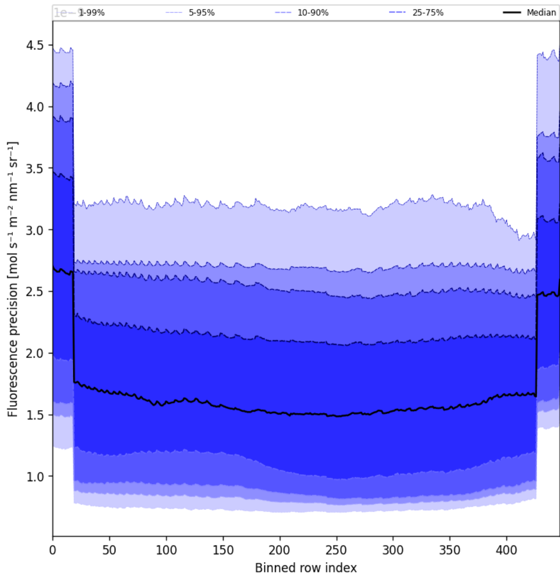
Figure 58: Along track statistics of “Fluorescence precision” for 2025-11-12 to 2025-11-14
