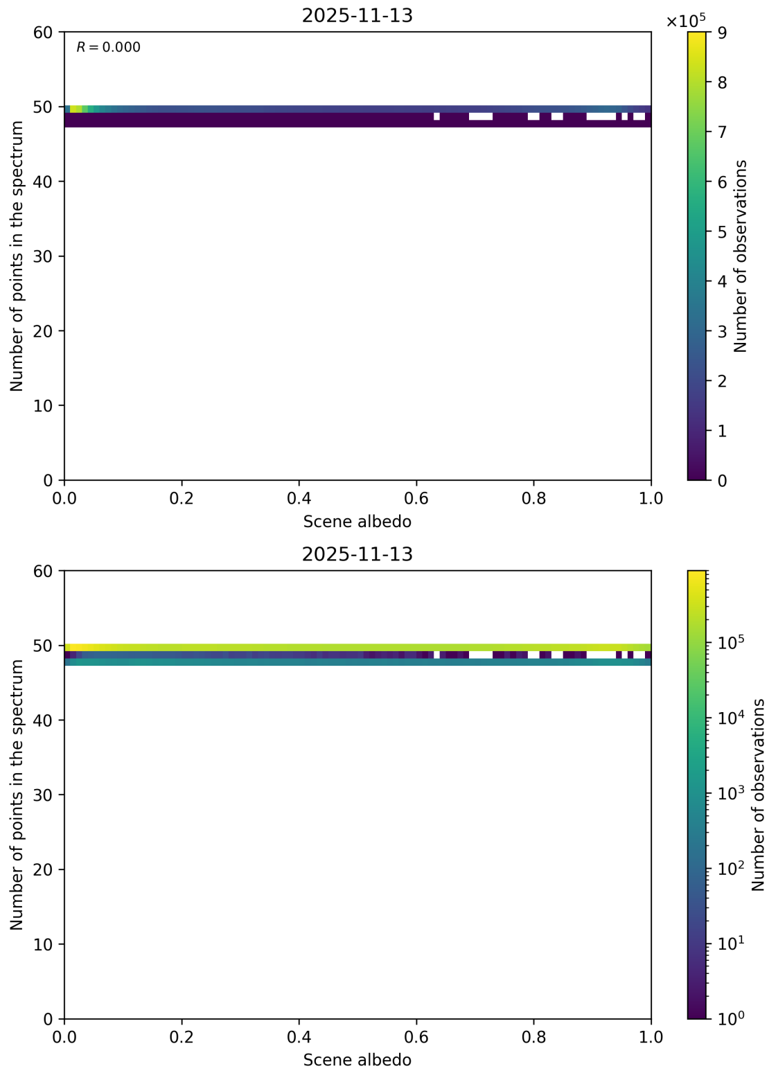
Figure 106: Scatter density plot of “Scene albedo” against “Number of points in the spectrum” for 2025-11-12 to 2025-11-14.
