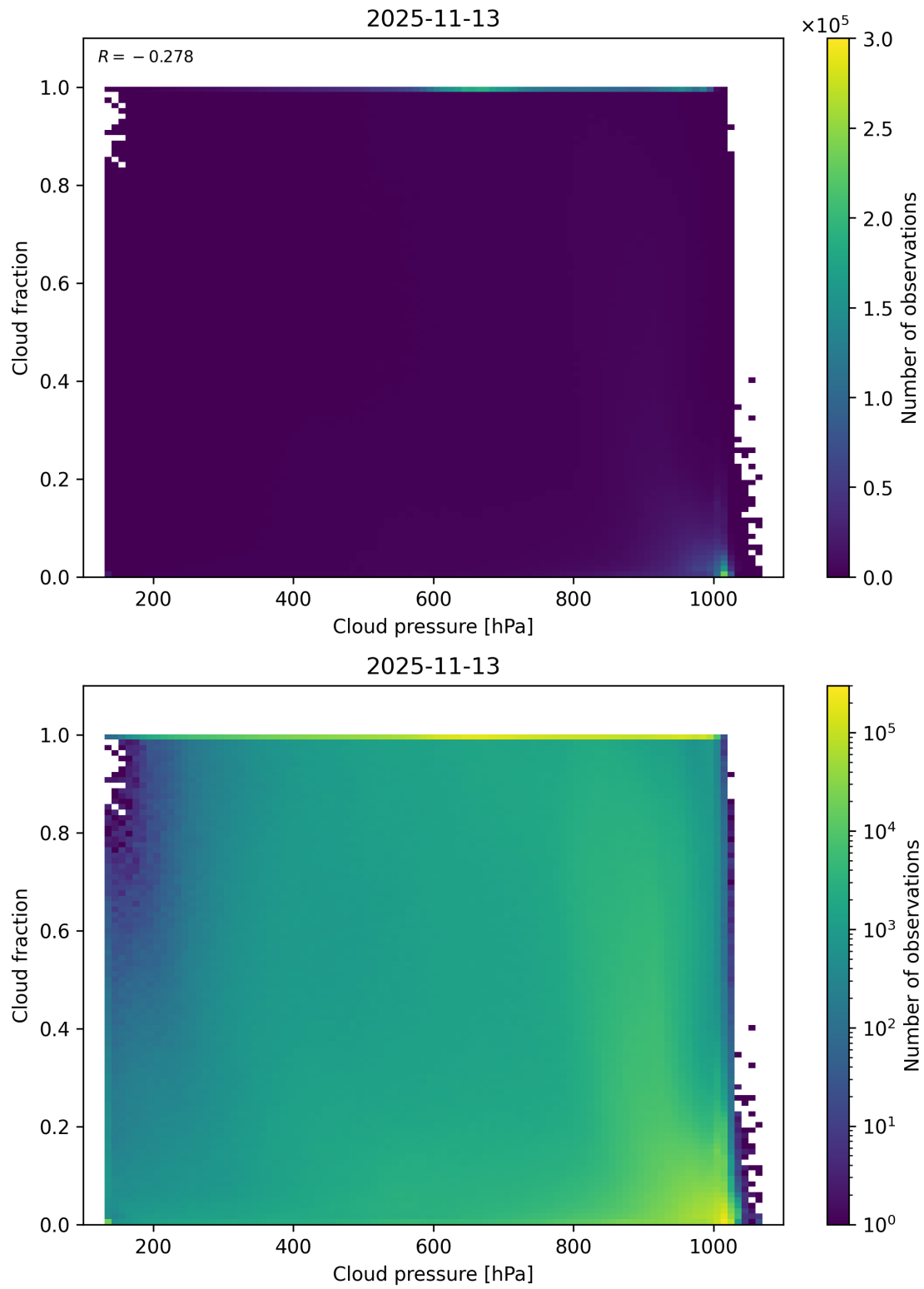
Figure 79: Scatter density plot of “Cloud pressure” against “Cloud fraction” for 2025-11-12 to 2025-11-14.
