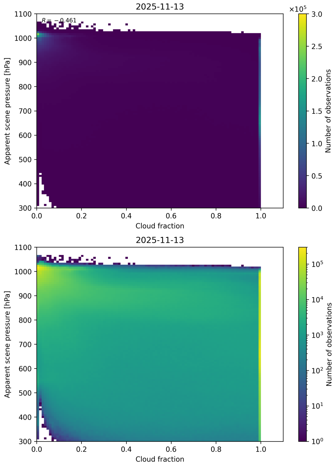
Figure 70: Scatter density plot of “Cloud fraction” against “Apparent scene pressure” for 2025-11-12 to 2025-11-14.
