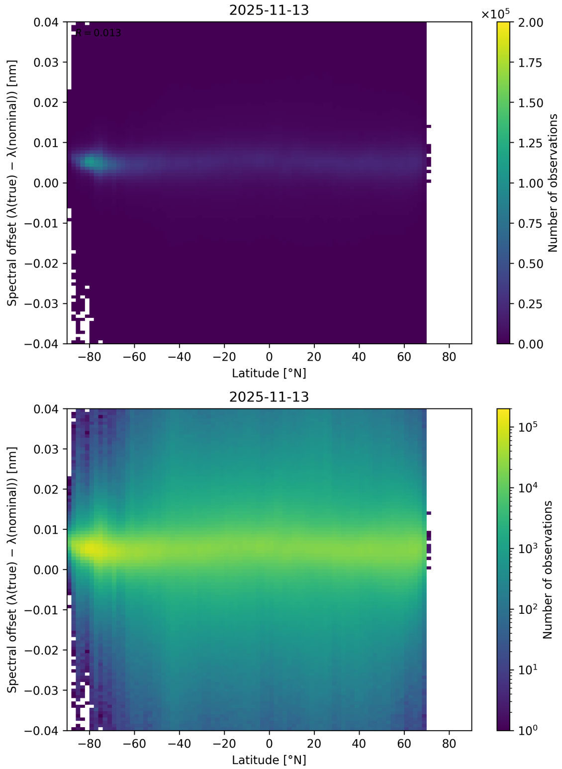
Figure 96: Scatter density plot of “Latitude” against “Spectral offset ( \lambda_{\text{true}} - \lambda_{\text{nominal}} )” for 2025-11-12 to 2025-11-14.
