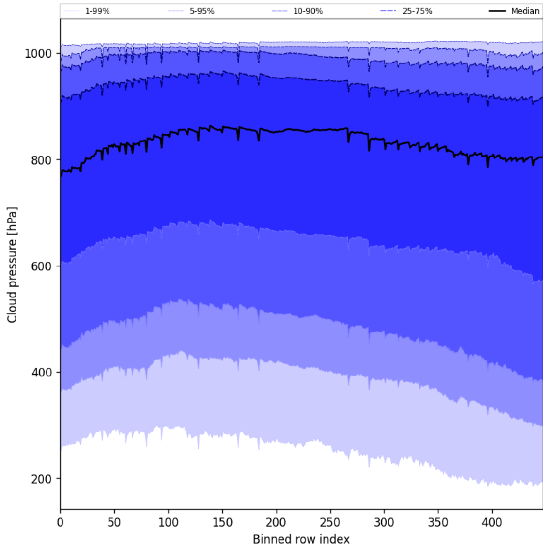
Figure 47: Along track statistics of “Cloud pressure” for 2025-11-12 to 2025-11-14
