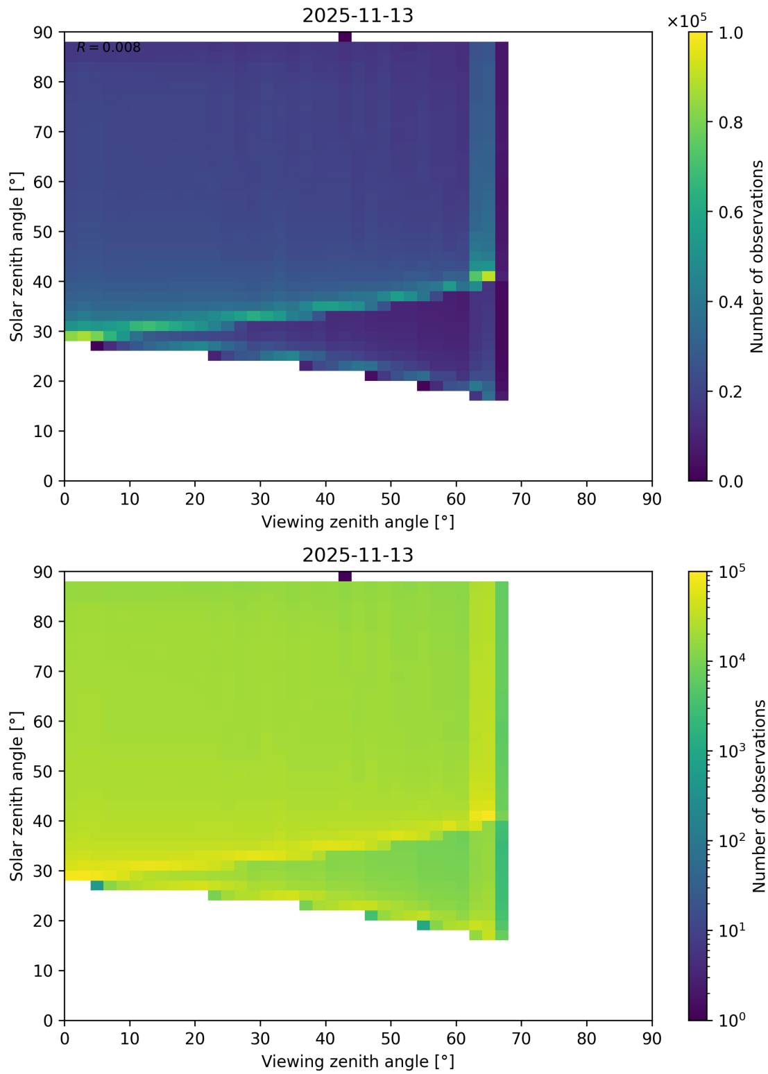
Figure 127: Scatter density plot of “Viewing zenith angle” against “Solar zenith angle” for 2025-11-12 to 2025-11-14.
