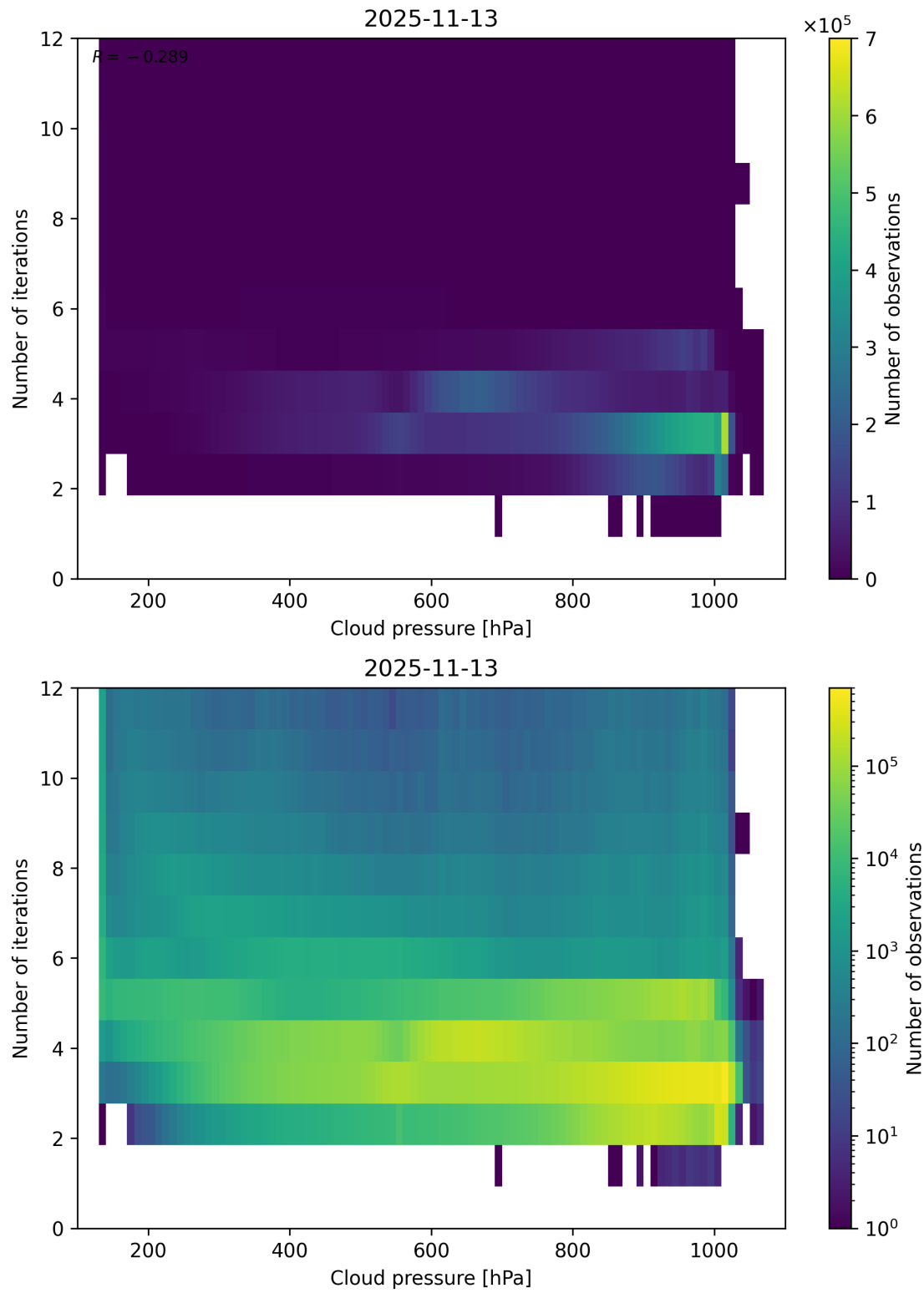
Figure 81: Scatter density plot of “Cloud pressure” against “Number of iterations” for 2025-11-12 to 2025-11-14.
