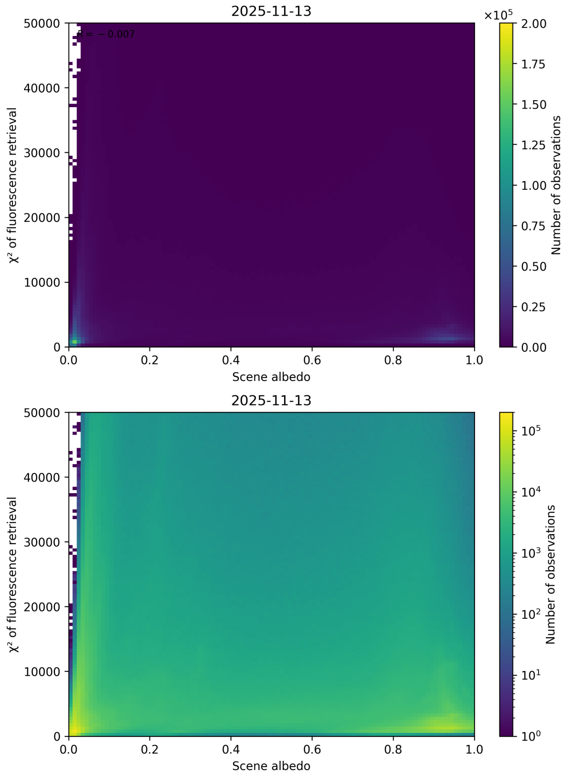
Figure 103: Scatter density plot of “Scene albedo” against “ \chi^2 of fluorescence retrieval” for 2025-11-12 to 2025-11-14.
