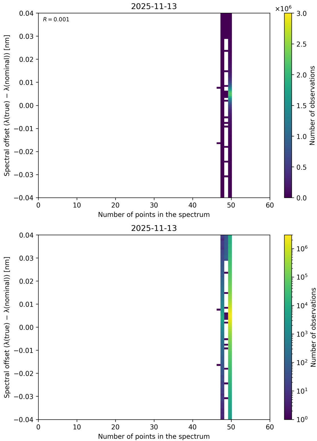
Figure 101: Scatter density plot of “Number of points in the spectrum” against “Spectral offset ( \lambda_{\text{true}} - \lambda_{\text{nominal}} )” for 2025-11-12 to 2025-11-14.
