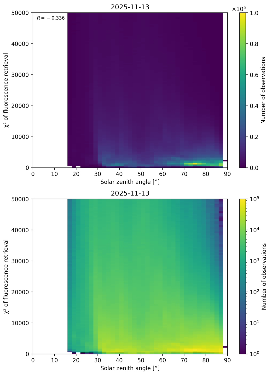
Figure 109: Scatter density plot of “Solar zenith angle” against “ \chi^2 of fluorescence retrieval” for 2025-11-12 to 2025-11-14.
