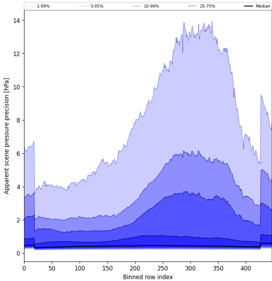
Figure 54: Along track statistics of “Apparent scene pressure precision” for 2025-11-12 to 2025-11-14
