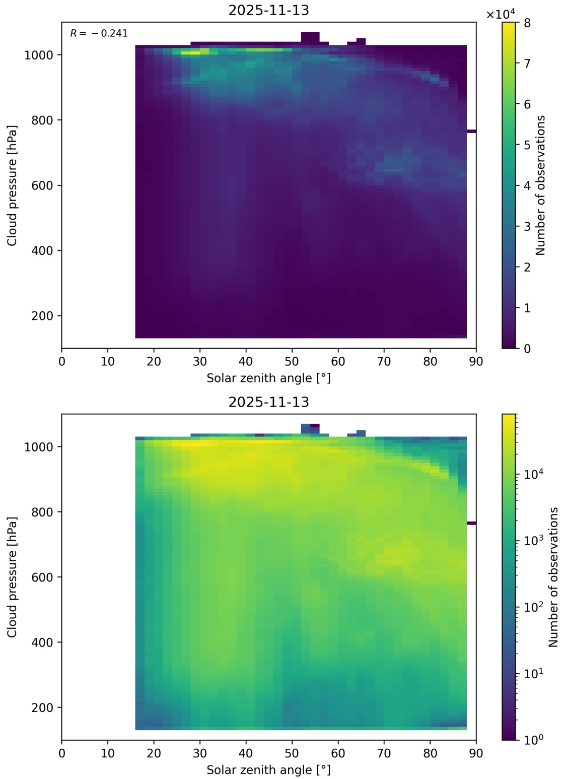
Figure 111: Scatter density plot of “Solar zenith angle” against “Cloud pressure” for 2025-11-12 to 2025-11-14.
