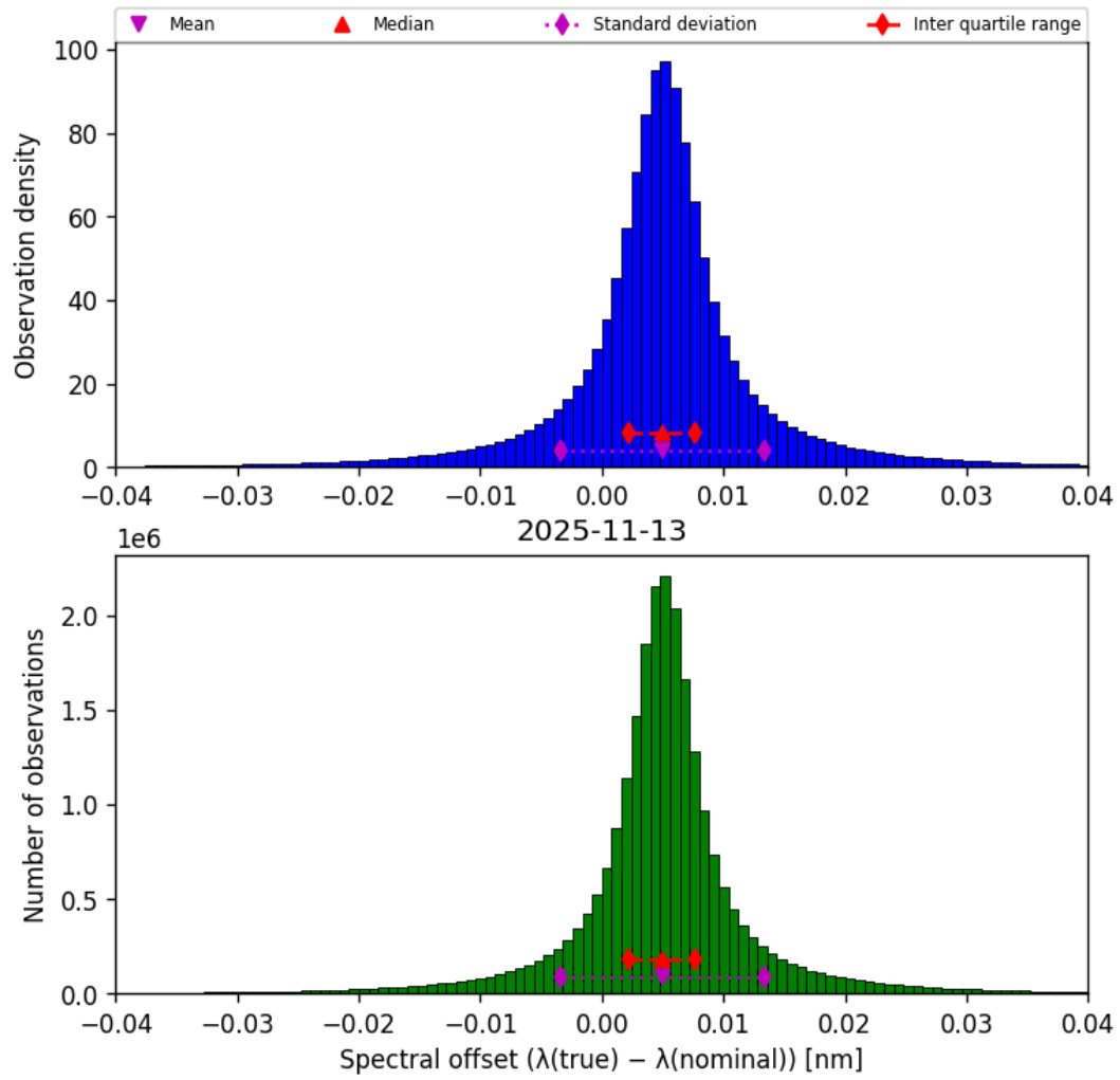
Figure 45: Histogram of “Spectral offset ( \lambda_{\text{true}} - \lambda_{\text{nominal}} )” for 2025-11-12 to 2025-11-14
