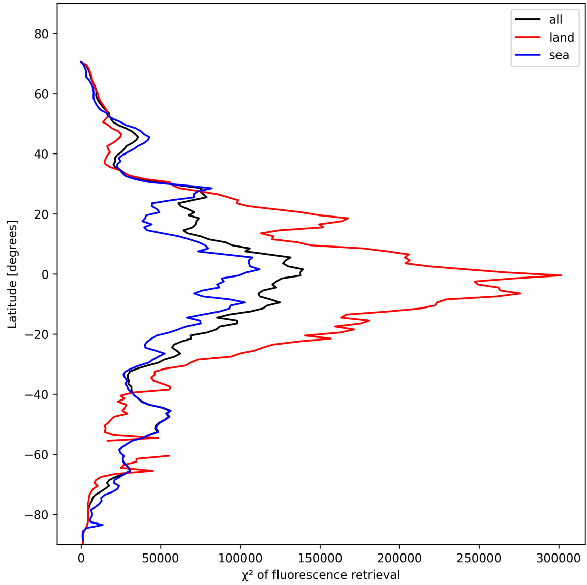
Figure 25: Zonal average of “ \chi^2 of fluorescence retrieval” for 2025-11-12 to 2025-11-14.
