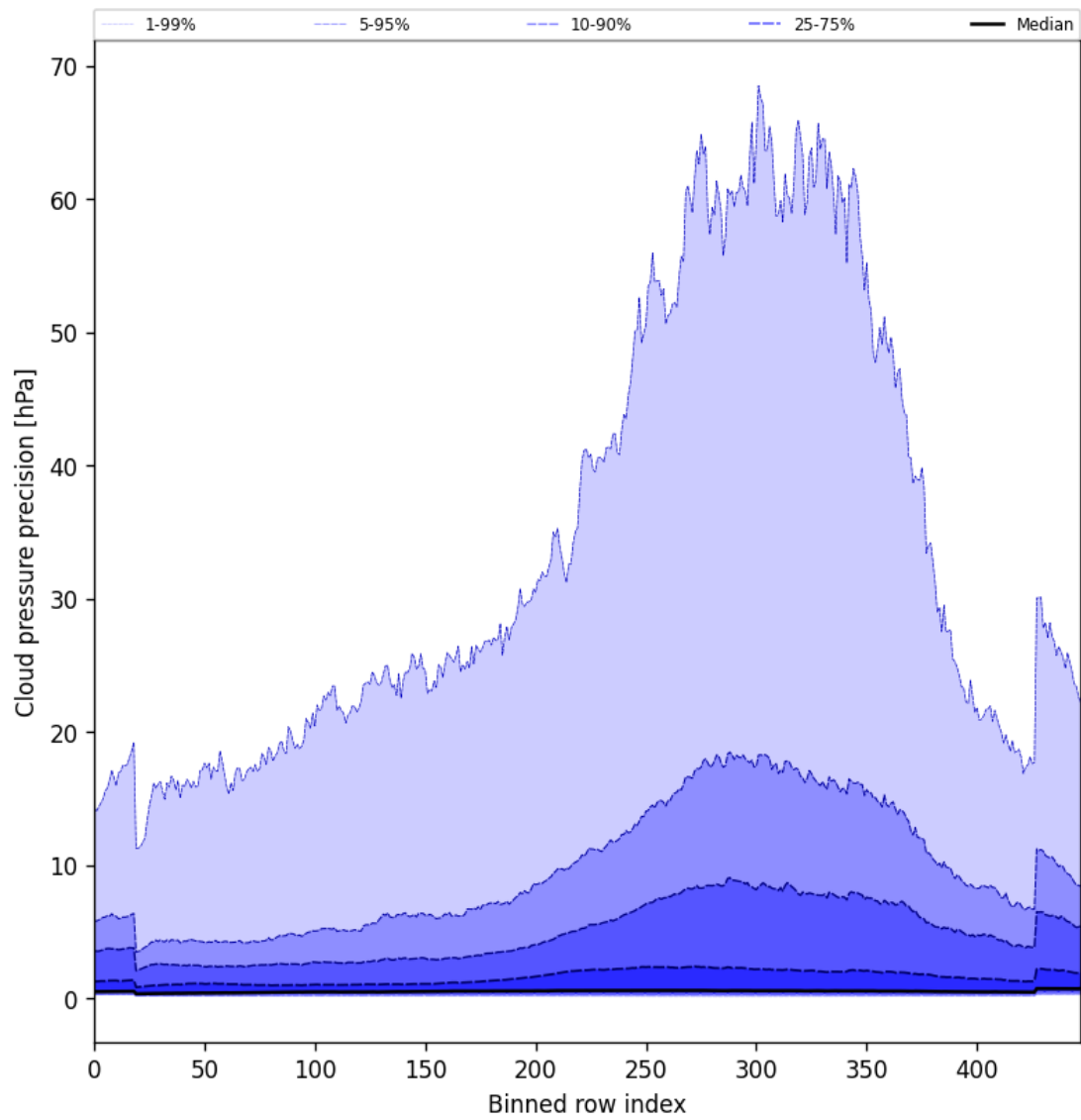
Figure 48: Along track statistics of “Cloud pressure precision” for 2025-11-12 to 2025-11-14
