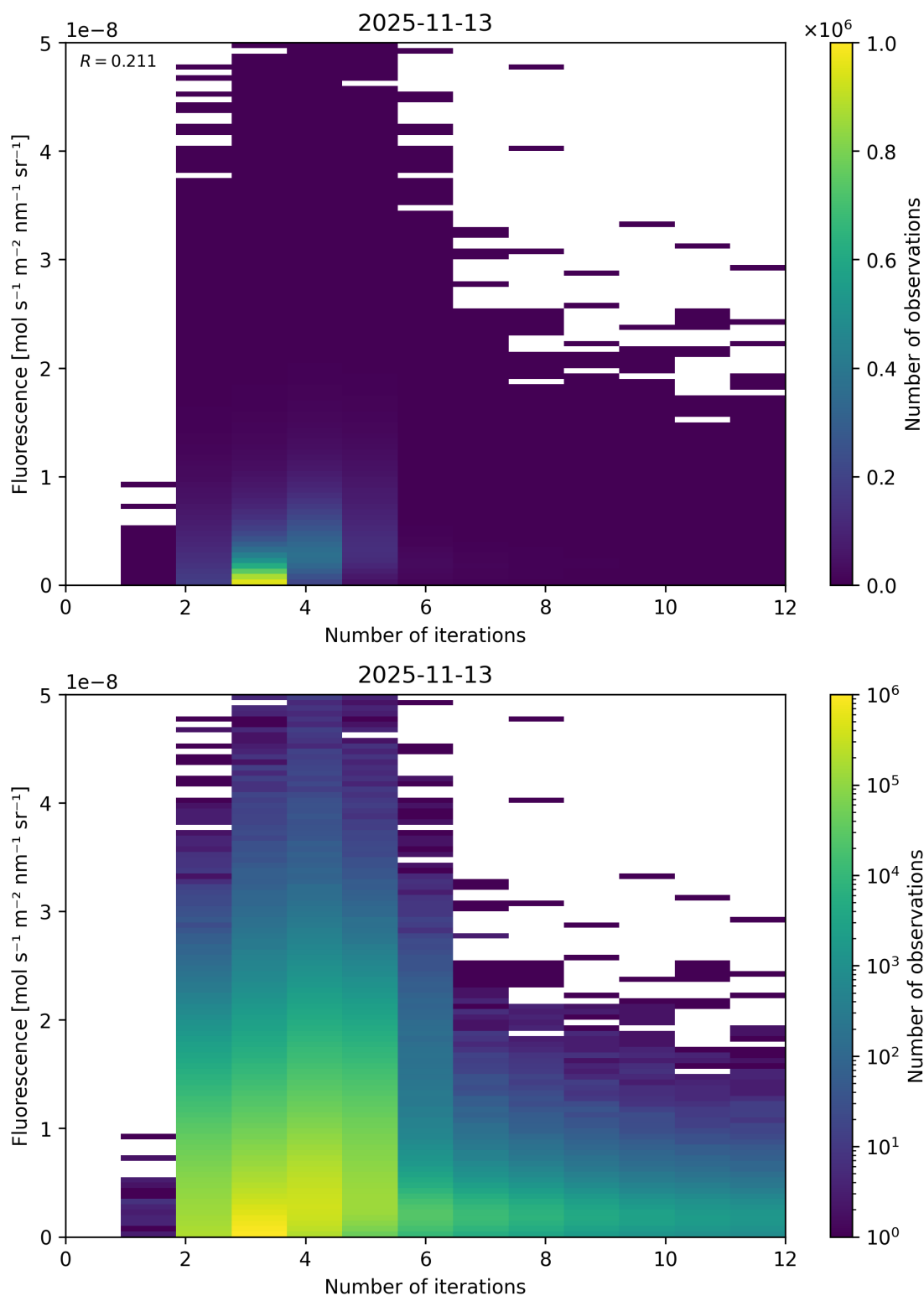
Figure 98: Scatter density plot of “Number of iterations” against “Fluorescence” for 2025-11-12 to 2025-11-14.
