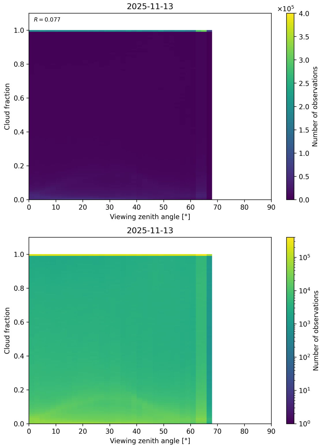
Figure 120: Scatter density plot of “Viewing zenith angle” against “Cloud fraction” for 2025-11-12 to 2025-11-14.
