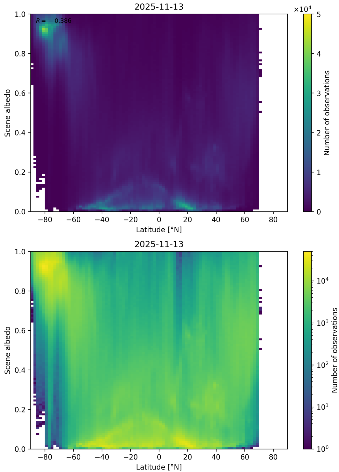
Figure 95: Scatter density plot of “Latitude” against “Scene albedo” for 2025-11-12 to 2025-11-14.
