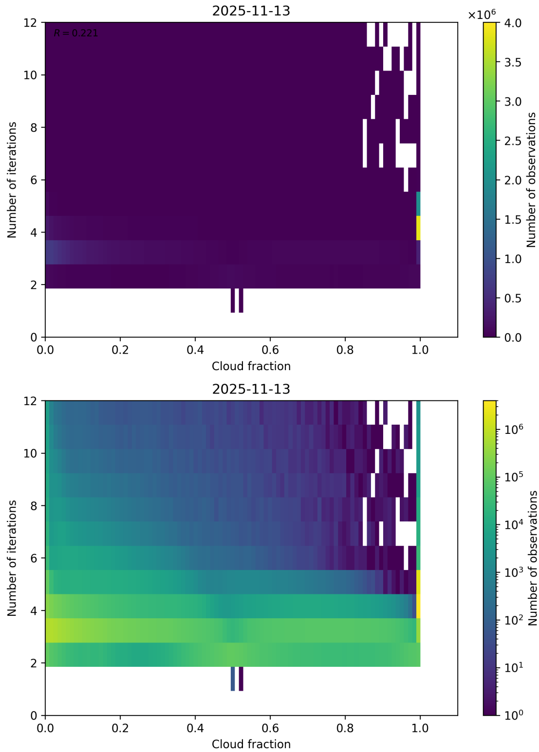
Figure 73: Scatter density plot of “Cloud fraction” against “Number of iterations” for 2025-11-12 to 2025-11-14.
