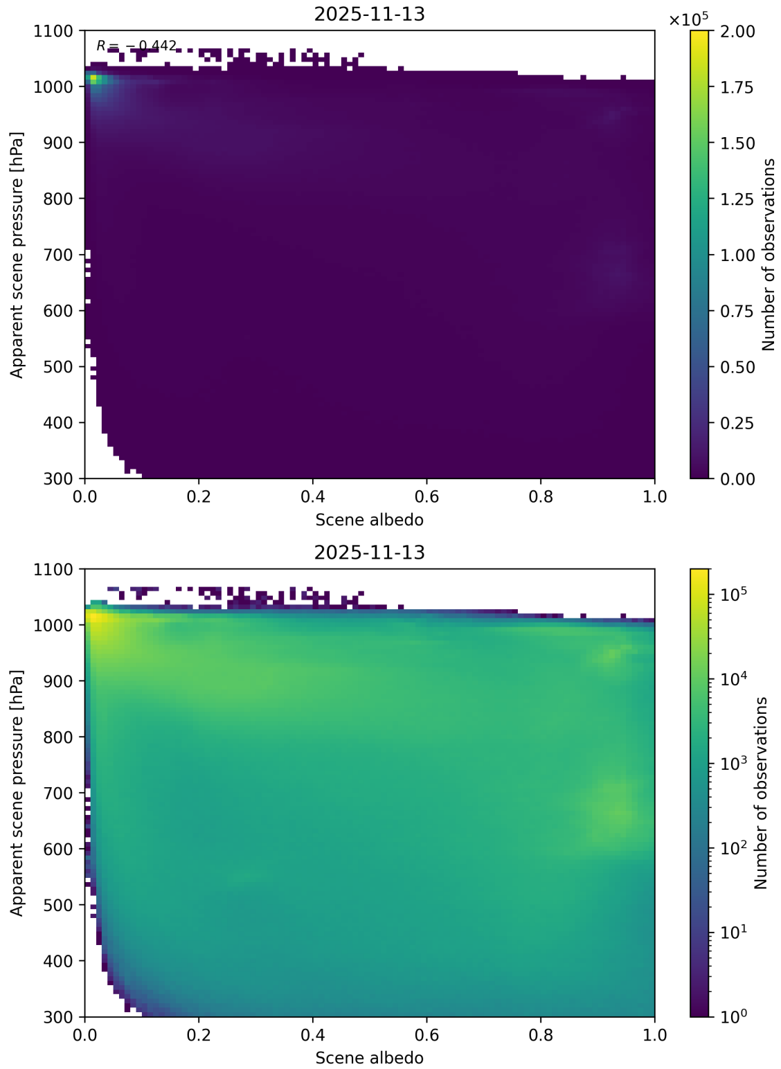
Figure 102: Scatter density plot of “Scene albedo” against “Apparent scene pressure” for 2025-11-12 to 2025-11-14.
