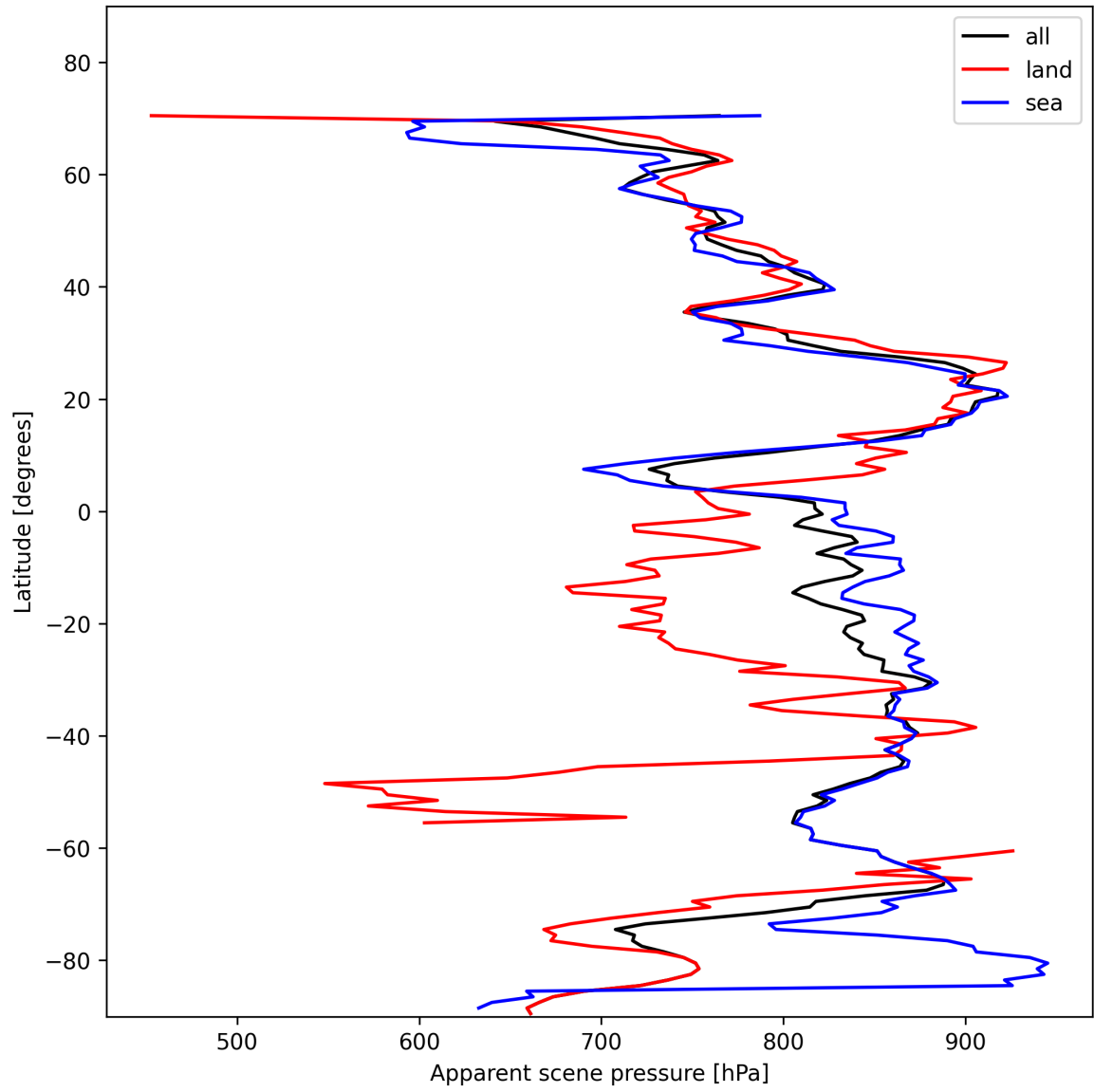
Figure 19: Zonal average of “Apparent scene pressure” for 2025-11-12 to 2025-11-14.
