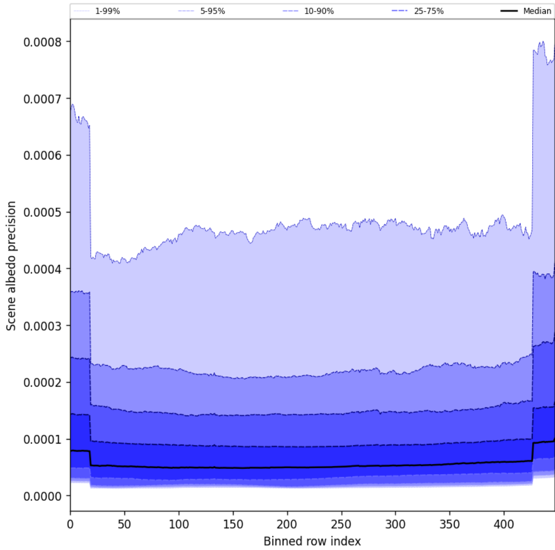
Figure 52: Along track statistics of “Scene albedo precision” for 2025-11-13 to 2025-11-15
