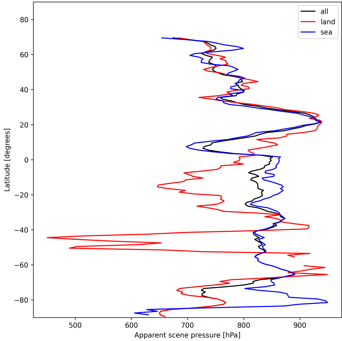
Figure 19: Zonal average of “Apparent scene pressure” for 2025-11-13 to 2025-11-15.
