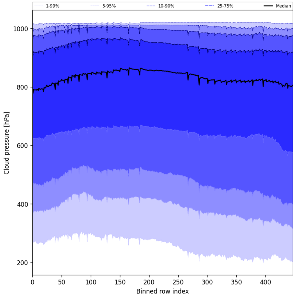
Figure 47: Along track statistics of “Cloud pressure” for 2025-11-13 to 2025-11-15
