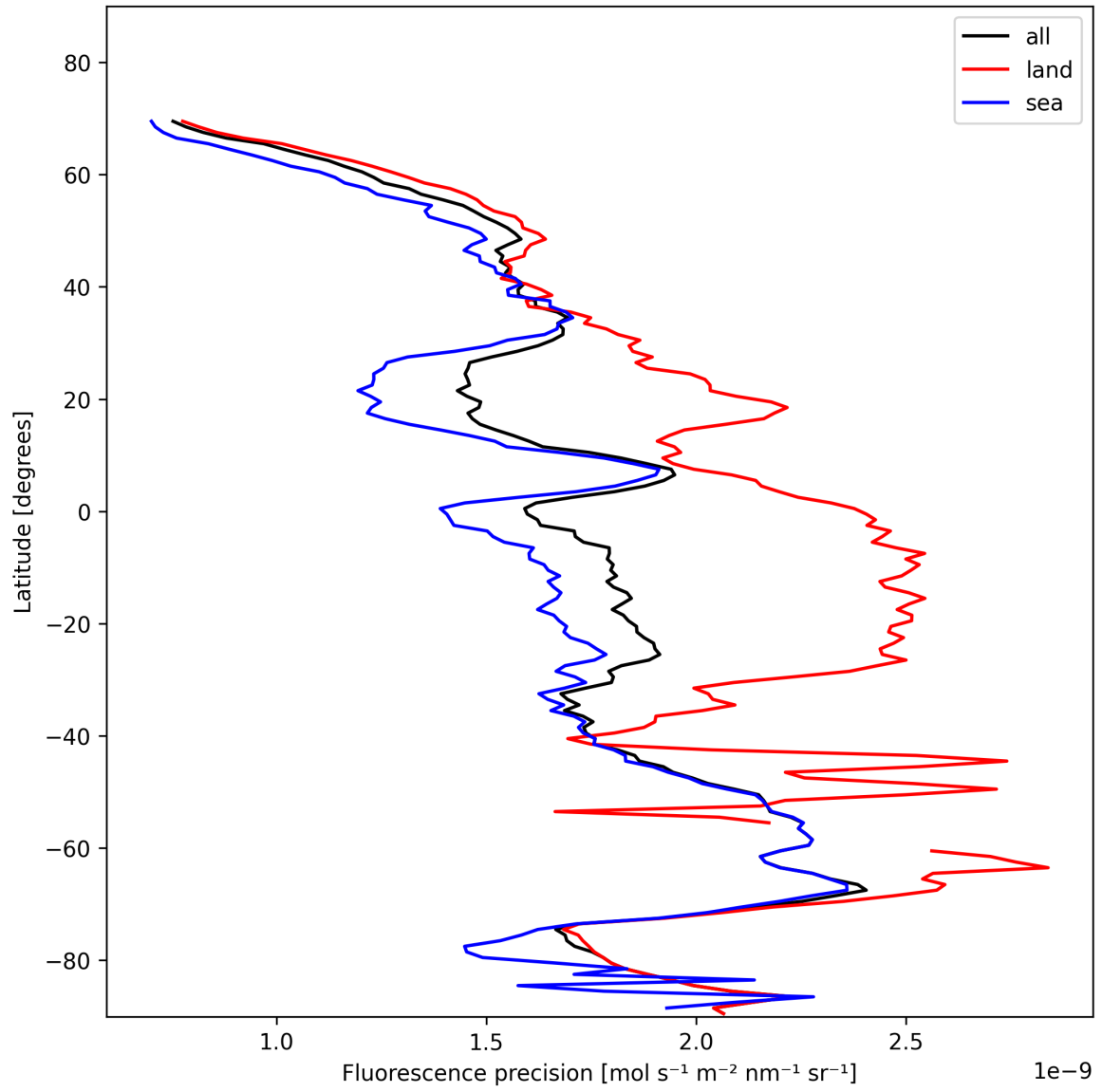
Figure 24: Zonal average of “Fluorescence precision” for 2025-11-13 to 2025-11-15.
