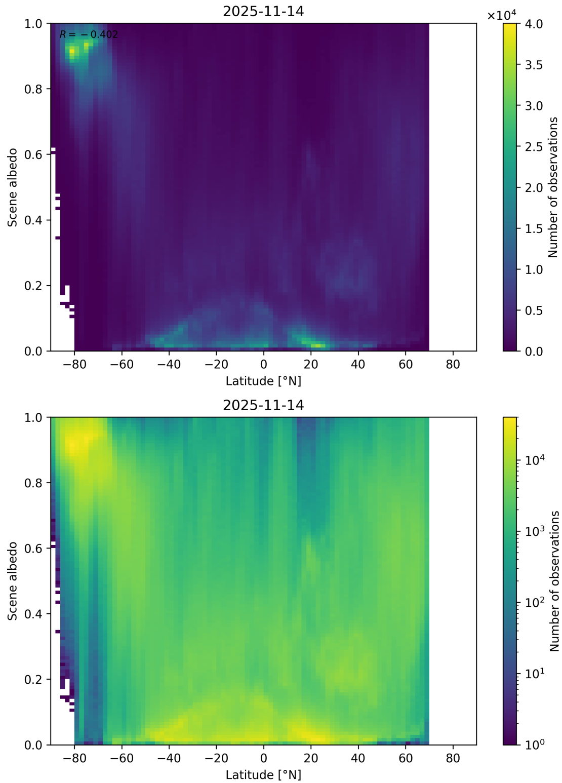
Figure 95: Scatter density plot of “Latitude” against “Scene albedo” for 2025-11-13 to 2025-11-15.
