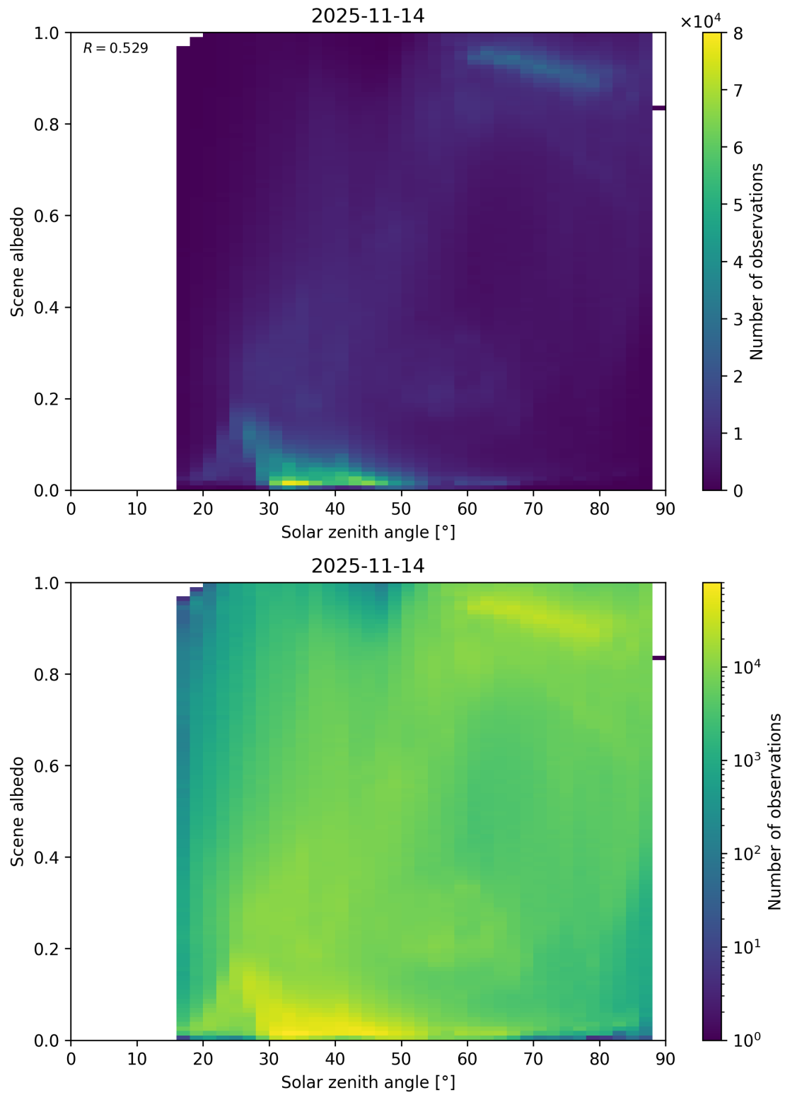
Figure 116: Scatter density plot of “Solar zenith angle” against “Scene albedo” for 2025-11-13 to 2025-11-15.
