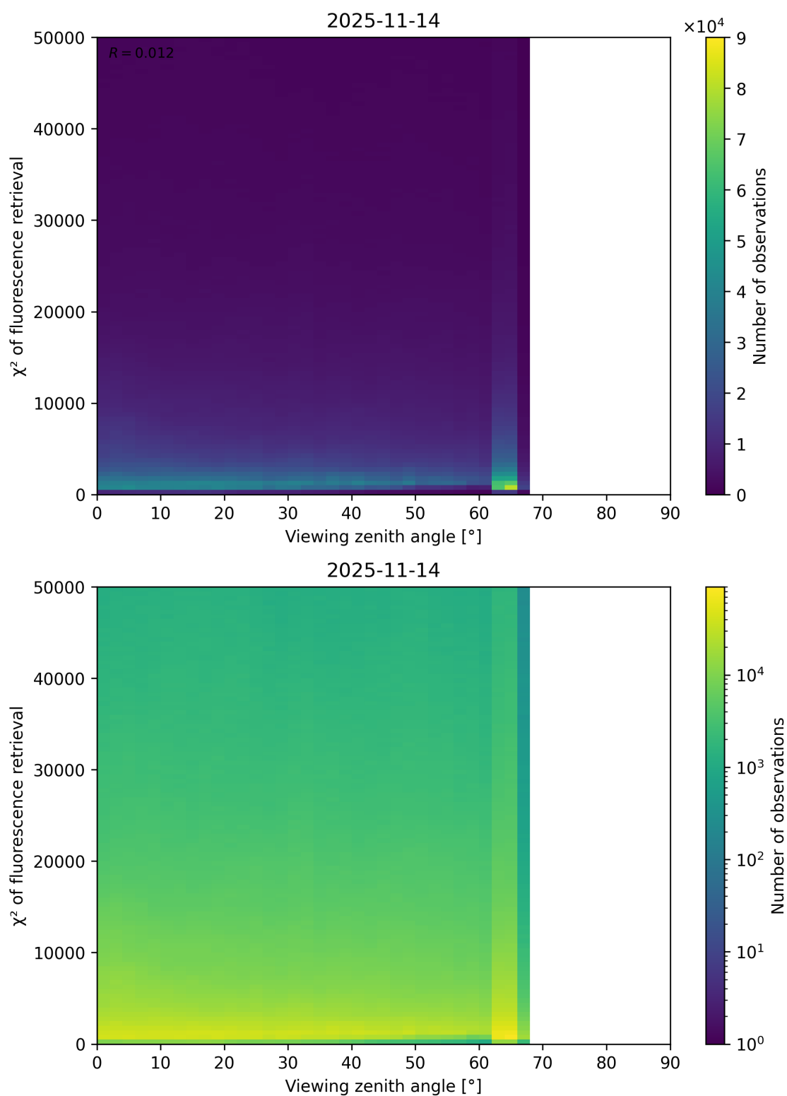
Figure 119: Scatter density plot of “Viewing zenith angle” against “ \chi^2 of fluorescence retrieval” for 2025-11-13 to 2025-11-15.
