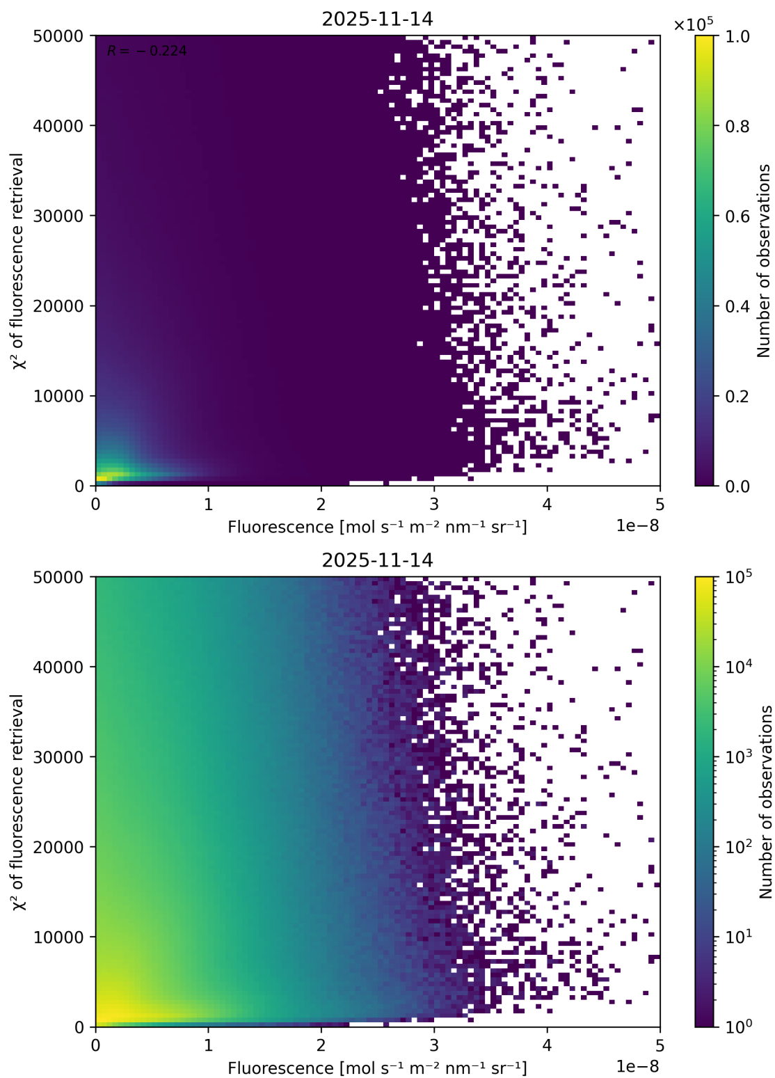
Figure 85: Scatter density plot of “Fluorescence” against “ \chi^2 of fluorescence retrieval” for 2025-11-13 to 2025-11-15.
