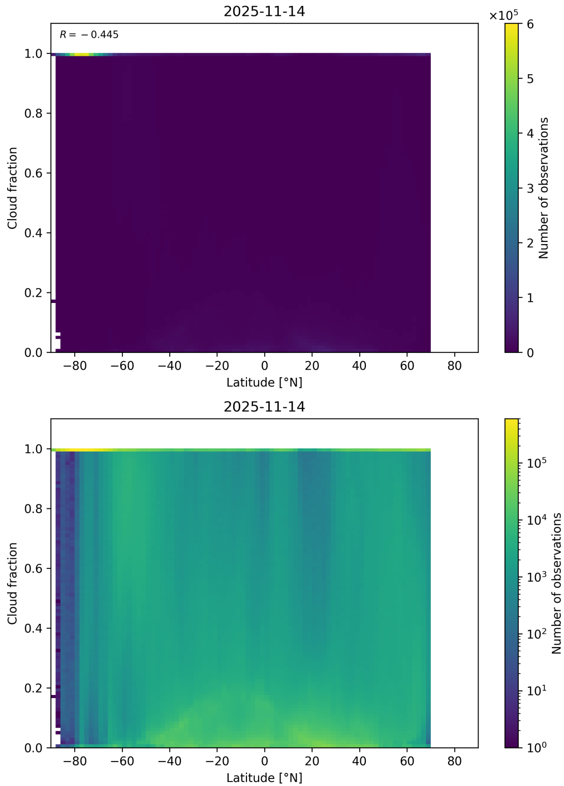
Figure 90: Scatter density plot of “Latitude” against “Cloud fraction” for 2025-11-13 to 2025-11-15.
