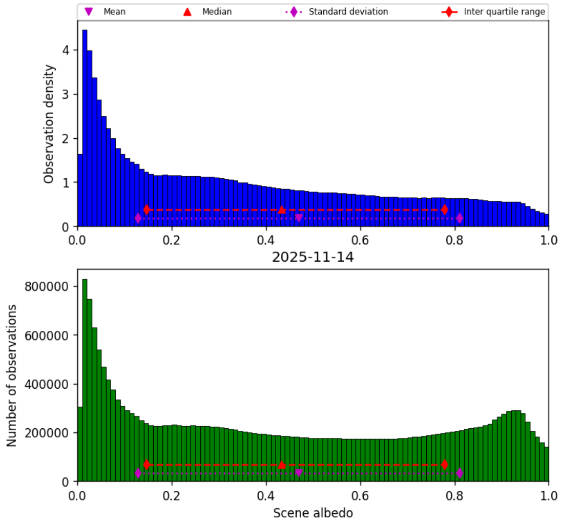
Figure 34: Histogram of “Scene albedo” for 2025-11-13 to 2025-11-15
