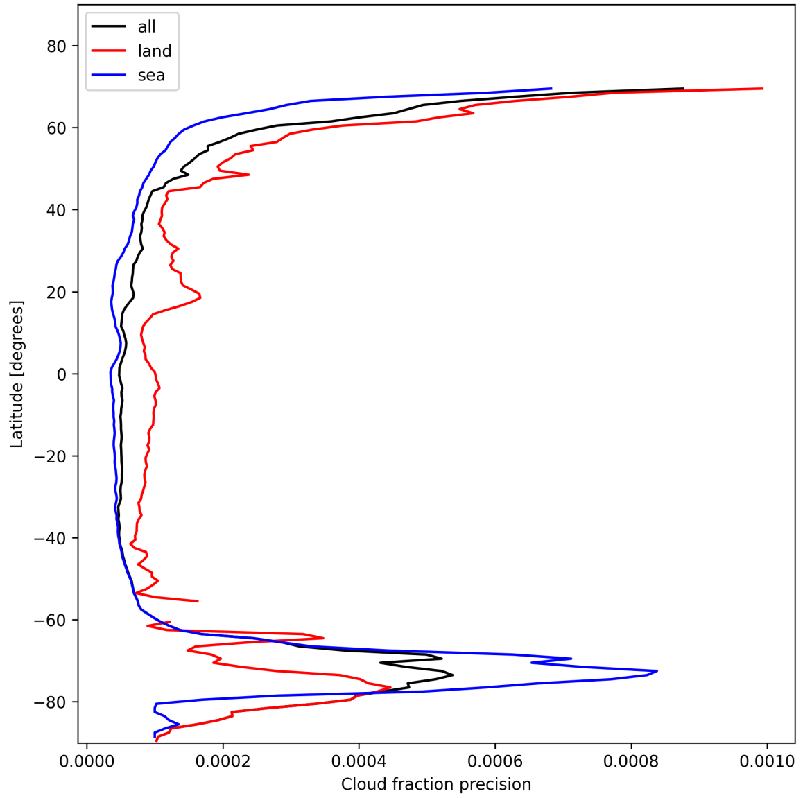
Figure 16: Zonal average of “Cloud fraction precision” for 2025-11-13 to 2025-11-15.
