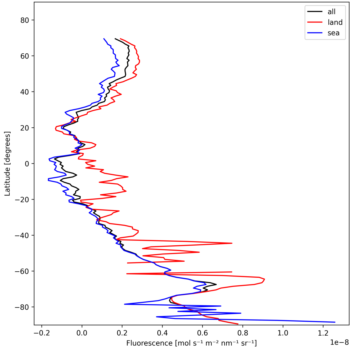
Figure 23: Zonal average of “Fluorescence” for 2025-11-13 to 2025-11-15.
