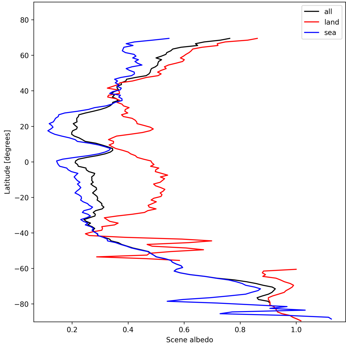
Figure 17: Zonal average of “Scene albedo” for 2025-11-13 to 2025-11-15.
