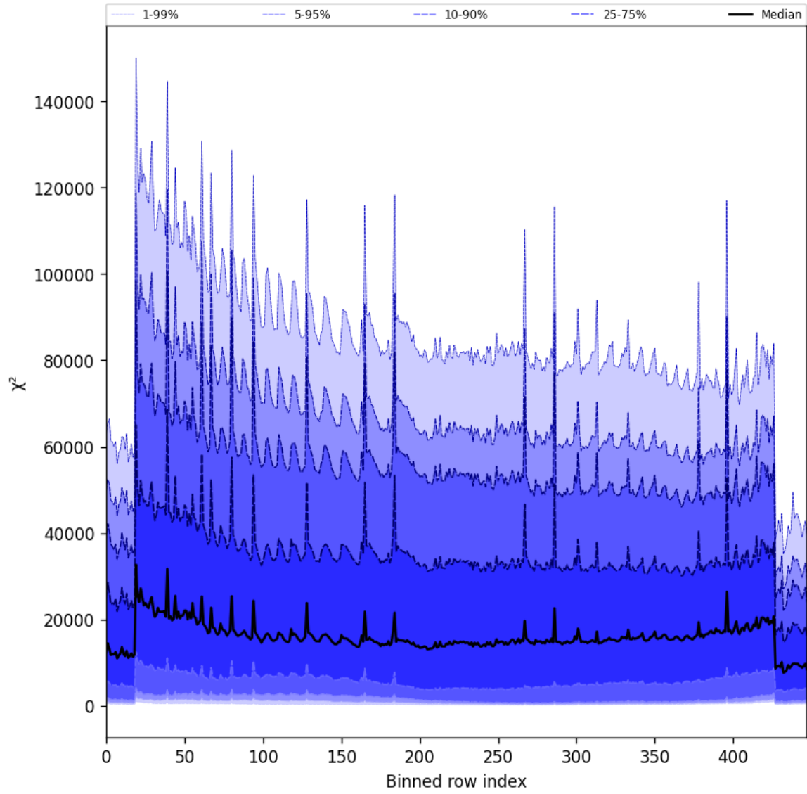
Figure 55: Along track statistics of “ \chi^2 ” for 2025-11-13 to 2025-11-15
