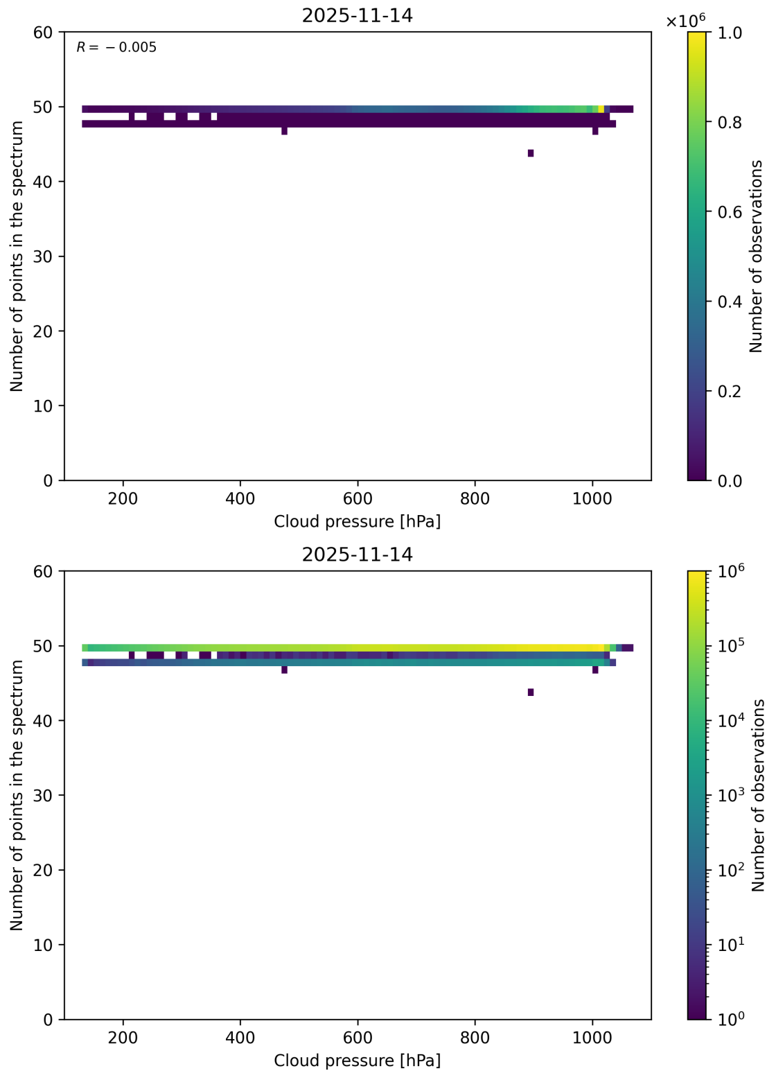
Figure 82: Scatter density plot of “Cloud pressure” against “Number of points in the spectrum” for 2025-11-13 to 2025-11-15.
