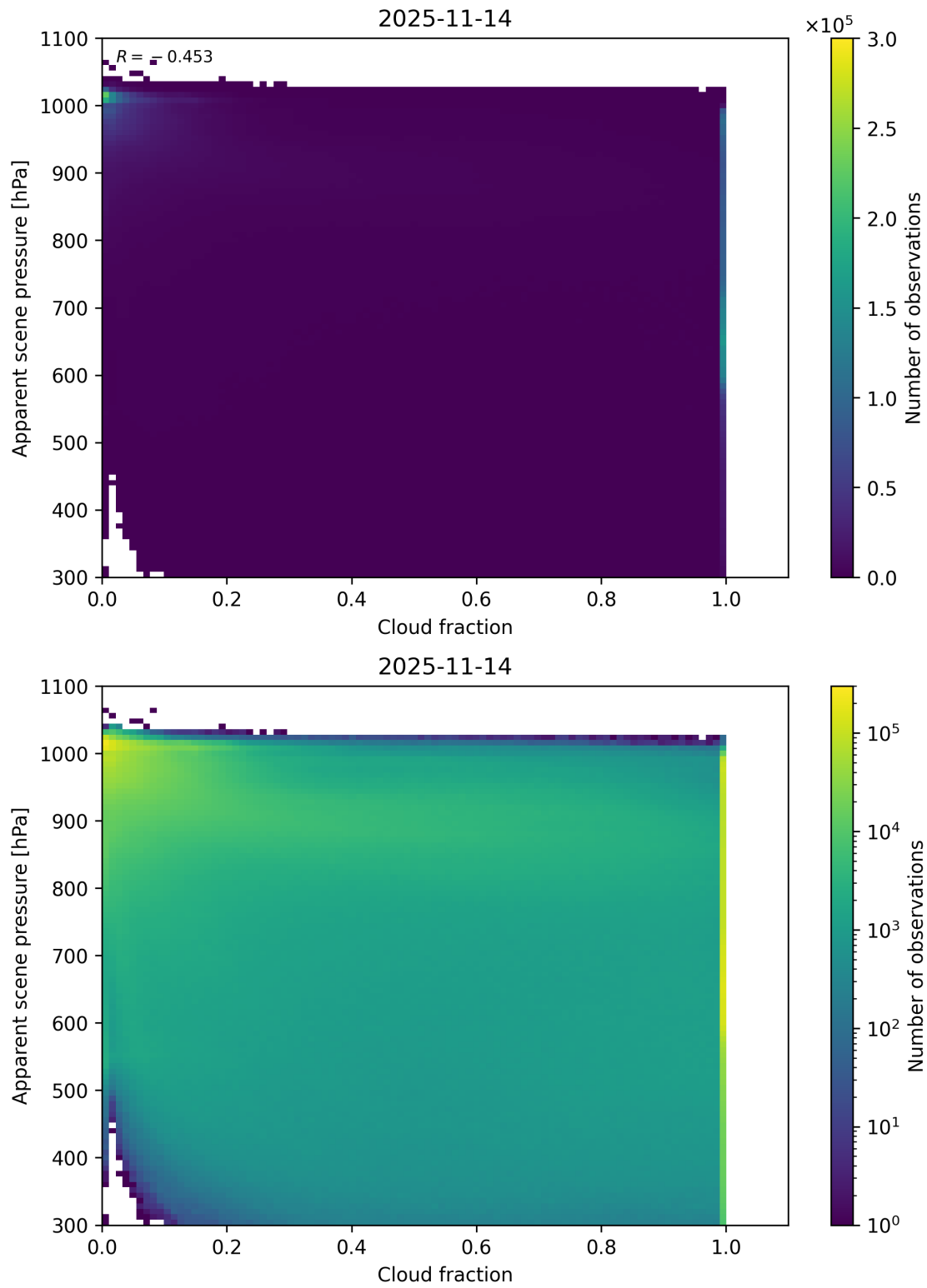
Figure 70: Scatter density plot of “Cloud fraction” against “Apparent scene pressure” for 2025-11-13 to 2025-11-15.
