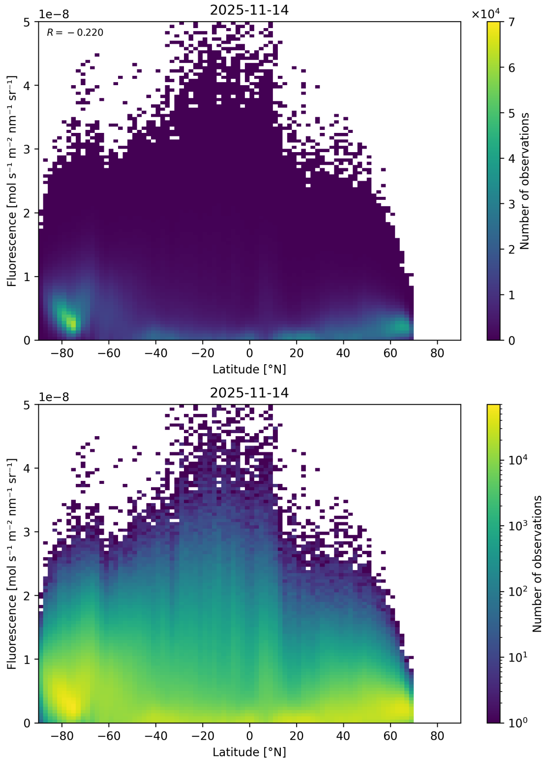
Figure 92: Scatter density plot of “Latitude” against “Fluorescence” for 2025-11-13 to 2025-11-15.
