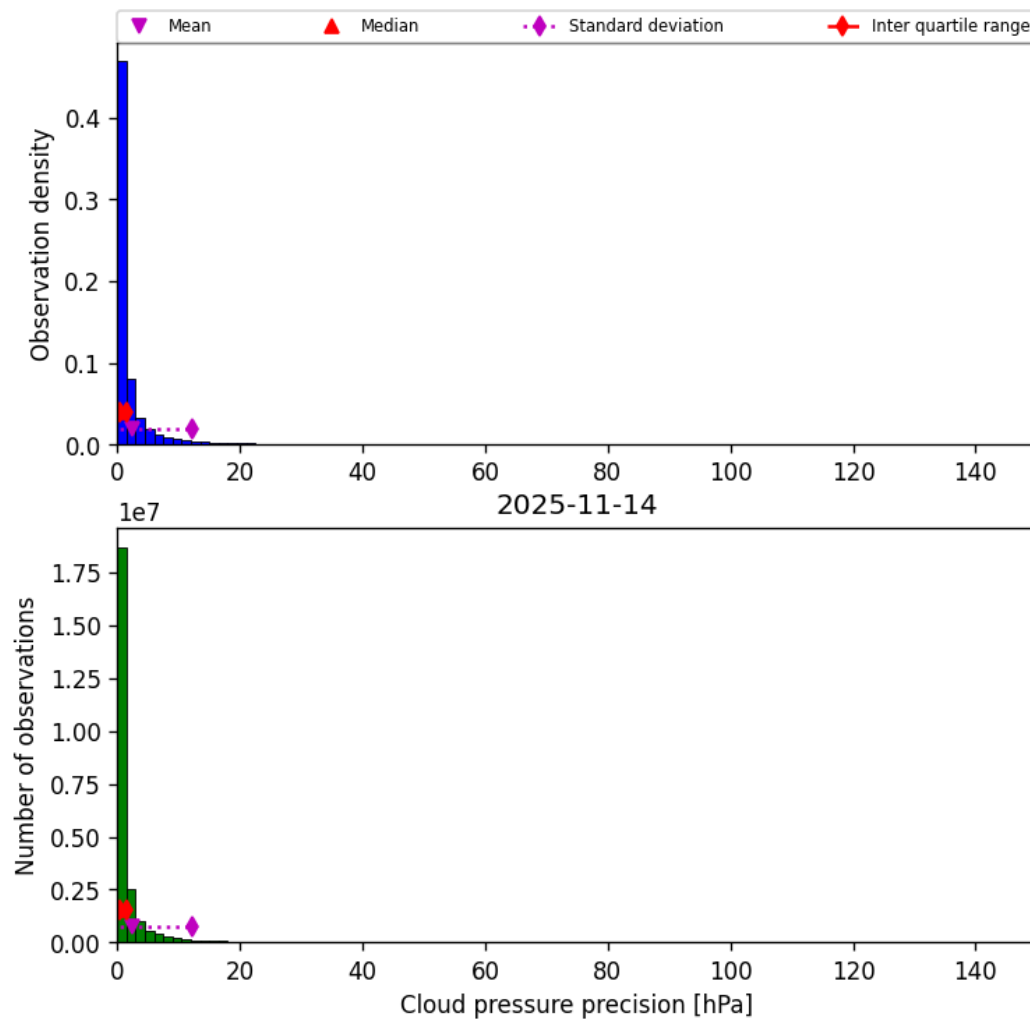
Figure 31: Histogram of “Cloud pressure precision” for 2025-11-13 to 2025-11-15
