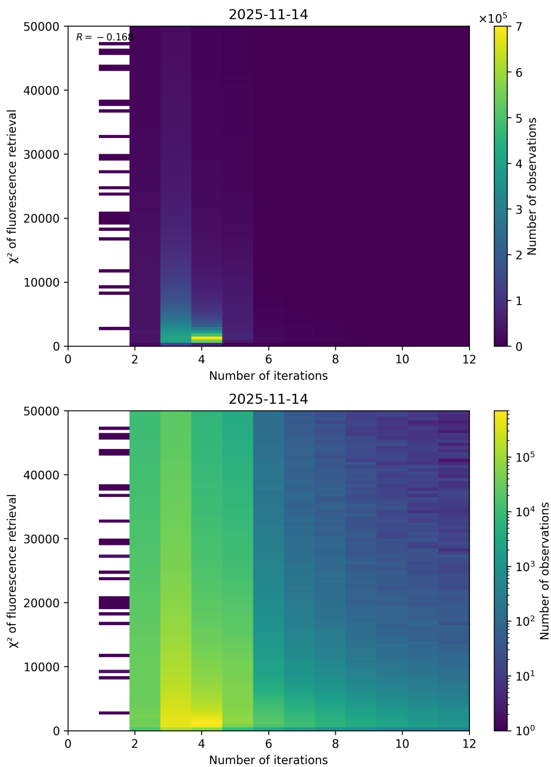
Figure 97: Scatter density plot of “Number of iterations” against “ \chi^2 of fluorescence retrieval” for 2025-11-13 to 2025-11-15.
