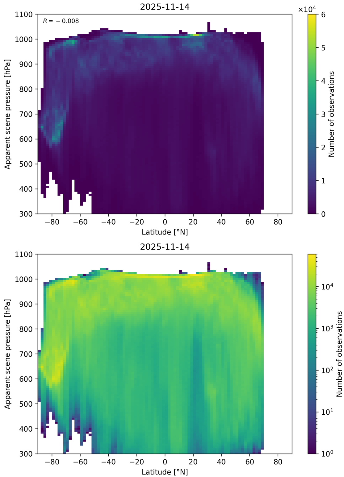
Figure 88: Scatter density plot of “Latitude” against “Apparent scene pressure” for 2025-11-13 to 2025-11-15.
