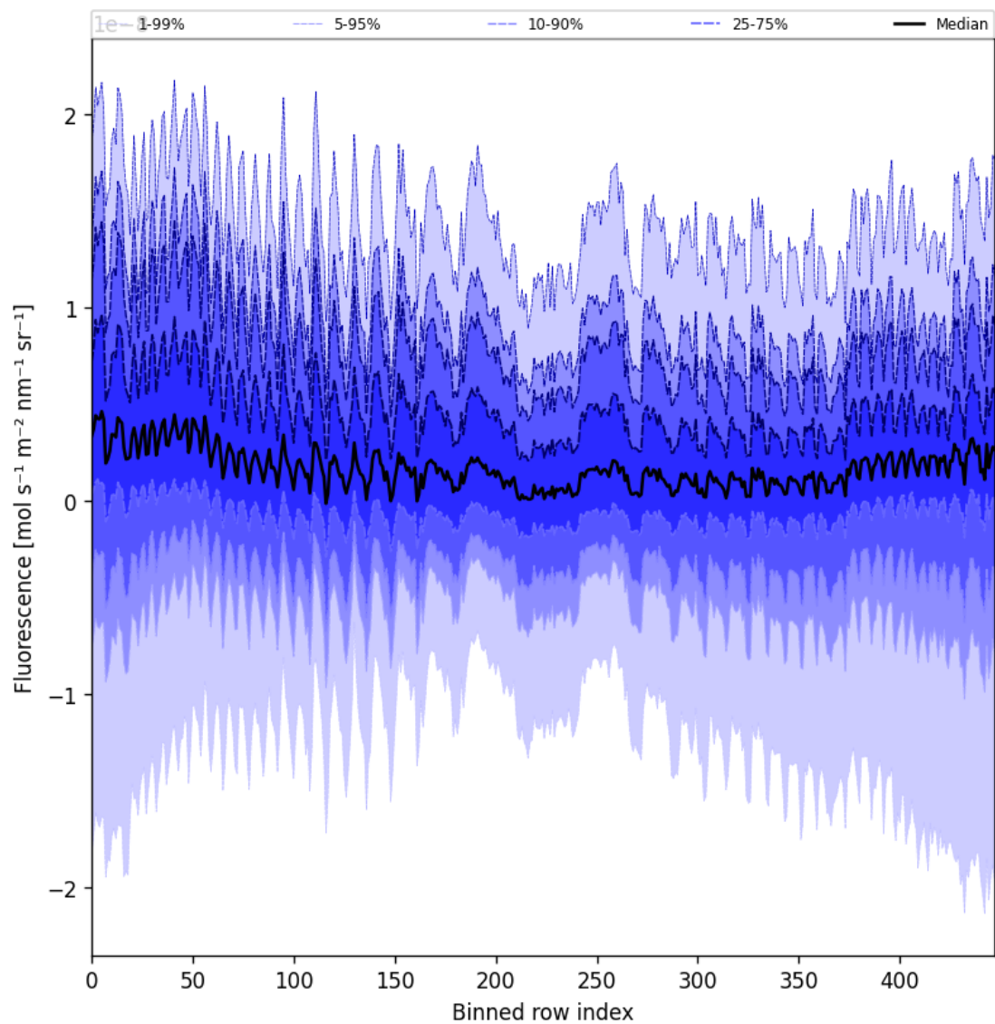
Figure 57: Along track statistics of “Fluorescence” for 2025-11-13 to 2025-11-15
