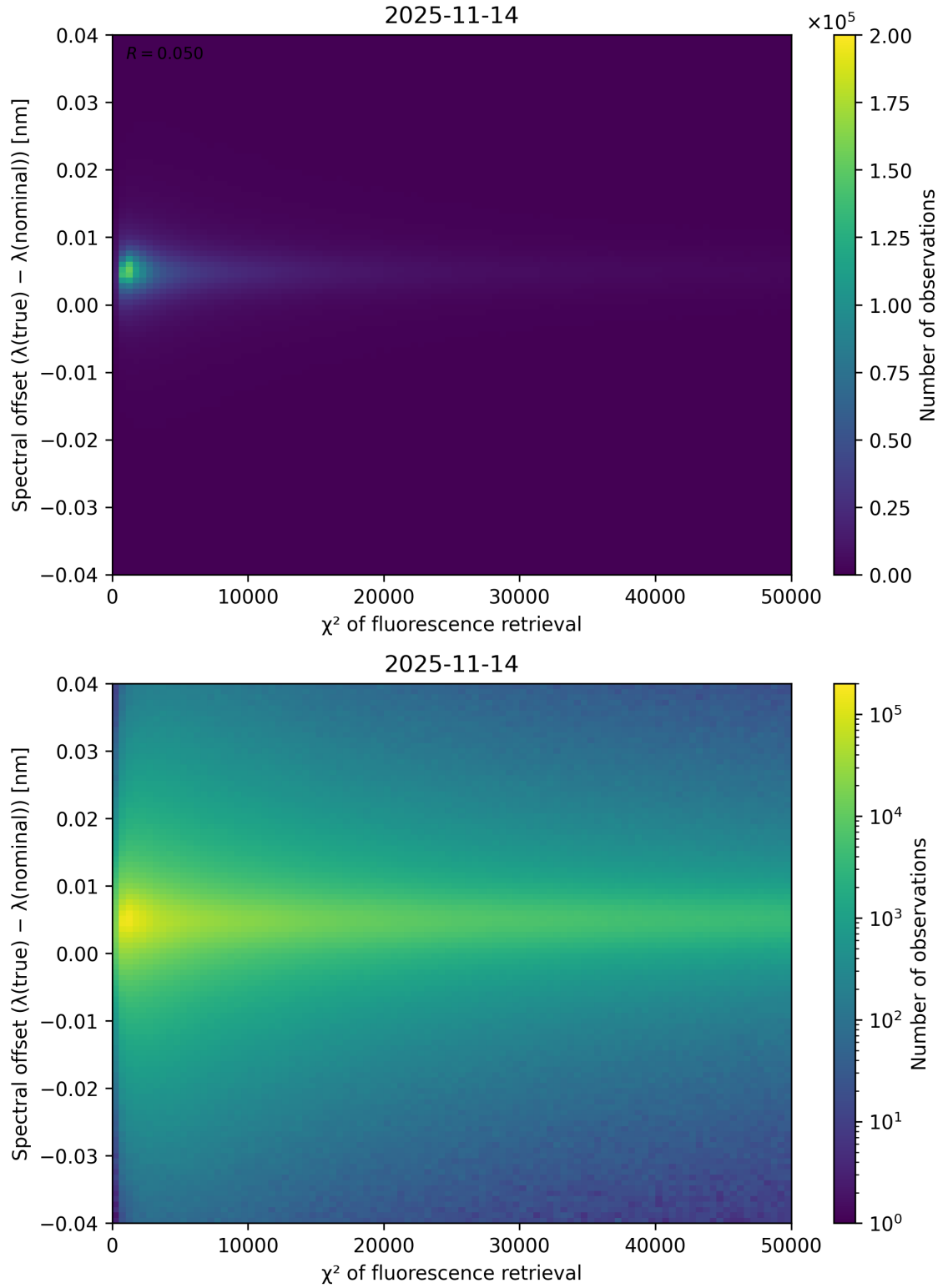
Figure 69: Scatter density plot of “ \chi^2 of fluorescence retrieval” against “Spectral offset ( \lambda_{\text{true}} - \lambda_{\text{nominal}} )” for 2025-11-13 to 2025-11-15.
