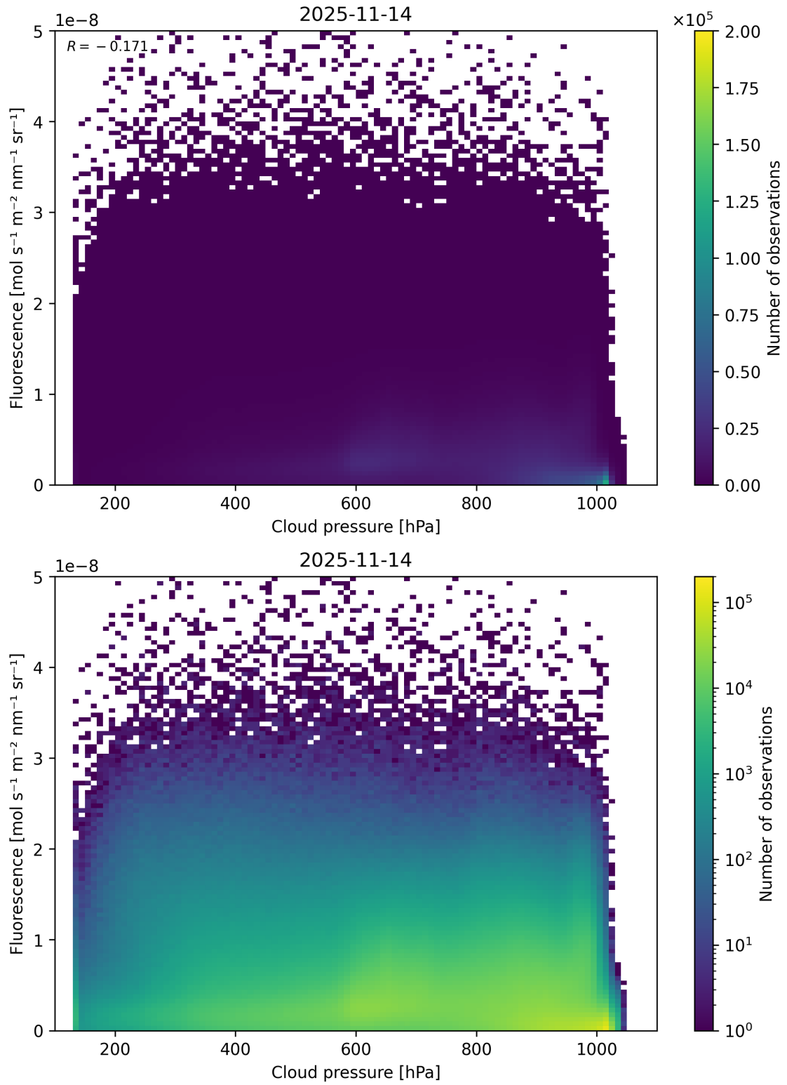
Figure 80: Scatter density plot of “Cloud pressure” against “Fluorescence” for 2025-11-13 to 2025-11-15.
