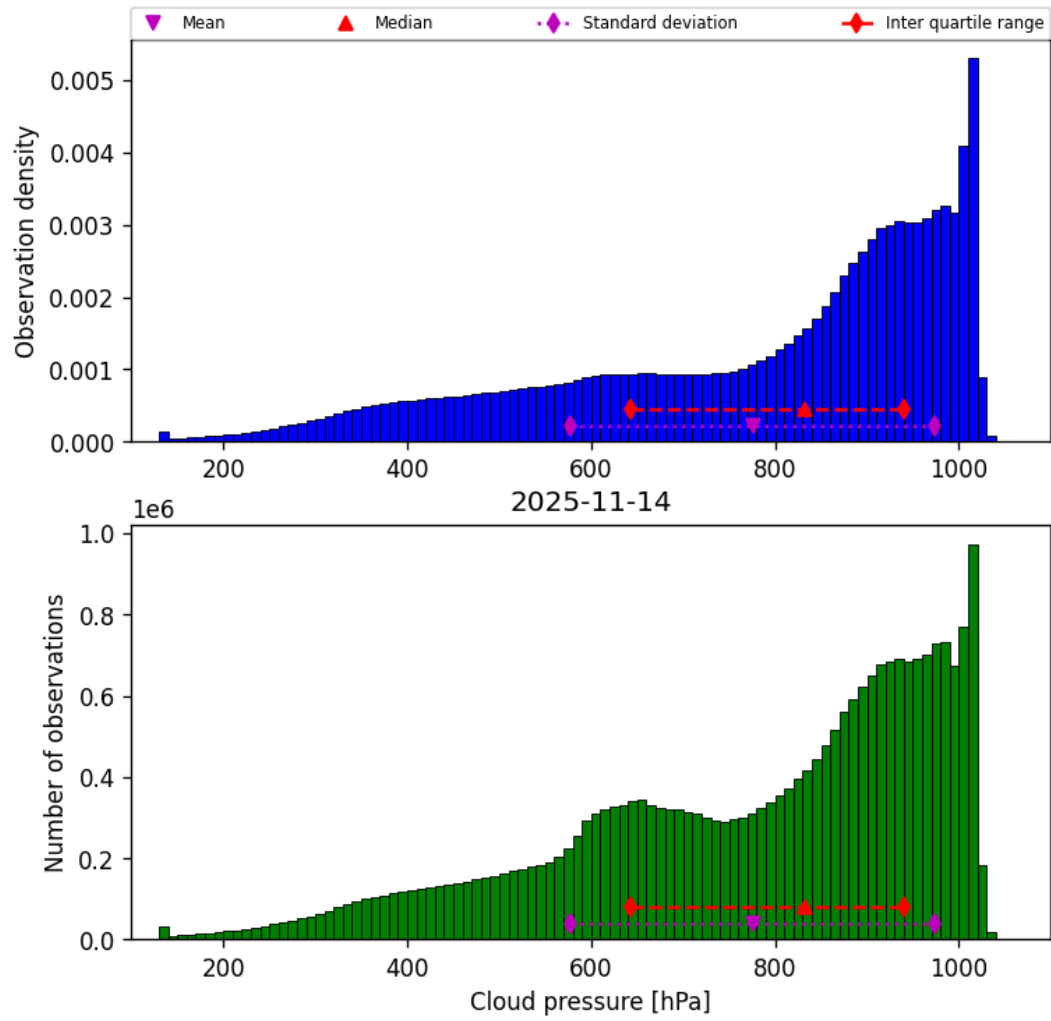
Figure 30: Histogram of “Cloud pressure” for 2025-11-13 to 2025-11-15
