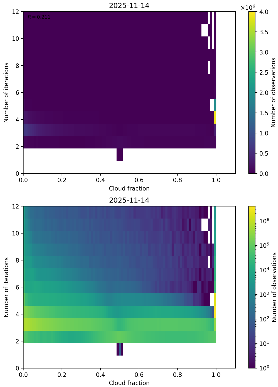
Figure 73: Scatter density plot of “Cloud fraction” against “Number of iterations” for 2025-11-13 to 2025-11-15.
