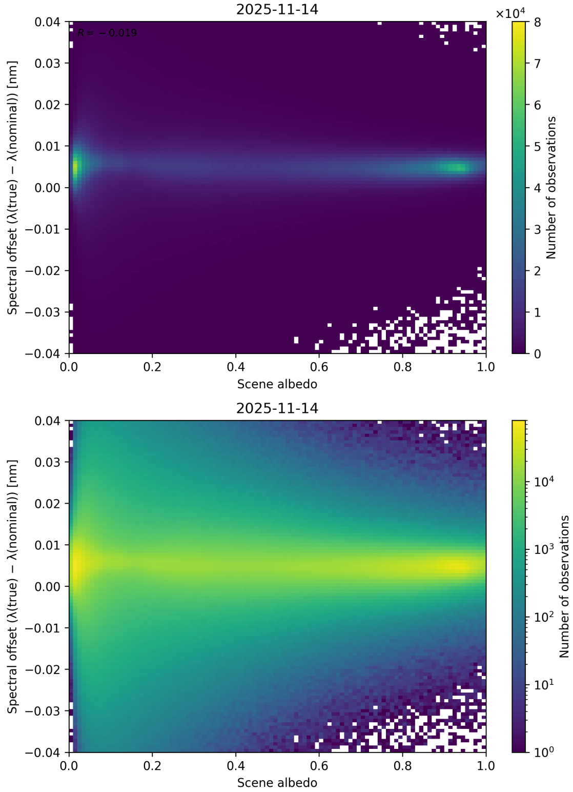
Figure 107: Scatter density plot of “Scene albedo” against “Spectral offset ( \lambda_{\text{true}} - \lambda_{\text{nominal}} )” for 2025-11-13 to 2025-11-15.
