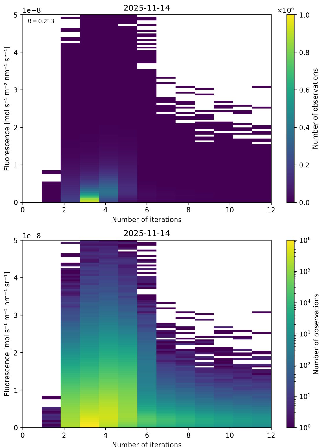
Figure 98: Scatter density plot of “Number of iterations” against “Fluorescence” for 2025-11-13 to 2025-11-15.
