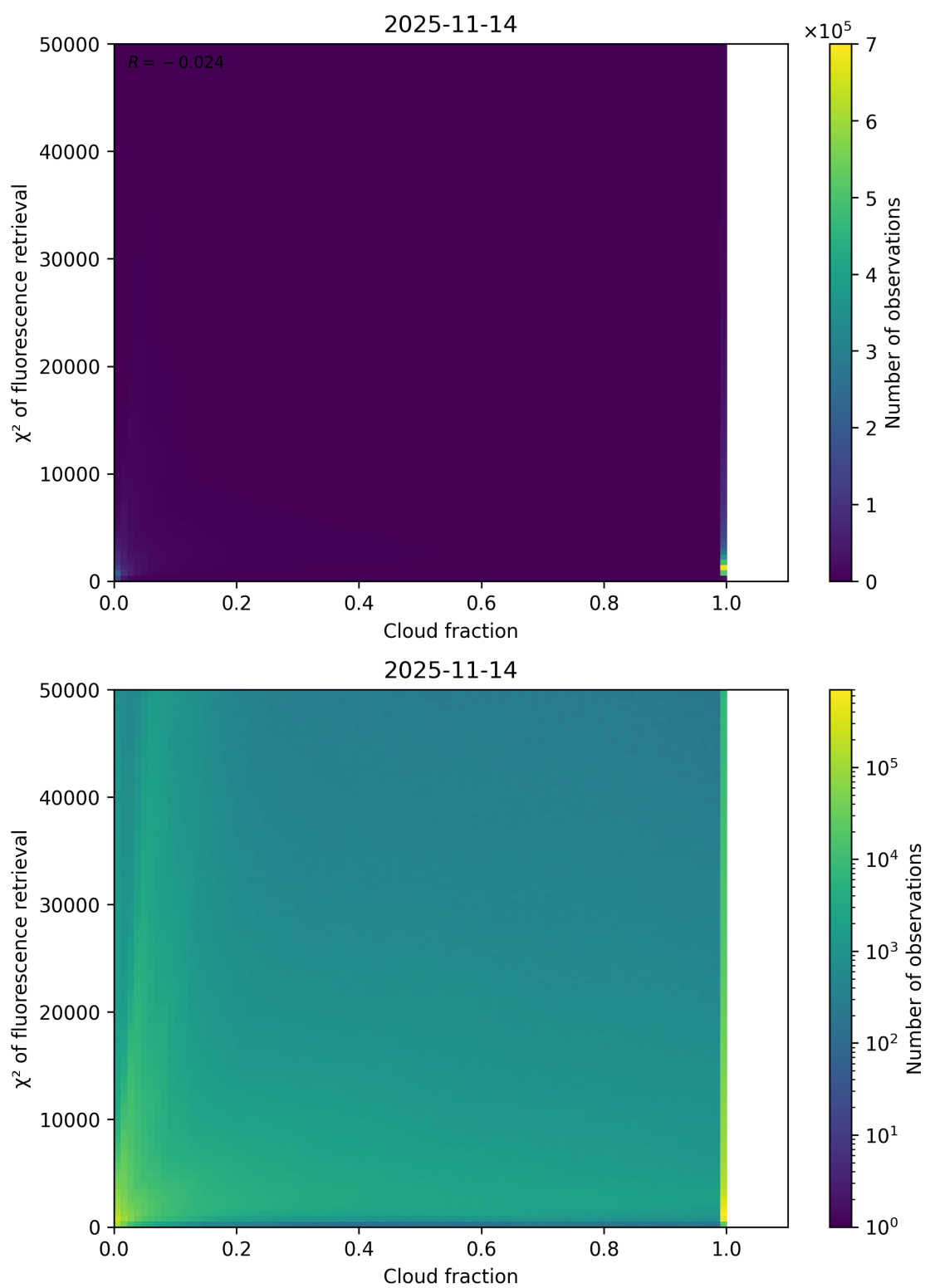
Figure 71: Scatter density plot of “Cloud fraction” against “ \chi^2 of fluorescence retrieval” for 2025-11-13 to 2025-11-15.
