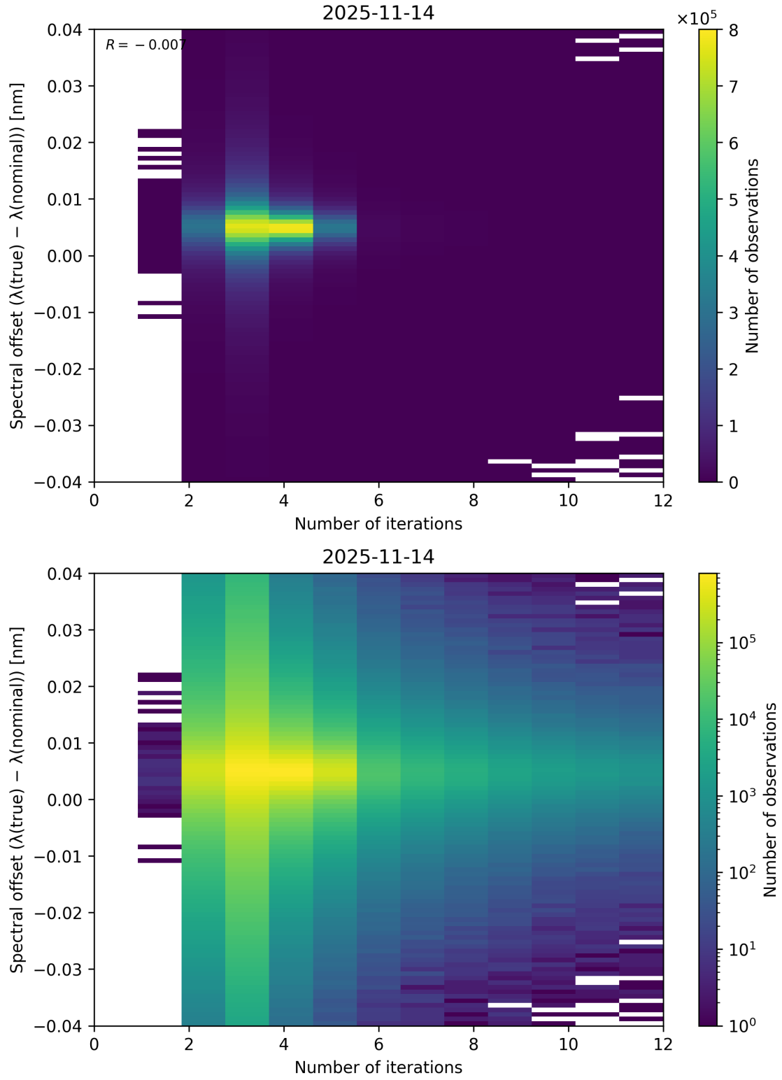
Figure 100: Scatter density plot of “Number of iterations” against “Spectral offset ( \lambda_{\text{true}} - \lambda_{\text{nominal}} )” for 2025-11-13 to 2025-11-15.
