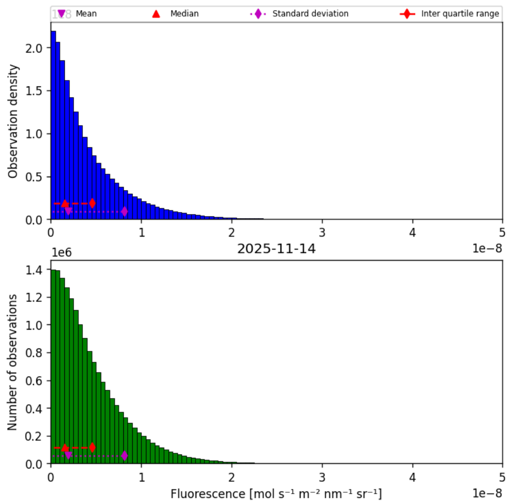
Figure 40: Histogram of “Fluorescence” for 2025-11-13 to 2025-11-15
