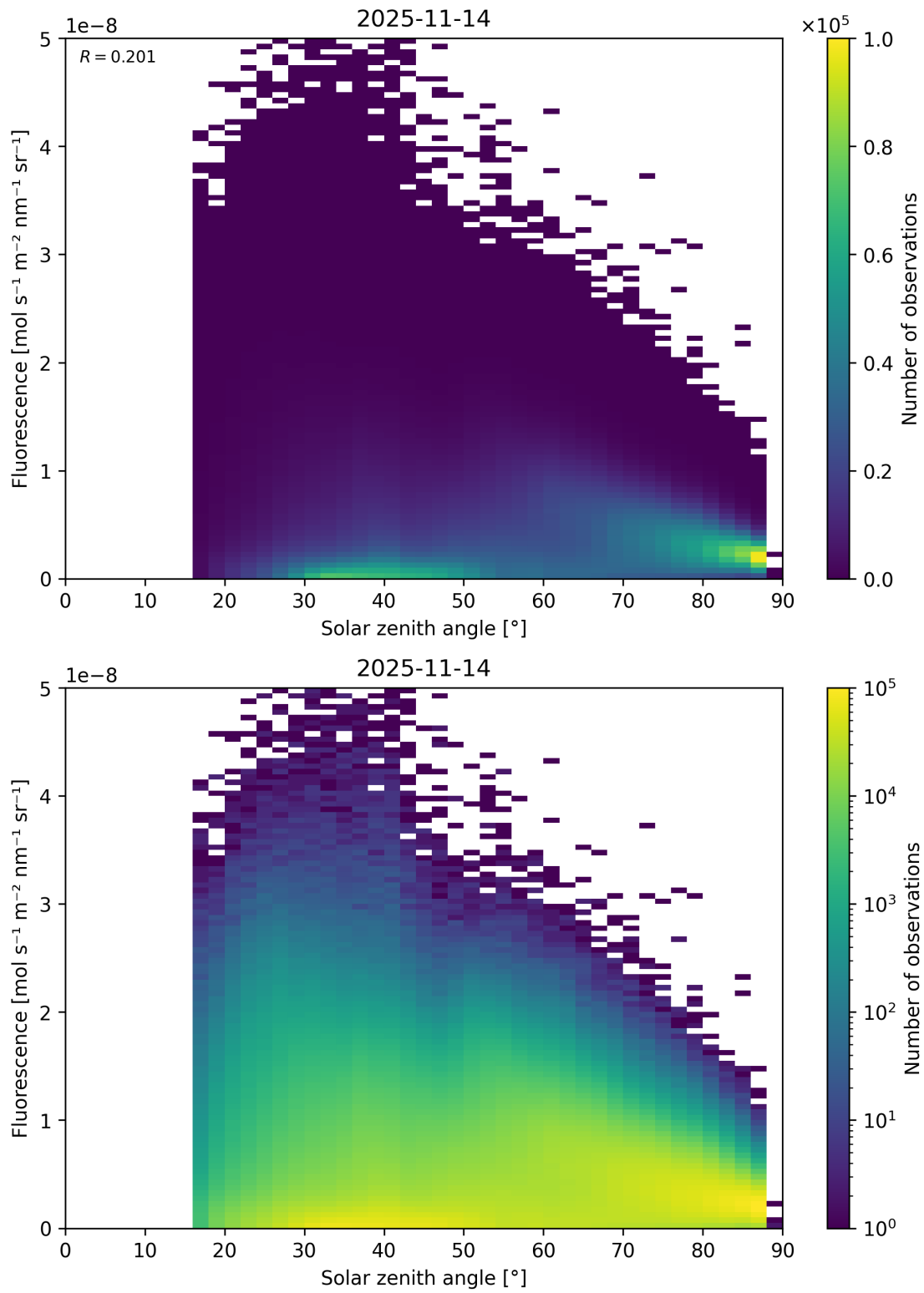
Figure 112: Scatter density plot of “Solar zenith angle” against “Fluorescence” for 2025-11-13 to 2025-11-15.
