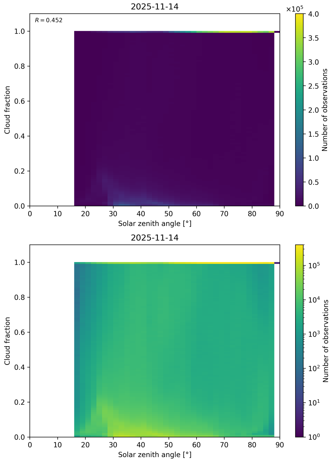
Figure 110: Scatter density plot of “Solar zenith angle” against “Cloud fraction” for 2025-11-13 to 2025-11-15.
