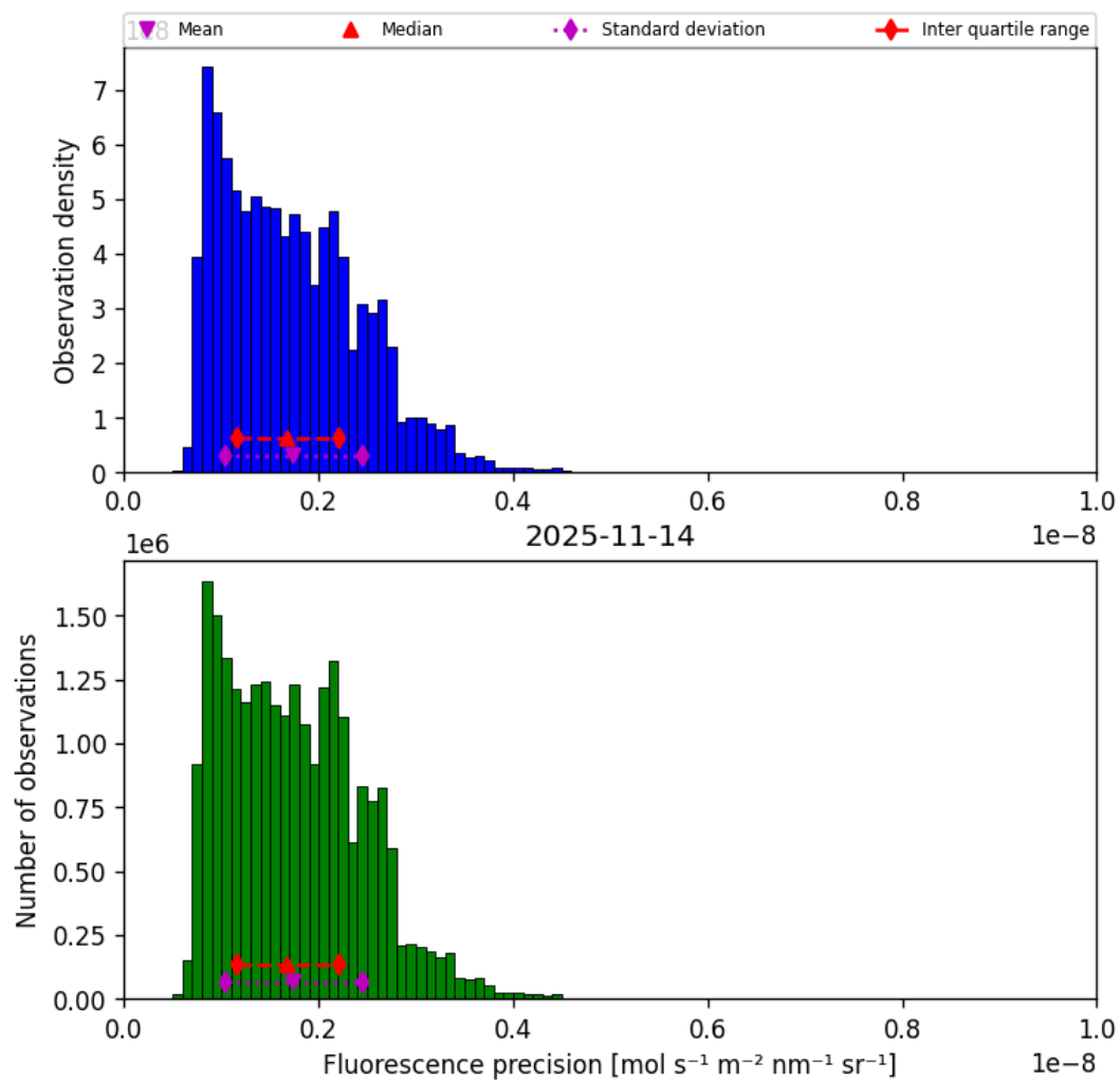
Figure 41: Histogram of “Fluorescence precision” for 2025-11-13 to 2025-11-15
