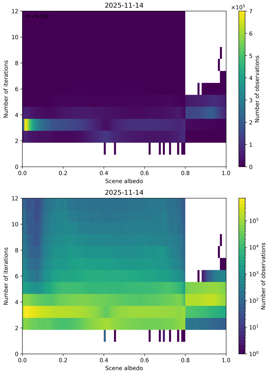
Figure 105: Scatter density plot of “Scene albedo” against “Number of iterations” for 2025-11-13 to 2025-11-15.
