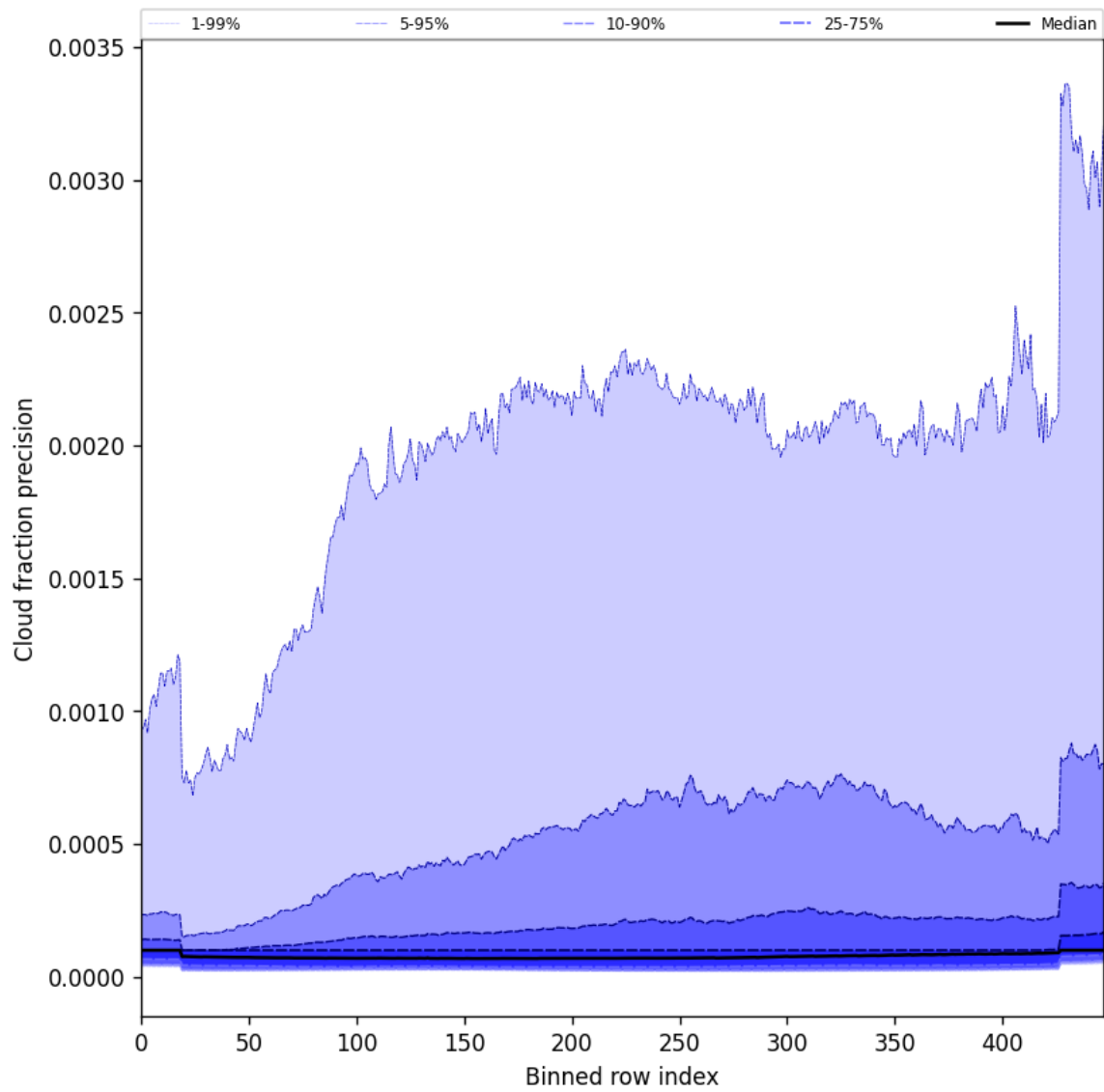
Figure 50: Along track statistics of “Cloud fraction precision” for 2025-11-13 to 2025-11-15
