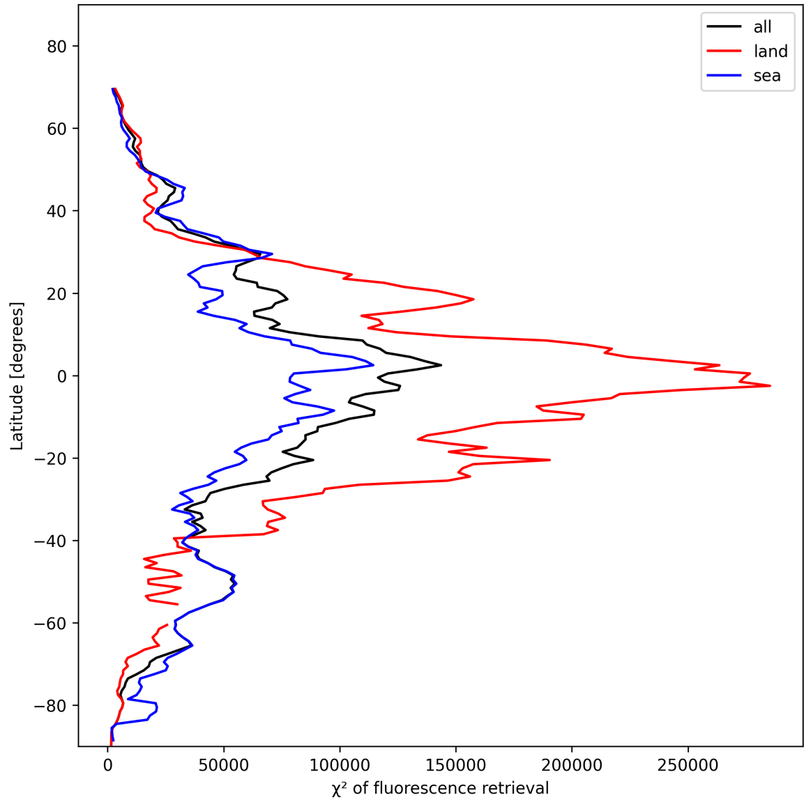
Figure 25: Zonal average of “ \chi^2 of fluorescence retrieval” for 2025-11-13 to 2025-11-15.
