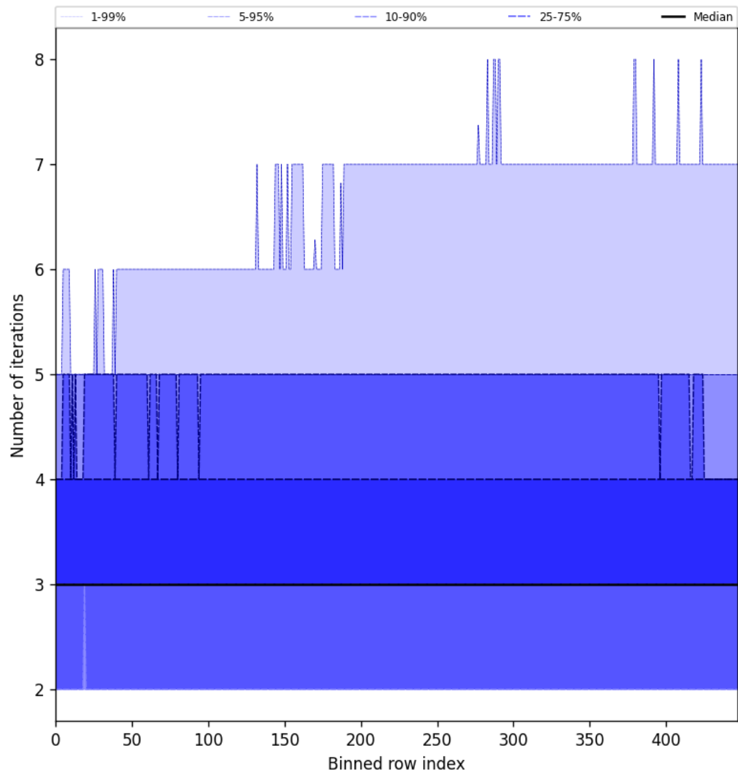
Figure 56: Along track statistics of “Number of iterations” for 2025-11-13 to 2025-11-15
