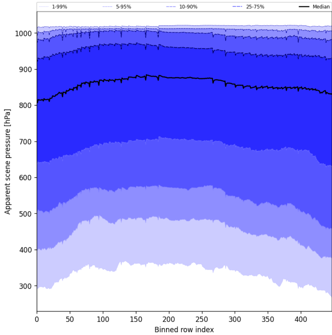
Figure 53: Along track statistics of “Apparent scene pressure” for 2025-11-13 to 2025-11-15
