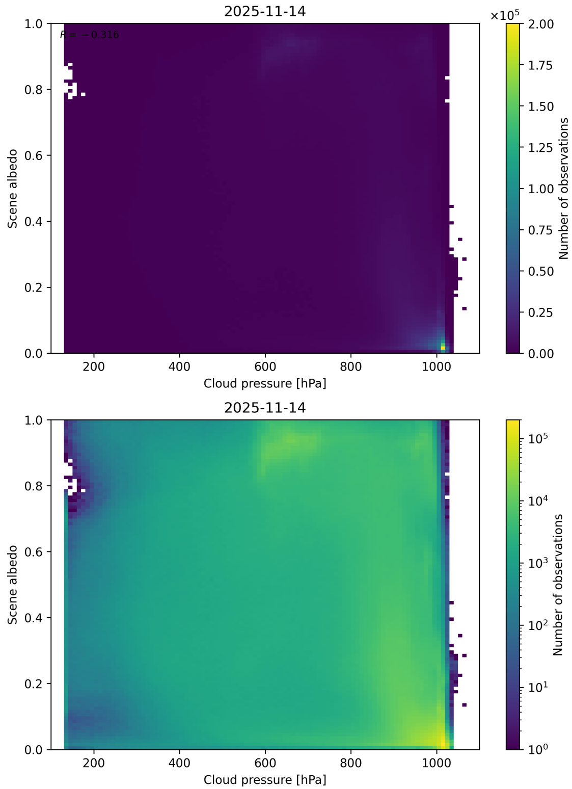
Figure 83: Scatter density plot of “Cloud pressure” against “Scene albedo” for 2025-11-13 to 2025-11-15.
