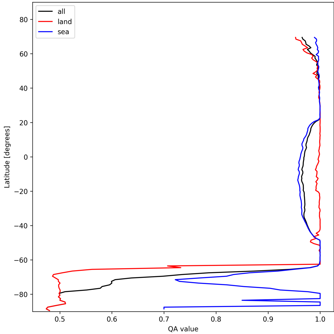
Figure 12: Zonal average of “QA value” for 2025-11-13 to 2025-11-15.
