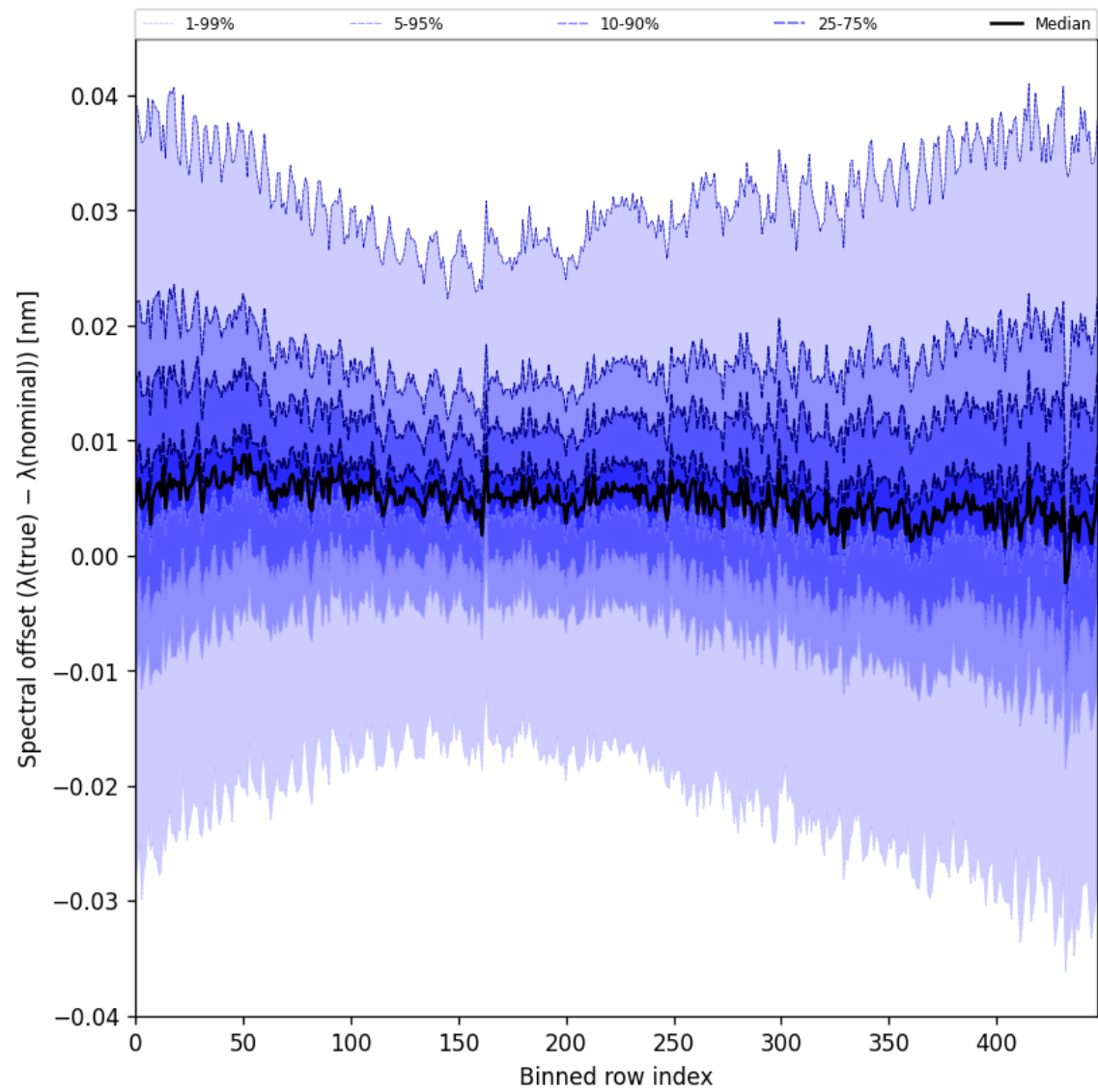
Figure 62: Along track statistics of “Spectral offset ( \lambda_{\text{true}} - \lambda_{\text{nominal}} )” for 2025-11-13 to 2025-11-15
