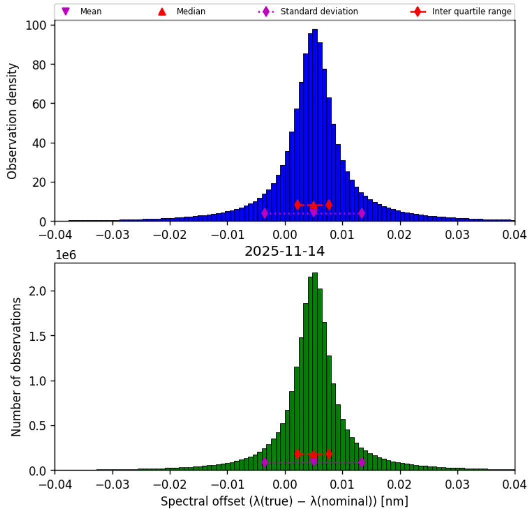
Figure 45: Histogram of “Spectral offset ( \lambda_{\text{true}} - \lambda_{\text{nominal}} )” for 2025-11-13 to 2025-11-15
