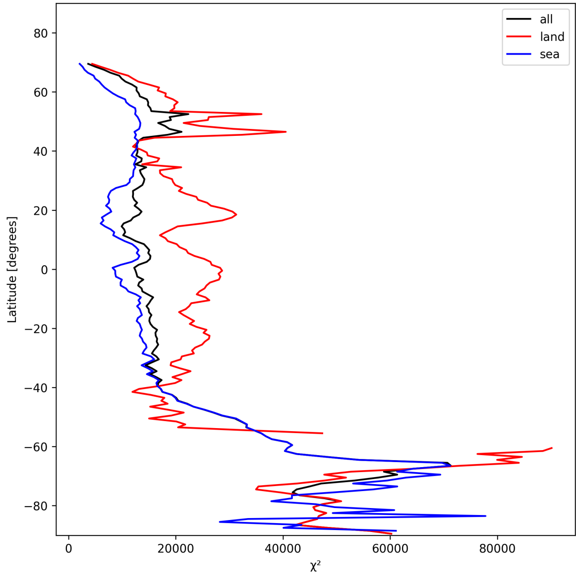
Figure 21: Zonal average of “ \chi^2 ” for 2025-11-13 to 2025-11-15.
