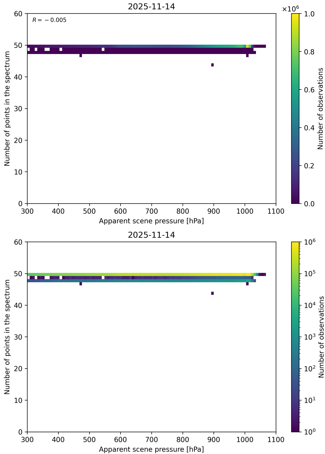
Figure 66: Scatter density plot of “Apparent scene pressure” against “Number of points in the spectrum” for 2025-11-13 to 2025-11-15.
