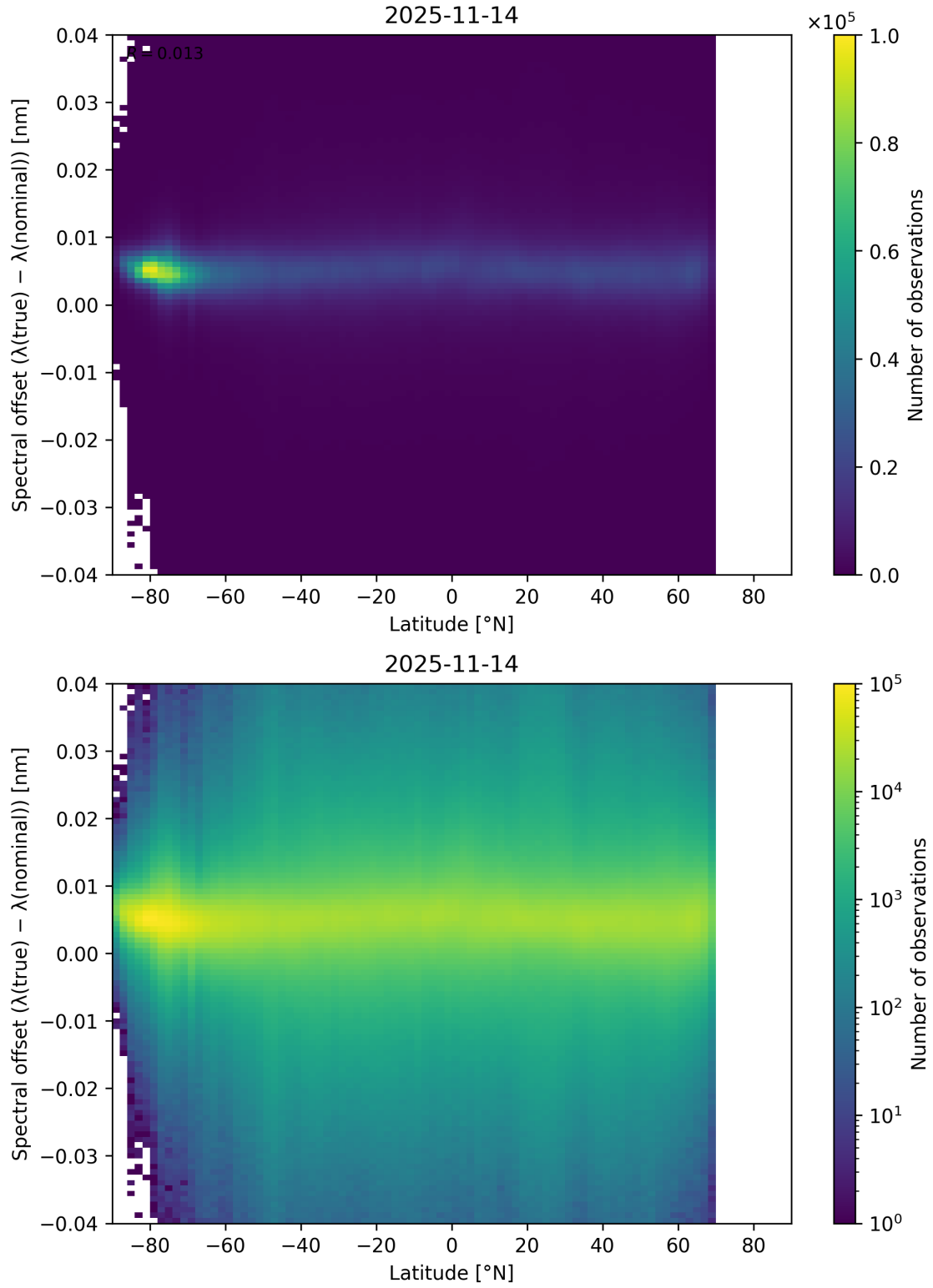
Figure 96: Scatter density plot of “Latitude” against “Spectral offset ( \lambda_{\text{true}} - \lambda_{\text{nominal}} )” for 2025-11-13 to 2025-11-15.
