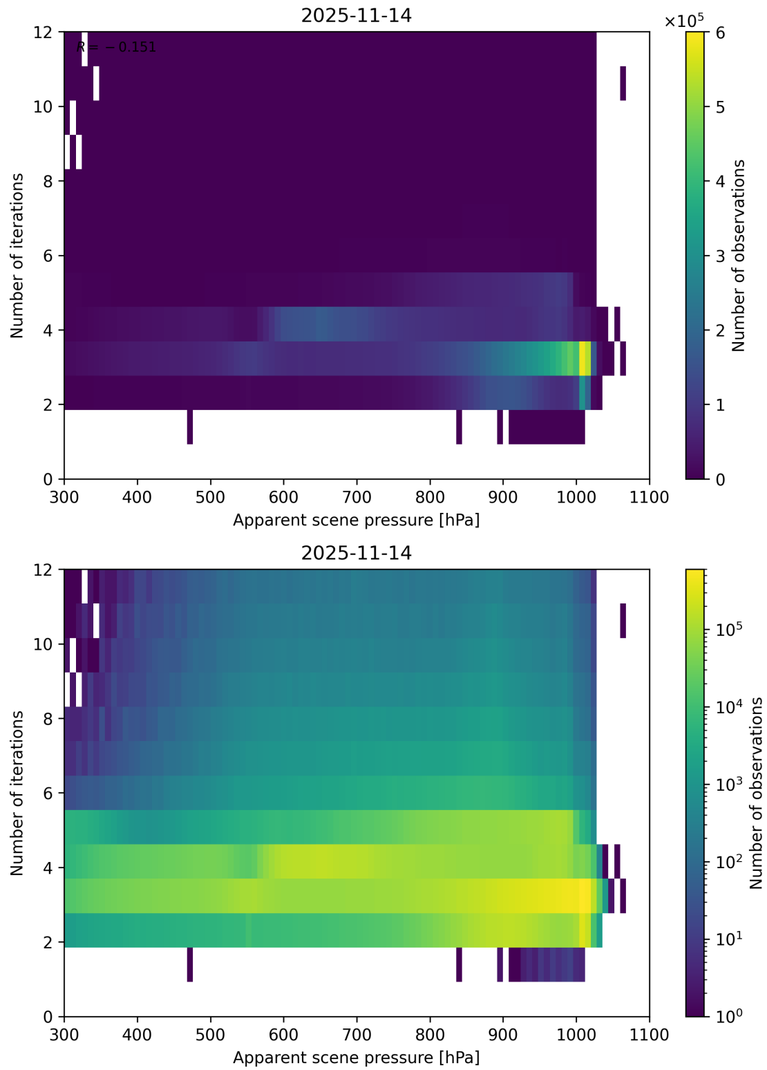
Figure 65: Scatter density plot of “Apparent scene pressure” against “Number of iterations” for 2025-11-13 to 2025-11-15.
