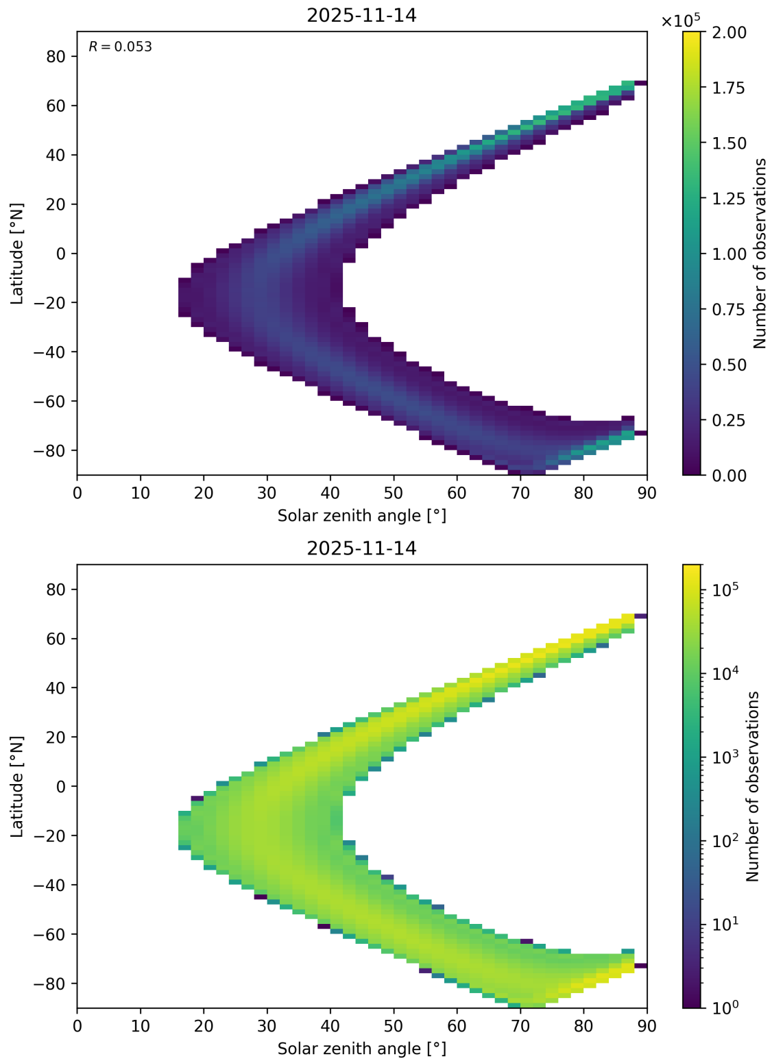
Figure 113: Scatter density plot of “Solar zenith angle” against “Latitude” for 2025-11-13 to 2025-11-15.
