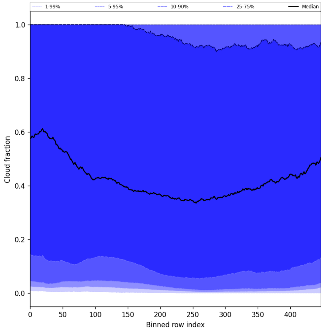
Figure 49: Along track statistics of “Cloud fraction” for 2025-11-13 to 2025-11-15
