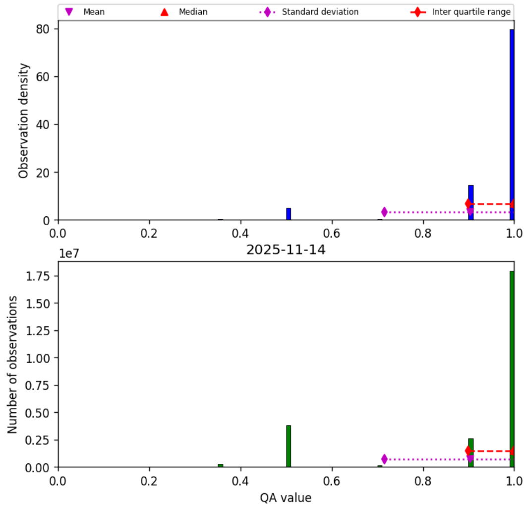
Figure 29: Histogram of “QA value” for 2025-11-13 to 2025-11-15
