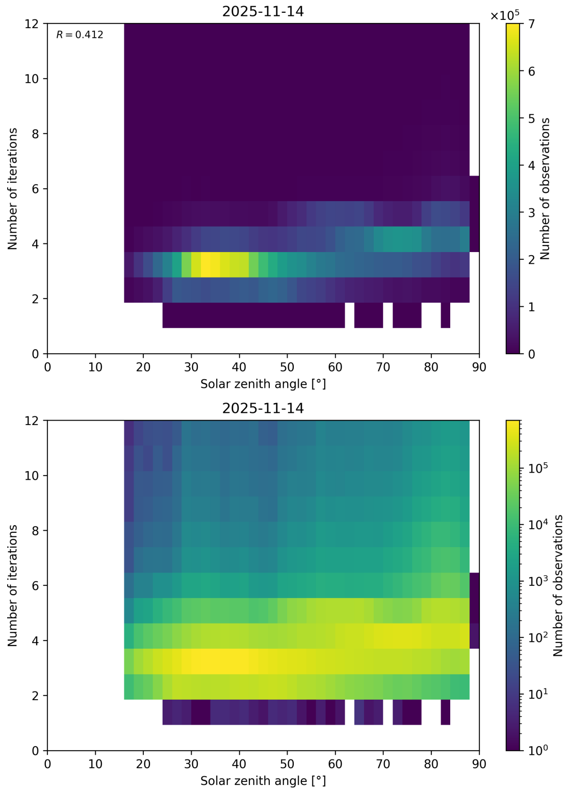
Figure 114: Scatter density plot of “Solar zenith angle” against “Number of iterations” for 2025-11-13 to 2025-11-15.
