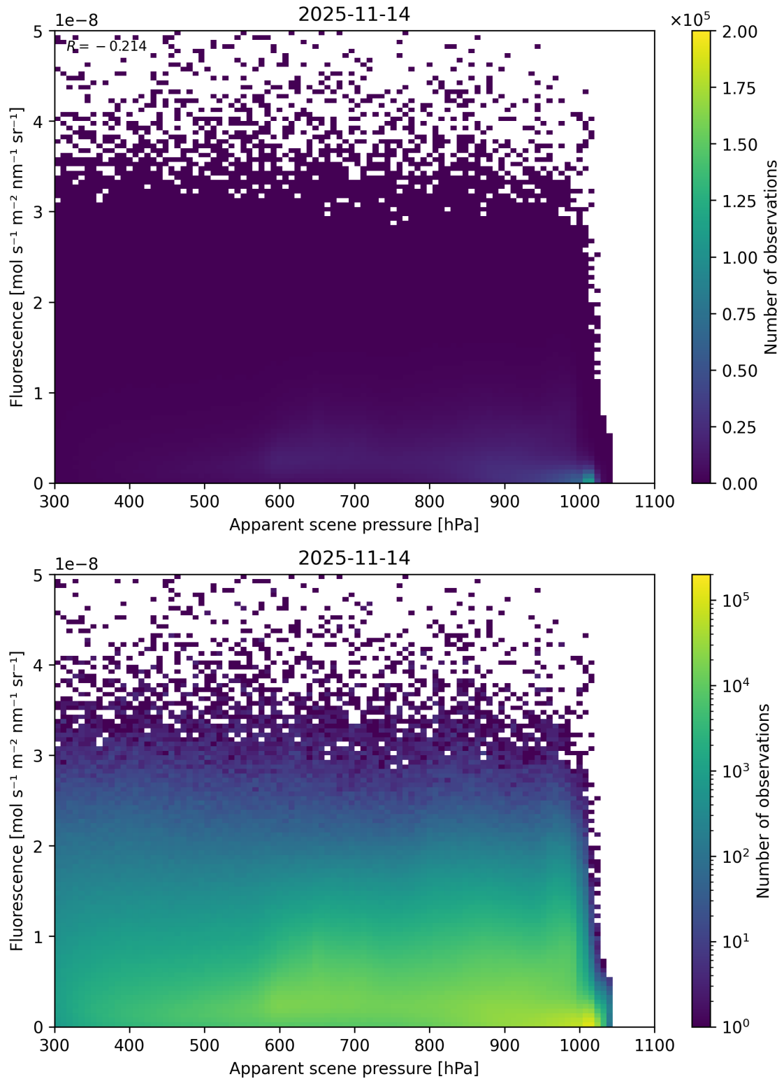
Figure 64: Scatter density plot of “Apparent scene pressure” against “Fluorescence” for 2025-11-13 to 2025-11-15.
