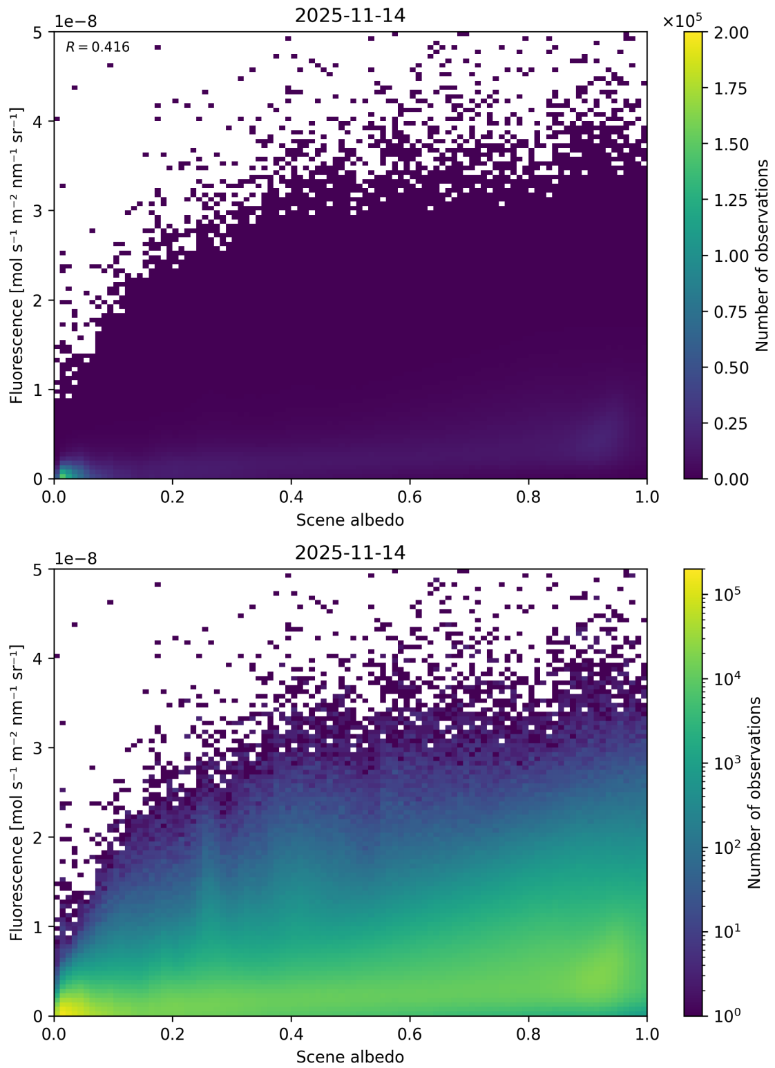
Figure 104: Scatter density plot of “Scene albedo” against “Fluorescence” for 2025-11-13 to 2025-11-15.
