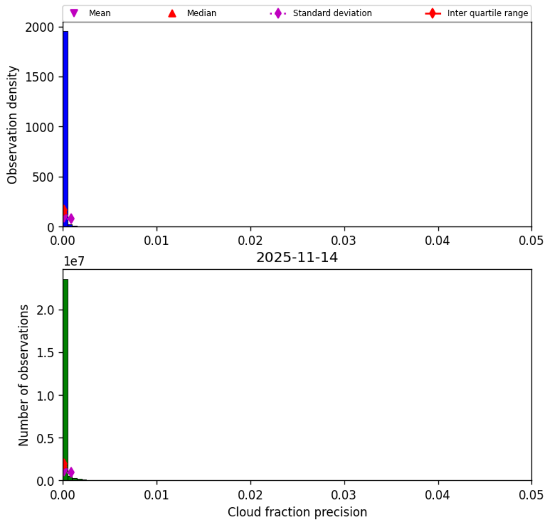
Figure 33: Histogram of “Cloud fraction precision” for 2025-11-13 to 2025-11-15
