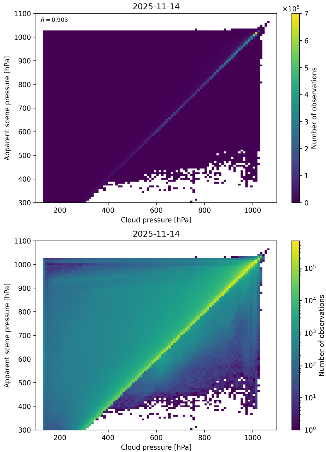
Figure 77: Scatter density plot of “Cloud pressure” against “Apparent scene pressure” for 2025-11-13 to 2025-11-15.
