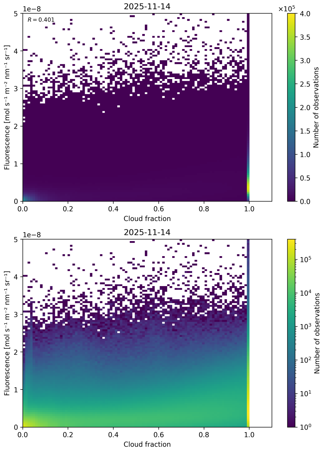
Figure 72: Scatter density plot of “Cloud fraction” against “Fluorescence” for 2025-11-13 to 2025-11-15.
