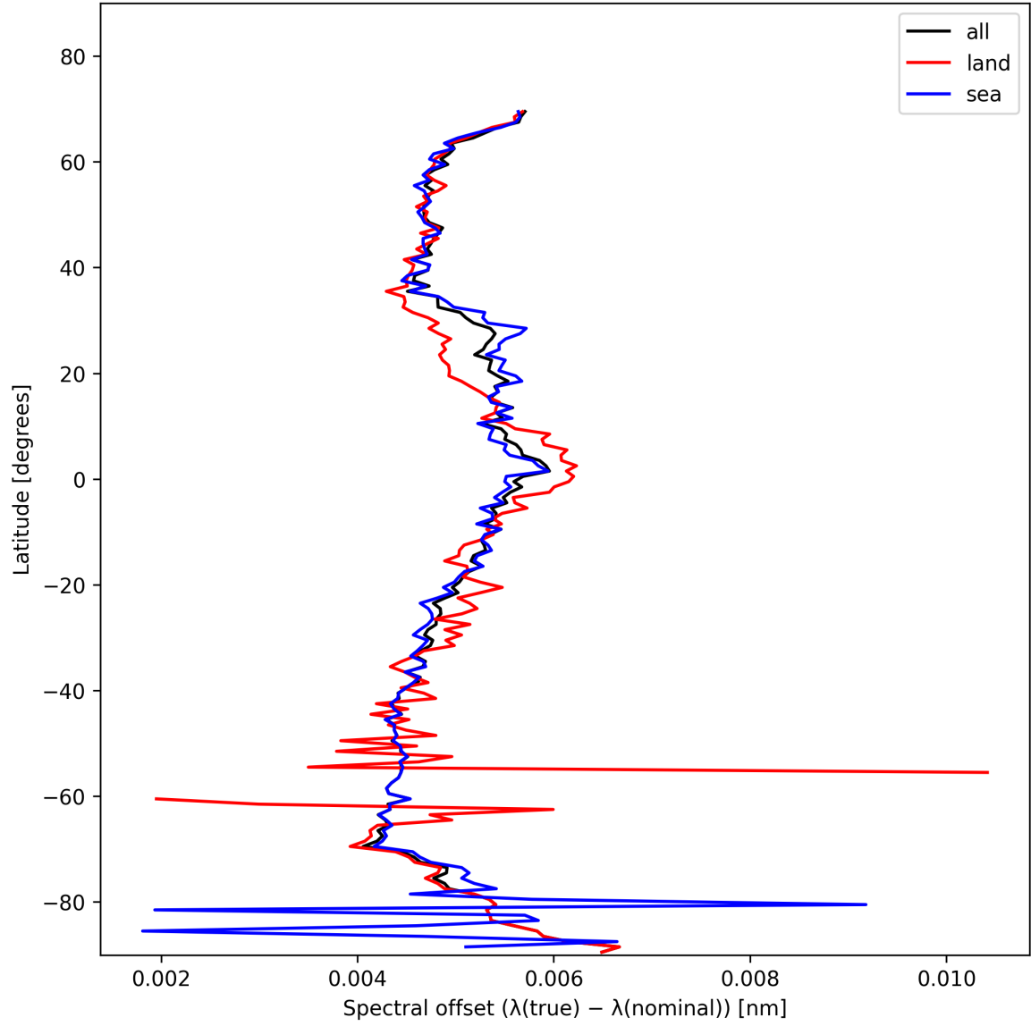
Figure 28: Zonal average of “Spectral offset ( \lambda_{\text{true}} - \lambda_{\text{nominal}} )” for 2025-11-13 to 2025-11-15.
