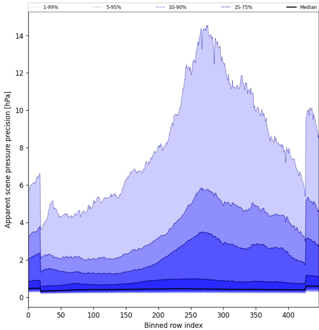
Figure 54: Along track statistics of “Apparent scene pressure precision” for 2025-11-13 to 2025-11-15
