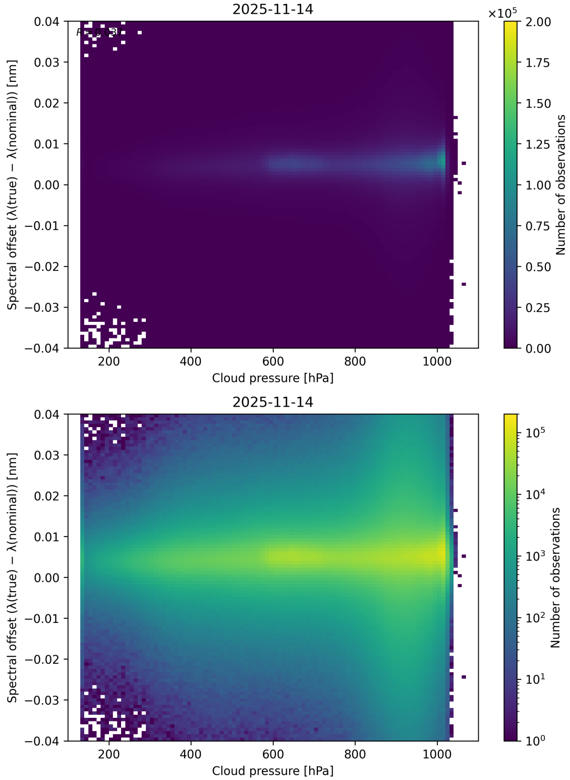
Figure 84: Scatter density plot of “Cloud pressure” against “Spectral offset ( \lambda_{\text{true}} - \lambda_{\text{nominal}} )” for 2025-11-13 to 2025-11-15.
