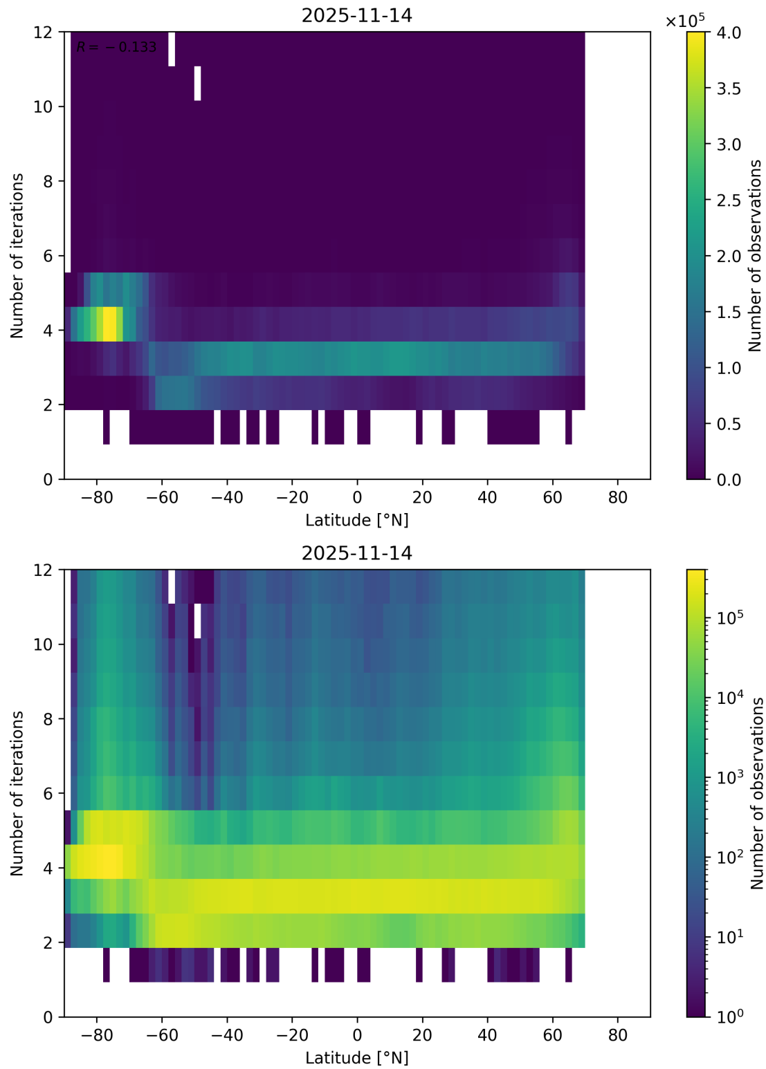
Figure 93: Scatter density plot of “Latitude” against “Number of iterations” for 2025-11-13 to 2025-11-15.
