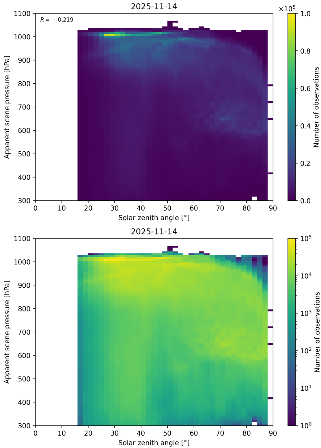
Figure 108: Scatter density plot of “Solar zenith angle” against “Apparent scene pressure” for 2025-11-13 to 2025-11-15.
