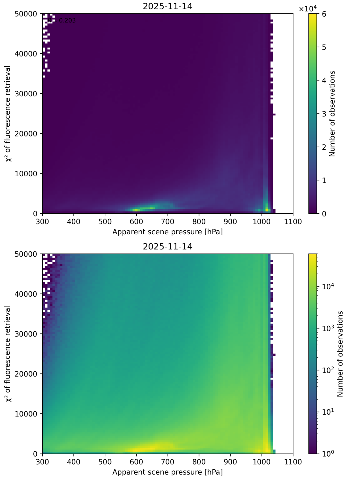
Figure 63: Scatter density plot of “Apparent scene pressure” against “ \chi^2 of fluorescence retrieval” for 2025-11-13 to 2025-11-15.
