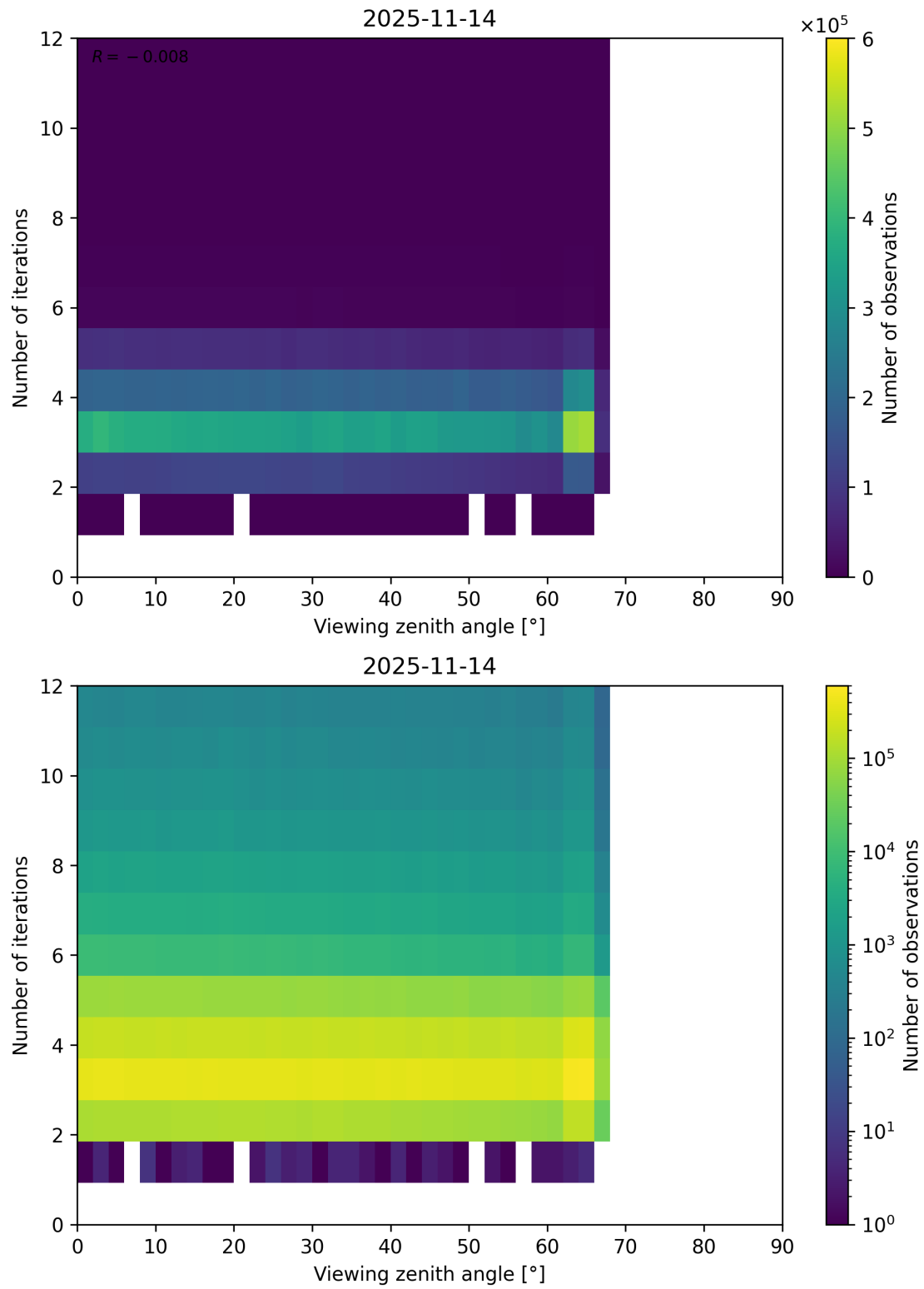
Figure 124: Scatter density plot of “Viewing zenith angle” against “Number of iterations” for 2025-11-13 to 2025-11-15.
