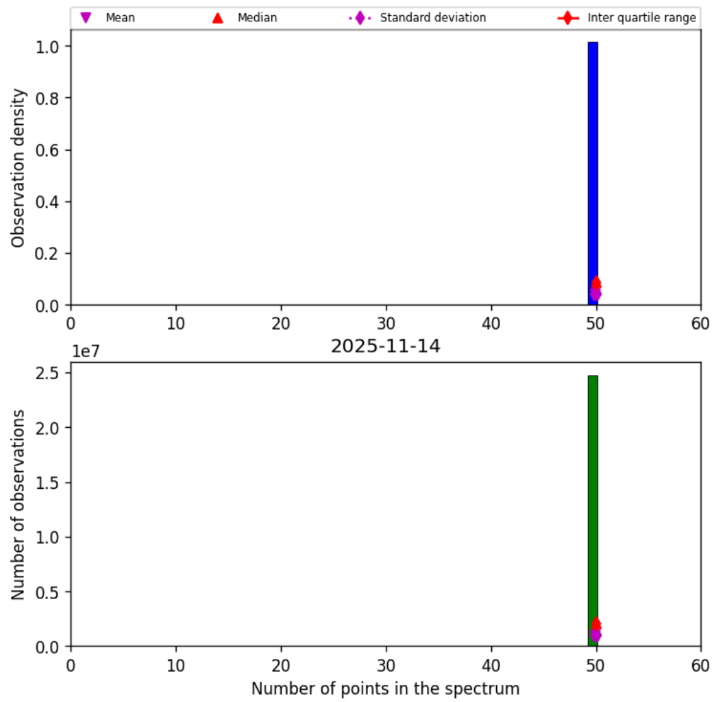
Figure 44: Histogram of “Number of points in the spectrum” for 2025-11-13 to 2025-11-15
