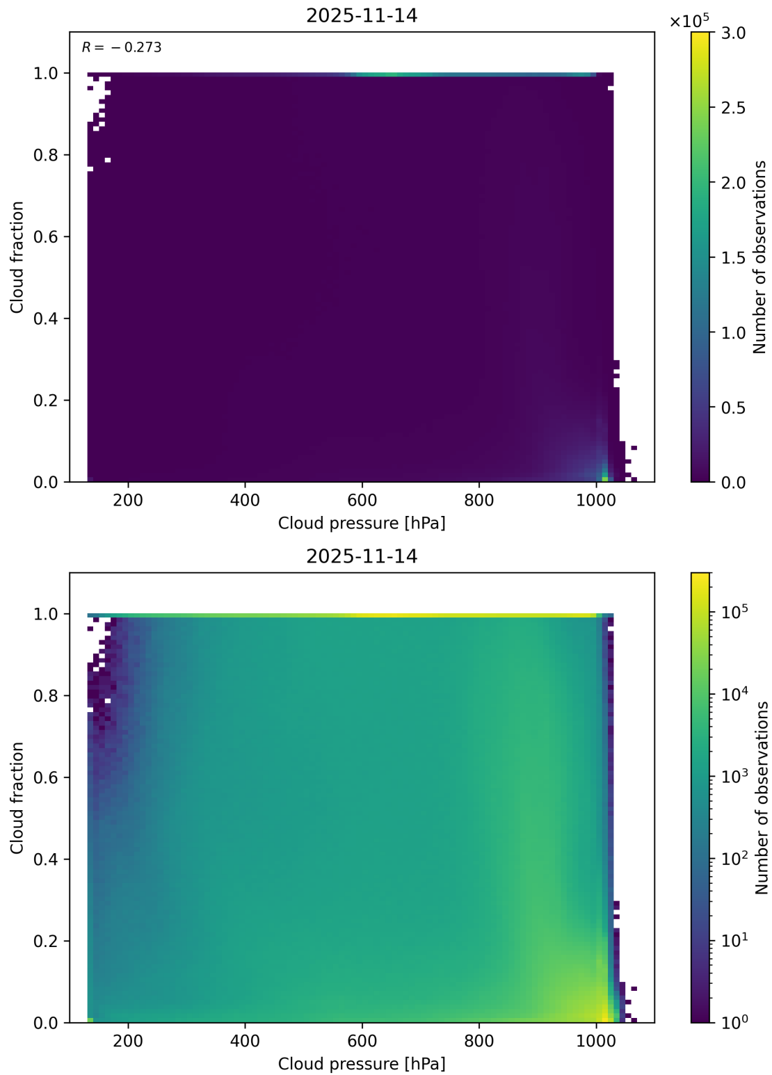
Figure 79: Scatter density plot of “Cloud pressure” against “Cloud fraction” for 2025-11-13 to 2025-11-15.
