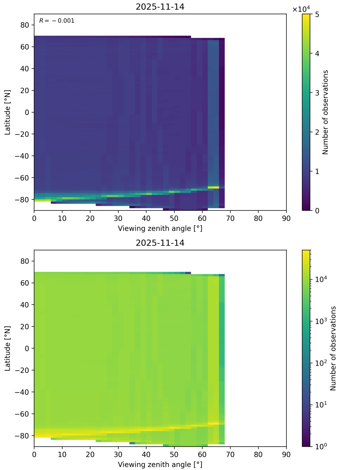
Figure 123: Scatter density plot of “Viewing zenith angle” against “Latitude” for 2025-11-13 to 2025-11-15.
