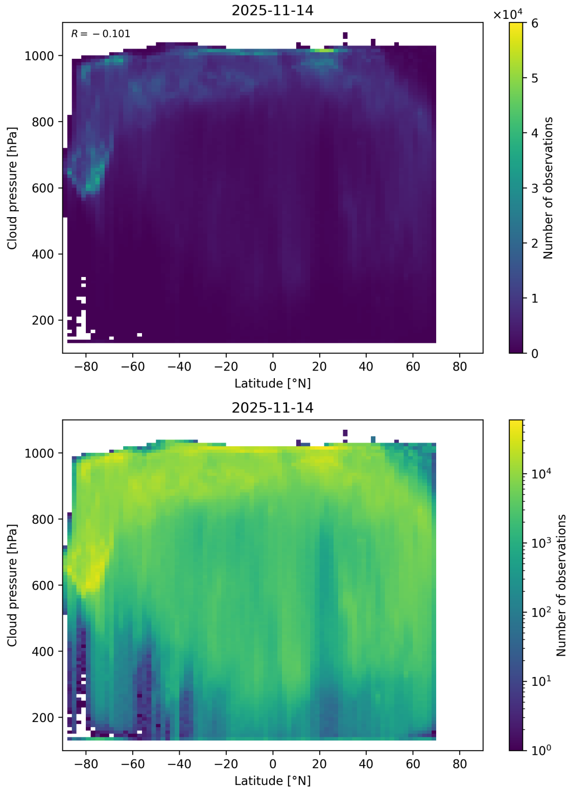
Figure 91: Scatter density plot of “Latitude” against “Cloud pressure” for 2025-11-13 to 2025-11-15.
