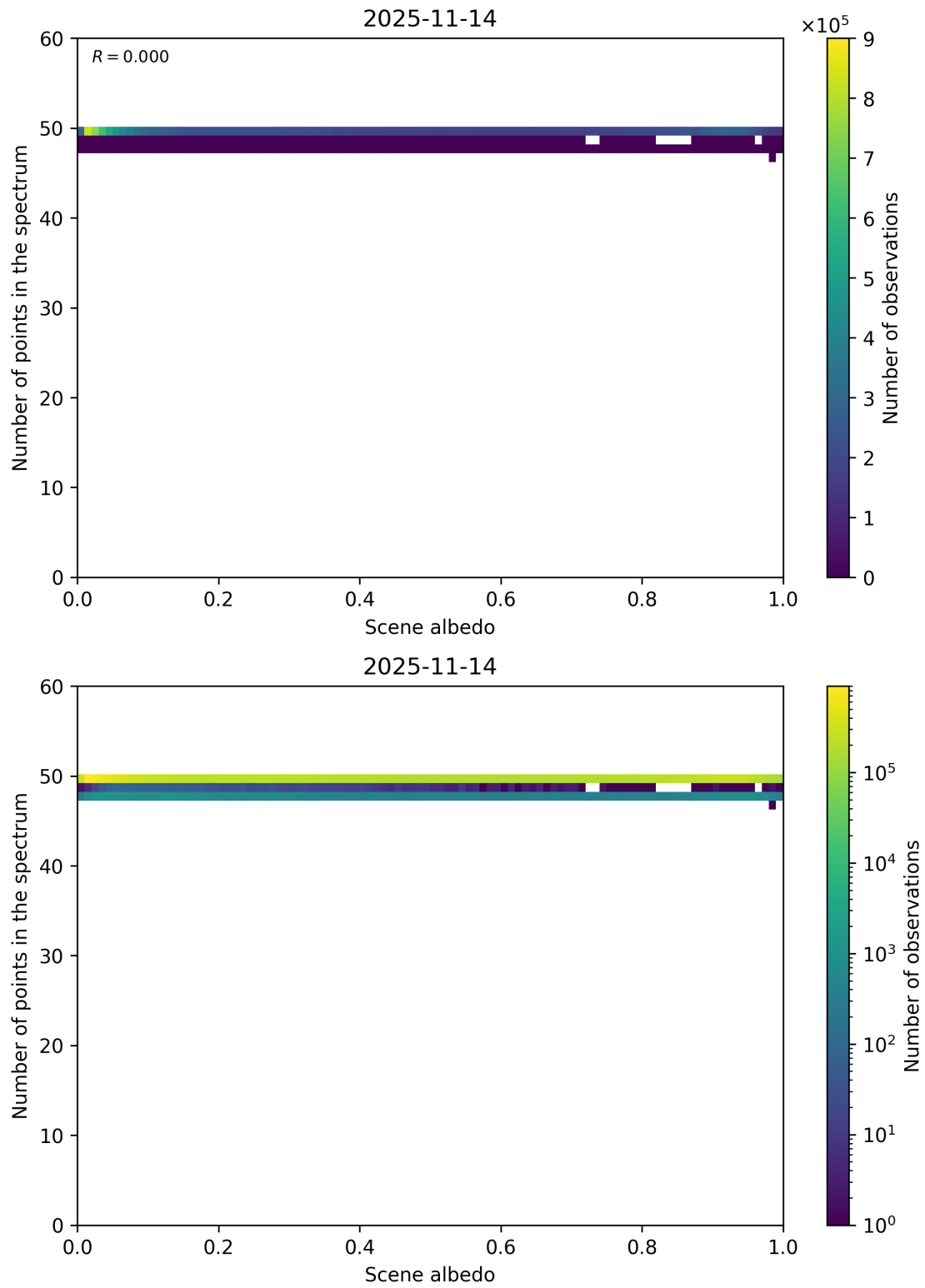
Figure 106: Scatter density plot of “Scene albedo” against “Number of points in the spectrum” for 2025-11-13 to 2025-11-15.
