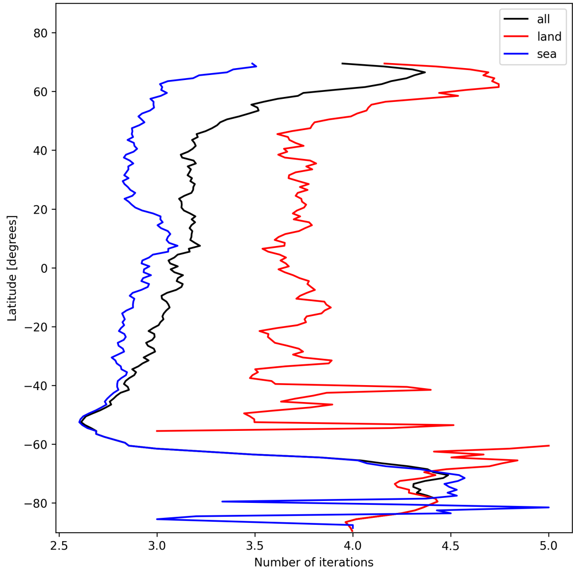
Figure 22: Zonal average of “Number of iterations” for 2025-11-13 to 2025-11-15.
