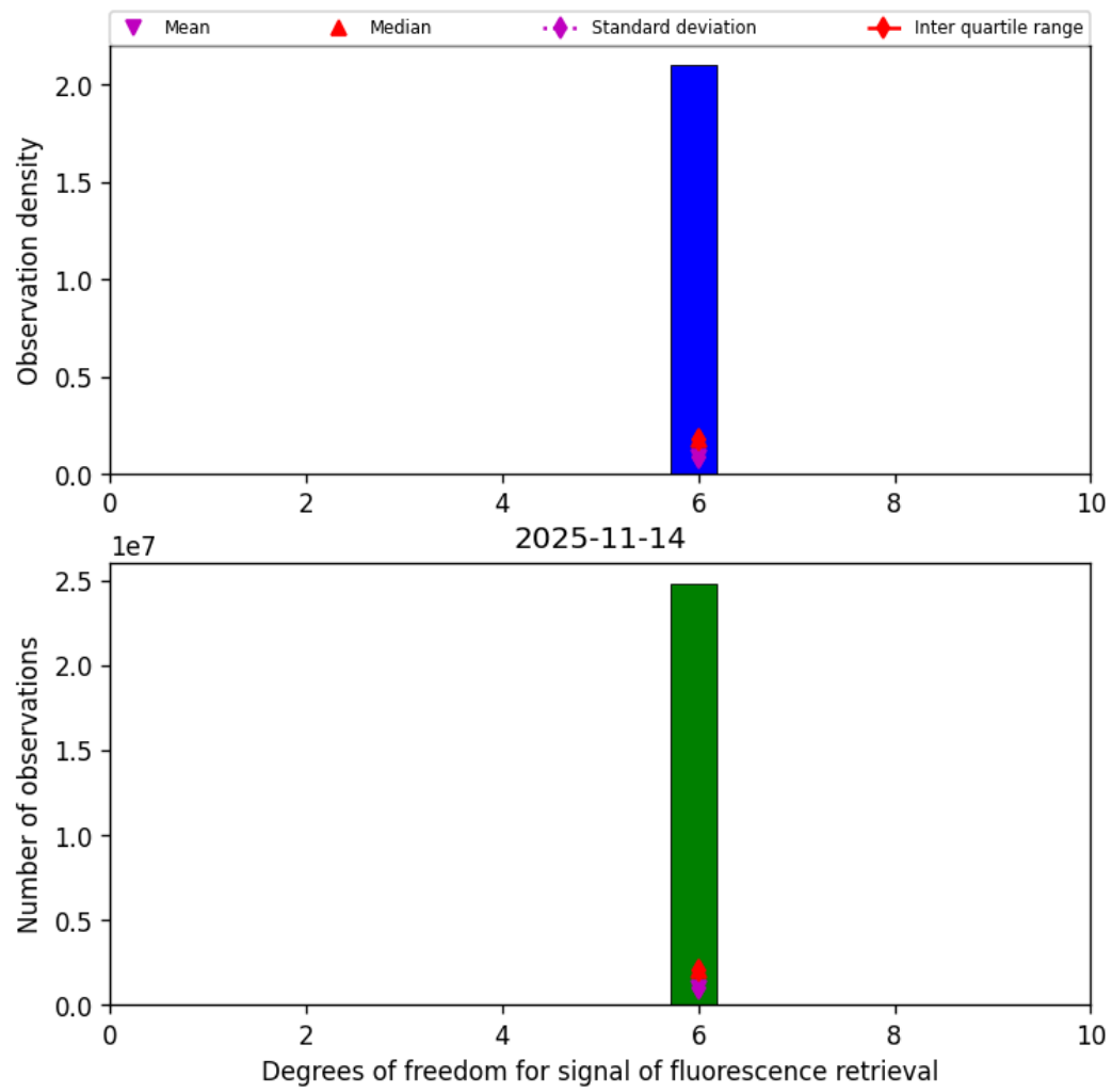
Figure 43: Histogram of “Degrees of freedom for signal of fluorescence retrieval” for 2025-11-13 to 2025-11-15
