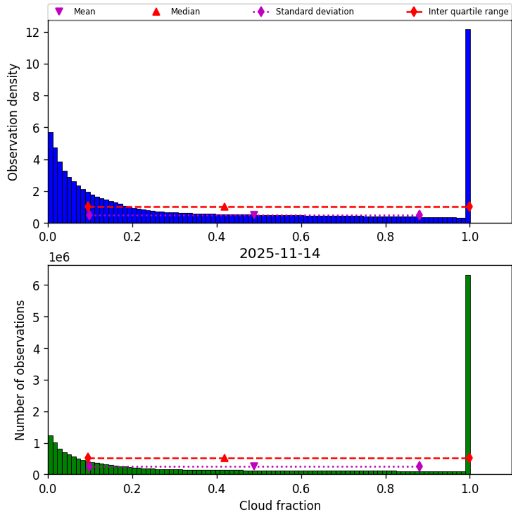
Figure 32: Histogram of “Cloud fraction” for 2025-11-13 to 2025-11-15
