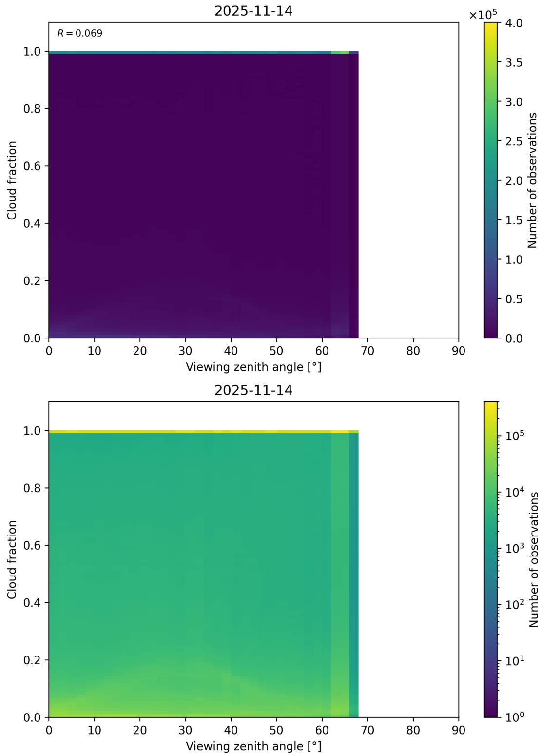
Figure 120: Scatter density plot of “Viewing zenith angle” against “Cloud fraction” for 2025-11-13 to 2025-11-15.
