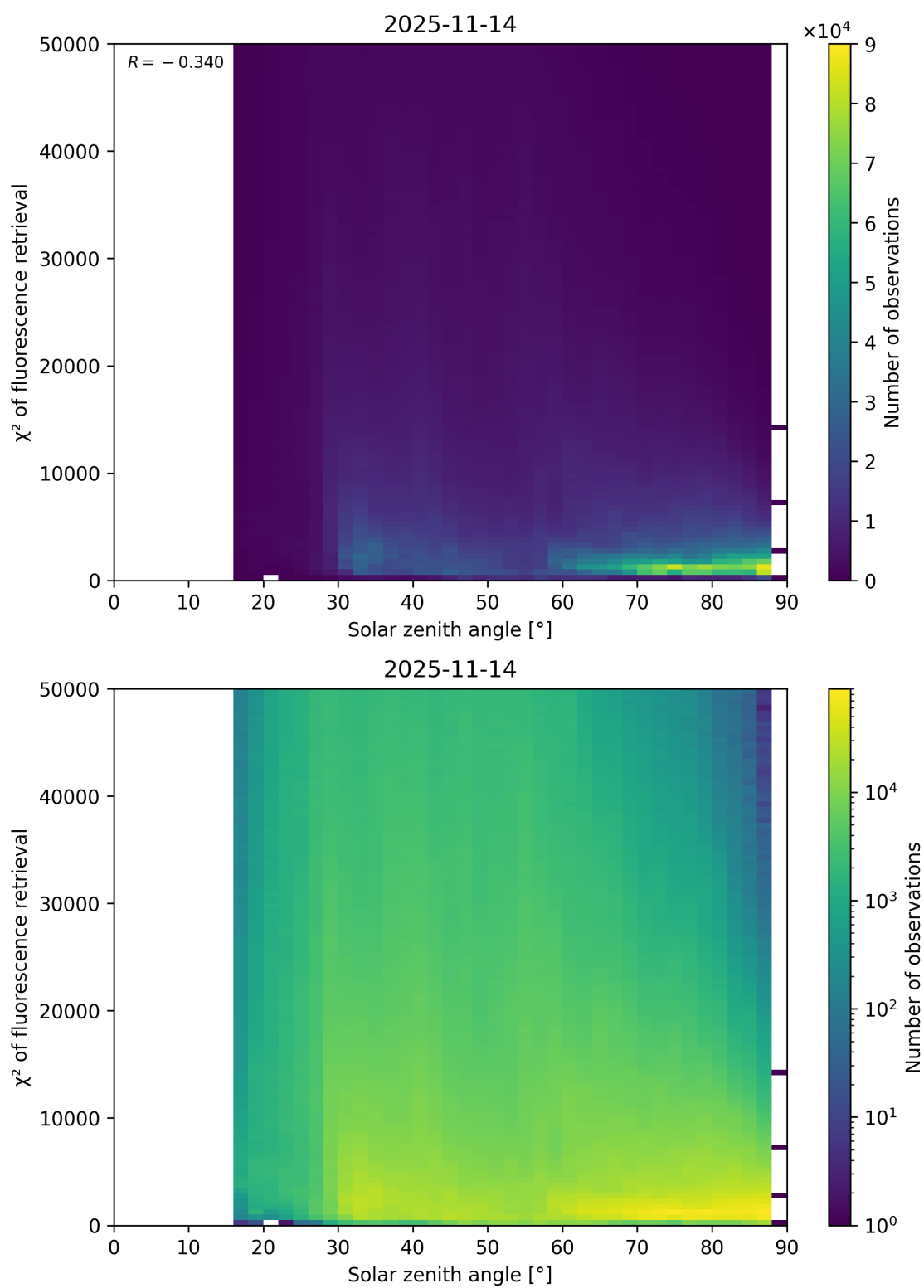
Figure 109: Scatter density plot of “Solar zenith angle” against “ \chi^2 of fluorescence retrieval” for 2025-11-13 to 2025-11-15.
