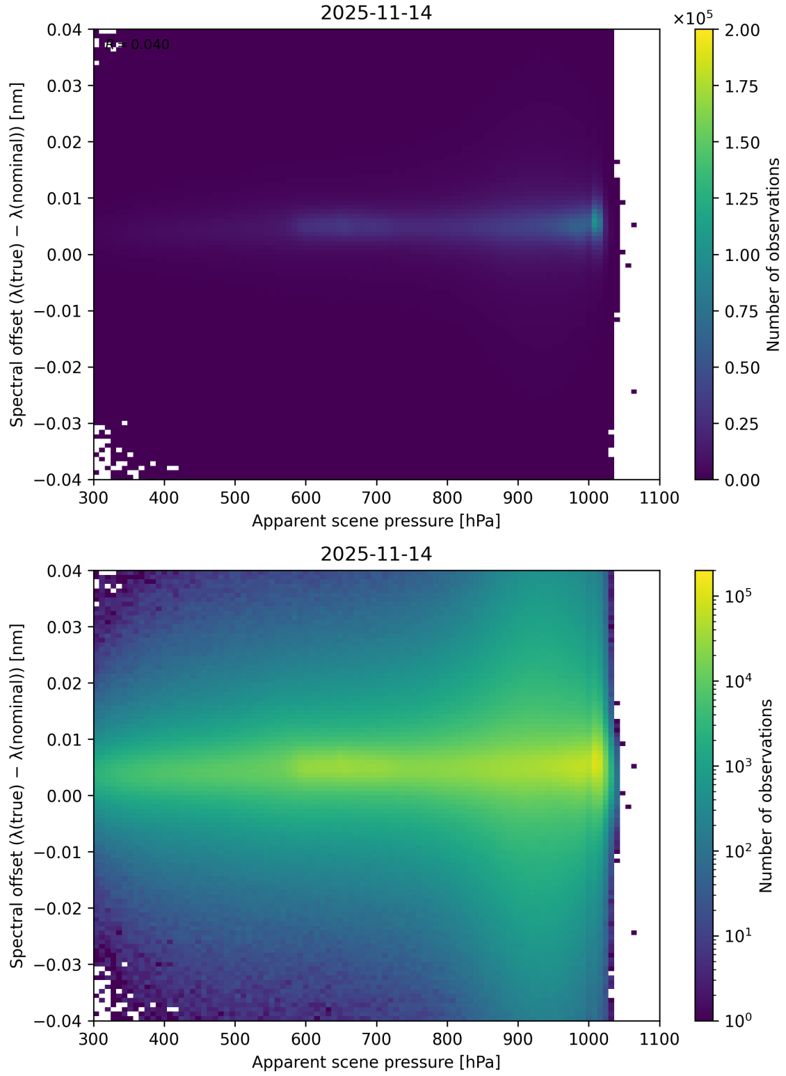
Figure 67: Scatter density plot of “Apparent scene pressure” against “Spectral offset ( \lambda_{\text{true}} - \lambda_{\text{nominal}} )” for 2025-11-13 to 2025-11-15.
