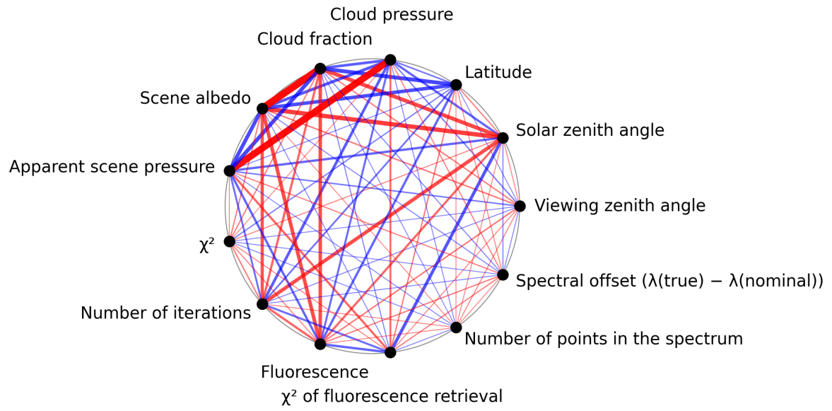
Figure 1: Map of correlation graph for 2025-11-13 to 2025-11-15.
