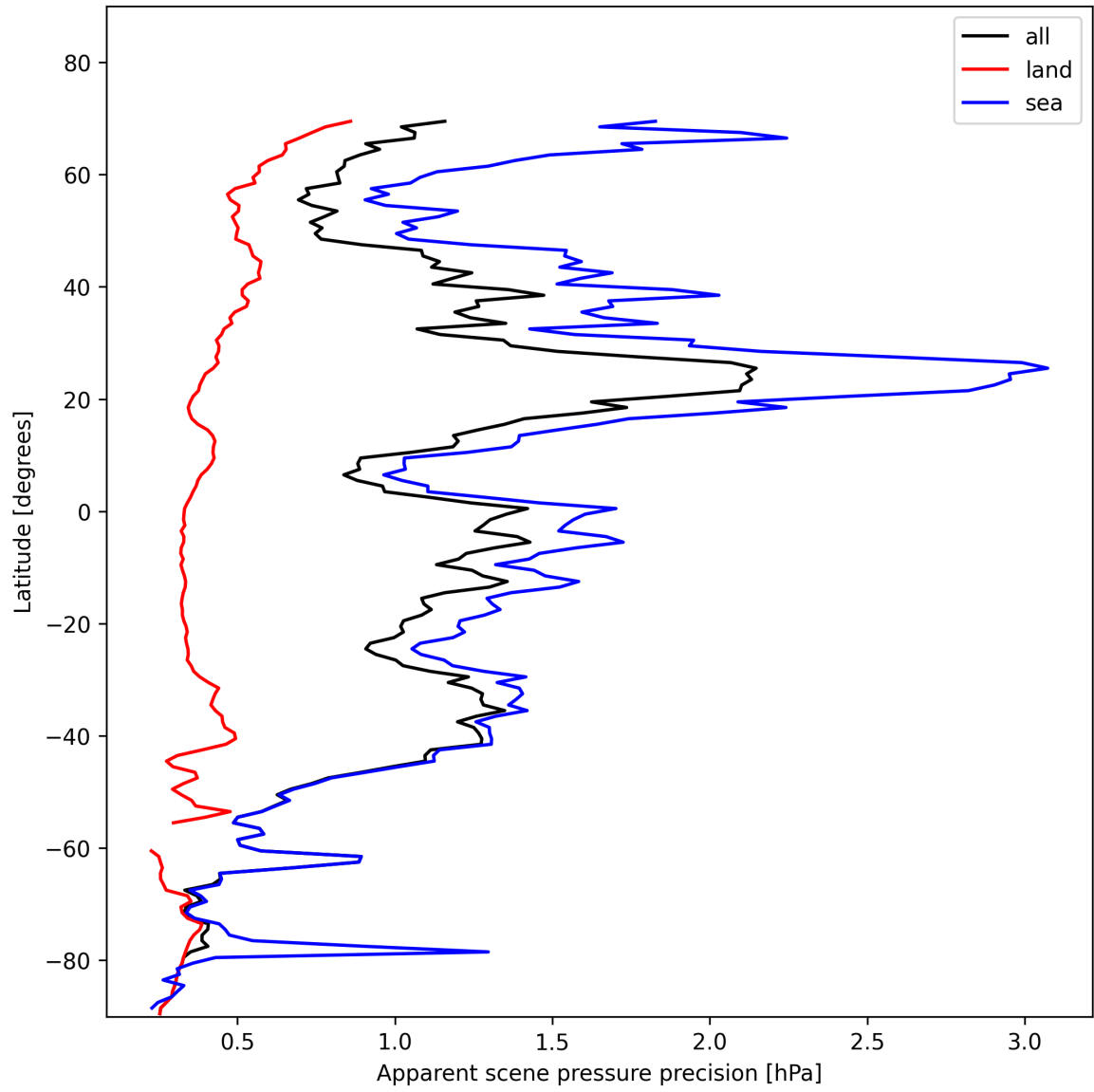
Figure 20: Zonal average of “Apparent scene pressure precision” for 2025-11-13 to 2025-11-15.
