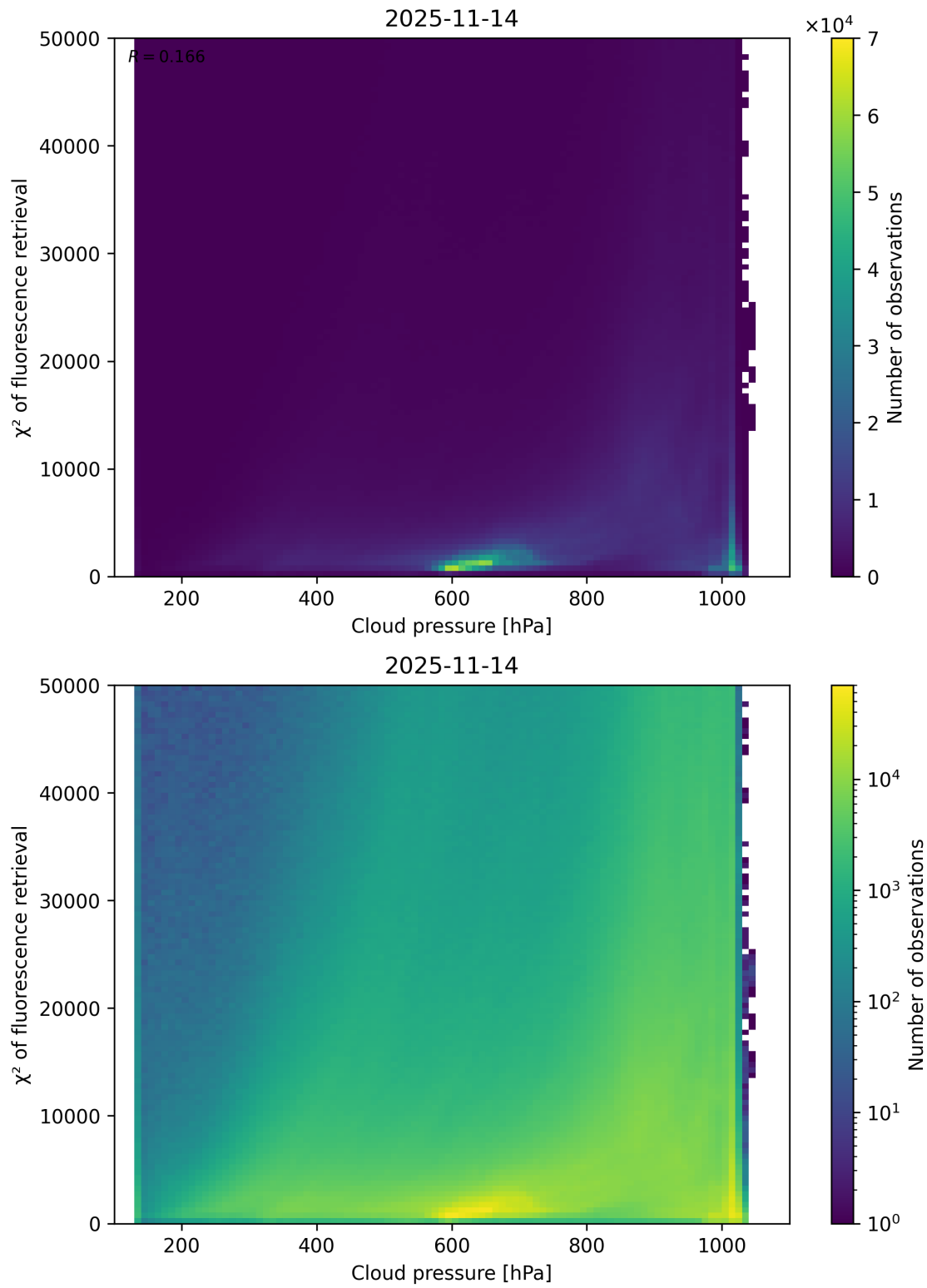
Figure 78: Scatter density plot of “Cloud pressure” against “ \chi^2 of fluorescence retrieval” for 2025-11-13 to 2025-11-15.
