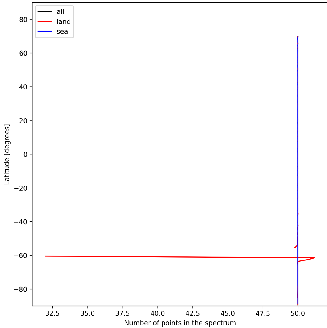
Figure 27: Zonal average of “Number of points in the spectrum” for 2025-11-13 to 2025-11-15.
