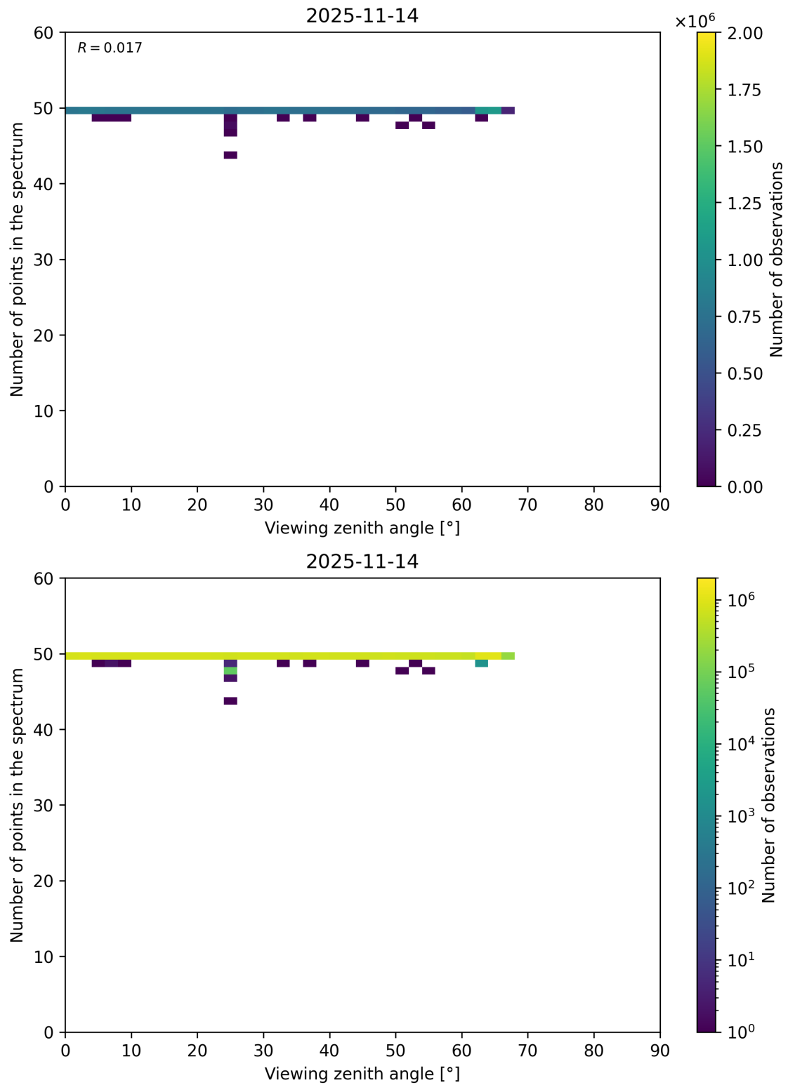
Figure 125: Scatter density plot of “Viewing zenith angle” against “Number of points in the spectrum” for 2025-11-13 to 2025-11-15.
