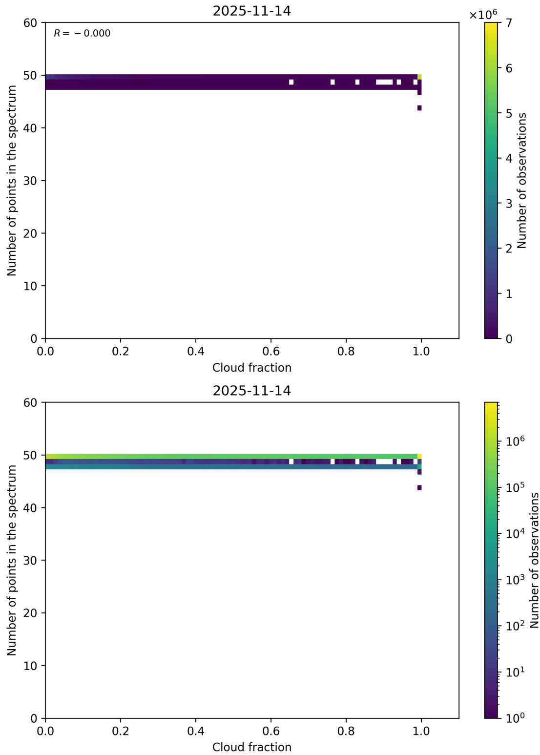
Figure 74: Scatter density plot of “Cloud fraction” against “Number of points in the spectrum” for 2025-11-13 to 2025-11-15.
