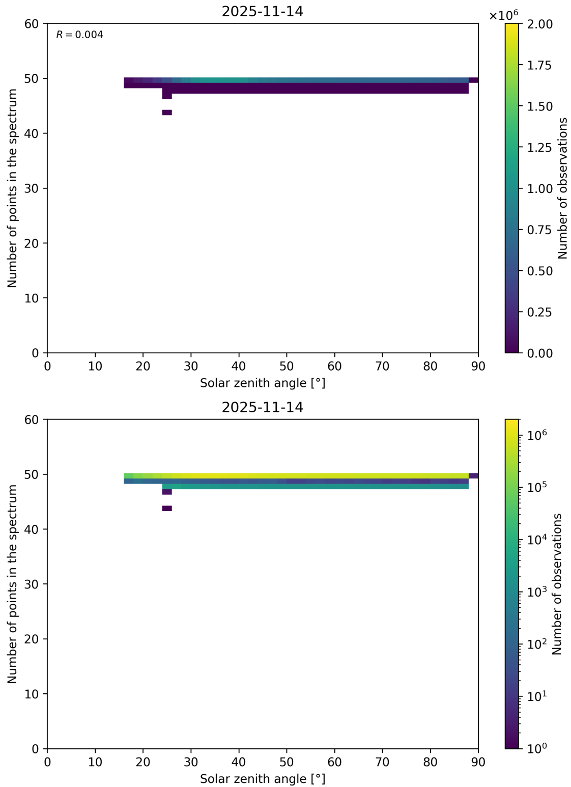
Figure 115: Scatter density plot of “Solar zenith angle” against “Number of points in the spectrum” for 2025-11-13 to 2025-11-15.
