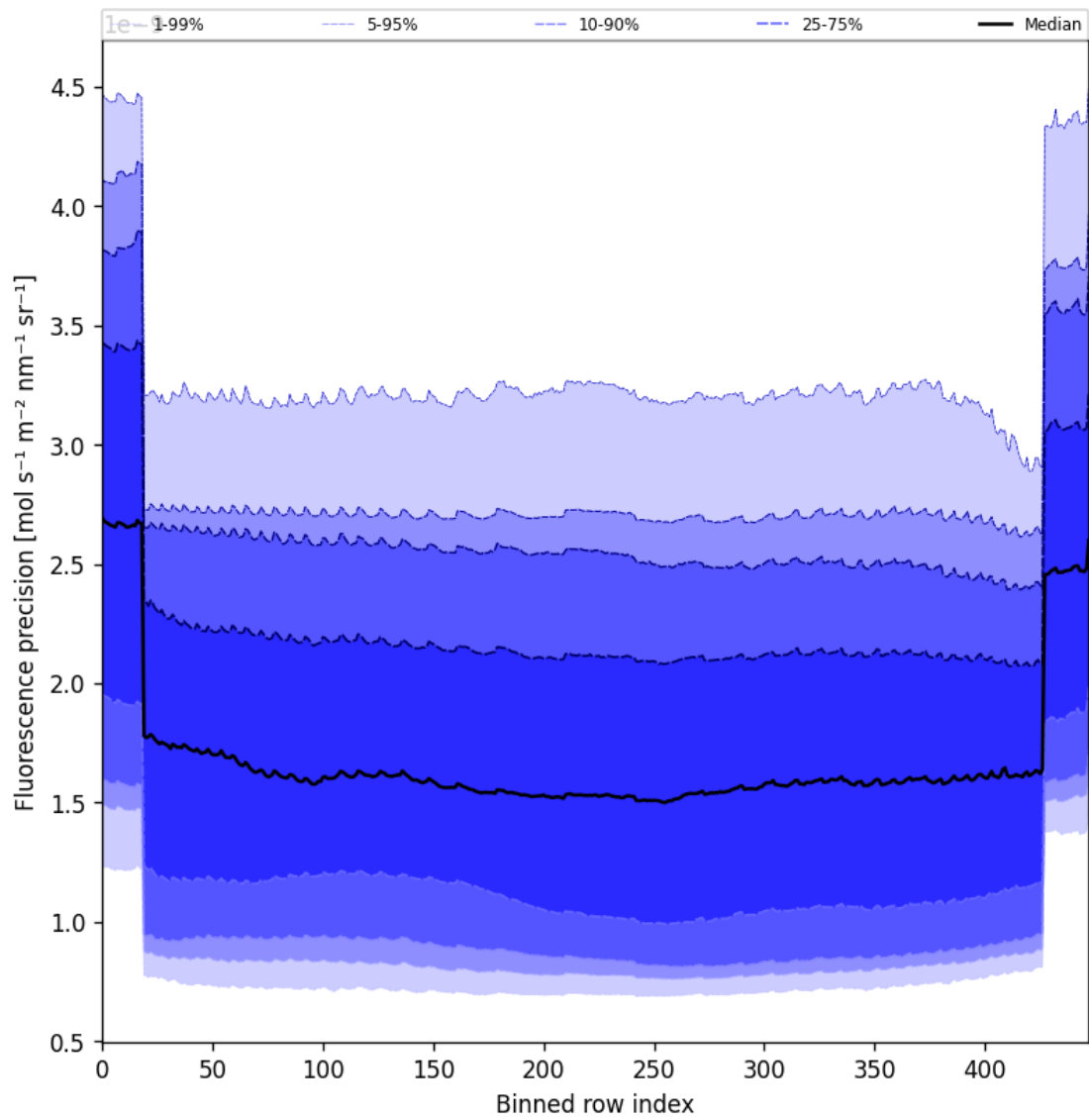
Figure 58: Along track statistics of “Fluorescence precision” for 2025-11-13 to 2025-11-15
