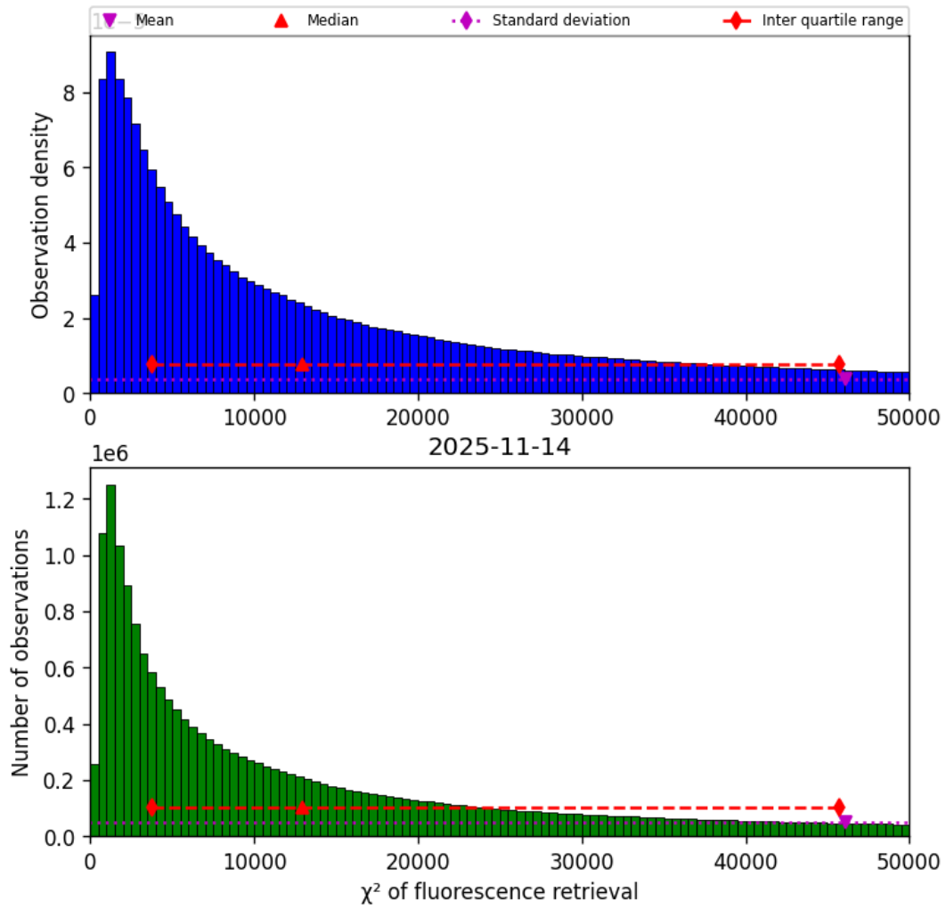
Figure 42: Histogram of “ \chi^2 of fluorescence retrieval” for 2025-11-13 to 2025-11-15
