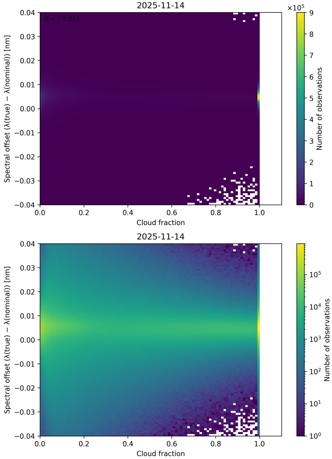
Figure 76: Scatter density plot of “Cloud fraction” against “Spectral offset ( \lambda_{\text{true}} - \lambda_{\text{nominal}} )” for 2025-11-13 to 2025-11-15.
