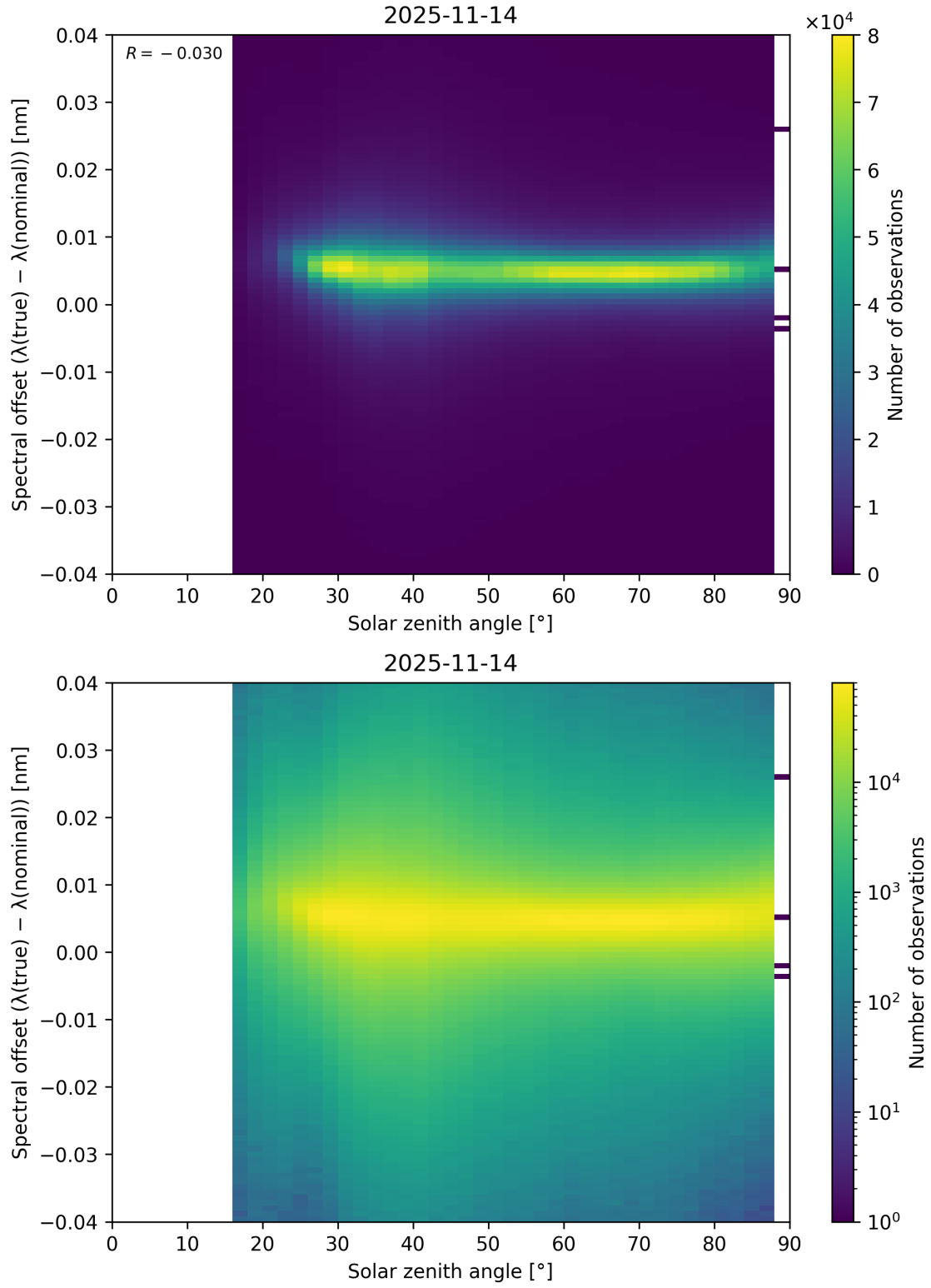
Figure 117: Scatter density plot of “Solar zenith angle” against “Spectral offset ( \lambda_{\text{true}} - \lambda_{\text{nominal}} )” for 2025-11-13 to 2025-11-15.
