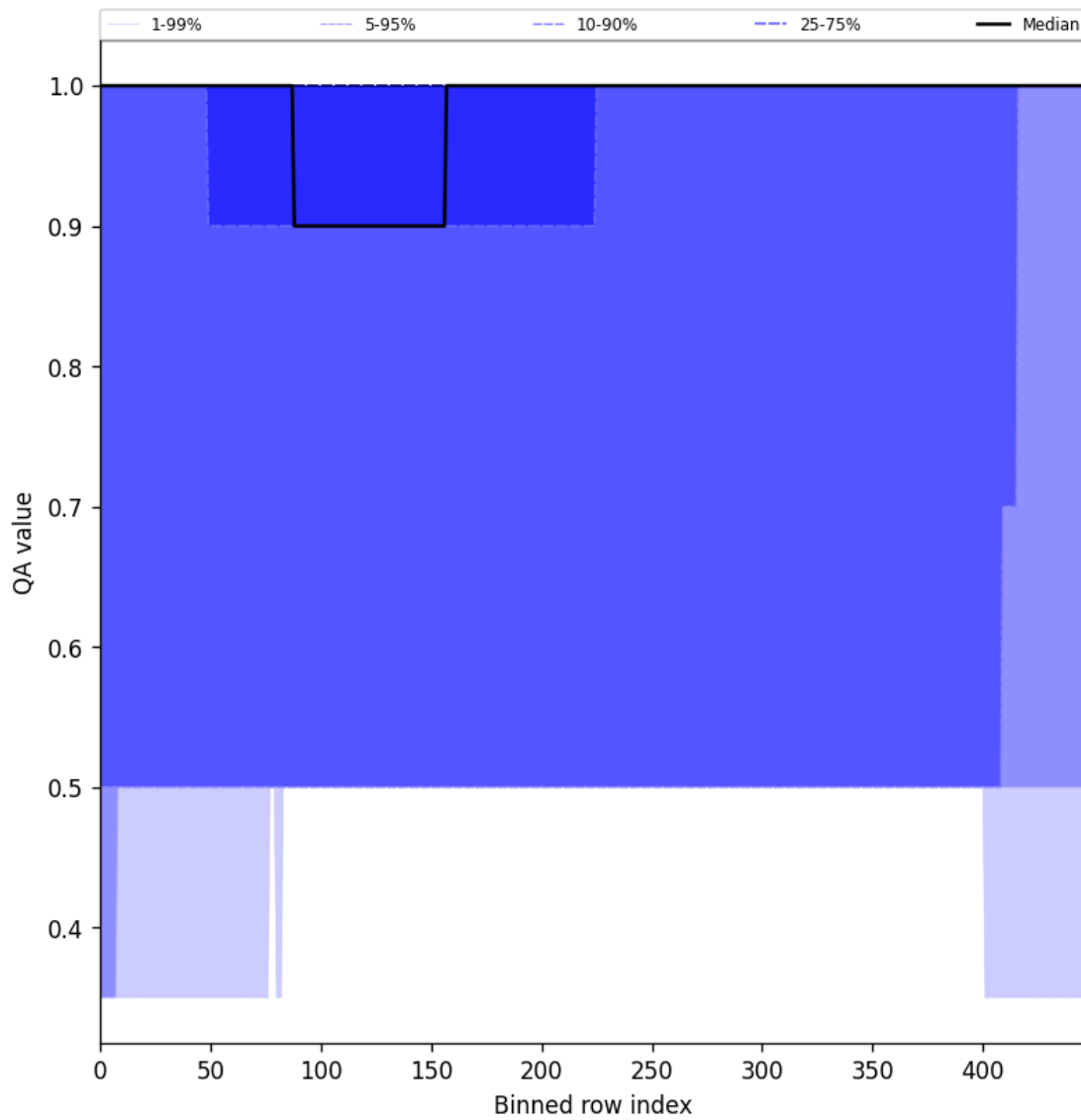
Figure 46: Along track statistics of “QA value” for 2025-11-13 to 2025-11-15
