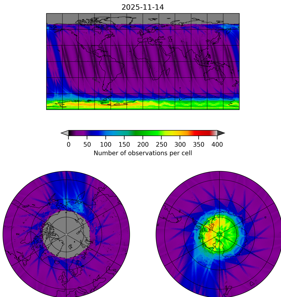
Figure 11: Map of the number of observations for 2025-11-13 to 2025-11-15
