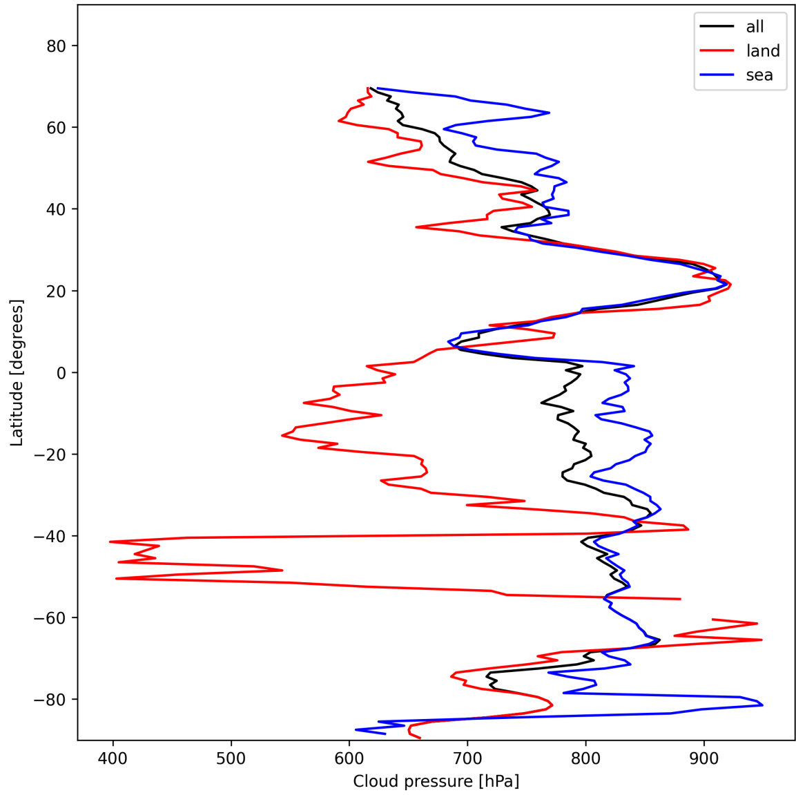
Figure 13: Zonal average of “Cloud pressure” for 2025-11-13 to 2025-11-15.
