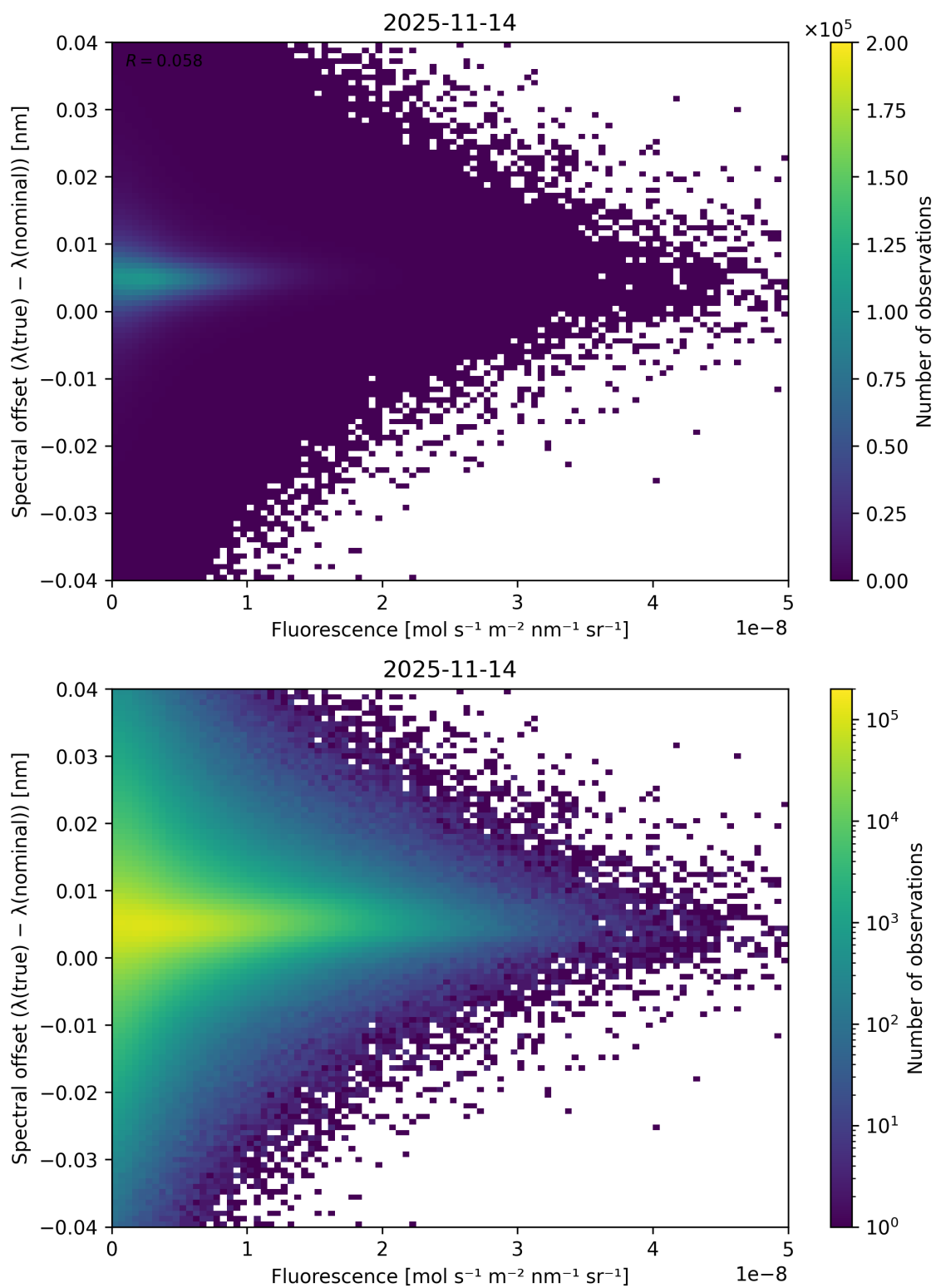
Figure 87: Scatter density plot of “Fluorescence” against “Spectral offset ( \lambda_{\text{true}} - \lambda_{\text{nominal}} )” for 2025-11-13 to 2025-11-15.
