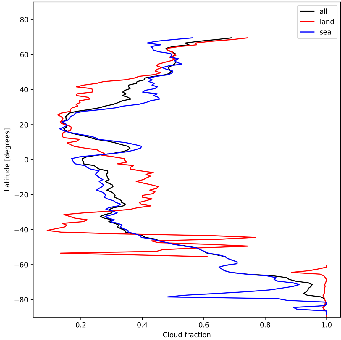
Figure 15: Zonal average of “Cloud fraction” for 2025-11-13 to 2025-11-15.
