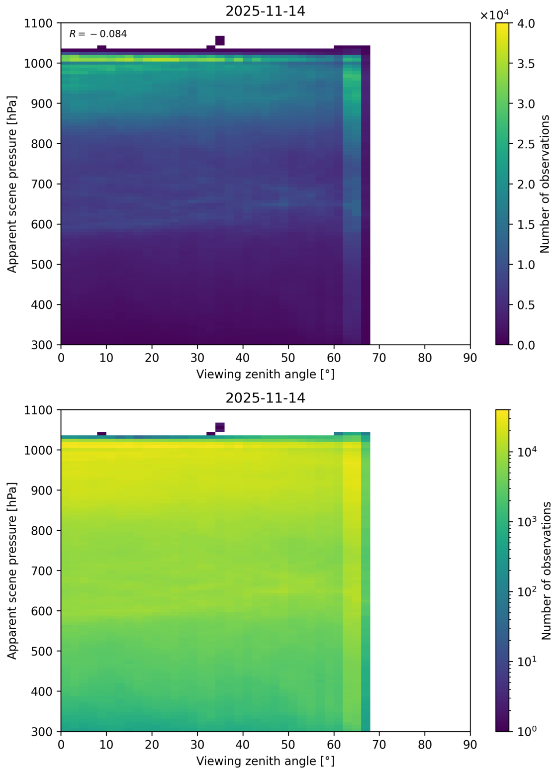
Figure 118: Scatter density plot of “Viewing zenith angle” against “Apparent scene pressure” for 2025-11-13 to 2025-11-15.
