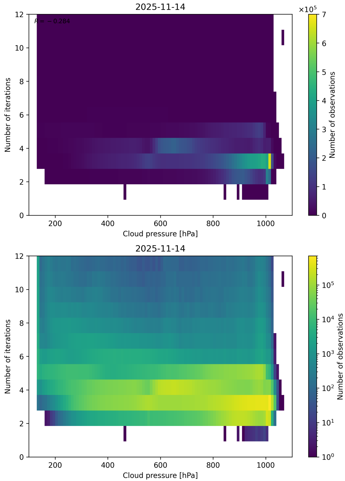
Figure 81: Scatter density plot of “Cloud pressure” against “Number of iterations” for 2025-11-13 to 2025-11-15.
