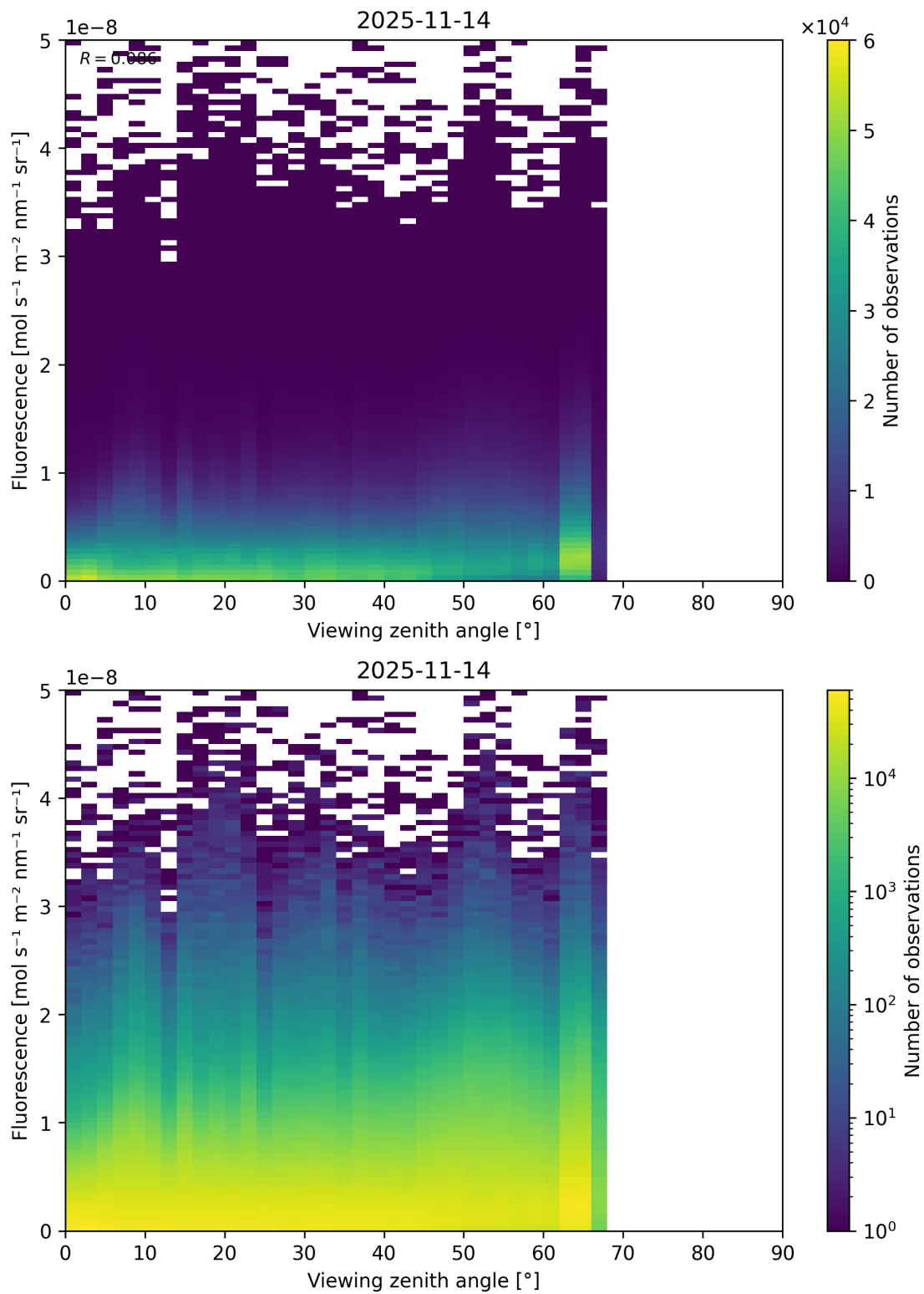
Figure 122: Scatter density plot of “Viewing zenith angle” against “Fluorescence” for 2025-11-13 to 2025-11-15.
