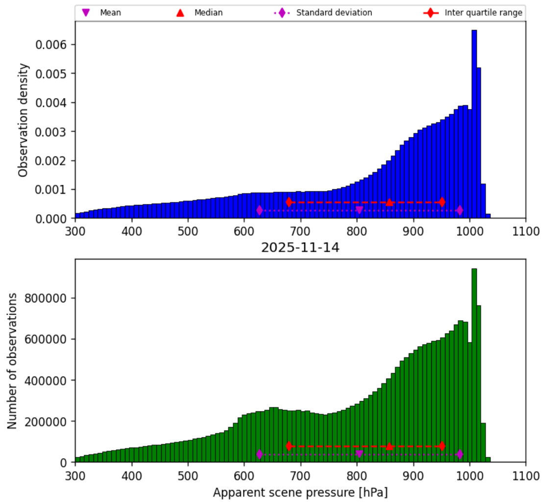
Figure 36: Histogram of “Apparent scene pressure” for 2025-11-13 to 2025-11-15
