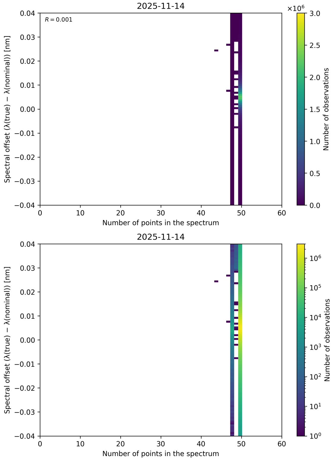
Figure 101: Scatter density plot of “Number of points in the spectrum” against “Spectral offset ( \lambda_{\text{true}} - \lambda_{\text{nominal}} )” for 2025-11-13 to 2025-11-15.
