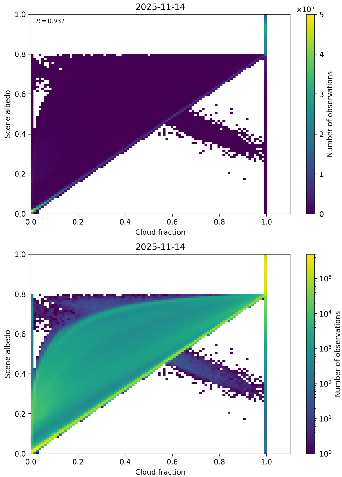
Figure 75: Scatter density plot of “Cloud fraction” against “Scene albedo” for 2025-11-13 to 2025-11-15.
