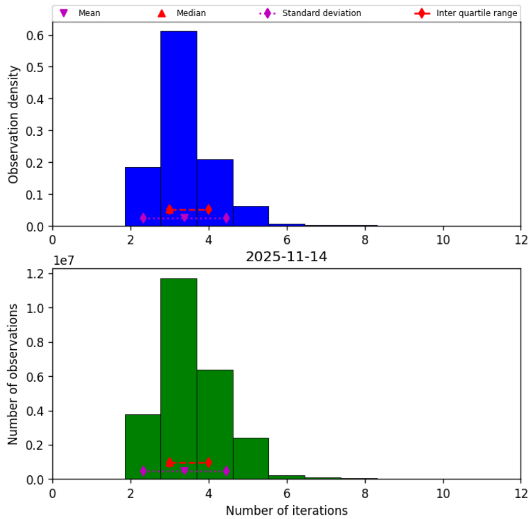
Figure 39: Histogram of “Number of iterations” for 2025-11-13 to 2025-11-15
