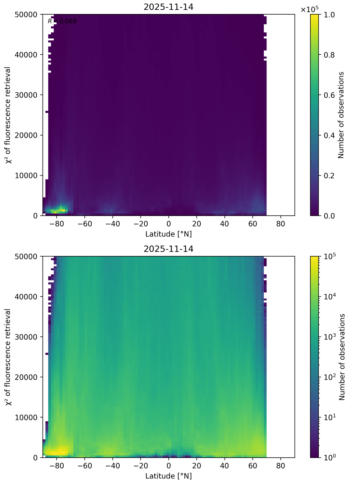
Figure 89: Scatter density plot of “Latitude” against “ \chi^2 of fluorescence retrieval” for 2025-11-13 to 2025-11-15.
