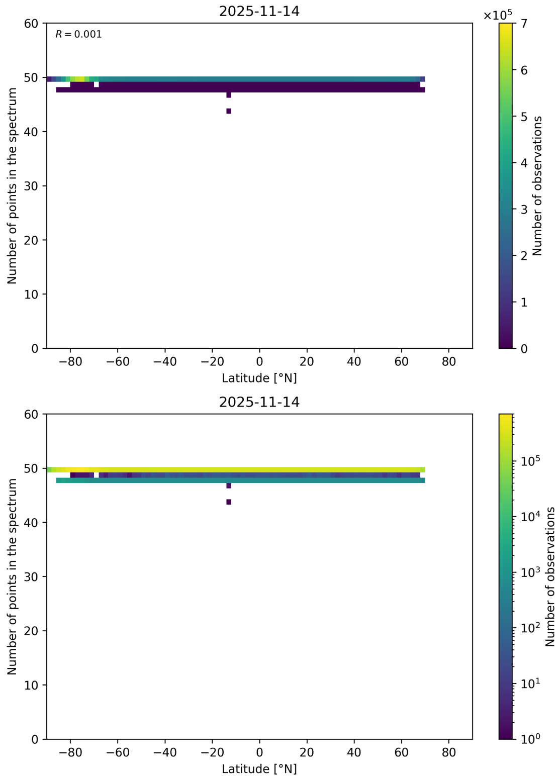
Figure 94: Scatter density plot of “Latitude” against “Number of points in the spectrum” for 2025-11-13 to 2025-11-15.
