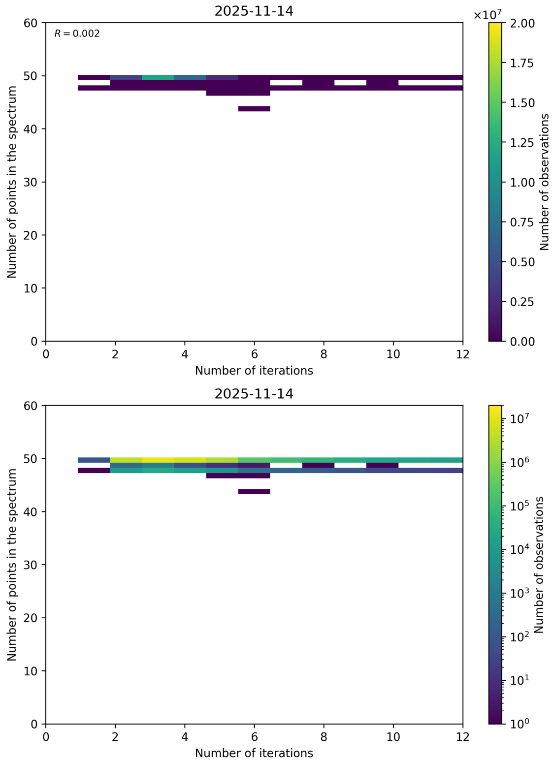
Figure 99: Scatter density plot of “Number of iterations” against “Number of points in the spectrum” for 2025-11-13 to 2025-11-15.
