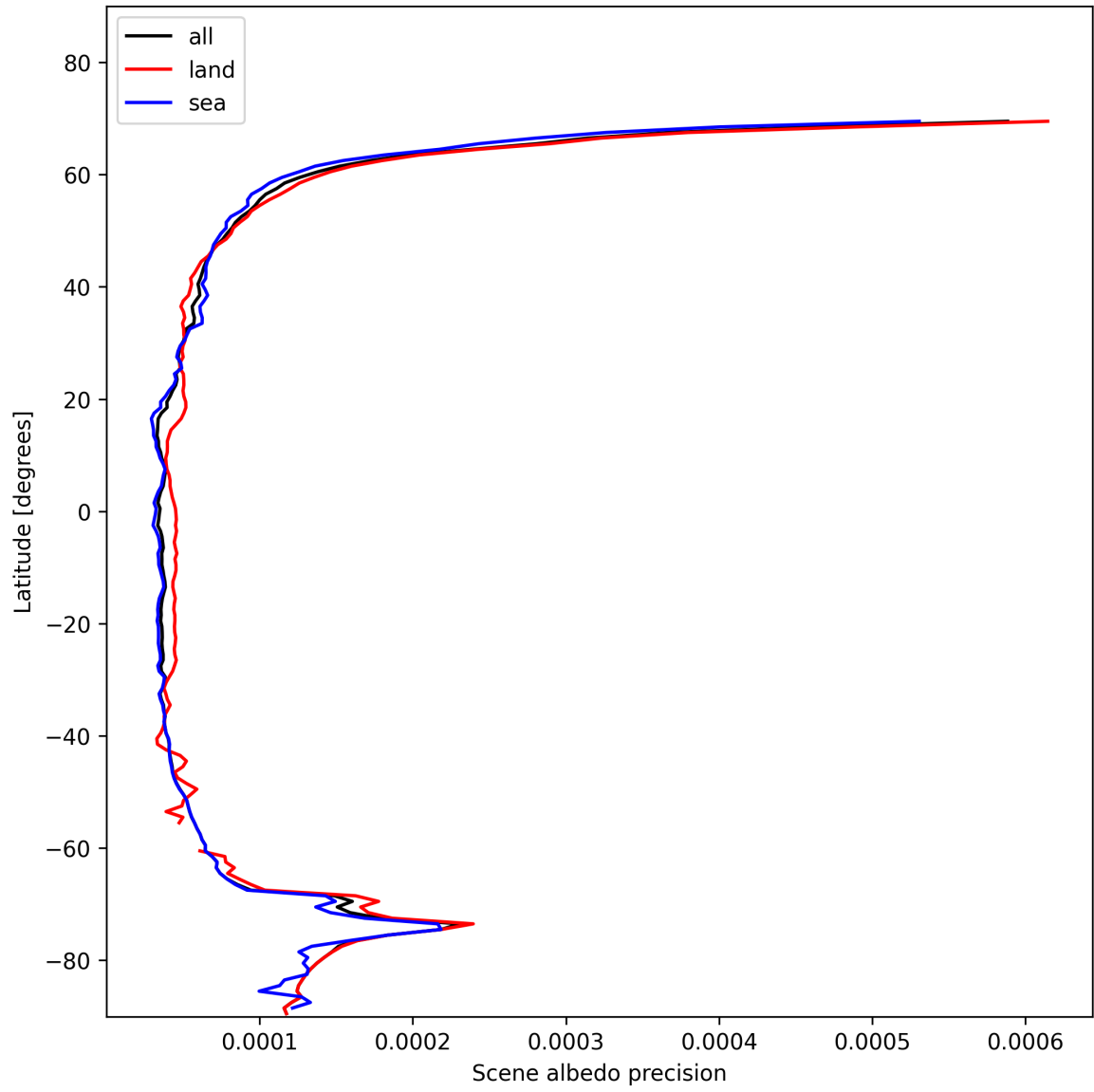
Figure 18: Zonal average of “Scene albedo precision” for 2025-11-13 to 2025-11-15.
