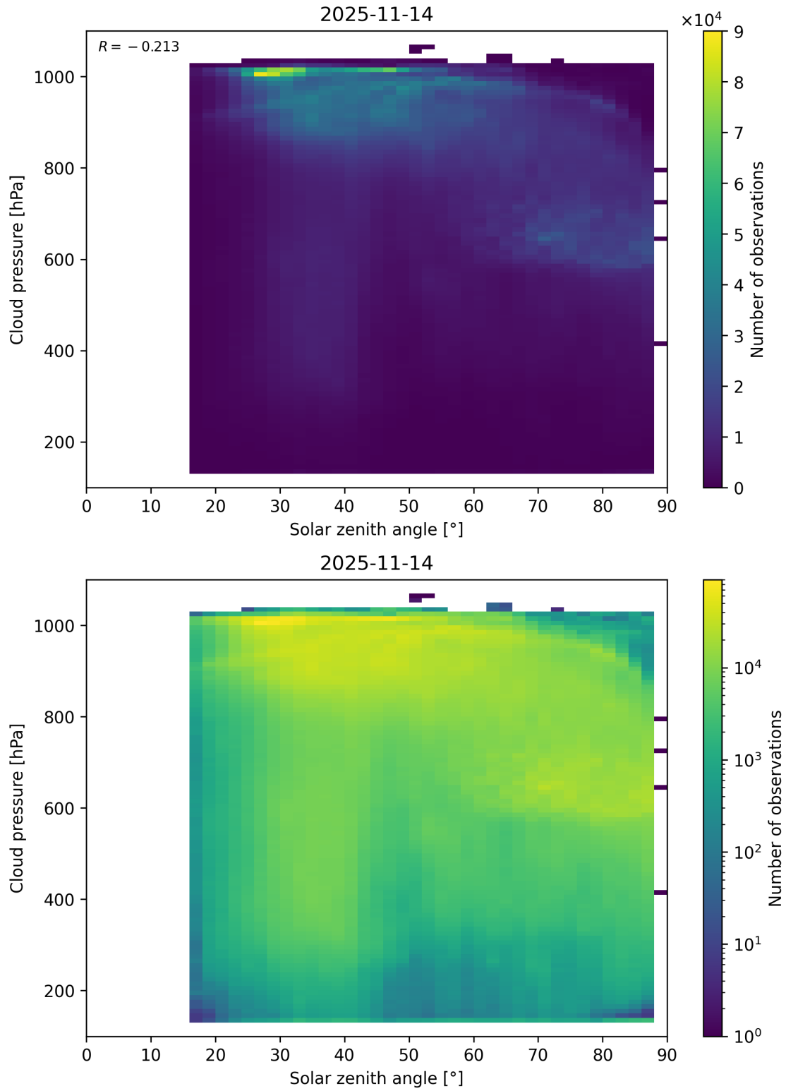
Figure 111: Scatter density plot of “Solar zenith angle” against “Cloud pressure” for 2025-11-13 to 2025-11-15.
