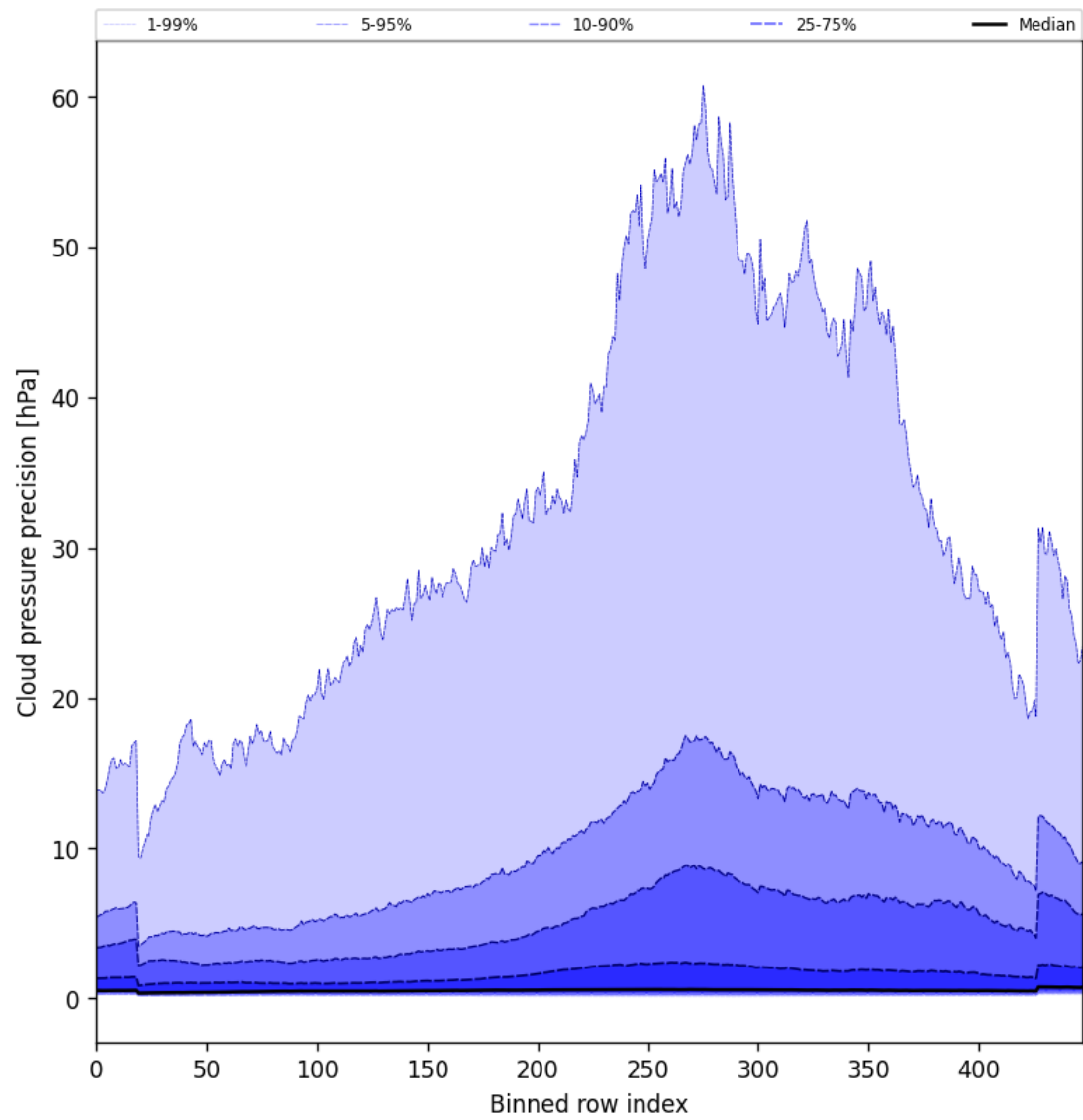
Figure 48: Along track statistics of “Cloud pressure precision” for 2025-11-13 to 2025-11-15
