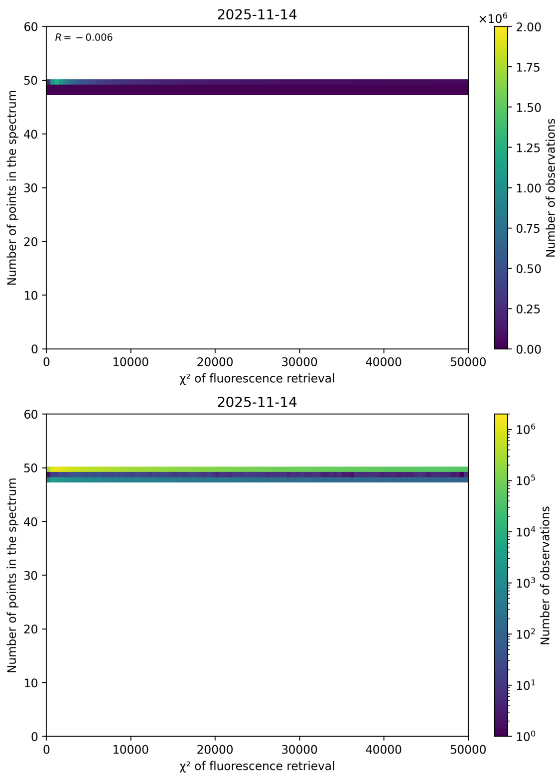
Figure 68: Scatter density plot of “ \chi^2 of fluorescence retrieval” against “Number of points in the spectrum” for 2025-11-13 to 2025-11-15.
