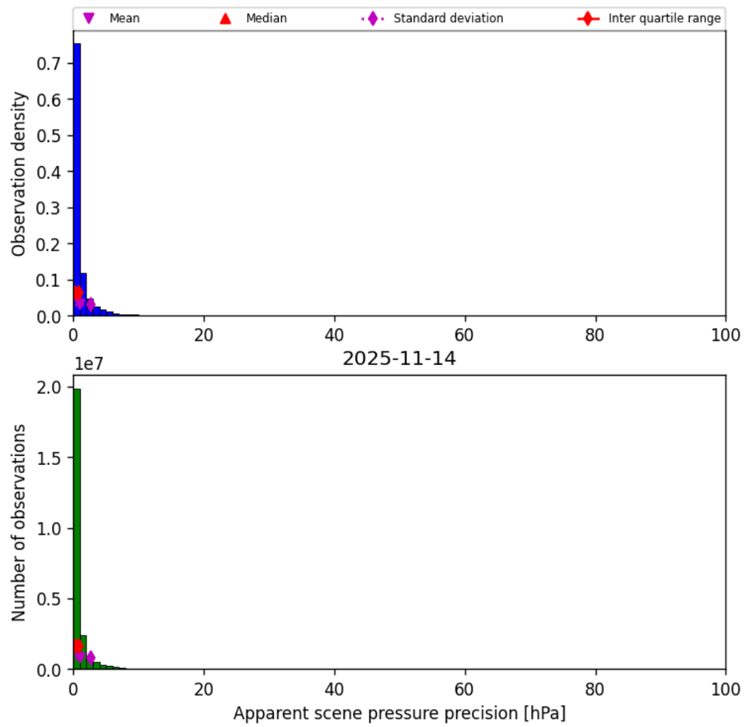
Figure 37: Histogram of “Apparent scene pressure precision” for 2025-11-13 to 2025-11-15
