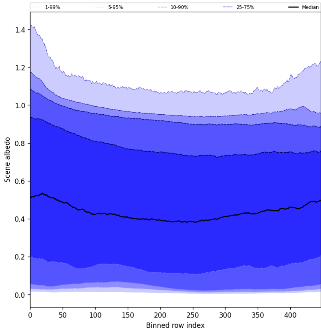
Figure 51: Along track statistics of “Scene albedo” for 2025-11-13 to 2025-11-15
