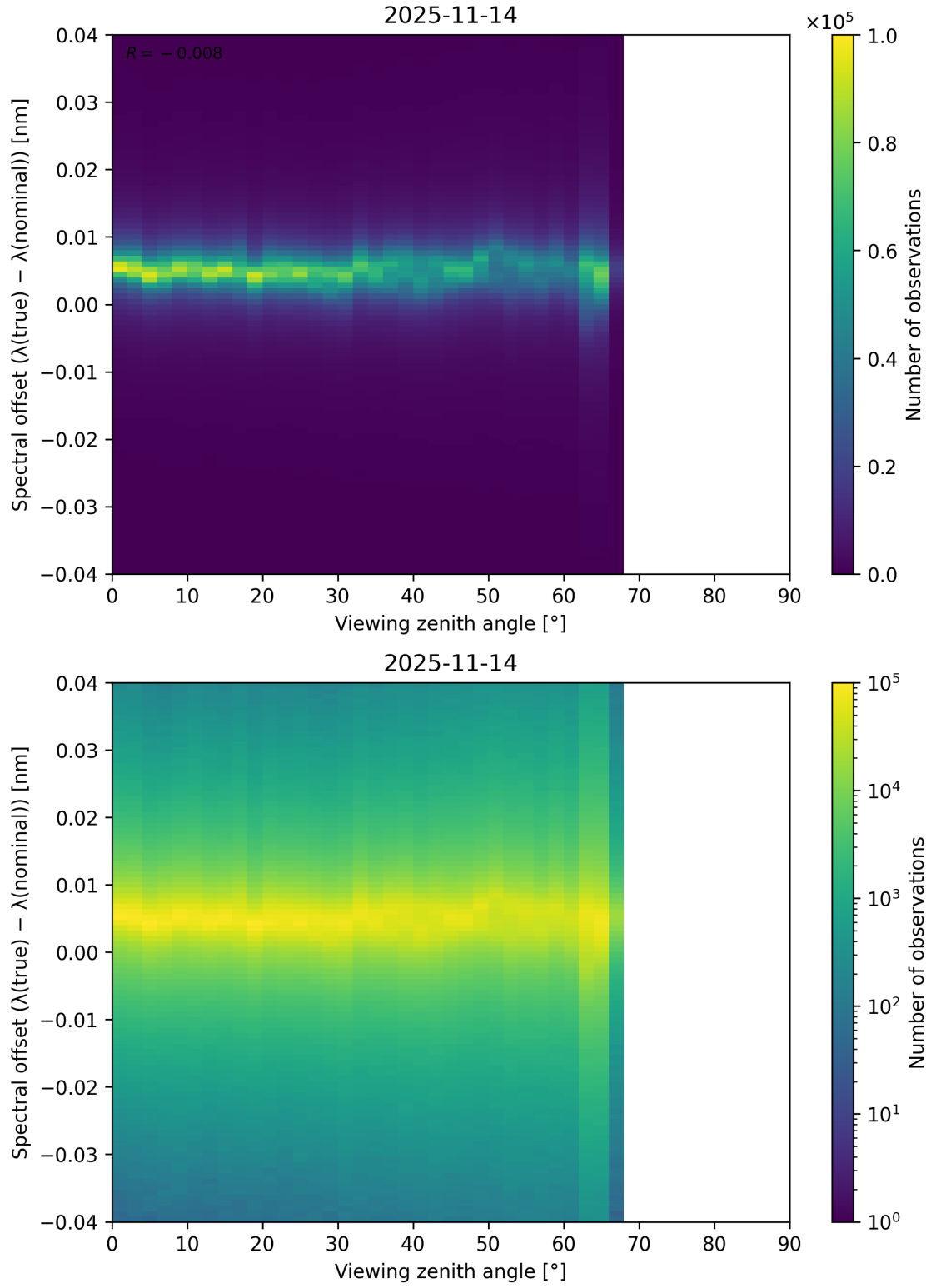
Figure 128: Scatter density plot of “Viewing zenith angle” against “Spectral offset ( \lambda_{\text{true}} - \lambda_{\text{nominal}} )” for 2025-11-13 to 2025-11-15.
