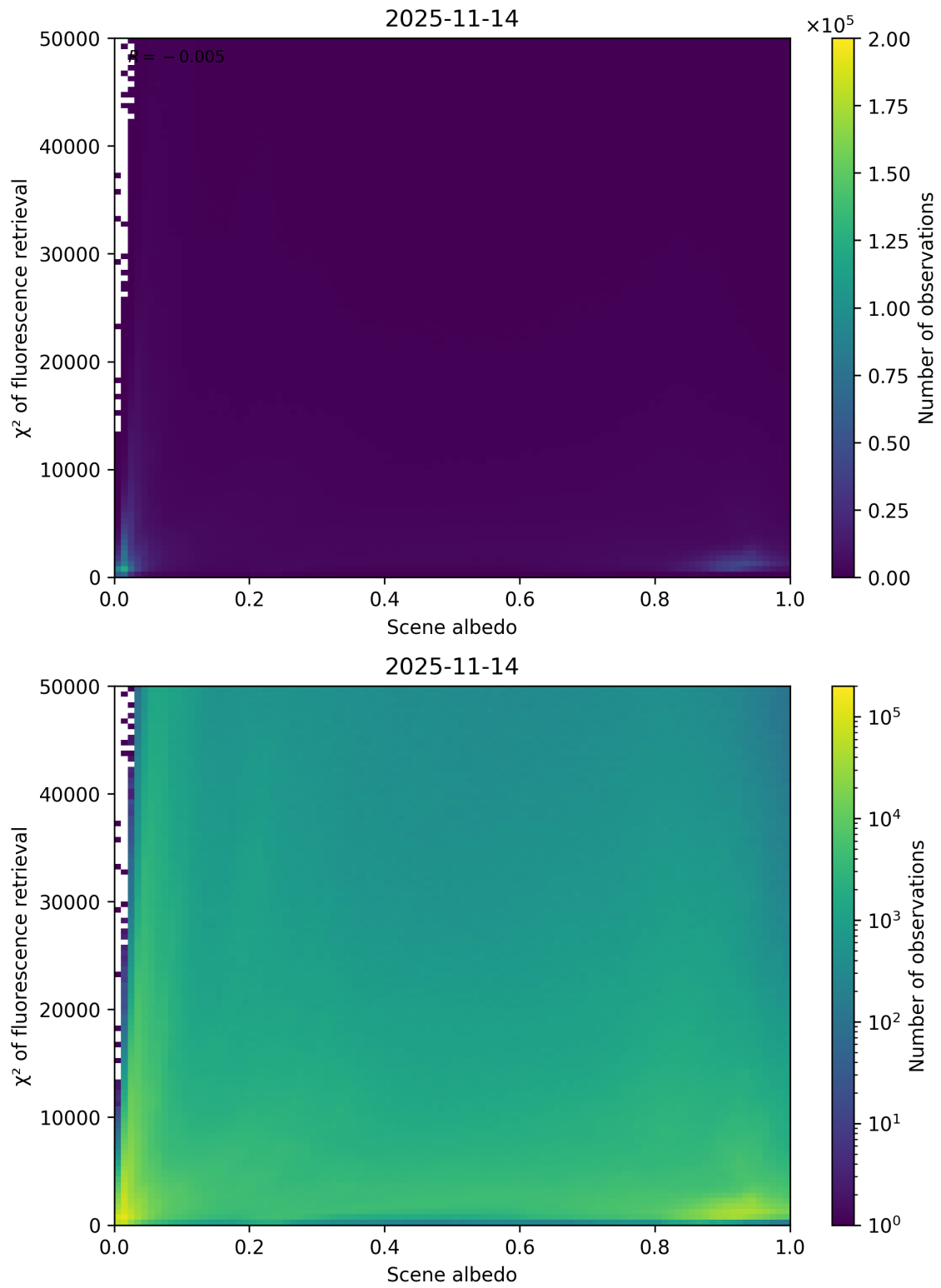
Figure 103: Scatter density plot of “Scene albedo” against “ \chi^2 of fluorescence retrieval” for 2025-11-13 to 2025-11-15.
