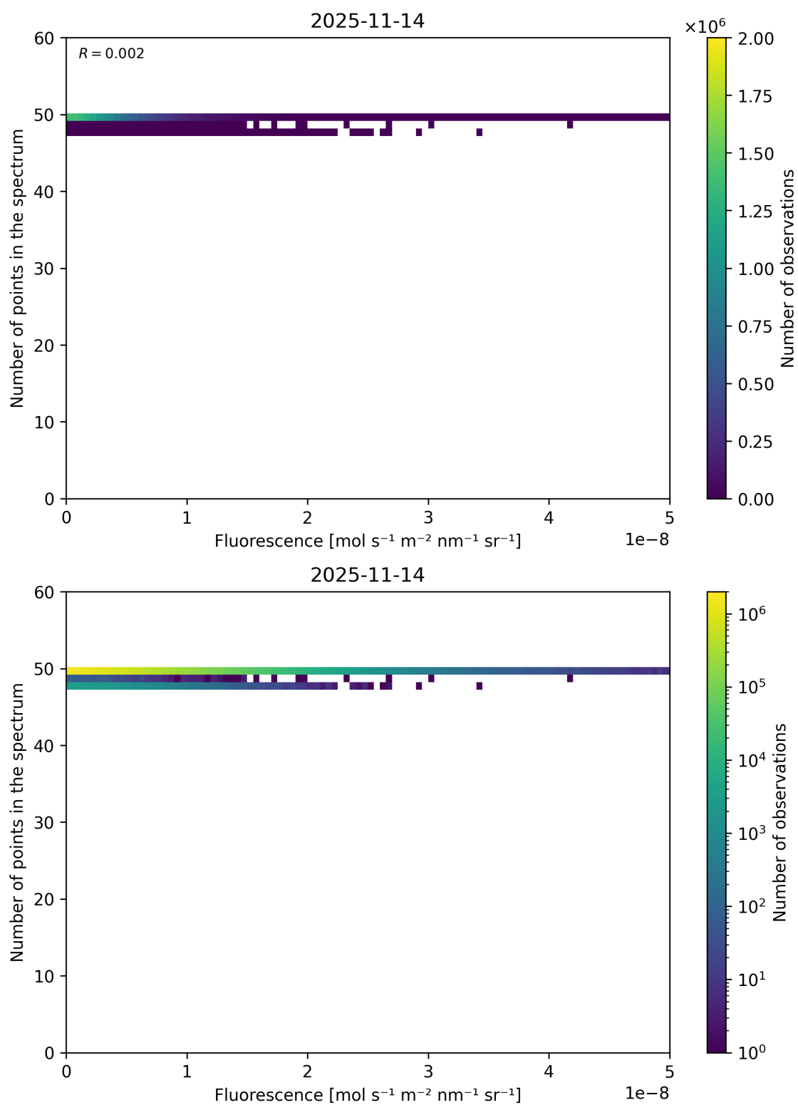
Figure 86: Scatter density plot of “Fluorescence” against “Number of points in the spectrum” for 2025-11-13 to 2025-11-15.
