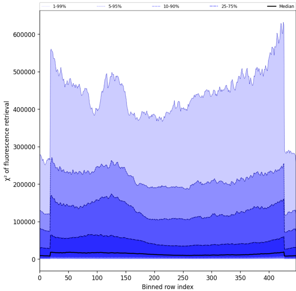
Figure 59: Along track statistics of “ \chi^2 of fluorescence retrieval” for 2025-11-13 to 2025-11-15
