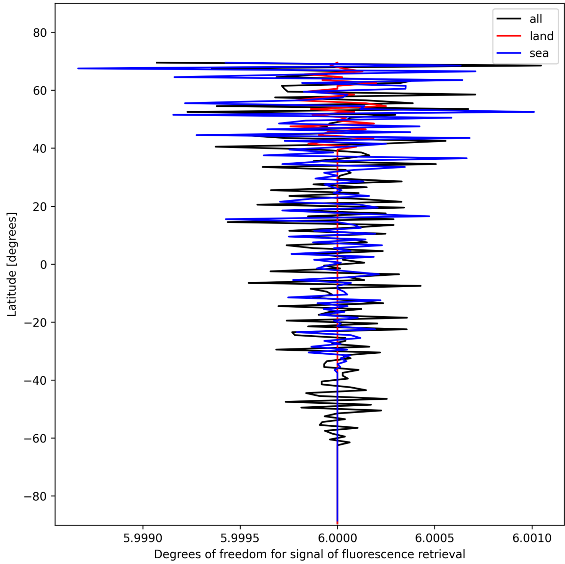
Figure 26: Zonal average of “Degrees of freedom for signal of fluorescence retrieval” for 2025-11-13 to 2025-11-15.
