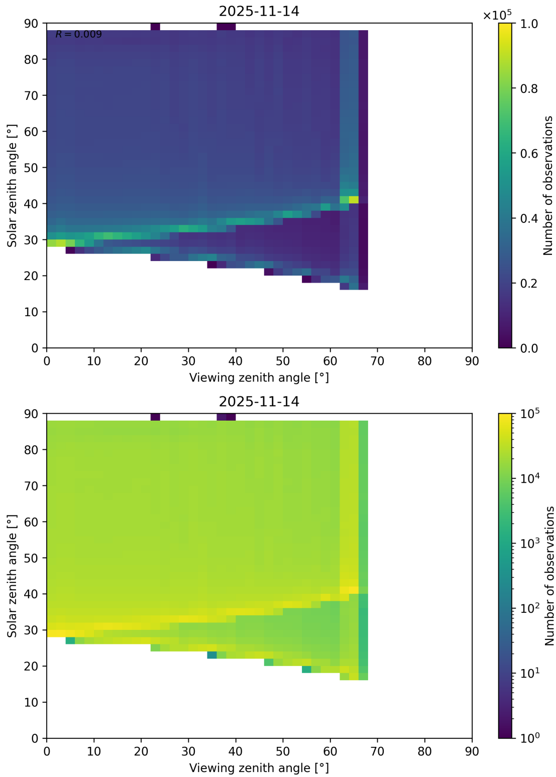
Figure 127: Scatter density plot of “Viewing zenith angle” against “Solar zenith angle” for 2025-11-13 to 2025-11-15.
