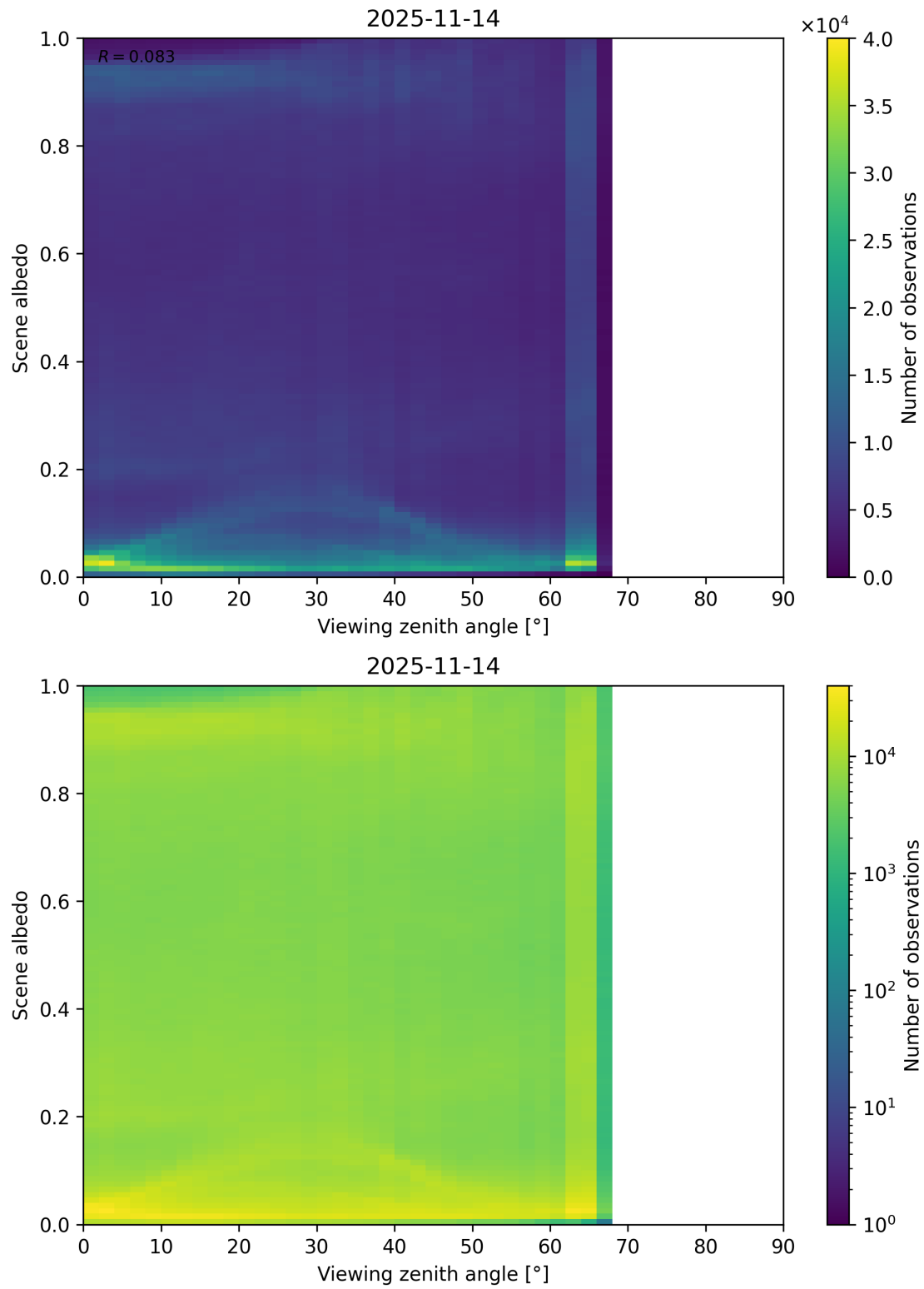
Figure 126: Scatter density plot of “Viewing zenith angle” against “Scene albedo” for 2025-11-13 to 2025-11-15.
