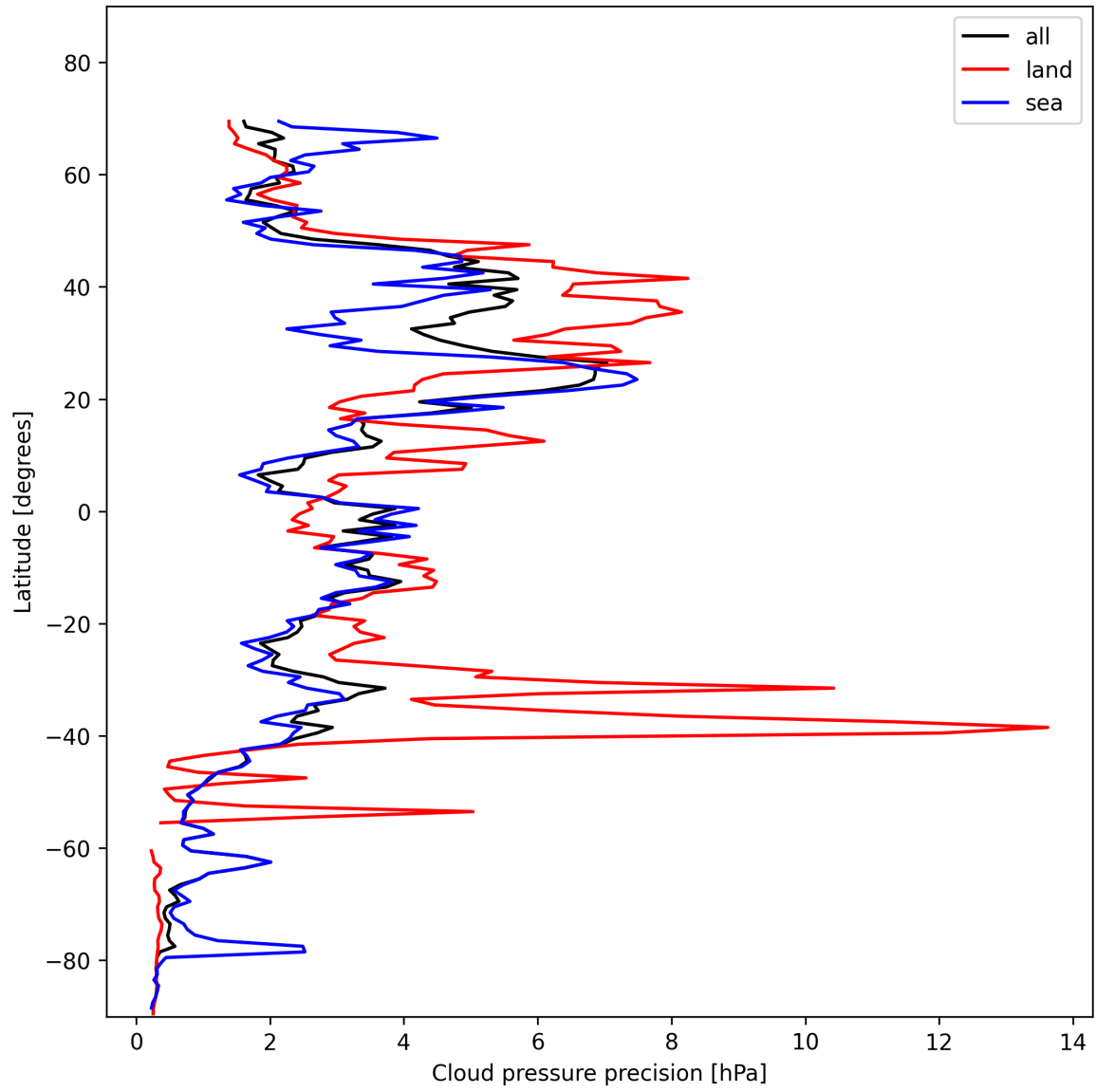
Figure 14: Zonal average of "Cloud pressure precision" for 2025-11-13 to 2025-11-15.
