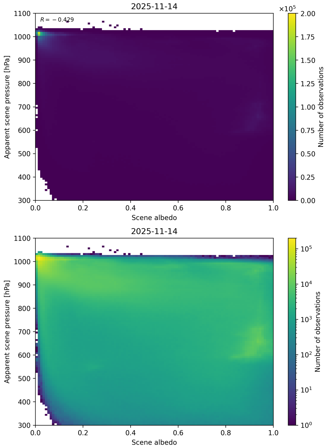
Figure 102: Scatter density plot of “Scene albedo” against “Apparent scene pressure” for 2025-11-13 to 2025-11-15.
