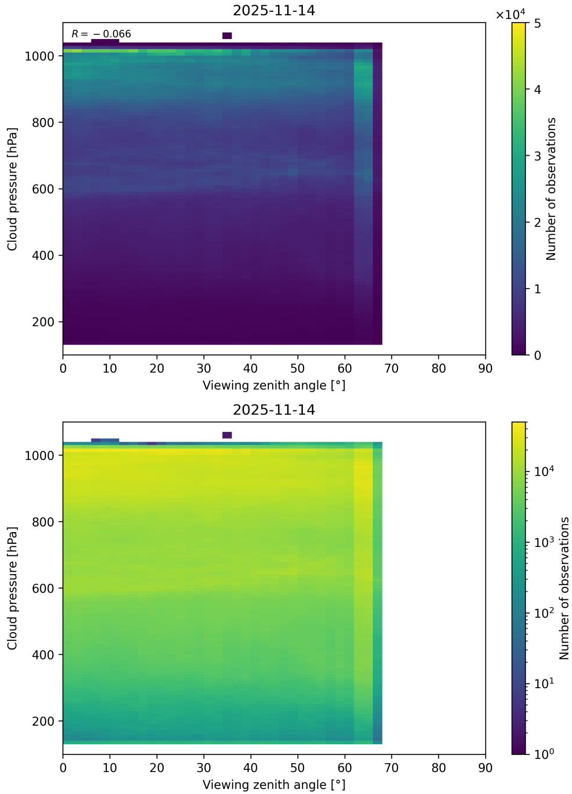
Figure 121: Scatter density plot of “Viewing zenith angle” against “Cloud pressure” for 2025-11-13 to 2025-11-15.
