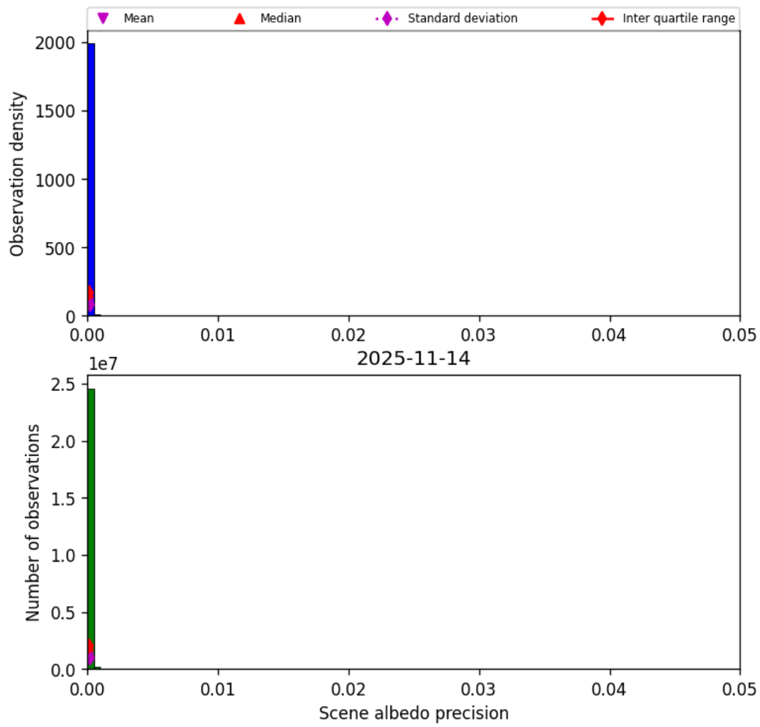
Figure 35: Histogram of “Scene albedo precision” for 2025-11-13 to 2025-11-15
