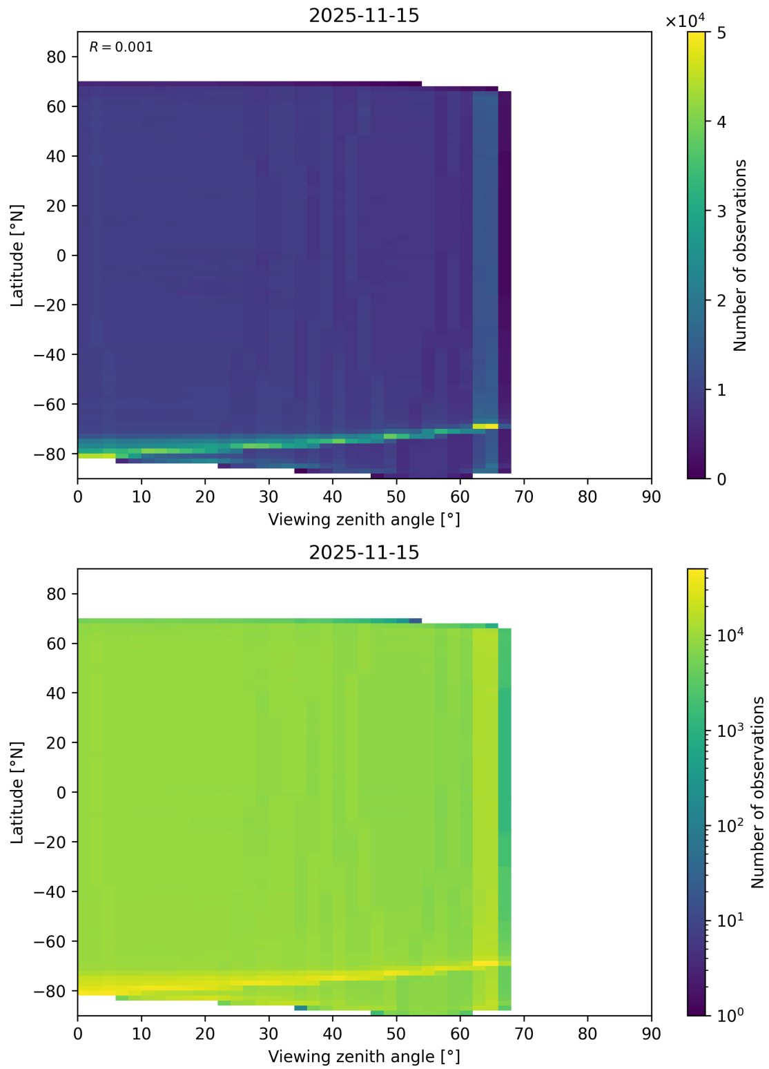
Figure 123: Scatter density plot of “Viewing zenith angle” against “Latitude” for 2025-11-14 to 2025-11-16.
