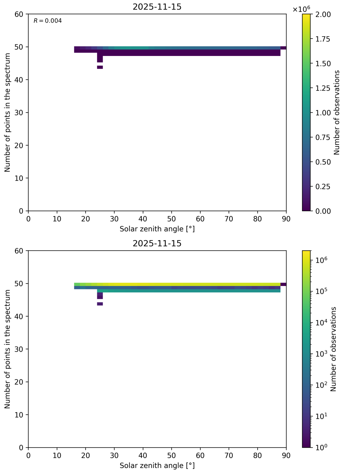
Figure 115: Scatter density plot of “Solar zenith angle” against “Number of points in the spectrum” for 2025-11-14 to 2025-11-16.
