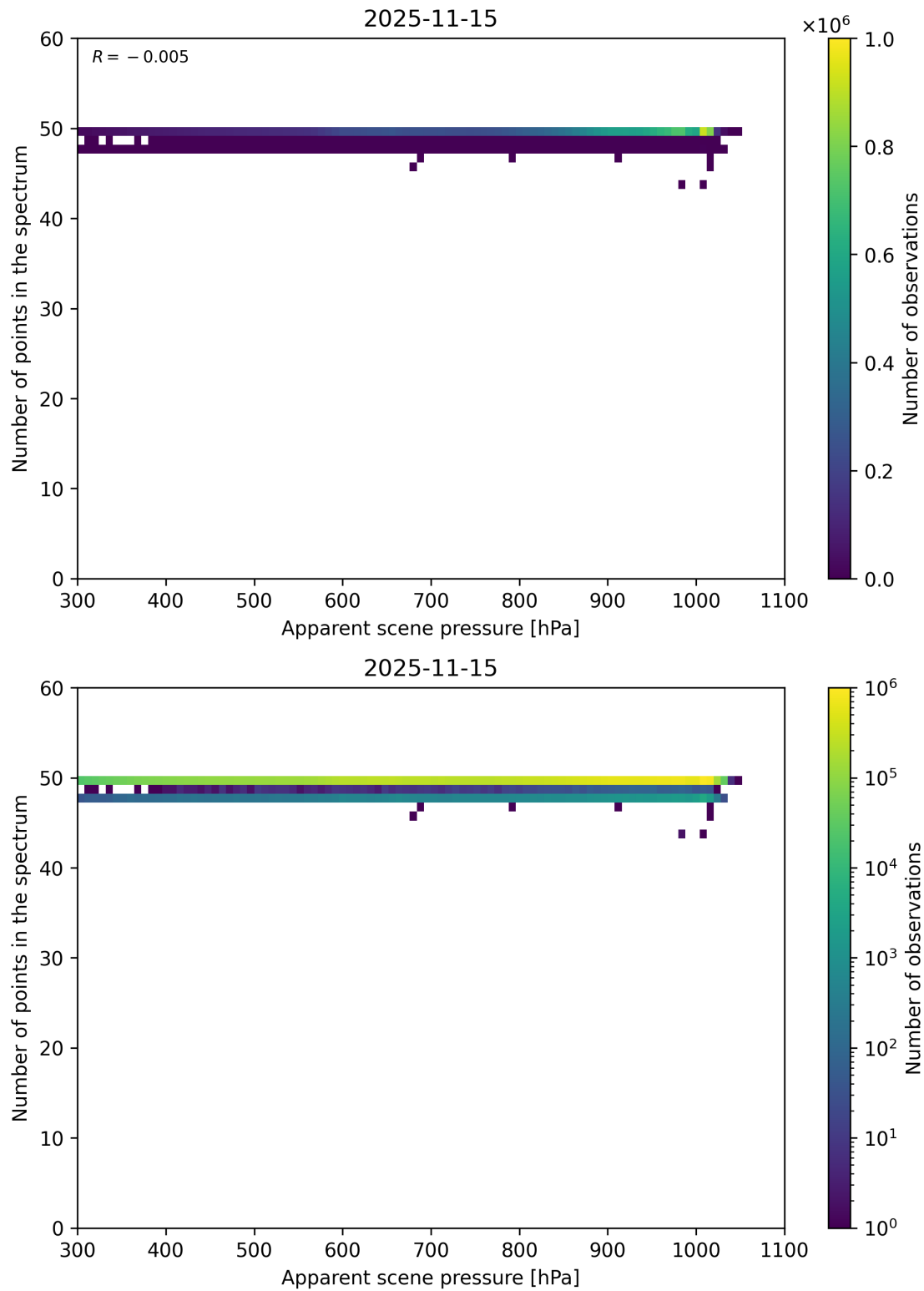
Figure 66: Scatter density plot of “Apparent scene pressure” against “Number of points in the spectrum” for 2025-11-14 to 2025-11-16.
