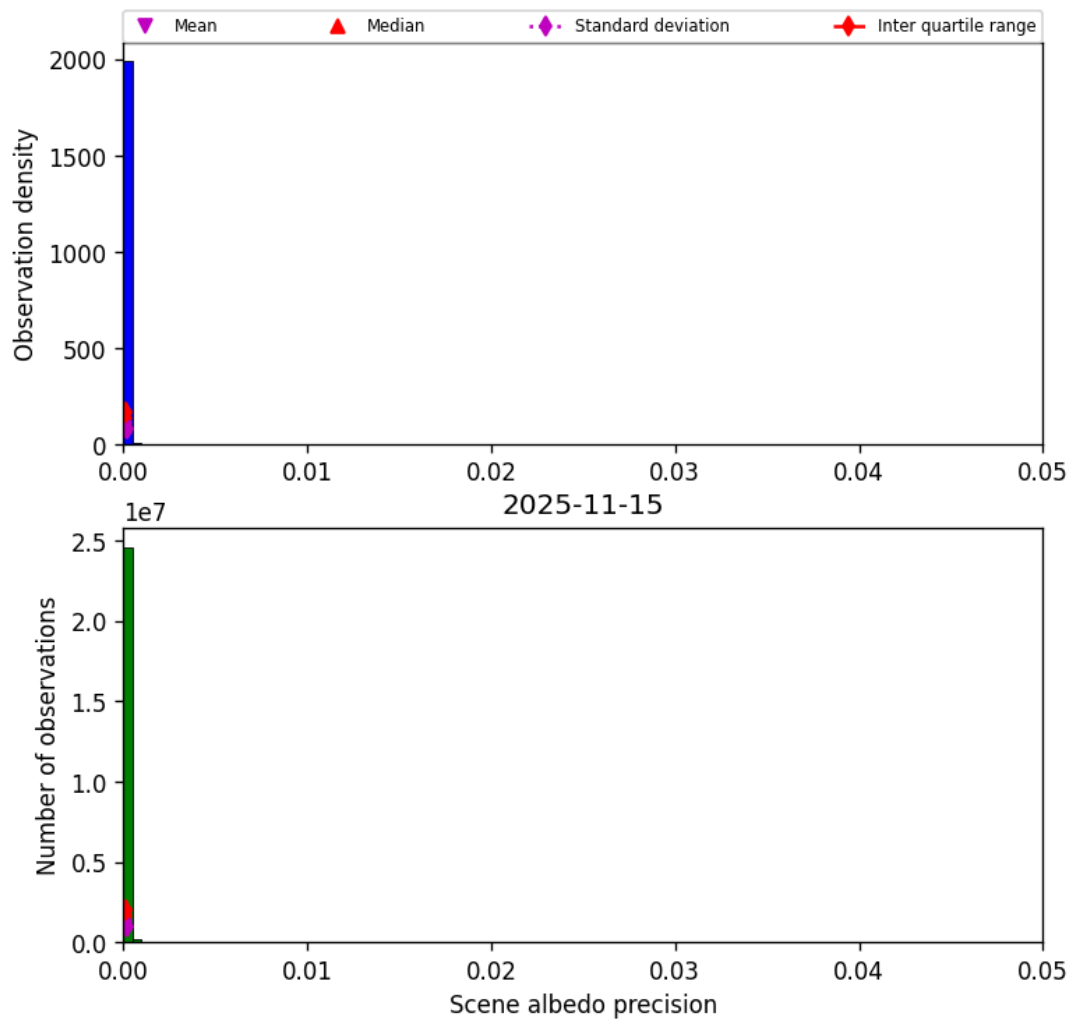
Figure 35: Histogram of “Scene albedo precision” for 2025-11-14 to 2025-11-16
