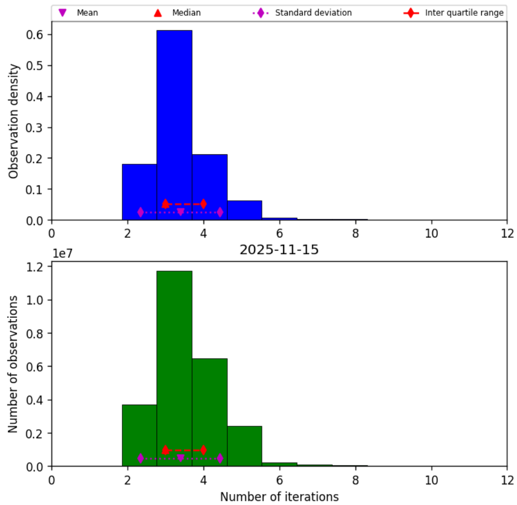
Figure 39: Histogram of “Number of iterations” for 2025-11-14 to 2025-11-16
