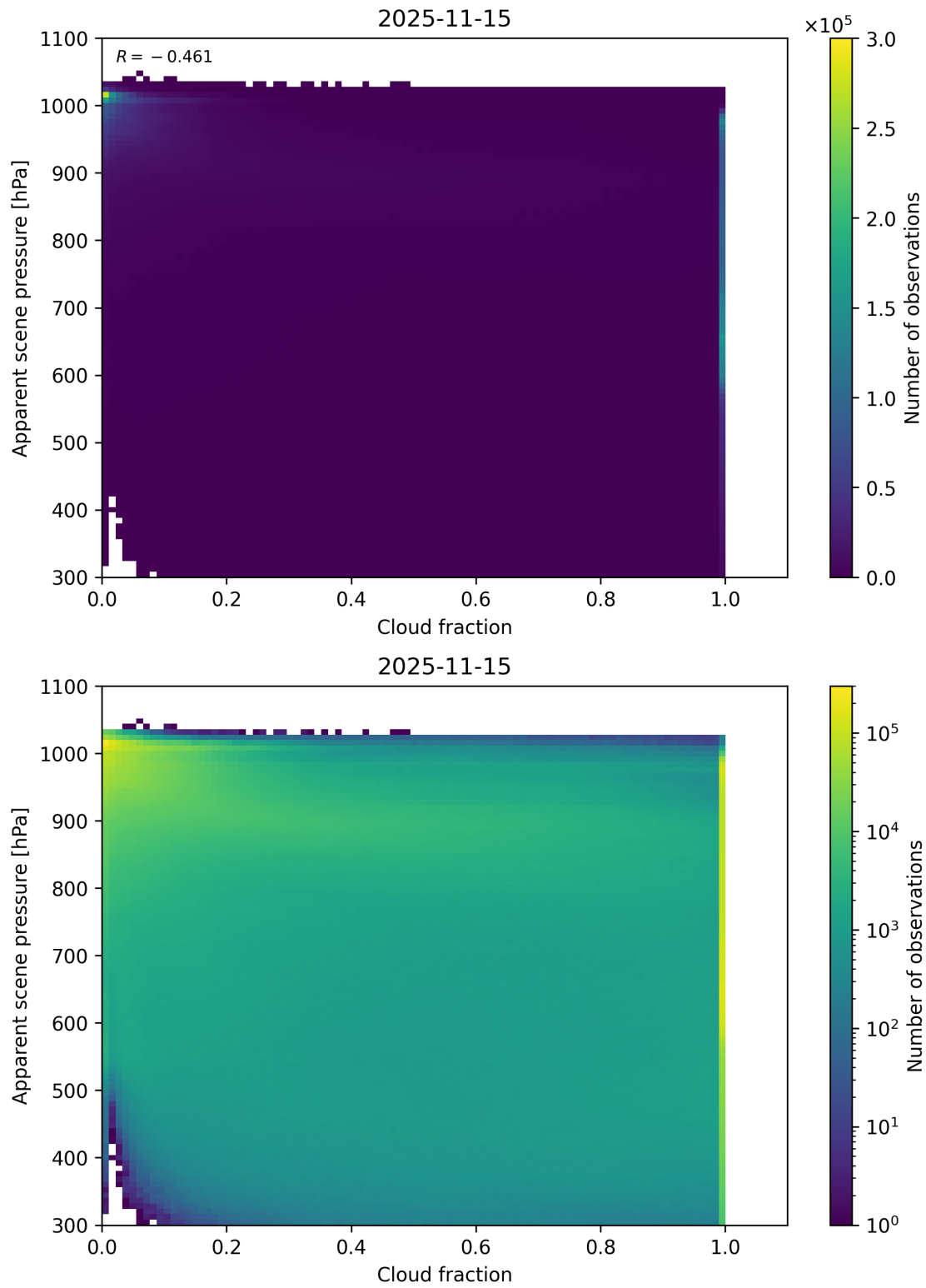
Figure 70: Scatter density plot of “Cloud fraction” against “Apparent scene pressure” for 2025-11-14 to 2025-11-16.
