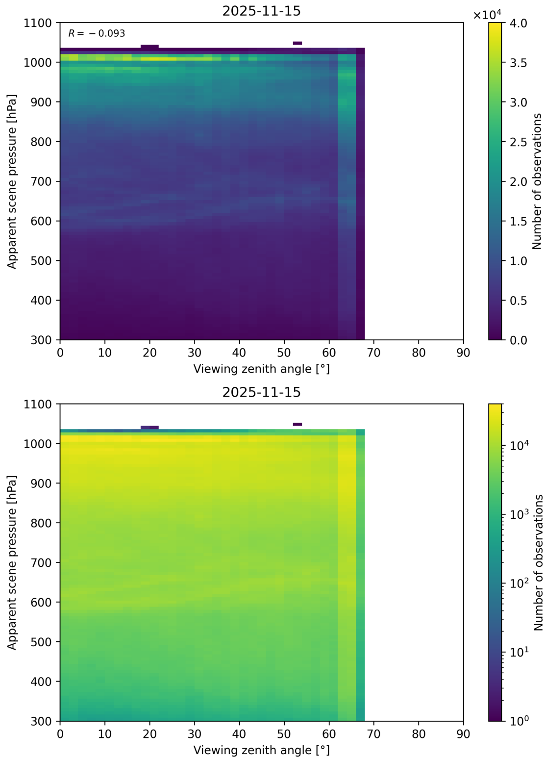
Figure 118: Scatter density plot of “Viewing zenith angle” against “Apparent scene pressure” for 2025-11-14 to 2025-11-16.
