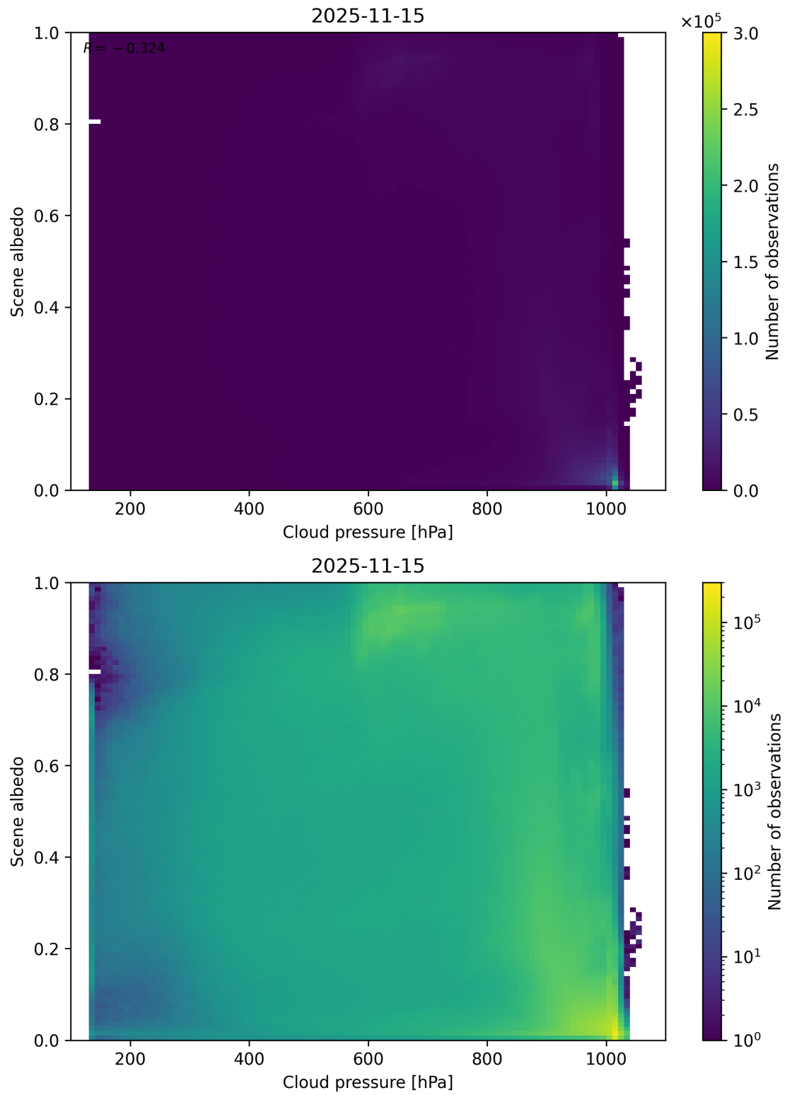
Figure 83: Scatter density plot of “Cloud pressure” against “Scene albedo” for 2025-11-14 to 2025-11-16.
