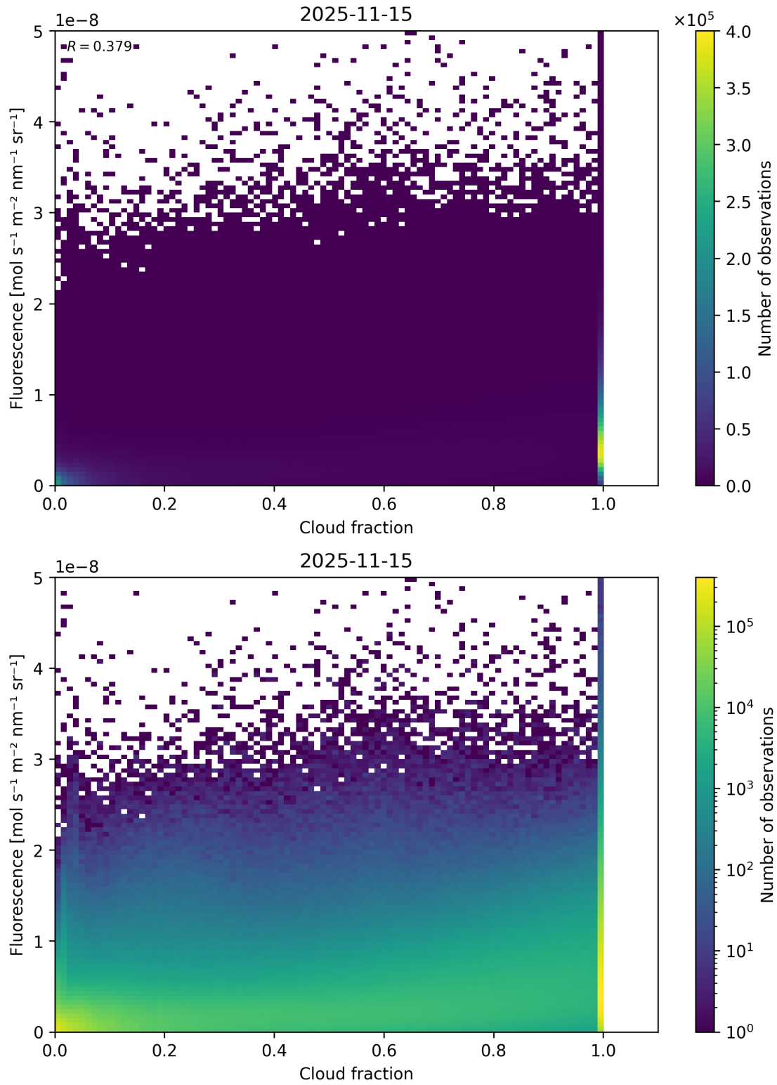
Figure 72: Scatter density plot of “Cloud fraction” against “Fluorescence” for 2025-11-14 to 2025-11-16.
