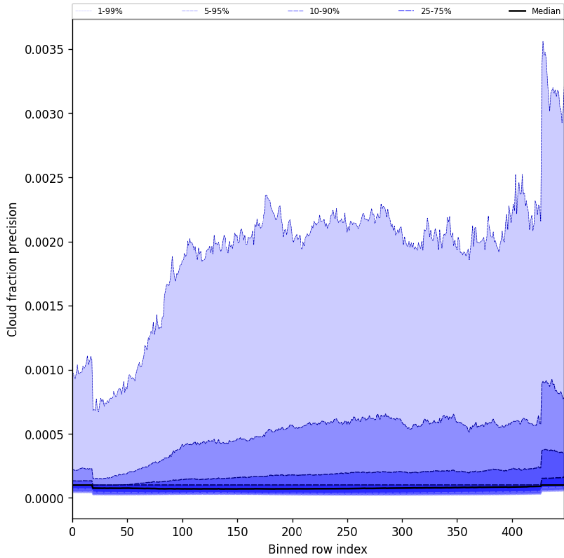
Figure 50: Along track statistics of “Cloud fraction precision” for 2025-11-14 to 2025-11-16
