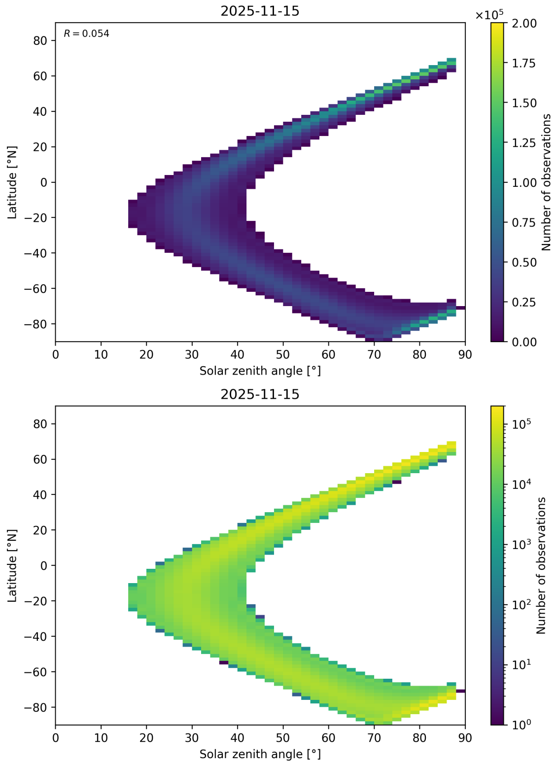
Figure 113: Scatter density plot of “Solar zenith angle” against “Latitude” for 2025-11-14 to 2025-11-16.
