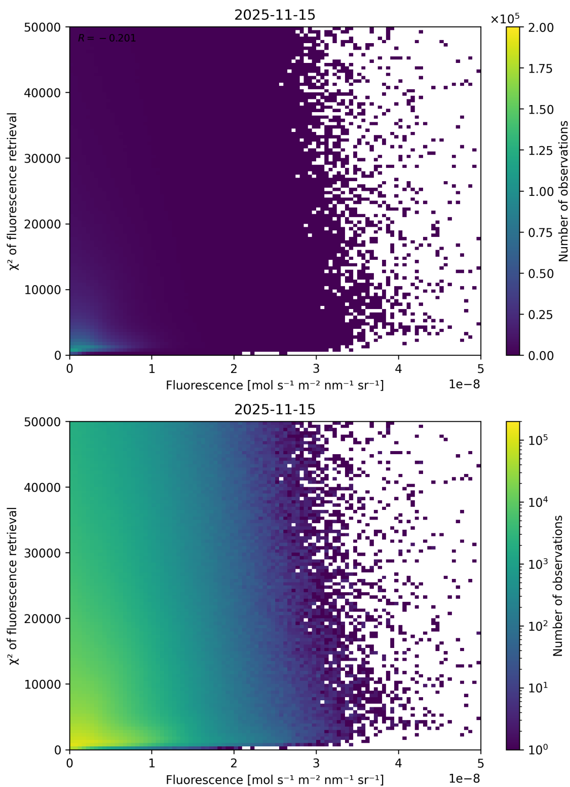
Figure 85: Scatter density plot of “Fluorescence” against “ \chi^2 of fluorescence retrieval” for 2025-11-14 to 2025-11-16.
