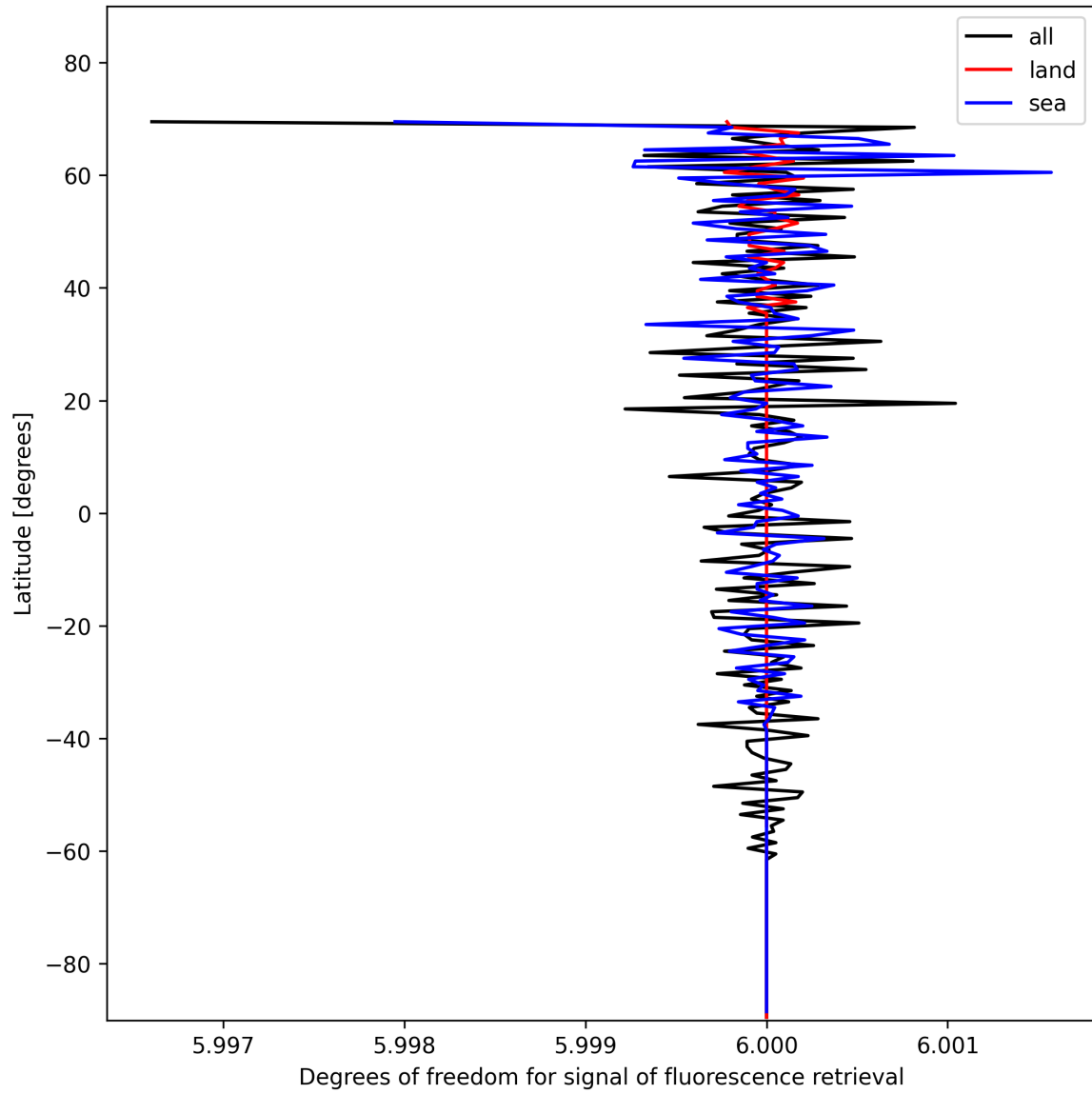
Figure 26: Zonal average of “Degrees of freedom for signal of fluorescence retrieval” for 2025-11-14 to 2025-11-16.
