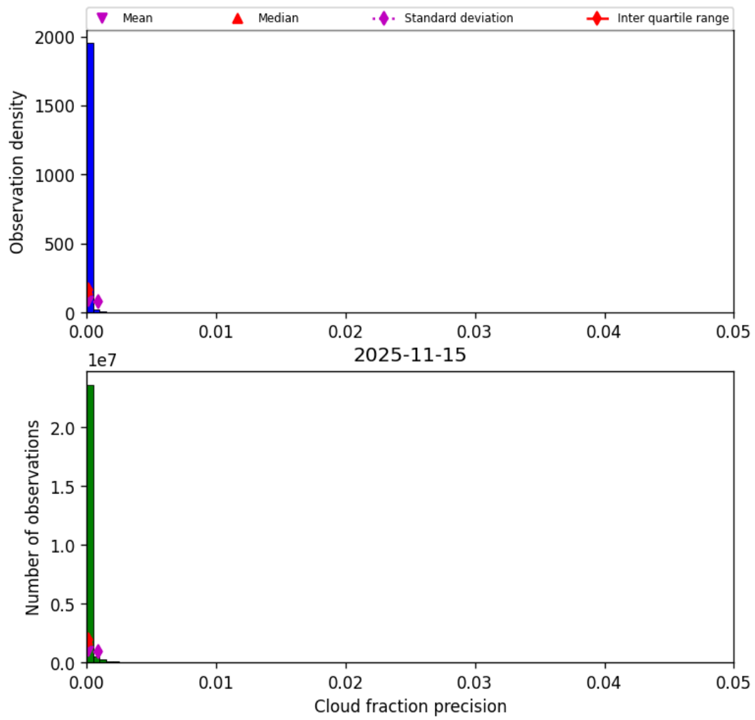
Figure 33: Histogram of “Cloud fraction precision” for 2025-11-14 to 2025-11-16
