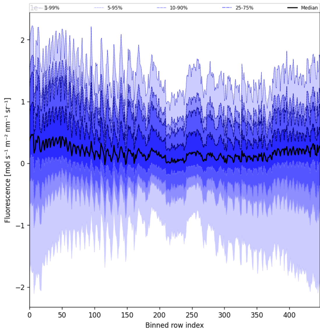
Figure 57: Along track statistics of “Fluorescence” for 2025-11-14 to 2025-11-16
