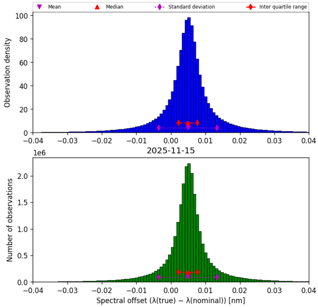
Figure 45: Histogram of “Spectral offset ( \lambda_{\text{true}} - \lambda_{\text{nominal}} )” for 2025-11-14 to 2025-11-16
