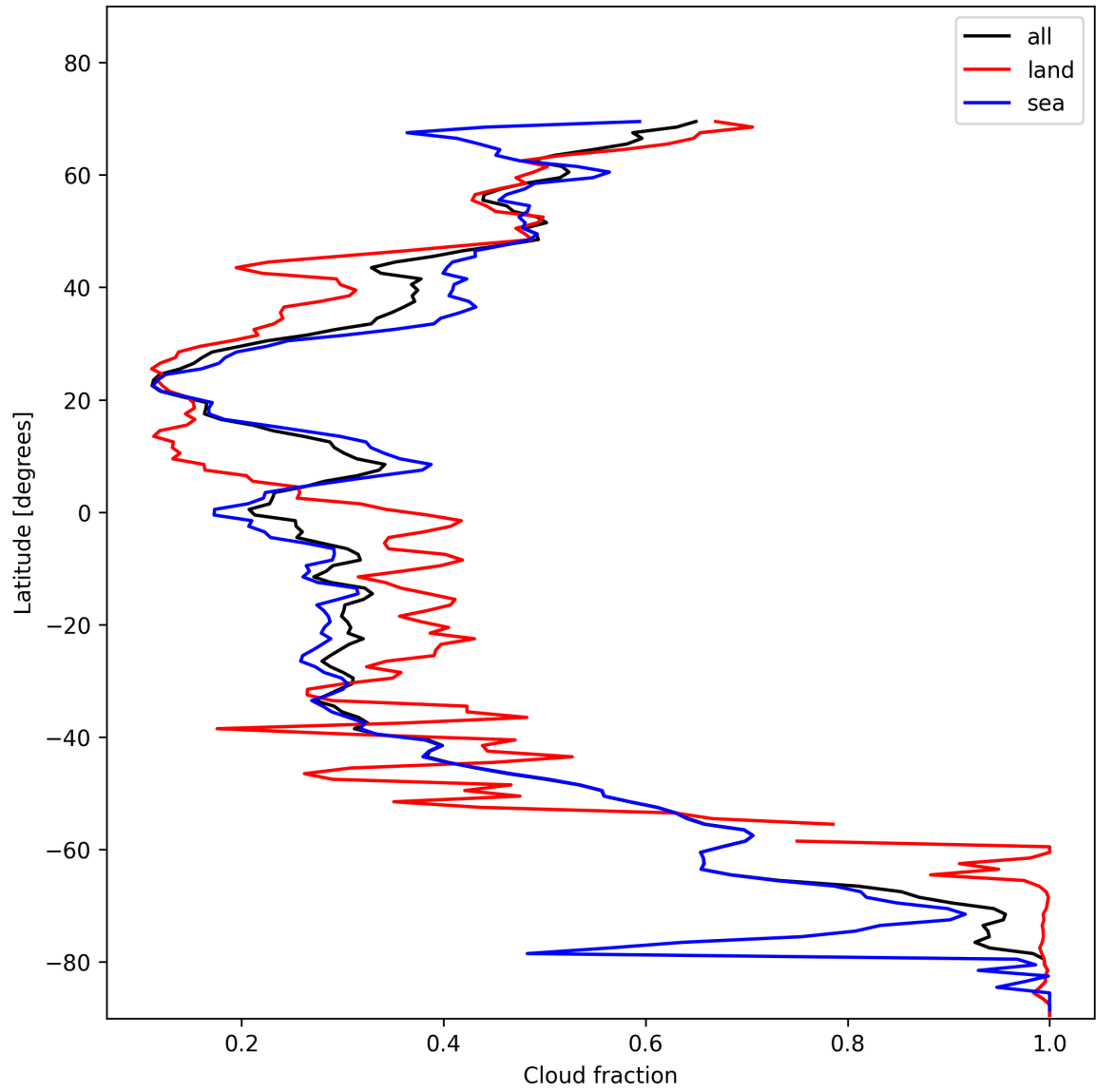
Figure 15: Zonal average of “Cloud fraction” for 2025-11-14 to 2025-11-16.
