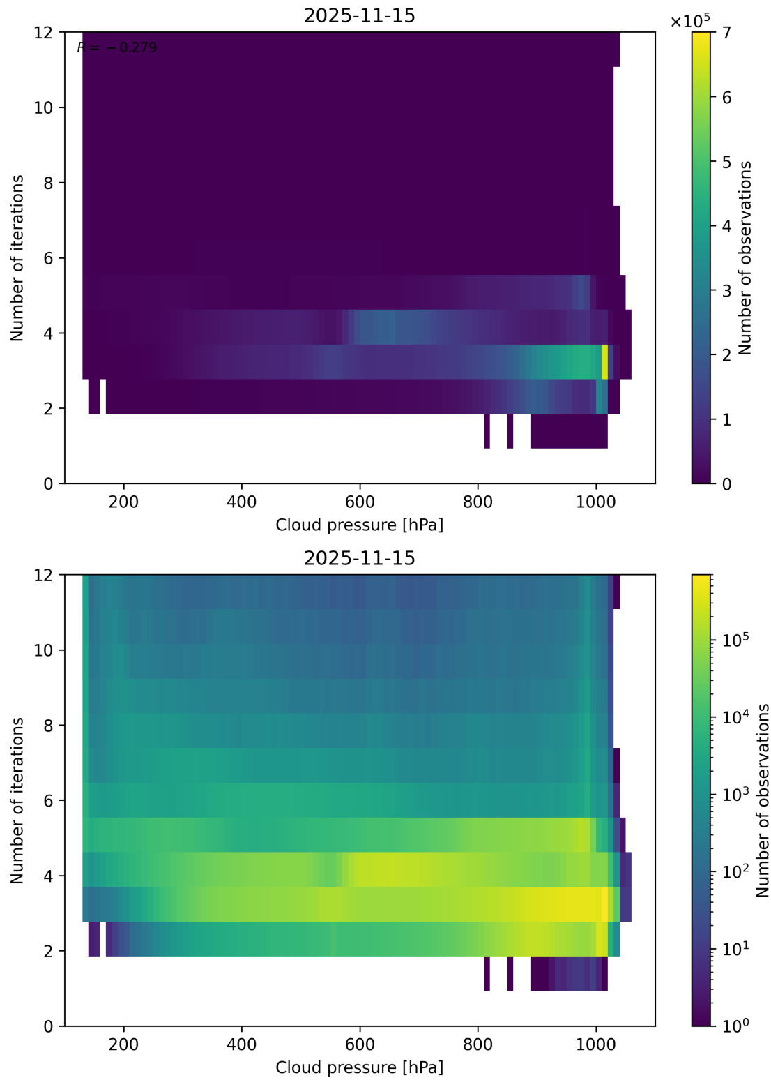
Figure 81: Scatter density plot of “Cloud pressure” against “Number of iterations” for 2025-11-14 to 2025-11-16.
