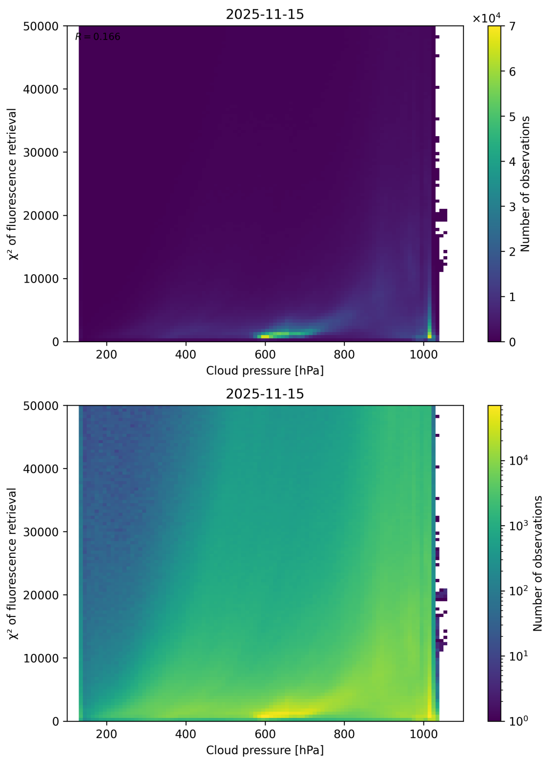
Figure 78: Scatter density plot of “Cloud pressure” against “ \chi^2 of fluorescence retrieval” for 2025-11-14 to 2025-11-16.
