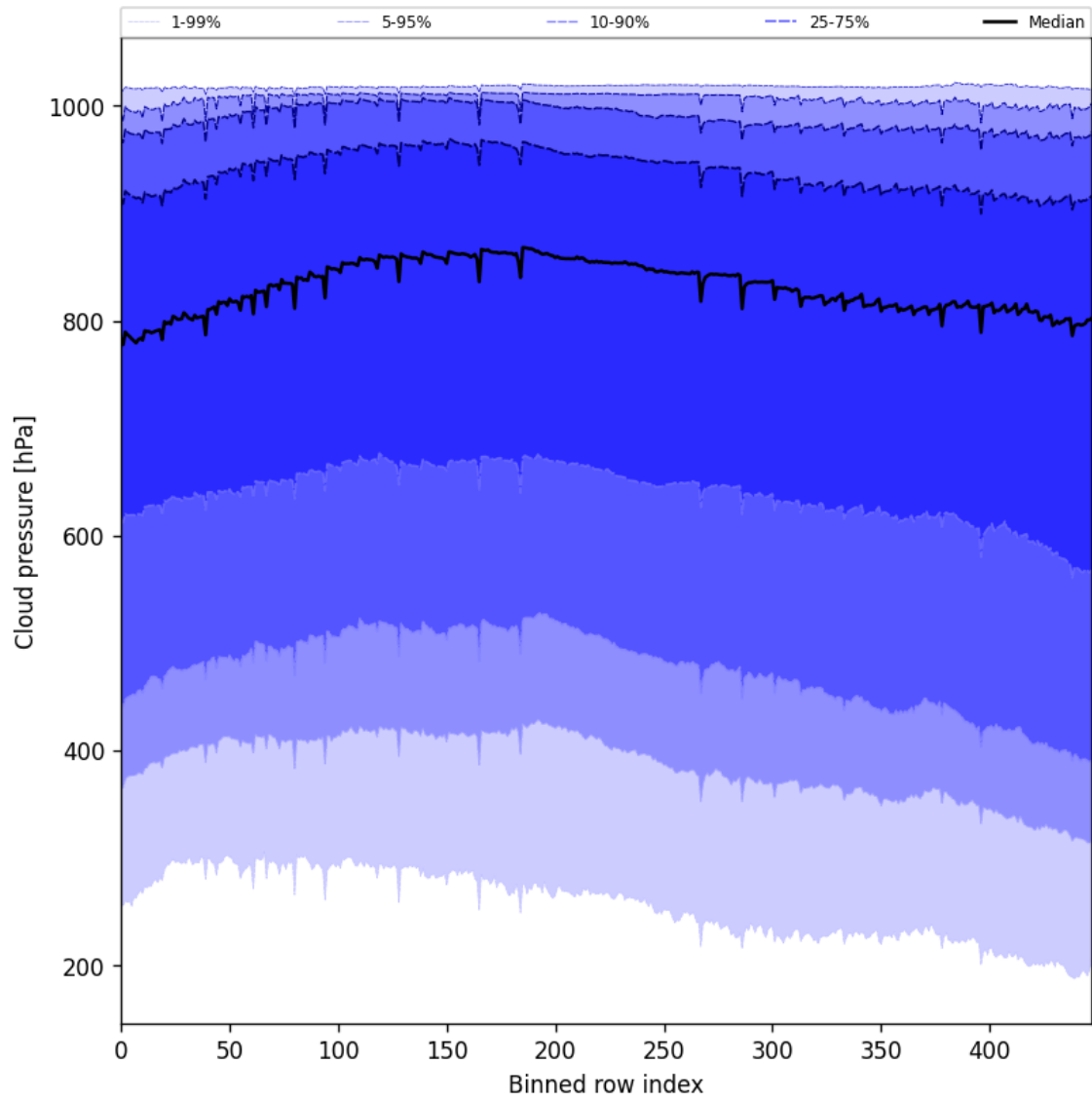
Figure 47: Along track statistics of “Cloud pressure” for 2025-11-14 to 2025-11-16
