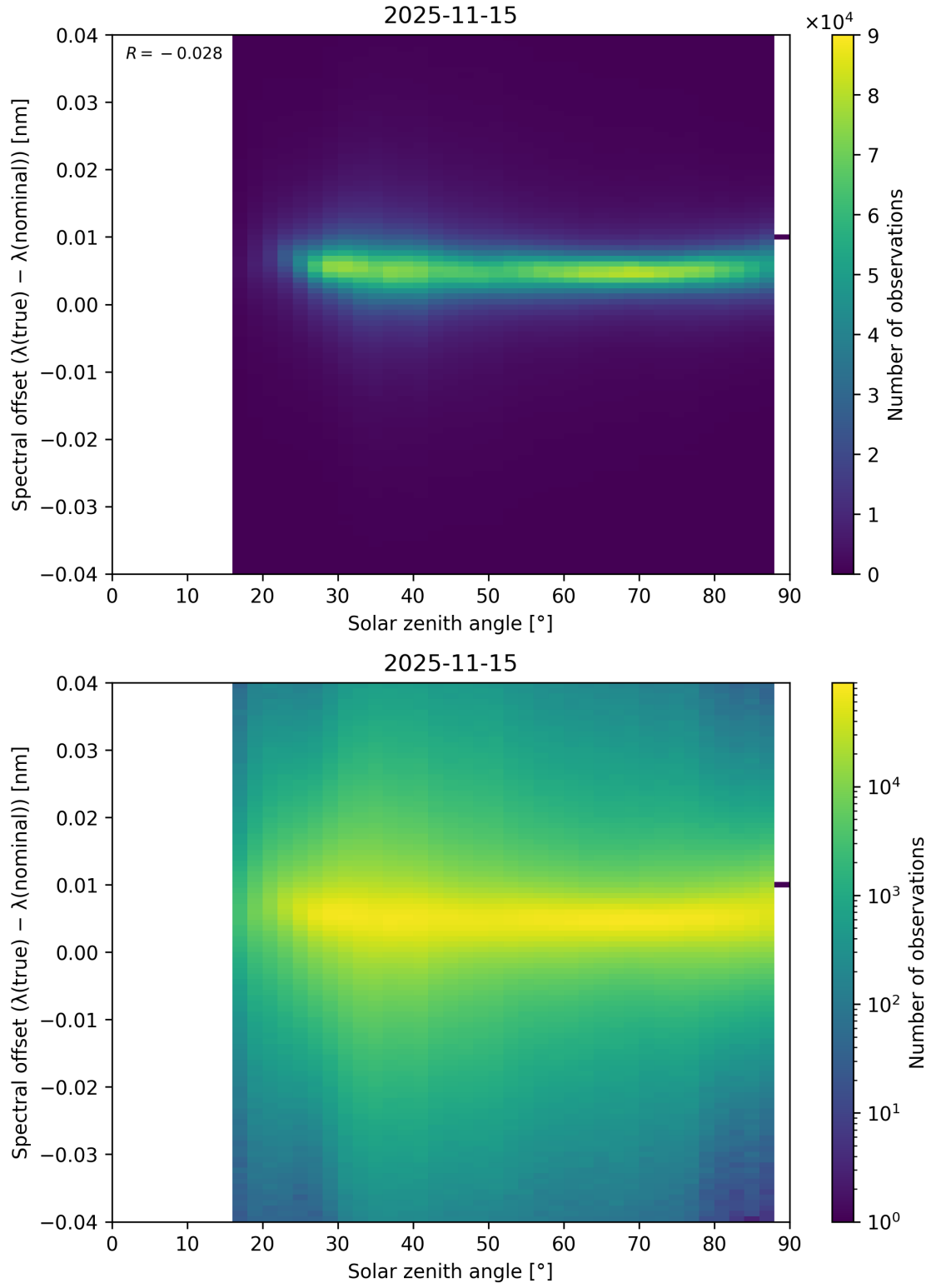
Figure 117: Scatter density plot of “Solar zenith angle” against “Spectral offset ( \lambda_{\text{true}} - \lambda_{\text{nominal}} )” for 2025-11-14 to 2025-11-16.
