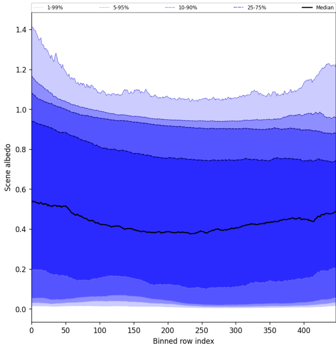
Figure 51: Along track statistics of “Scene albedo” for 2025-11-14 to 2025-11-16
