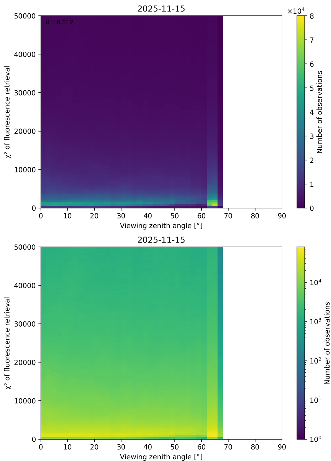
Figure 119: Scatter density plot of “Viewing zenith angle” against “ \chi^2 of fluorescence retrieval” for 2025-11-14 to 2025-11-16.
