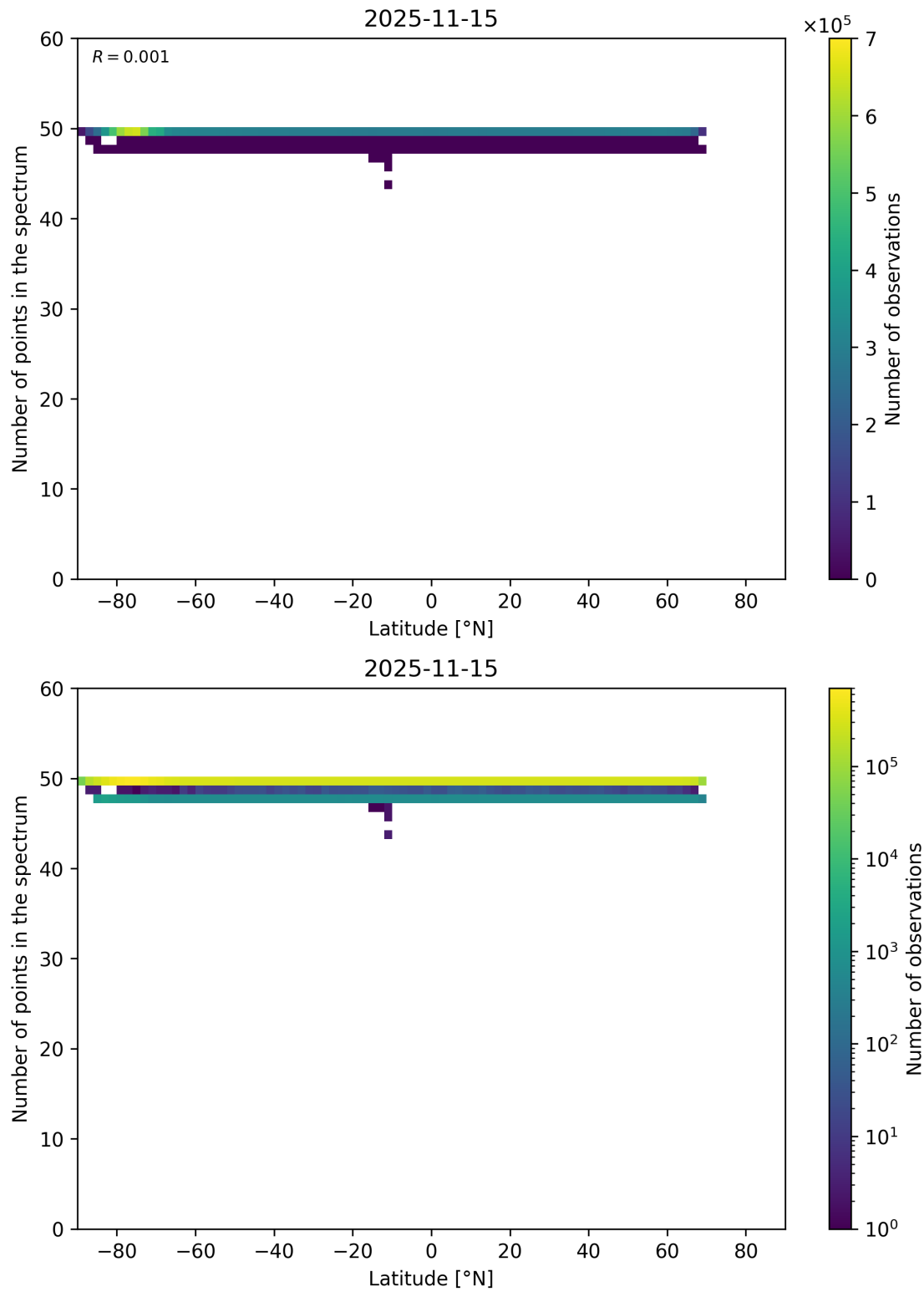
Figure 94: Scatter density plot of “Latitude” against “Number of points in the spectrum” for 2025-11-14 to 2025-11-16.
