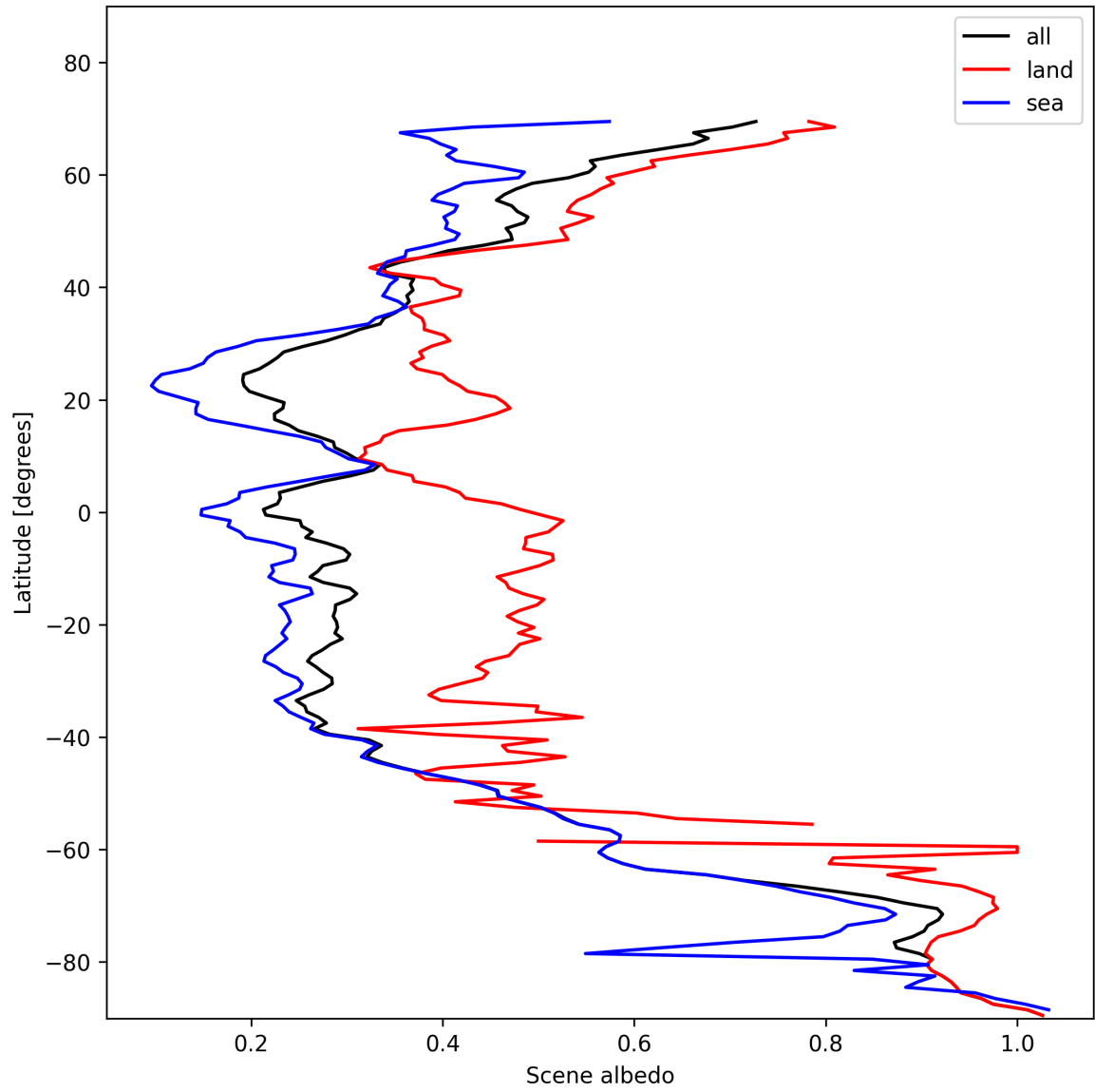
Figure 17: Zonal average of “Scene albedo” for 2025-11-14 to 2025-11-16.
