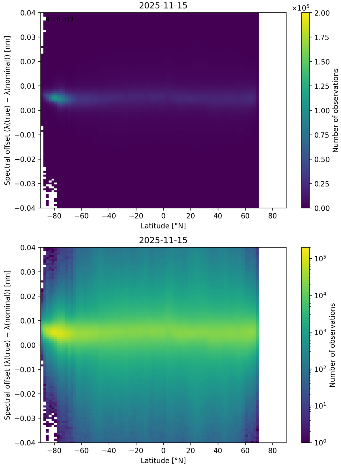
Figure 96: Scatter density plot of “Latitude” against “Spectral offset ( \lambda_{\text{true}} - \lambda_{\text{nominal}} )” for 2025-11-14 to 2025-11-16.
