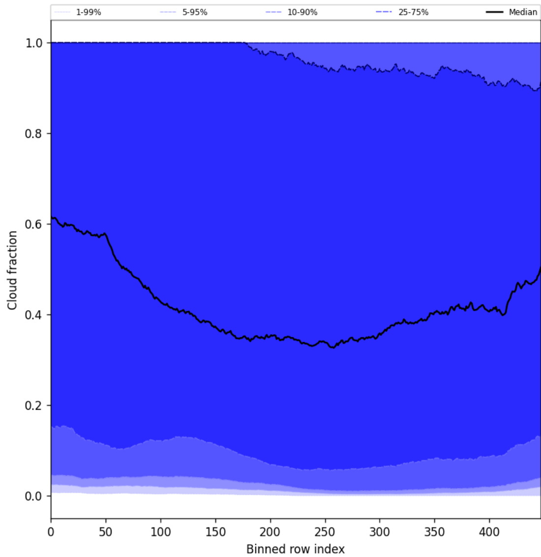
Figure 49: Along track statistics of “Cloud fraction” for 2025-11-14 to 2025-11-16
