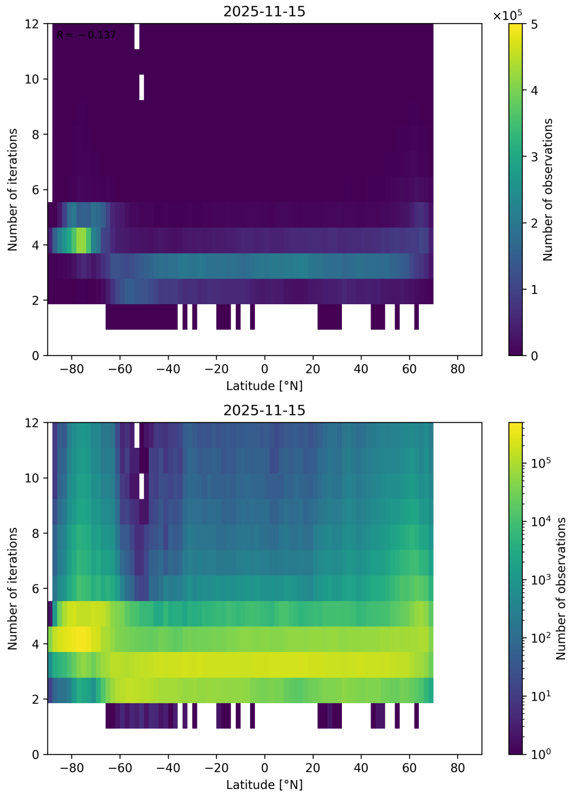
Figure 93: Scatter density plot of “Latitude” against “Number of iterations” for 2025-11-14 to 2025-11-16.
