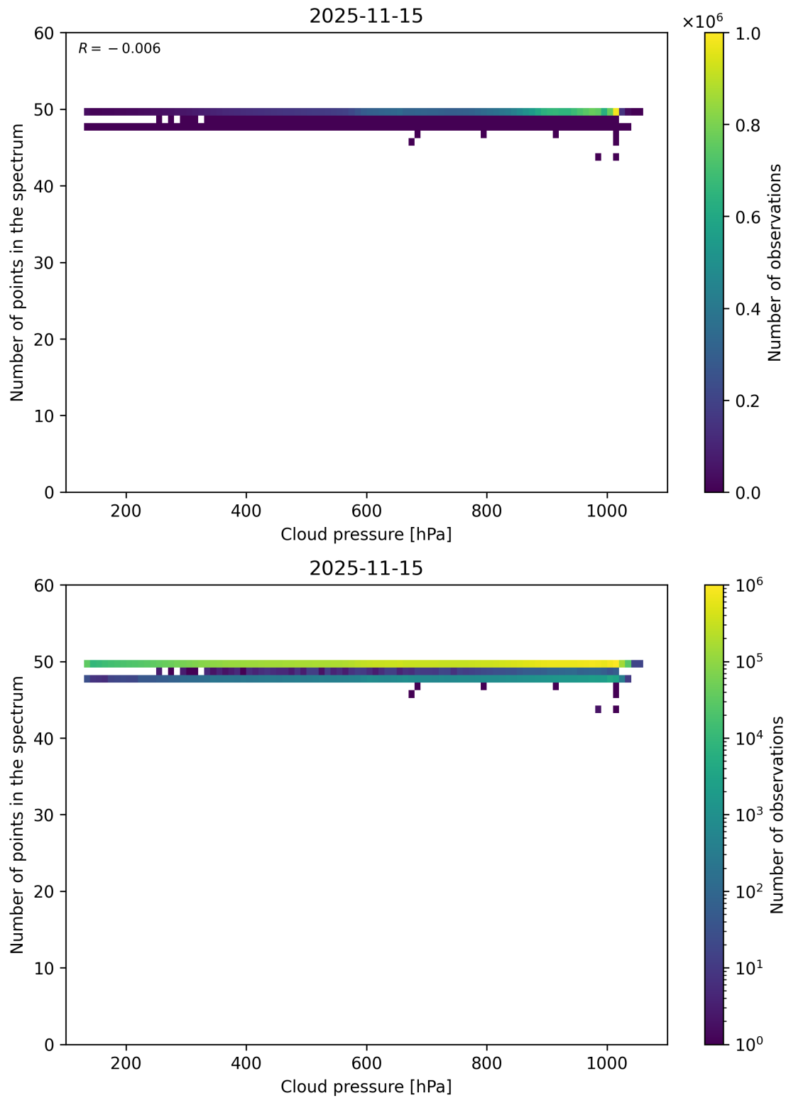
Figure 82: Scatter density plot of “Cloud pressure” against “Number of points in the spectrum” for 2025-11-14 to 2025-11-16.
