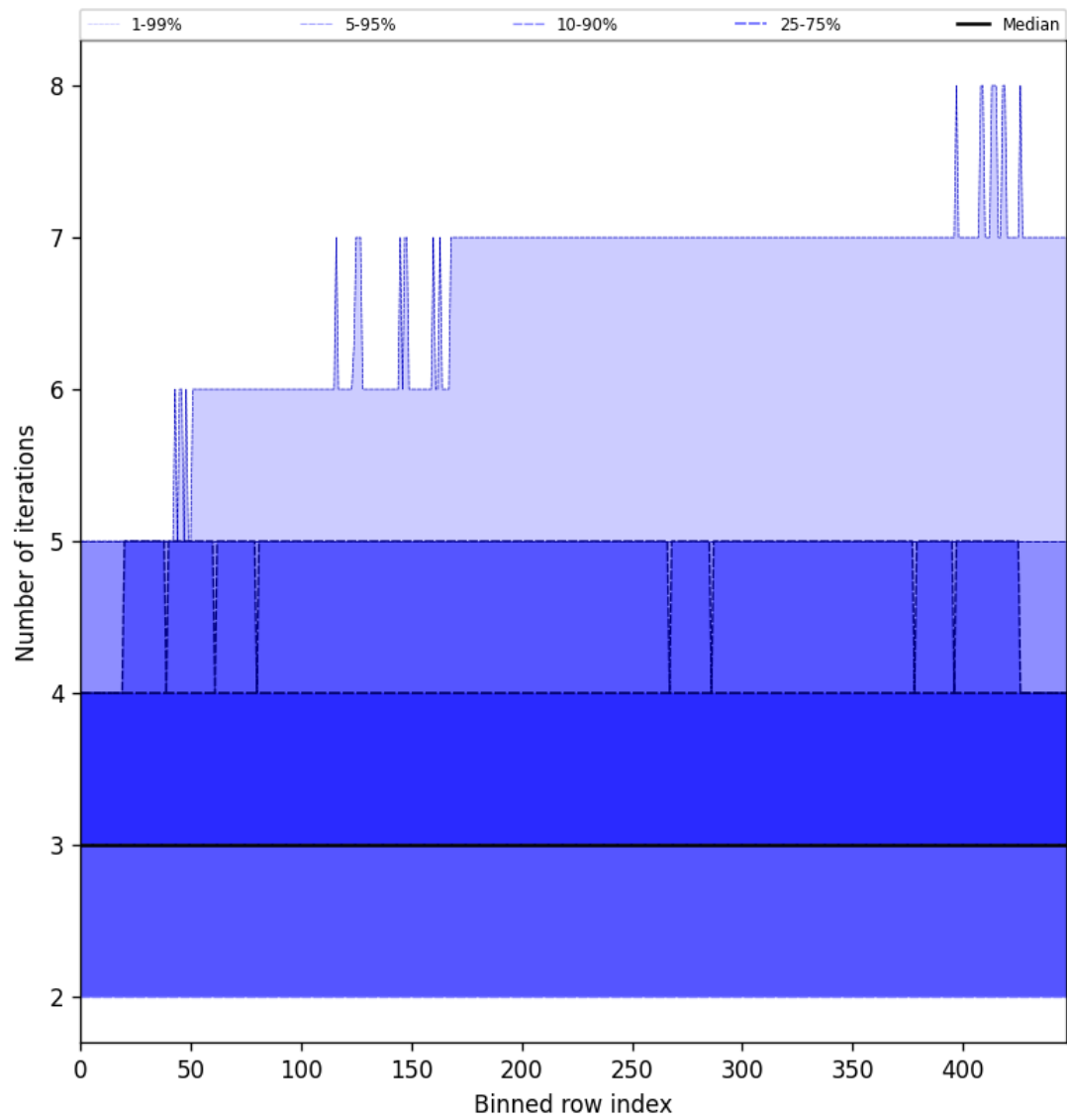
Figure 56: Along track statistics of “Number of iterations” for 2025-11-14 to 2025-11-16
