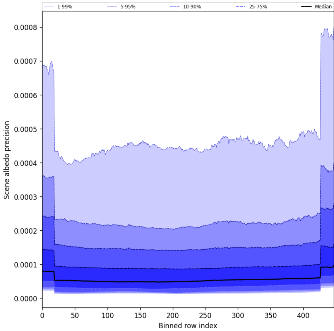
Figure 52: Along track statistics of “Scene albedo precision” for 2025-11-14 to 2025-11-16
