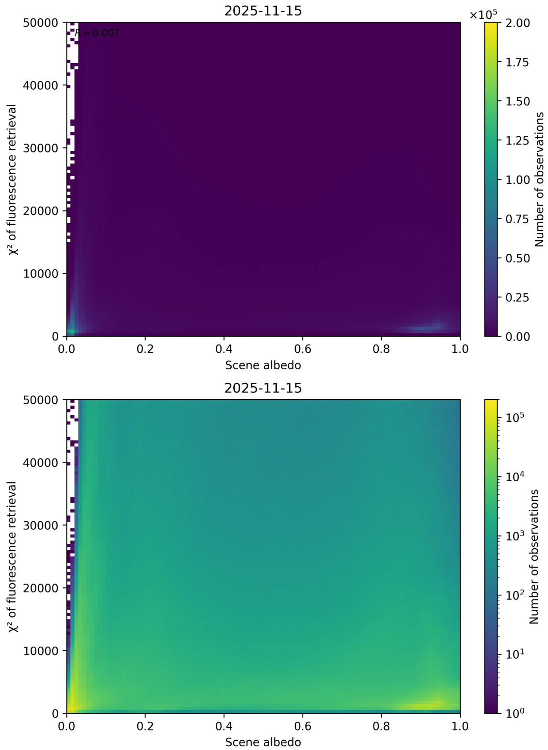
Figure 103: Scatter density plot of “Scene albedo” against “ \chi^2 of fluorescence retrieval” for 2025-11-14 to 2025-11-16.
