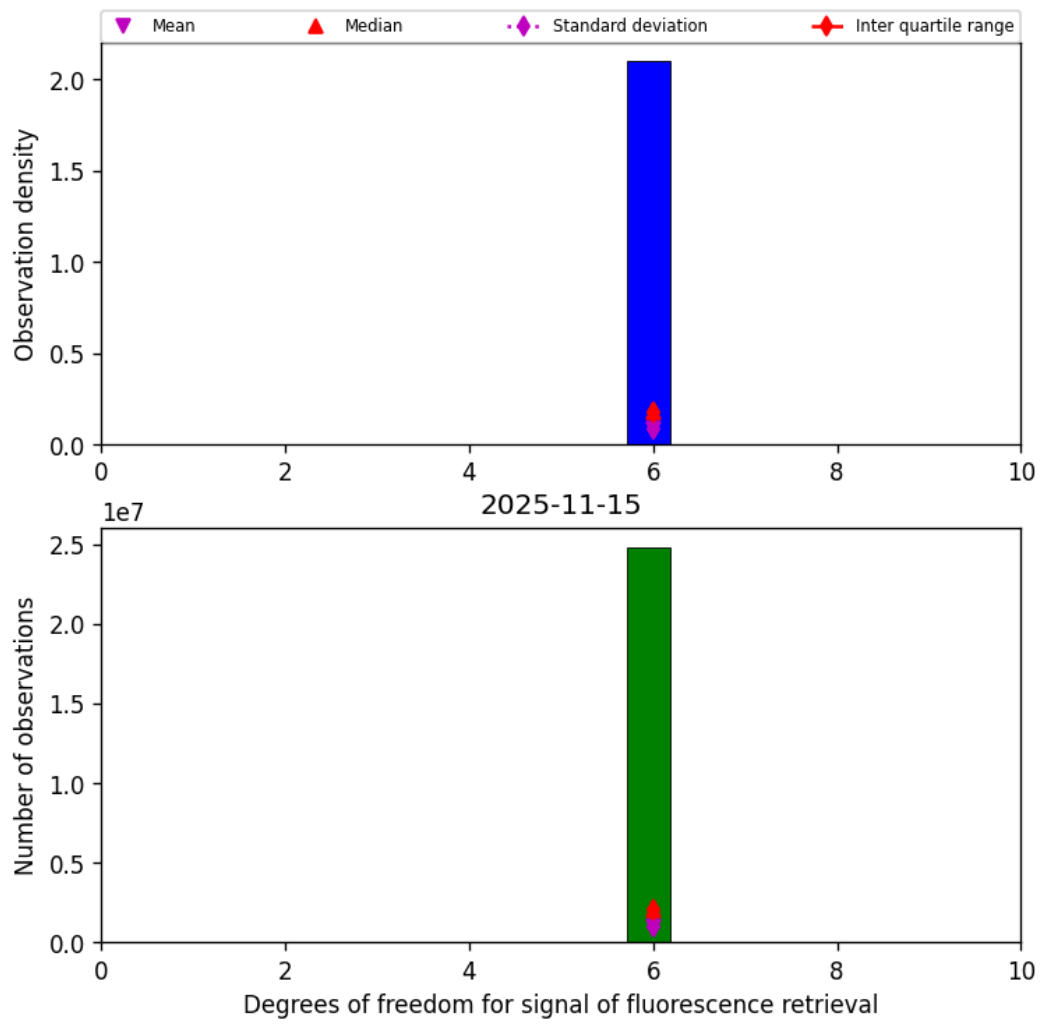
Figure 43: Histogram of "Degrees of freedom for signal of fluorescence retrieval" for 2025-11-14 to 2025-11-16
