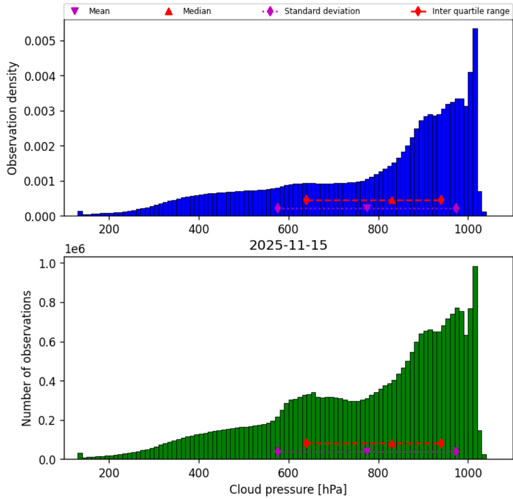
Figure 30: Histogram of “Cloud pressure” for 2025-11-14 to 2025-11-16
