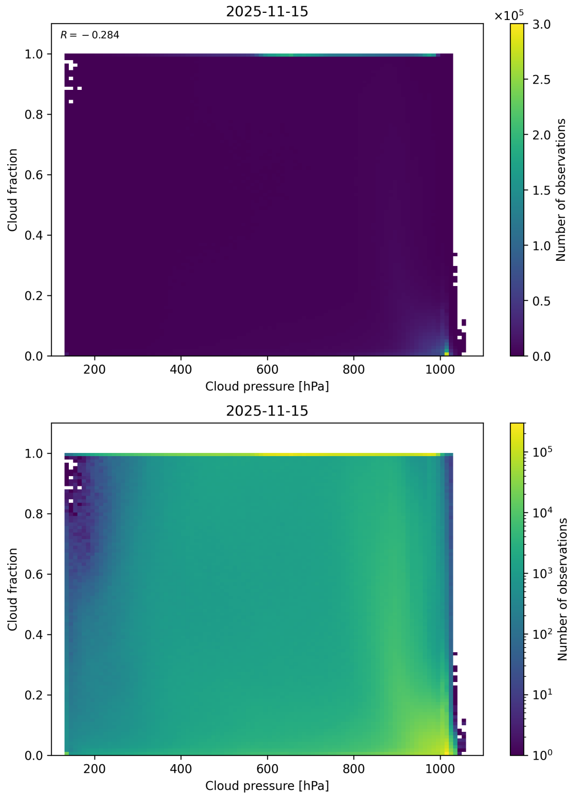
Figure 79: Scatter density plot of “Cloud pressure” against “Cloud fraction” for 2025-11-14 to 2025-11-16.
