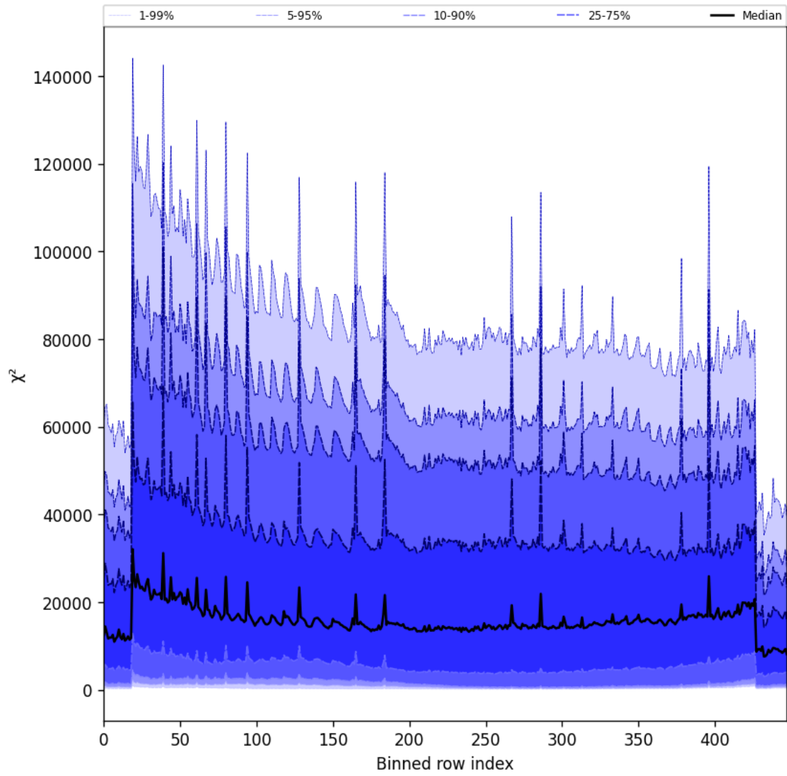
Figure 55: Along track statistics of “ \chi^2 ” for 2025-11-14 to 2025-11-16
