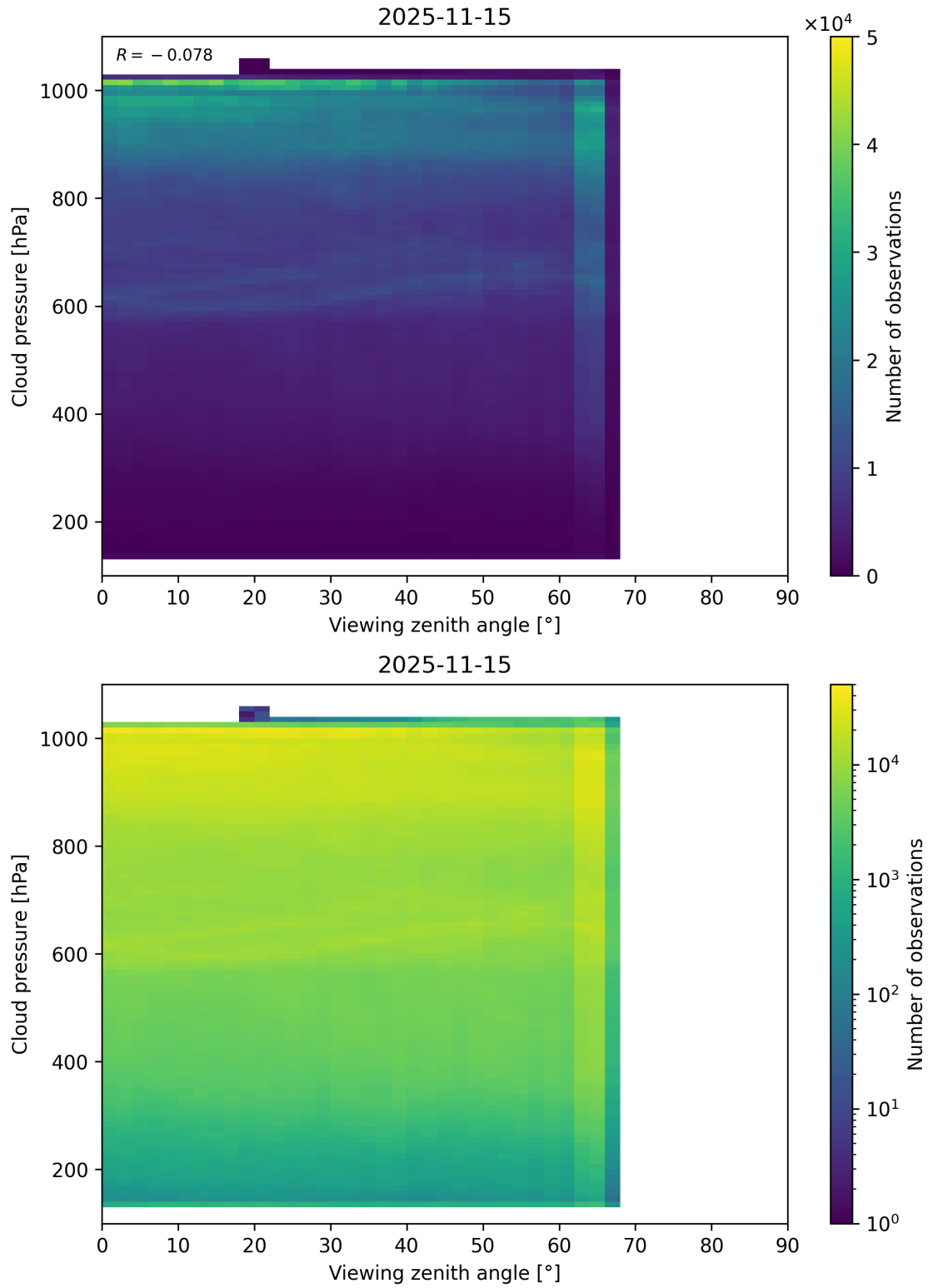
Figure 121: Scatter density plot of “Viewing zenith angle” against “Cloud pressure” for 2025-11-14 to 2025-11-16.
