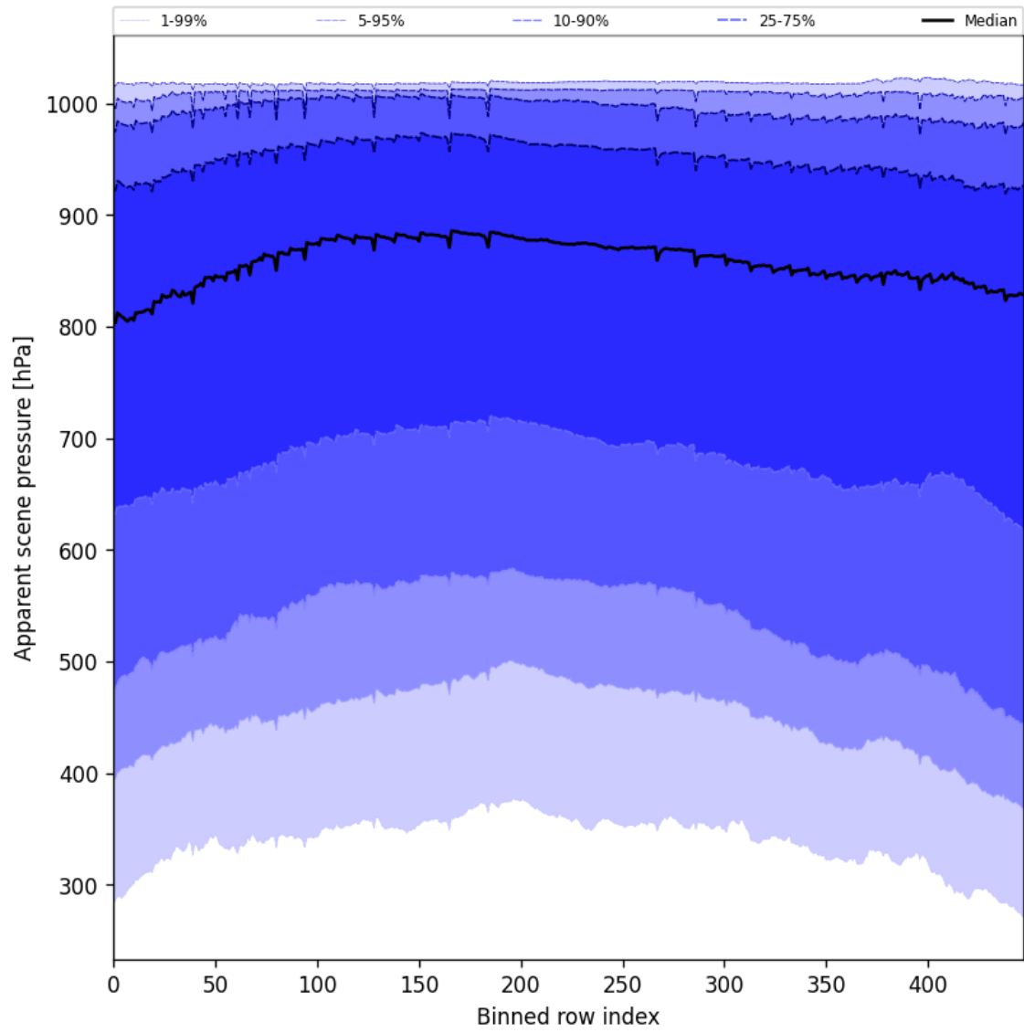
Figure 53: Along track statistics of “Apparent scene pressure” for 2025-11-14 to 2025-11-16
