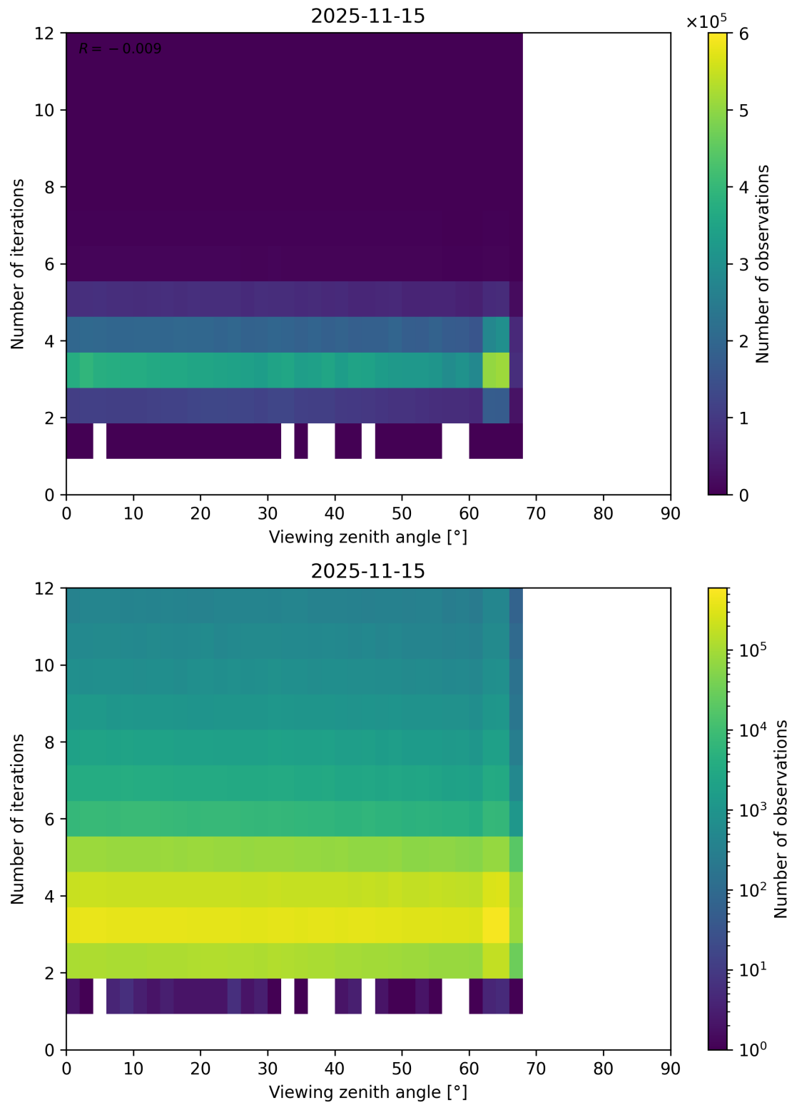
Figure 124: Scatter density plot of “Viewing zenith angle” against “Number of iterations” for 2025-11-14 to 2025-11-16.
