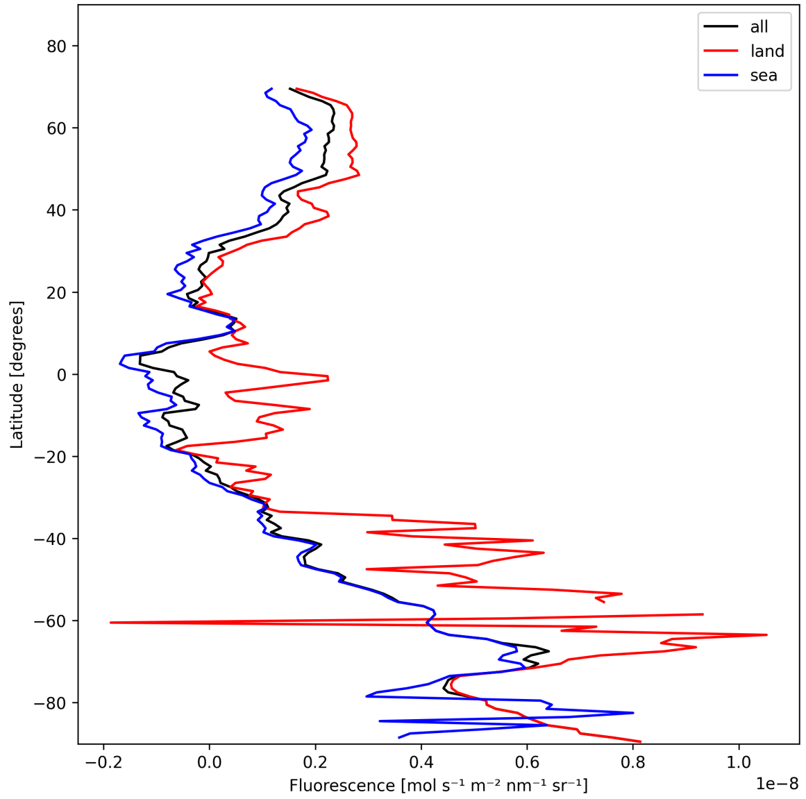
Figure 23: Zonal average of “Fluorescence” for 2025-11-14 to 2025-11-16.
