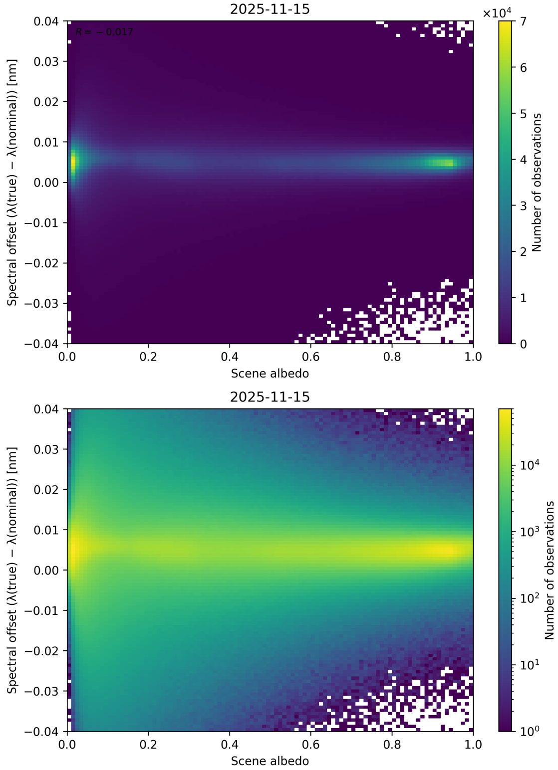
Figure 107: Scatter density plot of “Scene albedo” against “Spectral offset ( \lambda_{\text{true}} - \lambda_{\text{nominal}} )” for 2025-11-14 to 2025-11-16.
