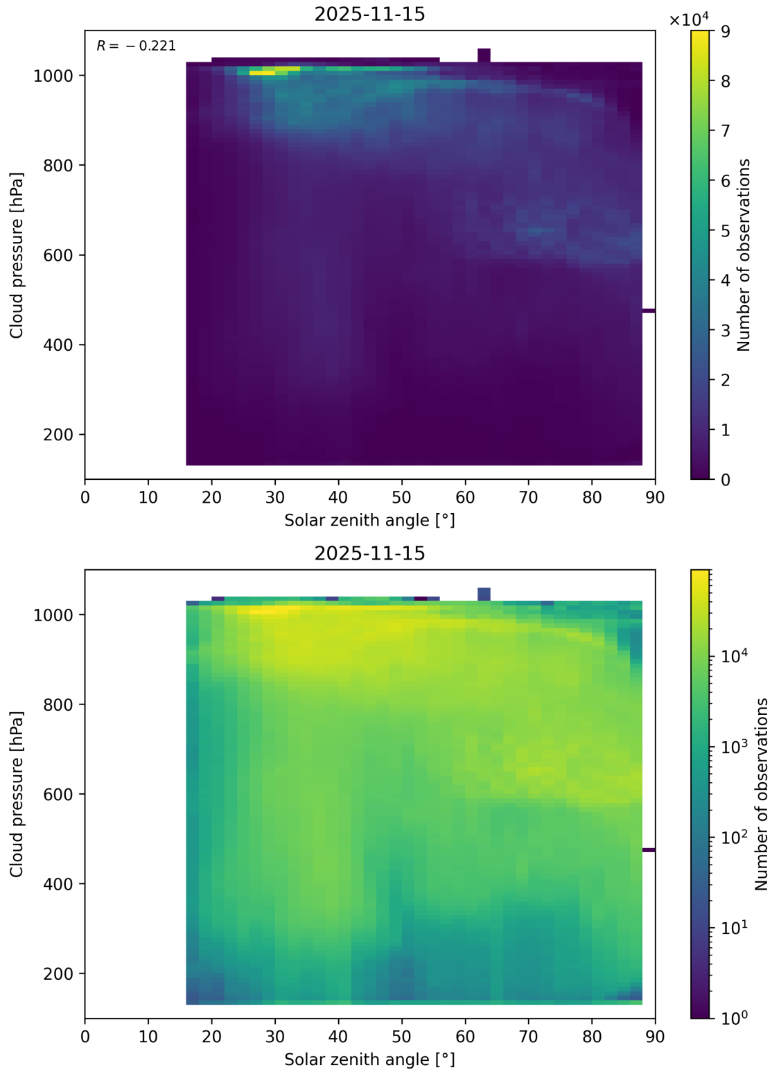
Figure 111: Scatter density plot of “Solar zenith angle” against “Cloud pressure” for 2025-11-14 to 2025-11-16.
