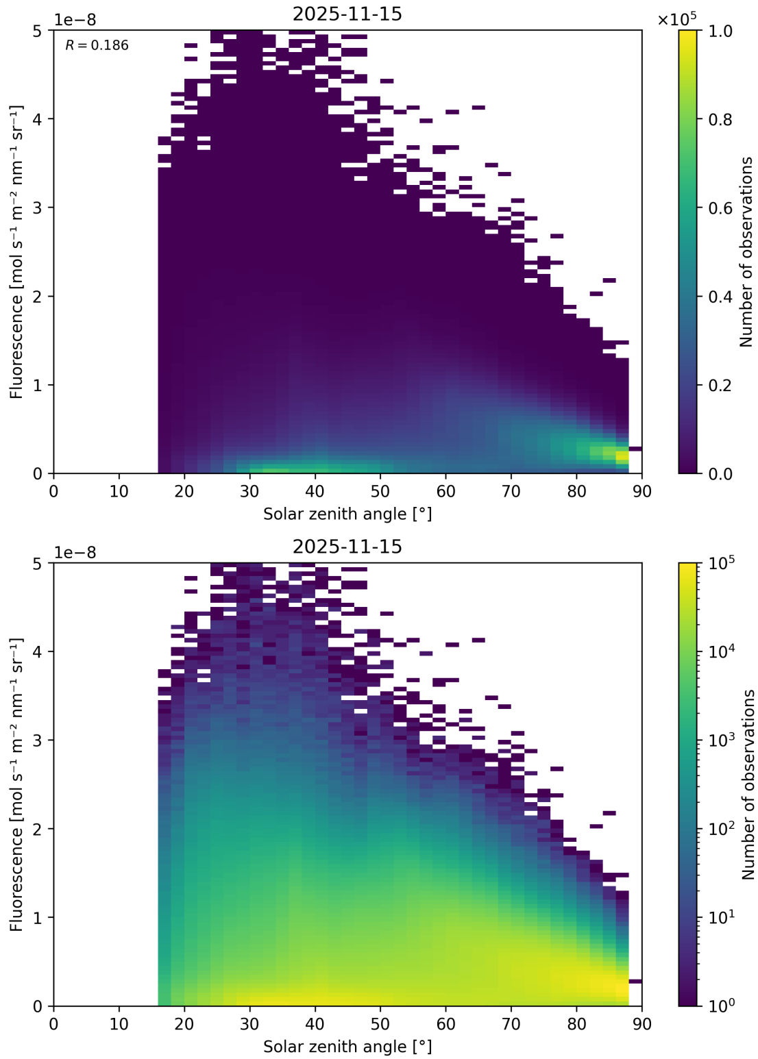
Figure 112: Scatter density plot of “Solar zenith angle” against “Fluorescence” for 2025-11-14 to 2025-11-16.
