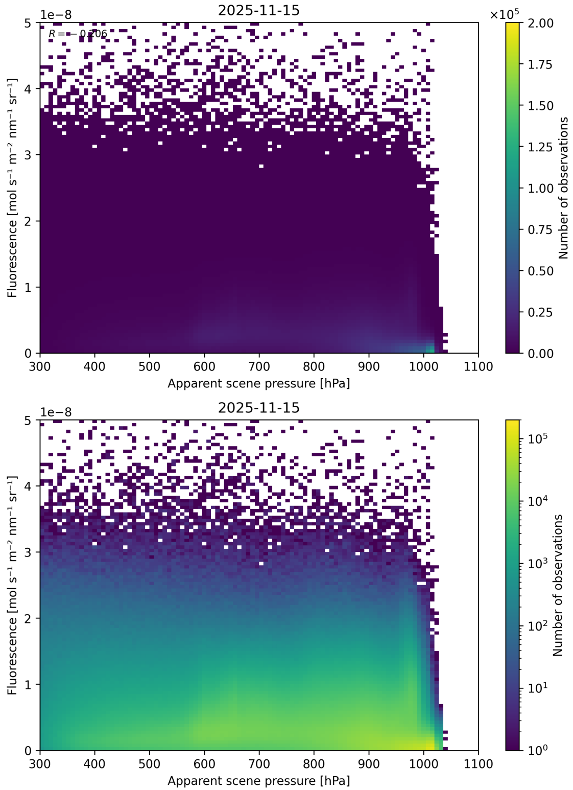
Figure 64: Scatter density plot of “Apparent scene pressure” against “Fluorescence” for 2025-11-14 to 2025-11-16.
