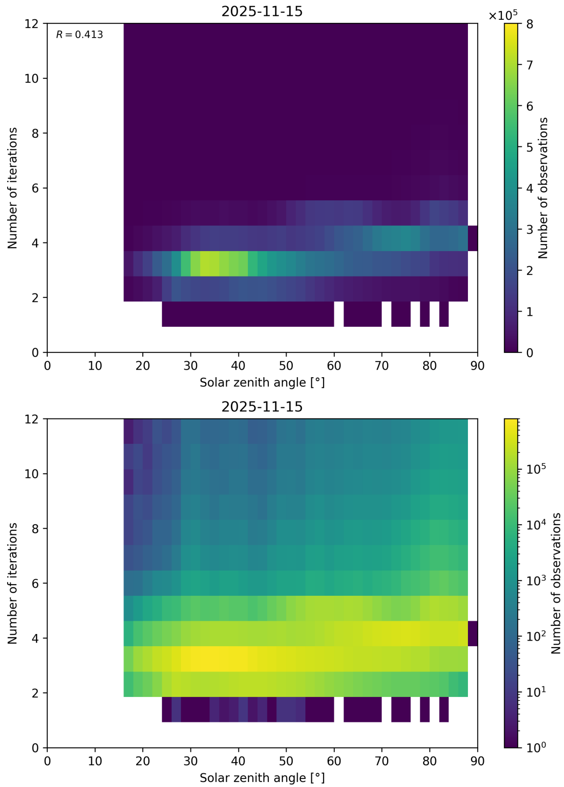
Figure 114: Scatter density plot of “Solar zenith angle” against “Number of iterations” for 2025-11-14 to 2025-11-16.
