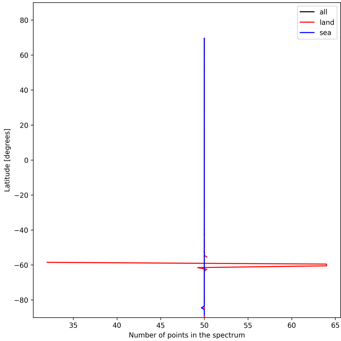
Figure 27: Zonal average of “Number of points in the spectrum” for 2025-11-14 to 2025-11-16.
