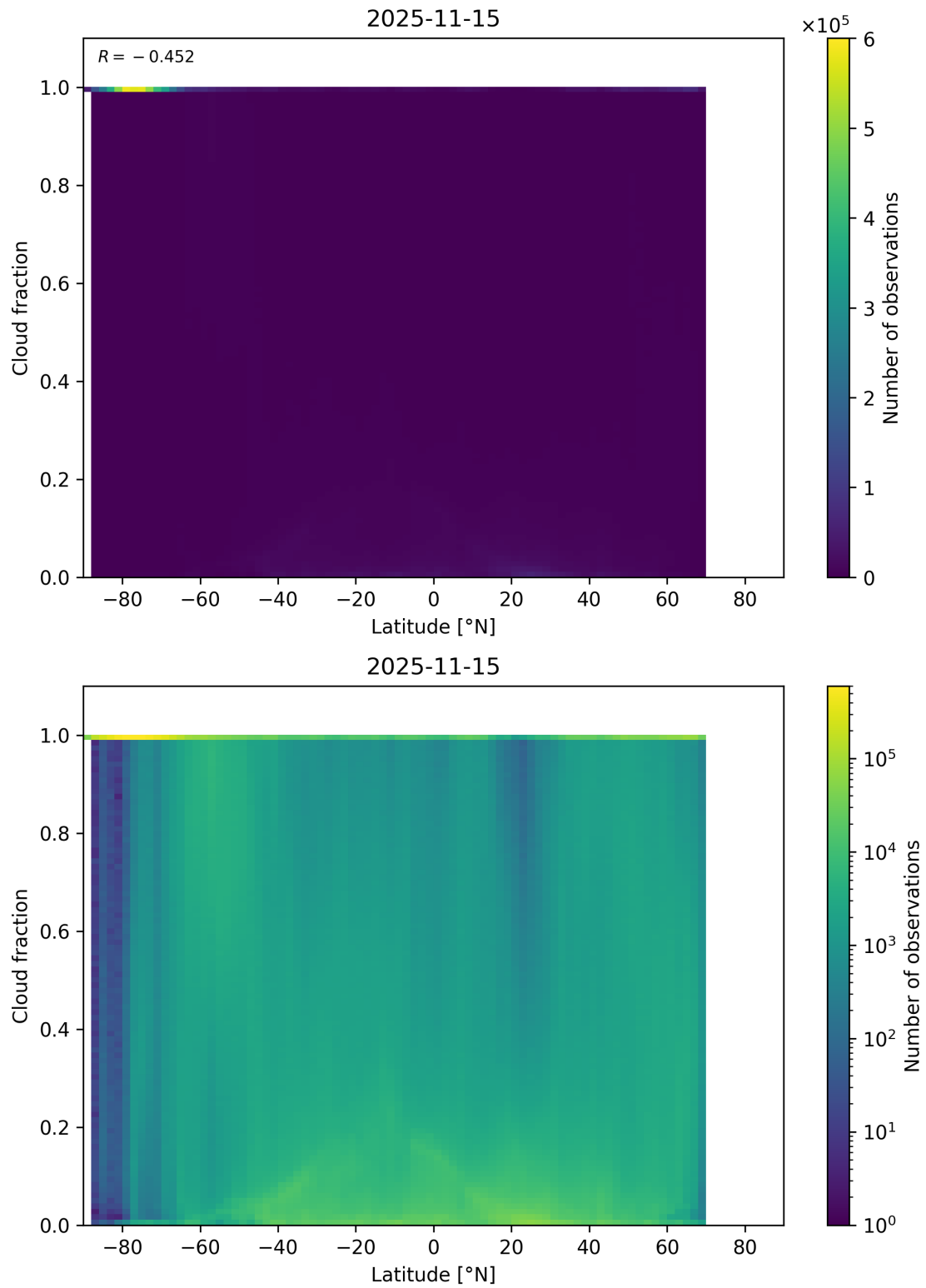
Figure 90: Scatter density plot of “Latitude” against “Cloud fraction” for 2025-11-14 to 2025-11-16.
