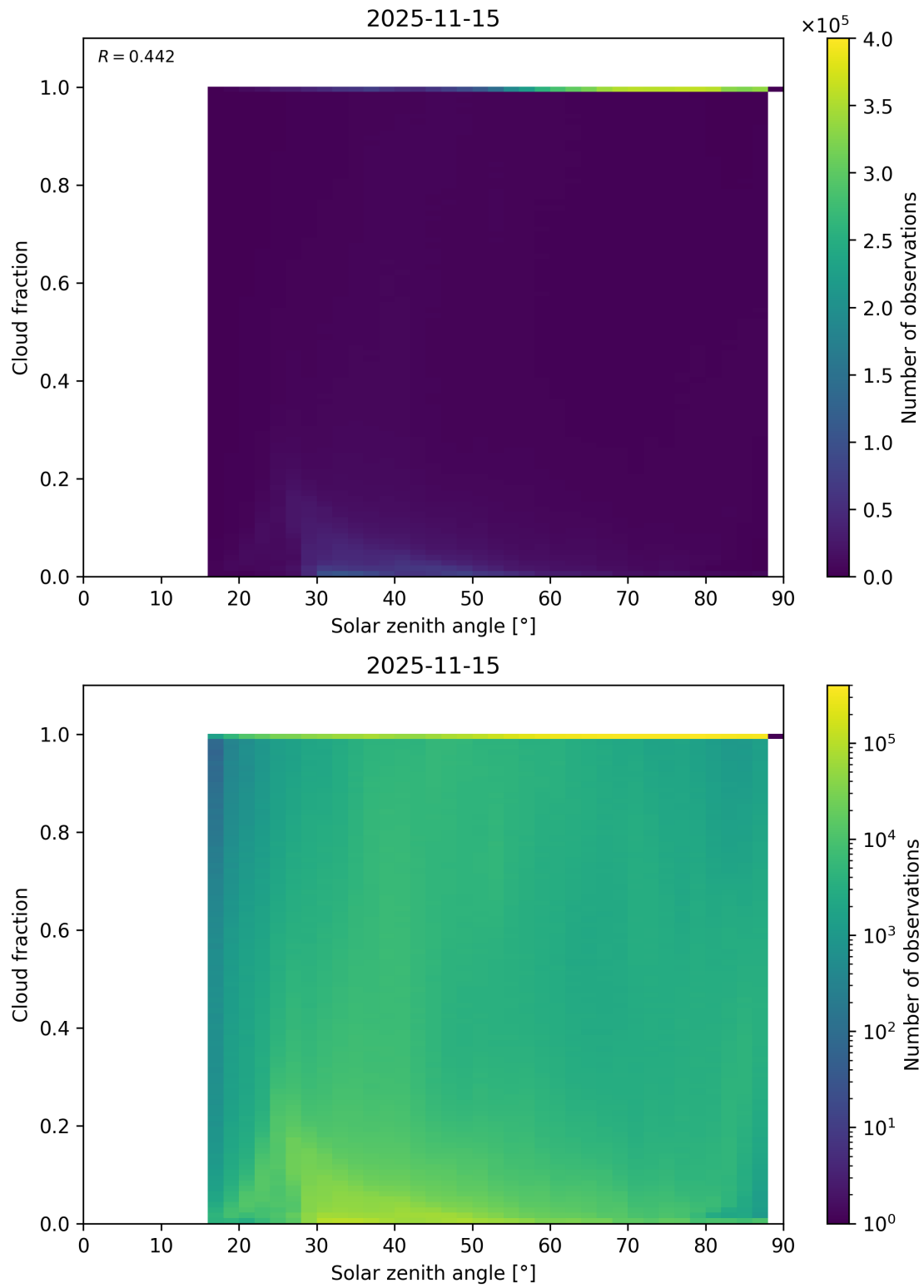
Figure 110: Scatter density plot of “Solar zenith angle” against “Cloud fraction” for 2025-11-14 to 2025-11-16.
