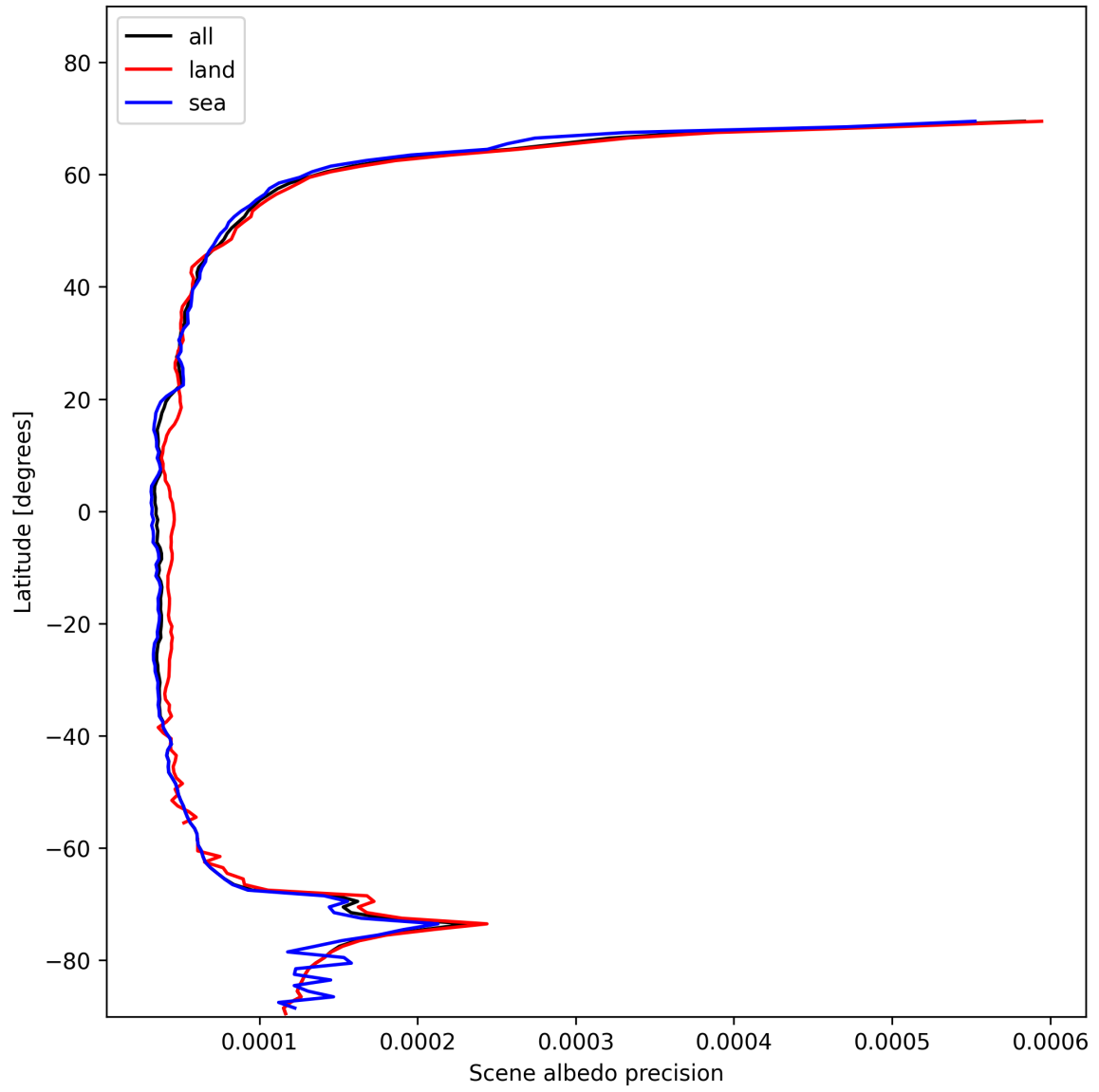
Figure 18: Zonal average of “Scene albedo precision” for 2025-11-14 to 2025-11-16.
