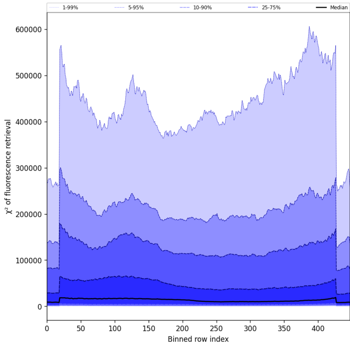
Figure 59: Along track statistics of “ \chi^2 of fluorescence retrieval” for 2025-11-14 to 2025-11-16
