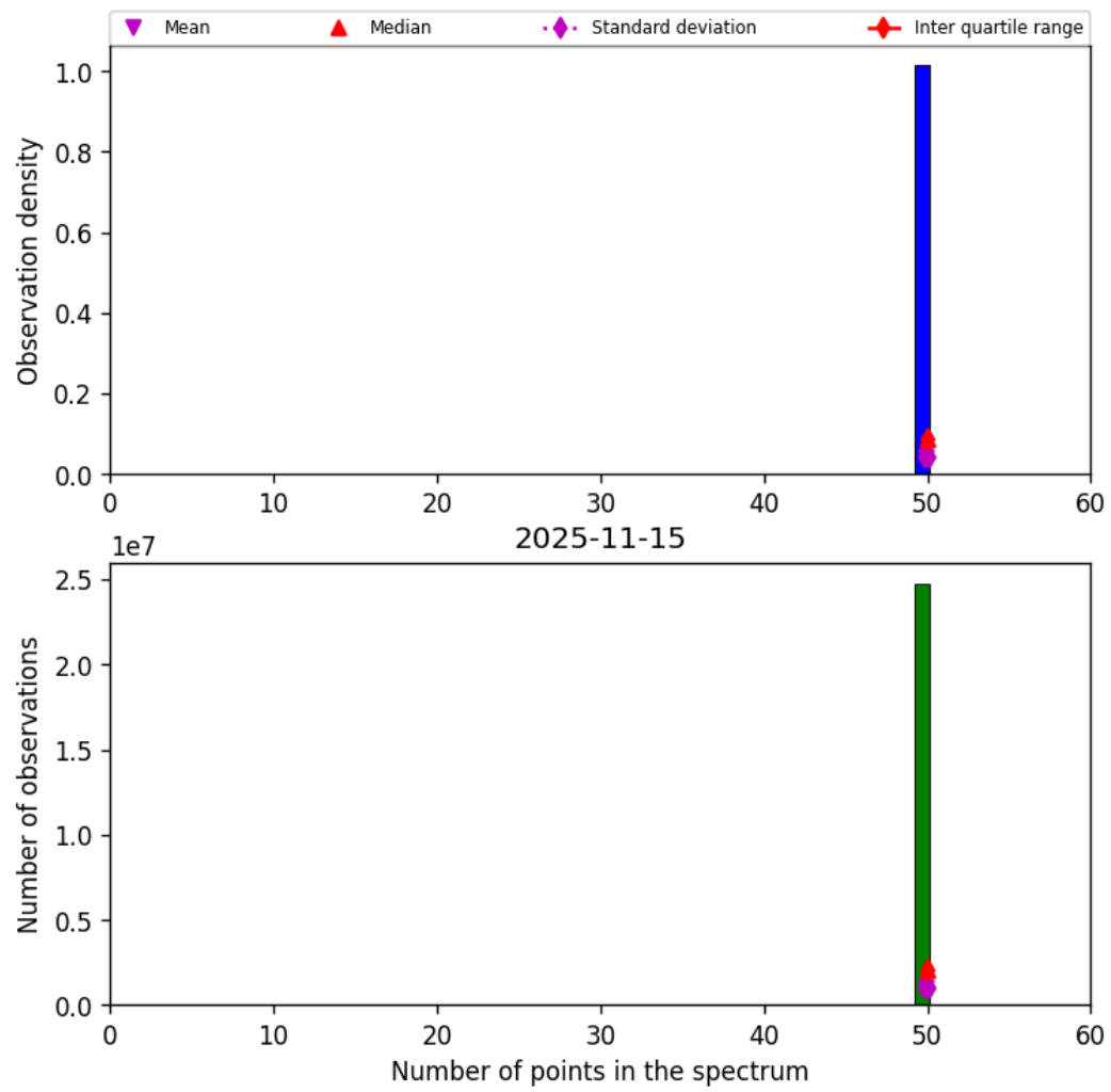
Figure 44: Histogram of “Number of points in the spectrum” for 2025-11-14 to 2025-11-16
