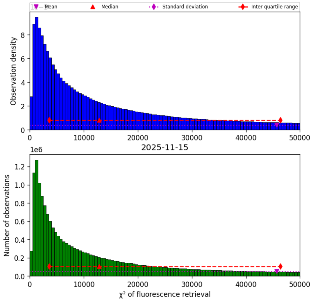
Figure 42: Histogram of “ \chi^2 of fluorescence retrieval” for 2025-11-14 to 2025-11-16
