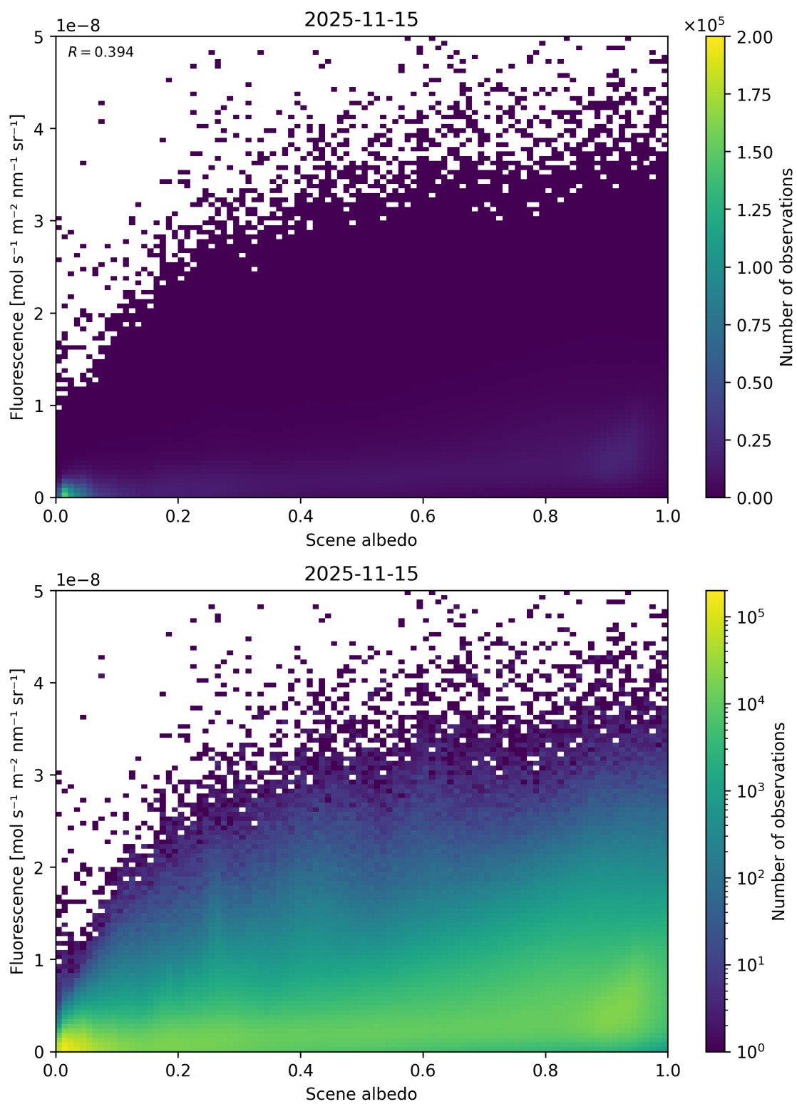
Figure 104: Scatter density plot of “Scene albedo” against “Fluorescence” for 2025-11-14 to 2025-11-16.
