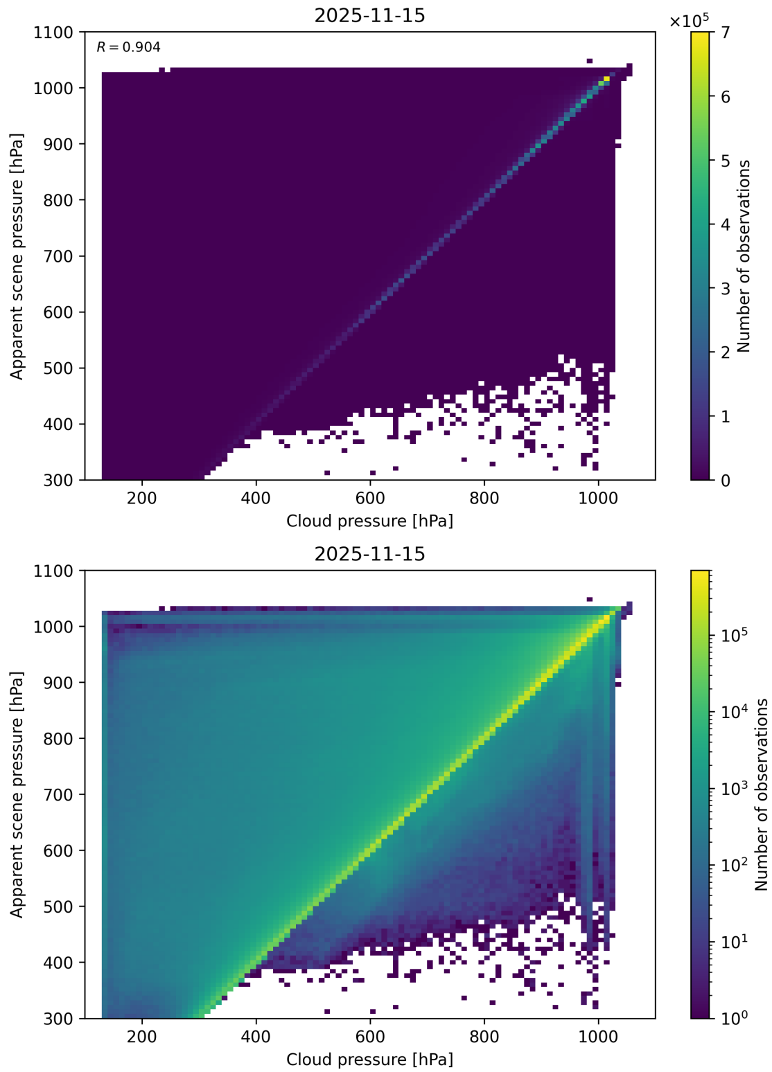
Figure 77: Scatter density plot of “Cloud pressure” against “Apparent scene pressure” for 2025-11-14 to 2025-11-16.
