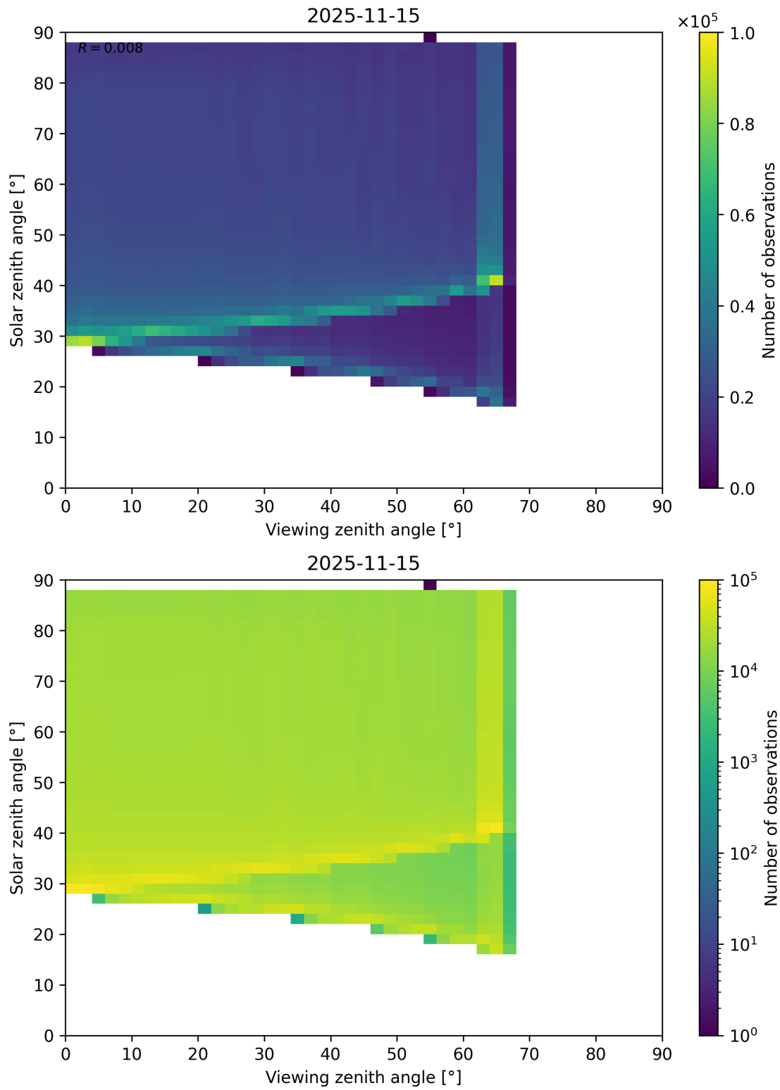
Figure 127: Scatter density plot of “Viewing zenith angle” against “Solar zenith angle” for 2025-11-14 to 2025-11-16.
