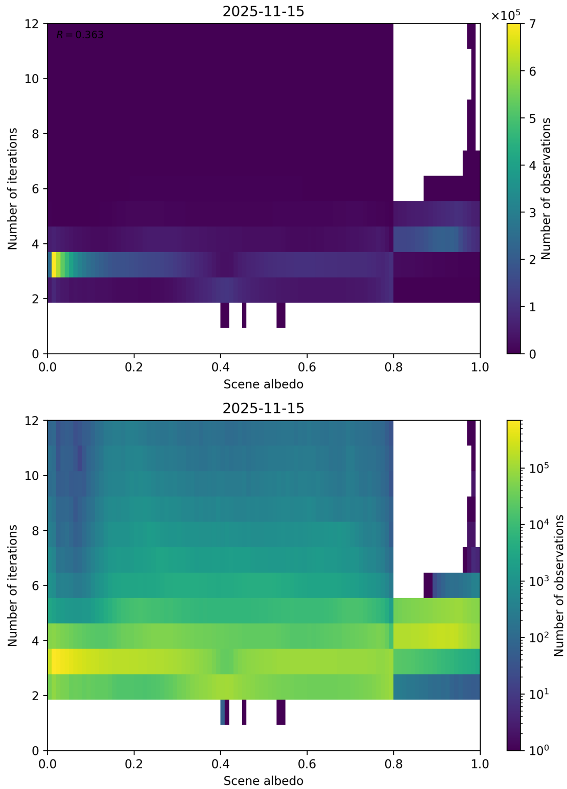
Figure 105: Scatter density plot of “Scene albedo” against “Number of iterations” for 2025-11-14 to 2025-11-16.
