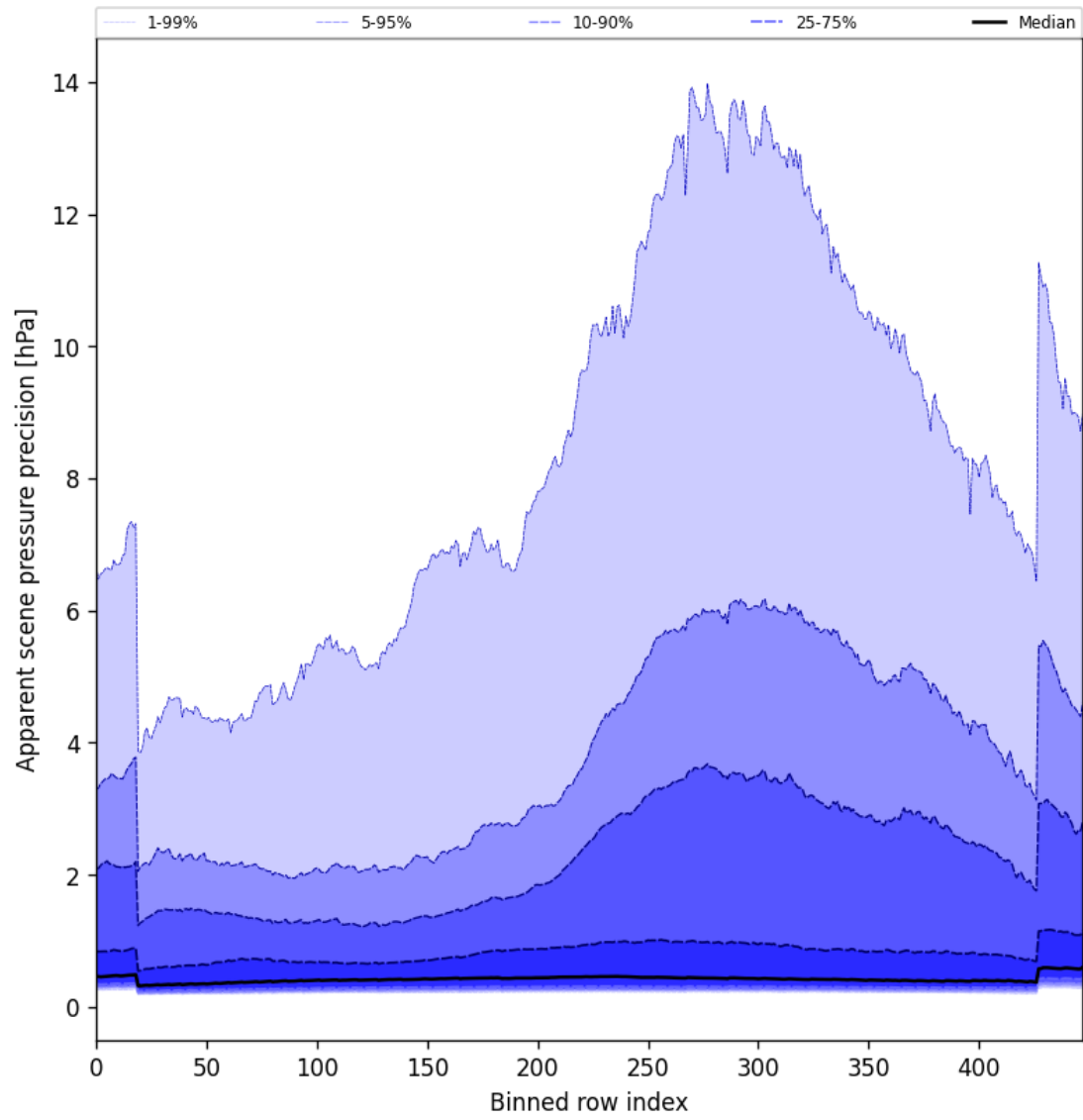
Figure 54: Along track statistics of “Apparent scene pressure precision” for 2025-11-14 to 2025-11-16
