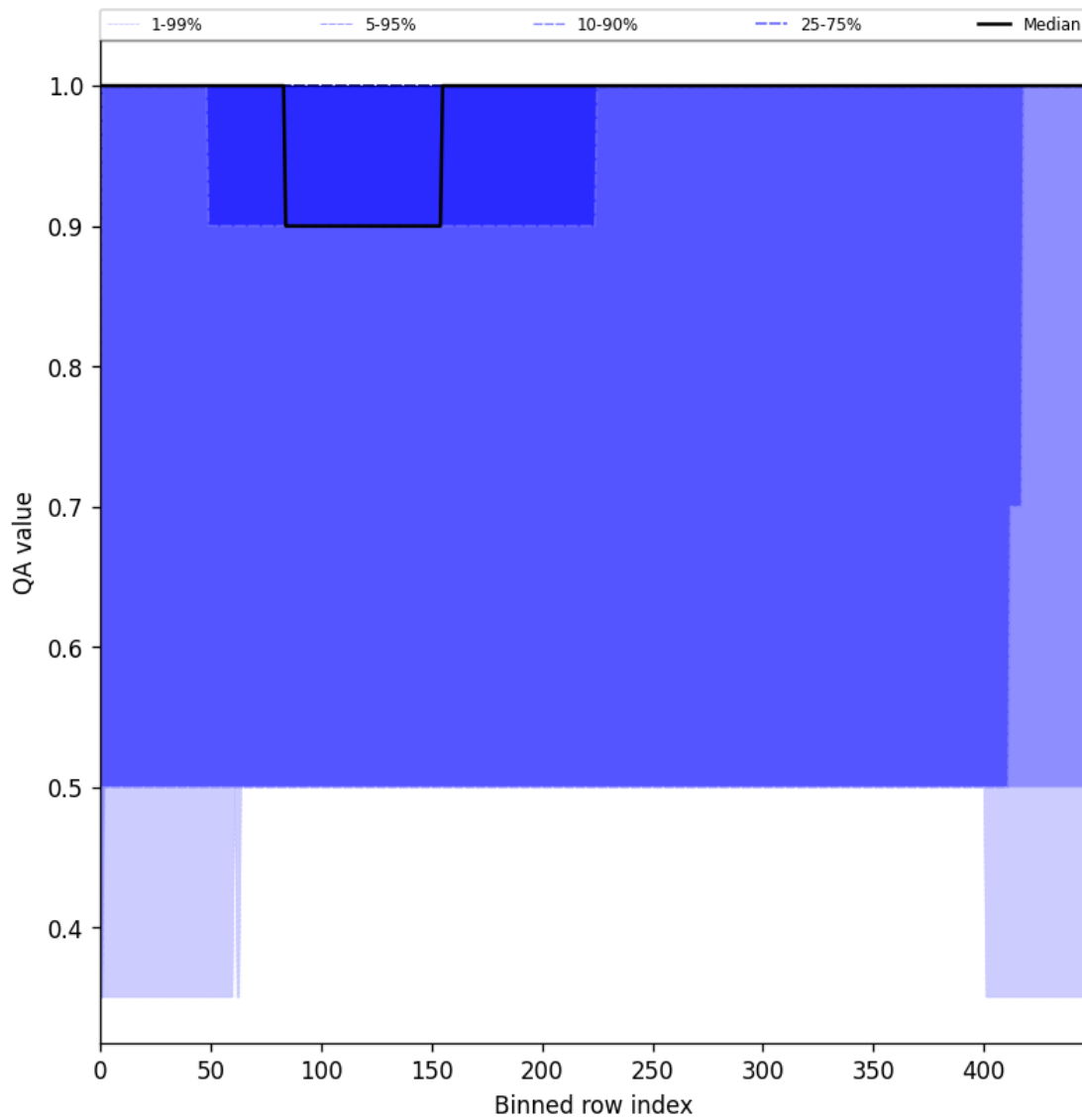
Figure 46: Along track statistics of “QA value” for 2025-11-14 to 2025-11-16
