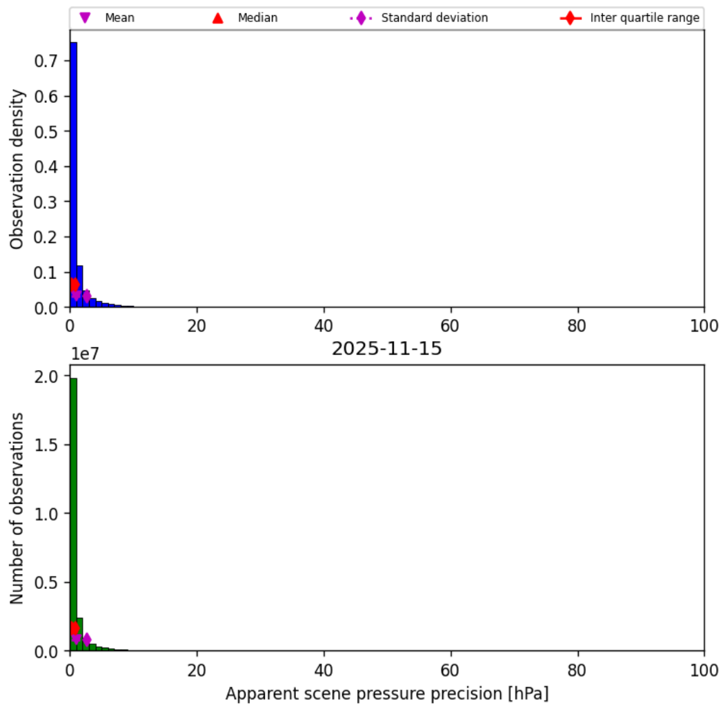
Figure 37: Histogram of “Apparent scene pressure precision” for 2025-11-14 to 2025-11-16
