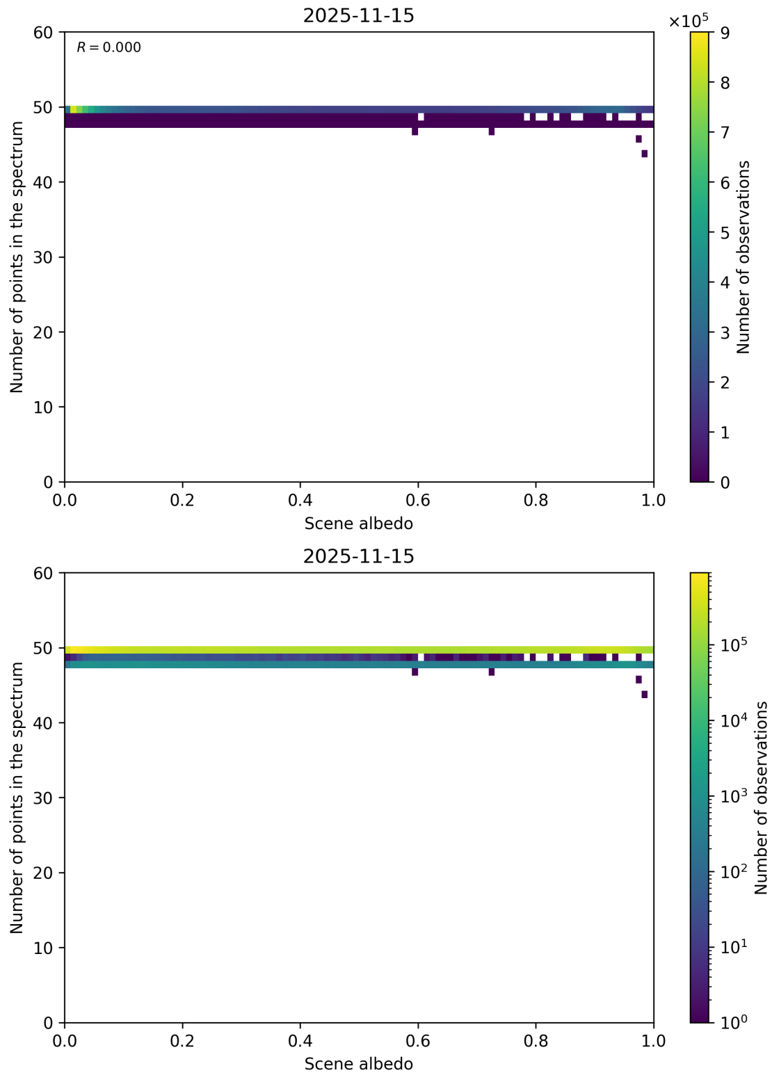
Figure 106: Scatter density plot of “Scene albedo” against “Number of points in the spectrum” for 2025-11-14 to 2025-11-16.
