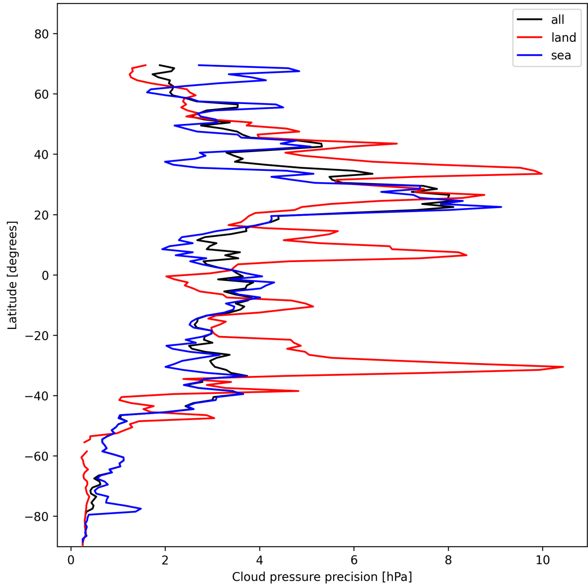
Figure 14: Zonal average of “Cloud pressure precision” for 2025-11-14 to 2025-11-16.
