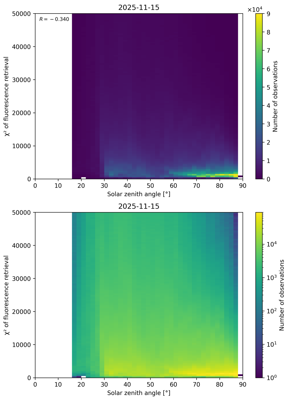
Figure 109: Scatter density plot of “Solar zenith angle” against “ \chi^2 of fluorescence retrieval” for 2025-11-14 to 2025-11-16.
