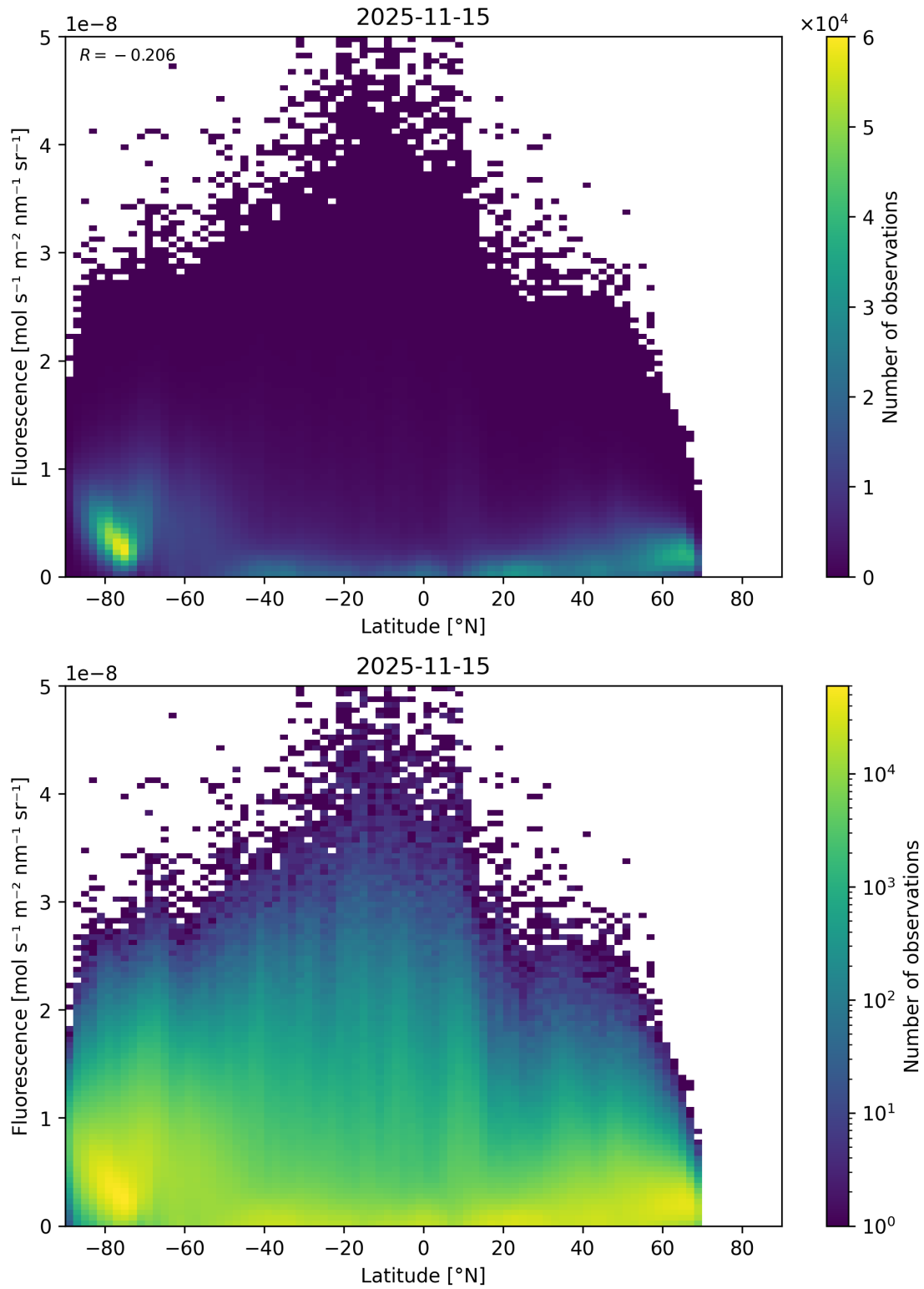
Figure 92: Scatter density plot of “Latitude” against “Fluorescence” for 2025-11-14 to 2025-11-16.
