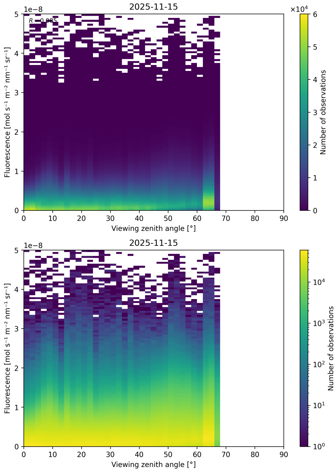
Figure 122: Scatter density plot of “Viewing zenith angle” against “Fluorescence” for 2025-11-14 to 2025-11-16.
