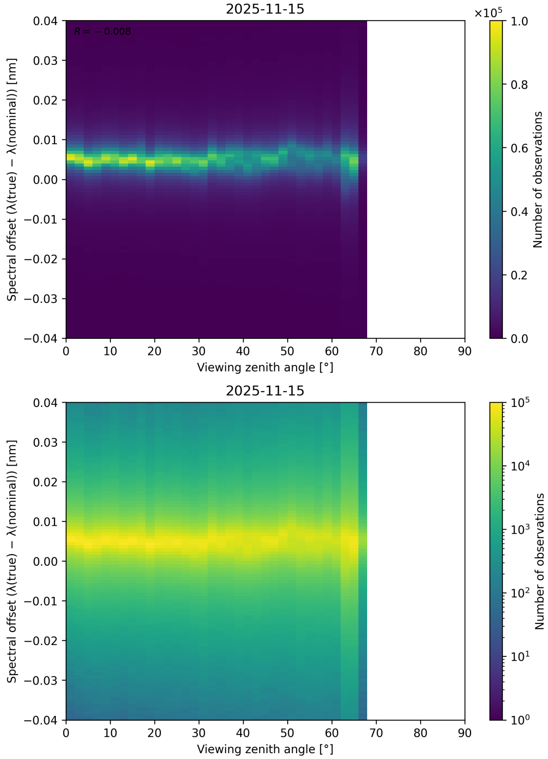
Figure 128: Scatter density plot of “Viewing zenith angle” against “Spectral offset ( \lambda_{\text{true}} - \lambda_{\text{nominal}} )” for 2025-11-14 to 2025-11-16.
