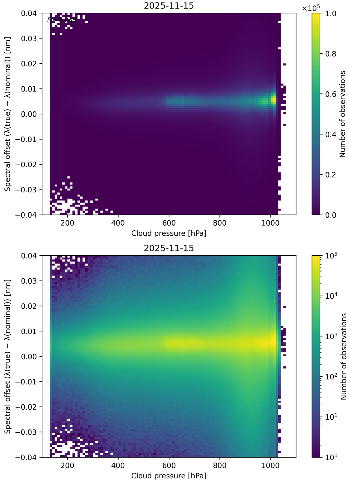
Figure 84: Scatter density plot of “Cloud pressure” against “Spectral offset ( \lambda_{\text{true}} - \lambda_{\text{nominal}} )” for 2025-11-14 to 2025-11-16.
