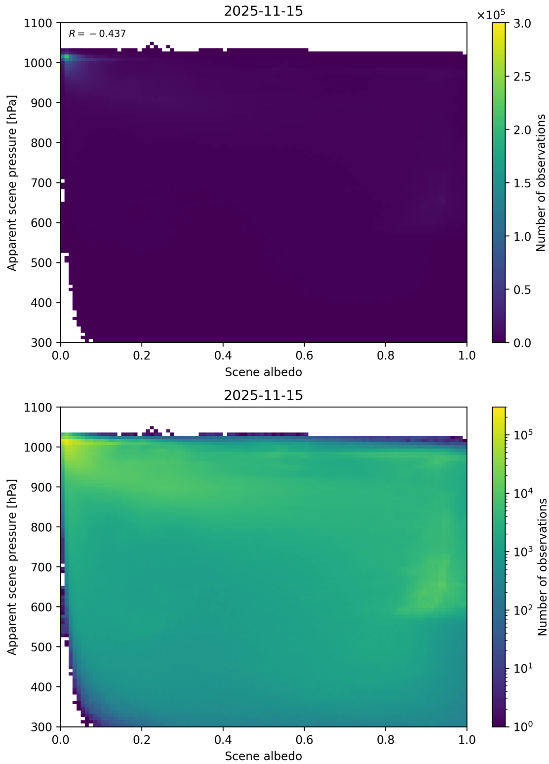
Figure 102: Scatter density plot of “Scene albedo” against “Apparent scene pressure” for 2025-11-14 to 2025-11-16.
