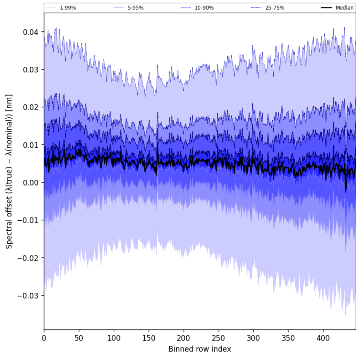
Figure 62: Along track statistics of “Spectral offset ( \lambda_{\text{true}} - \lambda_{\text{nominal}} )” for 2025-11-14 to 2025-11-16
