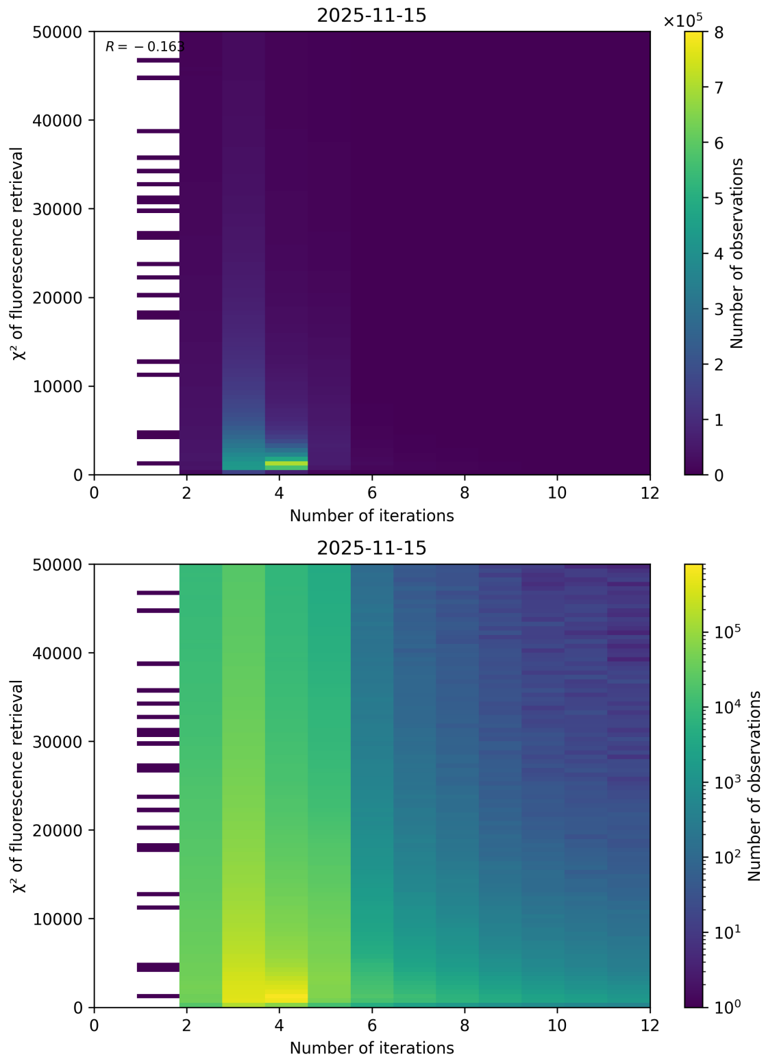
Figure 97: Scatter density plot of “Number of iterations” against “ \chi^2 of fluorescence retrieval” for 2025-11-14 to 2025-11-16.
