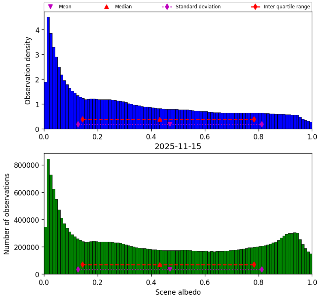
Figure 34: Histogram of “Scene albedo” for 2025-11-14 to 2025-11-16
