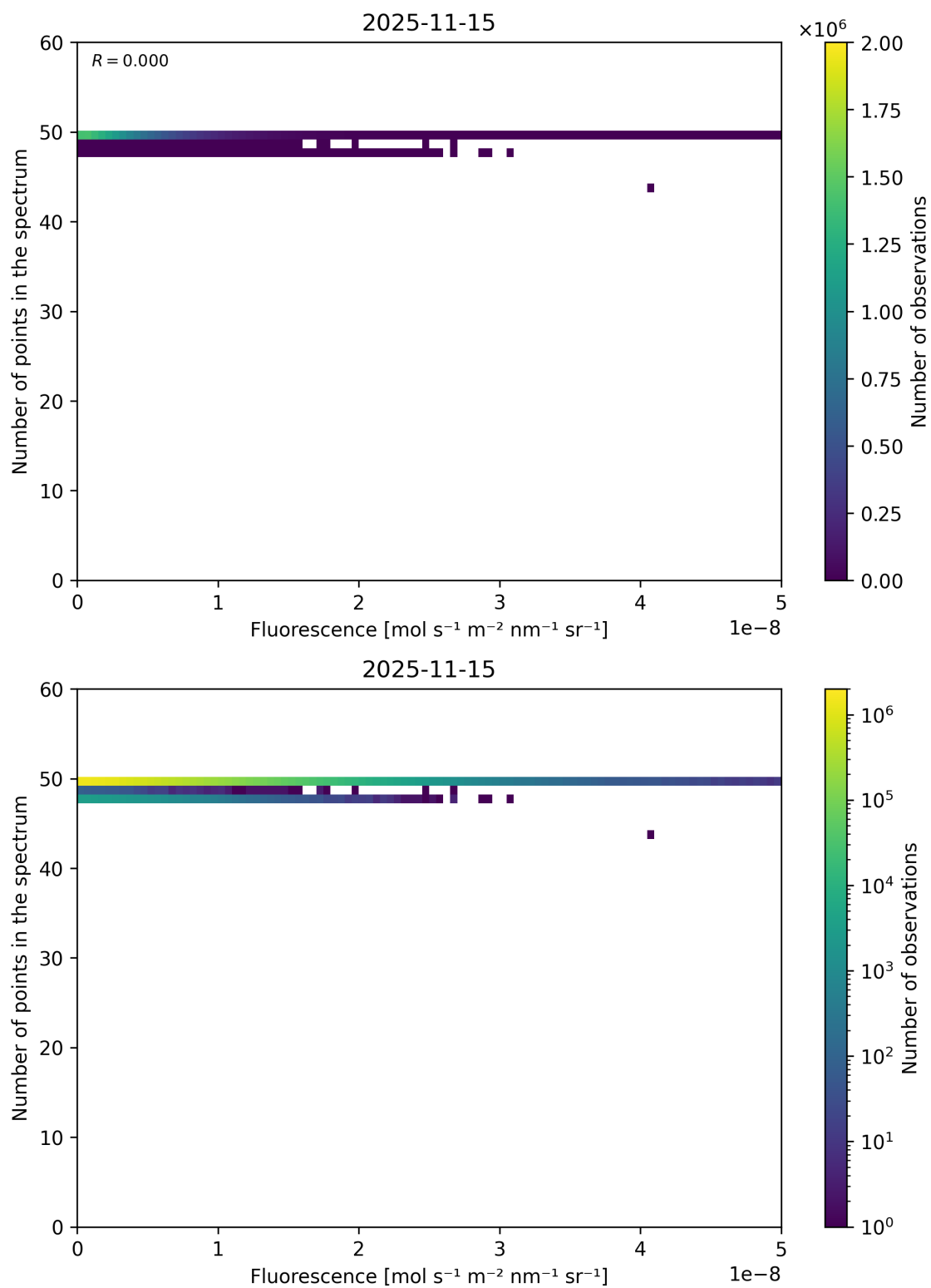
Figure 86: Scatter density plot of “Fluorescence” against “Number of points in the spectrum” for 2025-11-14 to 2025-11-16.
