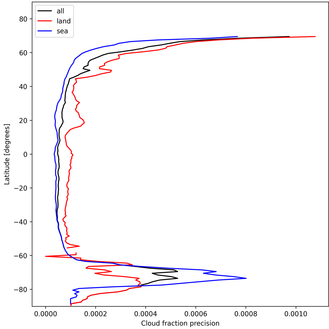
Figure 16: Zonal average of “Cloud fraction precision” for 2025-11-14 to 2025-11-16.
