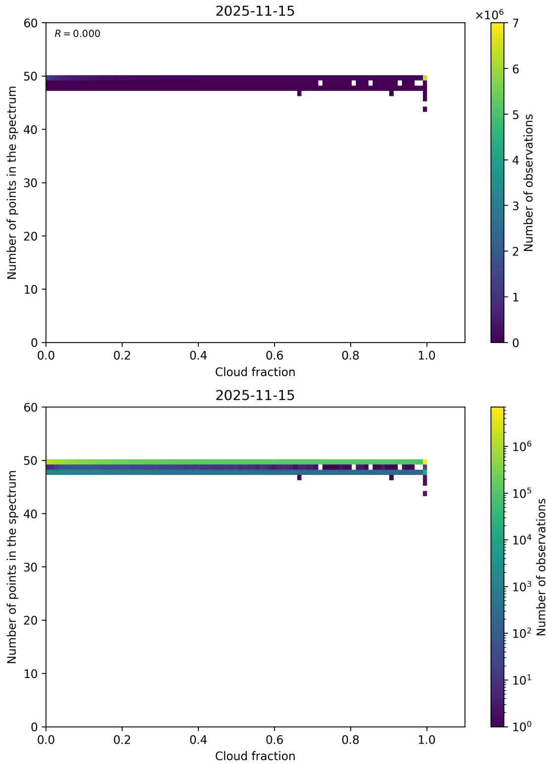
Figure 74: Scatter density plot of “Cloud fraction” against “Number of points in the spectrum” for 2025-11-14 to 2025-11-16.
