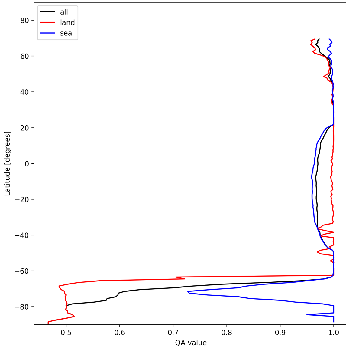
Figure 12: Zonal average of “QA value” for 2025-11-14 to 2025-11-16.
