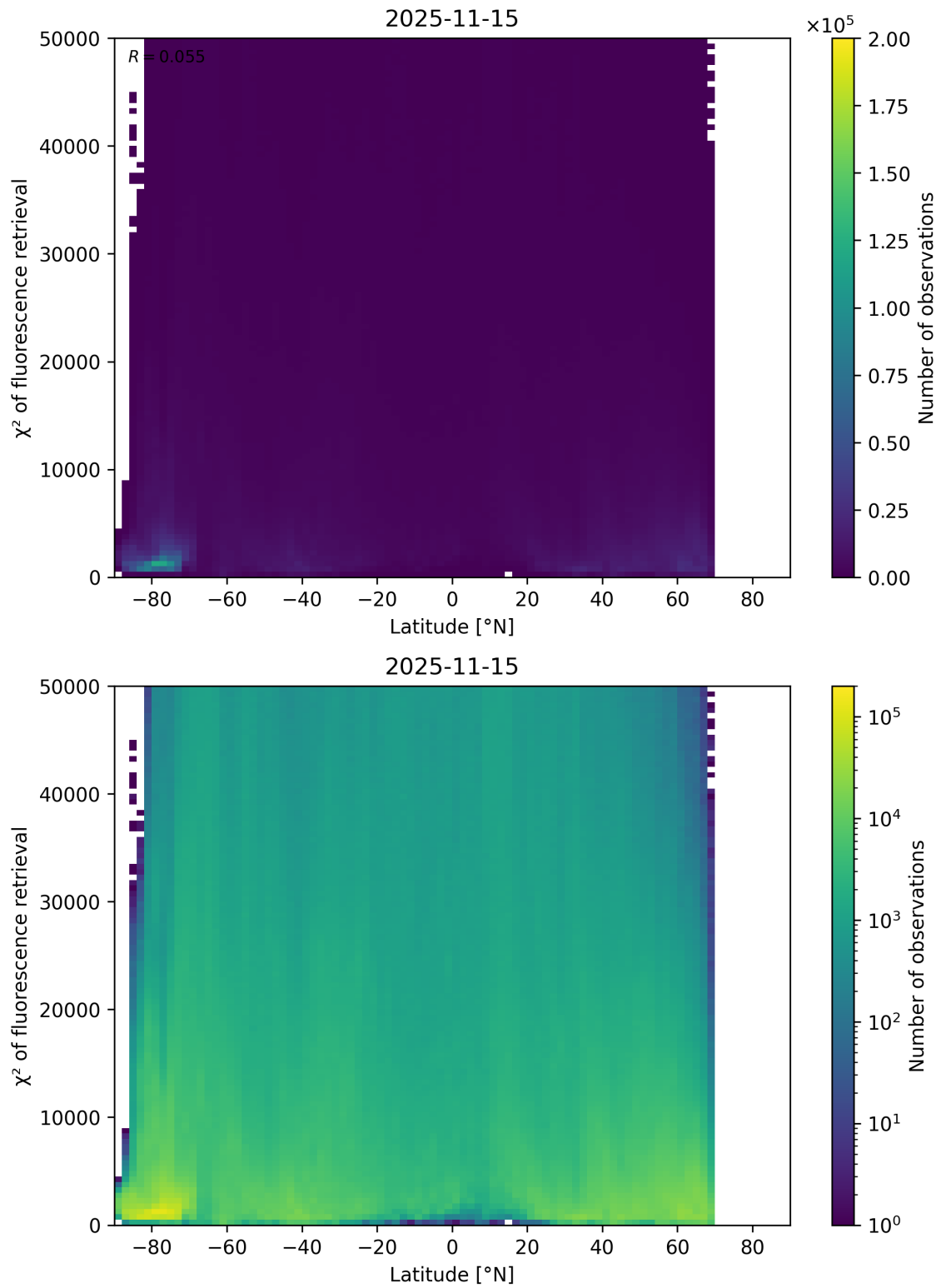
Figure 89: Scatter density plot of “Latitude” against “ \chi^2 of fluorescence retrieval” for 2025-11-14 to 2025-11-16.
