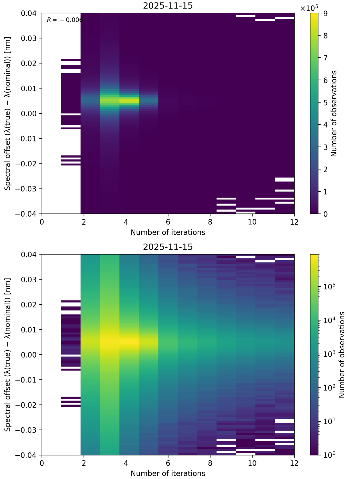
Figure 100: Scatter density plot of “Number of iterations” against “Spectral offset ( \lambda_{\text{true}} - \lambda_{\text{nominal}} )” for 2025-11-14 to 2025-11-16.
