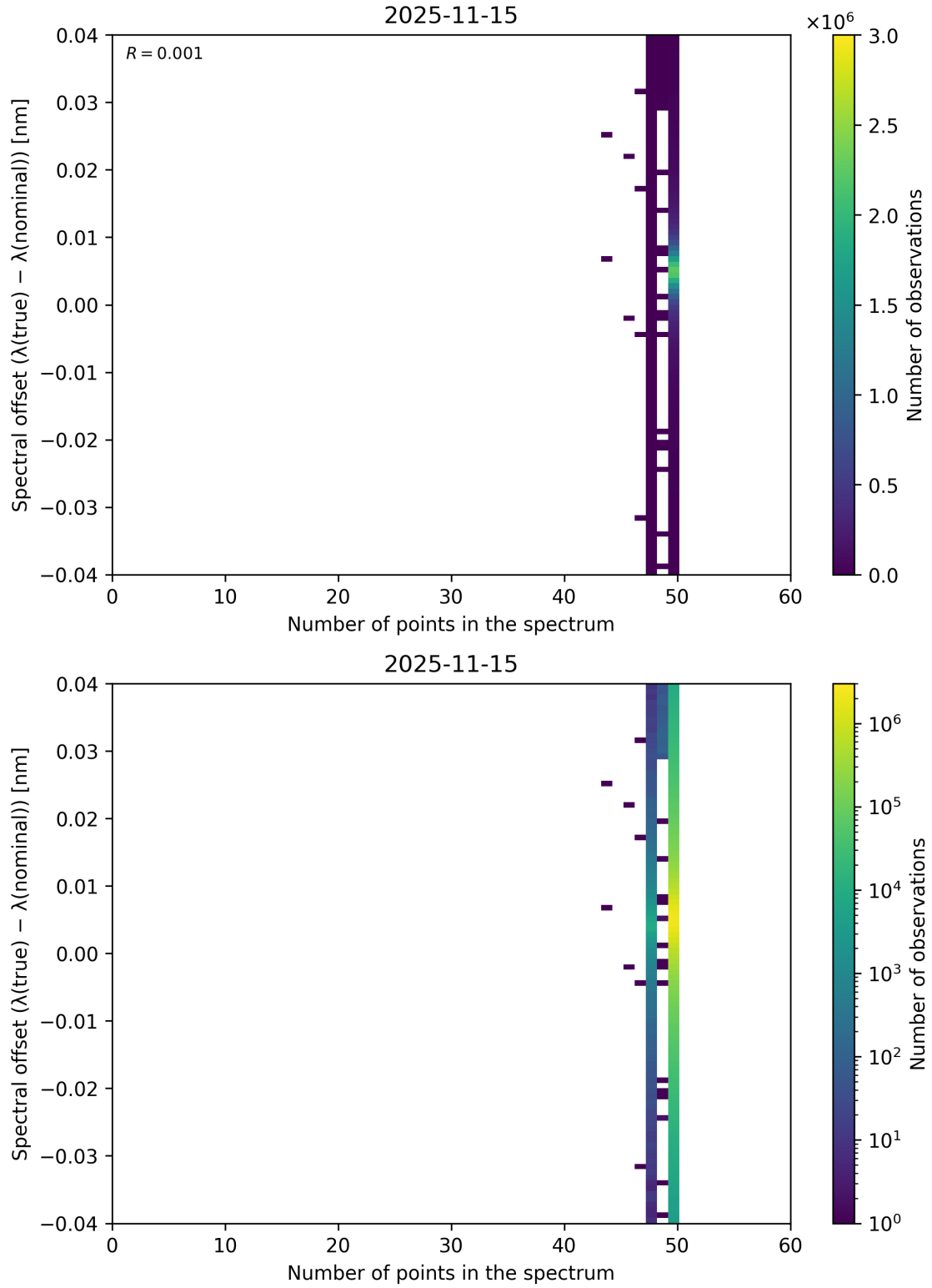
Figure 101: Scatter density plot of “Number of points in the spectrum” against “Spectral offset ( \lambda_{\text{true}} - \lambda_{\text{nominal}} )” for 2025-11-14 to 2025-11-16.
