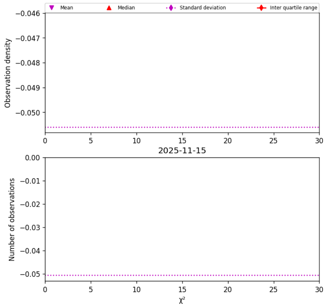
Figure 38: Histogram of " \chi^2 " for 2025-11-14 to 2025-11-16
