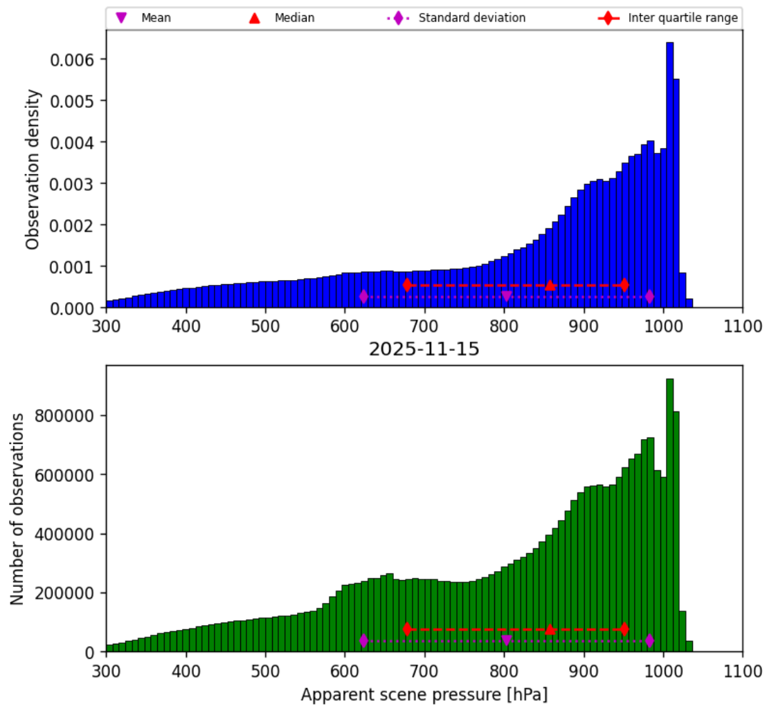
Figure 36: Histogram of “Apparent scene pressure” for 2025-11-14 to 2025-11-16
