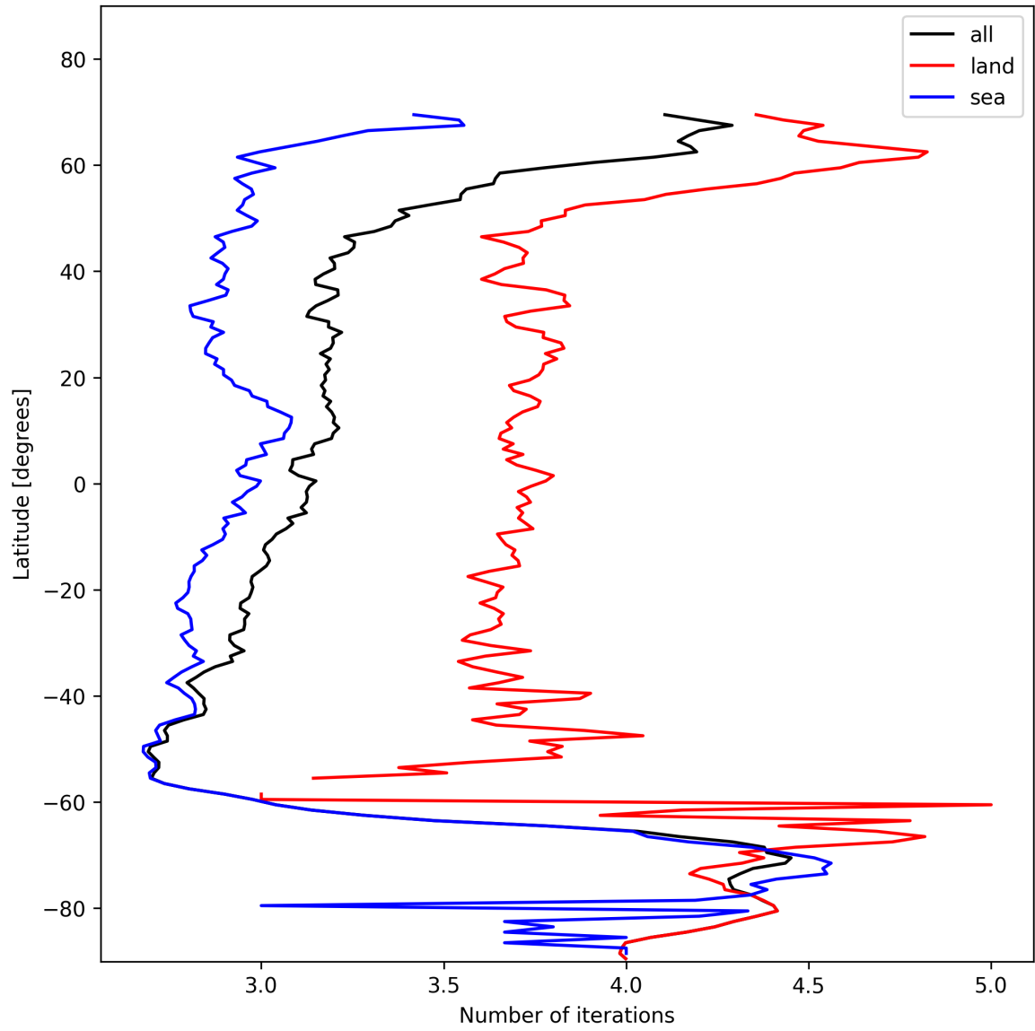
Figure 22: Zonal average of “Number of iterations” for 2025-11-14 to 2025-11-16.
