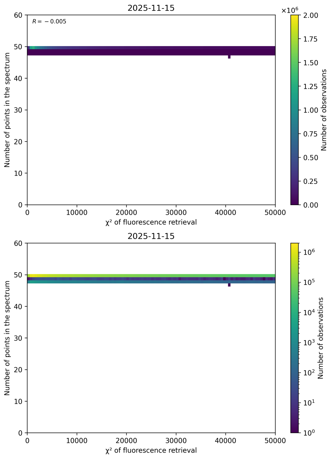
Figure 68: Scatter density plot of " \chi^2 of fluorescence retrieval" against "Number of points in the spectrum" for 2025-11-14 to 2025-11-16.
