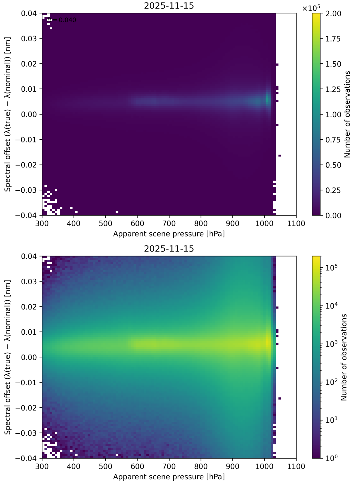
Figure 67: Scatter density plot of “Apparent scene pressure” against “Spectral offset ( \lambda_{\text{true}} - \lambda_{\text{nominal}} )” for 2025-11-14 to 2025-11-16.
