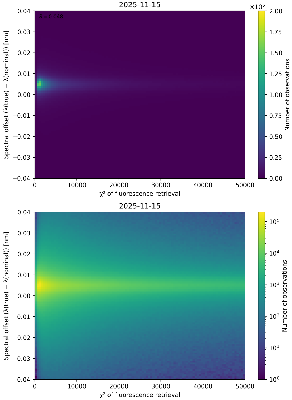
Figure 69: Scatter density plot of “ \chi^2 of fluorescence retrieval” against “Spectral offset ( \lambda_{\text{true}} - \lambda_{\text{nominal}} )” for 2025-11-14 to 2025-11-16.
