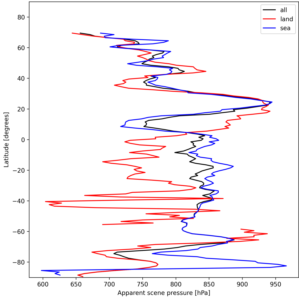
Figure 19: Zonal average of “Apparent scene pressure” for 2025-11-14 to 2025-11-16.
