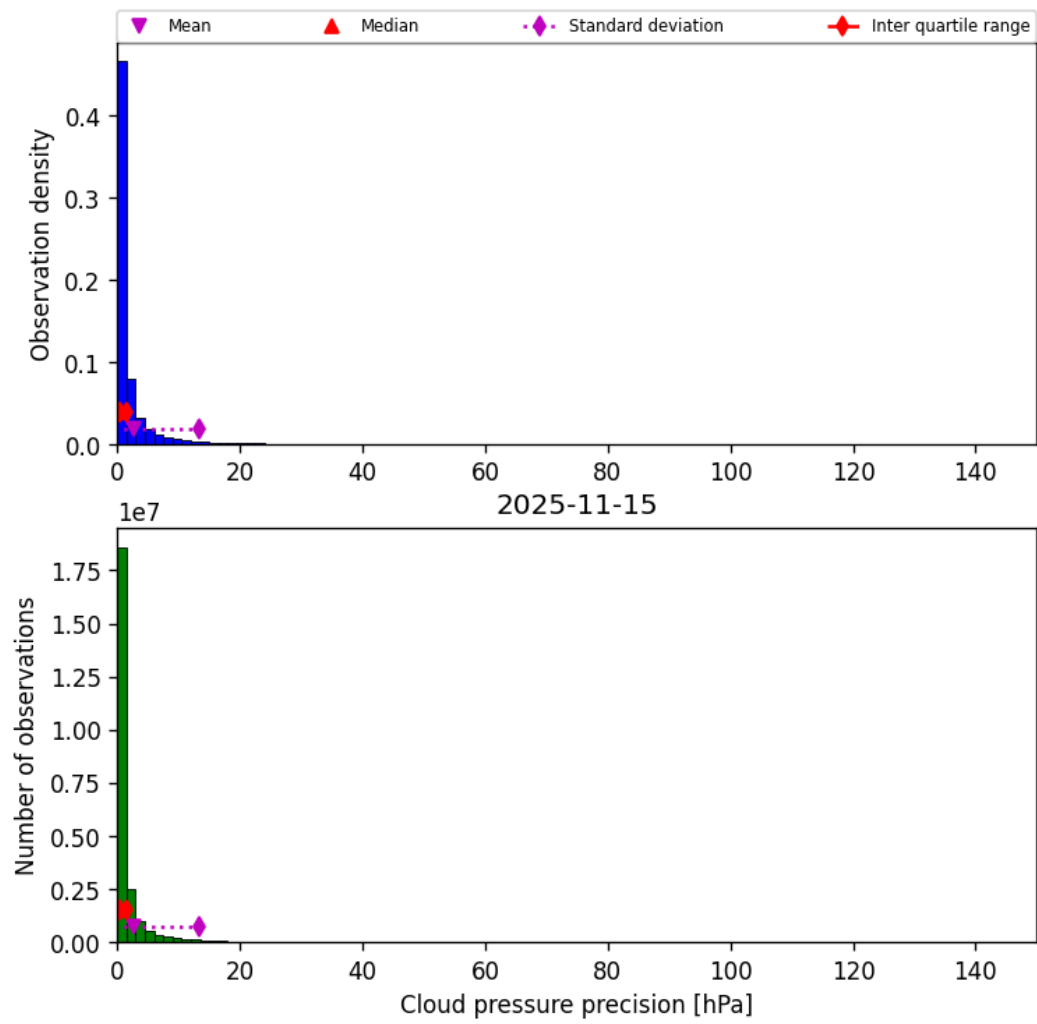
Figure 31: Histogram of “Cloud pressure precision” for 2025-11-14 to 2025-11-16
