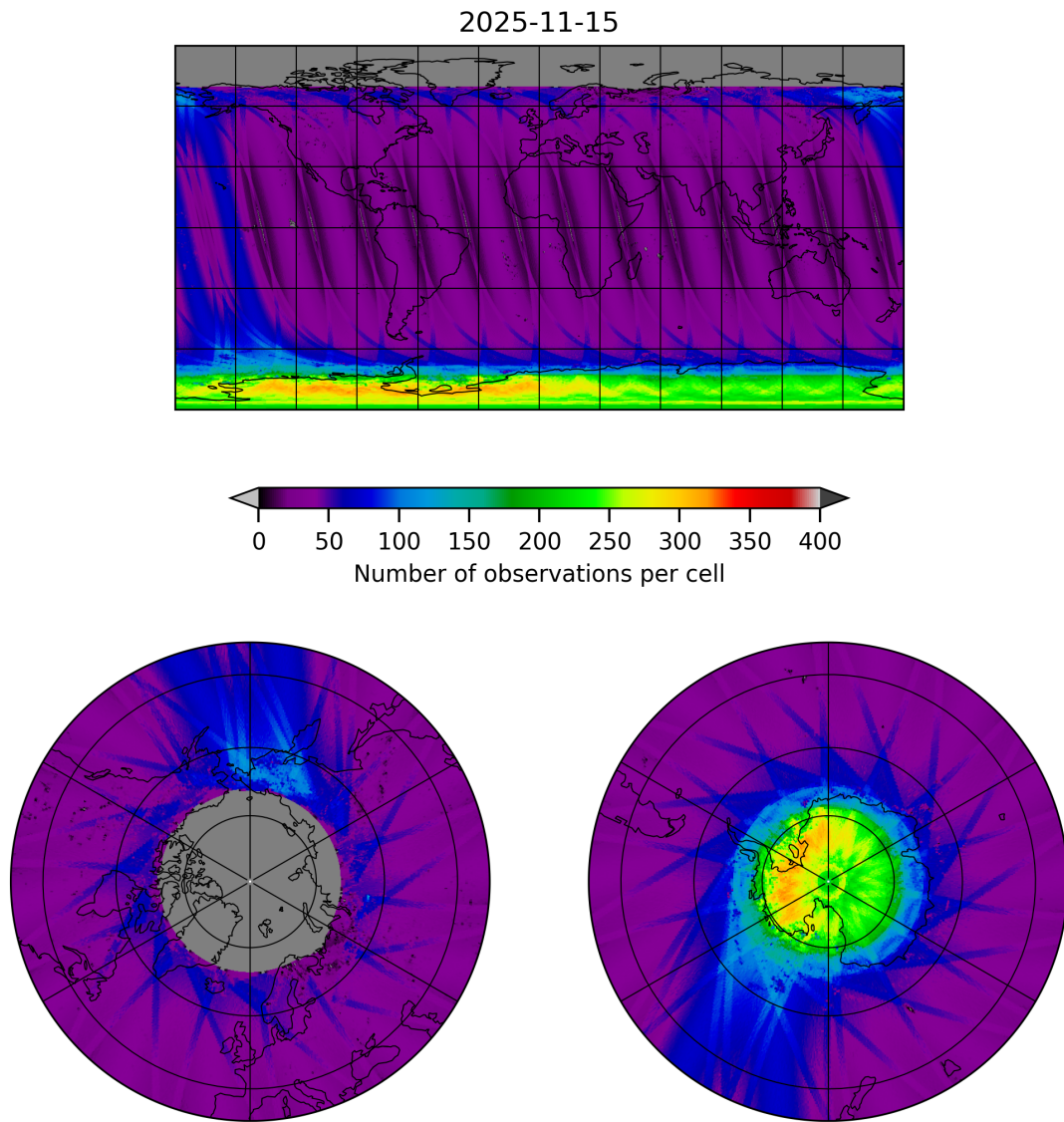
Figure 11: Map of the number of observations for 2025-11-14 to 2025-11-16
