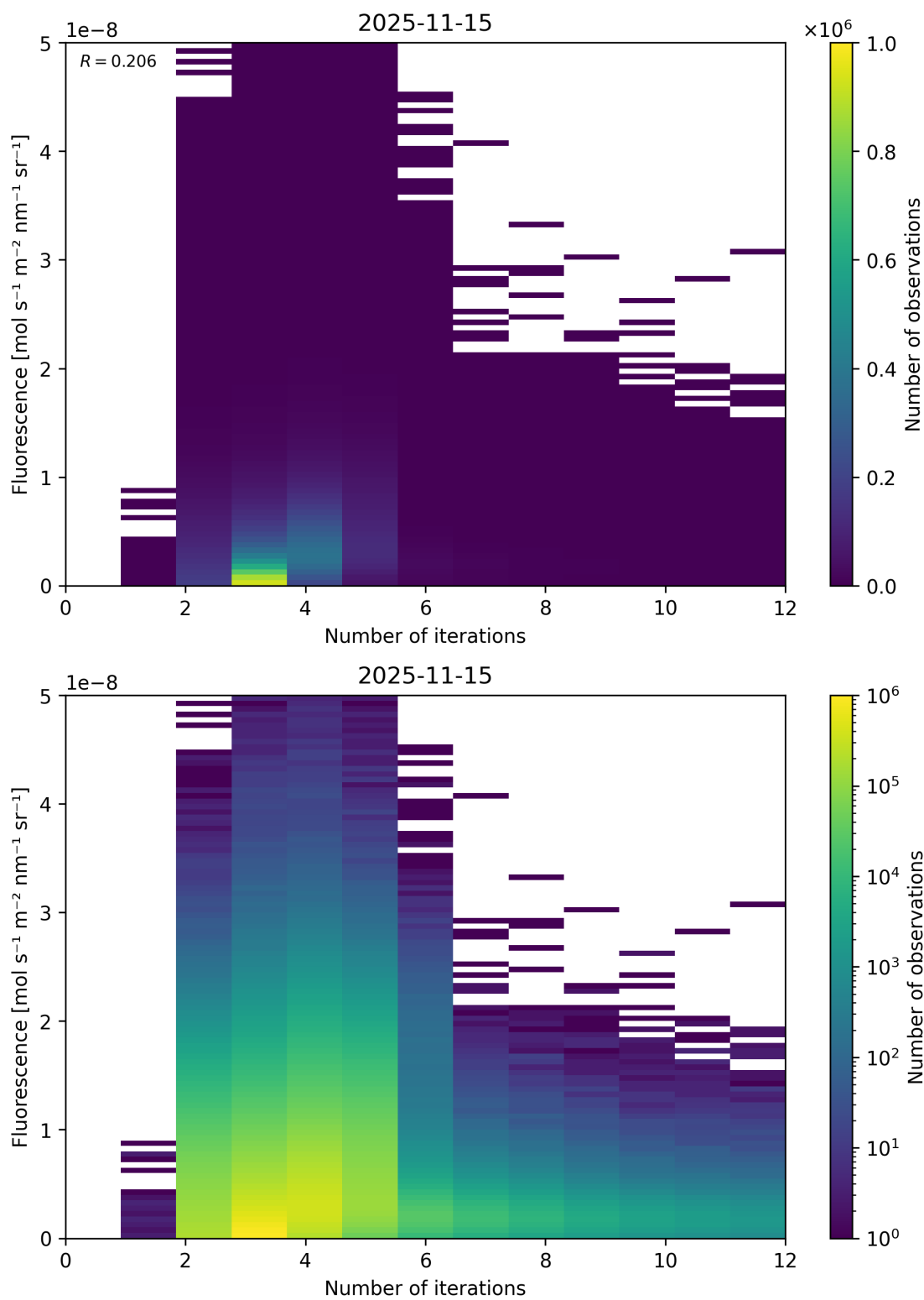
Figure 98: Scatter density plot of “Number of iterations” against “Fluorescence” for 2025-11-14 to 2025-11-16.
