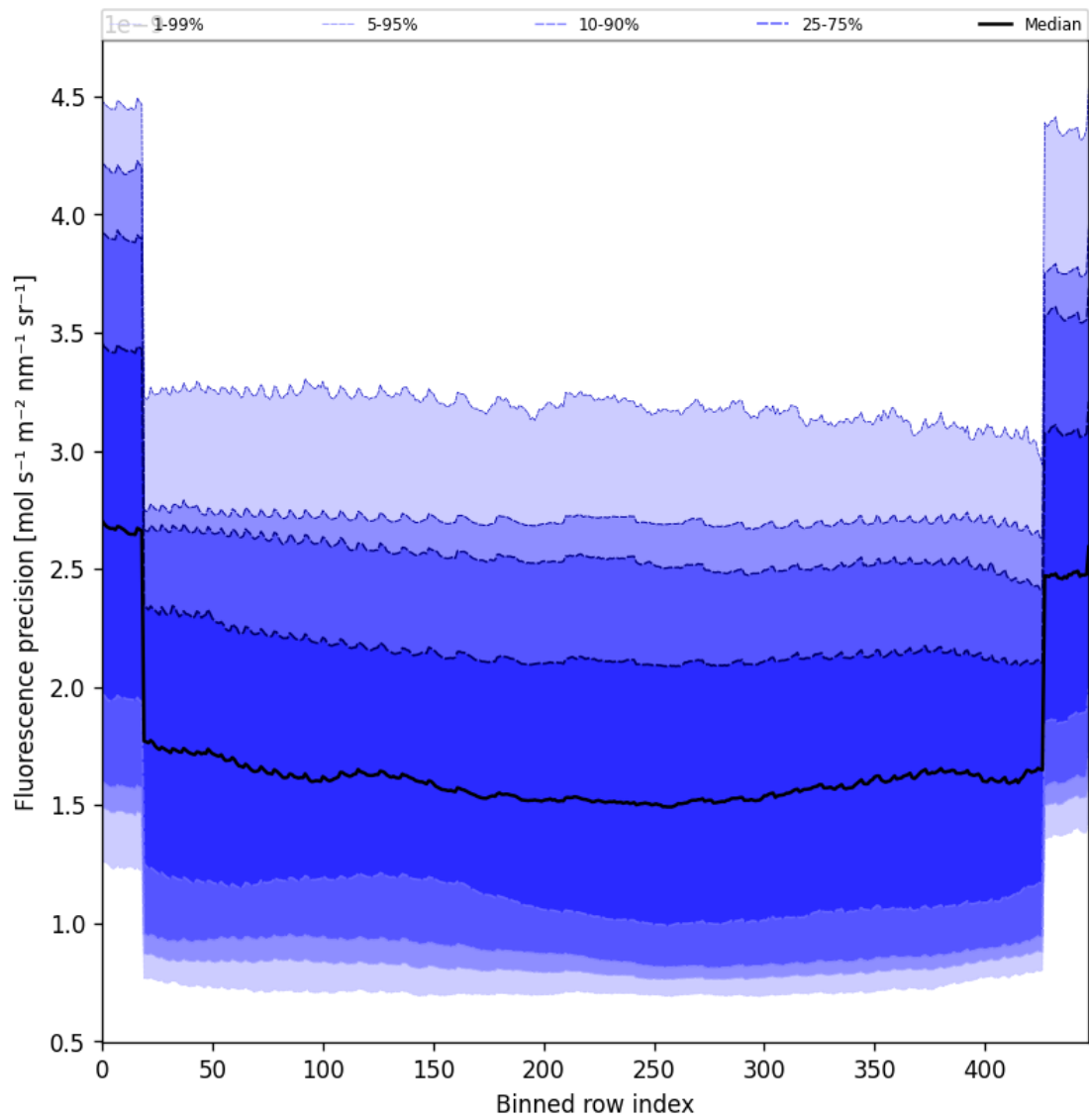
Figure 58: Along track statistics of “Fluorescence precision” for 2025-11-14 to 2025-11-16
