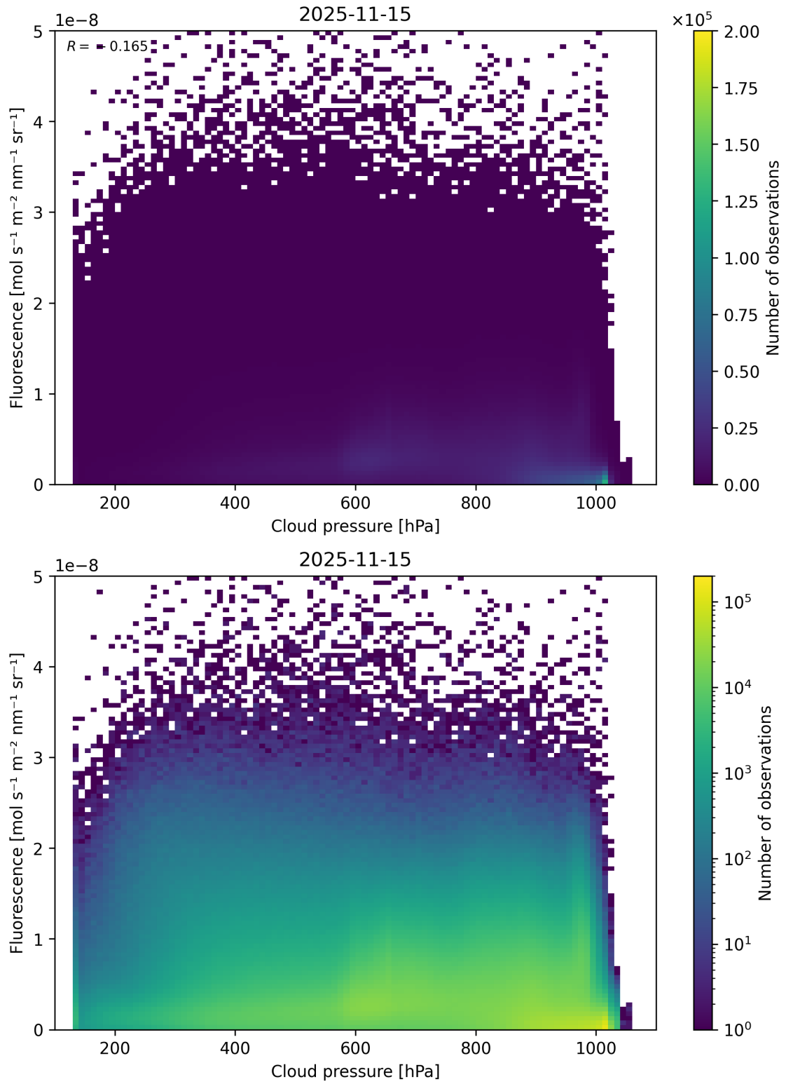
Figure 80: Scatter density plot of “Cloud pressure” against “Fluorescence” for 2025-11-14 to 2025-11-16.
