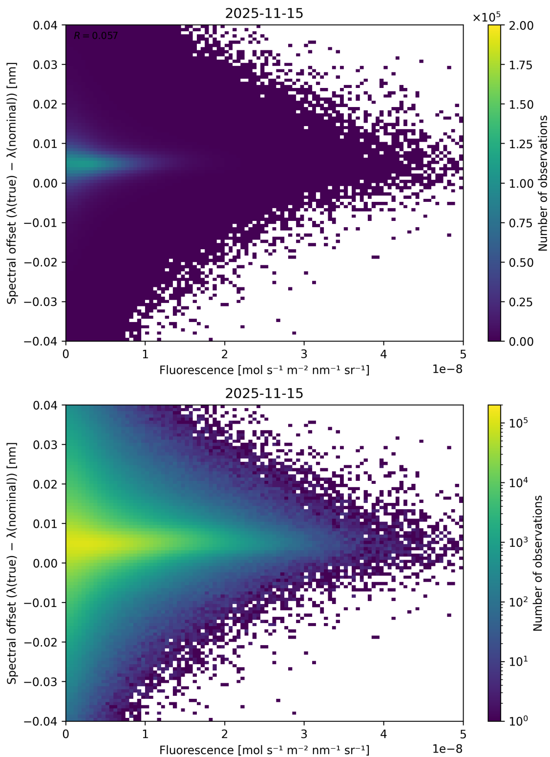
Figure 87: Scatter density plot of “Fluorescence” against “Spectral offset ( \lambda_{\text{true}} - \lambda_{\text{nominal}} )” for 2025-11-14 to 2025-11-16.
