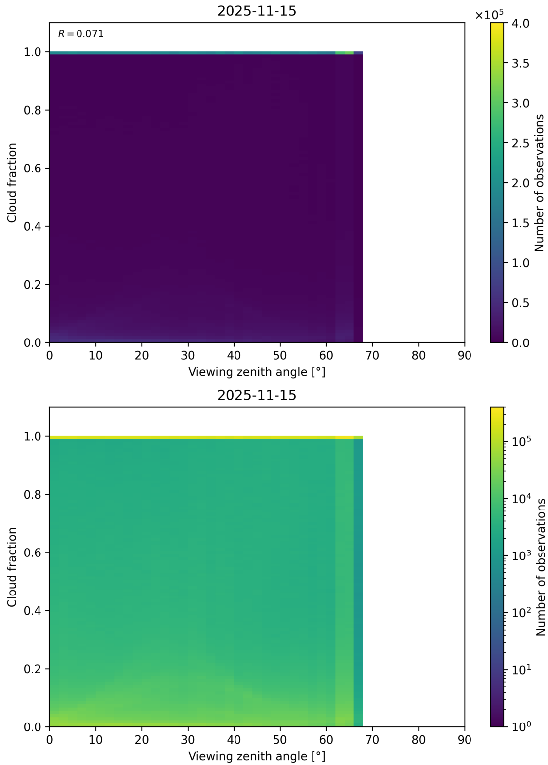
Figure 120: Scatter density plot of “Viewing zenith angle” against “Cloud fraction” for 2025-11-14 to 2025-11-16.
