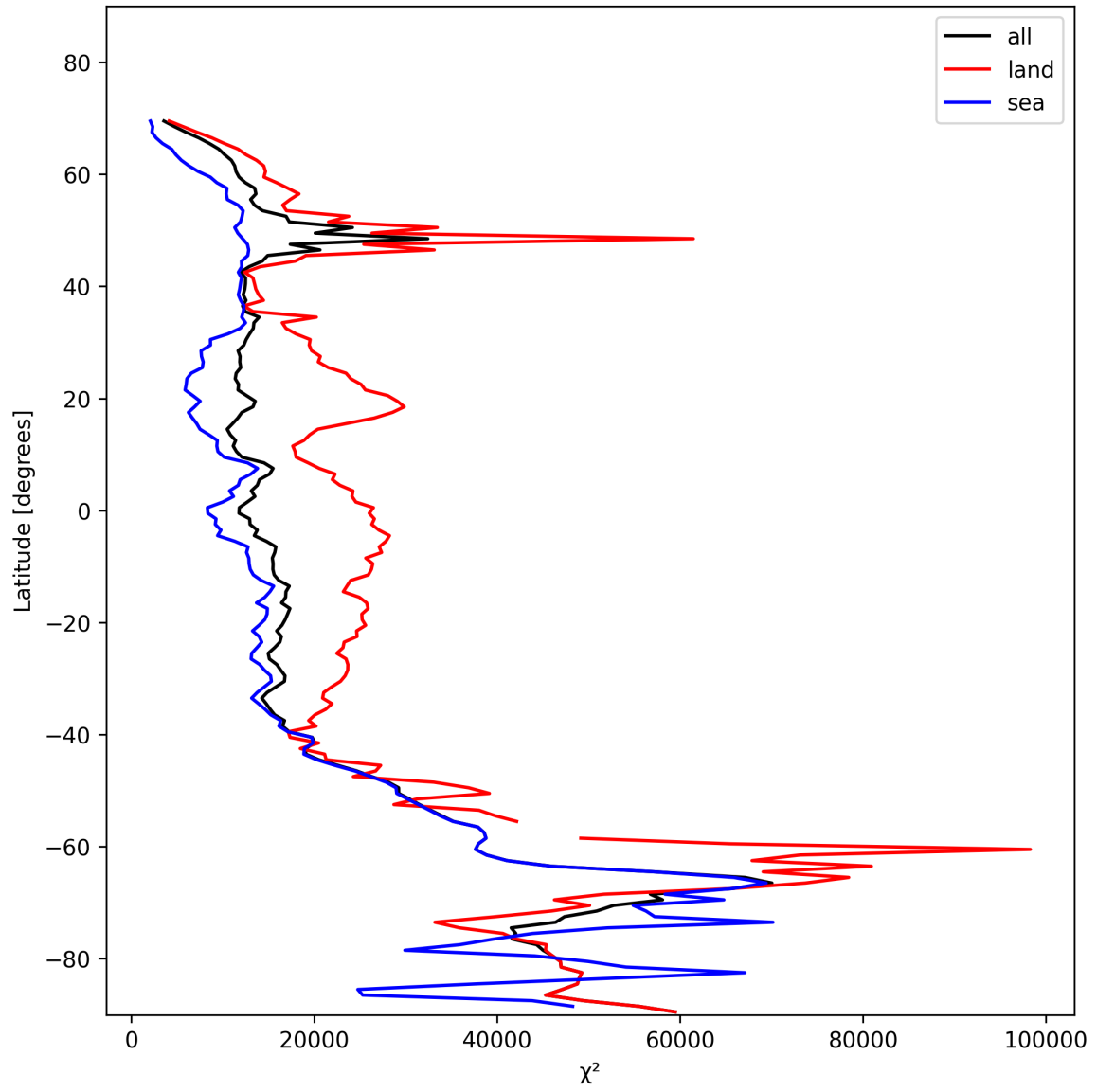
Figure 21: Zonal average of “ \chi^2 ” for 2025-11-14 to 2025-11-16.
