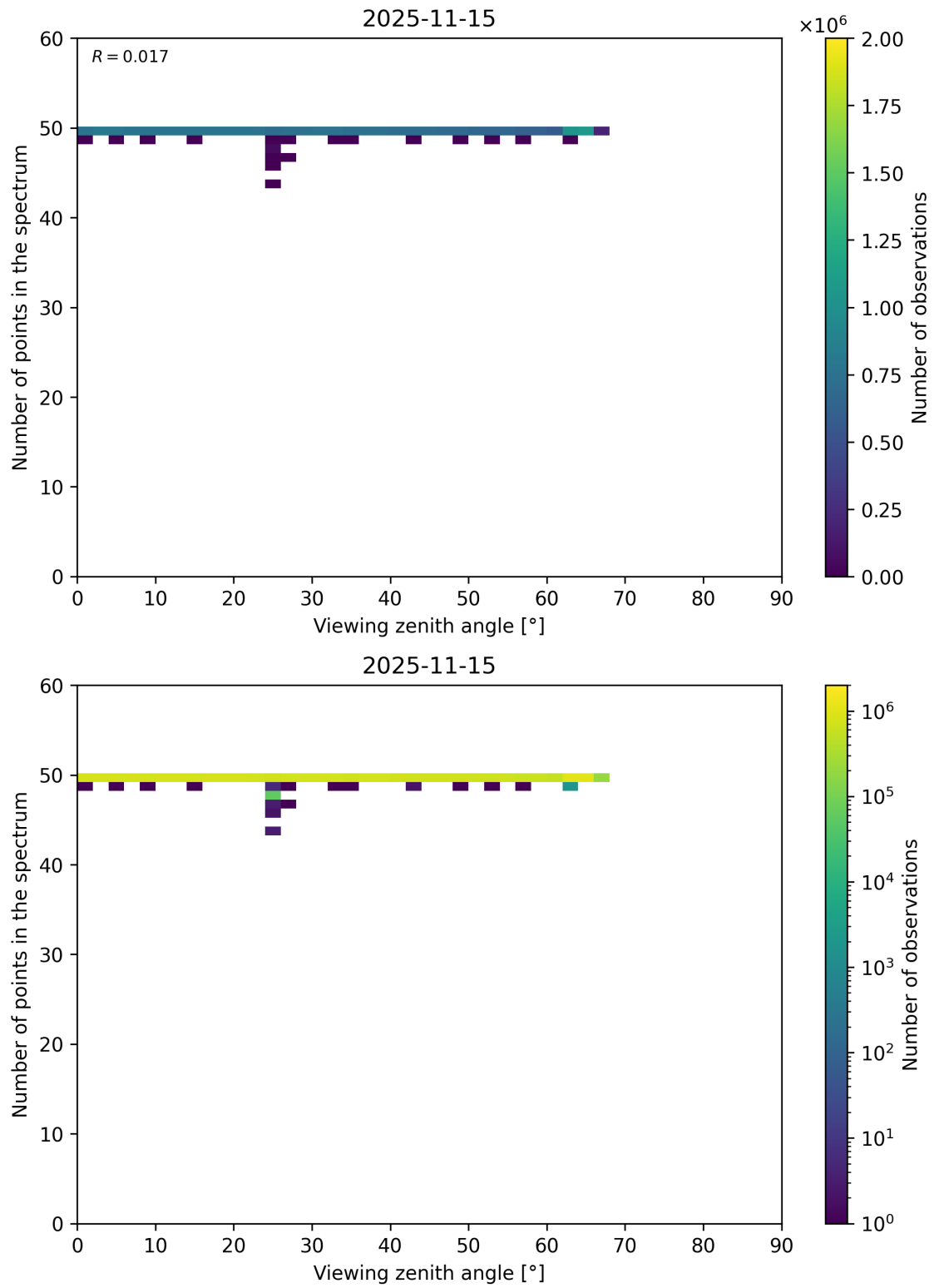
Figure 125: Scatter density plot of “Viewing zenith angle” against “Number of points in the spectrum” for 2025-11-14 to 2025-11-16.
