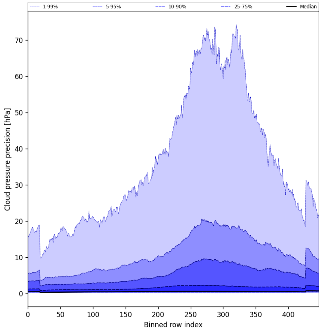
Figure 48: Along track statistics of “Cloud pressure precision” for 2025-11-14 to 2025-11-16
