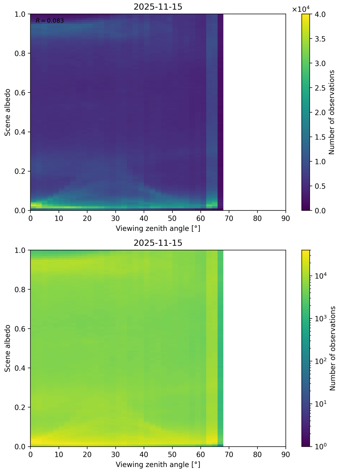
Figure 126: Scatter density plot of “Viewing zenith angle” against “Scene albedo” for 2025-11-14 to 2025-11-16.
