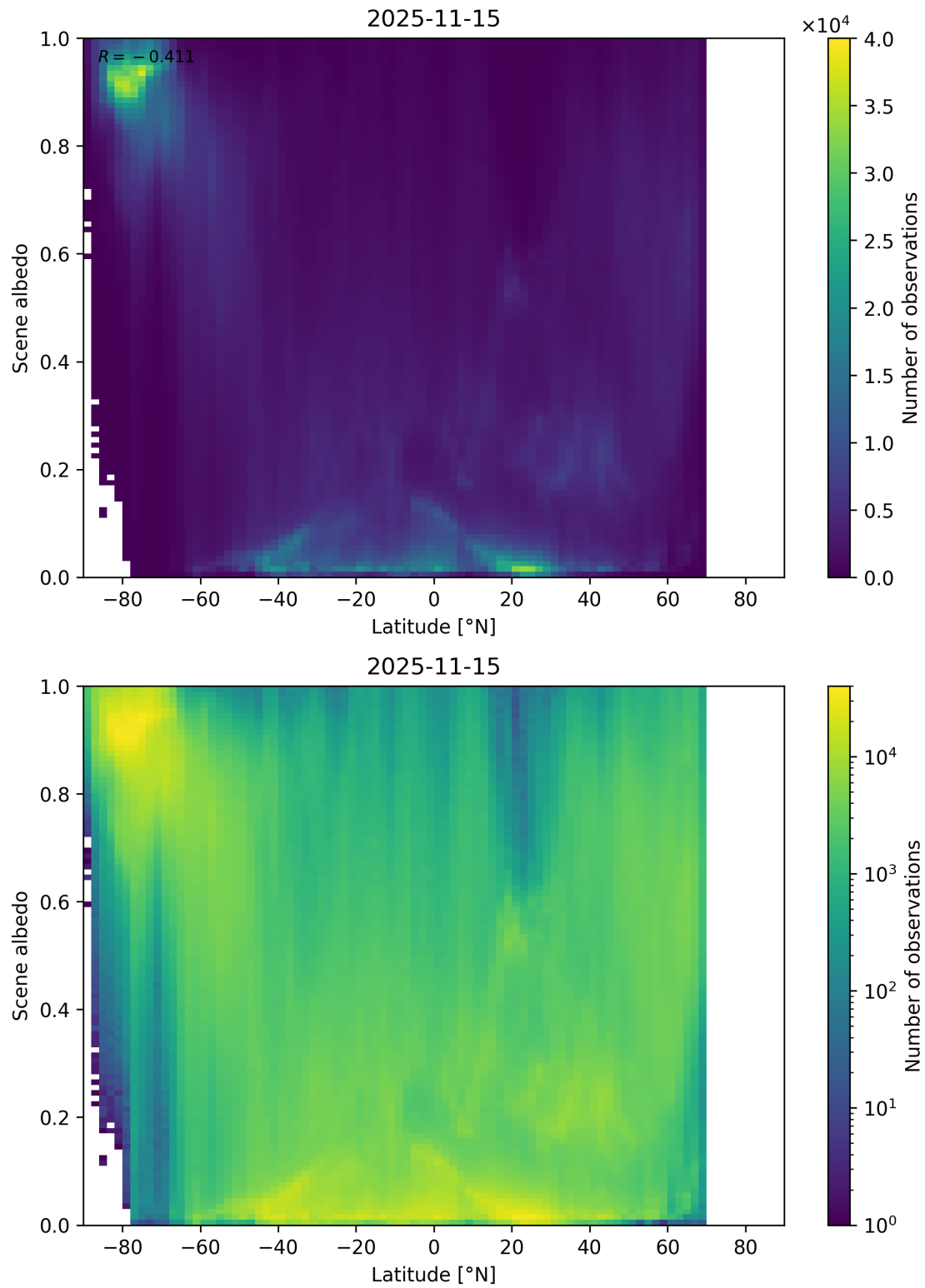
Figure 95: Scatter density plot of “Latitude” against “Scene albedo” for 2025-11-14 to 2025-11-16.
