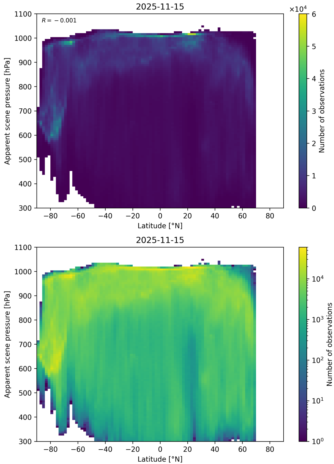
Figure 88: Scatter density plot of “Latitude” against “Apparent scene pressure” for 2025-11-14 to 2025-11-16.
