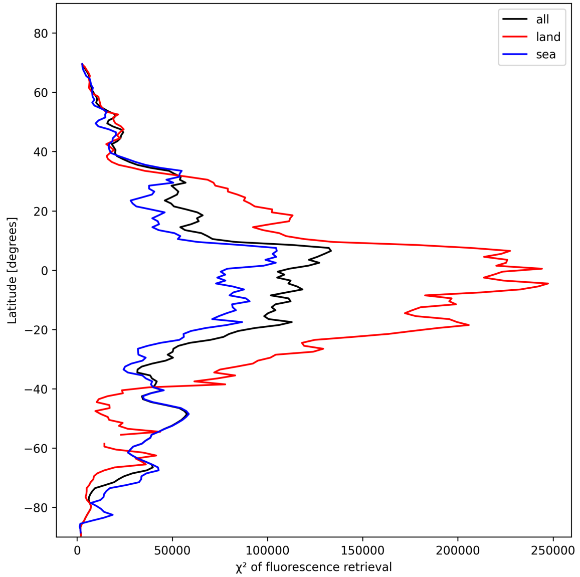
Figure 25: Zonal average of “ \chi^2 of fluorescence retrieval” for 2025-11-14 to 2025-11-16.
