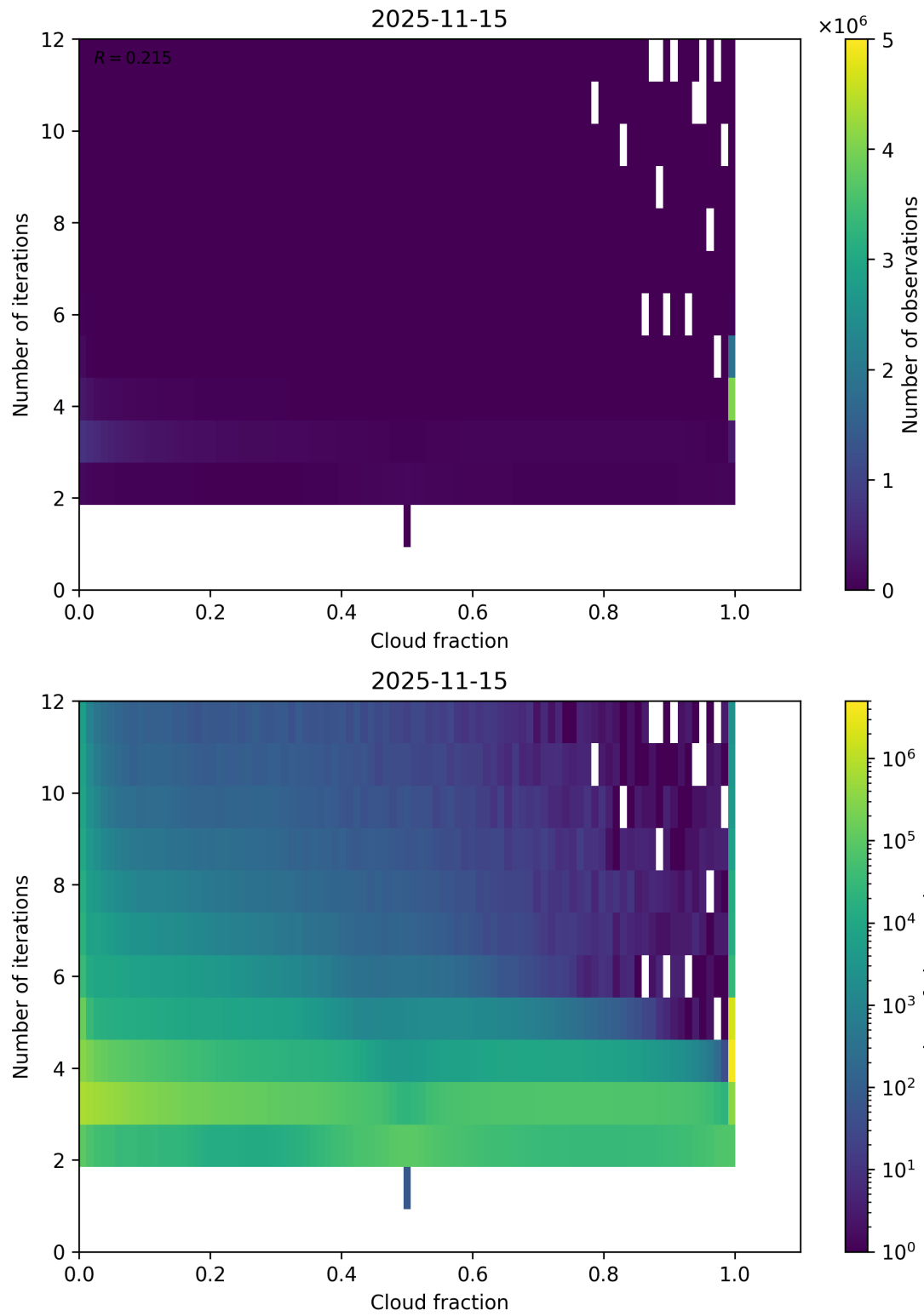
Figure 73: Scatter density plot of “Cloud fraction” against “Number of iterations” for 2025-11-14 to 2025-11-16.
