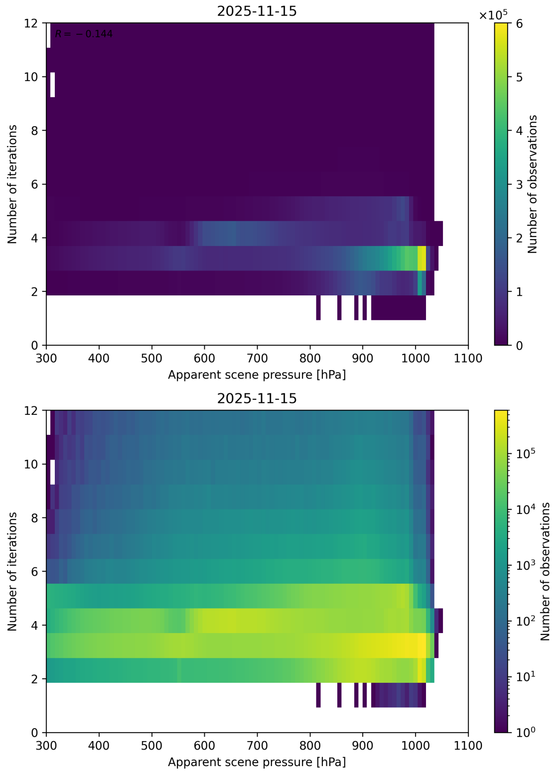
Figure 65: Scatter density plot of “Apparent scene pressure” against “Number of iterations” for 2025-11-14 to 2025-11-16.
