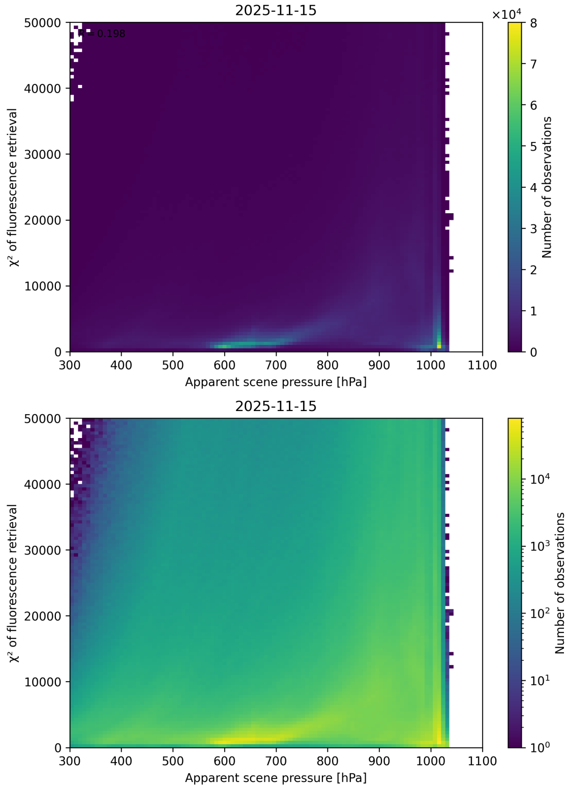
Figure 63: Scatter density plot of “Apparent scene pressure” against “ \chi^2 of fluorescence retrieval” for 2025-11-14 to 2025-11-16.
