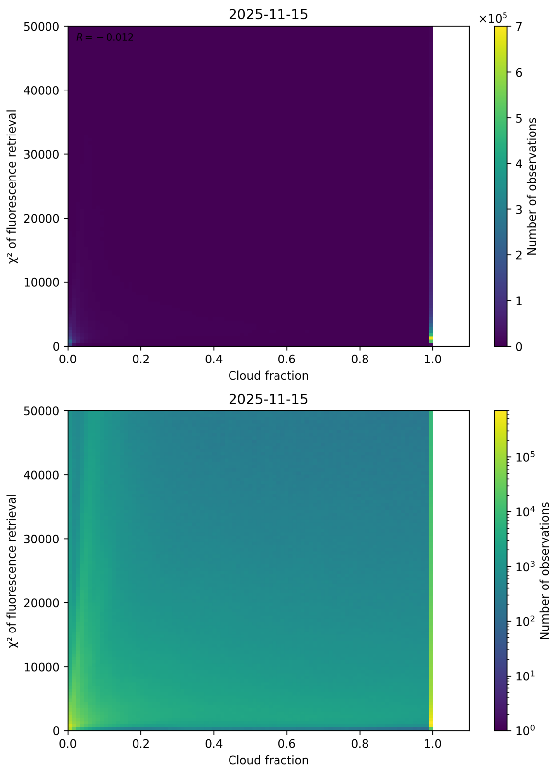
Figure 71: Scatter density plot of “Cloud fraction” against “ \chi^2 of fluorescence retrieval” for 2025-11-14 to 2025-11-16.
