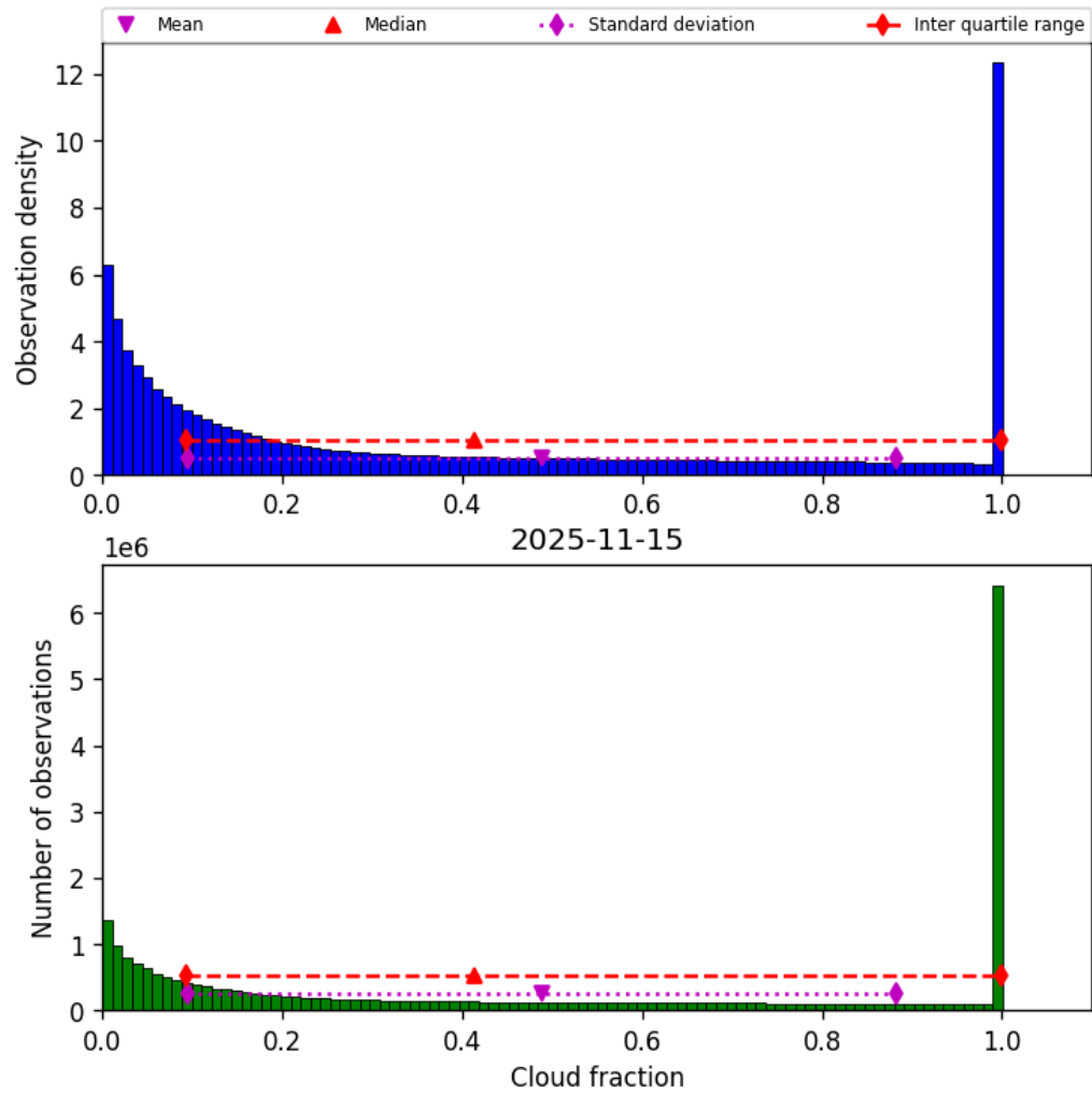
Figure 32: Histogram of “Cloud fraction” for 2025-11-14 to 2025-11-16
