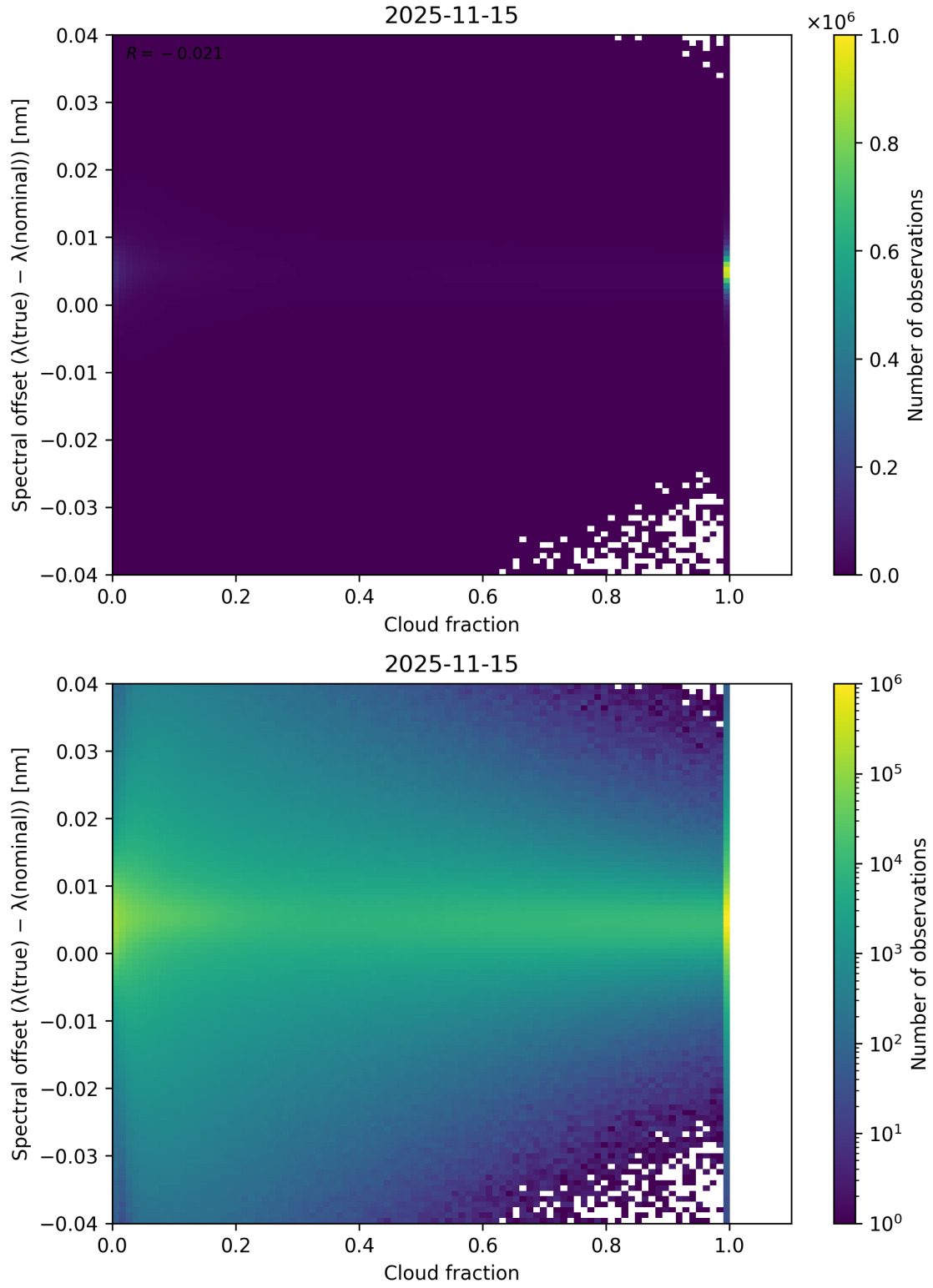
Figure 76: Scatter density plot of “Cloud fraction” against “Spectral offset ( \lambda_{\text{true}} - \lambda_{\text{nominal}} )” for 2025-11-14 to 2025-11-16.
