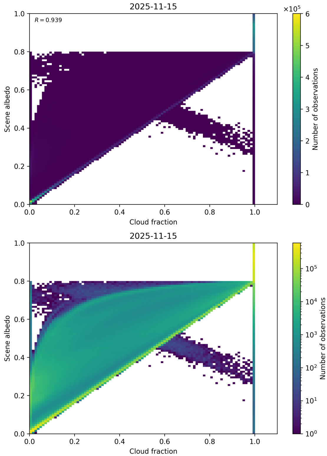
Figure 75: Scatter density plot of “Cloud fraction” against “Scene albedo” for 2025-11-14 to 2025-11-16.
