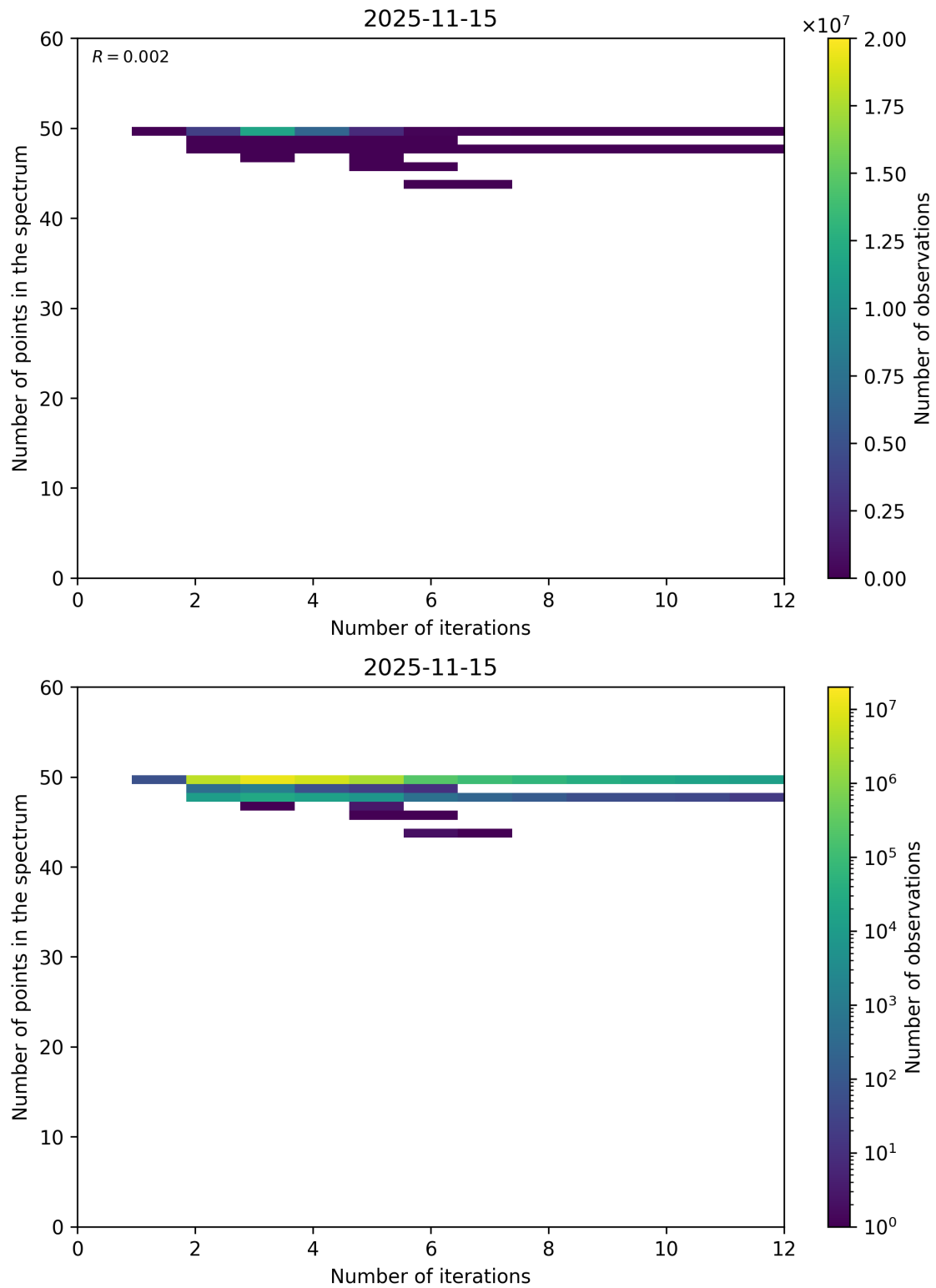
Figure 99: Scatter density plot of “Number of iterations” against “Number of points in the spectrum” for 2025-11-14 to 2025-11-16.
