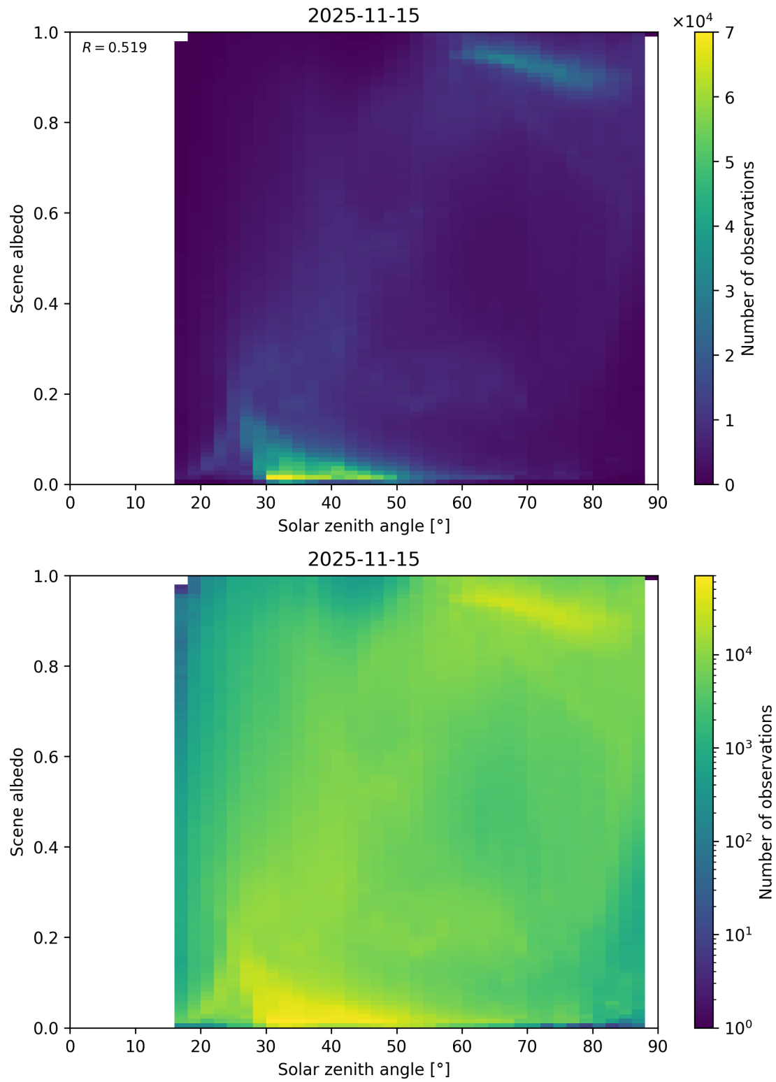
Figure 116: Scatter density plot of “Solar zenith angle” against “Scene albedo” for 2025-11-14 to 2025-11-16.
