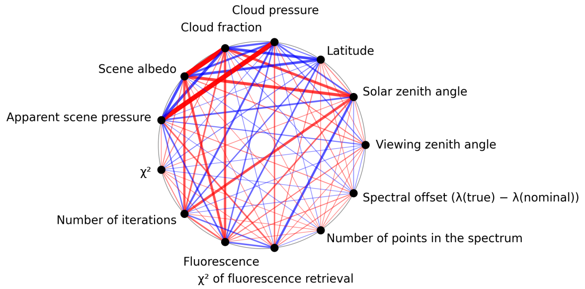
Figure 1: Map of correlation graph for 2025-11-14 to 2025-11-16.
