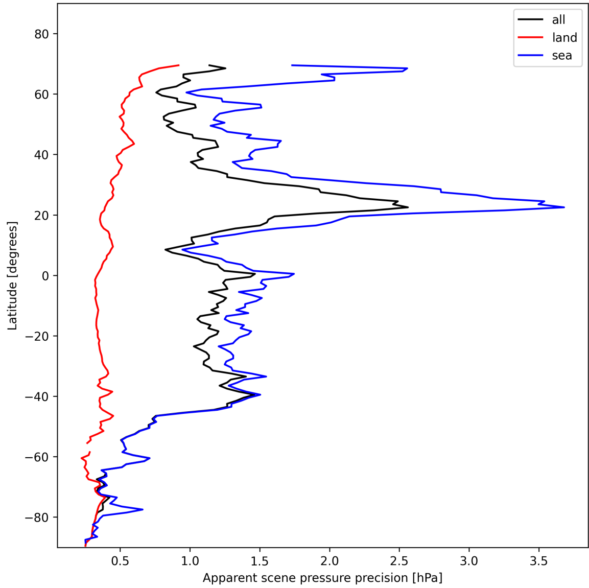
Figure 20: Zonal average of “Apparent scene pressure precision” for 2025-11-14 to 2025-11-16.
