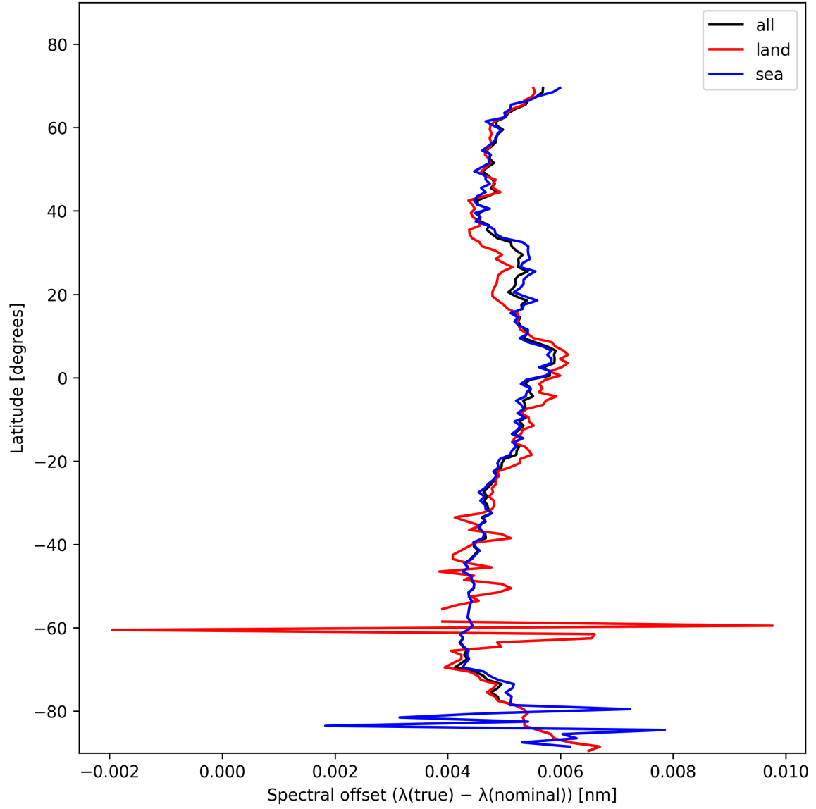
Figure 28: Zonal average of “Spectral offset ( \lambda_{\text{true}} - \lambda_{\text{nominal}} )” for 2025-11-14 to 2025-11-16.
