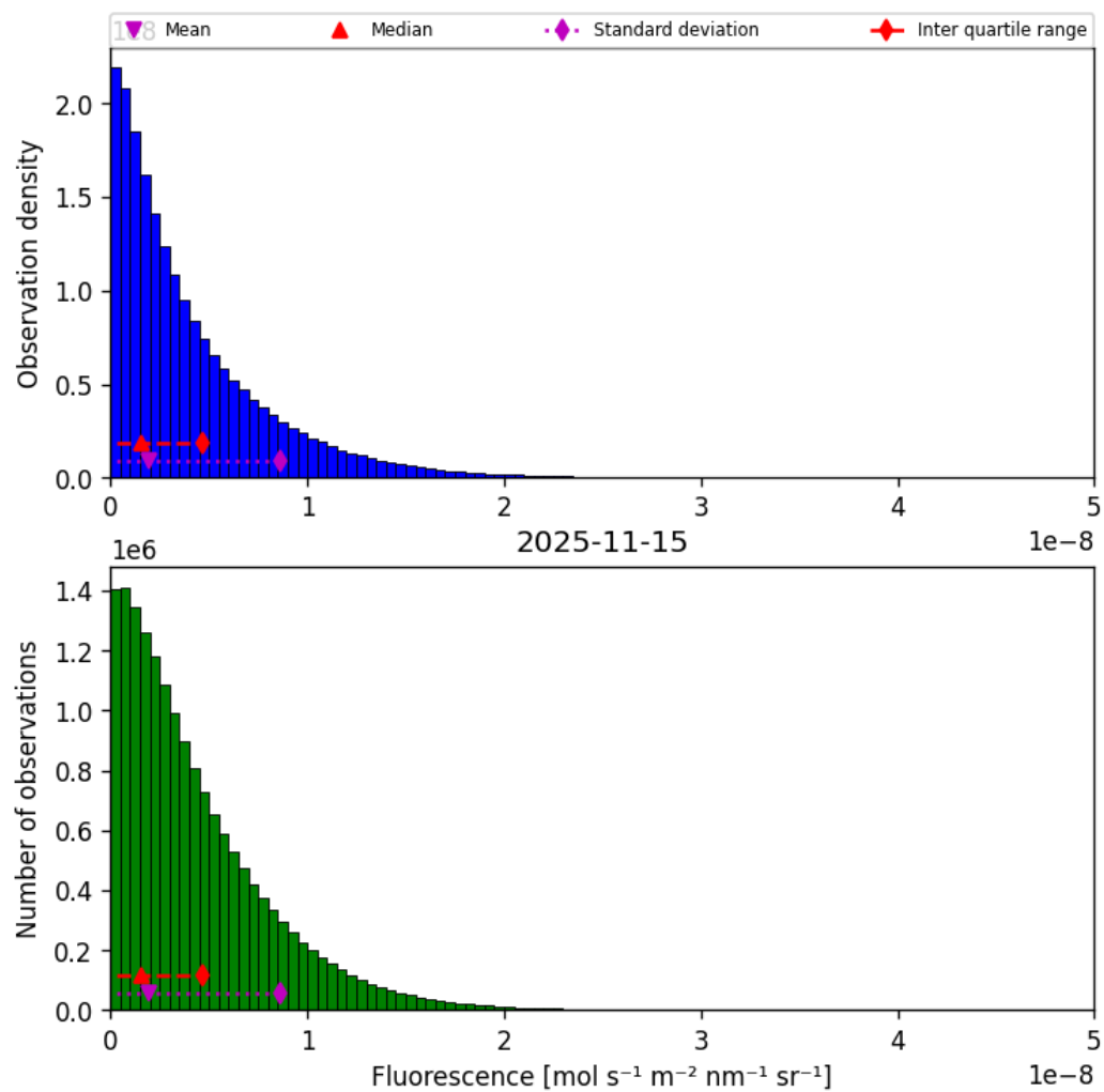
Figure 40: Histogram of “Fluorescence” for 2025-11-14 to 2025-11-16
