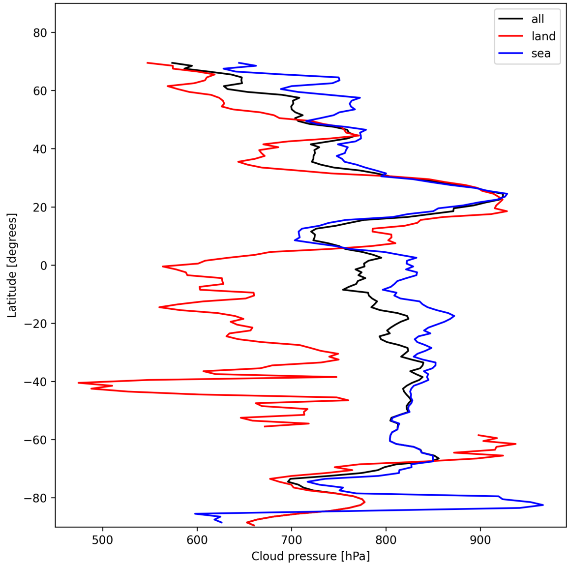
Figure 13: Zonal average of “Cloud pressure” for 2025-11-14 to 2025-11-16.
