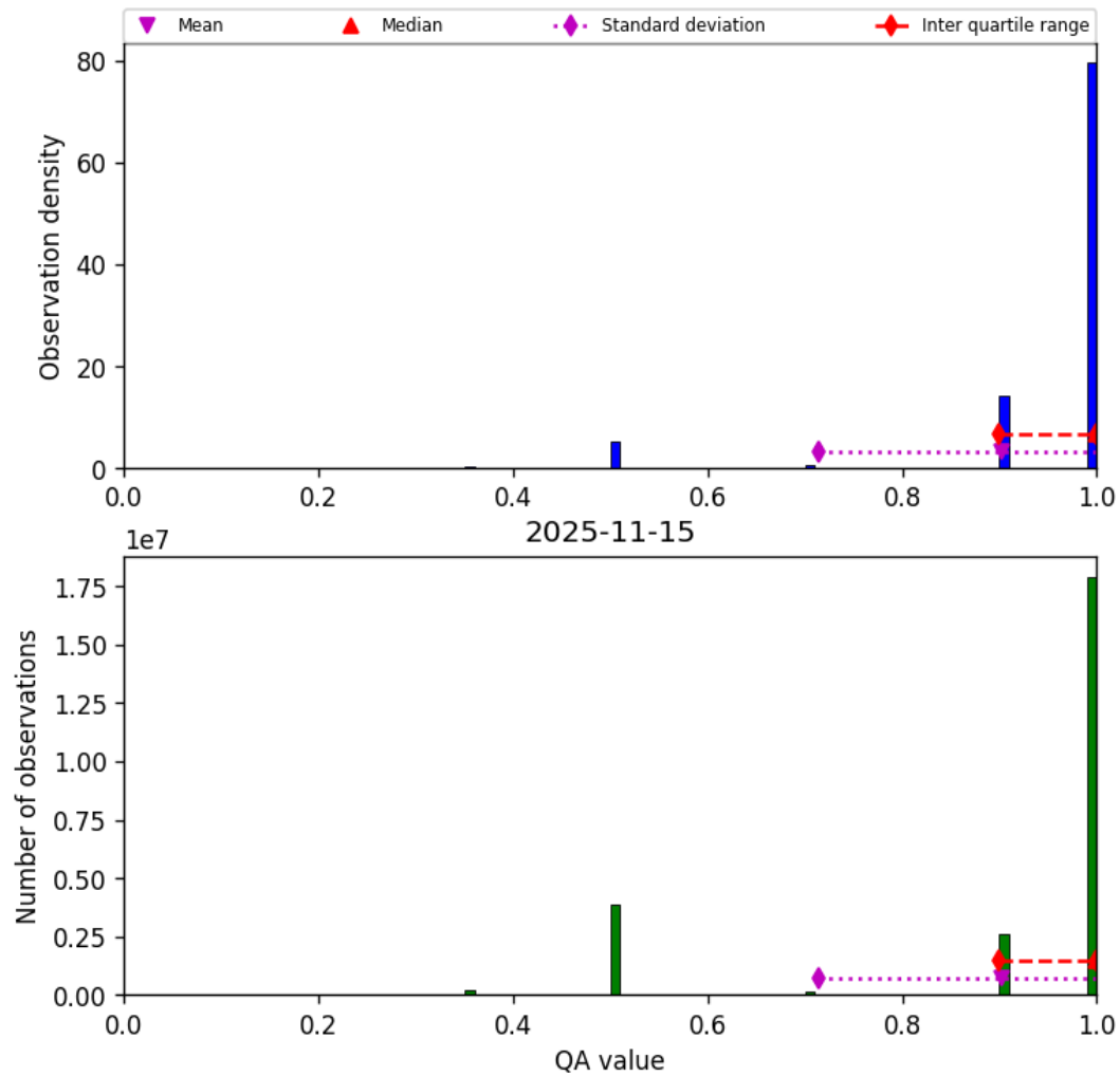
Figure 29: Histogram of “QA value” for 2025-11-14 to 2025-11-16
