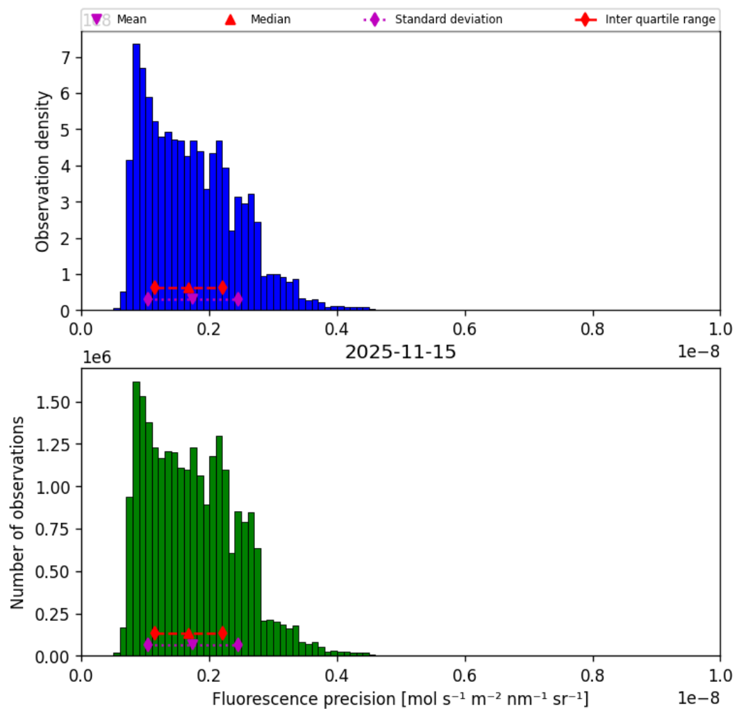
Figure 41: Histogram of “Fluorescence precision” for 2025-11-14 to 2025-11-16
