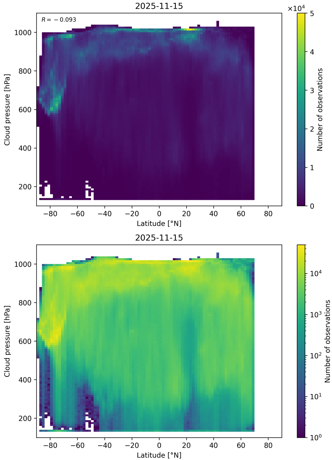
Figure 91: Scatter density plot of “Latitude” against “Cloud pressure” for 2025-11-14 to 2025-11-16.
