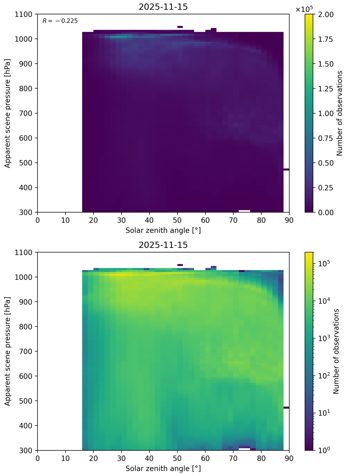
Figure 108: Scatter density plot of “Solar zenith angle” against “Apparent scene pressure” for 2025-11-14 to 2025-11-16.
