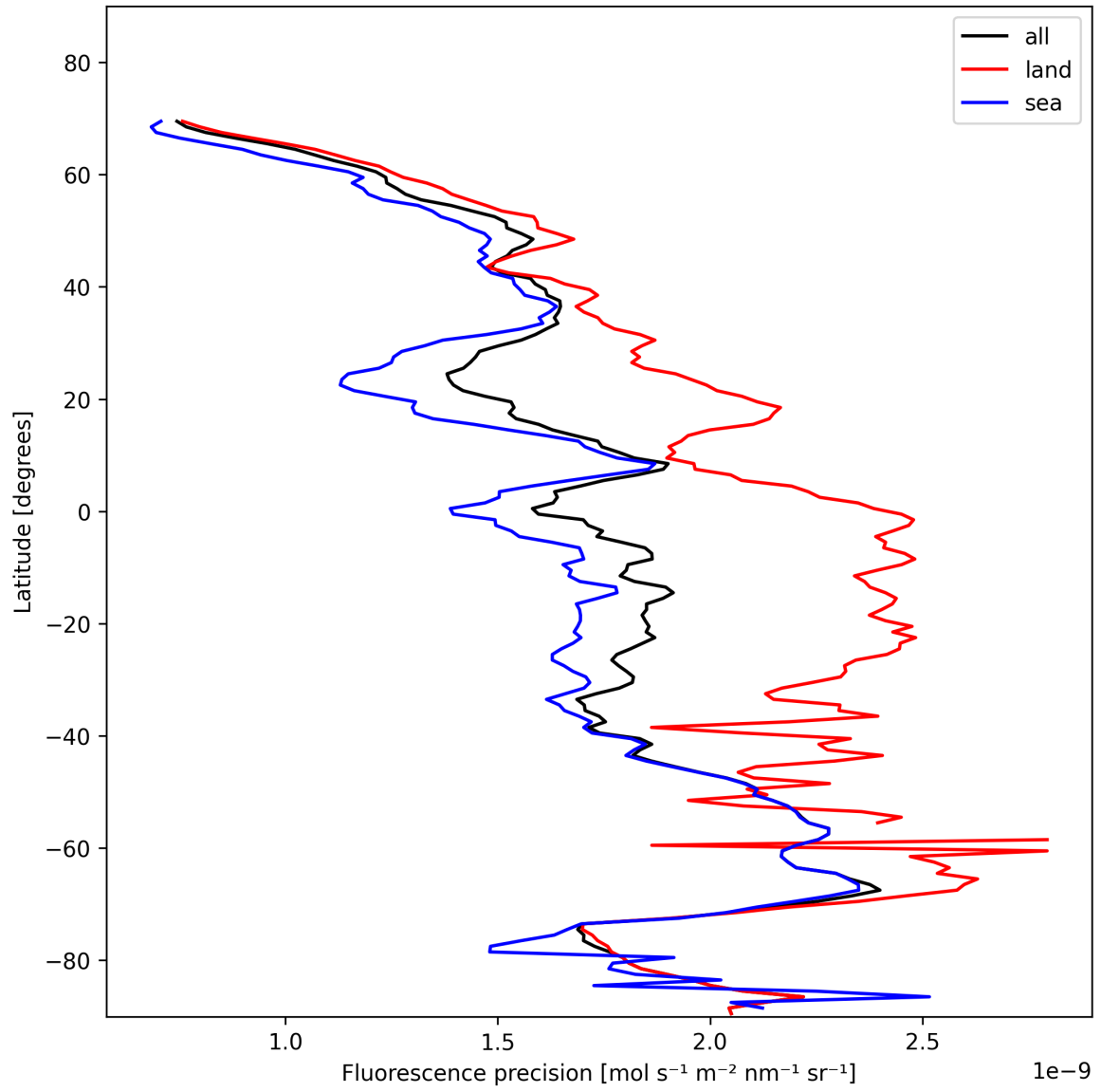
Figure 24: Zonal average of “Fluorescence precision” for 2025-11-14 to 2025-11-16.
