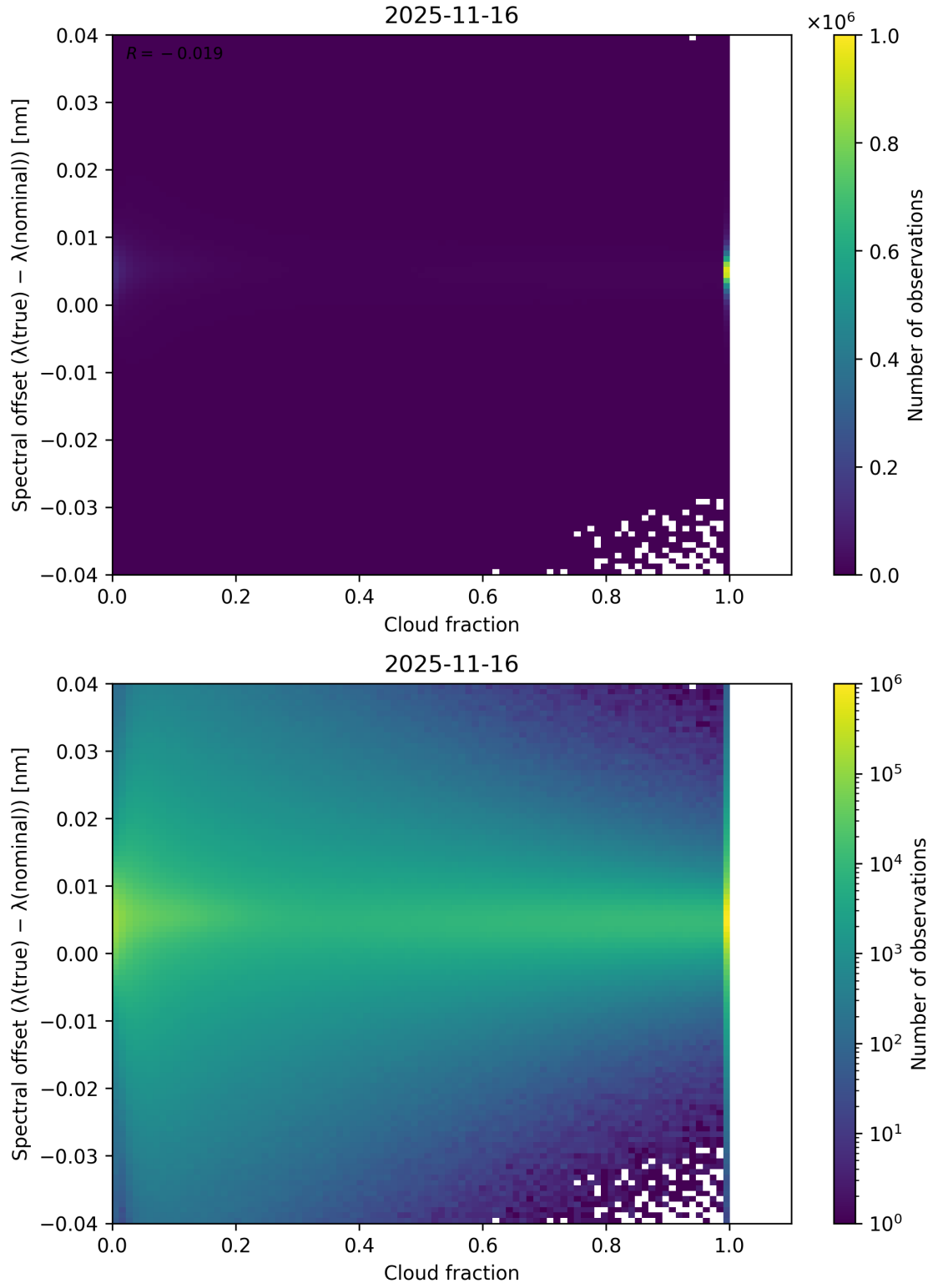
Figure 76: Scatter density plot of “Cloud fraction” against “Spectral offset ( \lambda_{\text{true}} - \lambda_{\text{nominal}} )” for 2025-11-15 to 2025-11-17.
