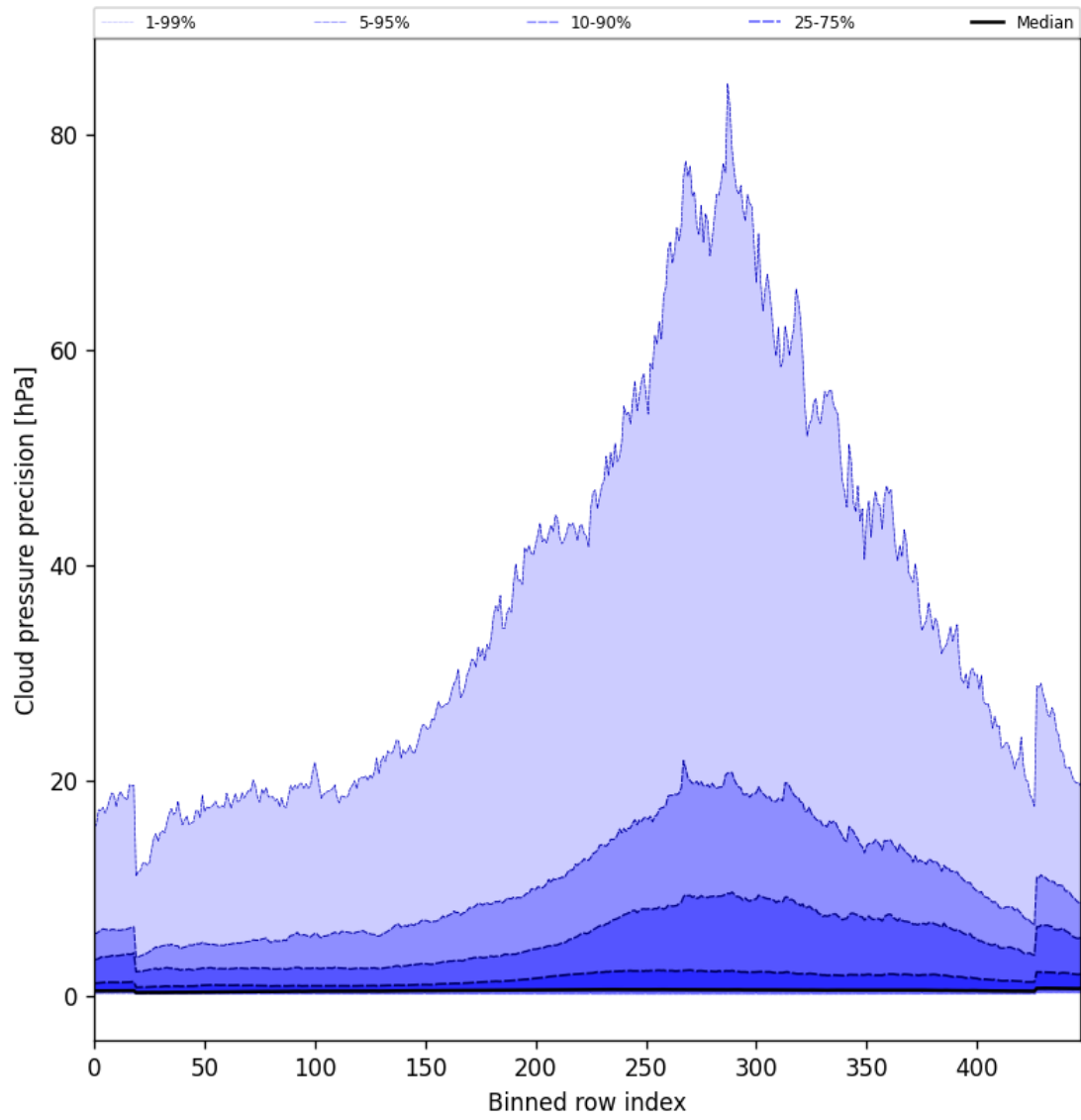
Figure 48: Along track statistics of “Cloud pressure precision” for 2025-11-15 to 2025-11-17
