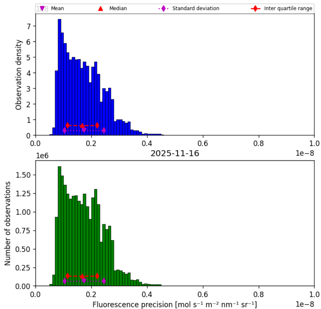
Figure 41: Histogram of “Fluorescence precision” for 2025-11-15 to 2025-11-17
