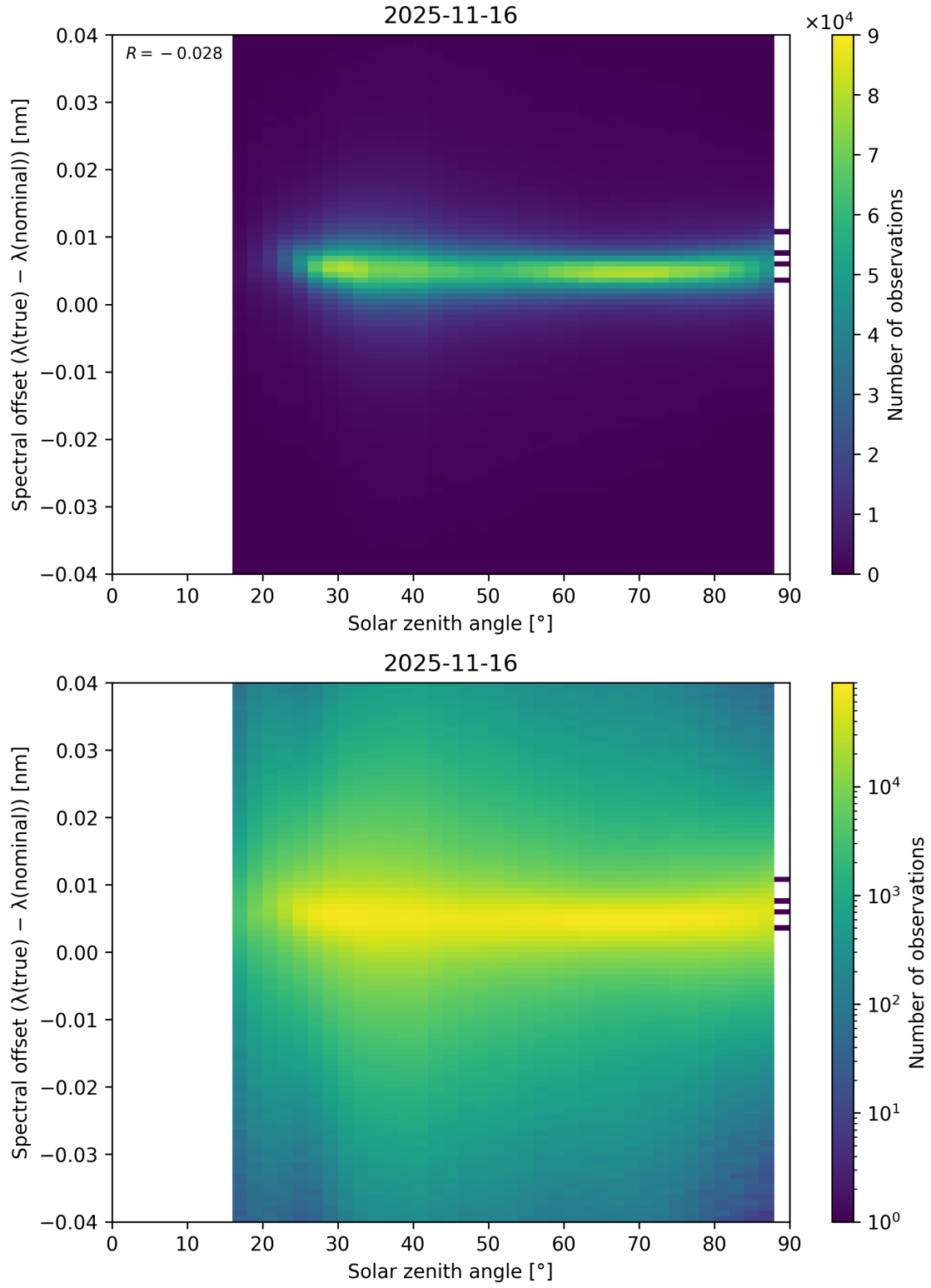
Figure 117: Scatter density plot of “Solar zenith angle” against “Spectral offset ( \lambda_{\text{true}} - \lambda_{\text{nominal}} )” for 2025-11-15 to 2025-11-17.
