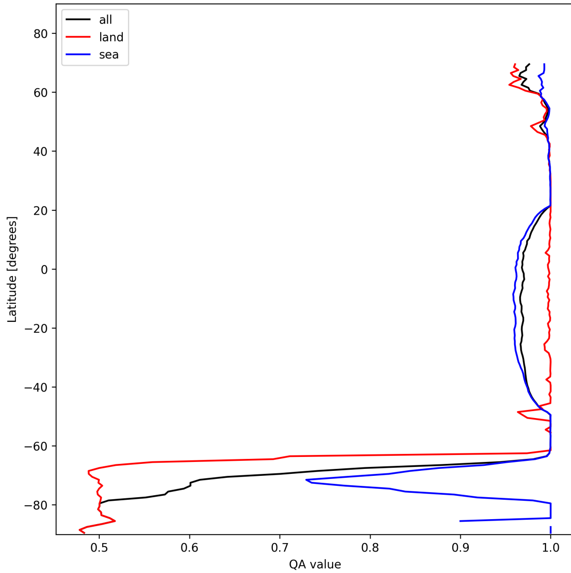
Figure 12: Zonal average of “QA value” for 2025-11-15 to 2025-11-17.
