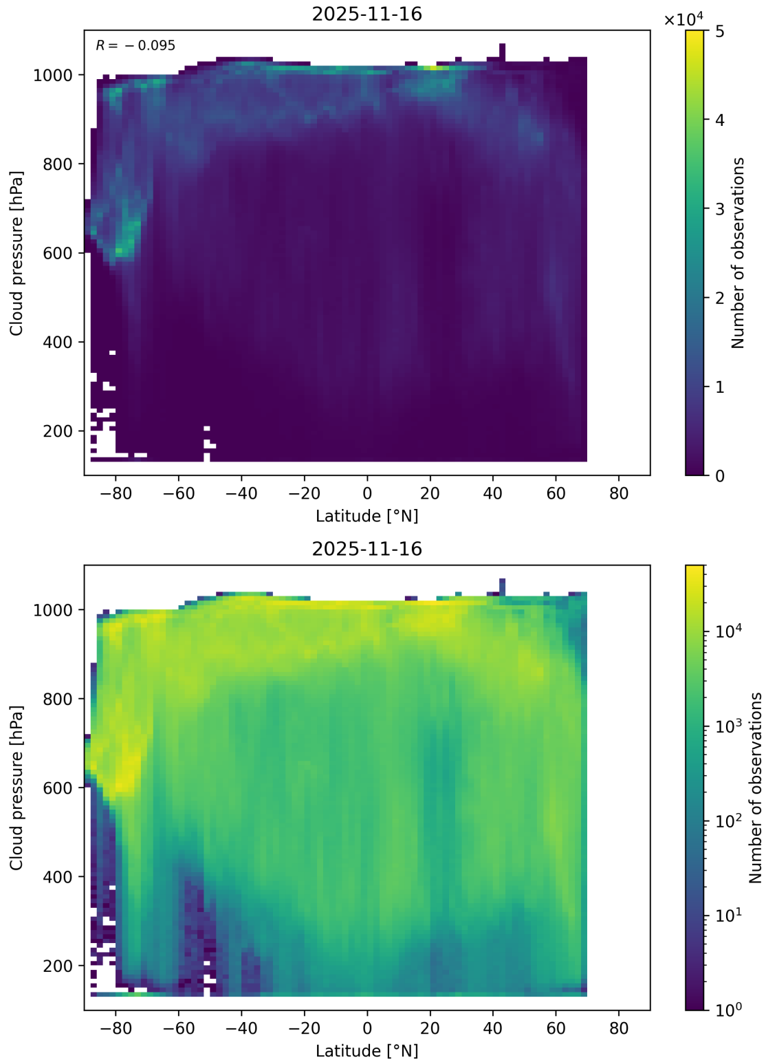
Figure 91: Scatter density plot of “Latitude” against “Cloud pressure” for 2025-11-15 to 2025-11-17.
