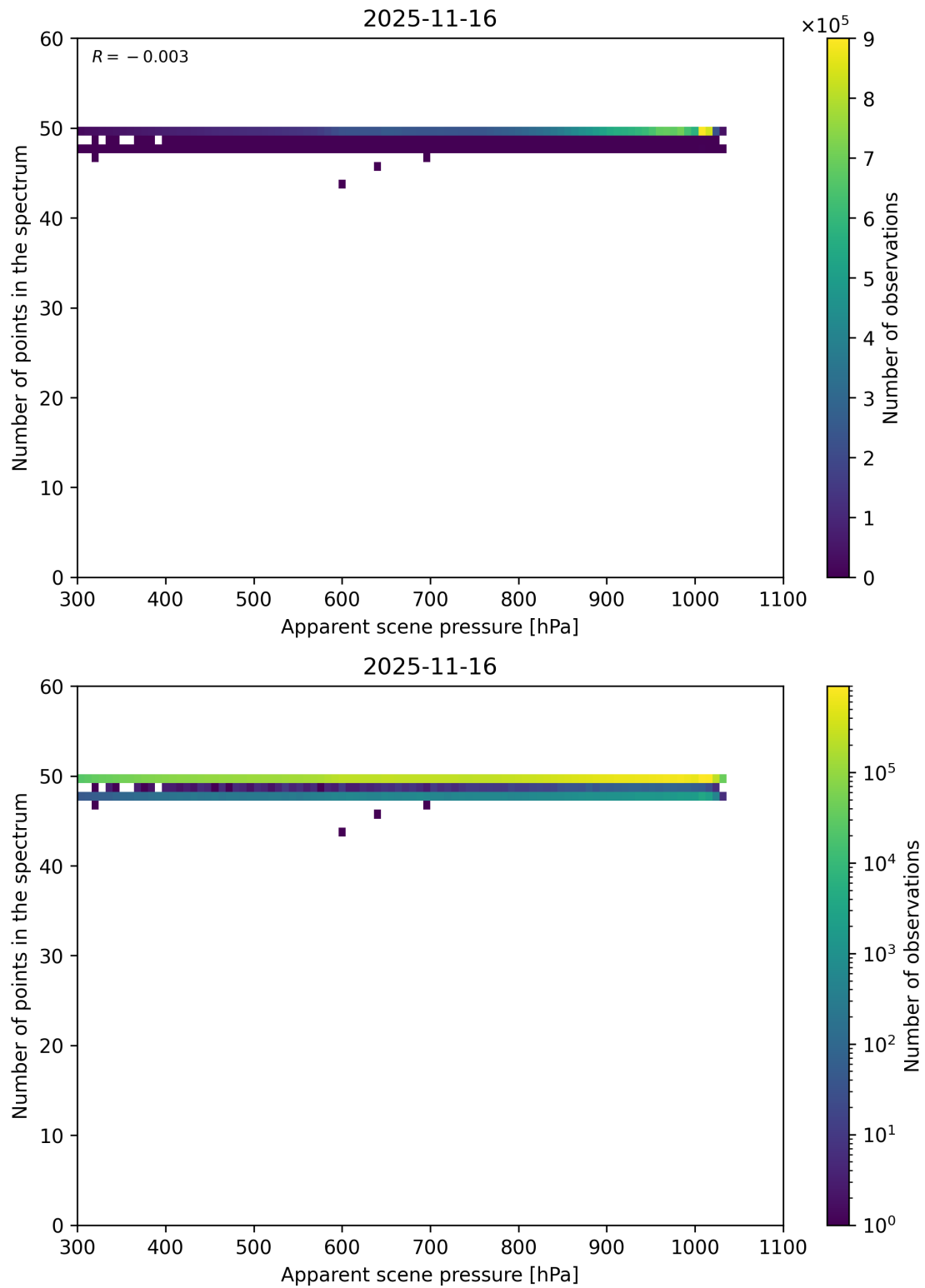
Figure 66: Scatter density plot of “Apparent scene pressure” against “Number of points in the spectrum” for 2025-11-15 to 2025-11-17.
