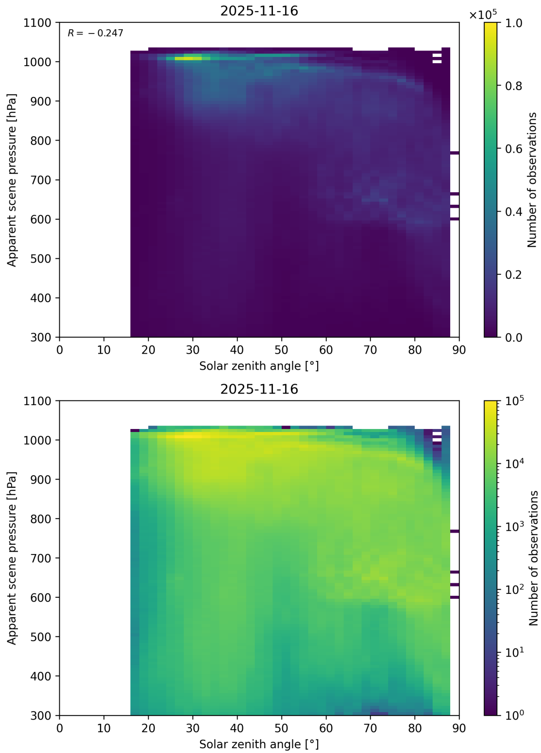
Figure 108: Scatter density plot of “Solar zenith angle” against “Apparent scene pressure” for 2025-11-15 to 2025-11-17.
