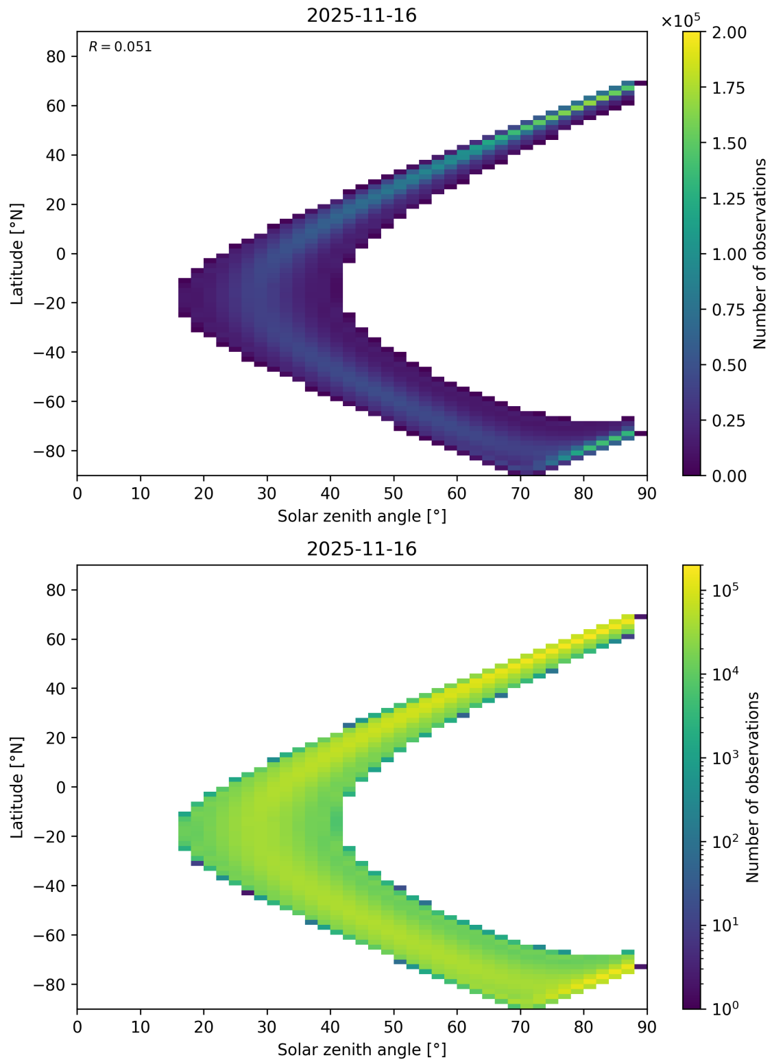
Figure 113: Scatter density plot of “Solar zenith angle” against “Latitude” for 2025-11-15 to 2025-11-17.
