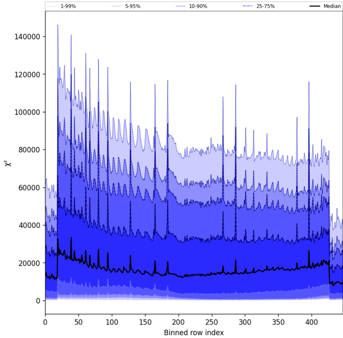
Figure 55: Along track statistics of “ \chi^2 ” for 2025-11-15 to 2025-11-17
