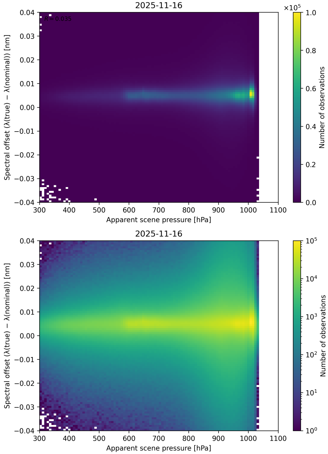
Figure 67: Scatter density plot of “Apparent scene pressure” against “Spectral offset ( \lambda_{\text{true}} - \lambda_{\text{nominal}} )” for 2025-11-15 to 2025-11-17.
