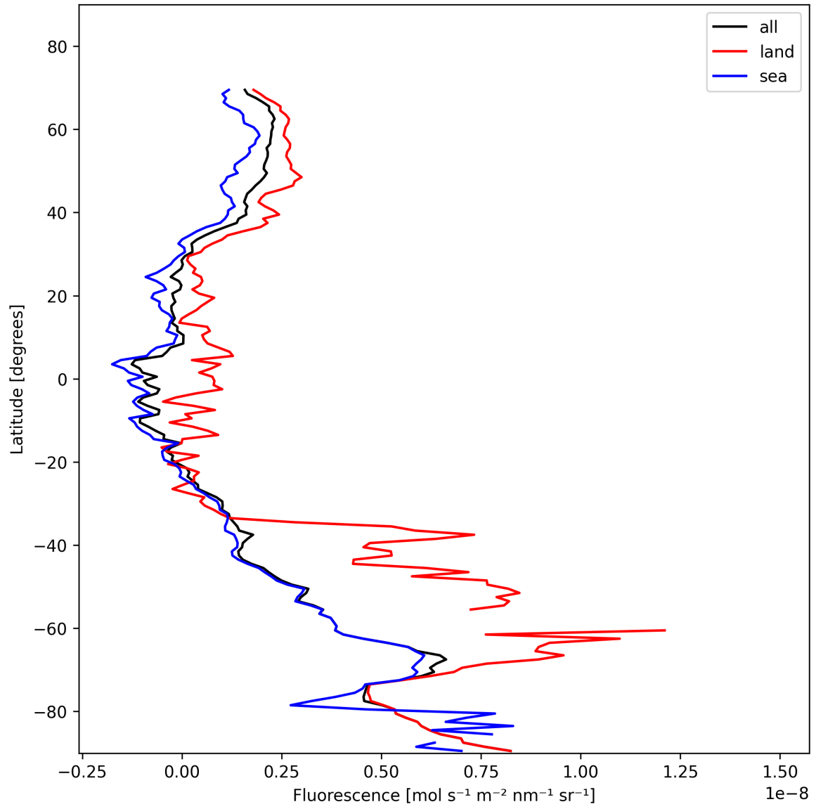
Figure 23: Zonal average of “Fluorescence” for 2025-11-15 to 2025-11-17.
