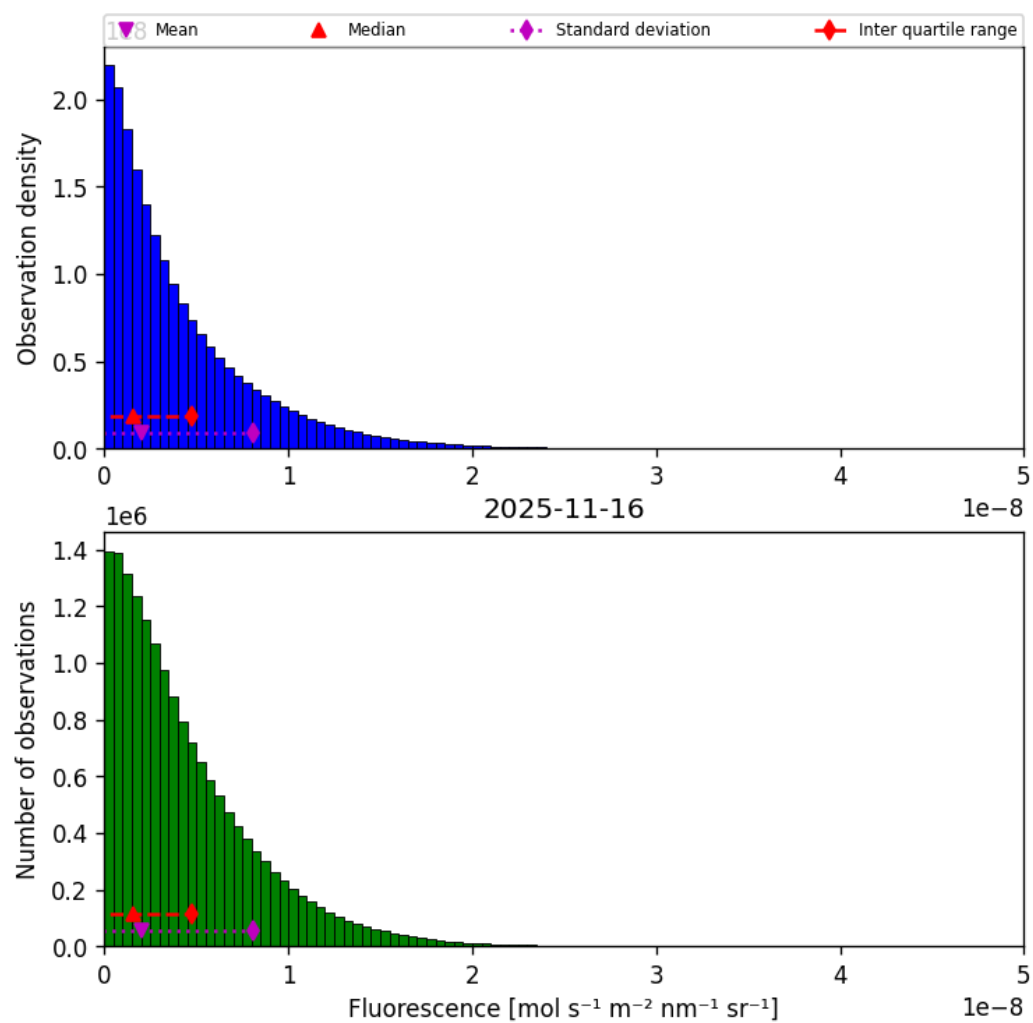
Figure 40: Histogram of “Fluorescence” for 2025-11-15 to 2025-11-17
