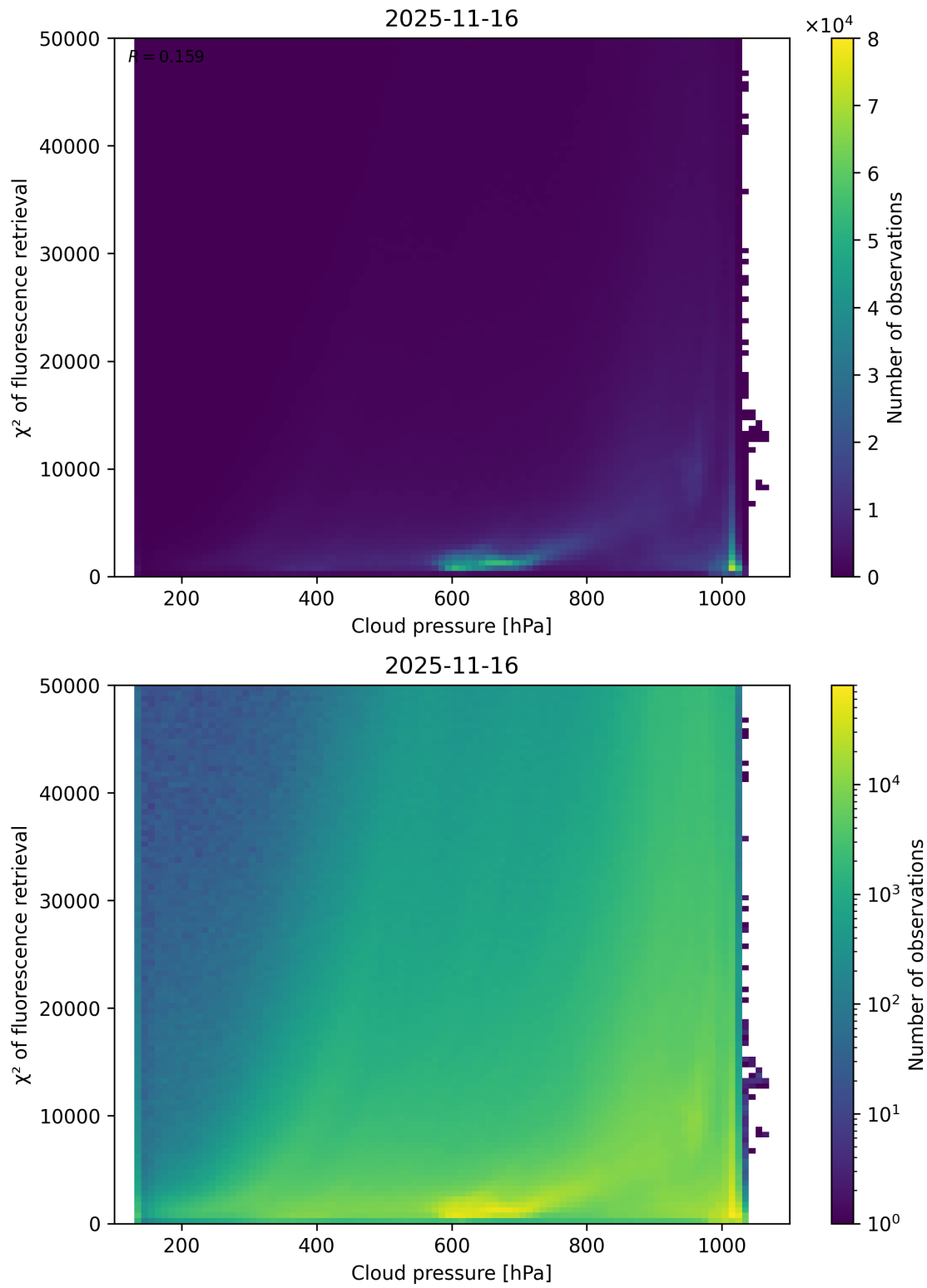
Figure 78: Scatter density plot of “Cloud pressure” against “ \chi^2 of fluorescence retrieval” for 2025-11-15 to 2025-11-17.
