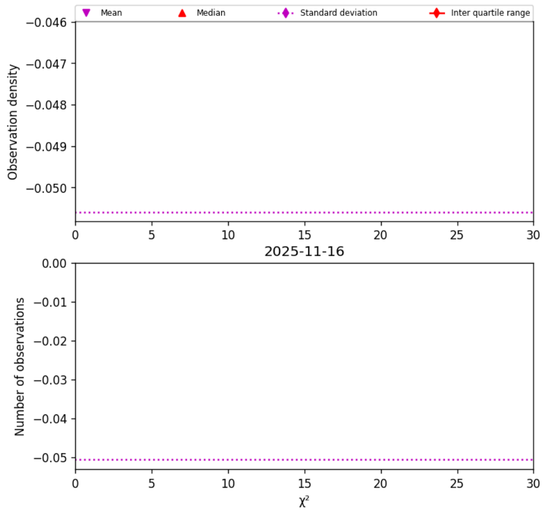
Figure 38: Histogram of " \chi^2 " for 2025-11-15 to 2025-11-17
