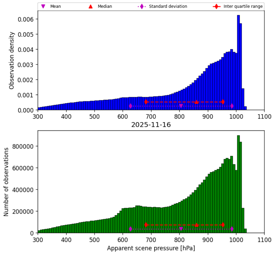
Figure 36: Histogram of “Apparent scene pressure” for 2025-11-15 to 2025-11-17
