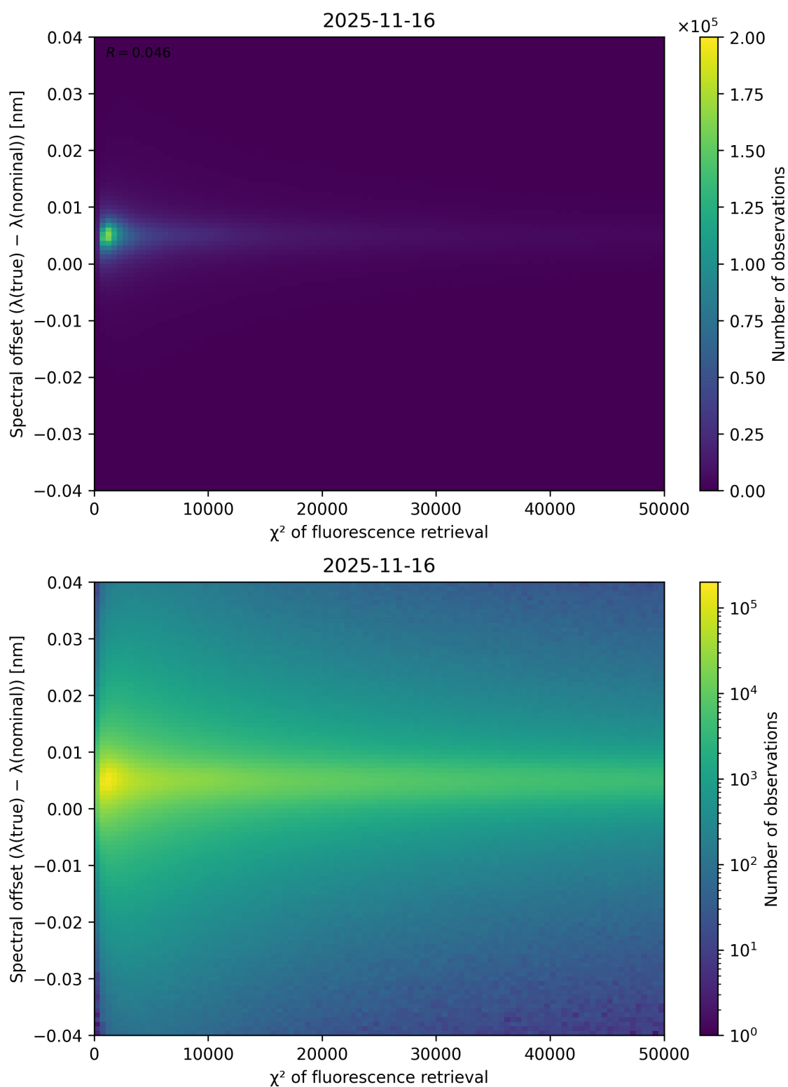
Figure 69: Scatter density plot of “ \chi^2 of fluorescence retrieval” against “Spectral offset ( \lambda_{\text{true}} - \lambda_{\text{nominal}} )” for 2025-11-15 to 2025-11-17.
