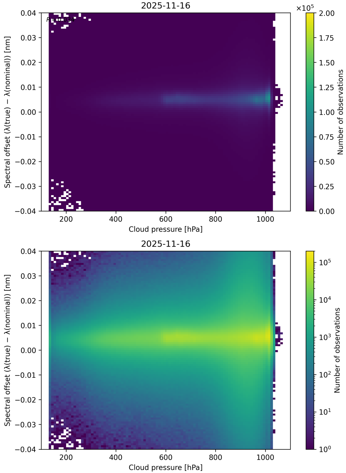
Figure 84: Scatter density plot of “Cloud pressure” against “Spectral offset ( \lambda_{\text{true}} - \lambda_{\text{nominal}} )” for 2025-11-15 to 2025-11-17.
