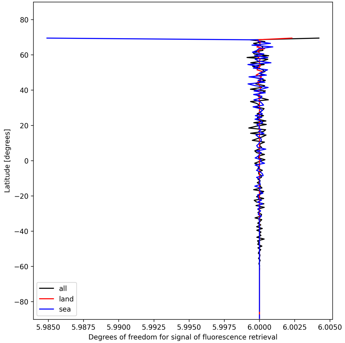
Figure 26: Zonal average of “Degrees of freedom for signal of fluorescence retrieval” for 2025-11-15 to 2025-11-17.
