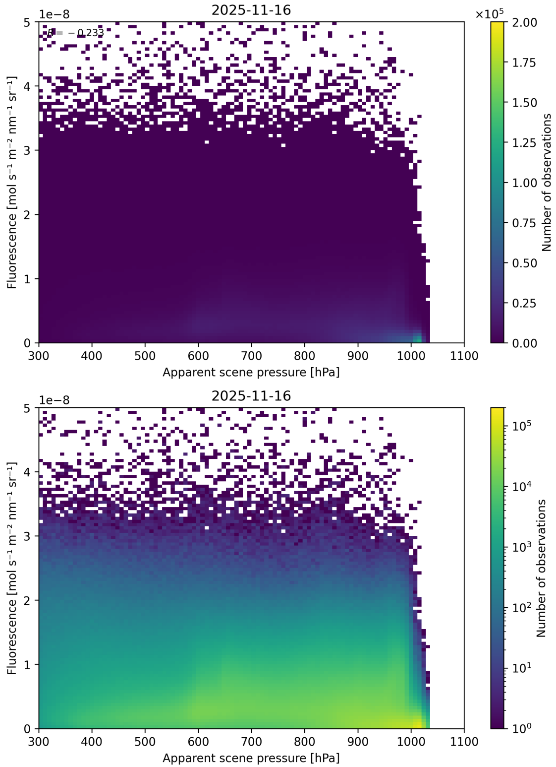
Figure 64: Scatter density plot of “Apparent scene pressure” against “Fluorescence” for 2025-11-15 to 2025-11-17.
