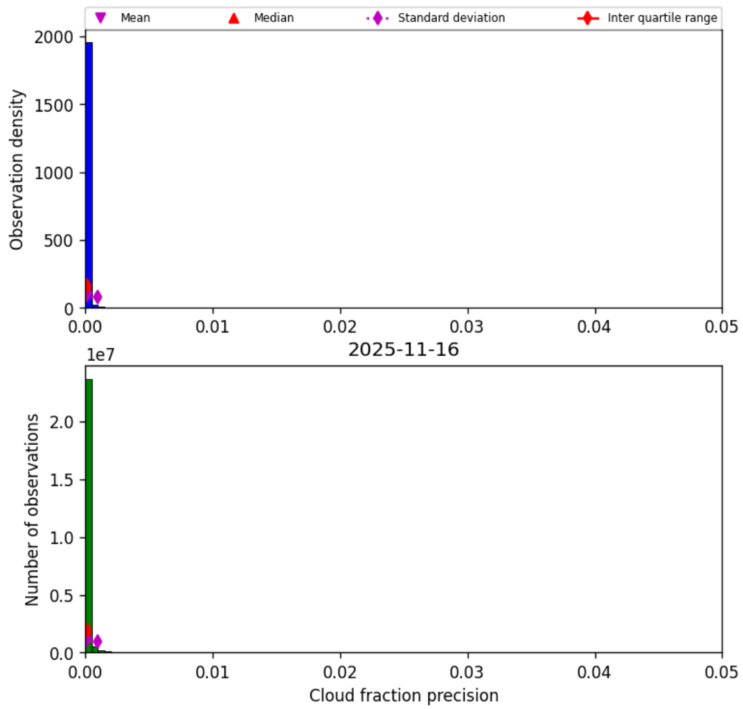
Figure 33: Histogram of “Cloud fraction precision” for 2025-11-15 to 2025-11-17
