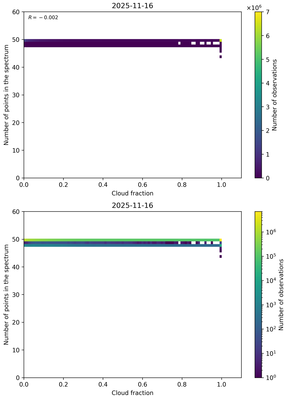
Figure 74: Scatter density plot of “Cloud fraction” against “Number of points in the spectrum” for 2025-11-15 to 2025-11-17.
