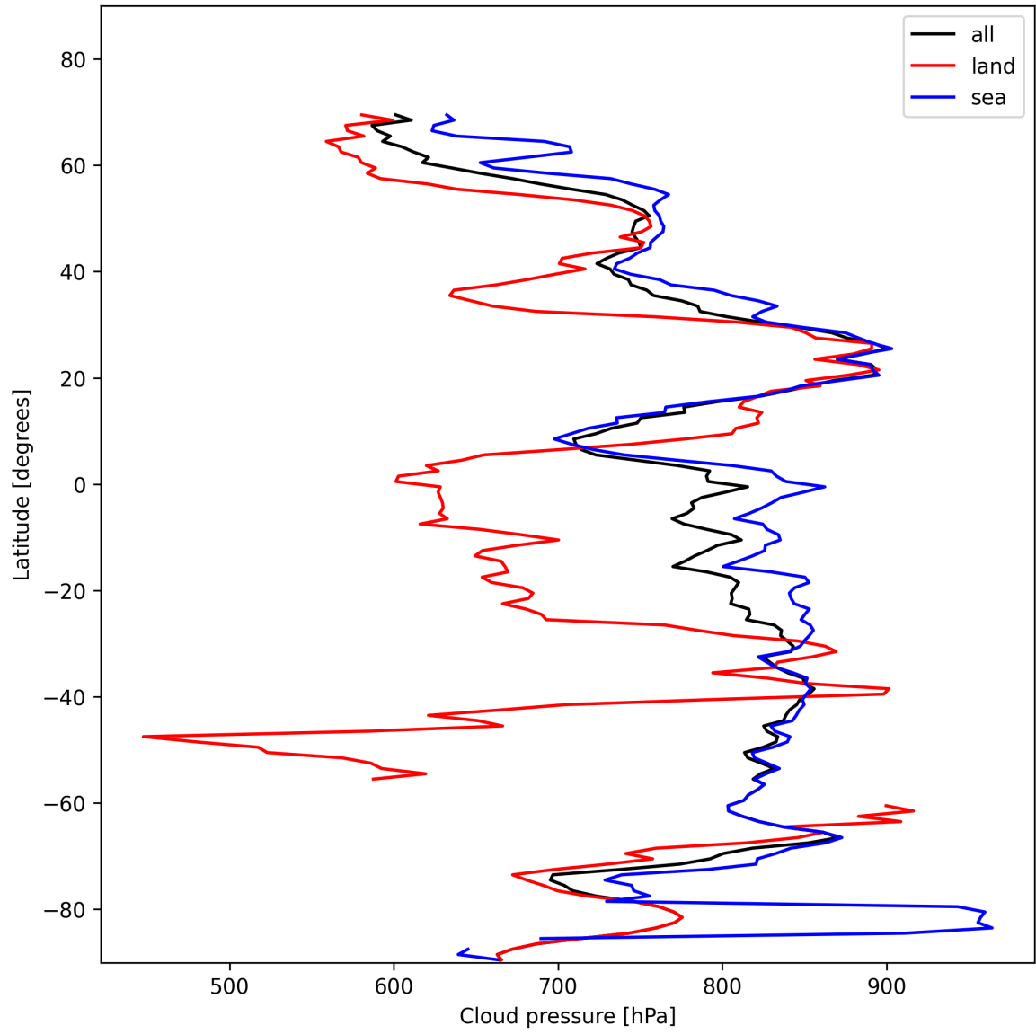
Figure 13: Zonal average of “Cloud pressure” for 2025-11-15 to 2025-11-17.
