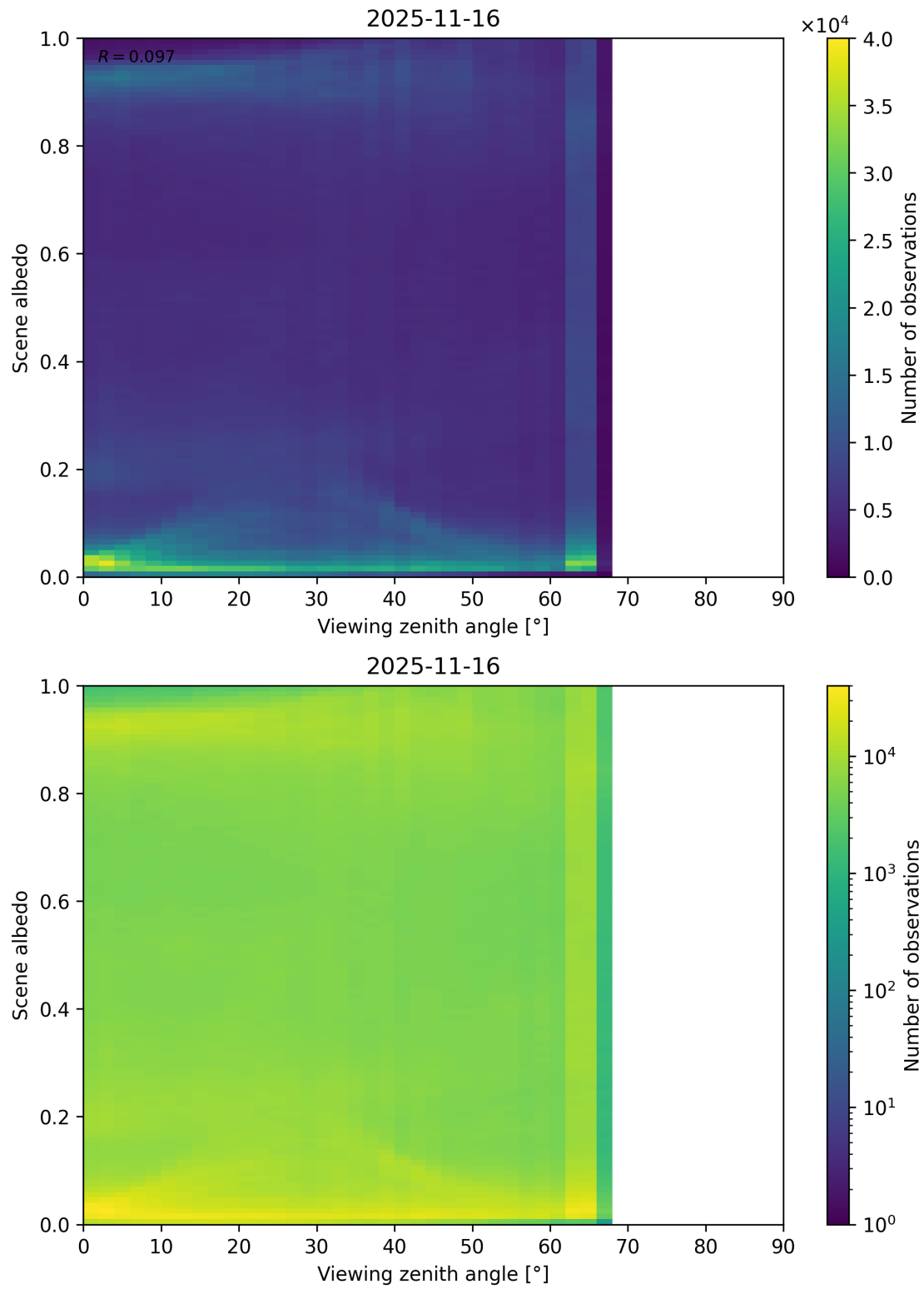
Figure 126: Scatter density plot of “Viewing zenith angle” against “Scene albedo” for 2025-11-15 to 2025-11-17.
