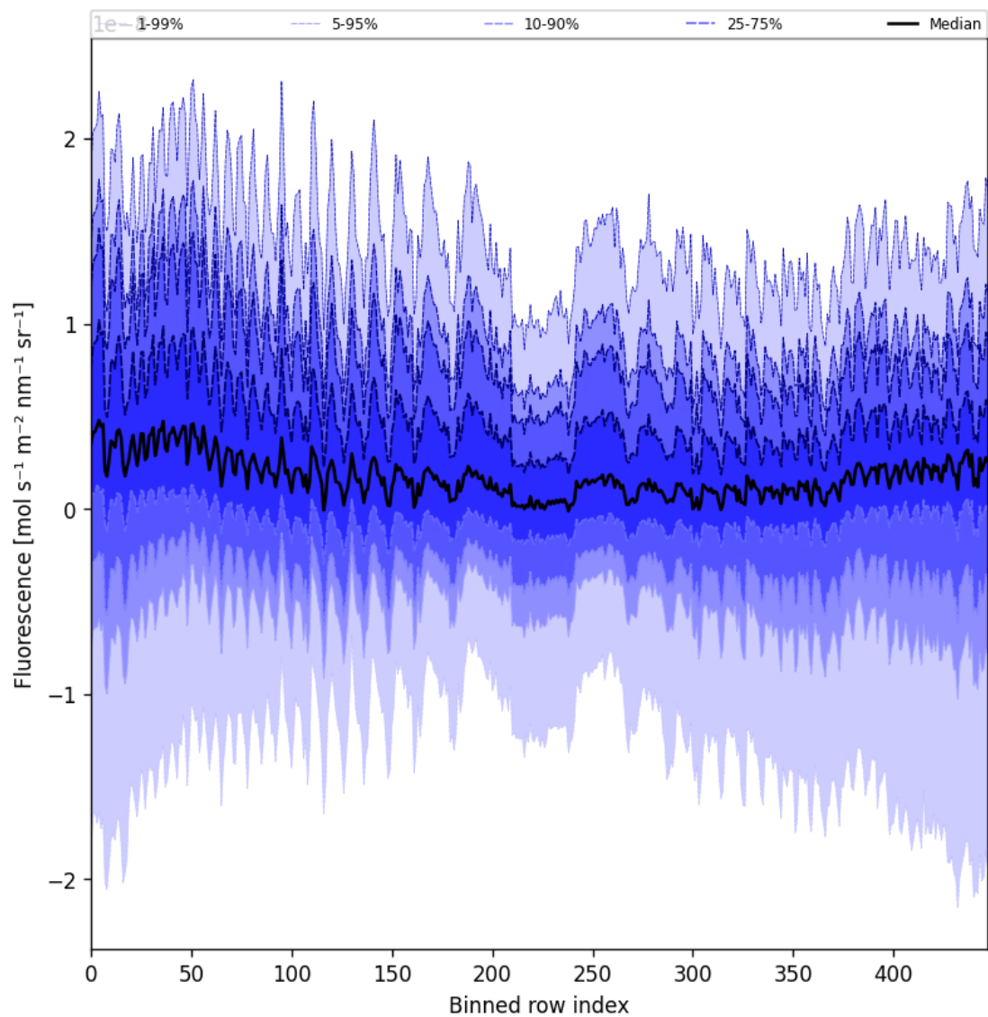
Figure 57: Along track statistics of “Fluorescence” for 2025-11-15 to 2025-11-17
