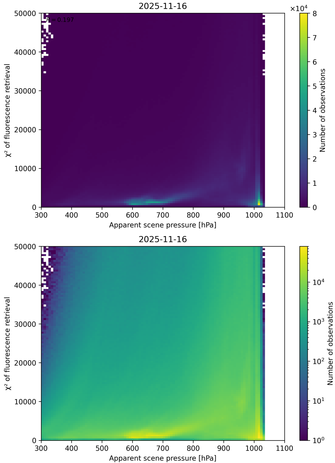
Figure 63: Scatter density plot of “Apparent scene pressure” against “ \chi^2 of fluorescence retrieval” for 2025-11-15 to 2025-11-17.
