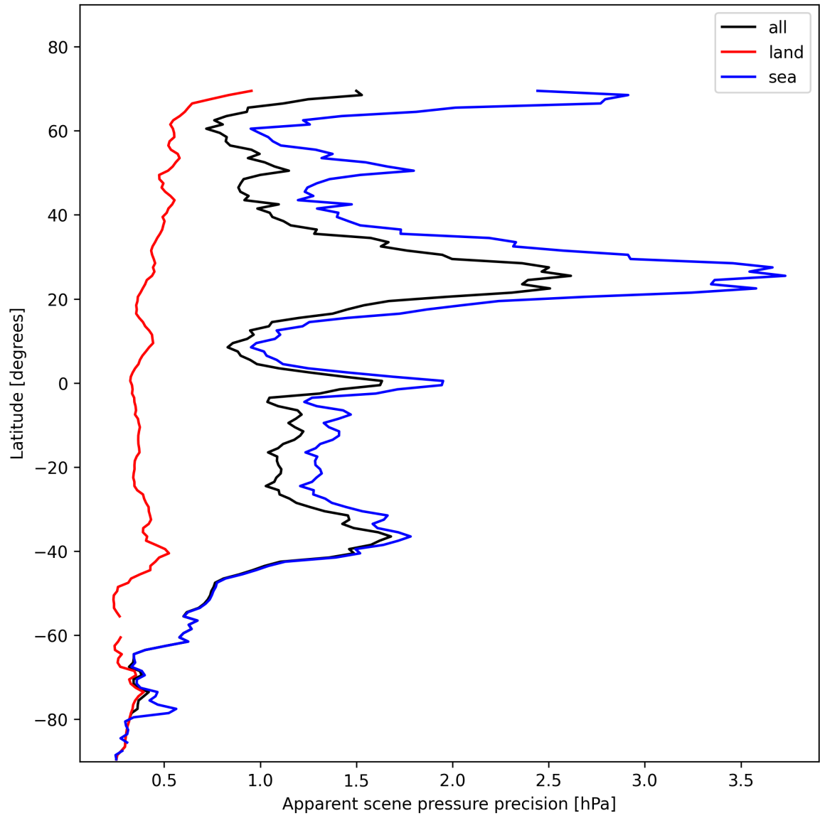
Figure 20: Zonal average of “Apparent scene pressure precision” for 2025-11-15 to 2025-11-17.
