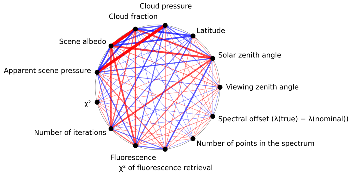
Figure 1: Map of correlation graph for 2025-11-15 to 2025-11-17.
