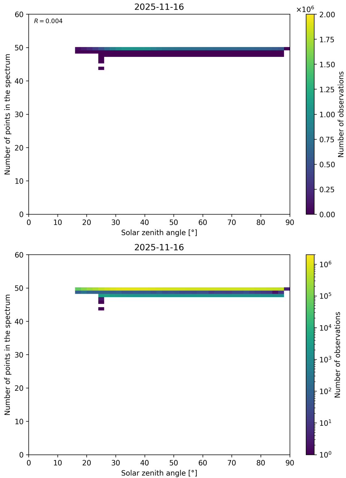
Figure 115: Scatter density plot of “Solar zenith angle” against “Number of points in the spectrum” for 2025-11-15 to 2025-11-17.
