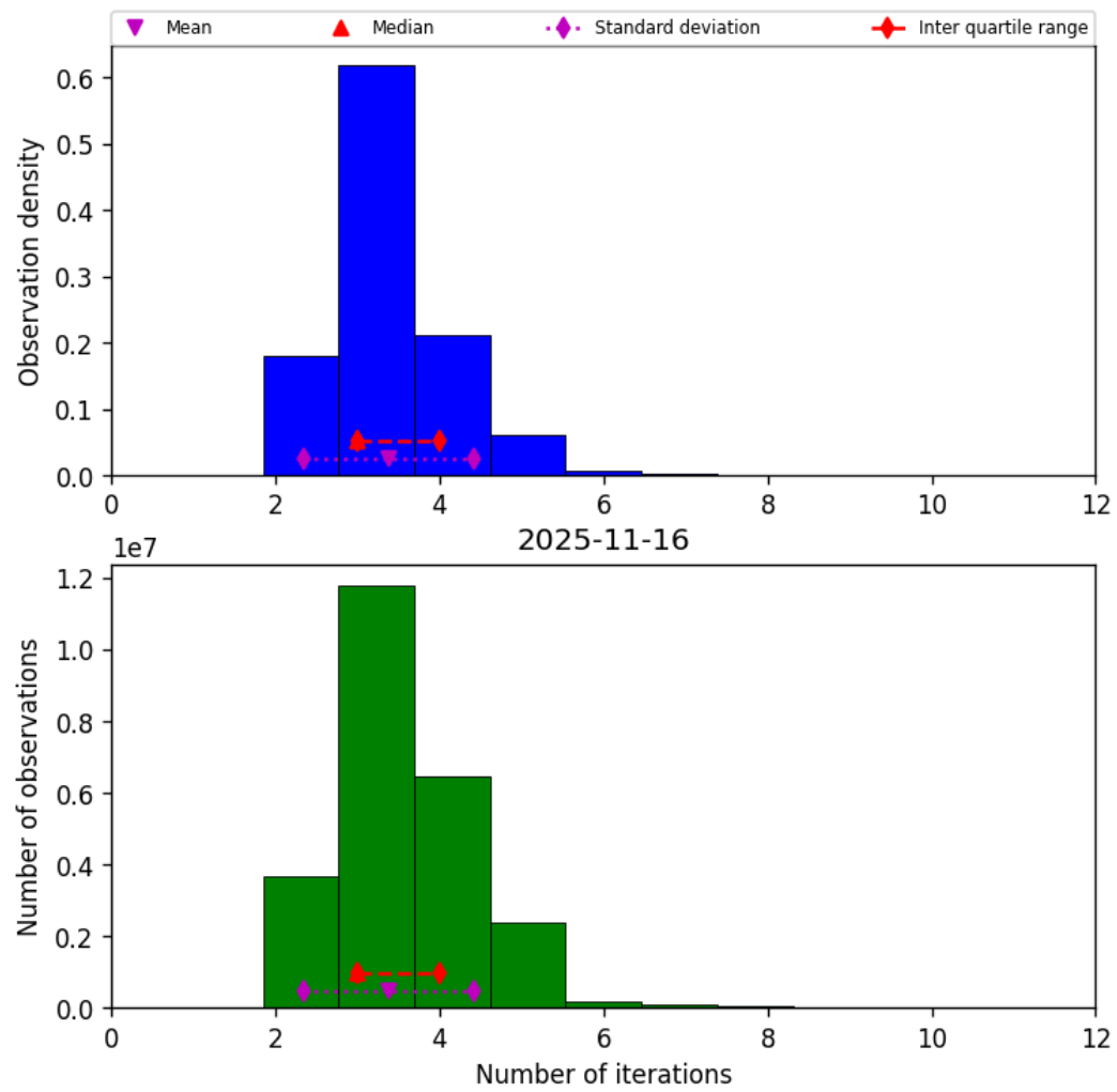
Figure 39: Histogram of “Number of iterations” for 2025-11-15 to 2025-11-17
