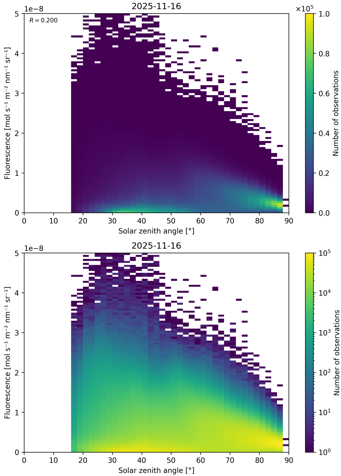
Figure 112: Scatter density plot of “Solar zenith angle” against “Fluorescence” for 2025-11-15 to 2025-11-17.
