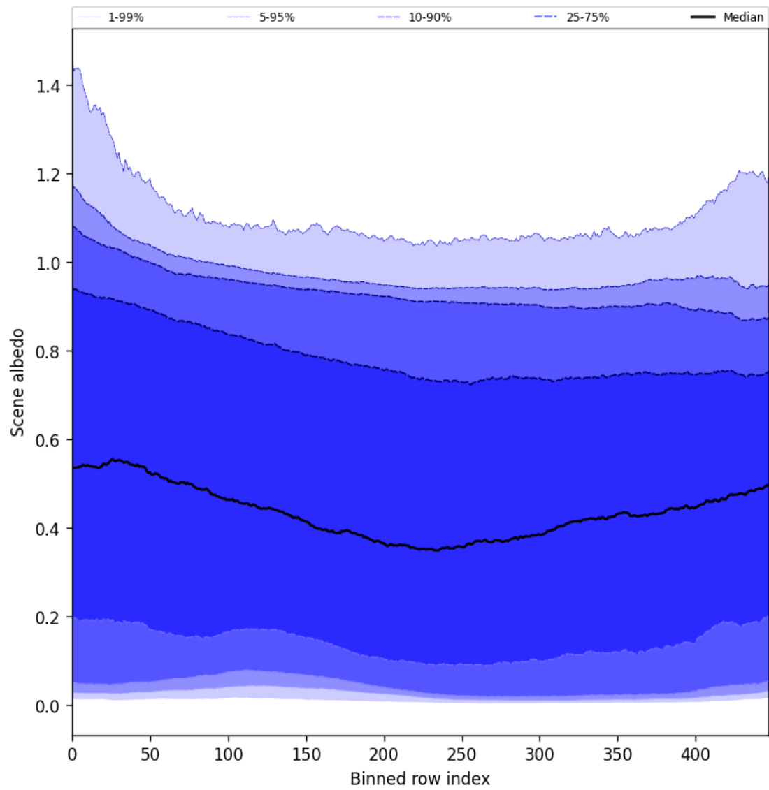
Figure 51: Along track statistics of “Scene albedo” for 2025-11-15 to 2025-11-17
