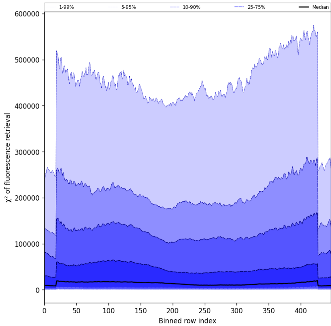
Figure 59: Along track statistics of “ \chi^2 of fluorescence retrieval” for 2025-11-15 to 2025-11-17
