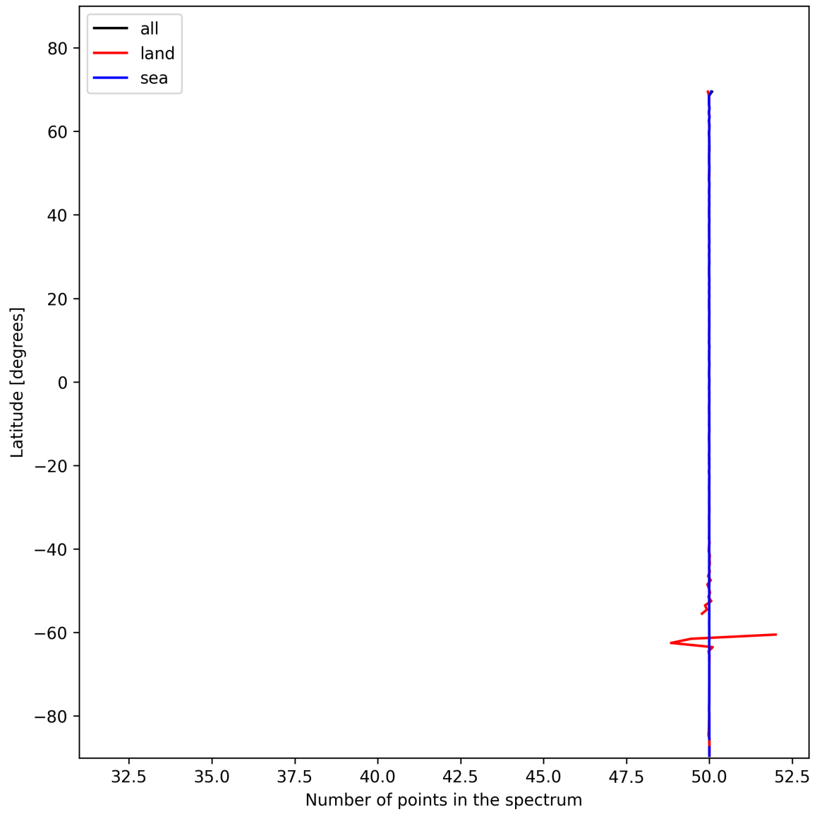
Figure 27: Zonal average of “Number of points in the spectrum” for 2025-11-15 to 2025-11-17.
