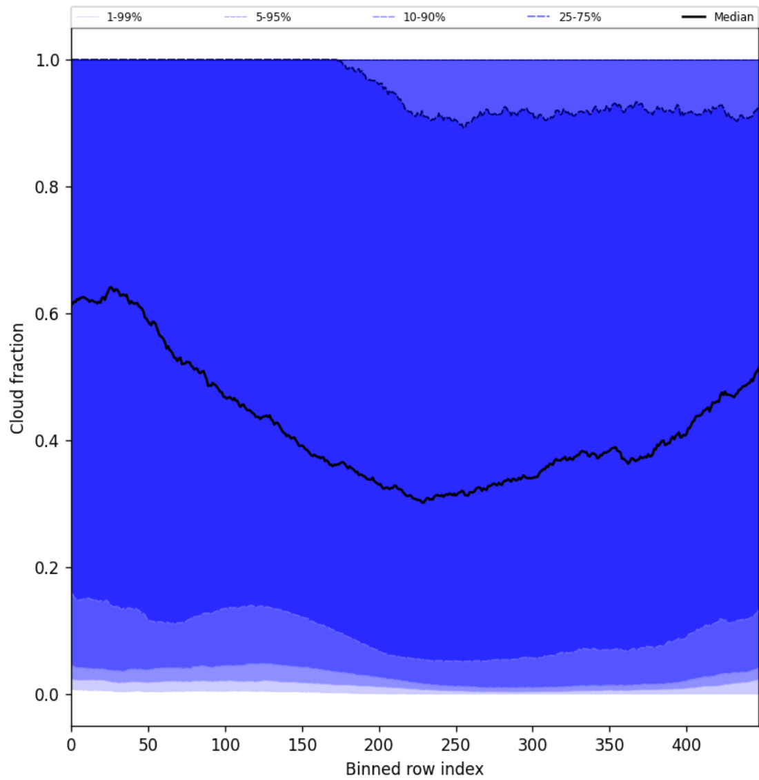
Figure 49: Along track statistics of “Cloud fraction” for 2025-11-15 to 2025-11-17
