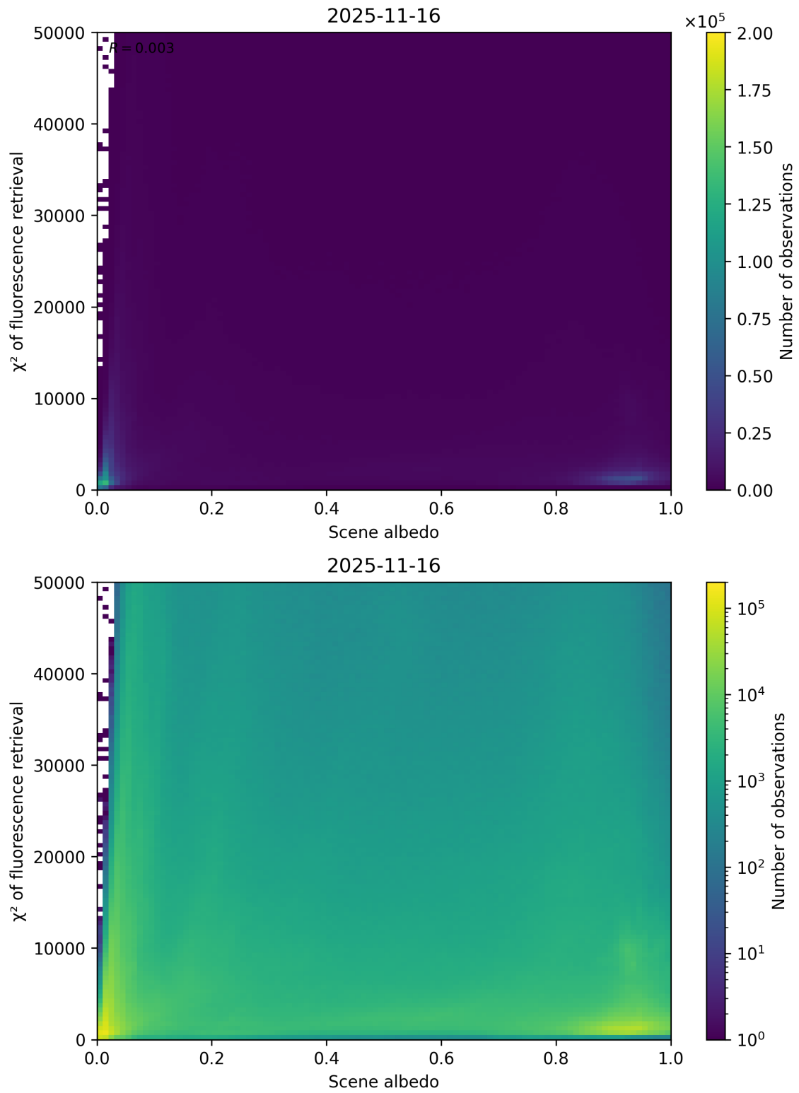
Figure 103: Scatter density plot of “Scene albedo” against “ \chi^2 of fluorescence retrieval” for 2025-11-15 to 2025-11-17.
