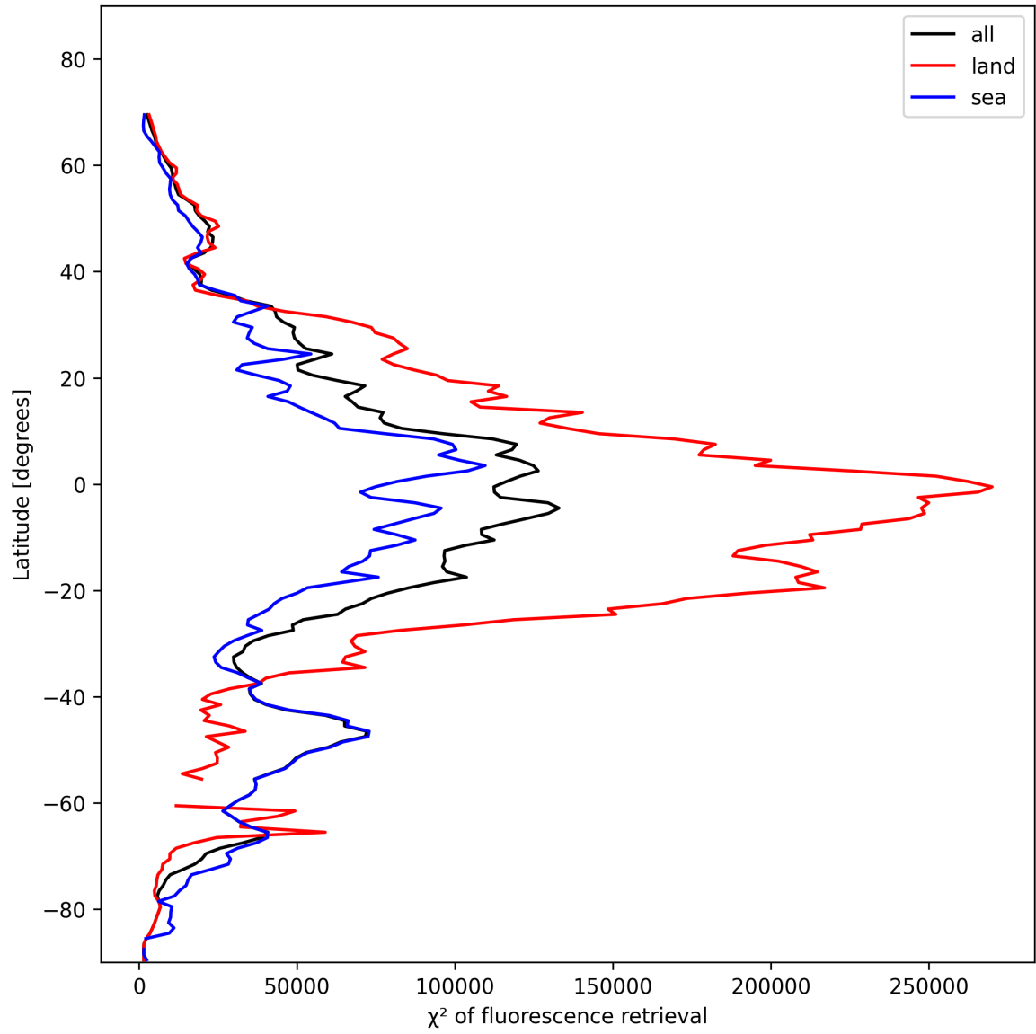
Figure 25: Zonal average of “ \chi^2 of fluorescence retrieval” for 2025-11-15 to 2025-11-17.
