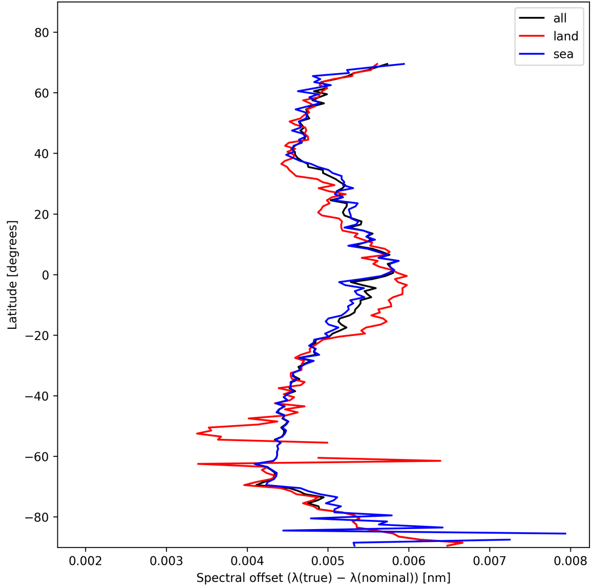
Figure 28: Zonal average of “Spectral offset ( \lambda_{\text{true}} - \lambda_{\text{nominal}} )” for 2025-11-15 to 2025-11-17.
