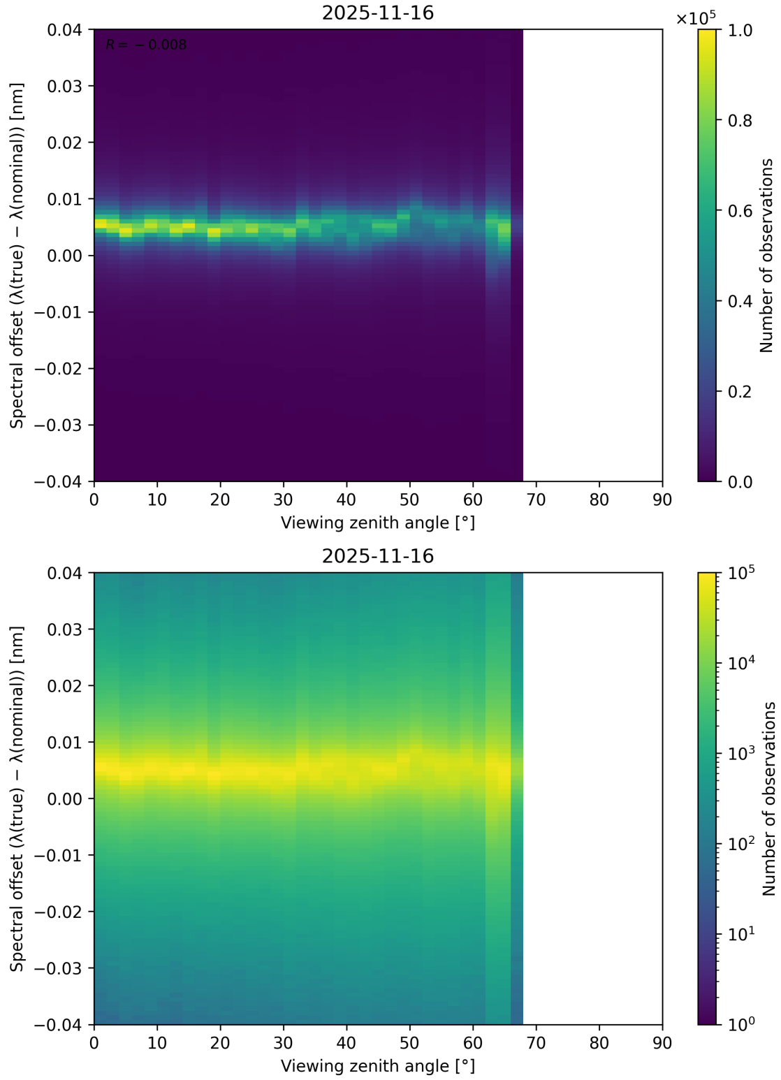
Figure 128: Scatter density plot of “Viewing zenith angle” against “Spectral offset ( \lambda_{\text{true}} - \lambda_{\text{nominal}} )” for 2025-11-15 to 2025-11-17.
