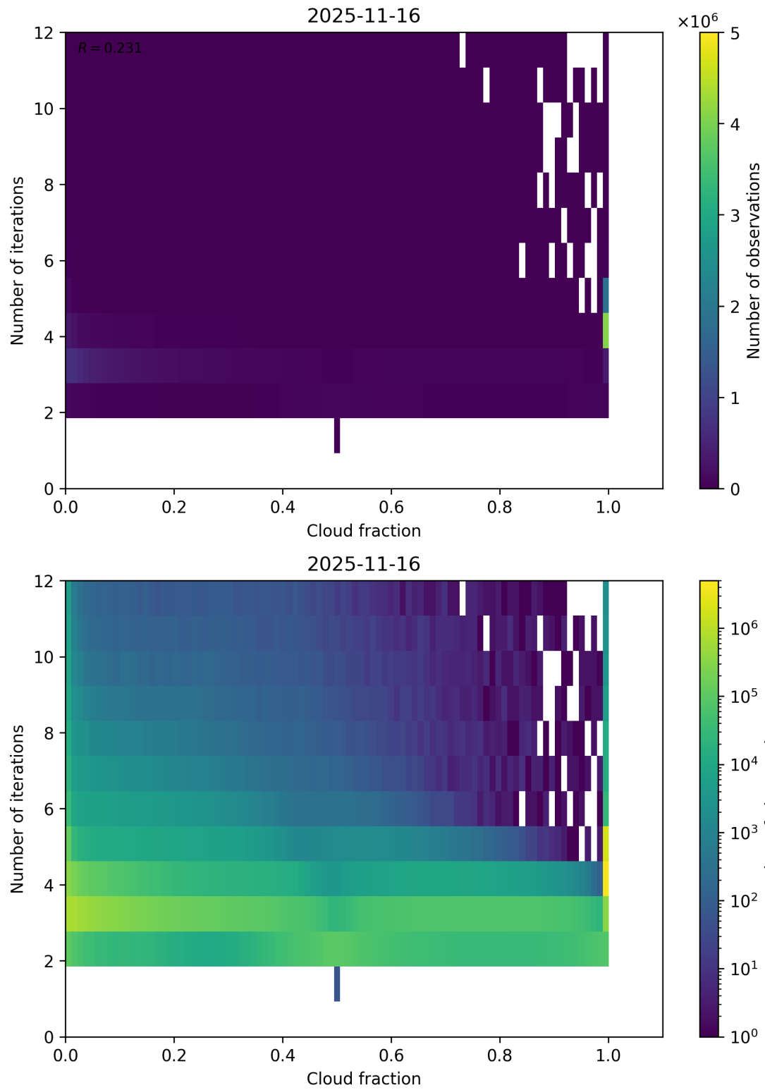
Figure 73: Scatter density plot of “Cloud fraction” against “Number of iterations” for 2025-11-15 to 2025-11-17.
