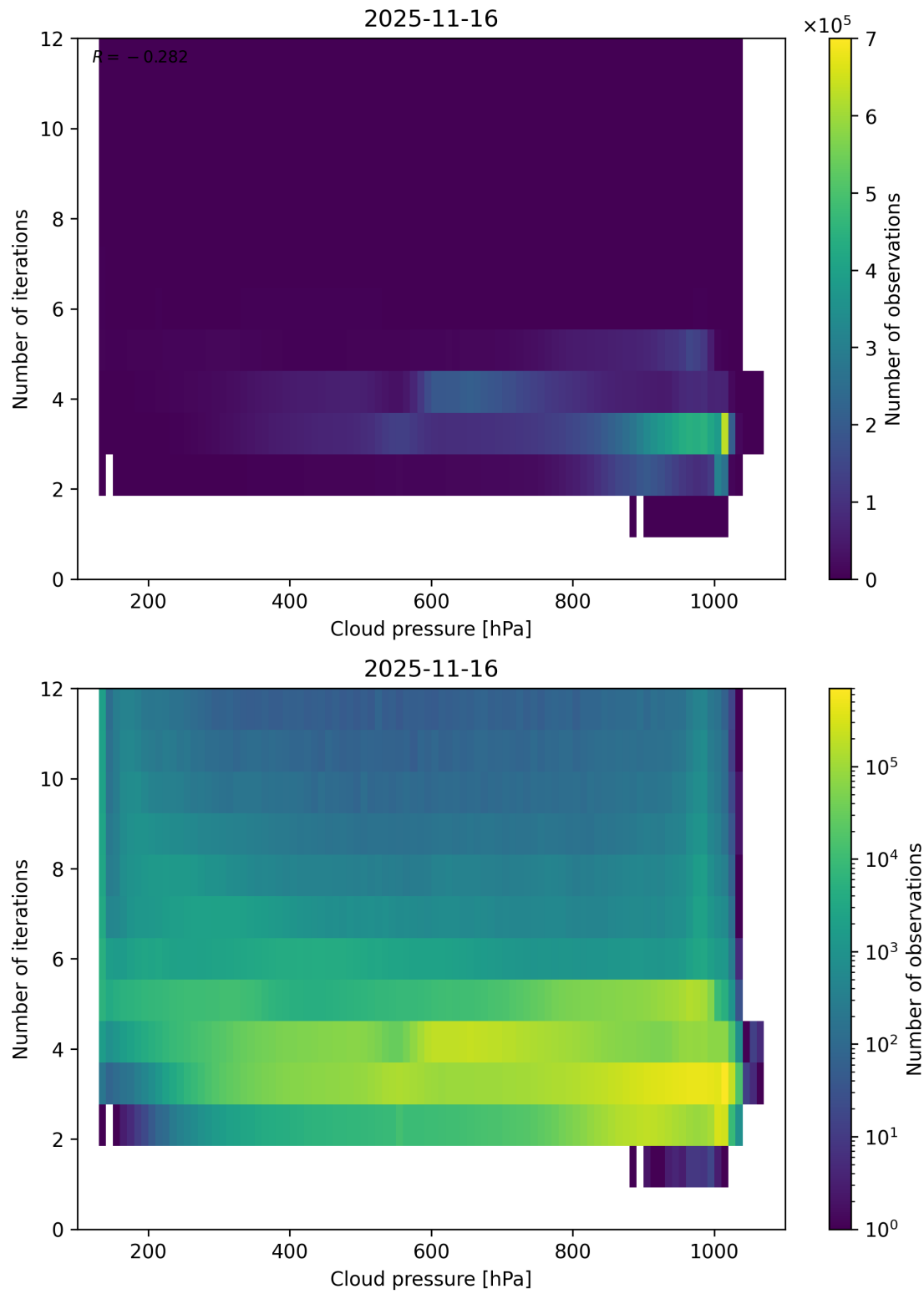
Figure 81: Scatter density plot of “Cloud pressure” against “Number of iterations” for 2025-11-15 to 2025-11-17.
