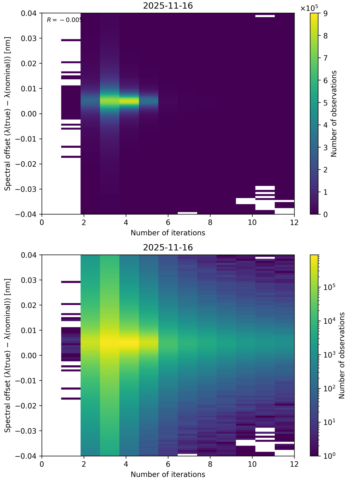
Figure 100: Scatter density plot of “Number of iterations” against “Spectral offset ( \lambda_{\text{true}} - \lambda_{\text{nominal}} )” for 2025-11-15 to 2025-11-17.
