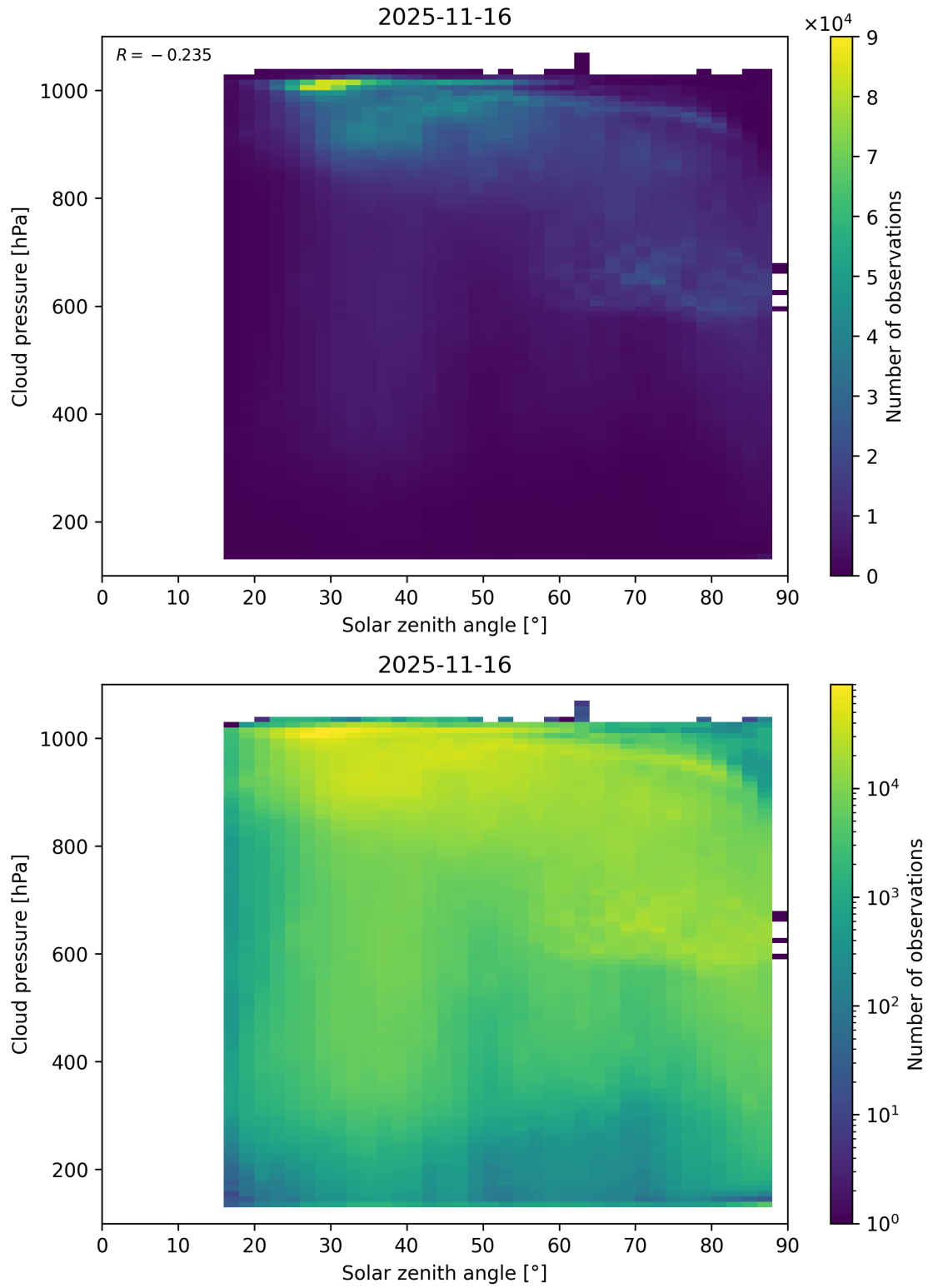
Figure 111: Scatter density plot of “Solar zenith angle” against “Cloud pressure” for 2025-11-15 to 2025-11-17.
