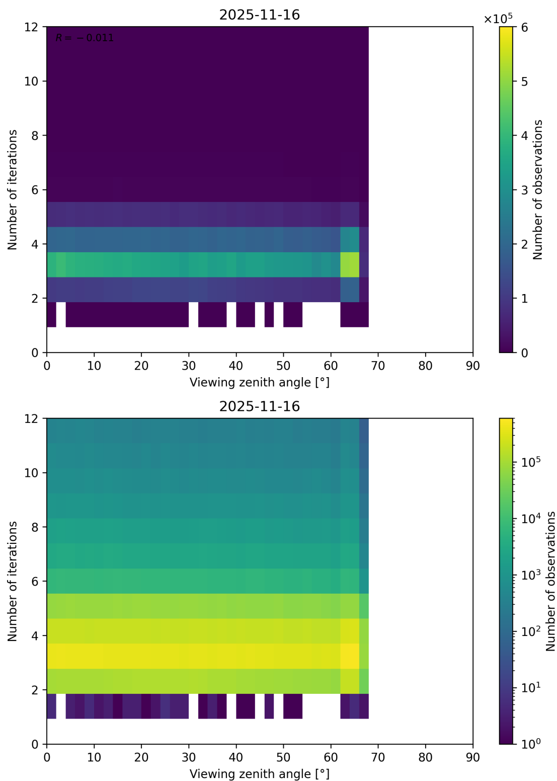
Figure 124: Scatter density plot of “Viewing zenith angle” against “Number of iterations” for 2025-11-15 to 2025-11-17.
