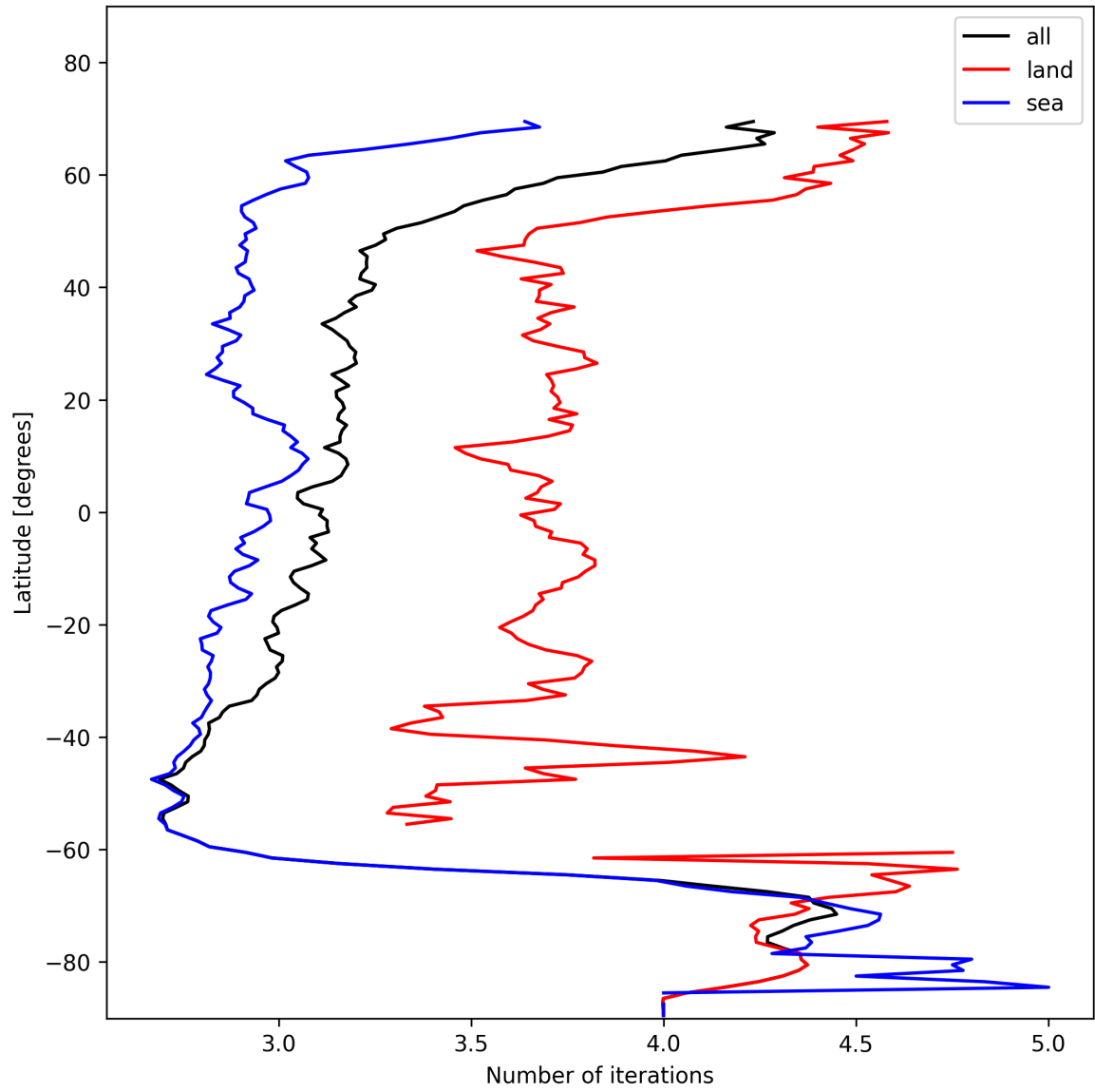
Figure 22: Zonal average of “Number of iterations” for 2025-11-15 to 2025-11-17.
