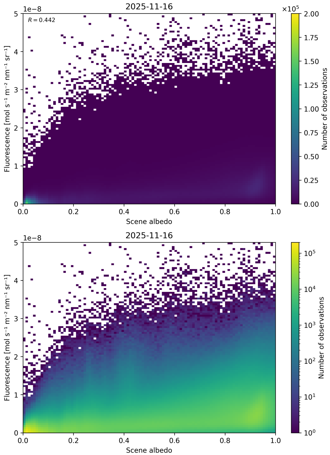
Figure 104: Scatter density plot of “Scene albedo” against “Fluorescence” for 2025-11-15 to 2025-11-17.
