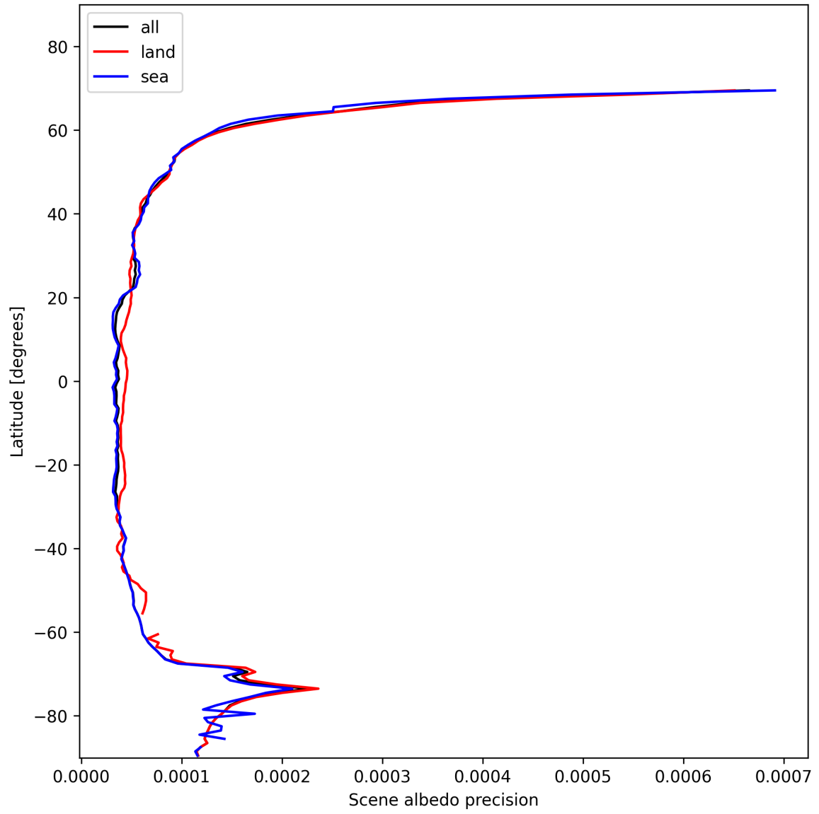
Figure 18: Zonal average of “Scene albedo precision” for 2025-11-15 to 2025-11-17.
