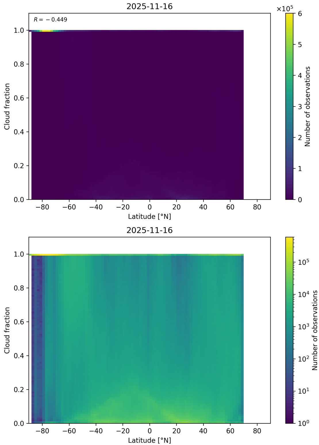
Figure 90: Scatter density plot of “Latitude” against “Cloud fraction” for 2025-11-15 to 2025-11-17.
