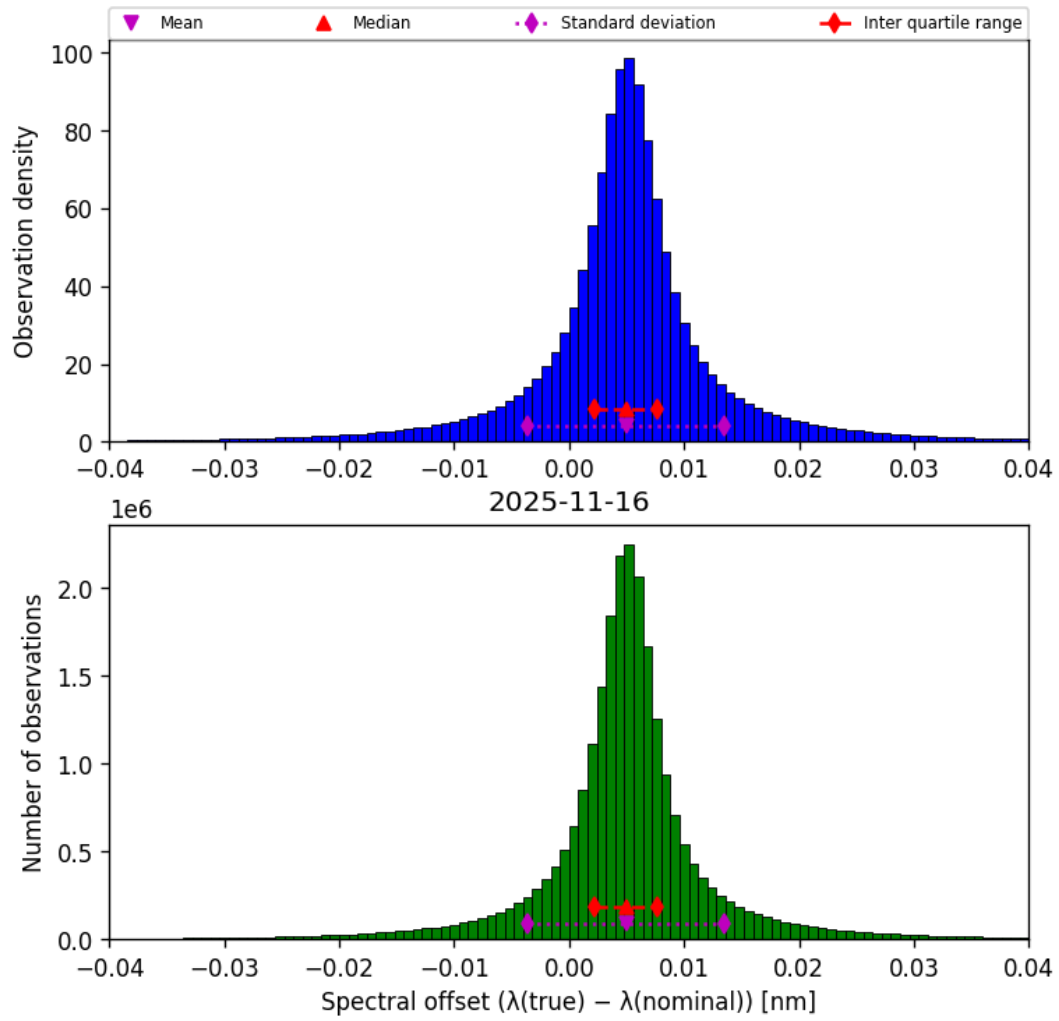
Figure 45: Histogram of “Spectral offset ( \lambda_{\text{true}} - \lambda_{\text{nominal}} )” for 2025-11-15 to 2025-11-17
