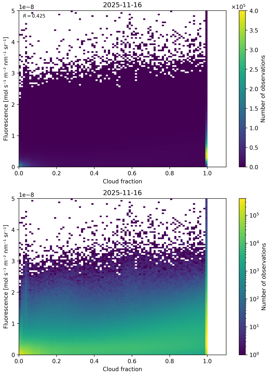
Figure 72: Scatter density plot of “Cloud fraction” against “Fluorescence” for 2025-11-15 to 2025-11-17.
