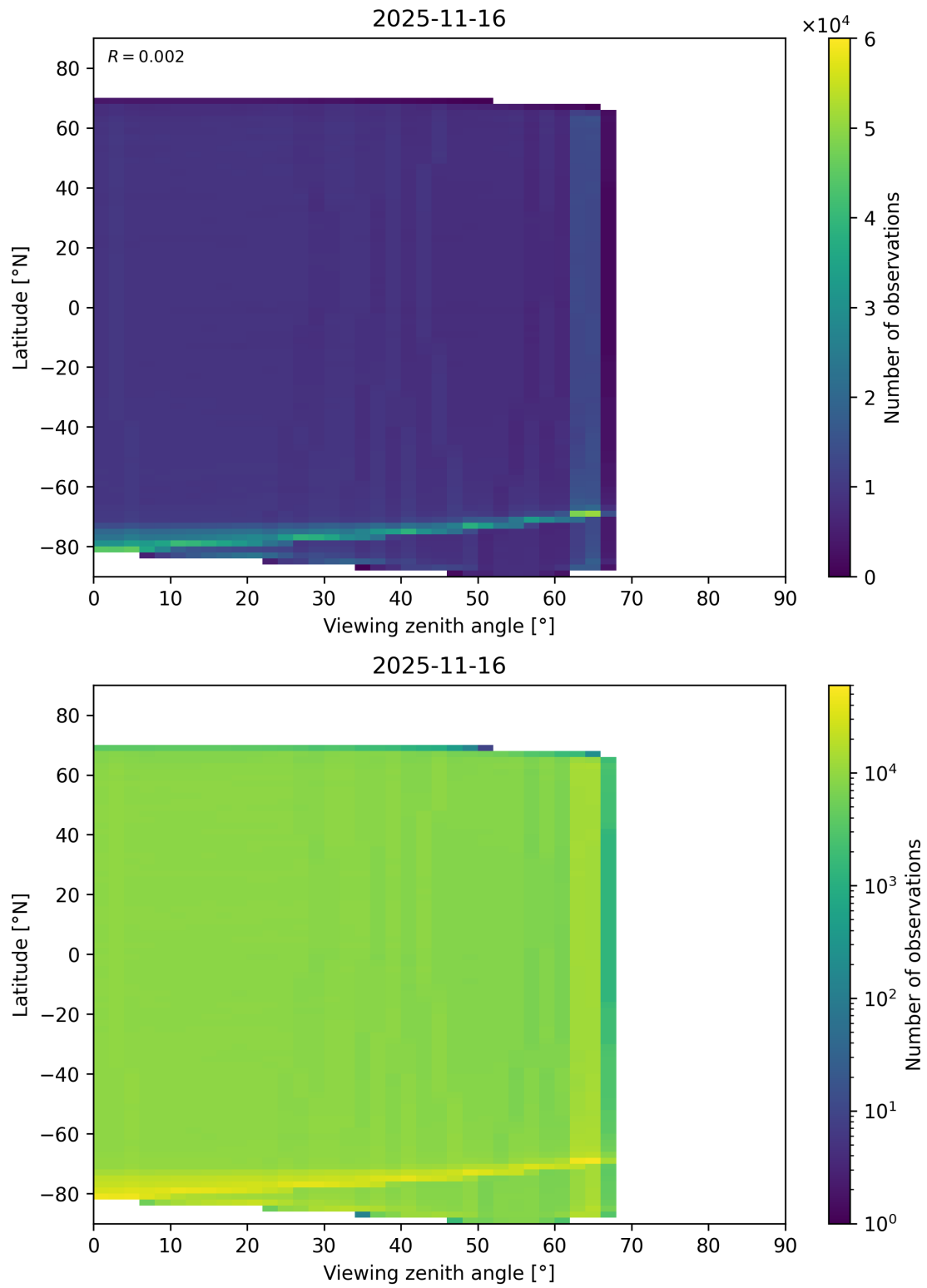
Figure 123: Scatter density plot of “Viewing zenith angle” against “Latitude” for 2025-11-15 to 2025-11-17.
