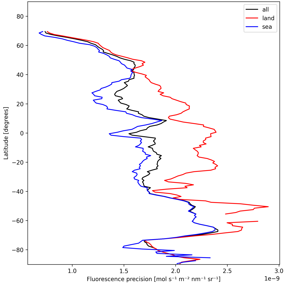
Figure 24: Zonal average of “Fluorescence precision” for 2025-11-15 to 2025-11-17.
