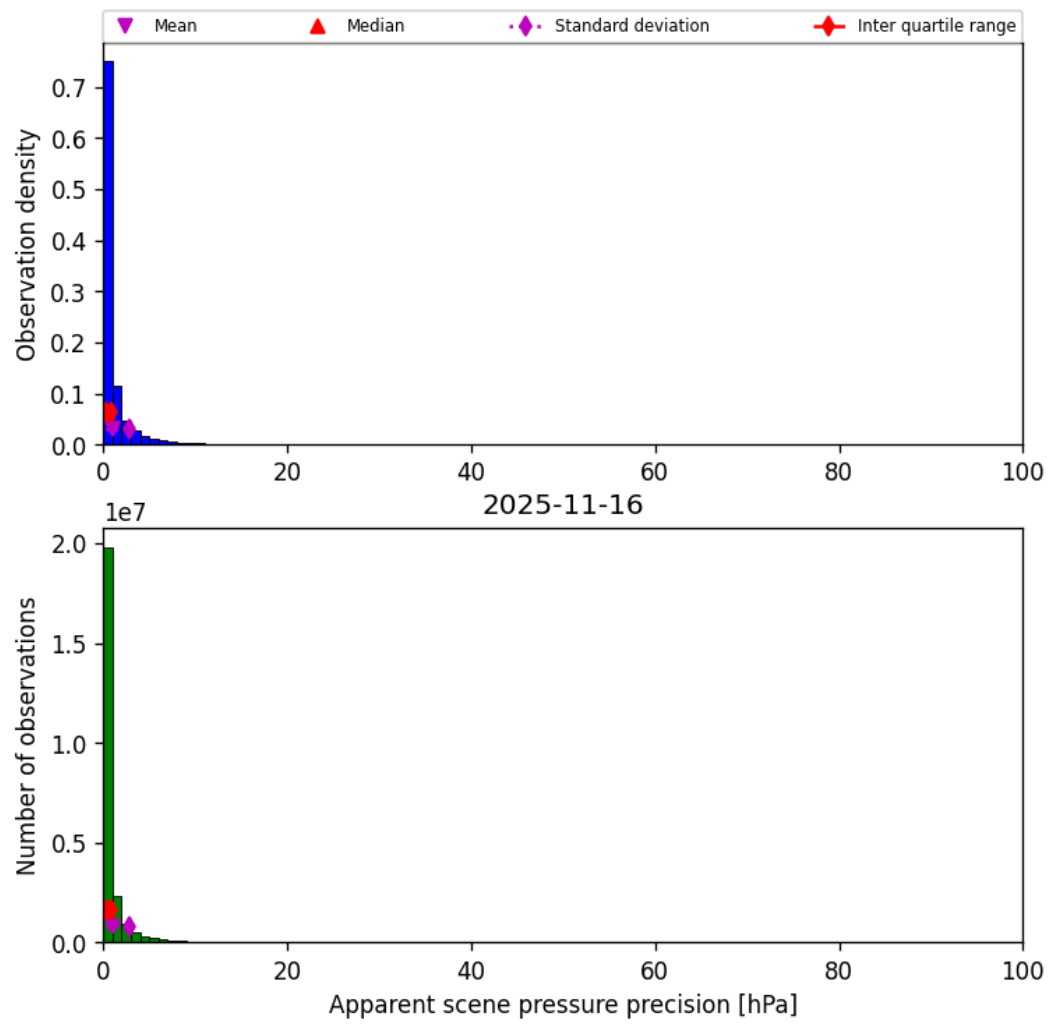
Figure 37: Histogram of "Apparent scene pressure precision" for 2025-11-15 to 2025-11-17
