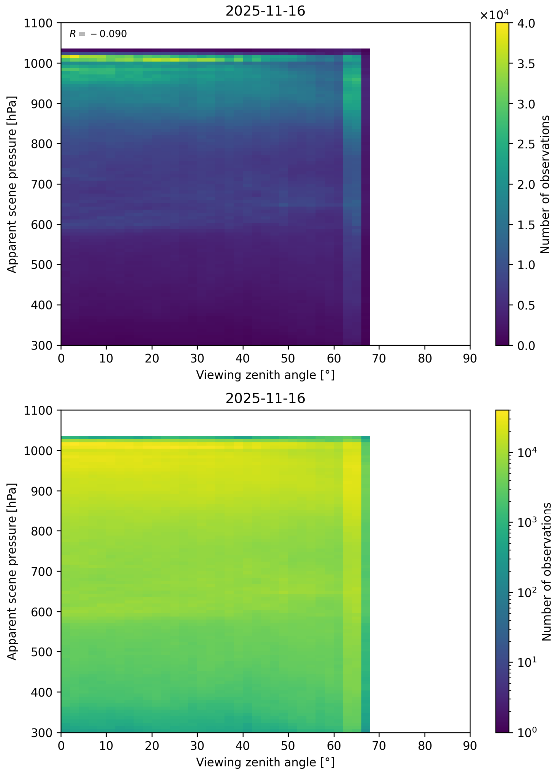
Figure 118: Scatter density plot of “Viewing zenith angle” against “Apparent scene pressure” for 2025-11-15 to 2025-11-17.
