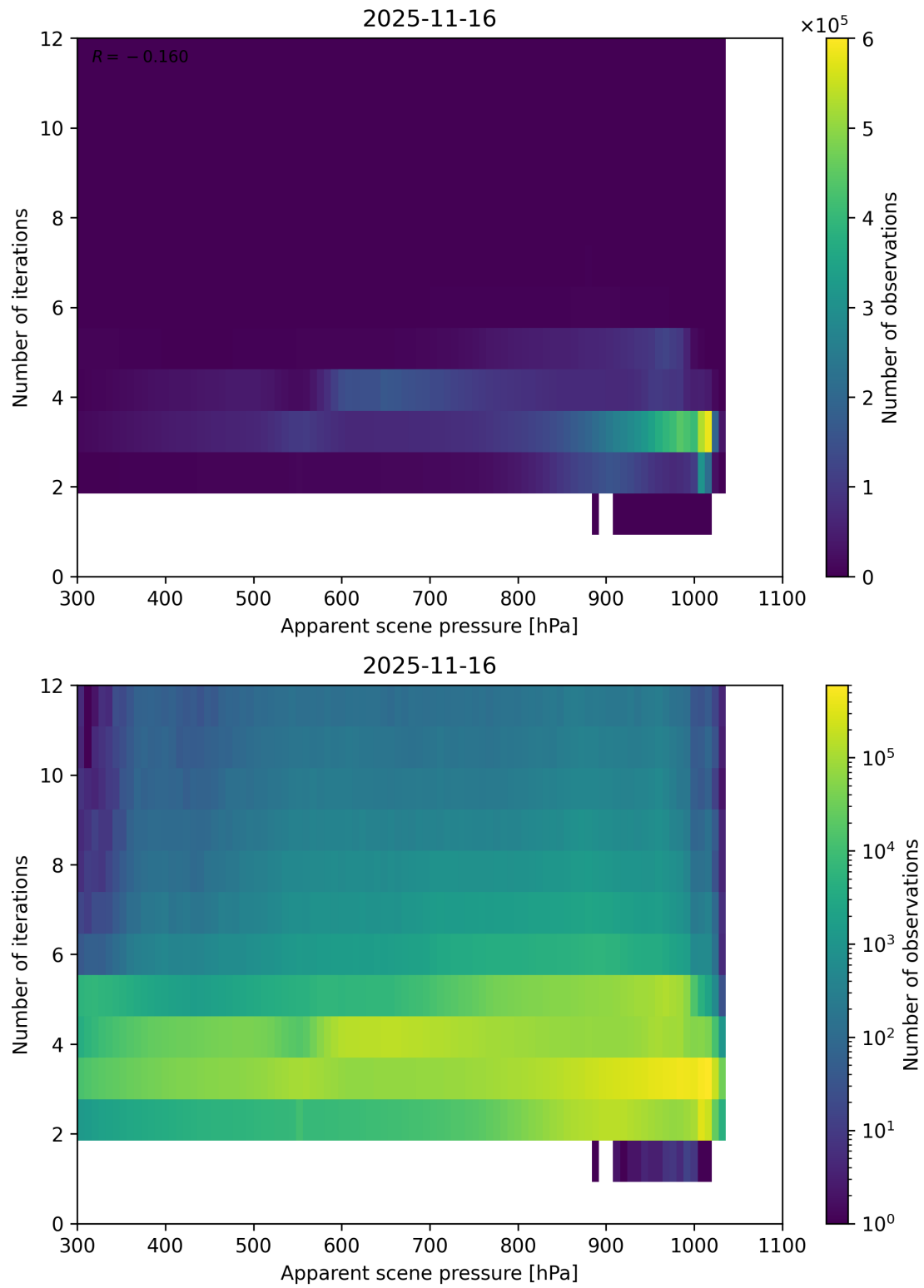
Figure 65: Scatter density plot of “Apparent scene pressure” against “Number of iterations” for 2025-11-15 to 2025-11-17.
