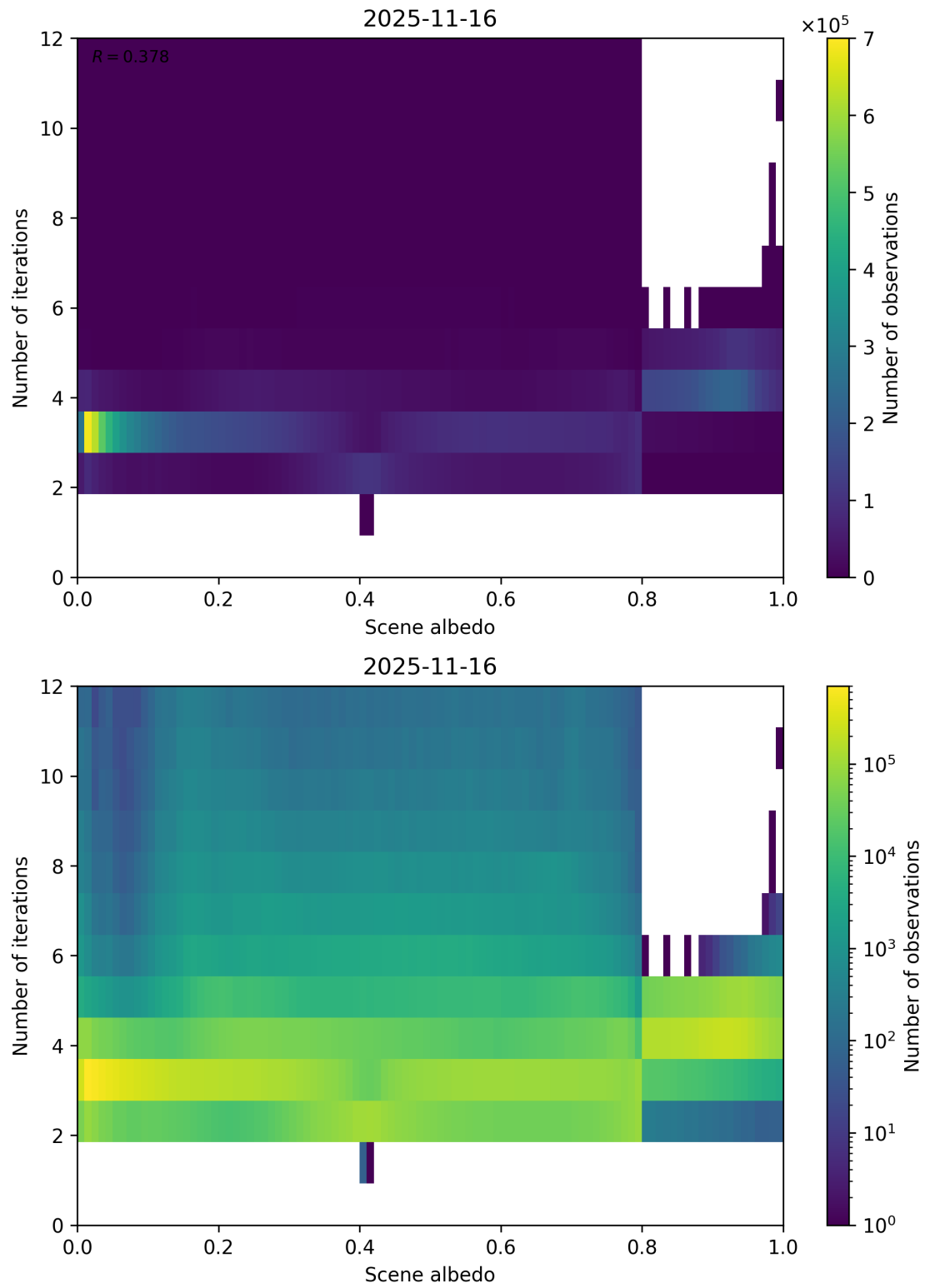
Figure 105: Scatter density plot of “Scene albedo” against “Number of iterations” for 2025-11-15 to 2025-11-17.
