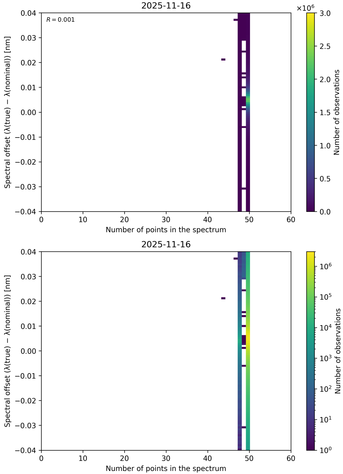
Figure 101: Scatter density plot of “Number of points in the spectrum” against “Spectral offset ( \lambda_{\text{true}} - \lambda_{\text{nominal}} )” for 2025-11-15 to 2025-11-17.
