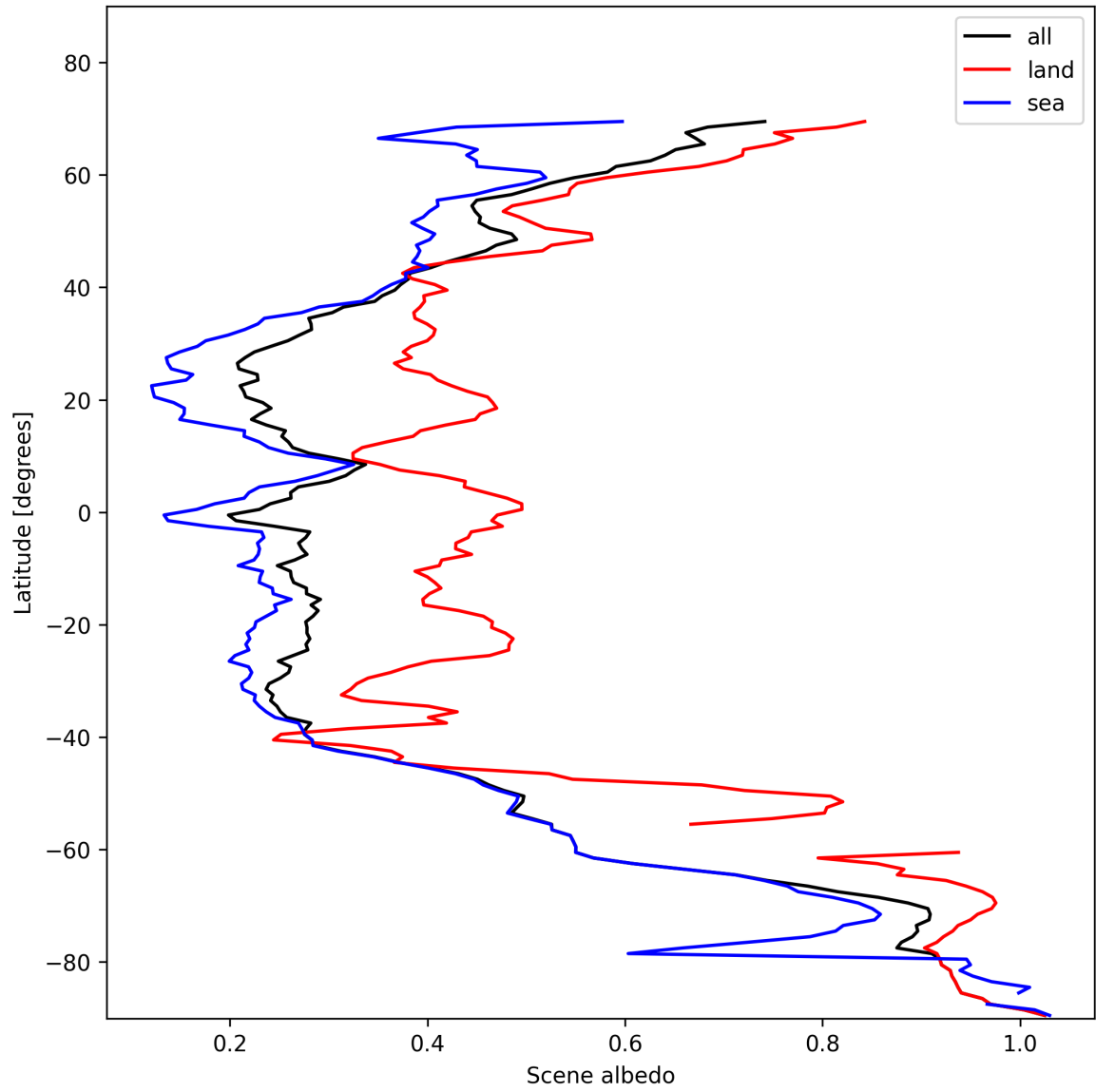
Figure 17: Zonal average of “Scene albedo” for 2025-11-15 to 2025-11-17.
