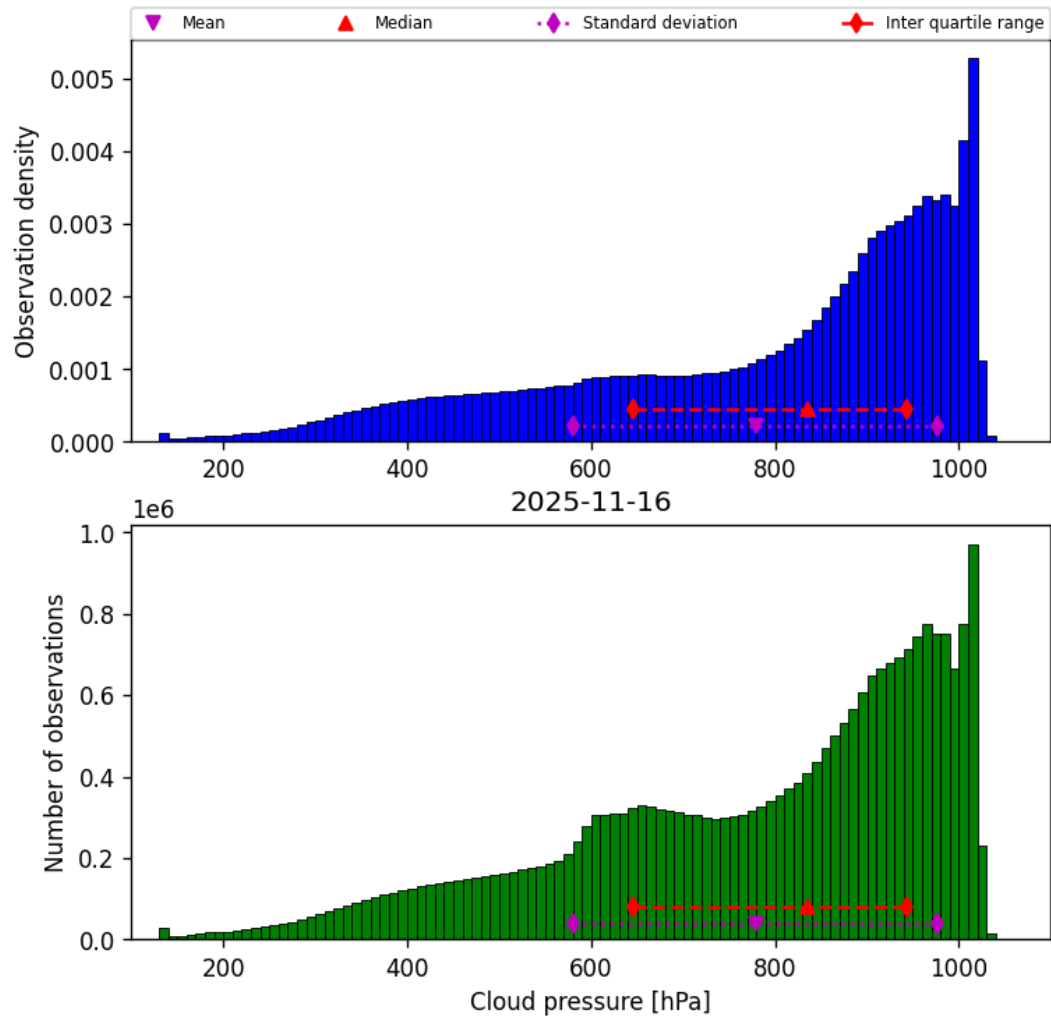
Figure 30: Histogram of “Cloud pressure” for 2025-11-15 to 2025-11-17
