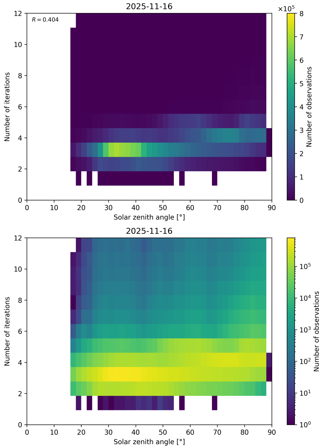
Figure 114: Scatter density plot of “Solar zenith angle” against “Number of iterations” for 2025-11-15 to 2025-11-17.
