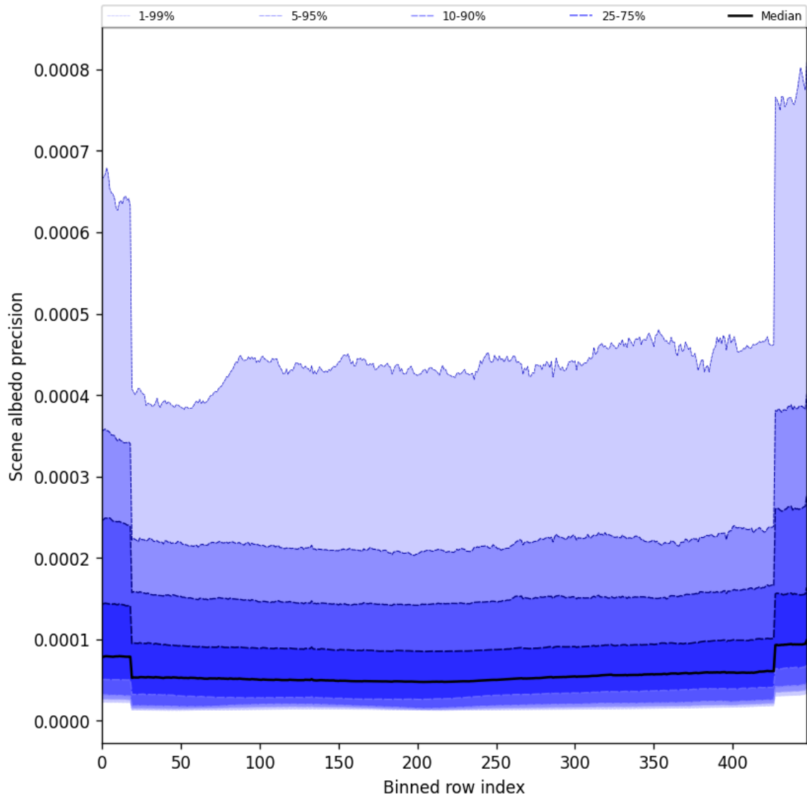
Figure 52: Along track statistics of “Scene albedo precision” for 2025-11-15 to 2025-11-17
