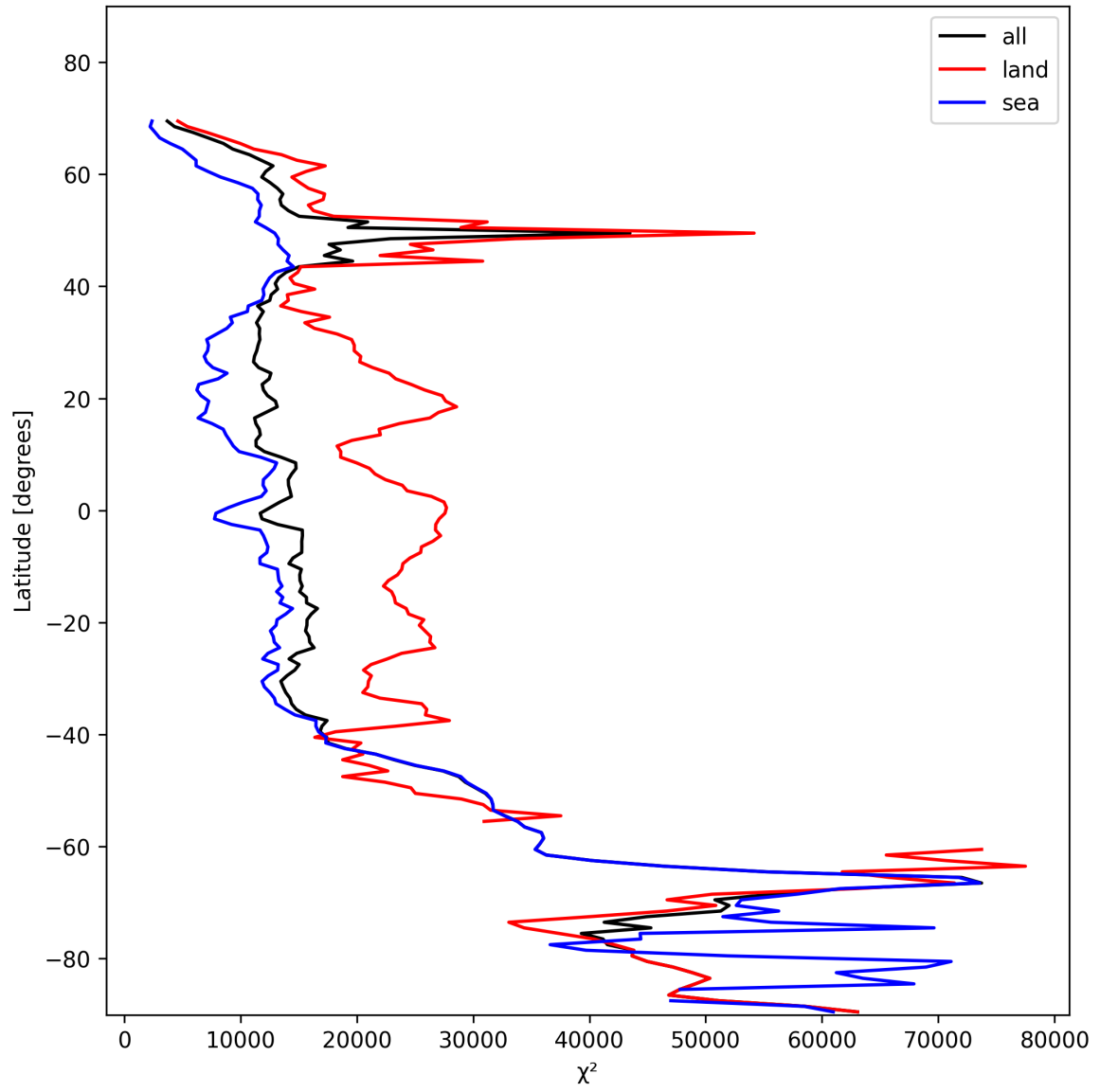
Figure 21: Zonal average of “ \chi^2 ” for 2025-11-15 to 2025-11-17.
