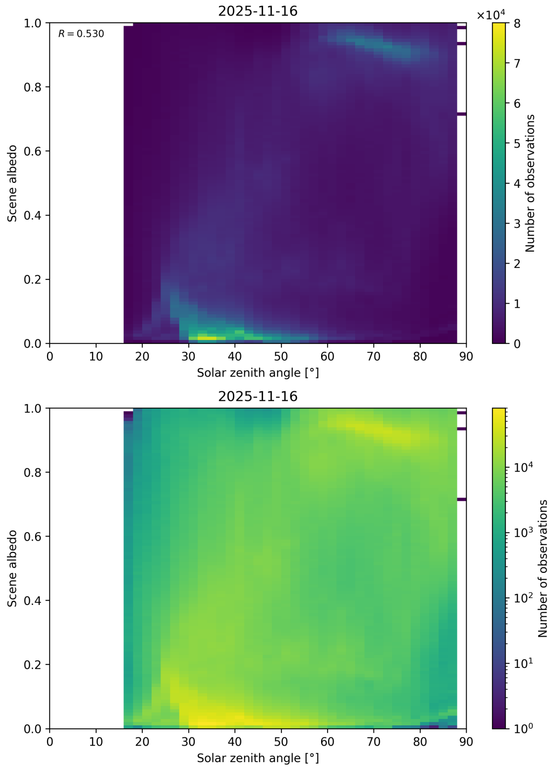
Figure 116: Scatter density plot of “Solar zenith angle” against “Scene albedo” for 2025-11-15 to 2025-11-17.
