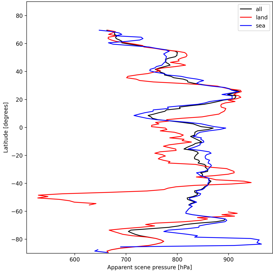
Figure 19: Zonal average of “Apparent scene pressure” for 2025-11-15 to 2025-11-17.
