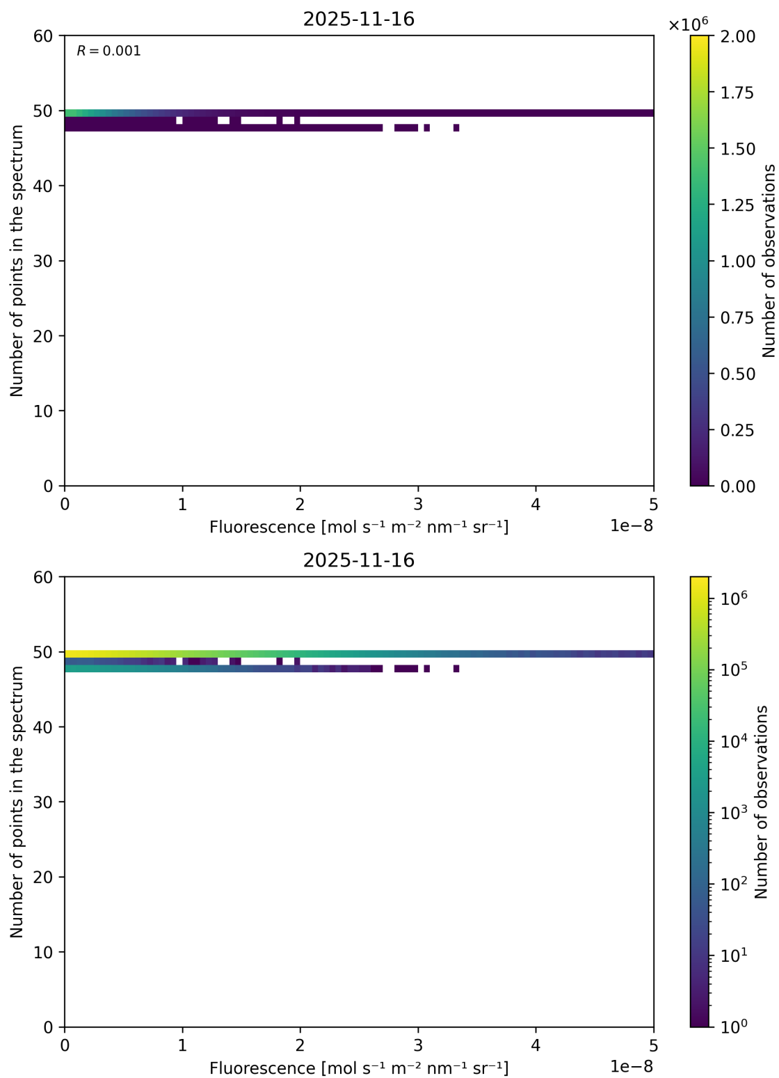
Figure 86: Scatter density plot of “Fluorescence” against “Number of points in the spectrum” for 2025-11-15 to 2025-11-17.
