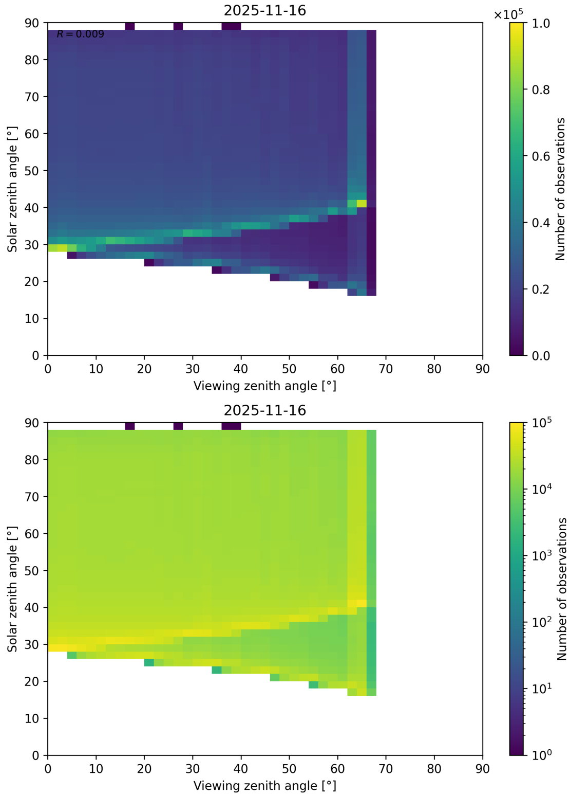
Figure 127: Scatter density plot of “Viewing zenith angle” against “Solar zenith angle” for 2025-11-15 to 2025-11-17.
