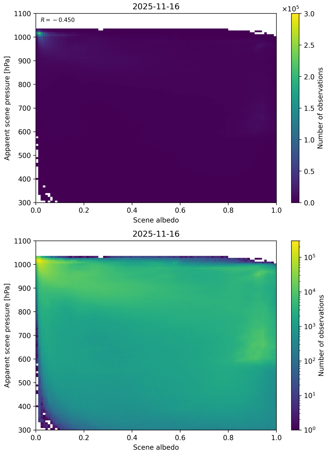
Figure 102: Scatter density plot of “Scene albedo” against “Apparent scene pressure” for 2025-11-15 to 2025-11-17.
