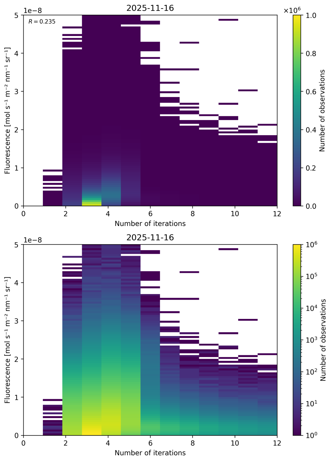
Figure 98: Scatter density plot of “Number of iterations” against “Fluorescence” for 2025-11-15 to 2025-11-17.
