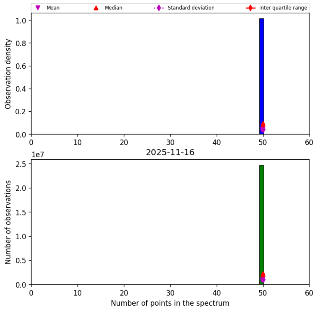
Figure 44: Histogram of “Number of points in the spectrum” for 2025-11-15 to 2025-11-17
