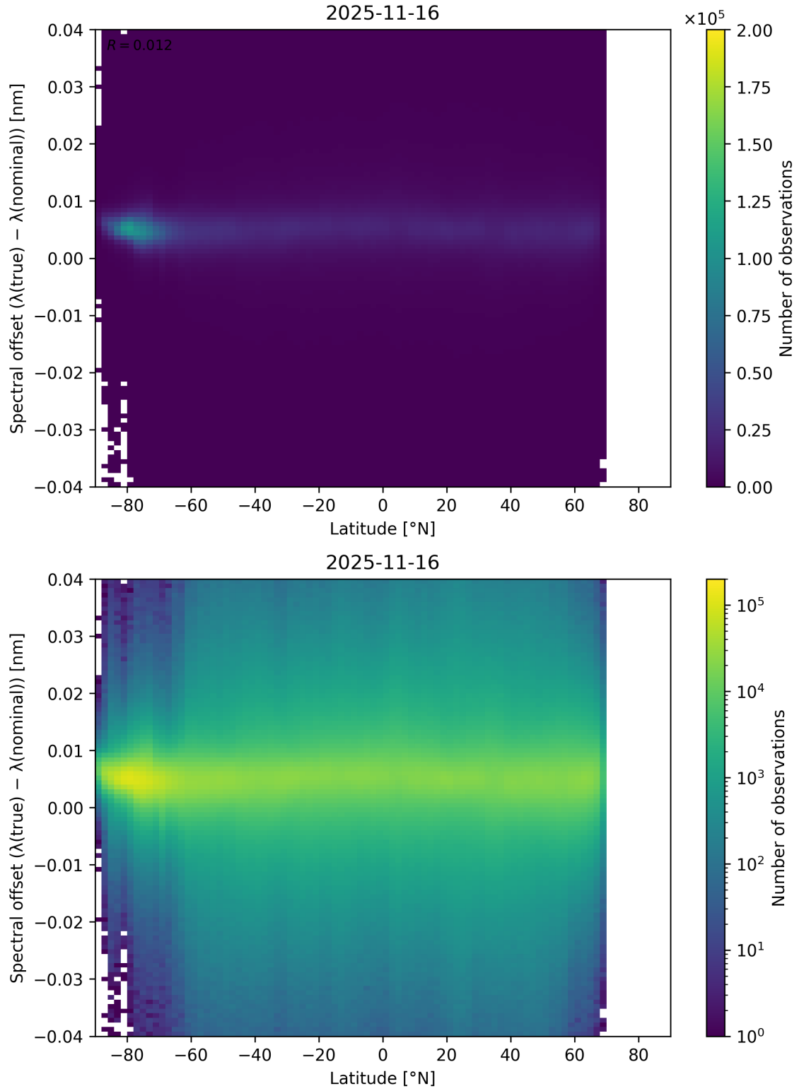
Figure 96: Scatter density plot of “Latitude” against “Spectral offset ( \lambda_{\text{true}} - \lambda_{\text{nominal}} )” for 2025-11-15 to 2025-11-17.
