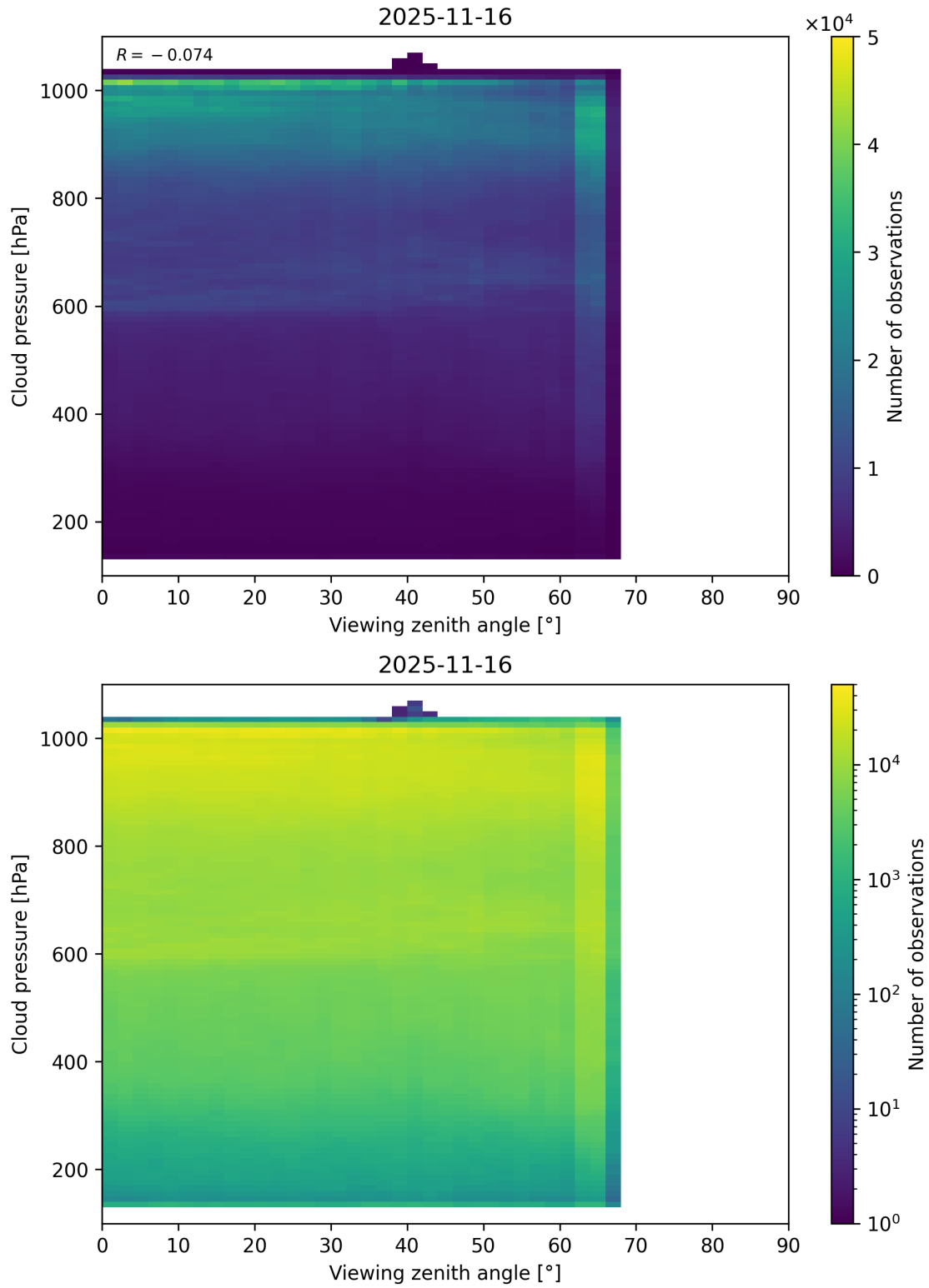
Figure 121: Scatter density plot of “Viewing zenith angle” against “Cloud pressure” for 2025-11-15 to 2025-11-17.
