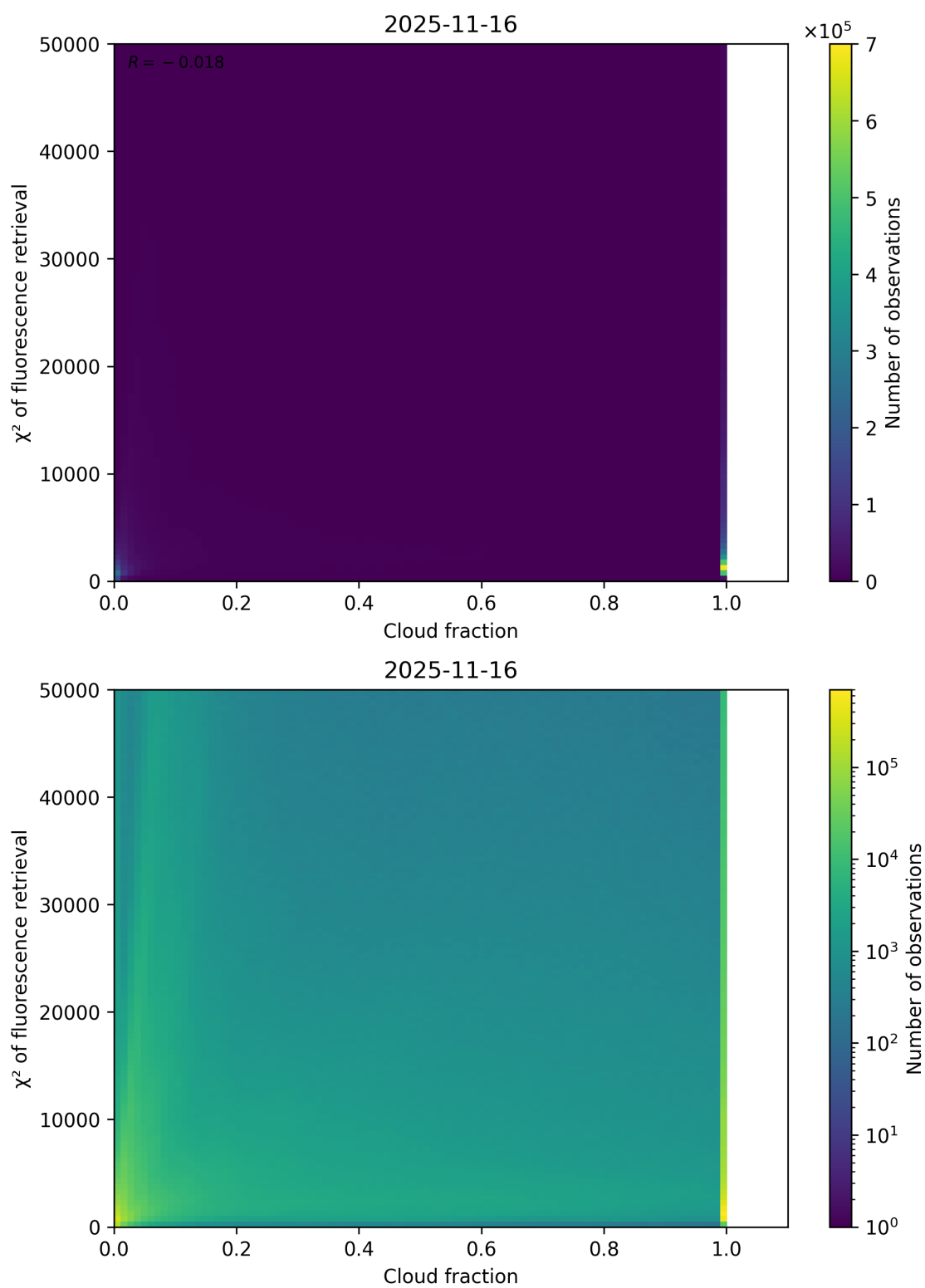
Figure 71: Scatter density plot of “Cloud fraction” against “ \chi^2 of fluorescence retrieval” for 2025-11-15 to 2025-11-17.
