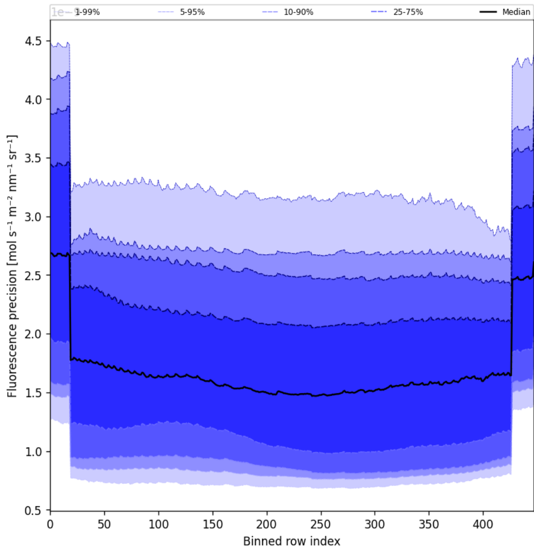
Figure 58: Along track statistics of “Fluorescence precision” for 2025-11-15 to 2025-11-17
