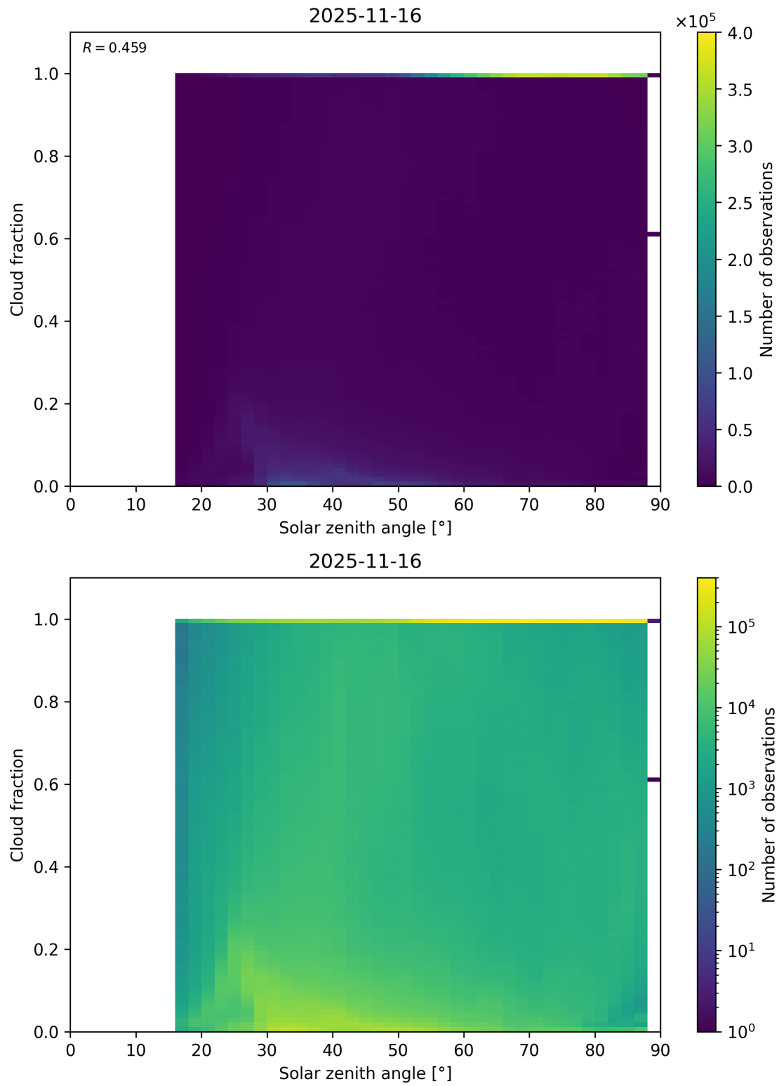
Figure 110: Scatter density plot of “Solar zenith angle” against “Cloud fraction” for 2025-11-15 to 2025-11-17.
