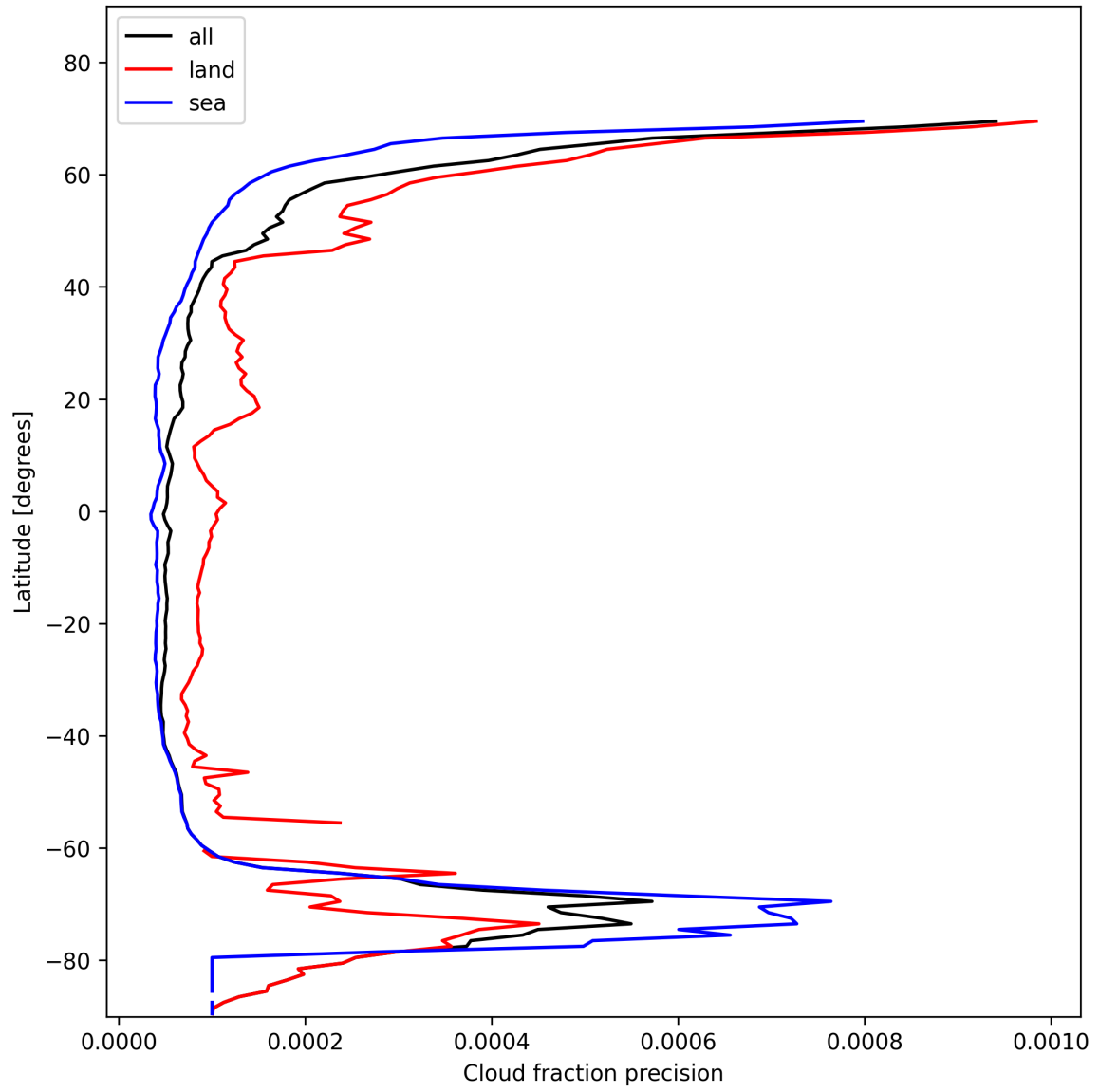
Figure 16: Zonal average of “Cloud fraction precision” for 2025-11-15 to 2025-11-17.
