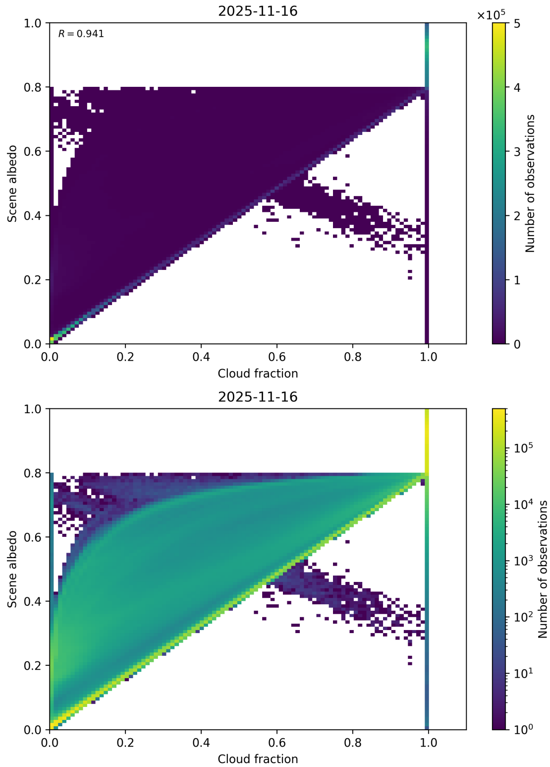
Figure 75: Scatter density plot of “Cloud fraction” against “Scene albedo” for 2025-11-15 to 2025-11-17.
