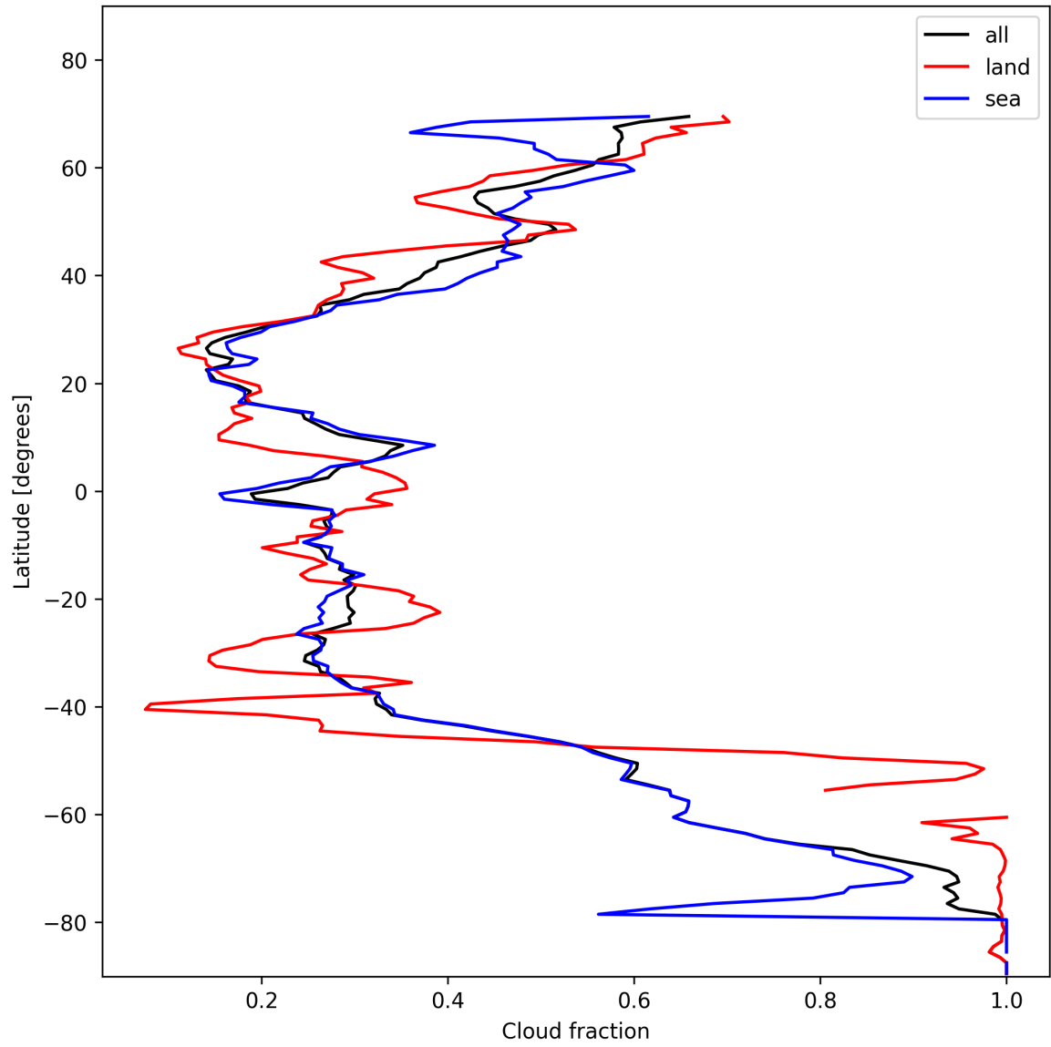
Figure 15: Zonal average of “Cloud fraction” for 2025-11-15 to 2025-11-17.
