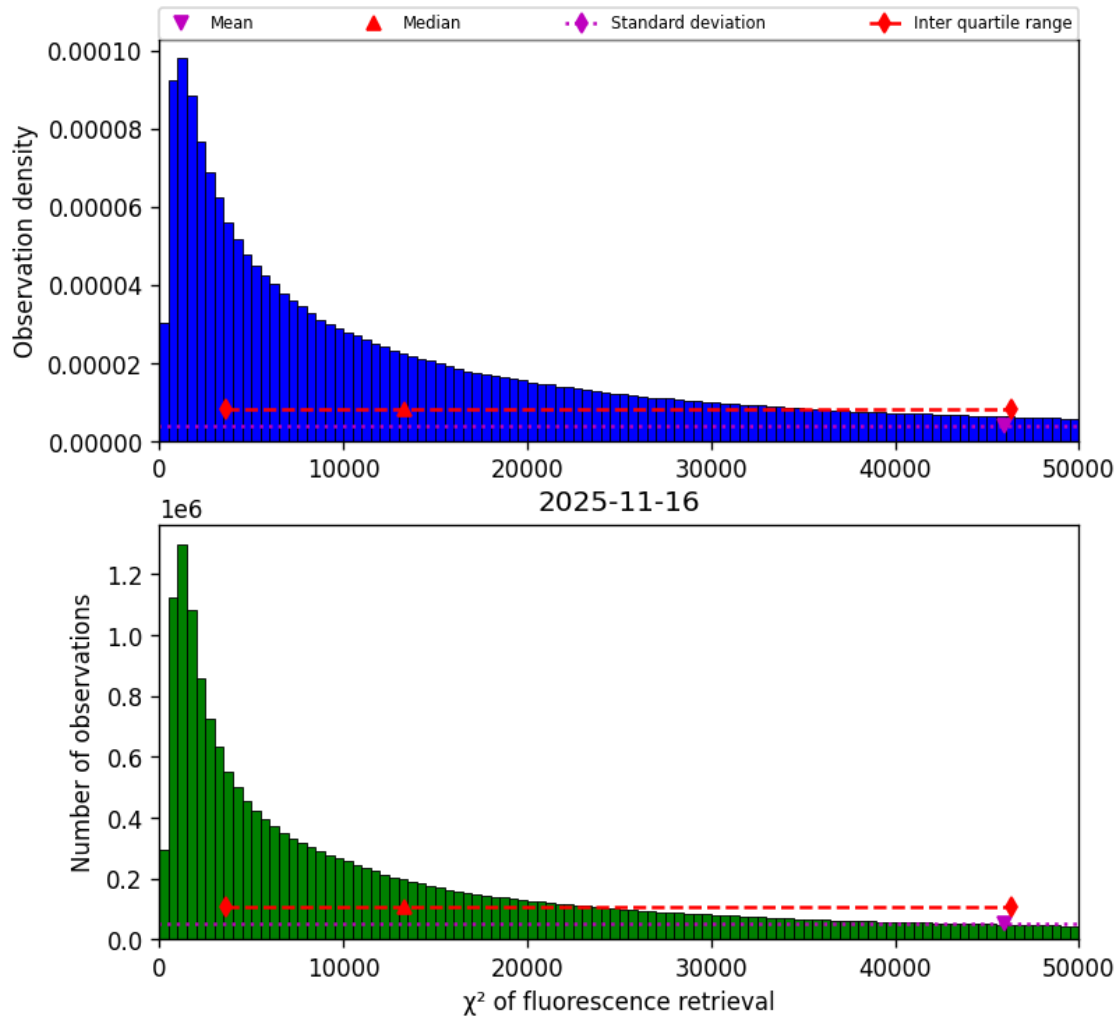
Figure 42: Histogram of “ \chi^2 of fluorescence retrieval” for 2025-11-15 to 2025-11-17
