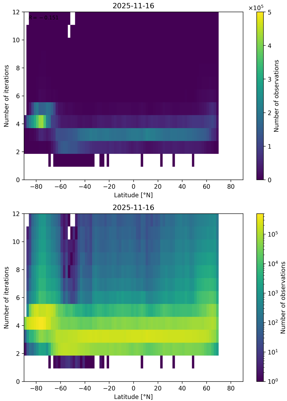
Figure 93: Scatter density plot of “Latitude” against “Number of iterations” for 2025-11-15 to 2025-11-17.
