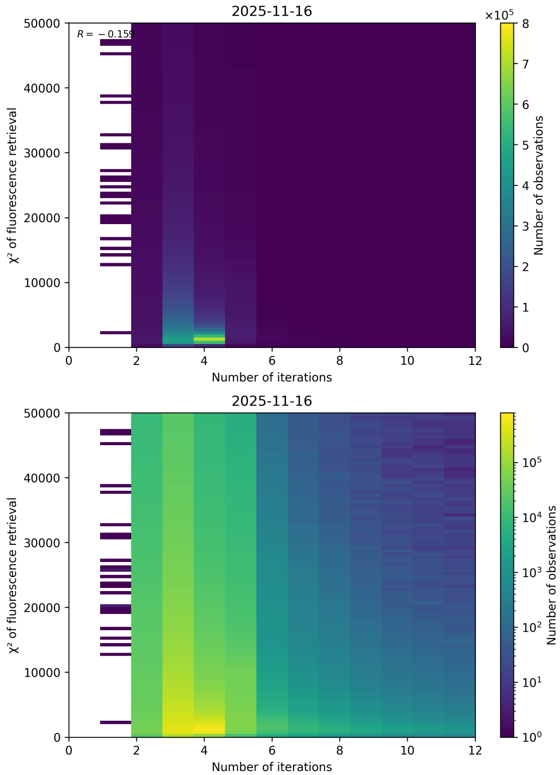
Figure 97: Scatter density plot of “Number of iterations” against “ \chi^2 of fluorescence retrieval” for 2025-11-15 to 2025-11-17.
