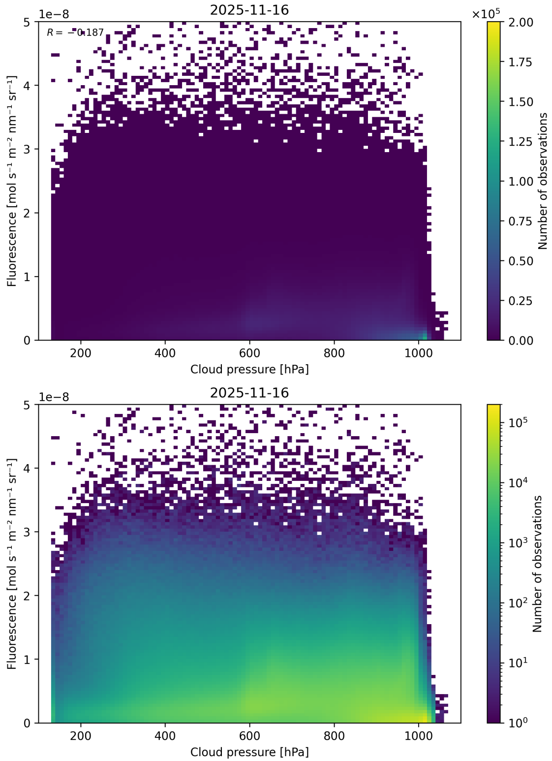
Figure 80: Scatter density plot of “Cloud pressure” against “Fluorescence” for 2025-11-15 to 2025-11-17.
