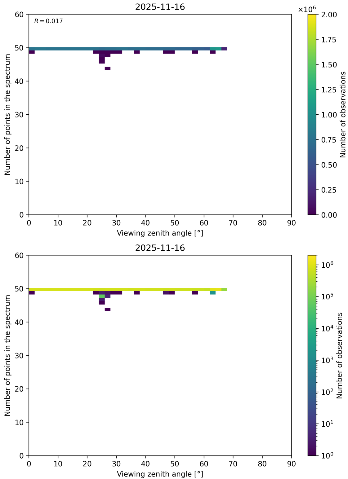
Figure 125: Scatter density plot of “Viewing zenith angle” against “Number of points in the spectrum” for 2025-11-15 to 2025-11-17.
