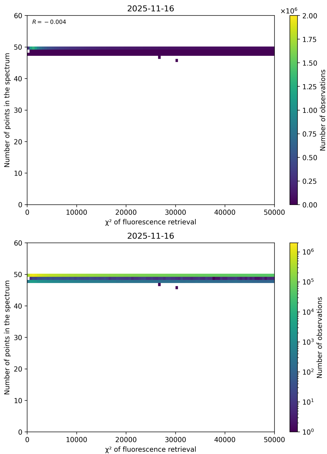
Figure 68: Scatter density plot of " \chi^2 of fluorescence retrieval" against "Number of points in the spectrum" for 2025-11-15 to 2025-11-17.
