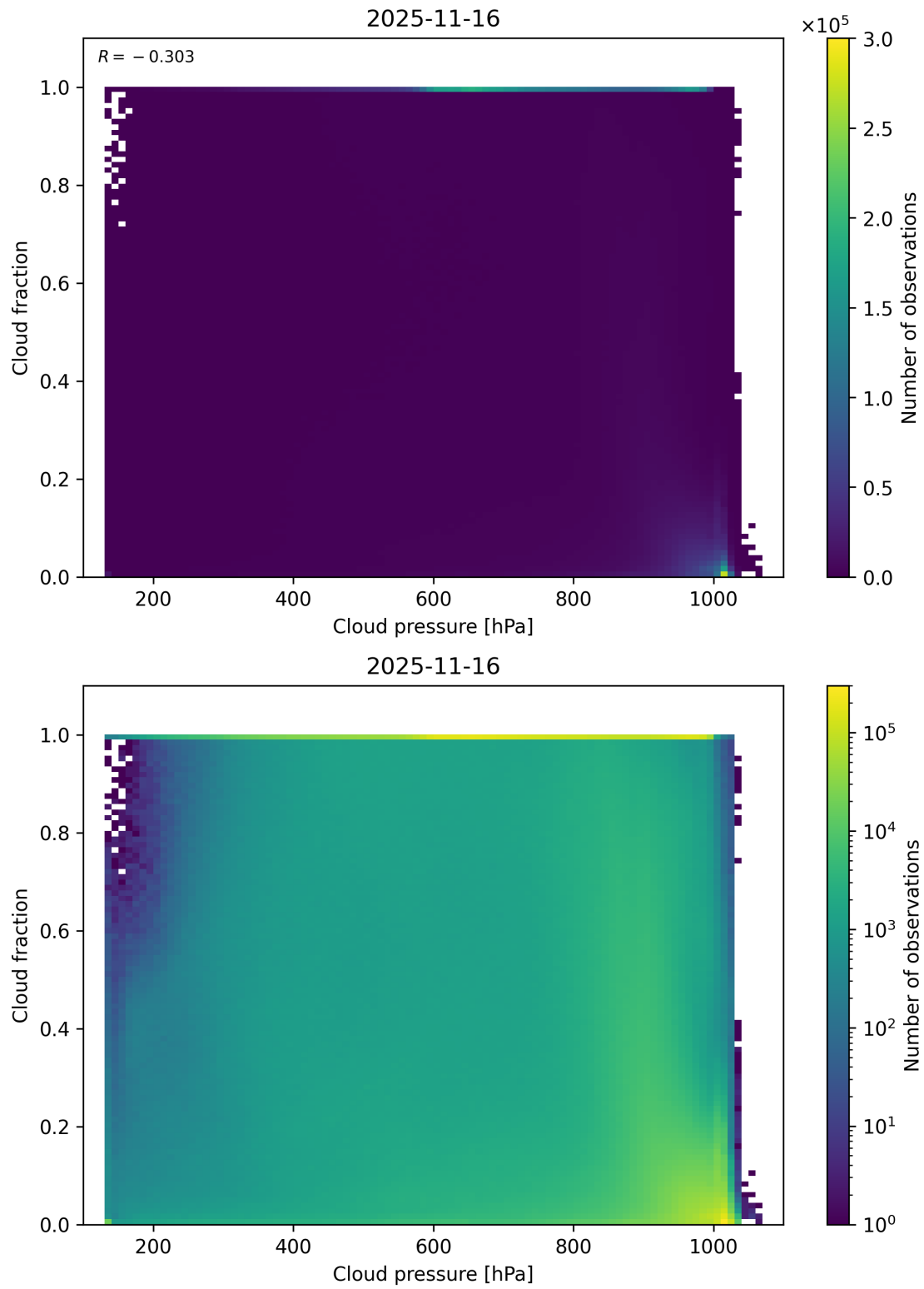
Figure 79: Scatter density plot of “Cloud pressure” against “Cloud fraction” for 2025-11-15 to 2025-11-17.
