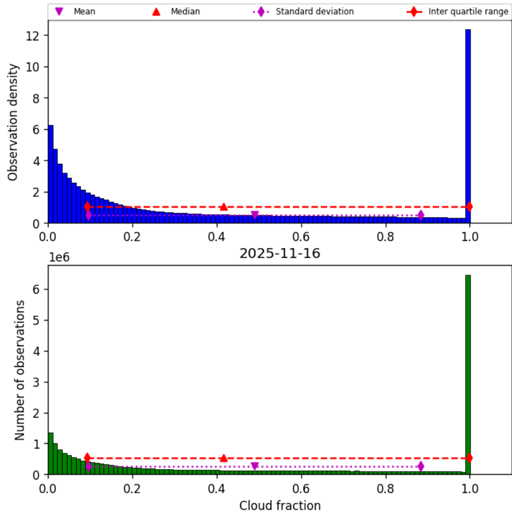
Figure 32: Histogram of “Cloud fraction” for 2025-11-15 to 2025-11-17
