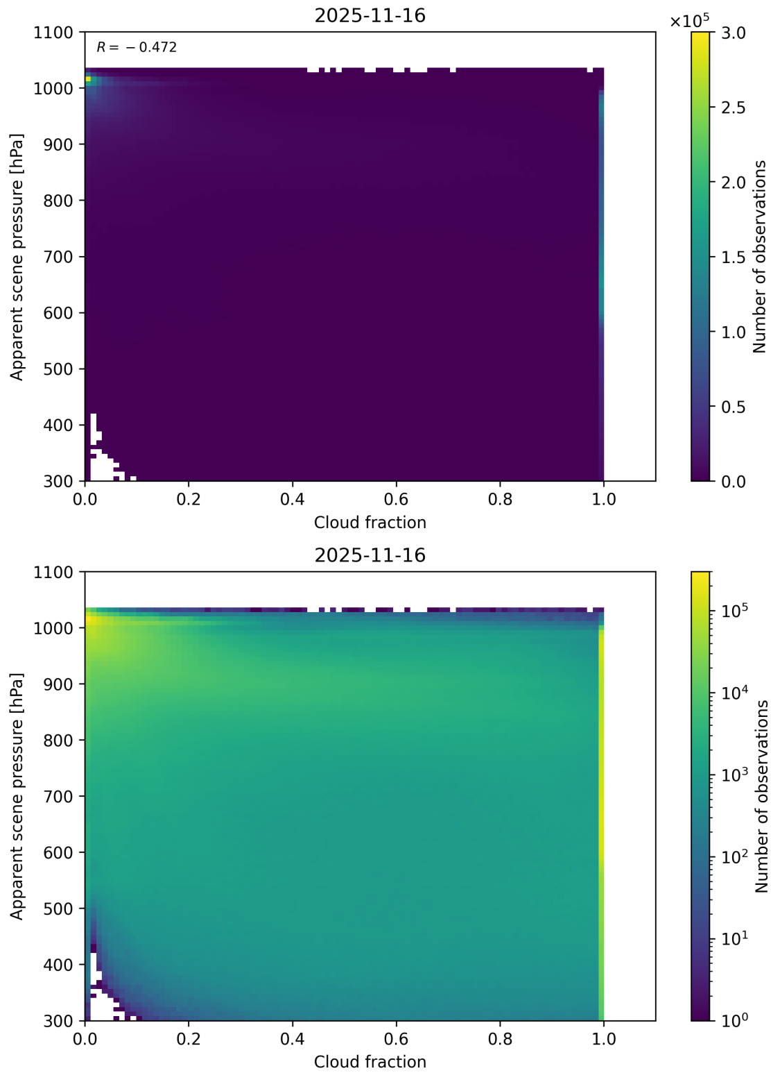
Figure 70: Scatter density plot of “Cloud fraction” against “Apparent scene pressure” for 2025-11-15 to 2025-11-17.
