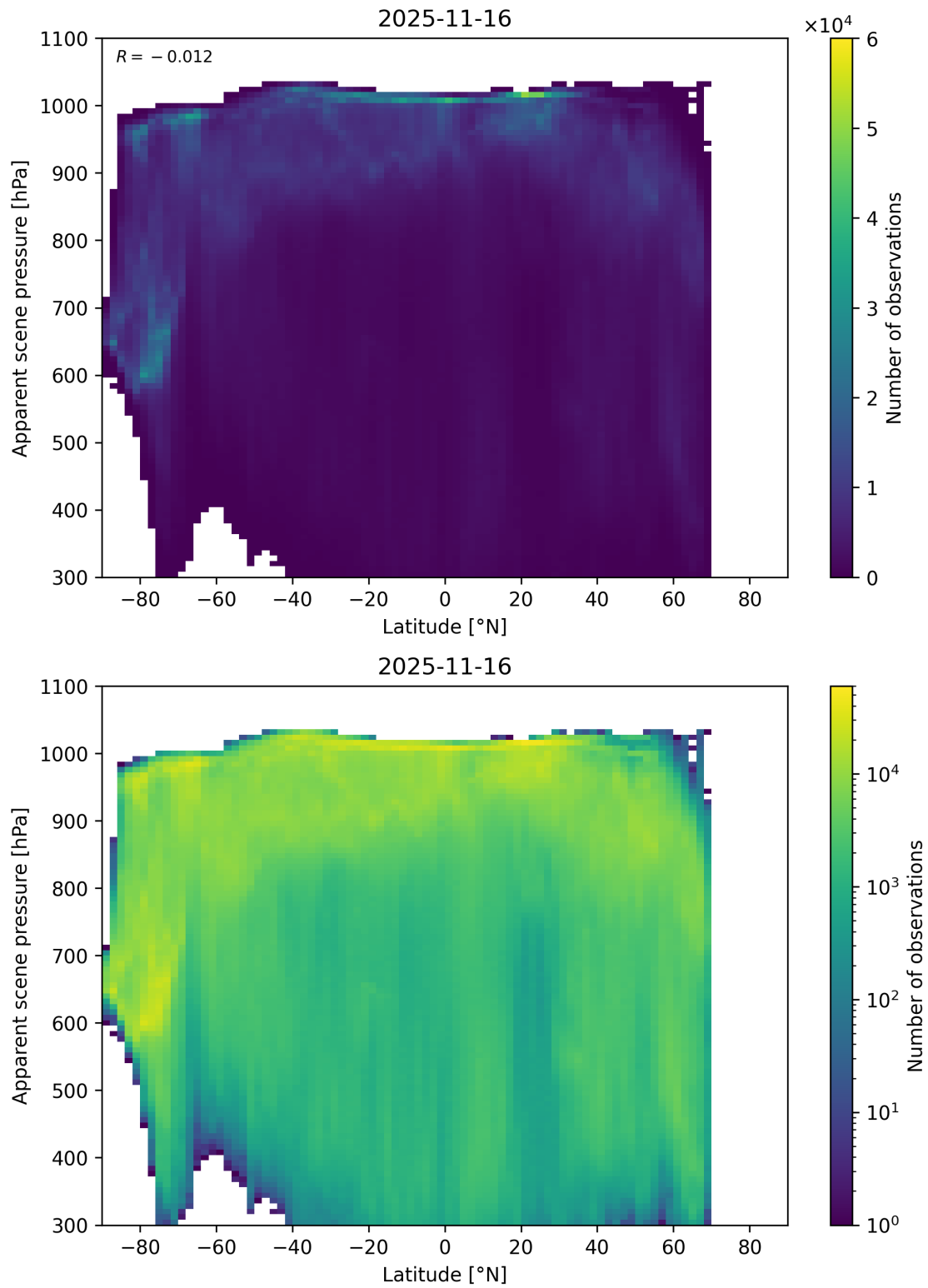
Figure 88: Scatter density plot of “Latitude” against “Apparent scene pressure” for 2025-11-15 to 2025-11-17.
