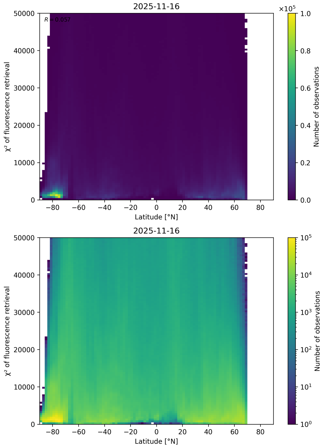
Figure 89: Scatter density plot of “Latitude” against “ \chi^2 of fluorescence retrieval” for 2025-11-15 to 2025-11-17.
