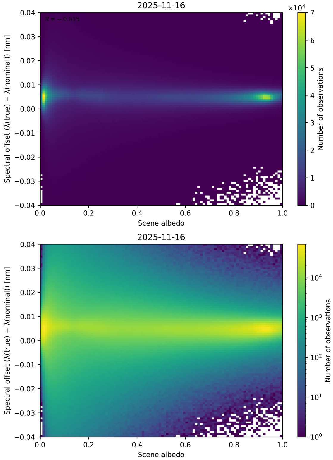
Figure 107: Scatter density plot of “Scene albedo” against “Spectral offset ( \lambda_{\text{true}} - \lambda_{\text{nominal}} )” for 2025-11-15 to 2025-11-17.
