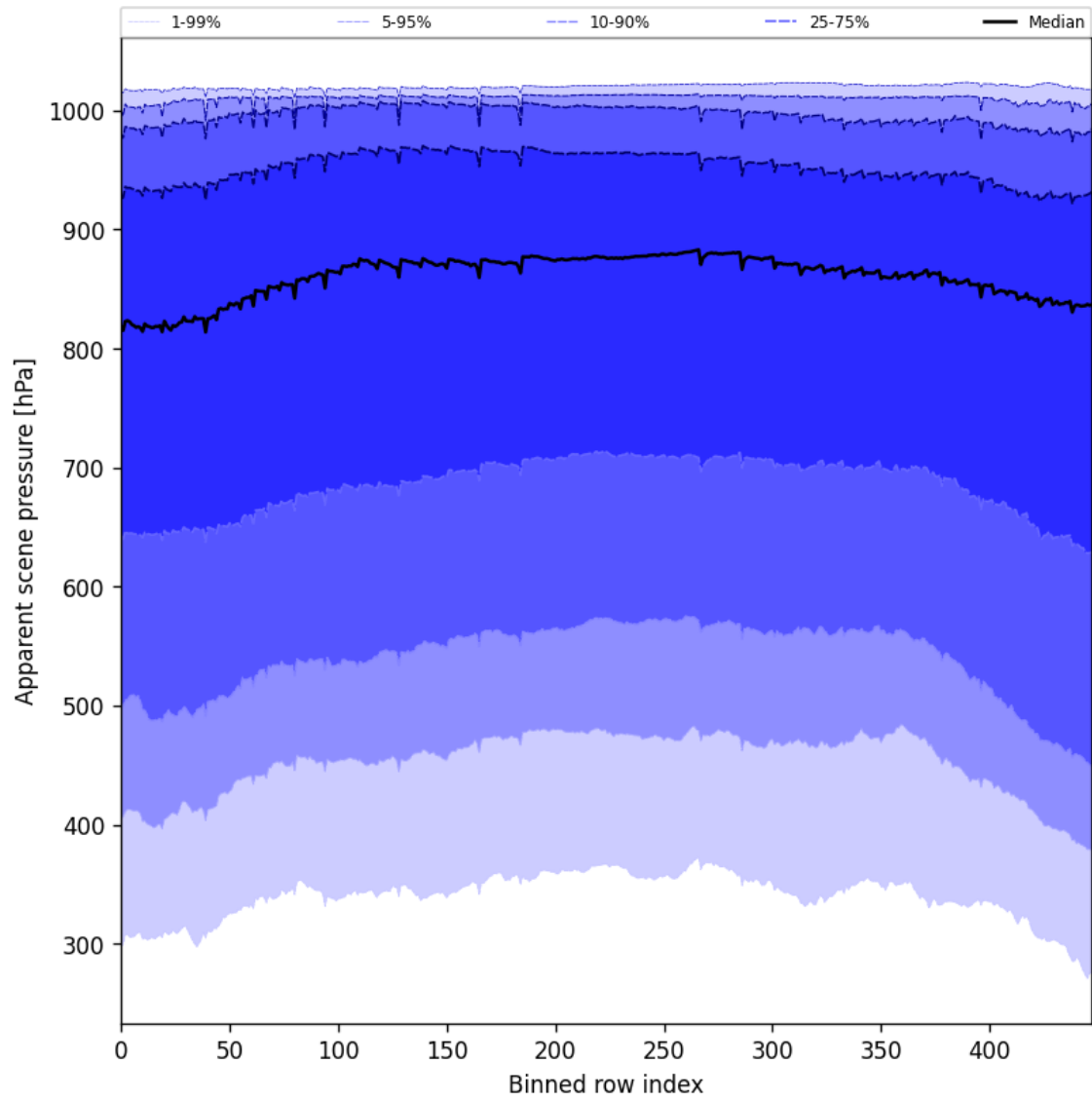
Figure 53: Along track statistics of “Apparent scene pressure” for 2025-11-15 to 2025-11-17
