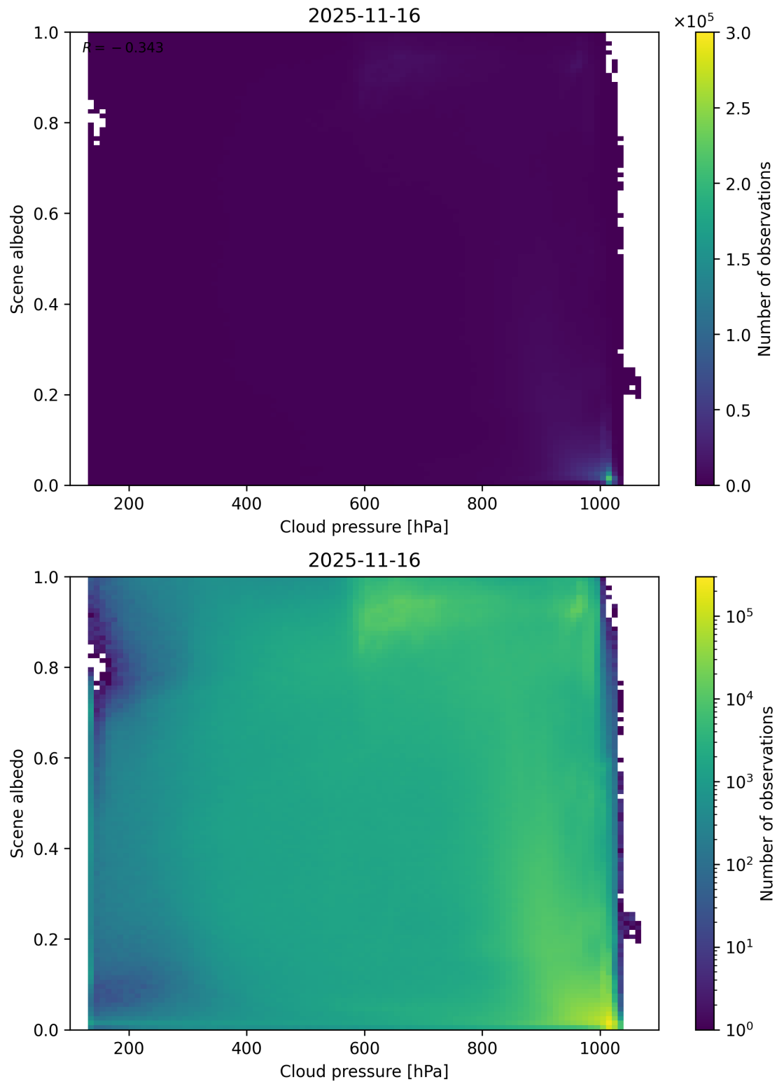
Figure 83: Scatter density plot of “Cloud pressure” against “Scene albedo” for 2025-11-15 to 2025-11-17.
