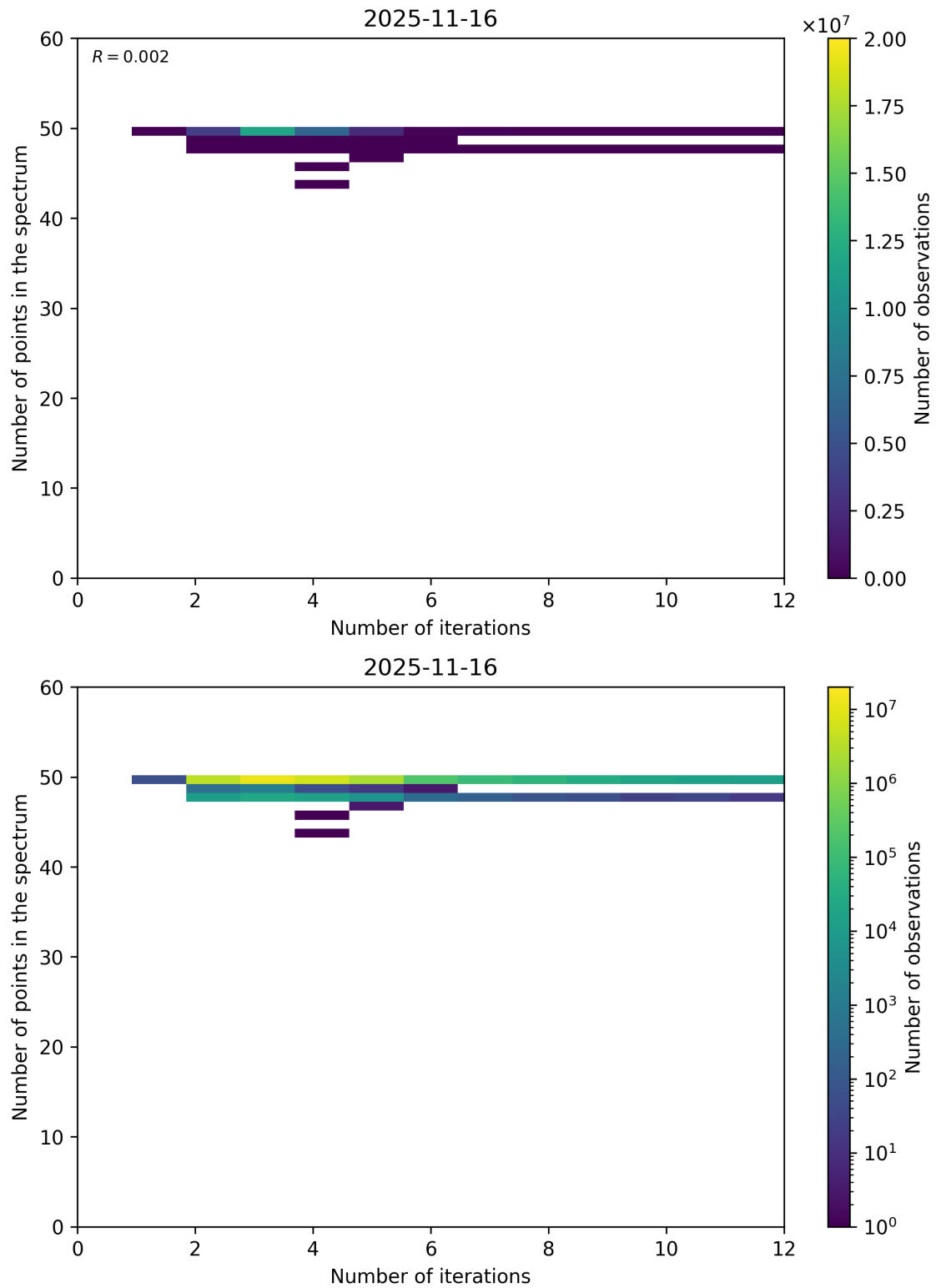
Figure 99: Scatter density plot of “Number of iterations” against “Number of points in the spectrum” for 2025-11-15 to 2025-11-17.
