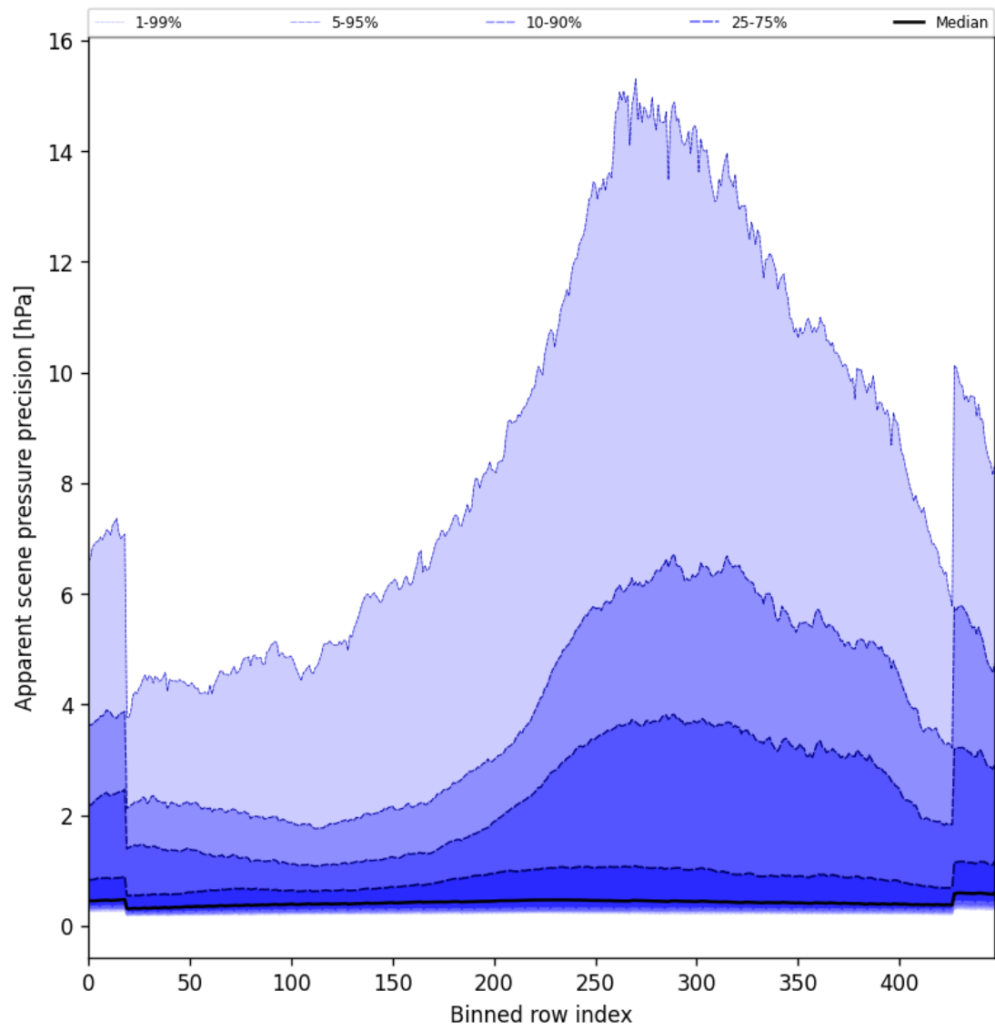
Figure 54: Along track statistics of “Apparent scene pressure precision” for 2025-11-15 to 2025-11-17
