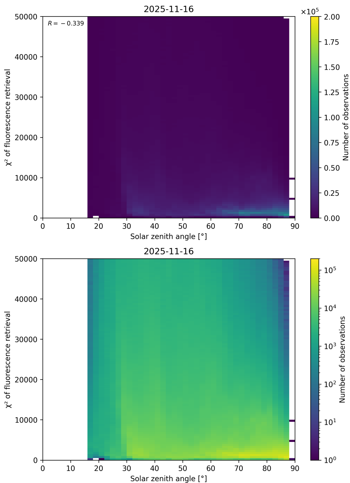
Figure 109: Scatter density plot of “Solar zenith angle” against “ \chi^2 of fluorescence retrieval” for 2025-11-15 to 2025-11-17.
