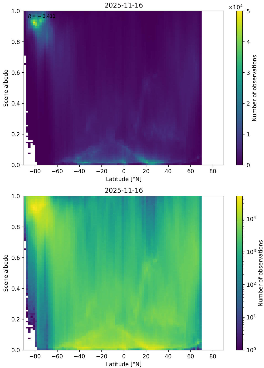
Figure 95: Scatter density plot of “Latitude” against “Scene albedo” for 2025-11-15 to 2025-11-17.
