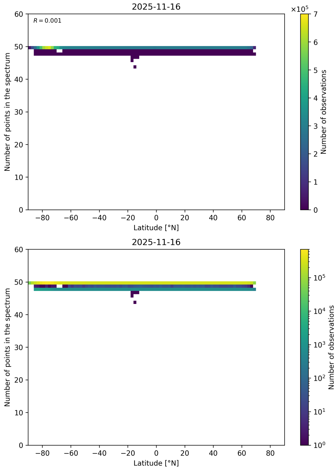
Figure 94: Scatter density plot of “Latitude” against “Number of points in the spectrum” for 2025-11-15 to 2025-11-17.
