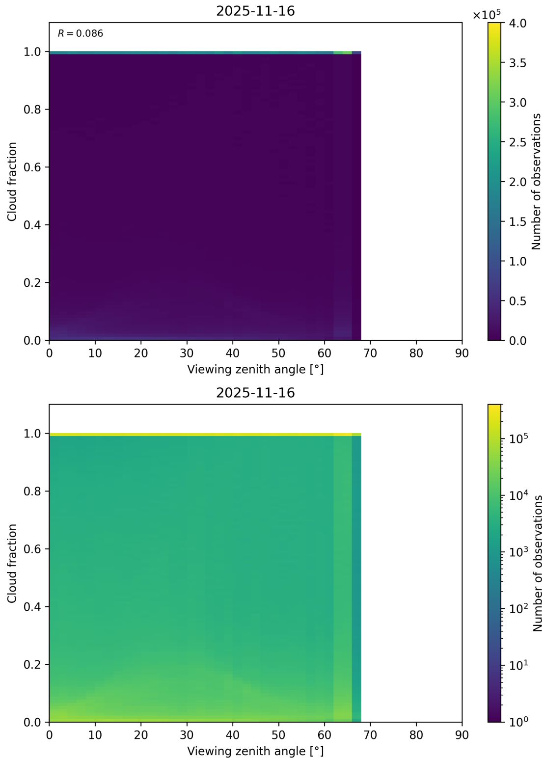
Figure 120: Scatter density plot of “Viewing zenith angle” against “Cloud fraction” for 2025-11-15 to 2025-11-17.
