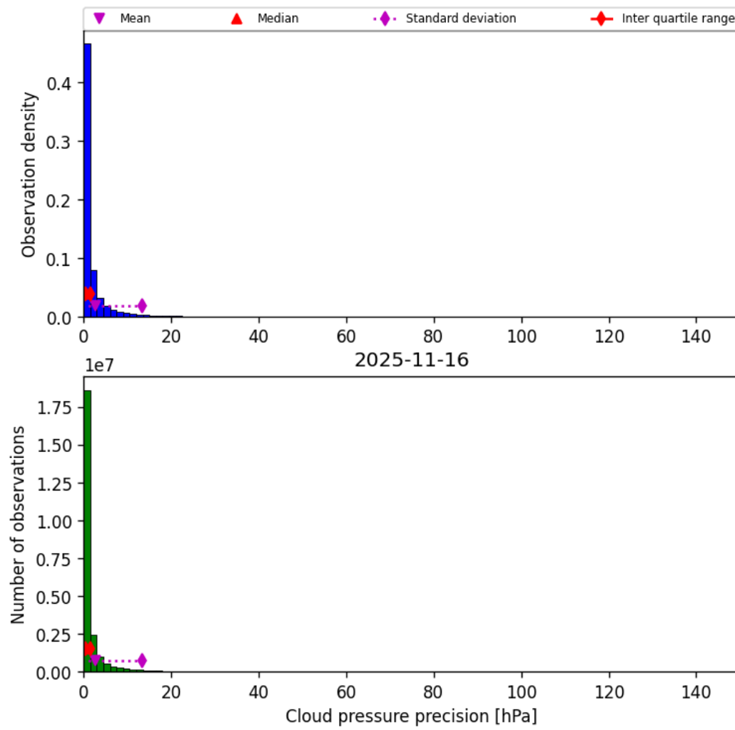
Figure 31: Histogram of “Cloud pressure precision” for 2025-11-15 to 2025-11-17
