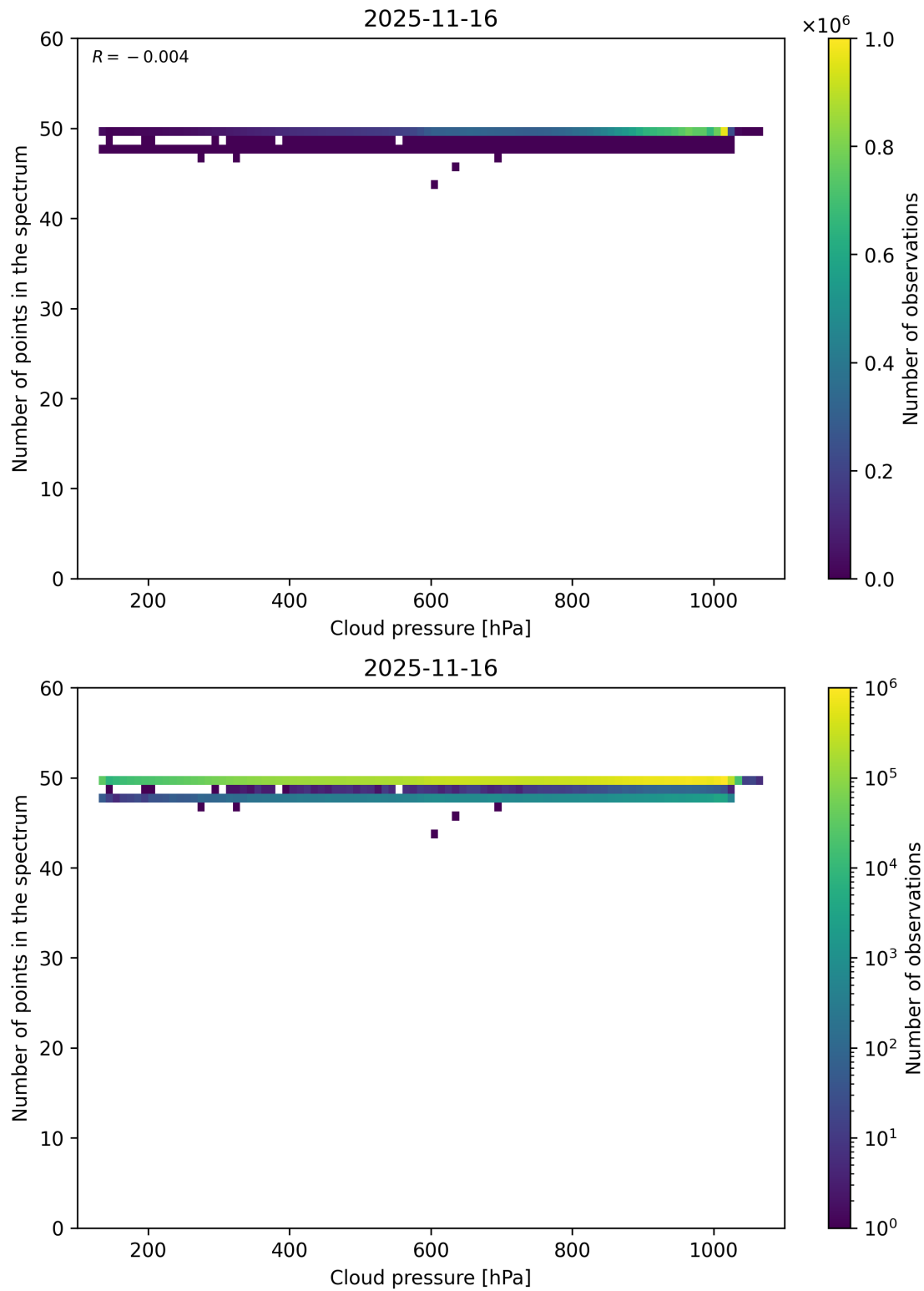
Figure 82: Scatter density plot of “Cloud pressure” against “Number of points in the spectrum” for 2025-11-15 to 2025-11-17.
