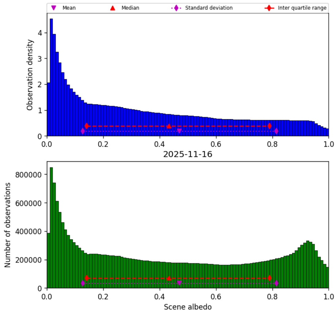
Figure 34: Histogram of “Scene albedo” for 2025-11-15 to 2025-11-17
