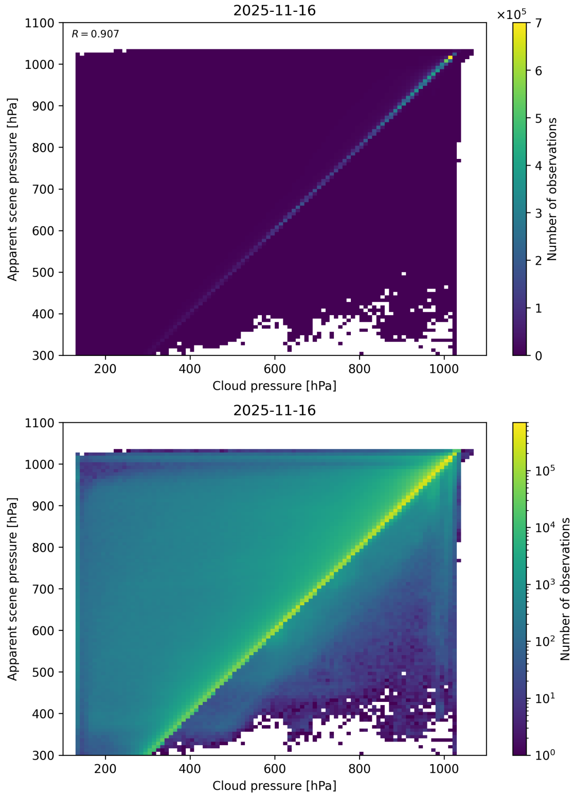
Figure 77: Scatter density plot of “Cloud pressure” against “Apparent scene pressure” for 2025-11-15 to 2025-11-17.
