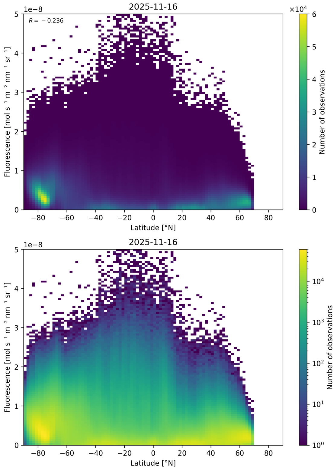
Figure 92: Scatter density plot of “Latitude” against “Fluorescence” for 2025-11-15 to 2025-11-17.
