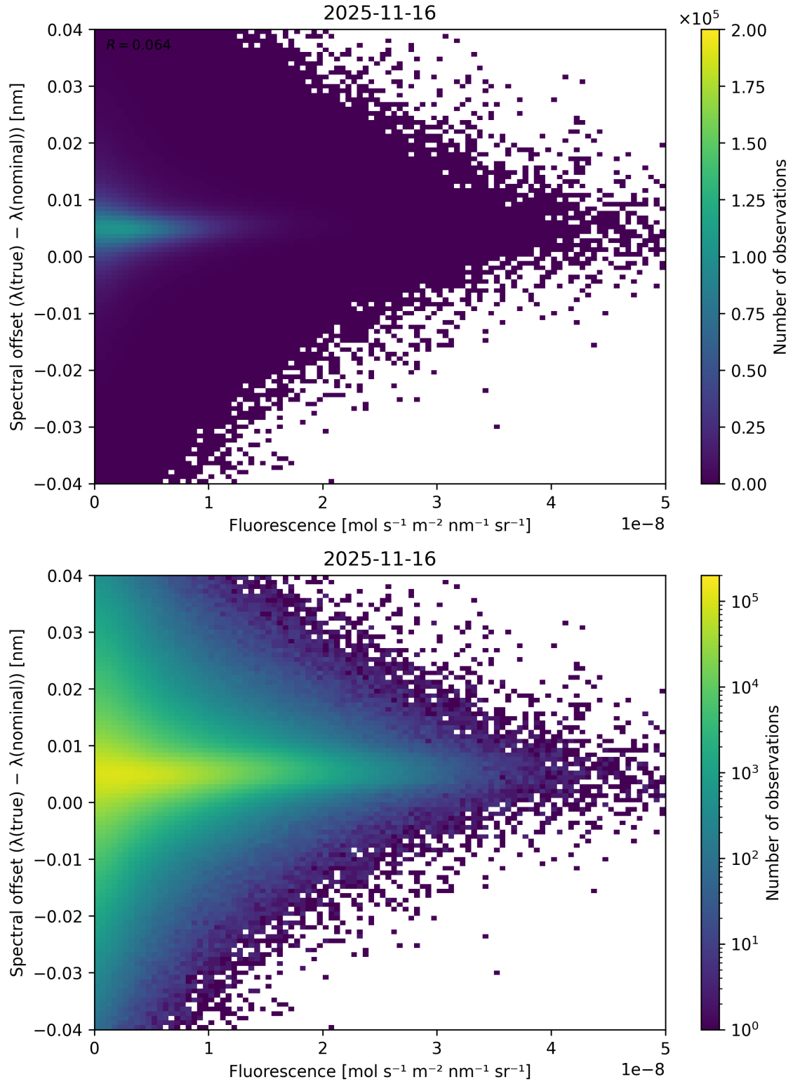
Figure 87: Scatter density plot of “Fluorescence” against “Spectral offset ( \lambda_{\text{true}} - \lambda_{\text{nominal}} )” for 2025-11-15 to 2025-11-17.
