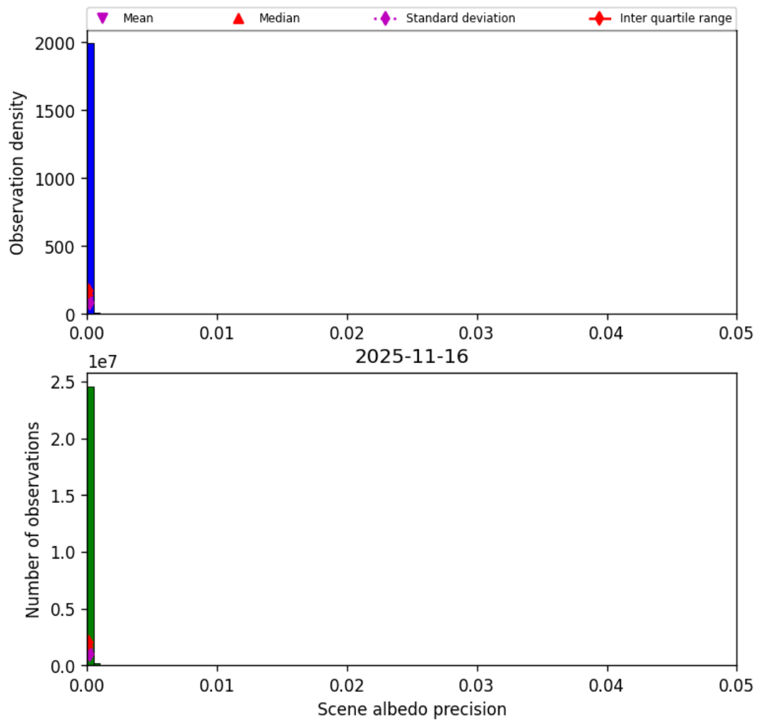
Figure 35: Histogram of “Scene albedo precision” for 2025-11-15 to 2025-11-17
