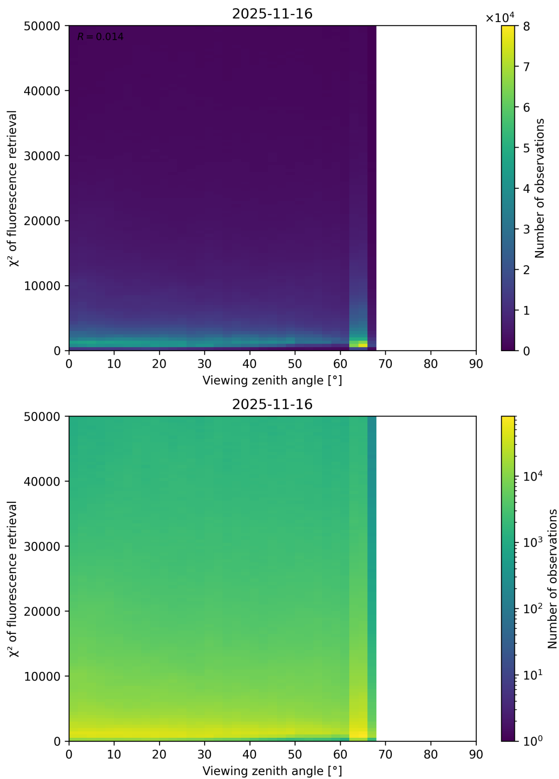
Figure 119: Scatter density plot of “Viewing zenith angle” against “ \chi^2 of fluorescence retrieval” for 2025-11-15 to 2025-11-17.
