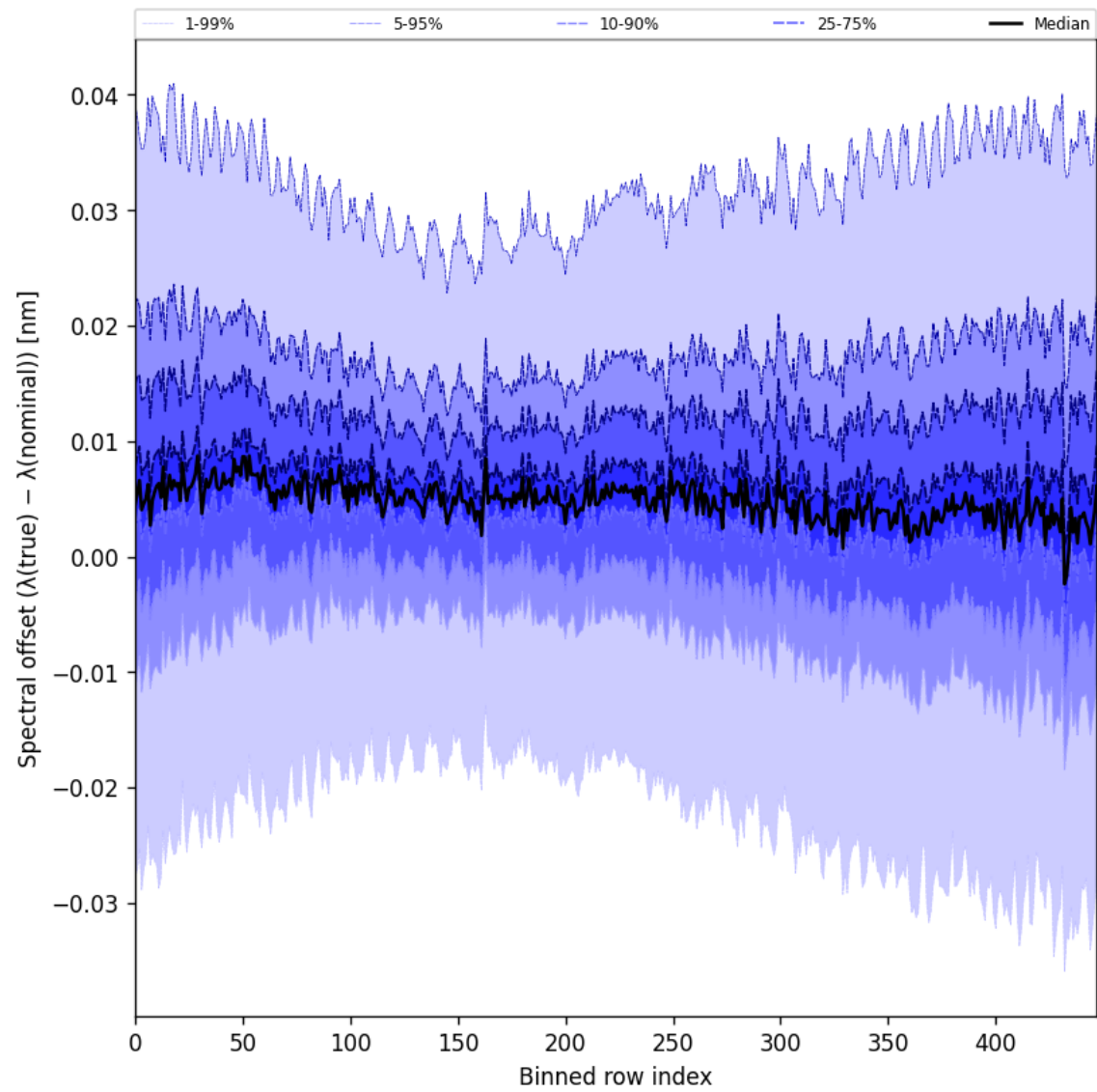
Figure 62: Along track statistics of “Spectral offset ( \lambda_{\text{true}} - \lambda_{\text{nominal}} )” for 2025-11-15 to 2025-11-17
