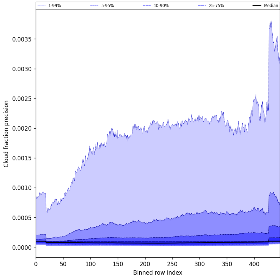
Figure 50: Along track statistics of “Cloud fraction precision” for 2025-11-15 to 2025-11-17
