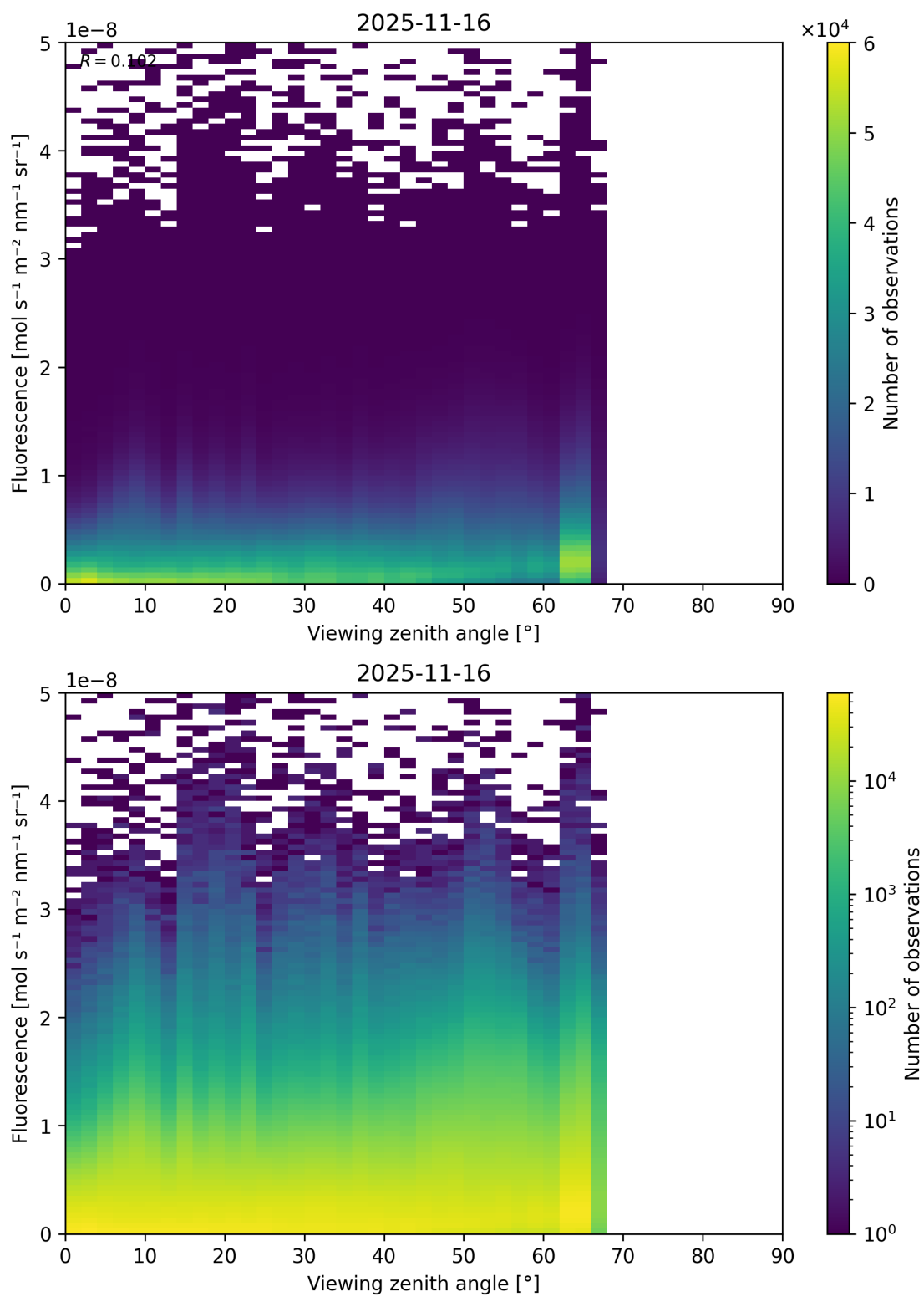
Figure 122: Scatter density plot of “Viewing zenith angle” against “Fluorescence” for 2025-11-15 to 2025-11-17.
