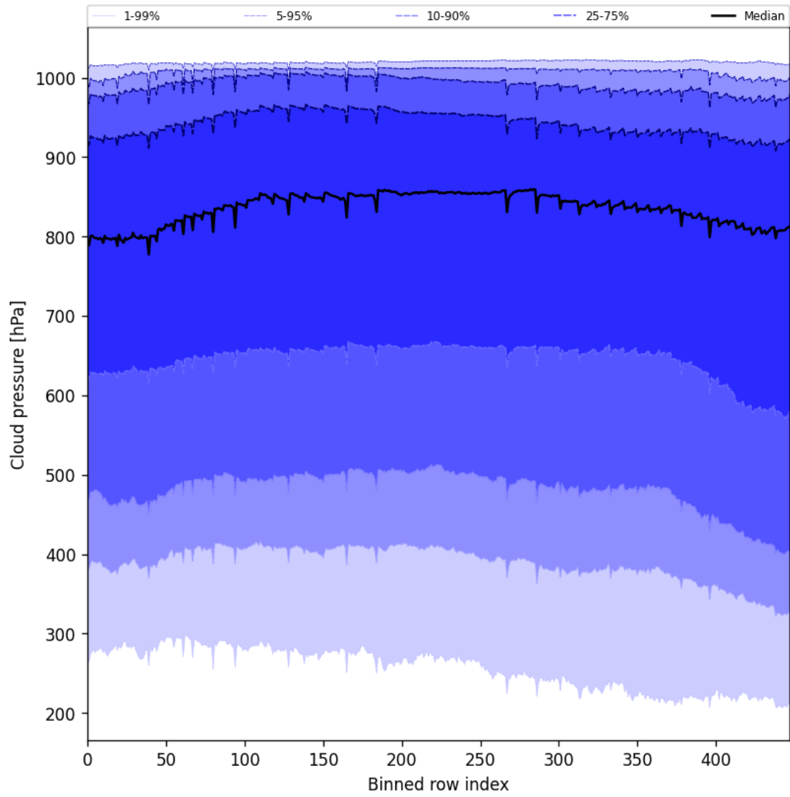
Figure 47: Along track statistics of “Cloud pressure” for 2025-11-15 to 2025-11-17
