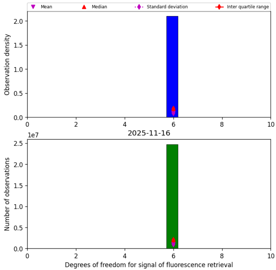
Figure 43: Histogram of “Degrees of freedom for signal of fluorescence retrieval” for 2025-11-15 to 2025-11-17
