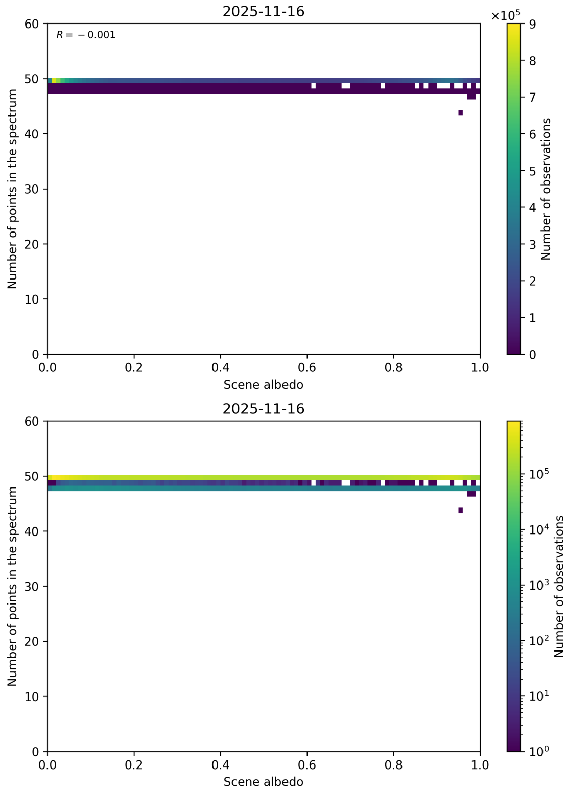
Figure 106: Scatter density plot of “Scene albedo” against “Number of points in the spectrum” for 2025-11-15 to 2025-11-17.
