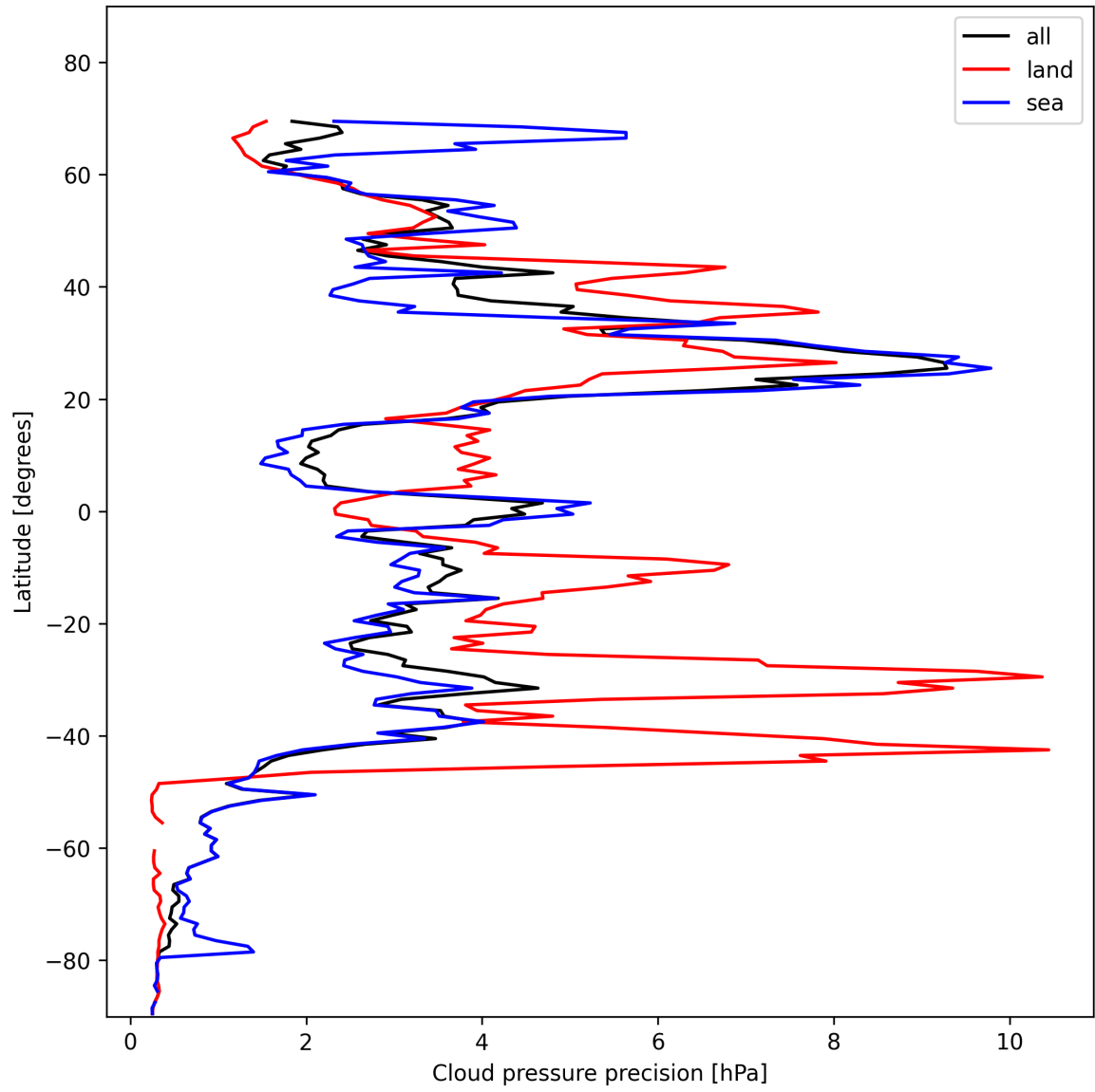
Figure 14: Zonal average of “Cloud pressure precision” for 2025-11-15 to 2025-11-17.
