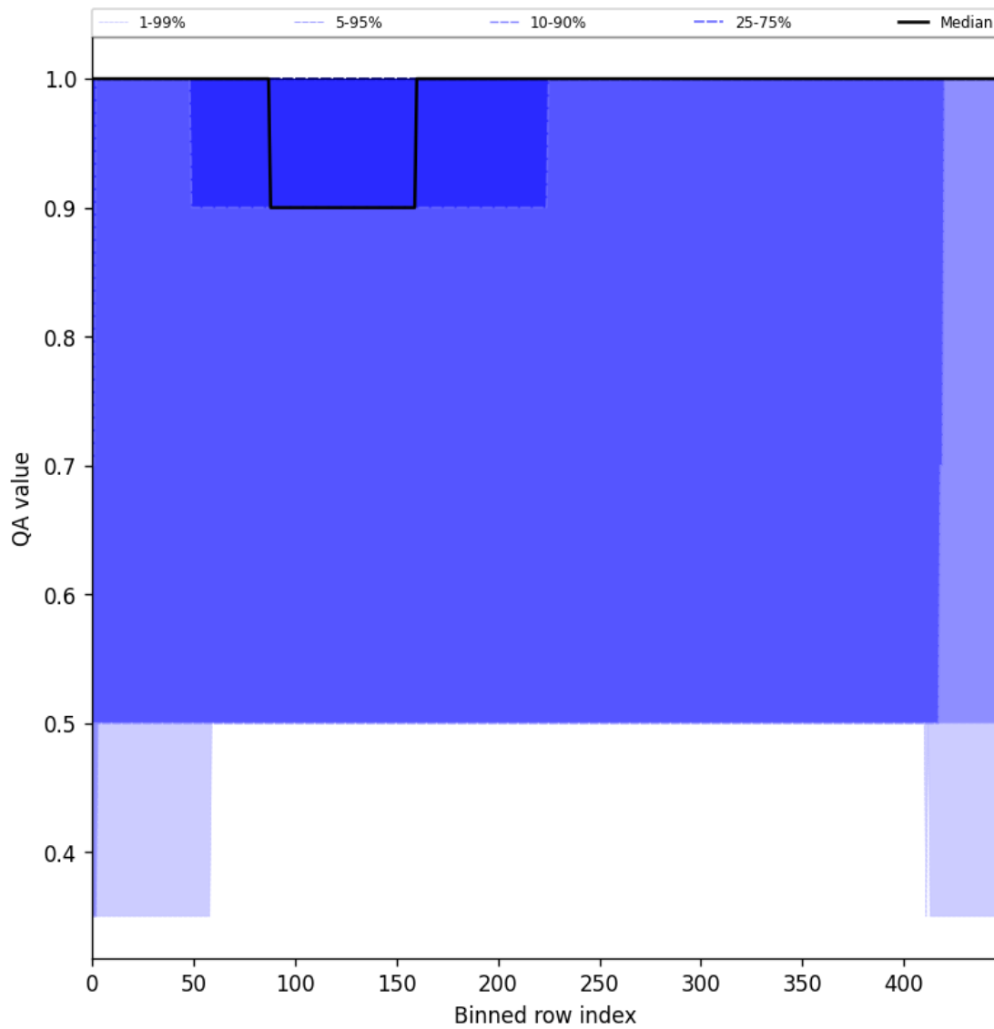
Figure 46: Along track statistics of “QA value” for 2025-11-15 to 2025-11-17
