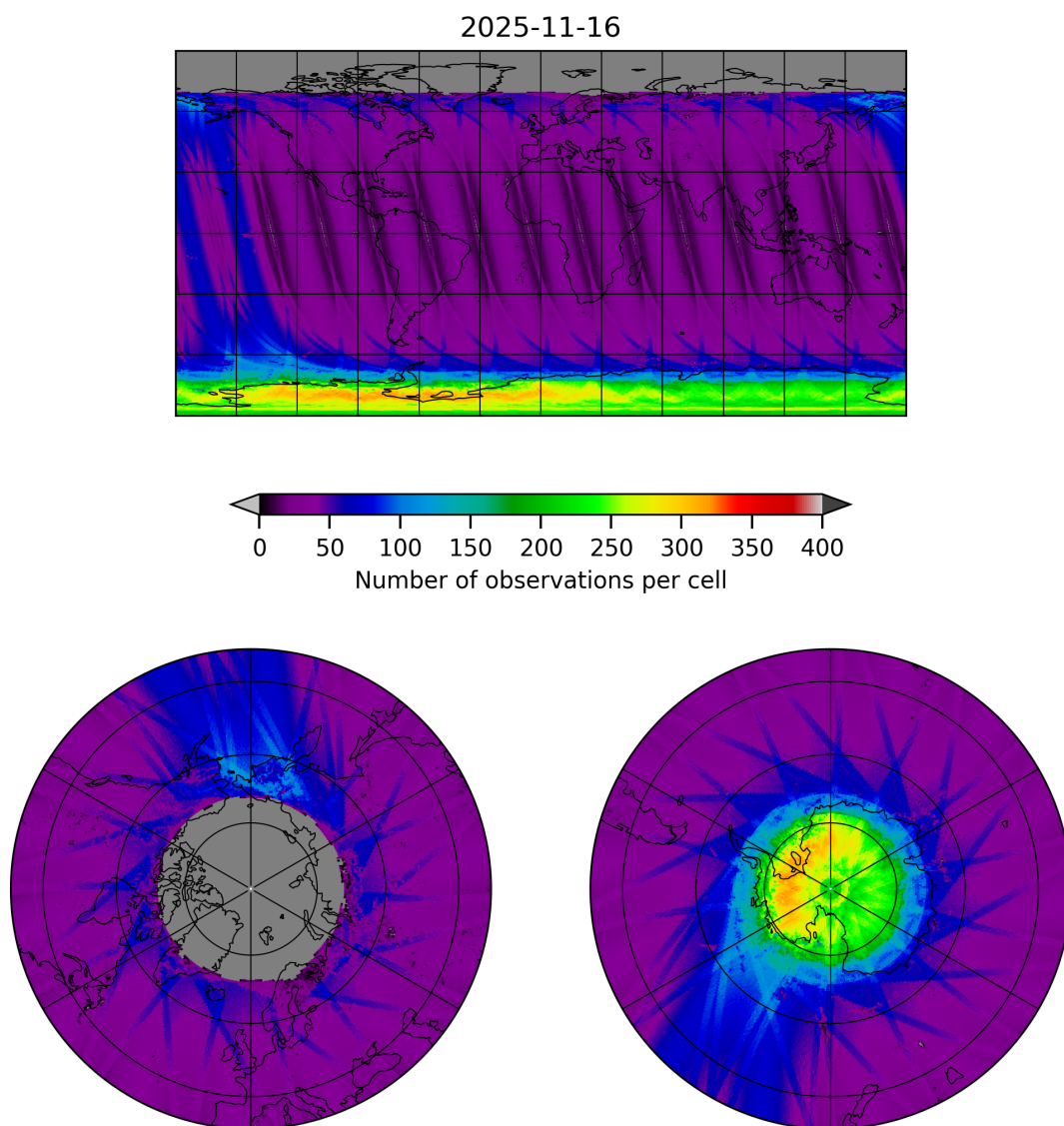
Figure 11: Map of the number of observations for 2025-11-15 to 2025-11-17
