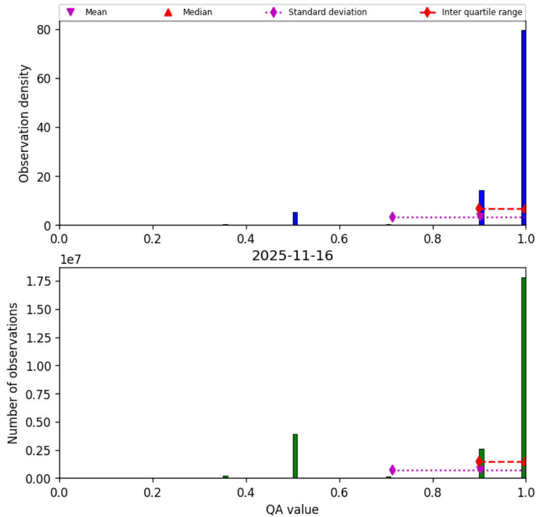
Figure 29: Histogram of “QA value” for 2025-11-15 to 2025-11-17
