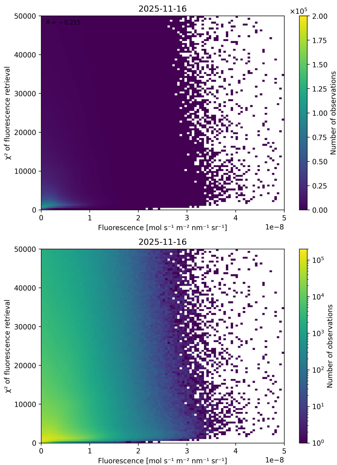
Figure 85: Scatter density plot of “Fluorescence” against “ \chi^2 of fluorescence retrieval” for 2025-11-15 to 2025-11-17.
