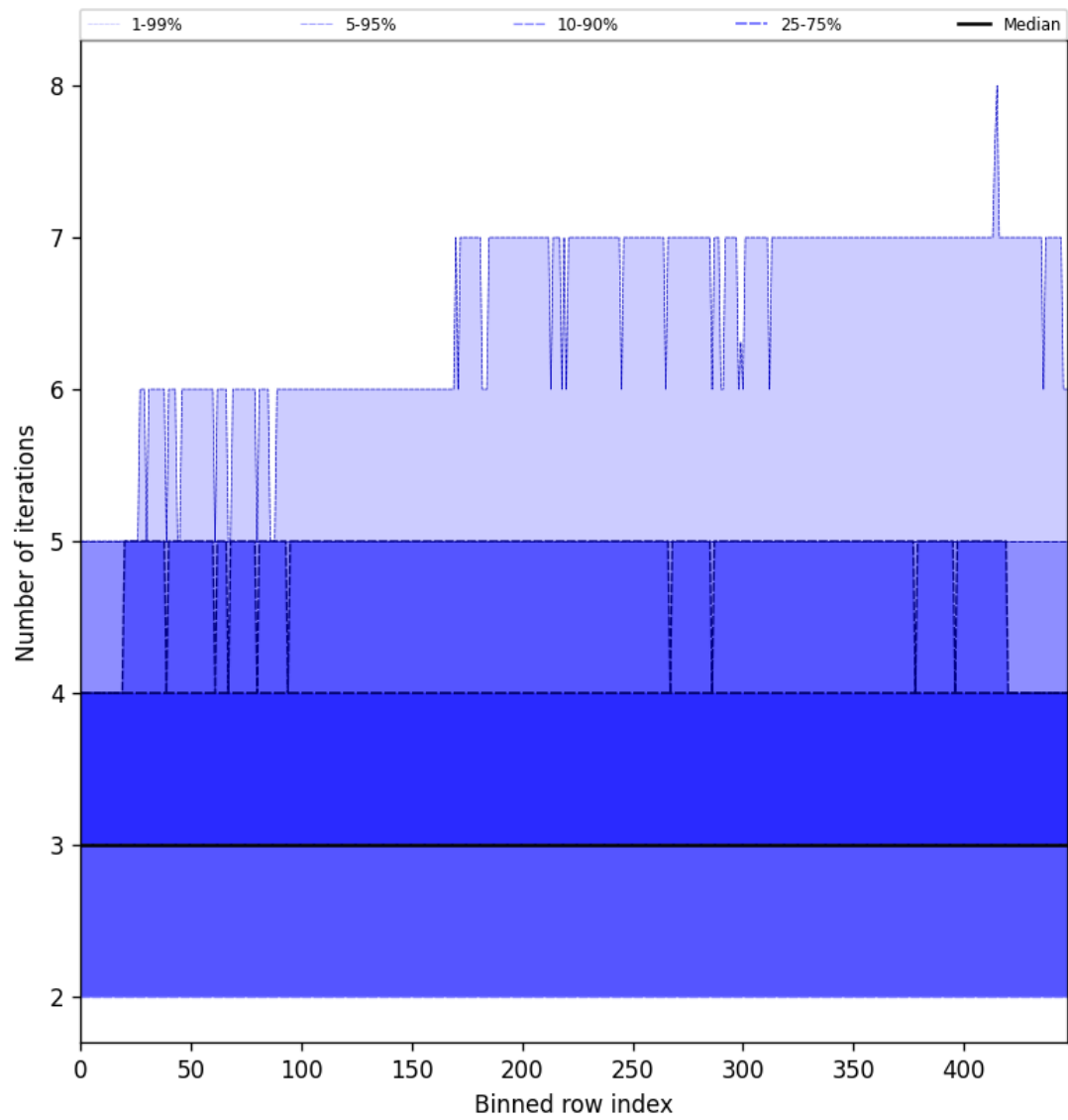
Figure 56: Along track statistics of “Number of iterations” for 2025-11-15 to 2025-11-17
