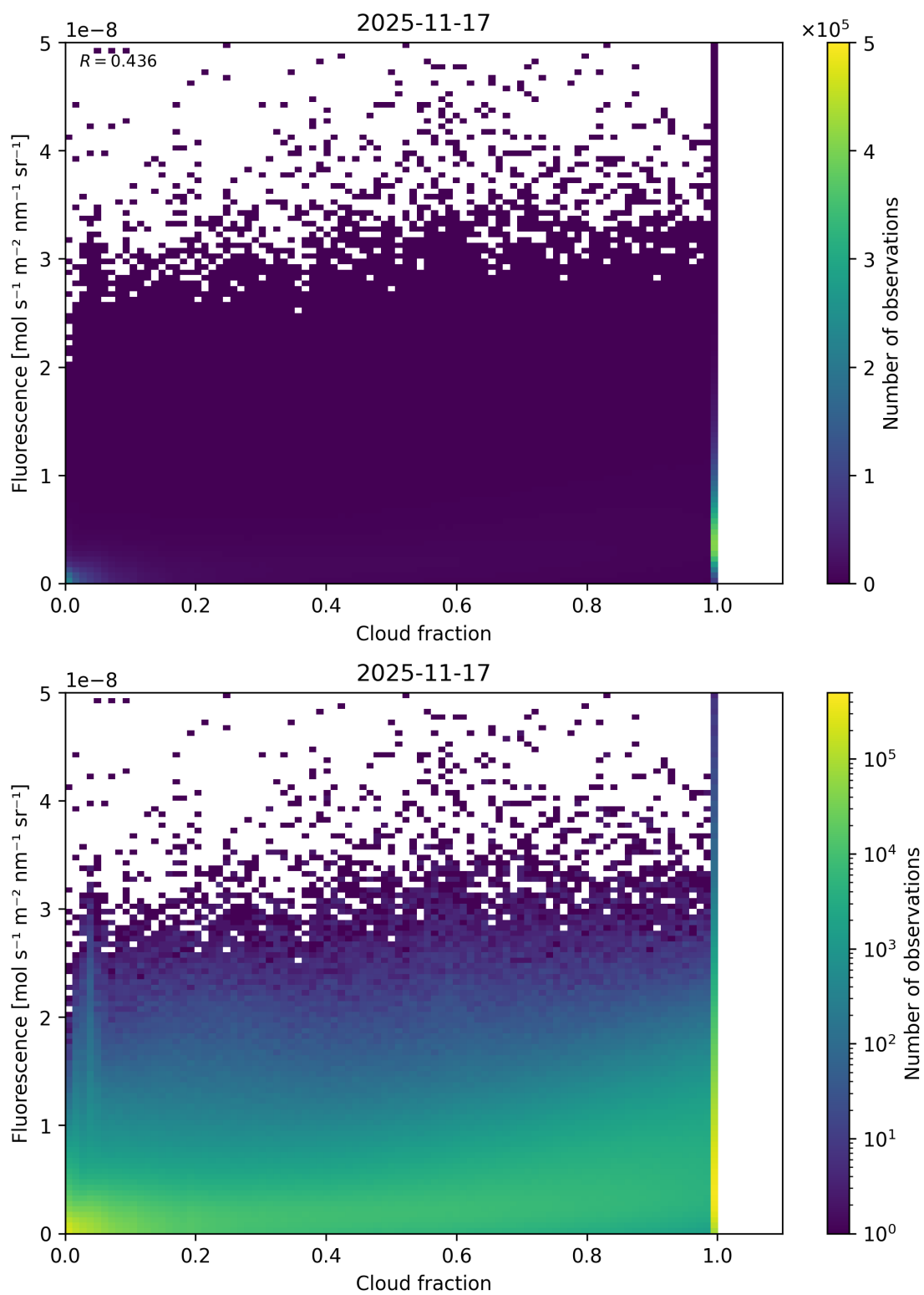
Figure 72: Scatter density plot of “Cloud fraction” against “Fluorescence” for 2025-11-16 to 2025-11-18.
