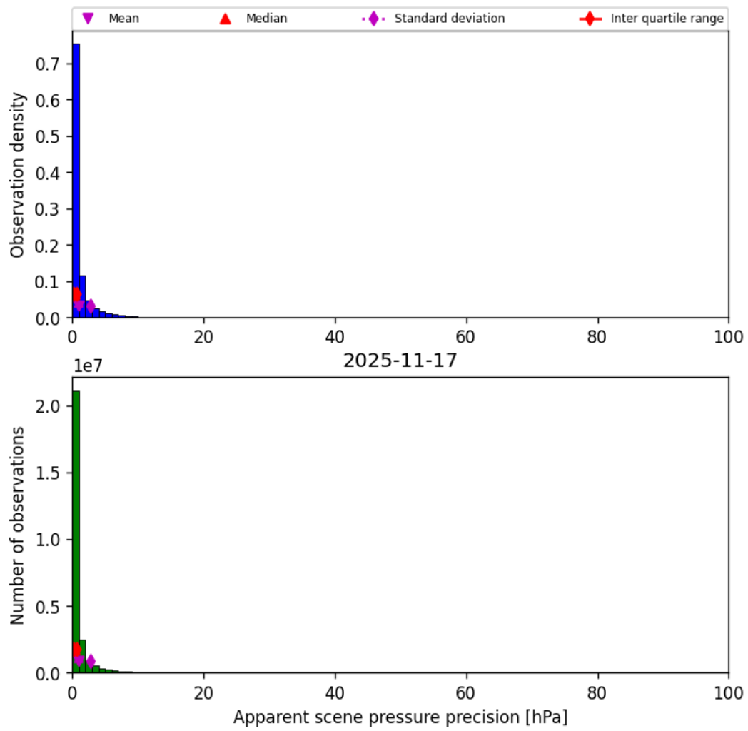
Figure 37: Histogram of “Apparent scene pressure precision” for 2025-11-16 to 2025-11-18
