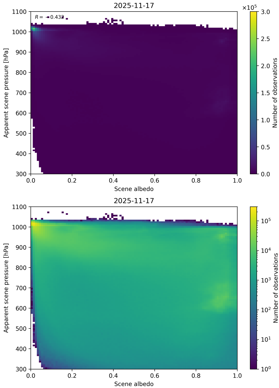
Figure 102: Scatter density plot of “Scene albedo” against “Apparent scene pressure” for 2025-11-16 to 2025-11-18.
