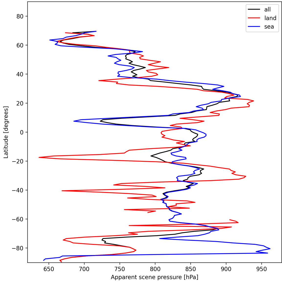
Figure 19: Zonal average of “Apparent scene pressure” for 2025-11-16 to 2025-11-18.
