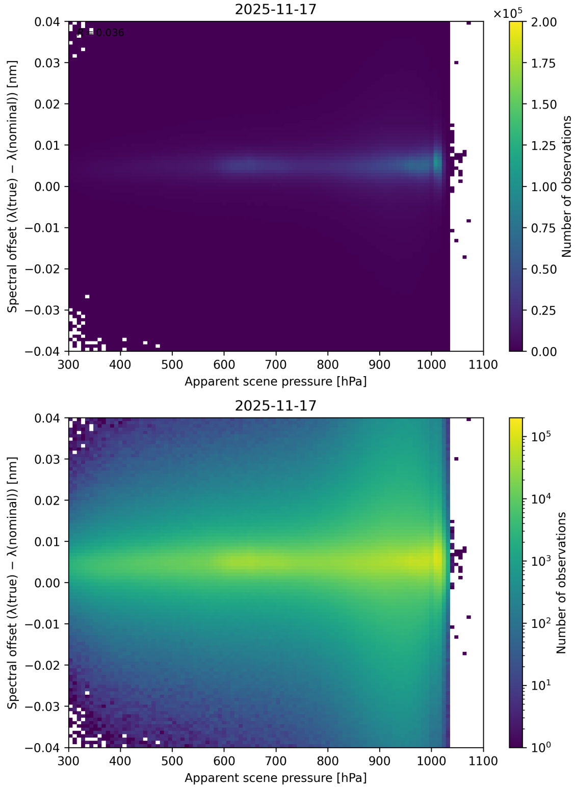
Figure 67: Scatter density plot of “Apparent scene pressure” against “Spectral offset ( \lambda_{\text{true}} - \lambda_{\text{nominal}} )” for 2025-11-16 to 2025-11-18.
