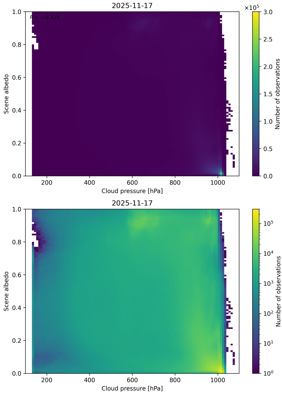
Figure 83: Scatter density plot of “Cloud pressure” against “Scene albedo” for 2025-11-16 to 2025-11-18.
