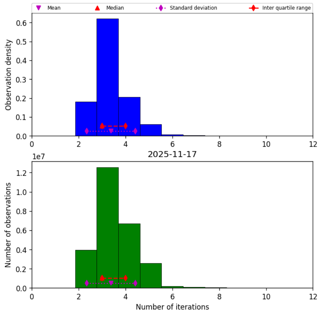
Figure 39: Histogram of “Number of iterations” for 2025-11-16 to 2025-11-18
