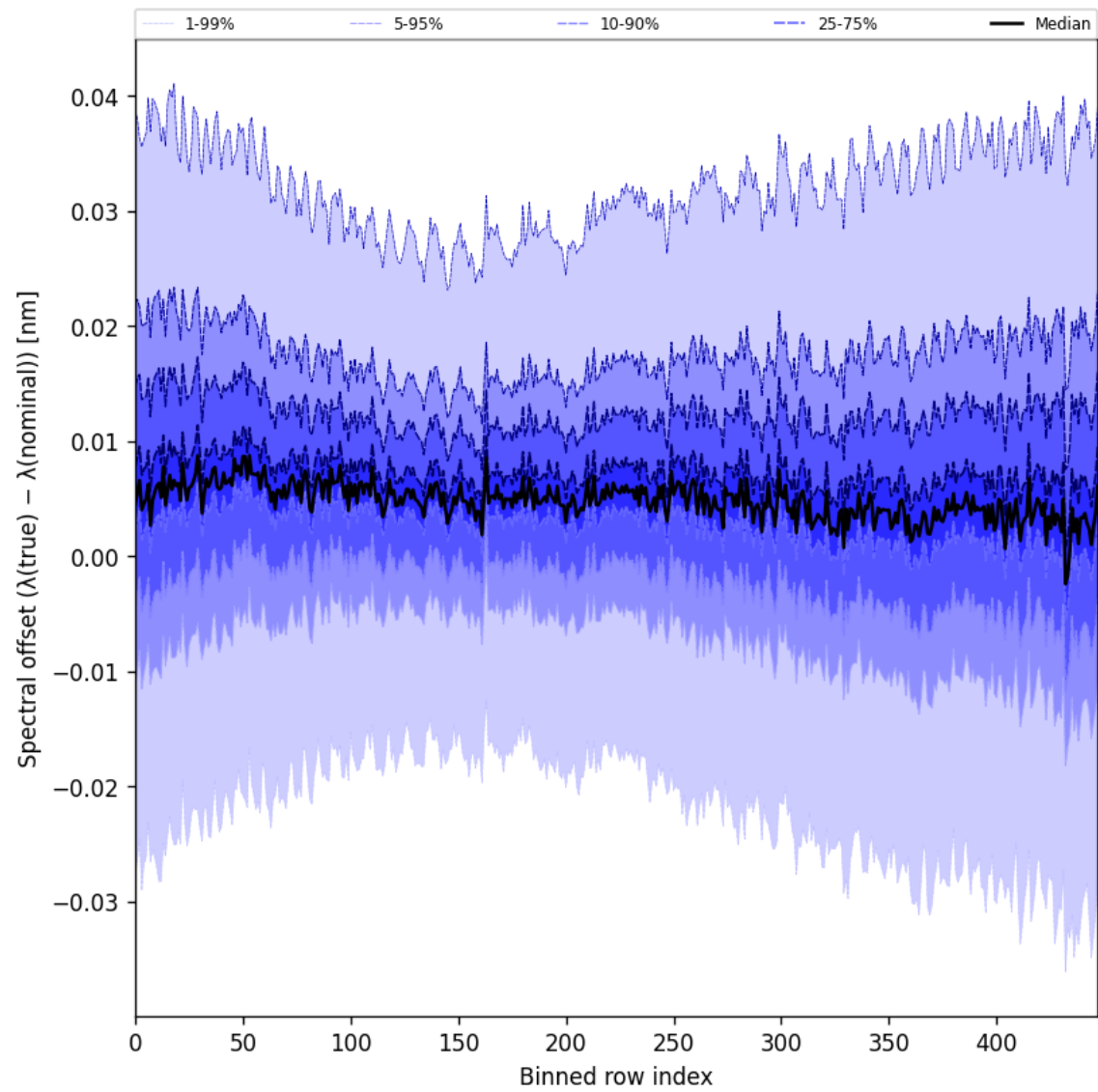
Figure 62: Along track statistics of “Spectral offset ( \lambda_{\text{true}} - \lambda_{\text{nominal}} )” for 2025-11-16 to 2025-11-18
