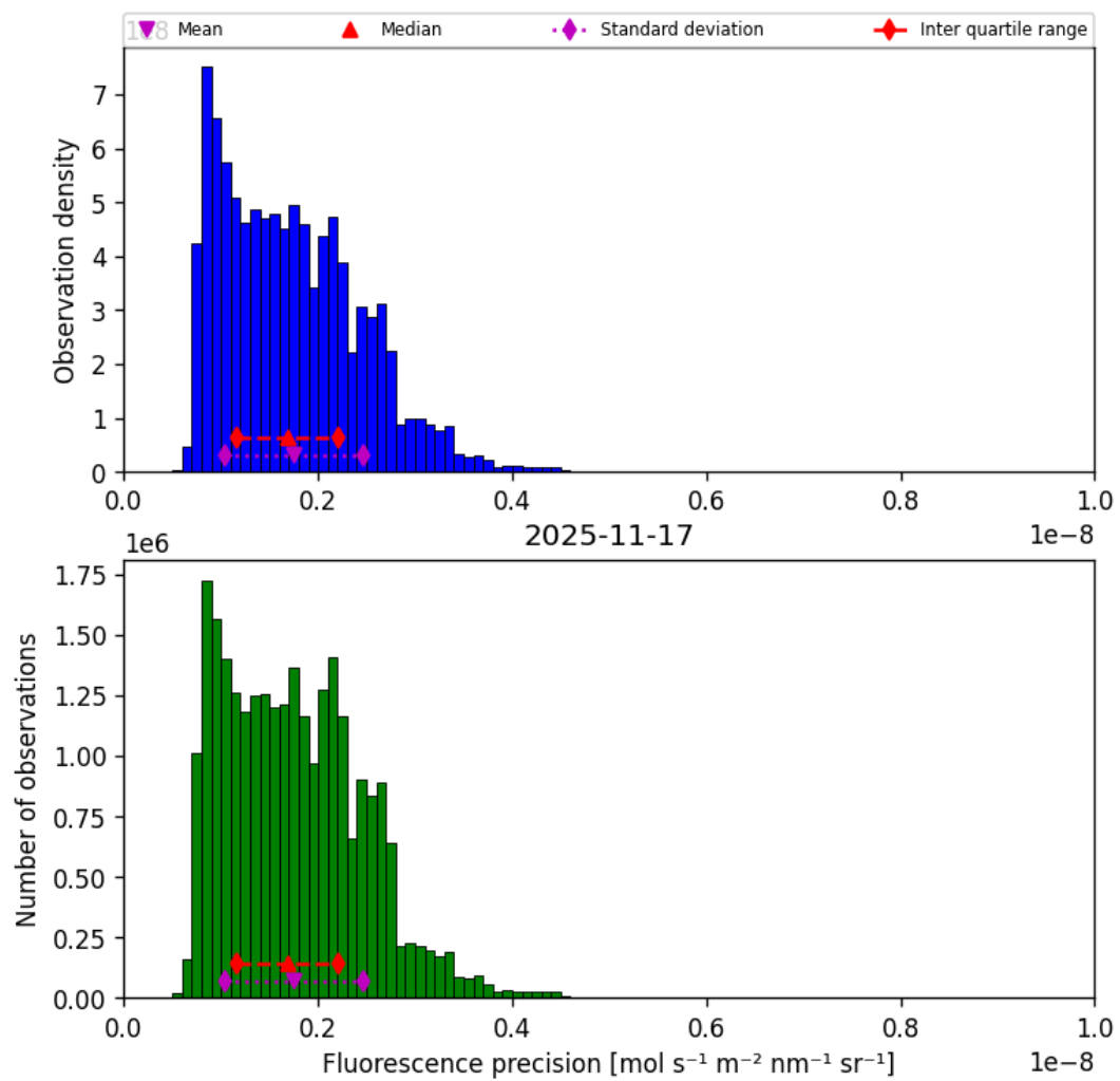
Figure 41: Histogram of “Fluorescence precision” for 2025-11-16 to 2025-11-18
