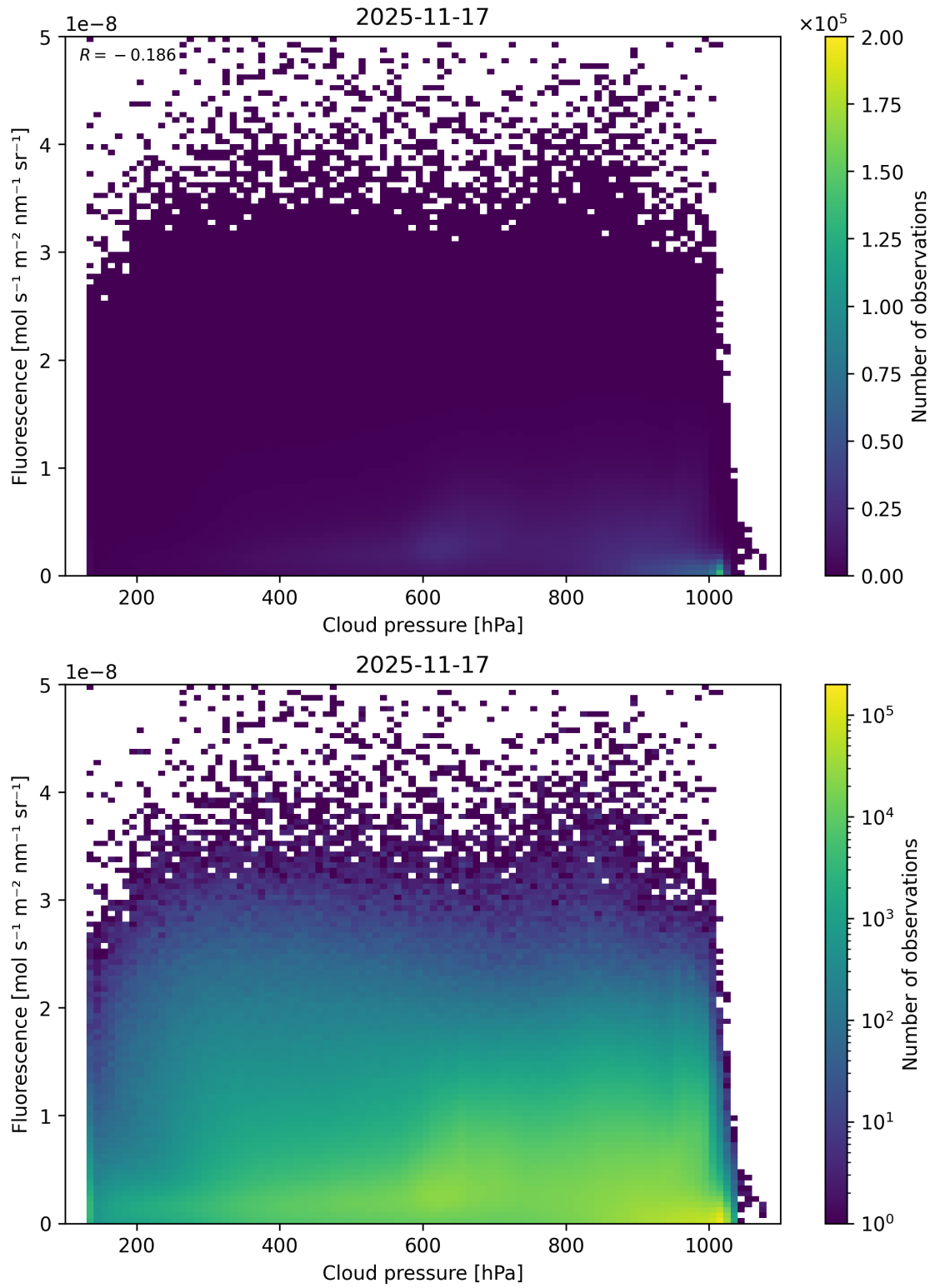
Figure 80: Scatter density plot of “Cloud pressure” against “Fluorescence” for 2025-11-16 to 2025-11-18.
