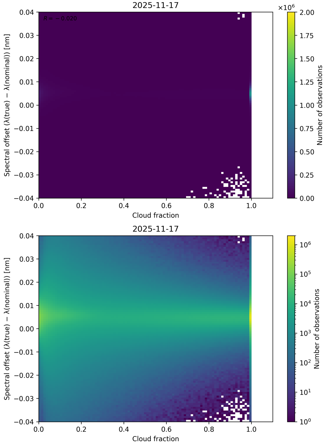
Figure 76: Scatter density plot of “Cloud fraction” against “Spectral offset ( \lambda_{\text{true}} - \lambda_{\text{nominal}} )” for 2025-11-16 to 2025-11-18.
