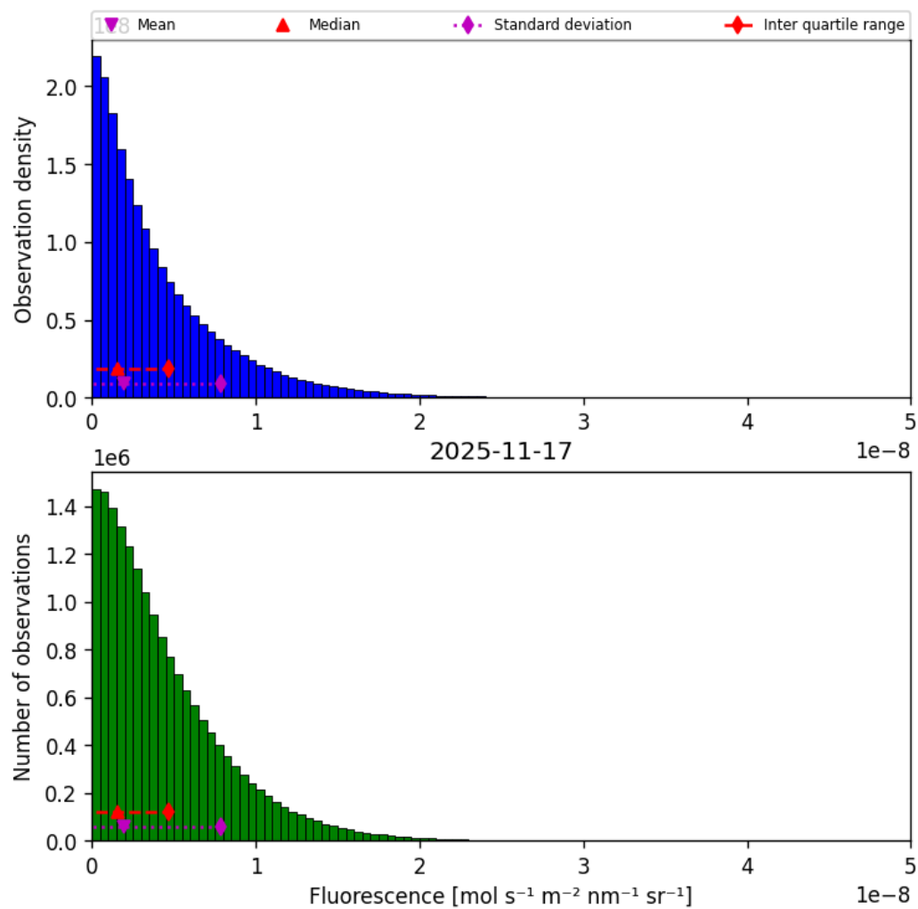
Figure 40: Histogram of “Fluorescence” for 2025-11-16 to 2025-11-18
