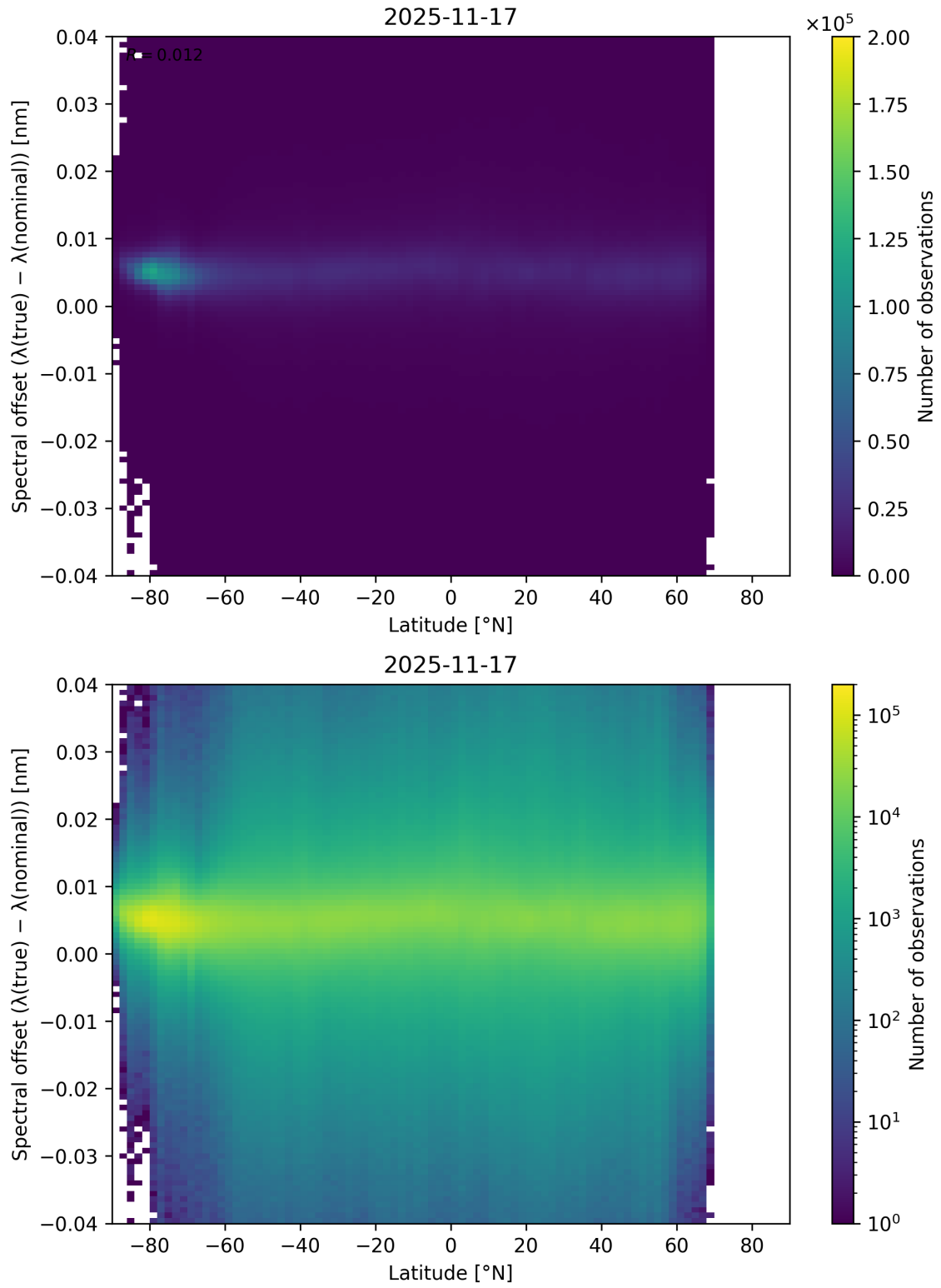
Figure 96: Scatter density plot of “Latitude” against “Spectral offset ( \lambda_{\text{true}} - \lambda_{\text{nominal}} )” for 2025-11-16 to 2025-11-18.
