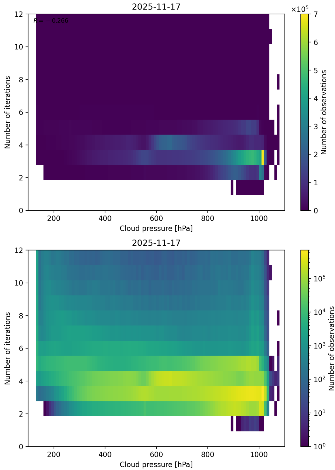
Figure 81: Scatter density plot of “Cloud pressure” against “Number of iterations” for 2025-11-16 to 2025-11-18.
