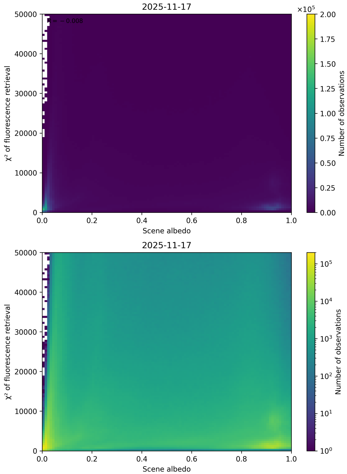
Figure 103: Scatter density plot of “Scene albedo” against “ \chi^2 of fluorescence retrieval” for 2025-11-16 to 2025-11-18.
