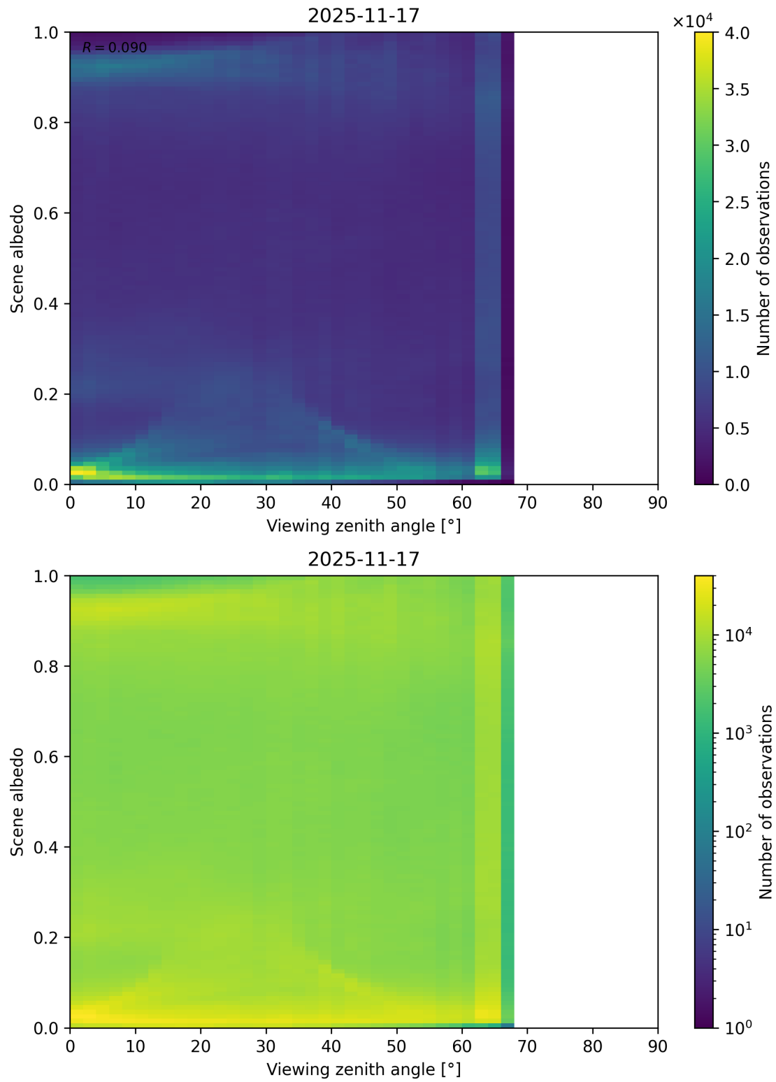
Figure 126: Scatter density plot of “Viewing zenith angle” against “Scene albedo” for 2025-11-16 to 2025-11-18.
