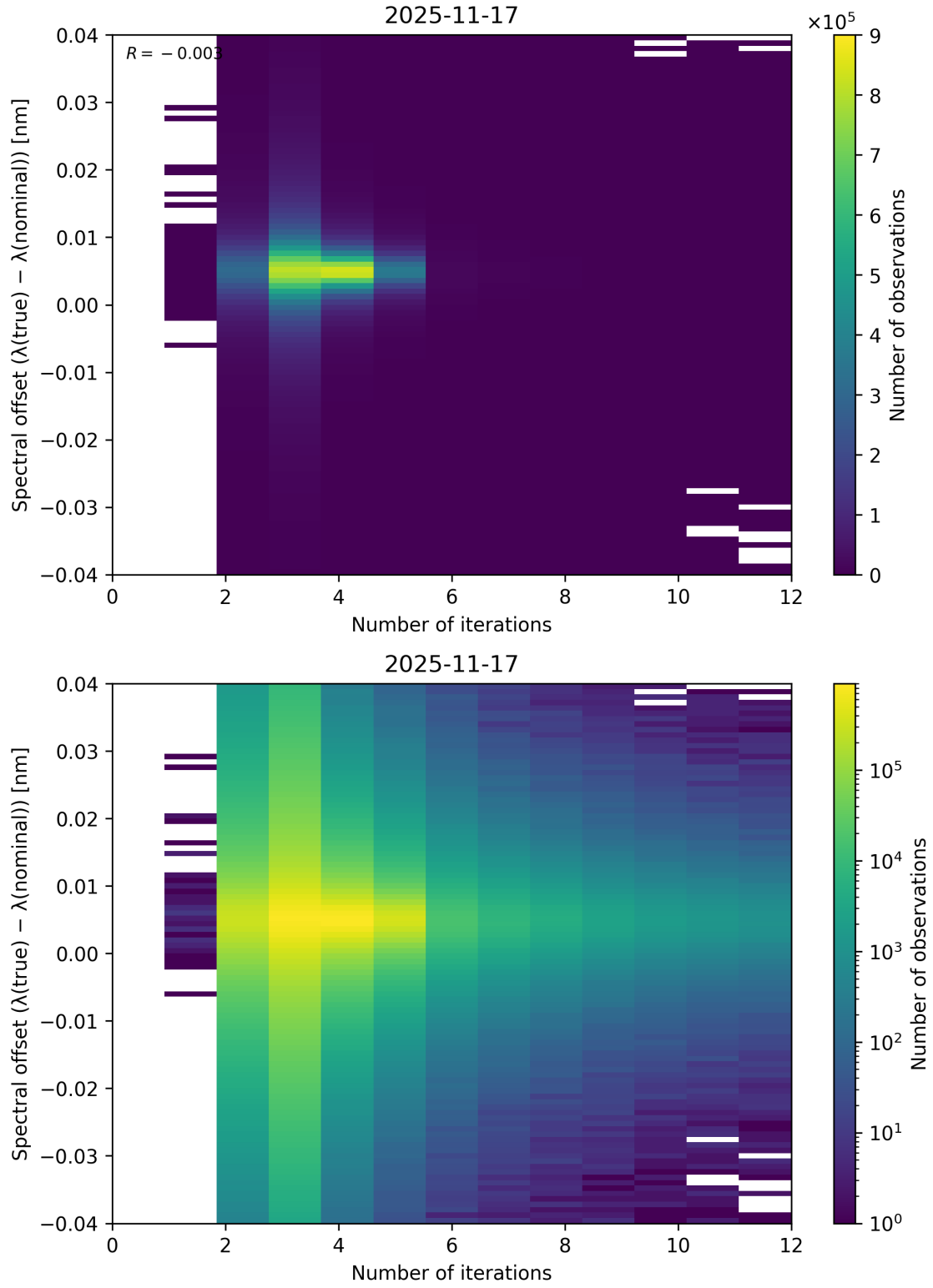
Figure 100: Scatter density plot of “Number of iterations” against “Spectral offset ( \lambda_{\text{true}} - \lambda_{\text{nominal}} )” for 2025-11-16 to 2025-11-18.
