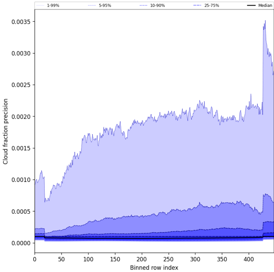
Figure 50: Along track statistics of “Cloud fraction precision” for 2025-11-16 to 2025-11-18
