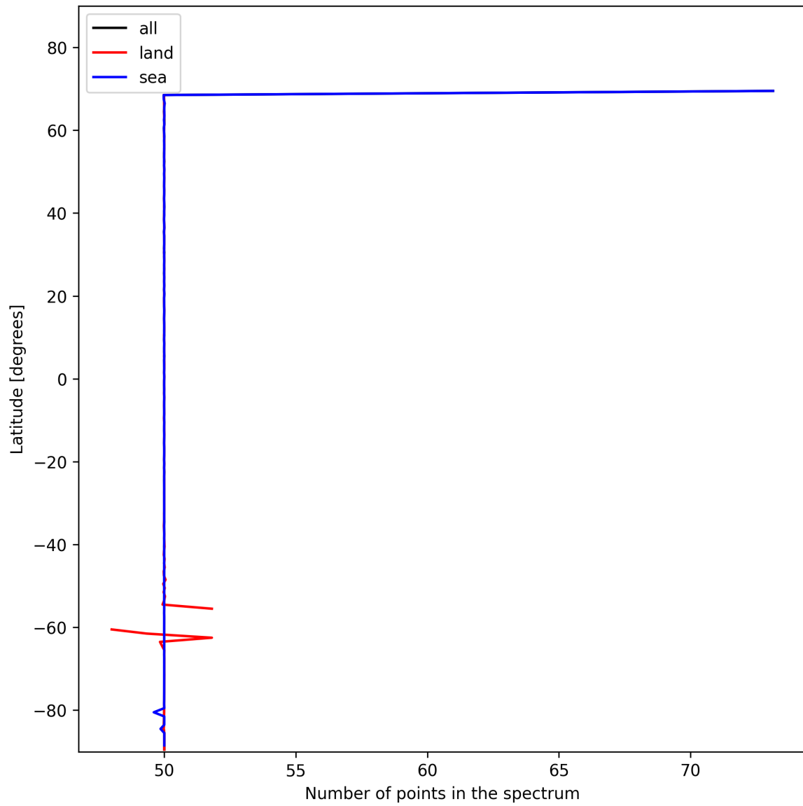
Figure 27: Zonal average of “Number of points in the spectrum” for 2025-11-16 to 2025-11-18.
