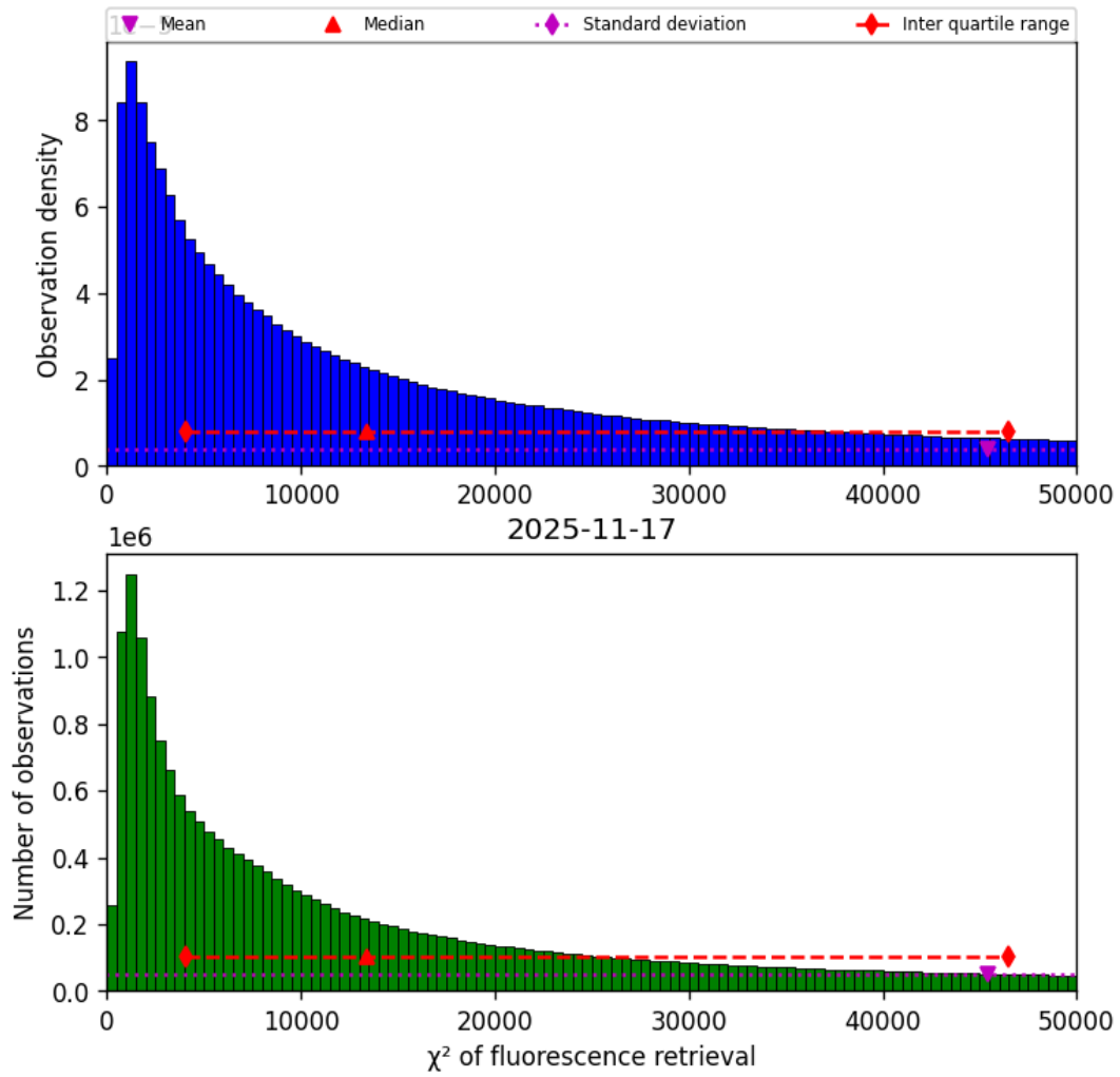
Figure 42: Histogram of “ \chi^2 of fluorescence retrieval” for 2025-11-16 to 2025-11-18
