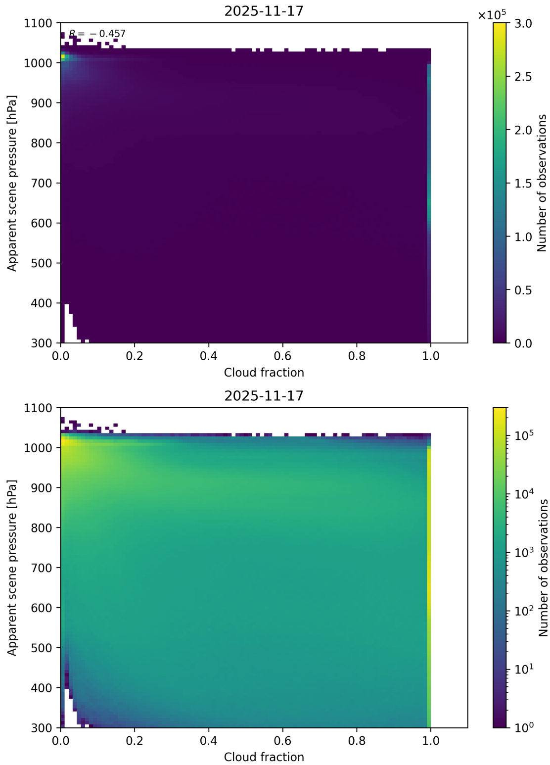
Figure 70: Scatter density plot of “Cloud fraction” against “Apparent scene pressure” for 2025-11-16 to 2025-11-18.
