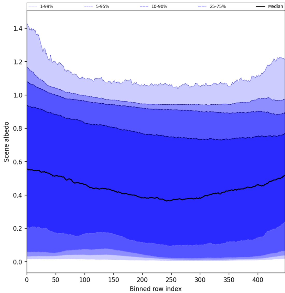
Figure 51: Along track statistics of “Scene albedo” for 2025-11-16 to 2025-11-18
