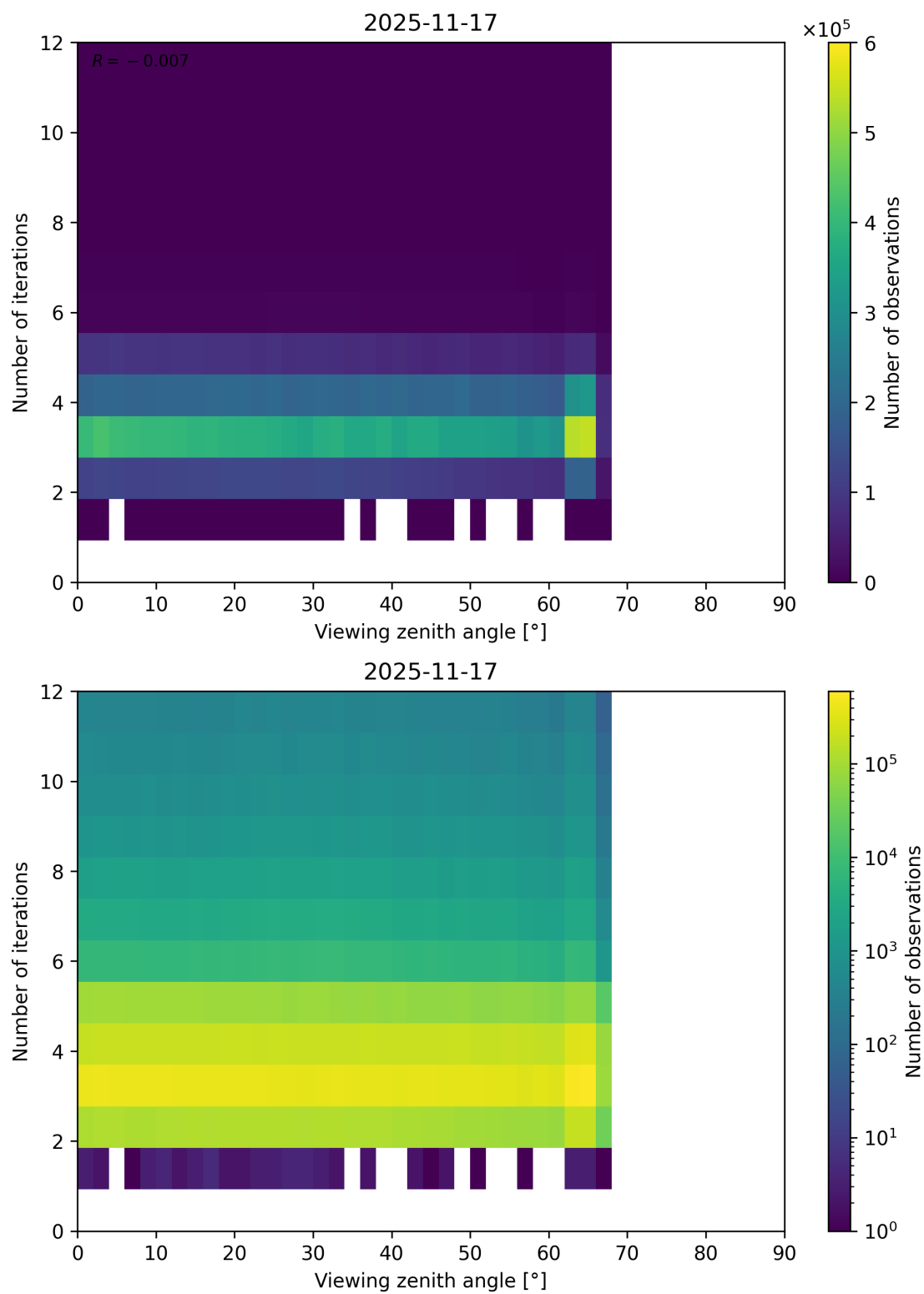
Figure 124: Scatter density plot of “Viewing zenith angle” against “Number of iterations” for 2025-11-16 to 2025-11-18.
