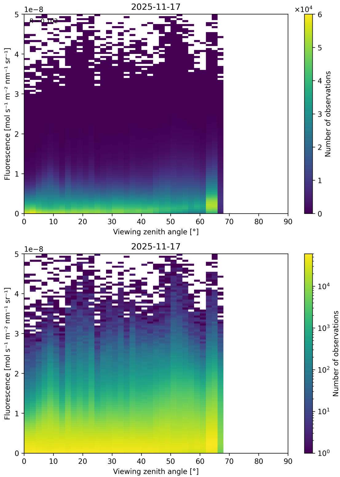
Figure 122: Scatter density plot of “Viewing zenith angle” against “Fluorescence” for 2025-11-16 to 2025-11-18.
