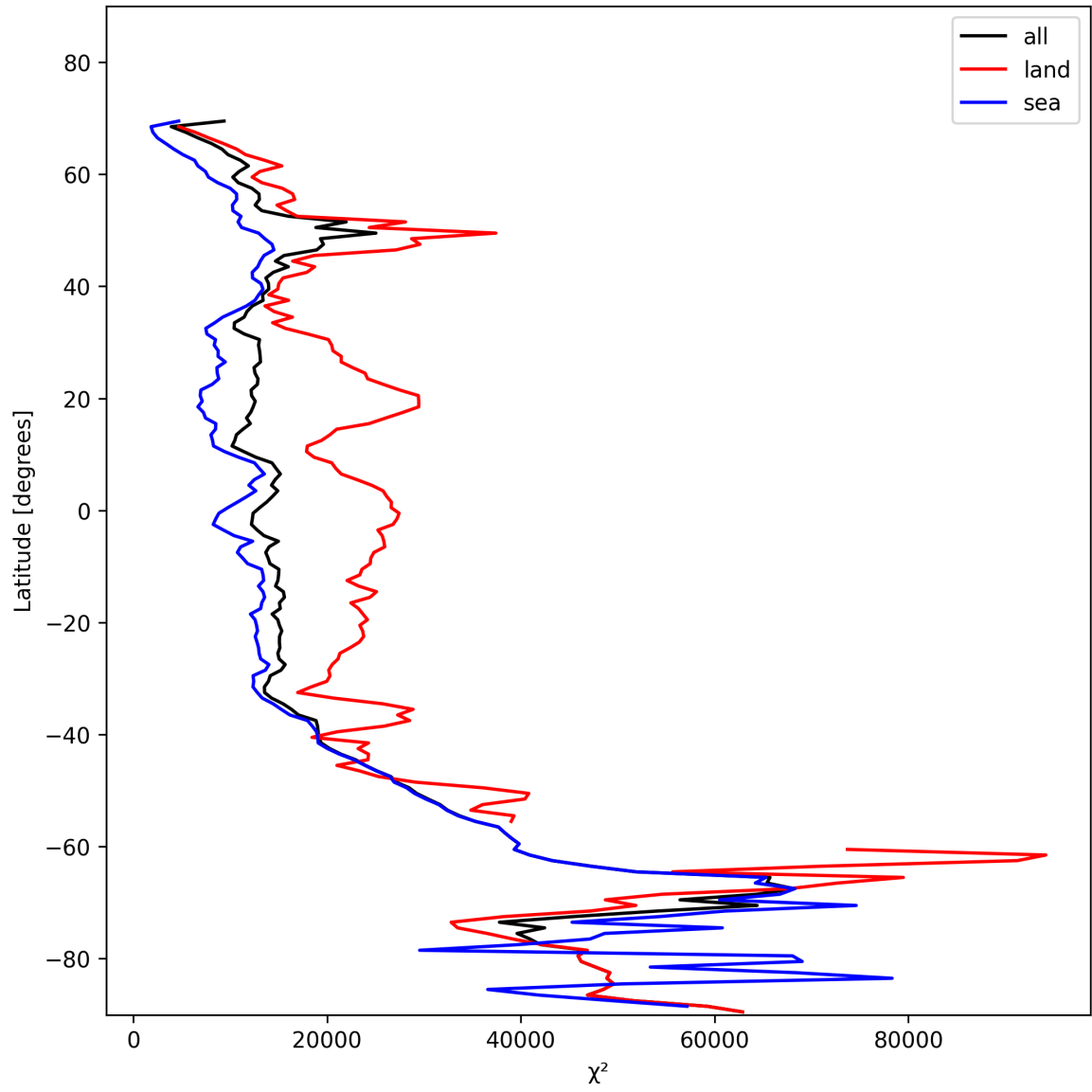
Figure 21: Zonal average of “ \chi^2 ” for 2025-11-16 to 2025-11-18.
