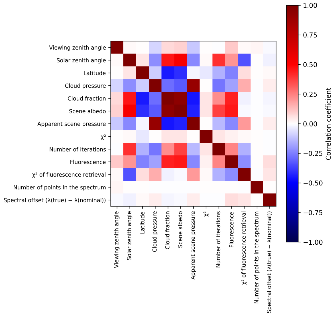
Figure 2: Map of correlation matrix for 2025-11-16 to 2025-11-18.
