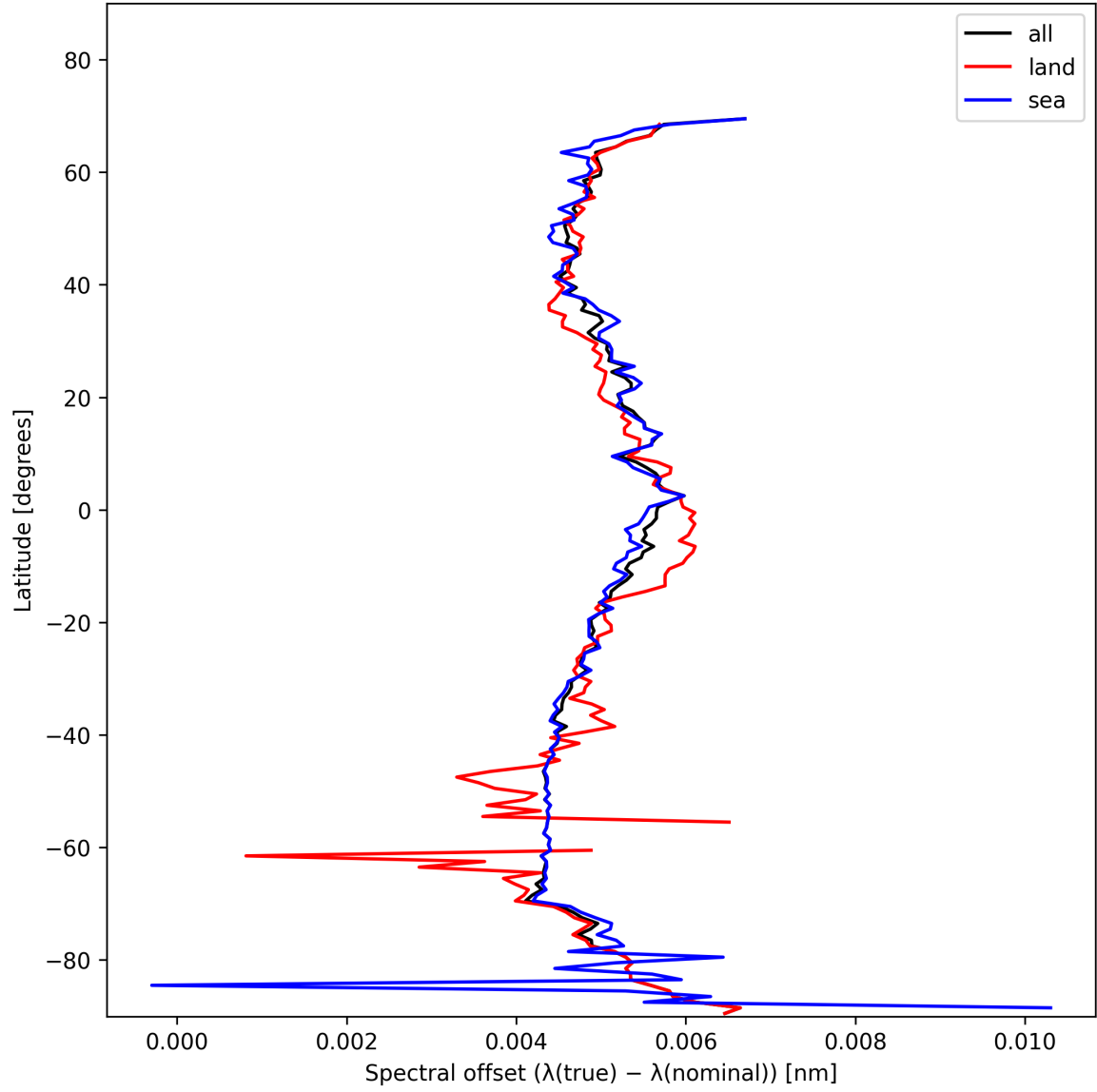
Figure 28: Zonal average of “Spectral offset ( \lambda_{\text{true}} - \lambda_{\text{nominal}} )” for 2025-11-16 to 2025-11-18.
