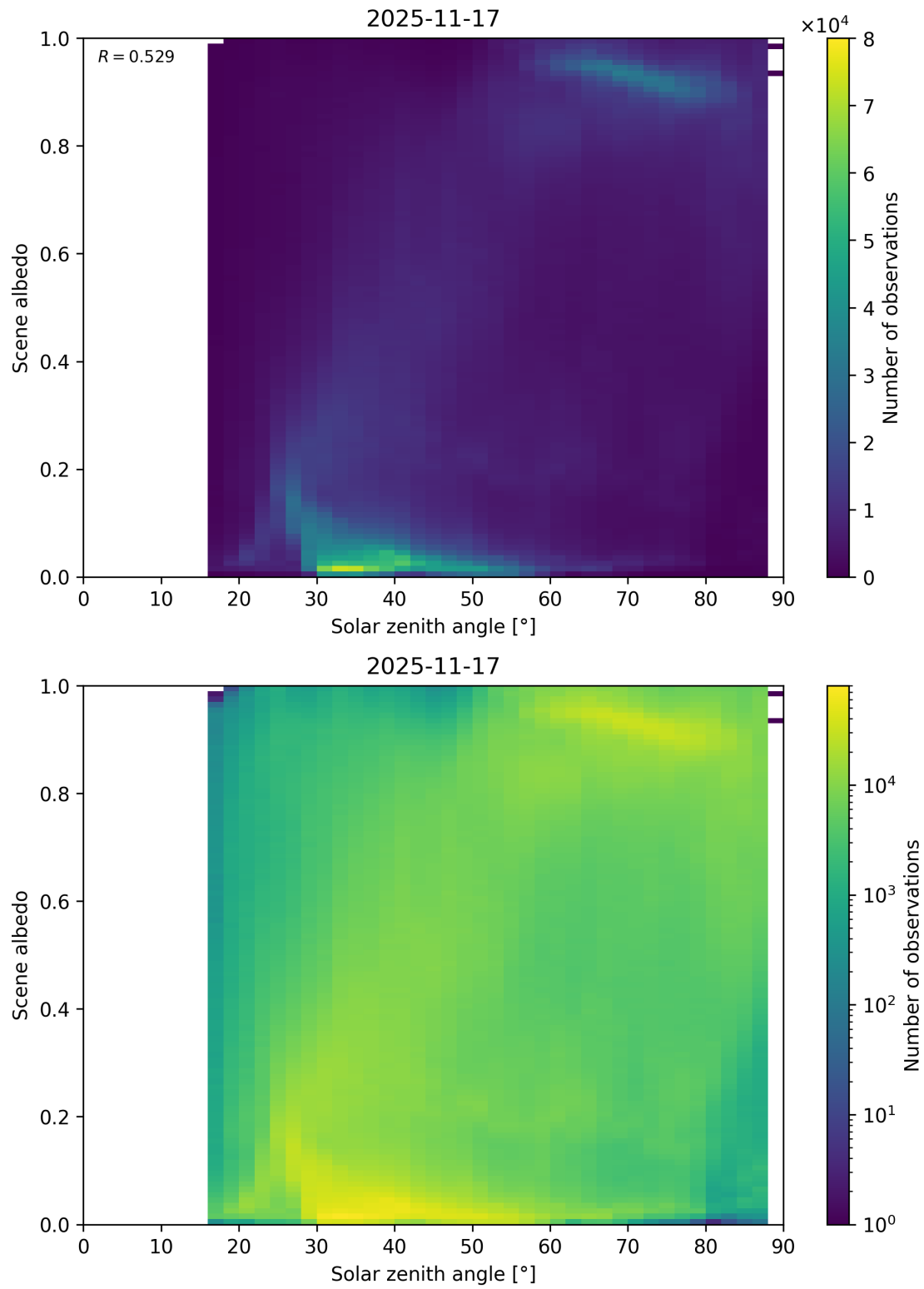
Figure 116: Scatter density plot of “Solar zenith angle” against “Scene albedo” for 2025-11-16 to 2025-11-18.
