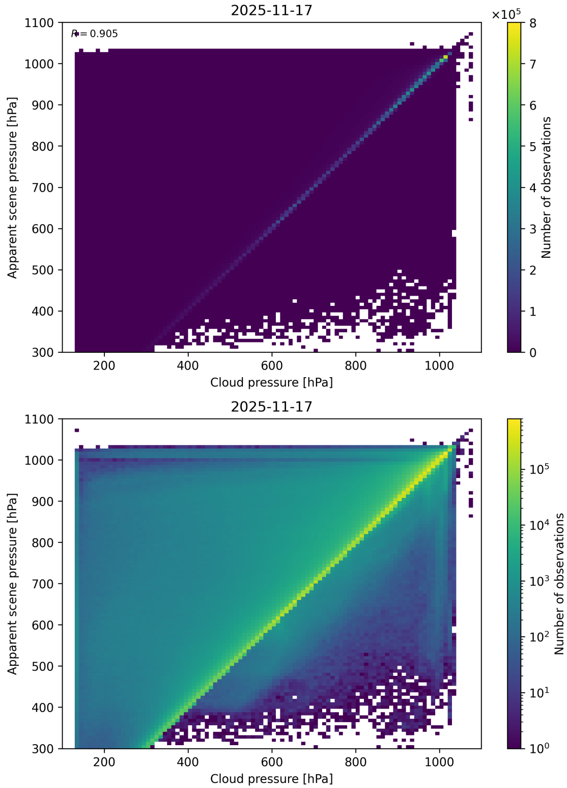
Figure 77: Scatter density plot of “Cloud pressure” against “Apparent scene pressure” for 2025-11-16 to 2025-11-18.
