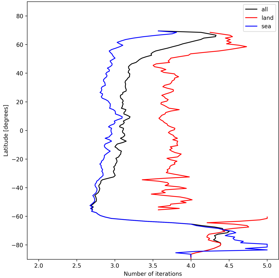
Figure 22: Zonal average of “Number of iterations” for 2025-11-16 to 2025-11-18.
