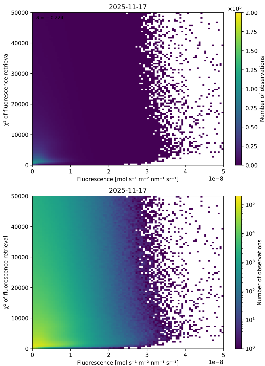
Figure 85: Scatter density plot of “Fluorescence” against “ \chi^2 of fluorescence retrieval” for 2025-11-16 to 2025-11-18.
