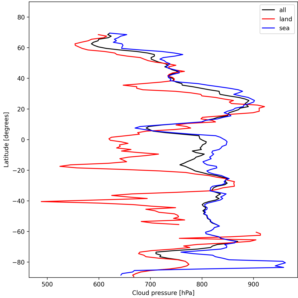
Figure 13: Zonal average of “Cloud pressure” for 2025-11-16 to 2025-11-18.
