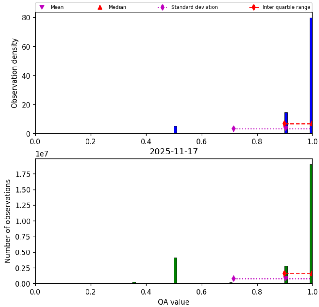
Figure 29: Histogram of “QA value” for 2025-11-16 to 2025-11-18
