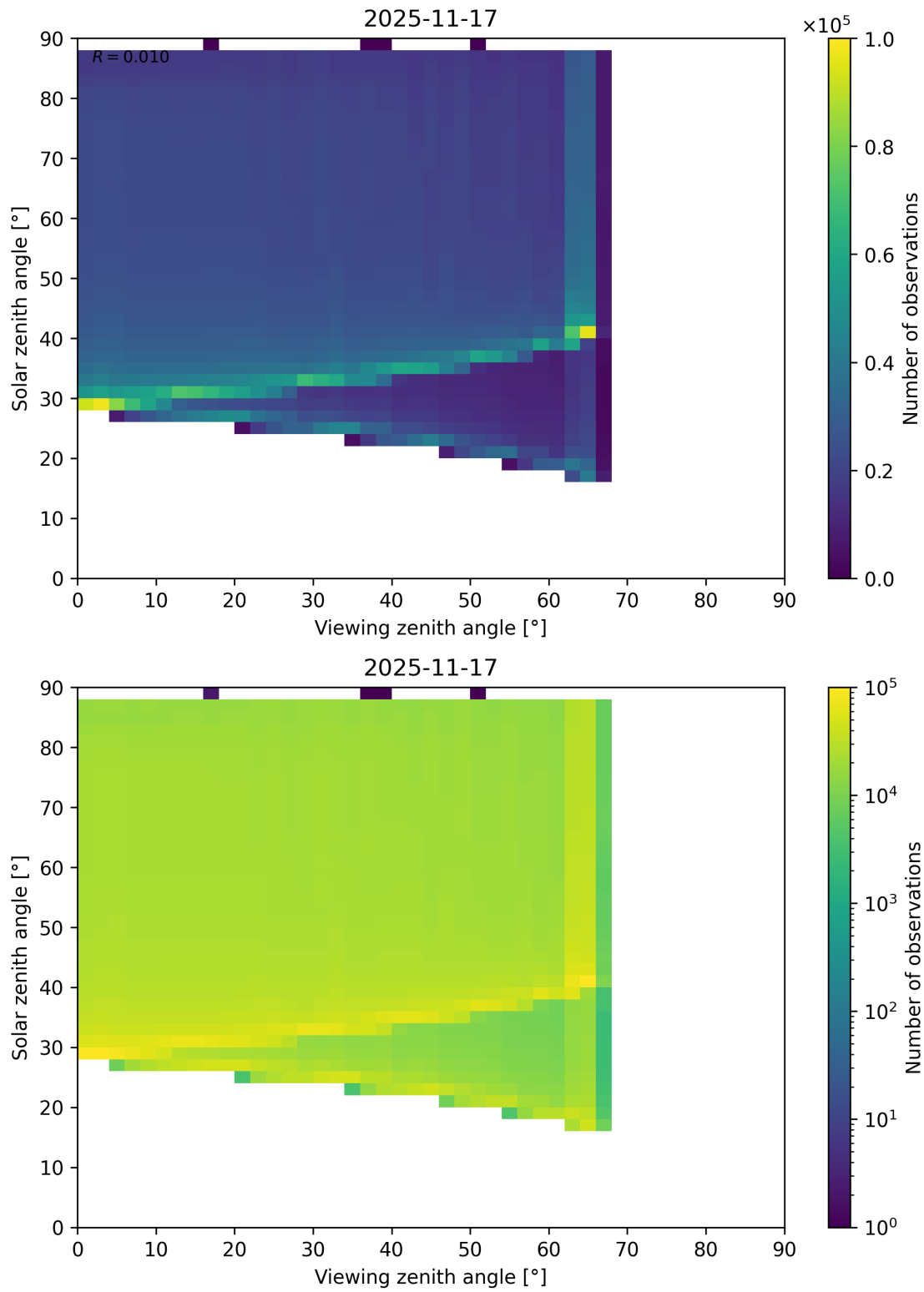
Figure 127: Scatter density plot of “Viewing zenith angle” against “Solar zenith angle” for 2025-11-16 to 2025-11-18.
