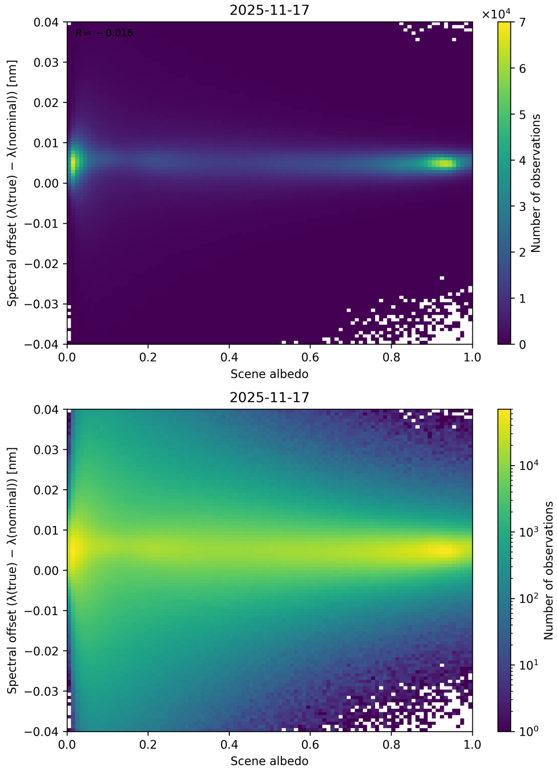
Figure 107: Scatter density plot of “Scene albedo” against “Spectral offset ( \lambda_{\text{true}} - \lambda_{\text{nominal}} )” for 2025-11-16 to 2025-11-18.
