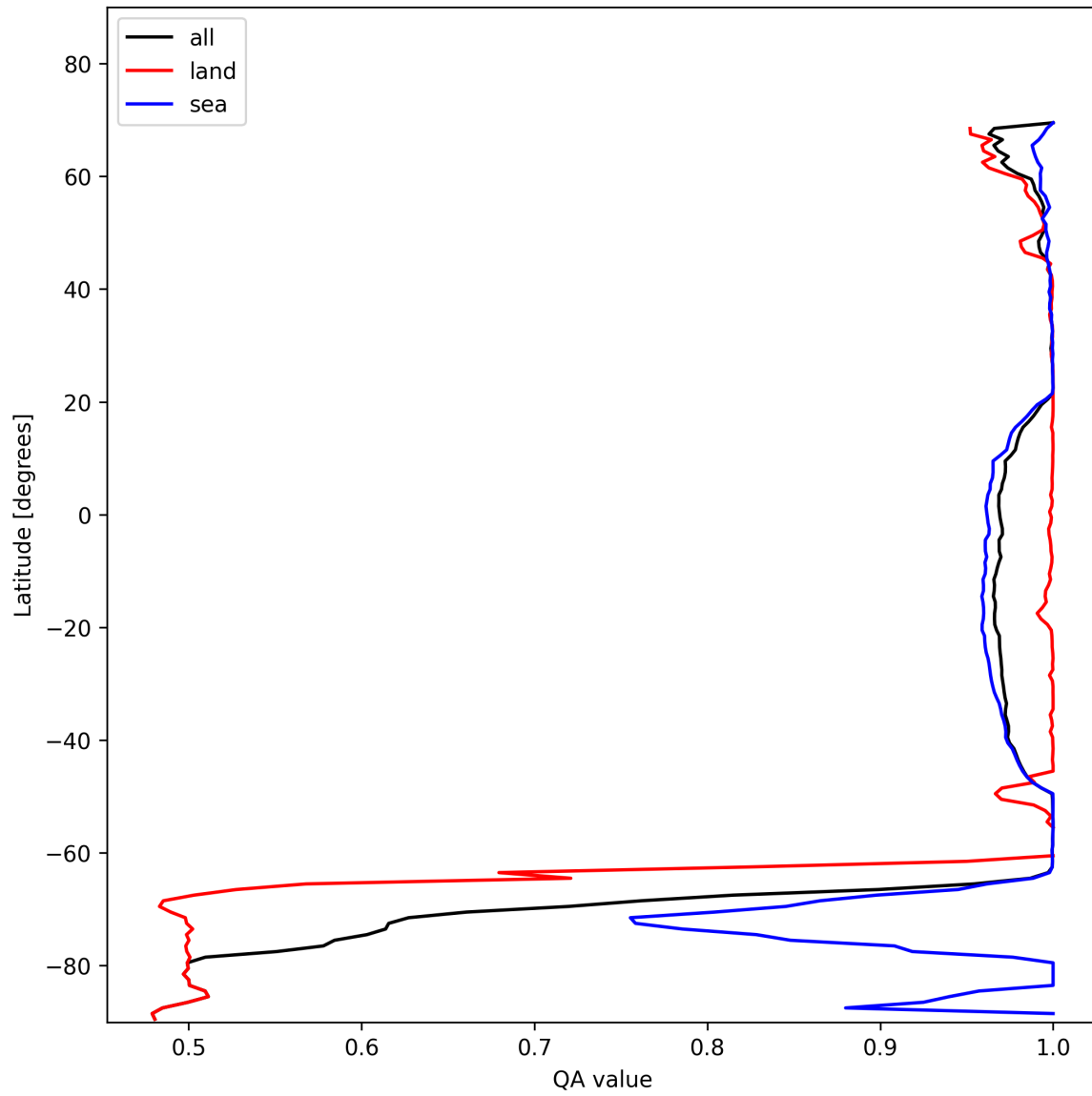
Figure 12: Zonal average of “QA value” for 2025-11-16 to 2025-11-18.
