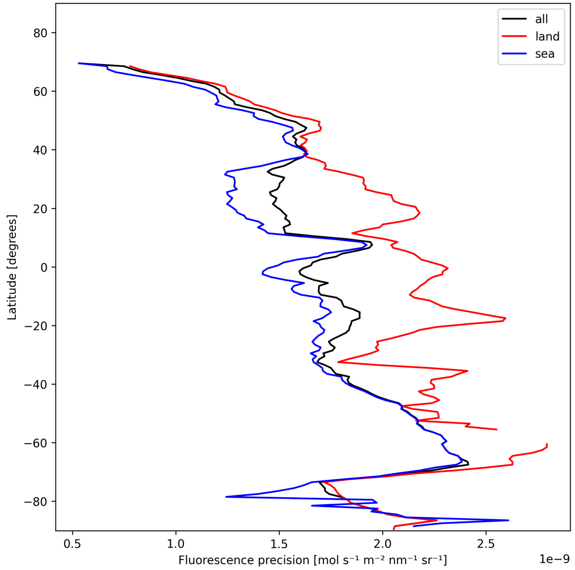
Figure 24: Zonal average of “Fluorescence precision” for 2025-11-16 to 2025-11-18.
