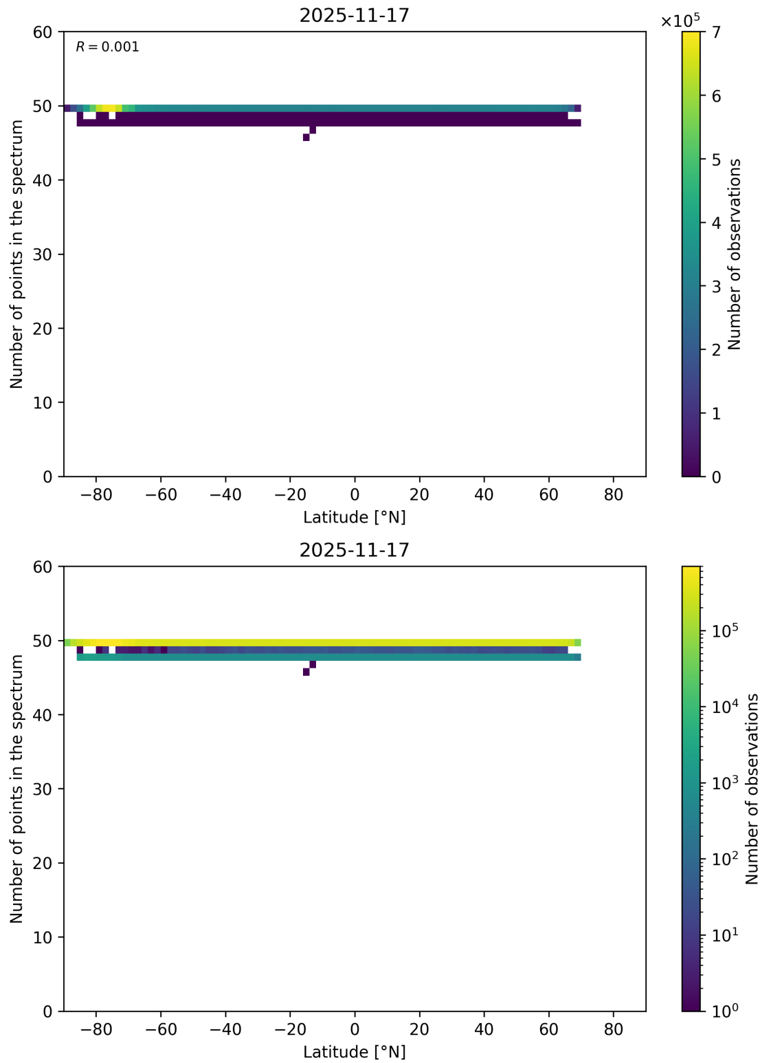
Figure 94: Scatter density plot of “Latitude” against “Number of points in the spectrum” for 2025-11-16 to 2025-11-18.
