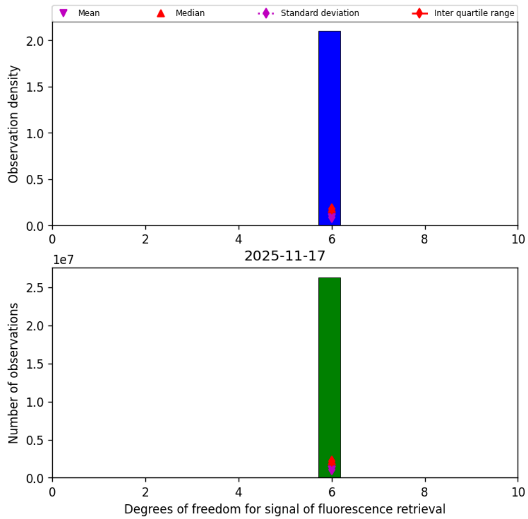
Figure 43: Histogram of “Degrees of freedom for signal of fluorescence retrieval” for 2025-11-16 to 2025-11-18
