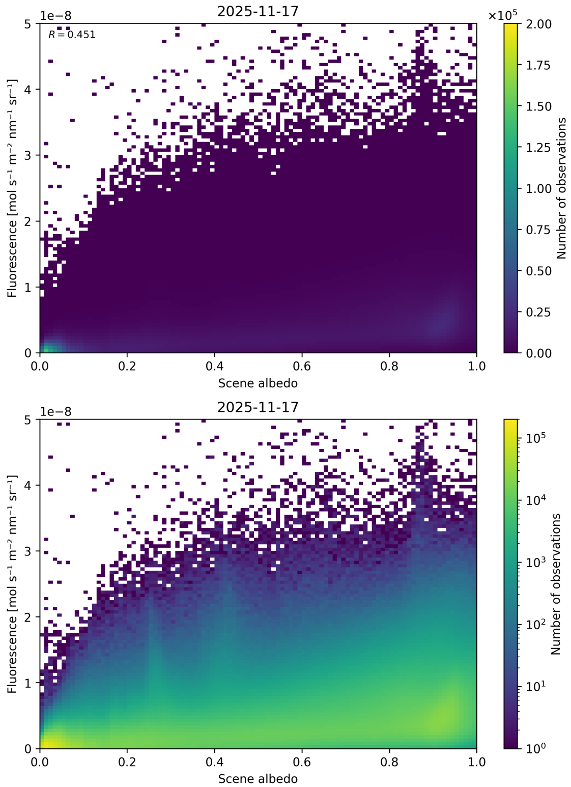
Figure 104: Scatter density plot of “Scene albedo” against “Fluorescence” for 2025-11-16 to 2025-11-18.
