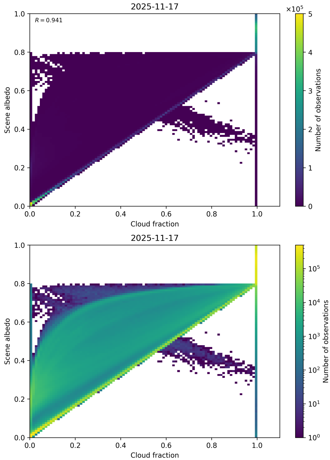
Figure 75: Scatter density plot of “Cloud fraction” against “Scene albedo” for 2025-11-16 to 2025-11-18.
