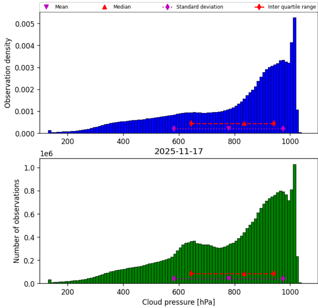
Figure 30: Histogram of “Cloud pressure” for 2025-11-16 to 2025-11-18
