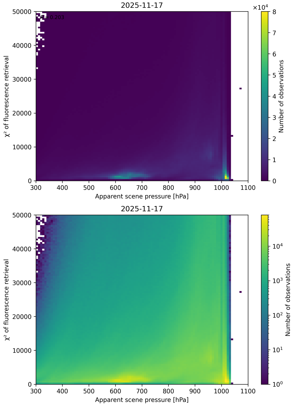
Figure 63: Scatter density plot of “Apparent scene pressure” against “ \chi^2 of fluorescence retrieval” for 2025-11-16 to 2025-11-18.
