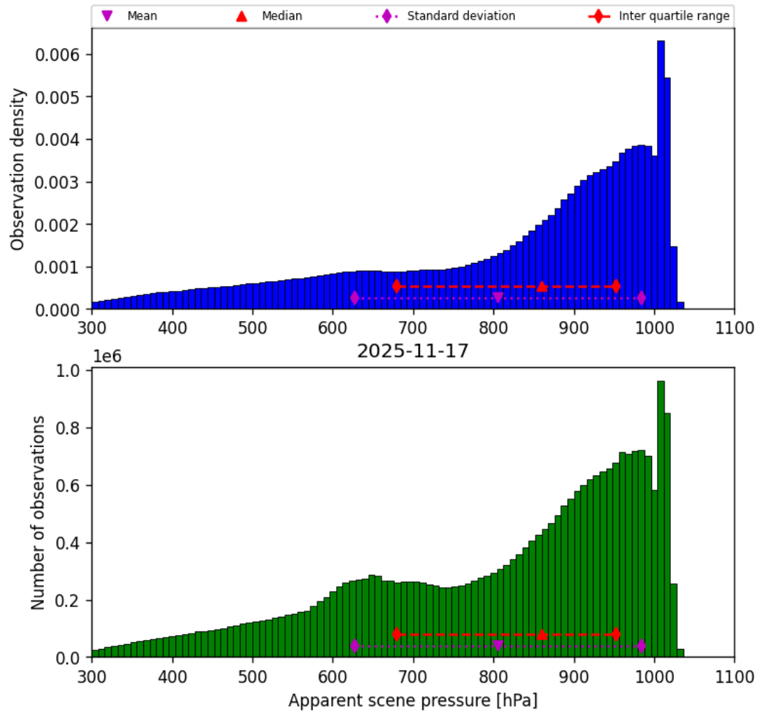
Figure 36: Histogram of “Apparent scene pressure” for 2025-11-16 to 2025-11-18
