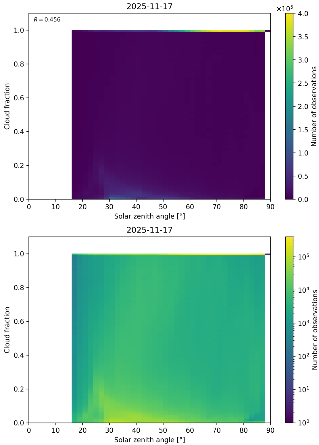
Figure 110: Scatter density plot of “Solar zenith angle” against “Cloud fraction” for 2025-11-16 to 2025-11-18.
