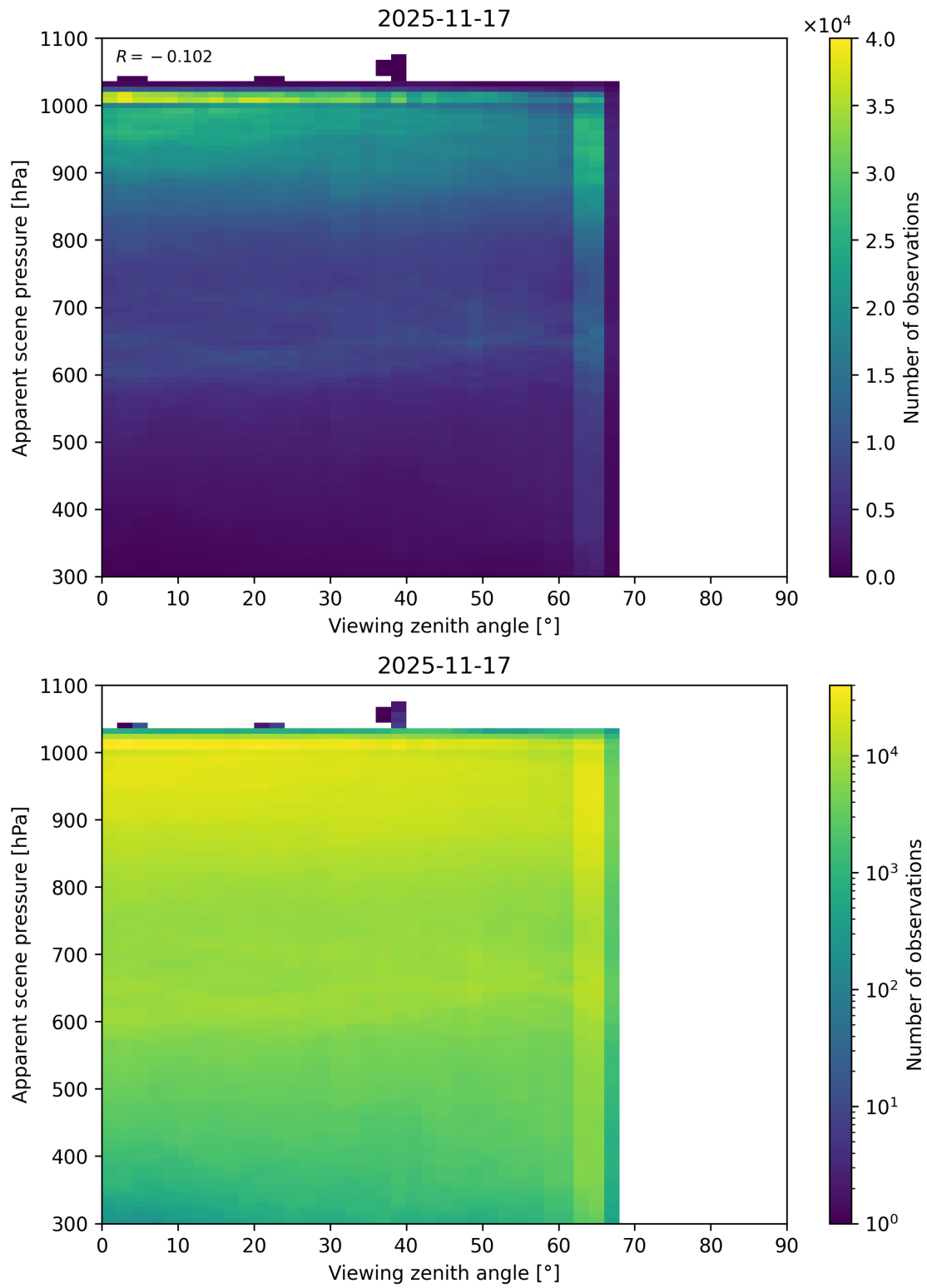
Figure 118: Scatter density plot of “Viewing zenith angle” against “Apparent scene pressure” for 2025-11-16 to 2025-11-18.
