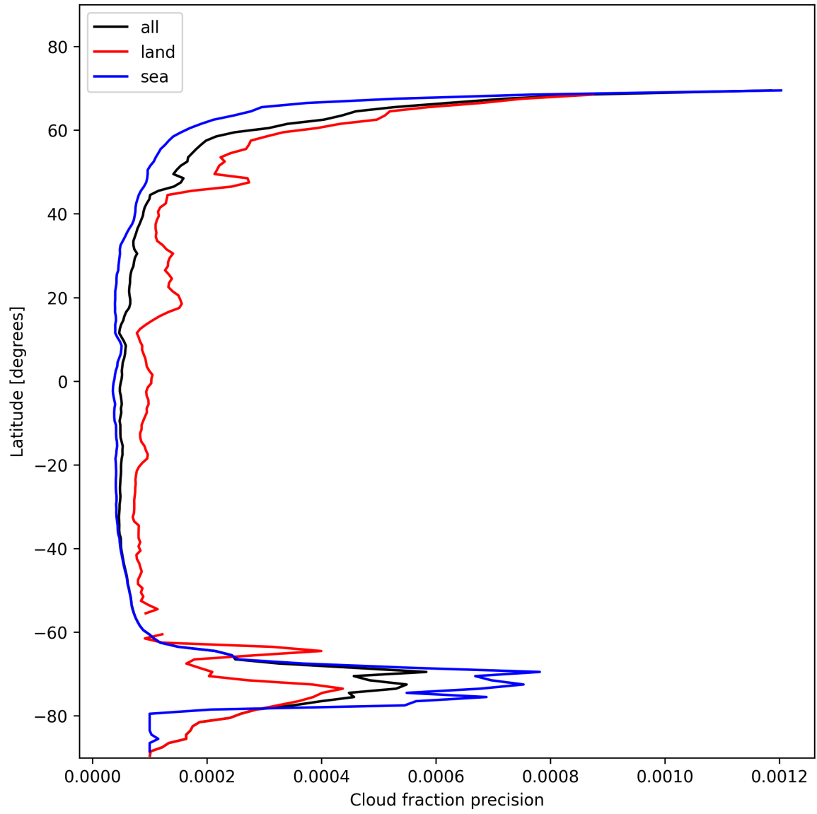
Figure 16: Zonal average of “Cloud fraction precision” for 2025-11-16 to 2025-11-18.
