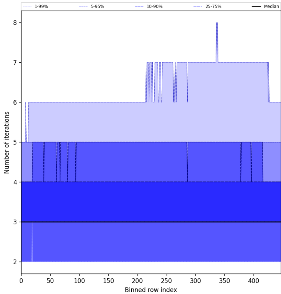
Figure 56: Along track statistics of “Number of iterations” for 2025-11-16 to 2025-11-18
