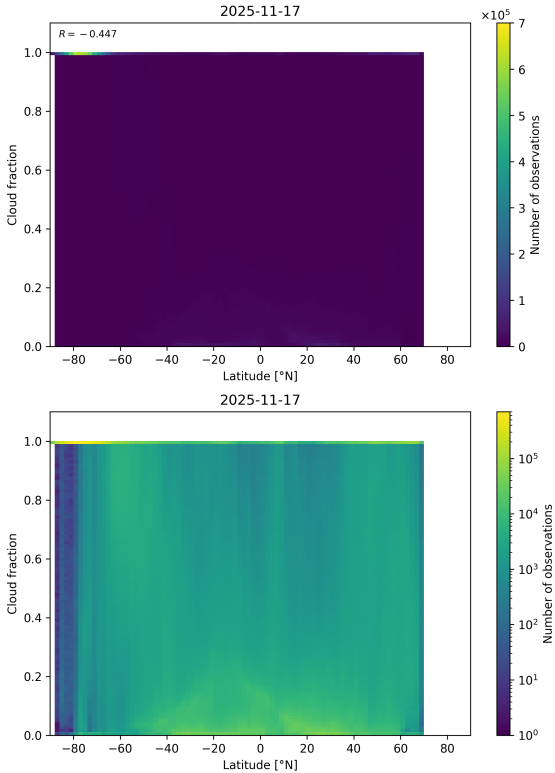
Figure 90: Scatter density plot of “Latitude” against “Cloud fraction” for 2025-11-16 to 2025-11-18.
