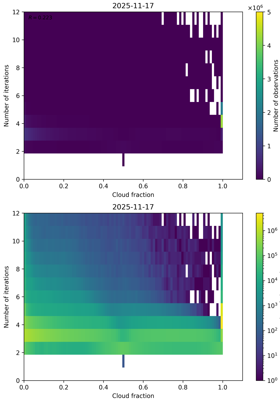
Figure 73: Scatter density plot of “Cloud fraction” against “Number of iterations” for 2025-11-16 to 2025-11-18.
