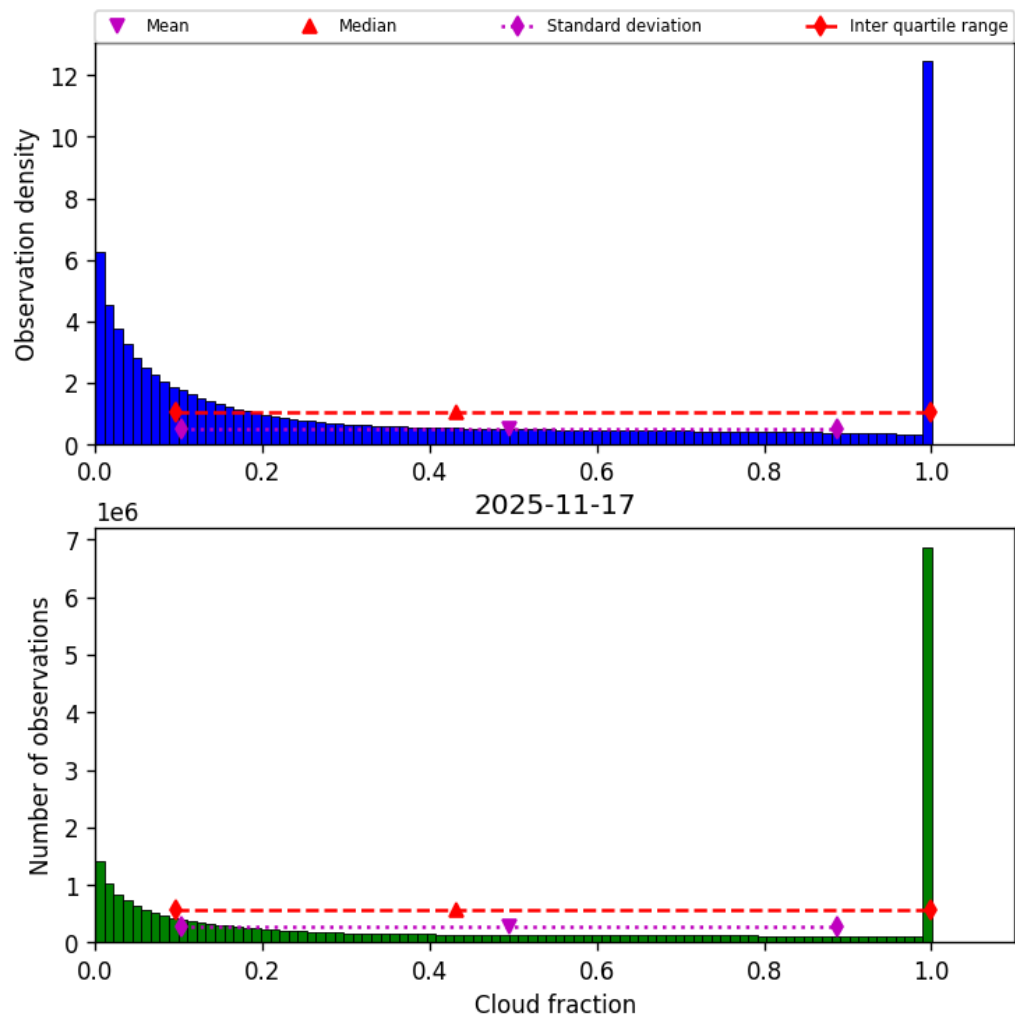
Figure 32: Histogram of “Cloud fraction” for 2025-11-16 to 2025-11-18
