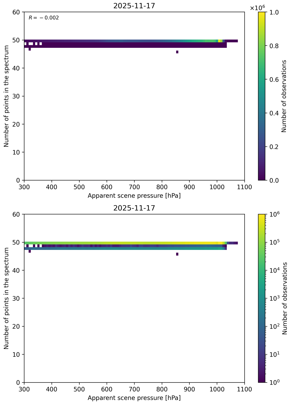
Figure 66: Scatter density plot of “Apparent scene pressure” against “Number of points in the spectrum” for 2025-11-16 to 2025-11-18.
