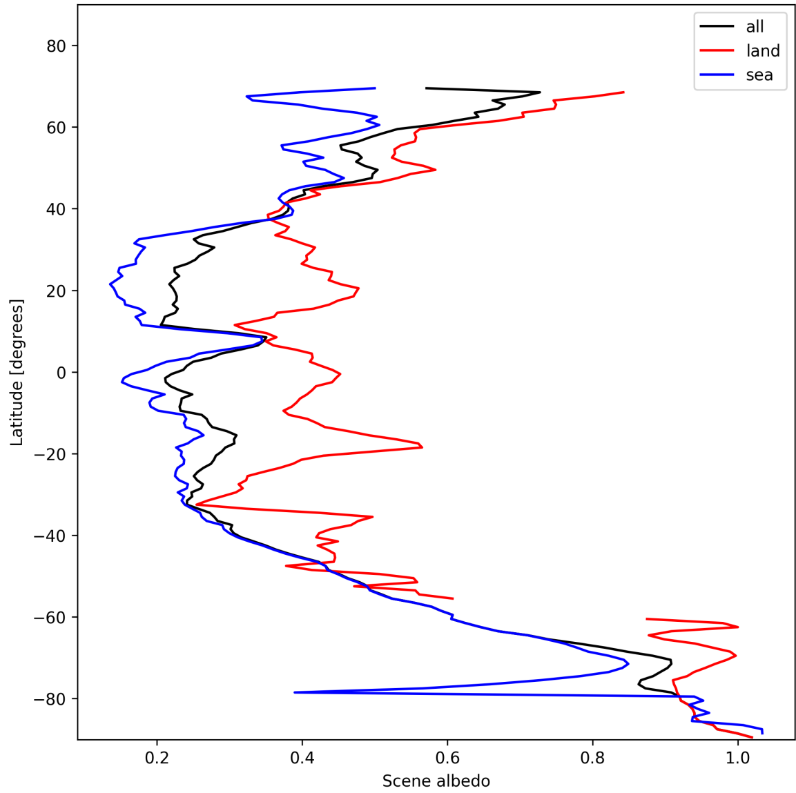
Figure 17: Zonal average of “Scene albedo” for 2025-11-16 to 2025-11-18.
