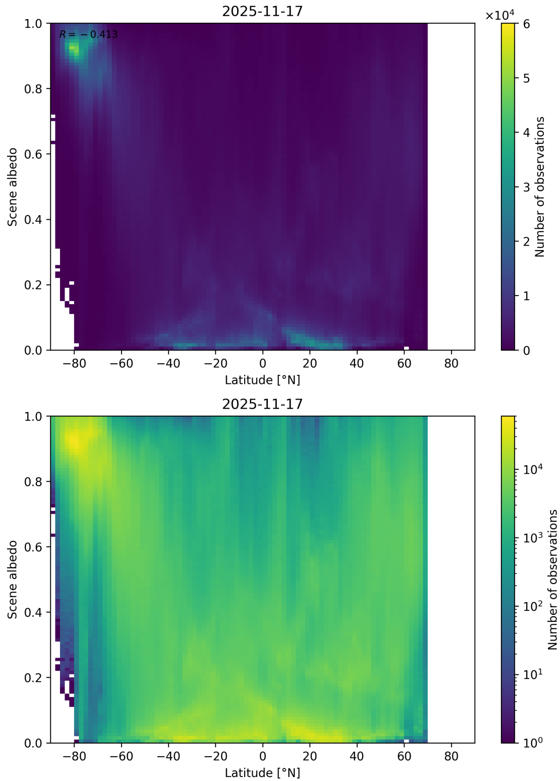
Figure 95: Scatter density plot of “Latitude” against “Scene albedo” for 2025-11-16 to 2025-11-18.
