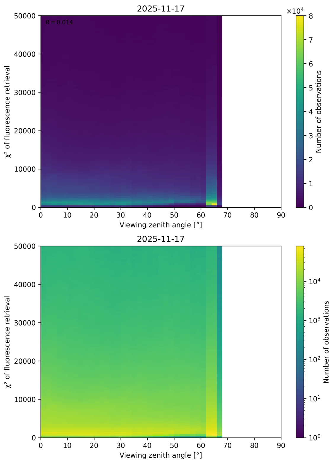
Figure 119: Scatter density plot of “Viewing zenith angle” against “ \chi^2 of fluorescence retrieval” for 2025-11-16 to 2025-11-18.
