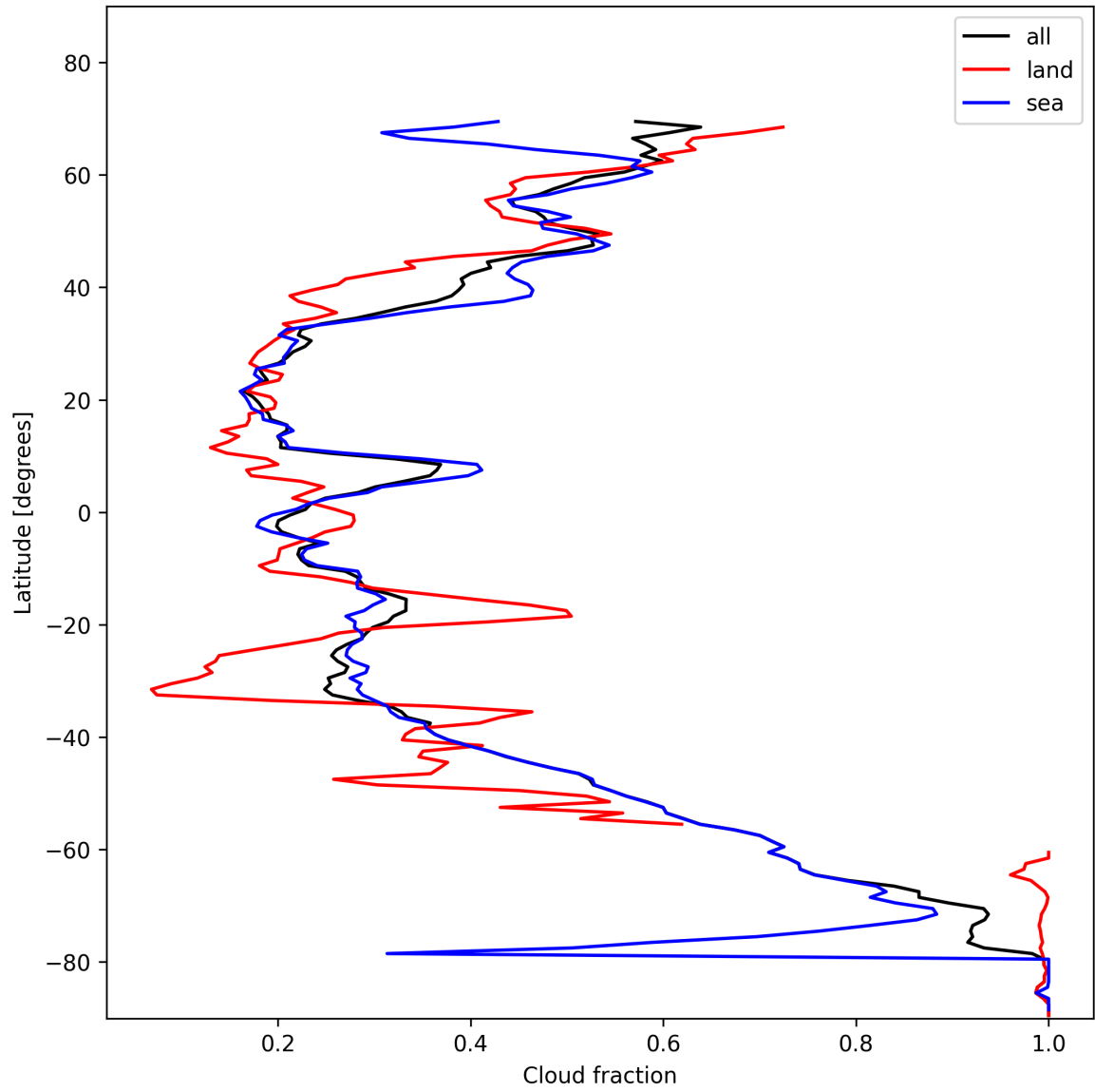
Figure 15: Zonal average of “Cloud fraction” for 2025-11-16 to 2025-11-18.
