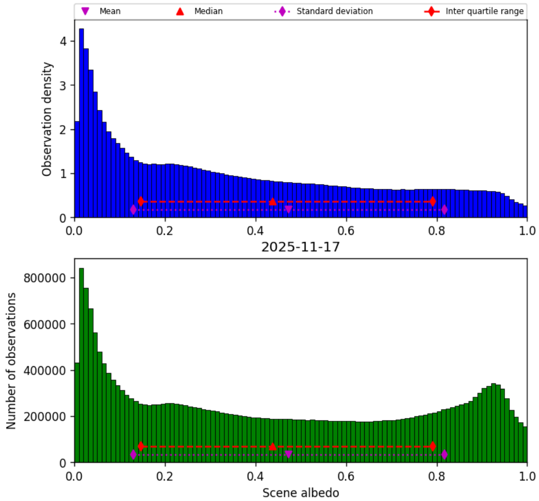
Figure 34: Histogram of “Scene albedo” for 2025-11-16 to 2025-11-18
