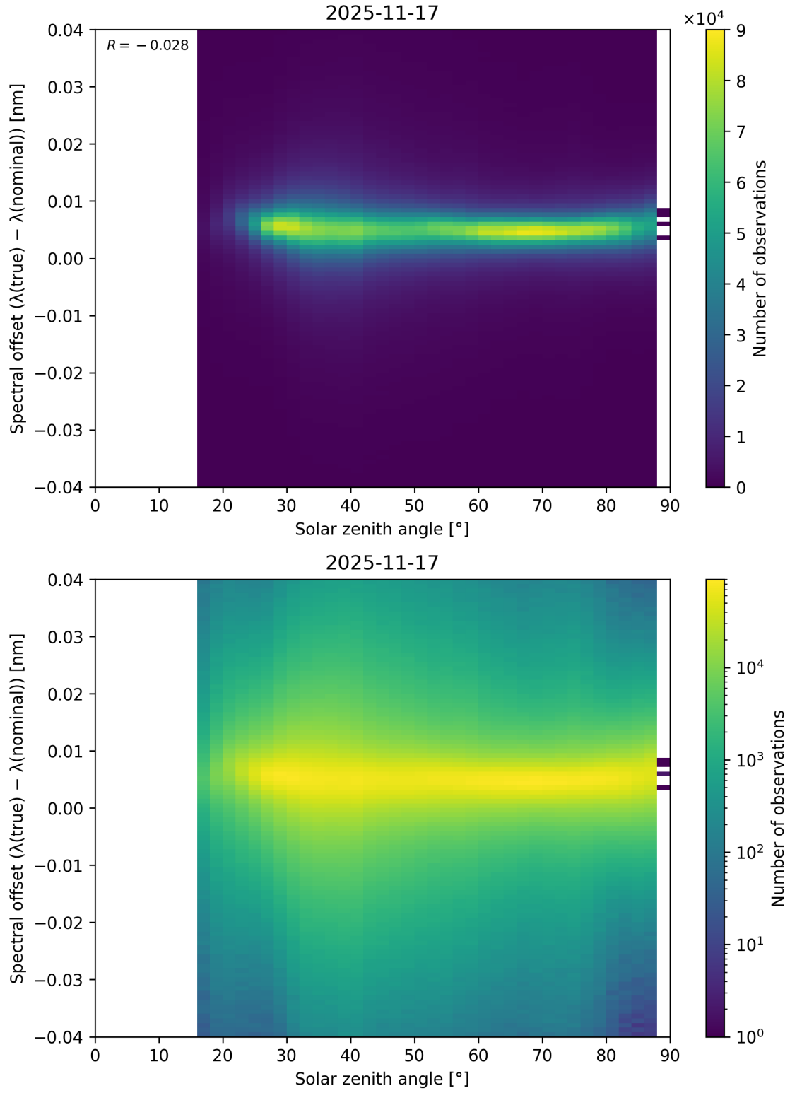
Figure 117: Scatter density plot of “Solar zenith angle” against “Spectral offset ( \lambda_{\text{true}} - \lambda_{\text{nominal}} )” for 2025-11-16 to 2025-11-18.
