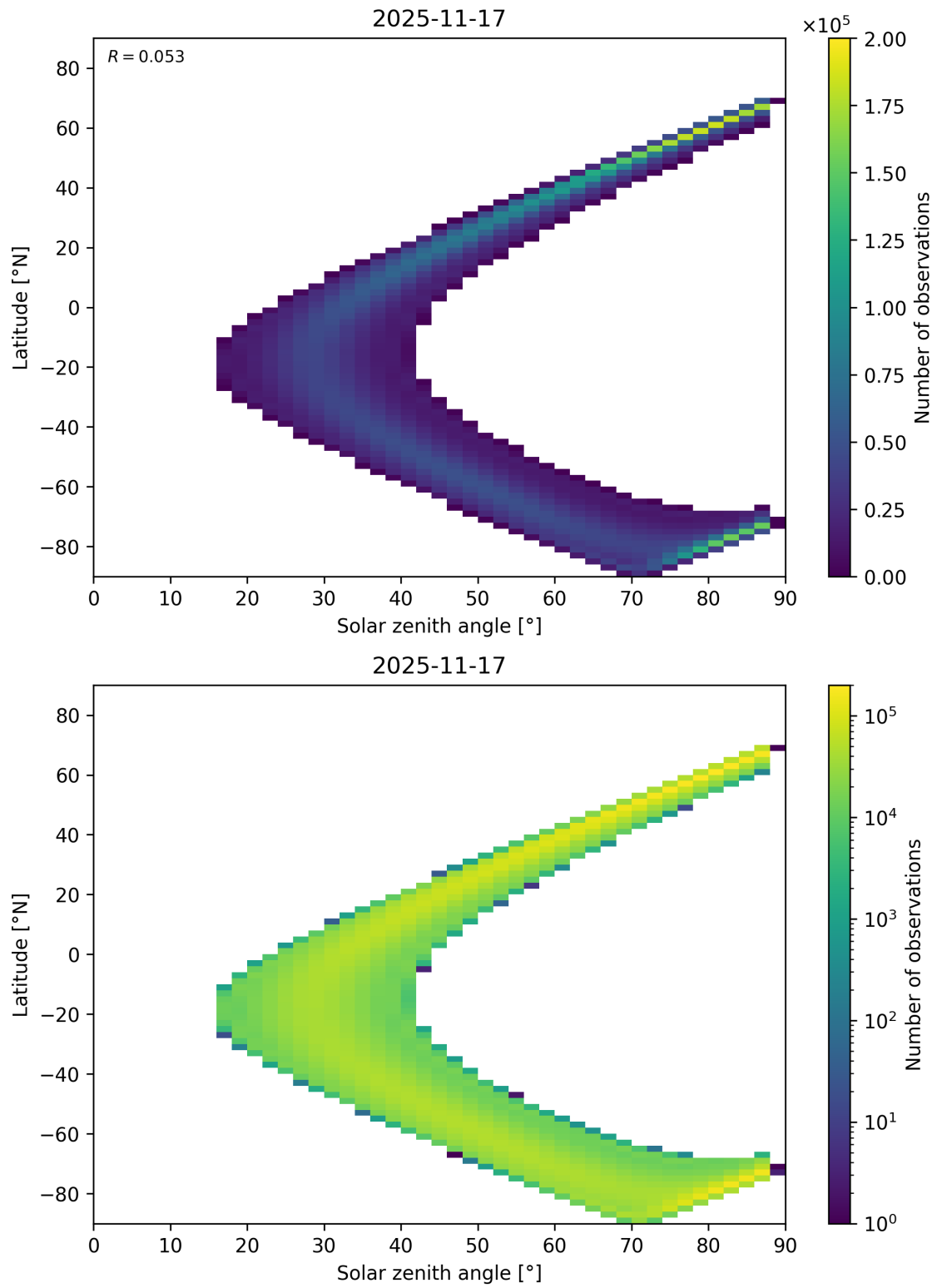
Figure 113: Scatter density plot of “Solar zenith angle” against “Latitude” for 2025-11-16 to 2025-11-18.
