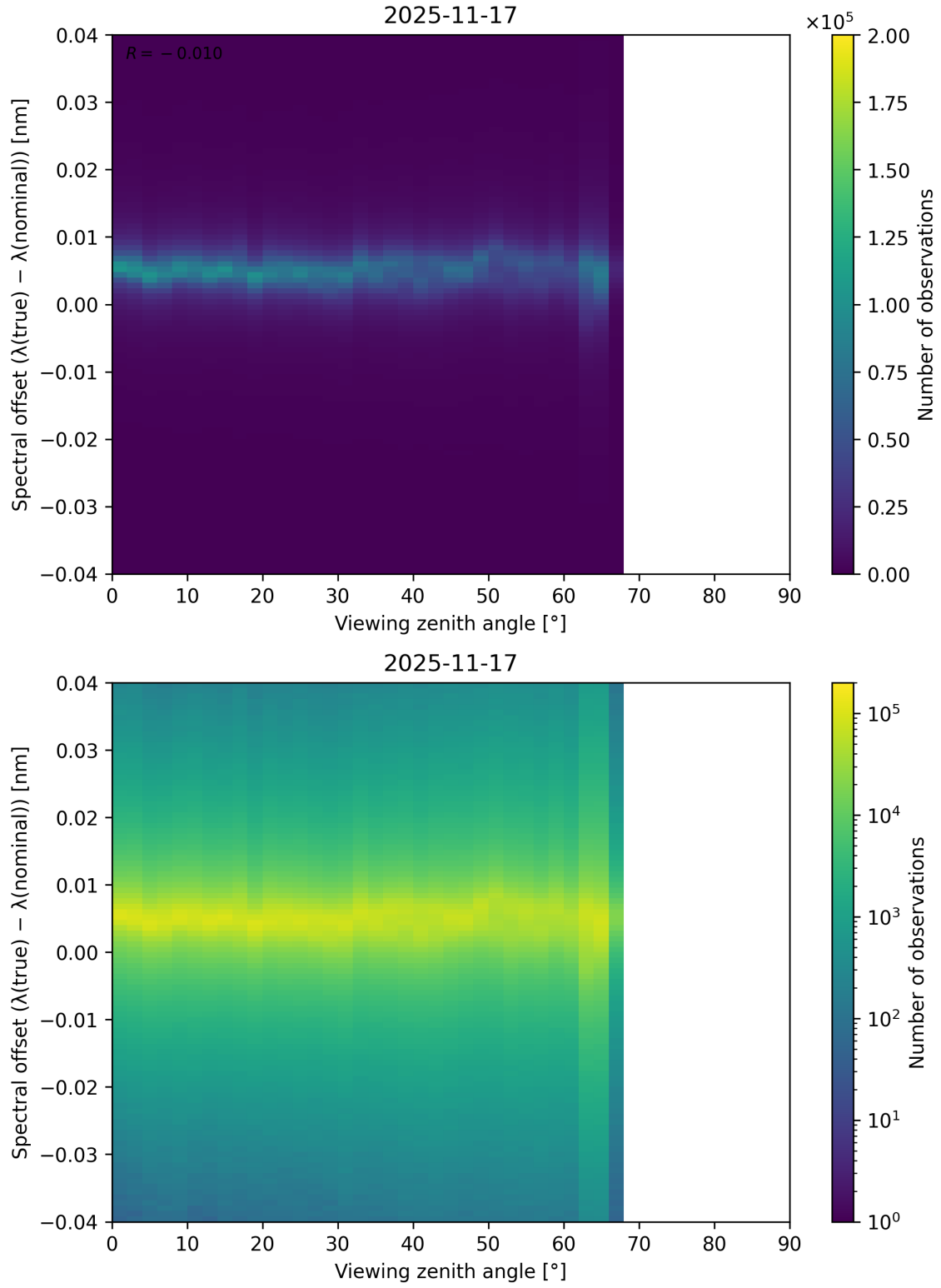
Figure 128: Scatter density plot of “Viewing zenith angle” against “Spectral offset ( \lambda_{\text{true}} - \lambda_{\text{nominal}} )” for 2025-11-16 to 2025-11-18.
