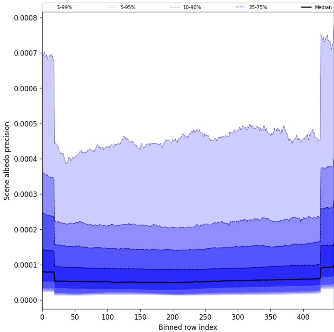
Figure 52: Along track statistics of “Scene albedo precision” for 2025-11-16 to 2025-11-18
