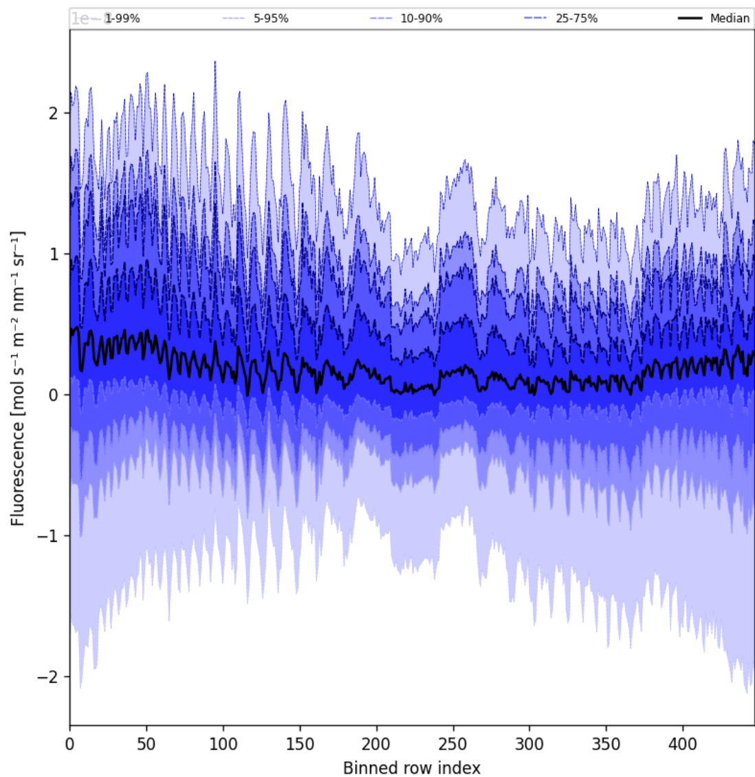
Figure 57: Along track statistics of “Fluorescence” for 2025-11-16 to 2025-11-18
