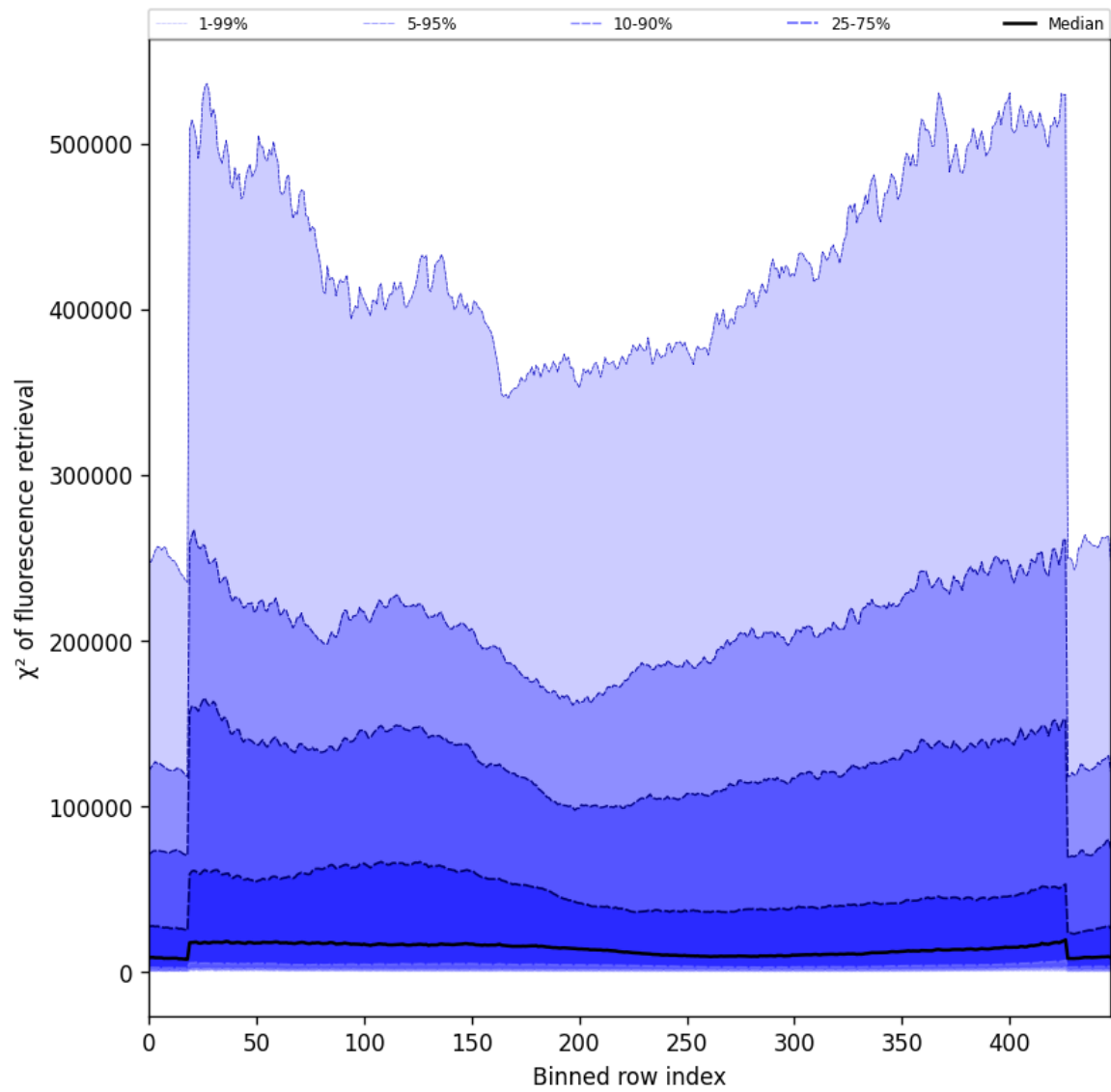
Figure 59: Along track statistics of “ \chi^2 of fluorescence retrieval” for 2025-11-16 to 2025-11-18
