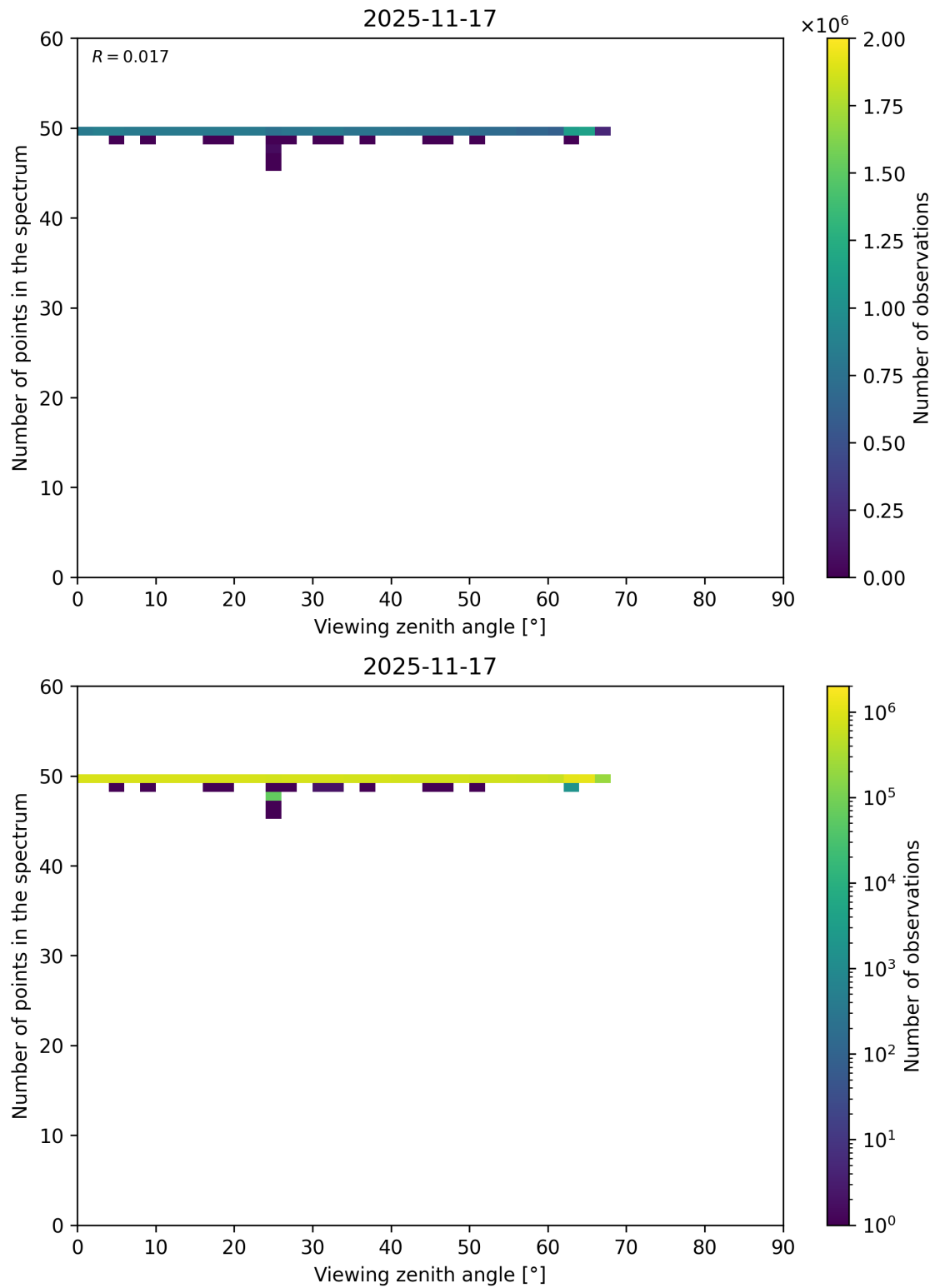
Figure 125: Scatter density plot of “Viewing zenith angle” against “Number of points in the spectrum” for 2025-11-16 to 2025-11-18.
