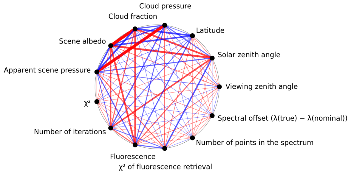
Figure 1: Map of correlation graph for 2025-11-16 to 2025-11-18.
