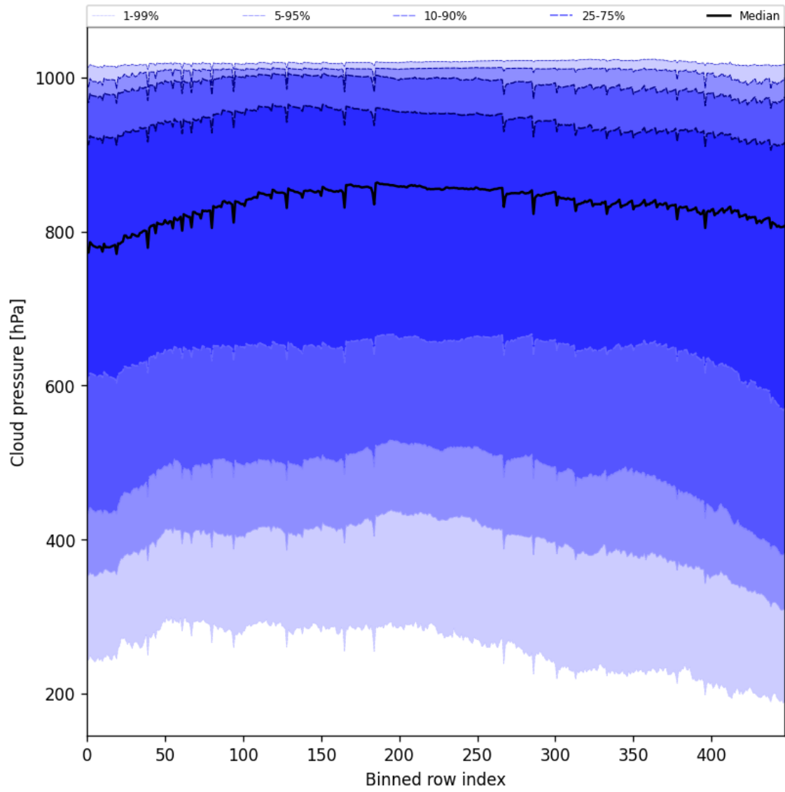
Figure 47: Along track statistics of “Cloud pressure” for 2025-11-16 to 2025-11-18
