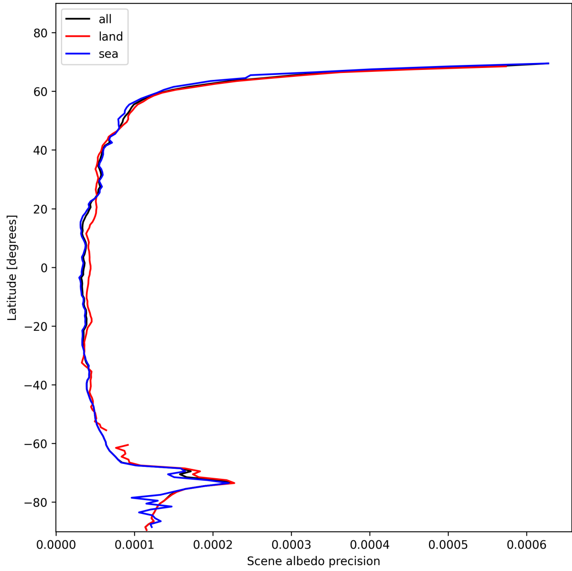
Figure 18: Zonal average of “Scene albedo precision” for 2025-11-16 to 2025-11-18.
