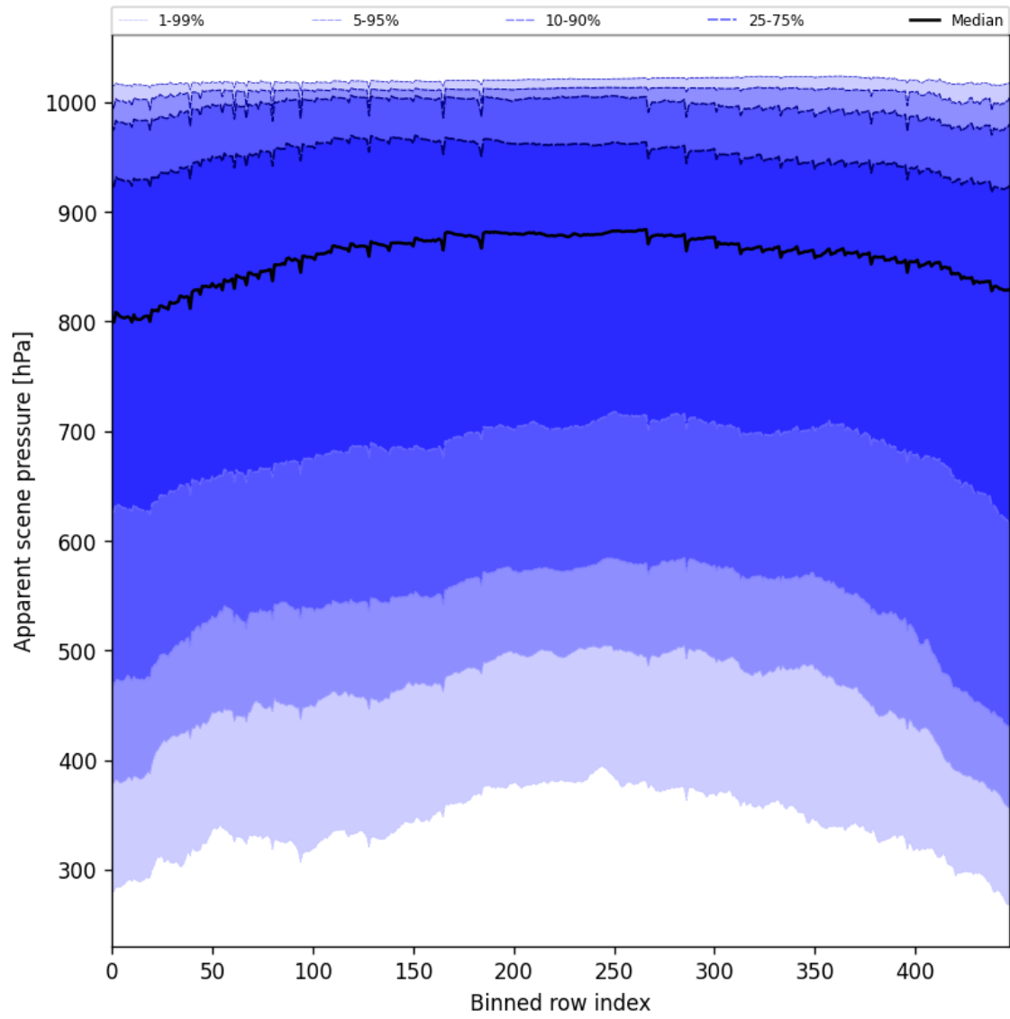
Figure 53: Along track statistics of “Apparent scene pressure” for 2025-11-16 to 2025-11-18
