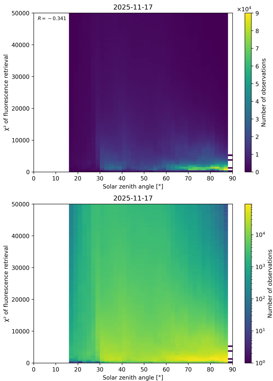
Figure 109: Scatter density plot of “Solar zenith angle” against “ \chi^2 of fluorescence retrieval” for 2025-11-16 to 2025-11-18.
