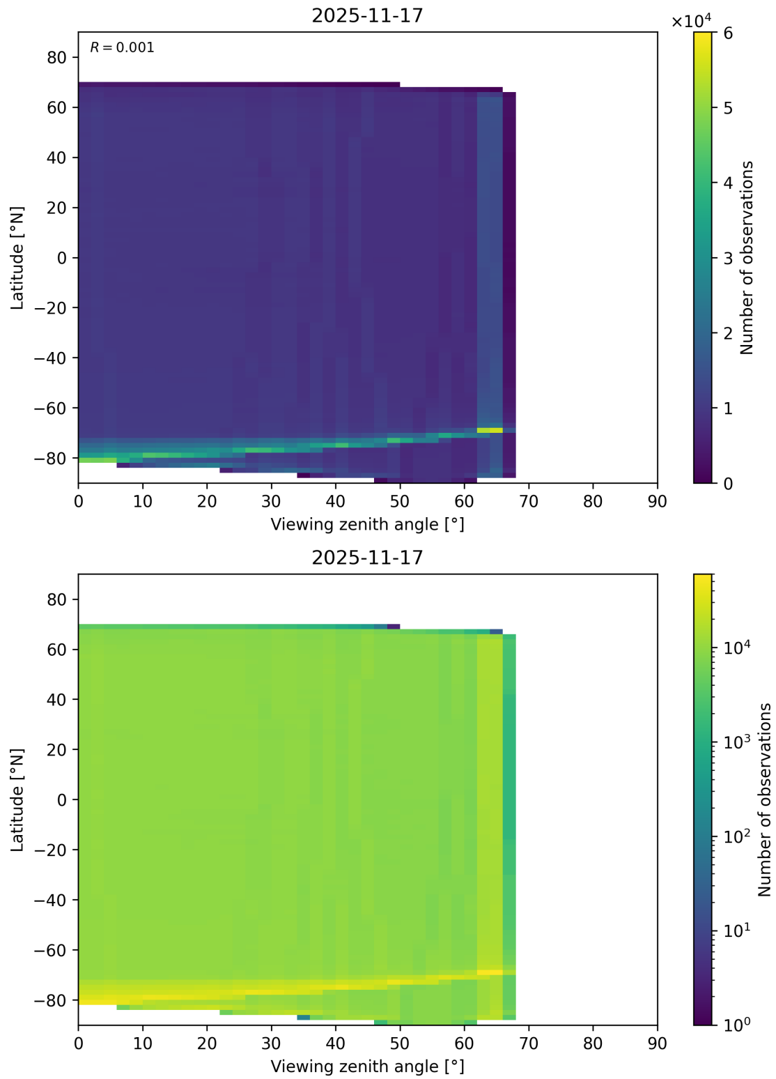
Figure 123: Scatter density plot of “Viewing zenith angle” against “Latitude” for 2025-11-16 to 2025-11-18.
