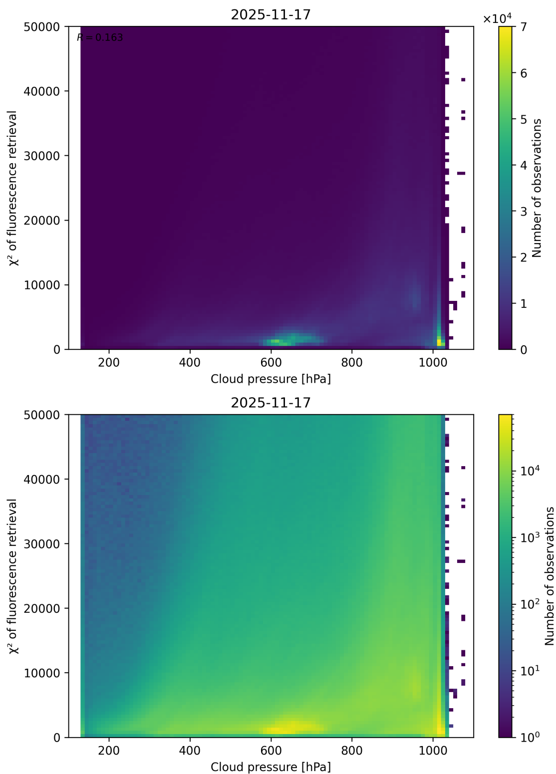
Figure 78: Scatter density plot of “Cloud pressure” against “ \chi^2 of fluorescence retrieval” for 2025-11-16 to 2025-11-18.
