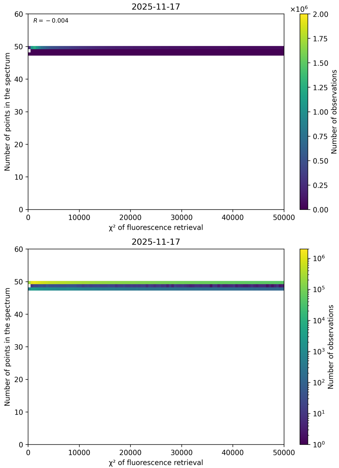
Figure 68: Scatter density plot of " \chi^2 of fluorescence retrieval" against "Number of points in the spectrum" for 2025-11-16 to 2025-11-18.
