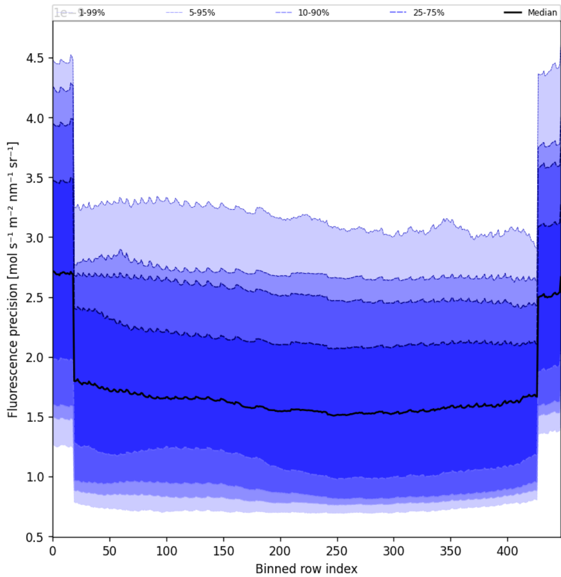
Figure 58: Along track statistics of “Fluorescence precision” for 2025-11-16 to 2025-11-18
