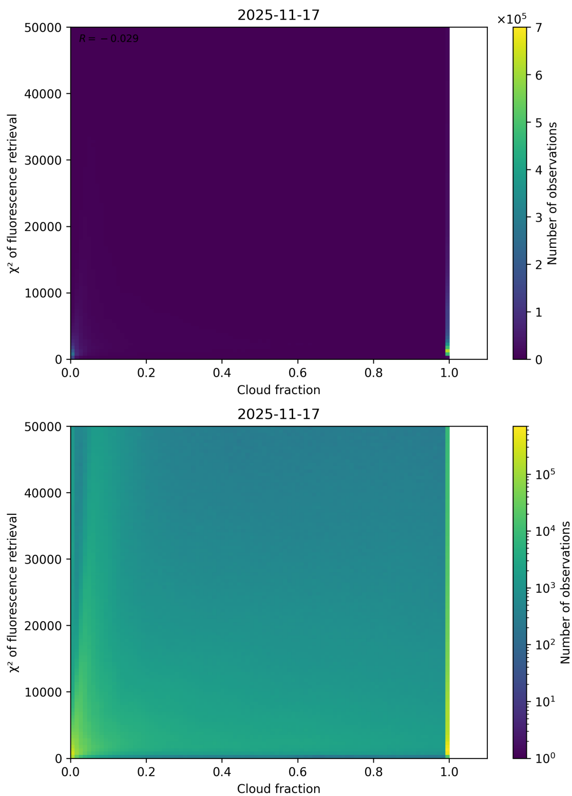
Figure 71: Scatter density plot of “Cloud fraction” against “ \chi^2 of fluorescence retrieval” for 2025-11-16 to 2025-11-18.
