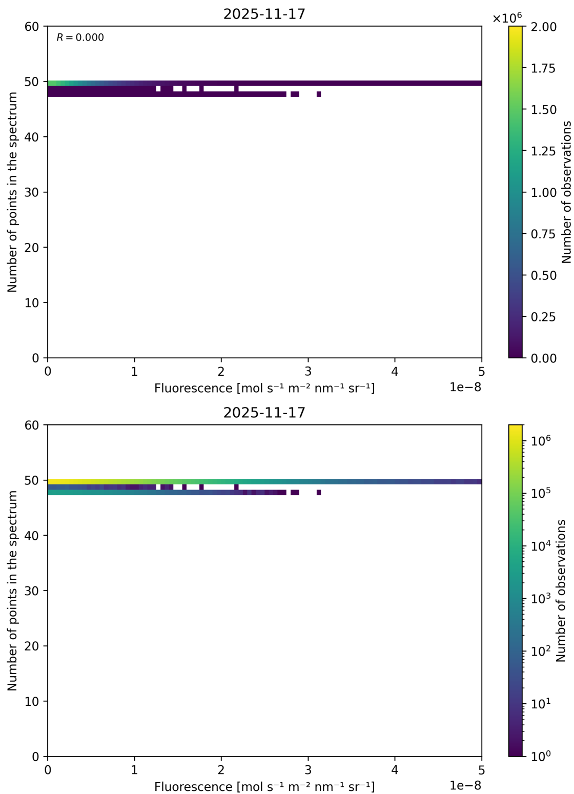
Figure 86: Scatter density plot of “Fluorescence” against “Number of points in the spectrum” for 2025-11-16 to 2025-11-18.
