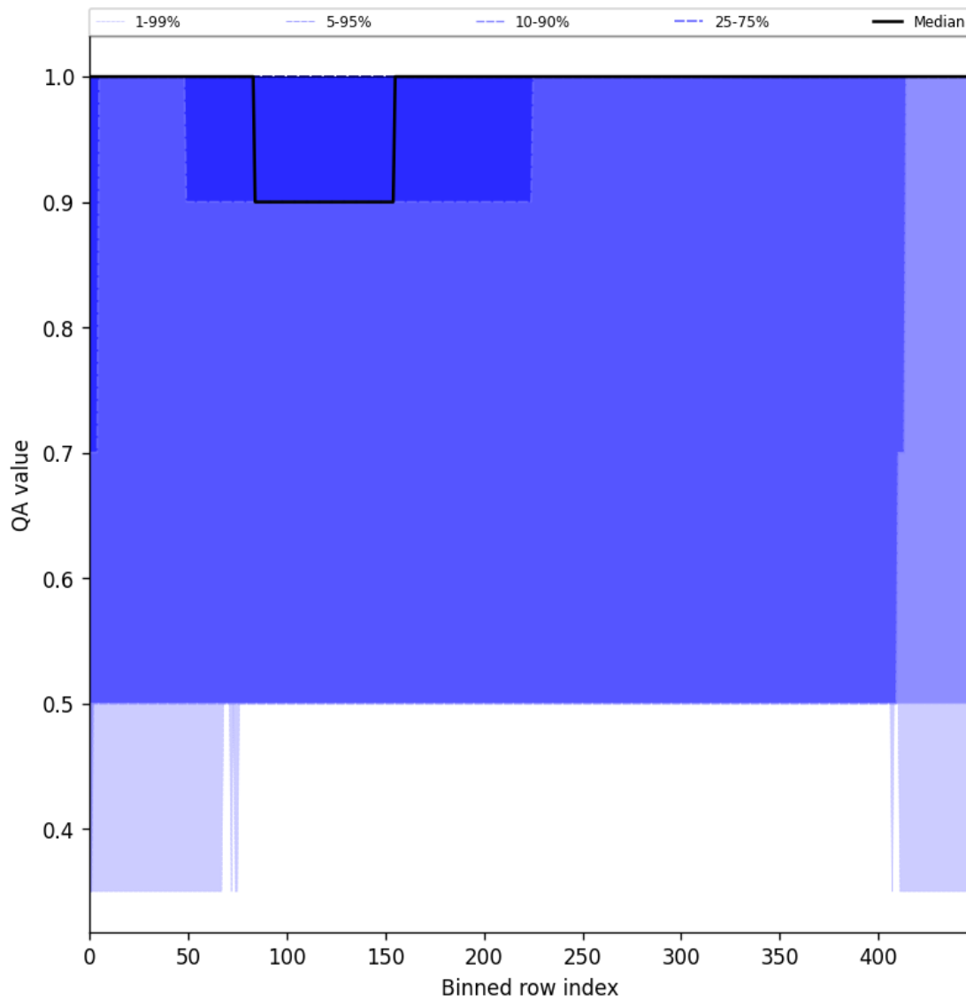
Figure 46: Along track statistics of “QA value” for 2025-11-16 to 2025-11-18
