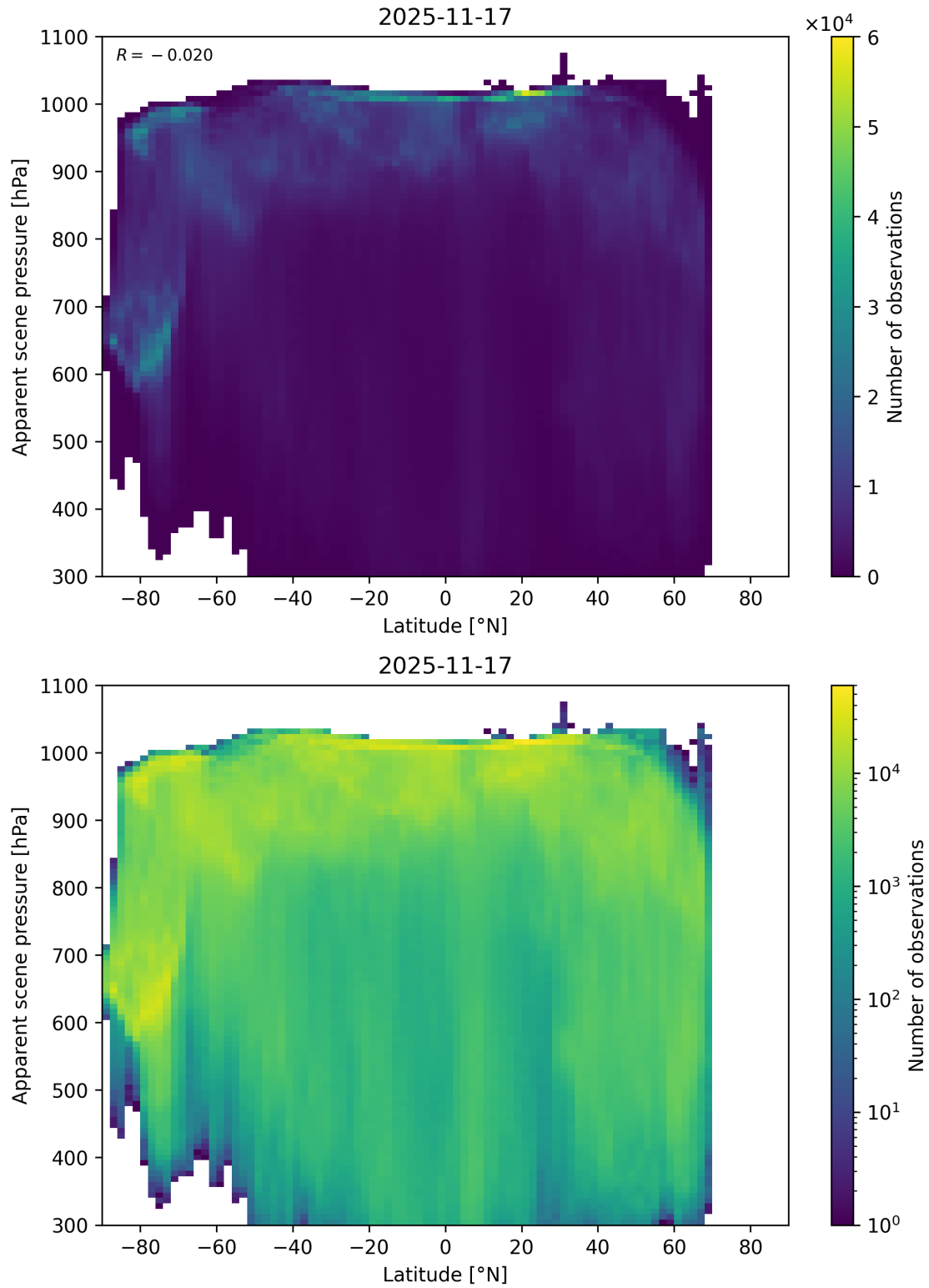
Figure 88: Scatter density plot of “Latitude” against “Apparent scene pressure” for 2025-11-16 to 2025-11-18.
