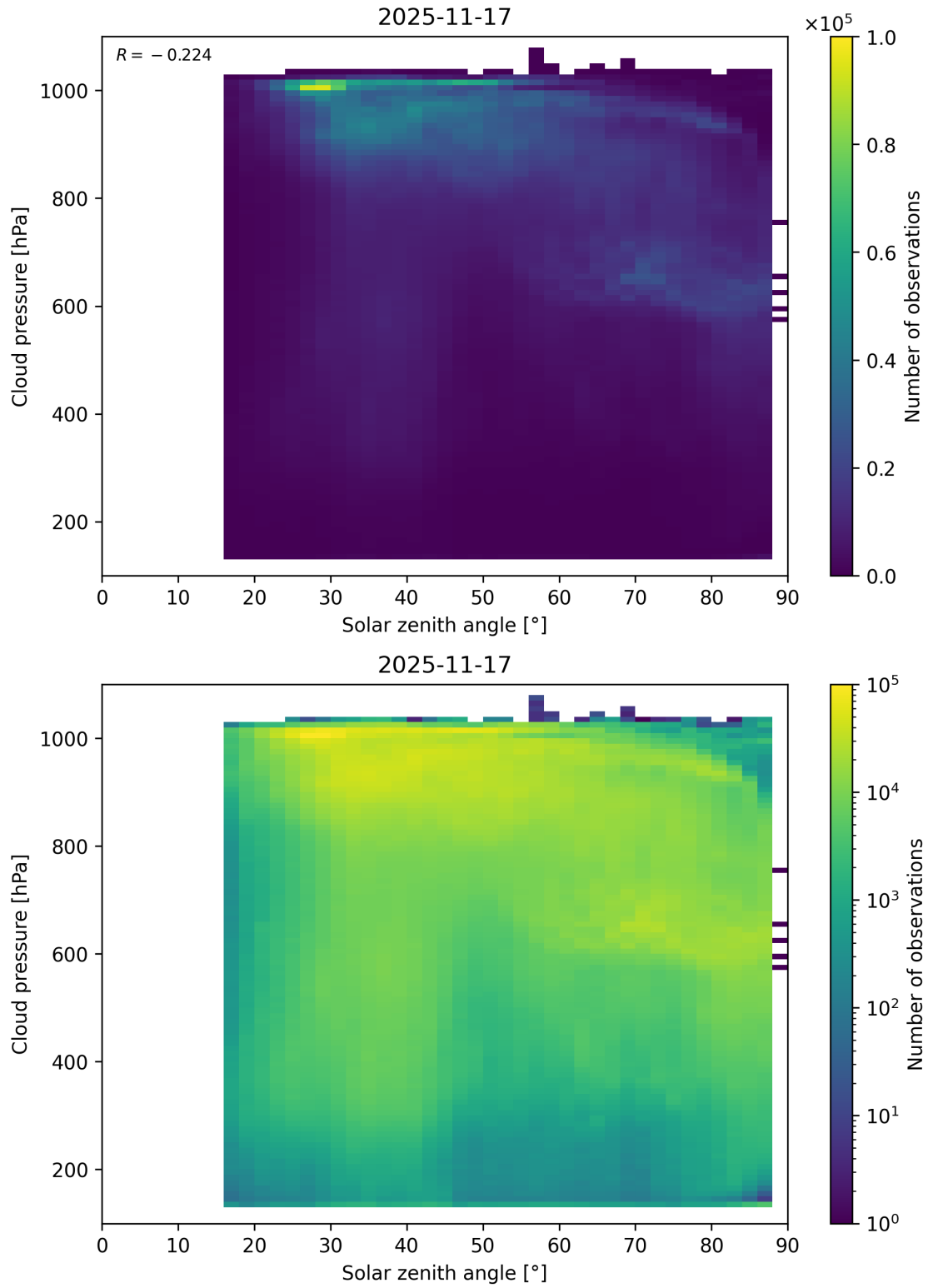
Figure 111: Scatter density plot of “Solar zenith angle” against “Cloud pressure” for 2025-11-16 to 2025-11-18.
