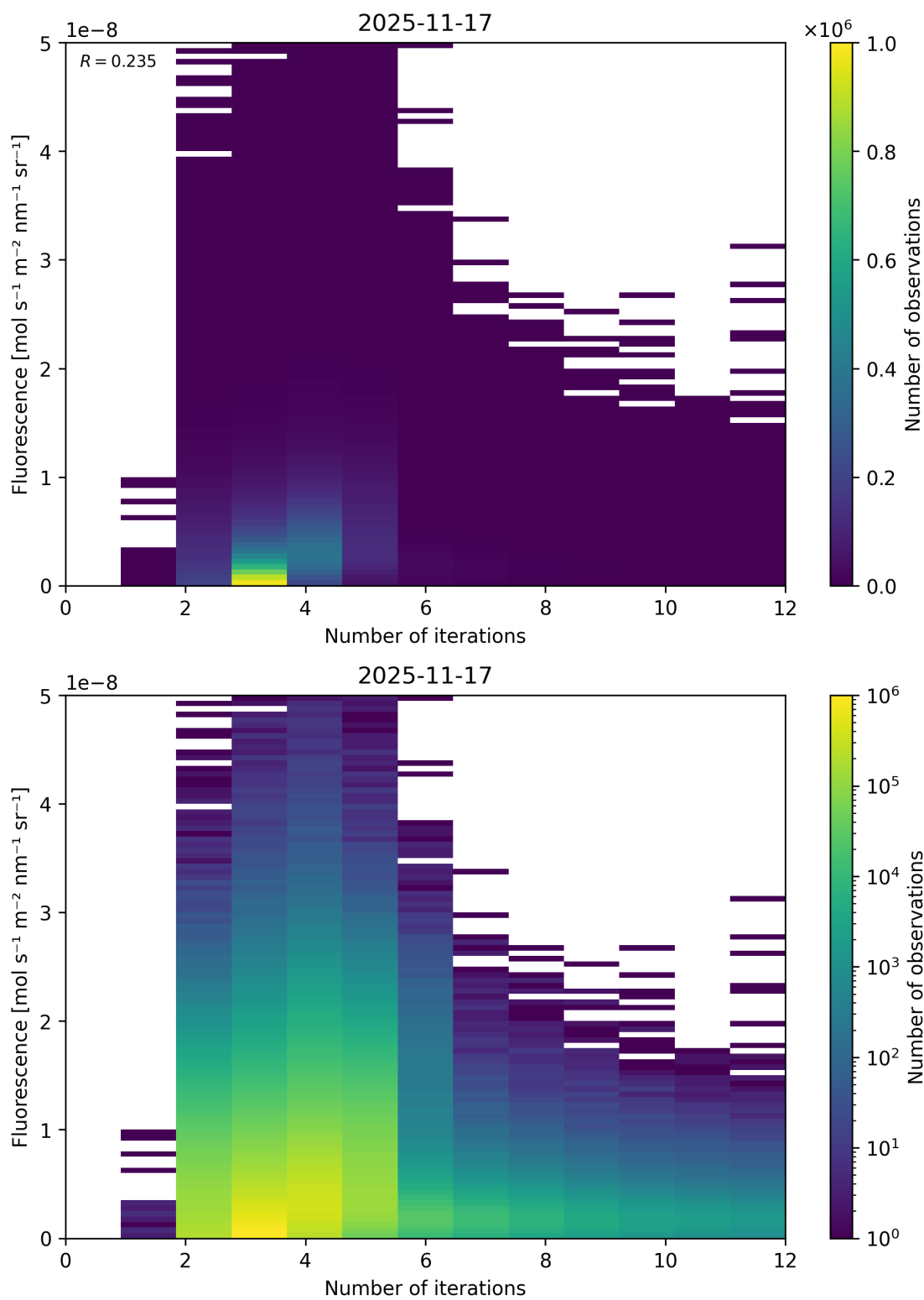
Figure 98: Scatter density plot of “Number of iterations” against “Fluorescence” for 2025-11-16 to 2025-11-18.
