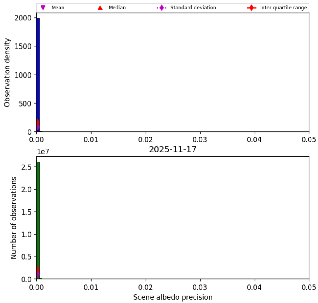
Figure 35: Histogram of “Scene albedo precision” for 2025-11-16 to 2025-11-18
