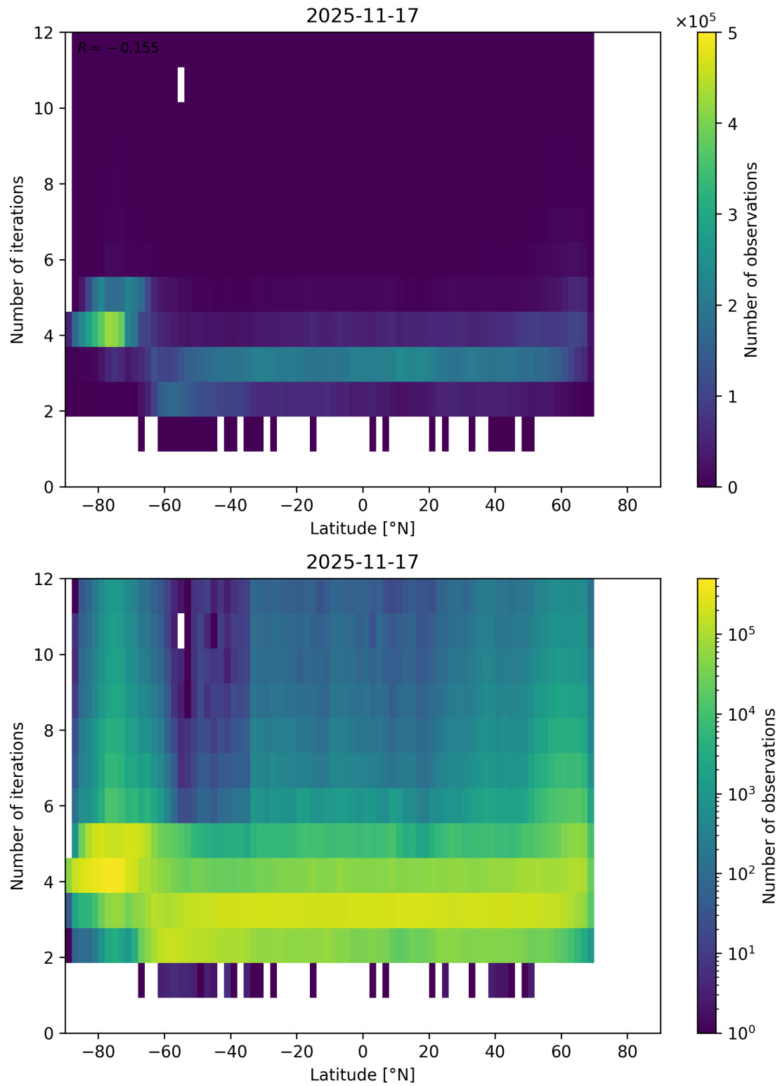
Figure 93: Scatter density plot of “Latitude” against “Number of iterations” for 2025-11-16 to 2025-11-18.
