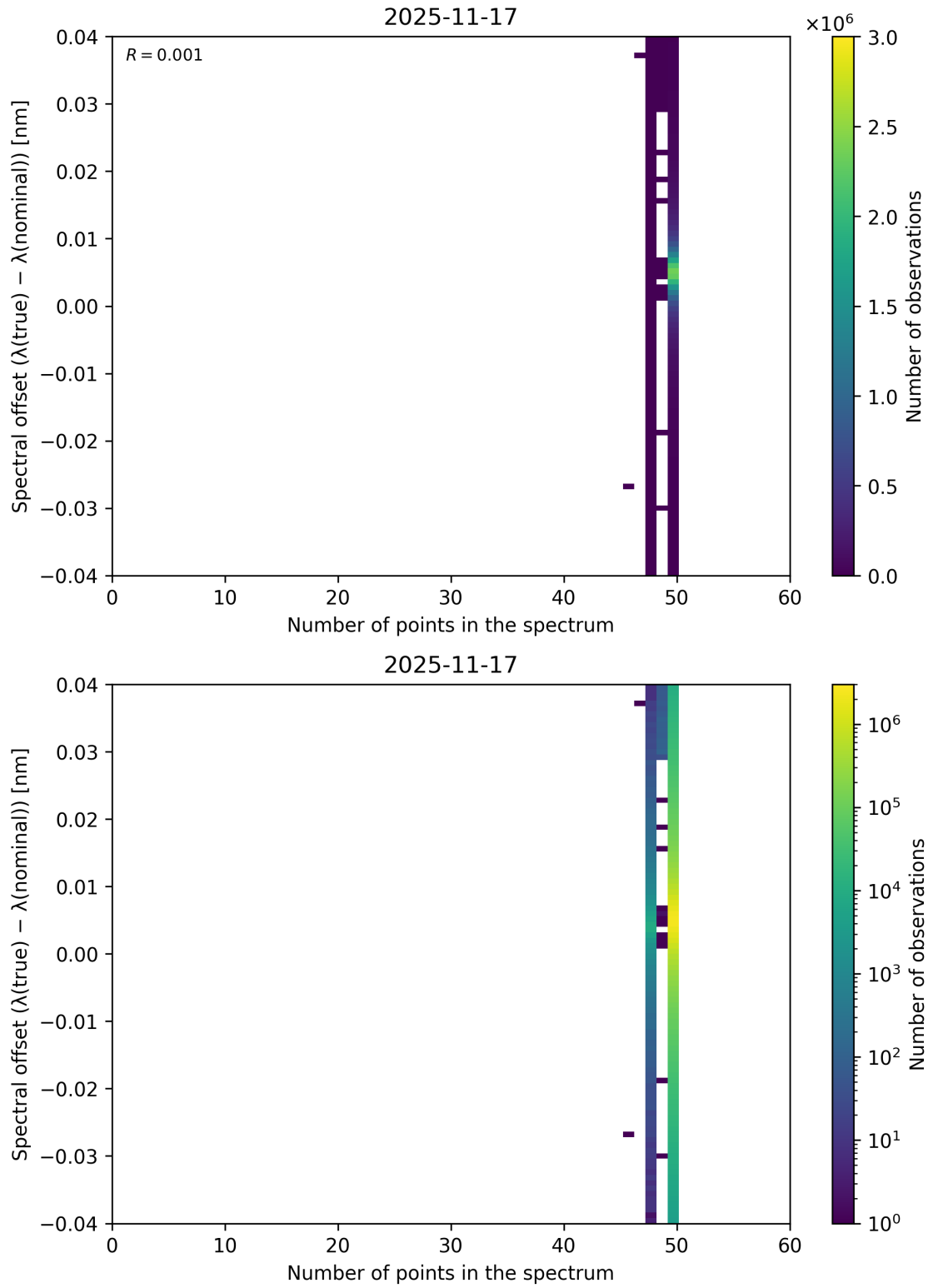
Figure 101: Scatter density plot of “Number of points in the spectrum” against “Spectral offset ( \lambda_{\text{true}} - \lambda_{\text{nominal}} )” for 2025-11-16 to 2025-11-18.
