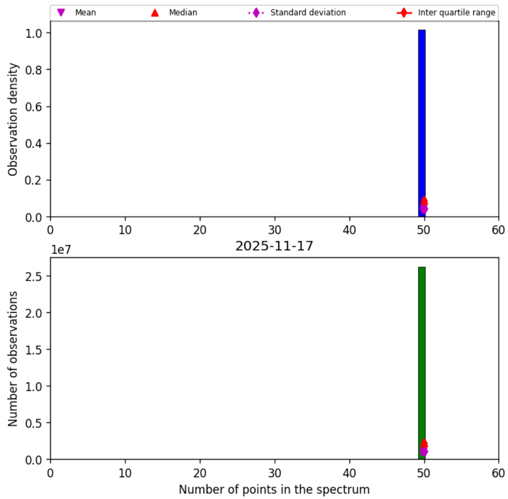
Figure 44: Histogram of "Number of points in the spectrum" for 2025-11-16 to 2025-11-18
