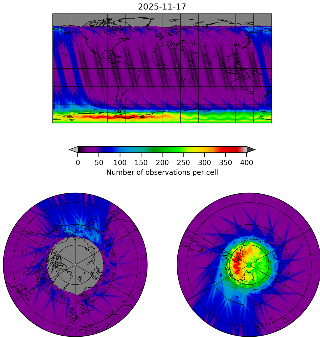
Figure 11: Map of the number of observations for 2025-11-16 to 2025-11-18
