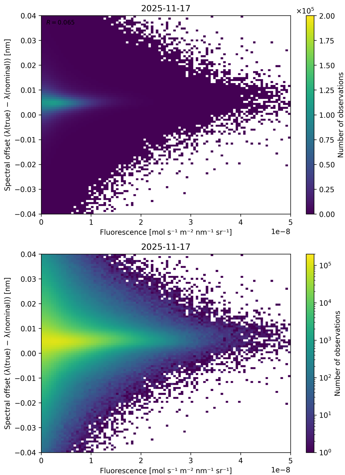
Figure 87: Scatter density plot of “Fluorescence” against “Spectral offset ( \lambda_{\text{true}} - \lambda_{\text{nominal}} )” for 2025-11-16 to 2025-11-18.
