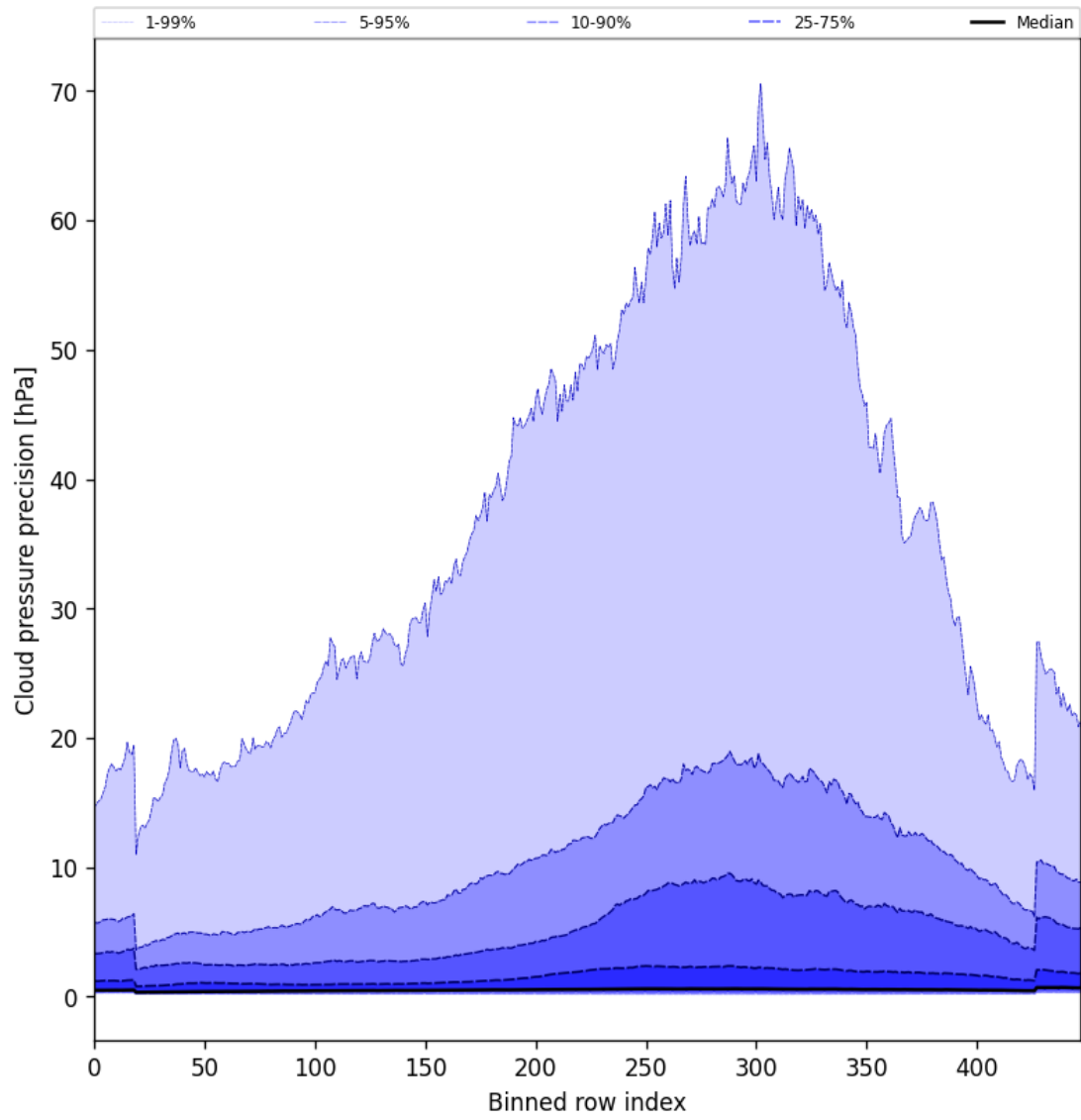
Figure 48: Along track statistics of “Cloud pressure precision” for 2025-11-16 to 2025-11-18
