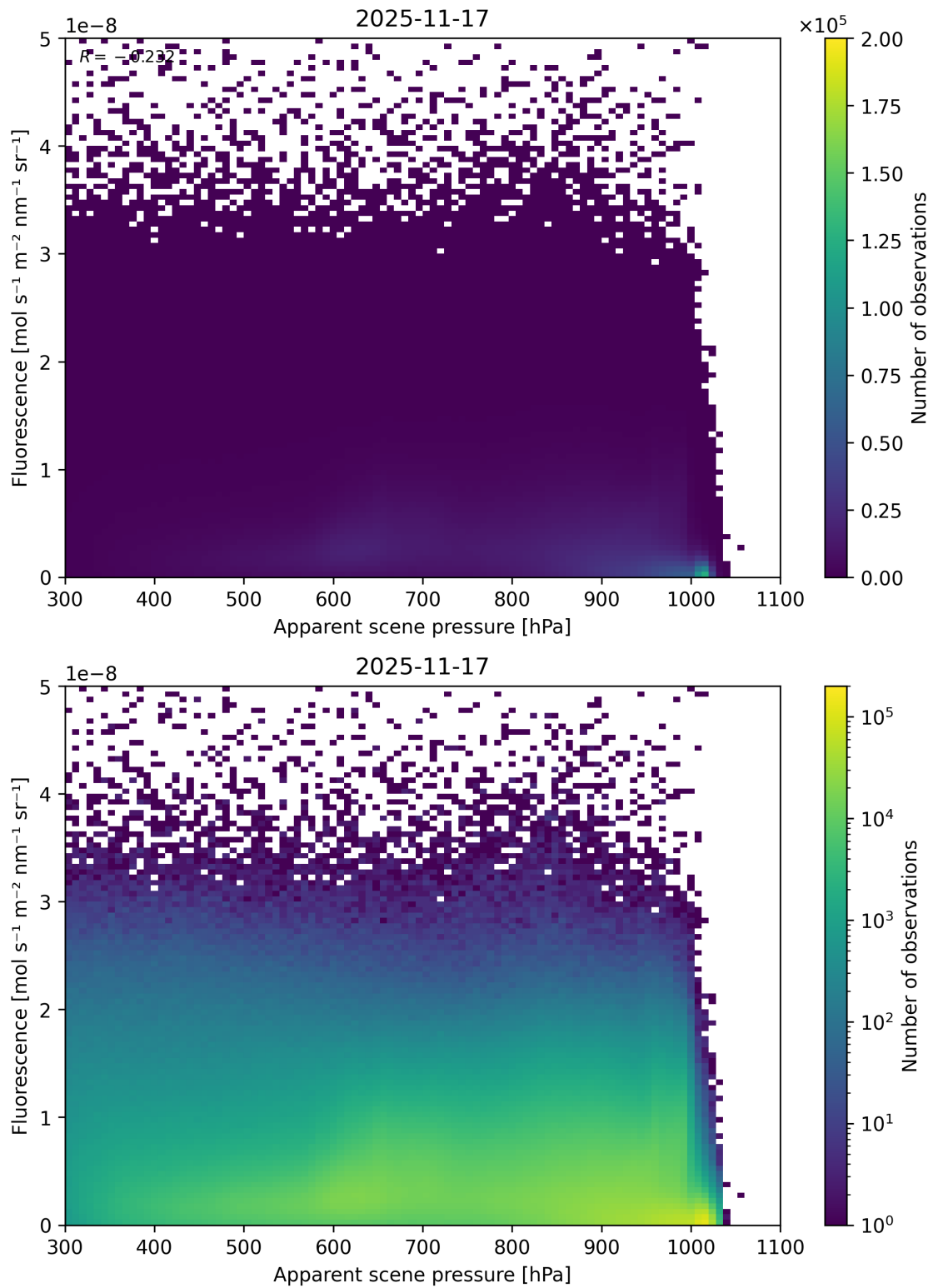
Figure 64: Scatter density plot of “Apparent scene pressure” against “Fluorescence” for 2025-11-16 to 2025-11-18.
