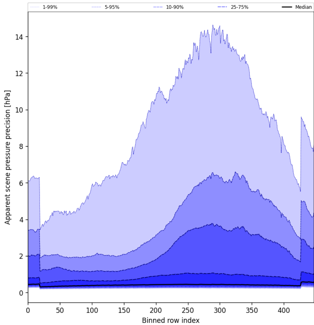
Figure 54: Along track statistics of “Apparent scene pressure precision” for 2025-11-16 to 2025-11-18
