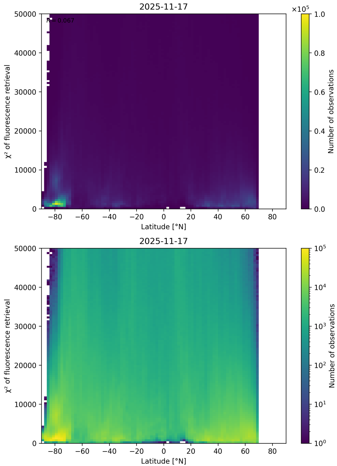
Figure 89: Scatter density plot of “Latitude” against “ \chi^2 of fluorescence retrieval” for 2025-11-16 to 2025-11-18.
