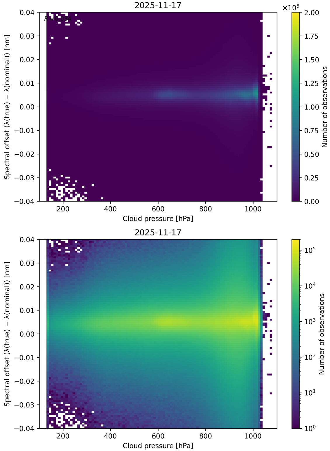
Figure 84: Scatter density plot of “Cloud pressure” against “Spectral offset ( \lambda_{\text{true}} - \lambda_{\text{nominal}} )” for 2025-11-16 to 2025-11-18.
