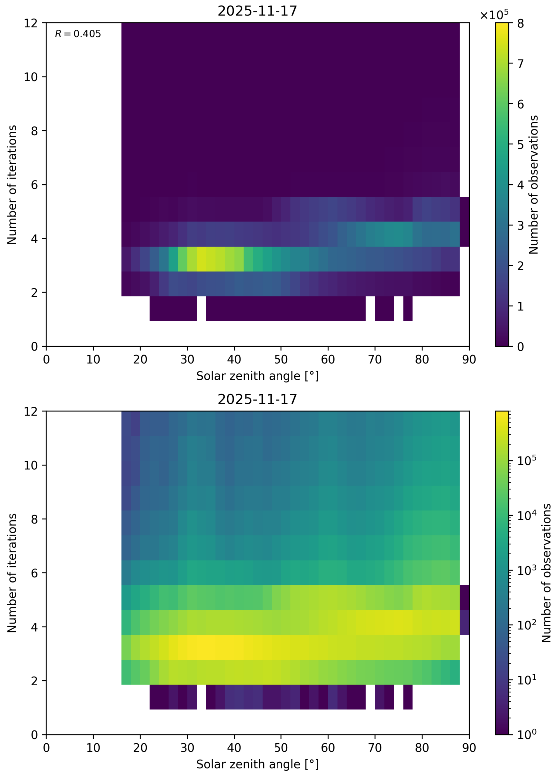
Figure 114: Scatter density plot of “Solar zenith angle” against “Number of iterations” for 2025-11-16 to 2025-11-18.
