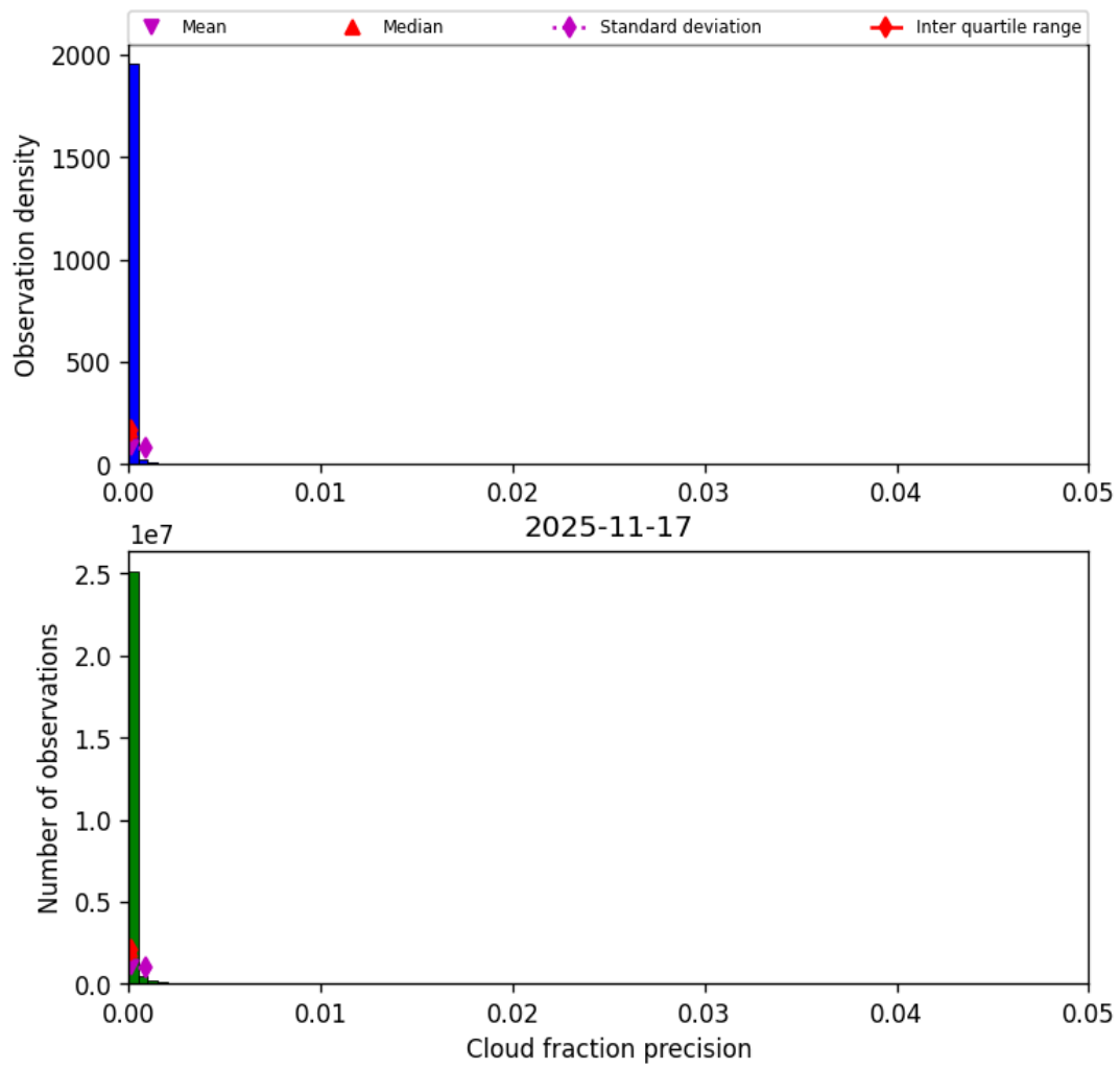
Figure 33: Histogram of “Cloud fraction precision” for 2025-11-16 to 2025-11-18
