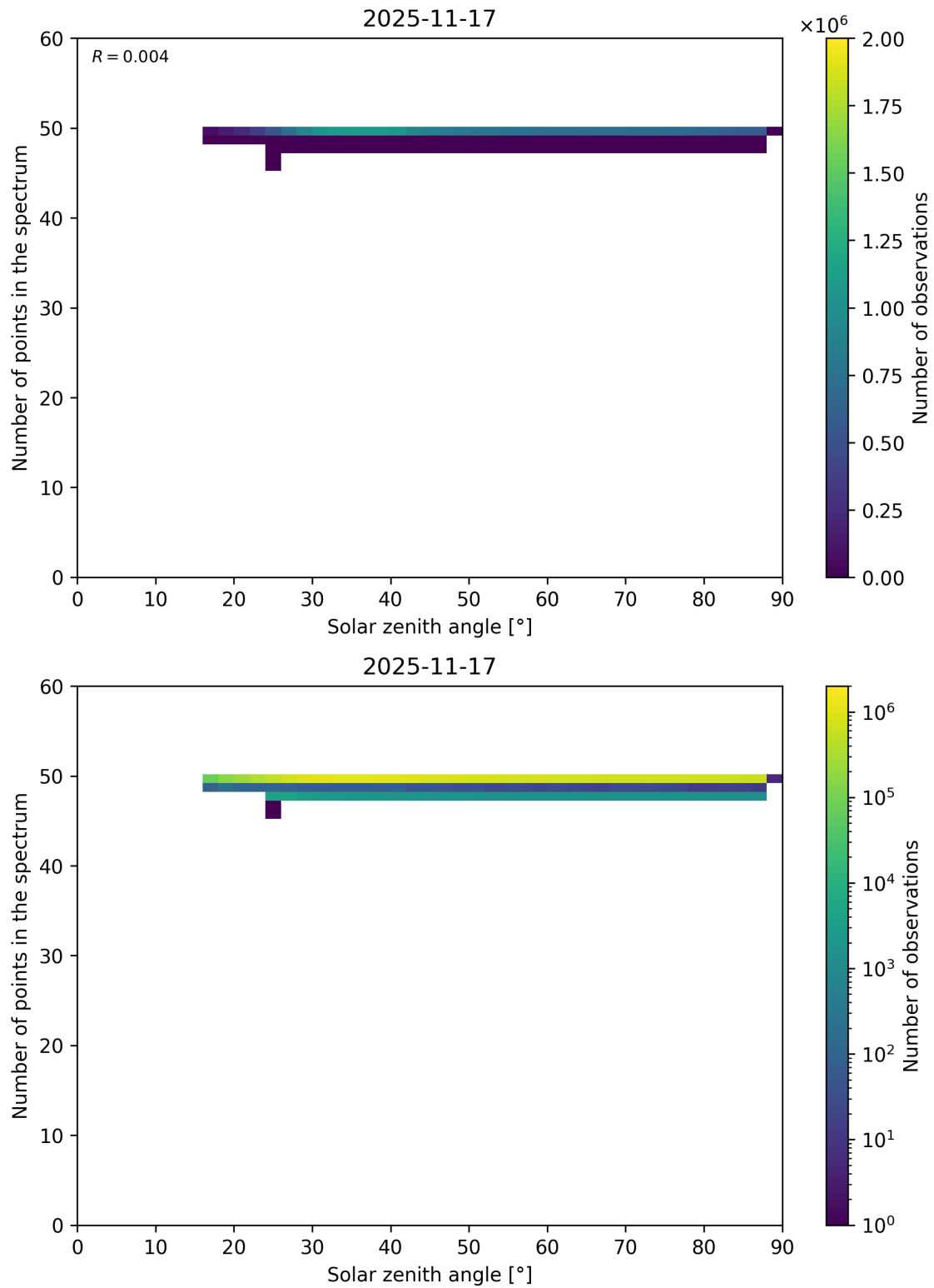
Figure 115: Scatter density plot of “Solar zenith angle” against “Number of points in the spectrum” for 2025-11-16 to 2025-11-18.
