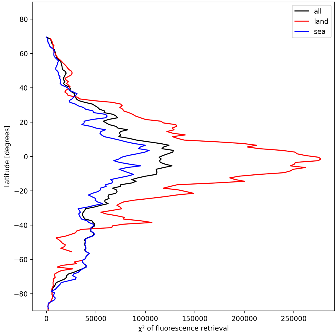
Figure 25: Zonal average of “ \chi^2 of fluorescence retrieval” for 2025-11-16 to 2025-11-18.
