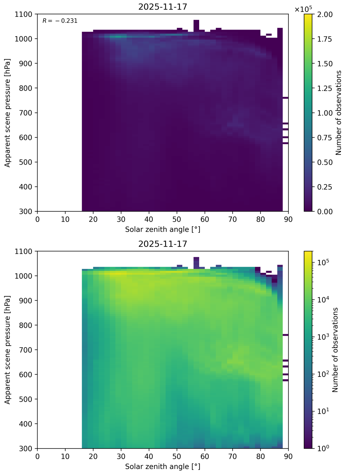
Figure 108: Scatter density plot of “Solar zenith angle” against “Apparent scene pressure” for 2025-11-16 to 2025-11-18.
