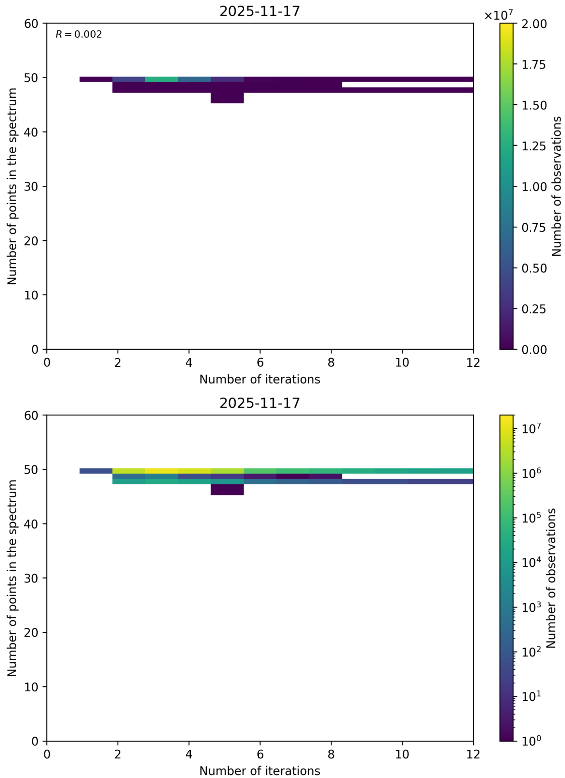
Figure 99: Scatter density plot of “Number of iterations” against “Number of points in the spectrum” for 2025-11-16 to 2025-11-18.
