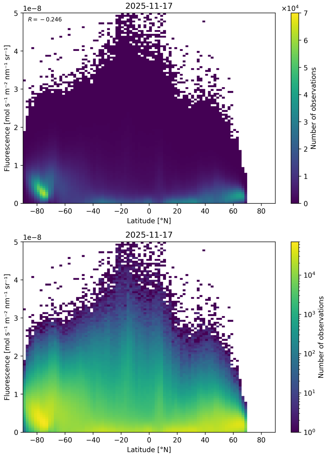
Figure 92: Scatter density plot of “Latitude” against “Fluorescence” for 2025-11-16 to 2025-11-18.
