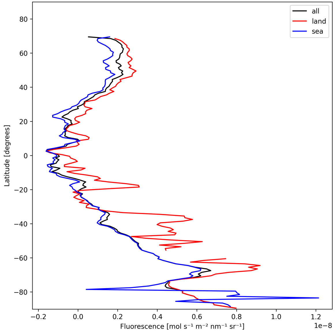
Figure 23: Zonal average of “Fluorescence” for 2025-11-16 to 2025-11-18.
