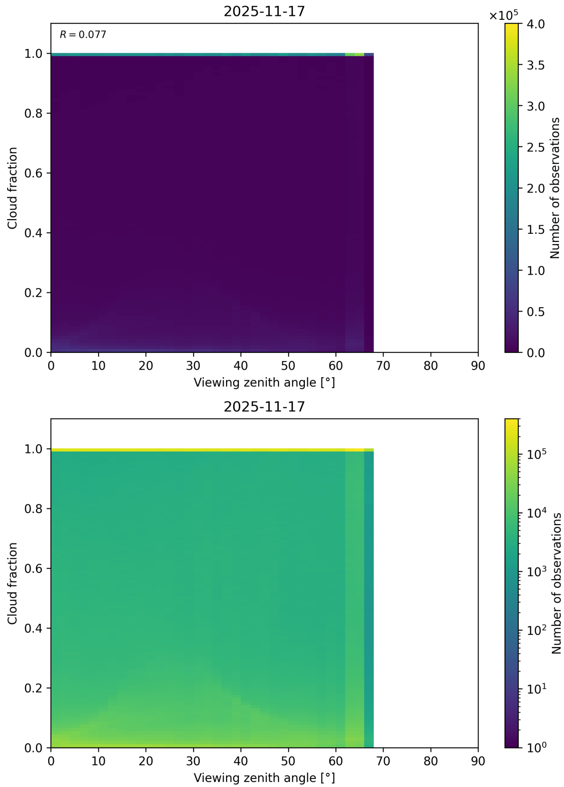
Figure 120: Scatter density plot of “Viewing zenith angle” against “Cloud fraction” for 2025-11-16 to 2025-11-18.
