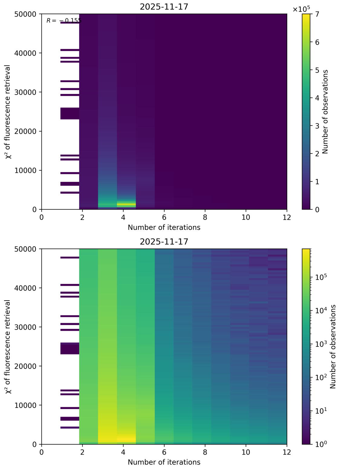
Figure 97: Scatter density plot of “Number of iterations” against “ \chi^2 of fluorescence retrieval” for 2025-11-16 to 2025-11-18.
