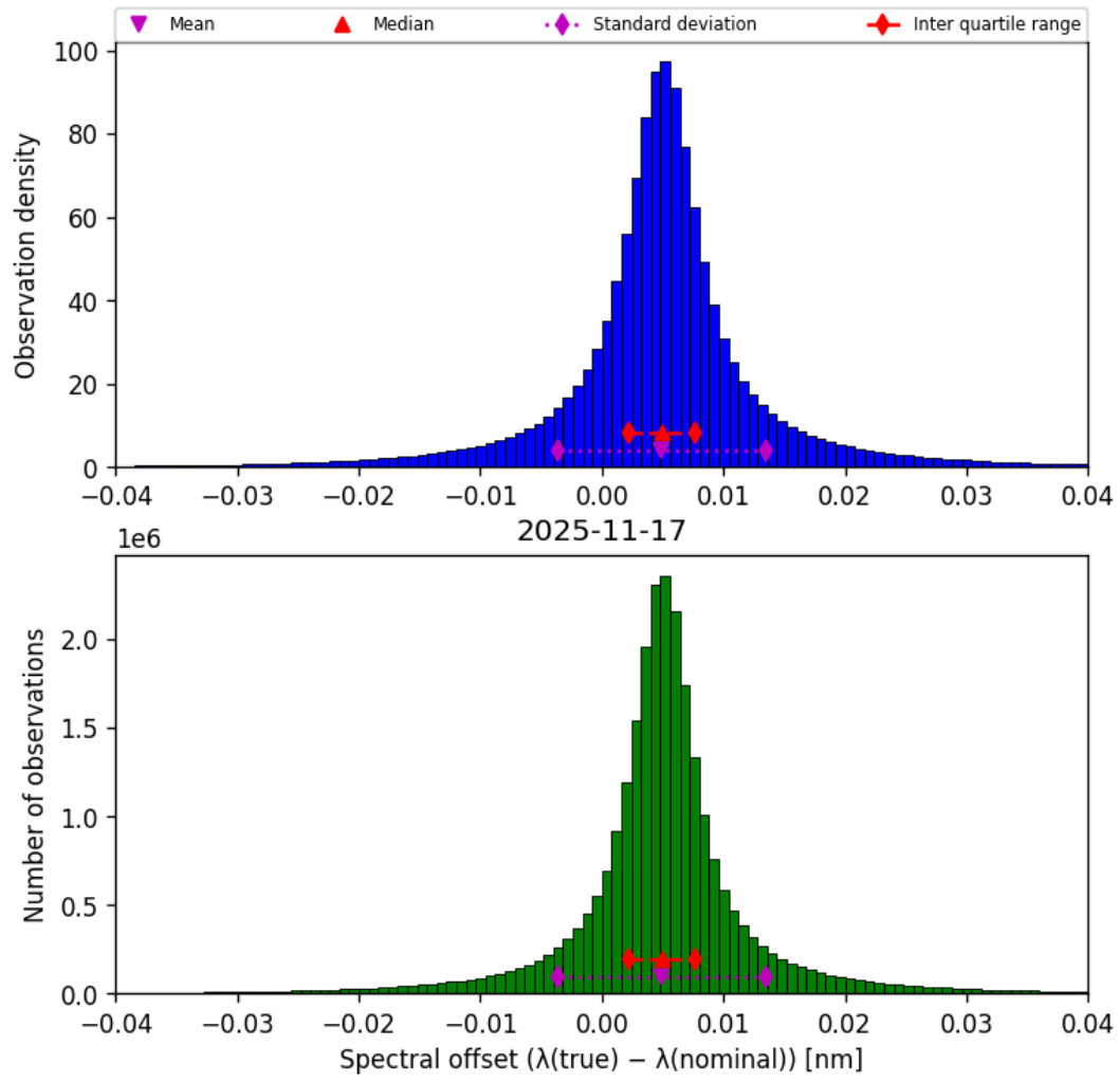
Figure 45: Histogram of “Spectral offset ( \lambda_{\text{true}} - \lambda_{\text{nominal}} )” for 2025-11-16 to 2025-11-18
