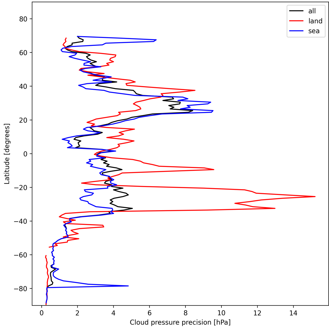
Figure 14: Zonal average of “Cloud pressure precision” for 2025-11-16 to 2025-11-18.
