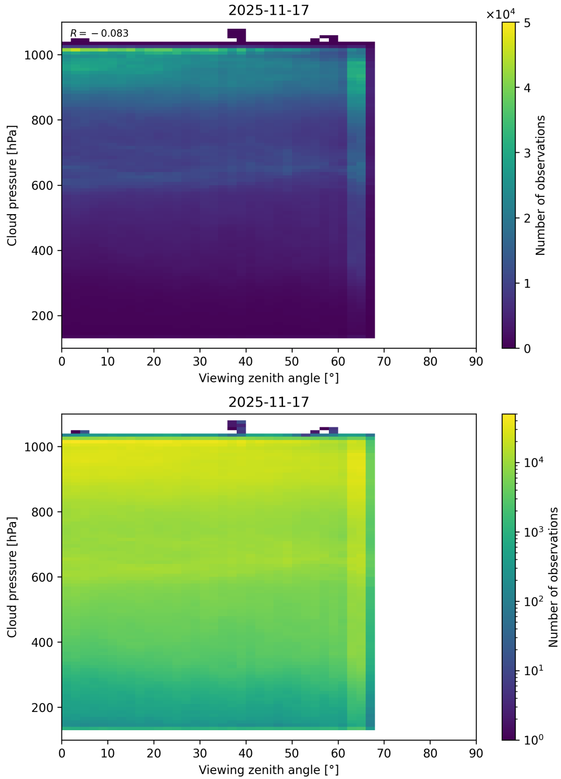
Figure 121: Scatter density plot of “Viewing zenith angle” against “Cloud pressure” for 2025-11-16 to 2025-11-18.
