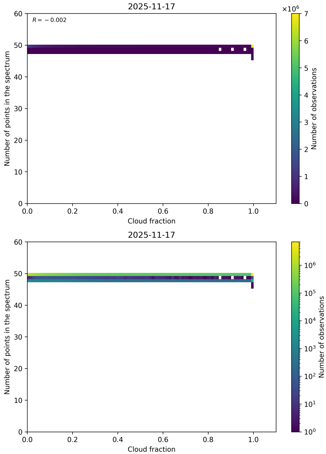
Figure 74: Scatter density plot of “Cloud fraction” against “Number of points in the spectrum” for 2025-11-16 to 2025-11-18.
