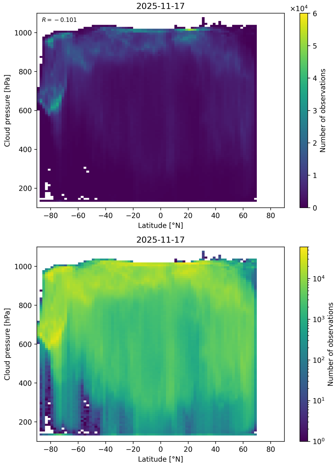
Figure 91: Scatter density plot of “Latitude” against “Cloud pressure” for 2025-11-16 to 2025-11-18.
