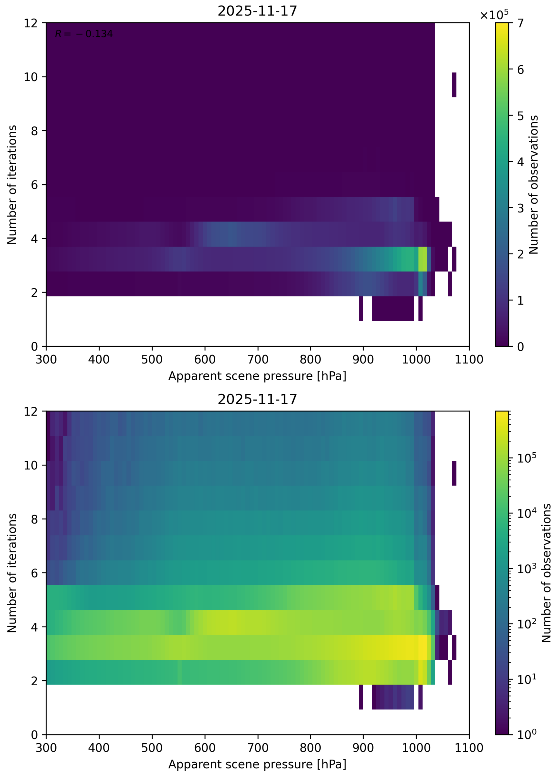
Figure 65: Scatter density plot of “Apparent scene pressure” against “Number of iterations” for 2025-11-16 to 2025-11-18.
