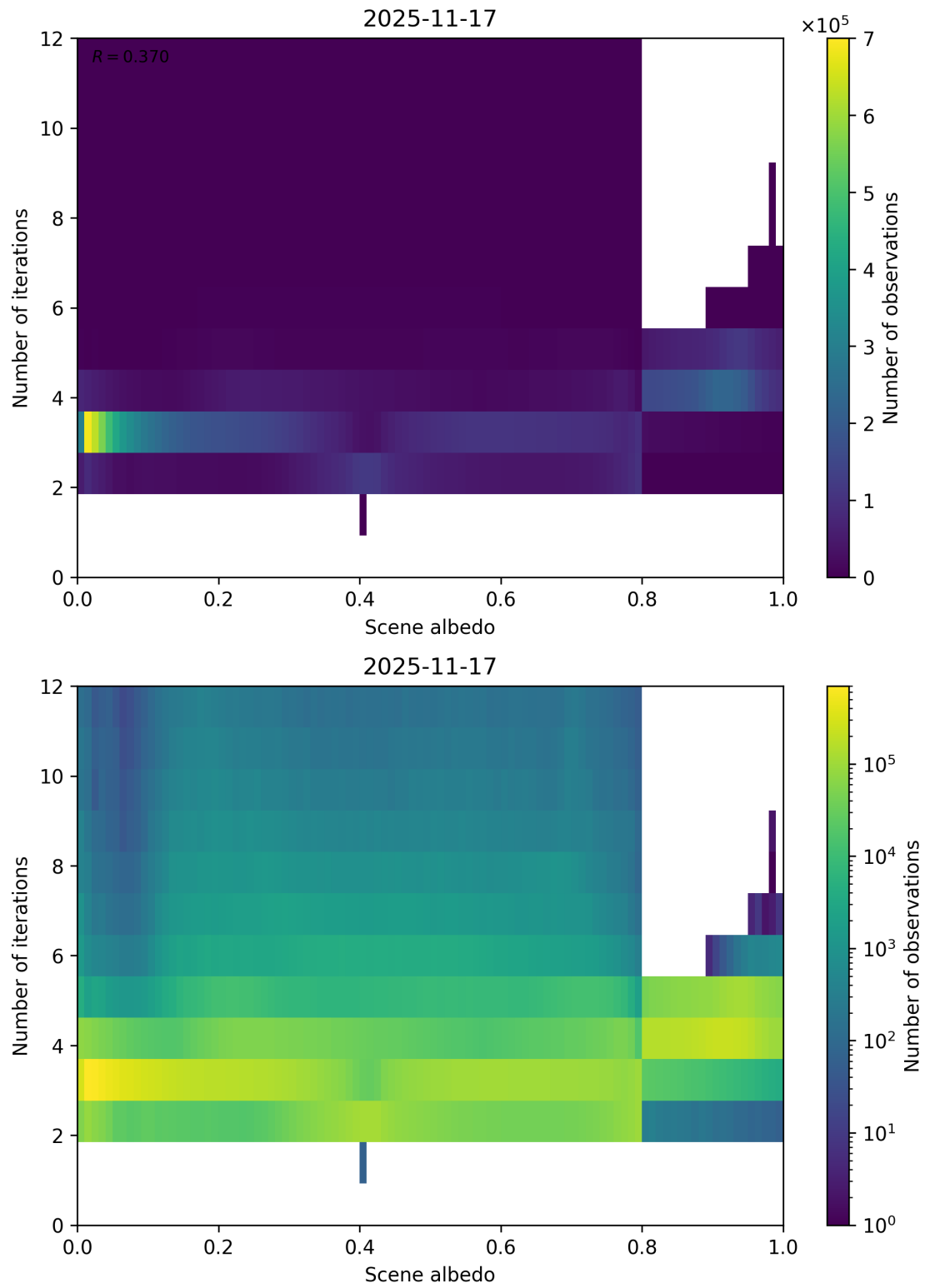
Figure 105: Scatter density plot of “Scene albedo” against “Number of iterations” for 2025-11-16 to 2025-11-18.
