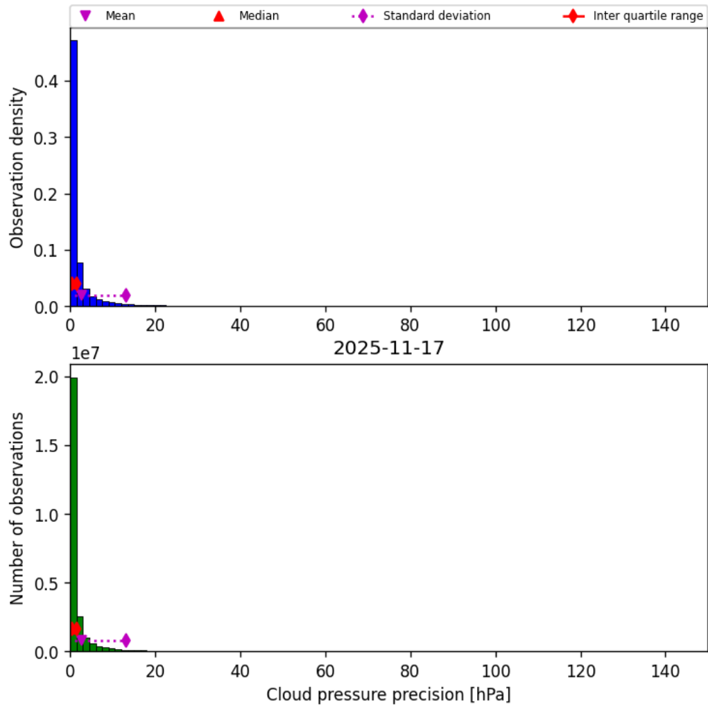
Figure 31: Histogram of “Cloud pressure precision” for 2025-11-16 to 2025-11-18
