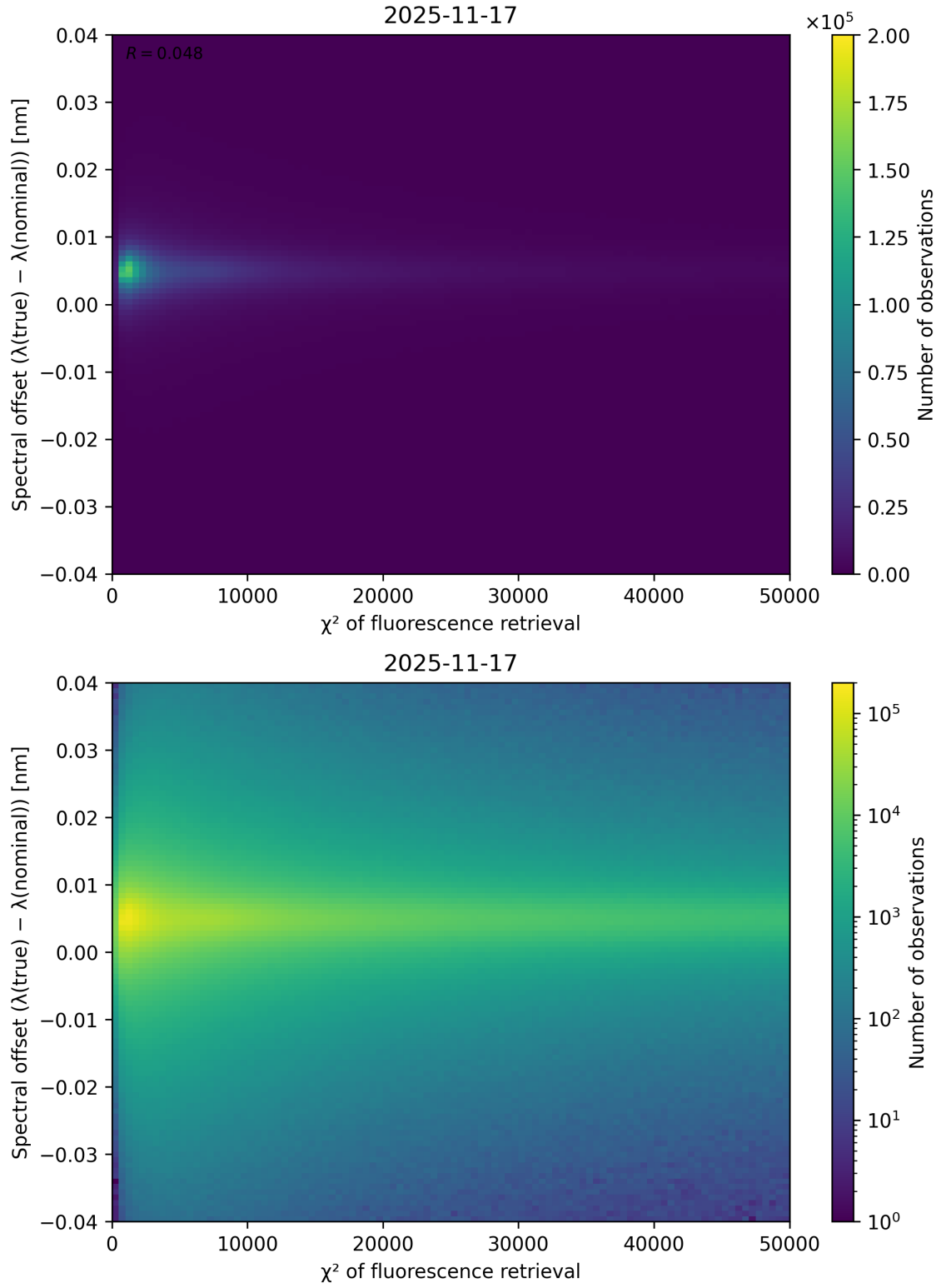
Figure 69: Scatter density plot of “ \chi^2 of fluorescence retrieval” against “Spectral offset ( \lambda_{\text{true}} - \lambda_{\text{nominal}} )” for 2025-11-16 to 2025-11-18.
