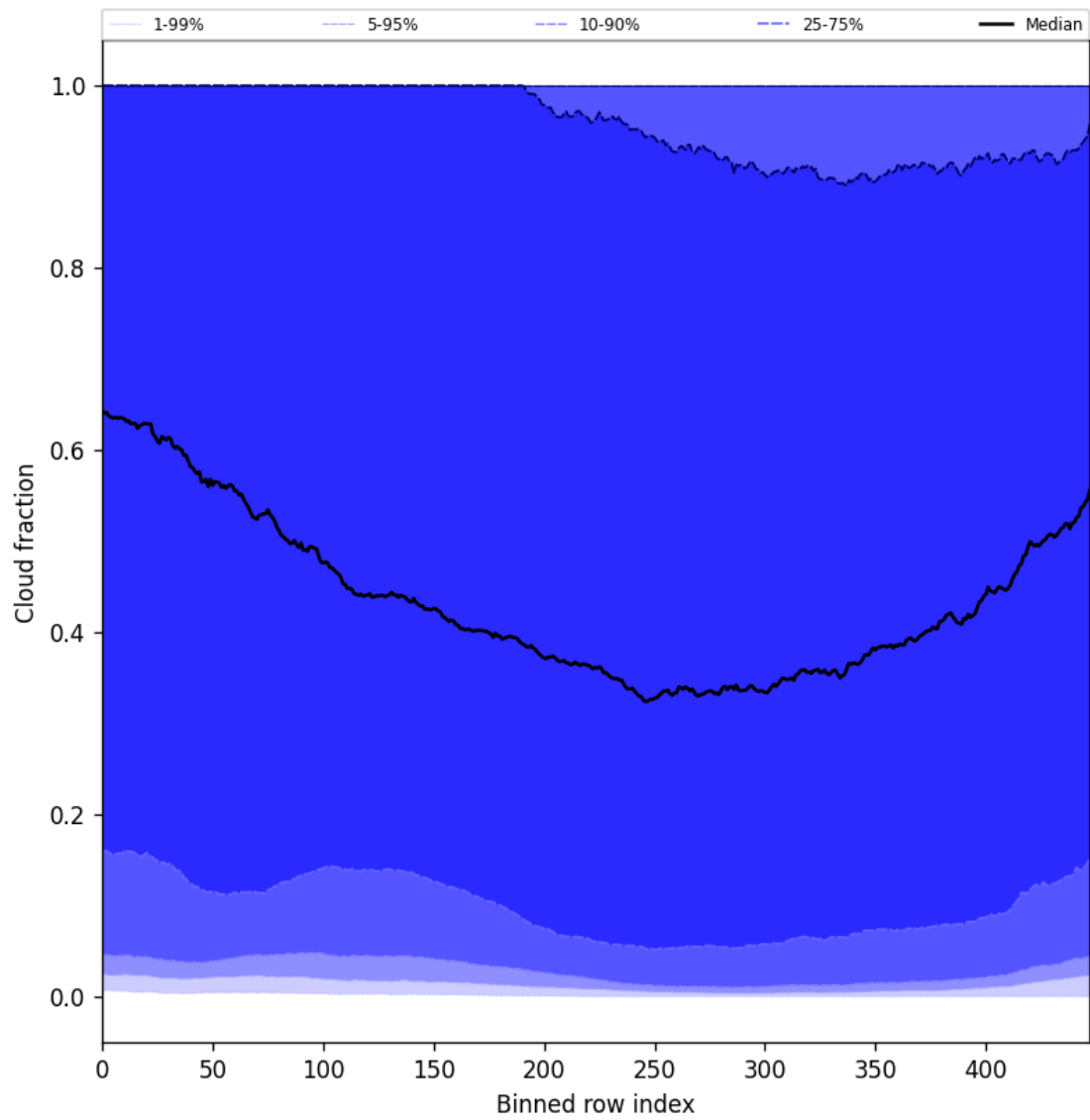
Figure 49: Along track statistics of “Cloud fraction” for 2025-11-16 to 2025-11-18
