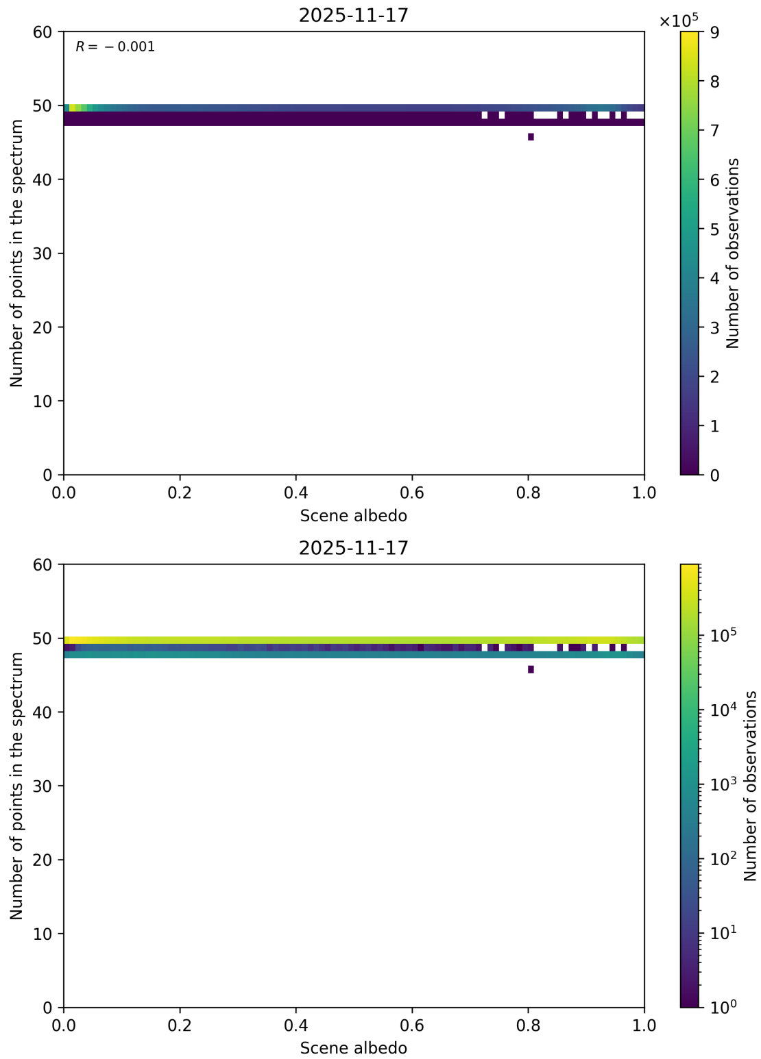
Figure 106: Scatter density plot of “Scene albedo” against “Number of points in the spectrum” for 2025-11-16 to 2025-11-18.
