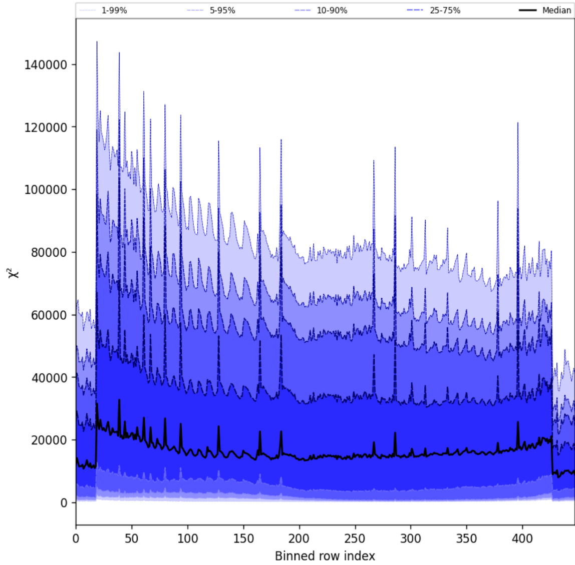
Figure 55: Along track statistics of “ \chi^2 ” for 2025-11-16 to 2025-11-18
