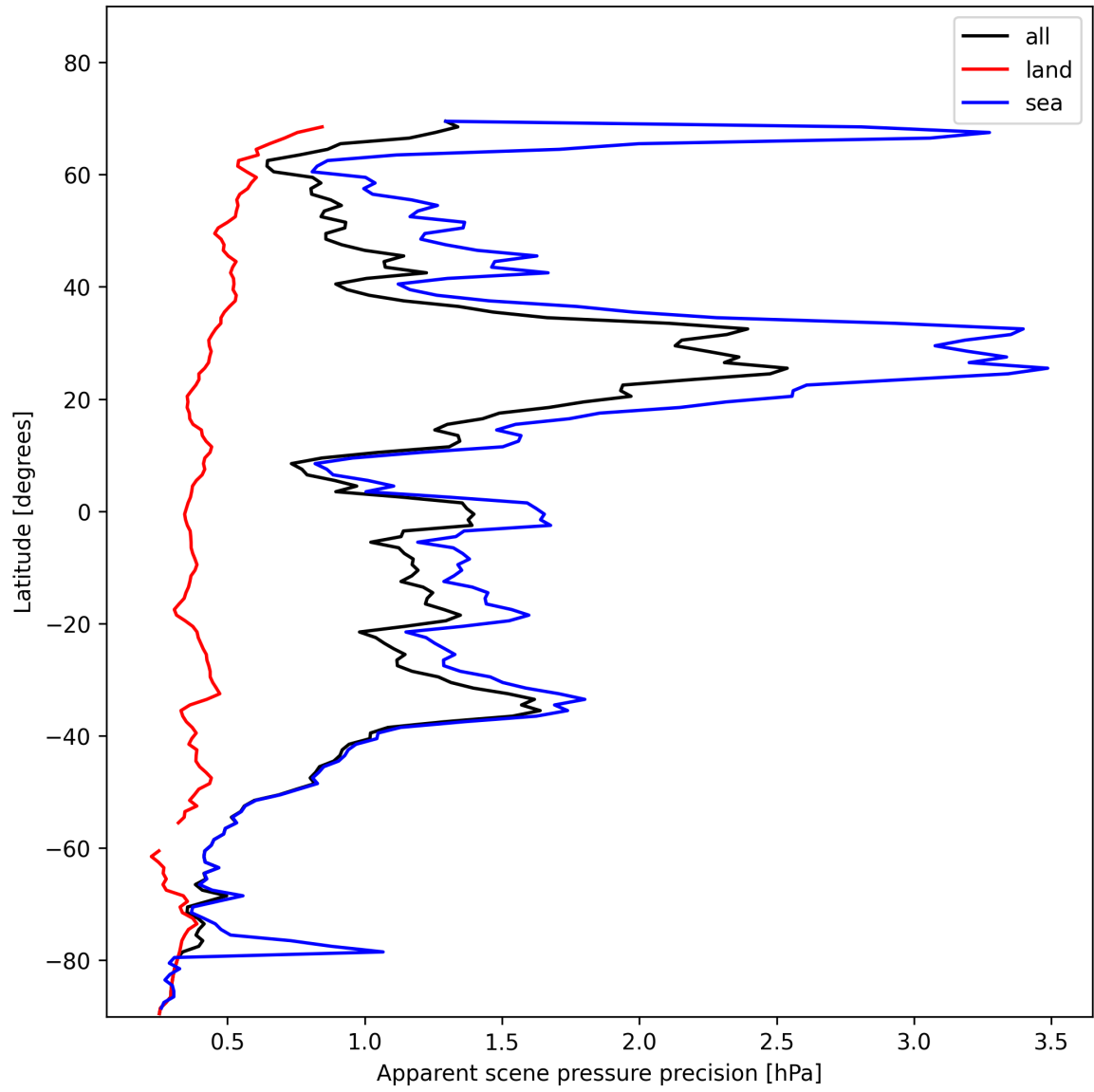
Figure 20: Zonal average of “Apparent scene pressure precision” for 2025-11-16 to 2025-11-18.
