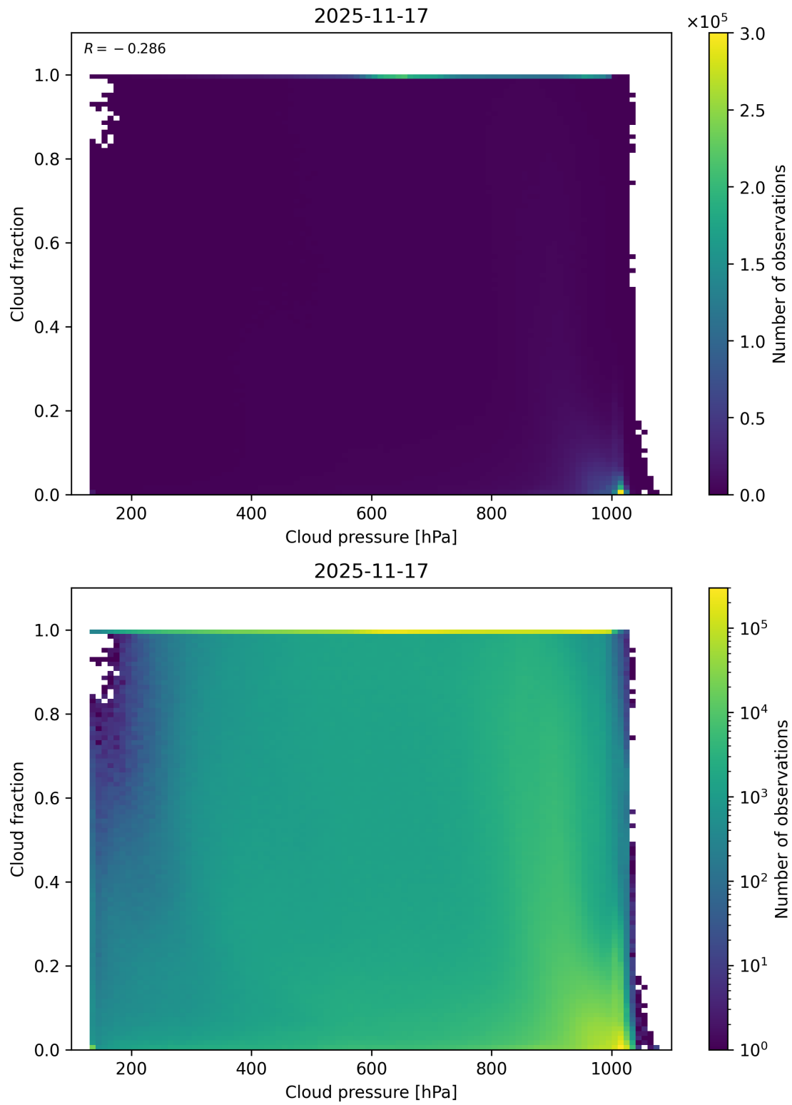
Figure 79: Scatter density plot of “Cloud pressure” against “Cloud fraction” for 2025-11-16 to 2025-11-18.
