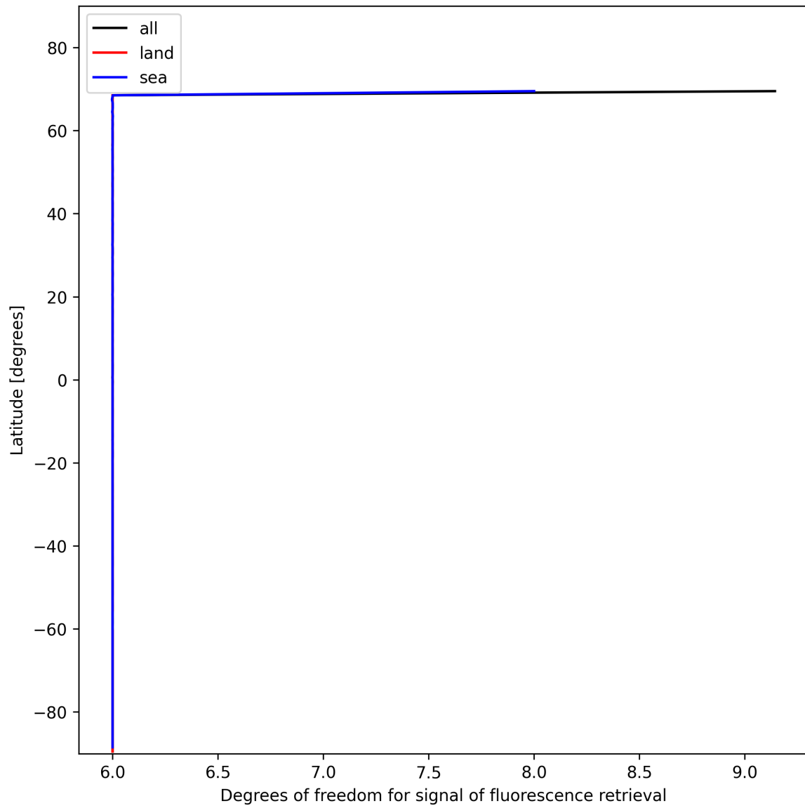
Figure 26: Zonal average of “Degrees of freedom for signal of fluorescence retrieval” for 2025-11-16 to 2025-11-18.
