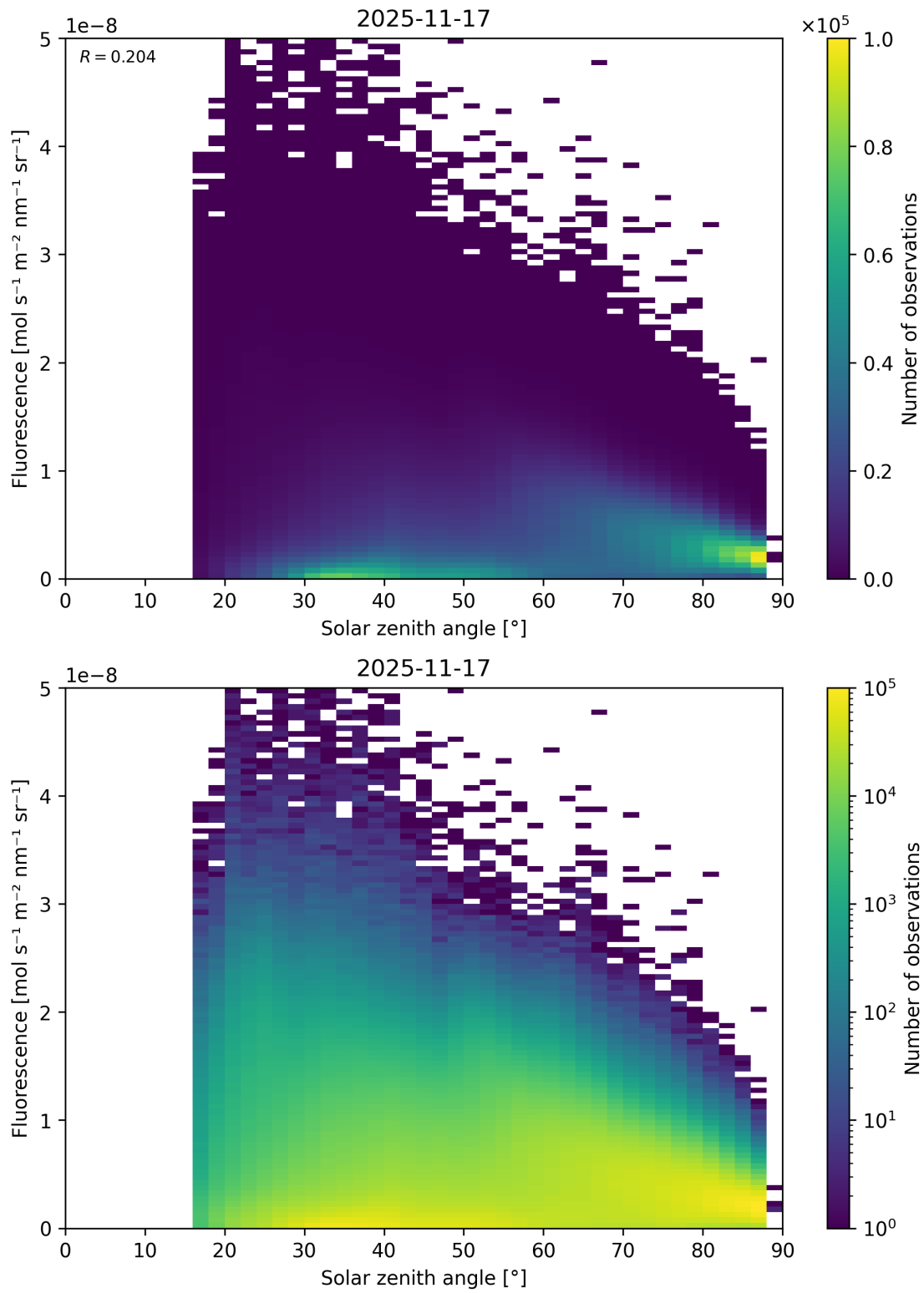
Figure 112: Scatter density plot of “Solar zenith angle” against “Fluorescence” for 2025-11-16 to 2025-11-18.
