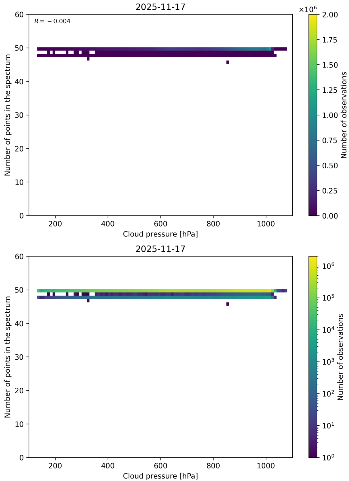
Figure 82: Scatter density plot of “Cloud pressure” against “Number of points in the spectrum” for 2025-11-16 to 2025-11-18.
