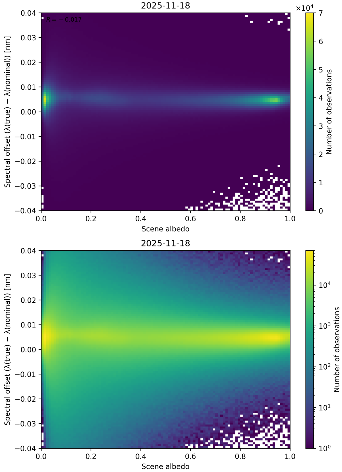
Figure 107: Scatter density plot of “Scene albedo” against “Spectral offset ( \lambda_{\text{true}} - \lambda_{\text{nominal}} )” for 2025-11-18 to 2025-11-19.
