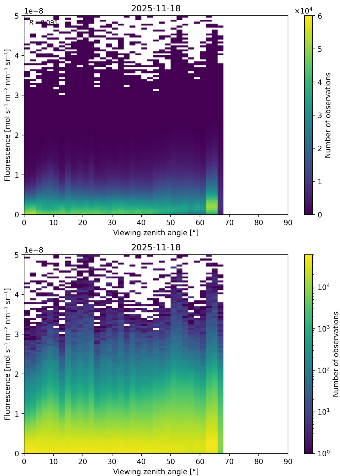
Figure 122: Scatter density plot of “Viewing zenith angle” against “Fluorescence” for 2025-11-18 to 2025-11-19.
