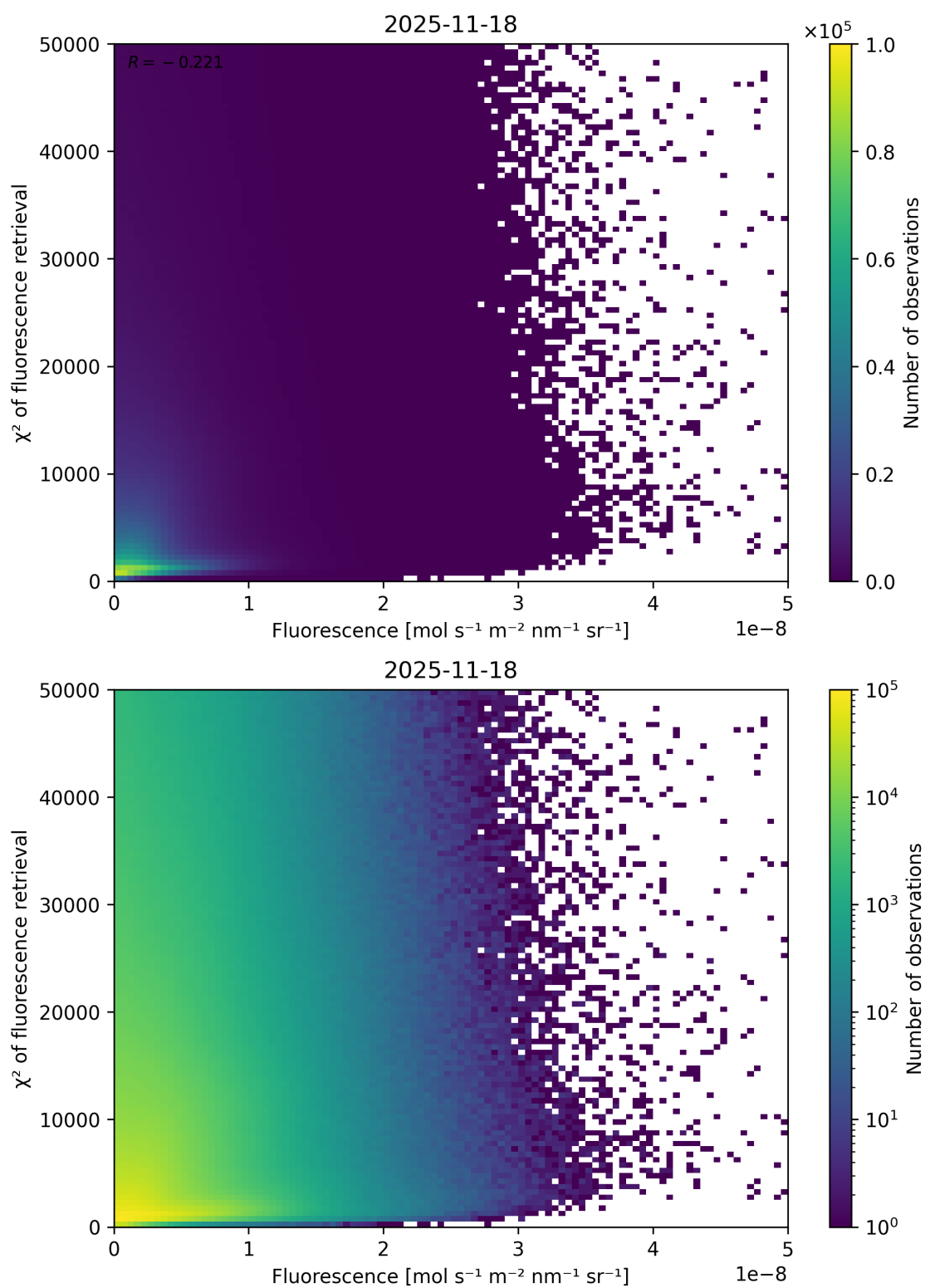
Figure 85: Scatter density plot of “Fluorescence” against “ \chi^2 of fluorescence retrieval” for 2025-11-18 to 2025-11-19.
