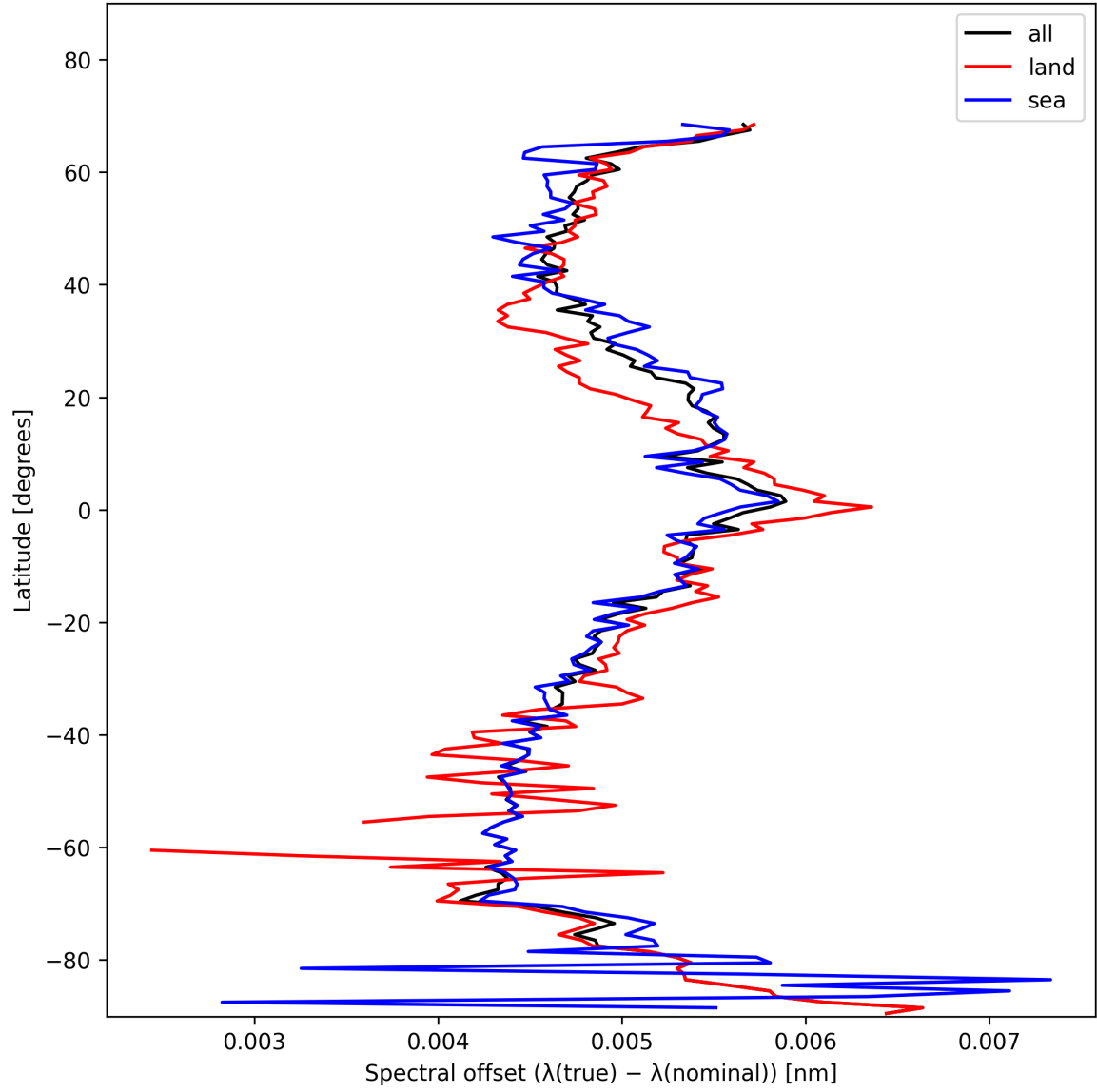
Figure 28: Zonal average of “Spectral offset ( \lambda_{\text{true}} - \lambda_{\text{nominal}} )” for 2025-11-18 to 2025-11-19.
