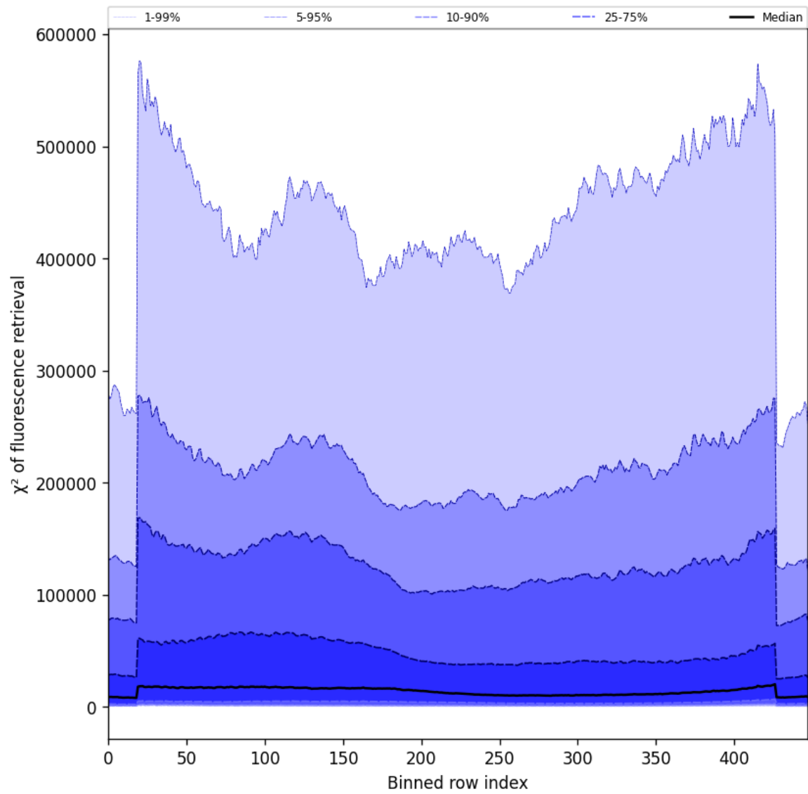
Figure 59: Along track statistics of “ \chi^2 of fluorescence retrieval” for 2025-11-18 to 2025-11-19
