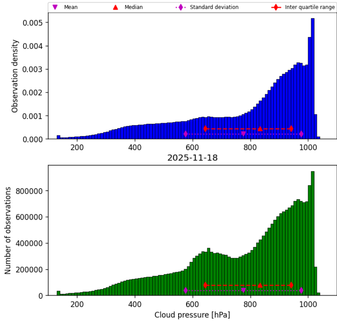
Figure 30: Histogram of “Cloud pressure” for 2025-11-18 to 2025-11-19
