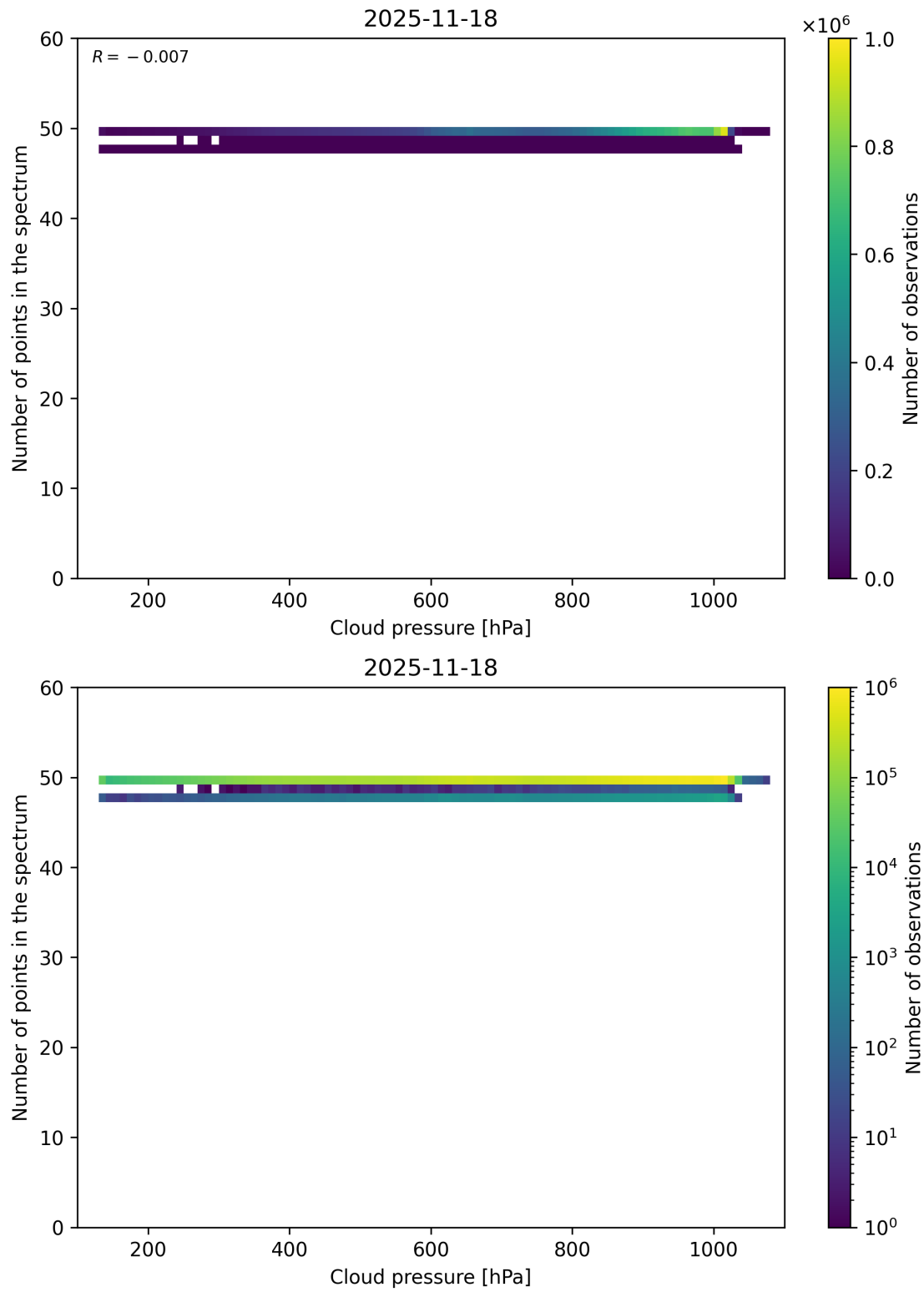
Figure 82: Scatter density plot of “Cloud pressure” against “Number of points in the spectrum” for 2025-11-18 to 2025-11-19.
