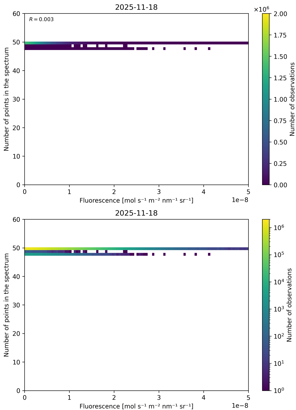
Figure 86: Scatter density plot of “Fluorescence” against “Number of points in the spectrum” for 2025-11-18 to 2025-11-19.
