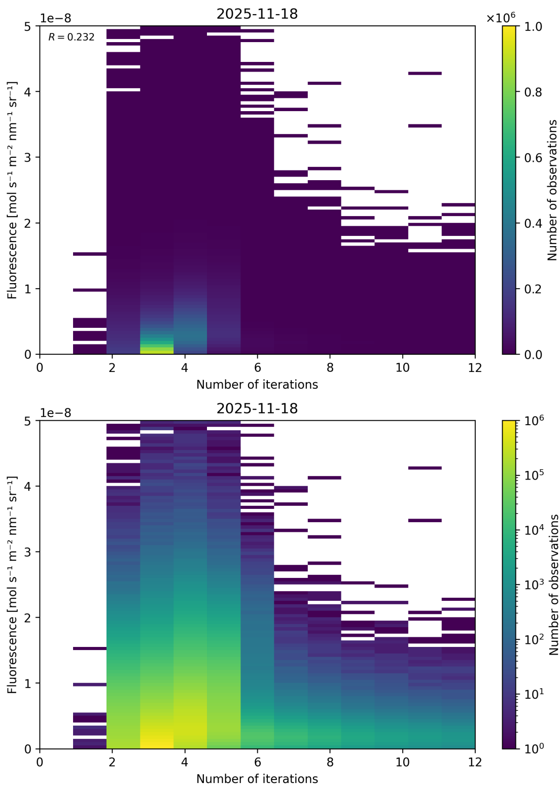
Figure 98: Scatter density plot of “Number of iterations” against “Fluorescence” for 2025-11-18 to 2025-11-19.
