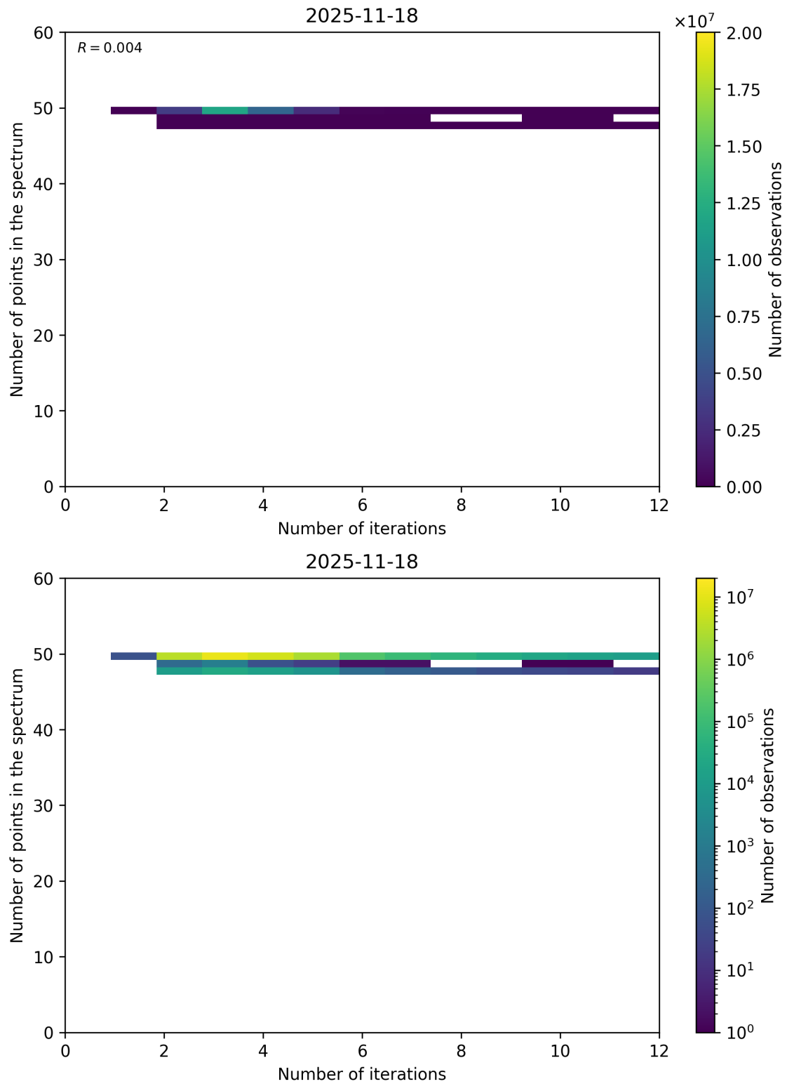
Figure 99: Scatter density plot of “Number of iterations” against “Number of points in the spectrum” for 2025-11-18 to 2025-11-19.
