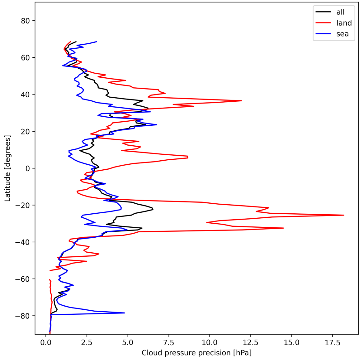
Figure 14: Zonal average of “Cloud pressure precision” for 2025-11-18 to 2025-11-19.
