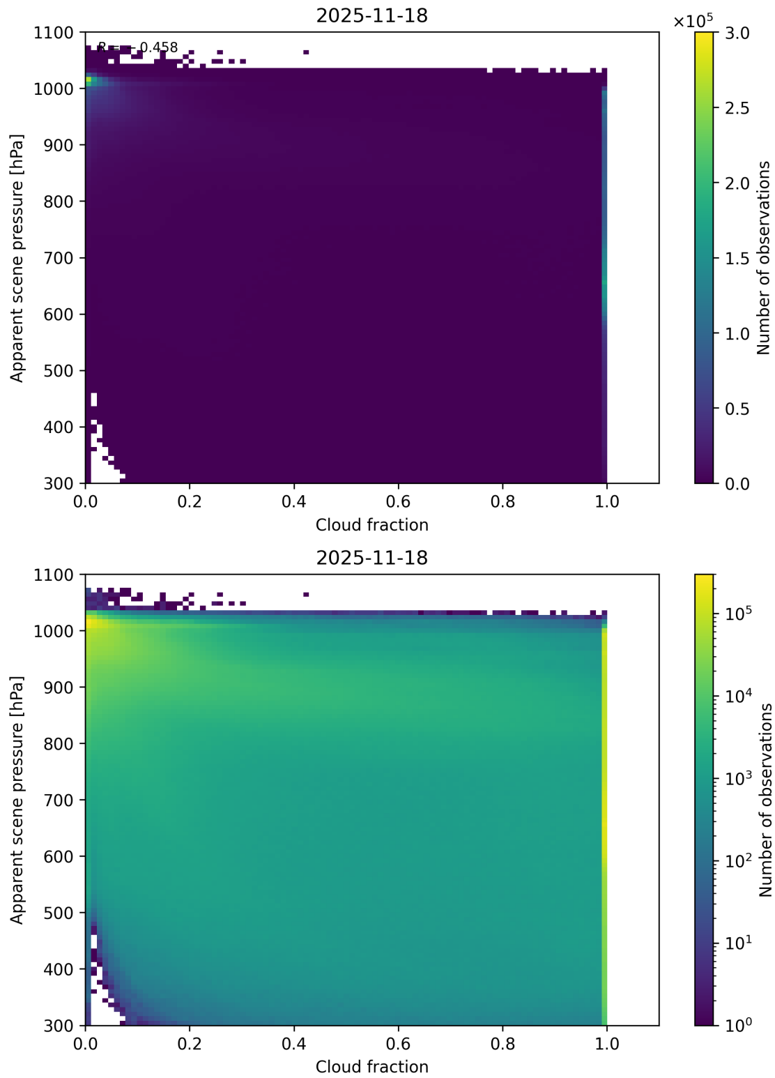
Figure 70: Scatter density plot of “Cloud fraction” against “Apparent scene pressure” for 2025-11-18 to 2025-11-19.
