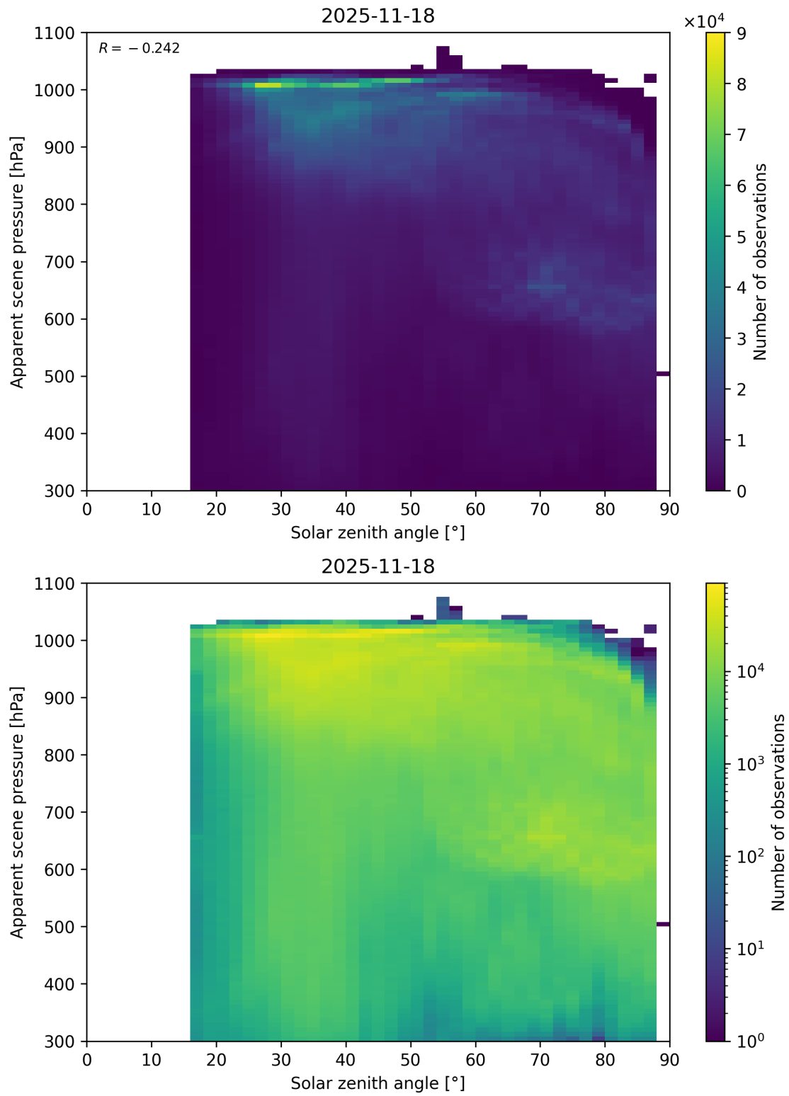
Figure 108: Scatter density plot of “Solar zenith angle” against “Apparent scene pressure” for 2025-11-18 to 2025-11-19.
