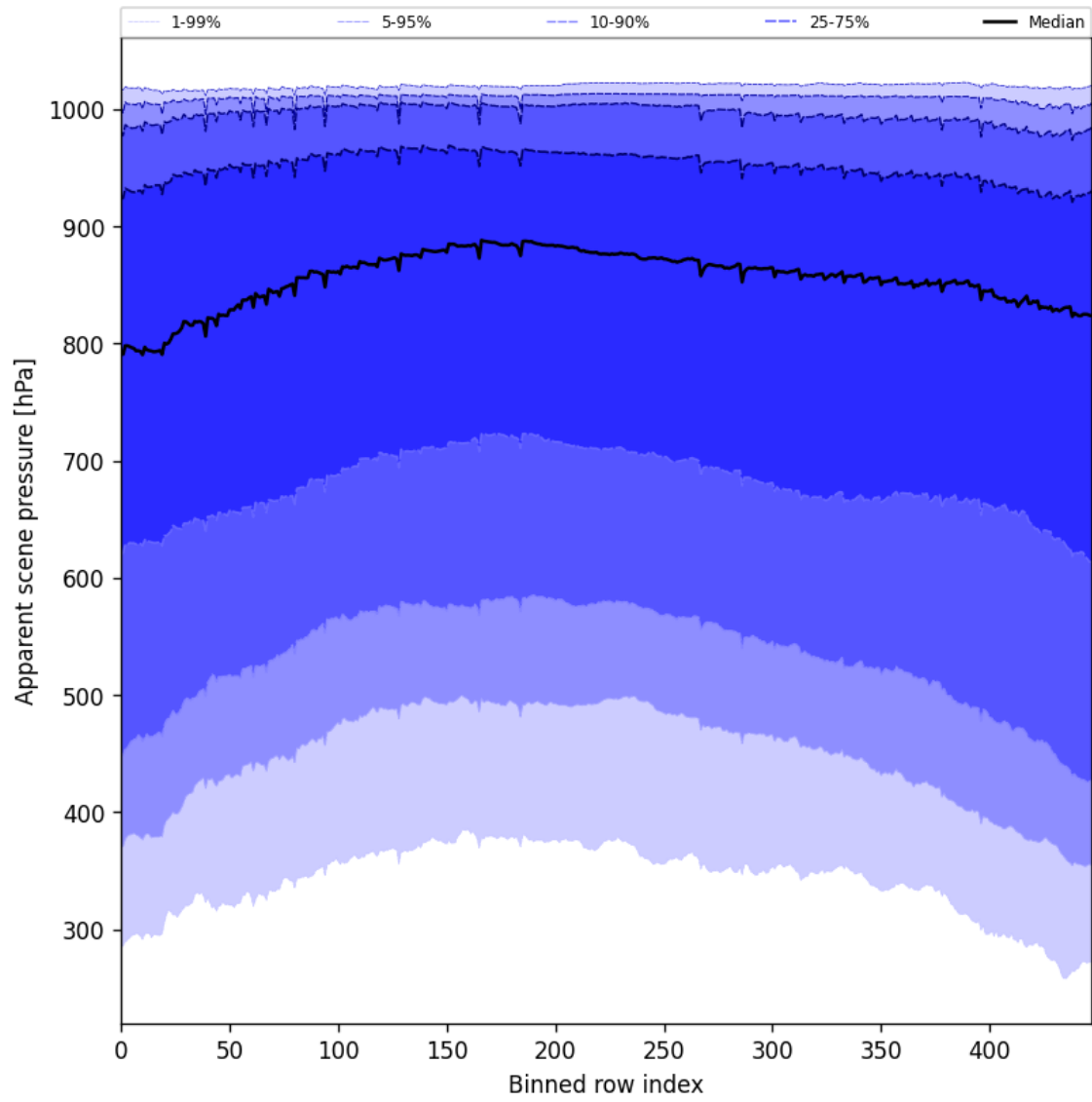
Figure 53: Along track statistics of “Apparent scene pressure” for 2025-11-18 to 2025-11-19
