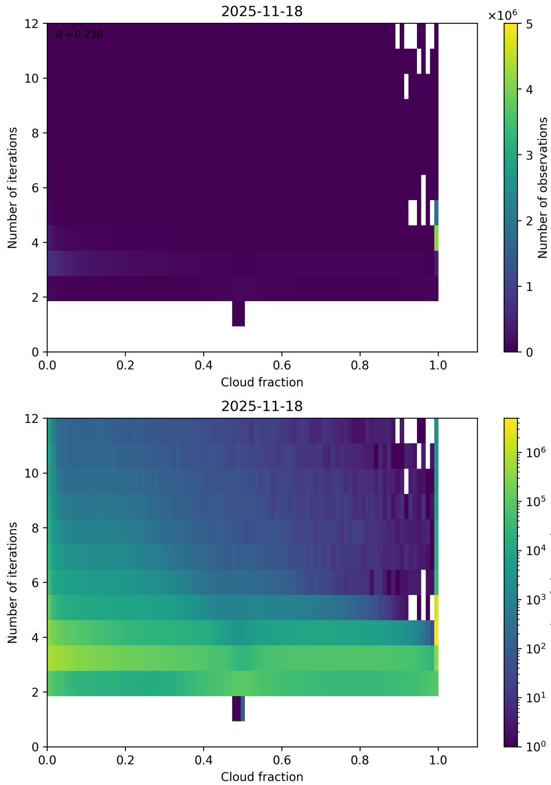
Figure 73: Scatter density plot of “Cloud fraction” against “Number of iterations” for 2025-11-18 to 2025-11-19.
