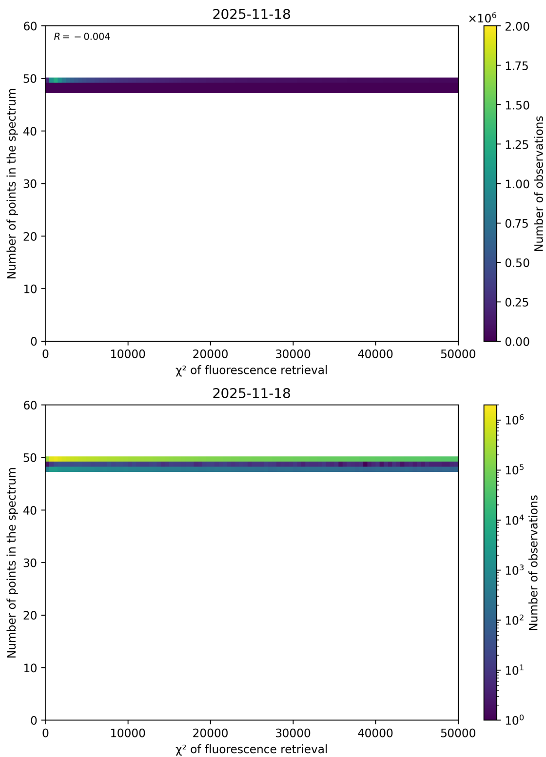
Figure 68: Scatter density plot of “ \chi^2 of fluorescence retrieval” against “Number of points in the spectrum” for 2025-11-18 to 2025-11-19.
