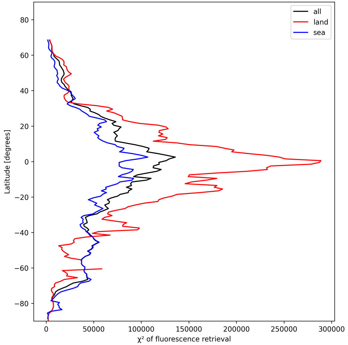
Figure 25: Zonal average of “ \chi^2 of fluorescence retrieval” for 2025-11-18 to 2025-11-19.
