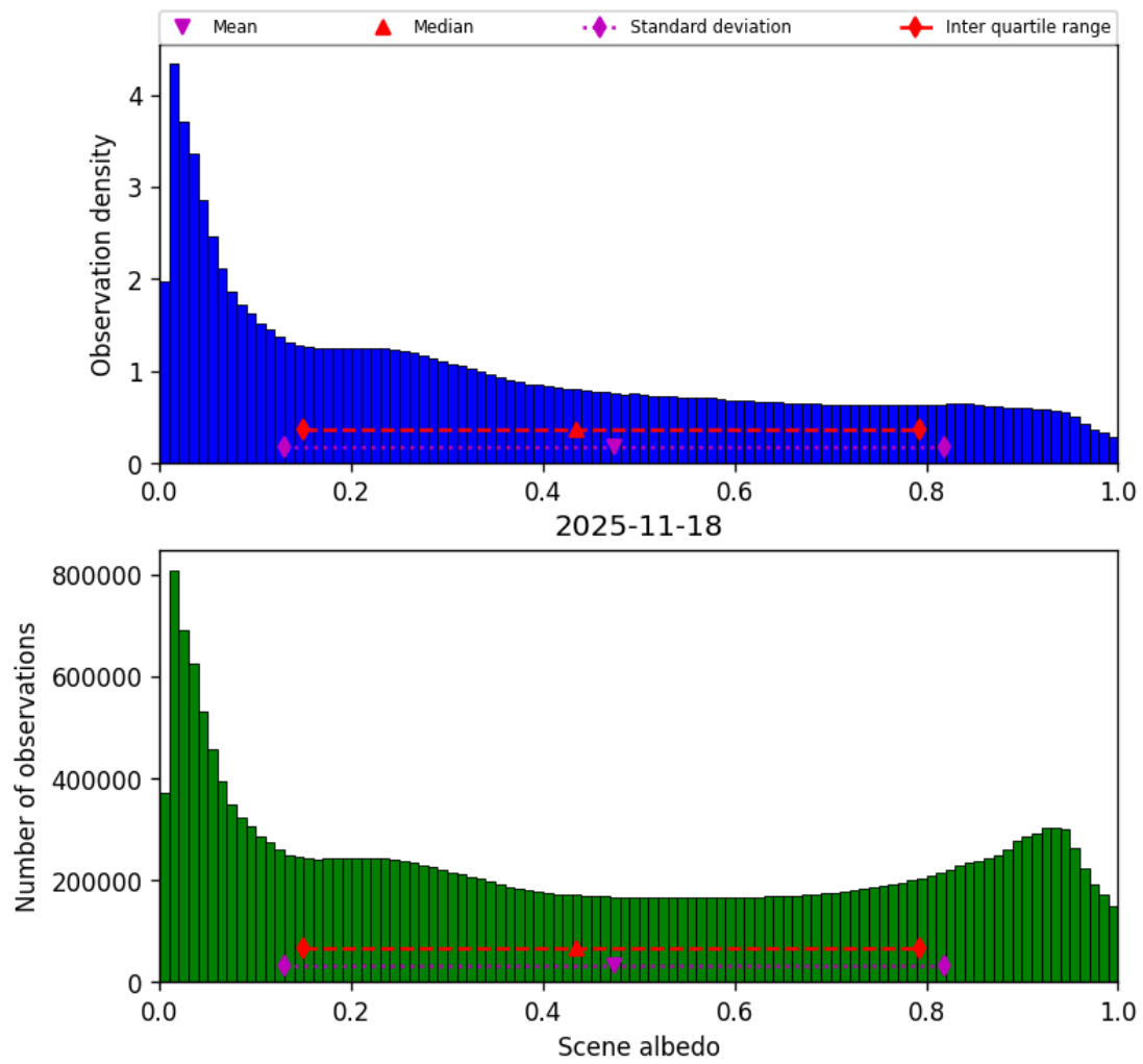
Figure 34: Histogram of “Scene albedo” for 2025-11-18 to 2025-11-19
