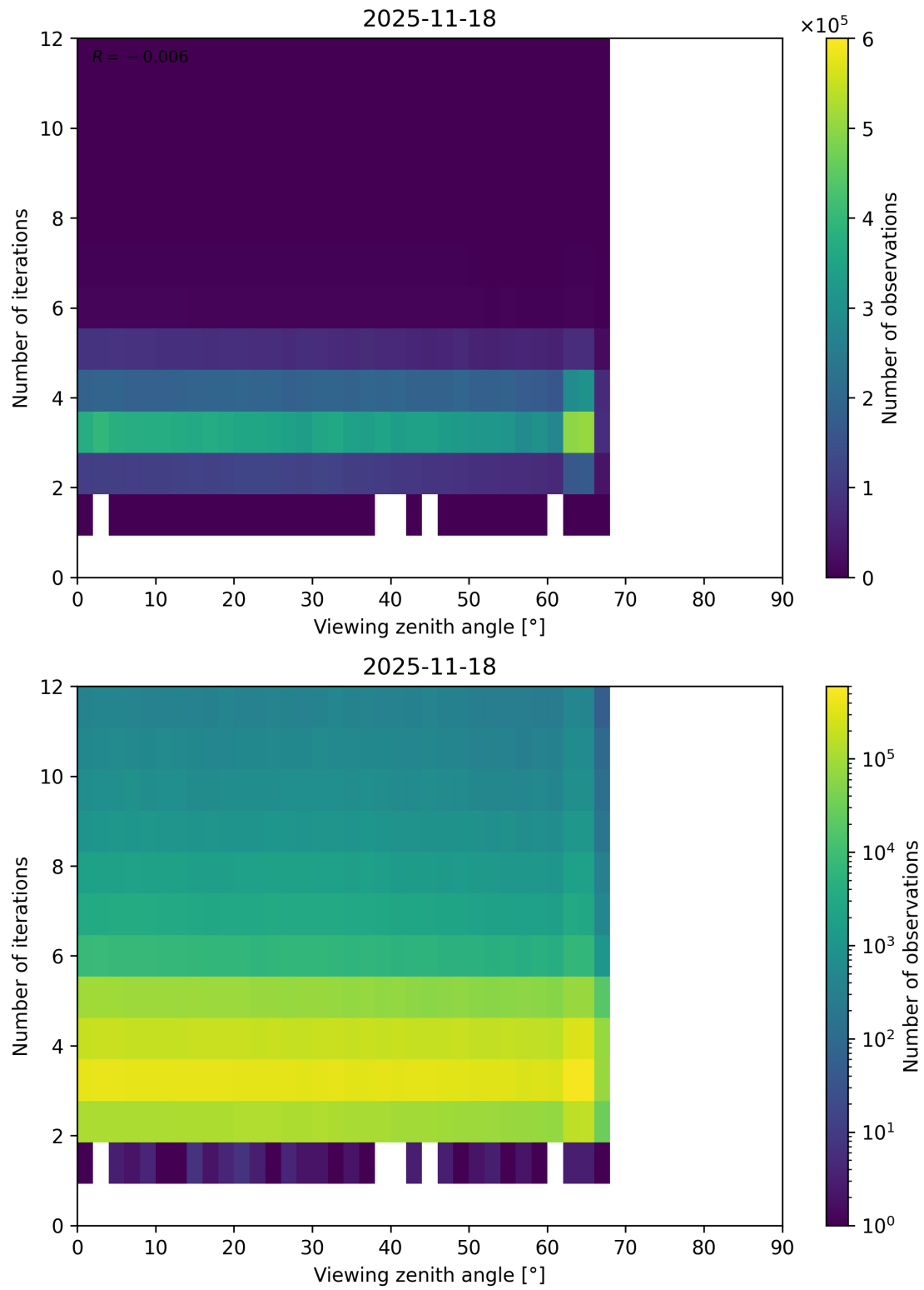
Figure 124: Scatter density plot of “Viewing zenith angle” against “Number of iterations” for 2025-11-18 to 2025-11-19.
