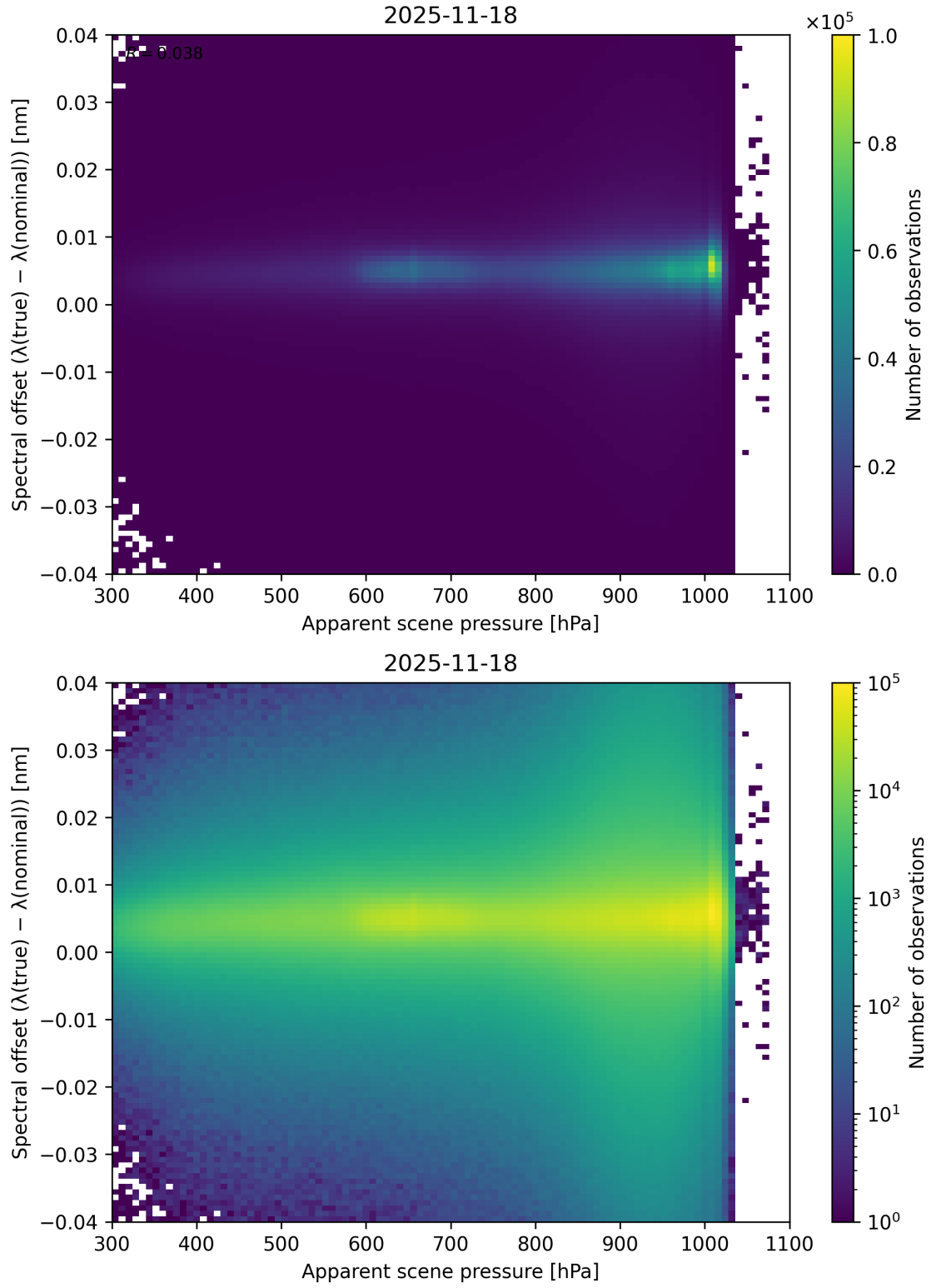
Figure 67: Scatter density plot of “Apparent scene pressure” against “Spectral offset ( \lambda_{\text{true}} - \lambda_{\text{nominal}} )” for 2025-11-18 to 2025-11-19.
