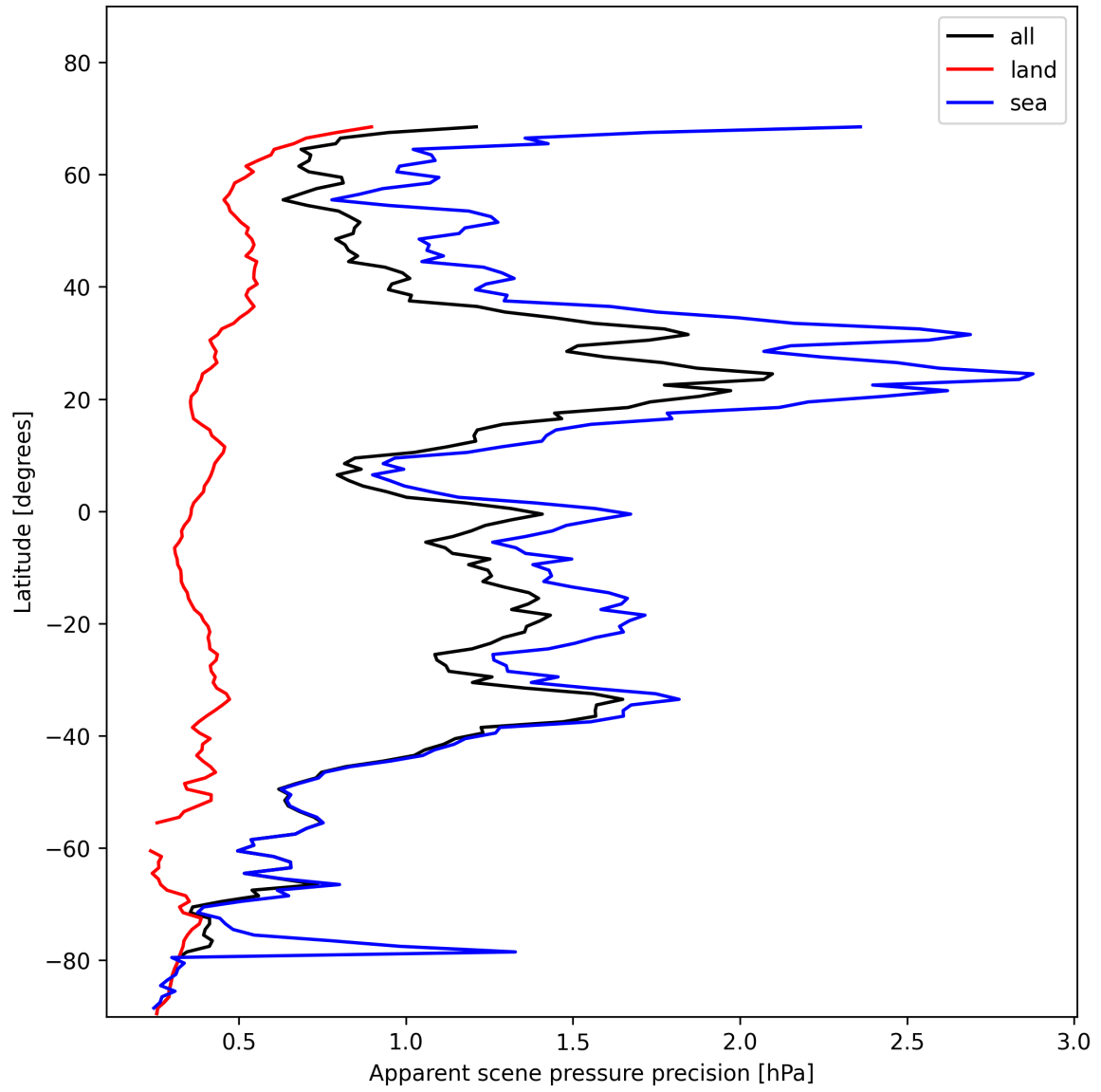
Figure 20: Zonal average of “Apparent scene pressure precision” for 2025-11-18 to 2025-11-19.
