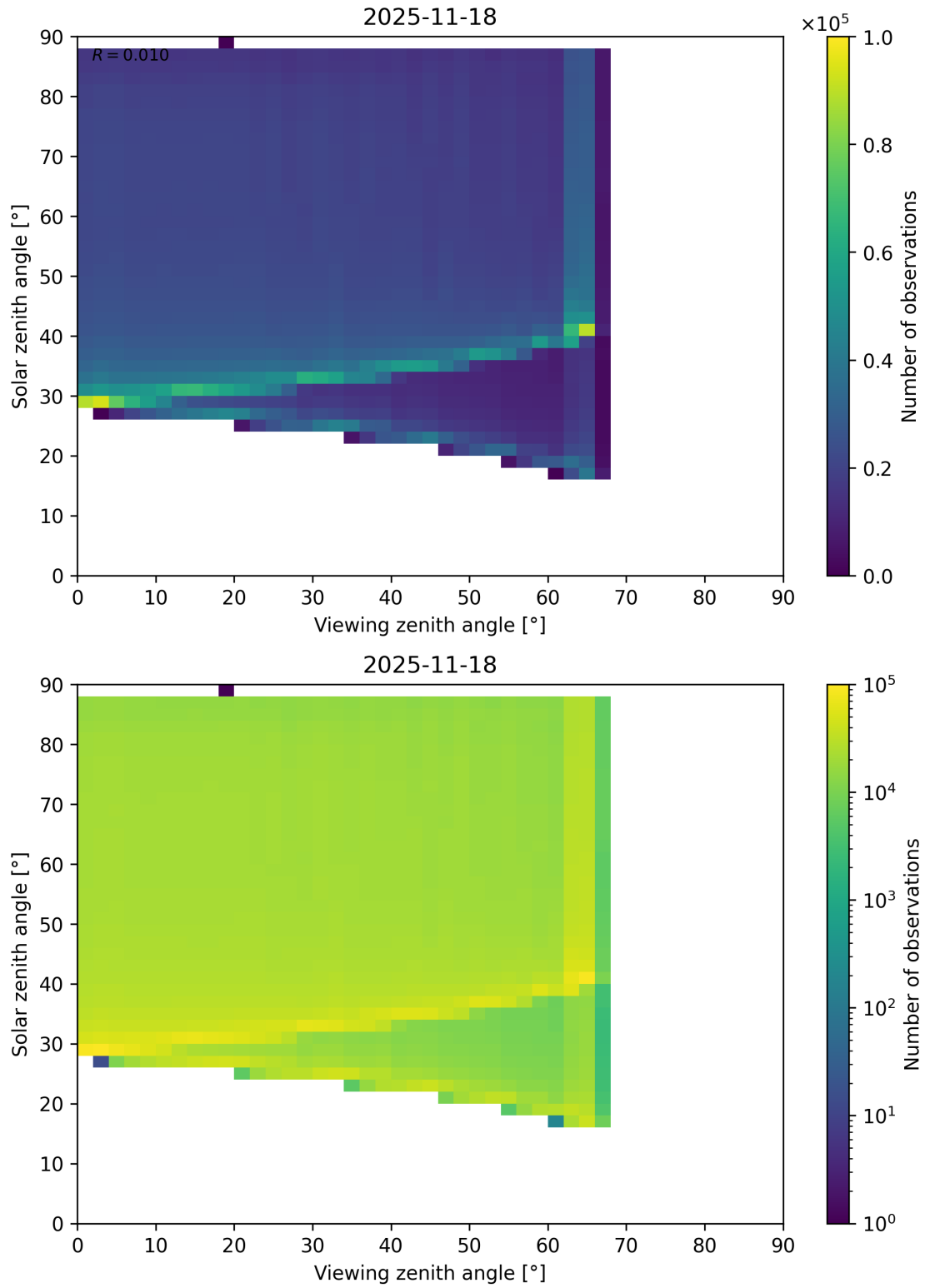
Figure 127: Scatter density plot of “Viewing zenith angle” against “Solar zenith angle” for 2025-11-18 to 2025-11-19.
