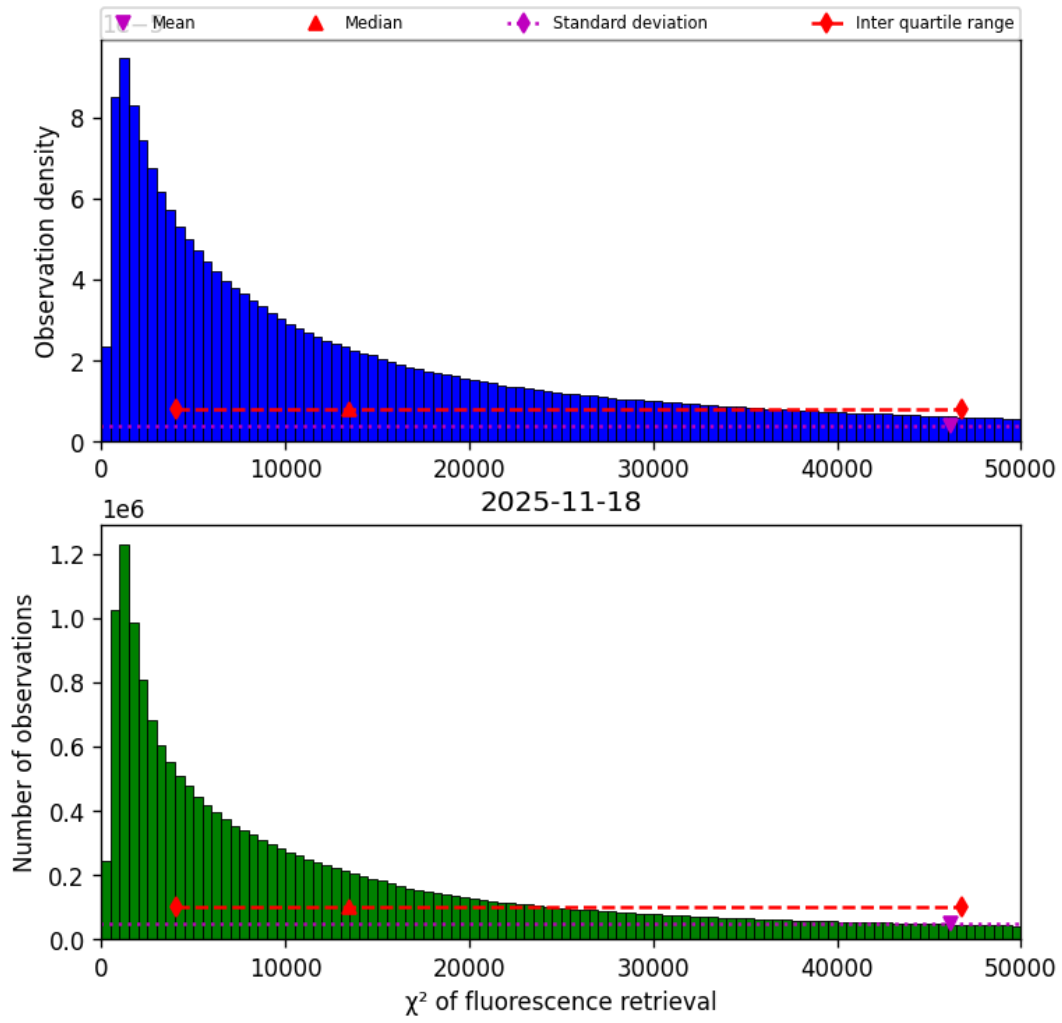
Figure 42: Histogram of “ \chi^2 of fluorescence retrieval” for 2025-11-18 to 2025-11-19
