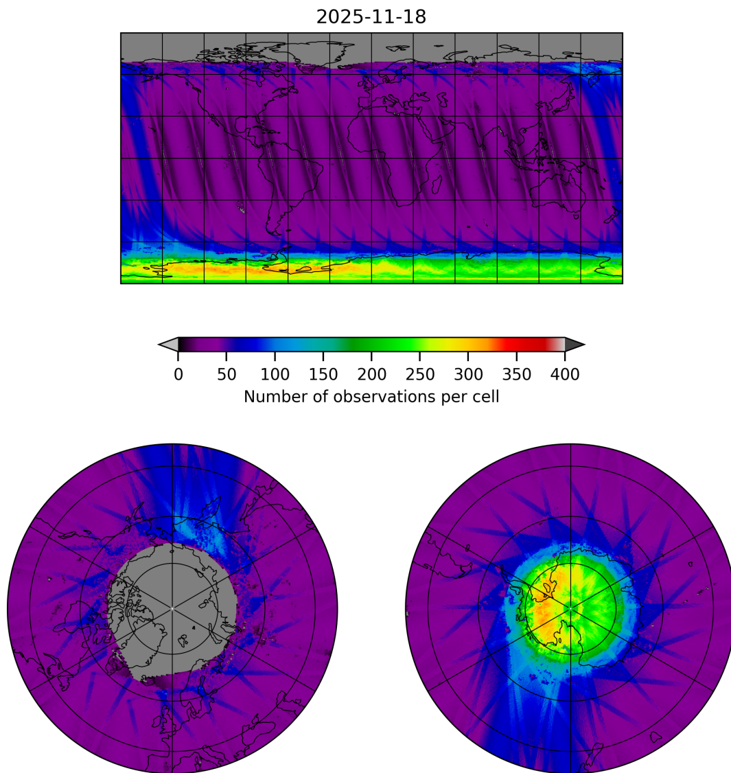
Figure 11: Map of the number of observations for 2025-11-18 to 2025-11-19
