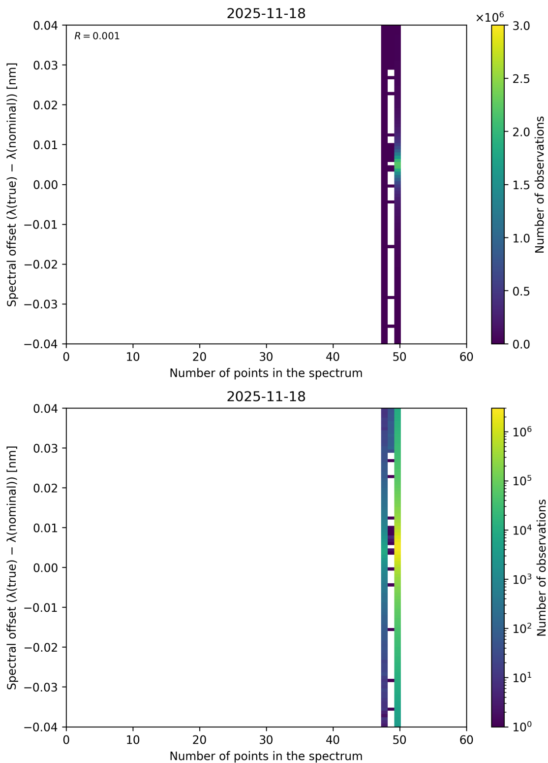
Figure 101: Scatter density plot of “Number of points in the spectrum” against “Spectral offset ( \lambda_{\text{true}} - \lambda_{\text{nominal}} )” for 2025-11-18 to 2025-11-19.
