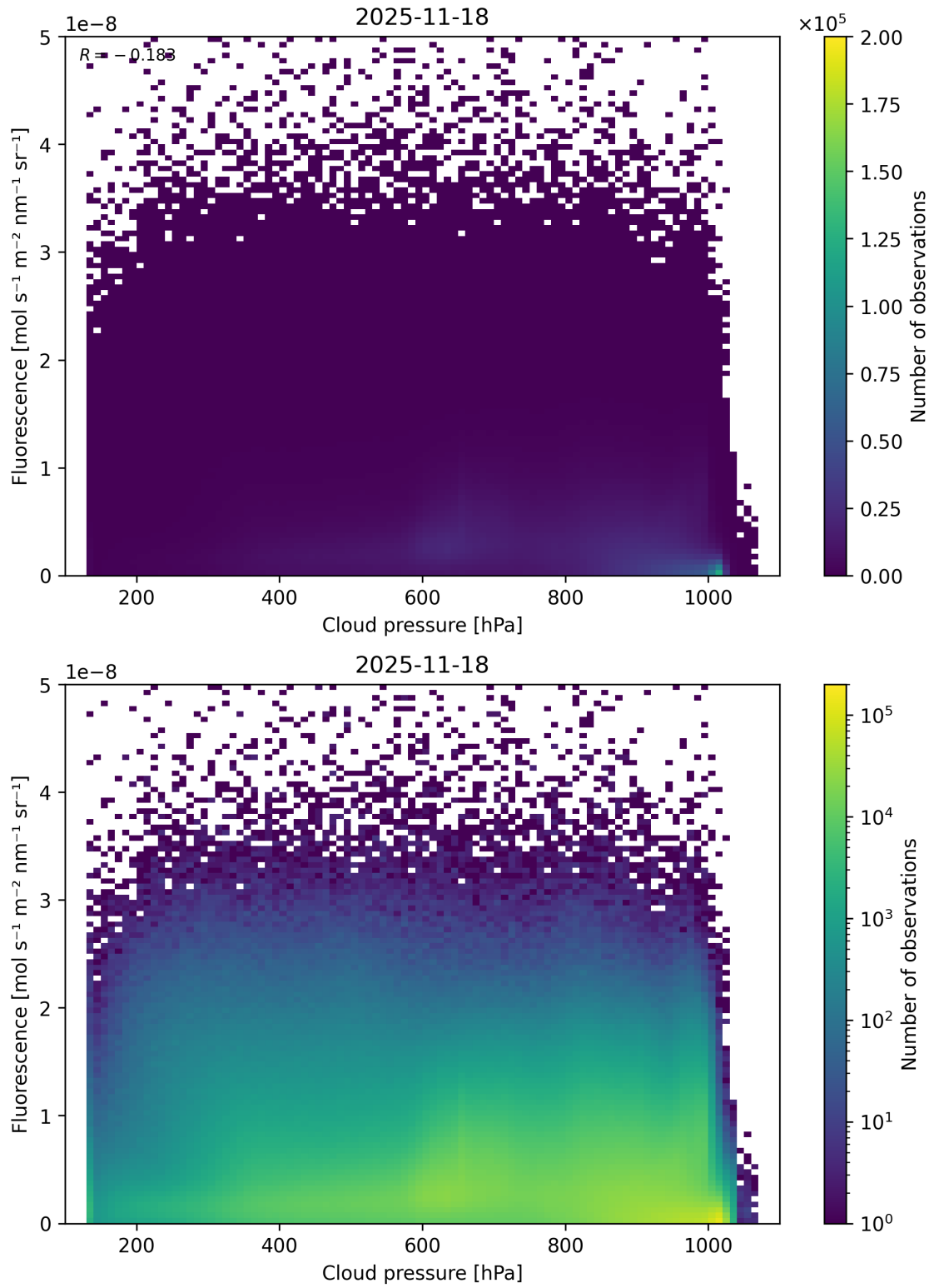
Figure 80: Scatter density plot of “Cloud pressure” against “Fluorescence” for 2025-11-18 to 2025-11-19.
