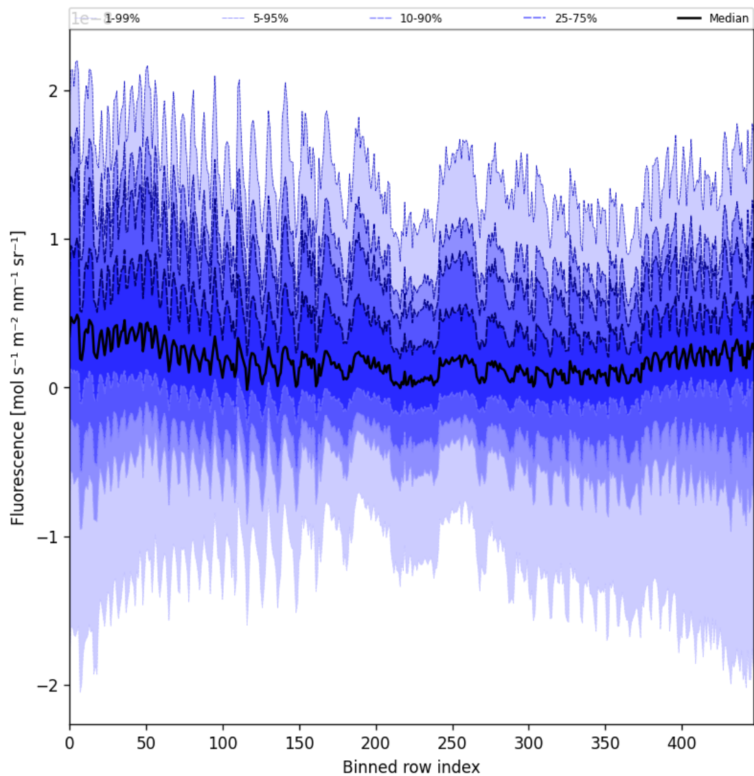
Figure 57: Along track statistics of “Fluorescence” for 2025-11-18 to 2025-11-19
