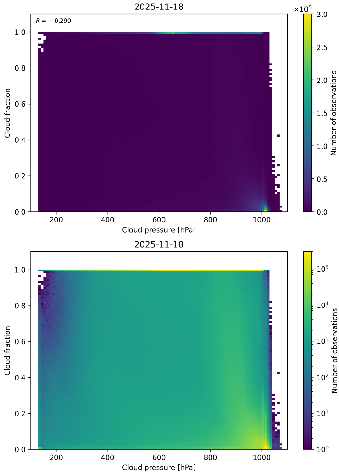
Figure 79: Scatter density plot of “Cloud pressure” against “Cloud fraction” for 2025-11-18 to 2025-11-19.
