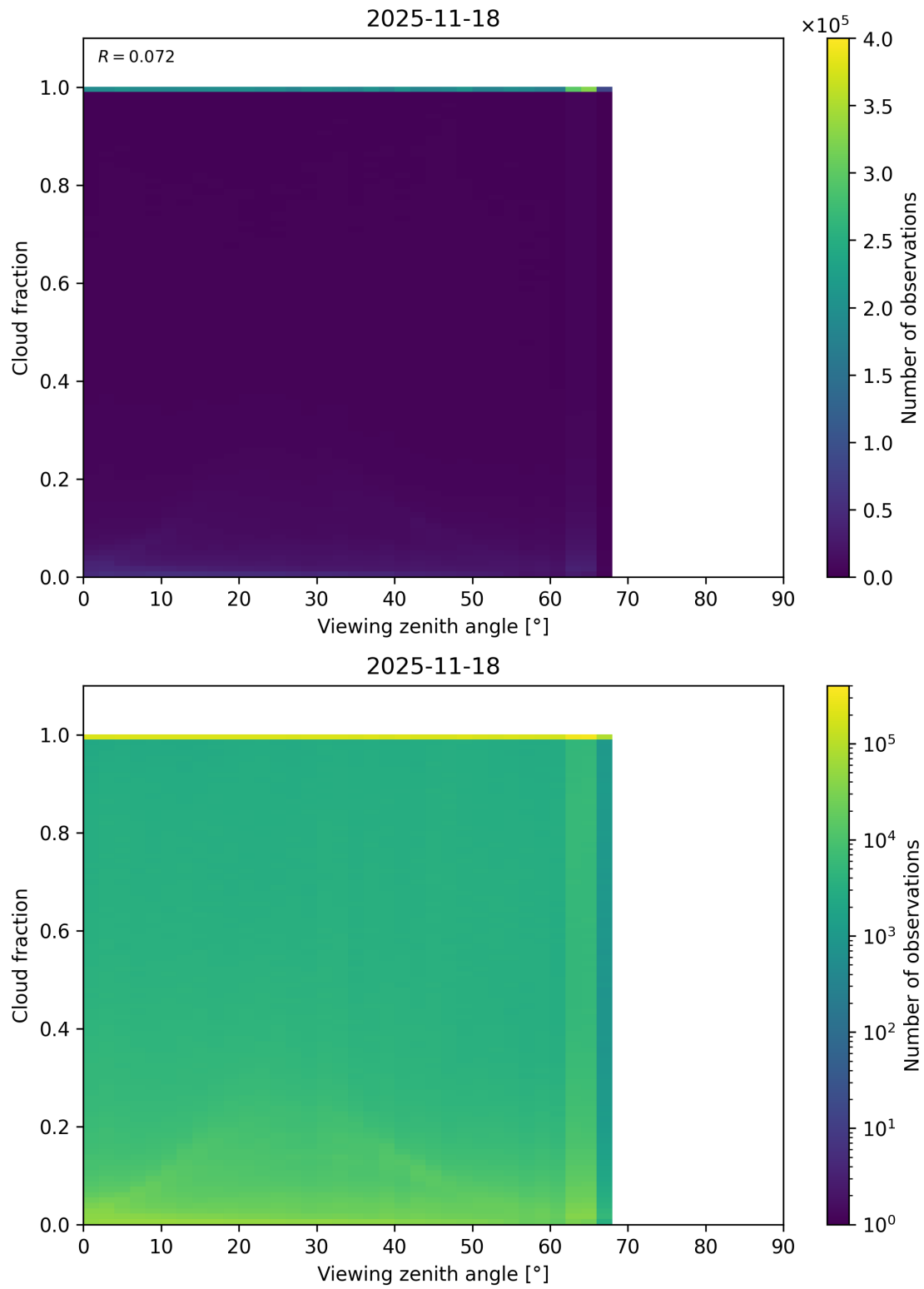
Figure 120: Scatter density plot of “Viewing zenith angle” against “Cloud fraction” for 2025-11-18 to 2025-11-19.
