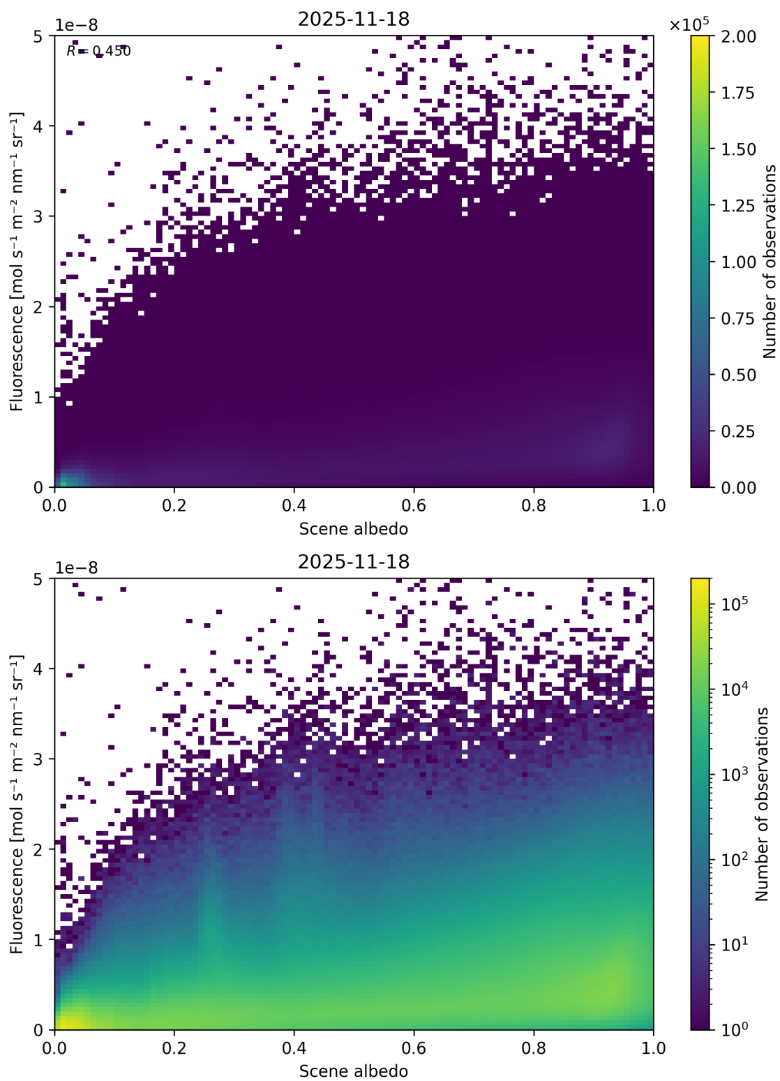
Figure 104: Scatter density plot of “Scene albedo” against “Fluorescence” for 2025-11-18 to 2025-11-19.
