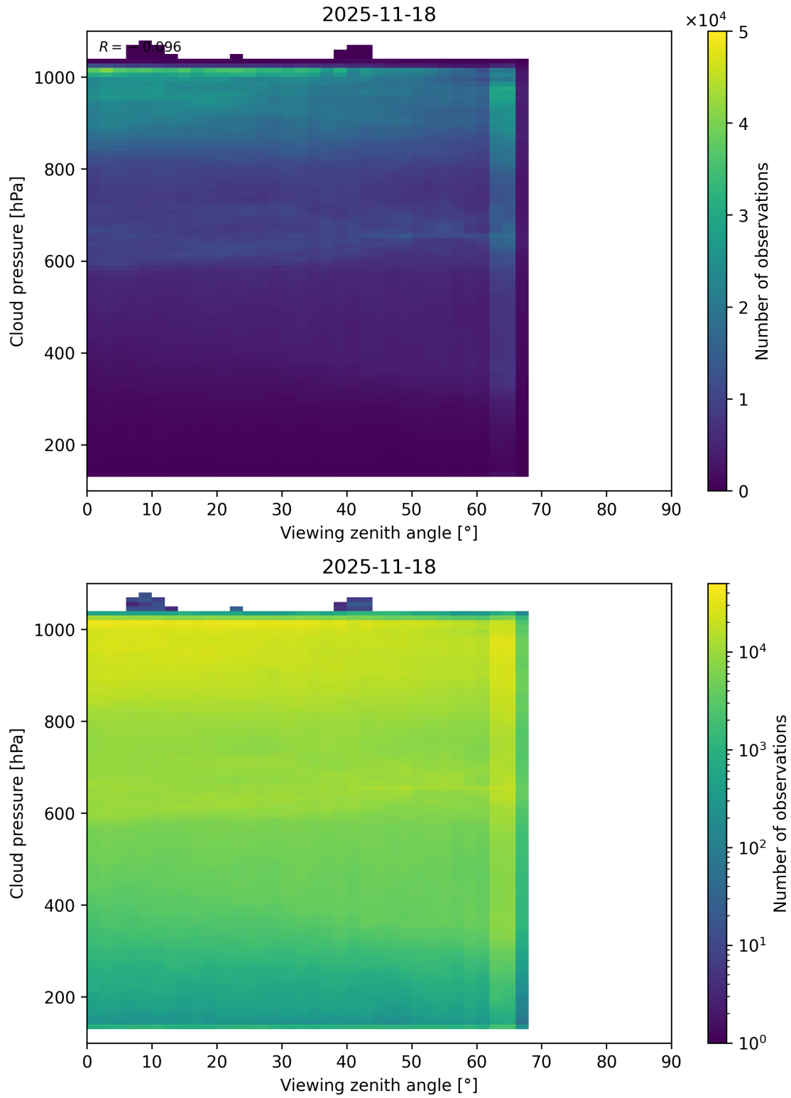
Figure 121: Scatter density plot of “Viewing zenith angle” against “Cloud pressure” for 2025-11-18 to 2025-11-19.
