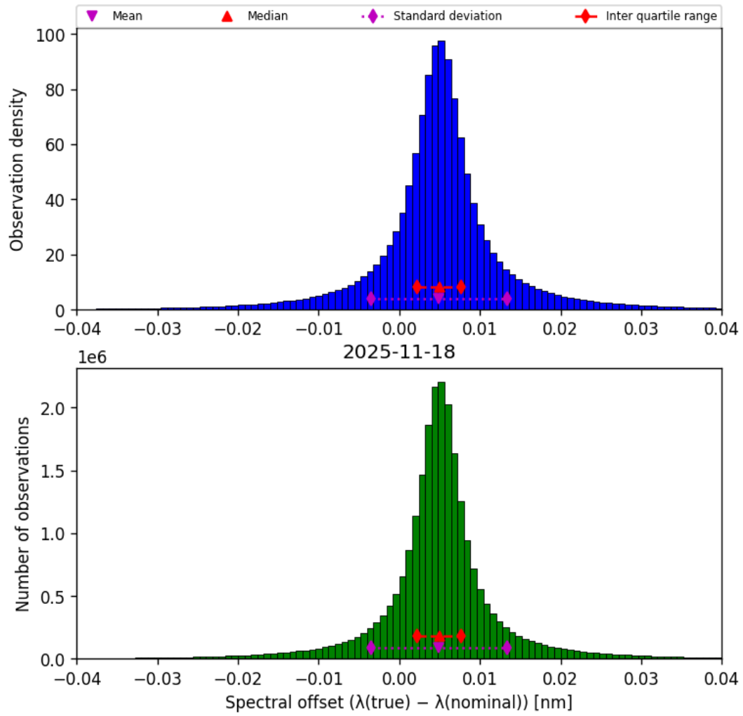
Figure 45: Histogram of “Spectral offset ( \lambda_{\text{true}} - \lambda_{\text{nominal}} )” for 2025-11-18 to 2025-11-19
