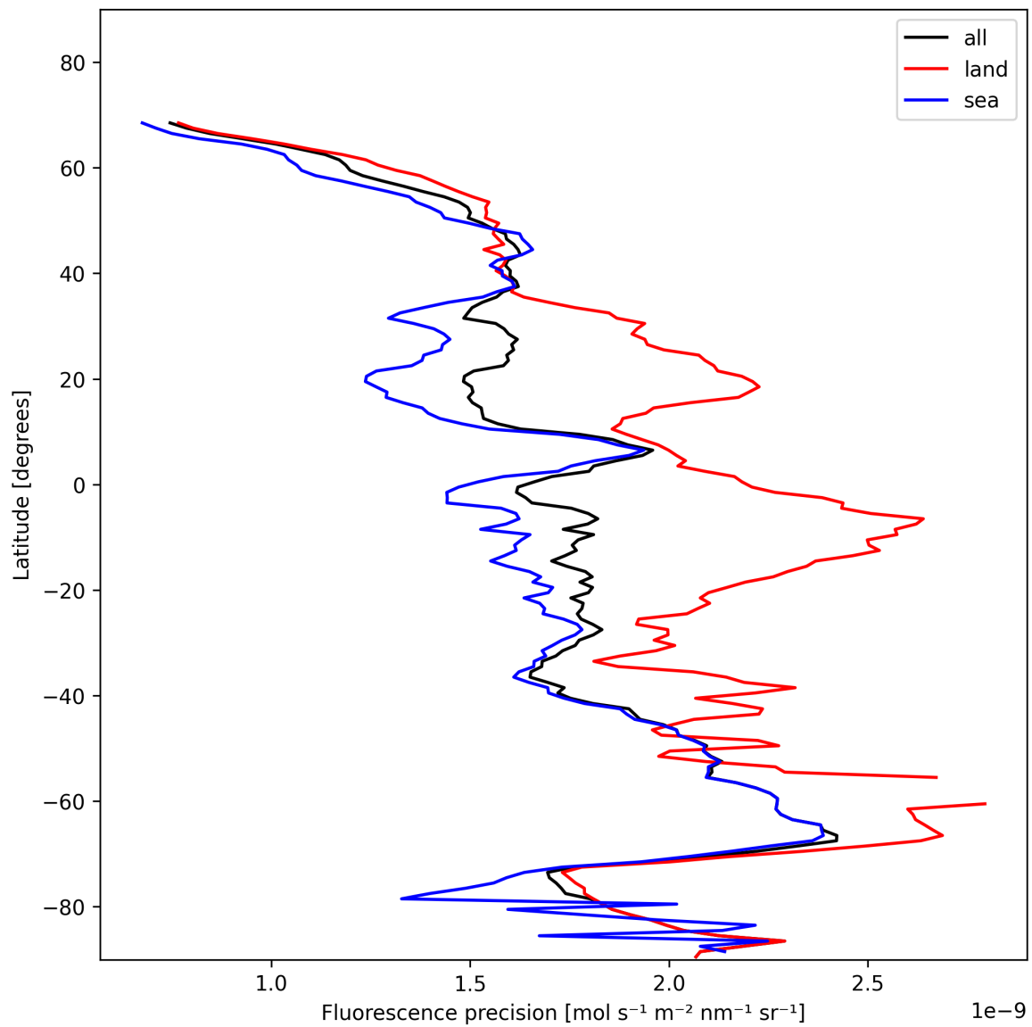
Figure 24: Zonal average of “Fluorescence precision” for 2025-11-18 to 2025-11-19.
