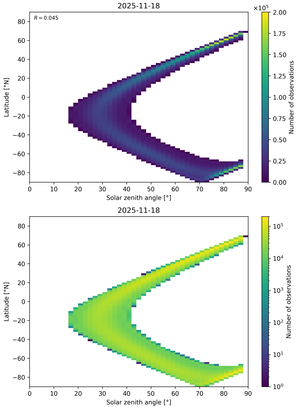
Figure 113: Scatter density plot of “Solar zenith angle” against “Latitude” for 2025-11-18 to 2025-11-19.
