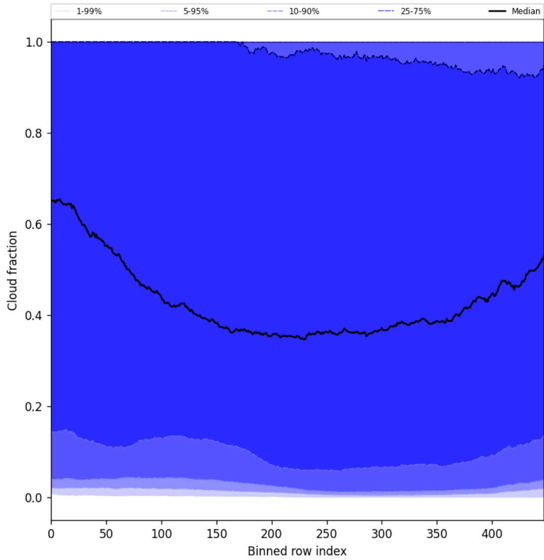
Figure 49: Along track statistics of “Cloud fraction” for 2025-11-18 to 2025-11-19
