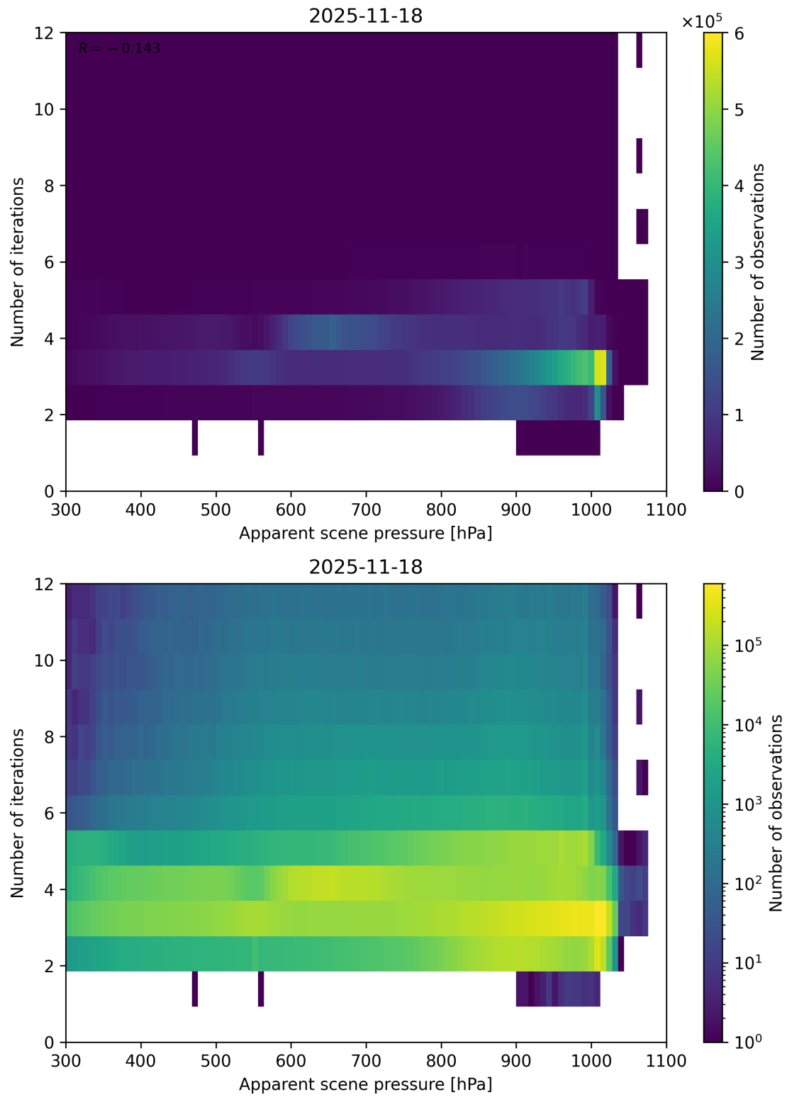
Figure 65: Scatter density plot of “Apparent scene pressure” against “Number of iterations” for 2025-11-18 to 2025-11-19.
