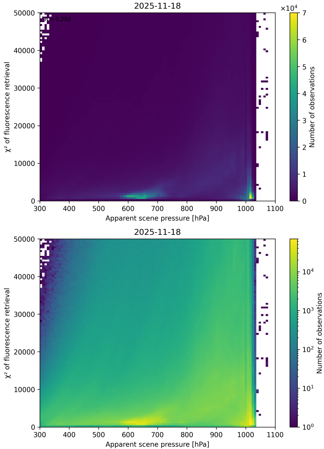
Figure 63: Scatter density plot of “Apparent scene pressure” against “ \chi^2 of fluorescence retrieval” for 2025-11-18 to 2025-11-19.
