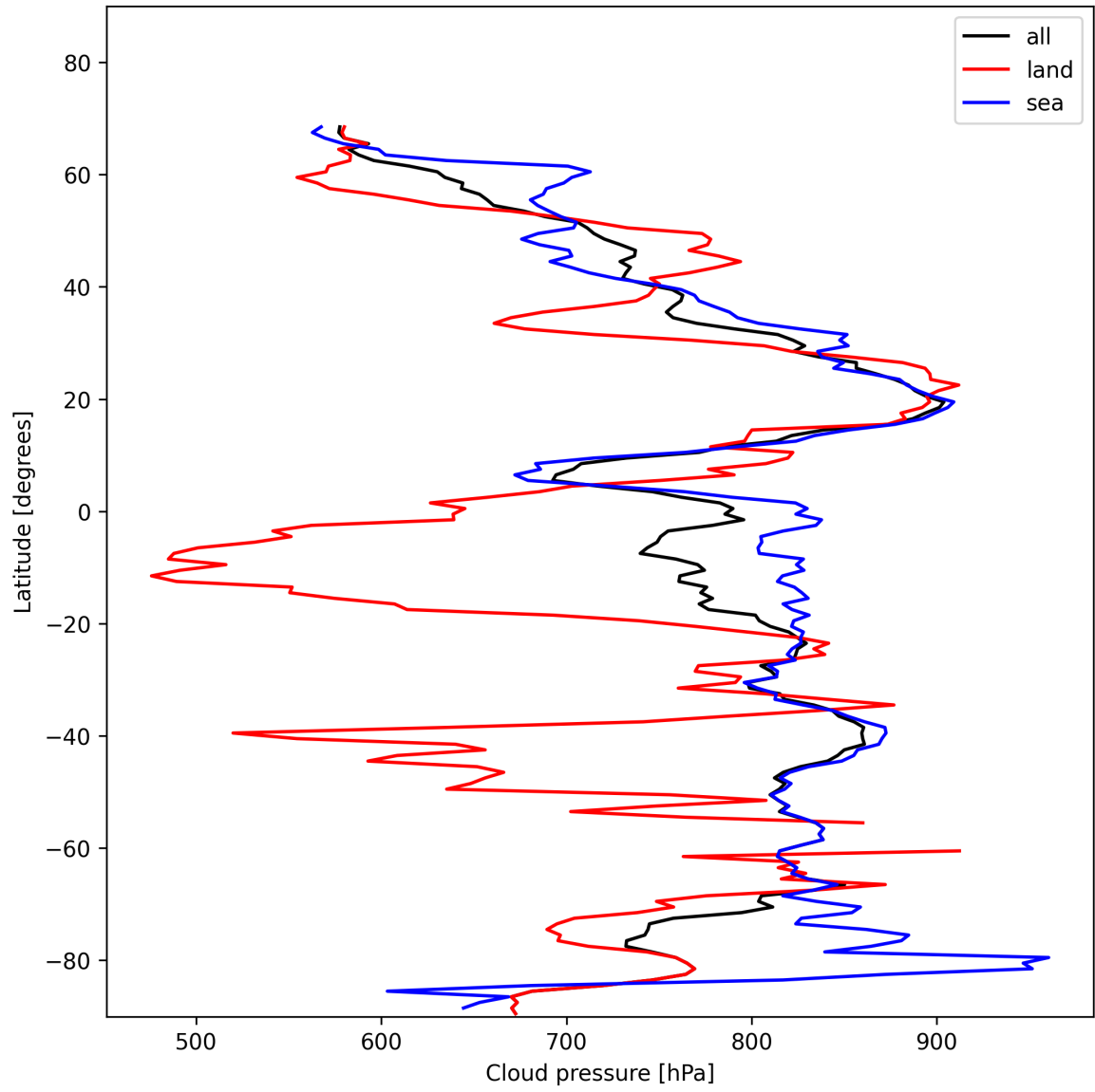
Figure 13: Zonal average of “Cloud pressure” for 2025-11-18 to 2025-11-19.
