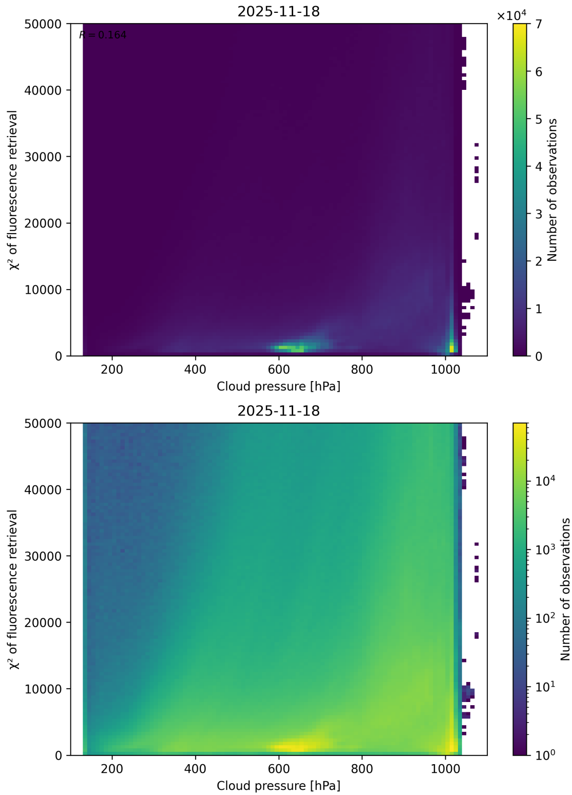
Figure 78: Scatter density plot of “Cloud pressure” against “ \chi^2 of fluorescence retrieval” for 2025-11-18 to 2025-11-19.
