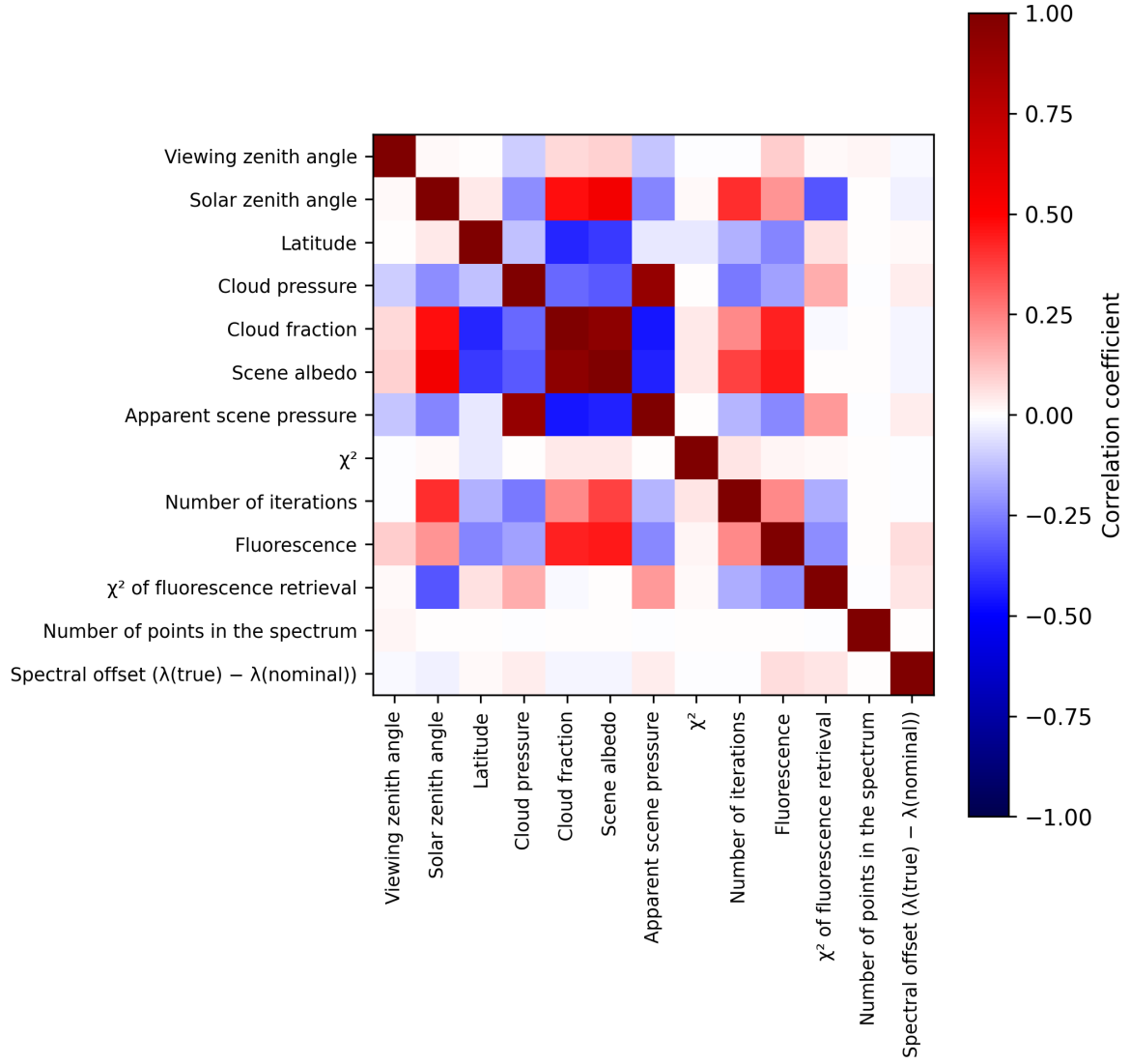
Figure 2: Map of correlation matrix for 2025-11-18 to 2025-11-19.
