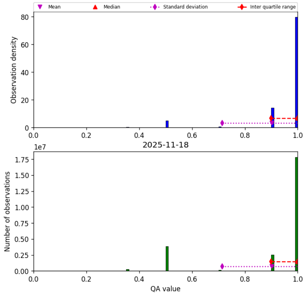
Figure 29: Histogram of “QA value” for 2025-11-18 to 2025-11-19
