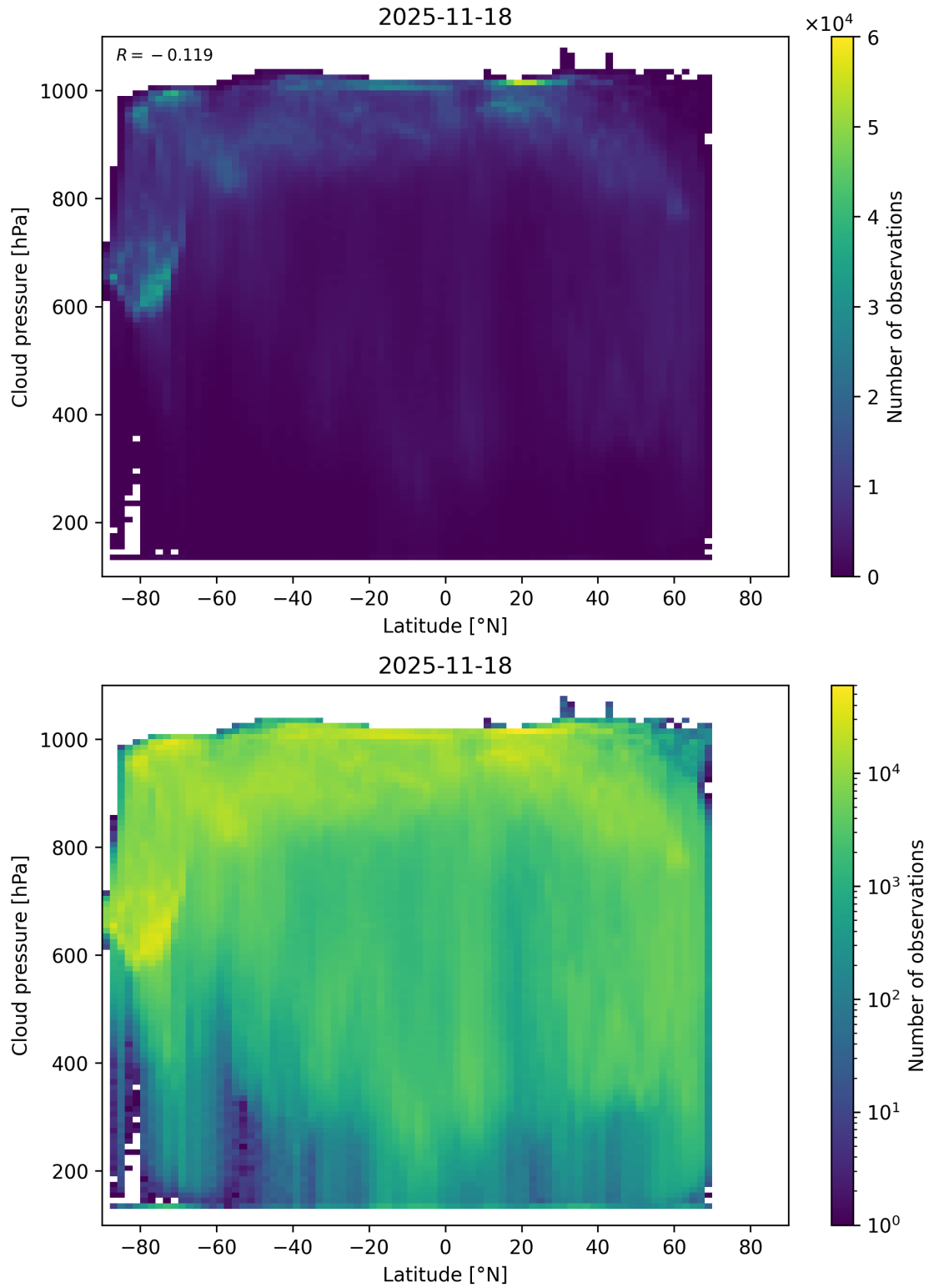
Figure 91: Scatter density plot of “Latitude” against “Cloud pressure” for 2025-11-18 to 2025-11-19.
