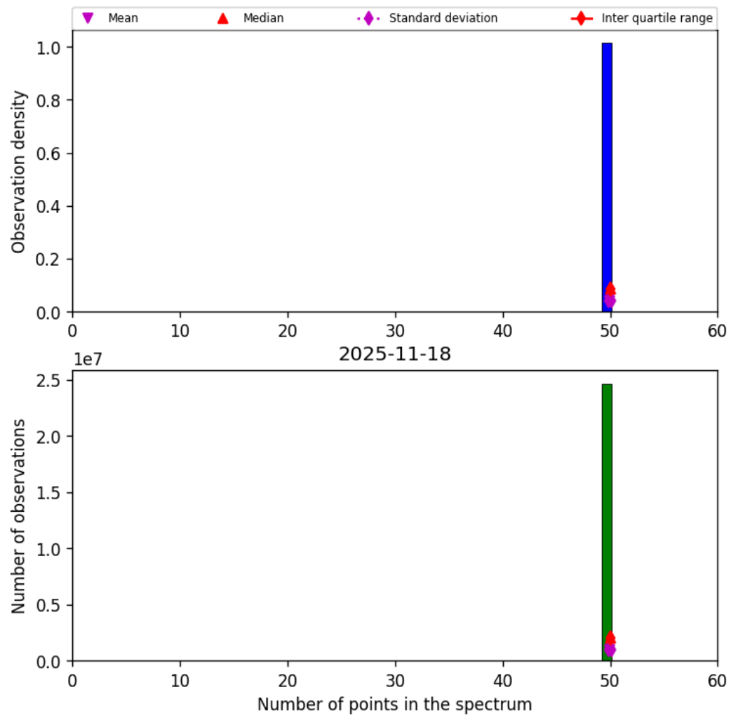
Figure 44: Histogram of “Number of points in the spectrum” for 2025-11-18 to 2025-11-19
