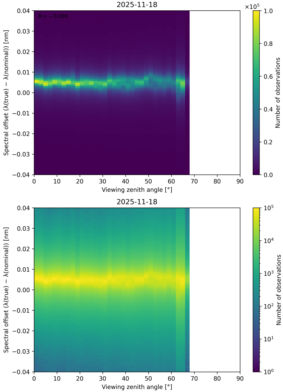
Figure 128: Scatter density plot of “Viewing zenith angle” against “Spectral offset ( \lambda_{\text{true}} - \lambda_{\text{nominal}} )” for 2025-11-18 to 2025-11-19.
