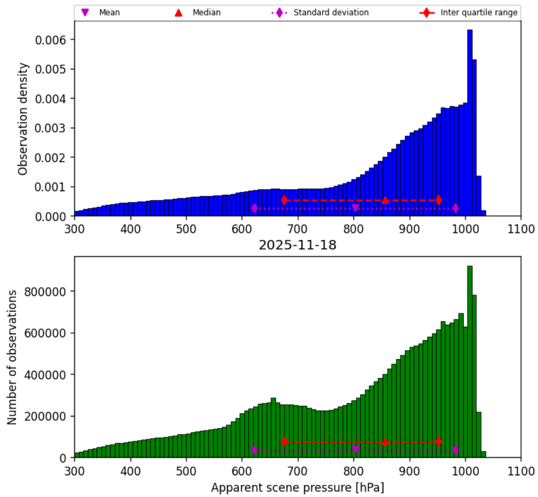
Figure 36: Histogram of “Apparent scene pressure” for 2025-11-18 to 2025-11-19
