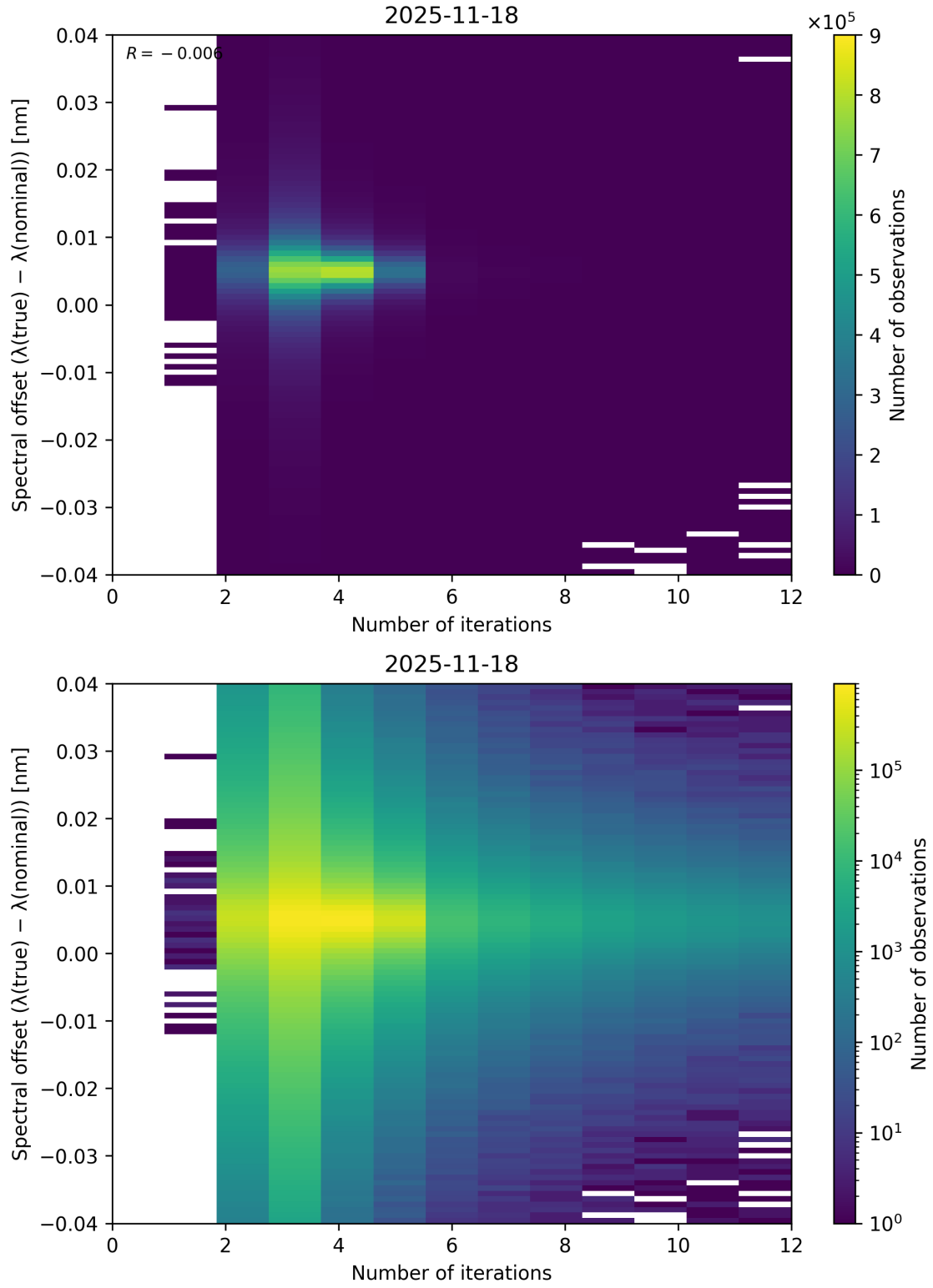
Figure 100: Scatter density plot of “Number of iterations” against “Spectral offset ( \lambda_{\text{true}} - \lambda_{\text{nominal}} )” for 2025-11-18 to 2025-11-19.
