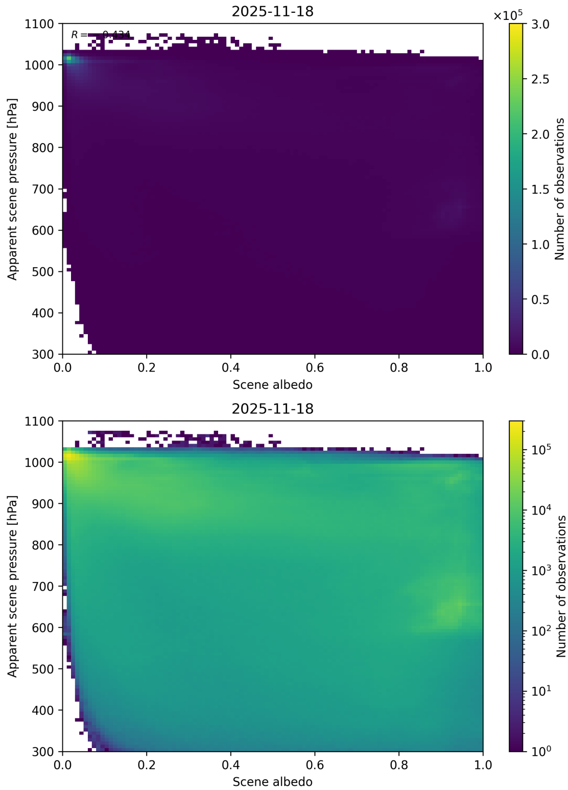
Figure 102: Scatter density plot of “Scene albedo” against “Apparent scene pressure” for 2025-11-18 to 2025-11-19.
