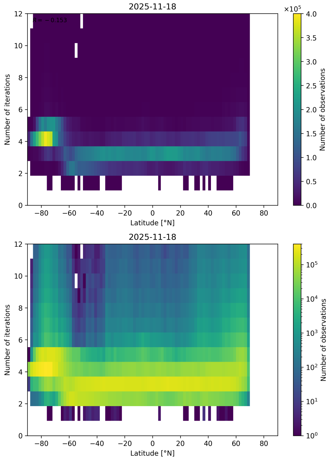
Figure 93: Scatter density plot of “Latitude” against “Number of iterations” for 2025-11-18 to 2025-11-19.
