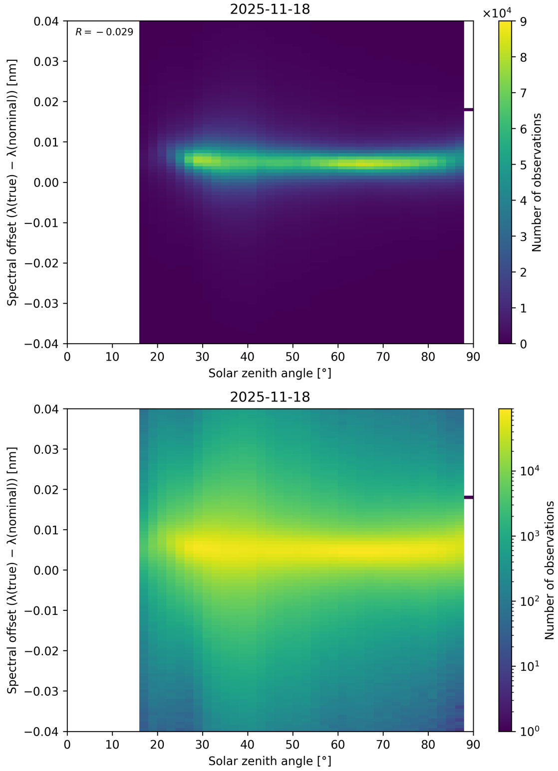
Figure 117: Scatter density plot of “Solar zenith angle” against “Spectral offset ( \lambda_{\text{true}} - \lambda_{\text{nominal}} )” for 2025-11-18 to 2025-11-19.
