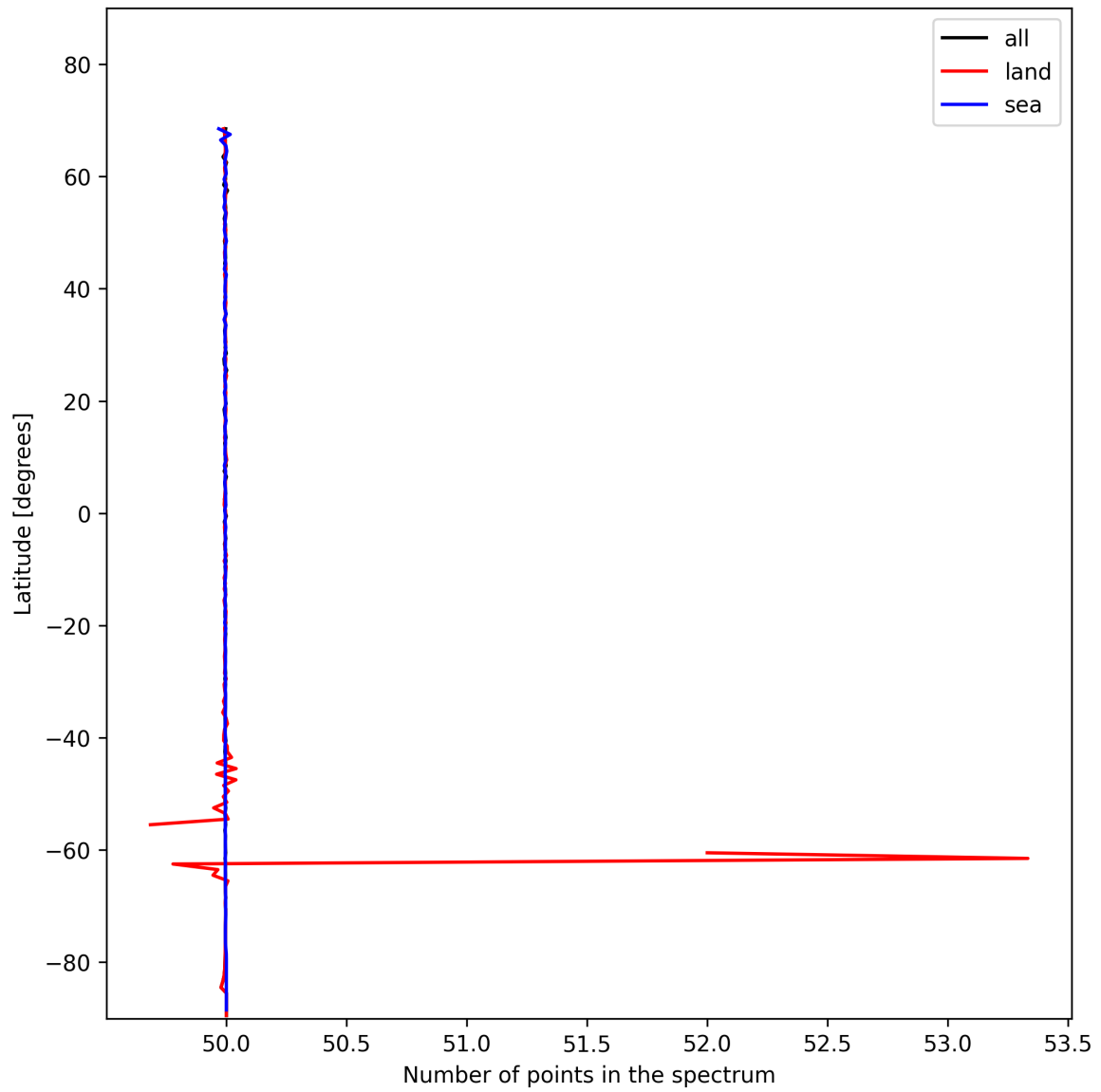
Figure 27: Zonal average of “Number of points in the spectrum” for 2025-11-18 to 2025-11-19.
