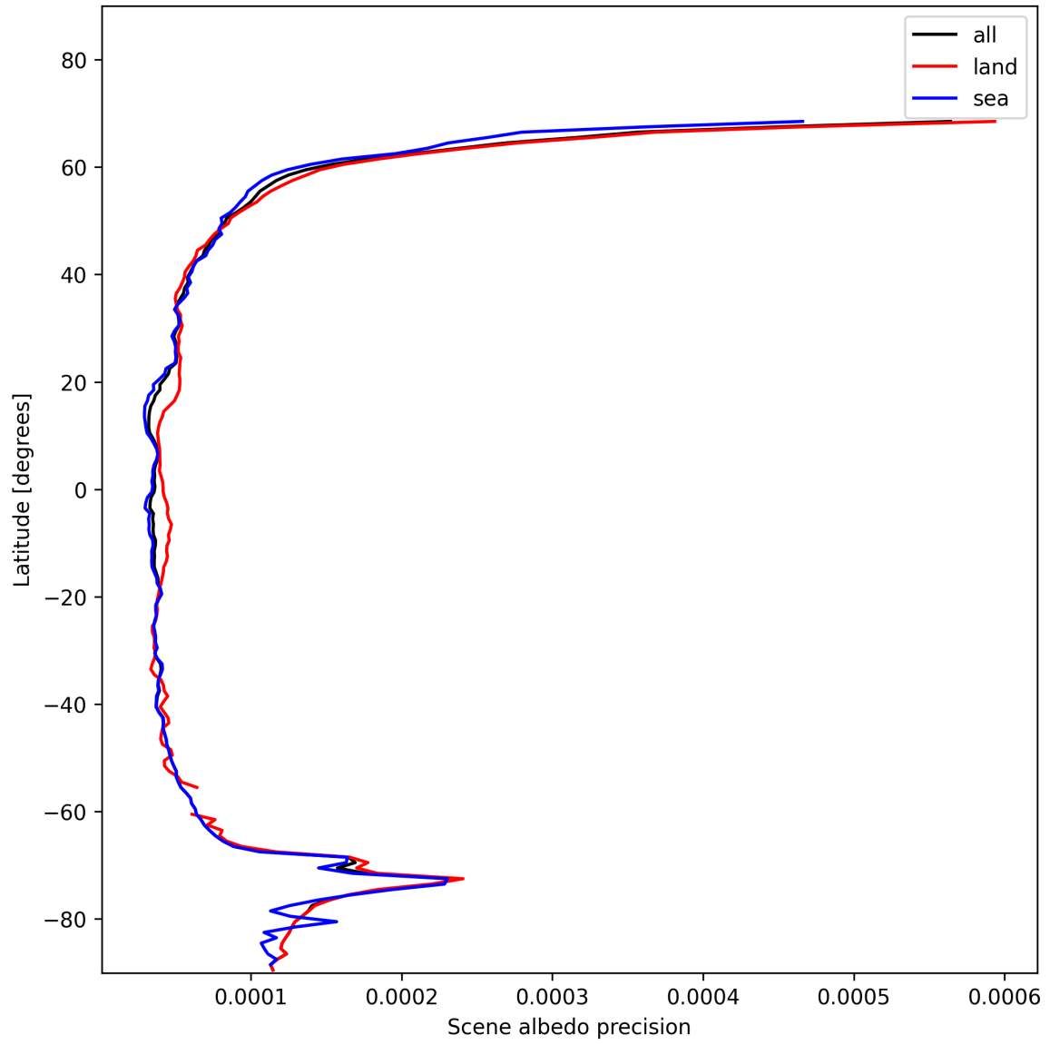
Figure 18: Zonal average of “Scene albedo precision” for 2025-11-18 to 2025-11-19.
