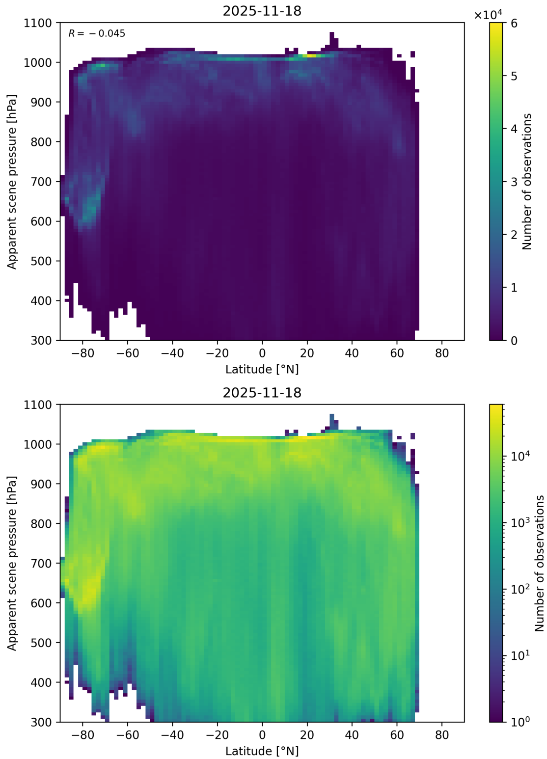
Figure 88: Scatter density plot of “Latitude” against “Apparent scene pressure” for 2025-11-18 to 2025-11-19.
