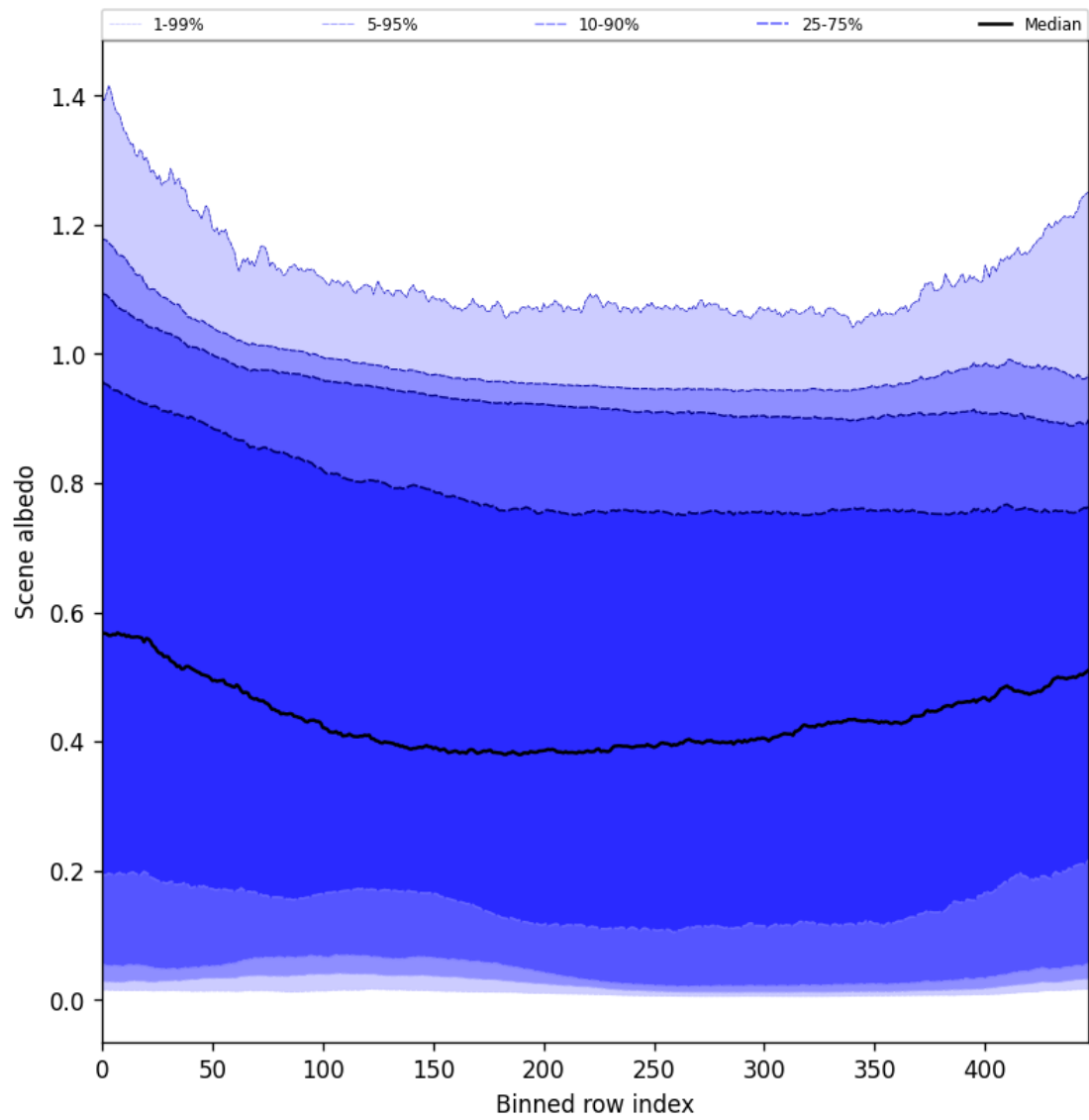
Figure 51: Along track statistics of “Scene albedo” for 2025-11-18 to 2025-11-19
