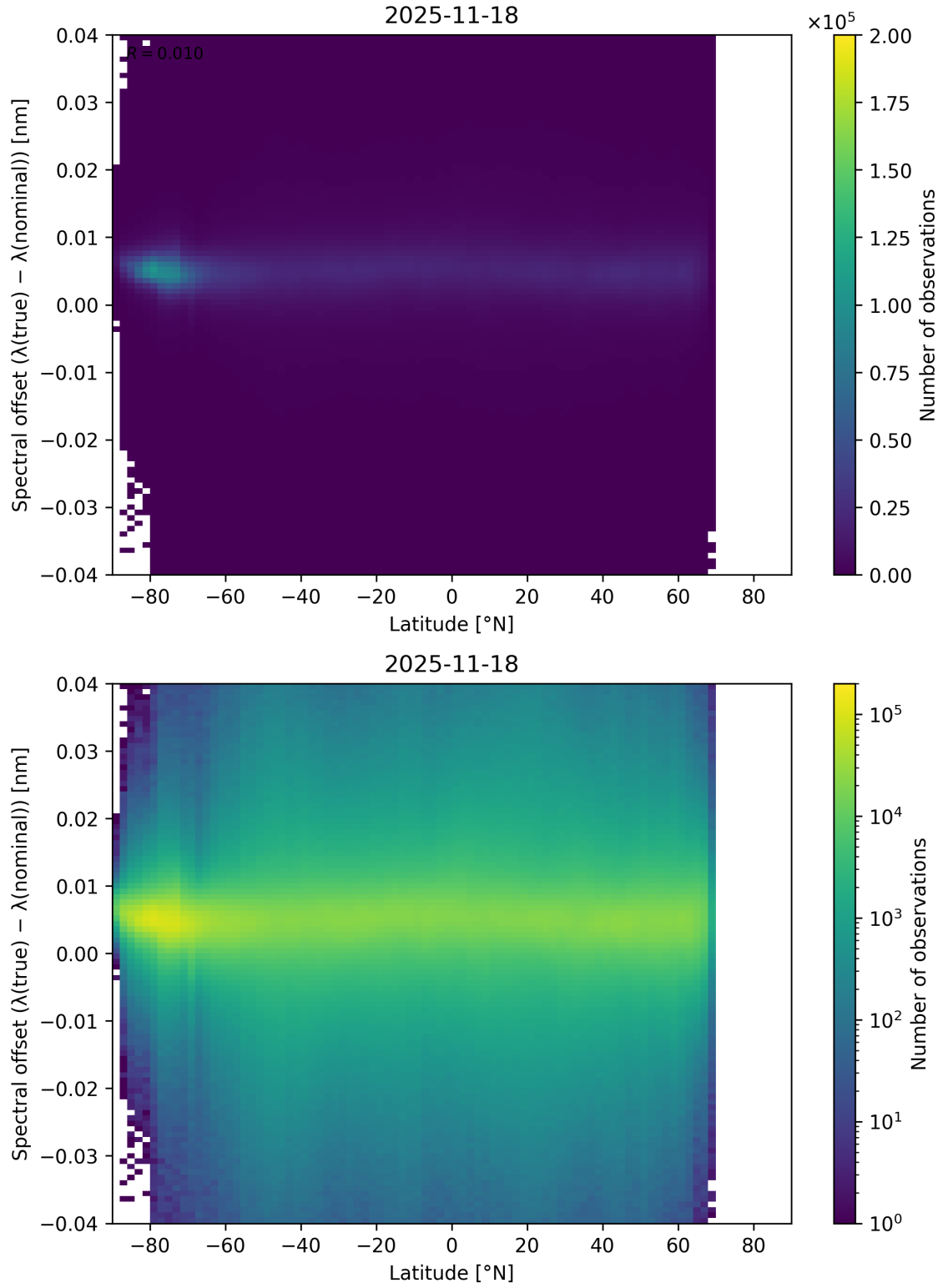
Figure 96: Scatter density plot of “Latitude” against “Spectral offset ( \lambda_{\text{true}} - \lambda_{\text{nominal}} )” for 2025-11-18 to 2025-11-19.
