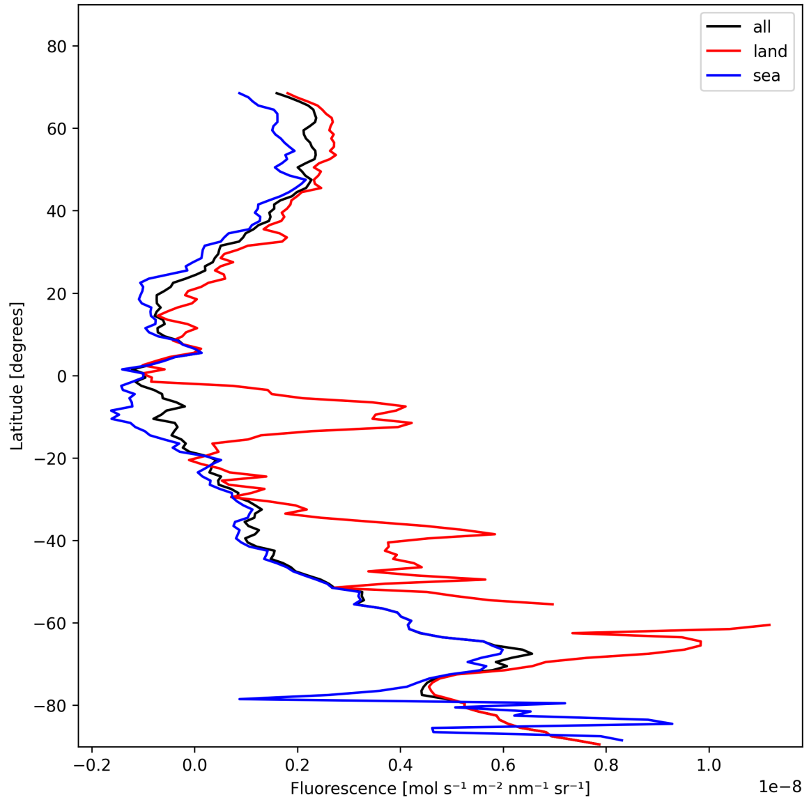
Figure 23: Zonal average of “Fluorescence” for 2025-11-18 to 2025-11-19.
