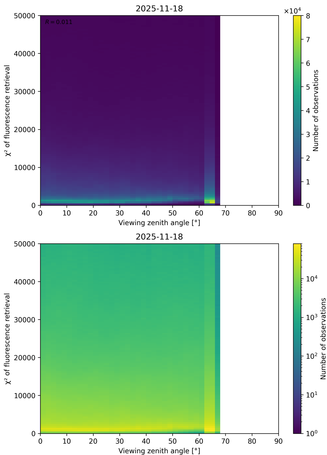
Figure 119: Scatter density plot of “Viewing zenith angle” against “ \chi^2 of fluorescence retrieval” for 2025-11-18 to 2025-11-19.
