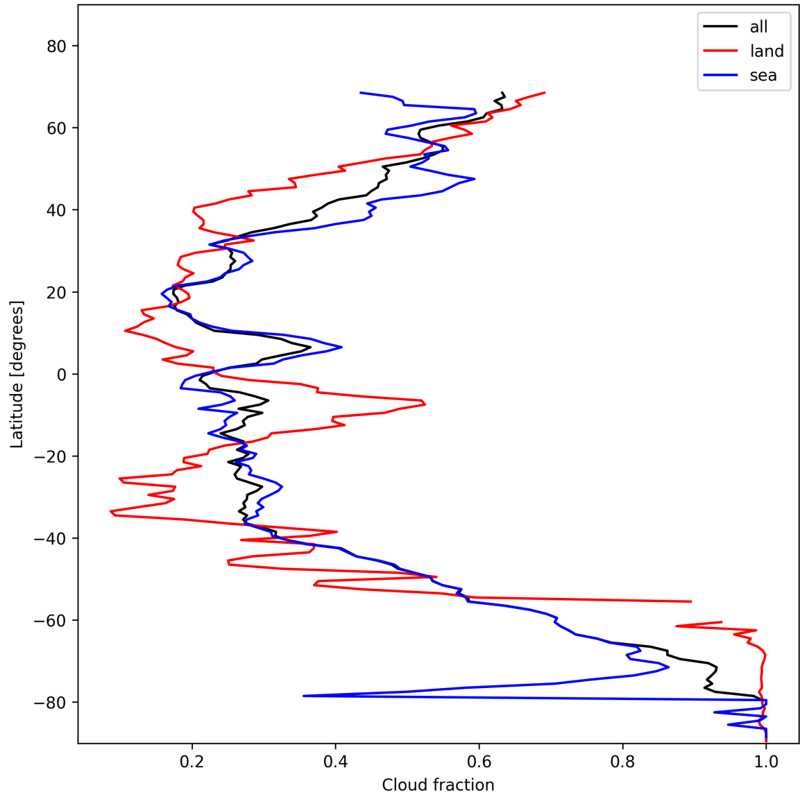
Figure 15: Zonal average of “Cloud fraction” for 2025-11-18 to 2025-11-19.
