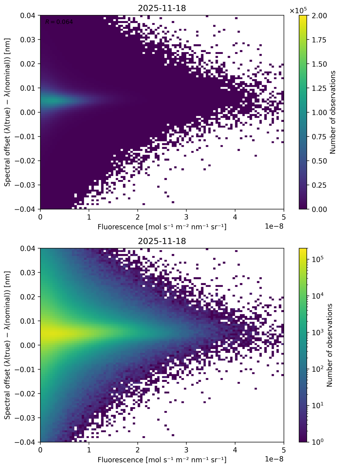
Figure 87: Scatter density plot of “Fluorescence” against “Spectral offset ( \lambda_{\text{true}} - \lambda_{\text{nominal}} )” for 2025-11-18 to 2025-11-19.
