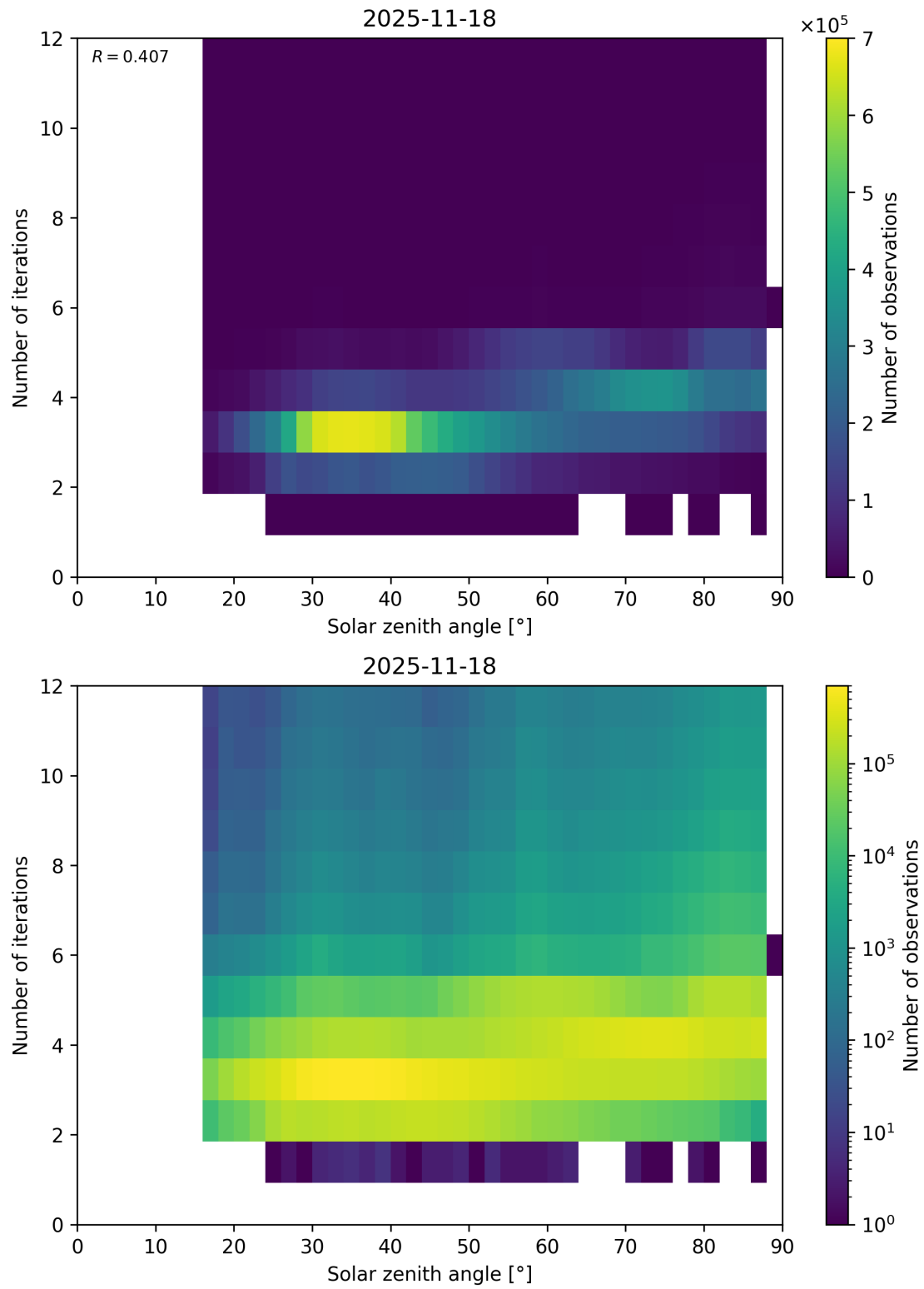
Figure 114: Scatter density plot of “Solar zenith angle” against “Number of iterations” for 2025-11-18 to 2025-11-19.
