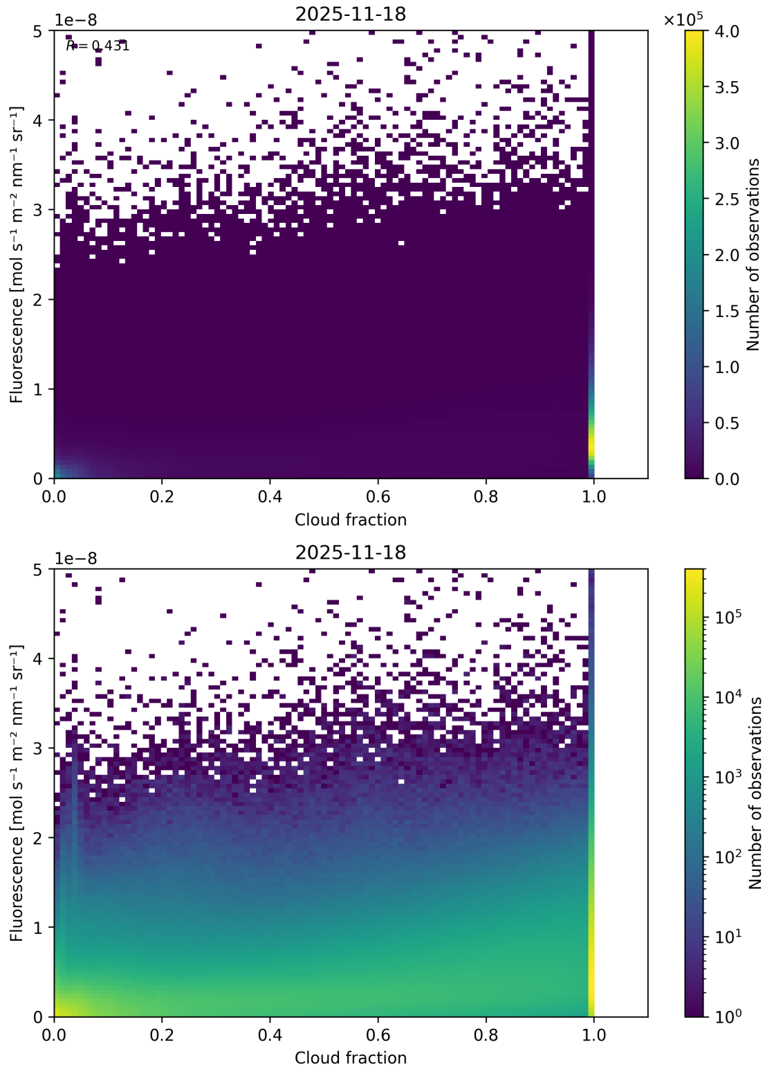
Figure 72: Scatter density plot of “Cloud fraction” against “Fluorescence” for 2025-11-18 to 2025-11-19.
