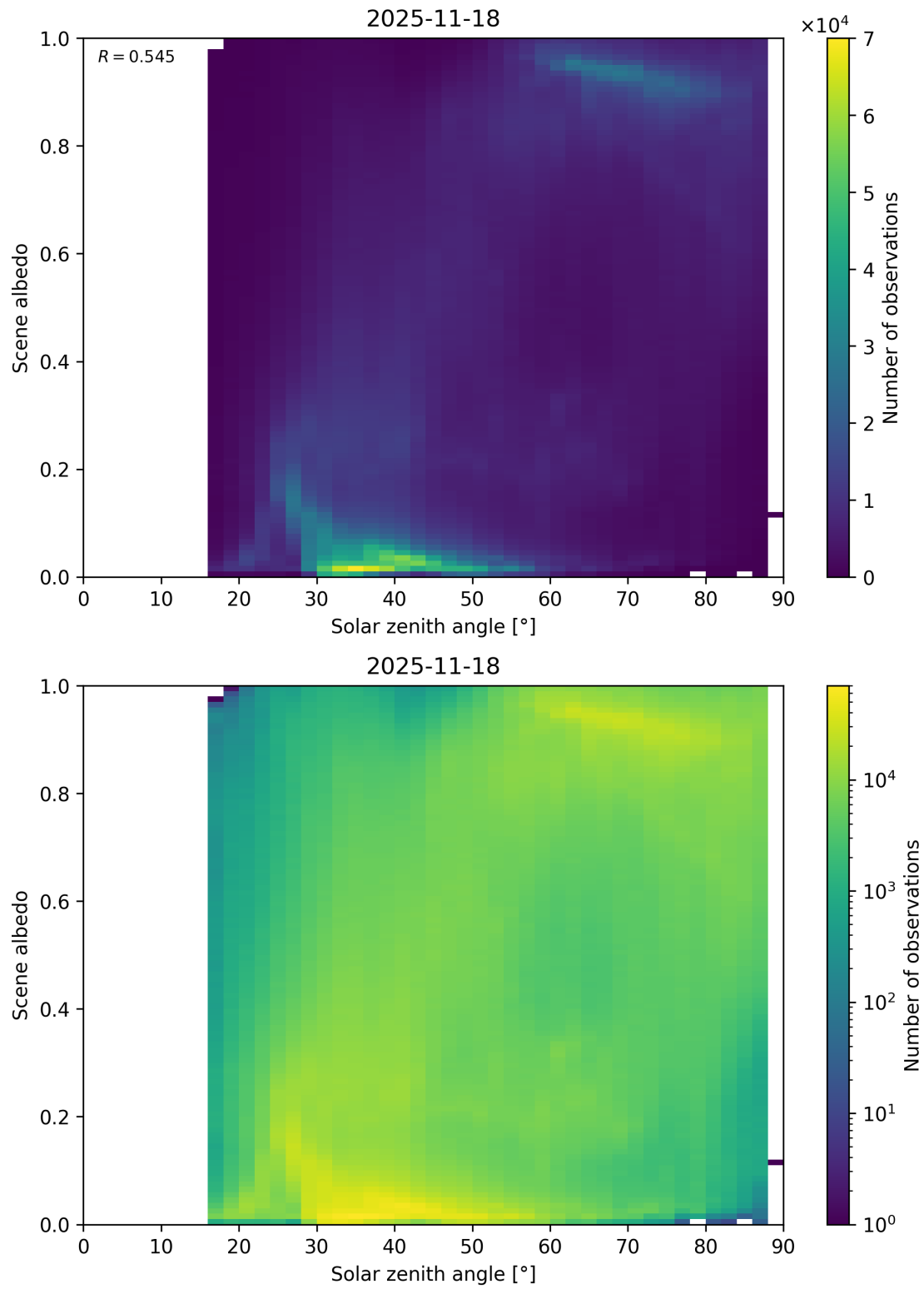
Figure 116: Scatter density plot of “Solar zenith angle” against “Scene albedo” for 2025-11-18 to 2025-11-19.
