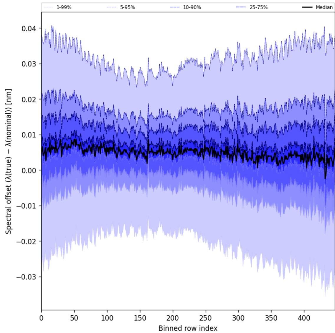
Figure 62: Along track statistics of “Spectral offset ( \lambda_{\text{true}} - \lambda_{\text{nominal}} )” for 2025-11-18 to 2025-11-19
