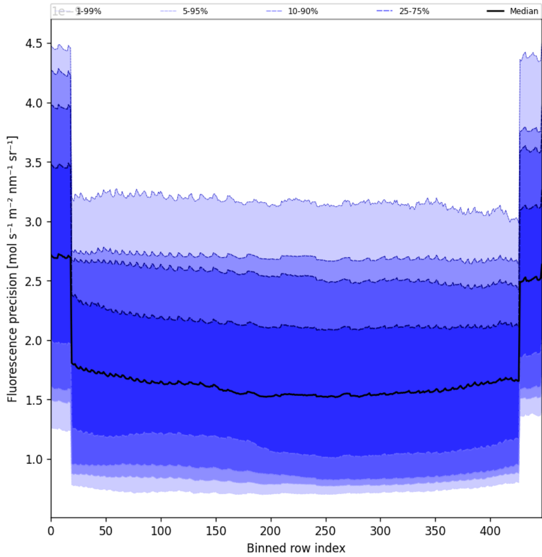
Figure 58: Along track statistics of “Fluorescence precision” for 2025-11-18 to 2025-11-19
