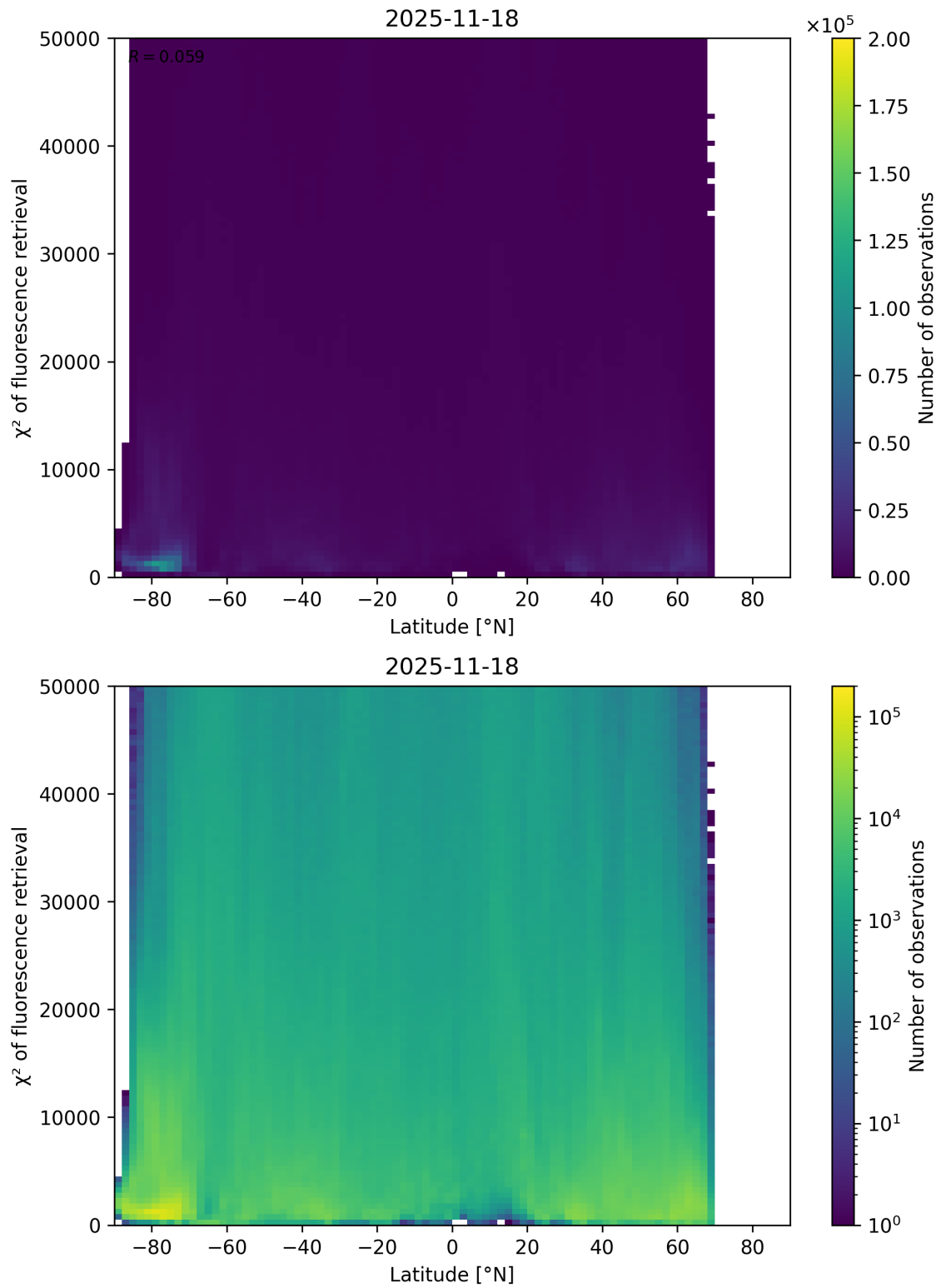
Figure 89: Scatter density plot of “Latitude” against “ \chi^2 of fluorescence retrieval” for 2025-11-18 to 2025-11-19.
