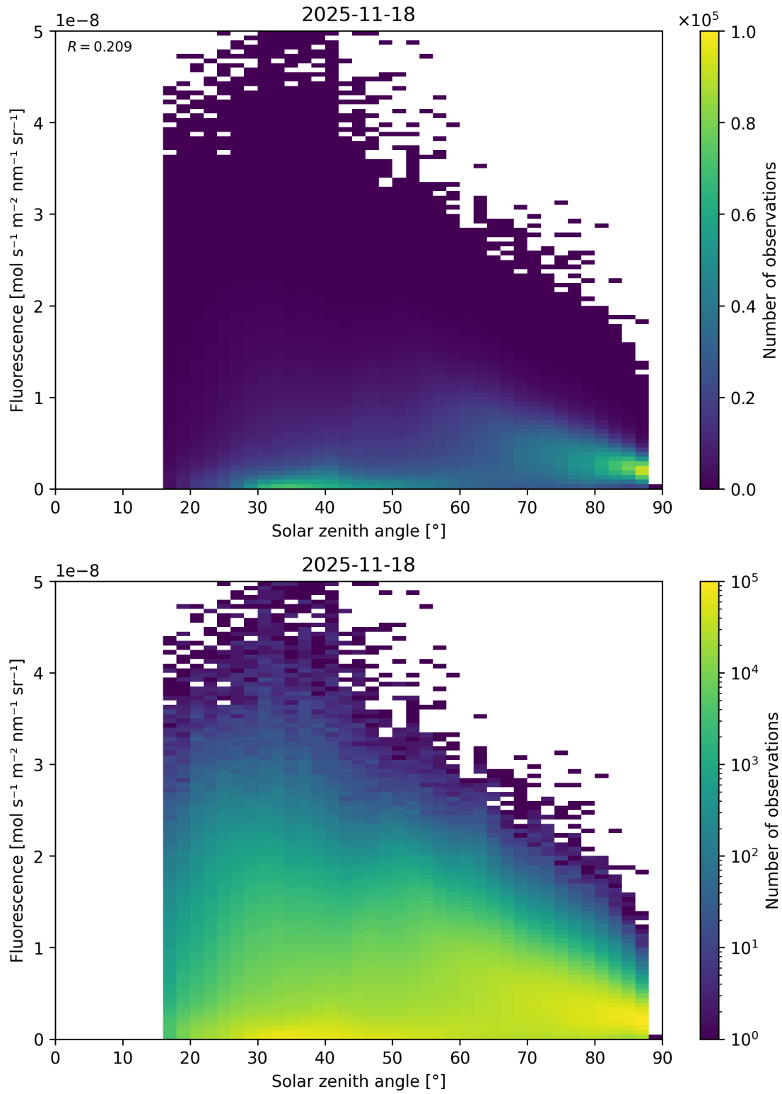
Figure 112: Scatter density plot of “Solar zenith angle” against “Fluorescence” for 2025-11-18 to 2025-11-19.
