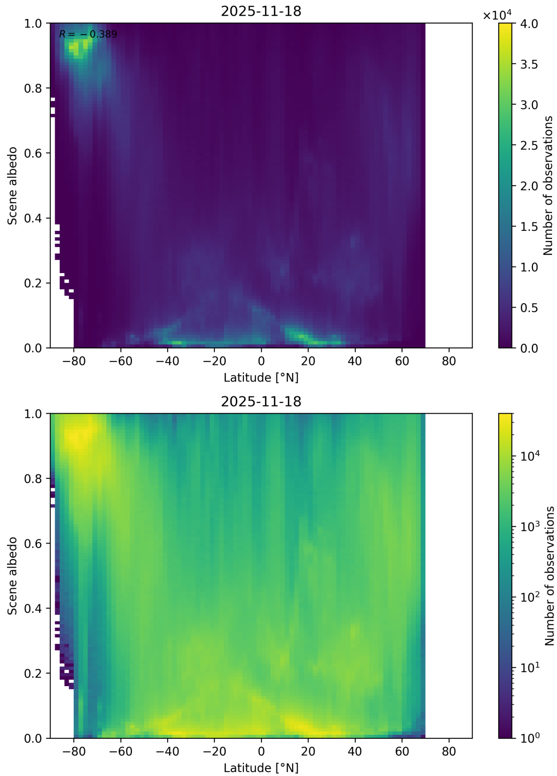
Figure 95: Scatter density plot of “Latitude” against “Scene albedo” for 2025-11-18 to 2025-11-19.
