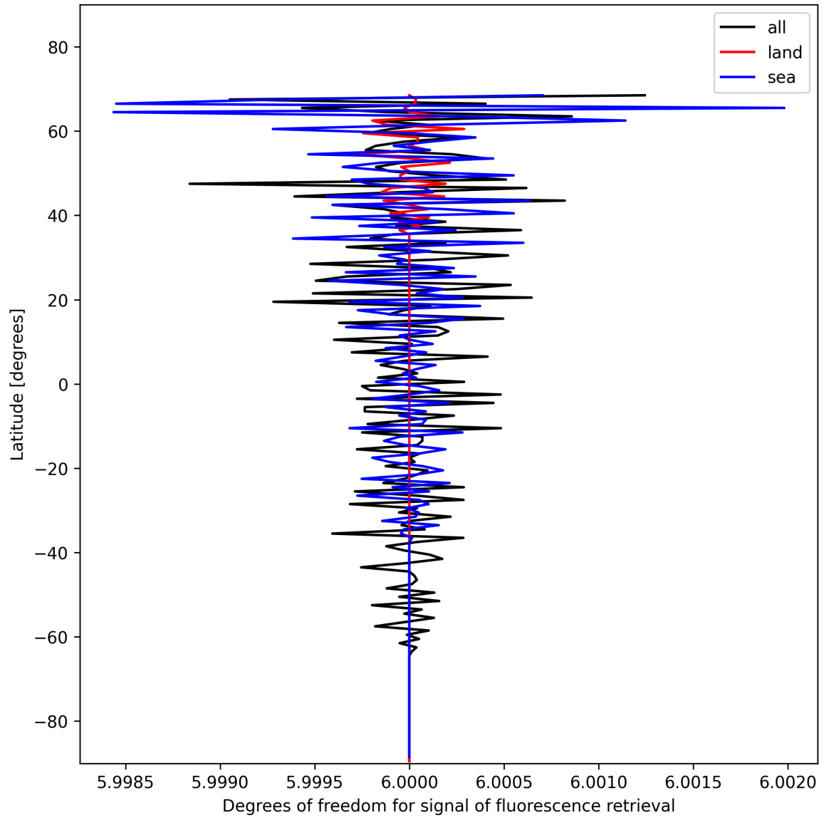
Figure 26: Zonal average of “Degrees of freedom for signal of fluorescence retrieval” for 2025-11-18 to 2025-11-19.
