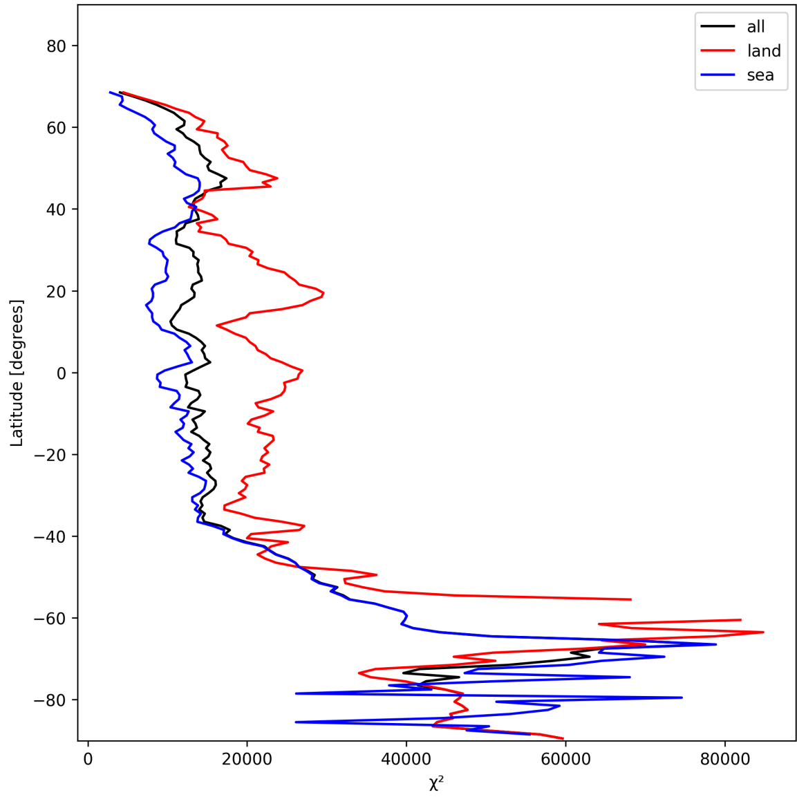
Figure 21: Zonal average of “ \chi^2 ” for 2025-11-18 to 2025-11-19.
