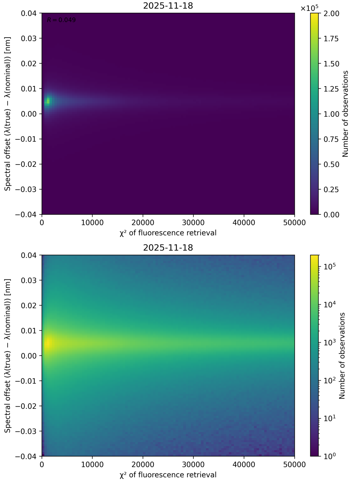
Figure 69: Scatter density plot of “ \chi^2 of fluorescence retrieval” against “Spectral offset ( \lambda_{\text{true}} - \lambda_{\text{nominal}} )” for 2025-11-18 to 2025-11-19.
