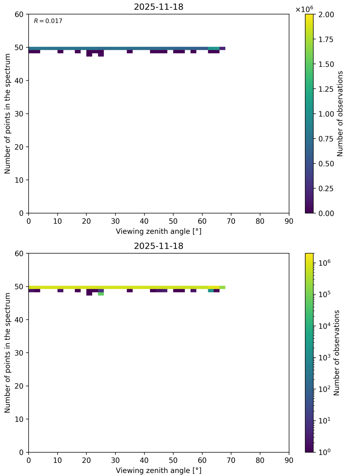
Figure 125: Scatter density plot of “Viewing zenith angle” against “Number of points in the spectrum” for 2025-11-18 to 2025-11-19.
