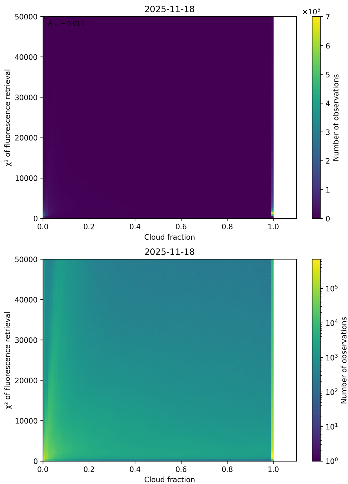
Figure 71: Scatter density plot of “Cloud fraction” against “ \chi^2 of fluorescence retrieval” for 2025-11-18 to 2025-11-19.
