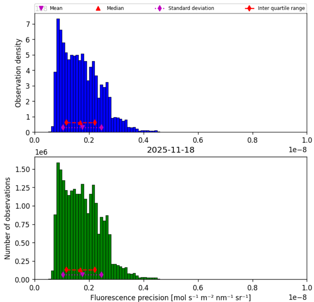
Figure 41: Histogram of “Fluorescence precision” for 2025-11-18 to 2025-11-19
