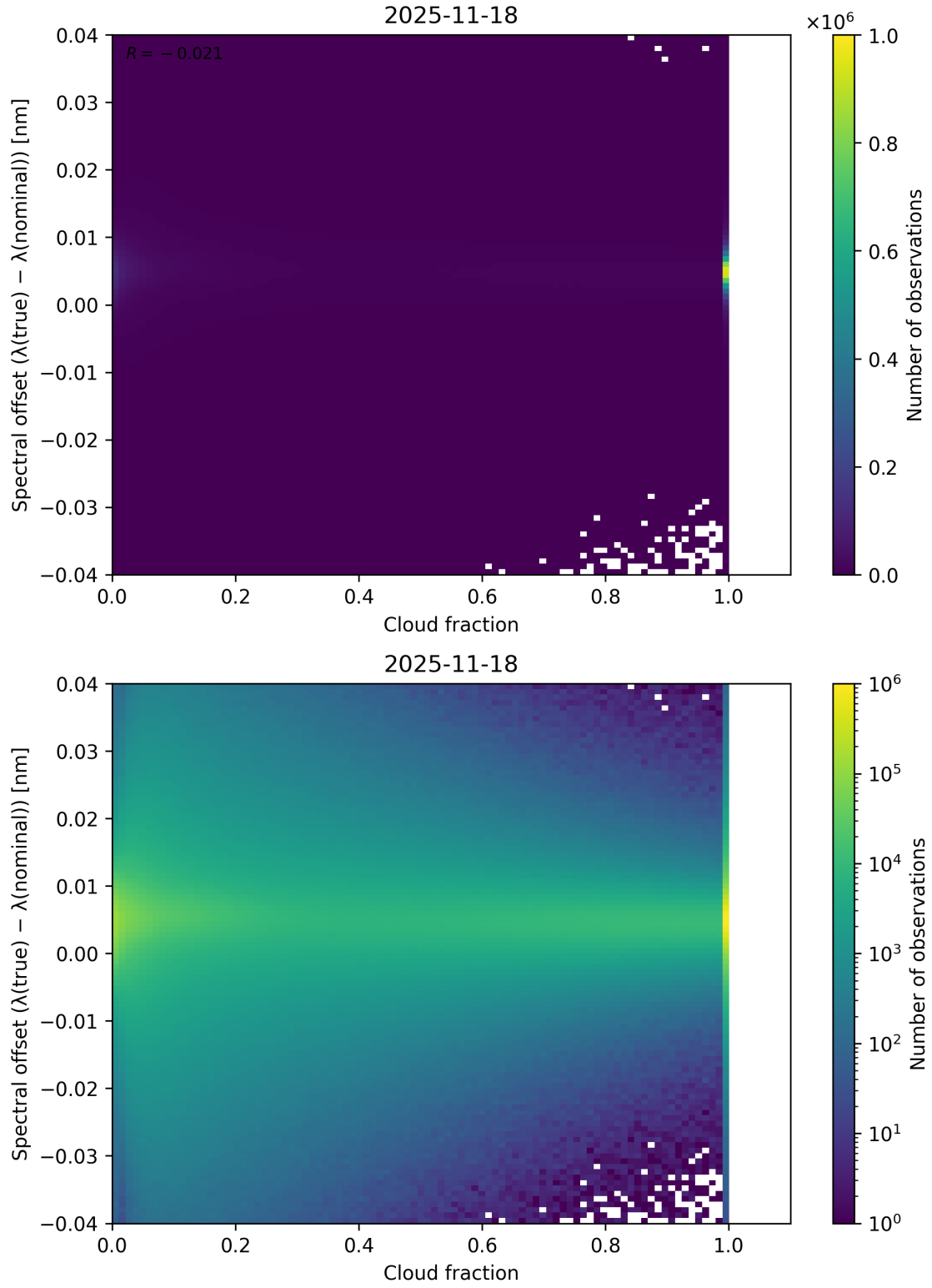
Figure 76: Scatter density plot of “Cloud fraction” against “Spectral offset ( \lambda_{\text{true}} - \lambda_{\text{nominal}} )” for 2025-11-18 to 2025-11-19.
