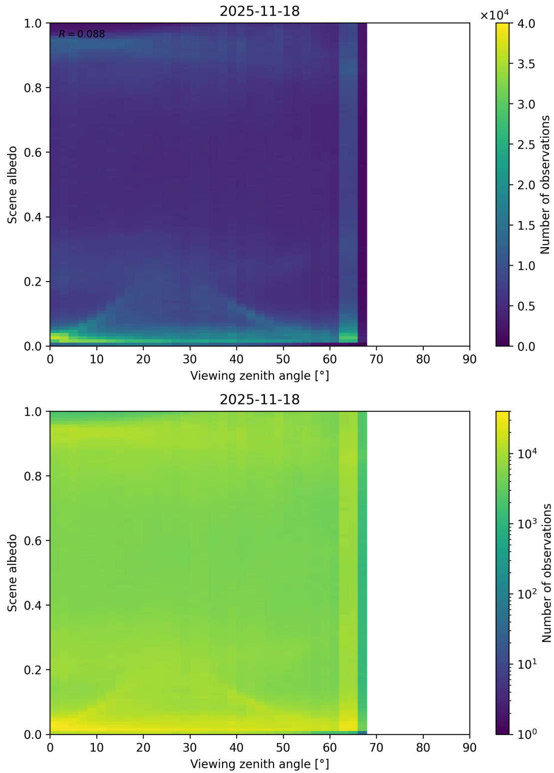
Figure 126: Scatter density plot of “Viewing zenith angle” against “Scene albedo” for 2025-11-18 to 2025-11-19.
