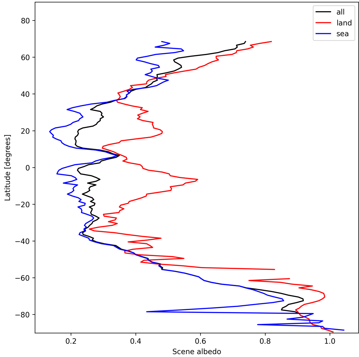
Figure 17: Zonal average of “Scene albedo” for 2025-11-18 to 2025-11-19.
