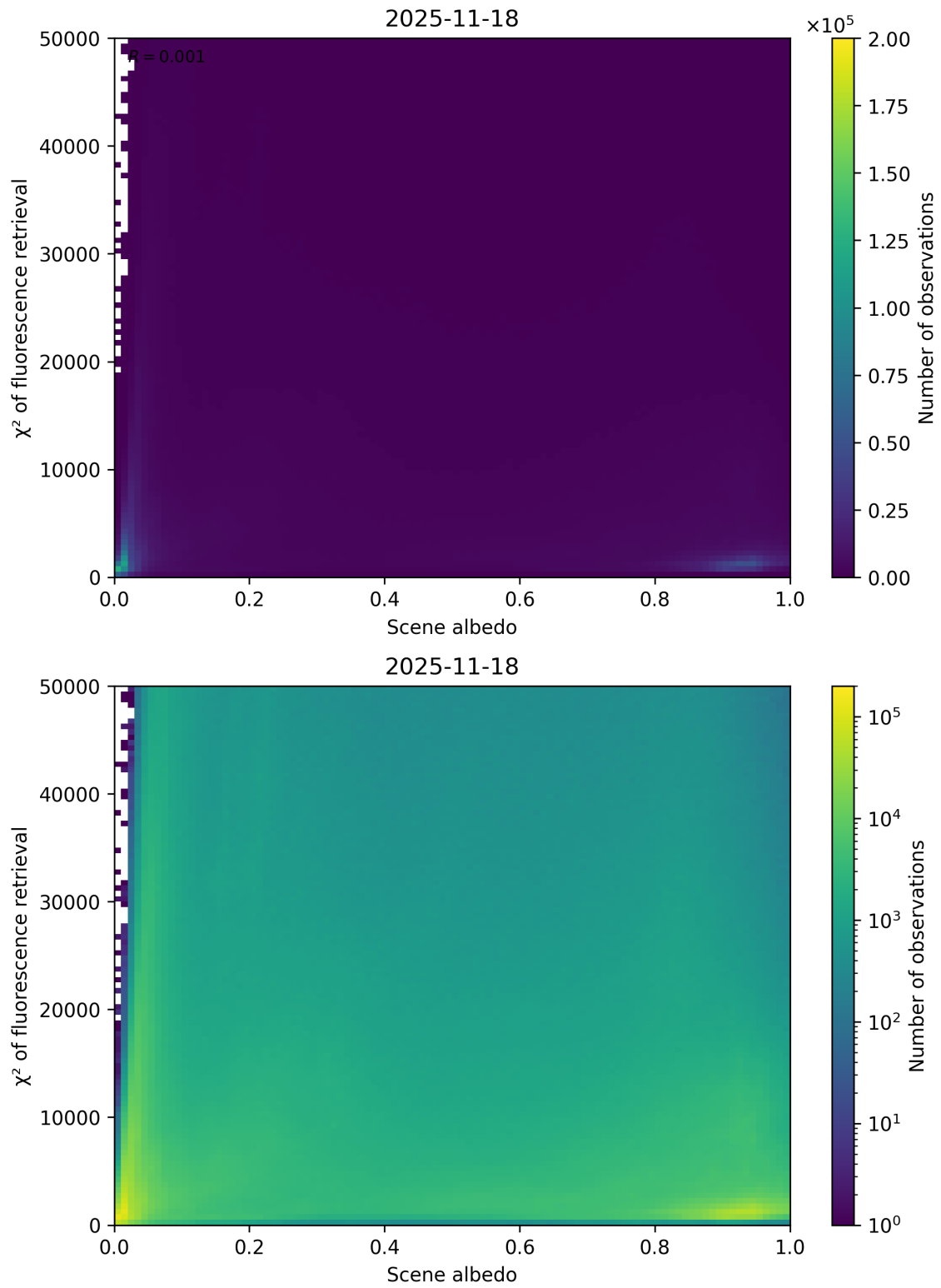
Figure 103: Scatter density plot of “Scene albedo” against “ \chi^2 of fluorescence retrieval” for 2025-11-18 to 2025-11-19.
