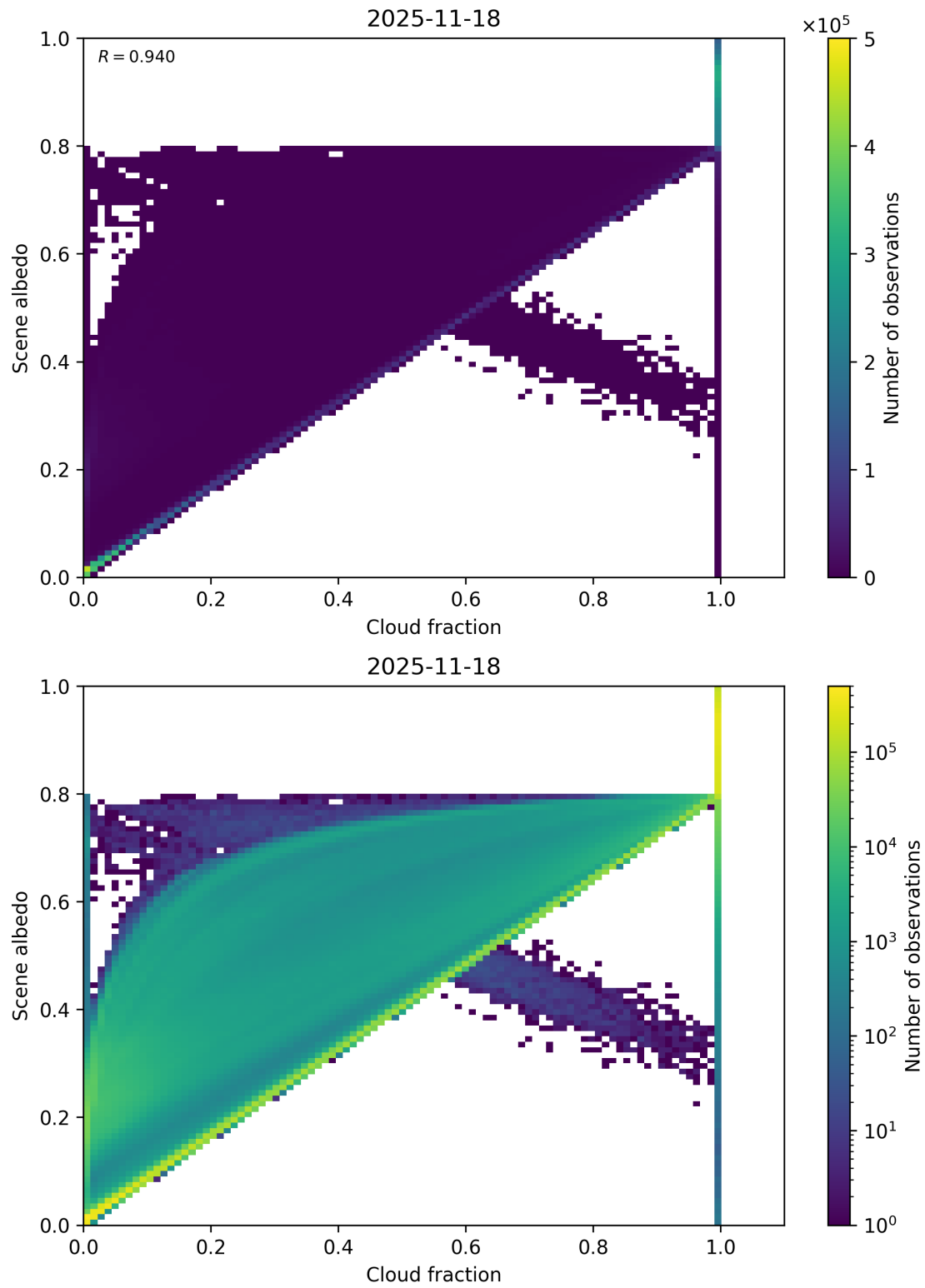
Figure 75: Scatter density plot of “Cloud fraction” against “Scene albedo” for 2025-11-18 to 2025-11-19.
