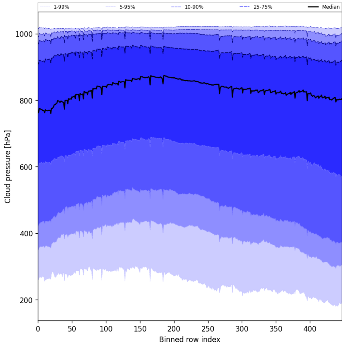
Figure 47: Along track statistics of “Cloud pressure” for 2025-11-18 to 2025-11-19
