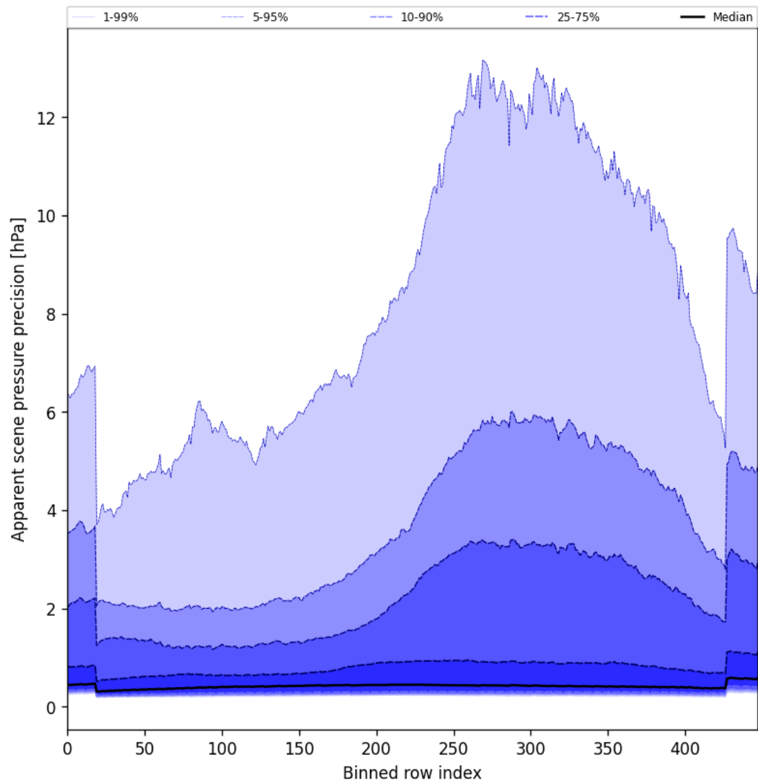
Figure 54: Along track statistics of “Apparent scene pressure precision” for 2025-11-18 to 2025-11-19
