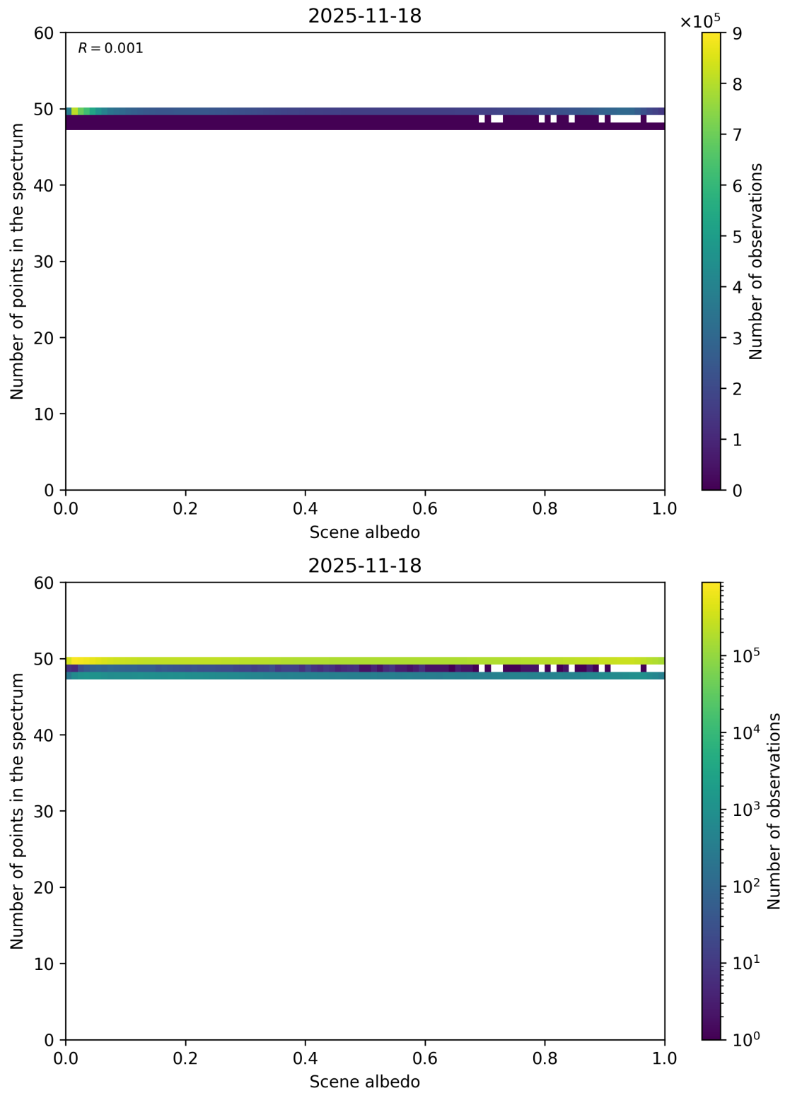
Figure 106: Scatter density plot of “Scene albedo” against “Number of points in the spectrum” for 2025-11-18 to 2025-11-19.
