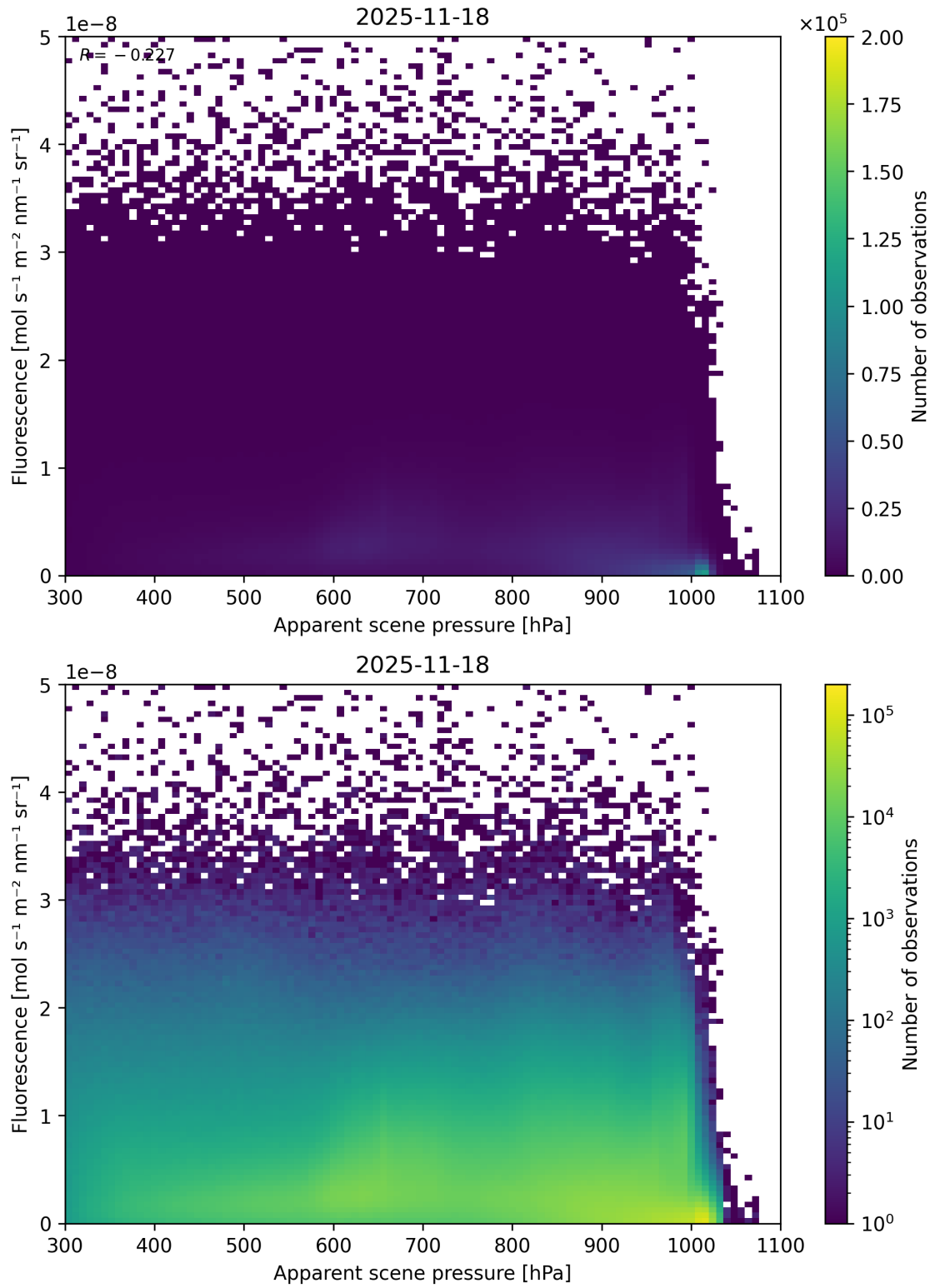
Figure 64: Scatter density plot of “Apparent scene pressure” against “Fluorescence” for 2025-11-18 to 2025-11-19.
