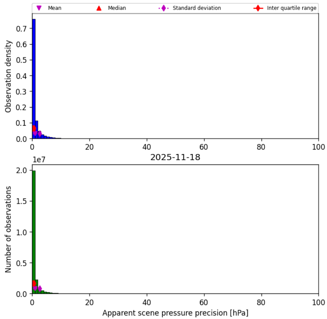
Figure 37: Histogram of “Apparent scene pressure precision” for 2025-11-18 to 2025-11-19
