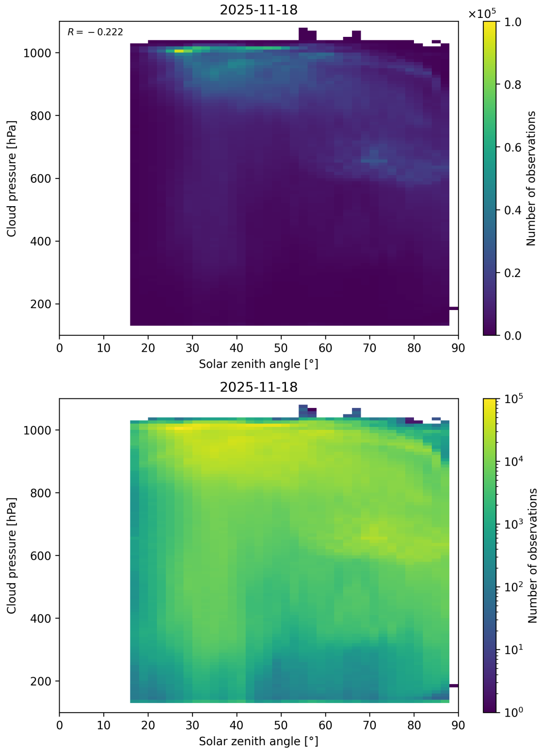
Figure 111: Scatter density plot of “Solar zenith angle” against “Cloud pressure” for 2025-11-18 to 2025-11-19.
