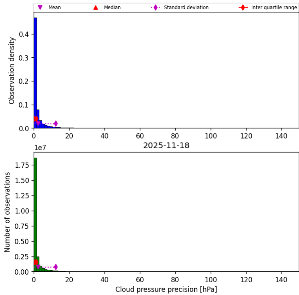
Figure 31: Histogram of “Cloud pressure precision” for 2025-11-18 to 2025-11-19
