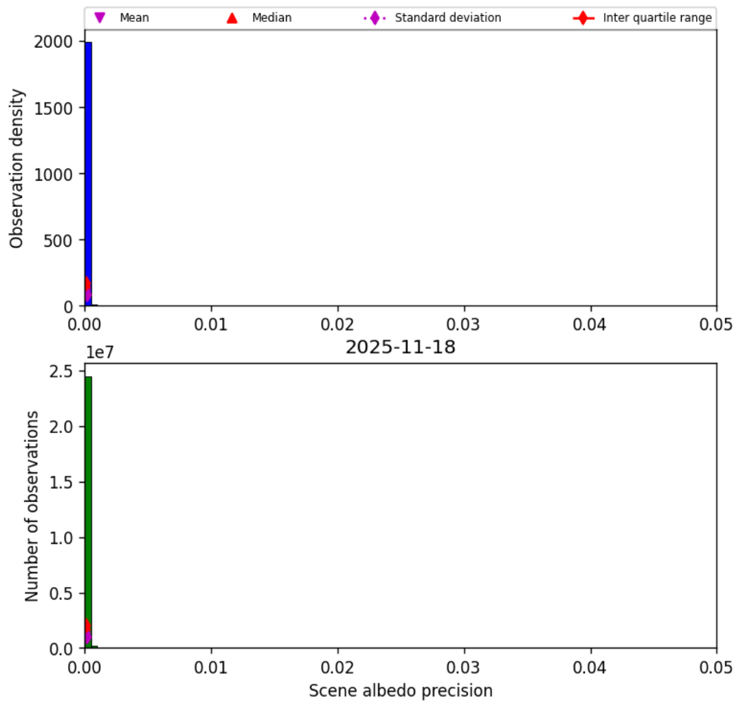
Figure 35: Histogram of “Scene albedo precision” for 2025-11-18 to 2025-11-19
