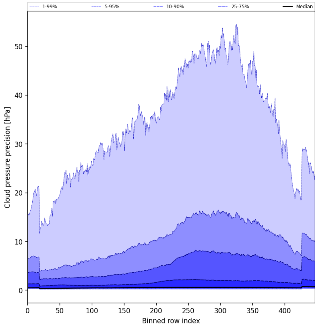
Figure 48: Along track statistics of “Cloud pressure precision” for 2025-11-18 to 2025-11-19
