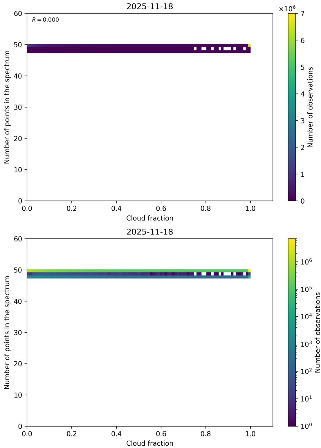
Figure 74: Scatter density plot of “Cloud fraction” against “Number of points in the spectrum” for 2025-11-18 to 2025-11-19.
