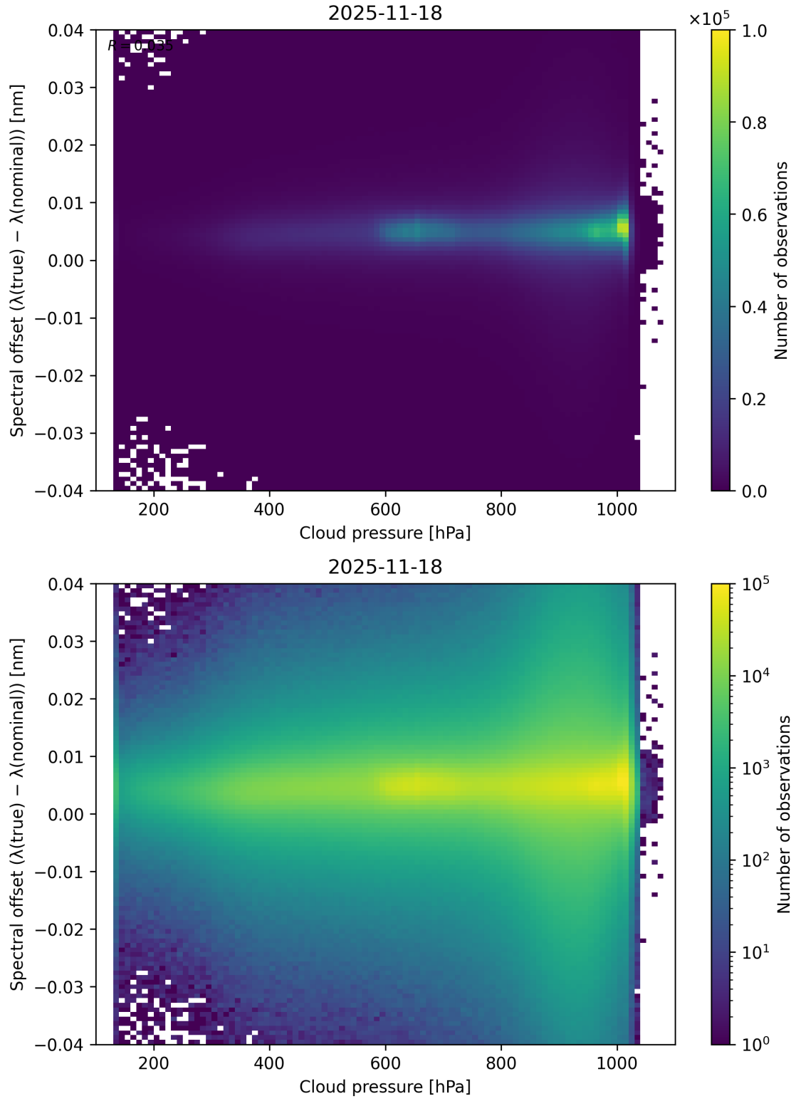
Figure 84: Scatter density plot of “Cloud pressure” against “Spectral offset ( \lambda_{\text{true}} - \lambda_{\text{nominal}} )” for 2025-11-18 to 2025-11-19.
