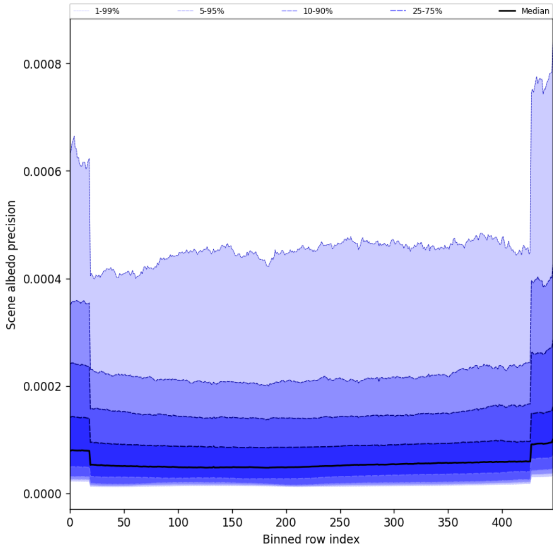
Figure 52: Along track statistics of “Scene albedo precision” for 2025-11-18 to 2025-11-19
