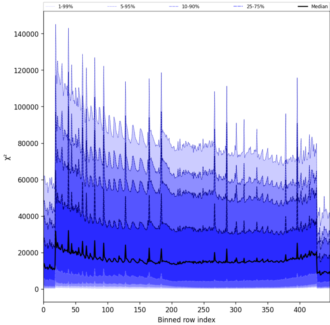
Figure 55: Along track statistics of “ \chi^2 ” for 2025-11-18 to 2025-11-19
