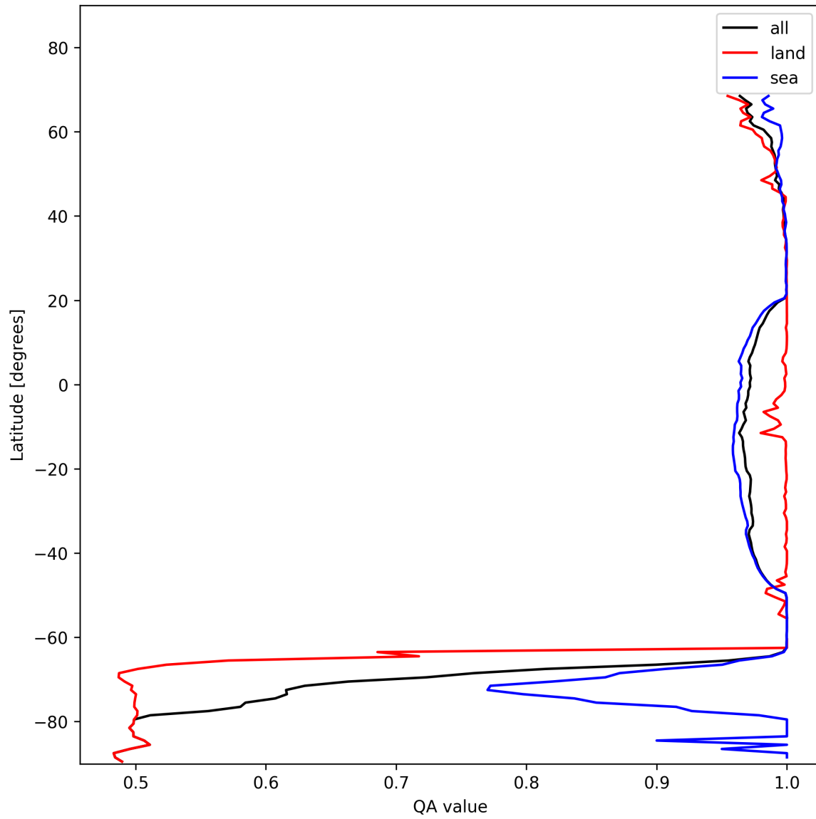
Figure 12: Zonal average of “QA value” for 2025-11-18 to 2025-11-19.
