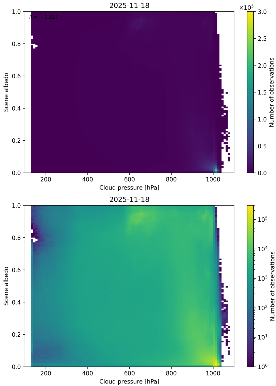
Figure 83: Scatter density plot of “Cloud pressure” against “Scene albedo” for 2025-11-18 to 2025-11-19.
