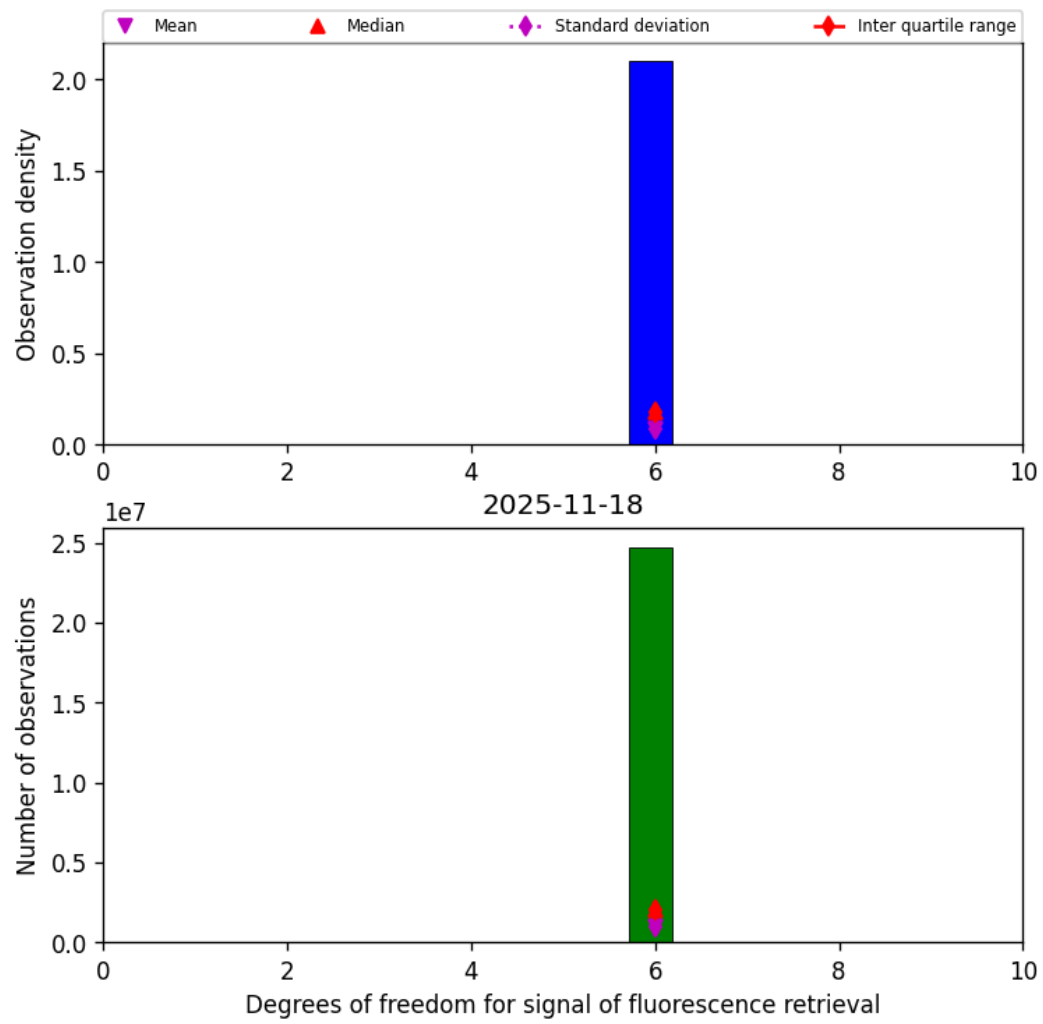
Figure 43: Histogram of “Degrees of freedom for signal of fluorescence retrieval” for 2025-11-18 to 2025-11-19
