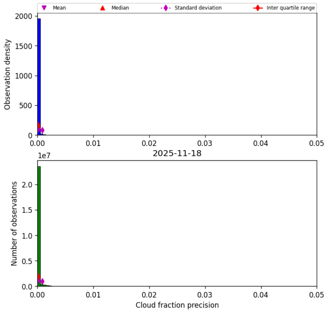
Figure 33: Histogram of “Cloud fraction precision” for 2025-11-18 to 2025-11-19
