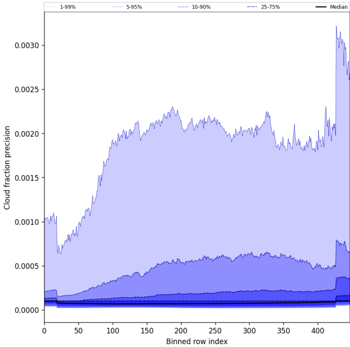
Figure 50: Along track statistics of “Cloud fraction precision” for 2025-11-18 to 2025-11-19
