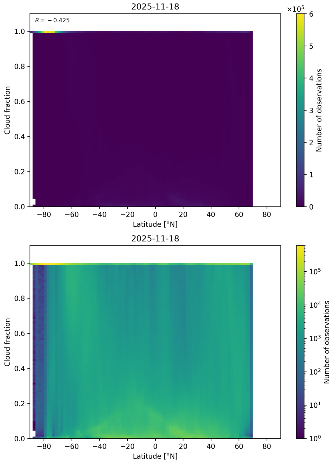
Figure 90: Scatter density plot of “Latitude” against “Cloud fraction” for 2025-11-18 to 2025-11-19.
