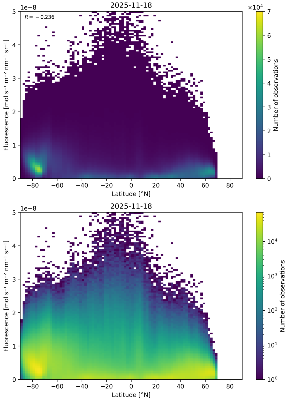
Figure 92: Scatter density plot of “Latitude” against “Fluorescence” for 2025-11-18 to 2025-11-19.
