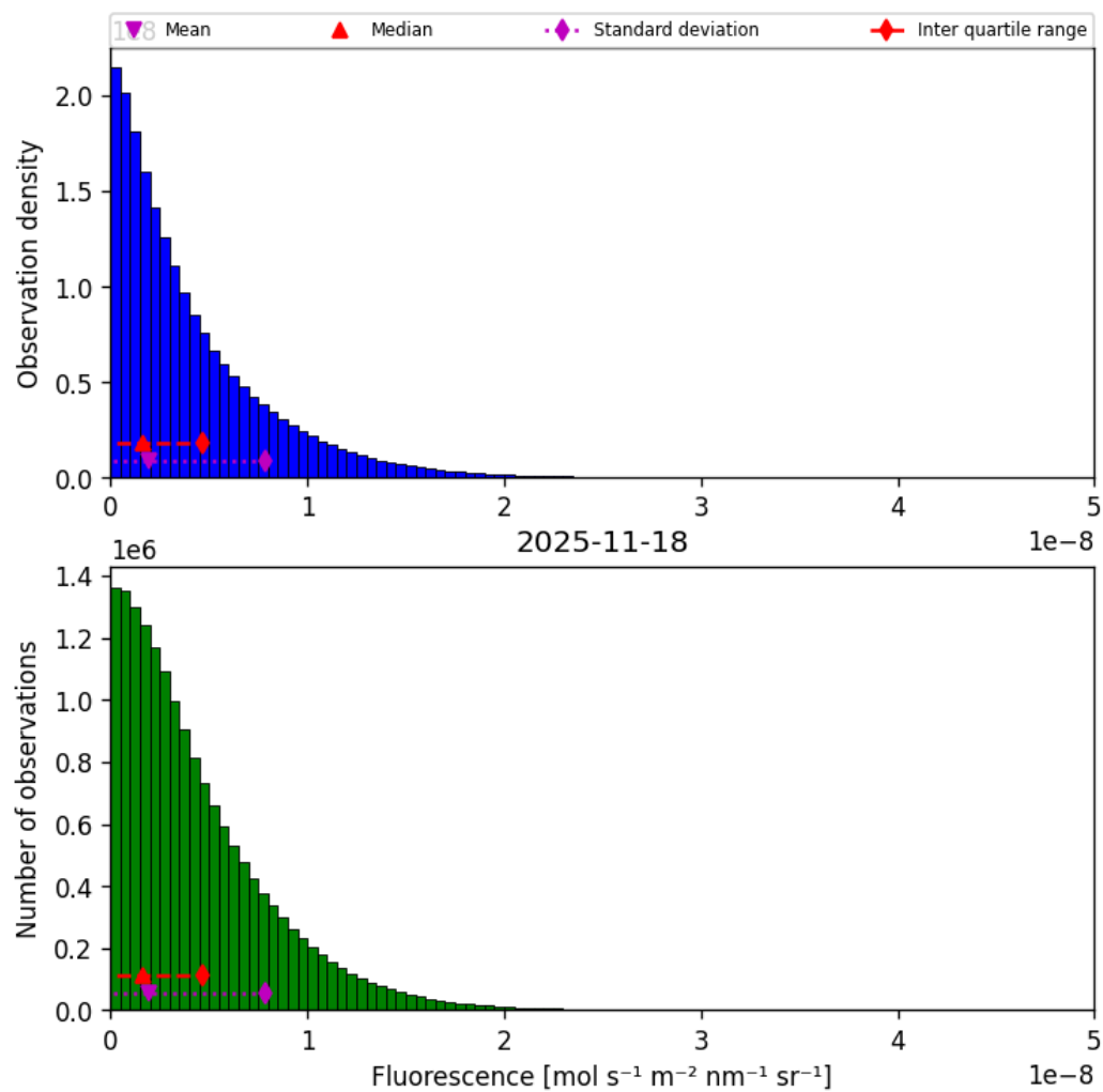
Figure 40: Histogram of “Fluorescence” for 2025-11-18 to 2025-11-19
