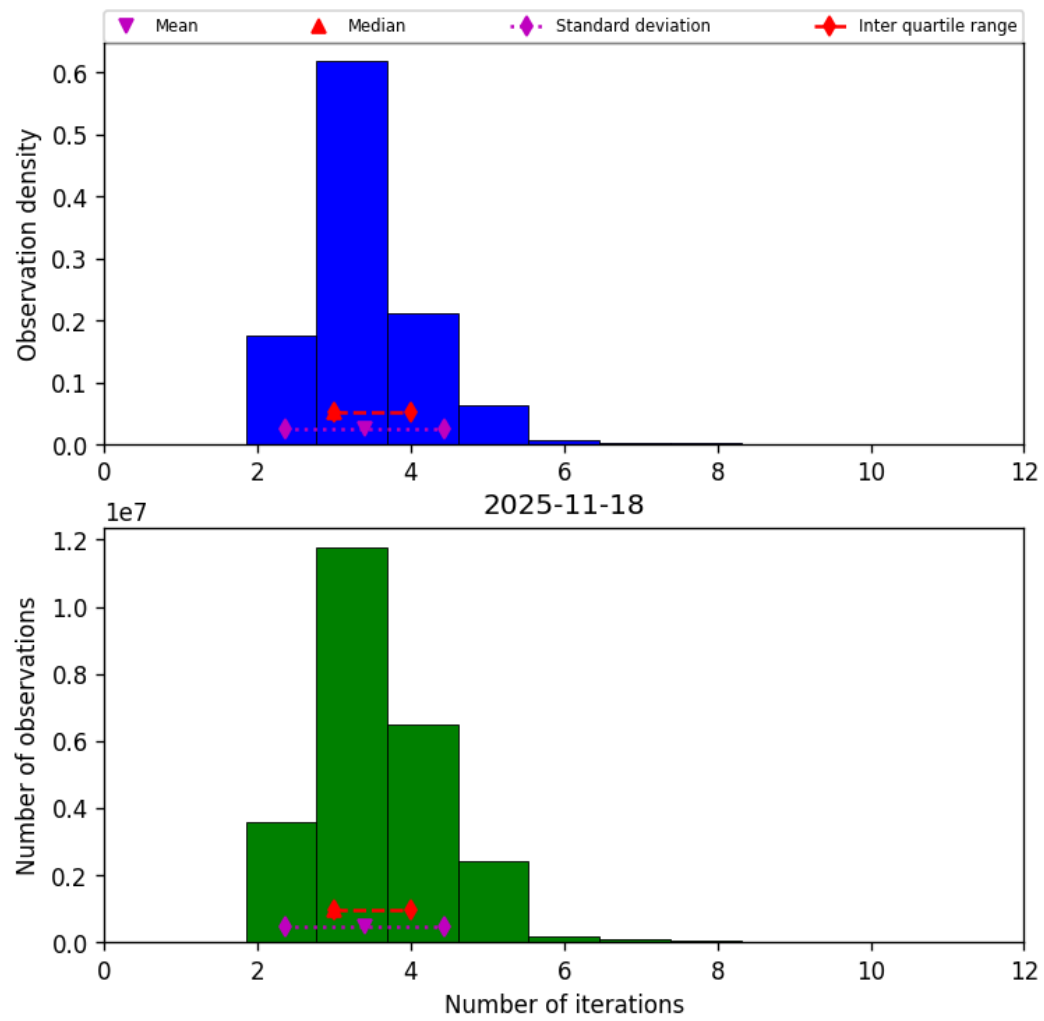
Figure 39: Histogram of “Number of iterations” for 2025-11-18 to 2025-11-19
