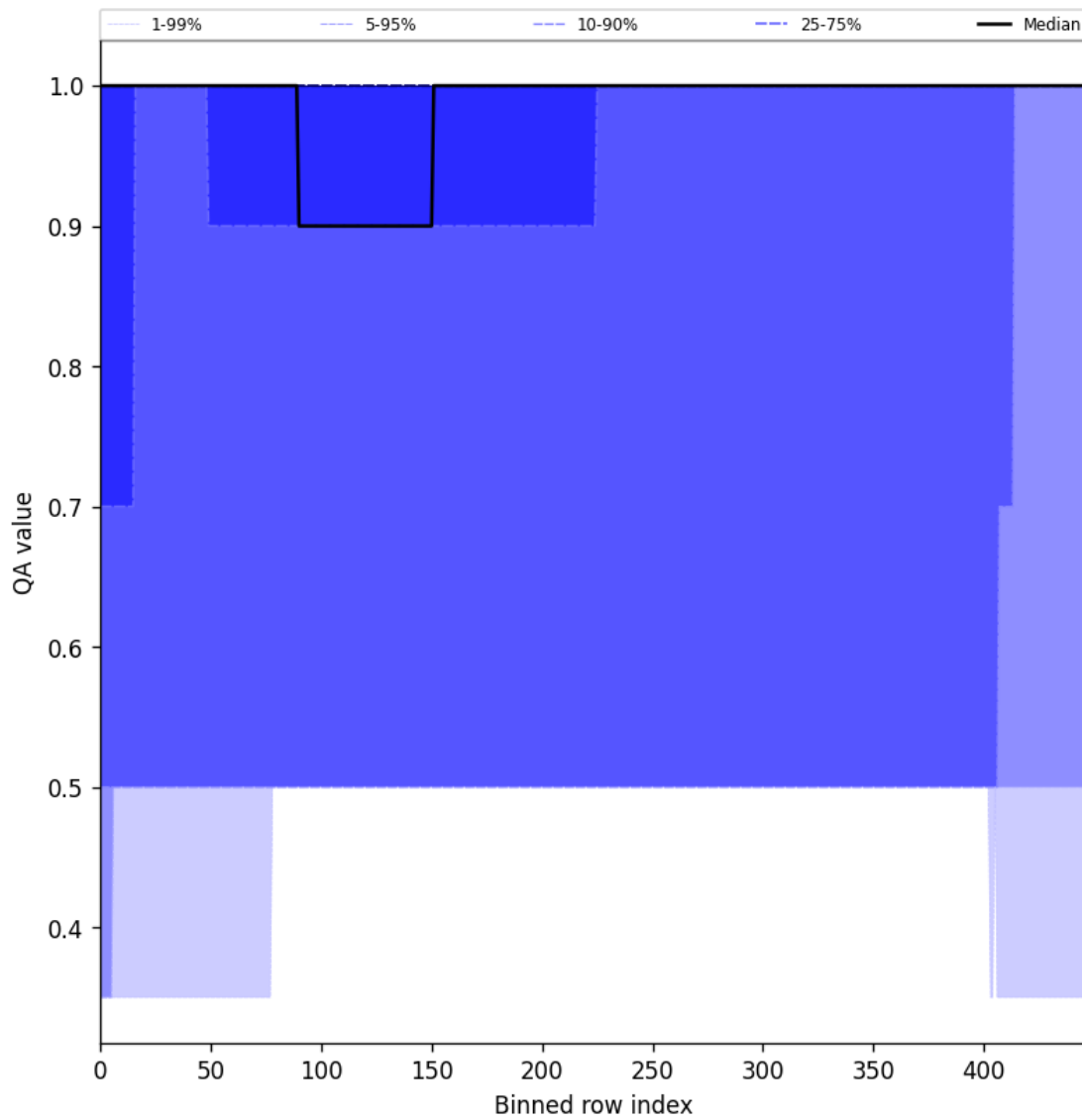
Figure 46: Along track statistics of “QA value” for 2025-11-18 to 2025-11-19
