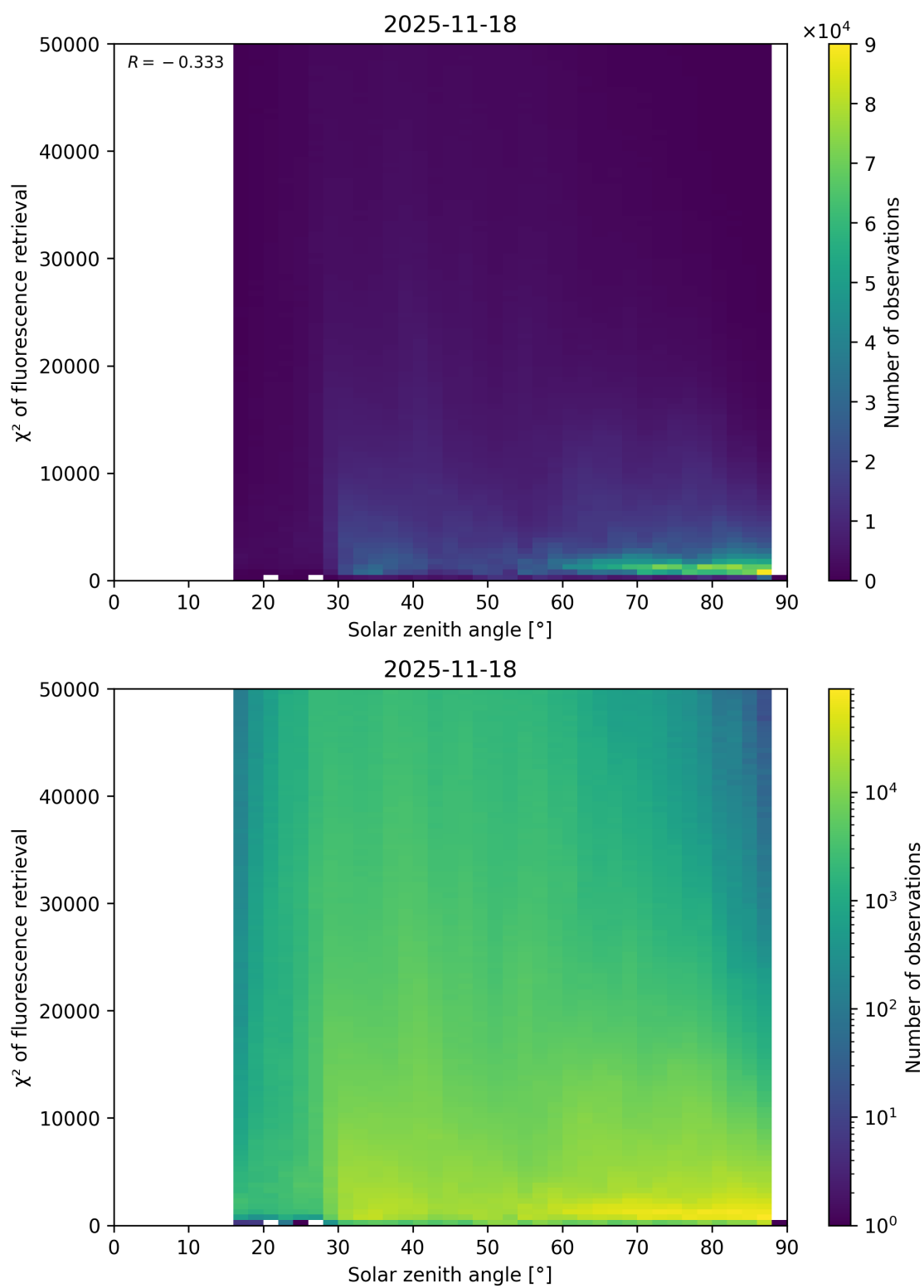
Figure 109: Scatter density plot of “Solar zenith angle” against “ \chi^2 of fluorescence retrieval” for 2025-11-18 to 2025-11-19.
