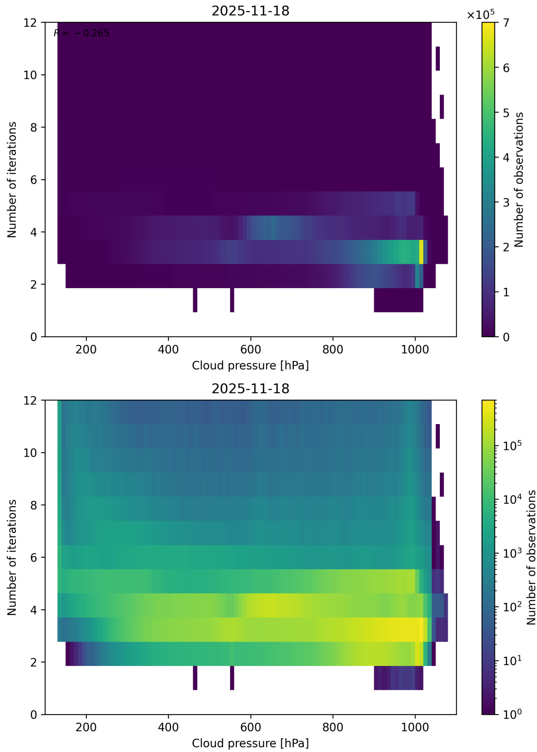
Figure 81: Scatter density plot of “Cloud pressure” against “Number of iterations” for 2025-11-18 to 2025-11-19.
