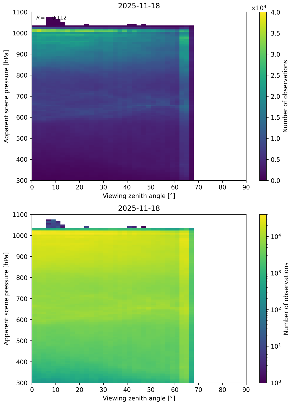
Figure 118: Scatter density plot of “Viewing zenith angle” against “Apparent scene pressure” for 2025-11-18 to 2025-11-19.
