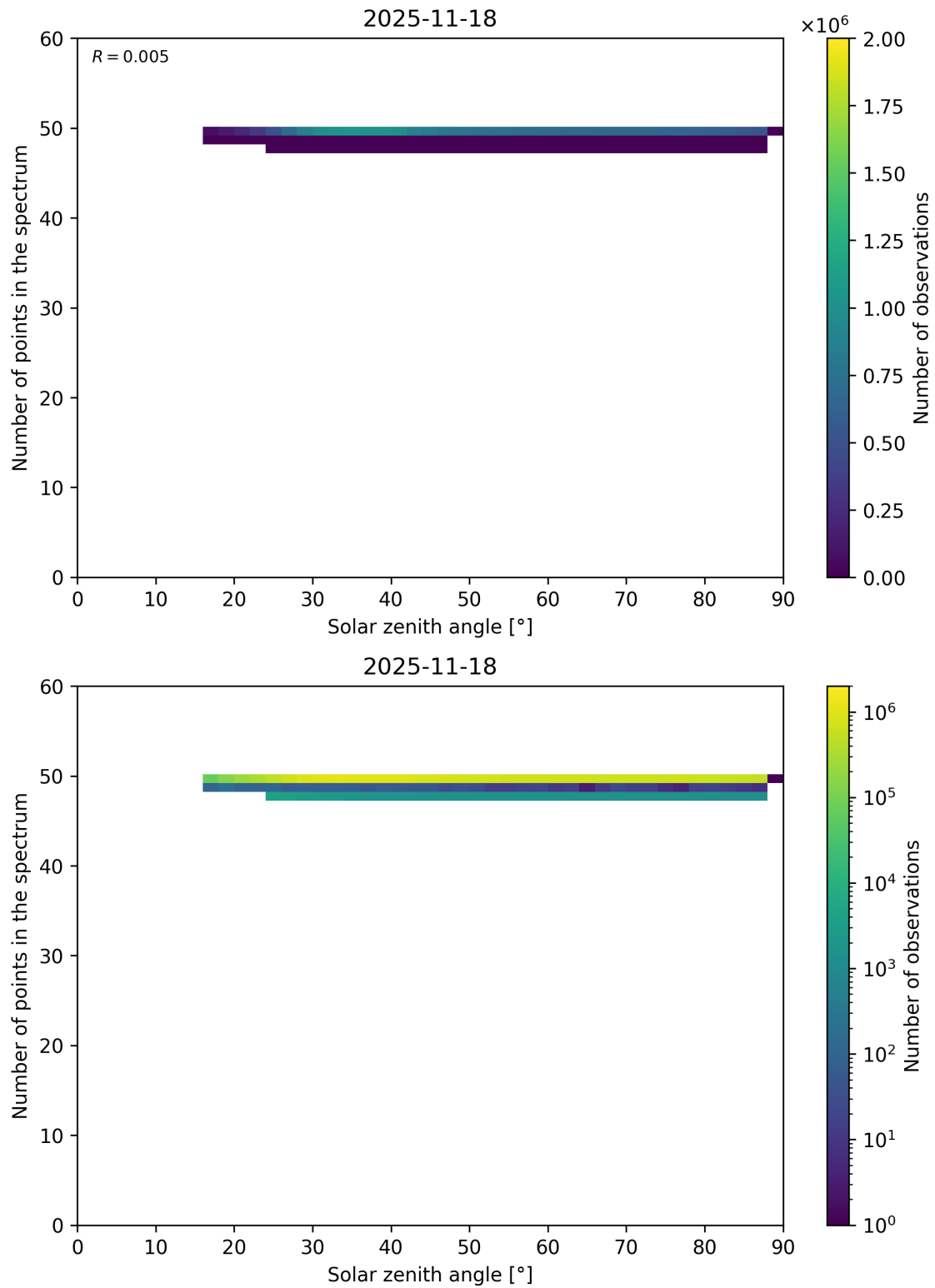
Figure 115: Scatter density plot of “Solar zenith angle” against “Number of points in the spectrum” for 2025-11-18 to 2025-11-19.
