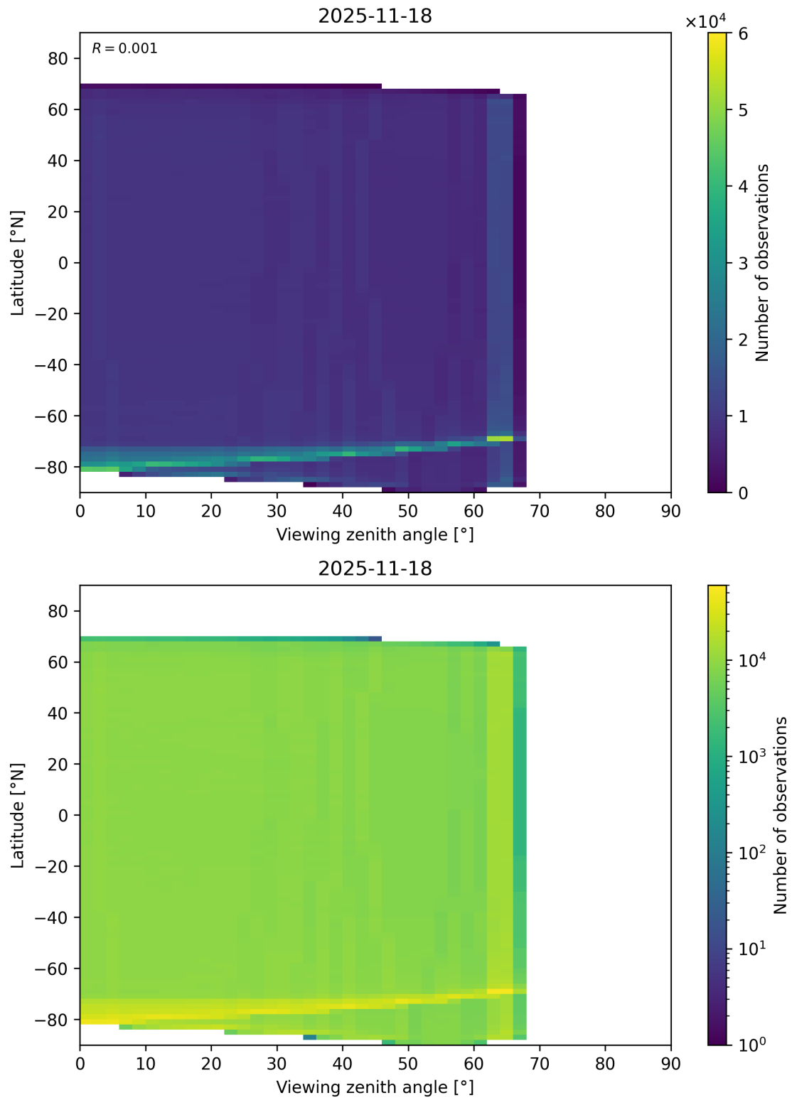
Figure 123: Scatter density plot of “Viewing zenith angle” against “Latitude” for 2025-11-18 to 2025-11-19.
