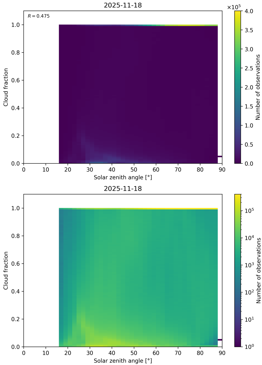
Figure 110: Scatter density plot of “Solar zenith angle” against “Cloud fraction” for 2025-11-18 to 2025-11-19.
