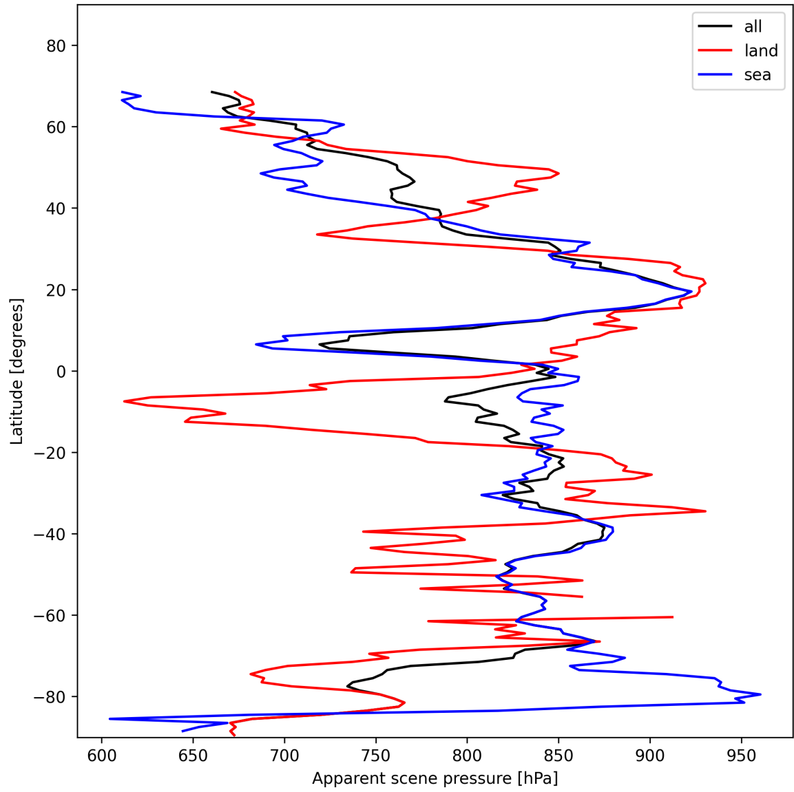
Figure 19: Zonal average of “Apparent scene pressure” for 2025-11-18 to 2025-11-19.
