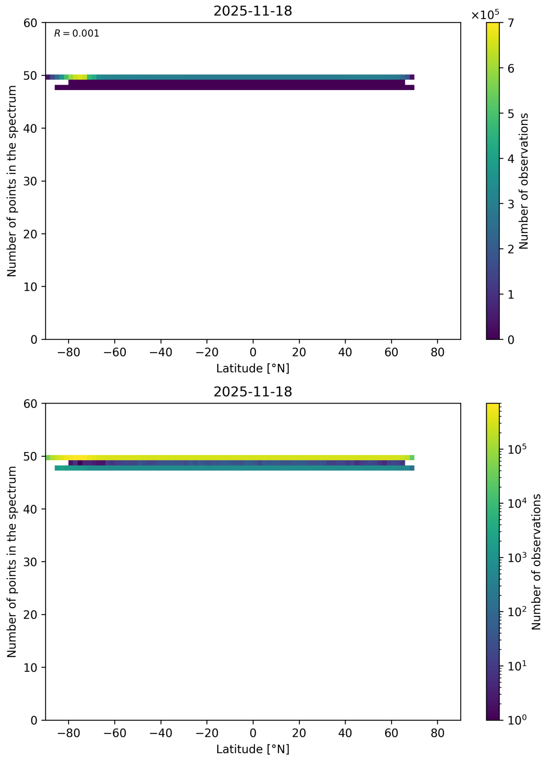
Figure 94: Scatter density plot of “Latitude” against “Number of points in the spectrum” for 2025-11-18 to 2025-11-19.
