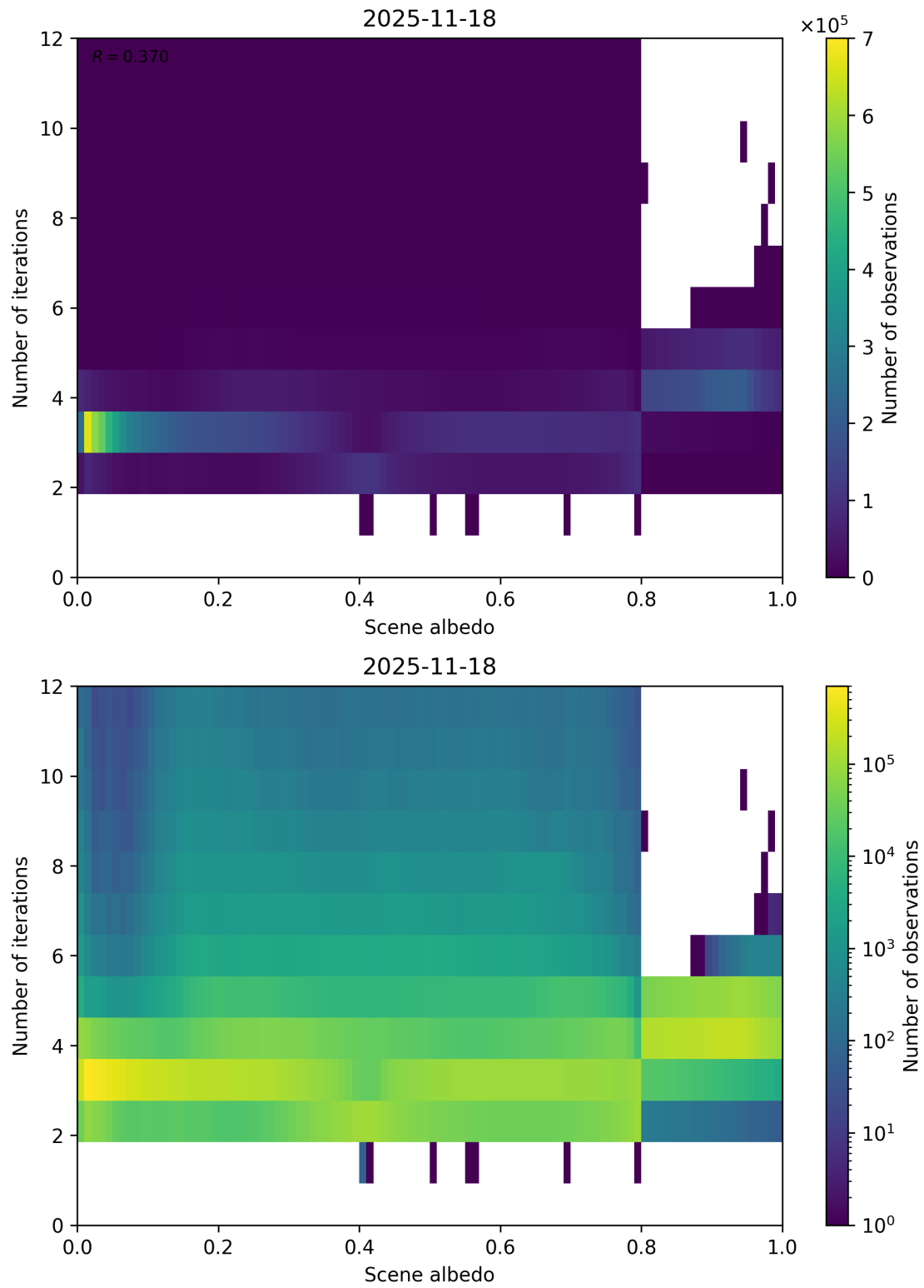
Figure 105: Scatter density plot of “Scene albedo” against “Number of iterations” for 2025-11-18 to 2025-11-19.
