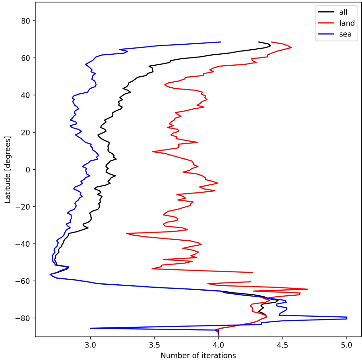
Figure 22: Zonal average of “Number of iterations” for 2025-11-18 to 2025-11-19.
