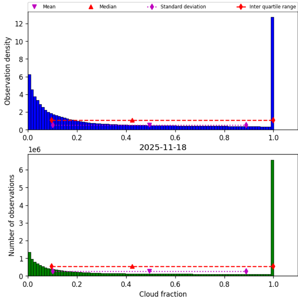
Figure 32: Histogram of “Cloud fraction” for 2025-11-18 to 2025-11-19
