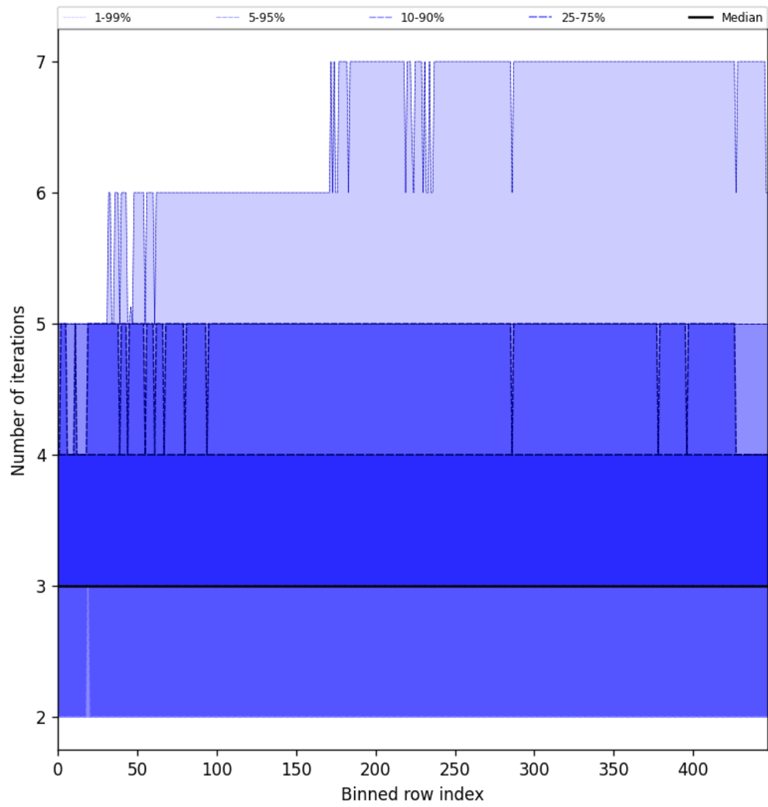
Figure 56: Along track statistics of “Number of iterations” for 2025-11-18 to 2025-11-19
