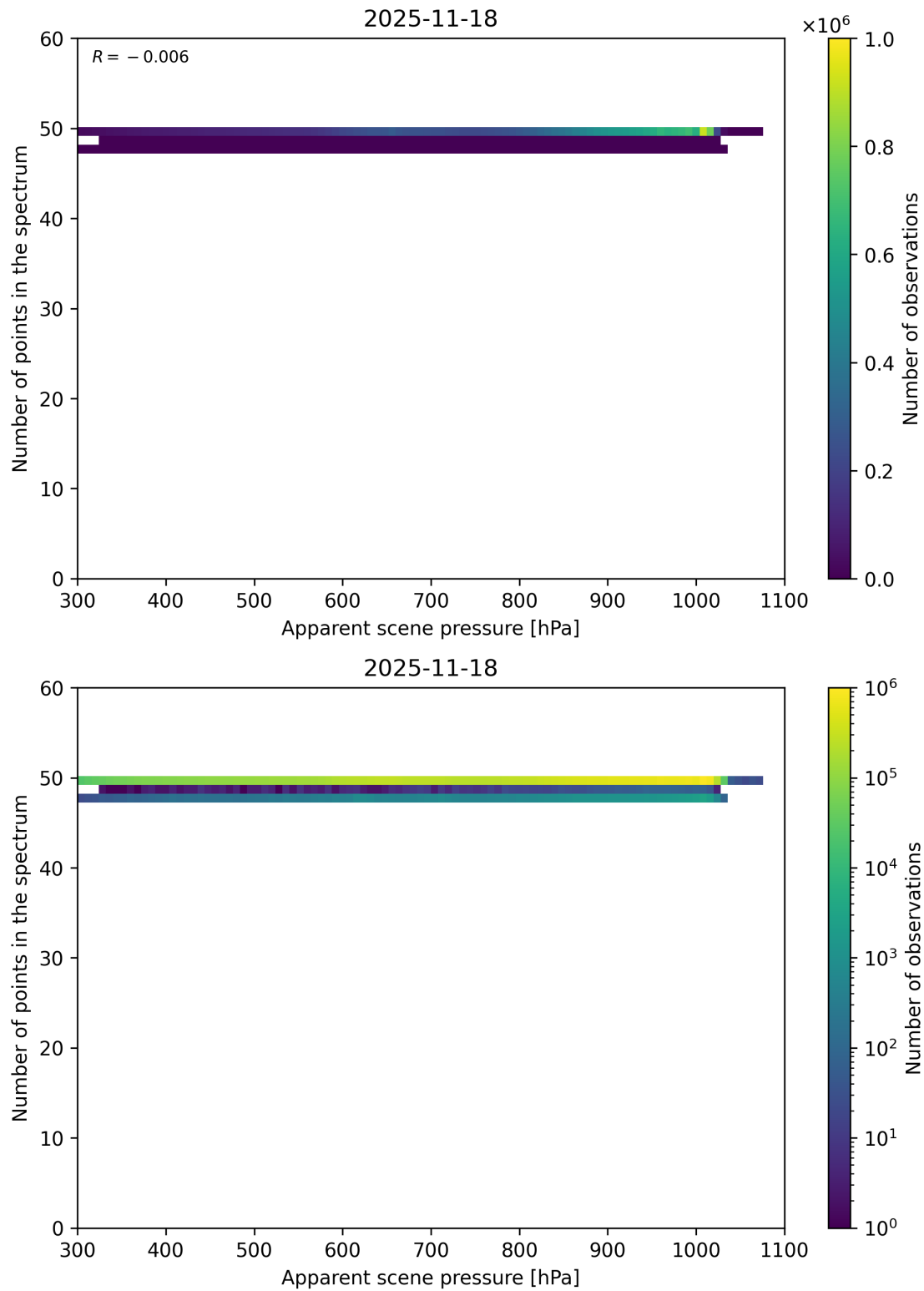
Figure 66: Scatter density plot of “Apparent scene pressure” against “Number of points in the spectrum” for 2025-11-18 to 2025-11-19.
