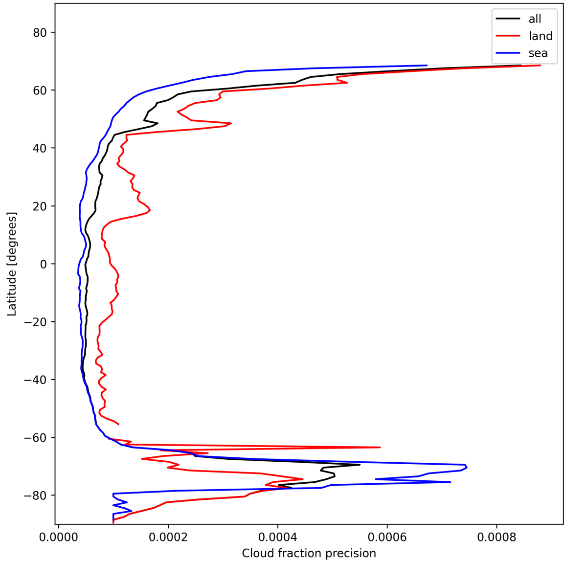
Figure 16: Zonal average of “Cloud fraction precision” for 2025-11-18 to 2025-11-19.
