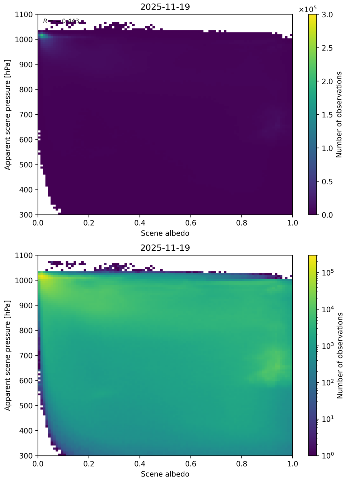
Figure 102: Scatter density plot of “Scene albedo” against “Apparent scene pressure” for 2025-11-18 to 2025-11-20.
