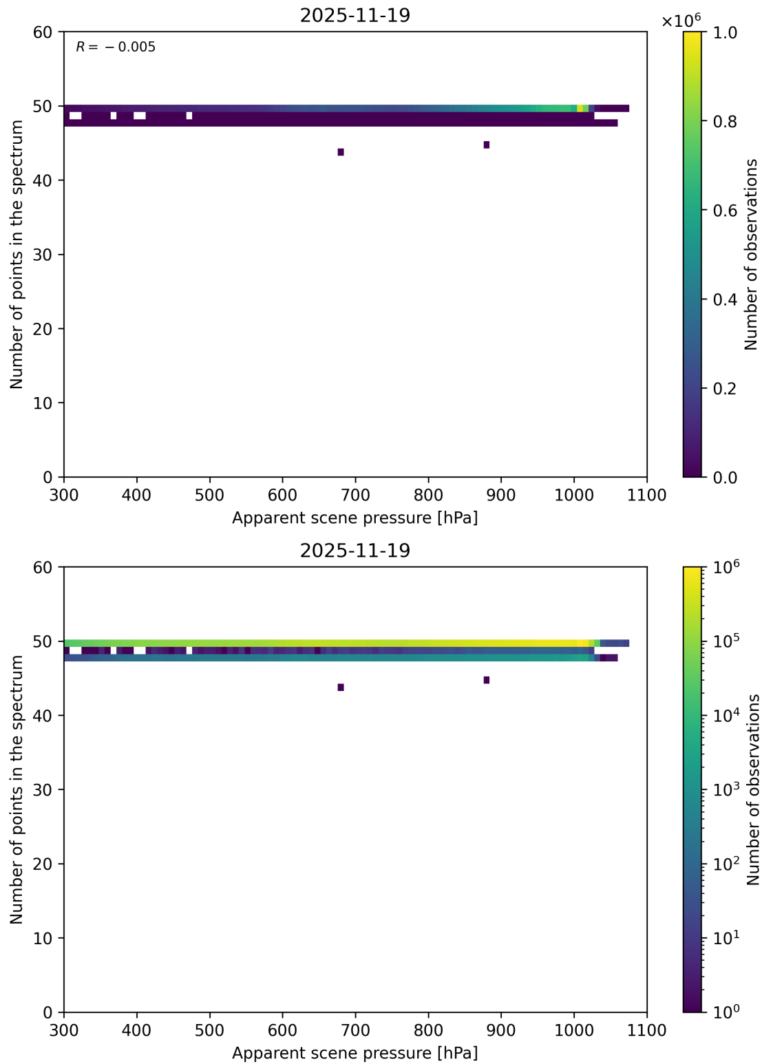
Figure 66: Scatter density plot of “Apparent scene pressure” against “Number of points in the spectrum” for 2025-11-18 to 2025-11-20.
