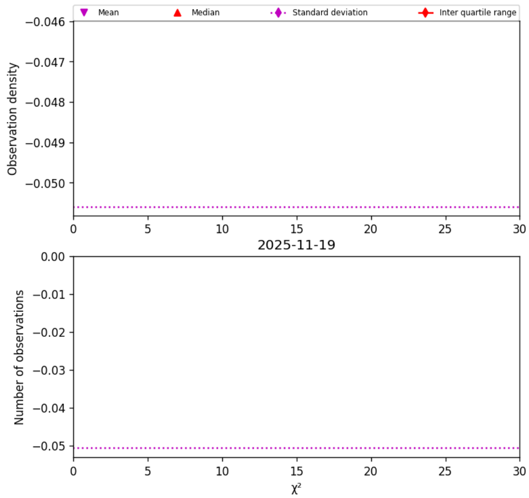
Figure 38: Histogram of " \chi^2 " for 2025-11-18 to 2025-11-20
