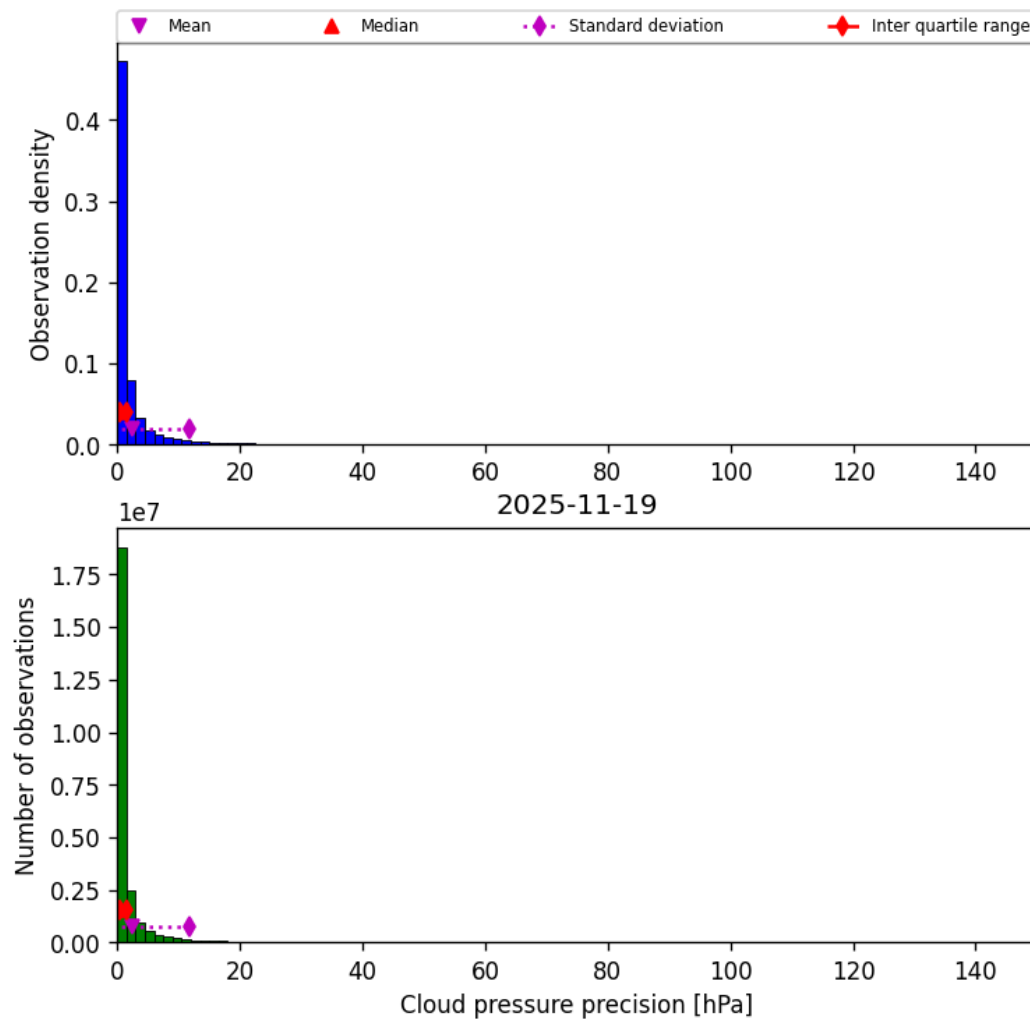
Figure 31: Histogram of “Cloud pressure precision” for 2025-11-18 to 2025-11-20
