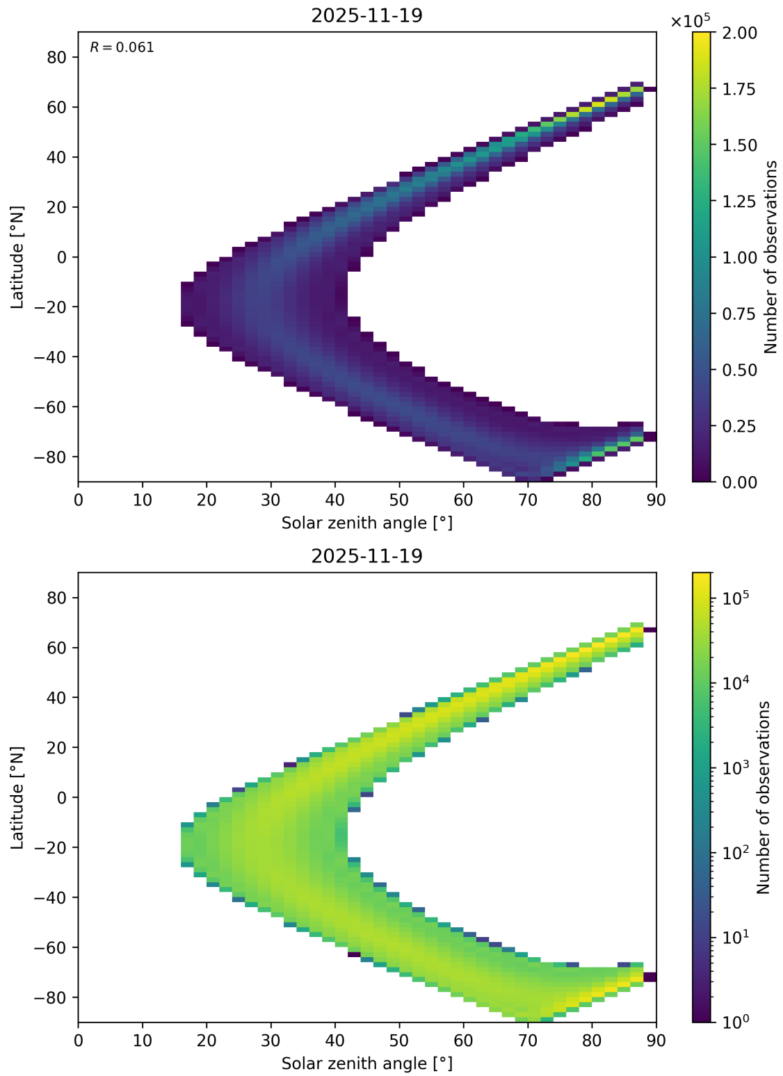
Figure 113: Scatter density plot of “Solar zenith angle” against “Latitude” for 2025-11-18 to 2025-11-20.
