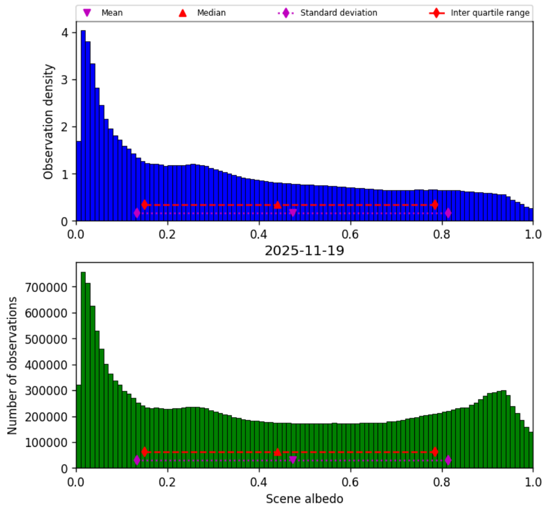
Figure 34: Histogram of “Scene albedo” for 2025-11-18 to 2025-11-20
