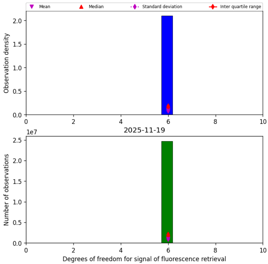
Figure 43: Histogram of “Degrees of freedom for signal of fluorescence retrieval” for 2025-11-18 to 2025-11-20
