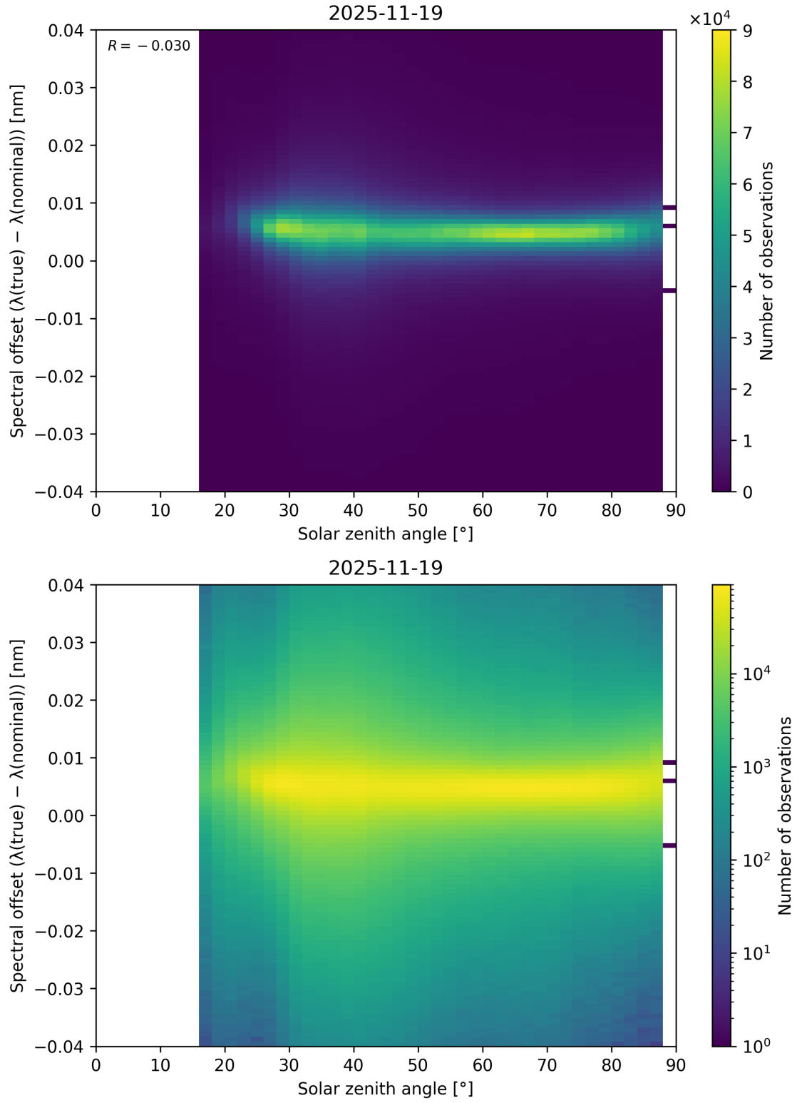
Figure 117: Scatter density plot of “Solar zenith angle” against “Spectral offset ( \lambda_{\text{true}} - \lambda_{\text{nominal}} )” for 2025-11-18 to 2025-11-20.
