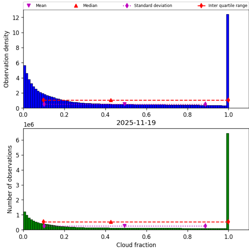
Figure 32: Histogram of “Cloud fraction” for 2025-11-18 to 2025-11-20
