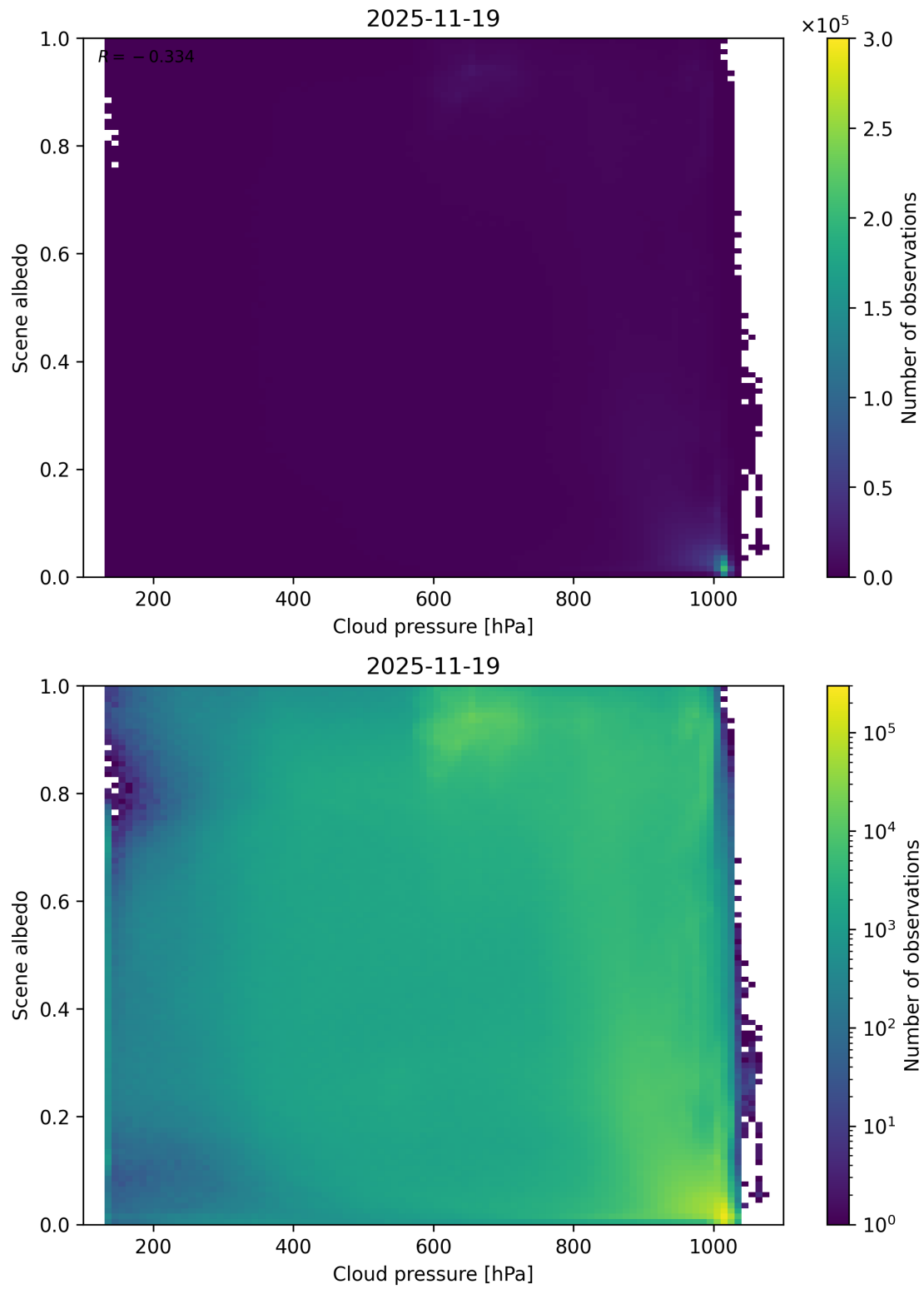
Figure 83: Scatter density plot of “Cloud pressure” against “Scene albedo” for 2025-11-18 to 2025-11-20.
