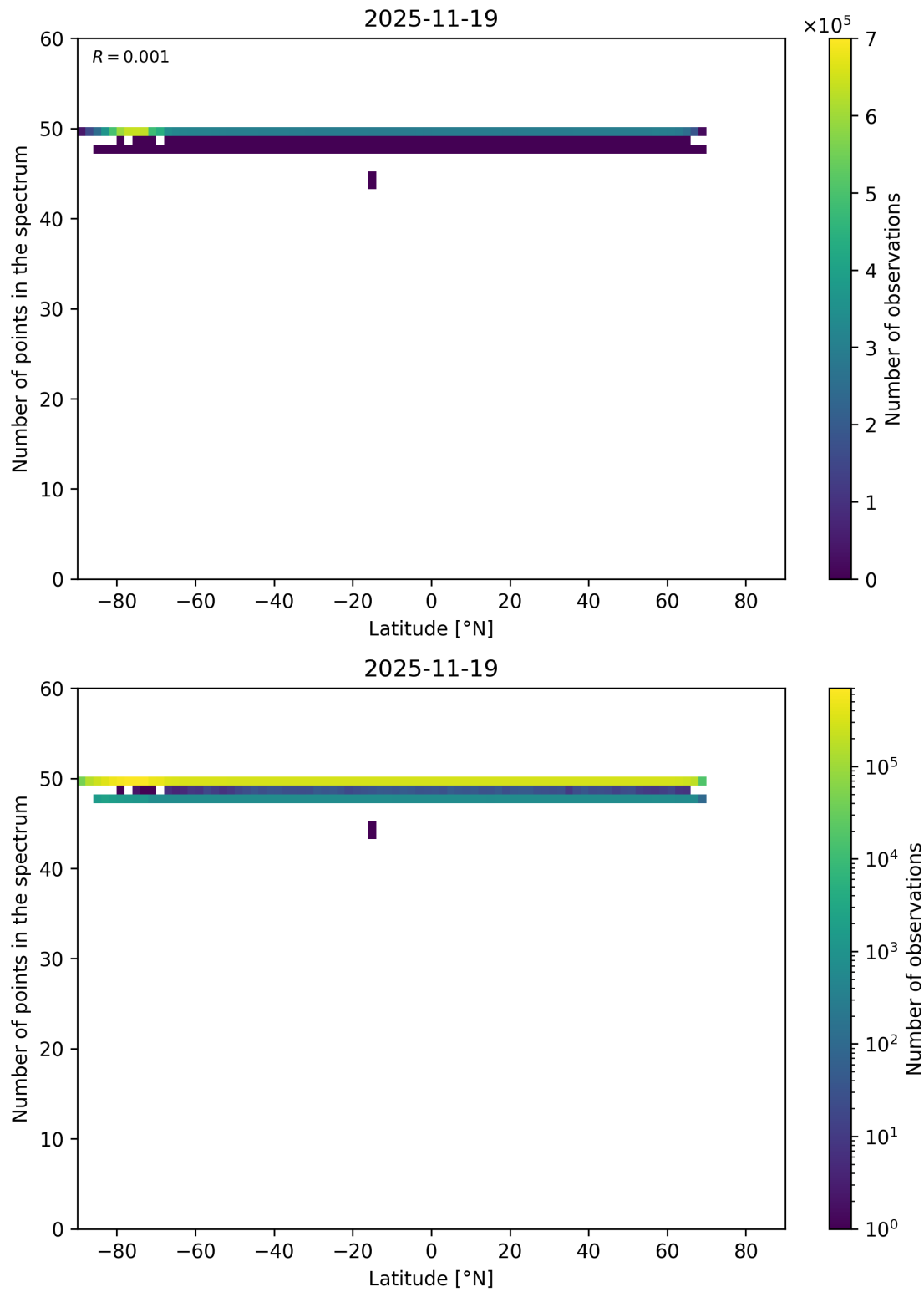
Figure 94: Scatter density plot of “Latitude” against “Number of points in the spectrum” for 2025-11-18 to 2025-11-20.
