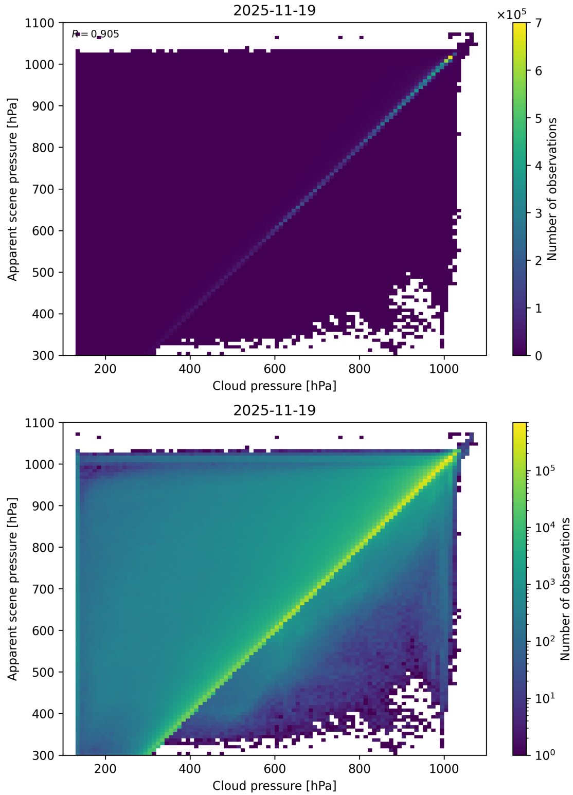
Figure 77: Scatter density plot of “Cloud pressure” against “Apparent scene pressure” for 2025-11-18 to 2025-11-20.
