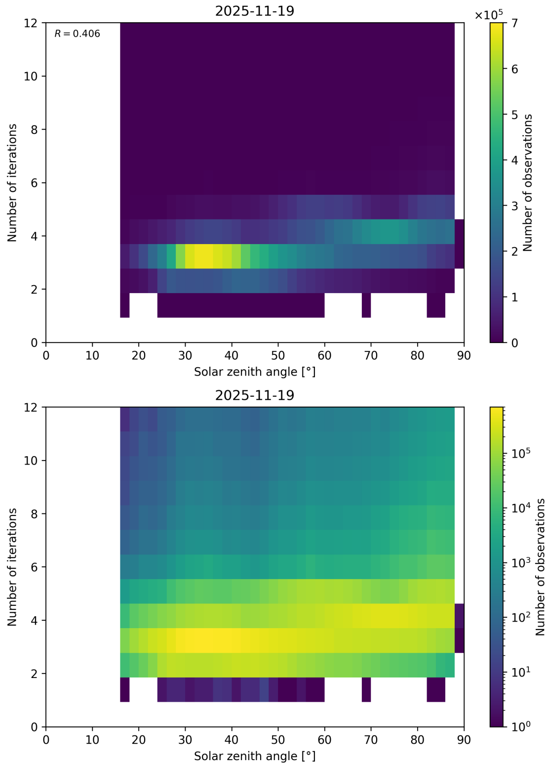
Figure 114: Scatter density plot of “Solar zenith angle” against “Number of iterations” for 2025-11-18 to 2025-11-20.
