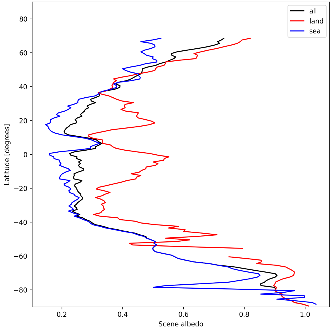
Figure 17: Zonal average of "Scene albedo" for 2025-11-18 to 2025-11-20.
