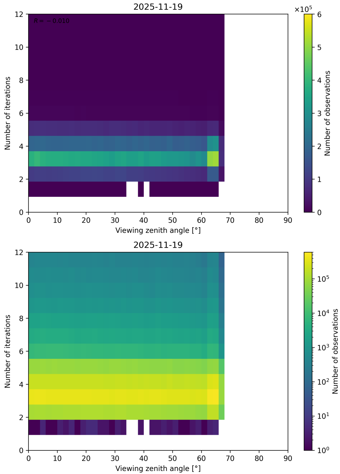
Figure 124: Scatter density plot of “Viewing zenith angle” against “Number of iterations” for 2025-11-18 to 2025-11-20.
