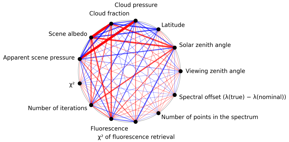
Figure 1: Map of correlation graph for 2025-11-18 to 2025-11-20.
