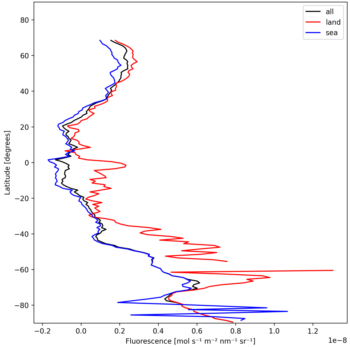
Figure 23: Zonal average of “Fluorescence” for 2025-11-18 to 2025-11-20.
