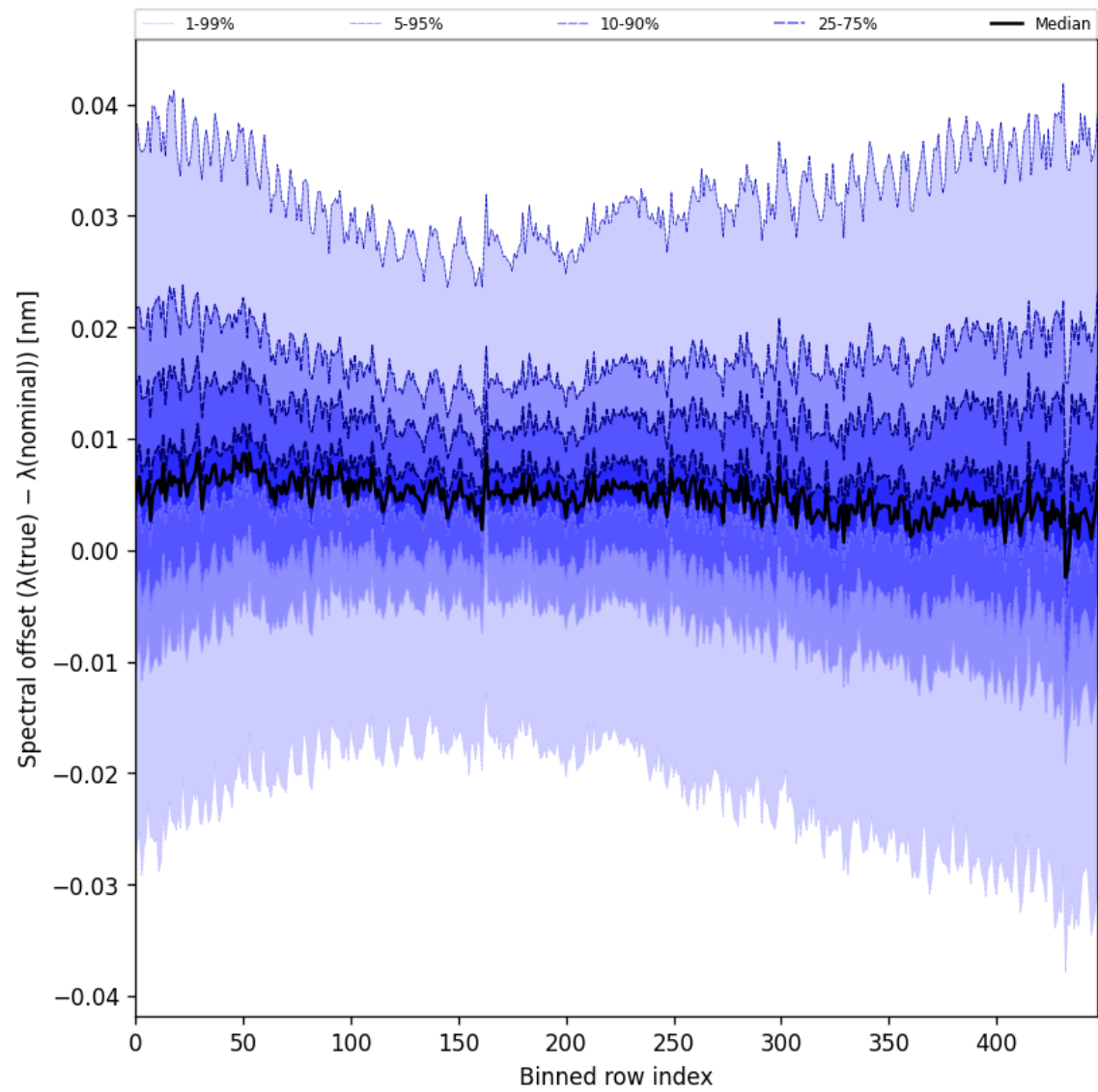
Figure 62: Along track statistics of “Spectral offset ( \lambda_{\text{true}} - \lambda_{\text{nominal}} )” for 2025-11-18 to 2025-11-20
