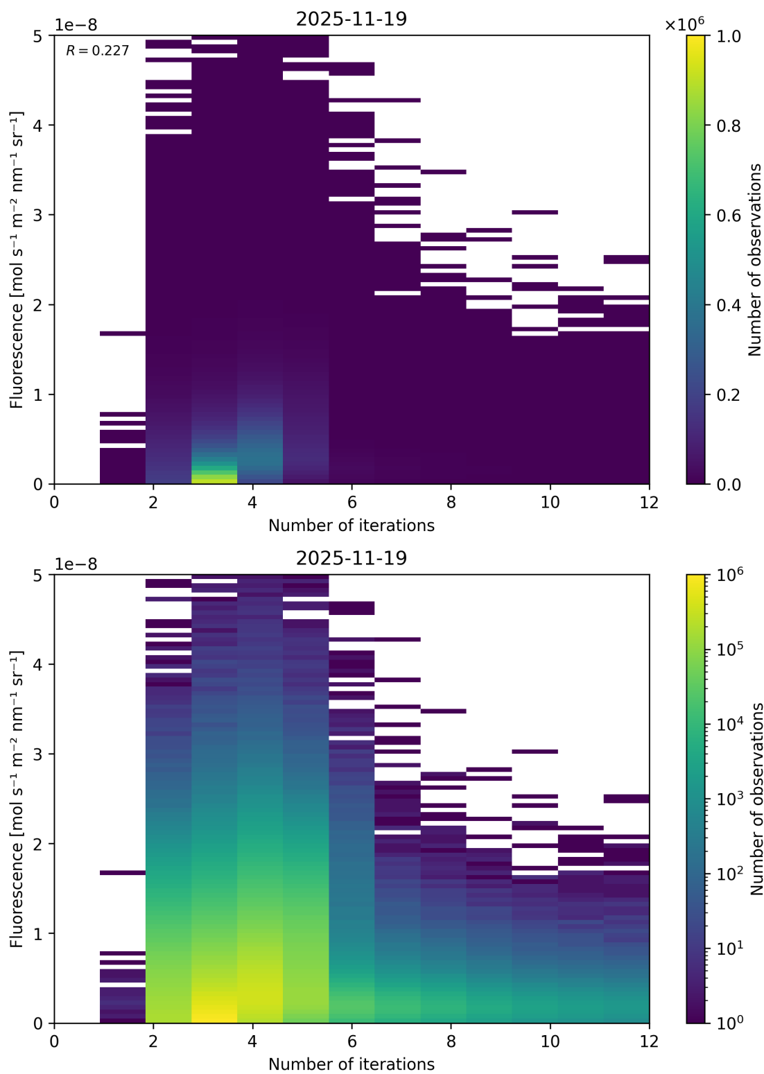
Figure 98: Scatter density plot of “Number of iterations” against “Fluorescence” for 2025-11-18 to 2025-11-20.
