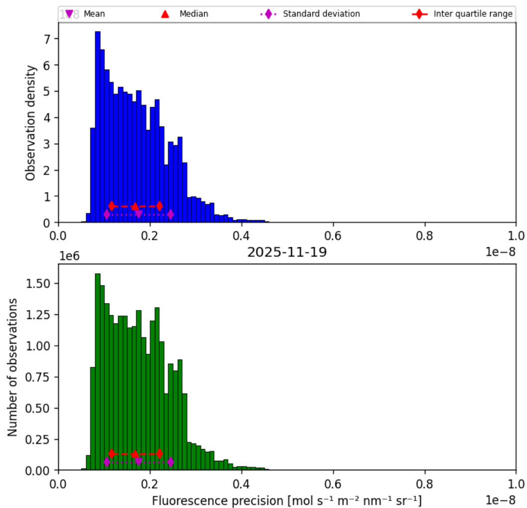
Figure 41: Histogram of “Fluorescence precision” for 2025-11-18 to 2025-11-20
