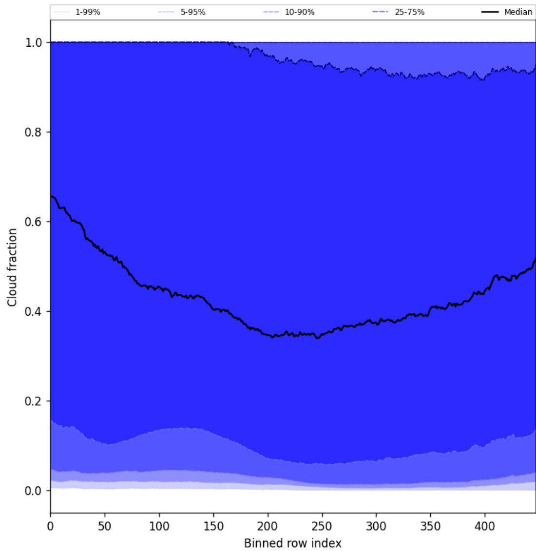
Figure 49: Along track statistics of “Cloud fraction” for 2025-11-18 to 2025-11-20
