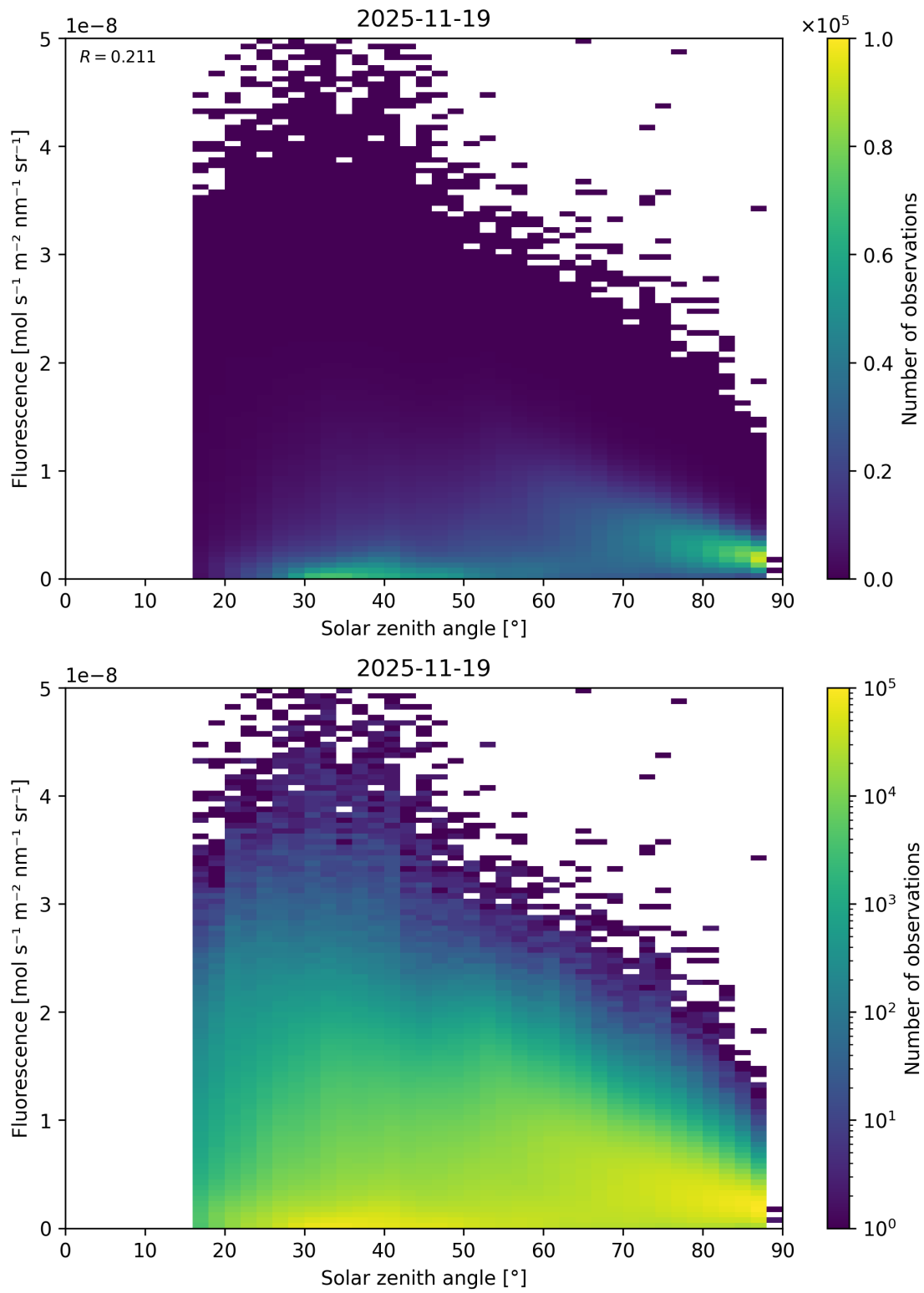
Figure 112: Scatter density plot of “Solar zenith angle” against “Fluorescence” for 2025-11-18 to 2025-11-20.
