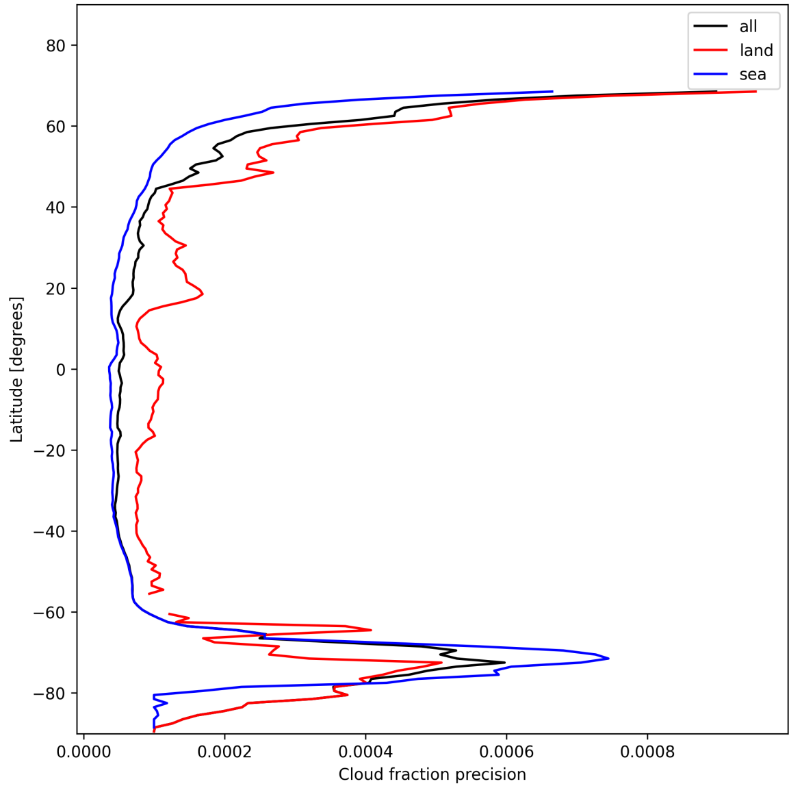
Figure 16: Zonal average of “Cloud fraction precision” for 2025-11-18 to 2025-11-20.
