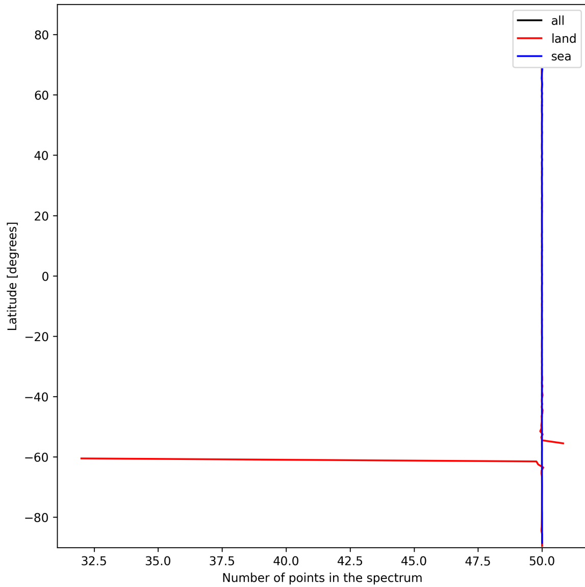
Figure 27: Zonal average of “Number of points in the spectrum” for 2025-11-18 to 2025-11-20.
