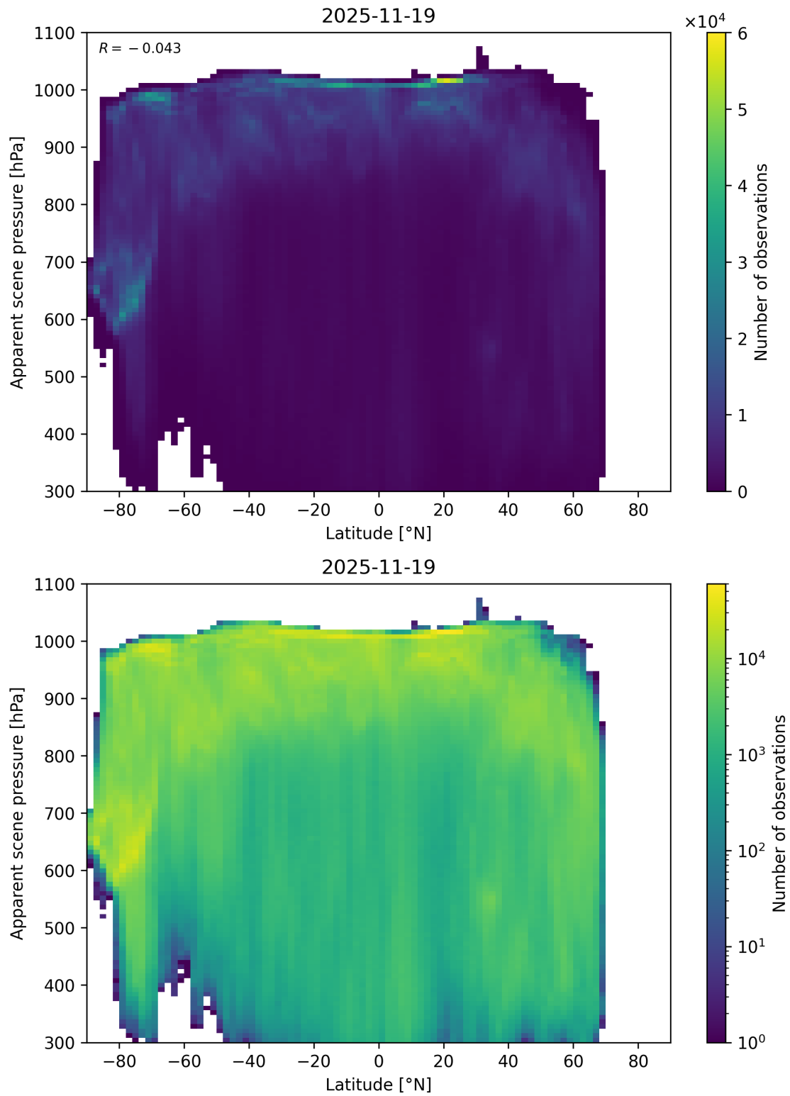
Figure 88: Scatter density plot of “Latitude” against “Apparent scene pressure” for 2025-11-18 to 2025-11-20.
