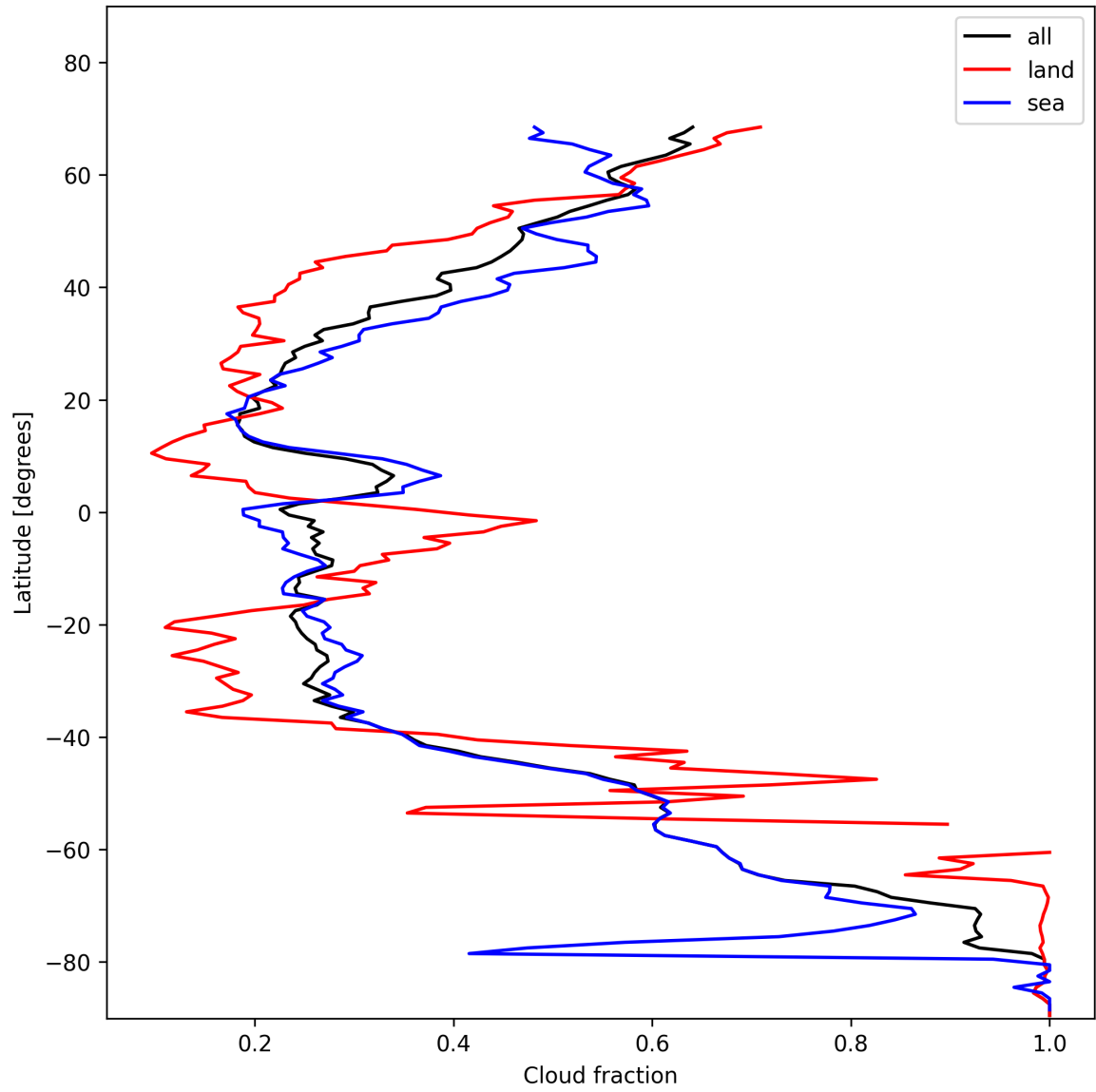
Figure 15: Zonal average of “Cloud fraction” for 2025-11-18 to 2025-11-20.
