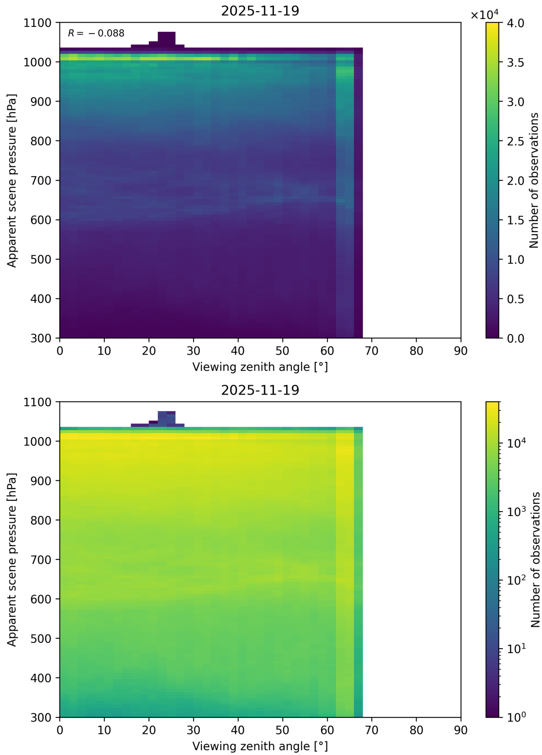
Figure 118: Scatter density plot of “Viewing zenith angle” against “Apparent scene pressure” for 2025-11-18 to 2025-11-20.
