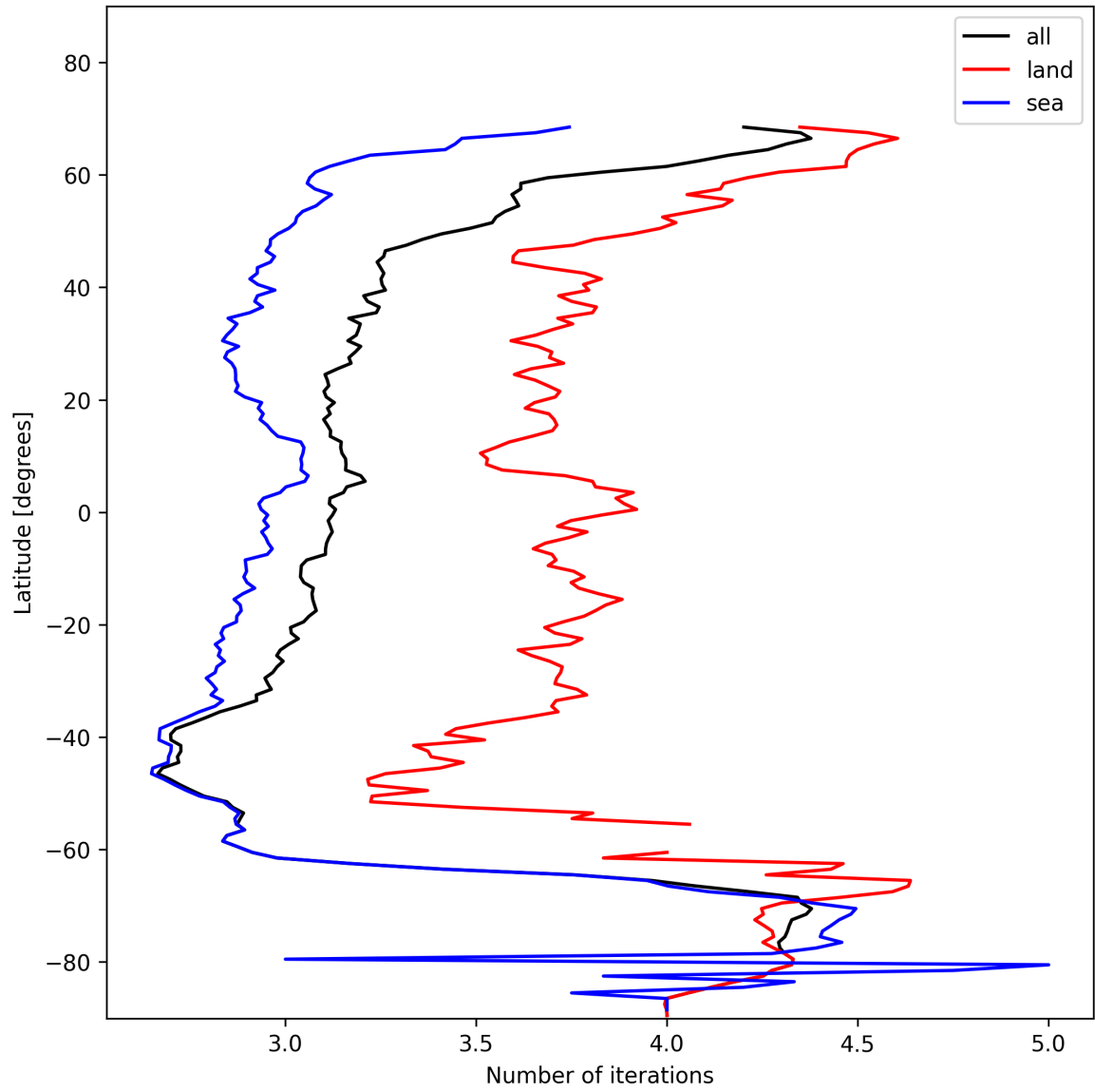
Figure 22: Zonal average of “Number of iterations” for 2025-11-18 to 2025-11-20.
