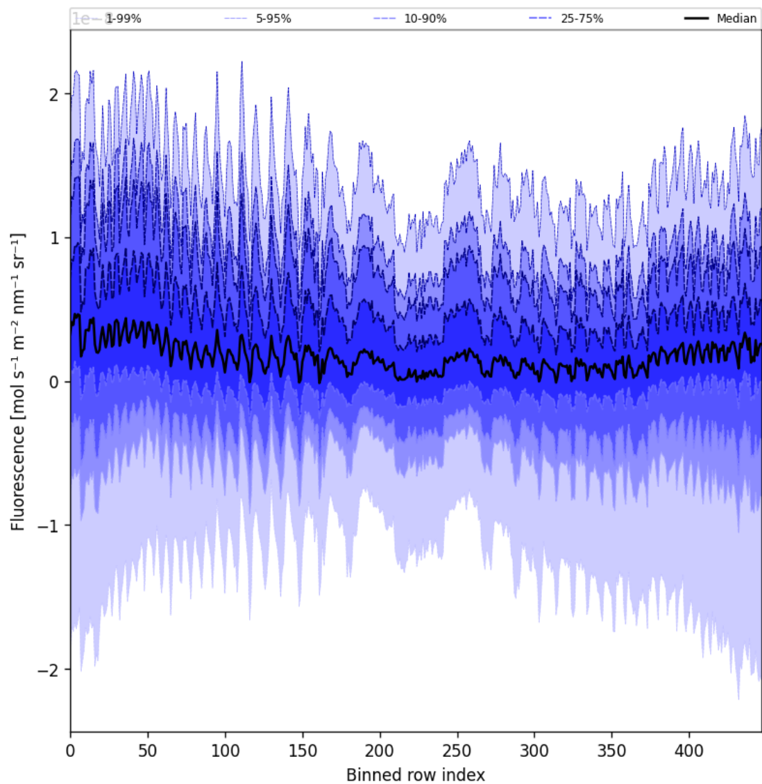
Figure 57: Along track statistics of “Fluorescence” for 2025-11-18 to 2025-11-20
