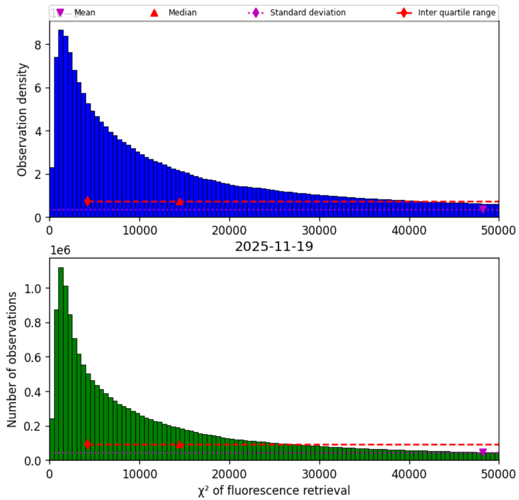
Figure 42: Histogram of “ \chi^2 of fluorescence retrieval” for 2025-11-18 to 2025-11-20
