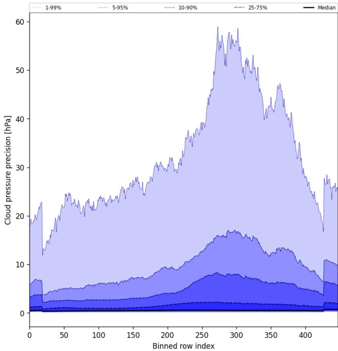
Figure 48: Along track statistics of “Cloud pressure precision” for 2025-11-18 to 2025-11-20
