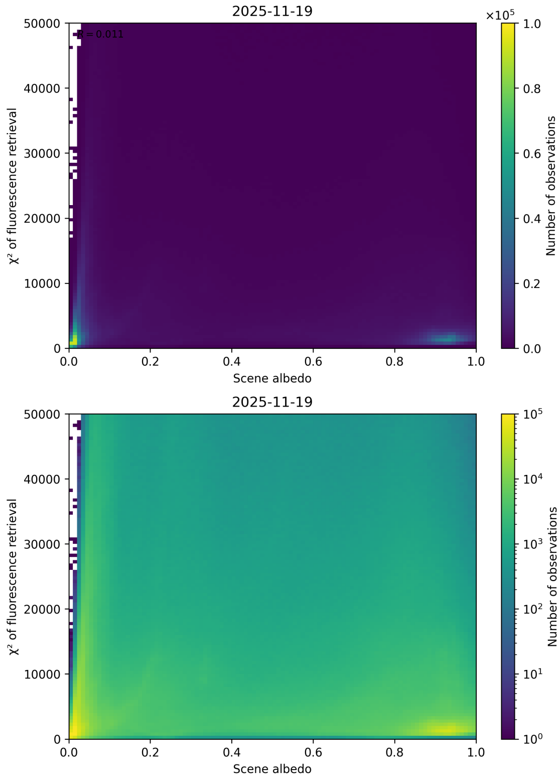
Figure 103: Scatter density plot of “Scene albedo” against “ \chi^2 of fluorescence retrieval” for 2025-11-18 to 2025-11-20.
