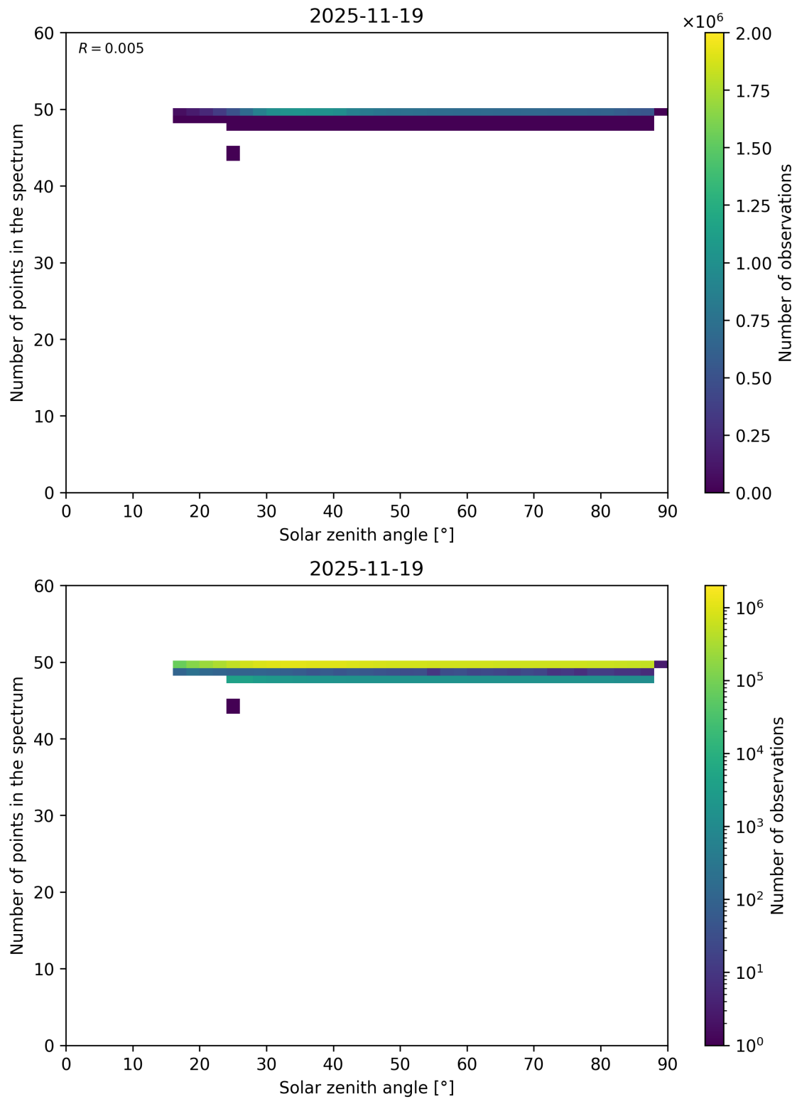
Figure 115: Scatter density plot of “Solar zenith angle” against “Number of points in the spectrum” for 2025-11-18 to 2025-11-20.
