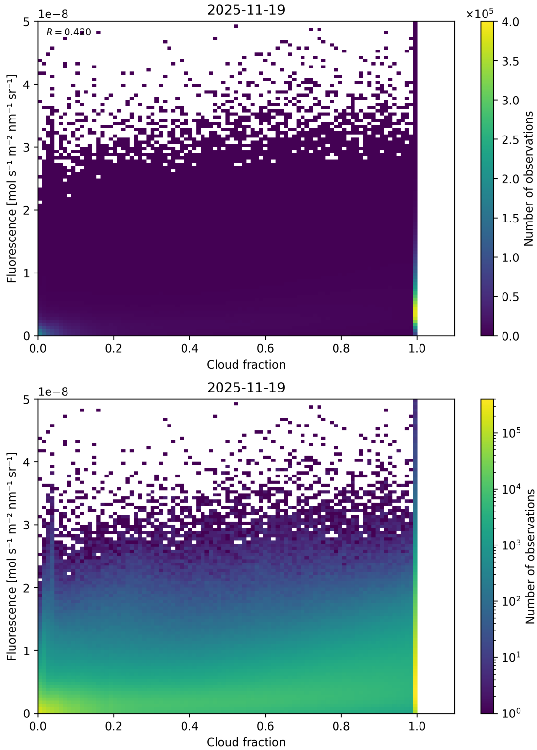
Figure 72: Scatter density plot of “Cloud fraction” against “Fluorescence” for 2025-11-18 to 2025-11-20.
