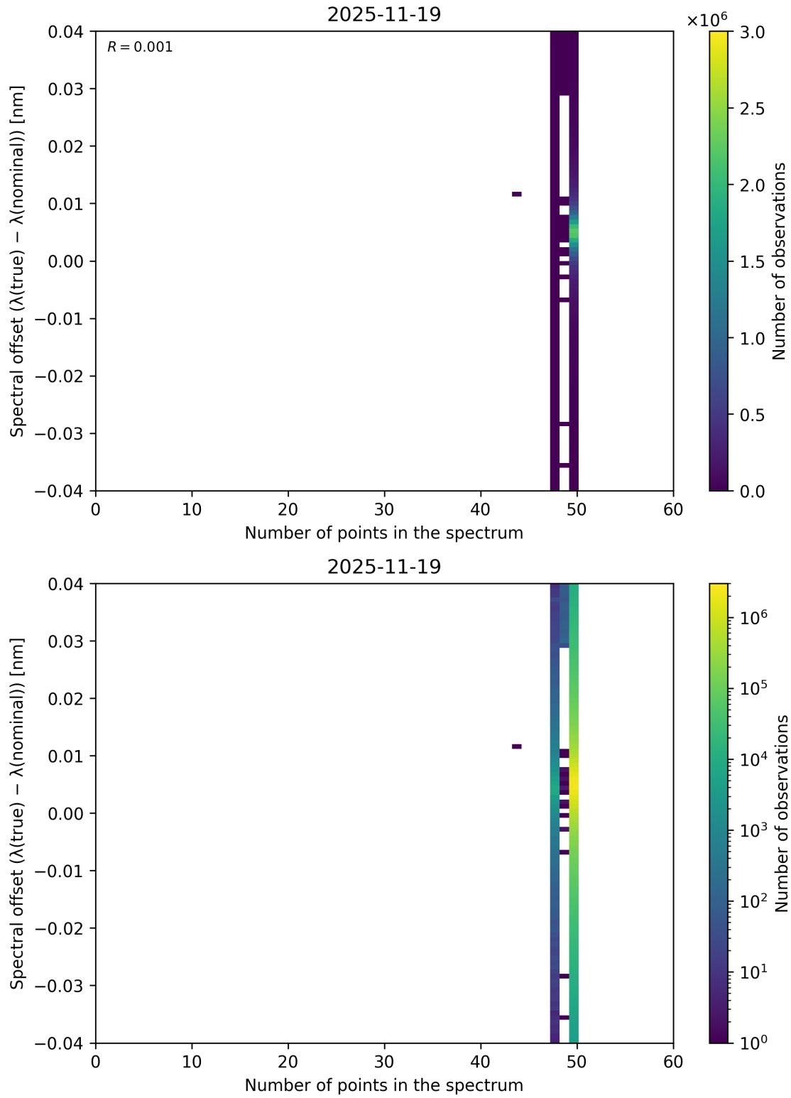
Figure 101: Scatter density plot of “Number of points in the spectrum” against “Spectral offset ( \lambda_{\text{true}} - \lambda_{\text{nominal}} )” for 2025-11-18 to 2025-11-20.
