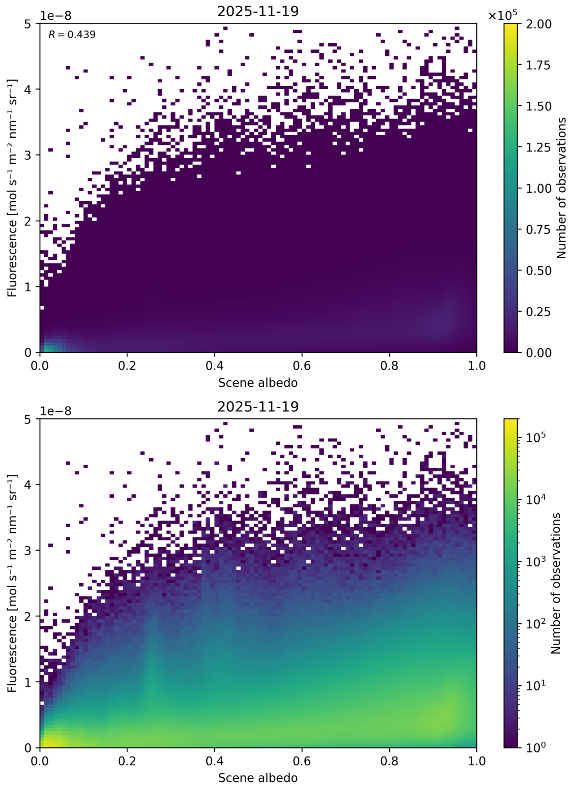
Figure 104: Scatter density plot of “Scene albedo” against “Fluorescence” for 2025-11-18 to 2025-11-20.
