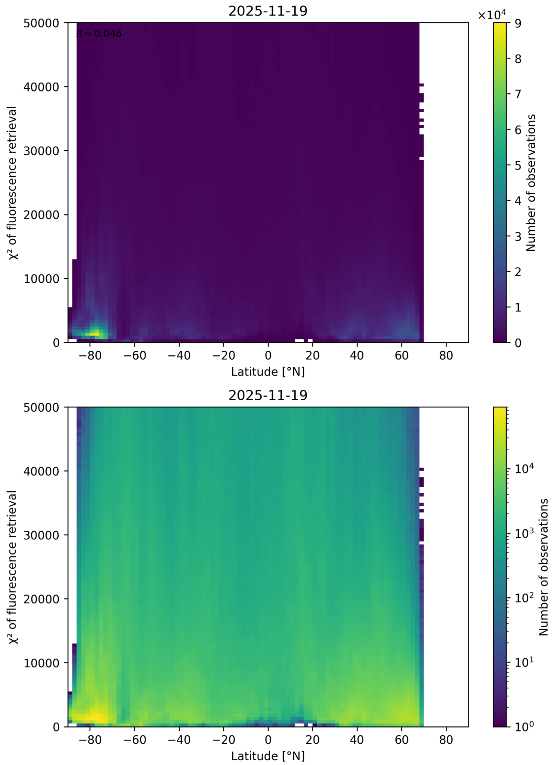
Figure 89: Scatter density plot of “Latitude” against “ \chi^2 of fluorescence retrieval” for 2025-11-18 to 2025-11-20.
