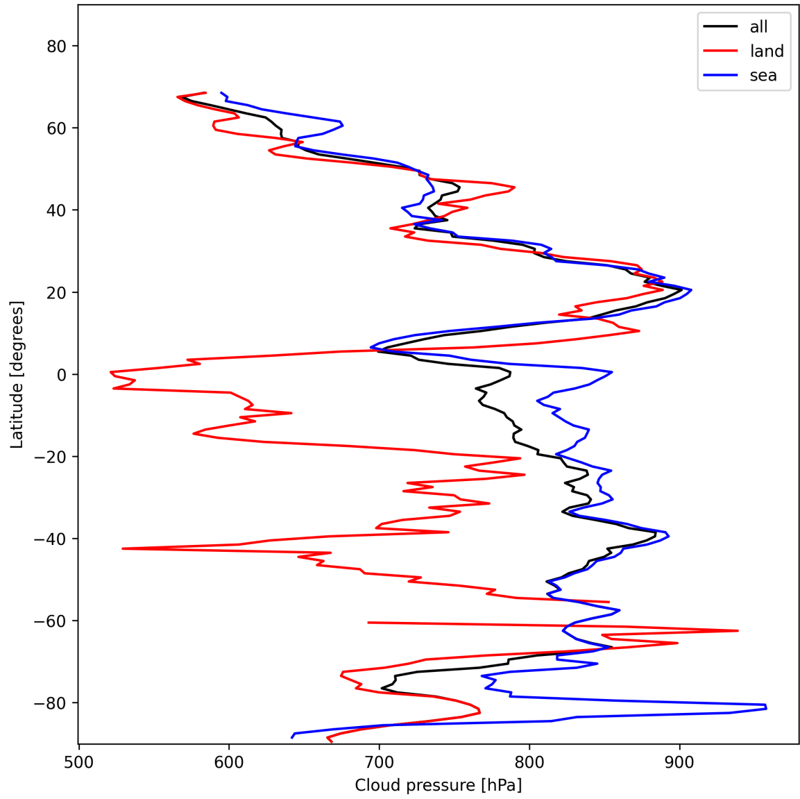
Figure 13: Zonal average of “Cloud pressure” for 2025-11-18 to 2025-11-20.
