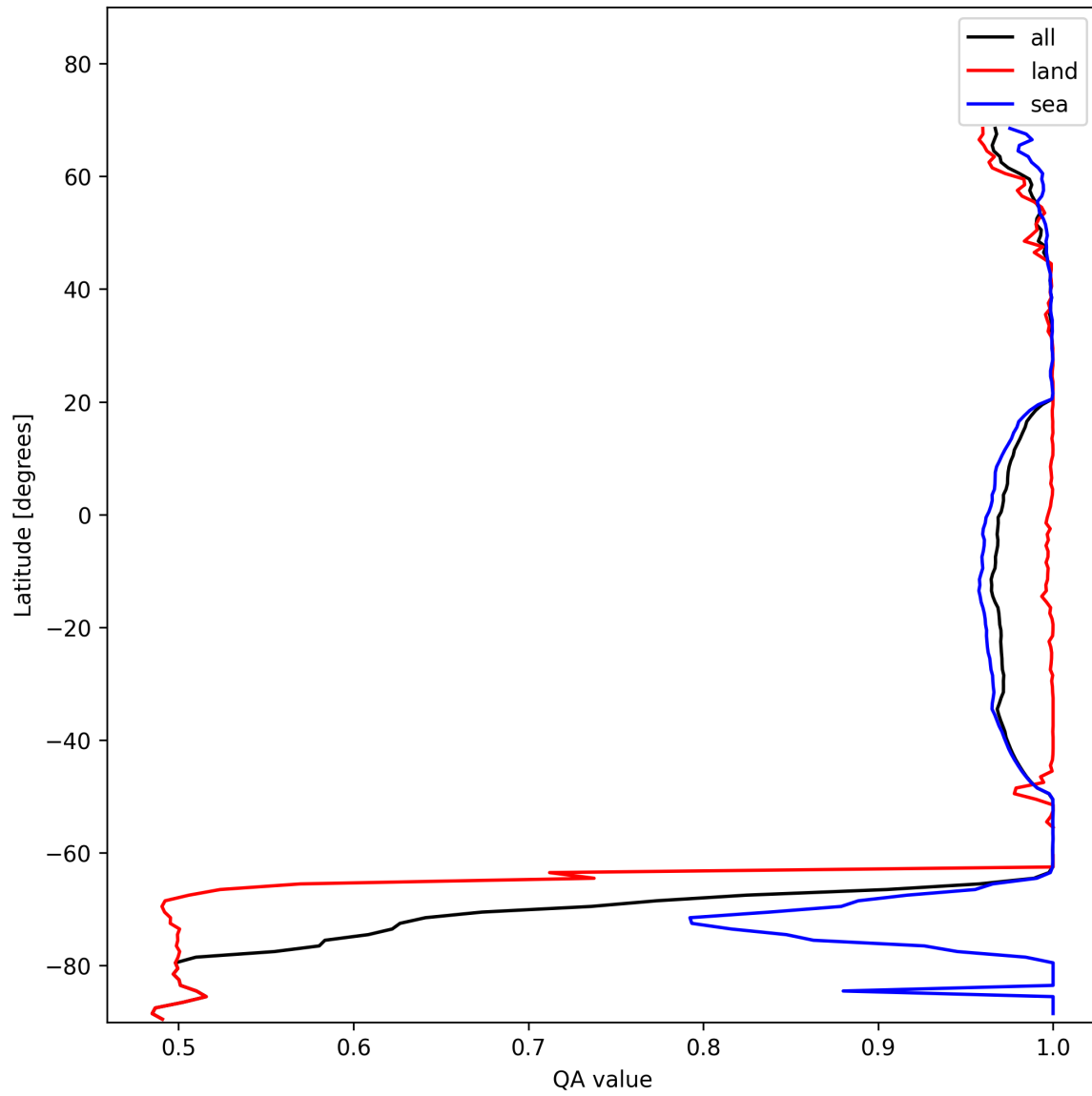
Figure 12: Zonal average of “QA value” for 2025-11-18 to 2025-11-20.
