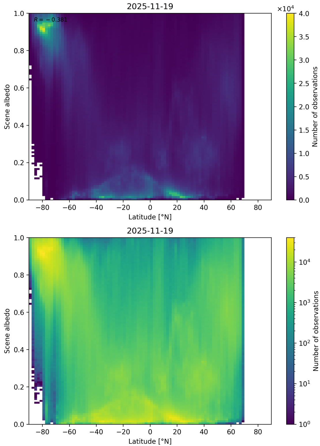
Figure 95: Scatter density plot of “Latitude” against “Scene albedo” for 2025-11-18 to 2025-11-20.
