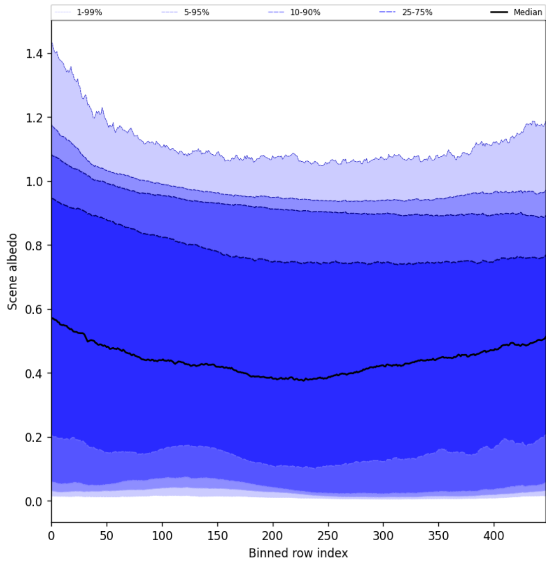
Figure 51: Along track statistics of “Scene albedo” for 2025-11-18 to 2025-11-20
