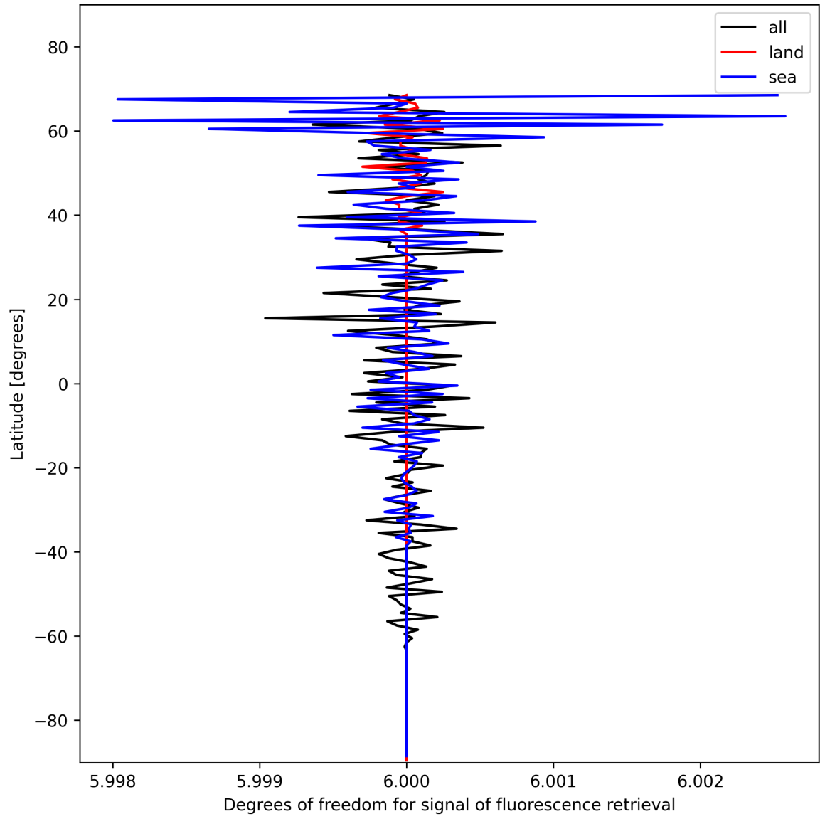
Figure 26: Zonal average of “Degrees of freedom for signal of fluorescence retrieval” for 2025-11-18 to 2025-11-20.
