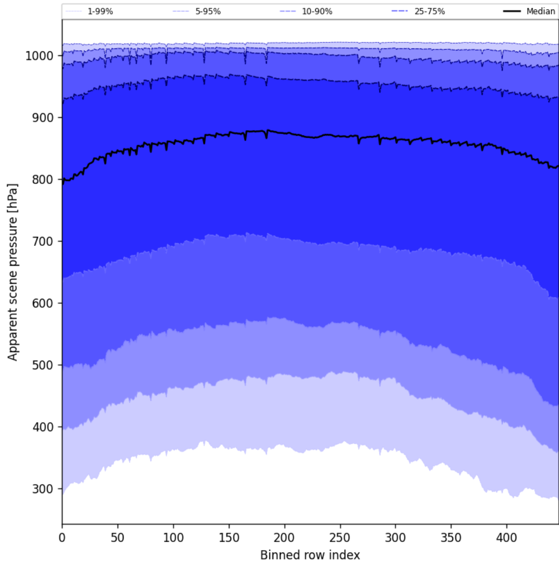
Figure 53: Along track statistics of “Apparent scene pressure” for 2025-11-18 to 2025-11-20
