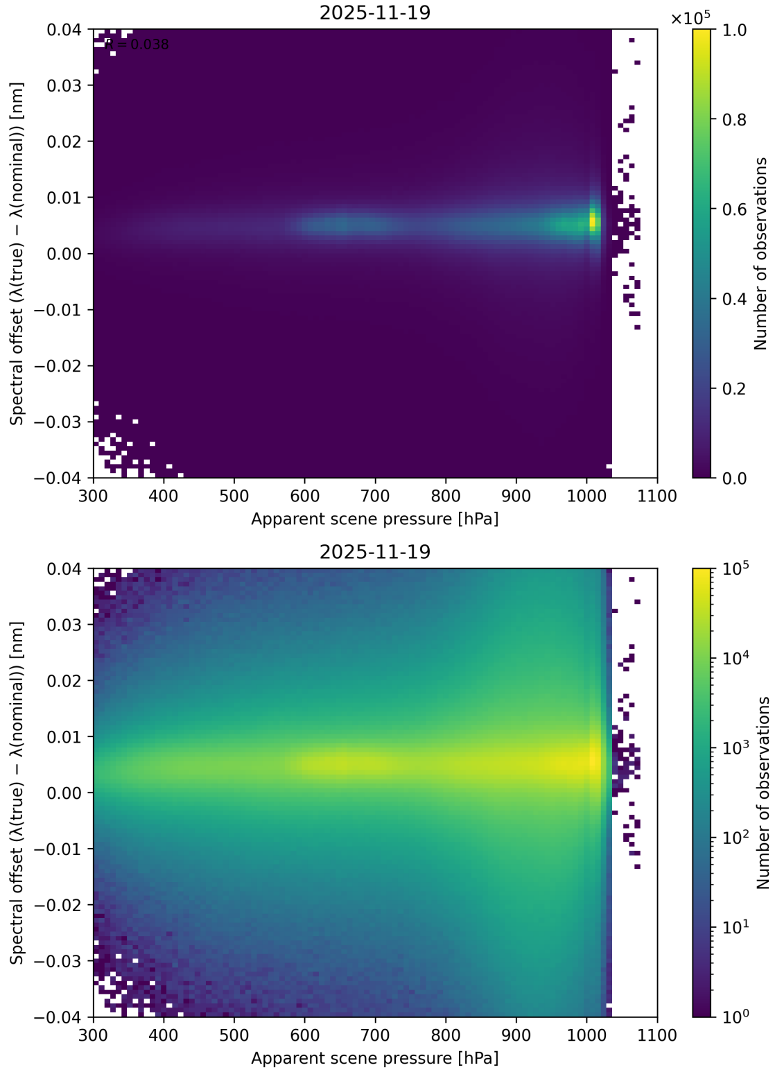
Figure 67: Scatter density plot of “Apparent scene pressure” against “Spectral offset ( \lambda_{\text{true}} - \lambda_{\text{nominal}} )” for 2025-11-18 to 2025-11-20.
