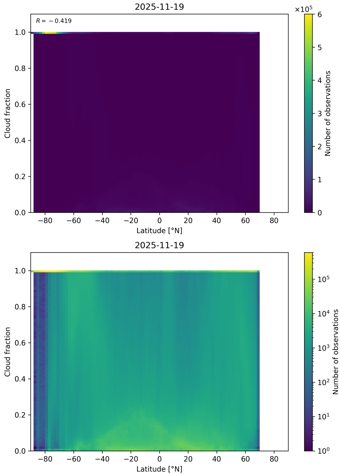
Figure 90: Scatter density plot of “Latitude” against “Cloud fraction” for 2025-11-18 to 2025-11-20.
