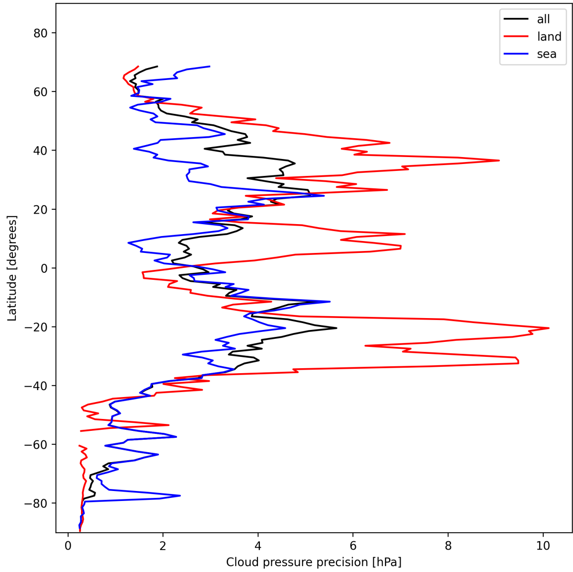
Figure 14: Zonal average of “Cloud pressure precision” for 2025-11-18 to 2025-11-20.
