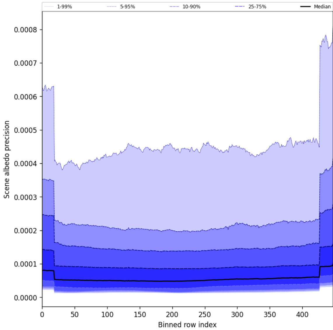
Figure 52: Along track statistics of “Scene albedo precision” for 2025-11-18 to 2025-11-20
