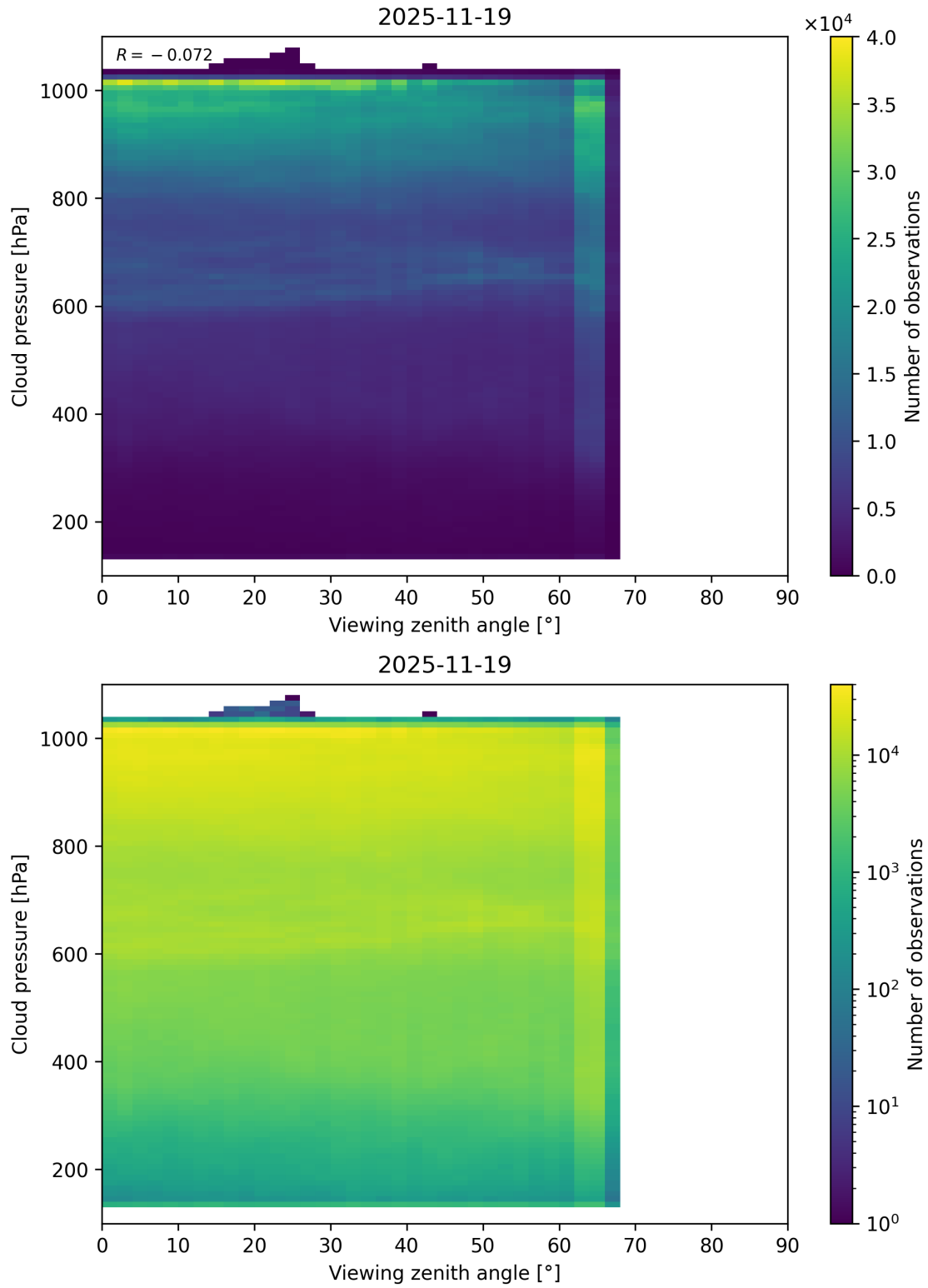
Figure 121: Scatter density plot of “Viewing zenith angle” against “Cloud pressure” for 2025-11-18 to 2025-11-20.
