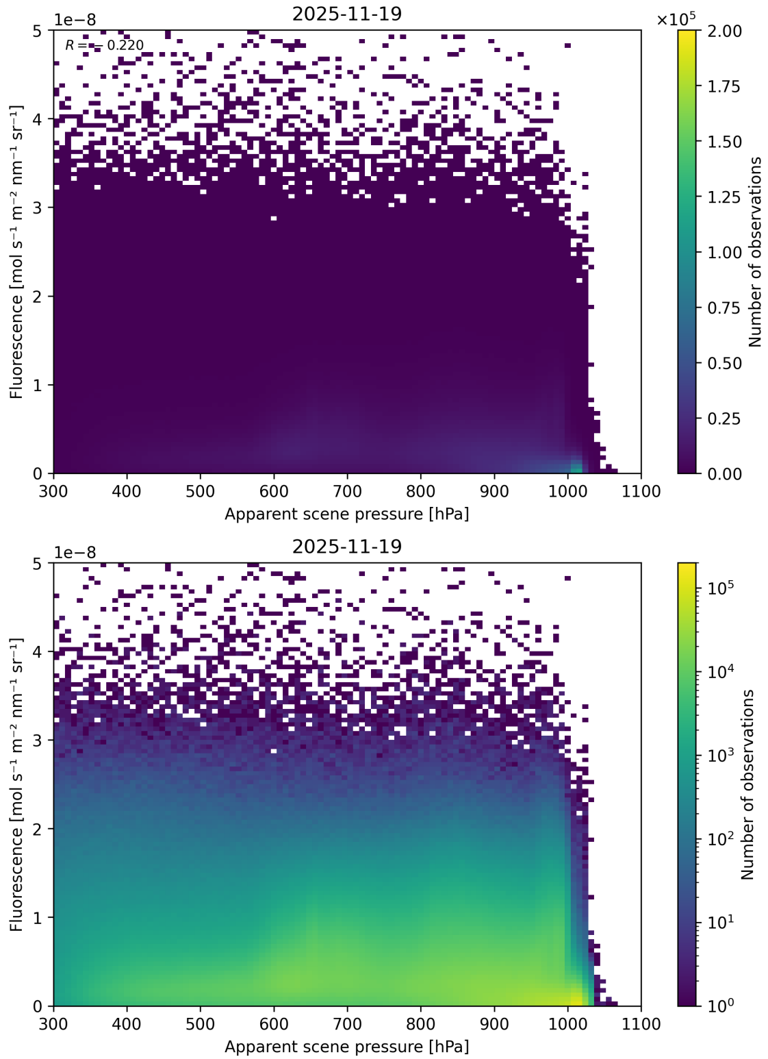
Figure 64: Scatter density plot of “Apparent scene pressure” against “Fluorescence” for 2025-11-18 to 2025-11-20.
