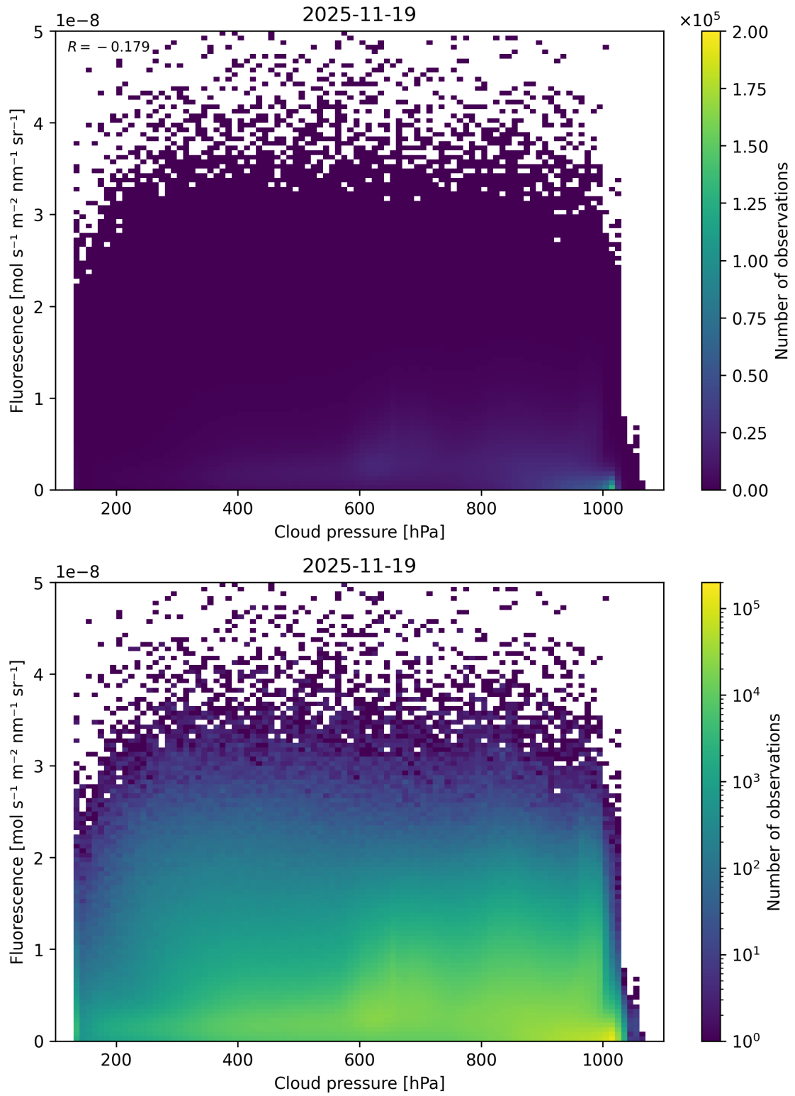
Figure 80: Scatter density plot of “Cloud pressure” against “Fluorescence” for 2025-11-18 to 2025-11-20.
