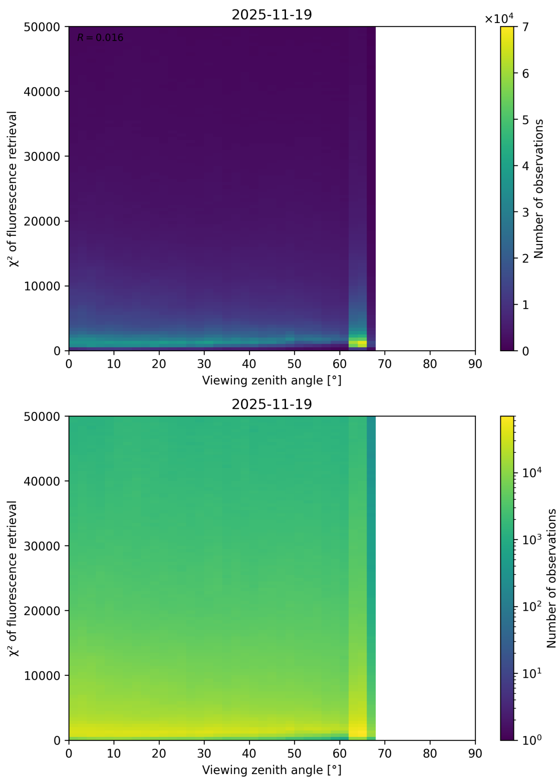
Figure 119: Scatter density plot of “Viewing zenith angle” against “ \chi^2 of fluorescence retrieval” for 2025-11-18 to 2025-11-20.
