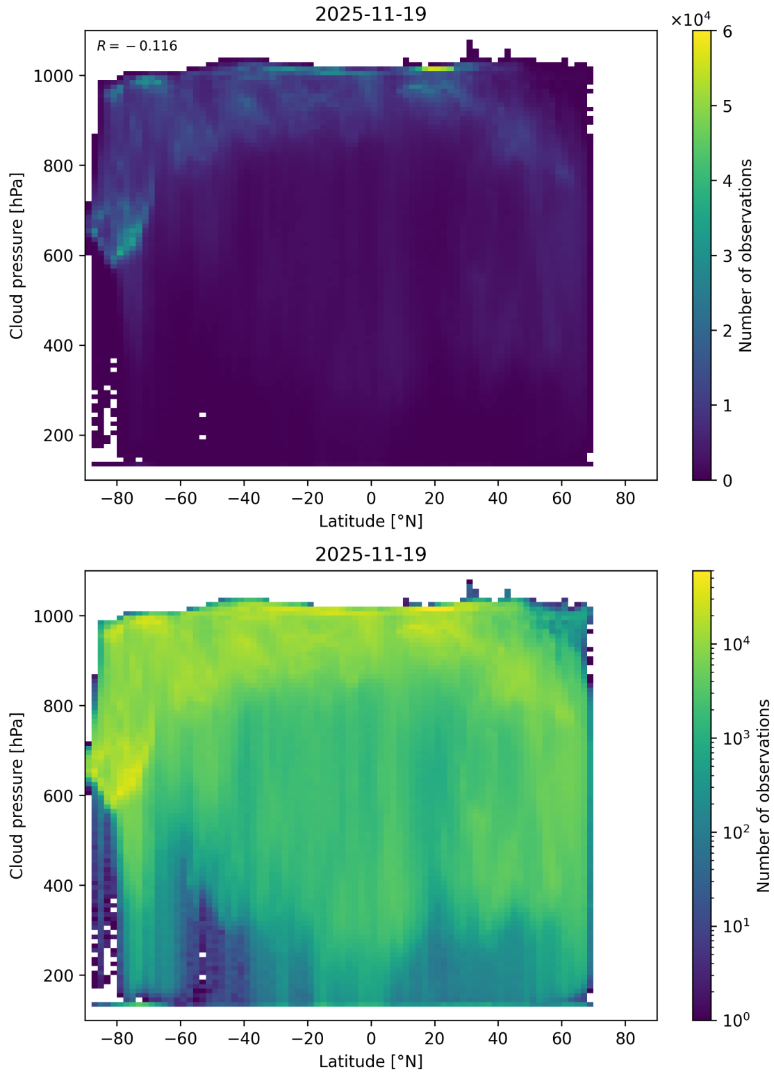
Figure 91: Scatter density plot of “Latitude” against “Cloud pressure” for 2025-11-18 to 2025-11-20.
