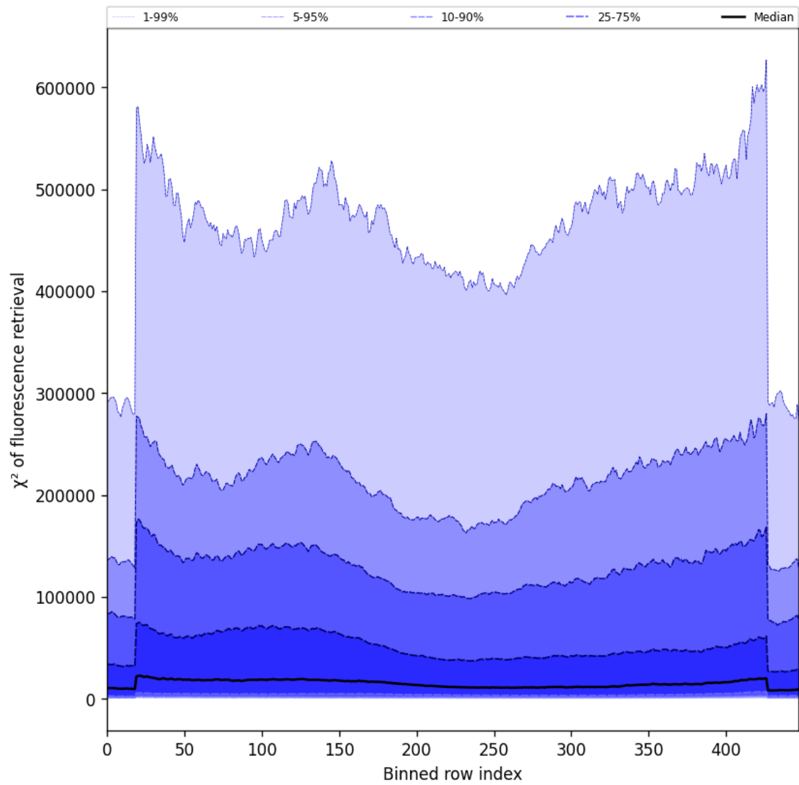
Figure 59: Along track statistics of “ \chi^2 of fluorescence retrieval” for 2025-11-18 to 2025-11-20
