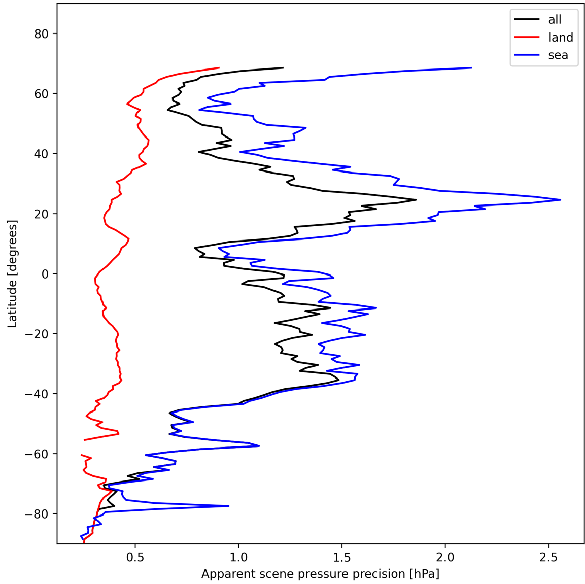
Figure 20: Zonal average of “Apparent scene pressure precision” for 2025-11-18 to 2025-11-20.
