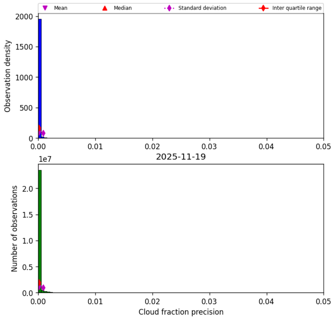
Figure 33: Histogram of “Cloud fraction precision” for 2025-11-18 to 2025-11-20
