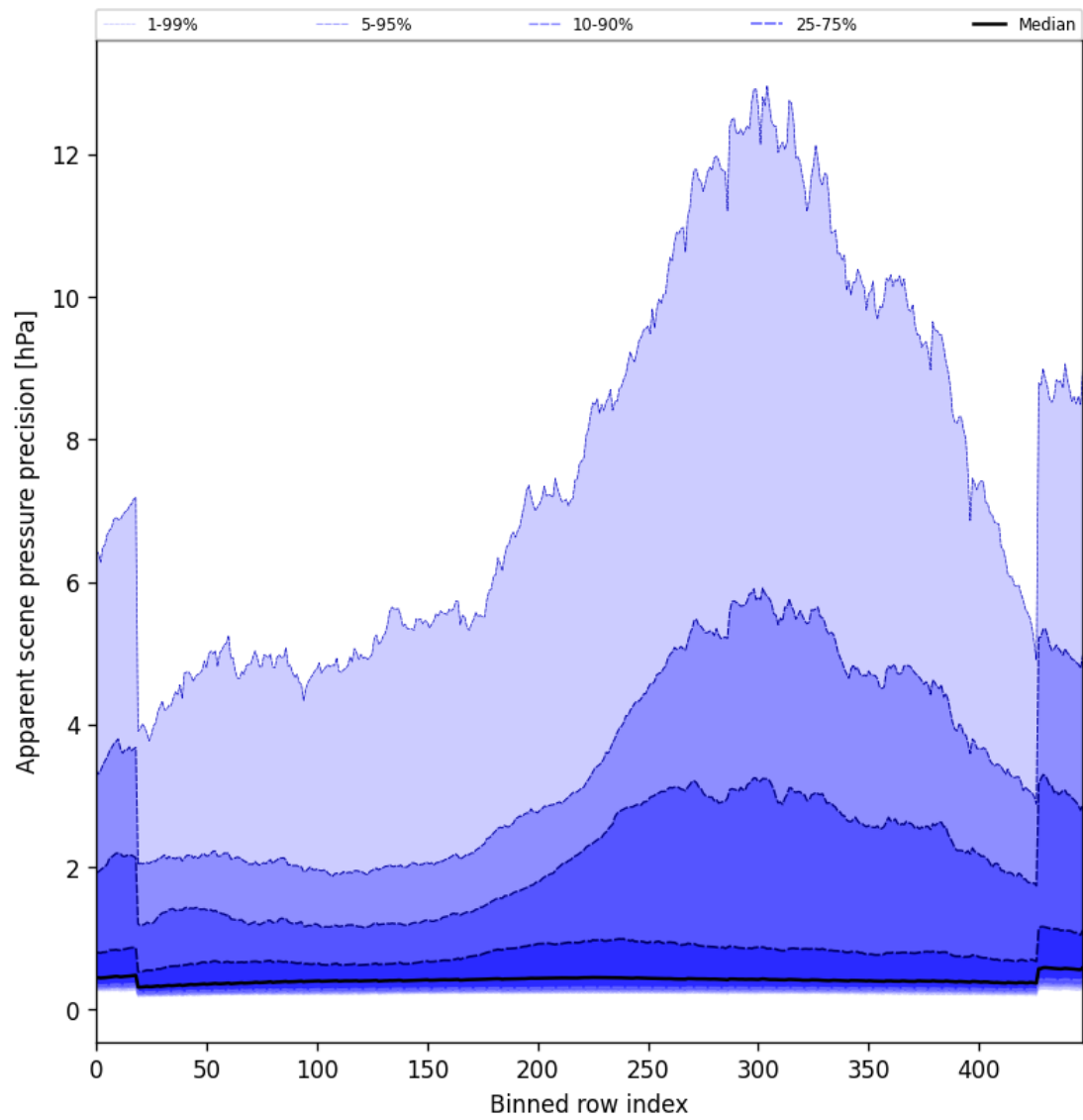
Figure 54: Along track statistics of “Apparent scene pressure precision” for 2025-11-18 to 2025-11-20
