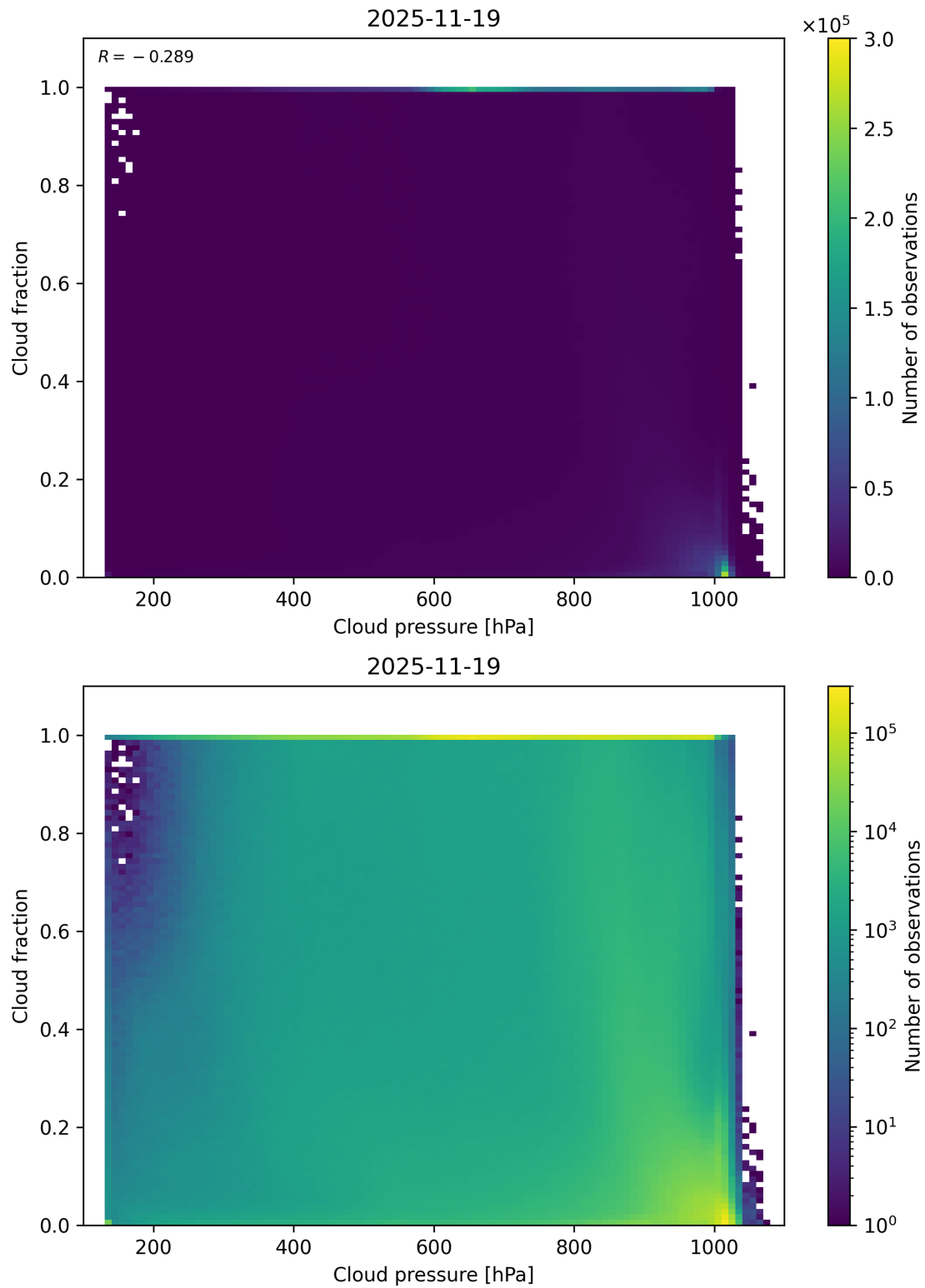
Figure 79: Scatter density plot of “Cloud pressure” against “Cloud fraction” for 2025-11-18 to 2025-11-20.
