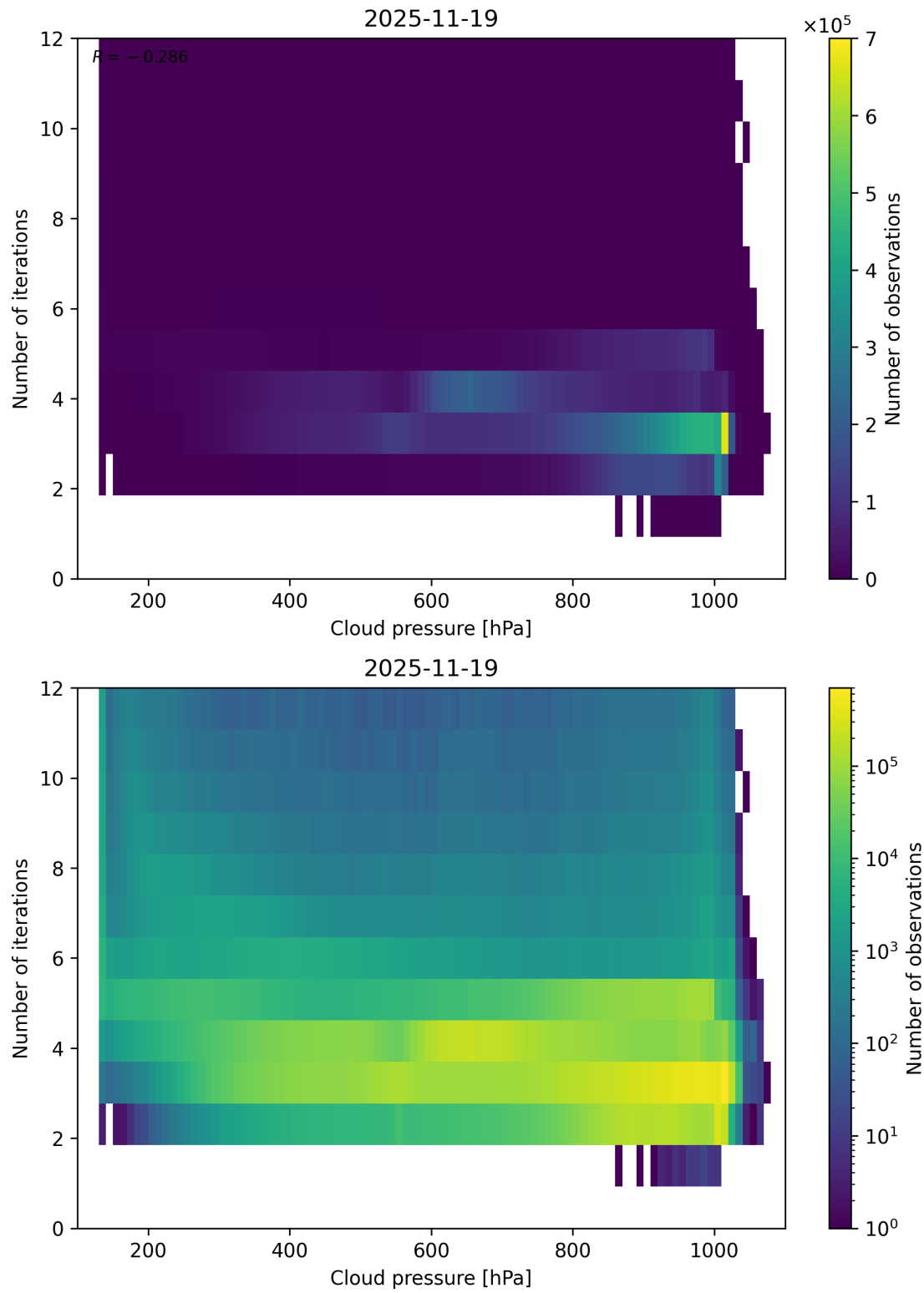
Figure 81: Scatter density plot of “Cloud pressure” against “Number of iterations” for 2025-11-18 to 2025-11-20.
