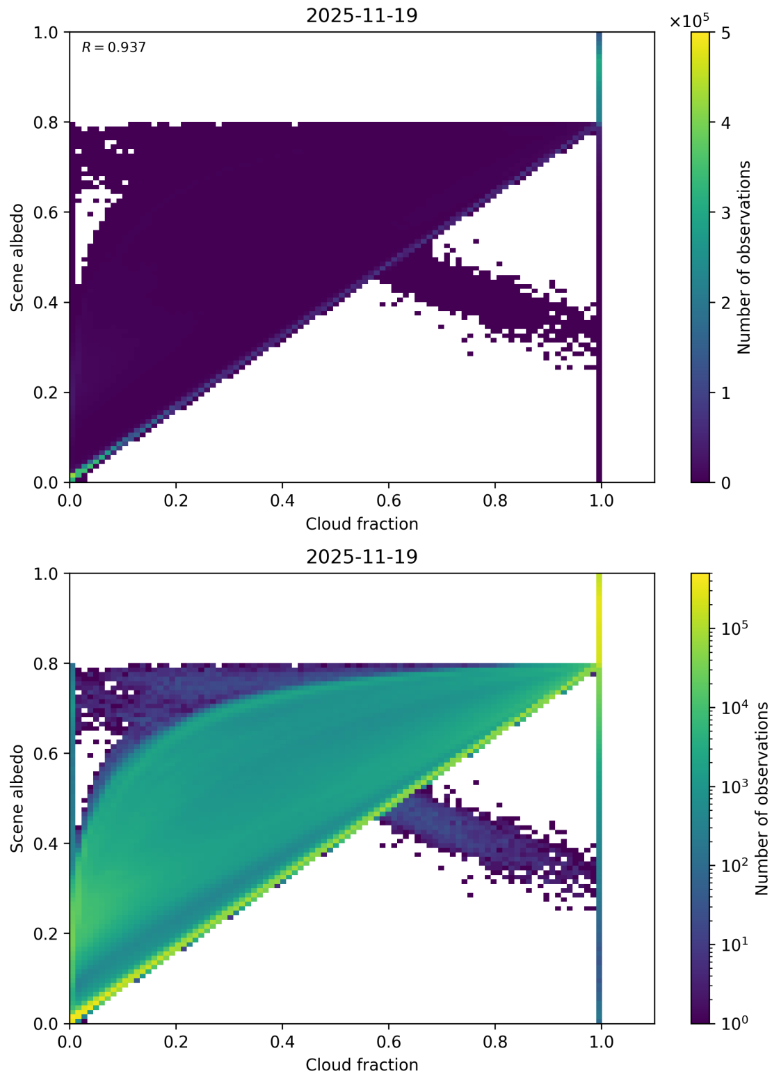
Figure 75: Scatter density plot of “Cloud fraction” against “Scene albedo” for 2025-11-18 to 2025-11-20.
