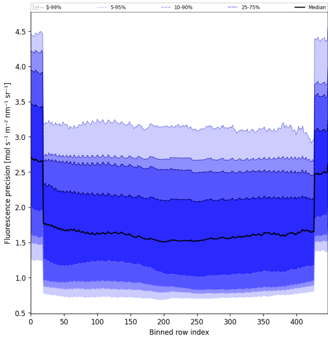
Figure 58: Along track statistics of “Fluorescence precision” for 2025-11-18 to 2025-11-20
