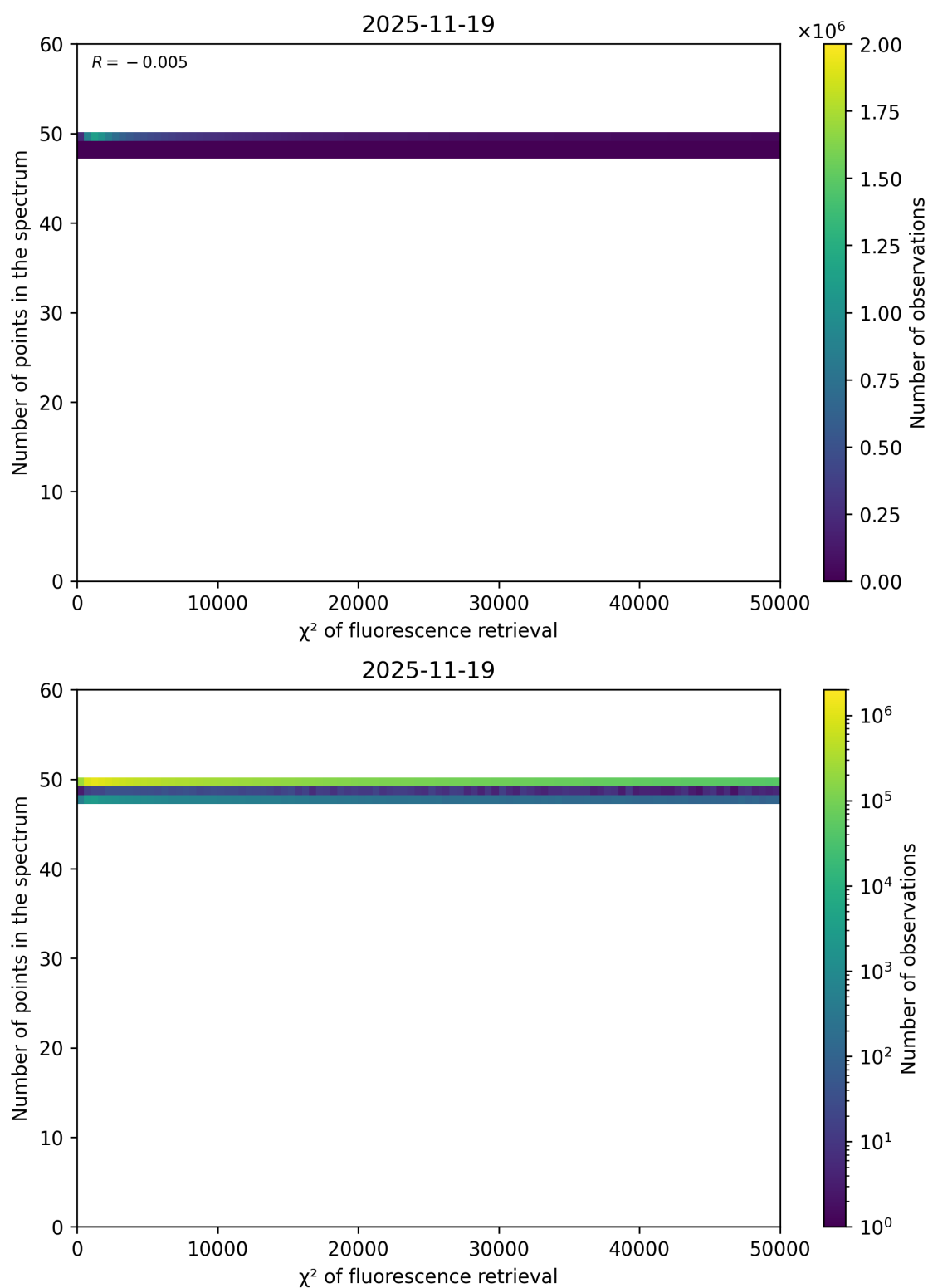
Figure 68: Scatter density plot of “ \chi^2 of fluorescence retrieval” against “Number of points in the spectrum” for 2025-11-18 to 2025-11-20.
