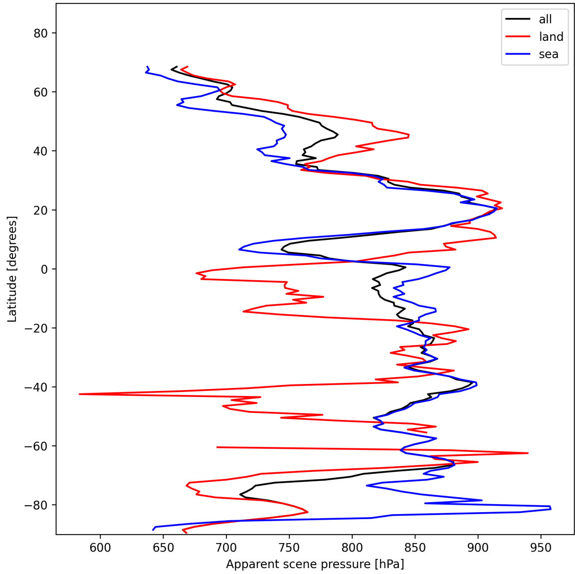
Figure 19: Zonal average of “Apparent scene pressure” for 2025-11-18 to 2025-11-20.
