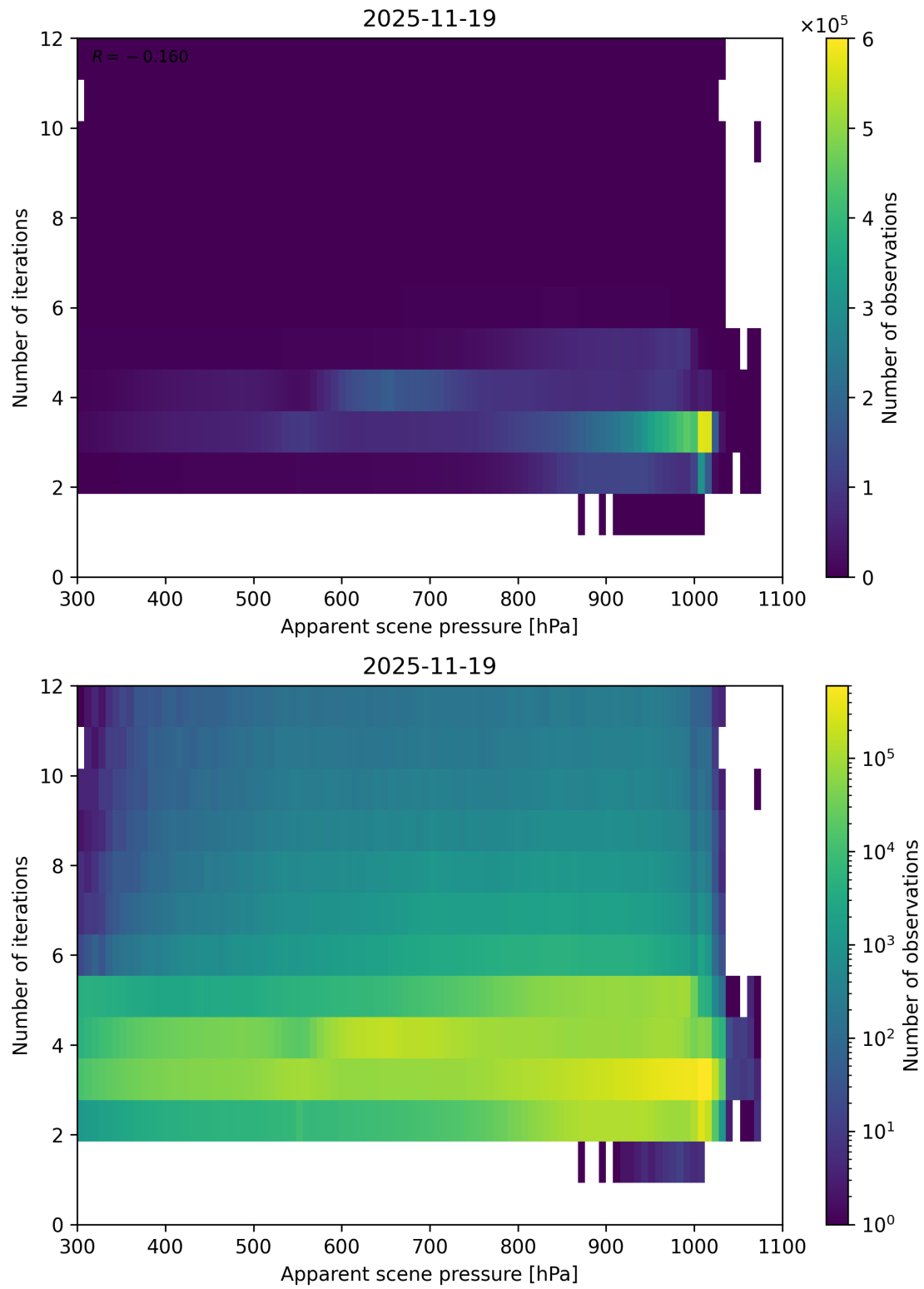
Figure 65: Scatter density plot of “Apparent scene pressure” against “Number of iterations” for 2025-11-18 to 2025-11-20.
