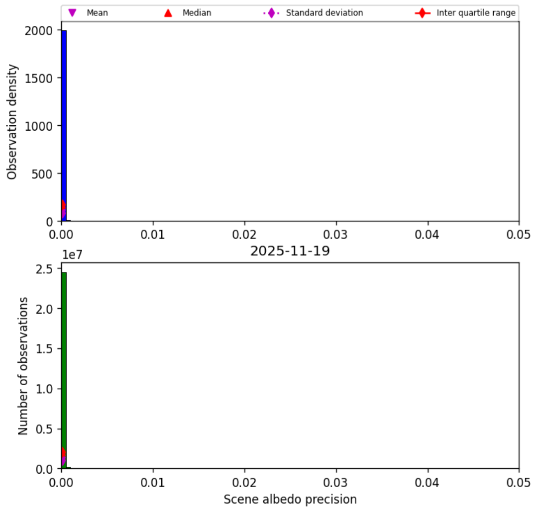
Figure 35: Histogram of “Scene albedo precision” for 2025-11-18 to 2025-11-20
