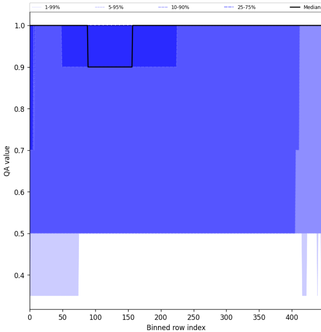
Figure 46: Along track statistics of “QA value” for 2025-11-18 to 2025-11-20
