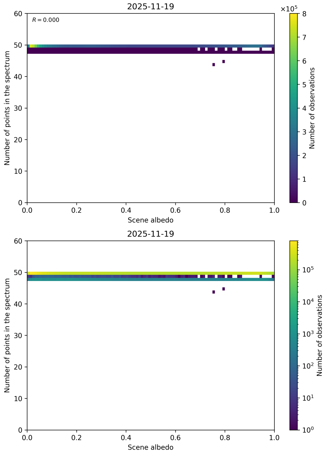
Figure 106: Scatter density plot of “Scene albedo” against “Number of points in the spectrum” for 2025-11-18 to 2025-11-20.
