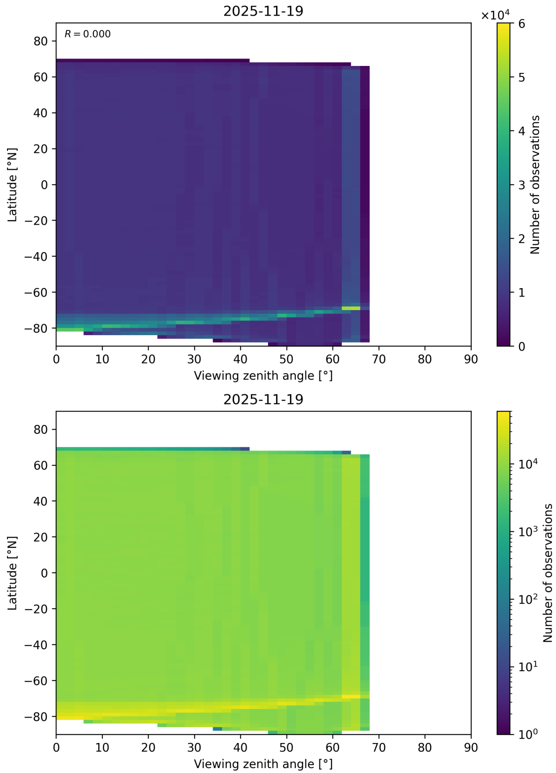
Figure 123: Scatter density plot of “Viewing zenith angle” against “Latitude” for 2025-11-18 to 2025-11-20.
