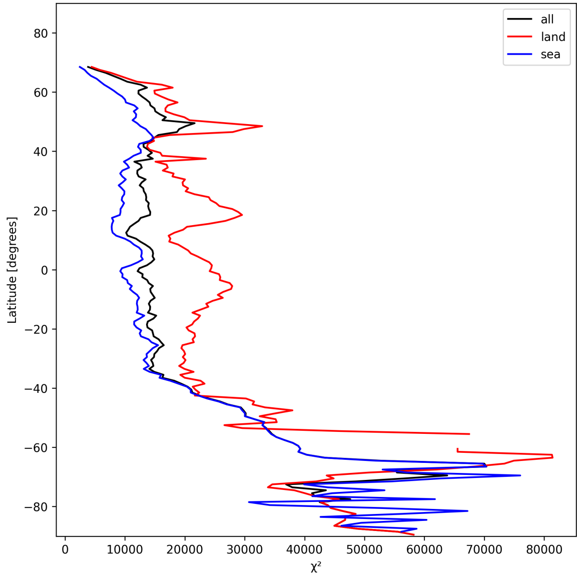
Figure 21: Zonal average of “ \chi^2 ” for 2025-11-18 to 2025-11-20.
