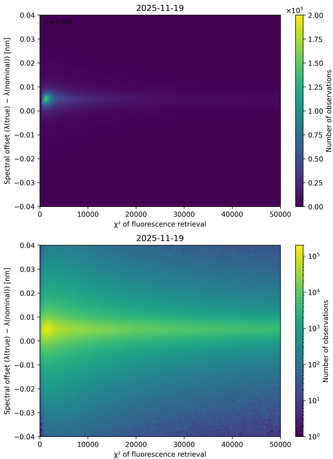
Figure 69: Scatter density plot of “ \chi^2 of fluorescence retrieval” against “Spectral offset ( \lambda_{\text{true}} - \lambda_{\text{nominal}} )” for 2025-11-18 to 2025-11-20.
