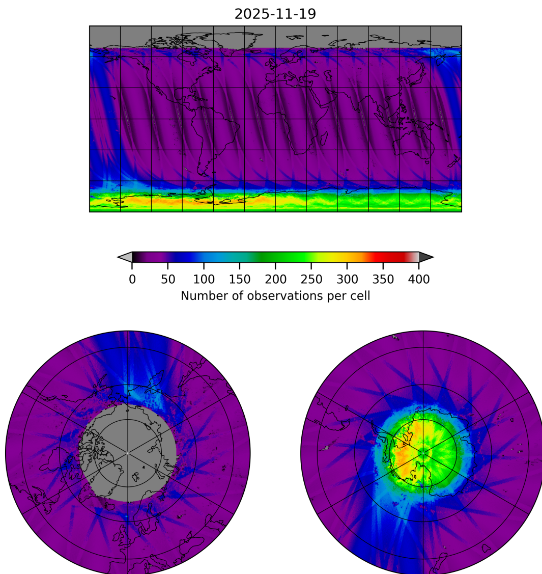
Figure 11: Map of the number of observations for 2025-11-18 to 2025-11-20
