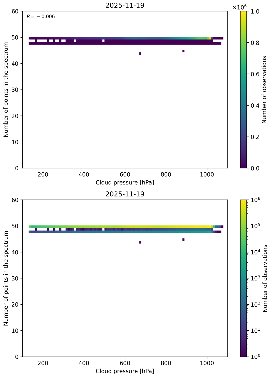
Figure 82: Scatter density plot of “Cloud pressure” against “Number of points in the spectrum” for 2025-11-18 to 2025-11-20.
