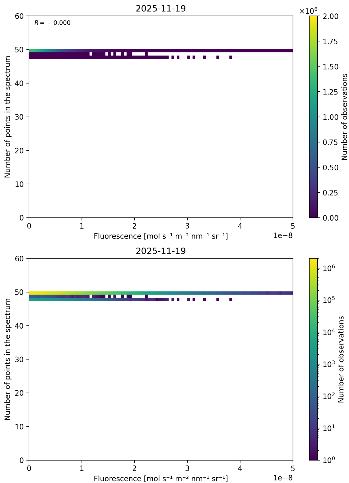
Figure 86: Scatter density plot of “Fluorescence” against “Number of points in the spectrum” for 2025-11-18 to 2025-11-20.
