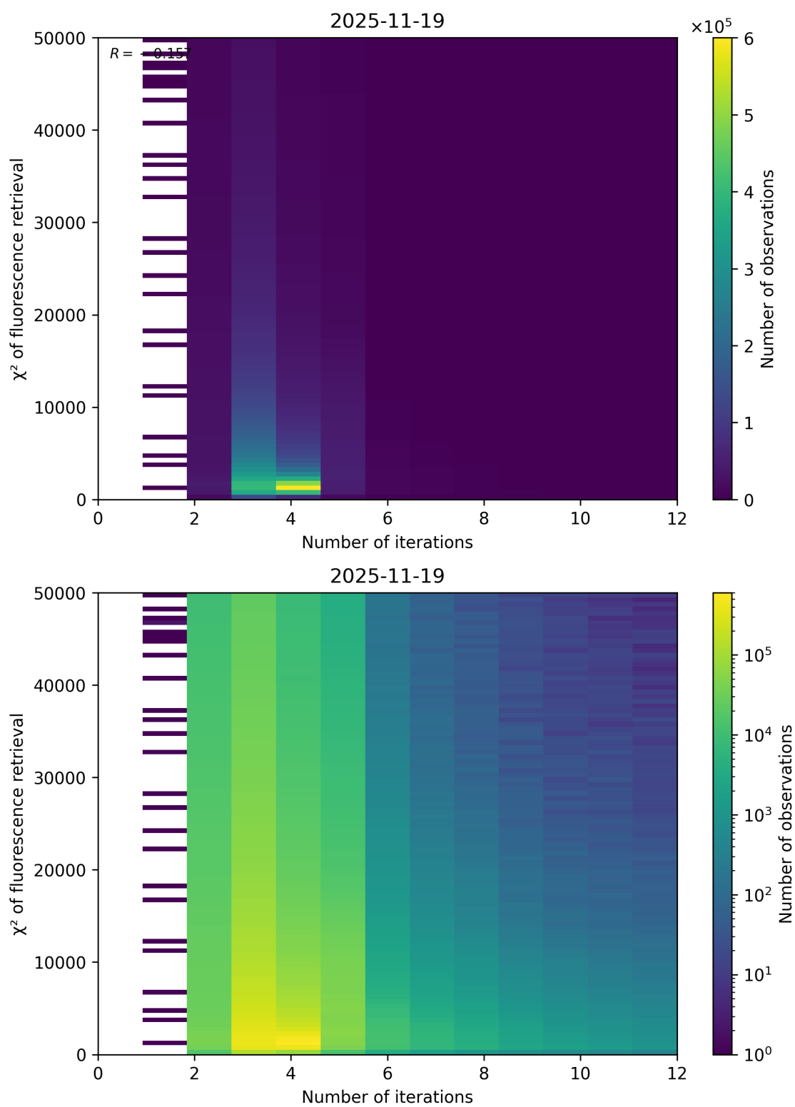
Figure 97: Scatter density plot of “Number of iterations” against “ \chi^2 of fluorescence retrieval” for 2025-11-18 to 2025-11-20.
