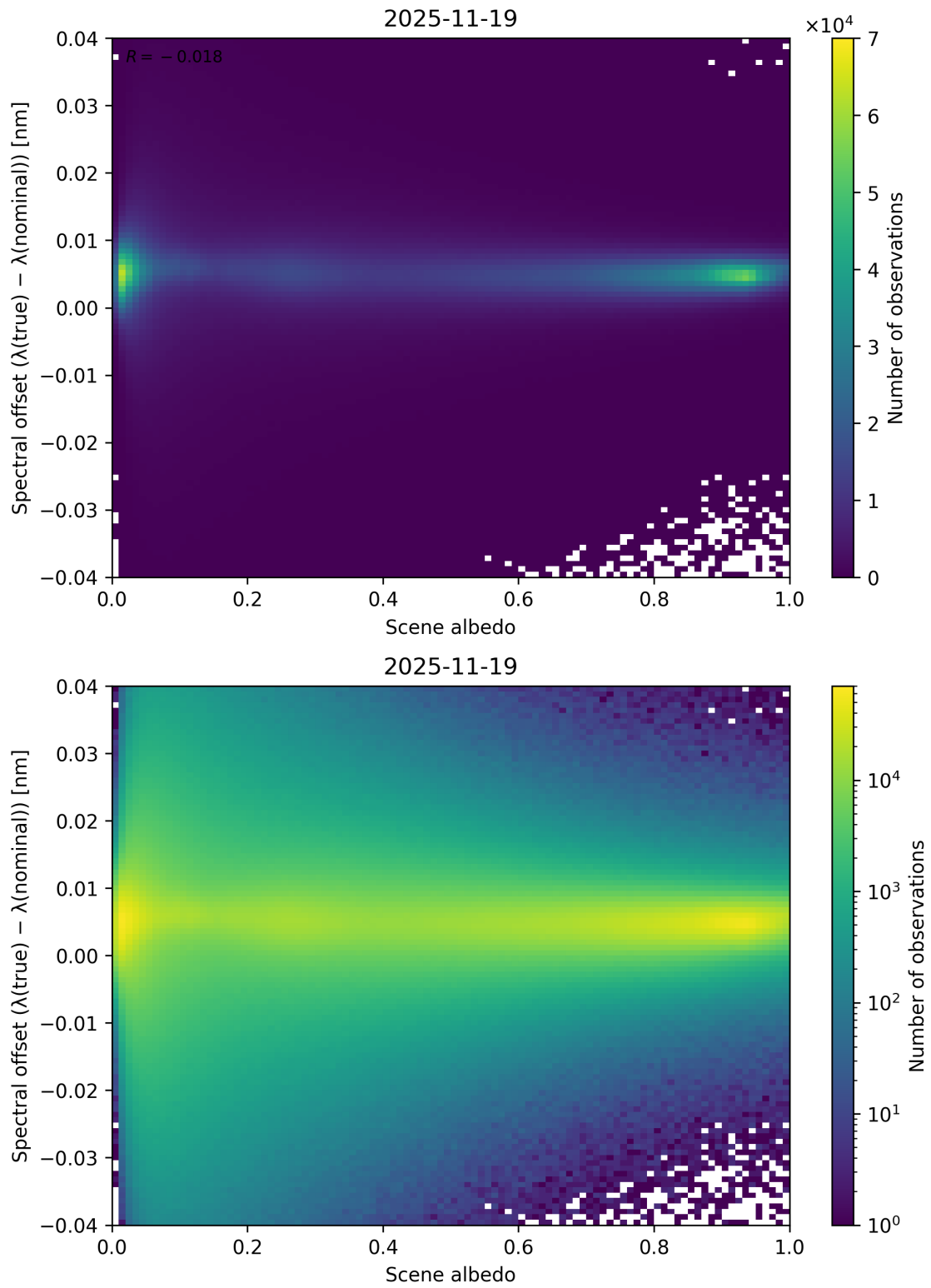
Figure 107: Scatter density plot of “Scene albedo” against “Spectral offset ( \lambda_{\text{true}} - \lambda_{\text{nominal}} )” for 2025-11-18 to 2025-11-20.
