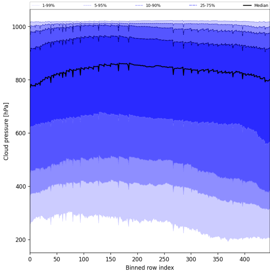
Figure 47: Along track statistics of “Cloud pressure” for 2025-11-18 to 2025-11-20
