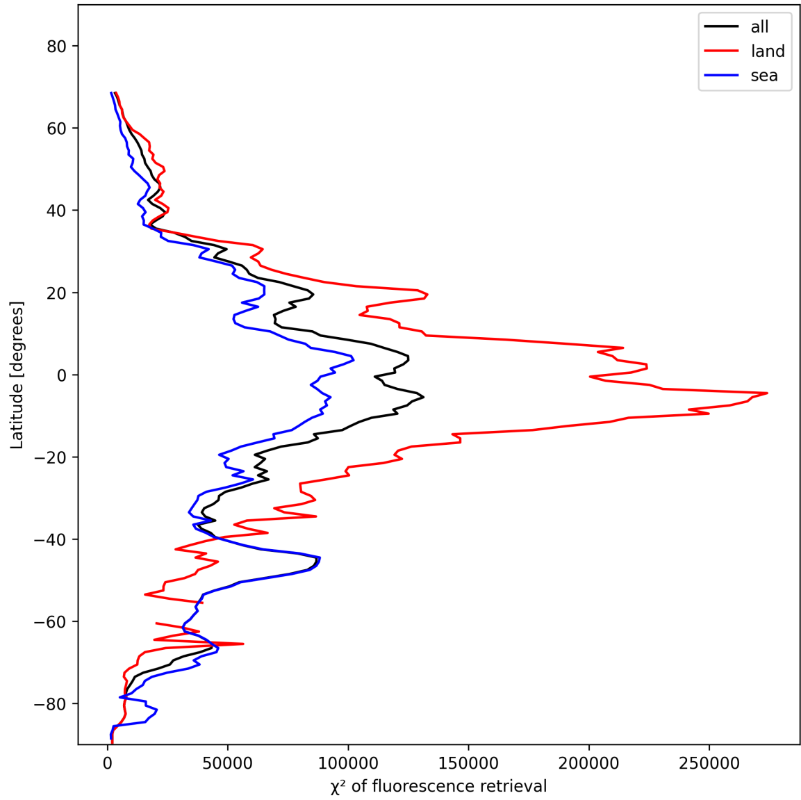
Figure 25: Zonal average of “ \chi^2 of fluorescence retrieval” for 2025-11-18 to 2025-11-20.
