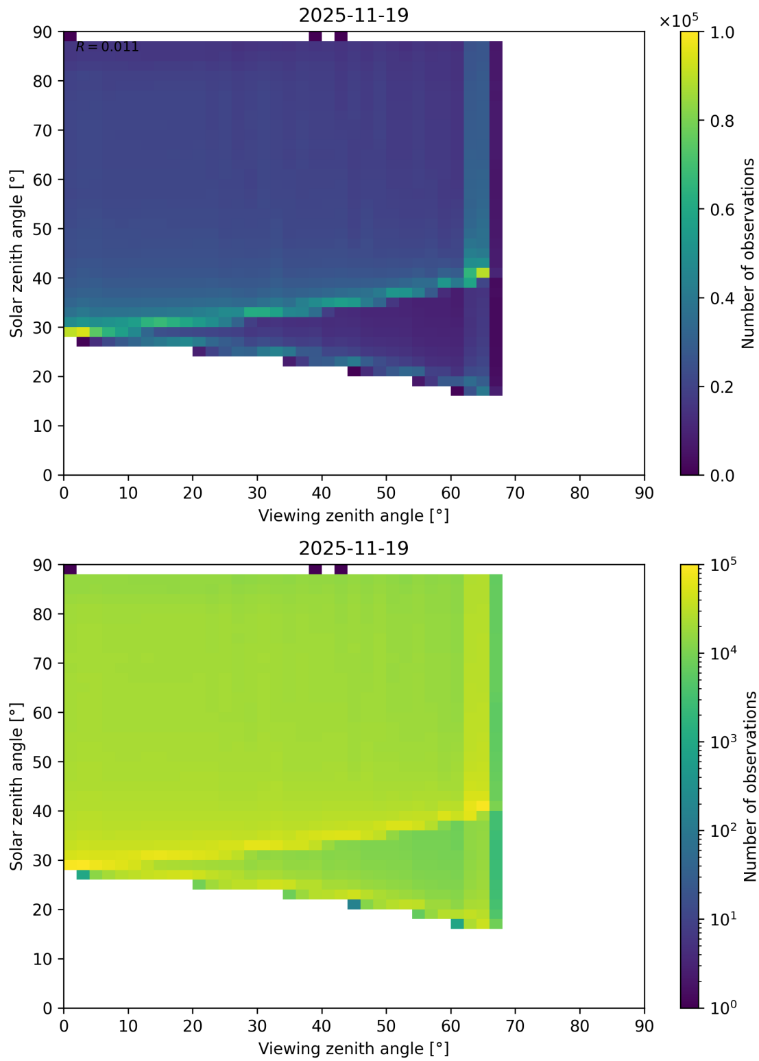
Figure 127: Scatter density plot of “Viewing zenith angle” against “Solar zenith angle” for 2025-11-18 to 2025-11-20.
