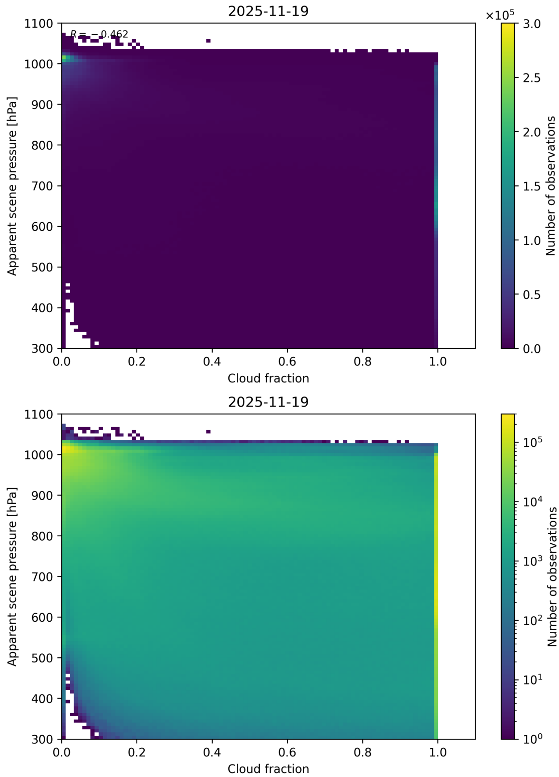
Figure 70: Scatter density plot of “Cloud fraction” against “Apparent scene pressure” for 2025-11-18 to 2025-11-20.
