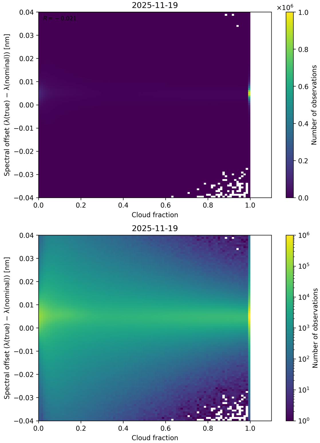
Figure 76: Scatter density plot of “Cloud fraction” against “Spectral offset ( \lambda_{\text{true}} - \lambda_{\text{nominal}} )” for 2025-11-18 to 2025-11-20.
