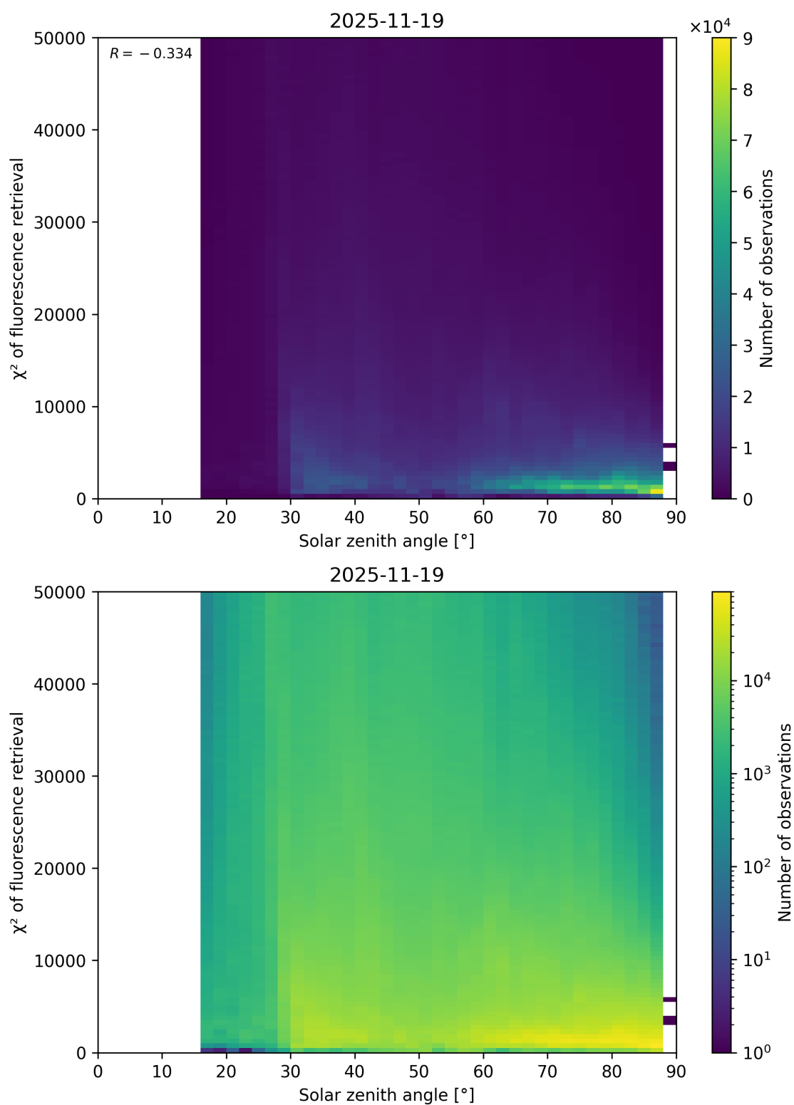
Figure 109: Scatter density plot of “Solar zenith angle” against “ \chi^2 of fluorescence retrieval” for 2025-11-18 to 2025-11-20.
