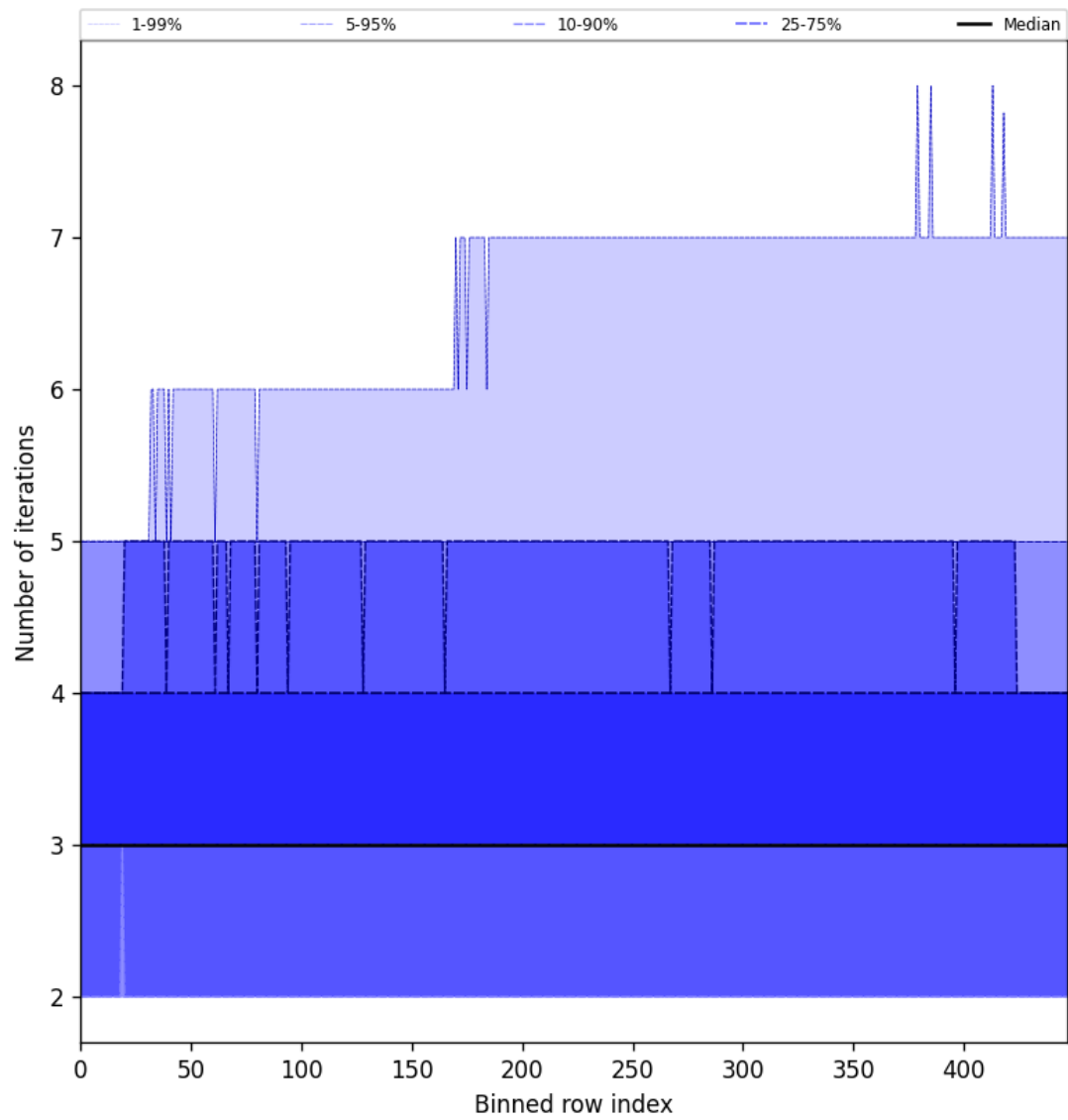
Figure 56: Along track statistics of “Number of iterations” for 2025-11-18 to 2025-11-20
