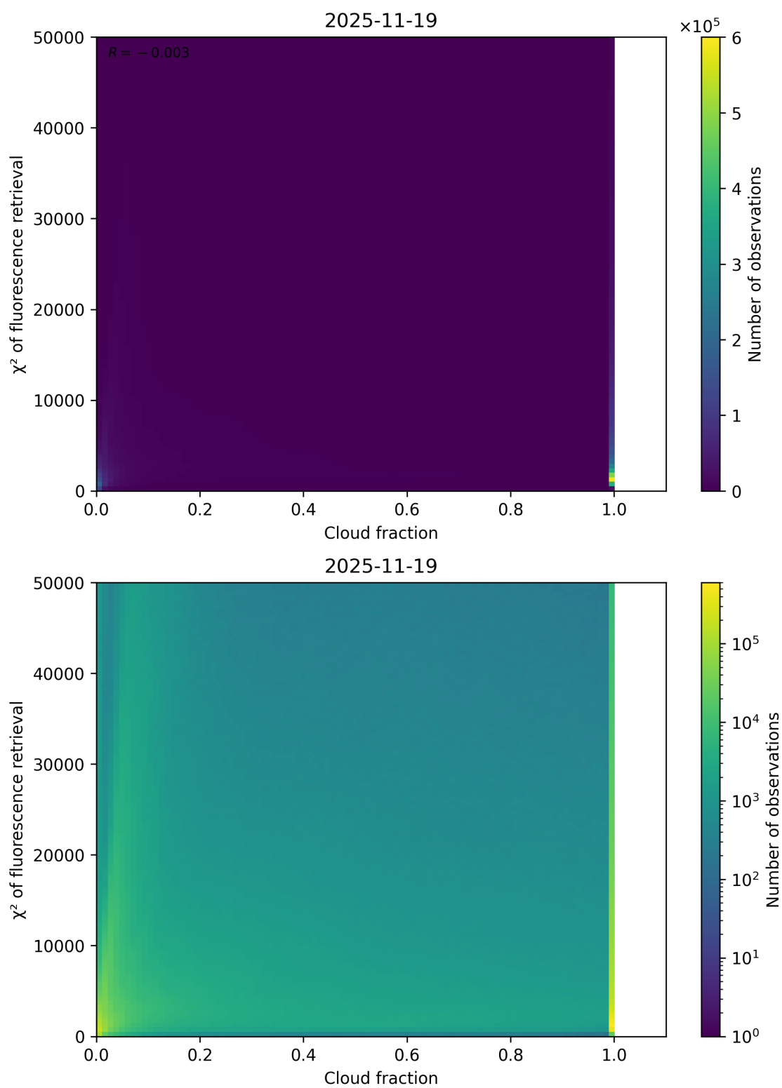
Figure 71: Scatter density plot of “Cloud fraction” against “ \chi^2 of fluorescence retrieval” for 2025-11-18 to 2025-11-20.
