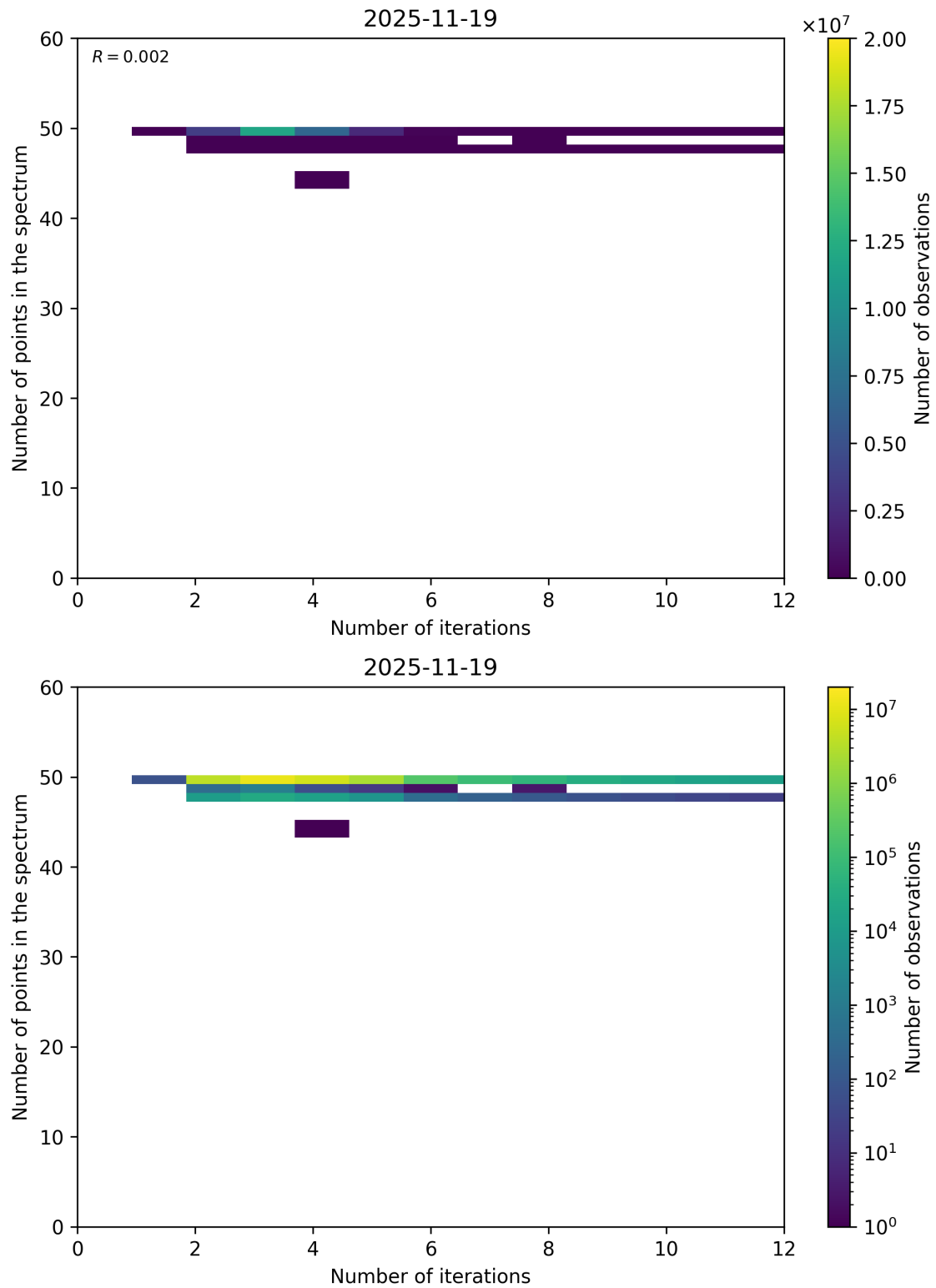
Figure 99: Scatter density plot of “Number of iterations” against “Number of points in the spectrum” for 2025-11-18 to 2025-11-20.
