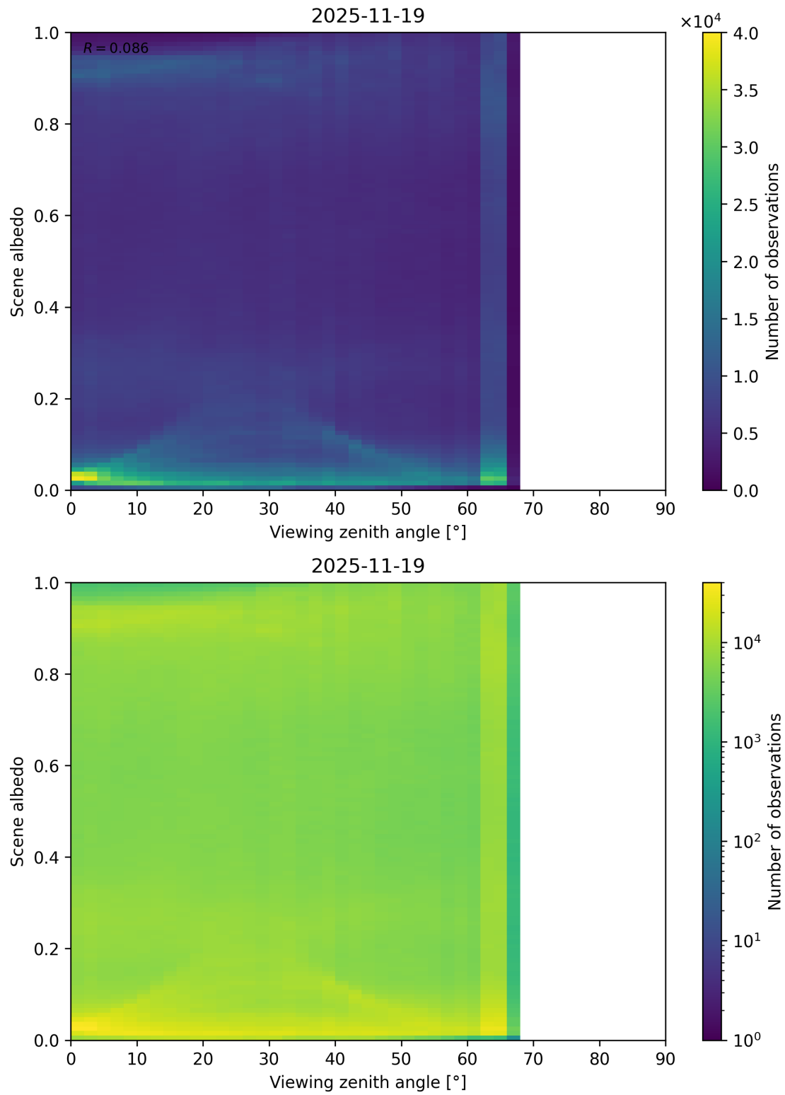
Figure 126: Scatter density plot of “Viewing zenith angle” against “Scene albedo” for 2025-11-18 to 2025-11-20.
