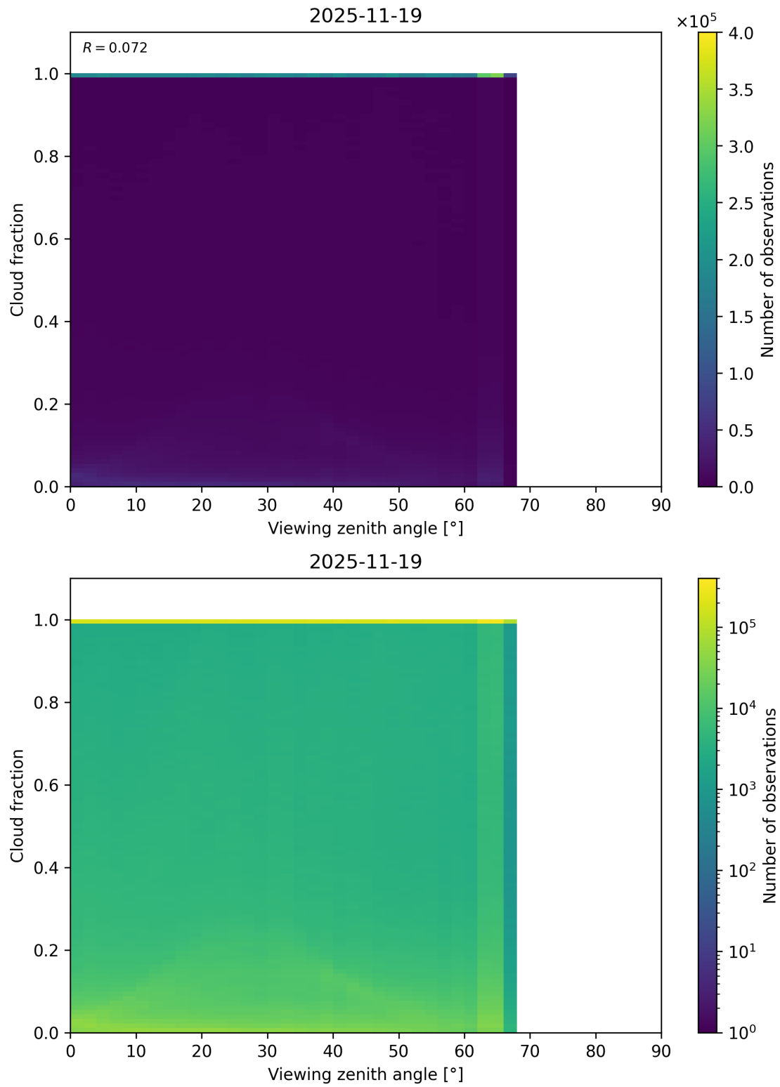
Figure 120: Scatter density plot of “Viewing zenith angle” against “Cloud fraction” for 2025-11-18 to 2025-11-20.
