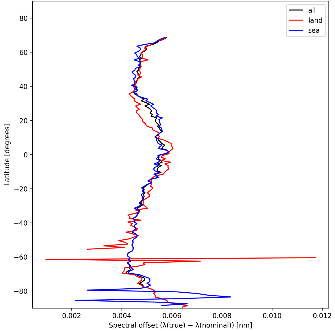
Figure 28: Zonal average of “Spectral offset ( \lambda_{\text{true}} - \lambda_{\text{nominal}} )” for 2025-11-18 to 2025-11-20.
