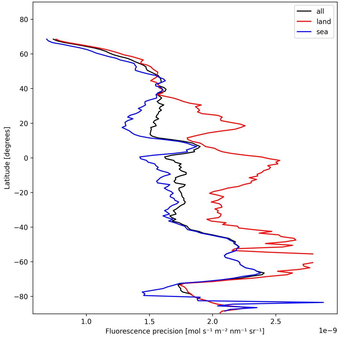
Figure 24: Zonal average of “Fluorescence precision” for 2025-11-18 to 2025-11-20.
