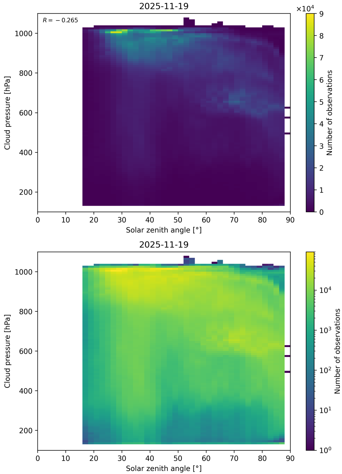
Figure 111: Scatter density plot of “Solar zenith angle” against “Cloud pressure” for 2025-11-18 to 2025-11-20.
