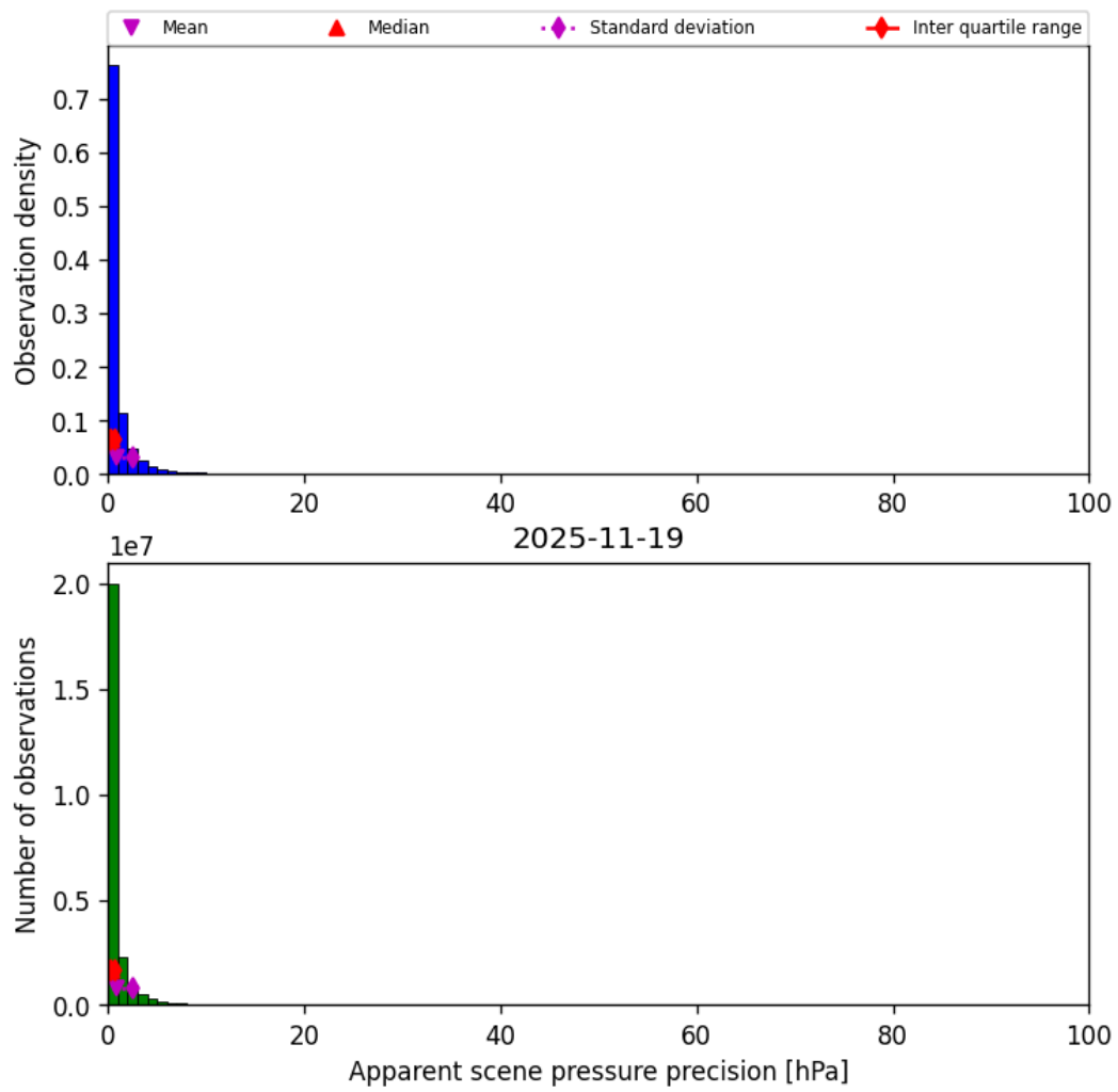
Figure 37: Histogram of “Apparent scene pressure precision” for 2025-11-18 to 2025-11-20
