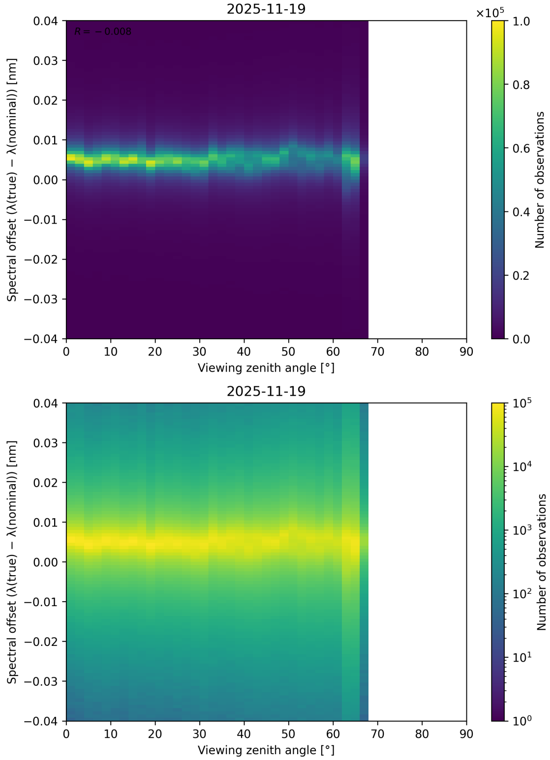
Figure 128: Scatter density plot of “Viewing zenith angle” against “Spectral offset ( \lambda_{\text{true}} - \lambda_{\text{nominal}} )” for 2025-11-18 to 2025-11-20.
