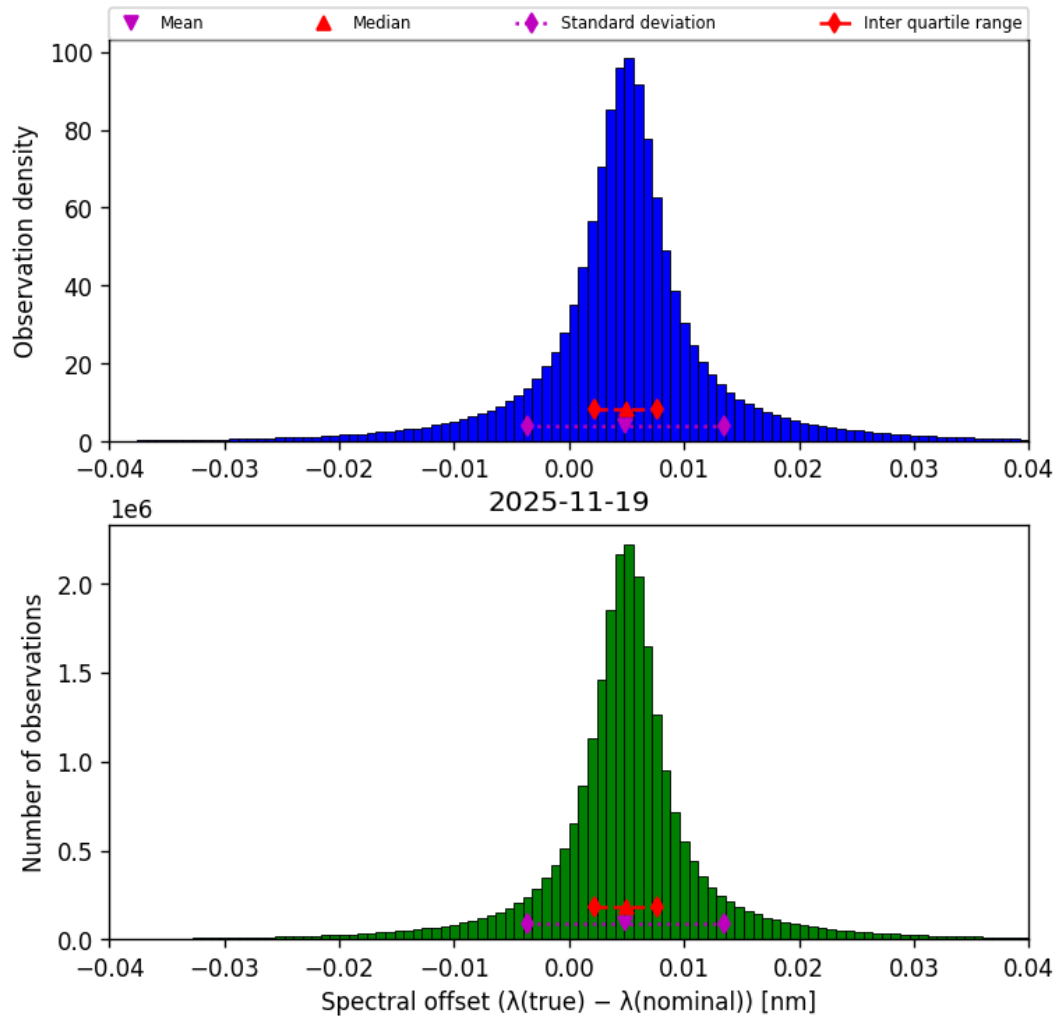
Figure 45: Histogram of “Spectral offset ( \lambda_{\text{true}} - \lambda_{\text{nominal}} )” for 2025-11-18 to 2025-11-20
