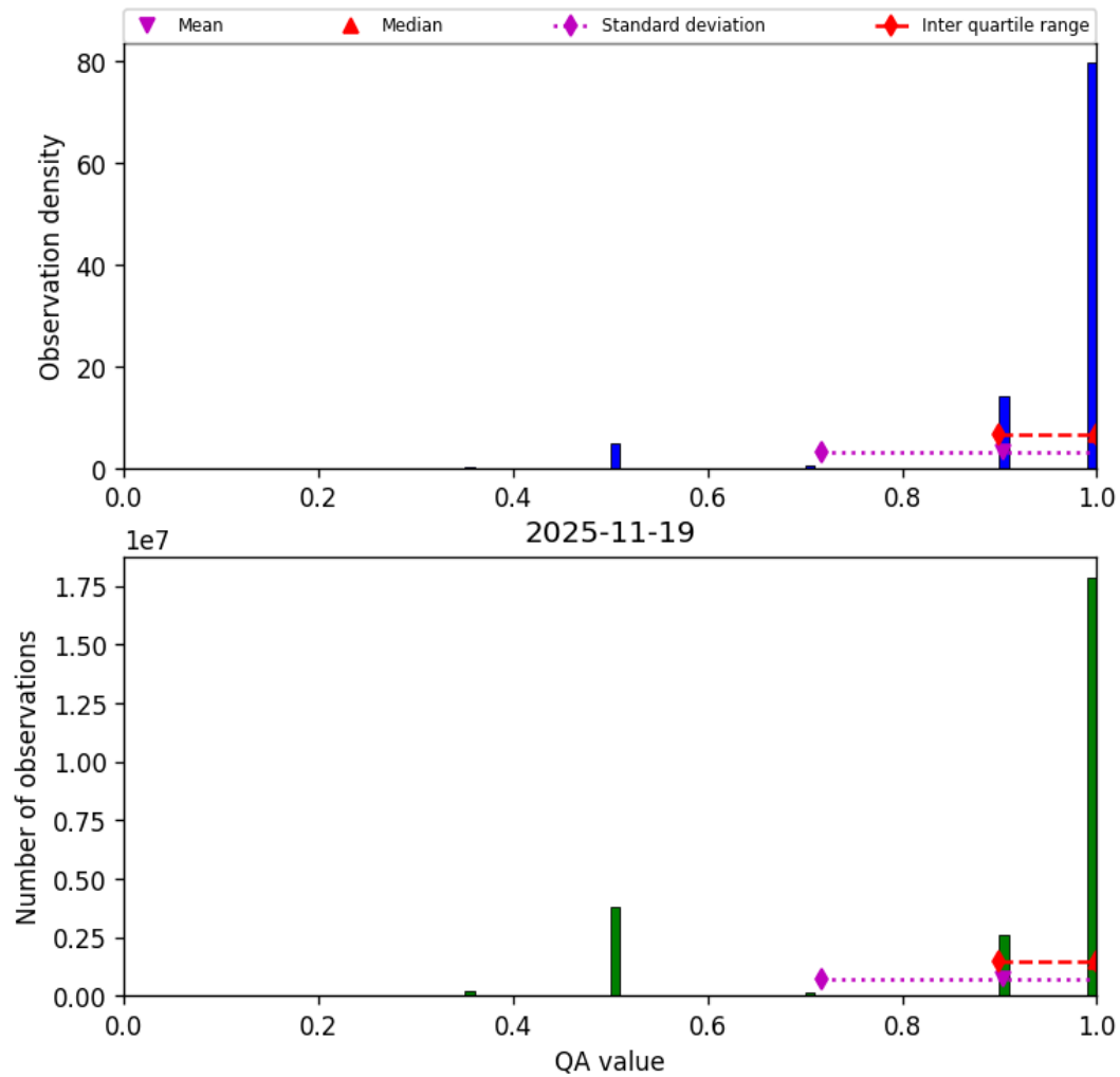
Figure 29: Histogram of “QA value” for 2025-11-18 to 2025-11-20
