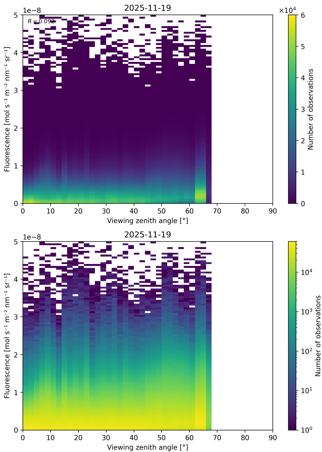
Figure 122: Scatter density plot of “Viewing zenith angle” against “Fluorescence” for 2025-11-18 to 2025-11-20.
