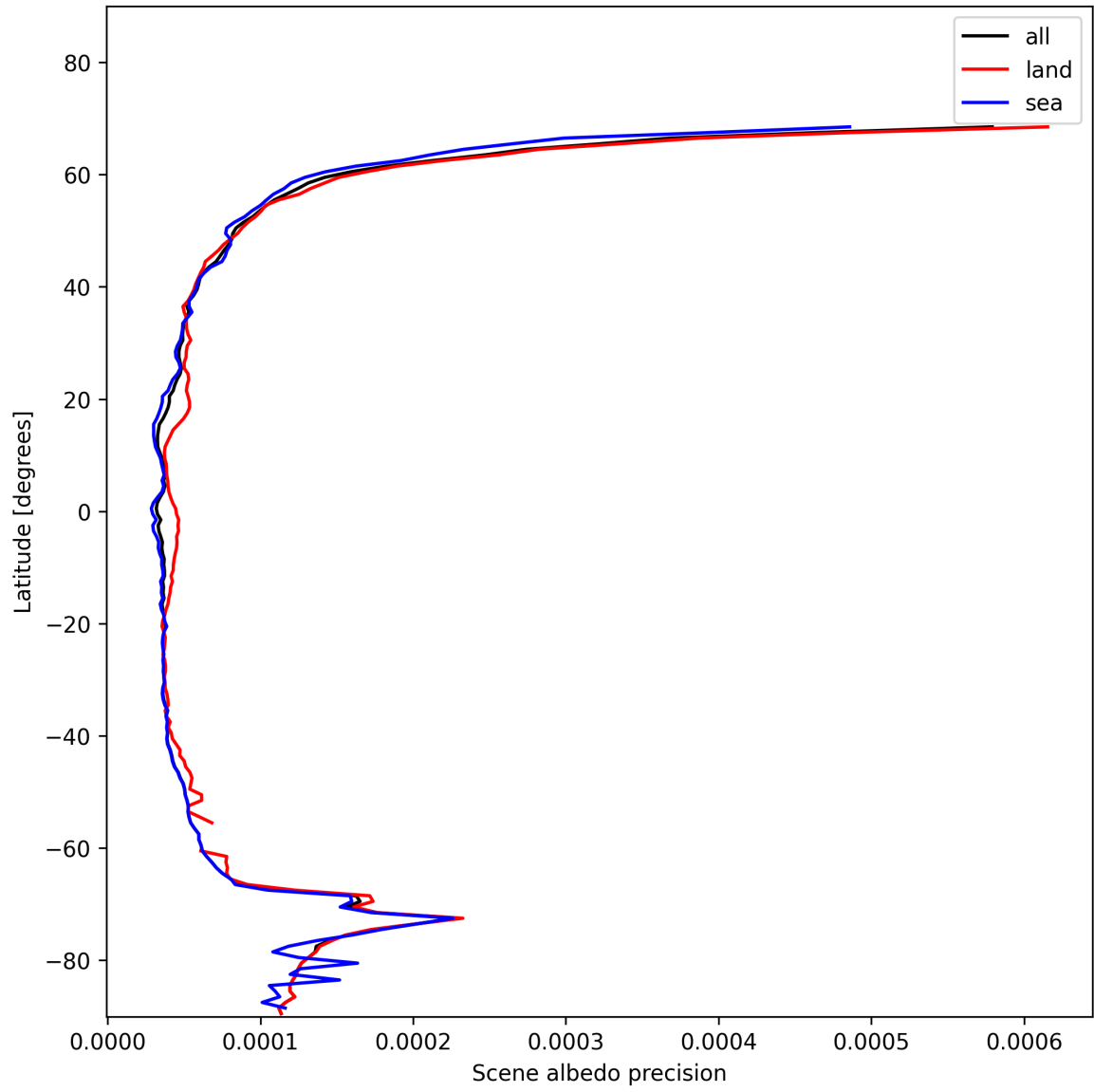
Figure 18: Zonal average of “Scene albedo precision” for 2025-11-18 to 2025-11-20.
