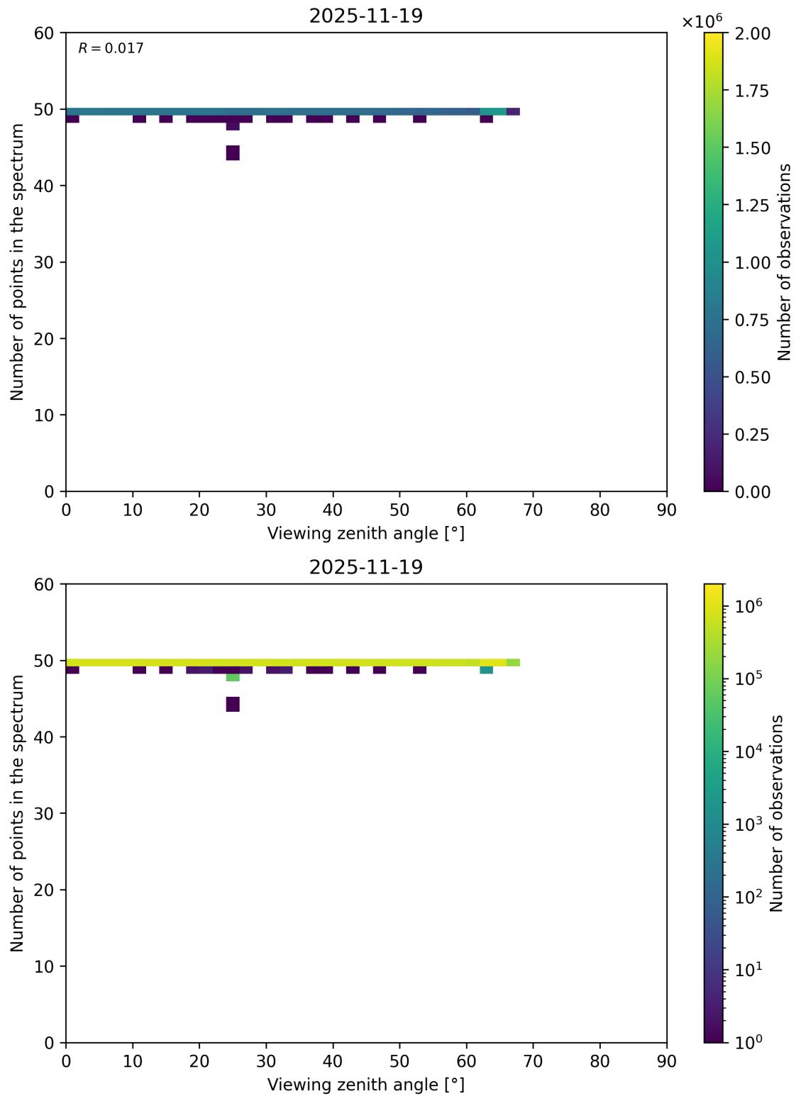
Figure 125: Scatter density plot of “Viewing zenith angle” against “Number of points in the spectrum” for 2025-11-18 to 2025-11-20.
