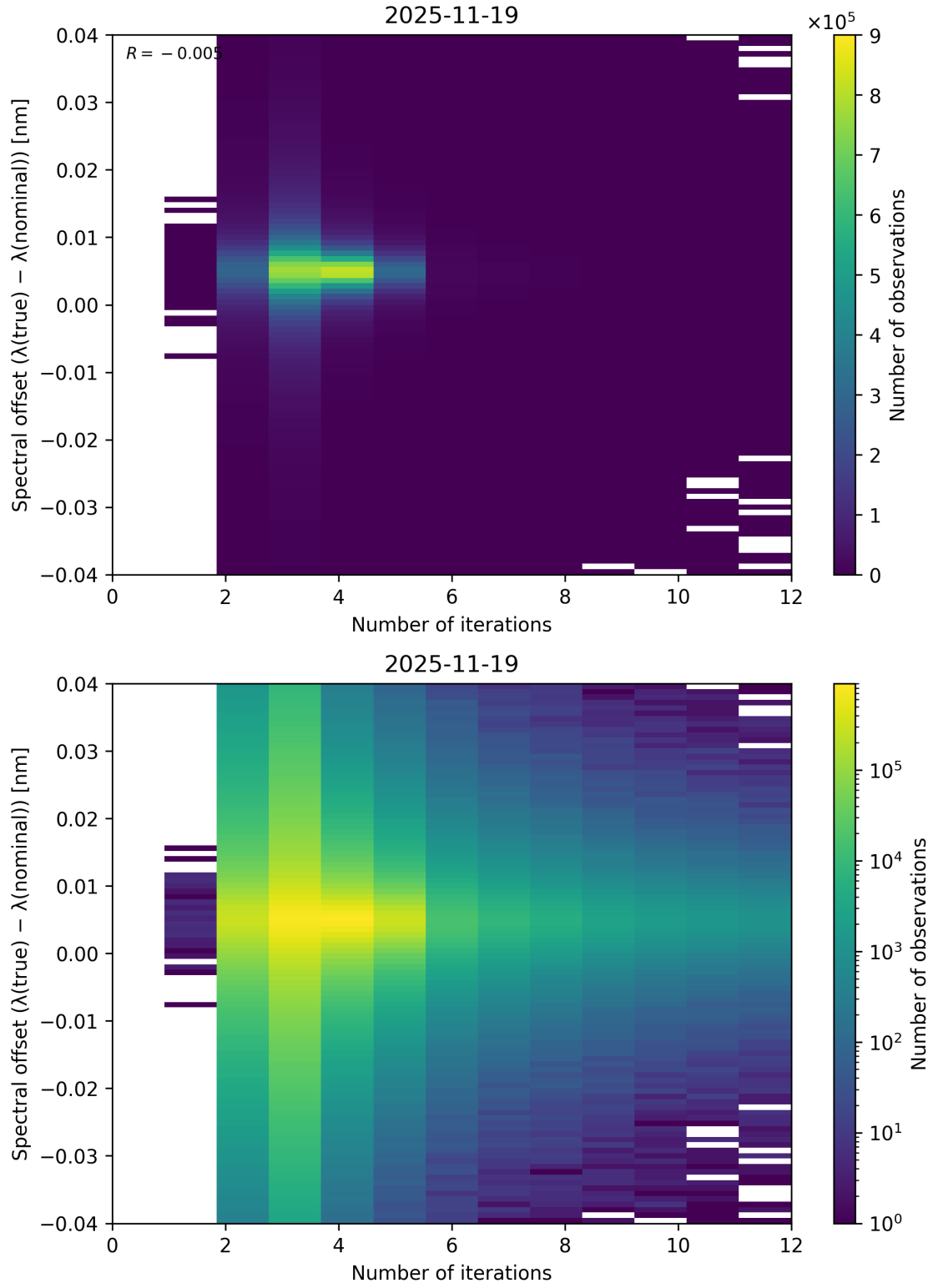
Figure 100: Scatter density plot of “Number of iterations” against “Spectral offset ( \lambda_{\text{true}} - \lambda_{\text{nominal}} )” for 2025-11-18 to 2025-11-20.
