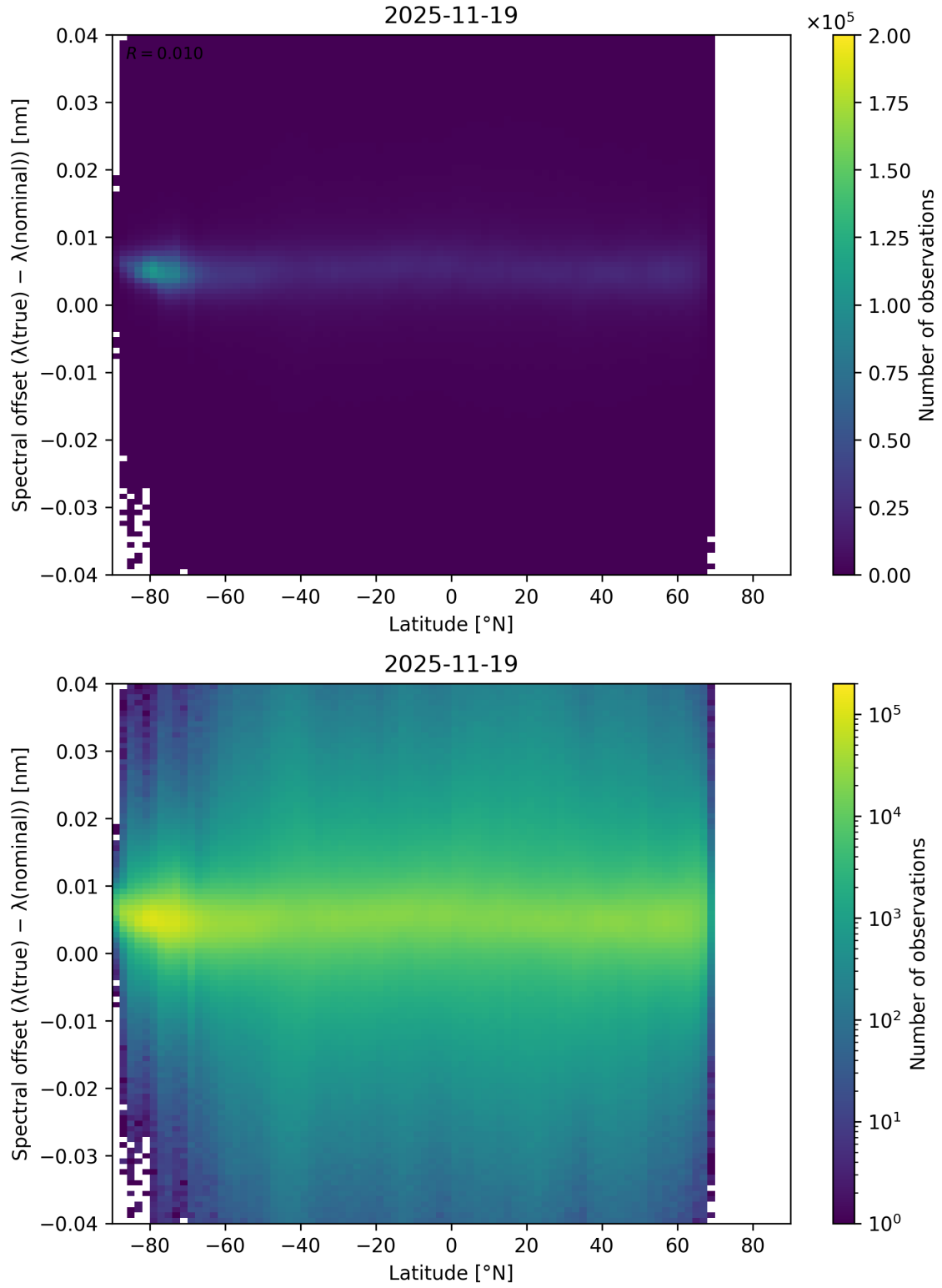
Figure 96: Scatter density plot of “Latitude” against “Spectral offset ( \lambda_{\text{true}} - \lambda_{\text{nominal}} )” for 2025-11-18 to 2025-11-20.
