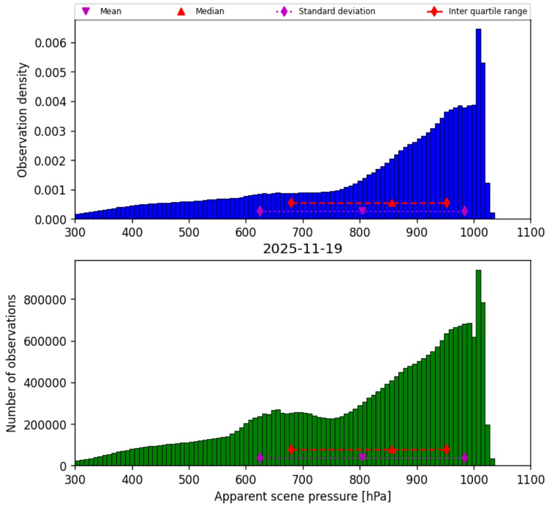
Figure 36: Histogram of “Apparent scene pressure” for 2025-11-18 to 2025-11-20
