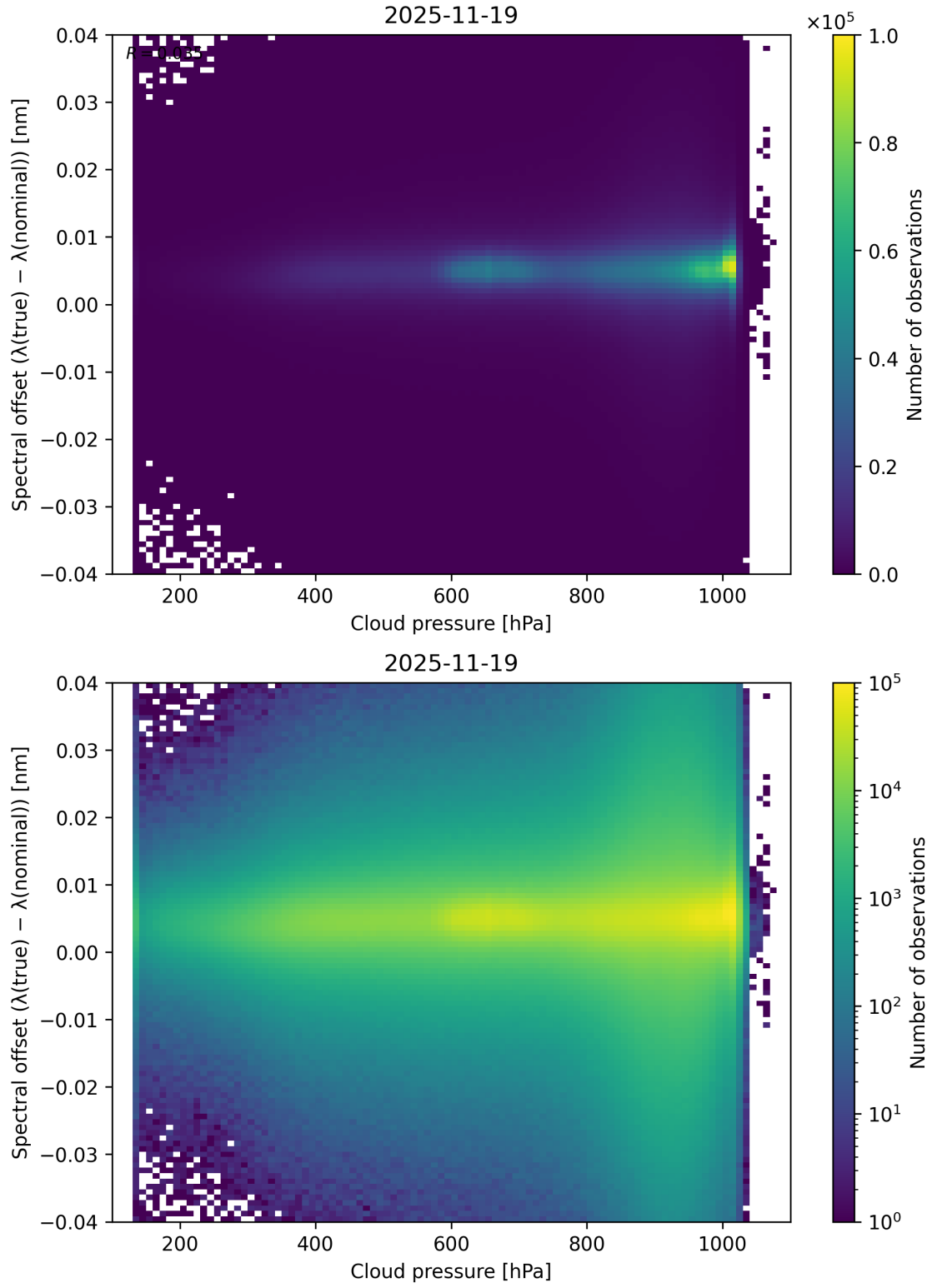
Figure 84: Scatter density plot of “Cloud pressure” against “Spectral offset ( \lambda_{\text{true}} - \lambda_{\text{nominal}} )” for 2025-11-18 to 2025-11-20.
