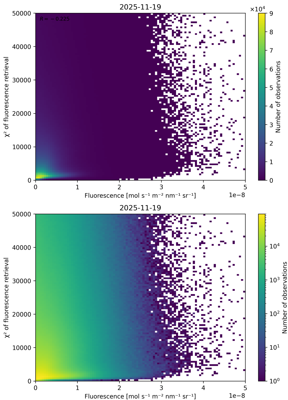
Figure 85: Scatter density plot of “Fluorescence” against “ \chi^2 of fluorescence retrieval” for 2025-11-18 to 2025-11-20.
