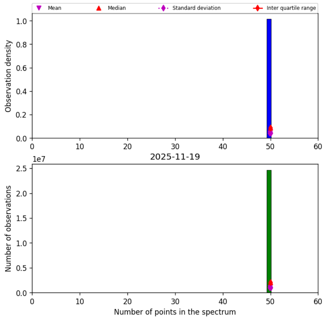
Figure 44: Histogram of “Number of points in the spectrum” for 2025-11-18 to 2025-11-20
