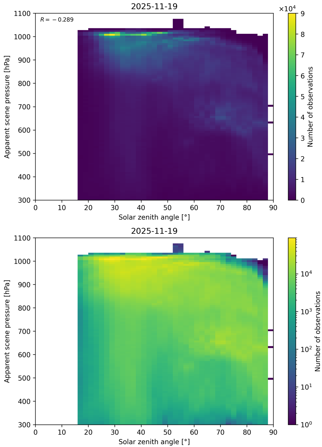
Figure 108: Scatter density plot of “Solar zenith angle” against “Apparent scene pressure” for 2025-11-18 to 2025-11-20.
