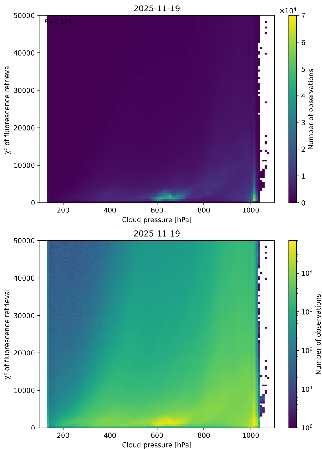
Figure 78: Scatter density plot of “Cloud pressure” against “ \chi^2 of fluorescence retrieval” for 2025-11-18 to 2025-11-20.
