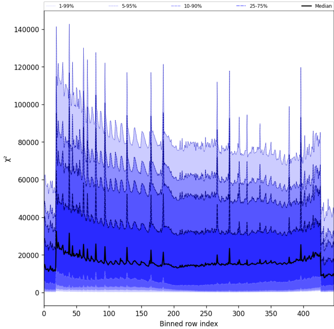
Figure 55: Along track statistics of “ \chi^2 ” for 2025-11-18 to 2025-11-20
