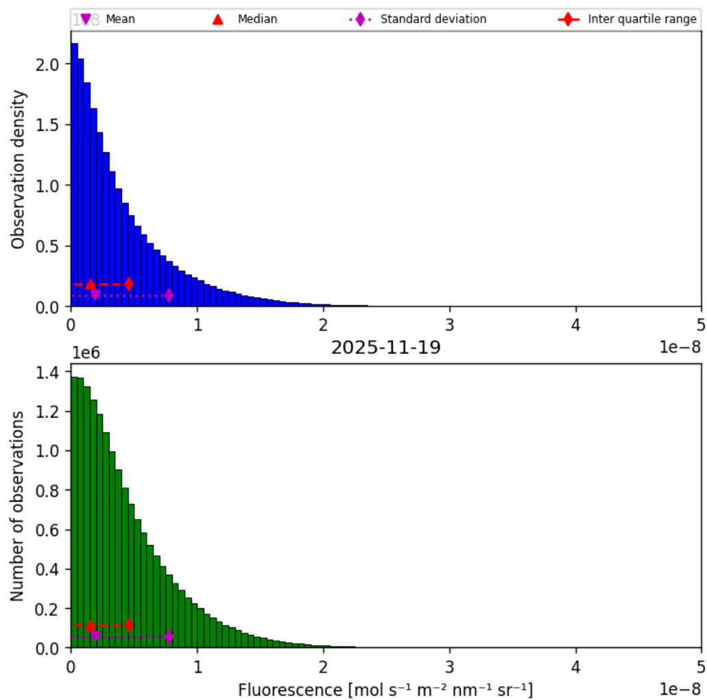
Figure 40: Histogram of “Fluorescence” for 2025-11-18 to 2025-11-20
