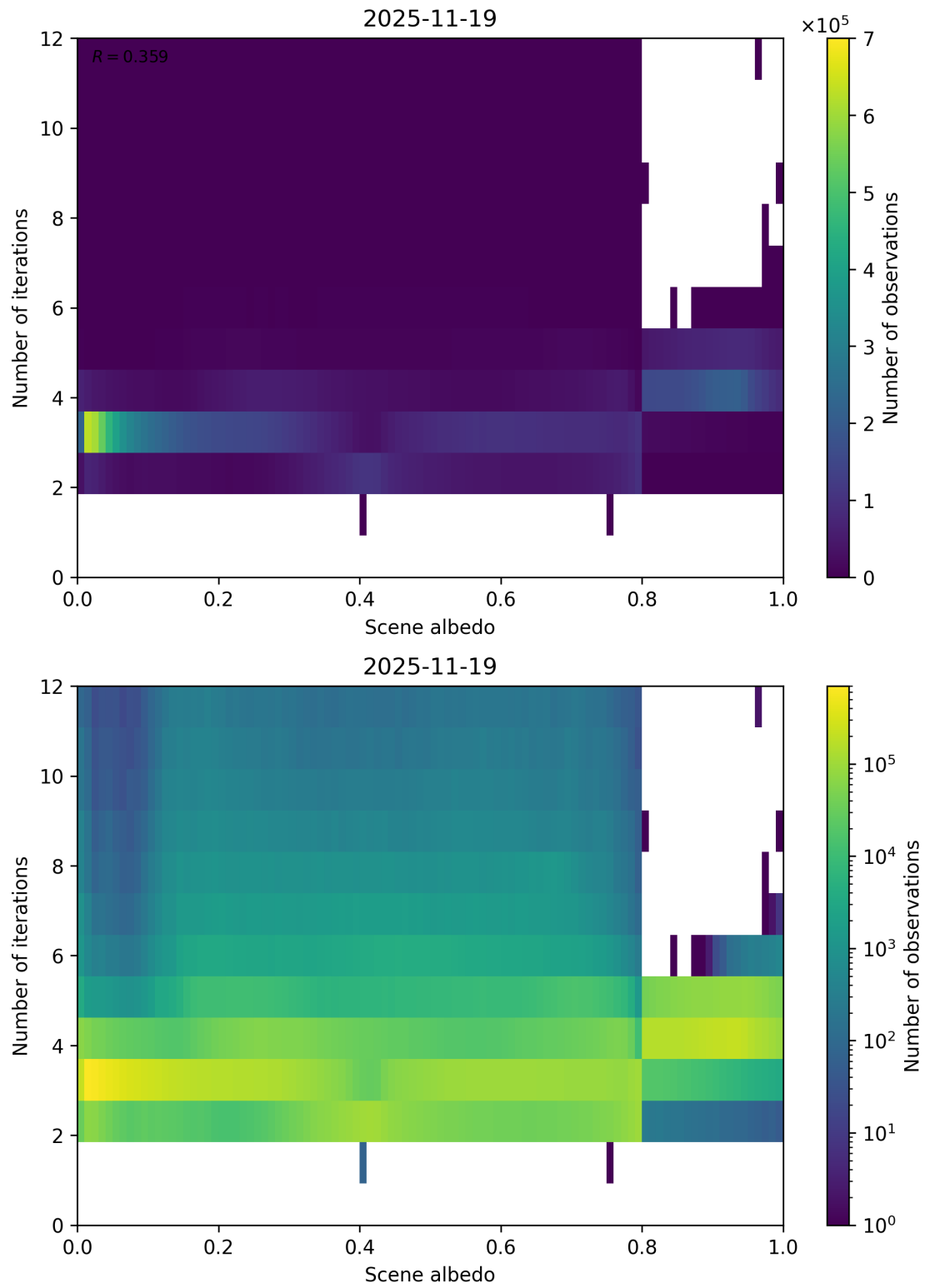
Figure 105: Scatter density plot of “Scene albedo” against “Number of iterations” for 2025-11-18 to 2025-11-20.
