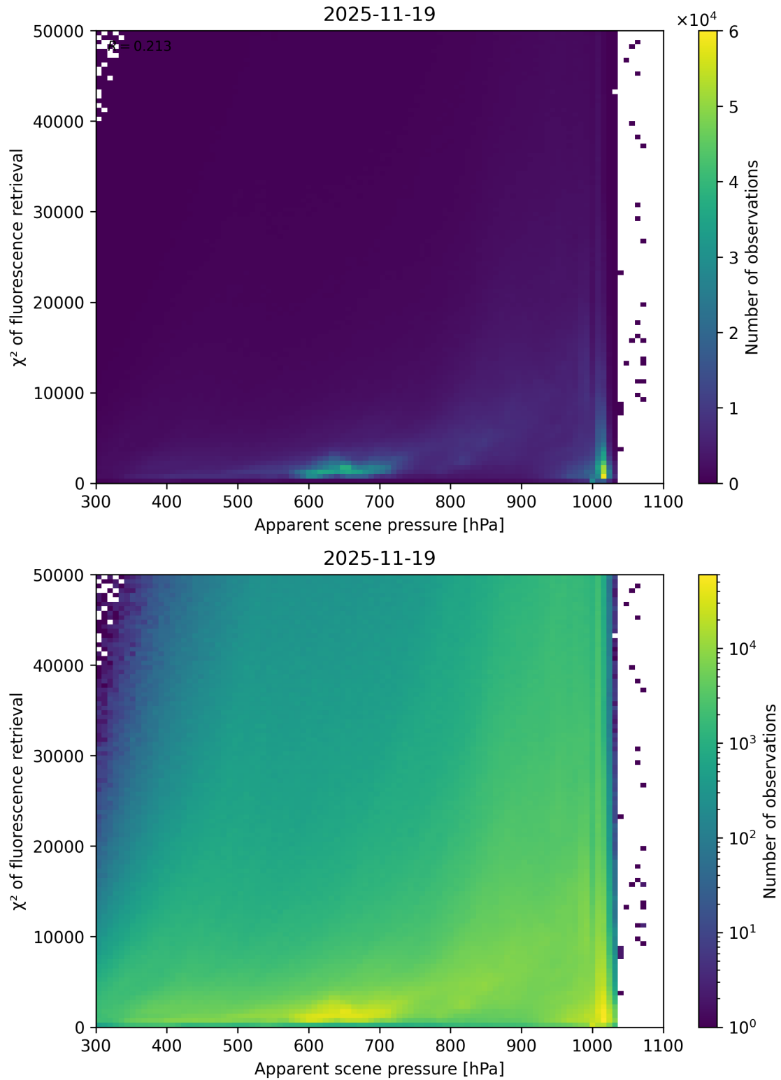
Figure 63: Scatter density plot of “Apparent scene pressure” against “ \chi^2 of fluorescence retrieval” for 2025-11-18 to 2025-11-20.
