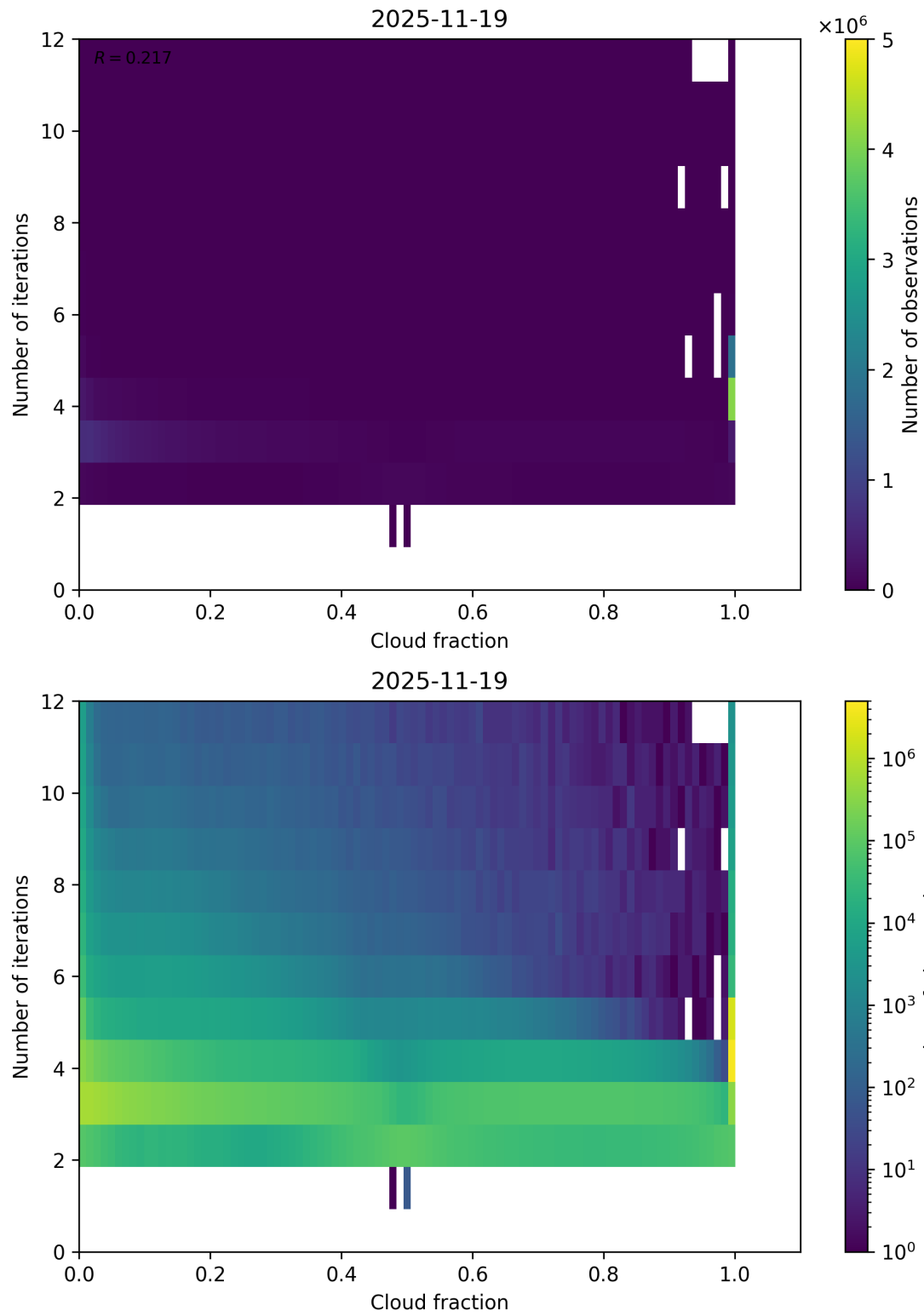
Figure 73: Scatter density plot of “Cloud fraction” against “Number of iterations” for 2025-11-18 to 2025-11-20.
