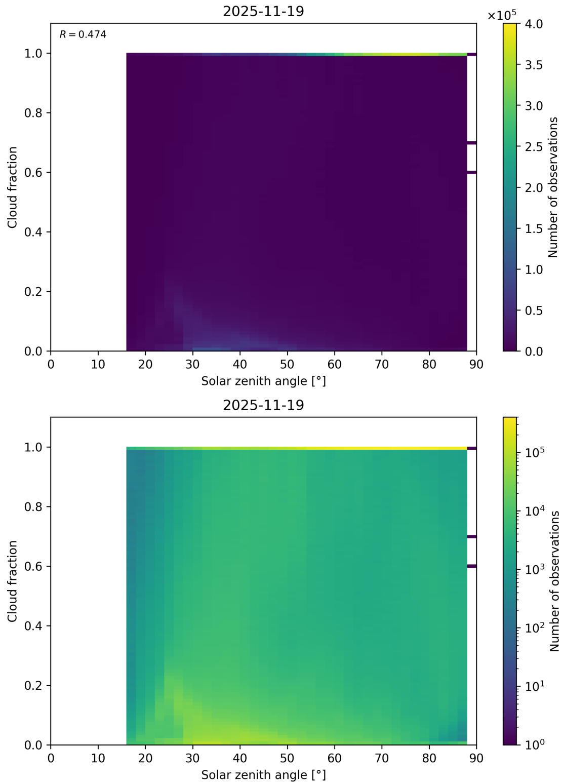
Figure 110: Scatter density plot of “Solar zenith angle” against “Cloud fraction” for 2025-11-18 to 2025-11-20.
