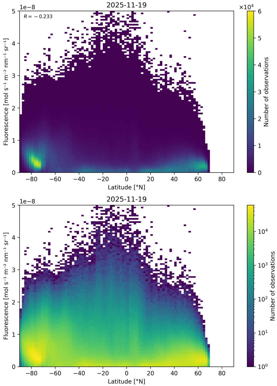
Figure 92: Scatter density plot of “Latitude” against “Fluorescence” for 2025-11-18 to 2025-11-20.
