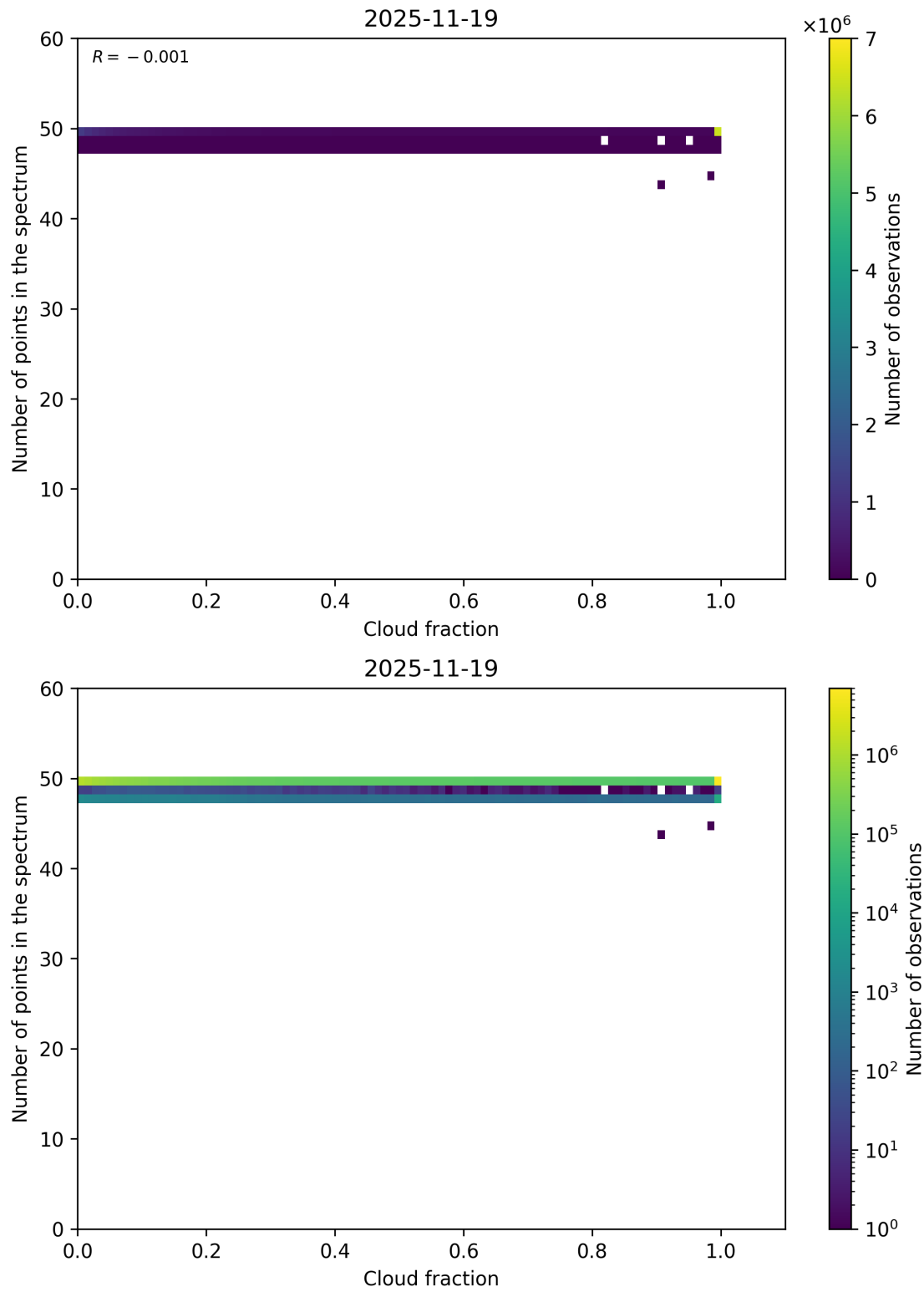
Figure 74: Scatter density plot of “Cloud fraction” against “Number of points in the spectrum” for 2025-11-18 to 2025-11-20.
