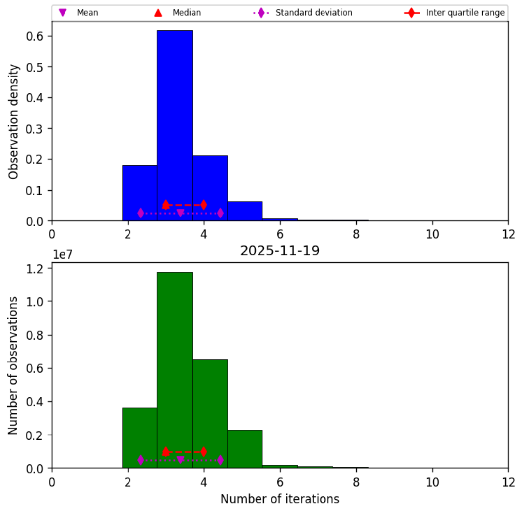
Figure 39: Histogram of “Number of iterations” for 2025-11-18 to 2025-11-20
