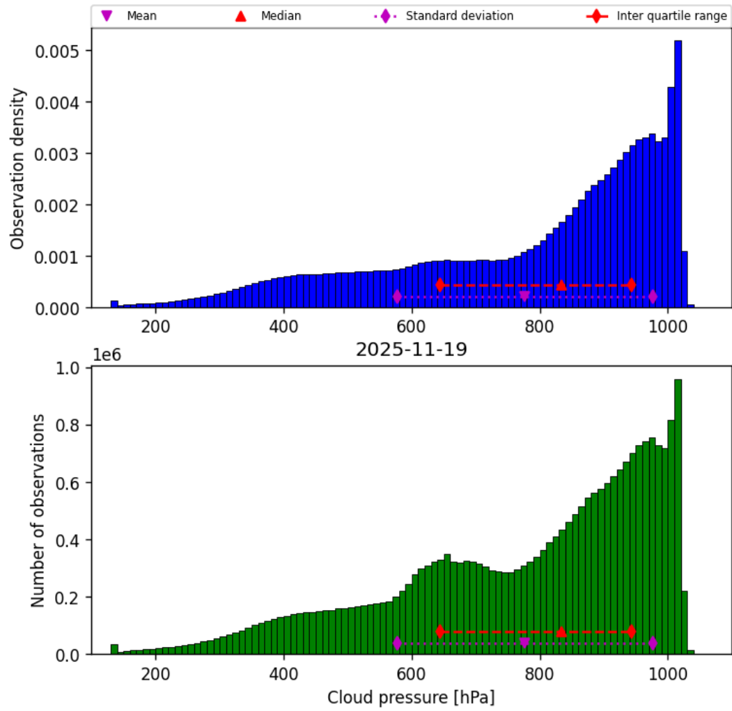
Figure 30: Histogram of “Cloud pressure” for 2025-11-18 to 2025-11-20
