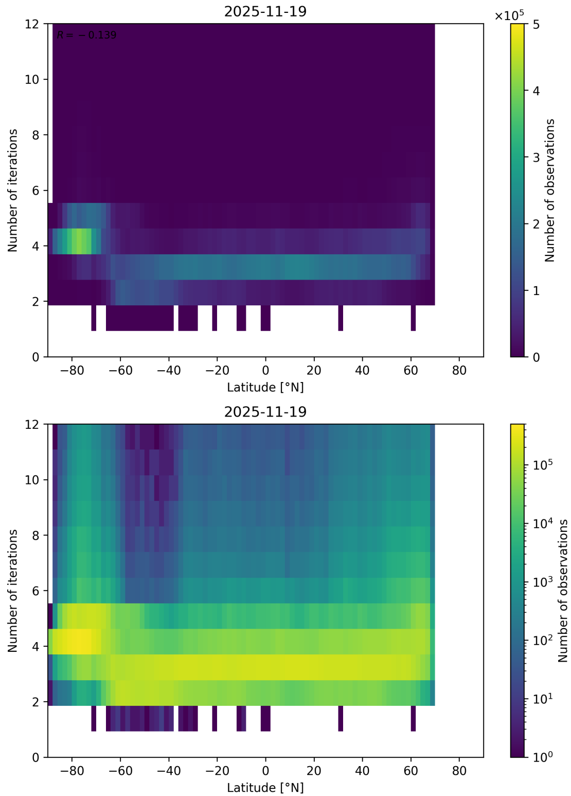
Figure 93: Scatter density plot of “Latitude” against “Number of iterations” for 2025-11-18 to 2025-11-20.
