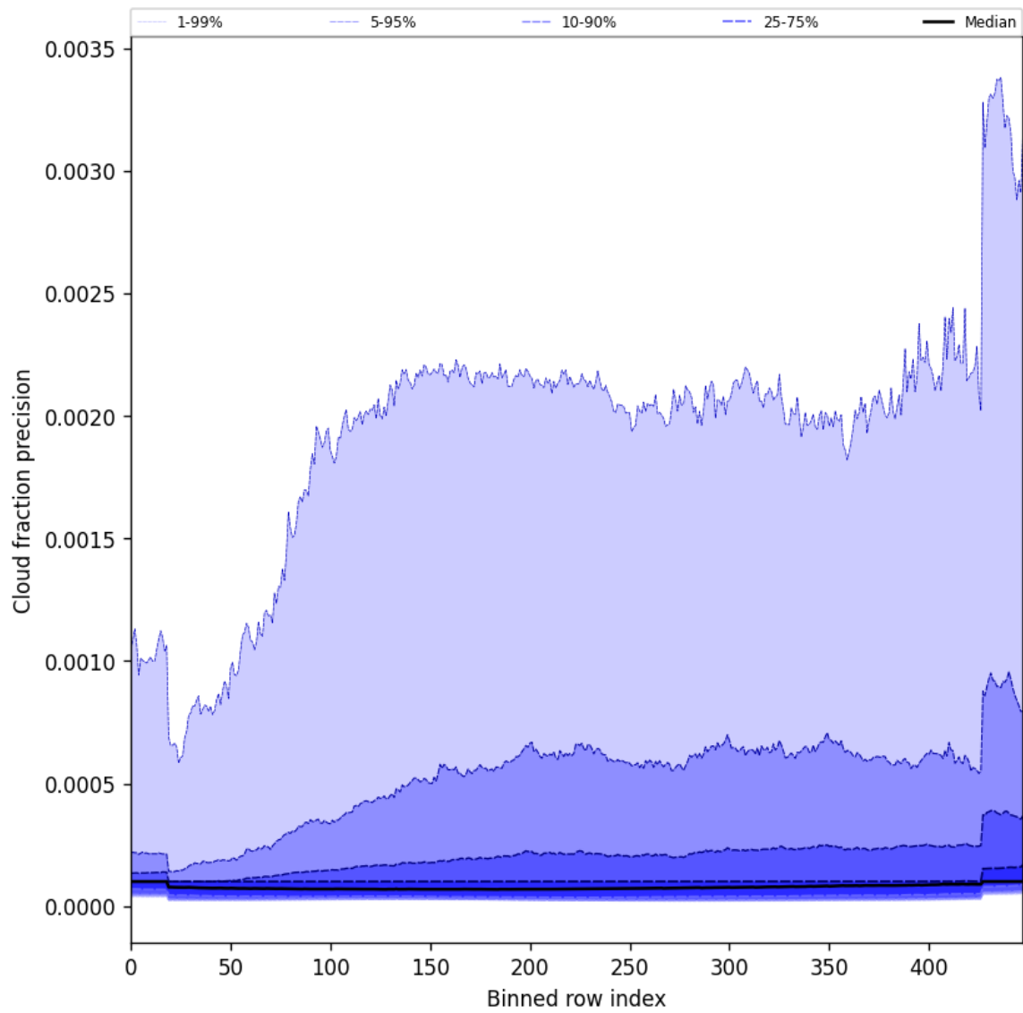
Figure 50: Along track statistics of “Cloud fraction precision” for 2025-11-18 to 2025-11-20
