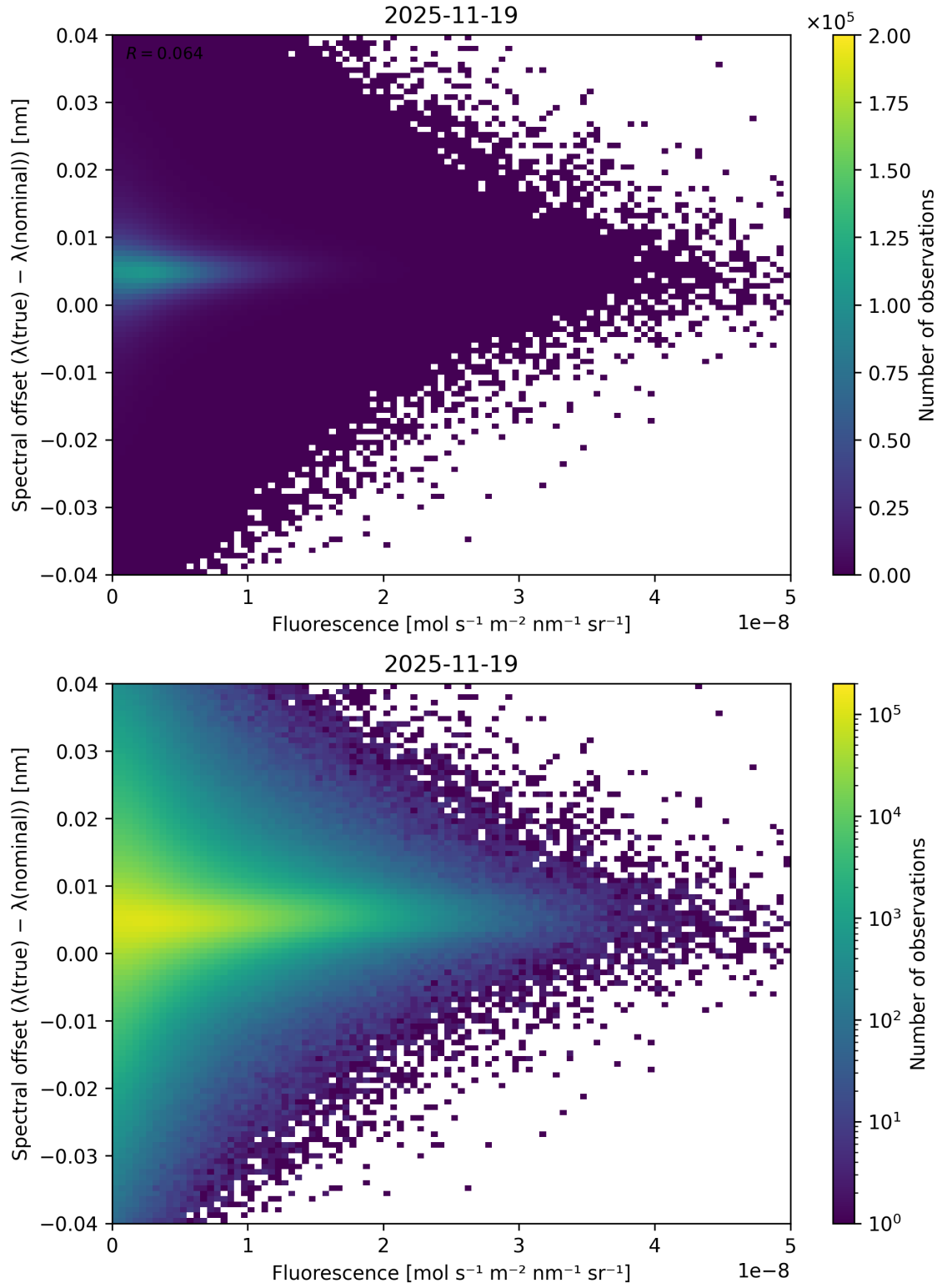
Figure 87: Scatter density plot of “Fluorescence” against “Spectral offset ( \lambda_{\text{true}} - \lambda_{\text{nominal}} )” for 2025-11-18 to 2025-11-20.
