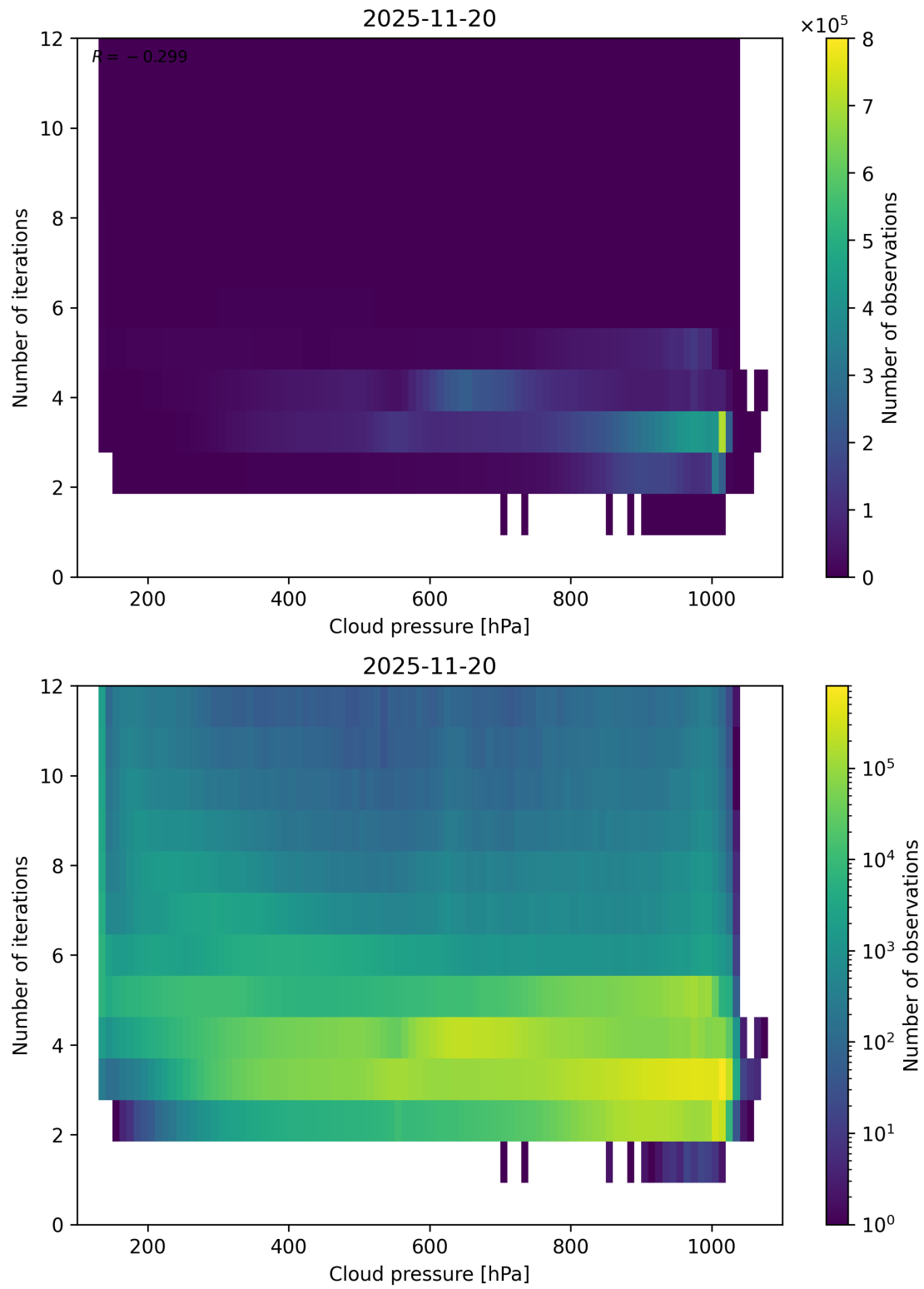
Figure 81: Scatter density plot of “Cloud pressure” against “Number of iterations” for 2025-11-19 to 2025-11-21.
