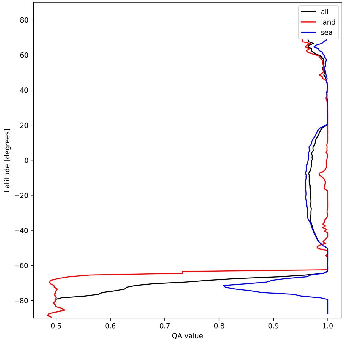
Figure 12: Zonal average of “QA value” for 2025-11-19 to 2025-11-21.
