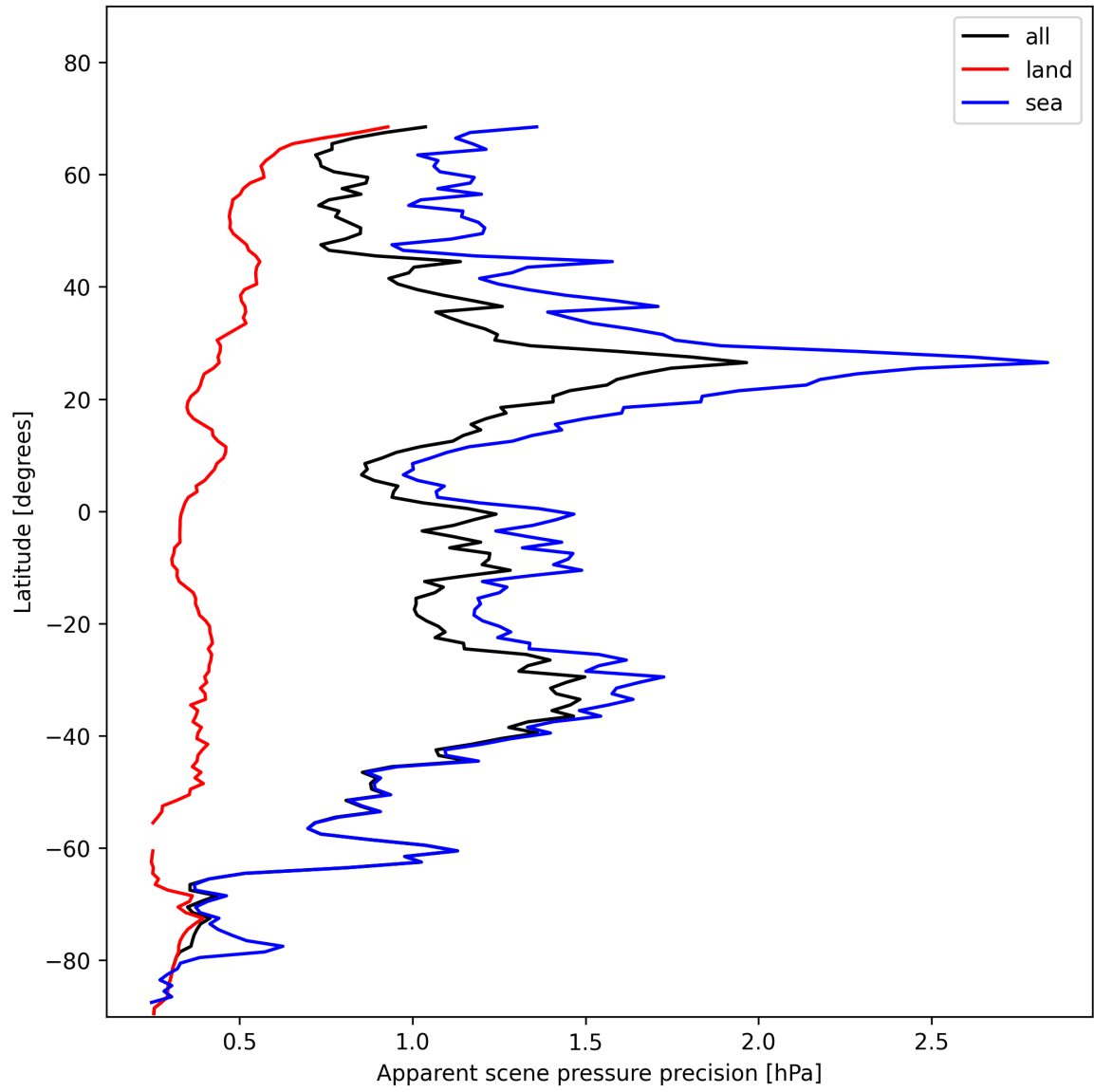
Figure 20: Zonal average of “Apparent scene pressure precision” for 2025-11-19 to 2025-11-21.
