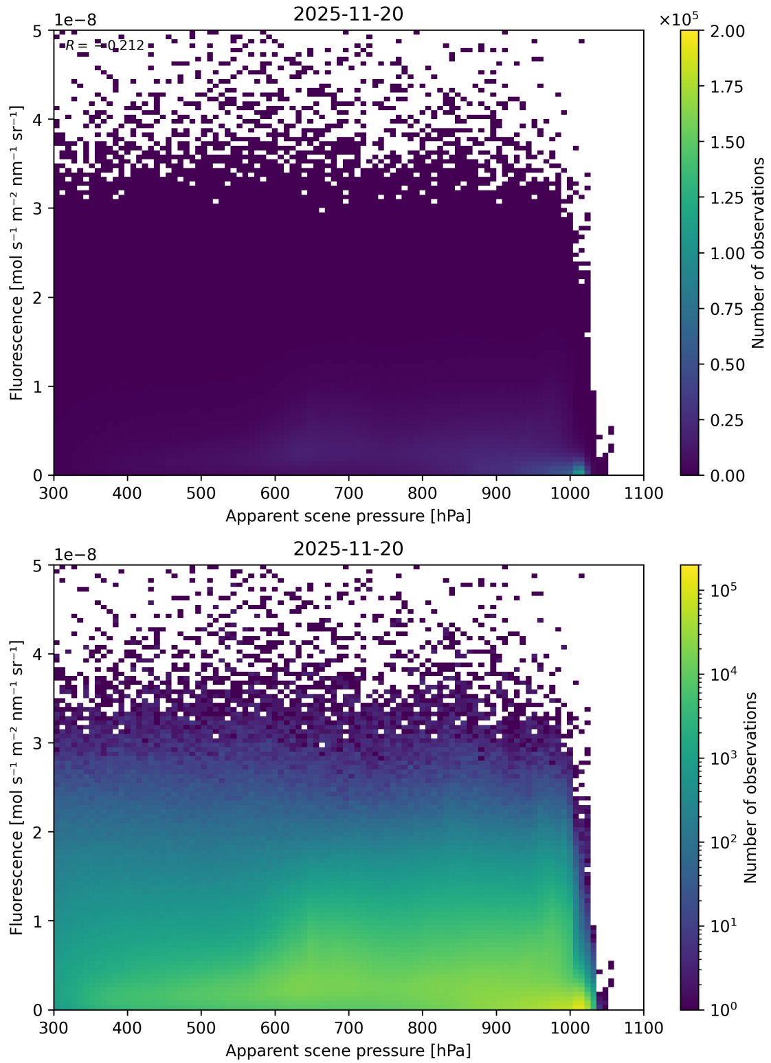
Figure 64: Scatter density plot of “Apparent scene pressure” against “Fluorescence” for 2025-11-19 to 2025-11-21.
