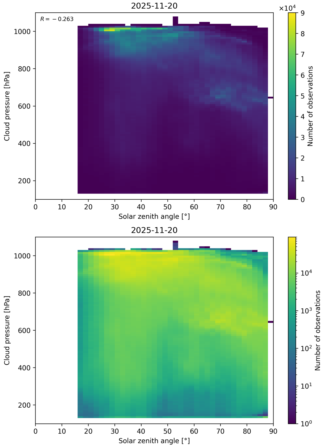
Figure 111: Scatter density plot of “Solar zenith angle” against “Cloud pressure” for 2025-11-19 to 2025-11-21.
