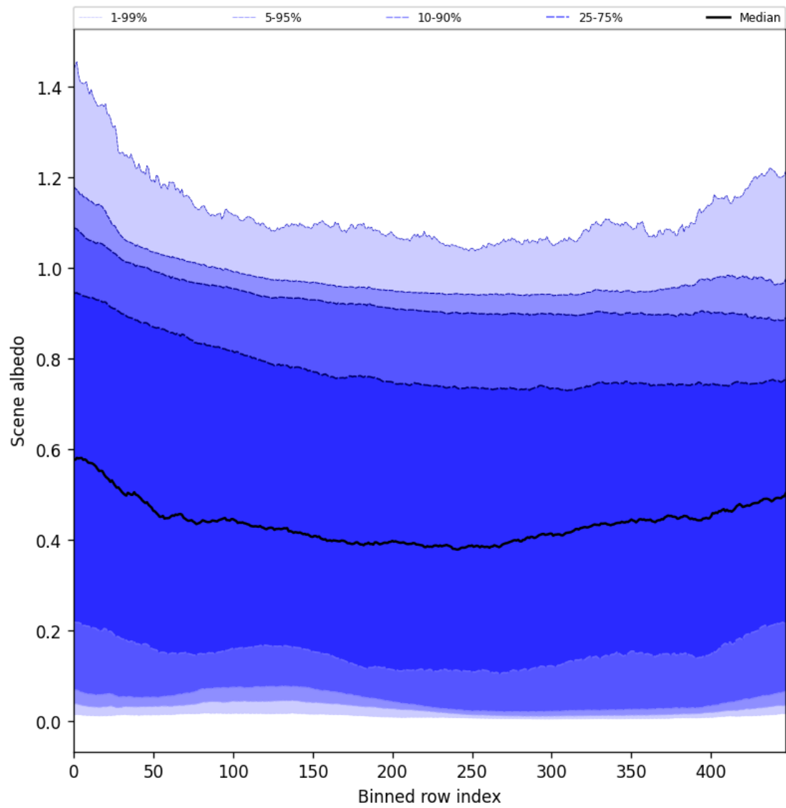
Figure 51: Along track statistics of “Scene albedo” for 2025-11-19 to 2025-11-21
