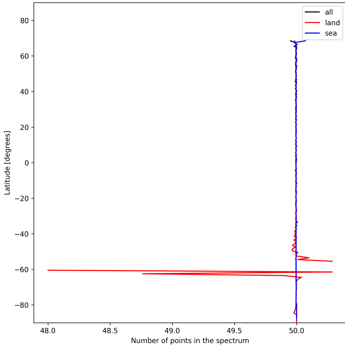
Figure 27: Zonal average of “Number of points in the spectrum” for 2025-11-19 to 2025-11-21.
