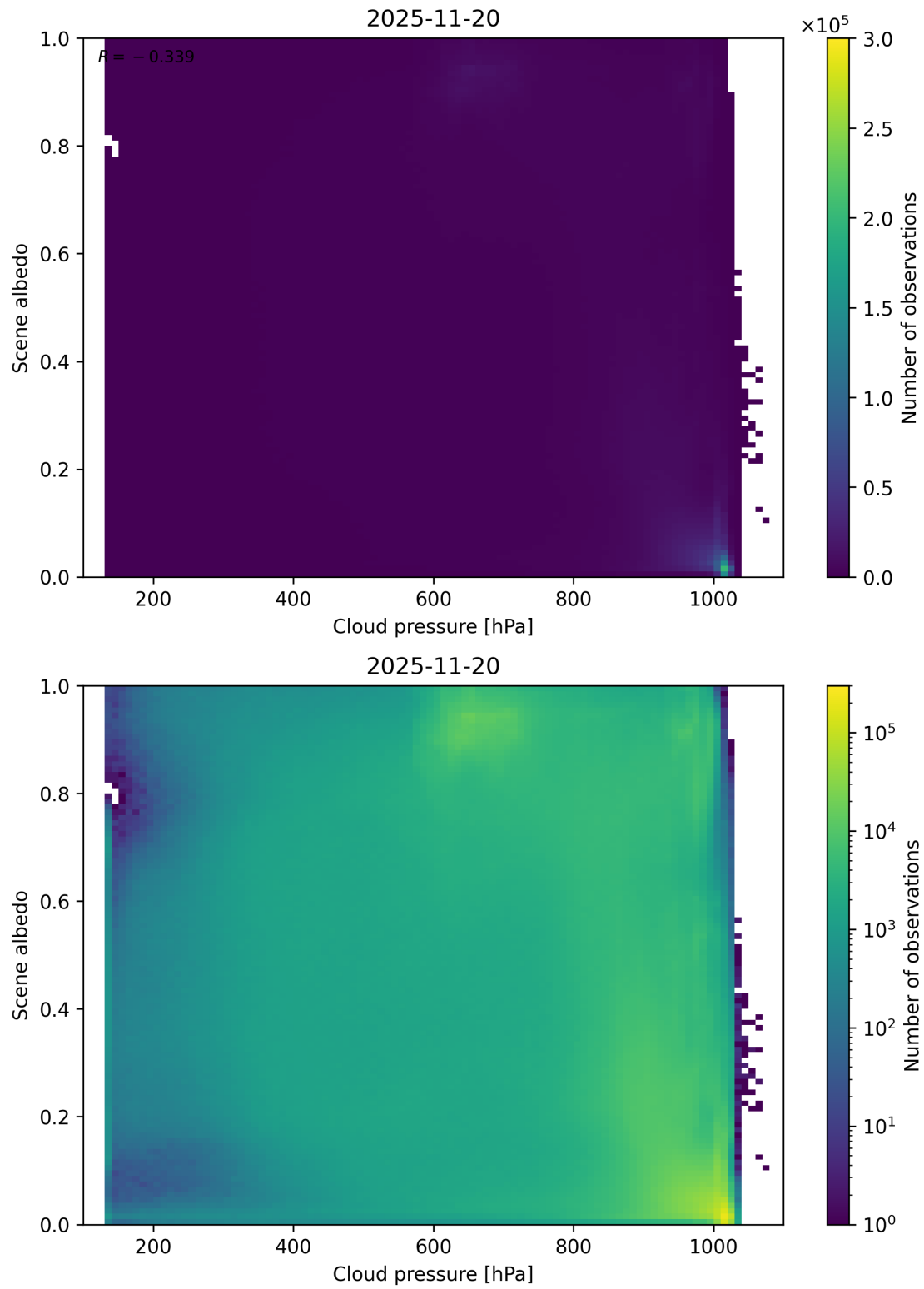
Figure 83: Scatter density plot of “Cloud pressure” against “Scene albedo” for 2025-11-19 to 2025-11-21.
