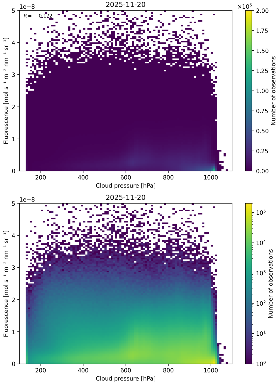
Figure 80: Scatter density plot of “Cloud pressure” against “Fluorescence” for 2025-11-19 to 2025-11-21.
