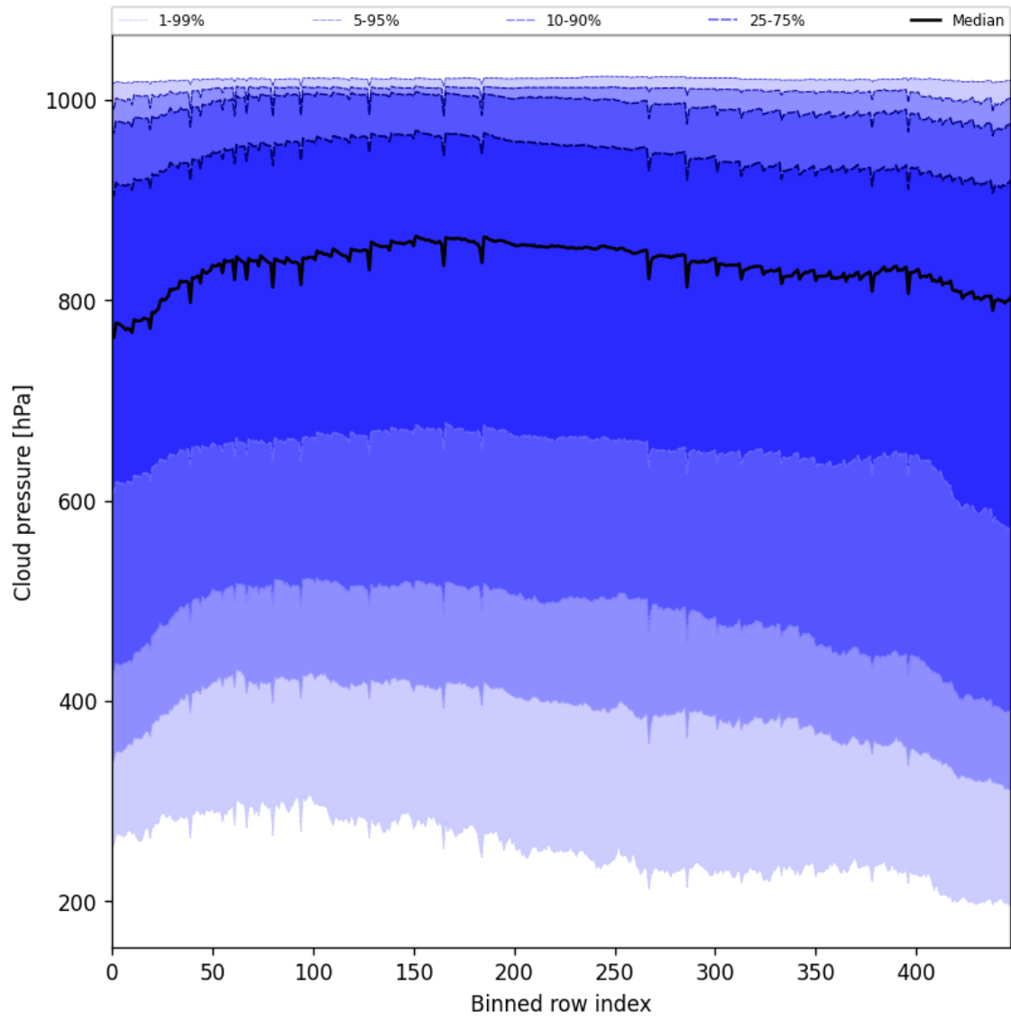
Figure 47: Along track statistics of “Cloud pressure” for 2025-11-19 to 2025-11-21
