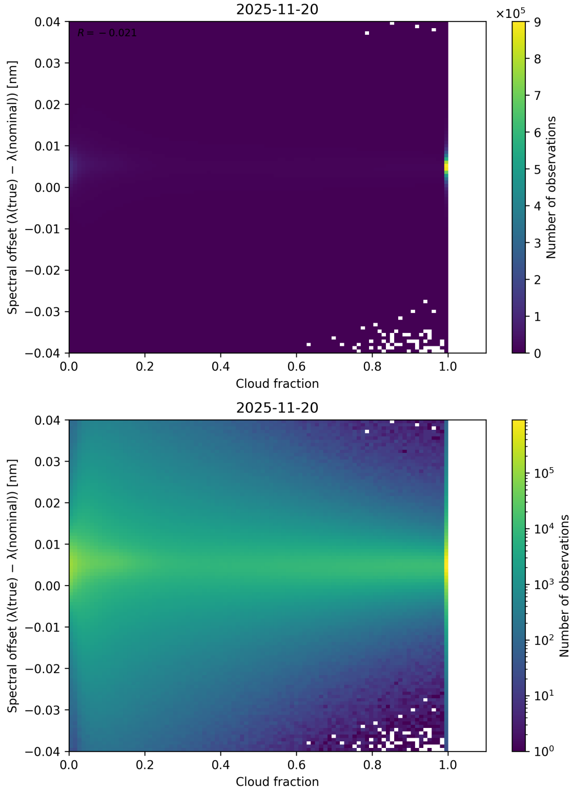
Figure 76: Scatter density plot of “Cloud fraction” against “Spectral offset ( \lambda_{\text{true}} - \lambda_{\text{nominal}} )” for 2025-11-19 to 2025-11-21.
