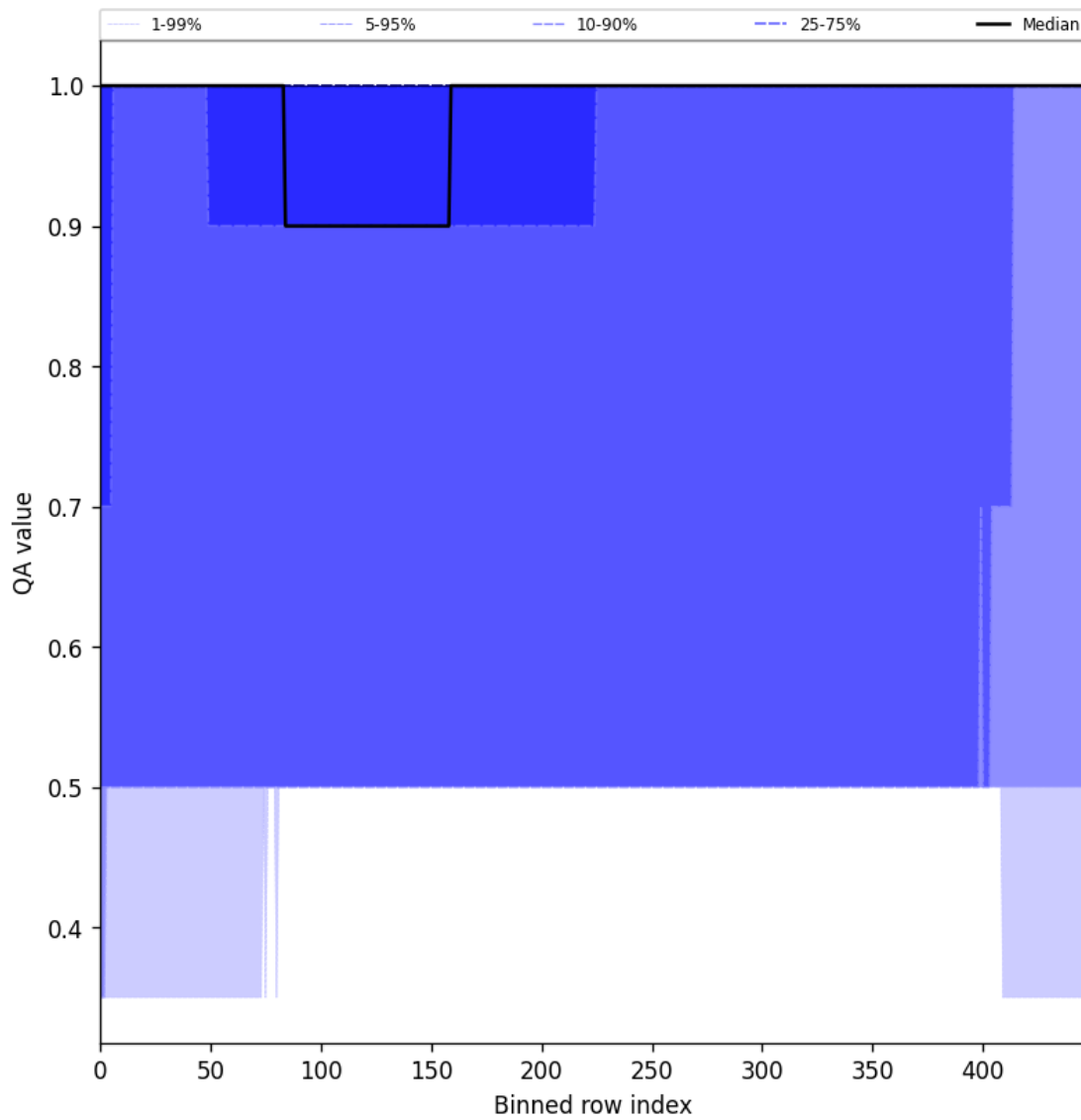
Figure 46: Along track statistics of “QA value” for 2025-11-19 to 2025-11-21
