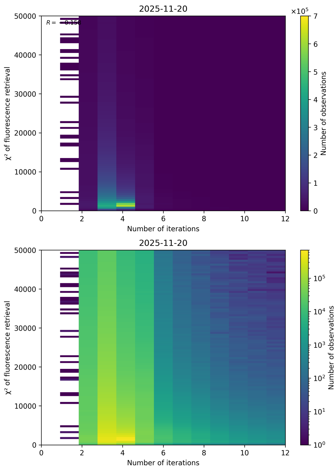
Figure 97: Scatter density plot of “Number of iterations” against “ \chi^2 of fluorescence retrieval” for 2025-11-19 to 2025-11-21.
