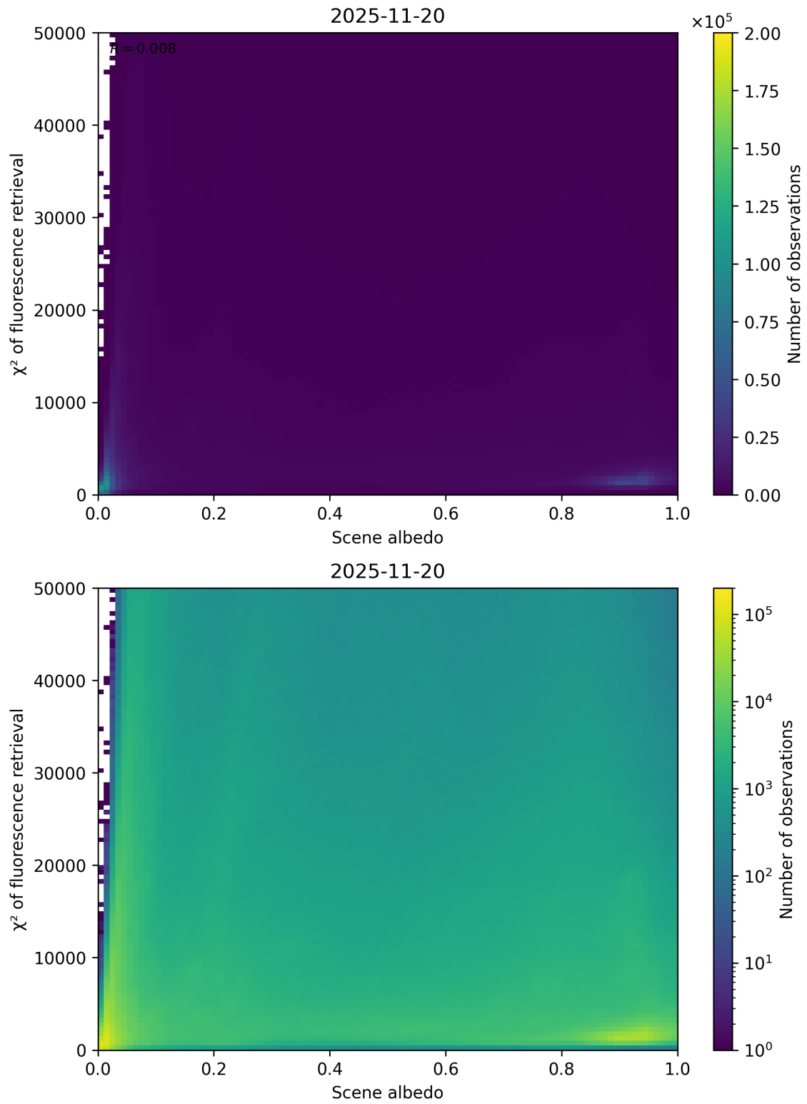
Figure 103: Scatter density plot of “Scene albedo” against “ \chi^2 of fluorescence retrieval” for 2025-11-19 to 2025-11-21.
