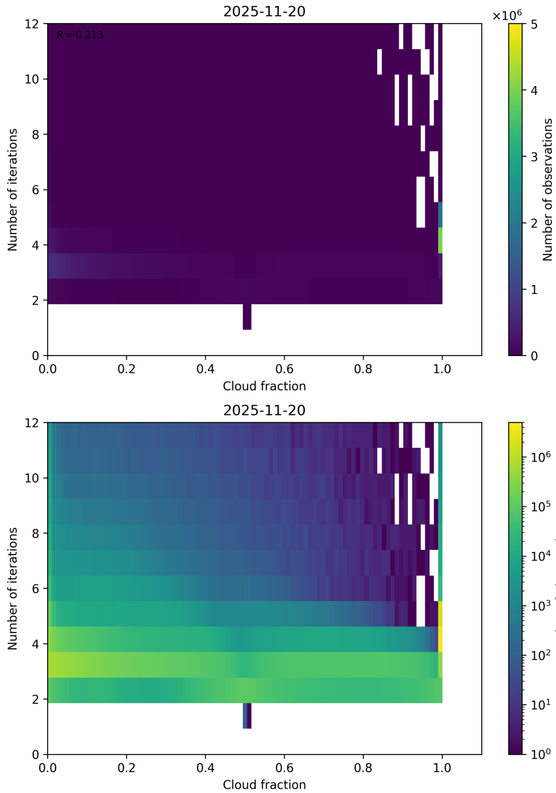
Figure 73: Scatter density plot of “Cloud fraction” against “Number of iterations” for 2025-11-19 to 2025-11-21.
