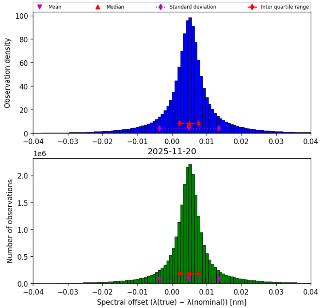
Figure 45: Histogram of “Spectral offset ( \lambda_{\text{true}} - \lambda_{\text{nominal}} )” for 2025-11-19 to 2025-11-21
