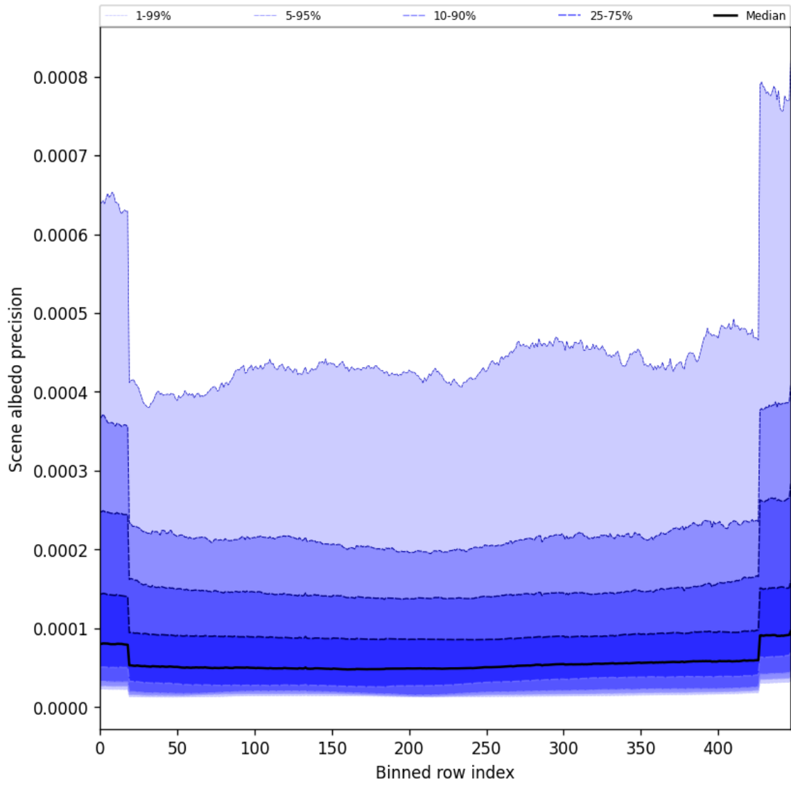
Figure 52: Along track statistics of “Scene albedo precision” for 2025-11-19 to 2025-11-21
