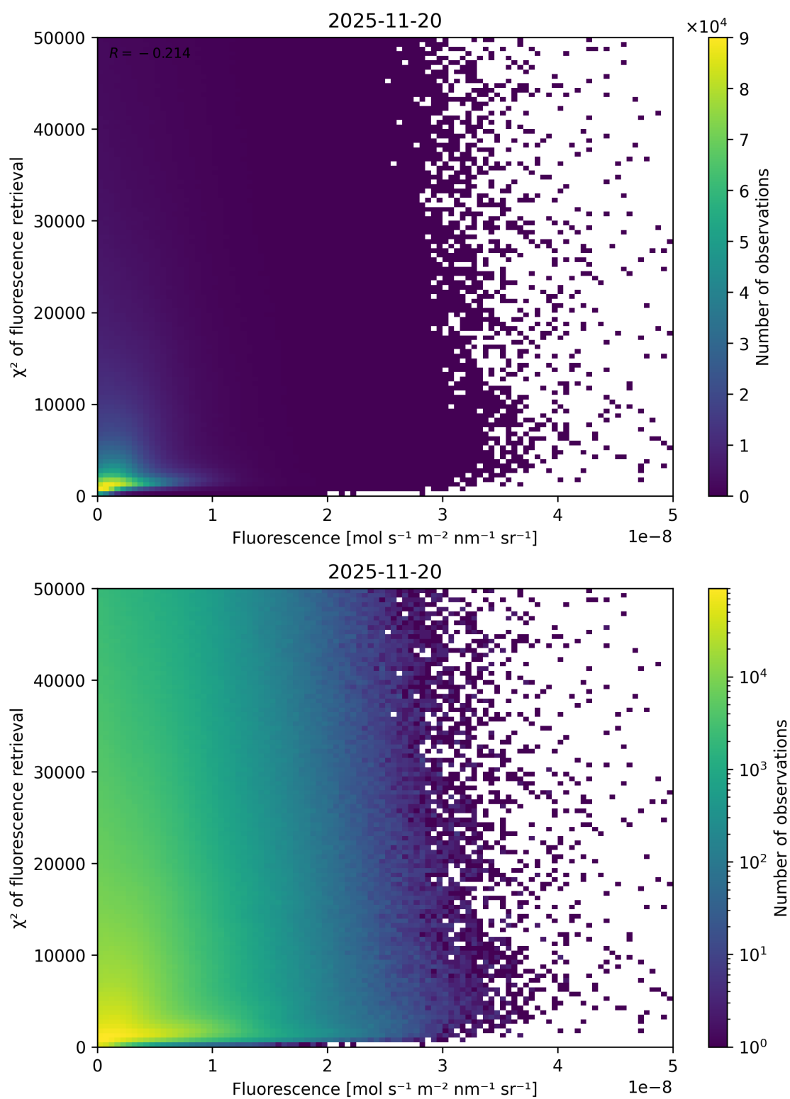
Figure 85: Scatter density plot of “Fluorescence” against “ \chi^2 of fluorescence retrieval” for 2025-11-19 to 2025-11-21.
