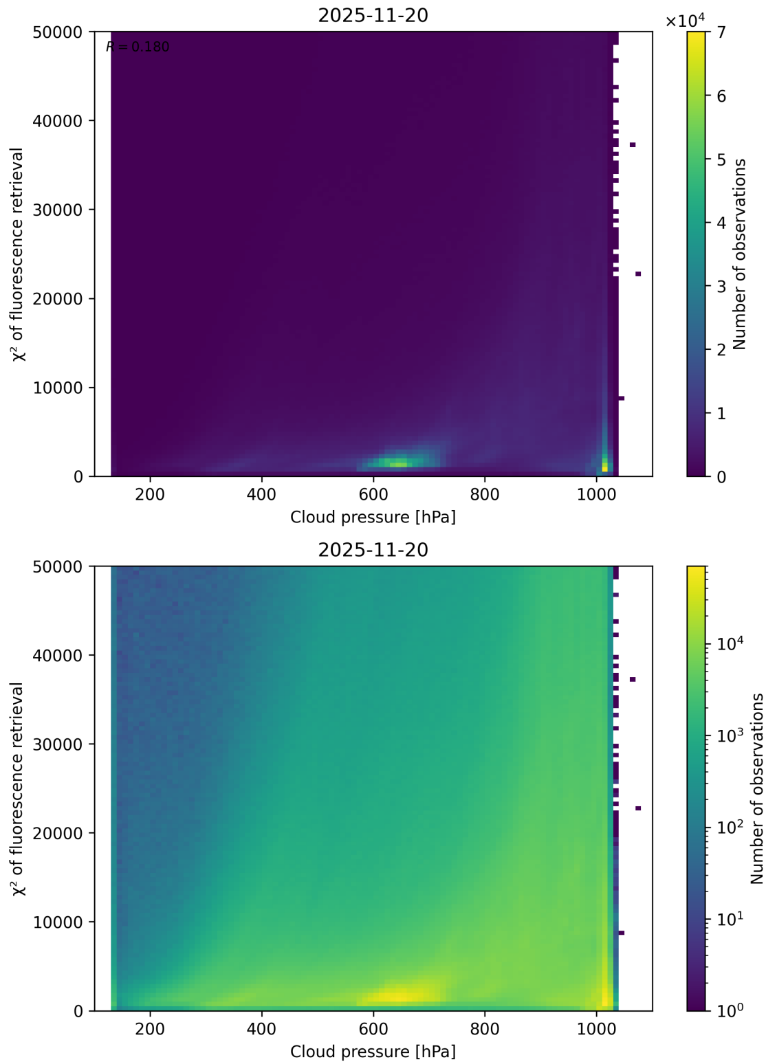
Figure 78: Scatter density plot of “Cloud pressure” against “ \chi^2 of fluorescence retrieval” for 2025-11-19 to 2025-11-21.
