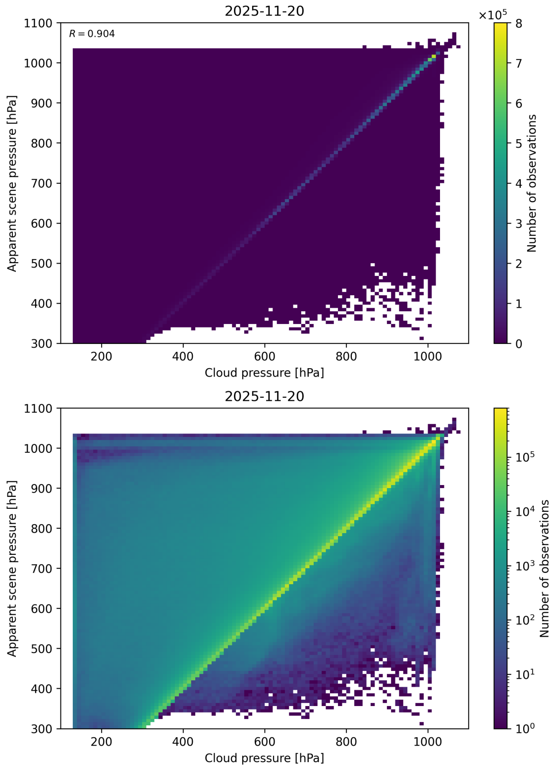
Figure 77: Scatter density plot of “Cloud pressure” against “Apparent scene pressure” for 2025-11-19 to 2025-11-21.
