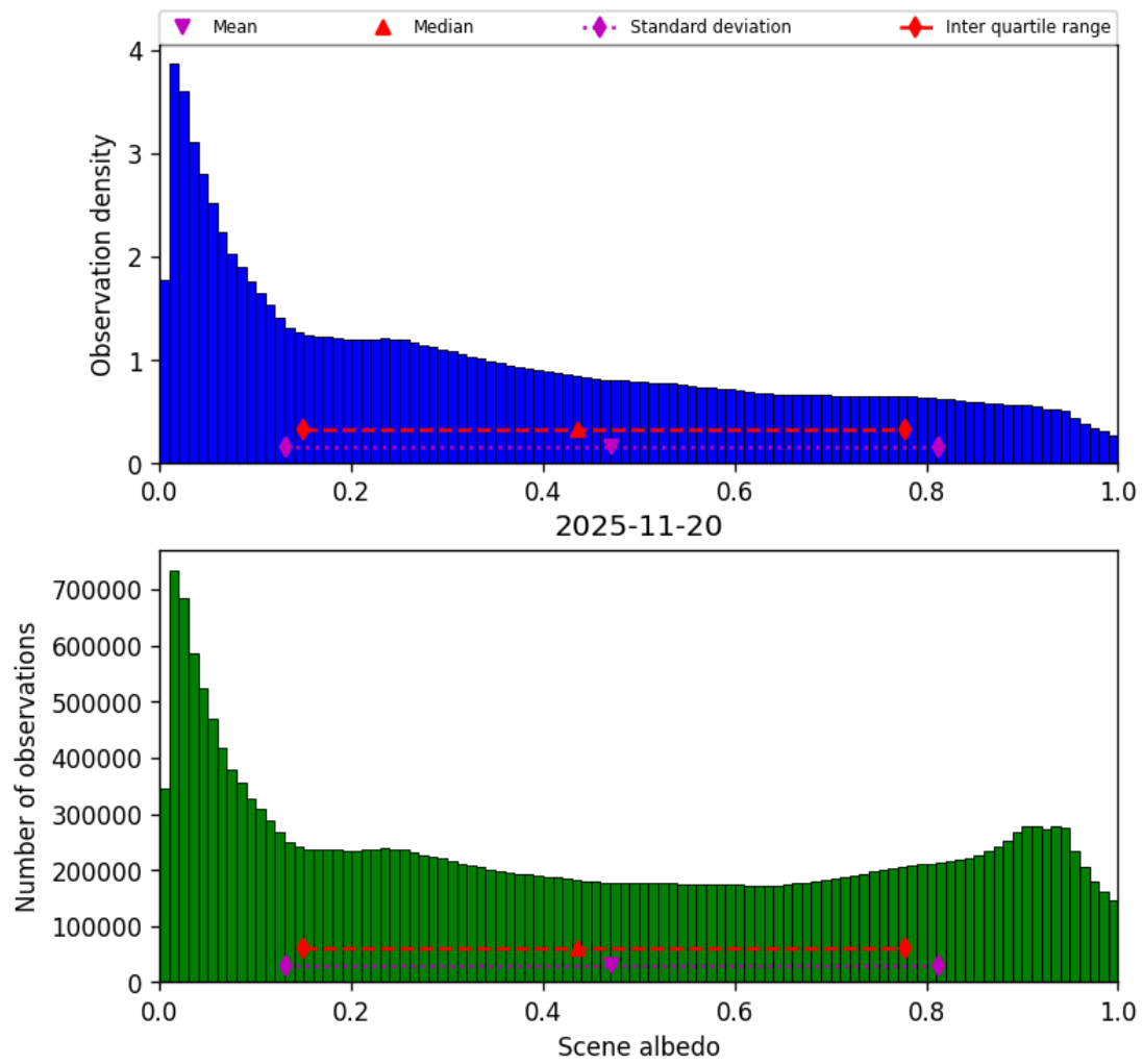
Figure 34: Histogram of “Scene albedo” for 2025-11-19 to 2025-11-21
