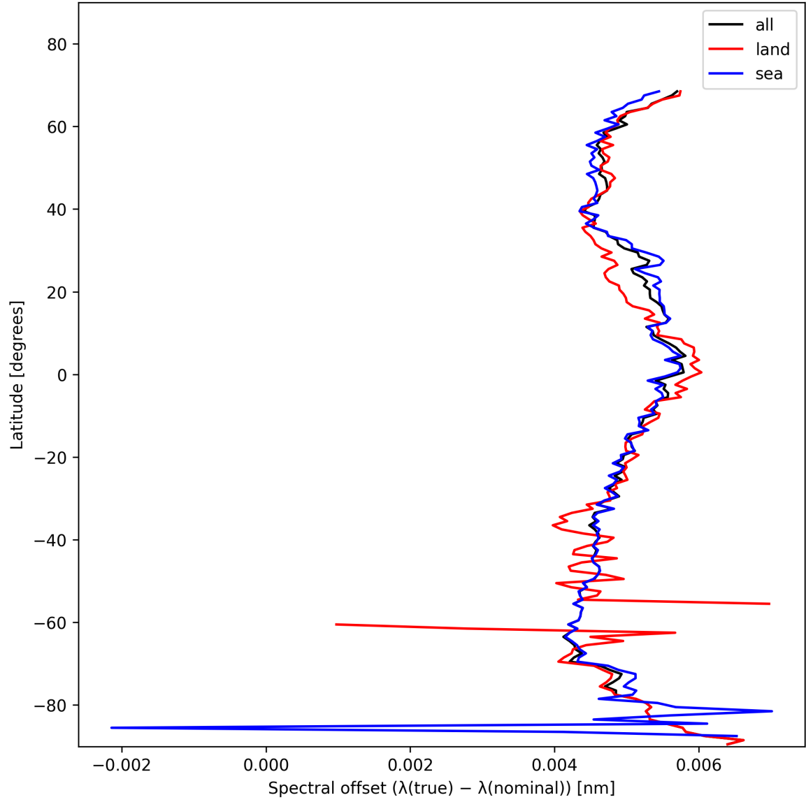
Figure 28: Zonal average of “Spectral offset ( \lambda_{\text{true}} - \lambda_{\text{nominal}} )” for 2025-11-19 to 2025-11-21.
