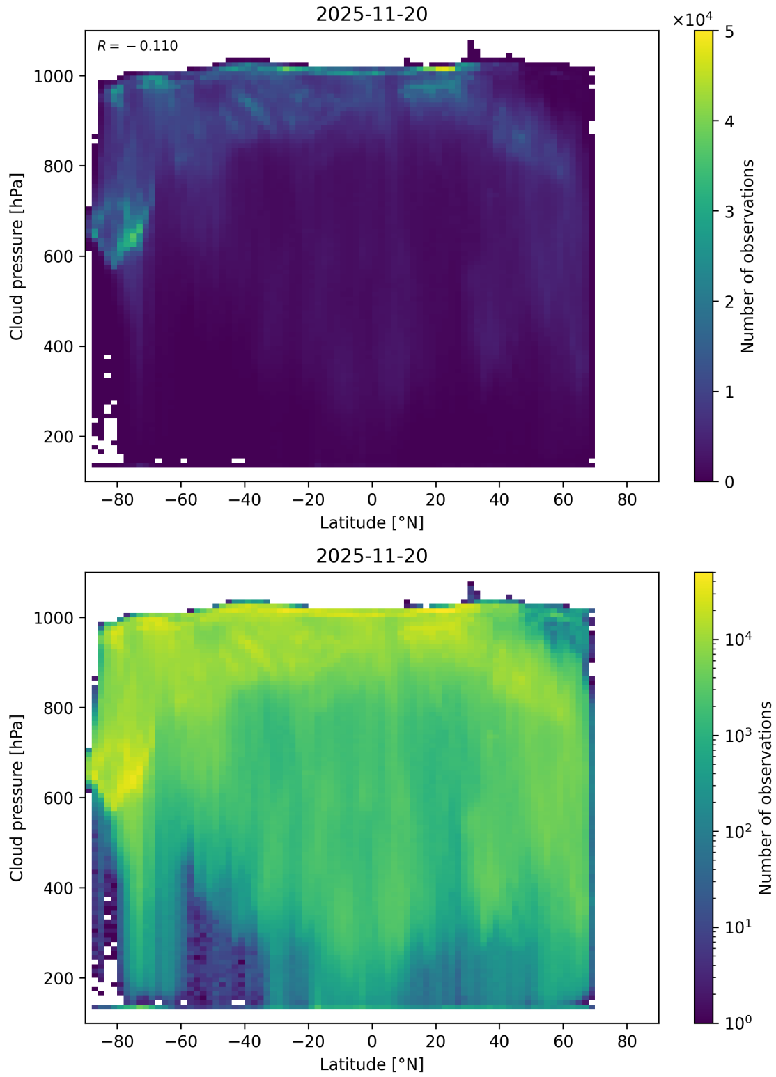
Figure 91: Scatter density plot of “Latitude” against “Cloud pressure” for 2025-11-19 to 2025-11-21.
