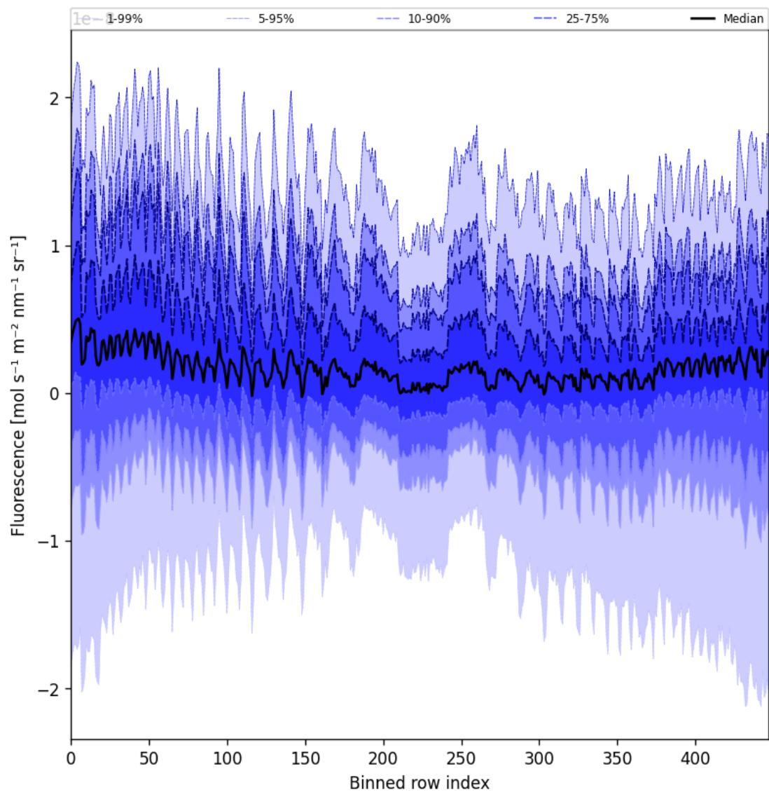
Figure 57: Along track statistics of “Fluorescence” for 2025-11-19 to 2025-11-21
