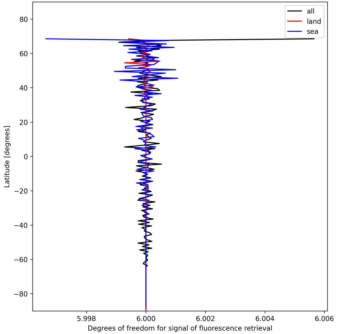
Figure 26: Zonal average of “Degrees of freedom for signal of fluorescence retrieval” for 2025-11-19 to 2025-11-21.
