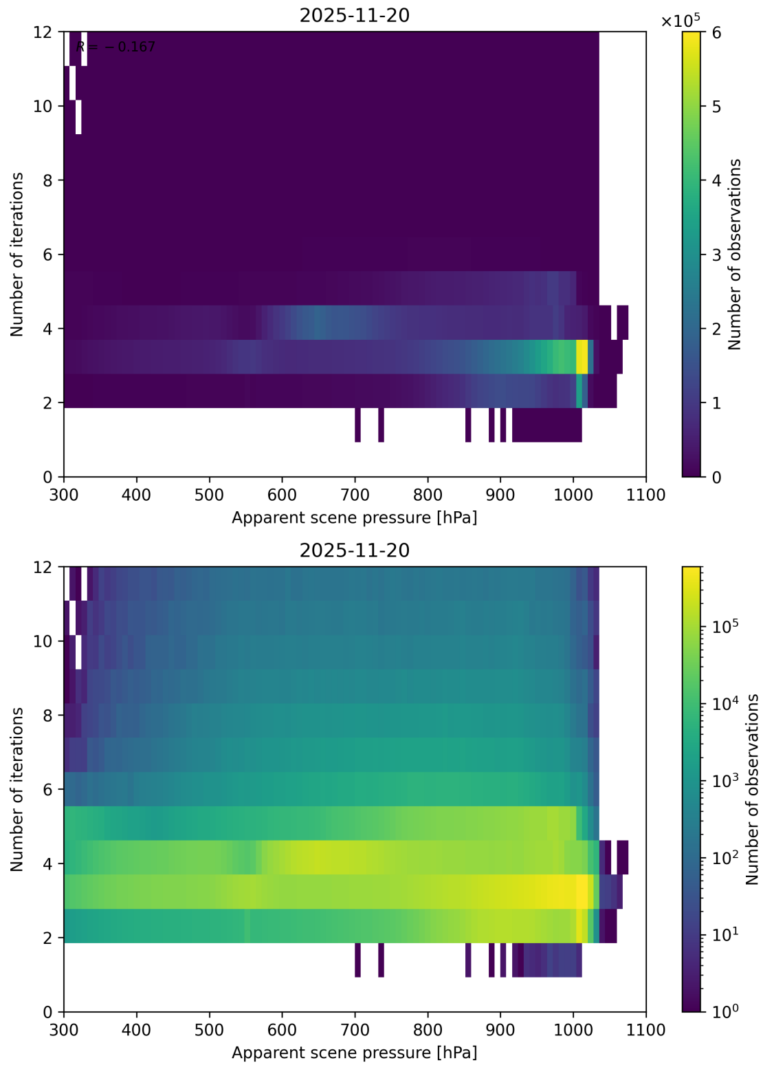
Figure 65: Scatter density plot of “Apparent scene pressure” against “Number of iterations” for 2025-11-19 to 2025-11-21.
