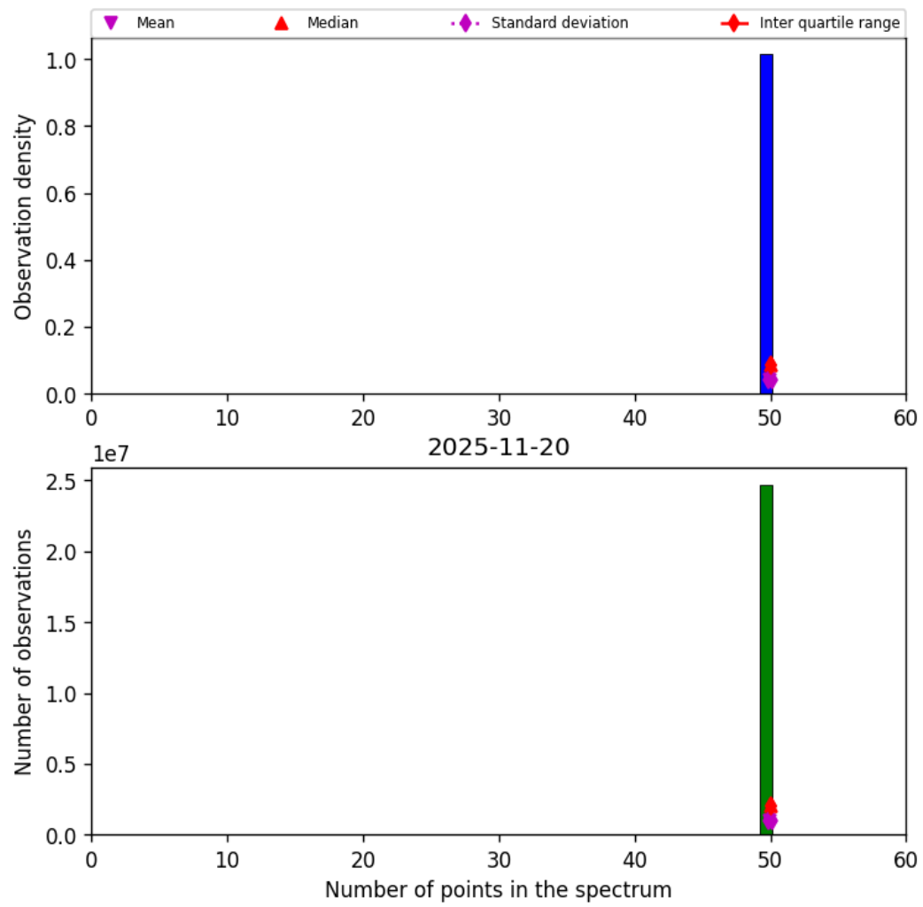
Figure 44: Histogram of “Number of points in the spectrum” for 2025-11-19 to 2025-11-21
