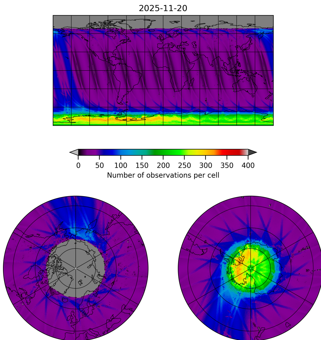
Figure 11: Map of the number of observations for 2025-11-19 to 2025-11-21
