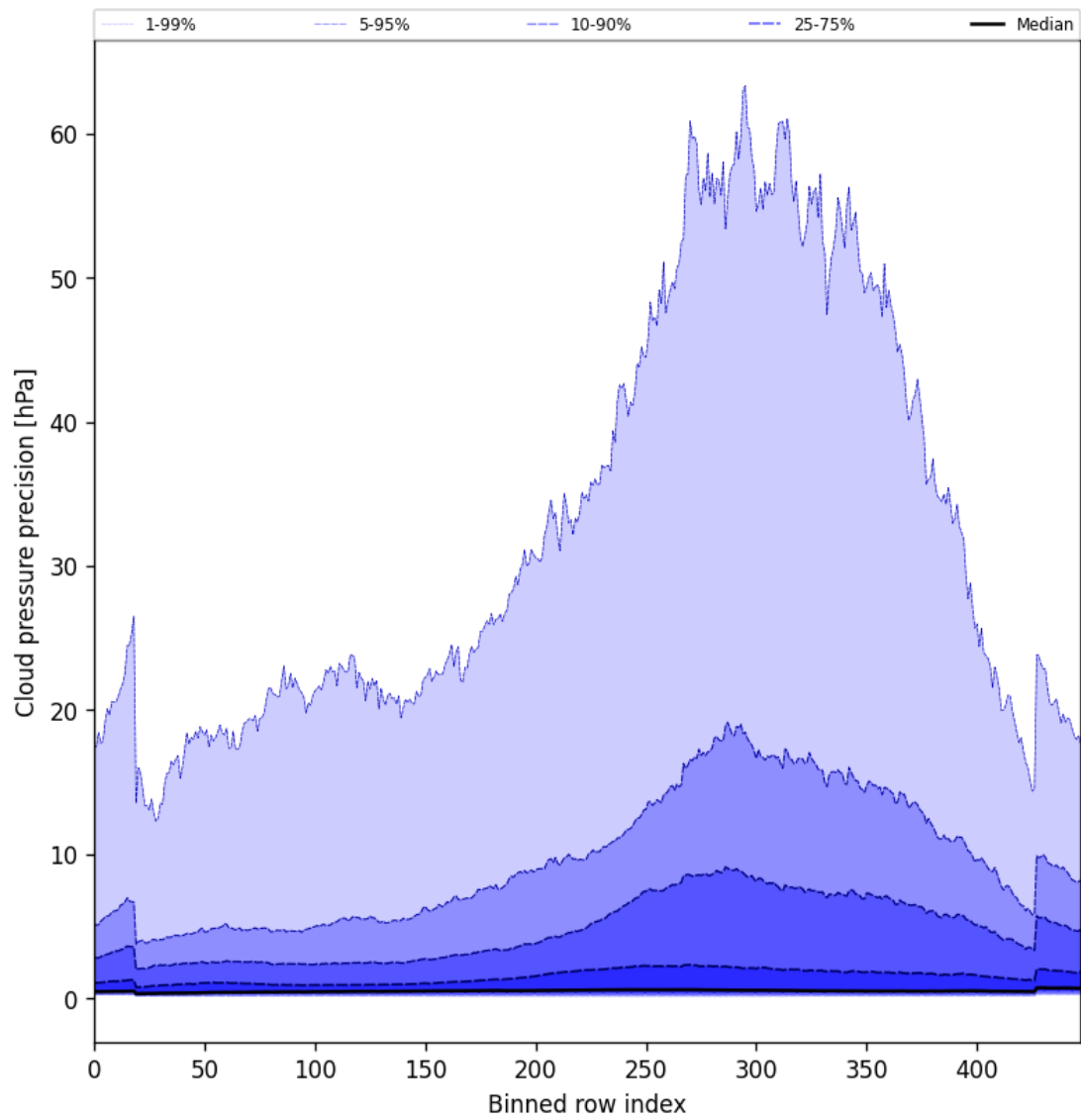
Figure 48: Along track statistics of “Cloud pressure precision” for 2025-11-19 to 2025-11-21
