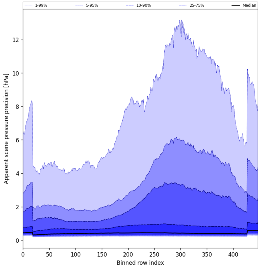
Figure 54: Along track statistics of “Apparent scene pressure precision” for 2025-11-19 to 2025-11-21
