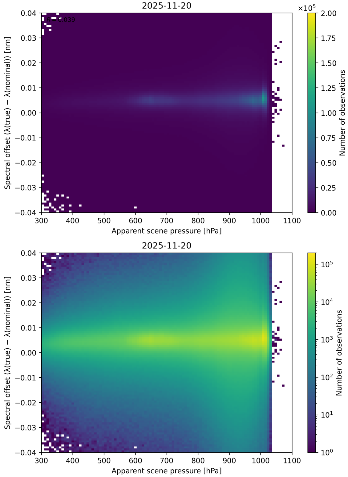
Figure 67: Scatter density plot of “Apparent scene pressure” against “Spectral offset ( \lambda_{\text{true}} - \lambda_{\text{nominal}} )” for 2025-11-19 to 2025-11-21.
