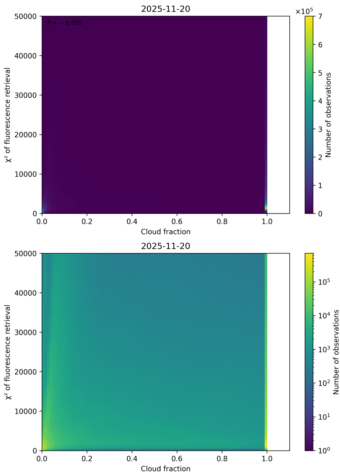
Figure 71: Scatter density plot of “Cloud fraction” against “ \chi^2 of fluorescence retrieval” for 2025-11-19 to 2025-11-21.
