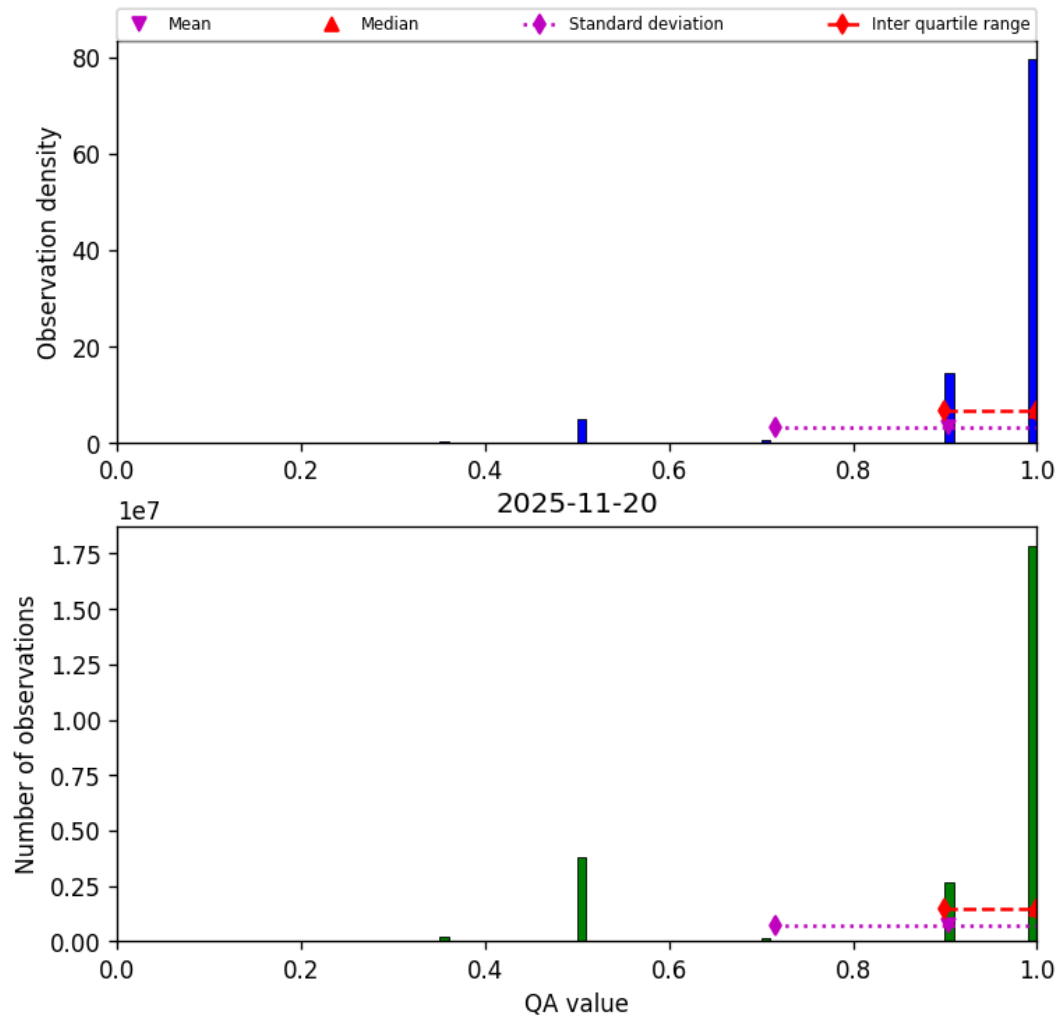
Figure 29: Histogram of “QA value” for 2025-11-19 to 2025-11-21
