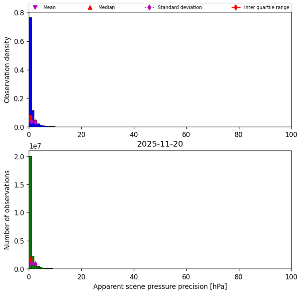
Figure 37: Histogram of “Apparent scene pressure precision” for 2025-11-19 to 2025-11-21
