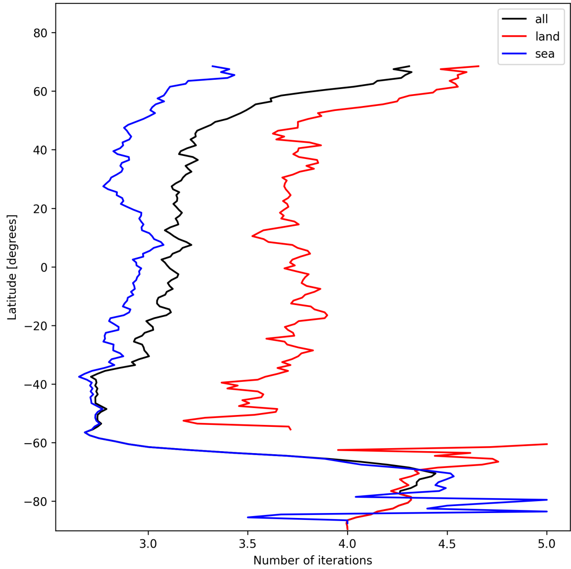
Figure 22: Zonal average of “Number of iterations” for 2025-11-19 to 2025-11-21.
