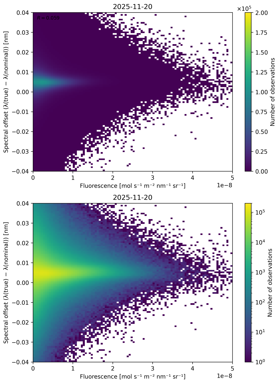
Figure 87: Scatter density plot of “Fluorescence” against “Spectral offset ( \lambda_{\text{true}} - \lambda_{\text{nominal}} )” for 2025-11-19 to 2025-11-21.
