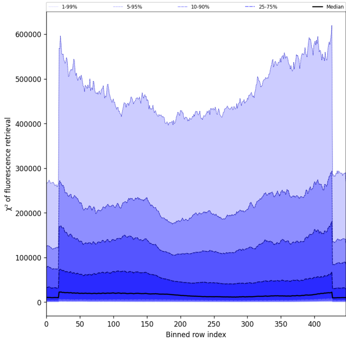
Figure 59: Along track statistics of “ \chi^2 of fluorescence retrieval” for 2025-11-19 to 2025-11-21
