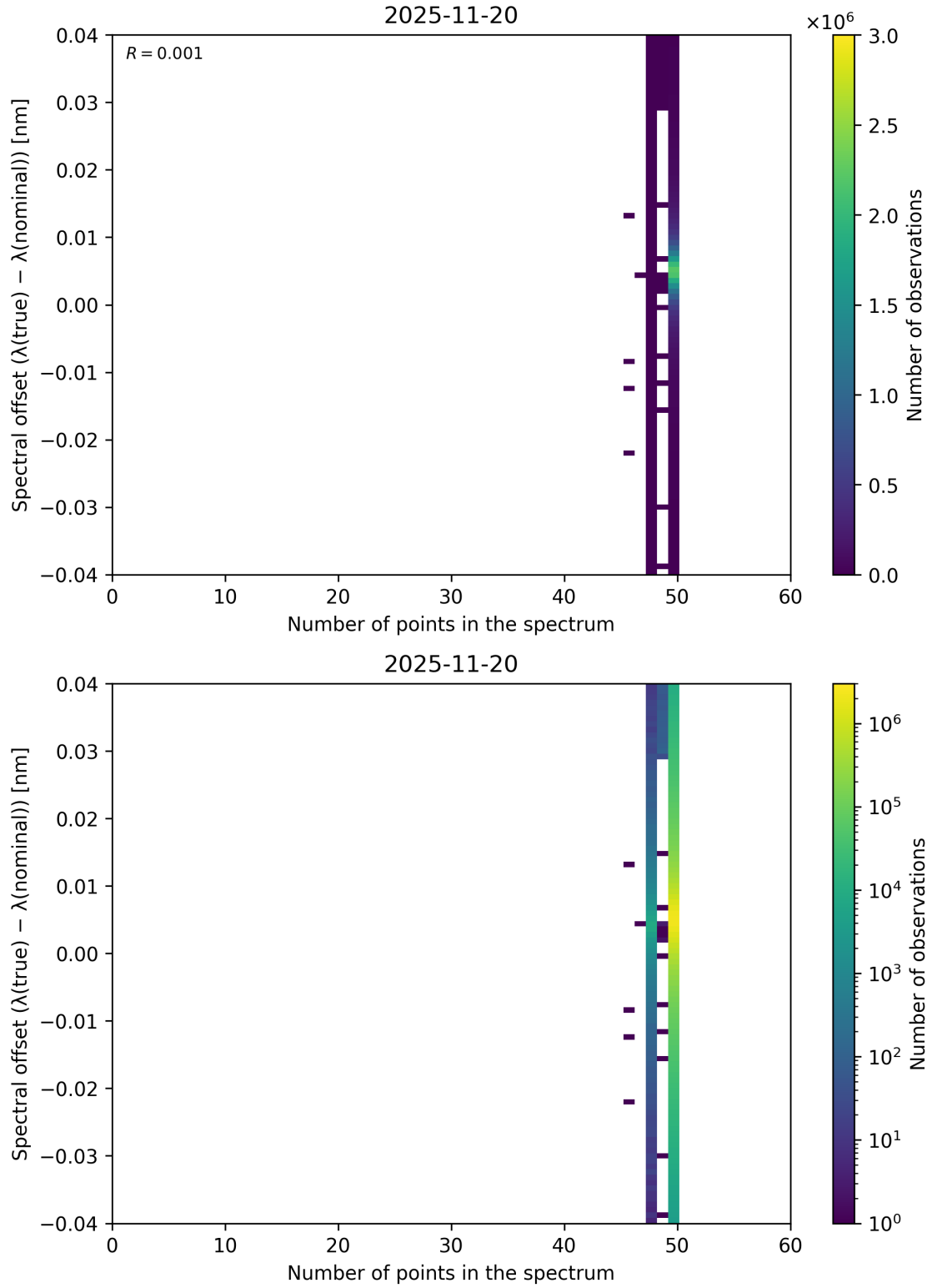
Figure 101: Scatter density plot of “Number of points in the spectrum” against “Spectral offset ( \lambda_{\text{true}} - \lambda_{\text{nominal}} )” for 2025-11-19 to 2025-11-21.
