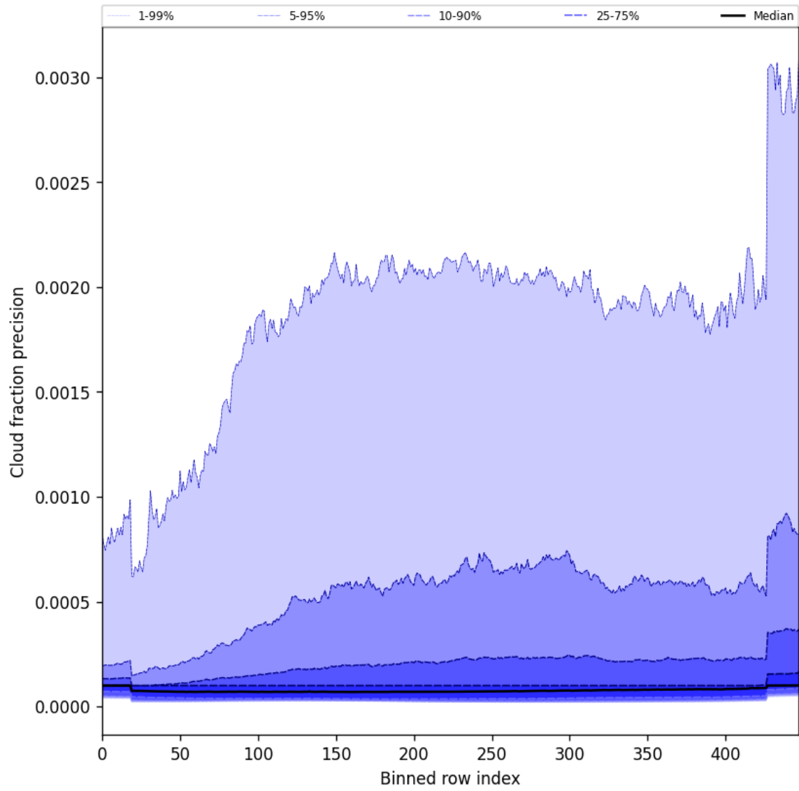
Figure 50: Along track statistics of “Cloud fraction precision” for 2025-11-19 to 2025-11-21
