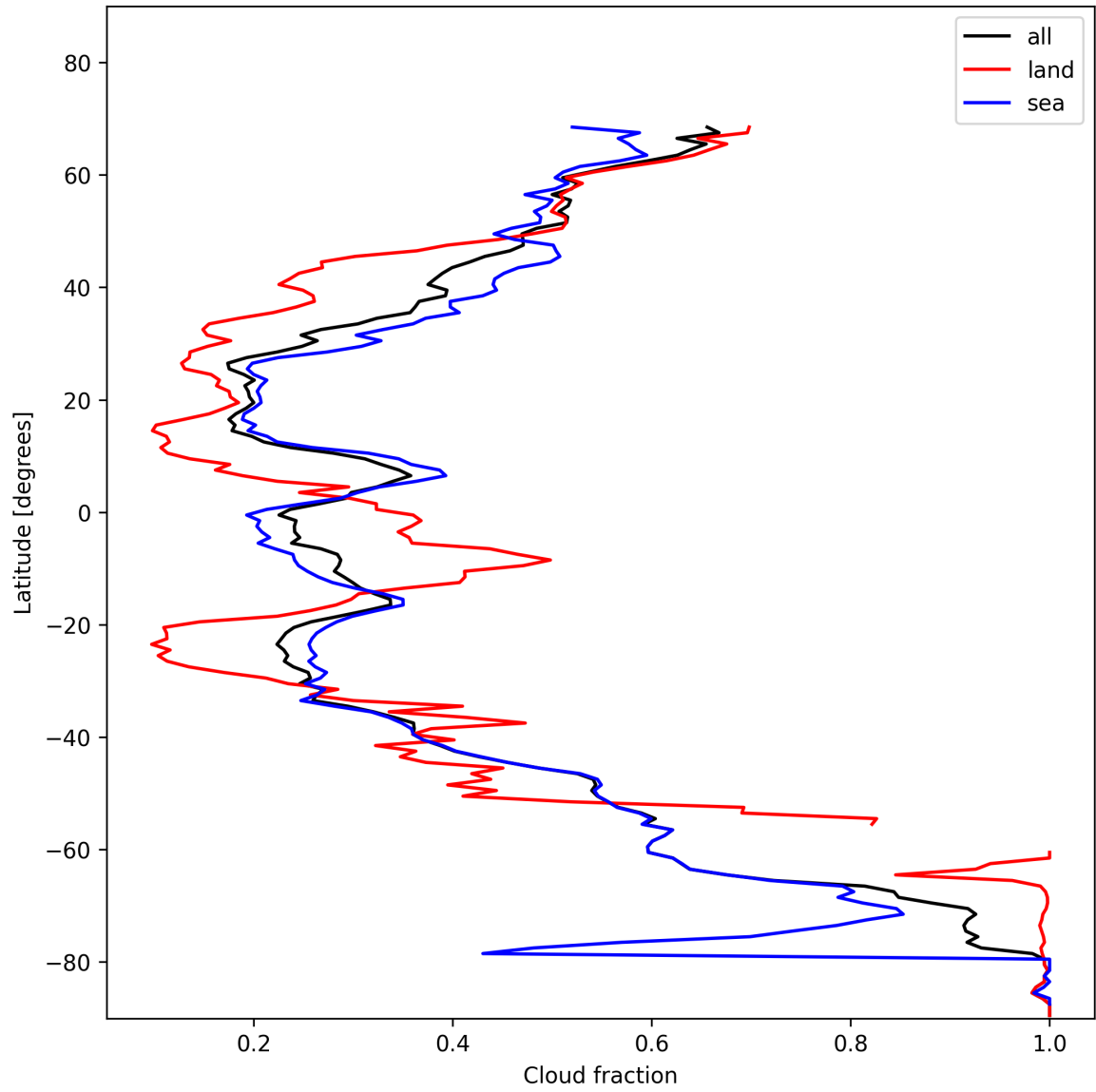
Figure 15: Zonal average of “Cloud fraction” for 2025-11-19 to 2025-11-21.
