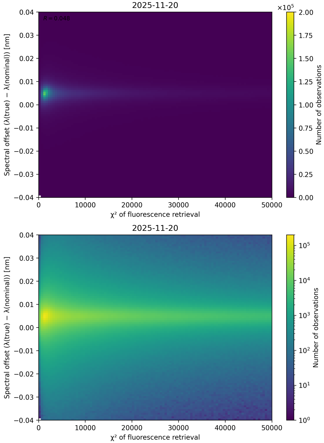
Figure 69: Scatter density plot of “ \chi^2 of fluorescence retrieval” against “Spectral offset ( \lambda_{\text{true}} - \lambda_{\text{nominal}} )” for 2025-11-19 to 2025-11-21.
