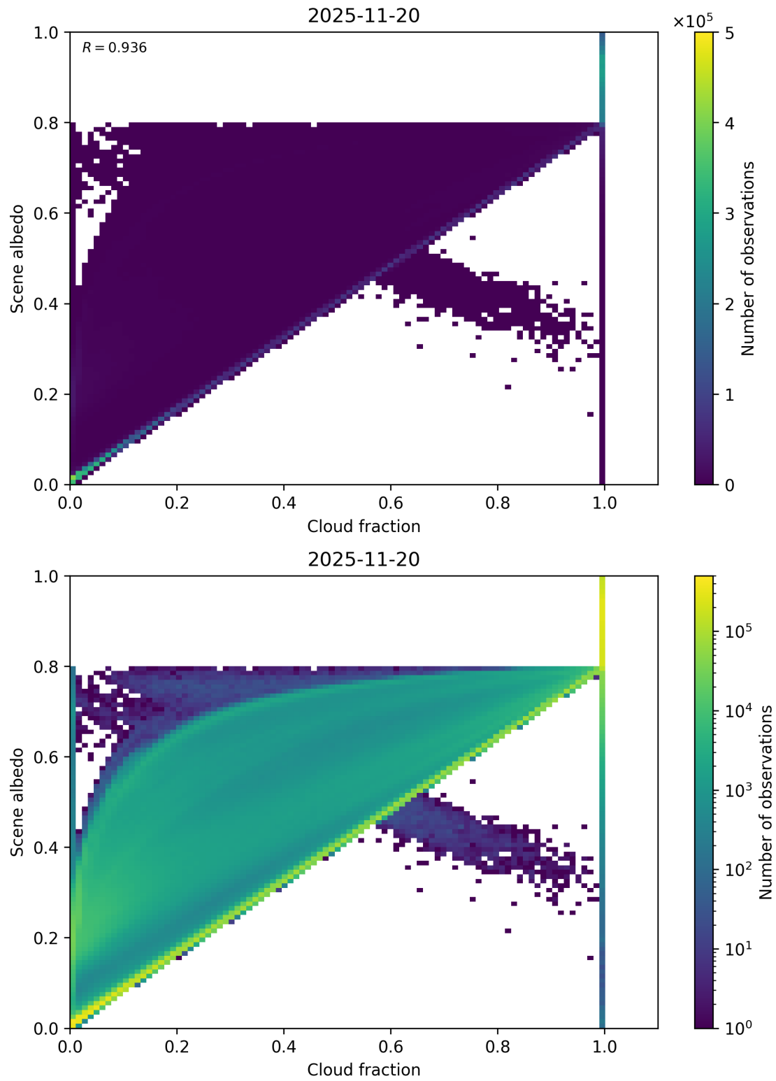
Figure 75: Scatter density plot of “Cloud fraction” against “Scene albedo” for 2025-11-19 to 2025-11-21.
