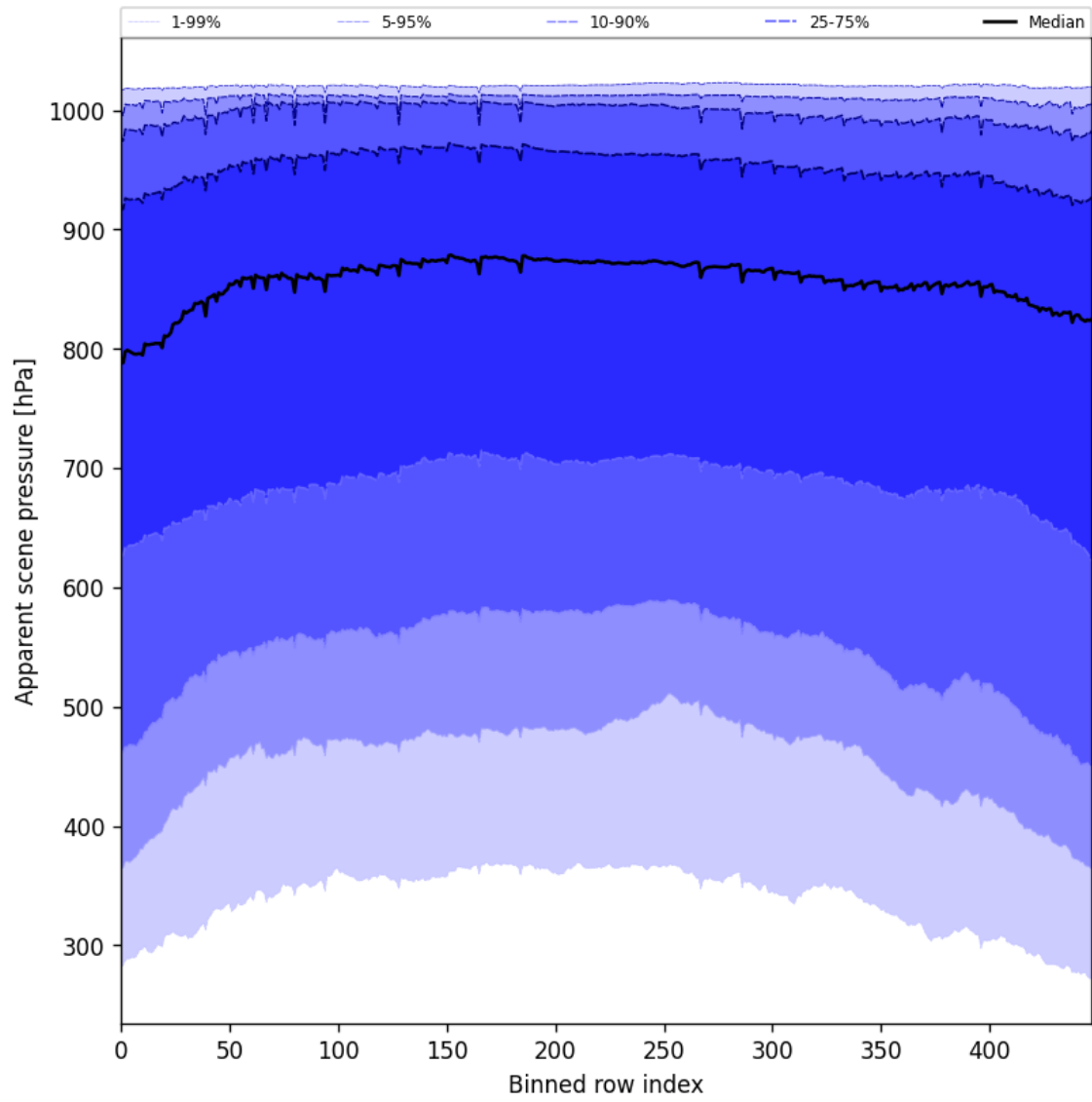
Figure 53: Along track statistics of “Apparent scene pressure” for 2025-11-19 to 2025-11-21
