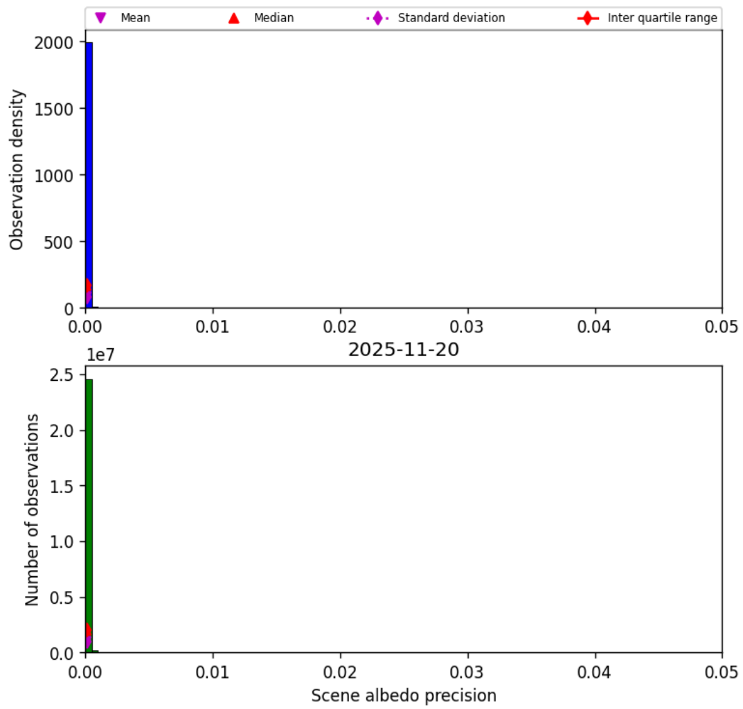
Figure 35: Histogram of “Scene albedo precision” for 2025-11-19 to 2025-11-21
