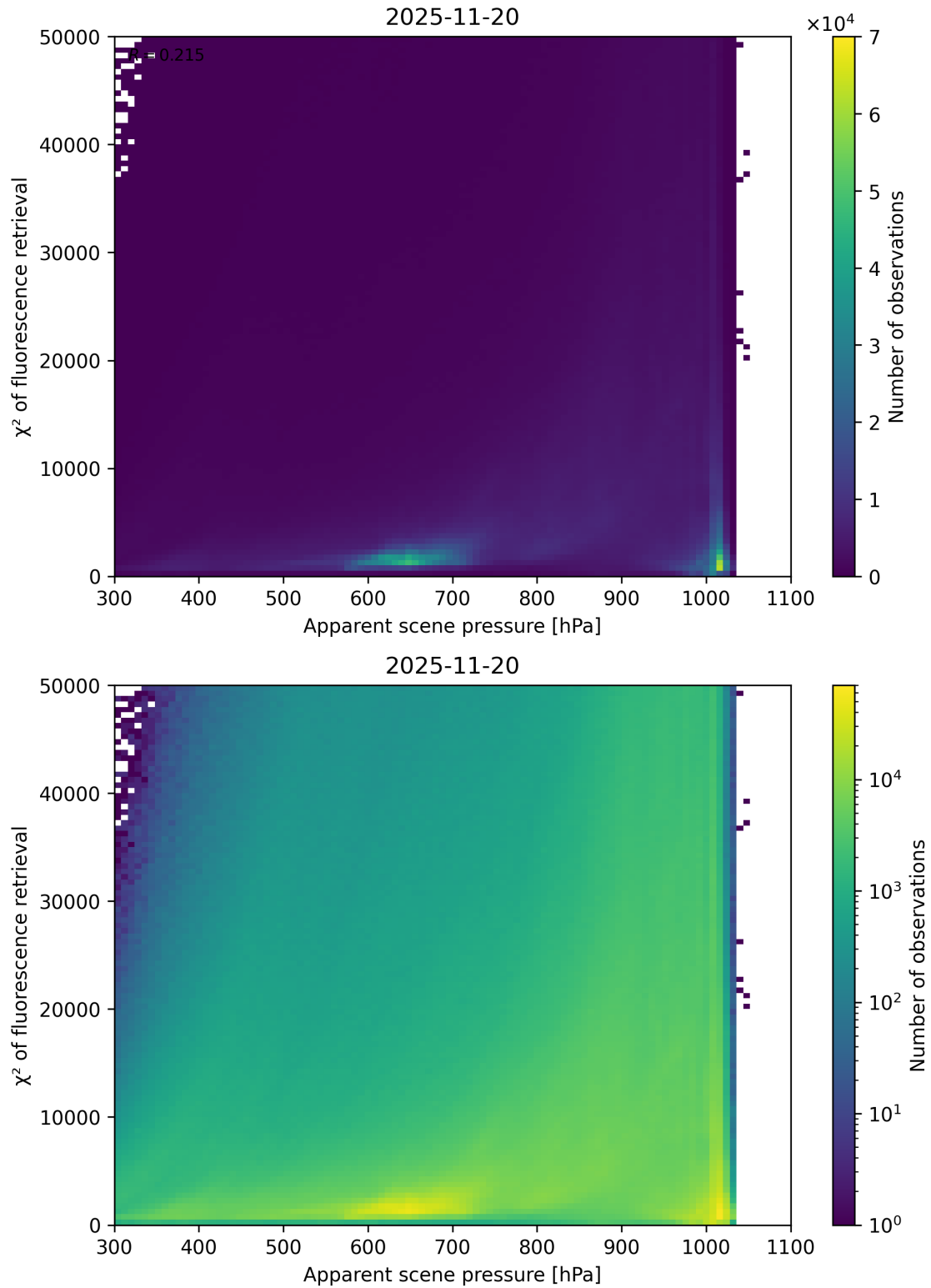
Figure 63: Scatter density plot of “Apparent scene pressure” against “ \chi^2 of fluorescence retrieval” for 2025-11-19 to 2025-11-21.
