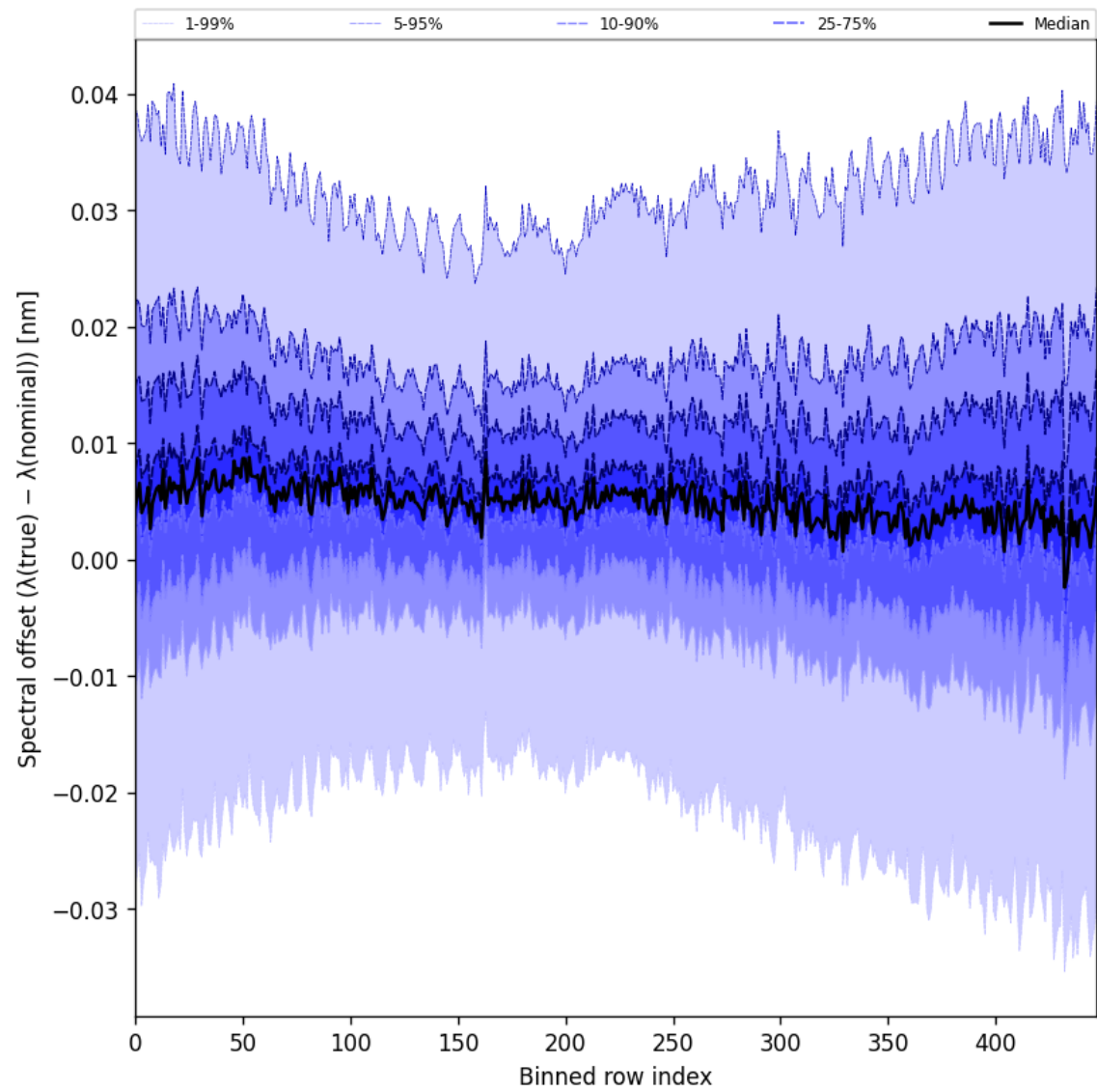
Figure 62: Along track statistics of “Spectral offset ( \lambda_{\text{true}} - \lambda_{\text{nominal}} )” for 2025-11-19 to 2025-11-21
