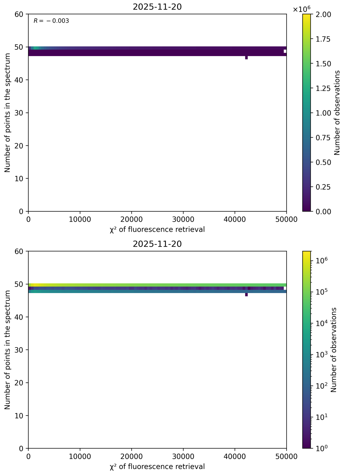
Figure 68: Scatter density plot of “ \chi^2 of fluorescence retrieval” against “Number of points in the spectrum” for 2025-11-19 to 2025-11-21.
