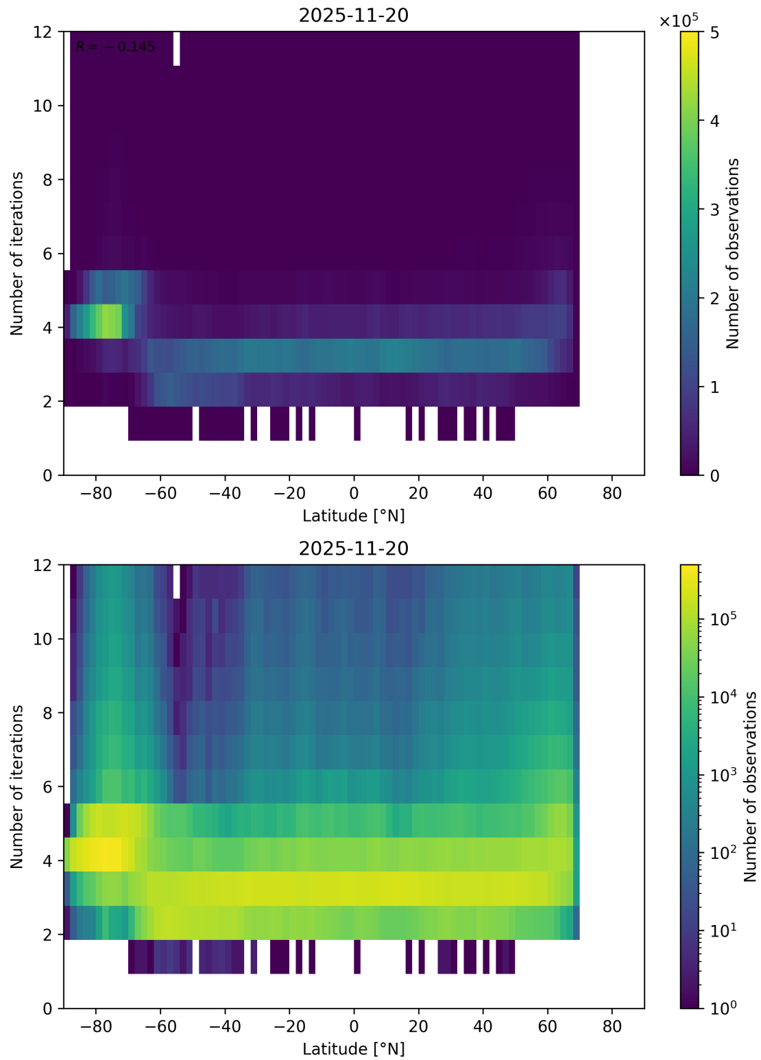
Figure 93: Scatter density plot of “Latitude” against “Number of iterations” for 2025-11-19 to 2025-11-21.
