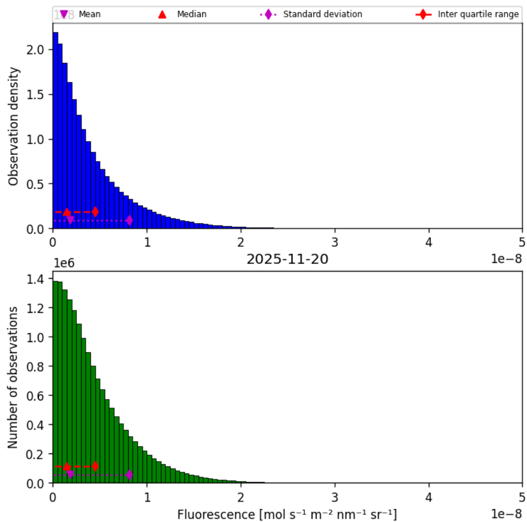
Figure 40: Histogram of “Fluorescence” for 2025-11-19 to 2025-11-21
