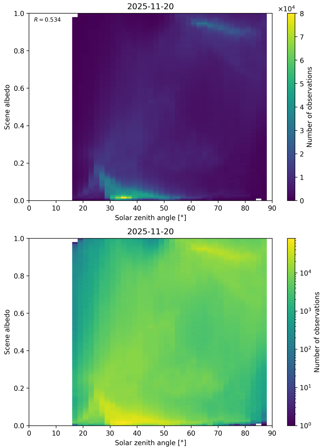
Figure 116: Scatter density plot of “Solar zenith angle” against “Scene albedo” for 2025-11-19 to 2025-11-21.
