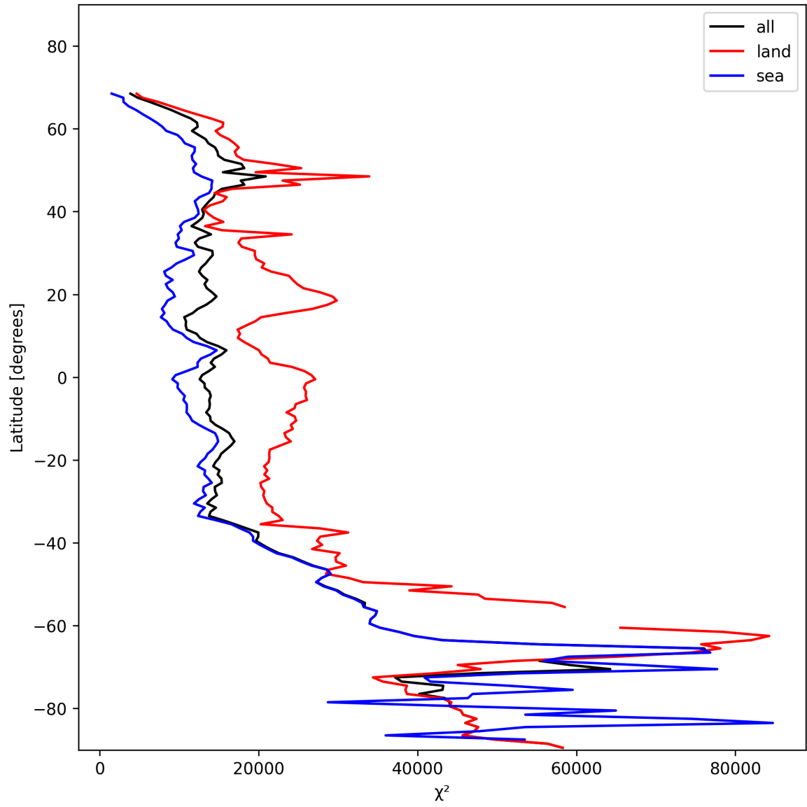
Figure 21: Zonal average of “ \chi^2 ” for 2025-11-19 to 2025-11-21.
