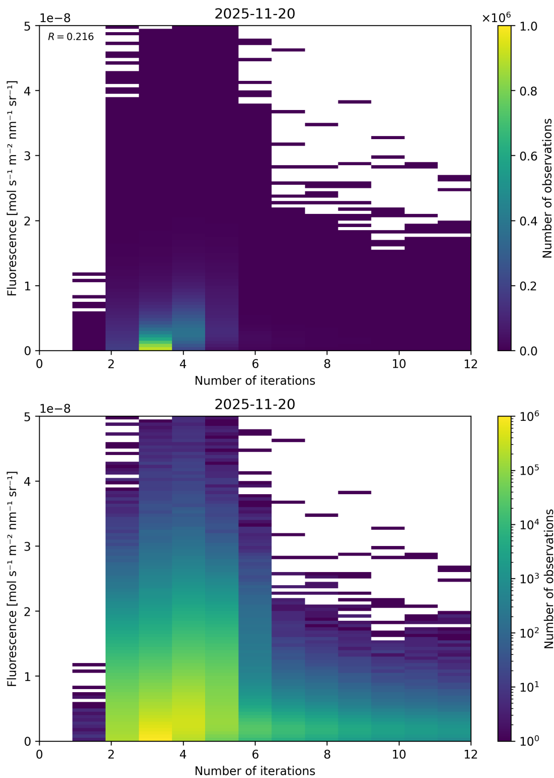
Figure 98: Scatter density plot of “Number of iterations” against “Fluorescence” for 2025-11-19 to 2025-11-21.
