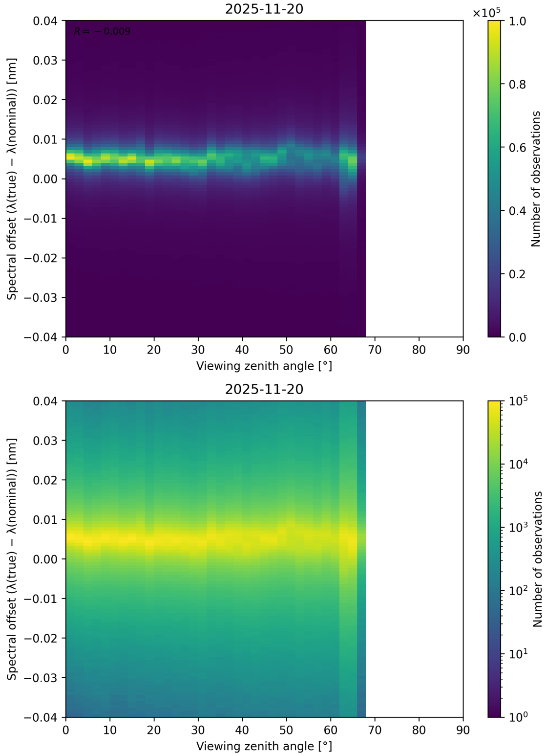
Figure 128: Scatter density plot of “Viewing zenith angle” against “Spectral offset ( \lambda_{\text{true}} - \lambda_{\text{nominal}} )” for 2025-11-19 to 2025-11-21.
