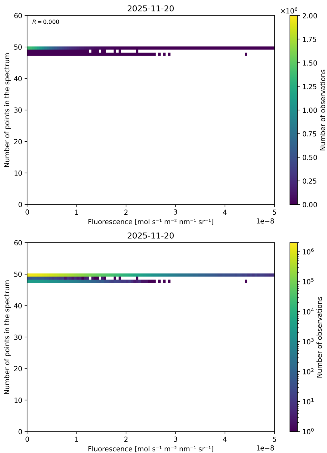
Figure 86: Scatter density plot of “Fluorescence” against “Number of points in the spectrum” for 2025-11-19 to 2025-11-21.
