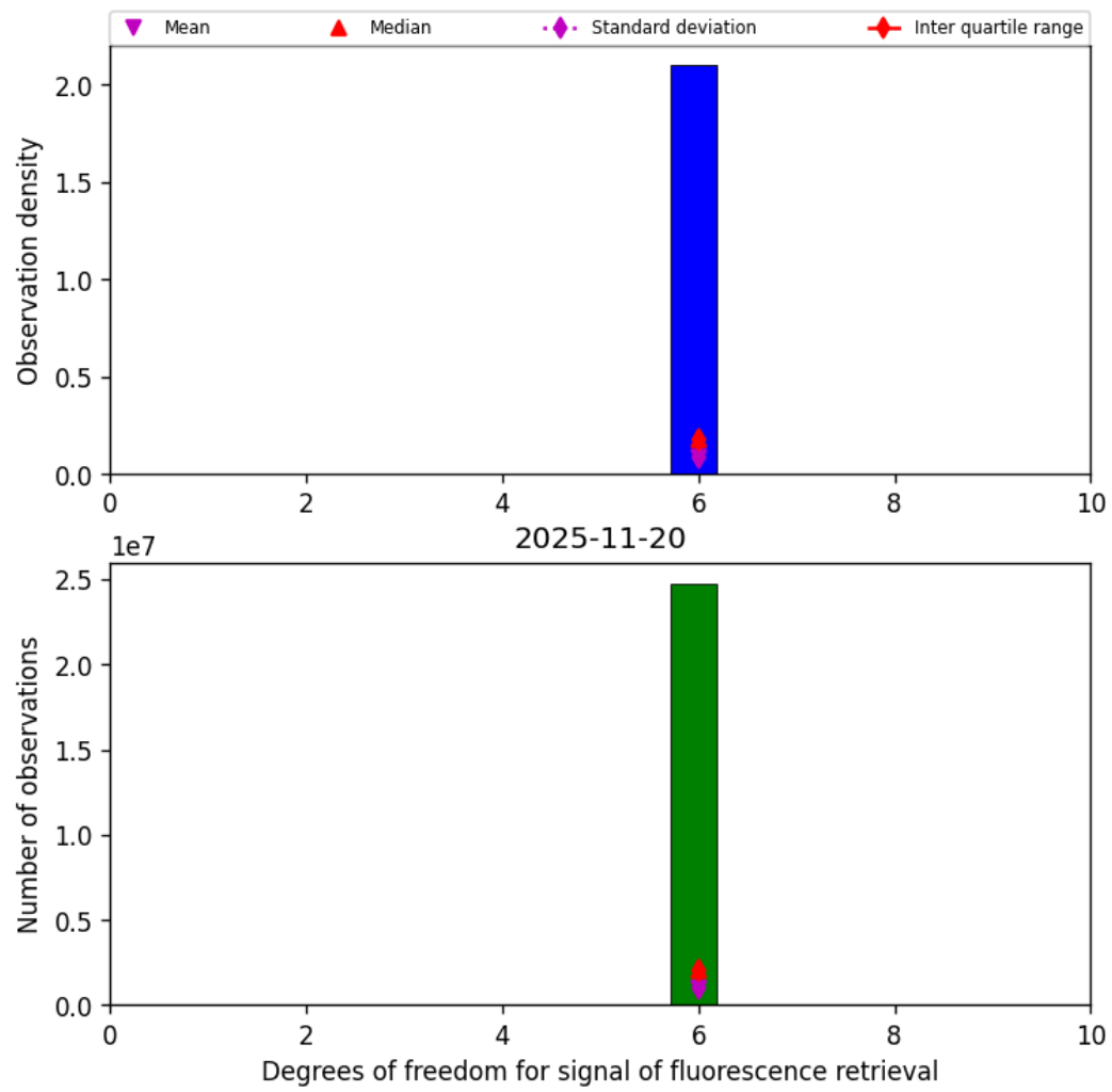
Figure 43: Histogram of “Degrees of freedom for signal of fluorescence retrieval” for 2025-11-19 to 2025-11-21
