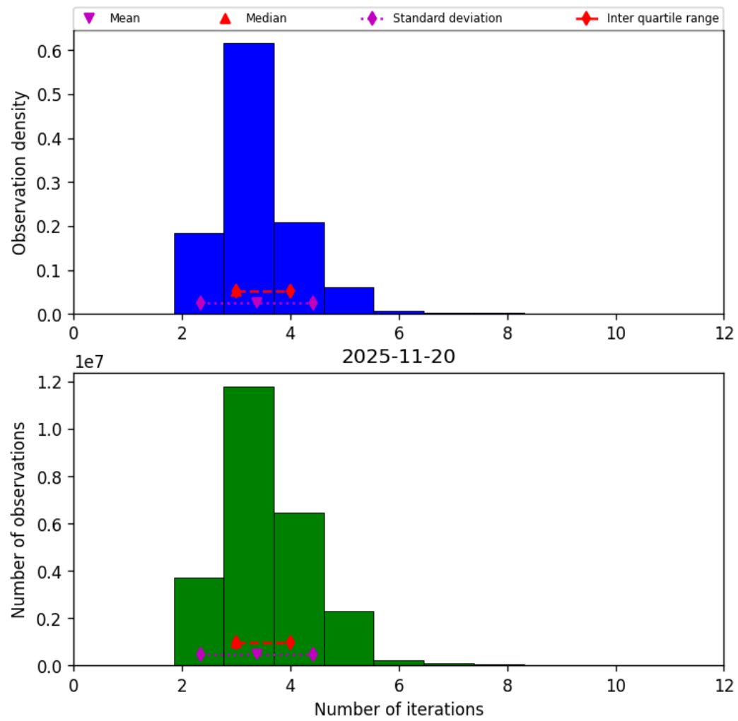
Figure 39: Histogram of “Number of iterations” for 2025-11-19 to 2025-11-21
