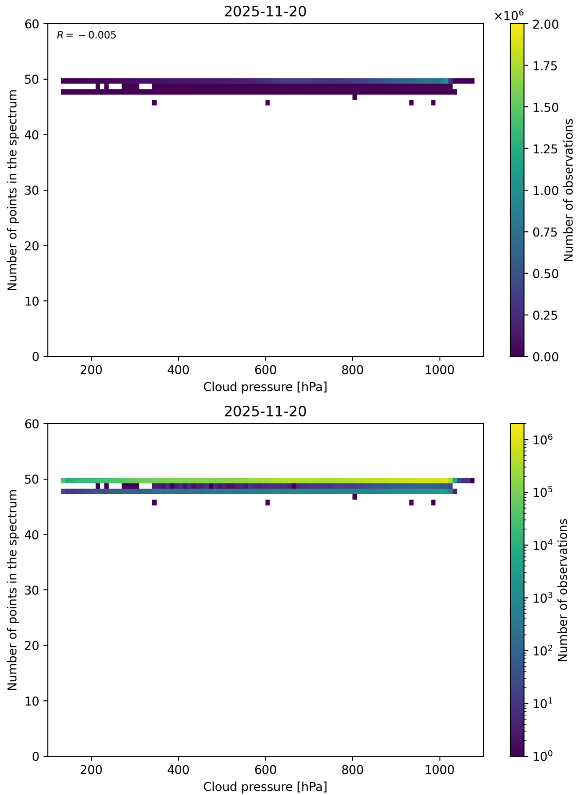
Figure 82: Scatter density plot of “Cloud pressure” against “Number of points in the spectrum” for 2025-11-19 to 2025-11-21.
