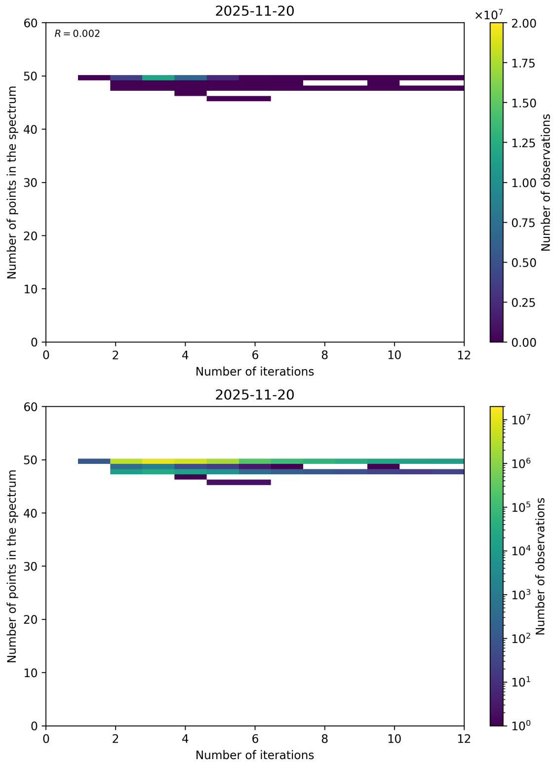
Figure 99: Scatter density plot of “Number of iterations” against “Number of points in the spectrum” for 2025-11-19 to 2025-11-21.
