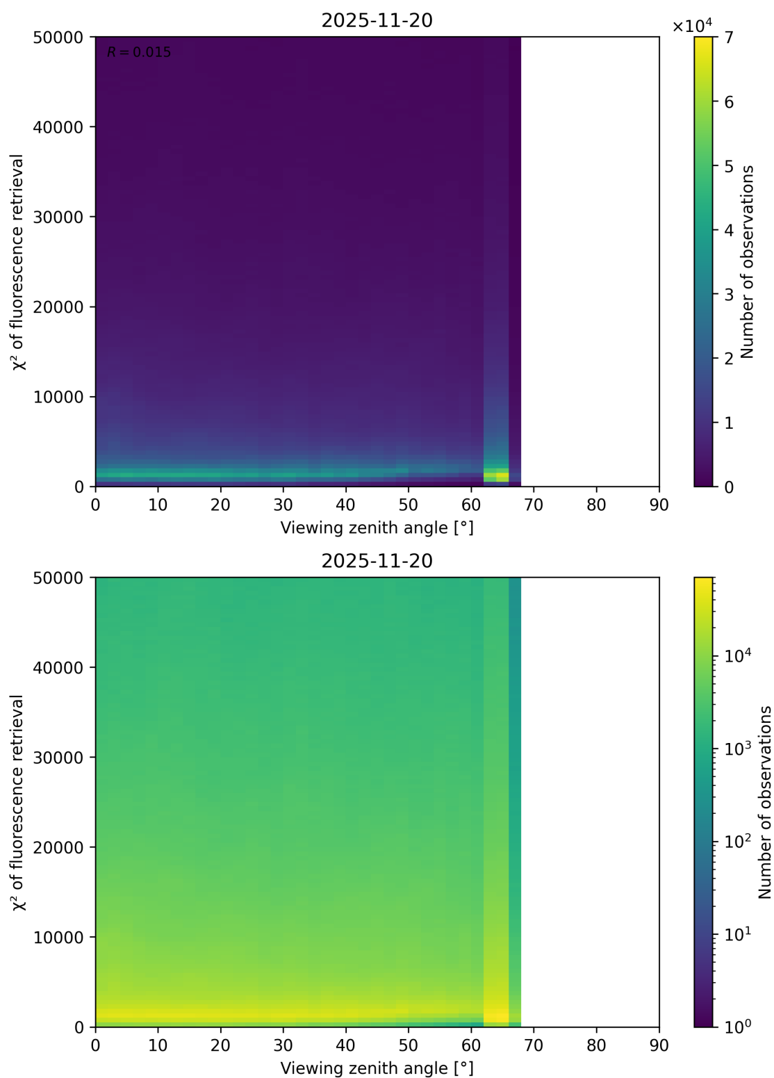
Figure 119: Scatter density plot of “Viewing zenith angle” against “ \chi^2 of fluorescence retrieval” for 2025-11-19 to 2025-11-21.
