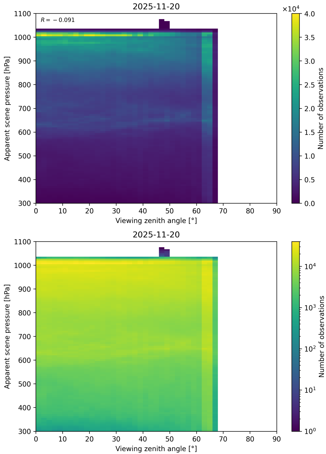
Figure 118: Scatter density plot of “Viewing zenith angle” against “Apparent scene pressure” for 2025-11-19 to 2025-11-21.
