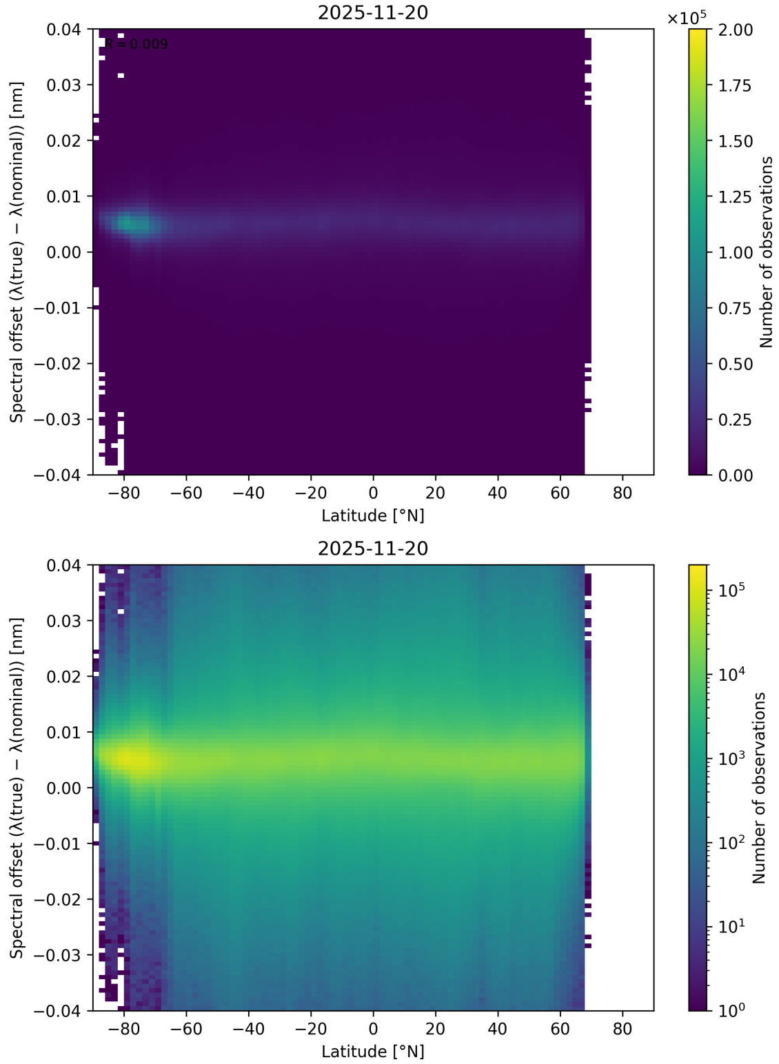
Figure 96: Scatter density plot of “Latitude” against “Spectral offset ( \lambda_{\text{true}} - \lambda_{\text{nominal}} )” for 2025-11-19 to 2025-11-21.
