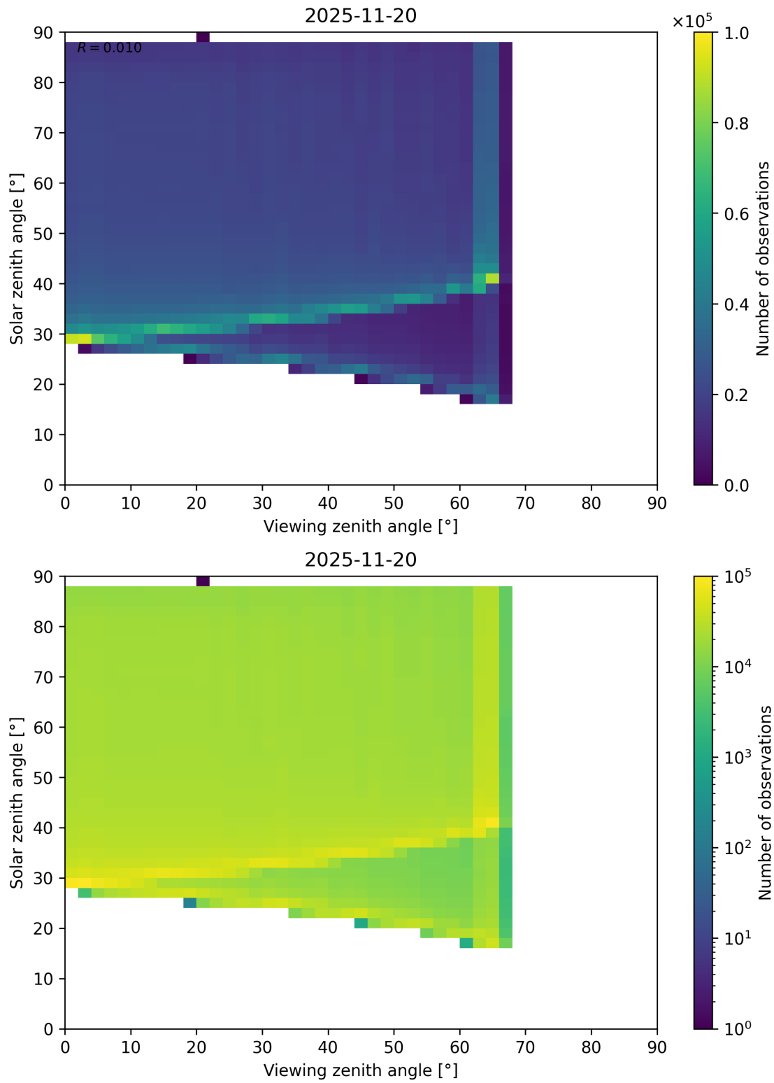
Figure 127: Scatter density plot of “Viewing zenith angle” against “Solar zenith angle” for 2025-11-19 to 2025-11-21.
