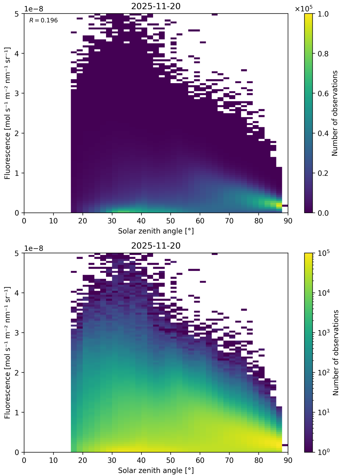
Figure 112: Scatter density plot of “Solar zenith angle” against “Fluorescence” for 2025-11-19 to 2025-11-21.
