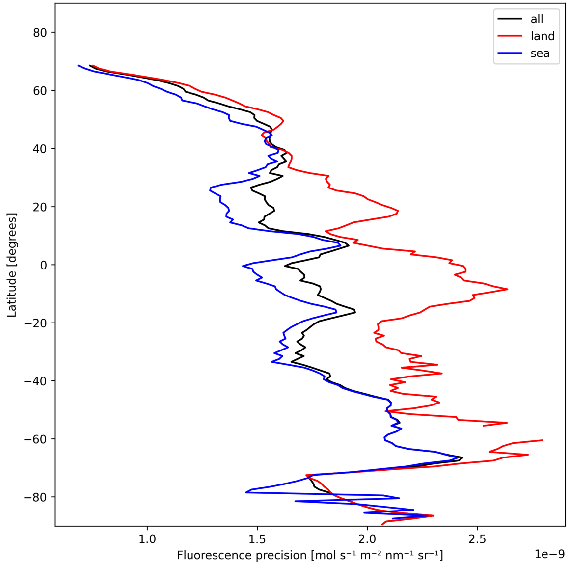
Figure 24: Zonal average of "Fluorescence precision" for 2025-11-19 to 2025-11-21.
