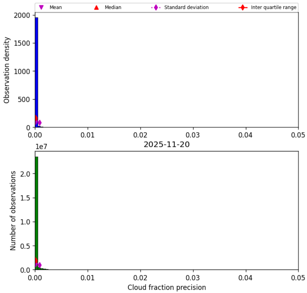
Figure 33: Histogram of “Cloud fraction precision” for 2025-11-19 to 2025-11-21
