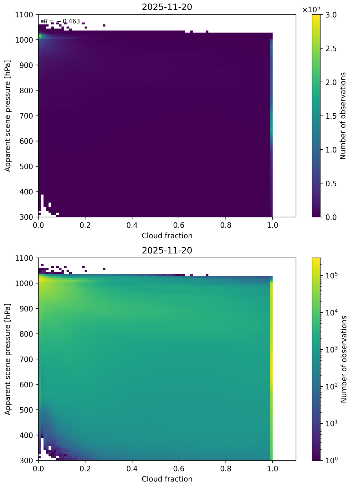
Figure 70: Scatter density plot of “Cloud fraction” against “Apparent scene pressure” for 2025-11-19 to 2025-11-21.
