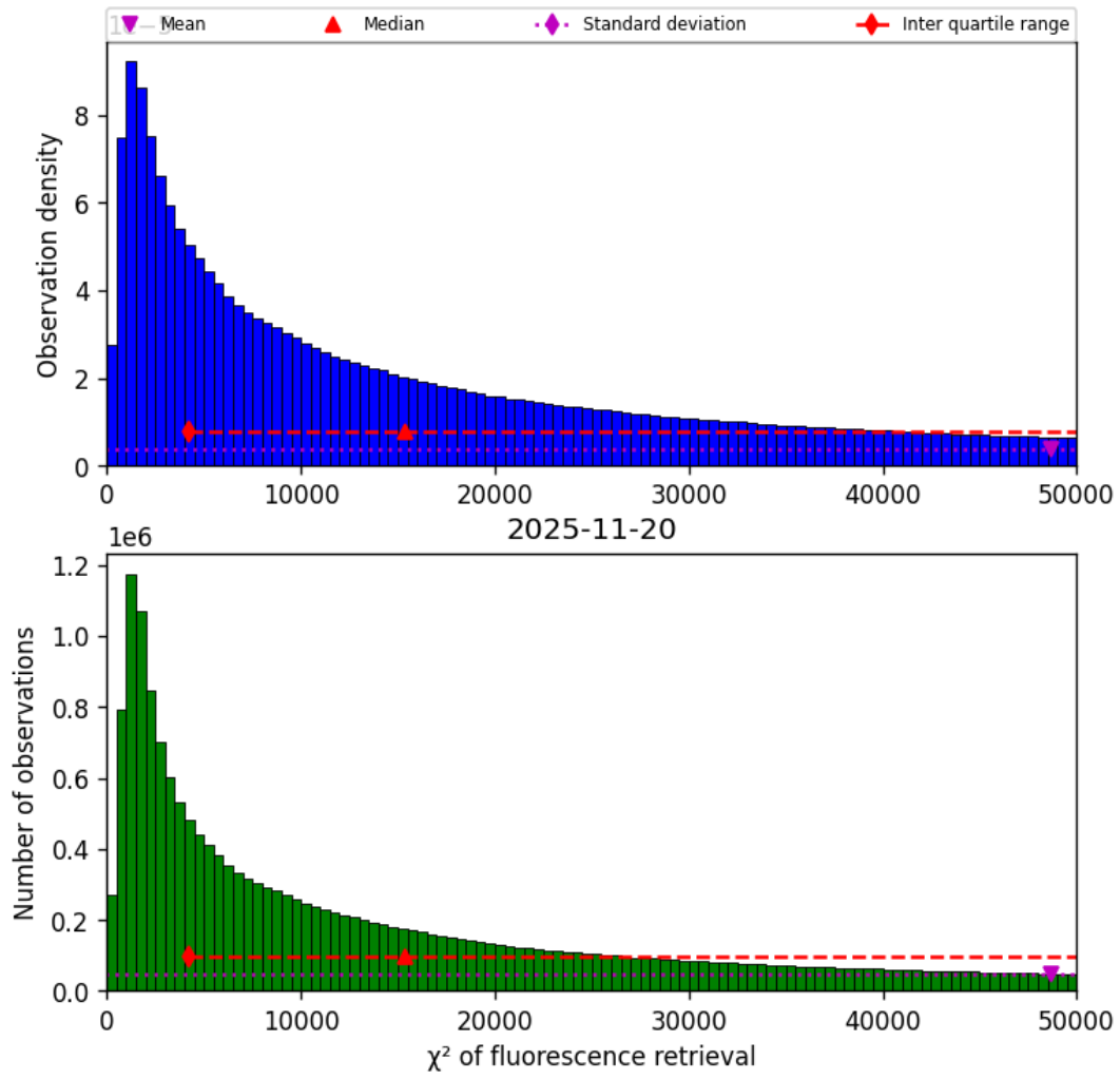
Figure 42: Histogram of “ \chi^2 of fluorescence retrieval” for 2025-11-19 to 2025-11-21
