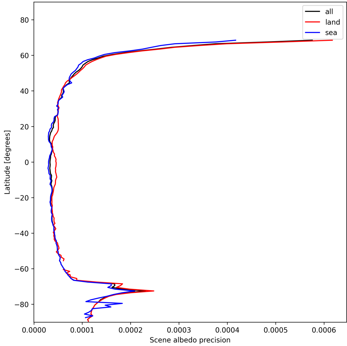
Figure 18: Zonal average of “Scene albedo precision” for 2025-11-19 to 2025-11-21.
