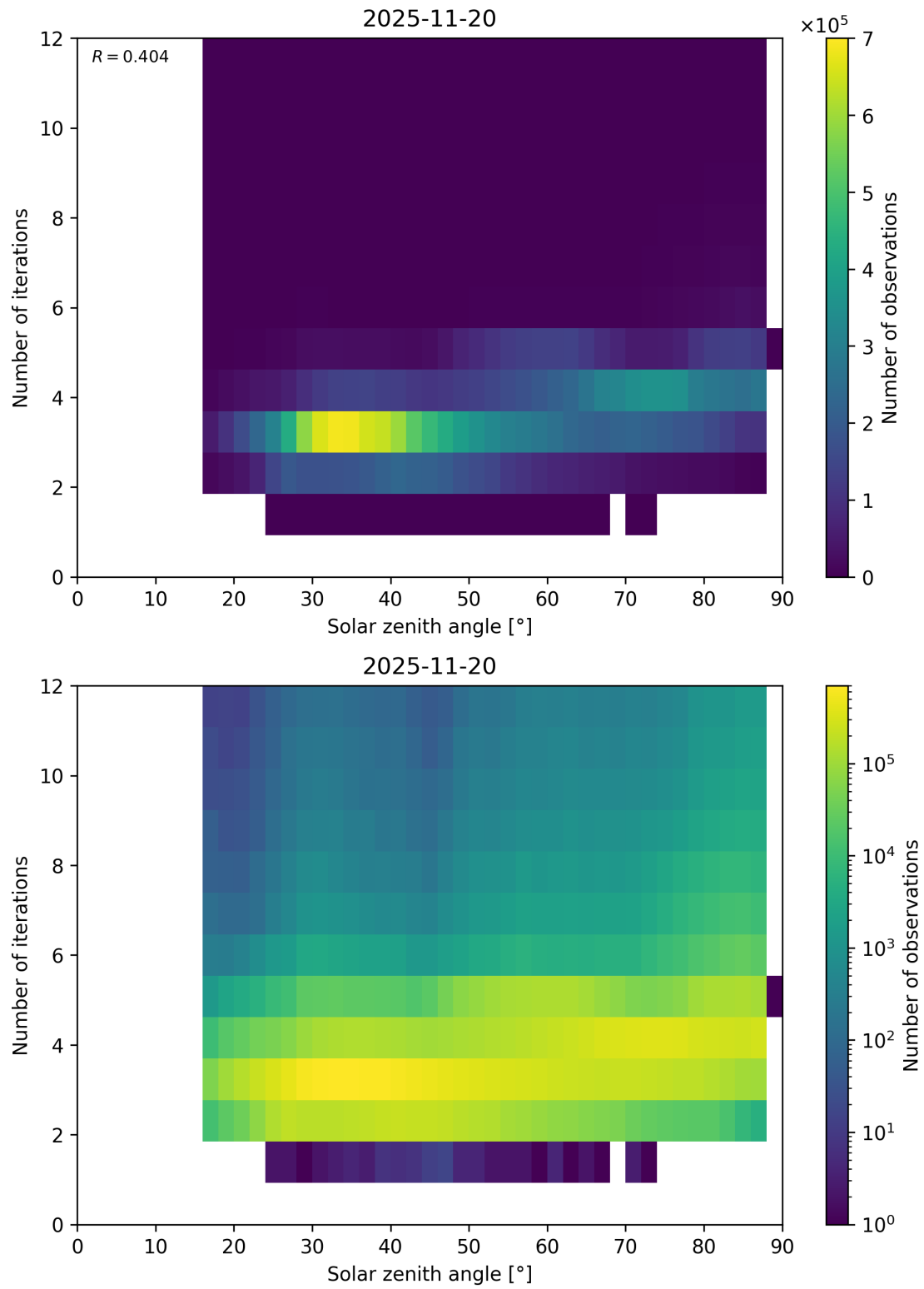
Figure 114: Scatter density plot of “Solar zenith angle” against “Number of iterations” for 2025-11-19 to 2025-11-21.
