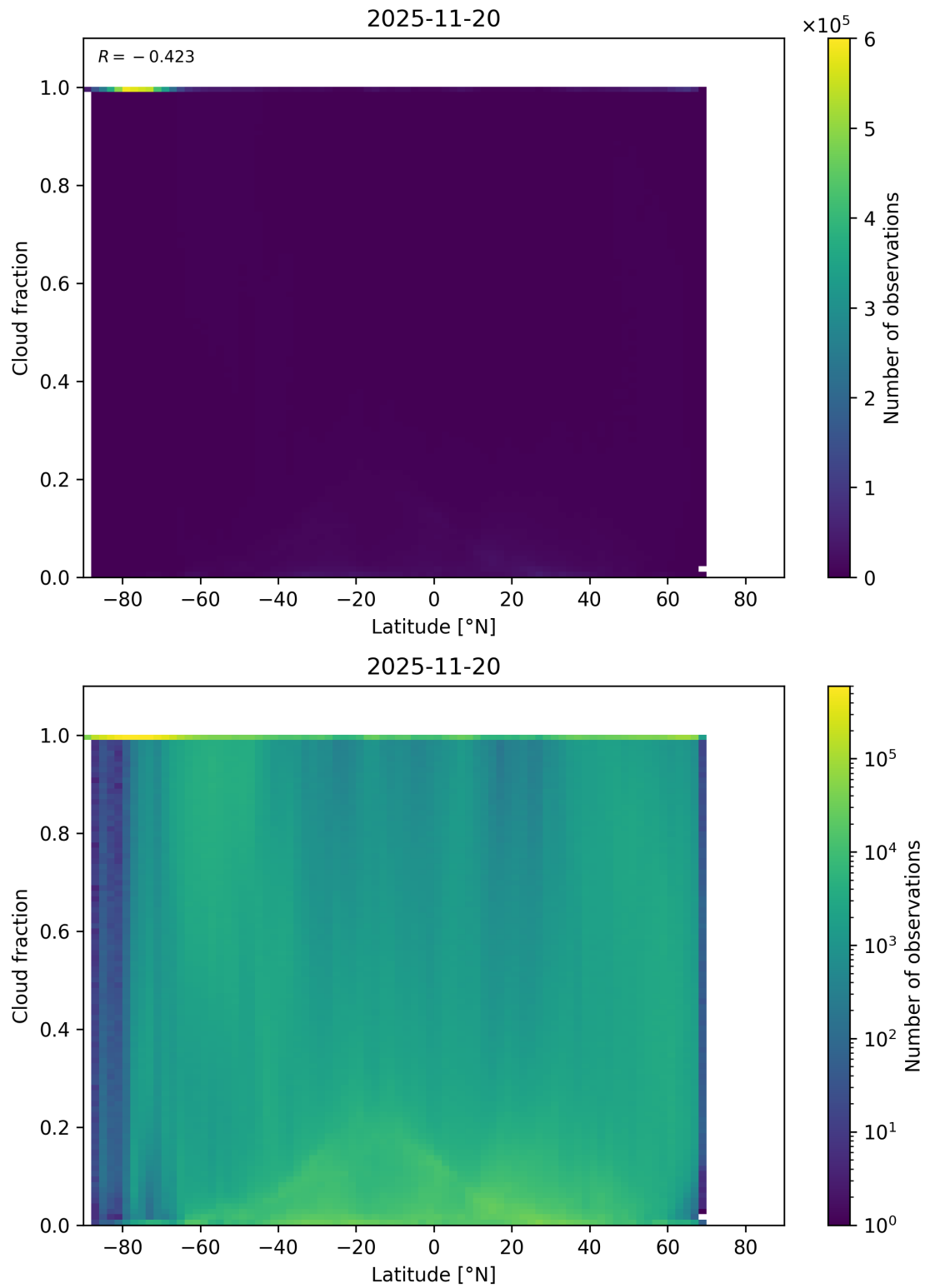
Figure 90: Scatter density plot of “Latitude” against “Cloud fraction” for 2025-11-19 to 2025-11-21.
