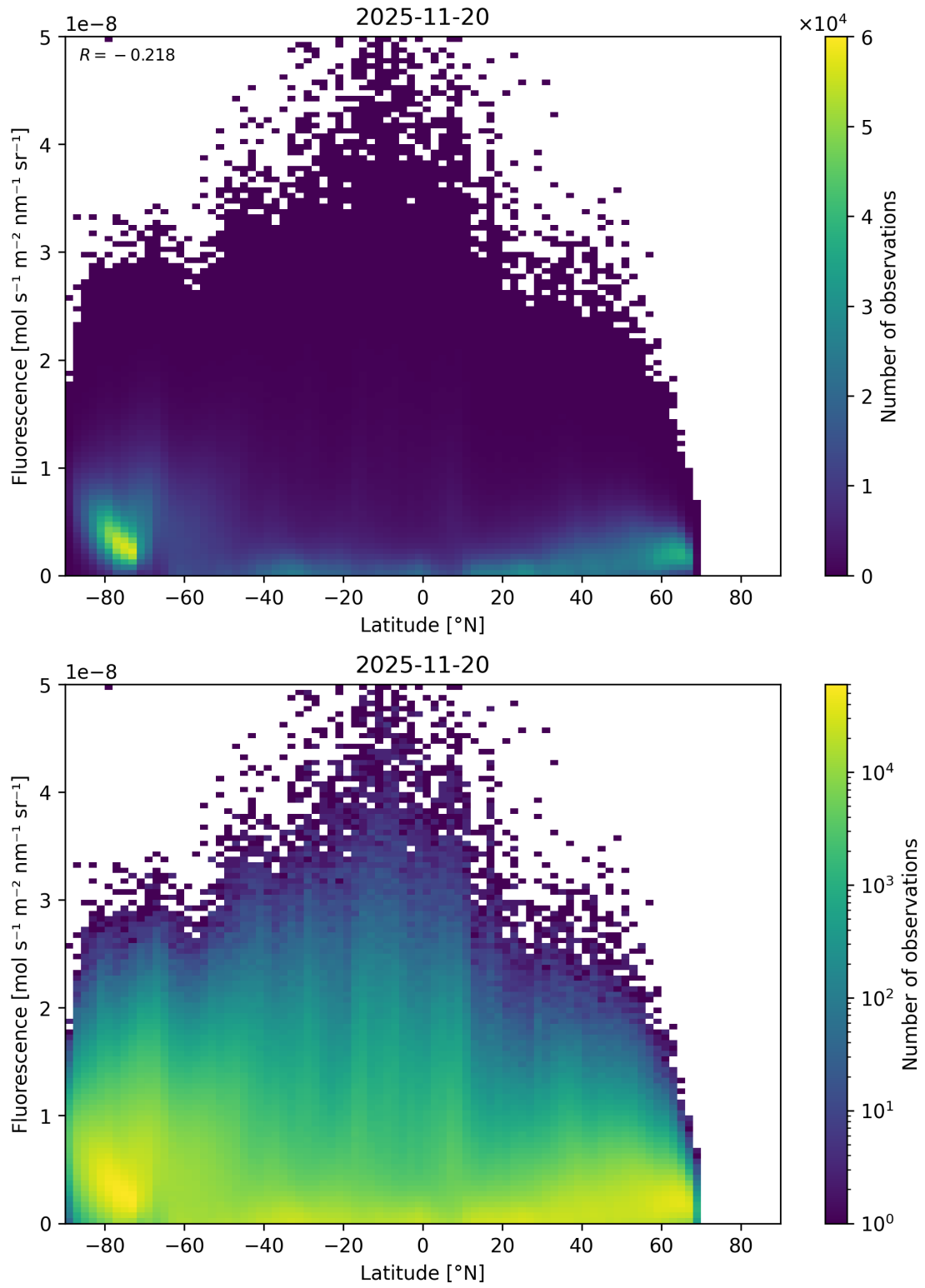
Figure 92: Scatter density plot of “Latitude” against “Fluorescence” for 2025-11-19 to 2025-11-21.
