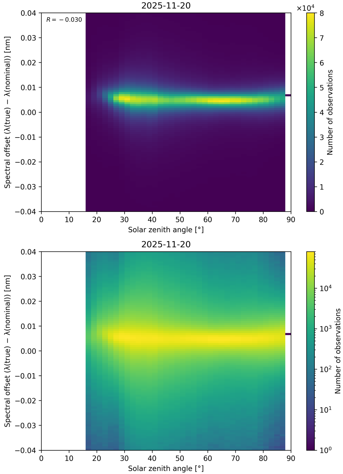
Figure 117: Scatter density plot of “Solar zenith angle” against “Spectral offset ( \lambda_{\text{true}} - \lambda_{\text{nominal}} )” for 2025-11-19 to 2025-11-21.
