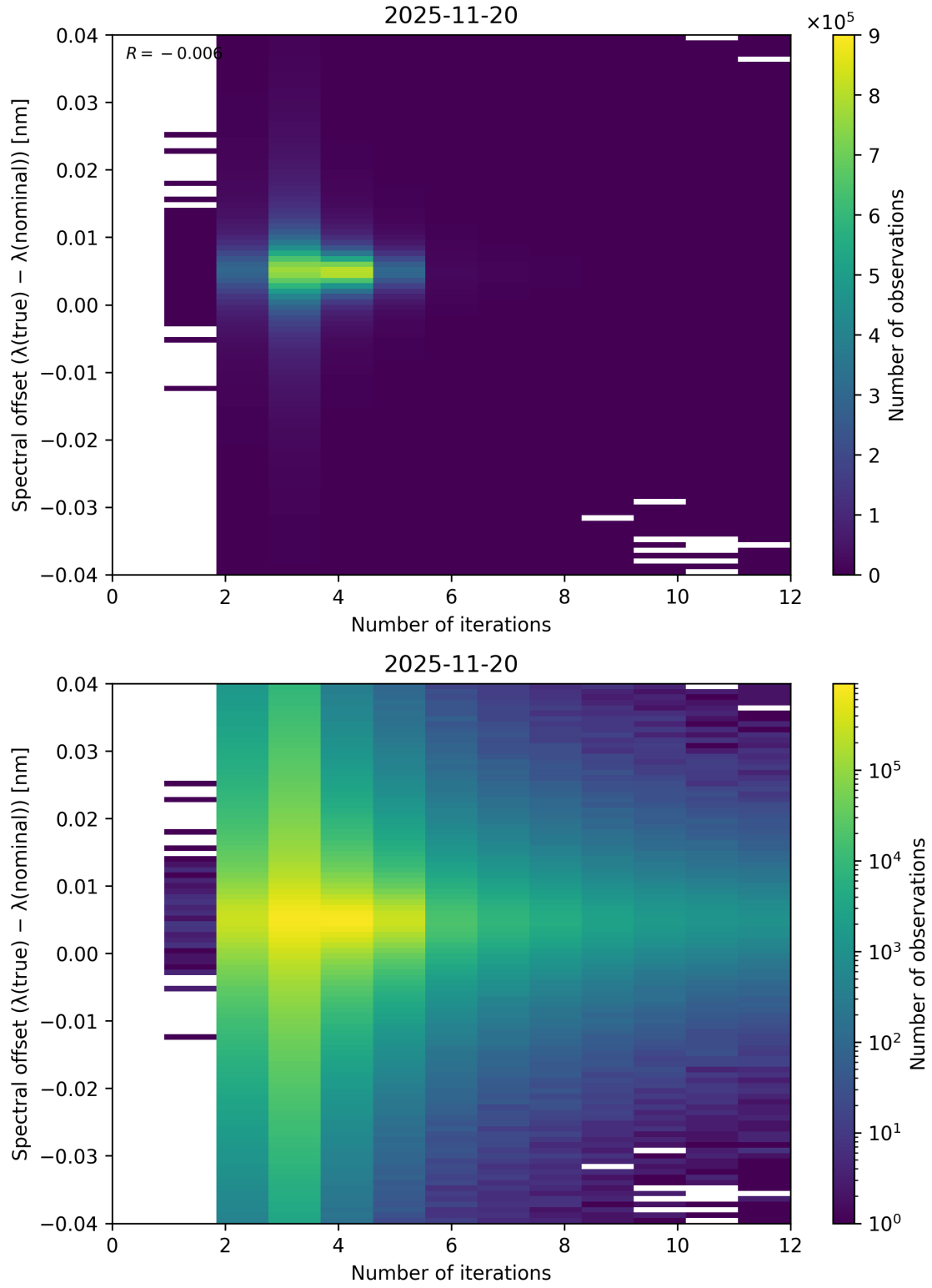
Figure 100: Scatter density plot of “Number of iterations” against “Spectral offset ( \lambda_{\text{true}} - \lambda_{\text{nominal}} )” for 2025-11-19 to 2025-11-21.
