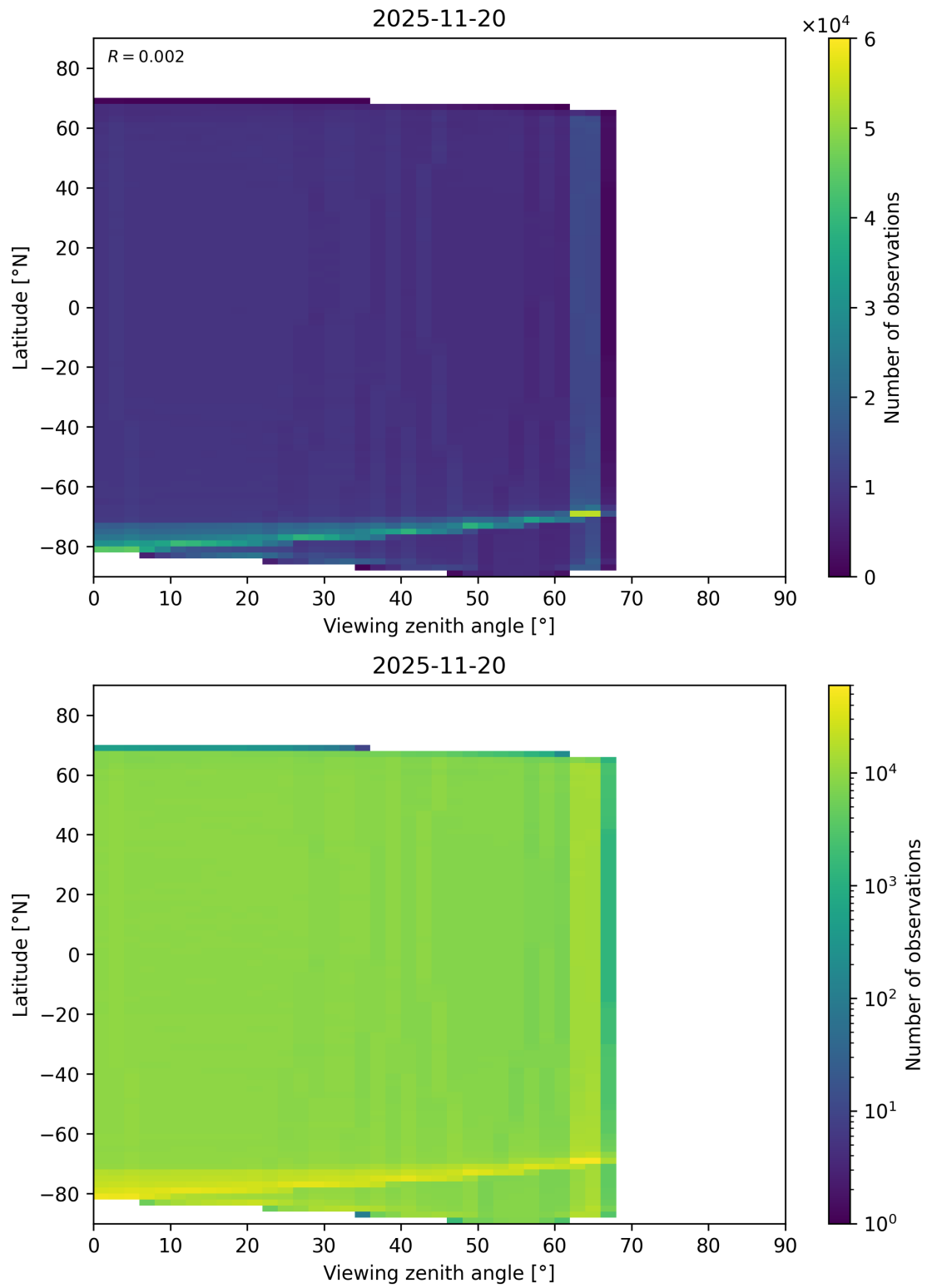
Figure 123: Scatter density plot of “Viewing zenith angle” against “Latitude” for 2025-11-19 to 2025-11-21.
