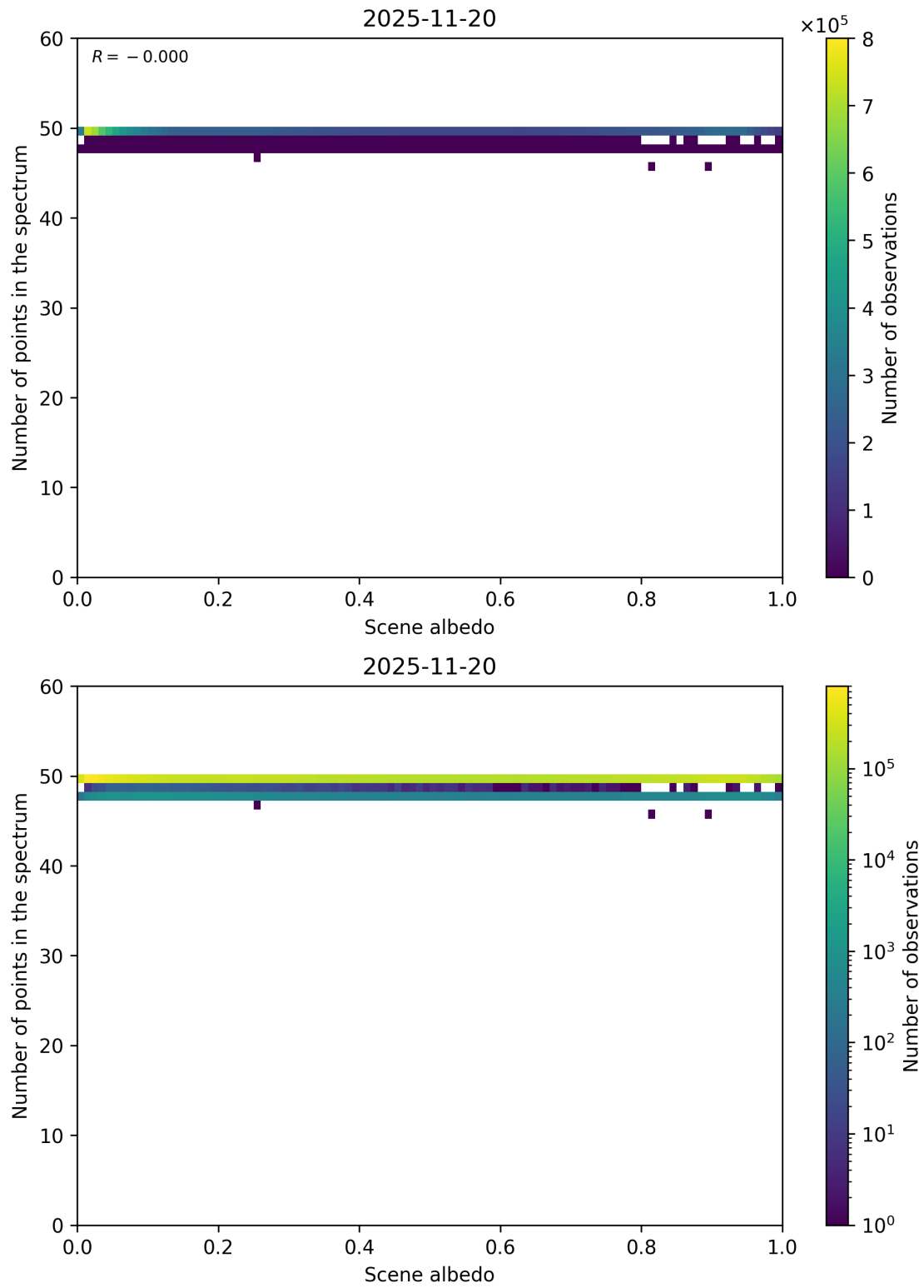
Figure 106: Scatter density plot of “Scene albedo” against “Number of points in the spectrum” for 2025-11-19 to 2025-11-21.
