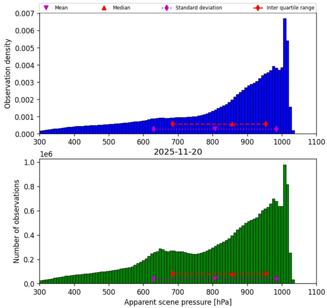
Figure 36: Histogram of “Apparent scene pressure” for 2025-11-19 to 2025-11-21
