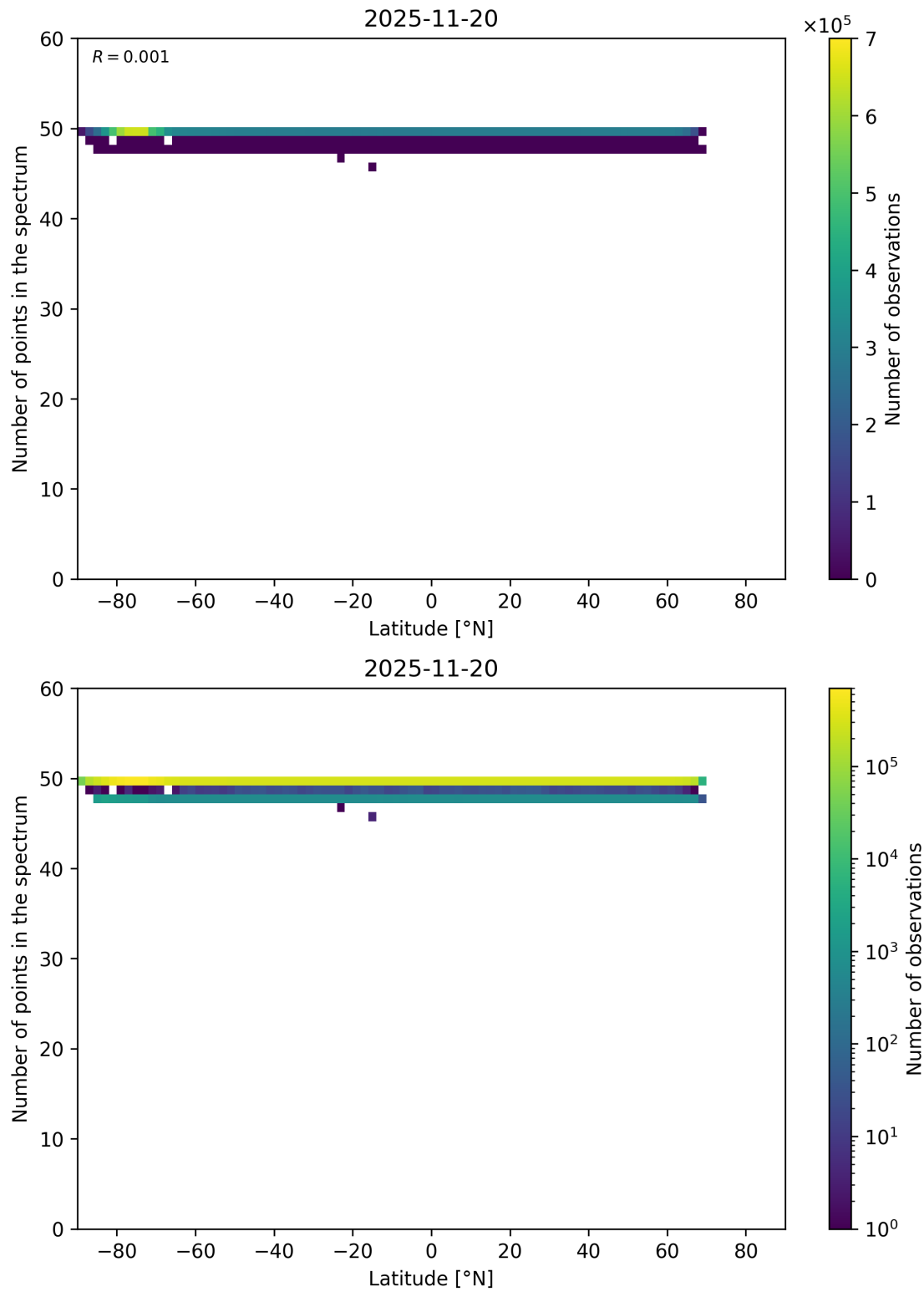
Figure 94: Scatter density plot of “Latitude” against “Number of points in the spectrum” for 2025-11-19 to 2025-11-21.
