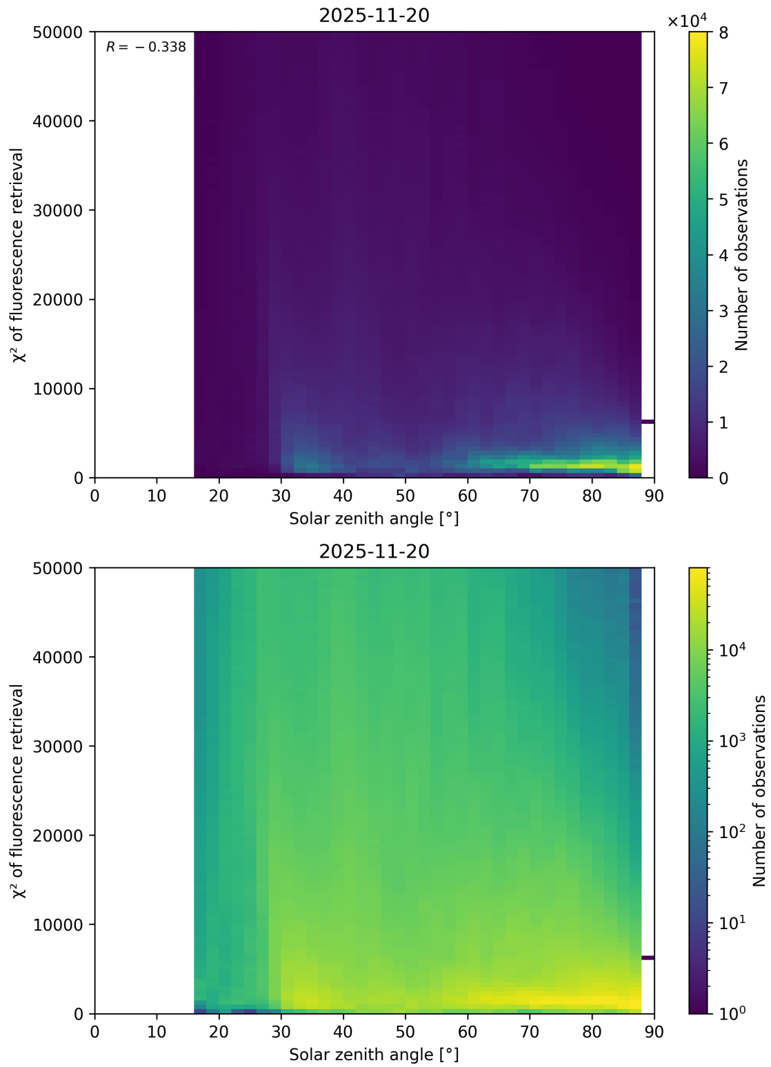
Figure 109: Scatter density plot of “Solar zenith angle” against “ \chi^2 of fluorescence retrieval” for 2025-11-19 to 2025-11-21.
