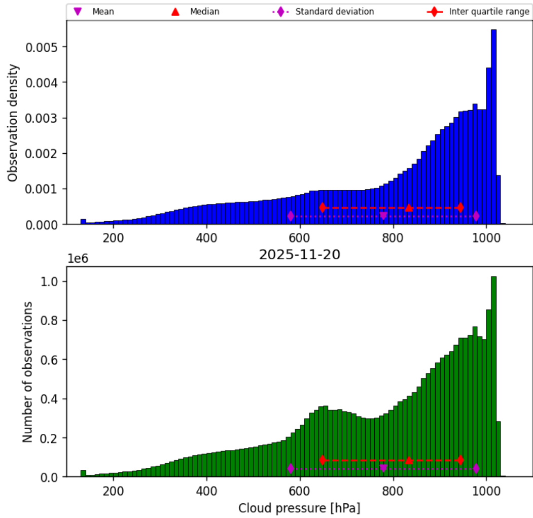
Figure 30: Histogram of “Cloud pressure” for 2025-11-19 to 2025-11-21
