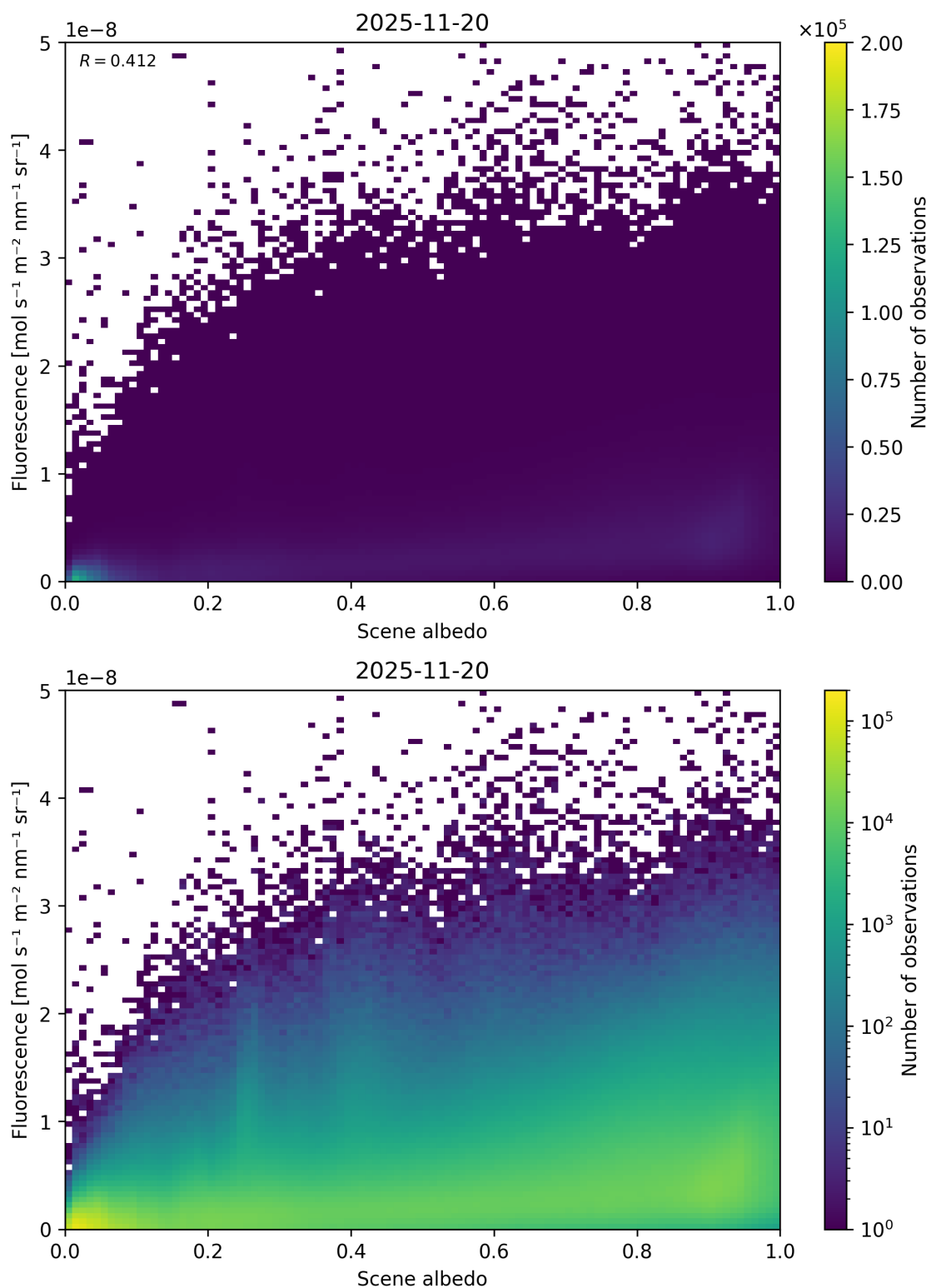
Figure 104: Scatter density plot of “Scene albedo” against “Fluorescence” for 2025-11-19 to 2025-11-21.
