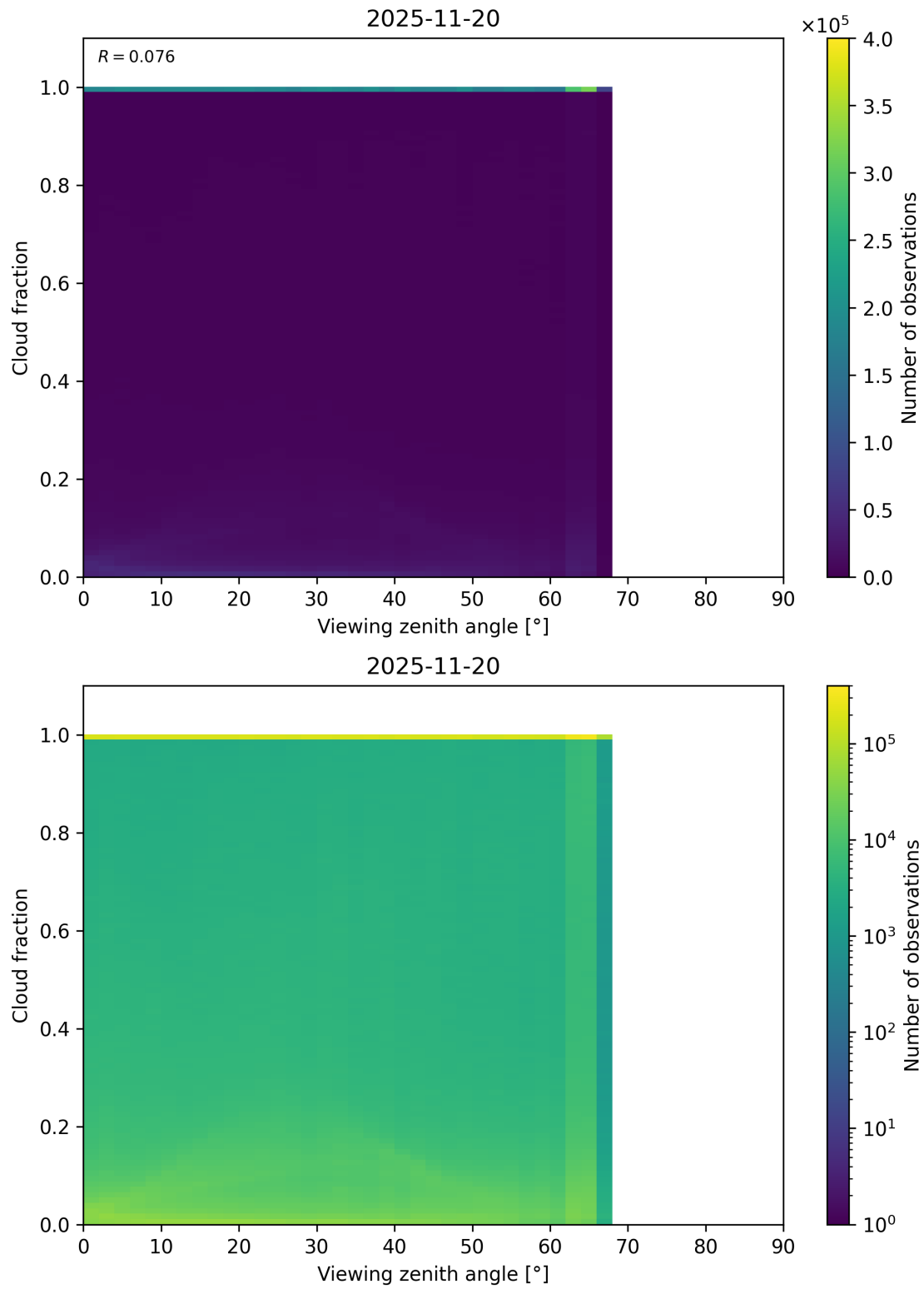
Figure 120: Scatter density plot of “Viewing zenith angle” against “Cloud fraction” for 2025-11-19 to 2025-11-21.
