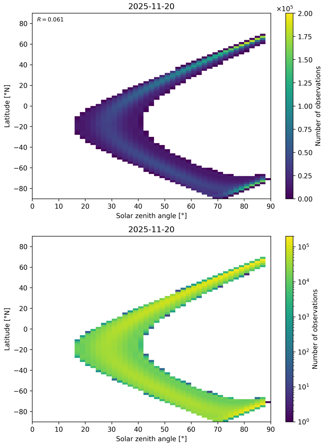
Figure 113: Scatter density plot of “Solar zenith angle” against “Latitude” for 2025-11-19 to 2025-11-21.
