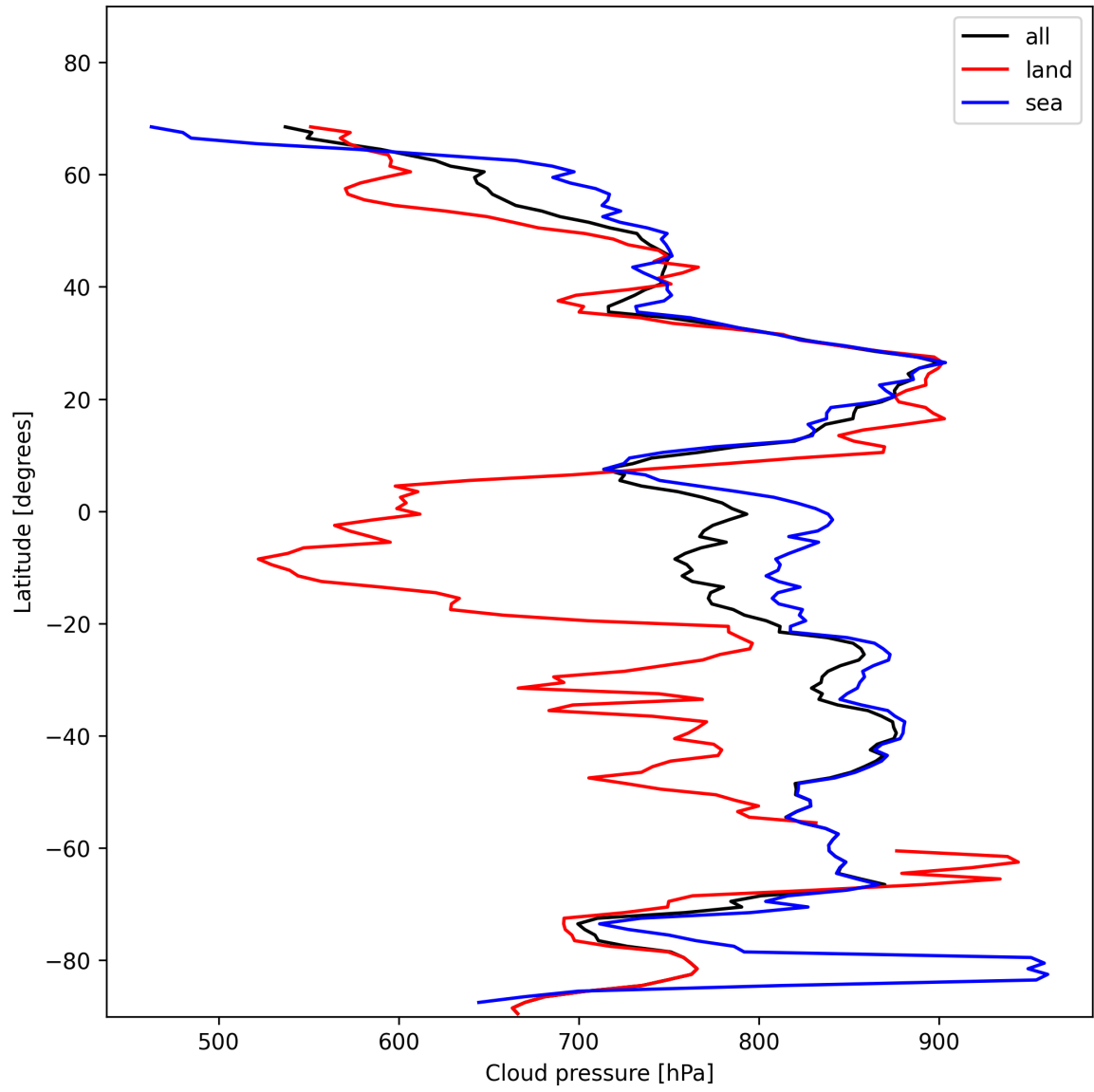
Figure 13: Zonal average of “Cloud pressure” for 2025-11-19 to 2025-11-21.
