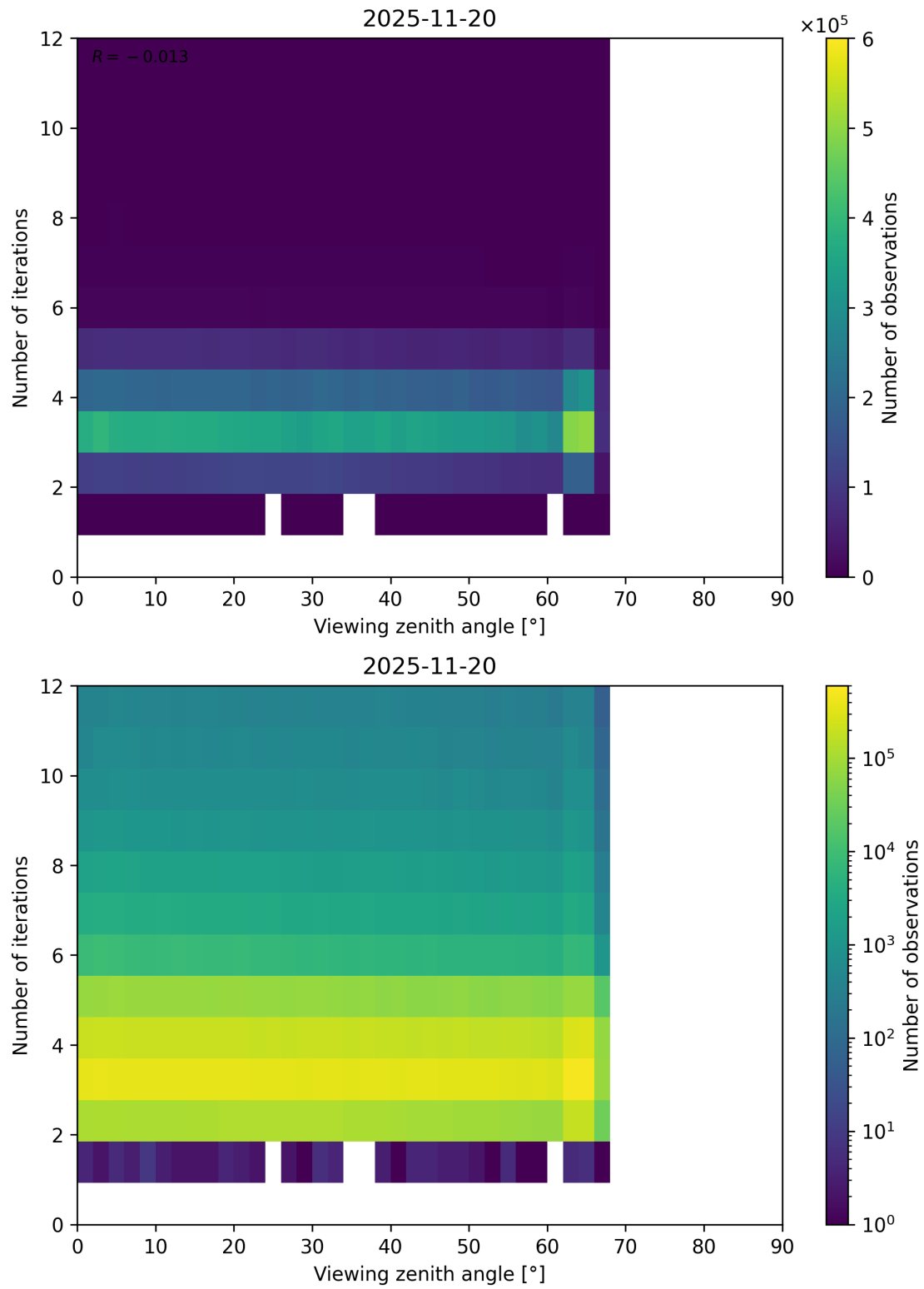
Figure 124: Scatter density plot of “Viewing zenith angle” against “Number of iterations” for 2025-11-19 to 2025-11-21.
