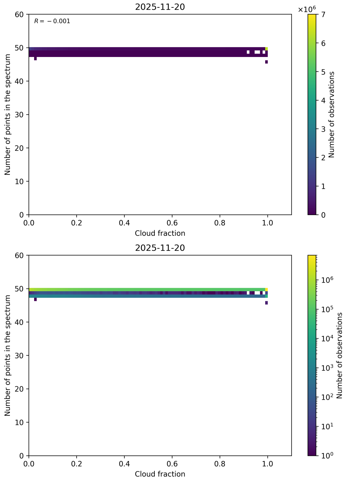
Figure 74: Scatter density plot of “Cloud fraction” against “Number of points in the spectrum” for 2025-11-19 to 2025-11-21.
