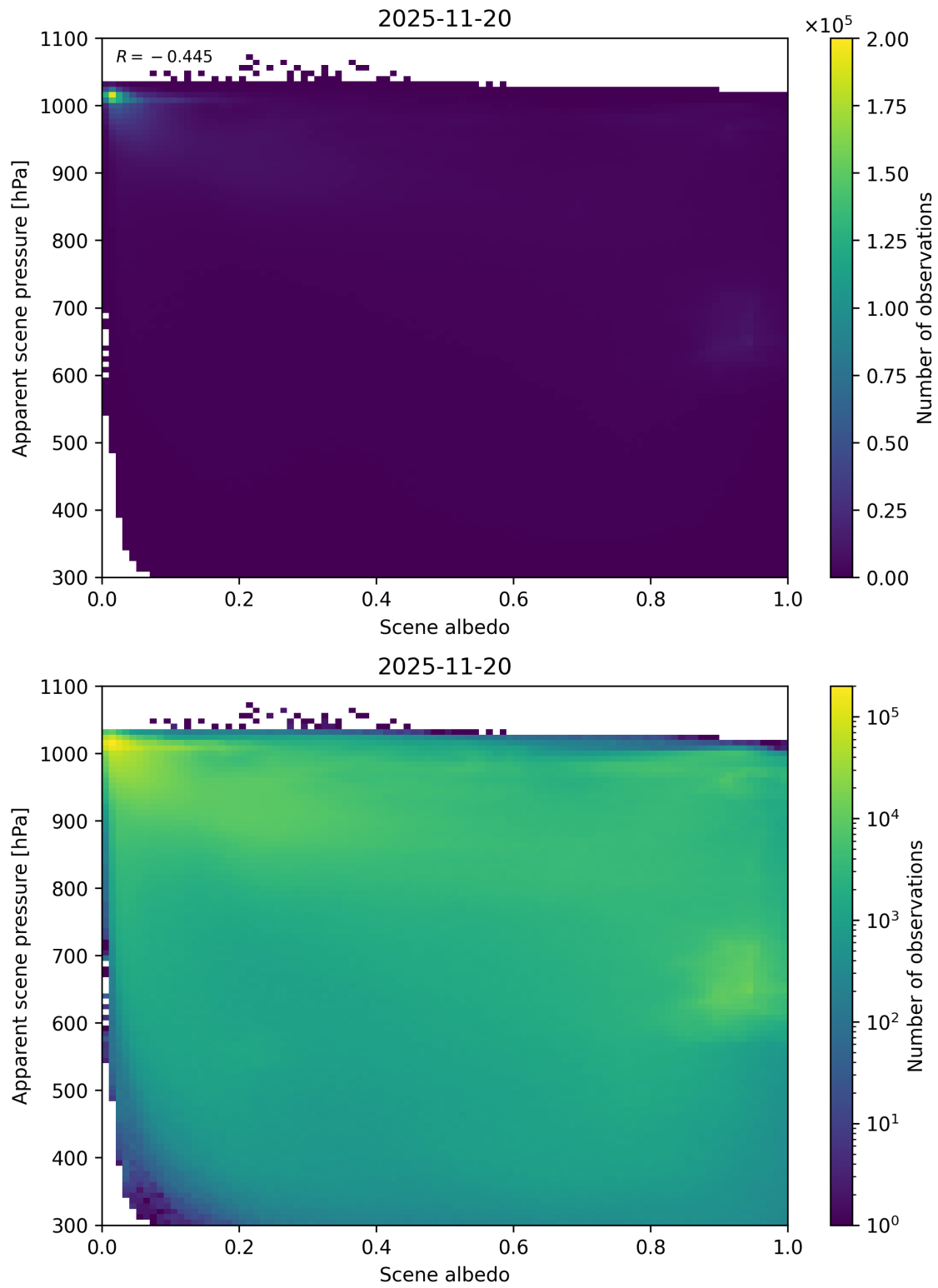
Figure 102: Scatter density plot of “Scene albedo” against “Apparent scene pressure” for 2025-11-19 to 2025-11-21.
