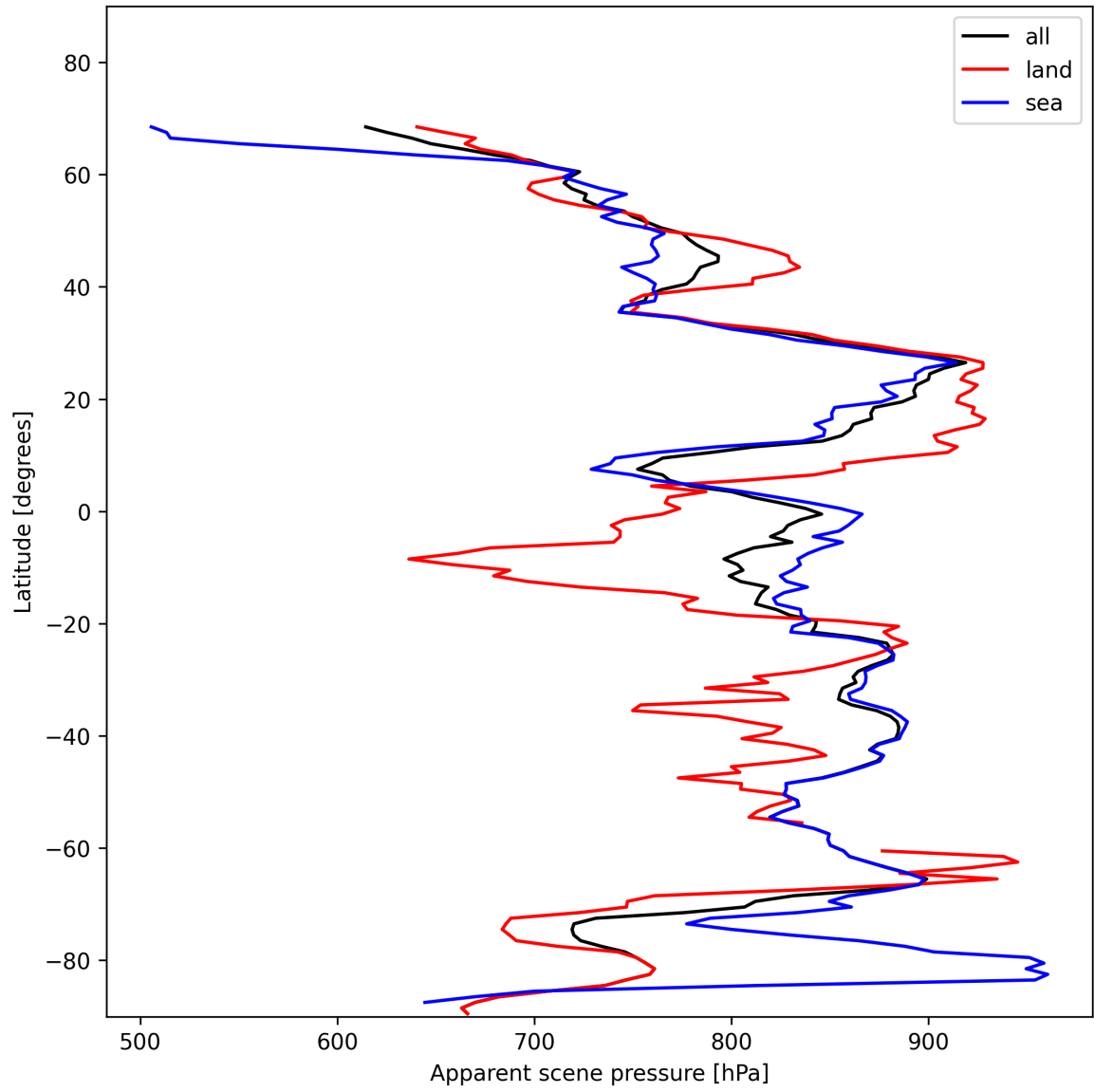
Figure 19: Zonal average of “Apparent scene pressure” for 2025-11-19 to 2025-11-21.
