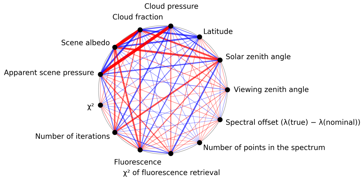
Figure 1: Map of correlation graph for 2025-11-19 to 2025-11-21.
