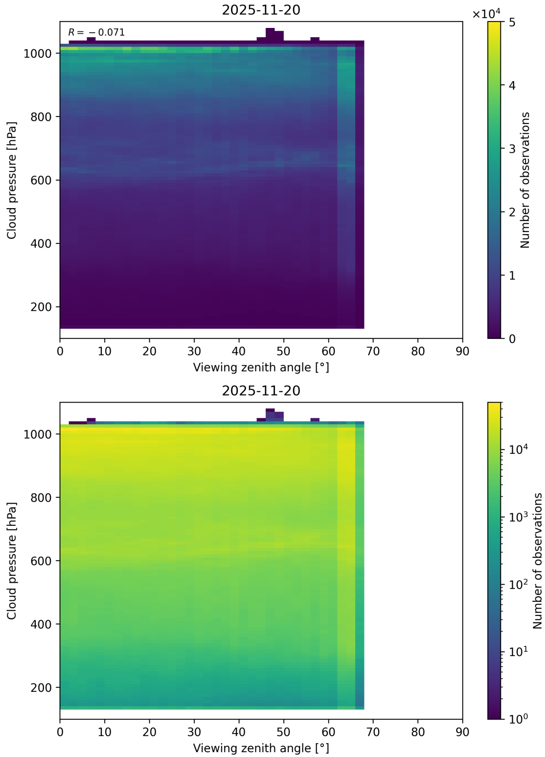
Figure 121: Scatter density plot of “Viewing zenith angle” against “Cloud pressure” for 2025-11-19 to 2025-11-21.
