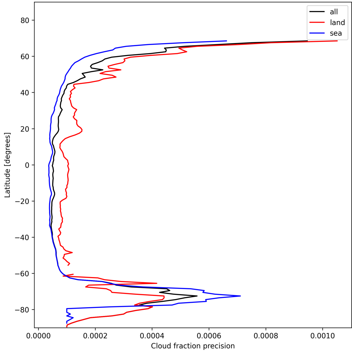
Figure 16: Zonal average of “Cloud fraction precision” for 2025-11-19 to 2025-11-21.
