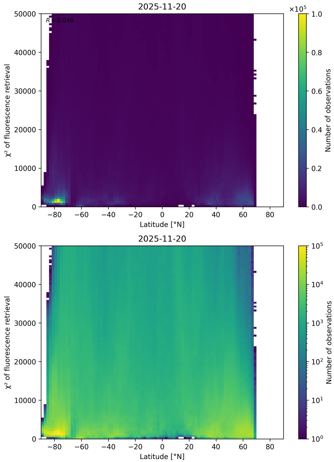
Figure 89: Scatter density plot of “Latitude” against “ \chi^2 of fluorescence retrieval” for 2025-11-19 to 2025-11-21.
