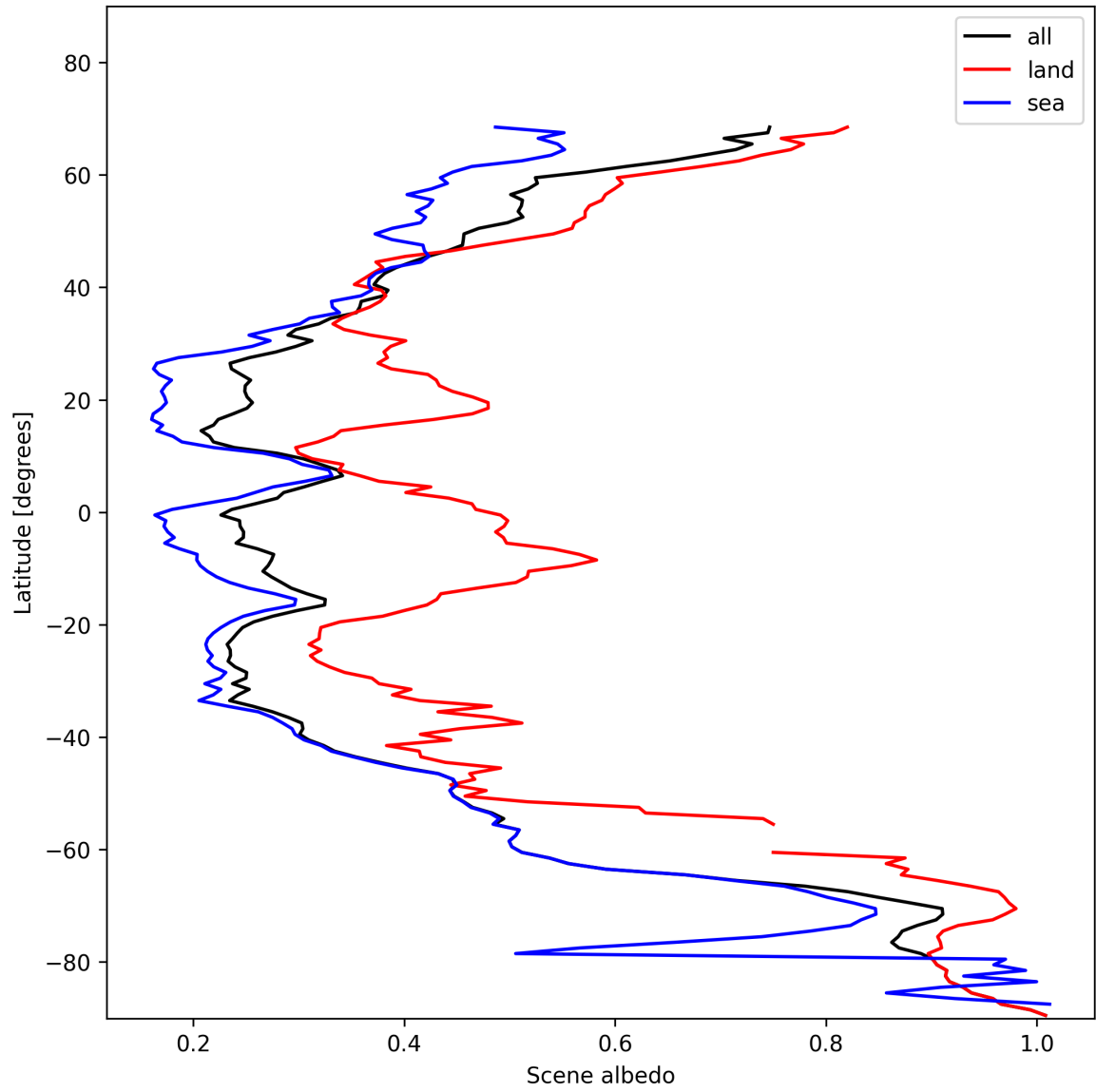
Figure 17: Zonal average of “Scene albedo” for 2025-11-19 to 2025-11-21.
