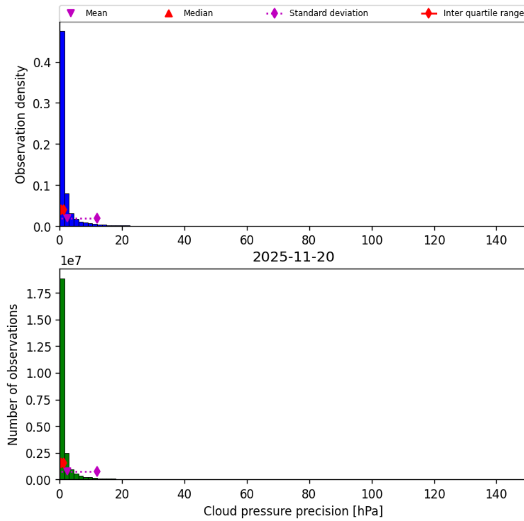
Figure 31: Histogram of “Cloud pressure precision” for 2025-11-19 to 2025-11-21
