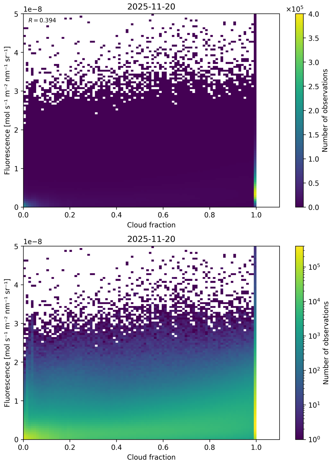
Figure 72: Scatter density plot of “Cloud fraction” against “Fluorescence” for 2025-11-19 to 2025-11-21.
