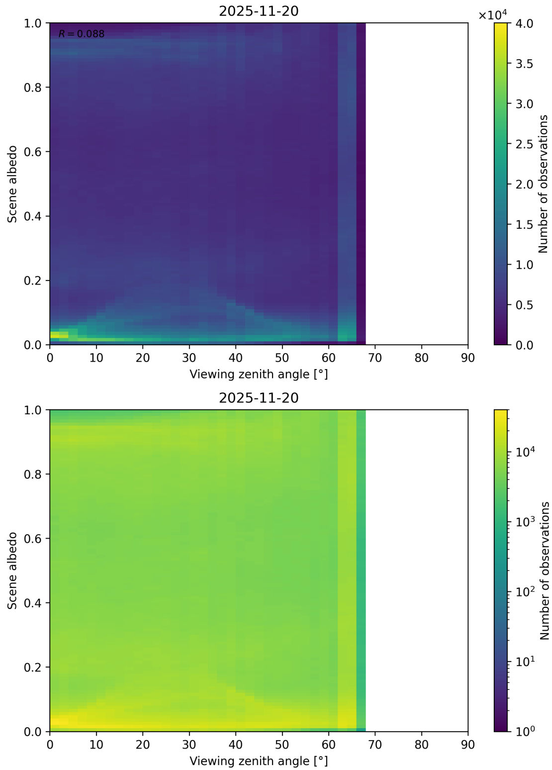
Figure 126: Scatter density plot of “Viewing zenith angle” against “Scene albedo” for 2025-11-19 to 2025-11-21.
