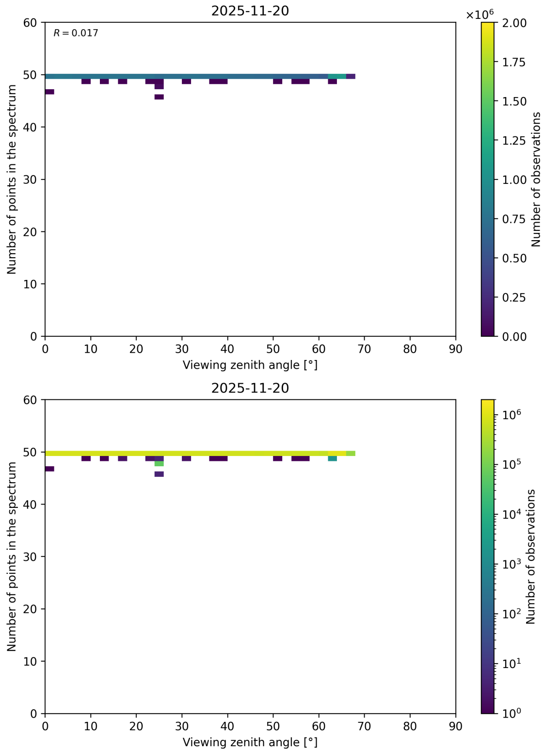
Figure 125: Scatter density plot of “Viewing zenith angle” against “Number of points in the spectrum” for 2025-11-19 to 2025-11-21.
