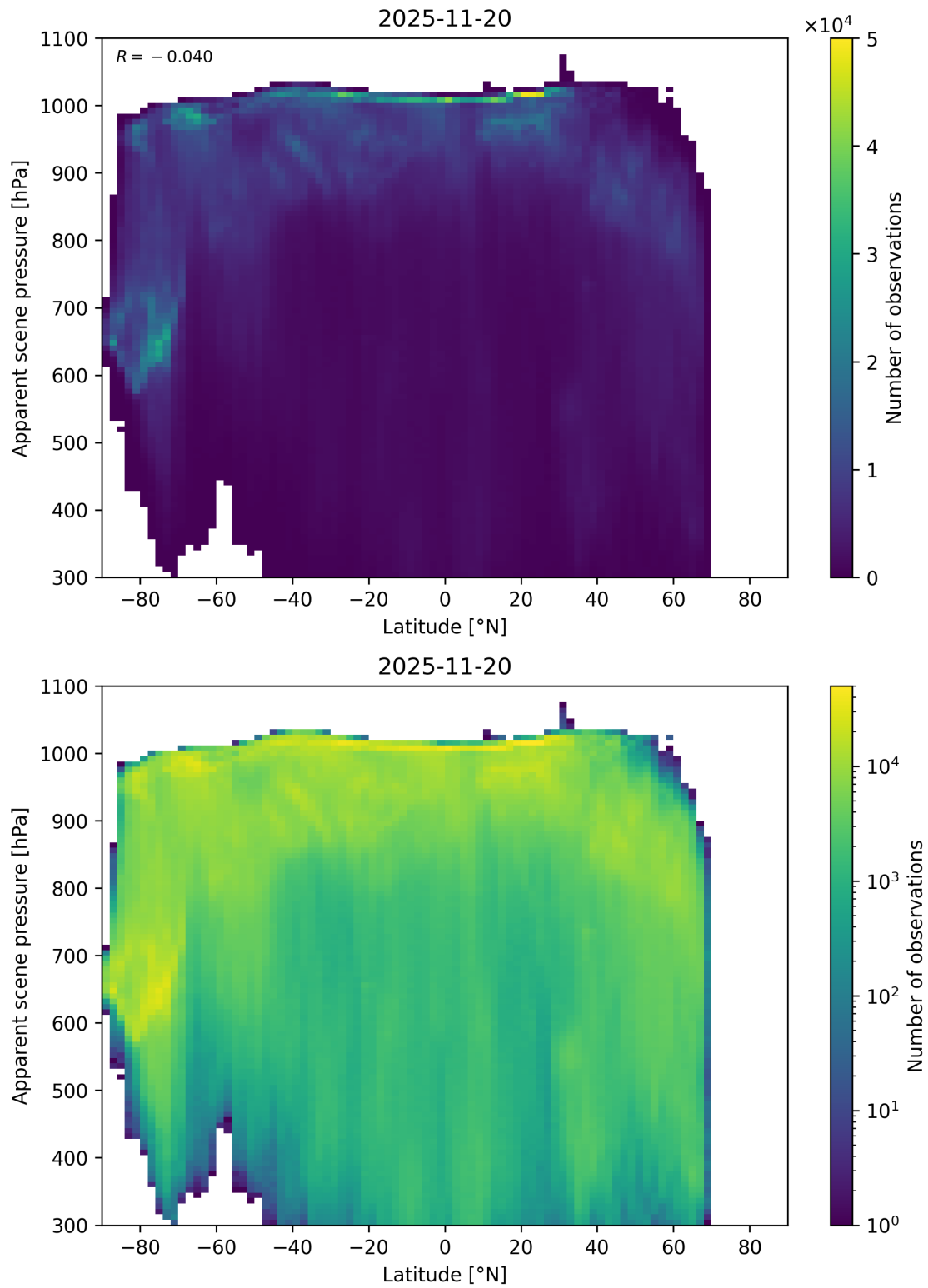
Figure 88: Scatter density plot of “Latitude” against “Apparent scene pressure” for 2025-11-19 to 2025-11-21.
