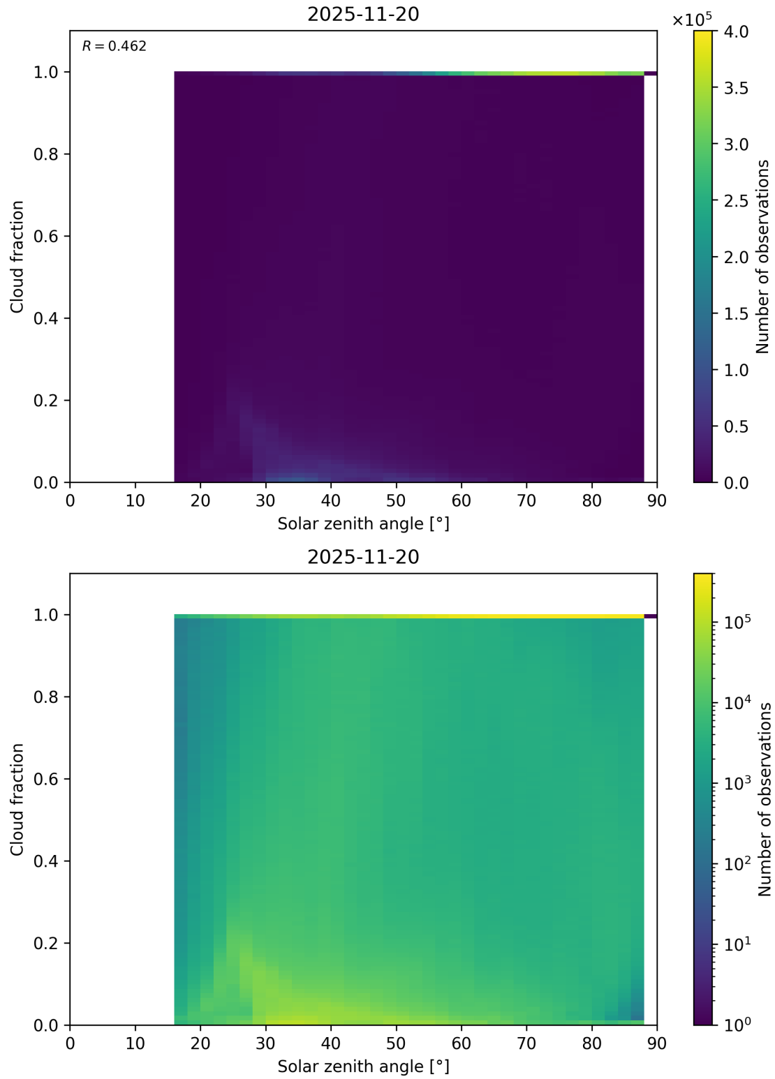
Figure 110: Scatter density plot of “Solar zenith angle” against “Cloud fraction” for 2025-11-19 to 2025-11-21.
