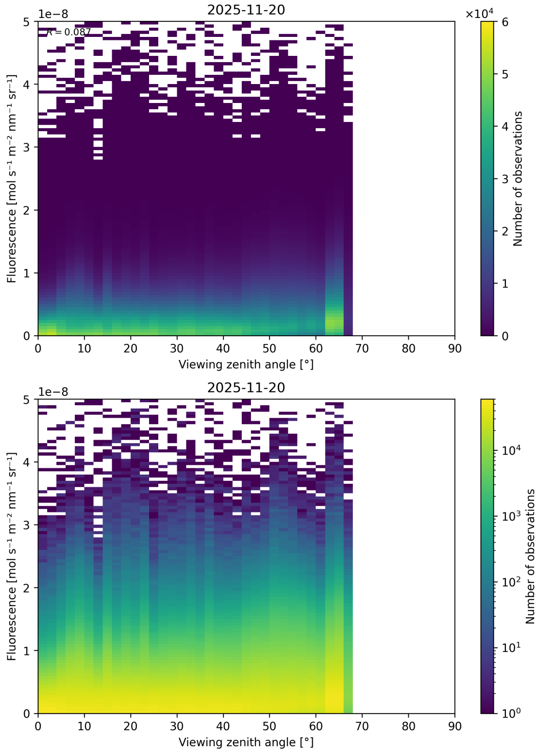
Figure 122: Scatter density plot of “Viewing zenith angle” against “Fluorescence” for 2025-11-19 to 2025-11-21.
