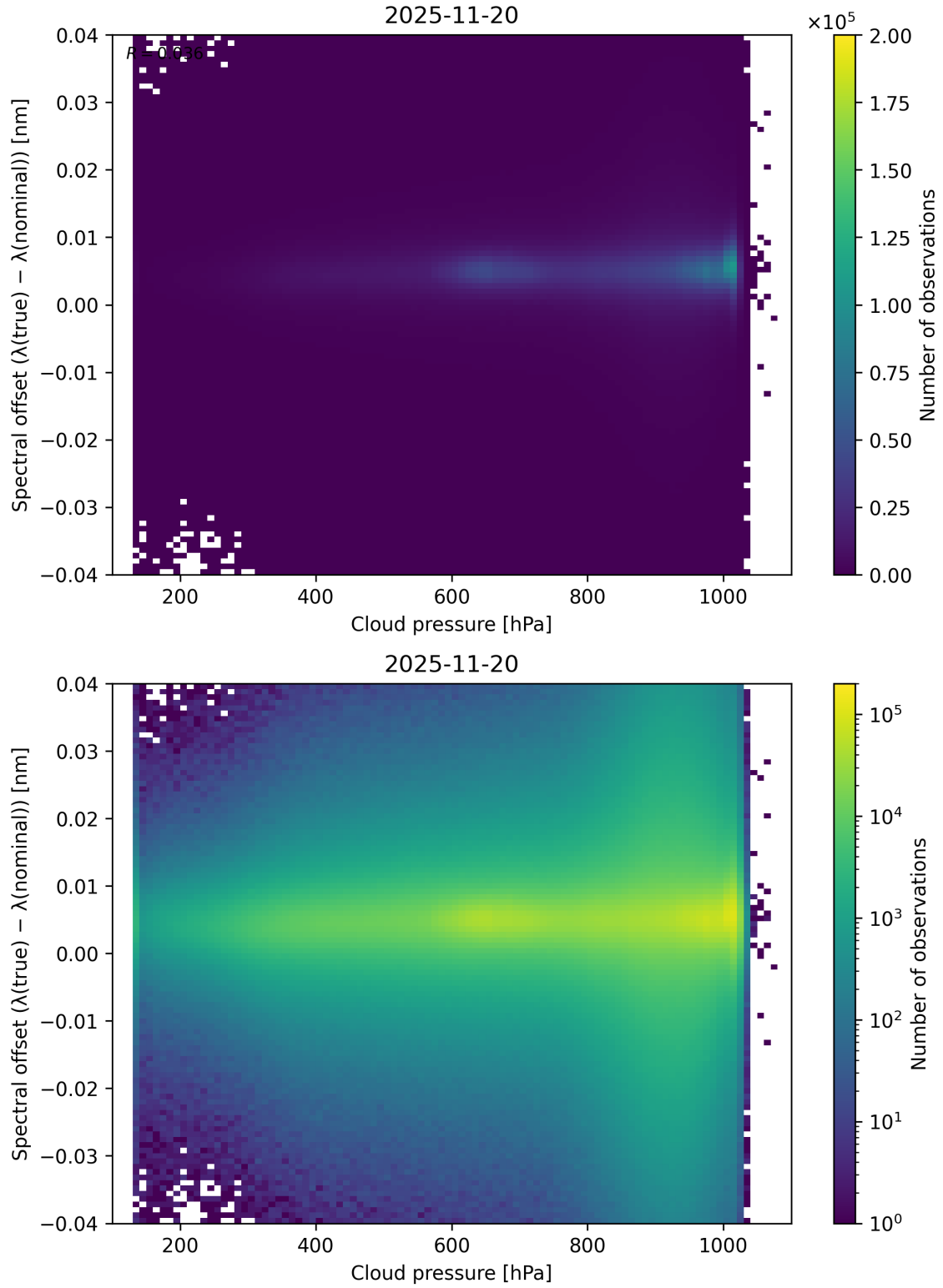
Figure 84: Scatter density plot of “Cloud pressure” against “Spectral offset ( \lambda_{\text{true}} - \lambda_{\text{nominal}} )” for 2025-11-19 to 2025-11-21.
