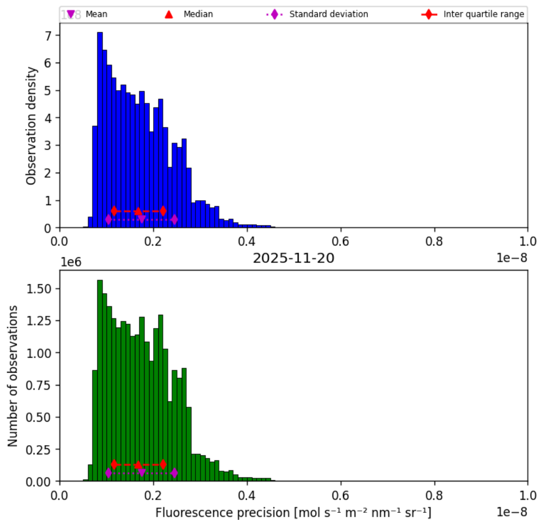
Figure 41: Histogram of “Fluorescence precision” for 2025-11-19 to 2025-11-21
