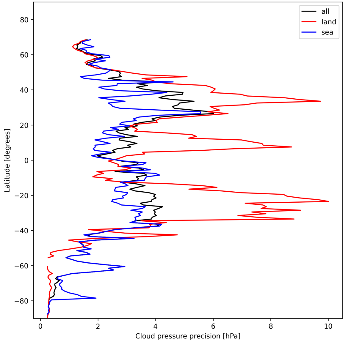
Figure 14: Zonal average of “Cloud pressure precision” for 2025-11-19 to 2025-11-21.
