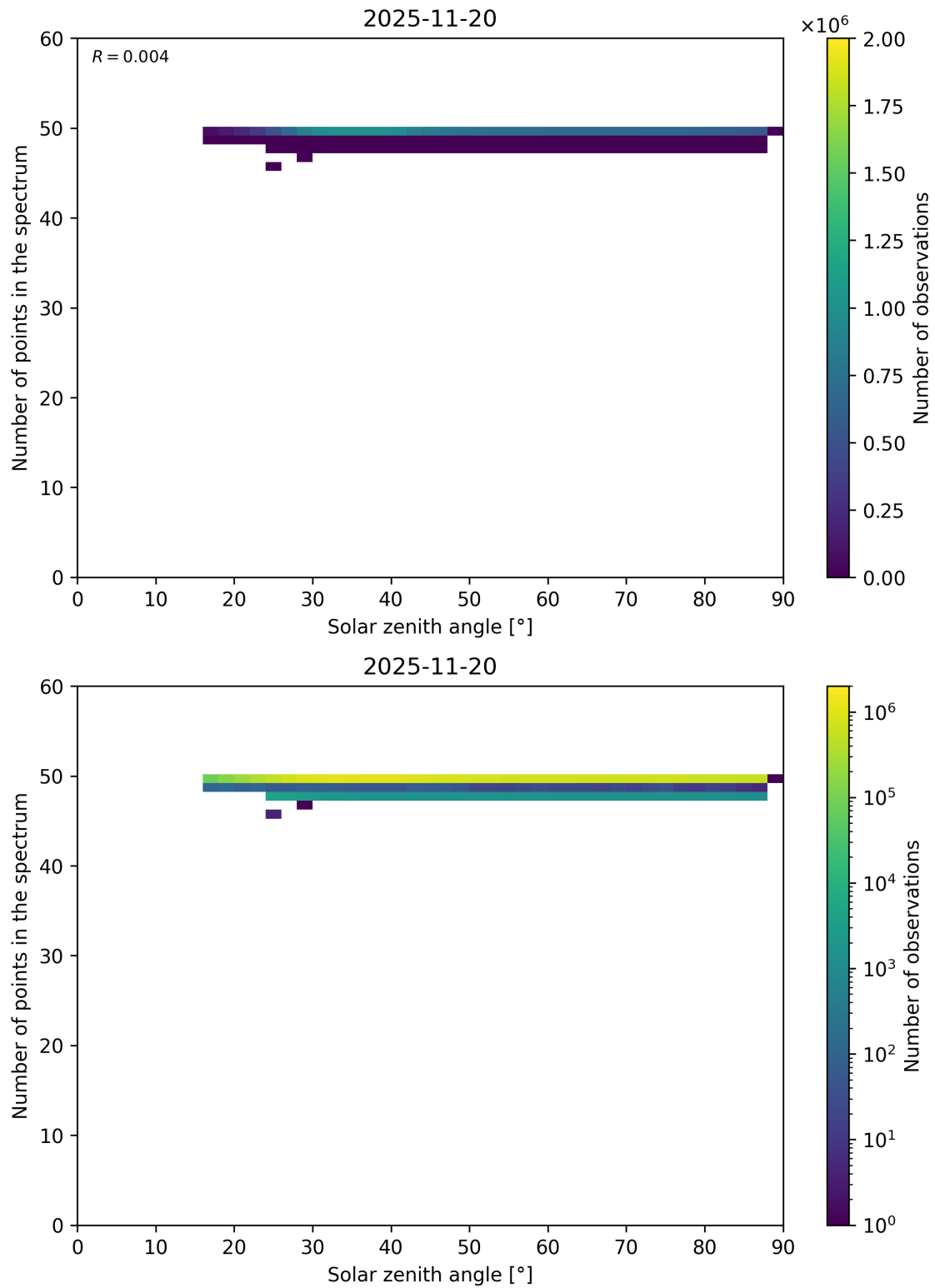
Figure 115: Scatter density plot of “Solar zenith angle” against “Number of points in the spectrum” for 2025-11-19 to 2025-11-21.
