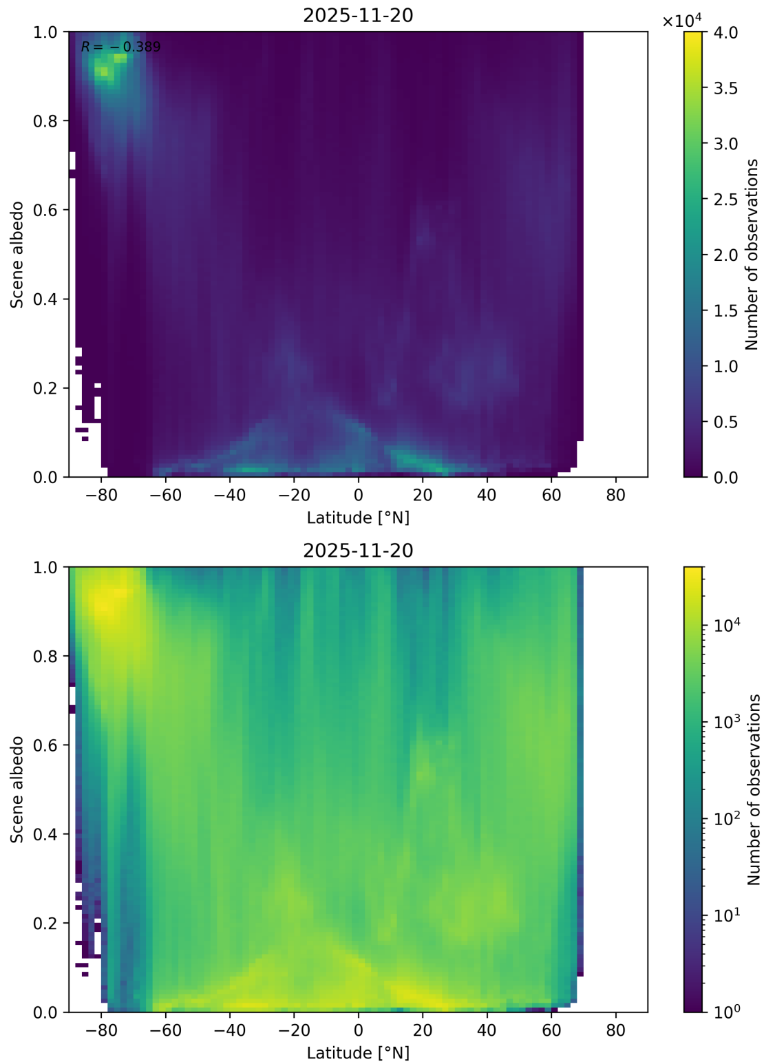
Figure 95: Scatter density plot of “Latitude” against “Scene albedo” for 2025-11-19 to 2025-11-21.
