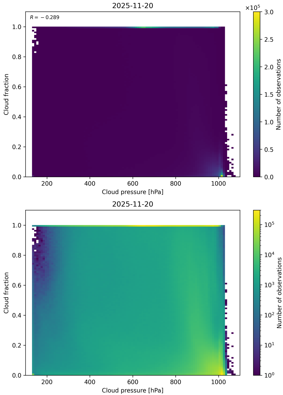
Figure 79: Scatter density plot of “Cloud pressure” against “Cloud fraction” for 2025-11-19 to 2025-11-21.
