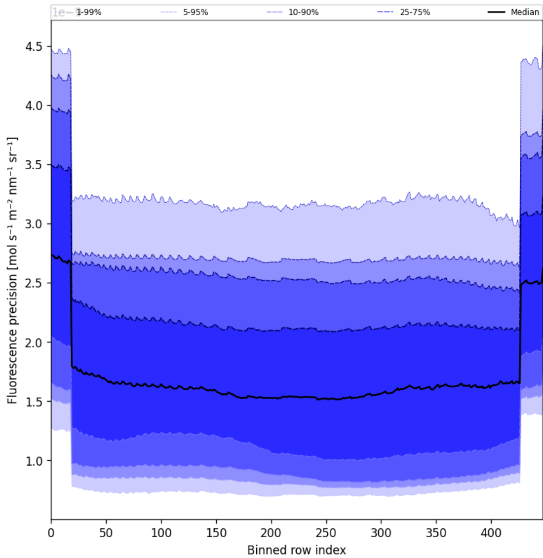
Figure 58: Along track statistics of “Fluorescence precision” for 2025-11-19 to 2025-11-21
