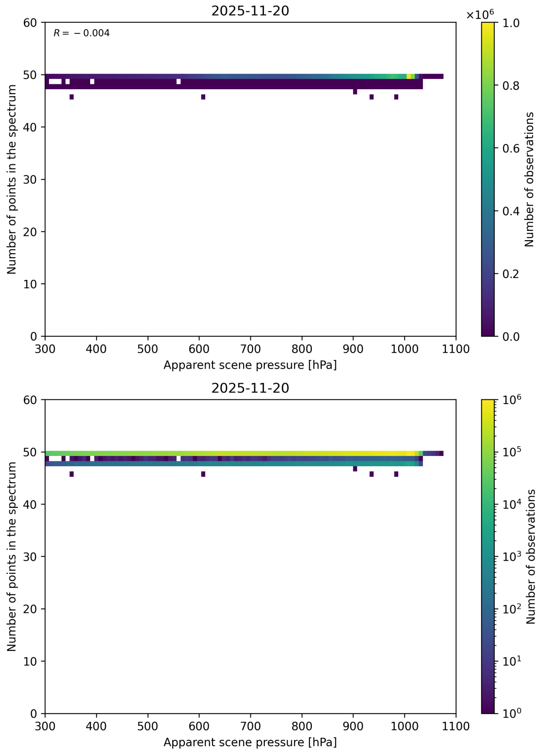
Figure 66: Scatter density plot of “Apparent scene pressure” against “Number of points in the spectrum” for 2025-11-19 to 2025-11-21.
