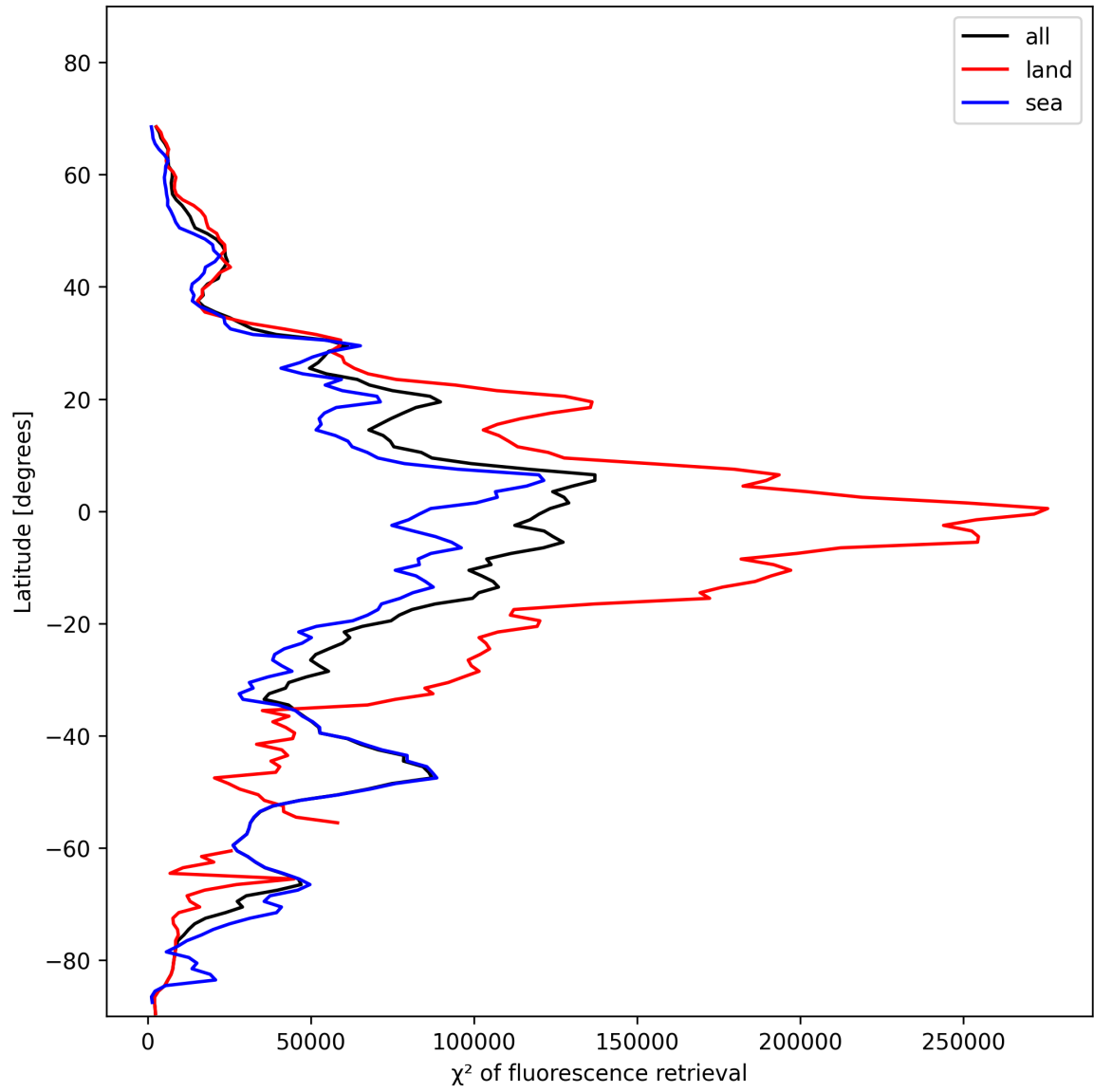
Figure 25: Zonal average of “ \chi^2 of fluorescence retrieval” for 2025-11-19 to 2025-11-21.
