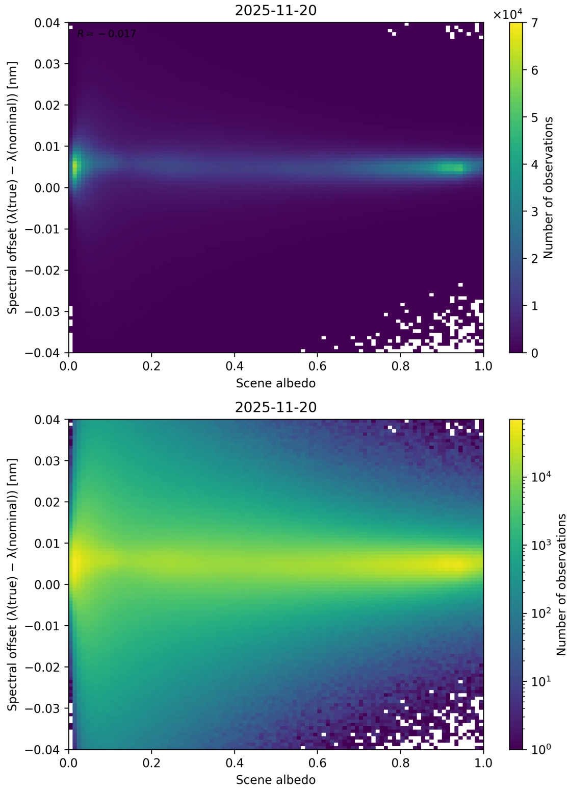
Figure 107: Scatter density plot of “Scene albedo” against “Spectral offset ( \lambda_{\text{true}} - \lambda_{\text{nominal}} )” for 2025-11-19 to 2025-11-21.
