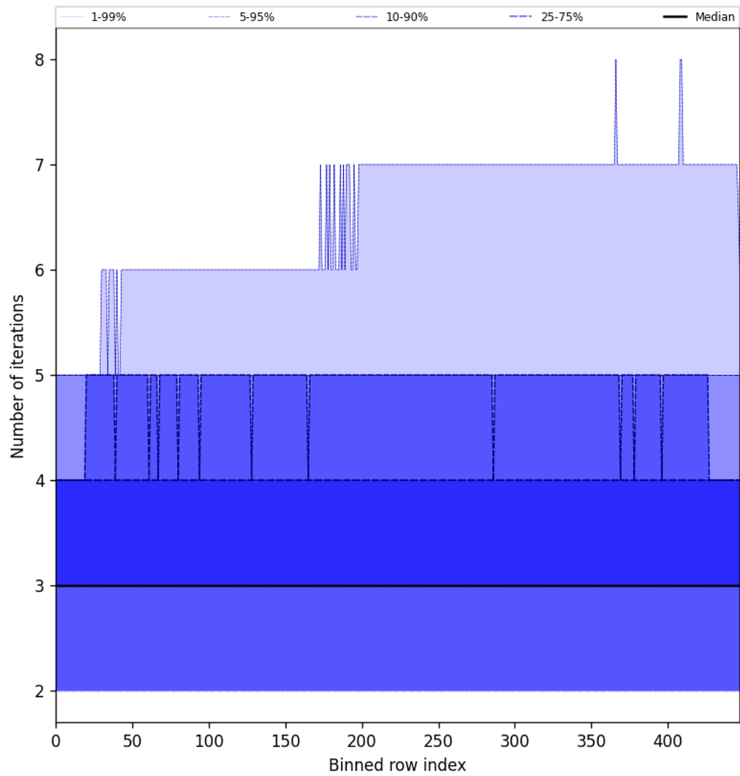
Figure 56: Along track statistics of “Number of iterations” for 2025-11-19 to 2025-11-21
