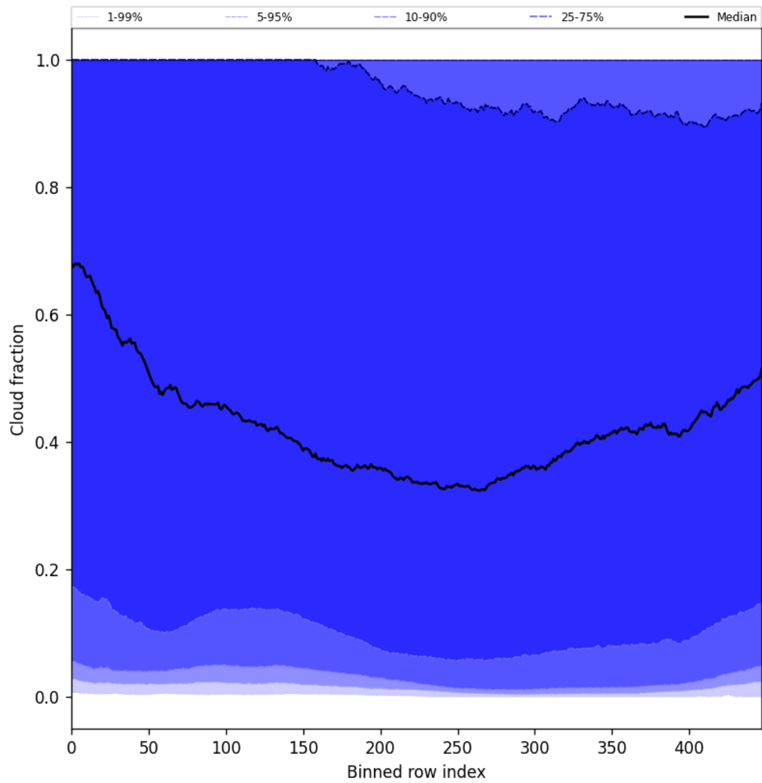
Figure 49: Along track statistics of “Cloud fraction” for 2025-11-19 to 2025-11-21
