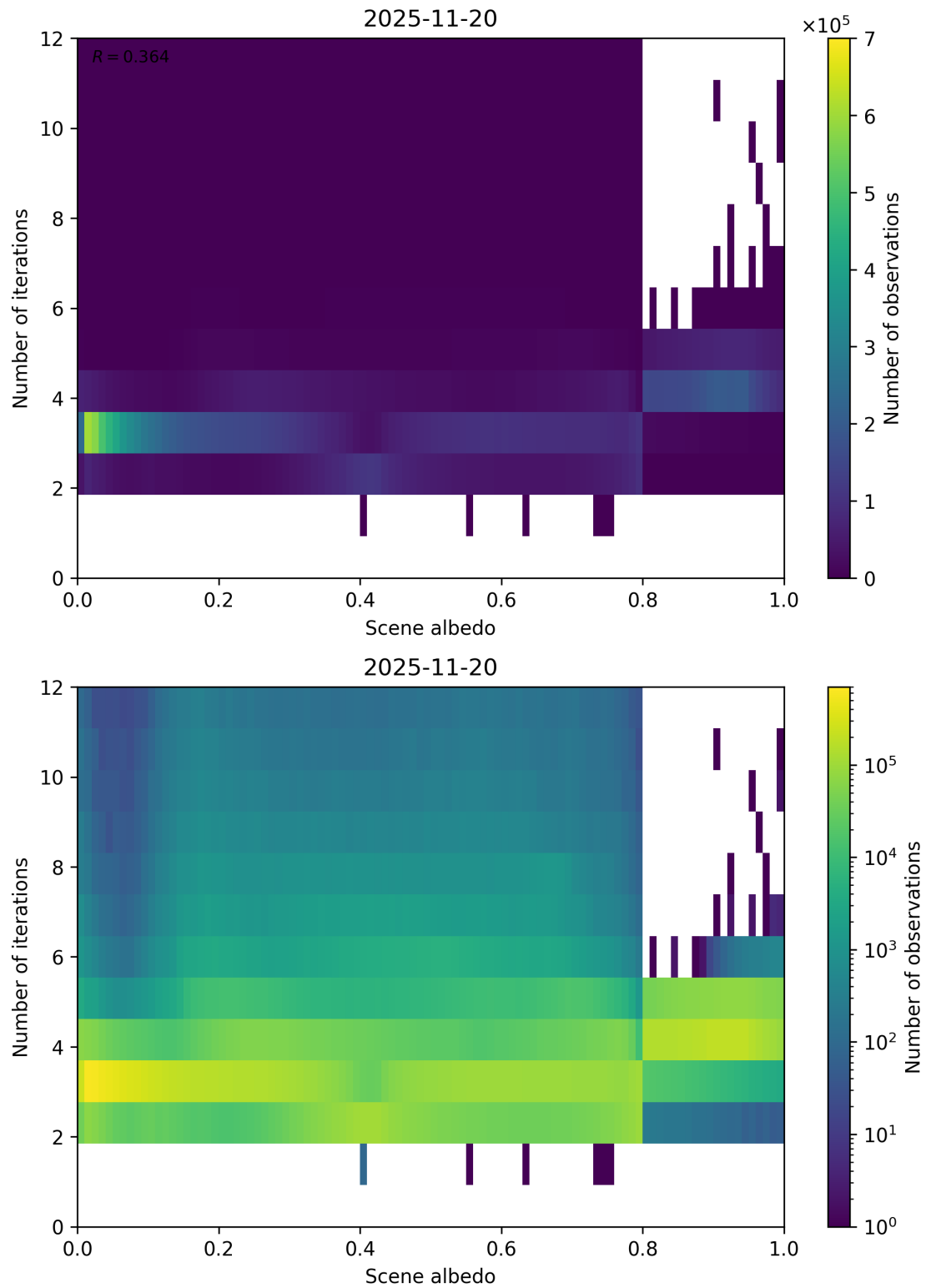
Figure 105: Scatter density plot of “Scene albedo” against “Number of iterations” for 2025-11-19 to 2025-11-21.
