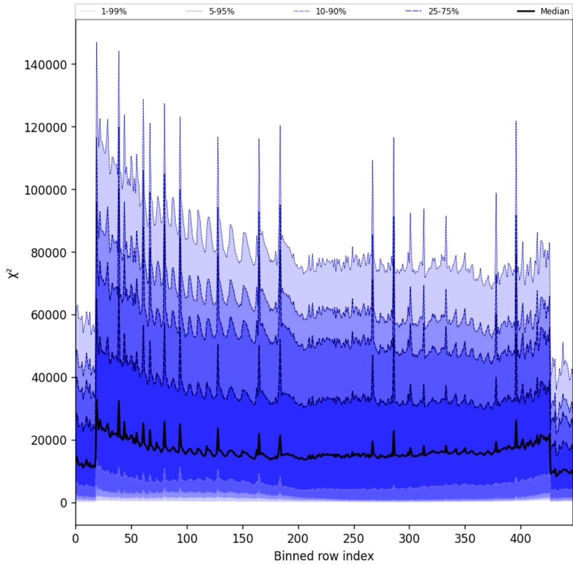
Figure 55: Along track statistics of “ \chi^2 ” for 2025-11-19 to 2025-11-21
