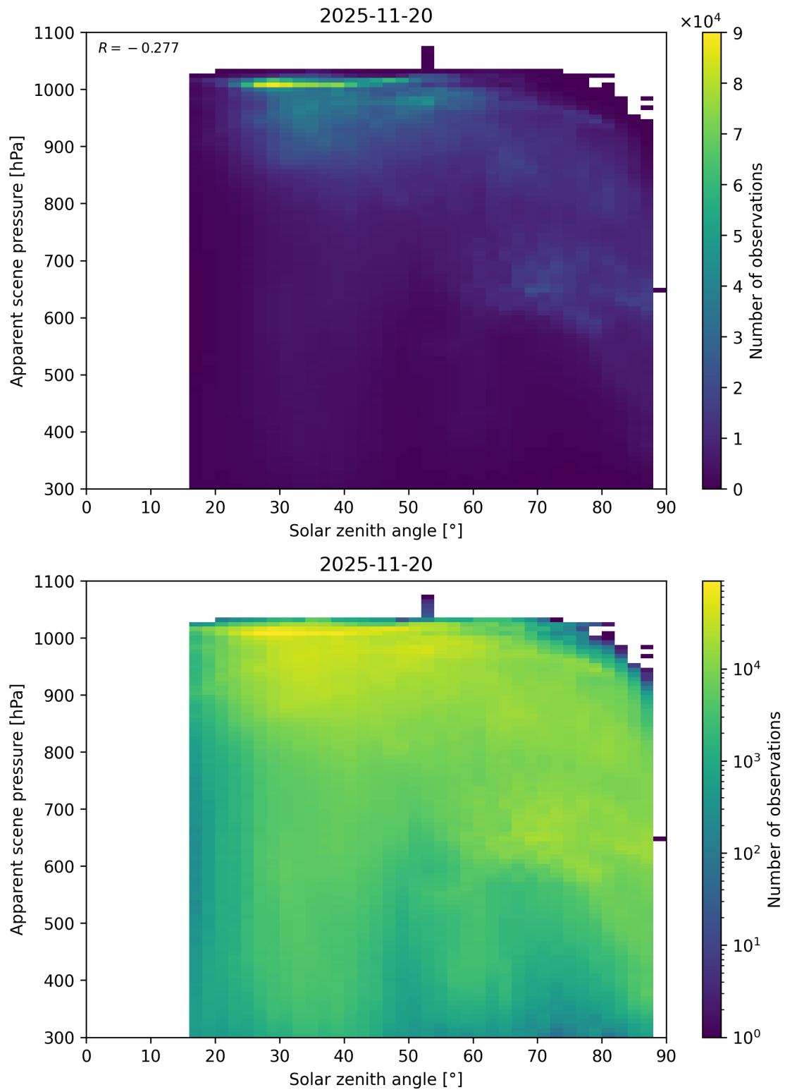
Figure 108: Scatter density plot of “Solar zenith angle” against “Apparent scene pressure” for 2025-11-19 to 2025-11-21.
