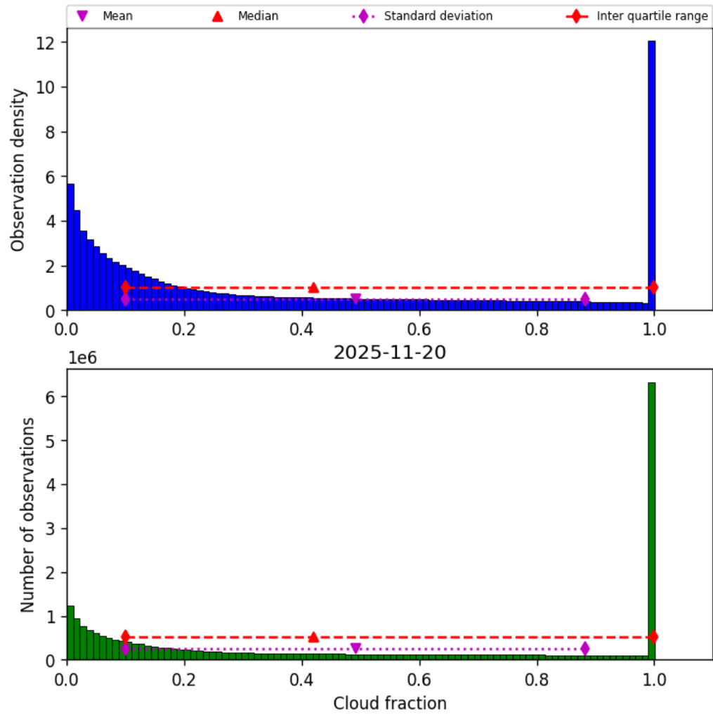
Figure 32: Histogram of “Cloud fraction” for 2025-11-19 to 2025-11-21
