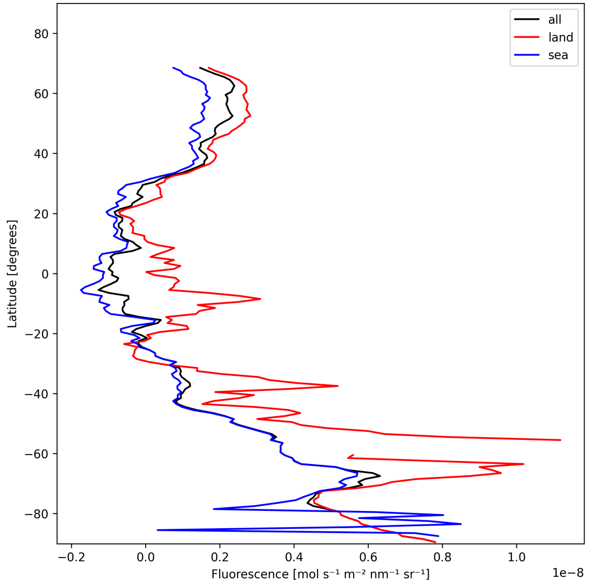
Figure 23: Zonal average of “Fluorescence” for 2025-11-19 to 2025-11-21.
