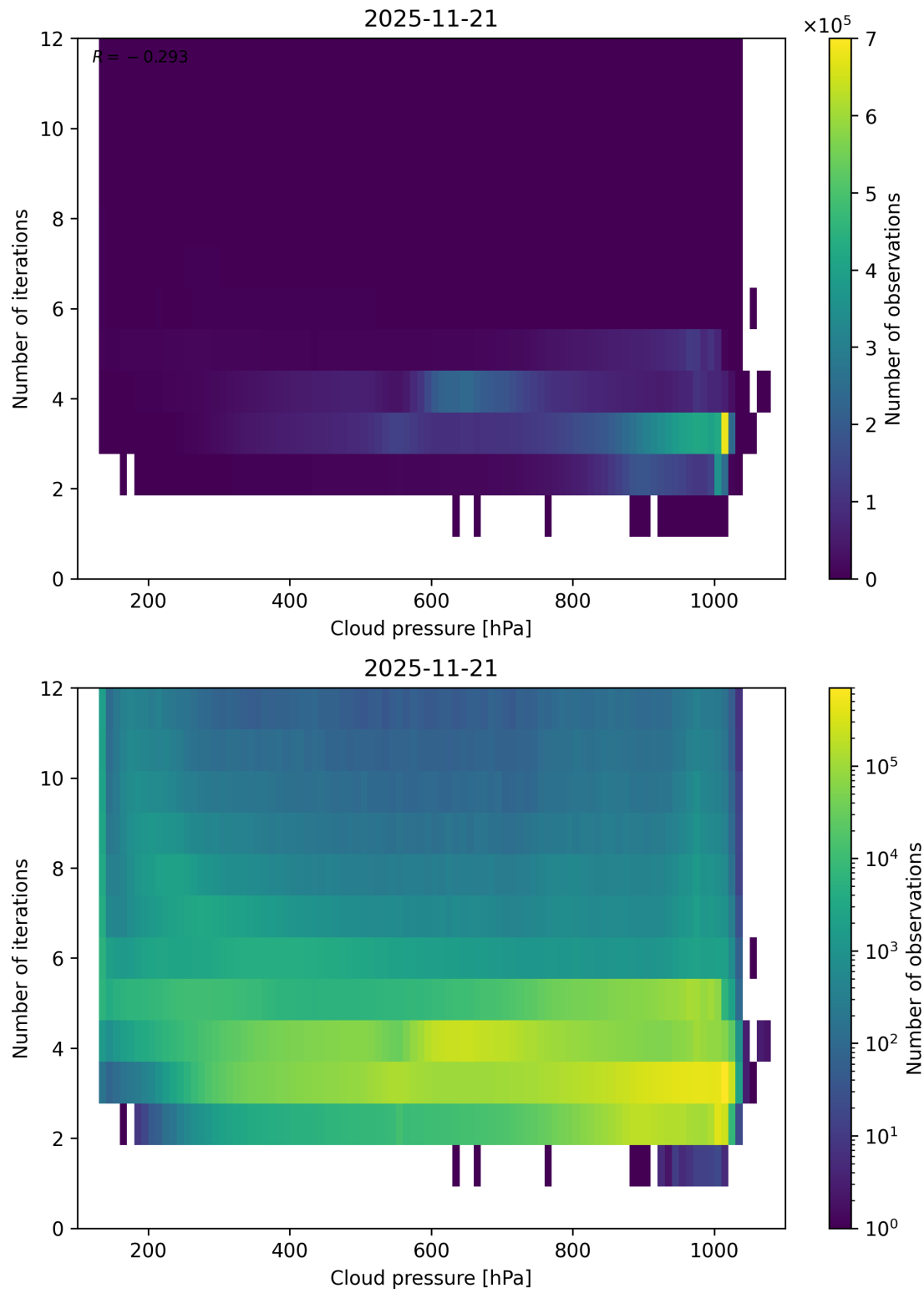
Figure 81: Scatter density plot of “Cloud pressure” against “Number of iterations” for 2025-11-20 to 2025-11-22.
