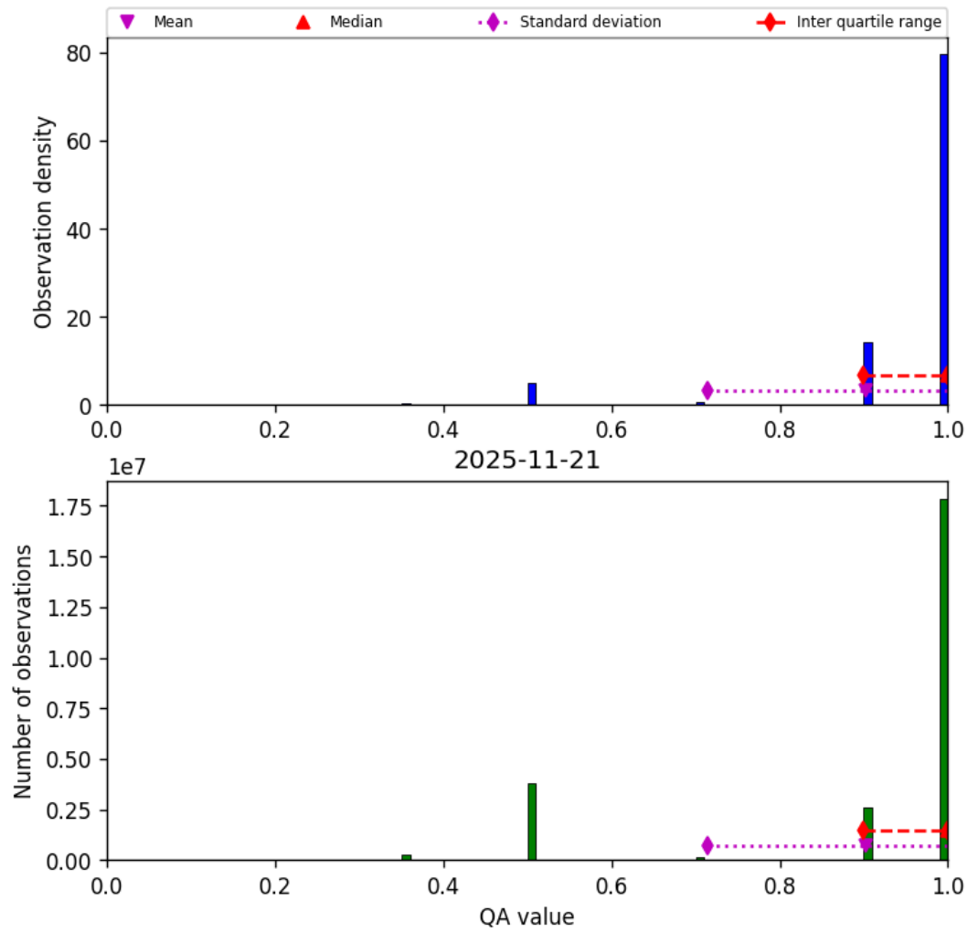
Figure 29: Histogram of “QA value” for 2025-11-20 to 2025-11-22
