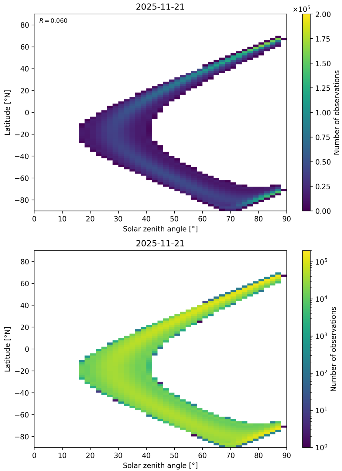
Figure 113: Scatter density plot of “Solar zenith angle” against “Latitude” for 2025-11-20 to 2025-11-22.
