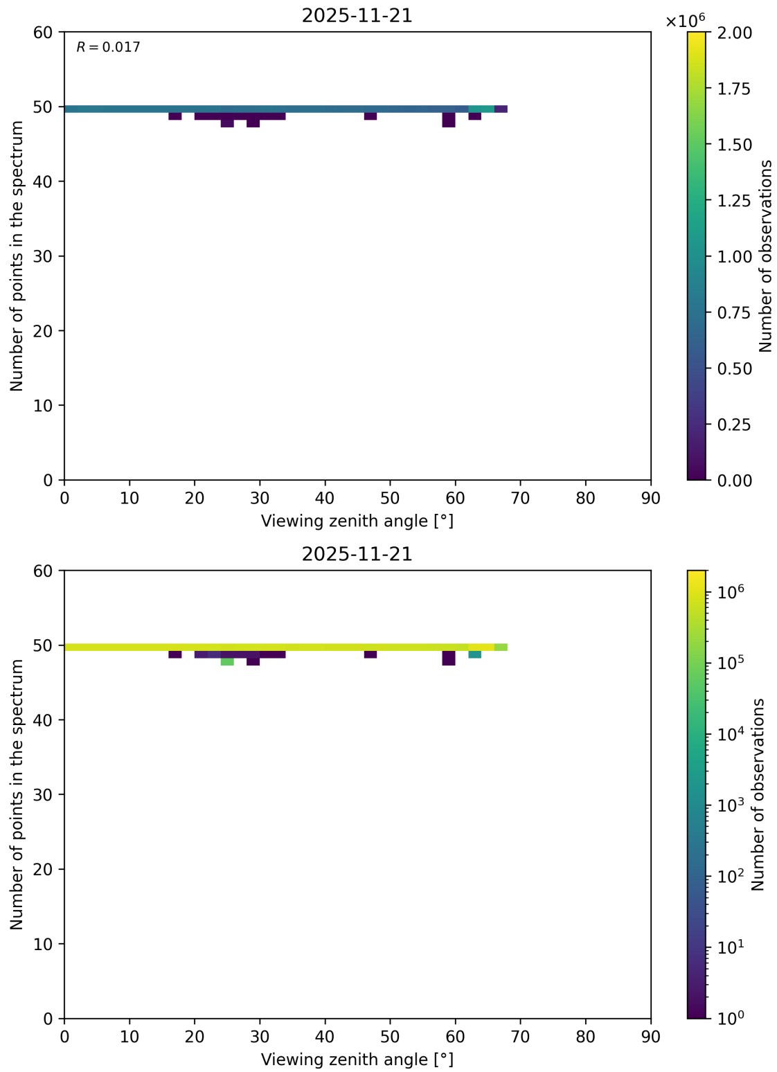
Figure 125: Scatter density plot of “Viewing zenith angle” against “Number of points in the spectrum” for 2025-11-20 to 2025-11-22.
