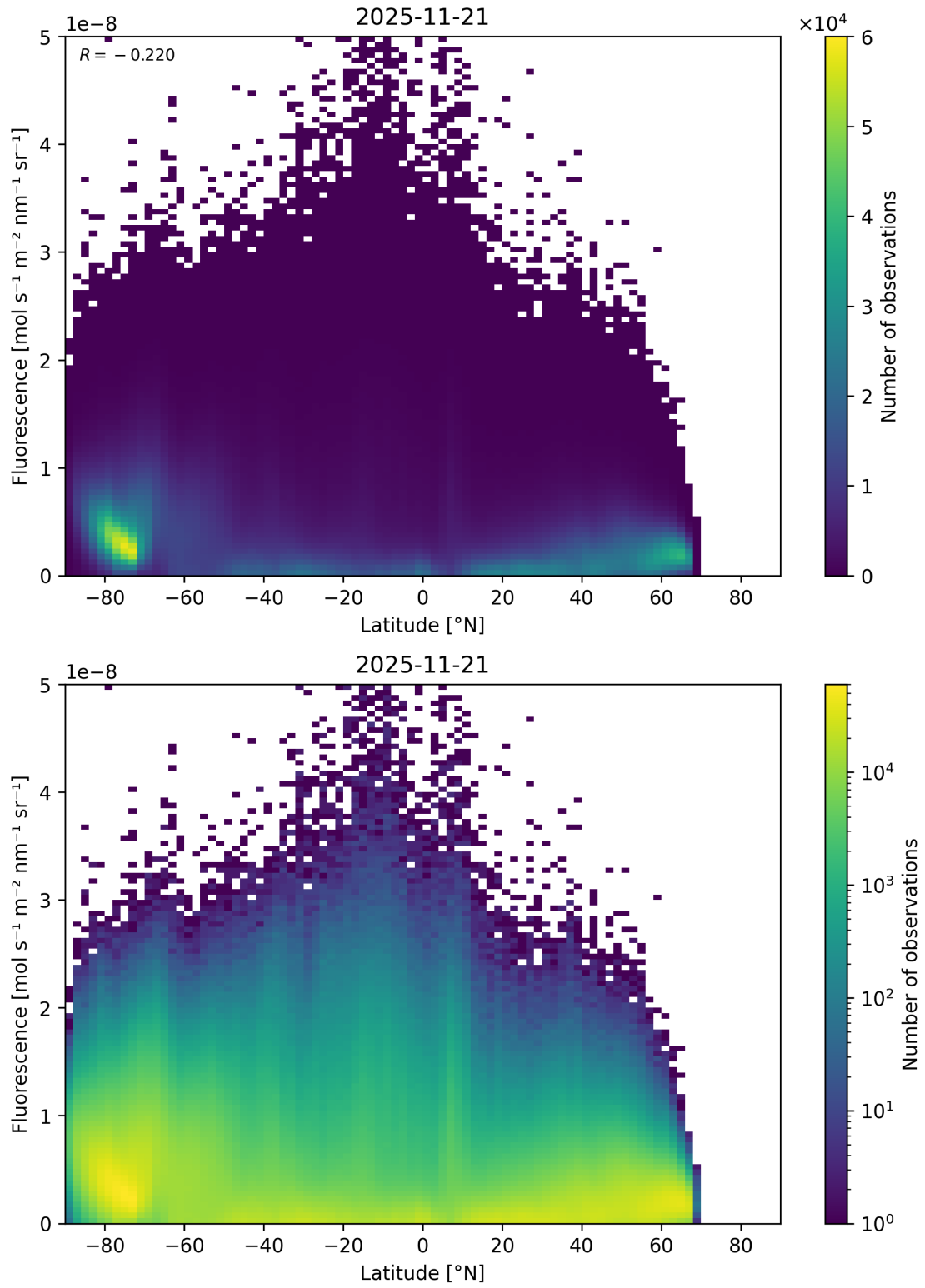
Figure 92: Scatter density plot of “Latitude” against “Fluorescence” for 2025-11-20 to 2025-11-22.
