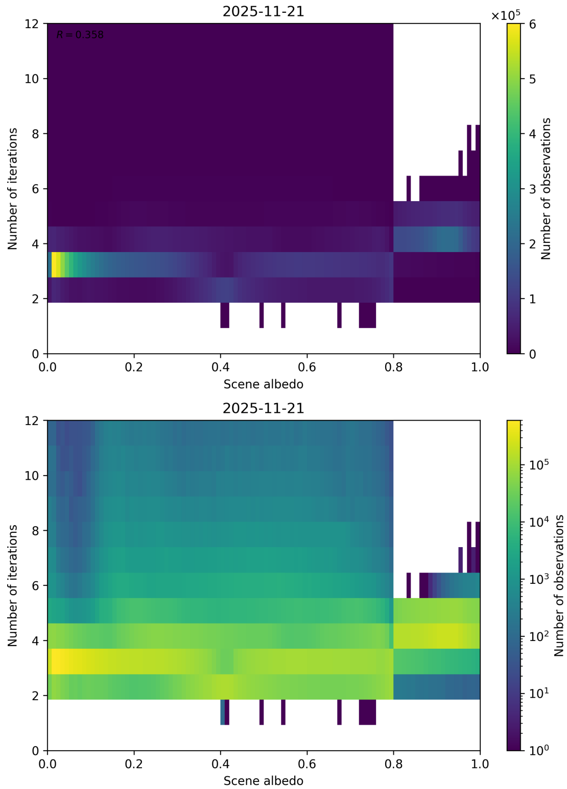
Figure 105: Scatter density plot of “Scene albedo” against “Number of iterations” for 2025-11-20 to 2025-11-22.
