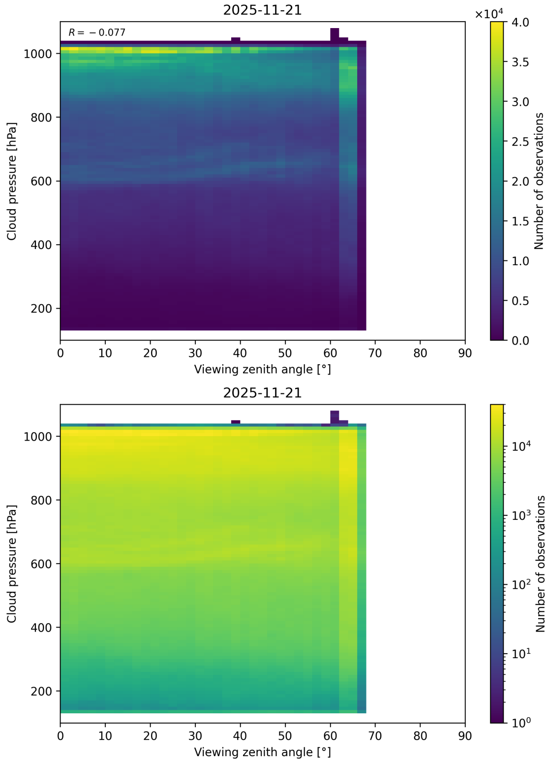
Figure 121: Scatter density plot of “Viewing zenith angle” against “Cloud pressure” for 2025-11-20 to 2025-11-22.
