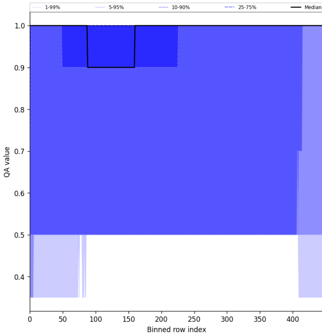
Figure 46: Along track statistics of “QA value” for 2025-11-20 to 2025-11-22
