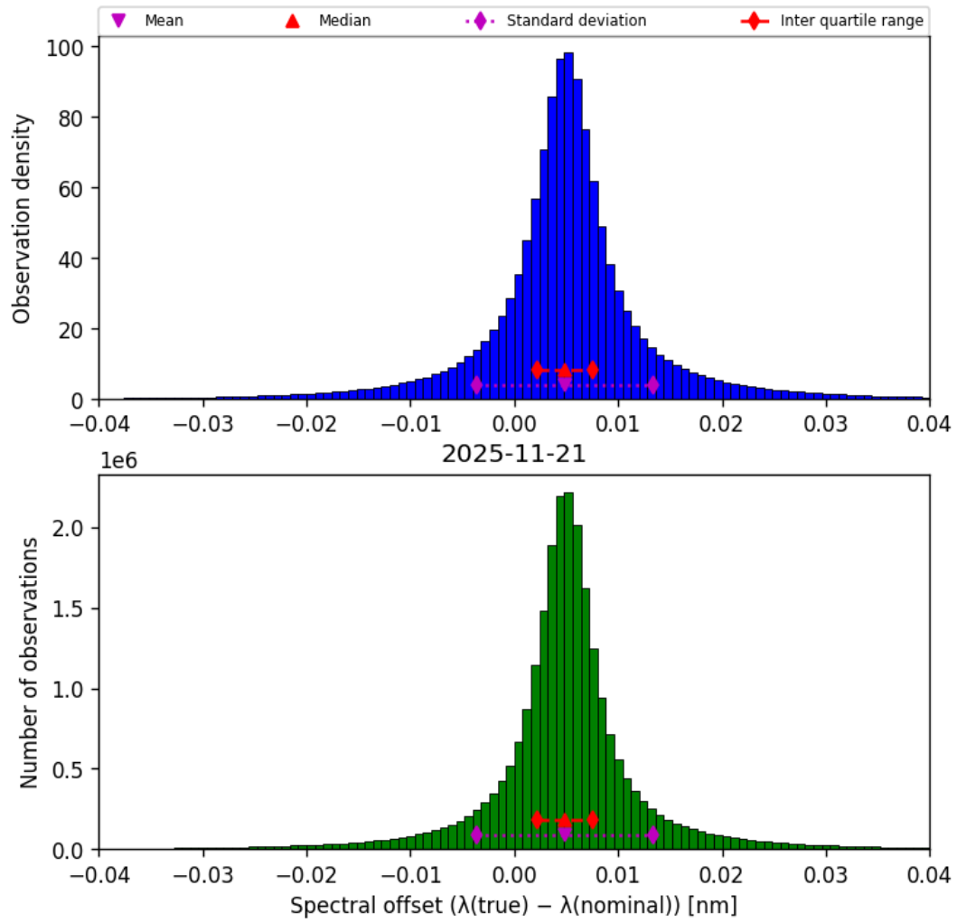
Figure 45: Histogram of “Spectral offset ( \lambda_{\text{true}} - \lambda_{\text{nominal}} )” for 2025-11-20 to 2025-11-22
