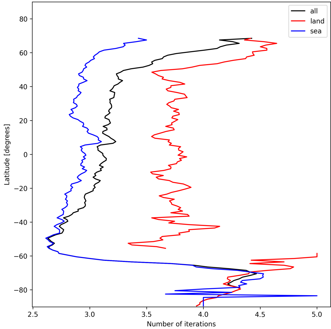
Figure 22: Zonal average of “Number of iterations” for 2025-11-20 to 2025-11-22.
