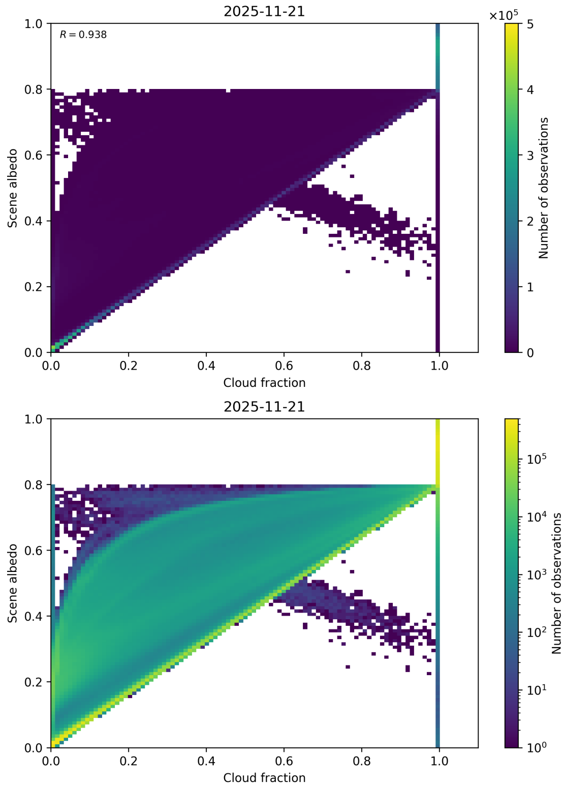
Figure 75: Scatter density plot of “Cloud fraction” against “Scene albedo” for 2025-11-20 to 2025-11-22.
