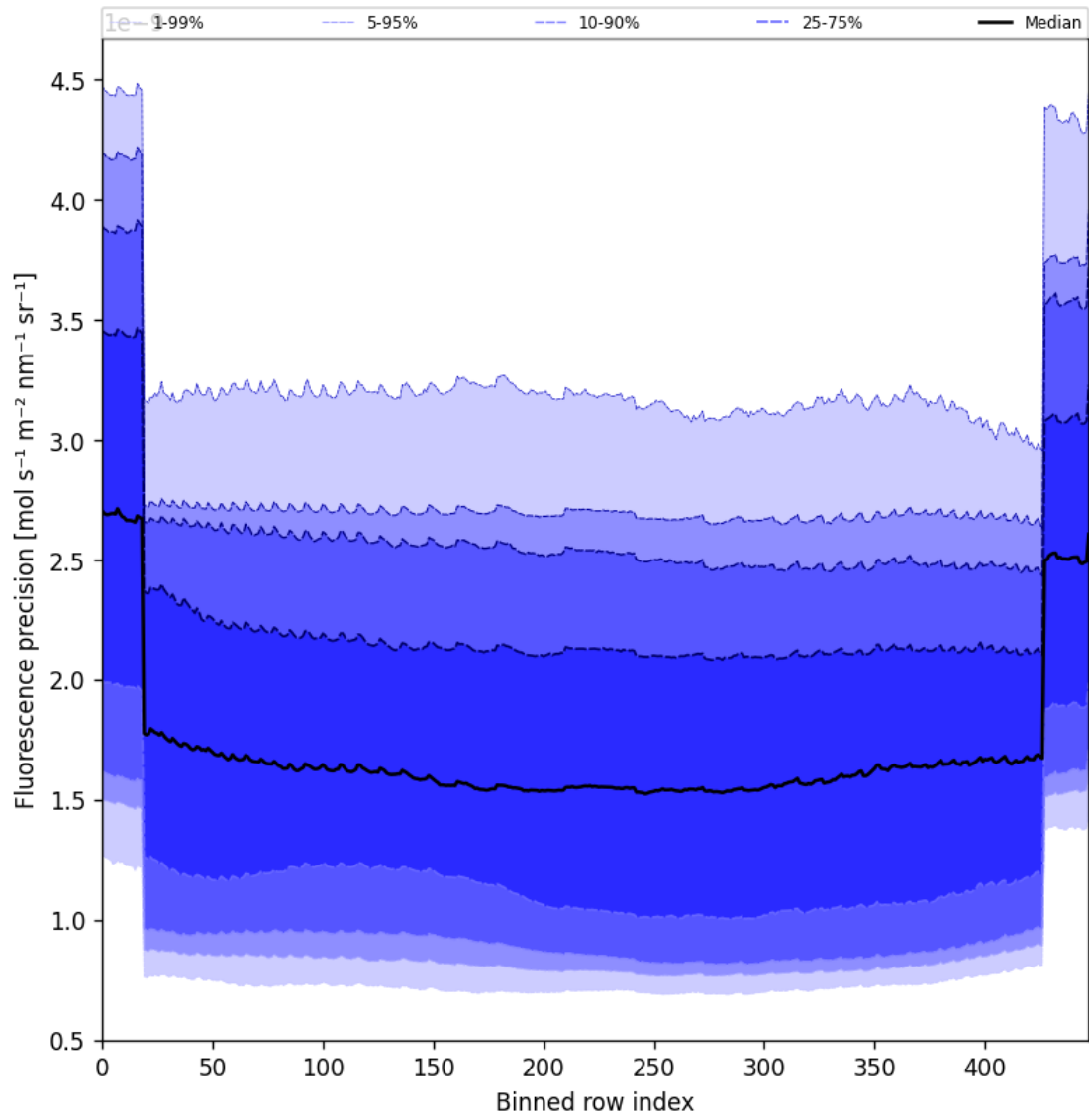
Figure 58: Along track statistics of “Fluorescence precision” for 2025-11-20 to 2025-11-22
