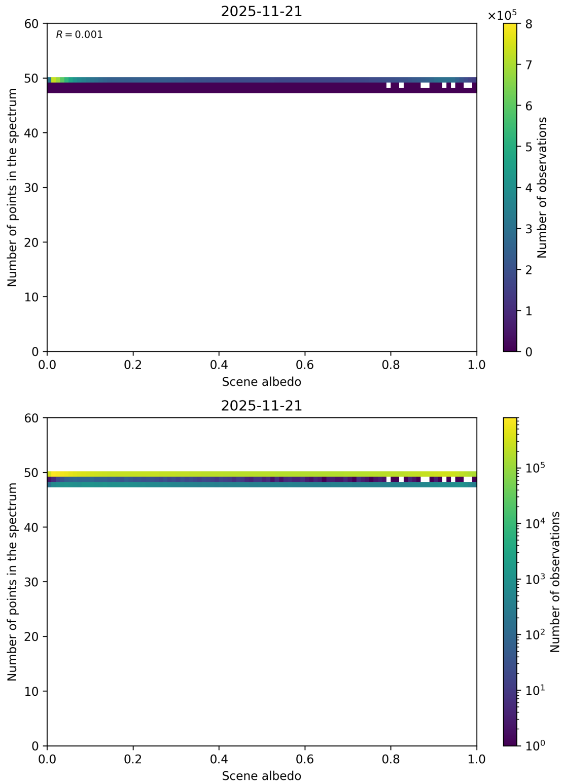
Figure 106: Scatter density plot of “Scene albedo” against “Number of points in the spectrum” for 2025-11-20 to 2025-11-22.
