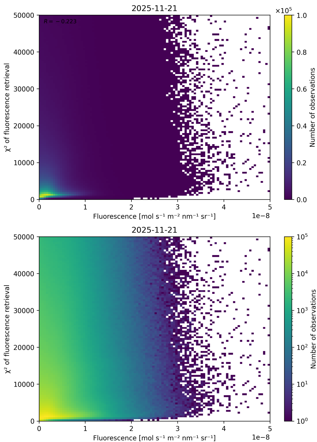
Figure 85: Scatter density plot of “Fluorescence” against “ \chi^2 of fluorescence retrieval” for 2025-11-20 to 2025-11-22.
