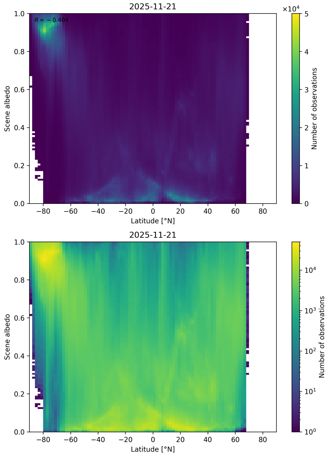
Figure 95: Scatter density plot of “Latitude” against “Scene albedo” for 2025-11-20 to 2025-11-22.
