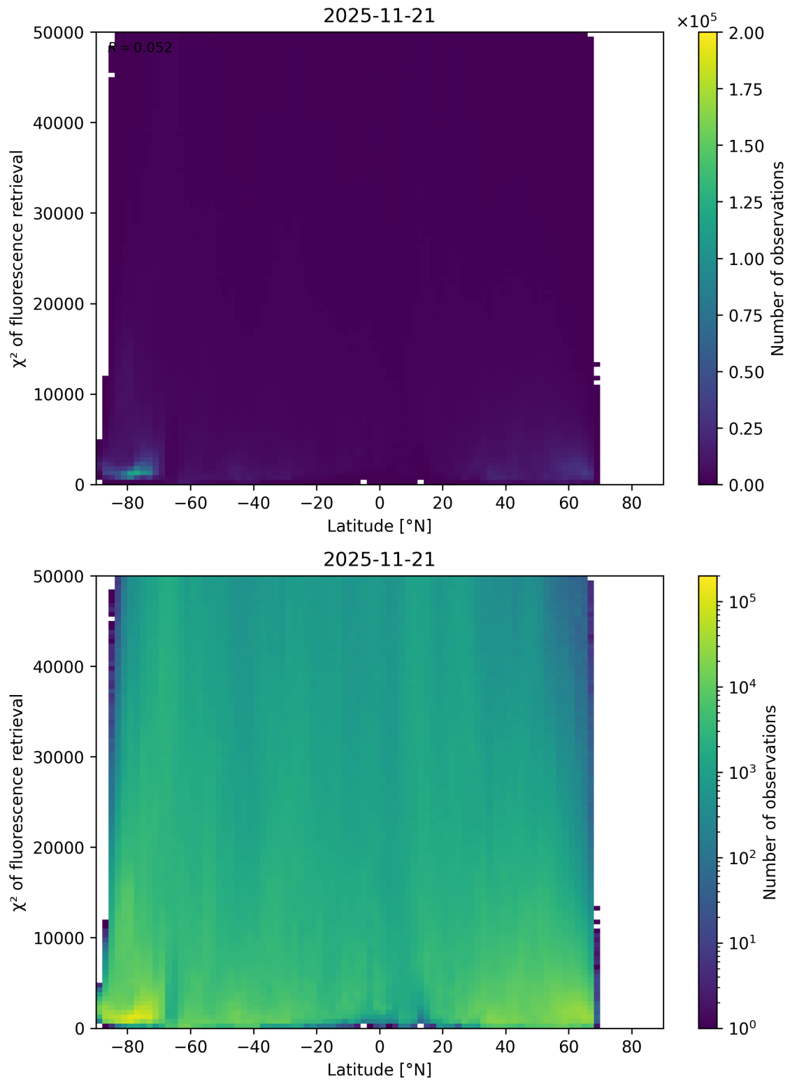
Figure 89: Scatter density plot of “Latitude” against “ \chi^2 of fluorescence retrieval” for 2025-11-20 to 2025-11-22.
