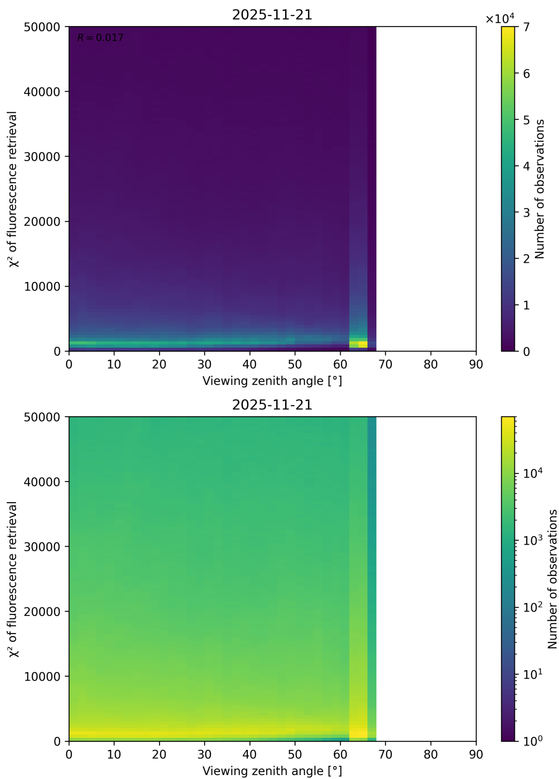
Figure 119: Scatter density plot of “Viewing zenith angle” against “ \chi^2 of fluorescence retrieval” for 2025-11-20 to 2025-11-22.
