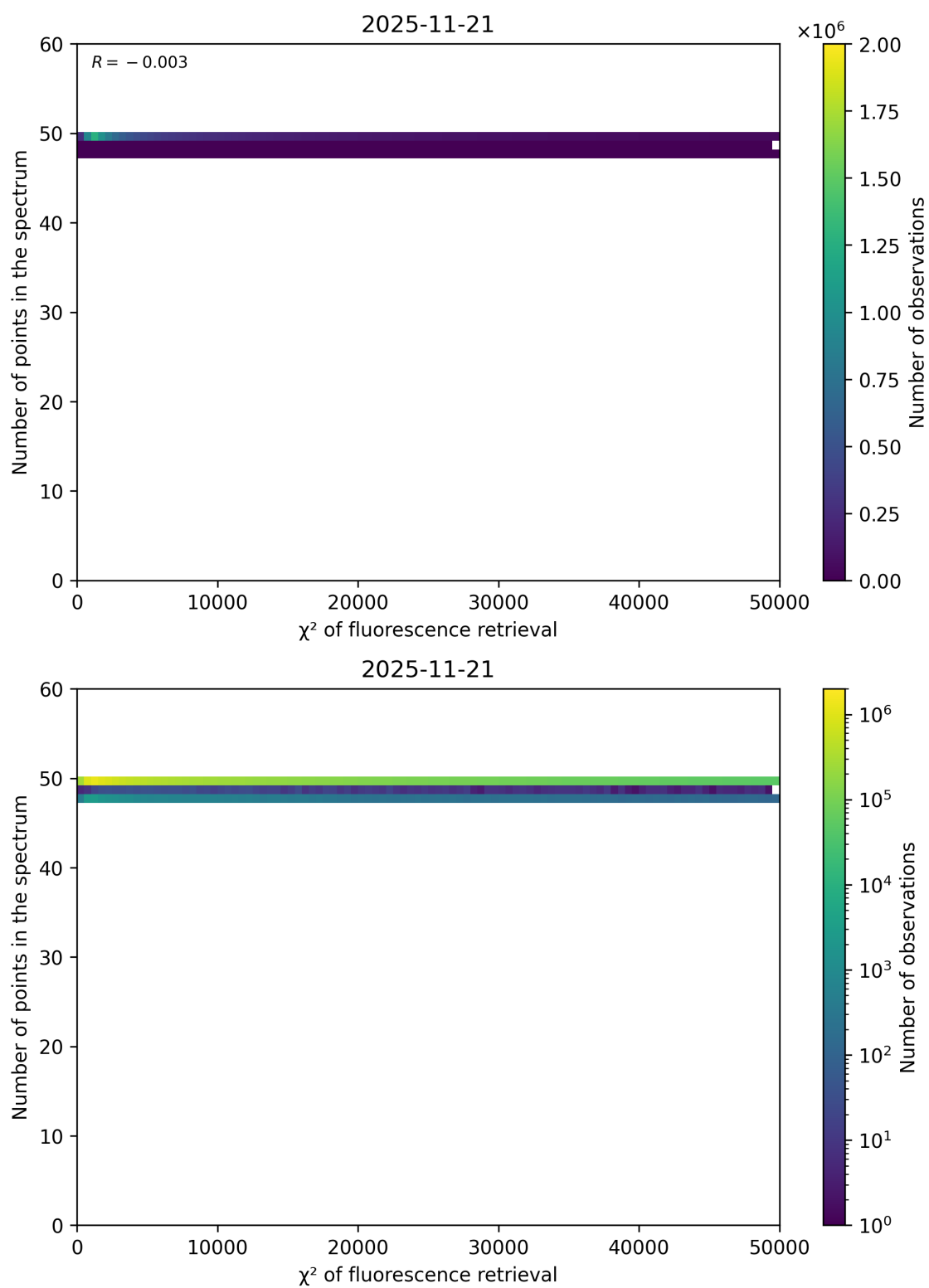
Figure 68: Scatter density plot of " \chi^2 of fluorescence retrieval" against "Number of points in the spectrum" for 2025-11-20 to 2025-11-22.
