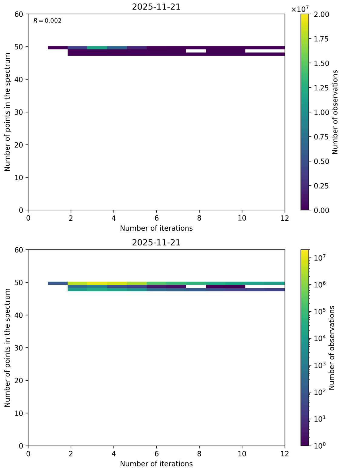
Figure 99: Scatter density plot of “Number of iterations” against “Number of points in the spectrum” for 2025-11-20 to 2025-11-22.
