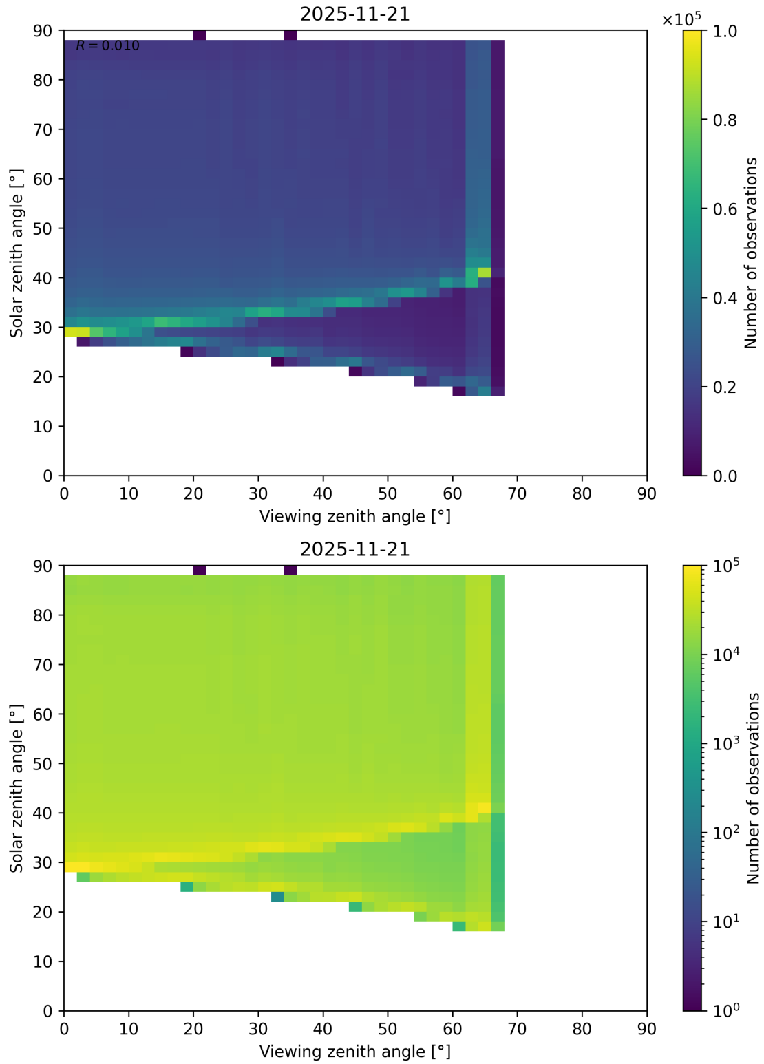
Figure 127: Scatter density plot of “Viewing zenith angle” against “Solar zenith angle” for 2025-11-20 to 2025-11-22.
