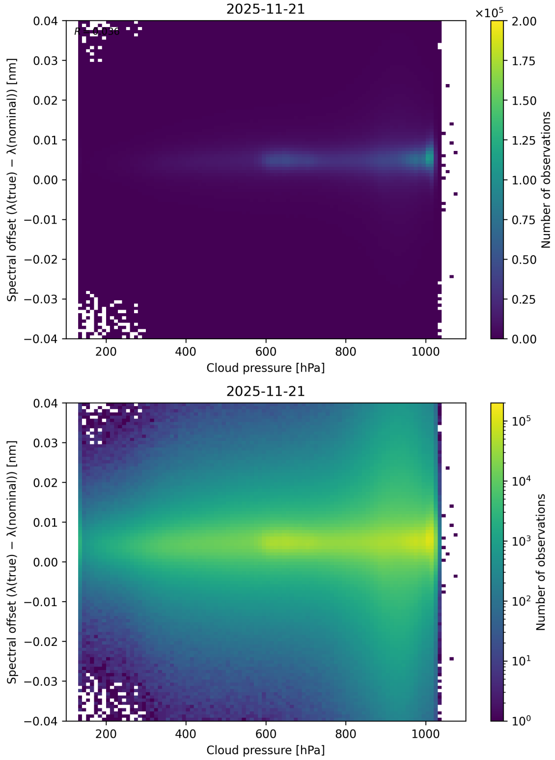
Figure 84: Scatter density plot of “Cloud pressure” against “Spectral offset ( \lambda_{\text{true}} - \lambda_{\text{nominal}} )” for 2025-11-20 to 2025-11-22.
