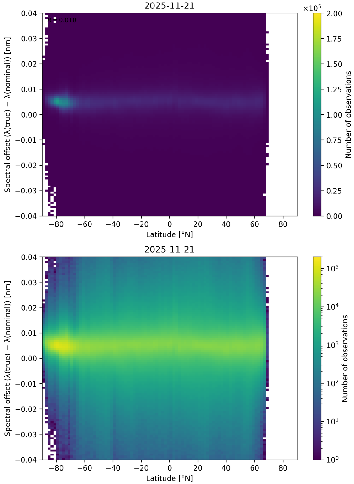
Figure 96: Scatter density plot of “Latitude” against “Spectral offset ( \lambda_{\text{true}} - \lambda_{\text{nominal}} )” for 2025-11-20 to 2025-11-22.
