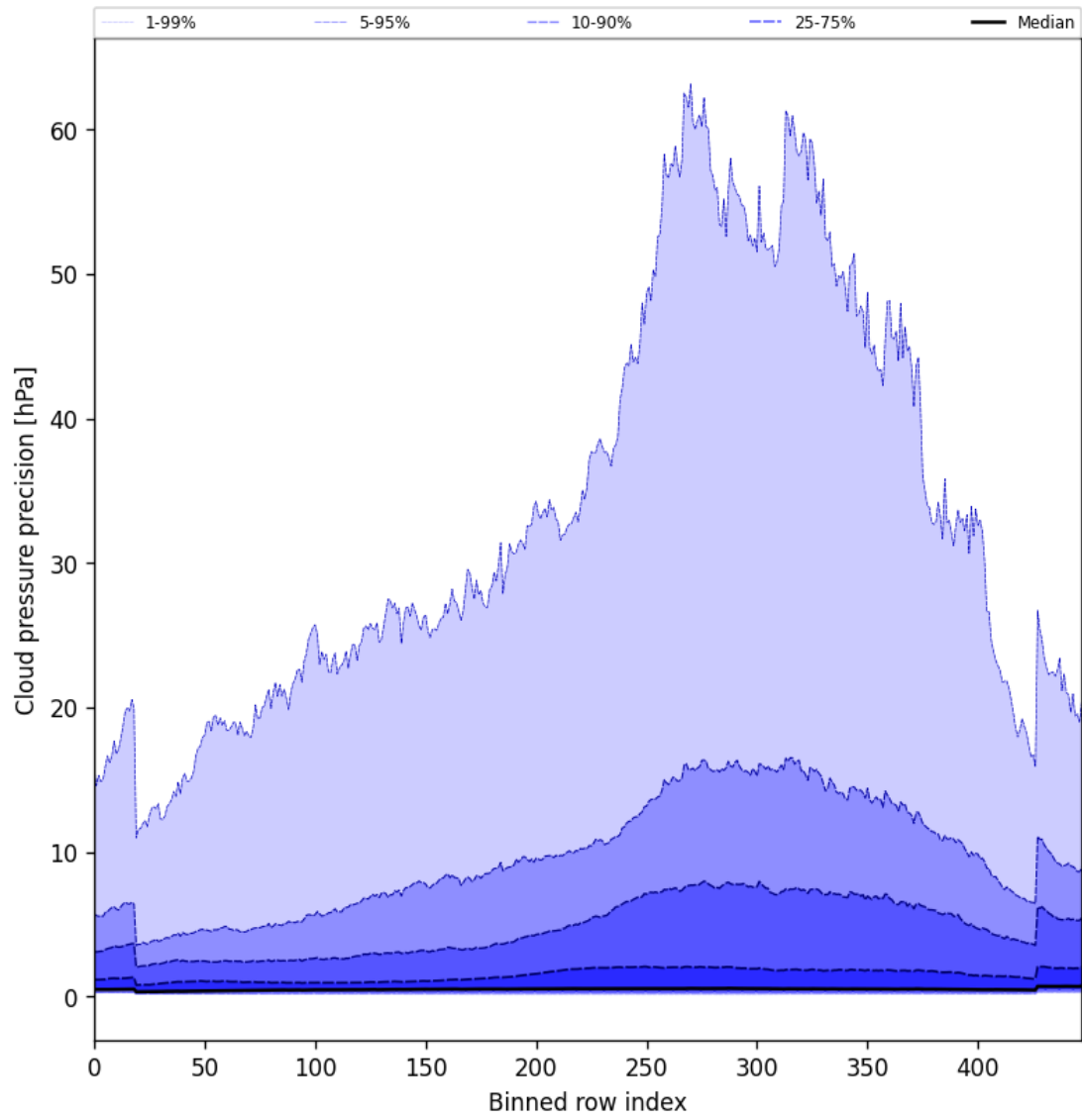
Figure 48: Along track statistics of “Cloud pressure precision” for 2025-11-20 to 2025-11-22
