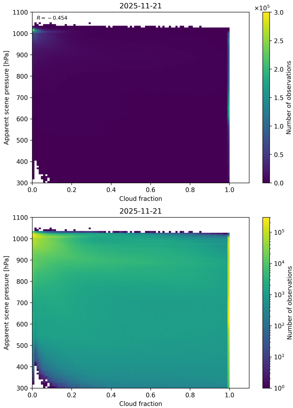
Figure 70: Scatter density plot of “Cloud fraction” against “Apparent scene pressure” for 2025-11-20 to 2025-11-22.
