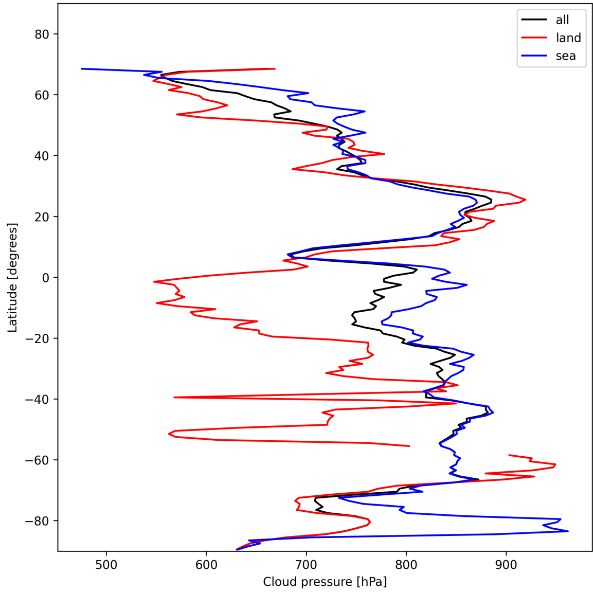
Figure 13: Zonal average of “Cloud pressure” for 2025-11-20 to 2025-11-22.
