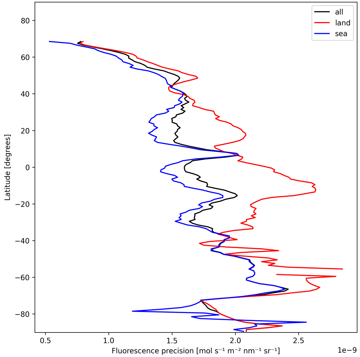
Figure 24: Zonal average of “Fluorescence precision” for 2025-11-20 to 2025-11-22.
