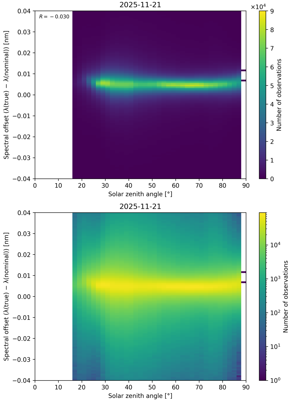
Figure 117: Scatter density plot of “Solar zenith angle” against “Spectral offset ( \lambda_{\text{true}} - \lambda_{\text{nominal}} )” for 2025-11-20 to 2025-11-22.
