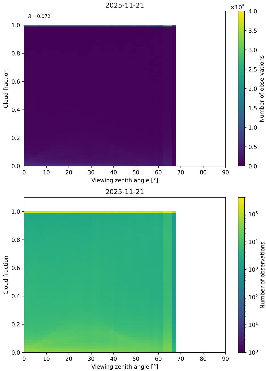
Figure 120: Scatter density plot of “Viewing zenith angle” against “Cloud fraction” for 2025-11-20 to 2025-11-22.
