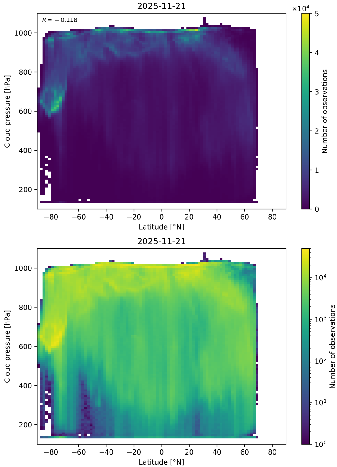
Figure 91: Scatter density plot of “Latitude” against “Cloud pressure” for 2025-11-20 to 2025-11-22.
