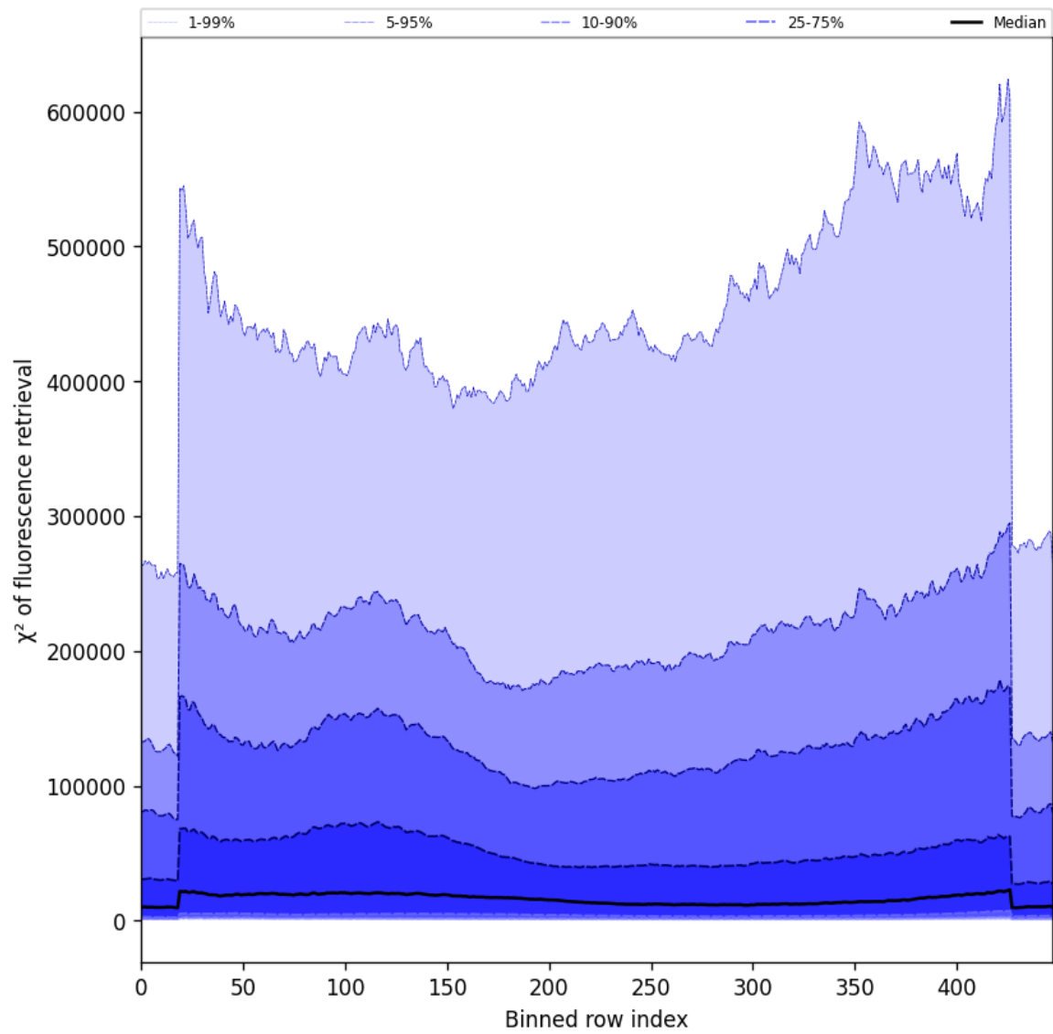
Figure 59: Along track statistics of “ \chi^2 of fluorescence retrieval” for 2025-11-20 to 2025-11-22
