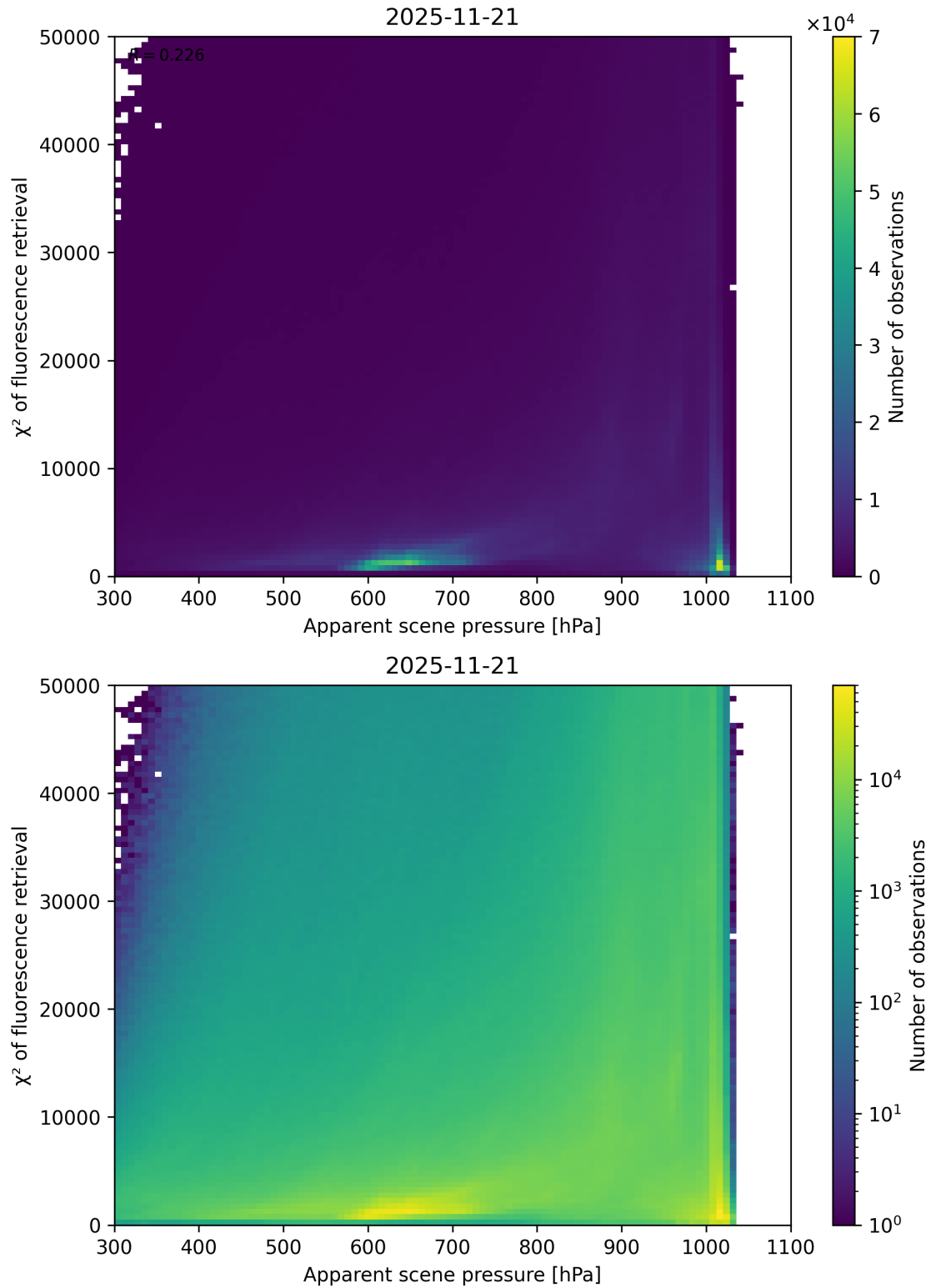
Figure 63: Scatter density plot of “Apparent scene pressure” against “ \chi^2 of fluorescence retrieval” for 2025-11-20 to 2025-11-22.
