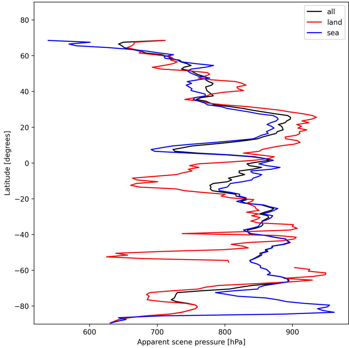
Figure 19: Zonal average of “Apparent scene pressure” for 2025-11-20 to 2025-11-22.
