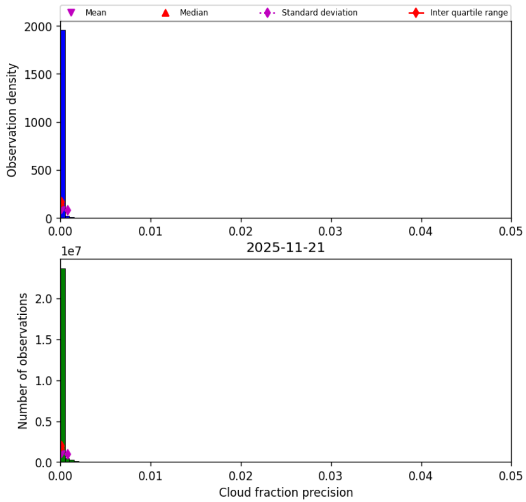
Figure 33: Histogram of “Cloud fraction precision” for 2025-11-20 to 2025-11-22
