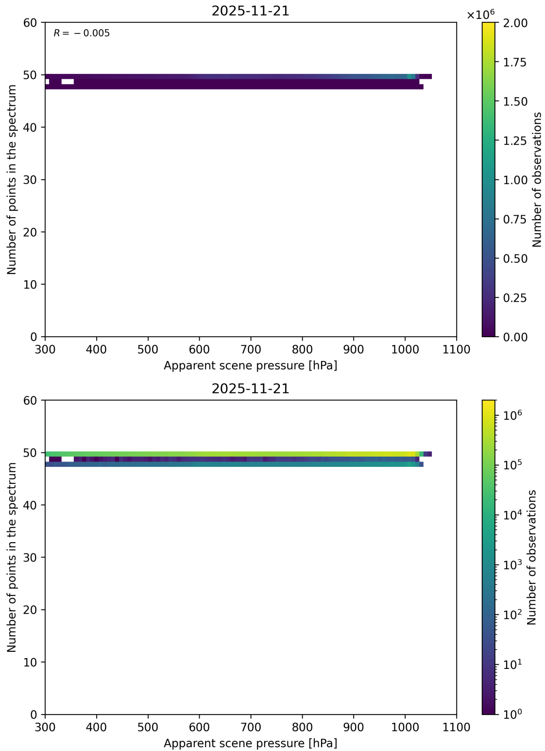
Figure 66: Scatter density plot of “Apparent scene pressure” against “Number of points in the spectrum” for 2025-11-20 to 2025-11-22.
