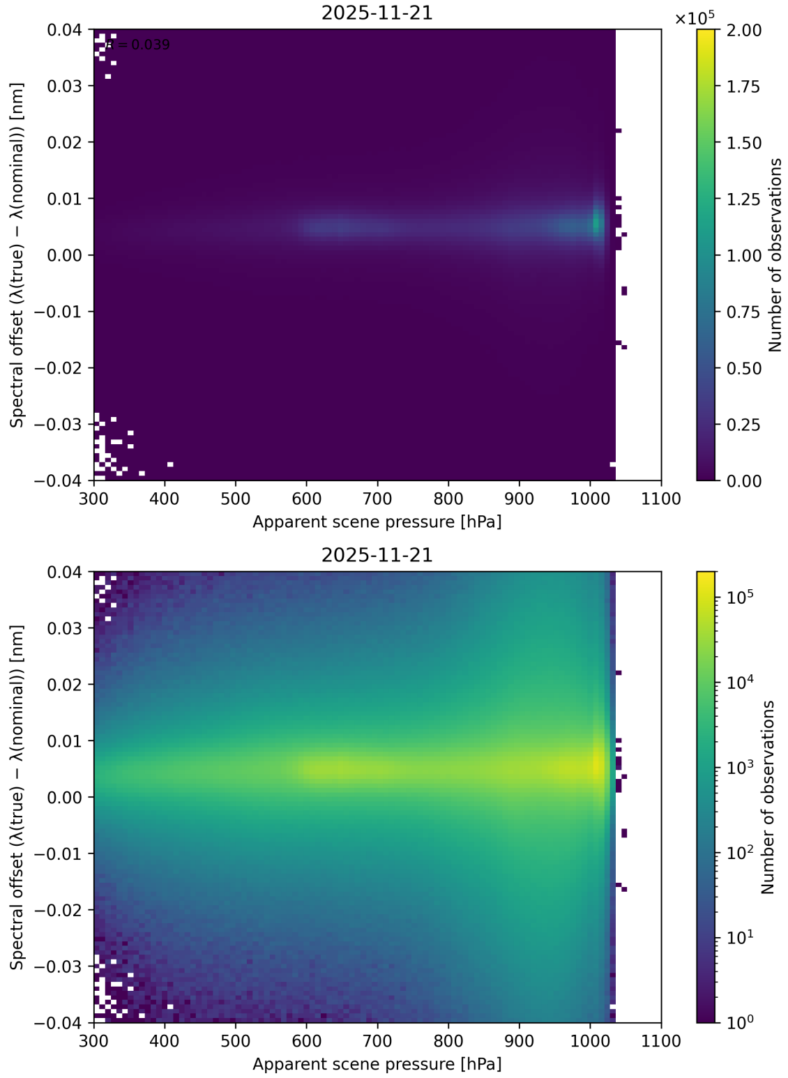
Figure 67: Scatter density plot of “Apparent scene pressure” against “Spectral offset ( \lambda_{\text{true}} - \lambda_{\text{nominal}} )” for 2025-11-20 to 2025-11-22.
