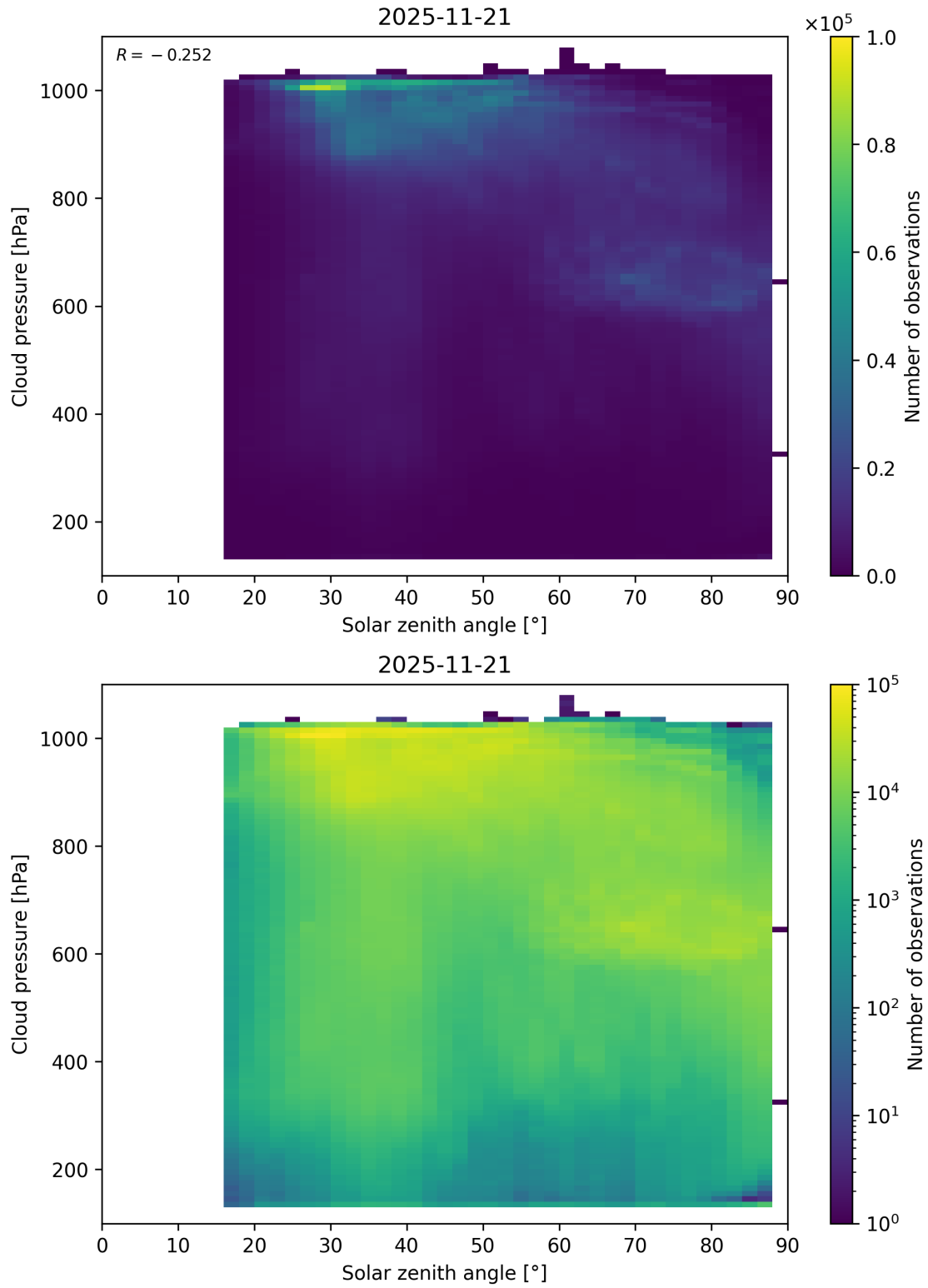
Figure 111: Scatter density plot of “Solar zenith angle” against “Cloud pressure” for 2025-11-20 to 2025-11-22.
