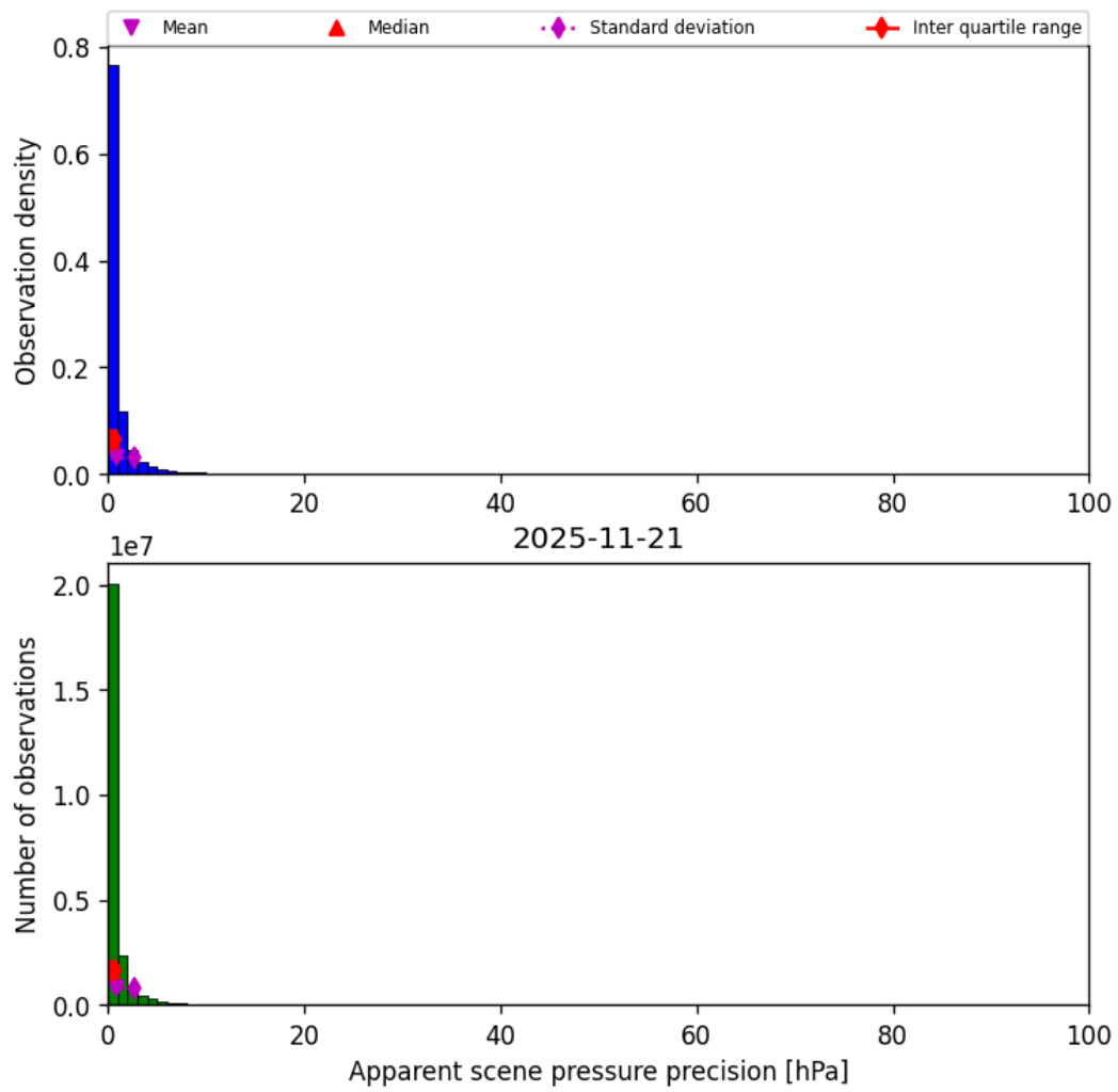
Figure 37: Histogram of “Apparent scene pressure precision” for 2025-11-20 to 2025-11-22
