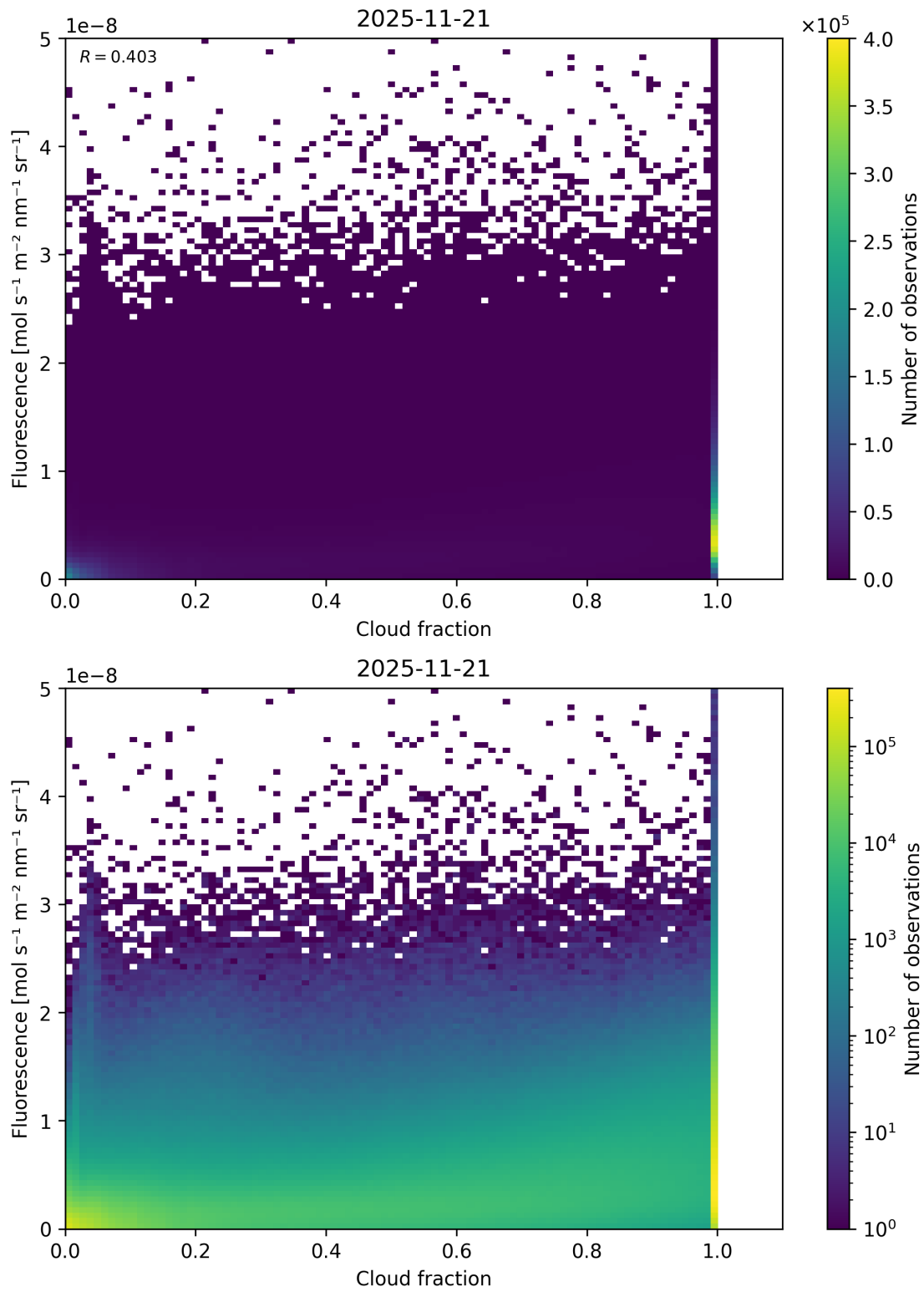
Figure 72: Scatter density plot of “Cloud fraction” against “Fluorescence” for 2025-11-20 to 2025-11-22.
