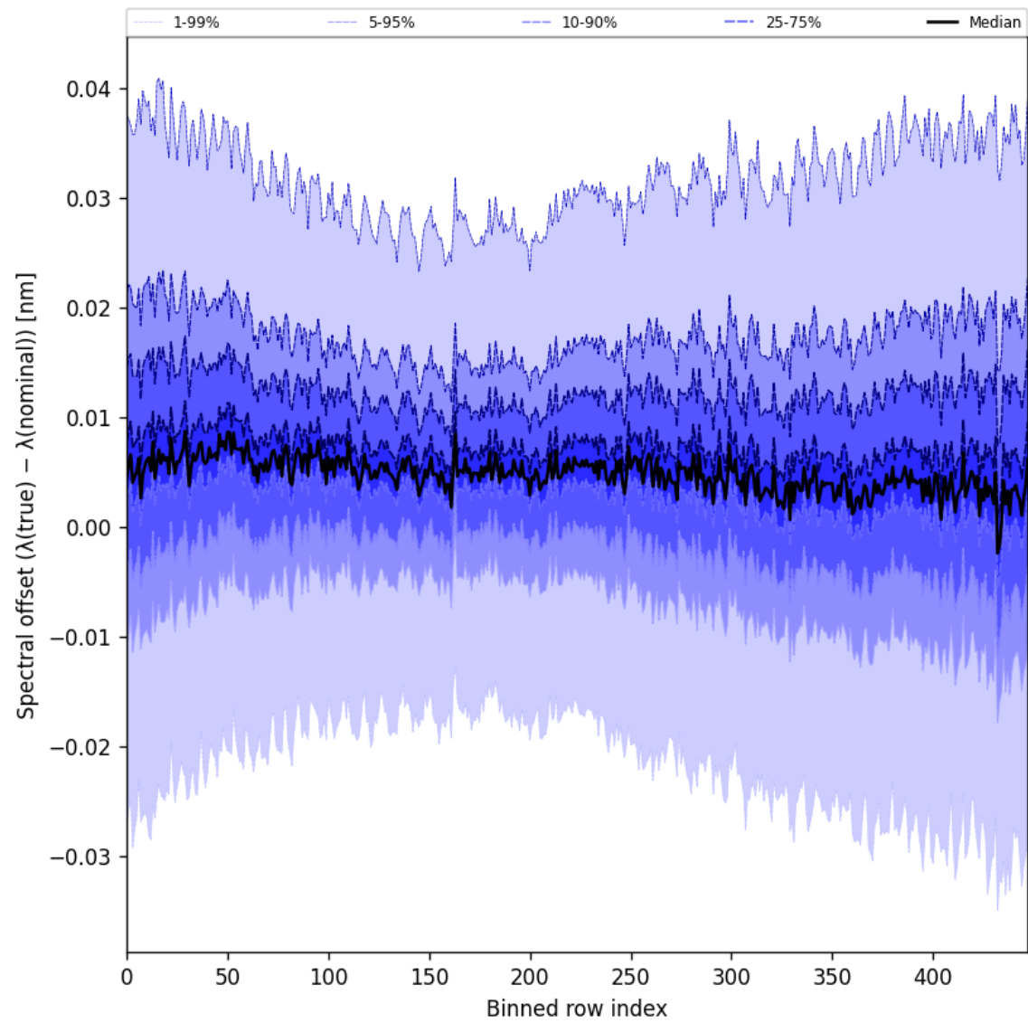
Figure 62: Along track statistics of “Spectral offset ( \lambda_{\text{true}} - \lambda_{\text{nominal}} )” for 2025-11-20 to 2025-11-22
