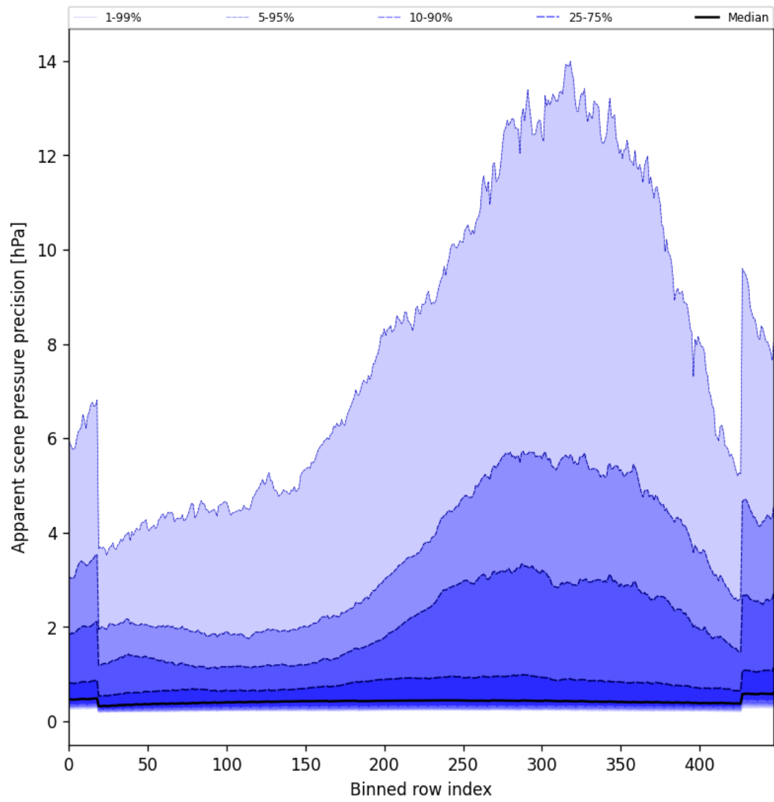
Figure 54: Along track statistics of “Apparent scene pressure precision” for 2025-11-20 to 2025-11-22
