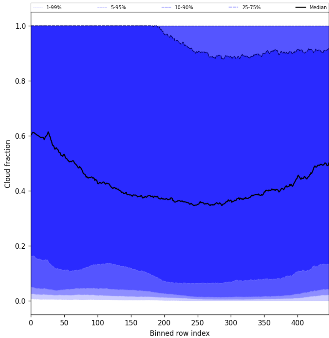
Figure 49: Along track statistics of “Cloud fraction” for 2025-11-20 to 2025-11-22
