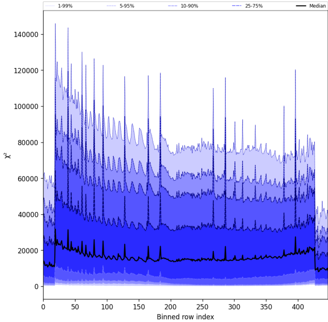
Figure 55: Along track statistics of “ \chi^2 ” for 2025-11-20 to 2025-11-22
