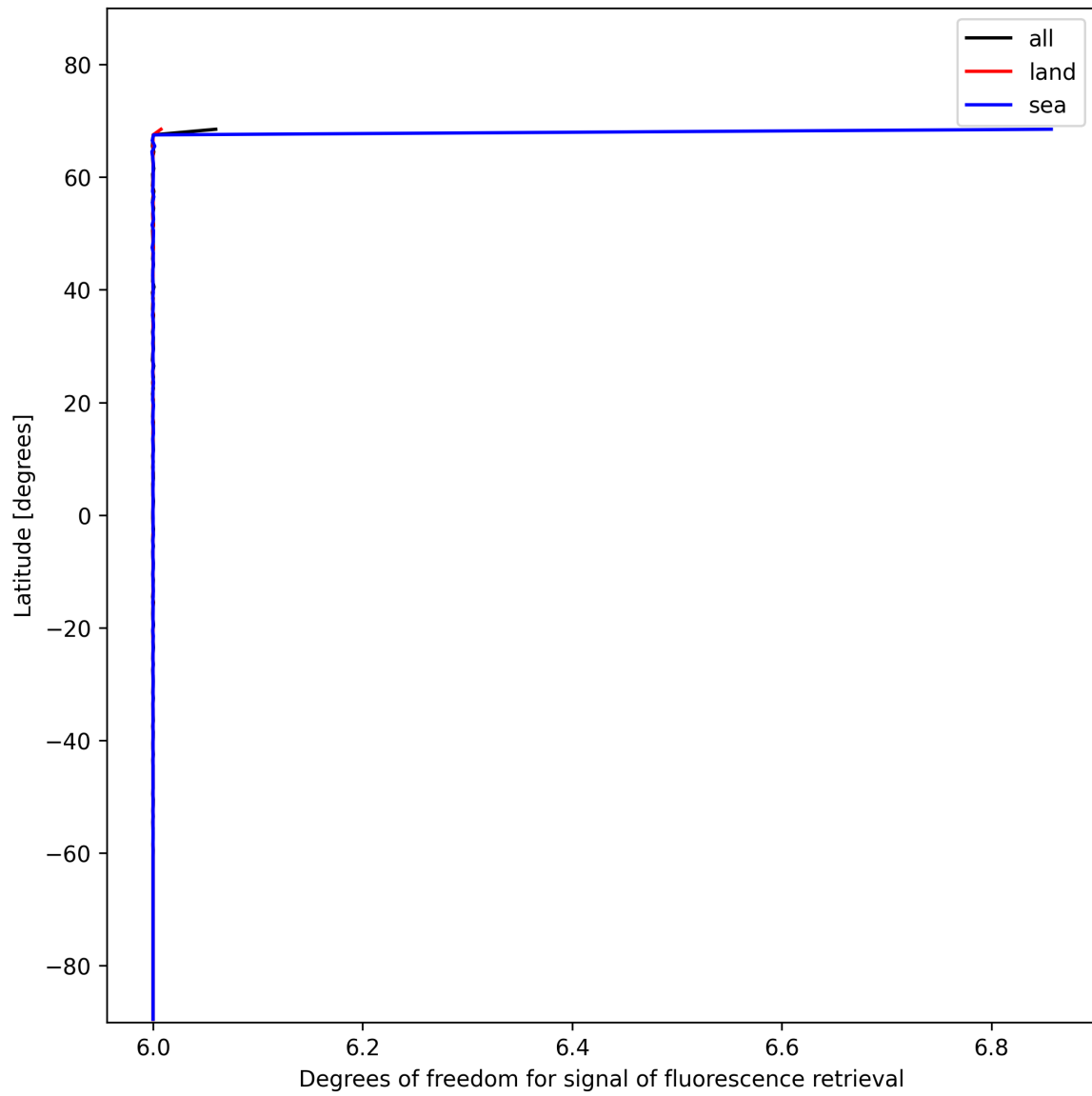
Figure 26: Zonal average of “Degrees of freedom for signal of fluorescence retrieval” for 2025-11-20 to 2025-11-22.
