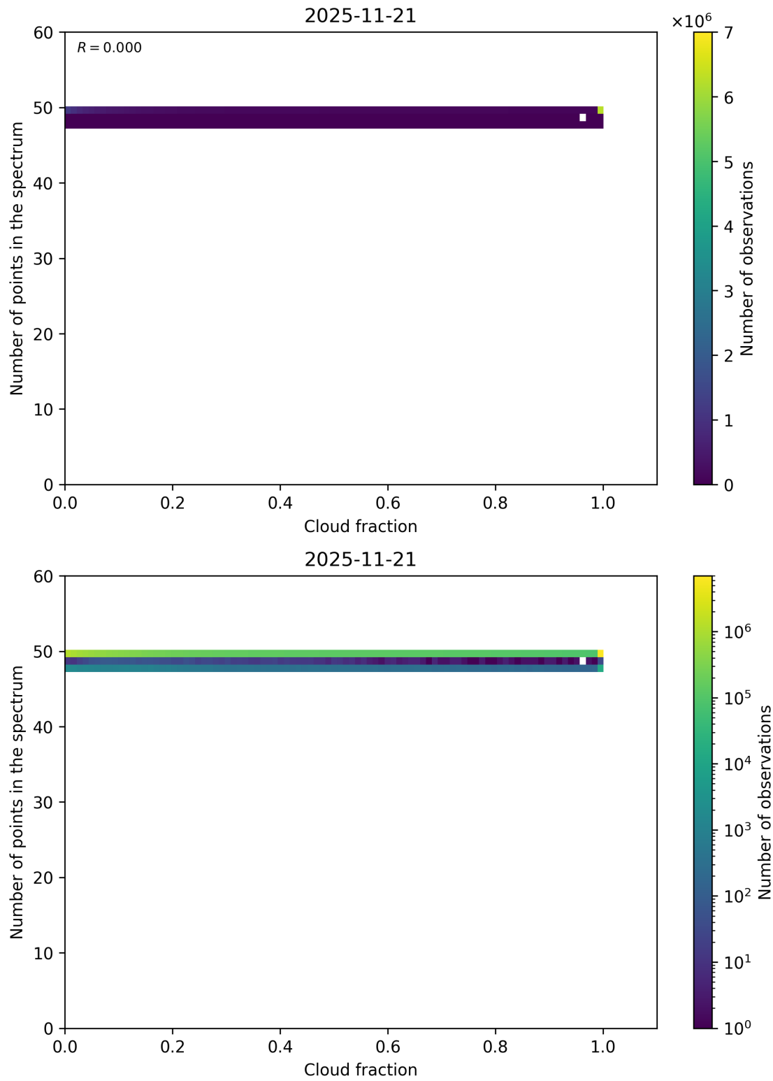
Figure 74: Scatter density plot of “Cloud fraction” against “Number of points in the spectrum” for 2025-11-20 to 2025-11-22.
