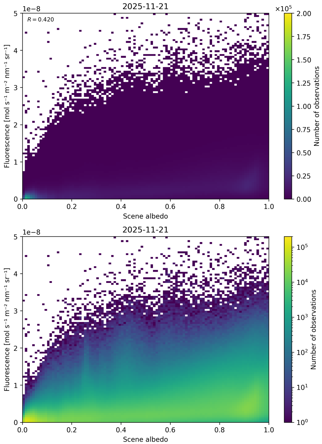
Figure 104: Scatter density plot of “Scene albedo” against “Fluorescence” for 2025-11-20 to 2025-11-22.
