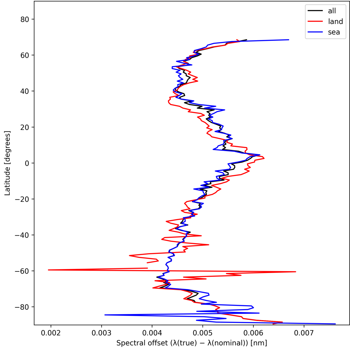
Figure 28: Zonal average of “Spectral offset ( \lambda_{\text{true}} - \lambda_{\text{nominal}} )” for 2025-11-20 to 2025-11-22.
