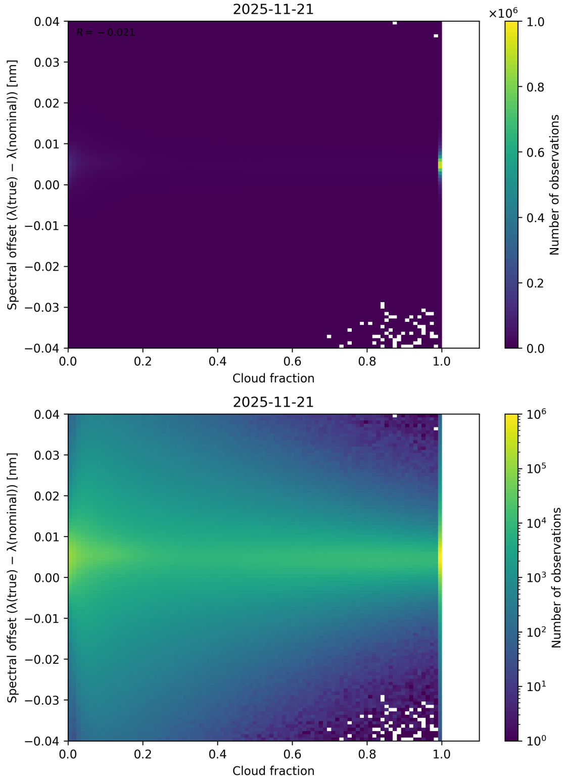
Figure 76: Scatter density plot of “Cloud fraction” against “Spectral offset ( \lambda_{\text{true}} - \lambda_{\text{nominal}} )” for 2025-11-20 to 2025-11-22.
