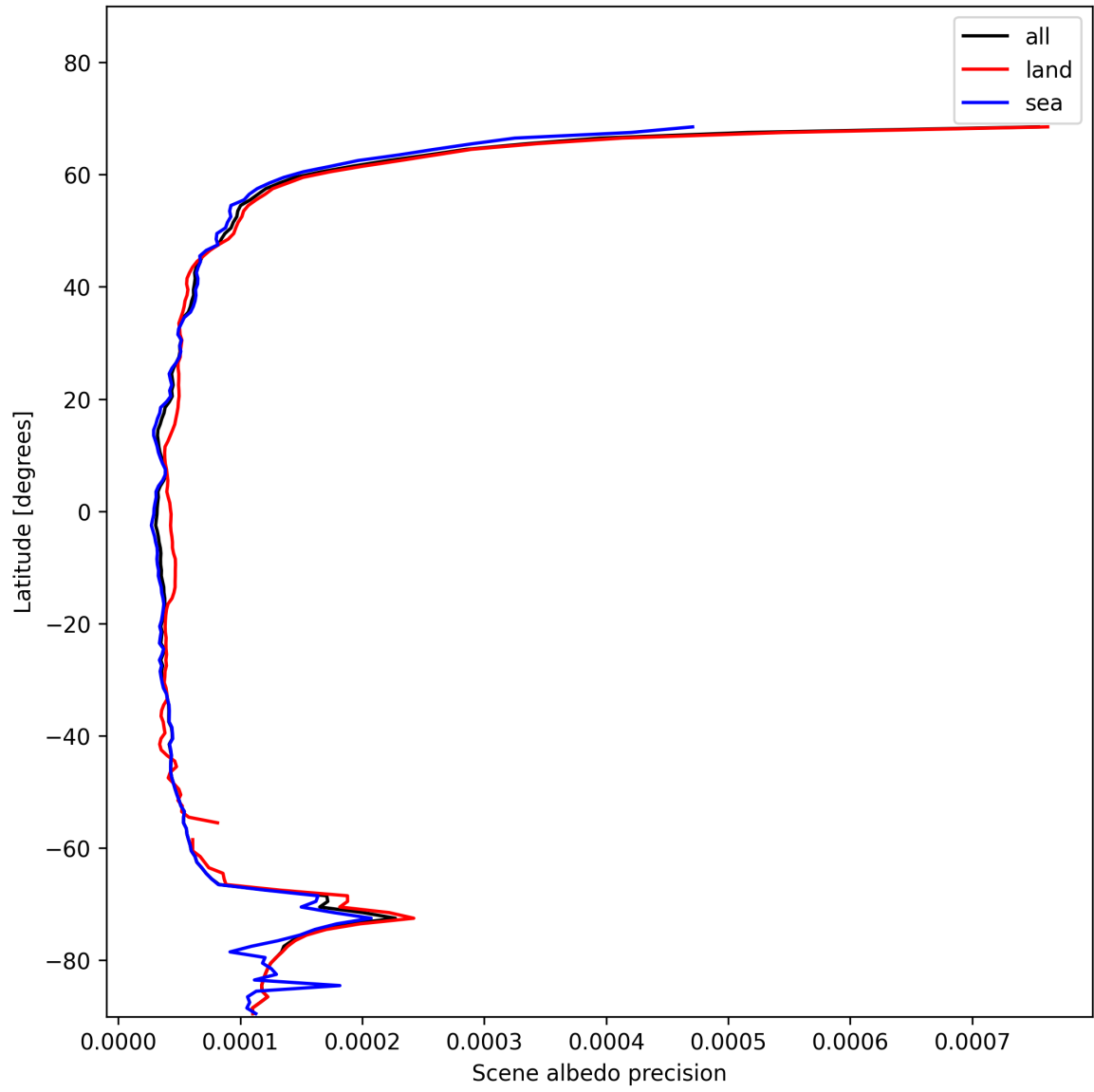
Figure 18: Zonal average of “Scene albedo precision” for 2025-11-20 to 2025-11-22.
