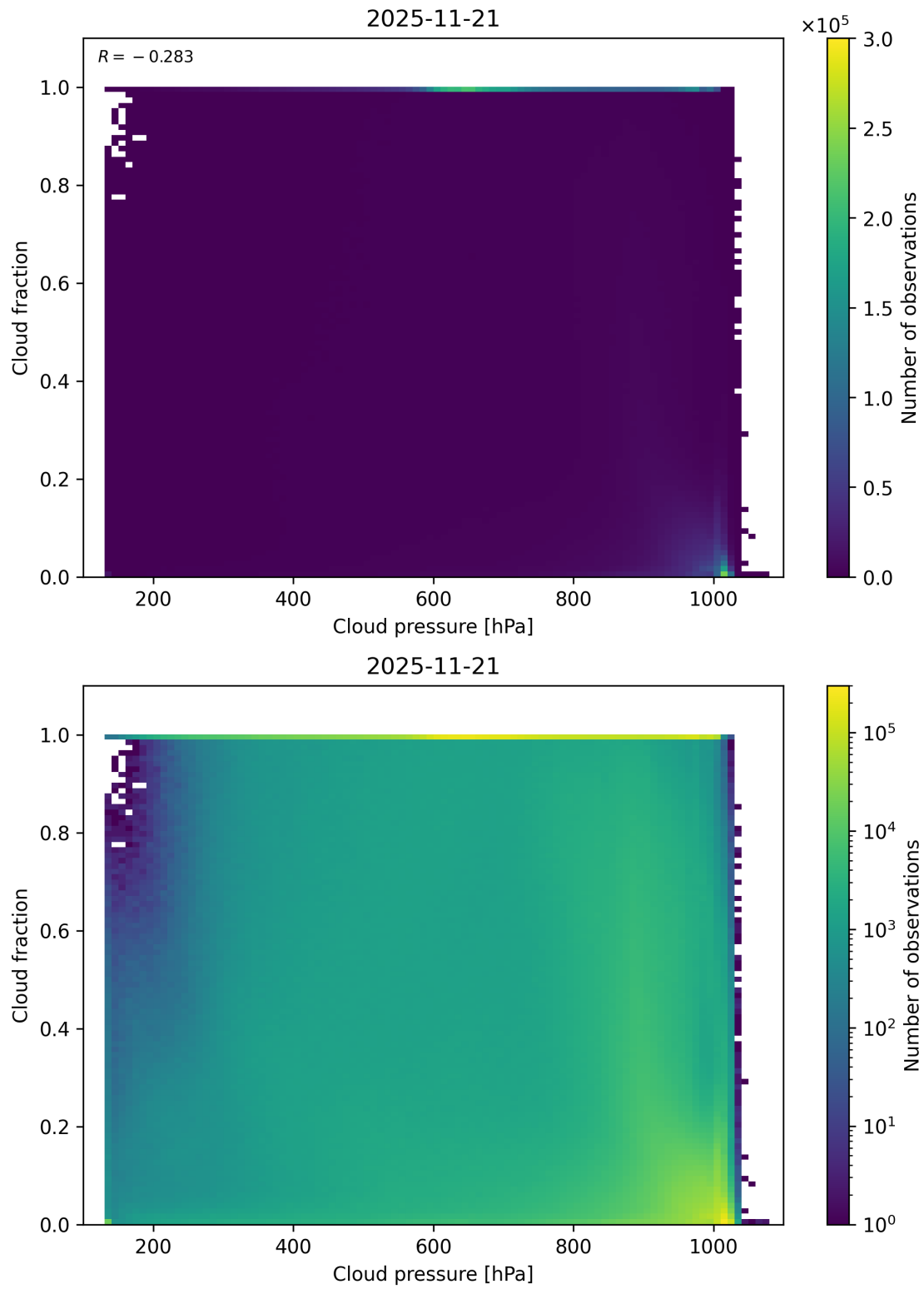
Figure 79: Scatter density plot of “Cloud pressure” against “Cloud fraction” for 2025-11-20 to 2025-11-22.
