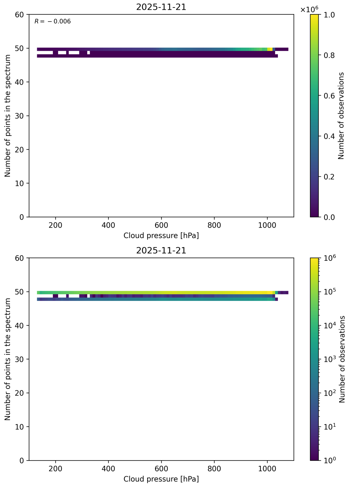
Figure 82: Scatter density plot of “Cloud pressure” against “Number of points in the spectrum” for 2025-11-20 to 2025-11-22.
