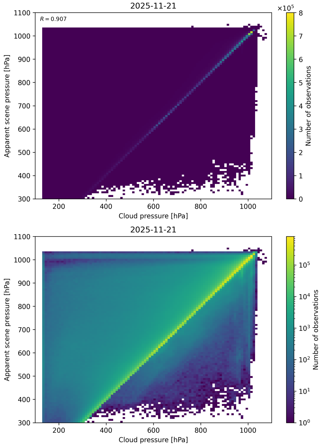
Figure 77: Scatter density plot of “Cloud pressure” against “Apparent scene pressure” for 2025-11-20 to 2025-11-22.
