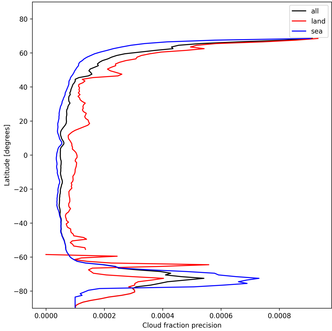
Figure 16: Zonal average of “Cloud fraction precision” for 2025-11-20 to 2025-11-22.
