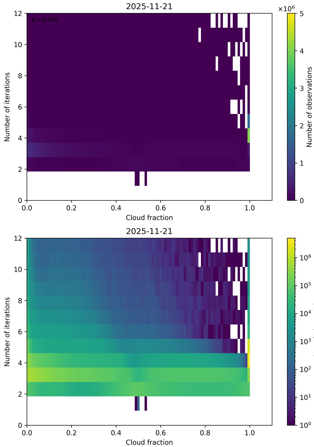
Figure 73: Scatter density plot of “Cloud fraction” against “Number of iterations” for 2025-11-20 to 2025-11-22.
