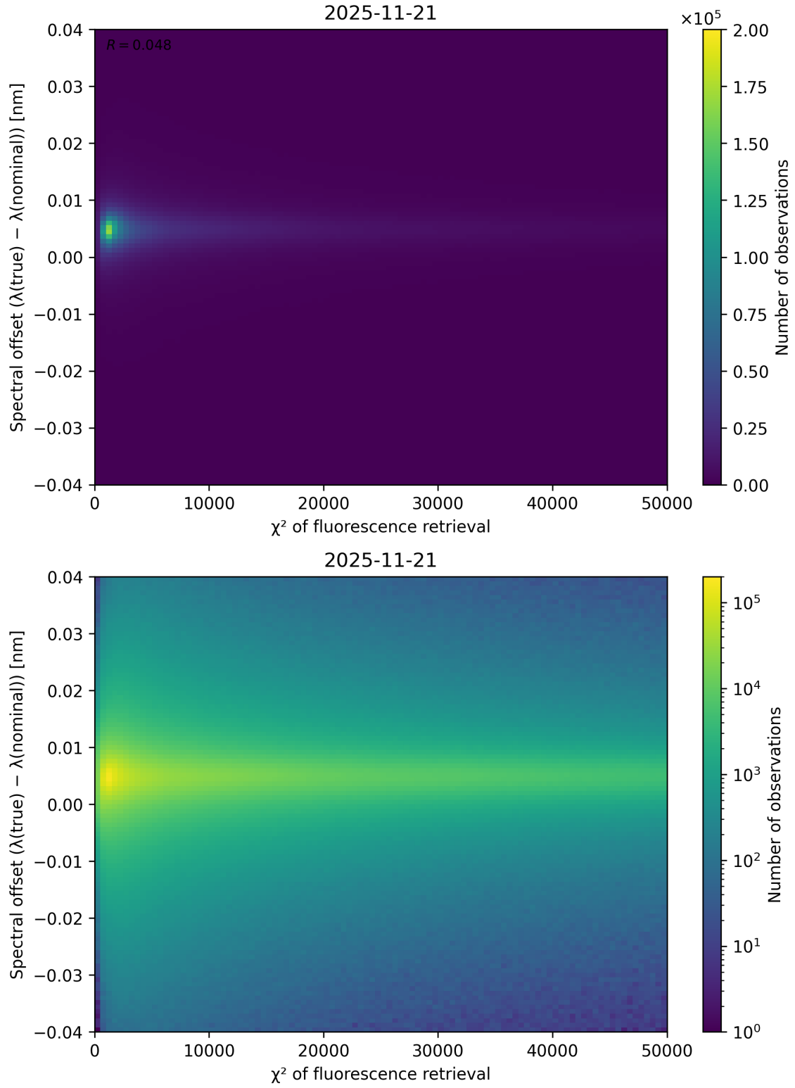
Figure 69: Scatter density plot of “ \chi^2 of fluorescence retrieval” against “Spectral offset ( \lambda_{\text{true}} - \lambda_{\text{nominal}} )” for 2025-11-20 to 2025-11-22.
