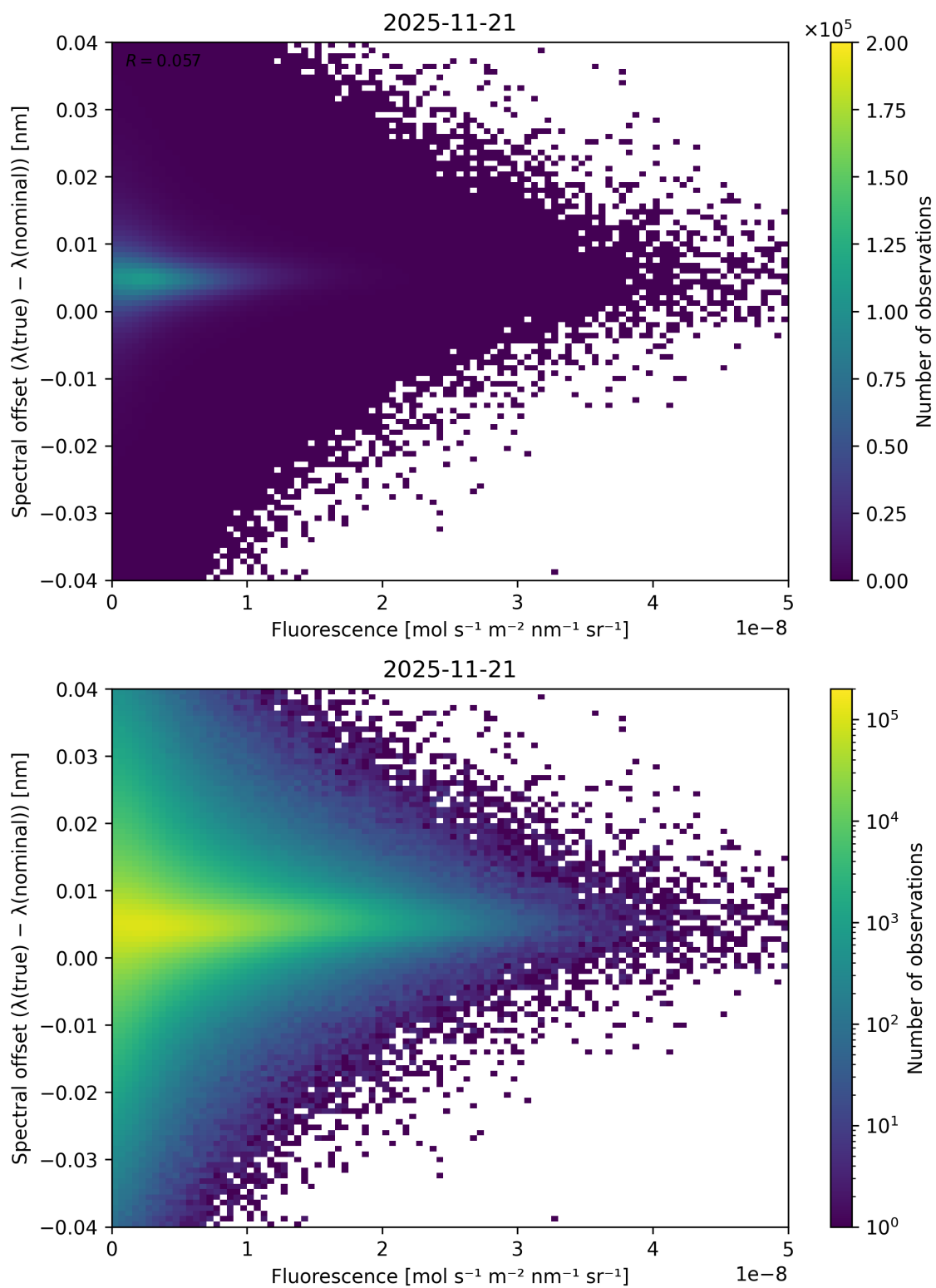
Figure 87: Scatter density plot of “Fluorescence” against “Spectral offset ( \lambda_{\text{true}} - \lambda_{\text{nominal}} )” for 2025-11-20 to 2025-11-22.
