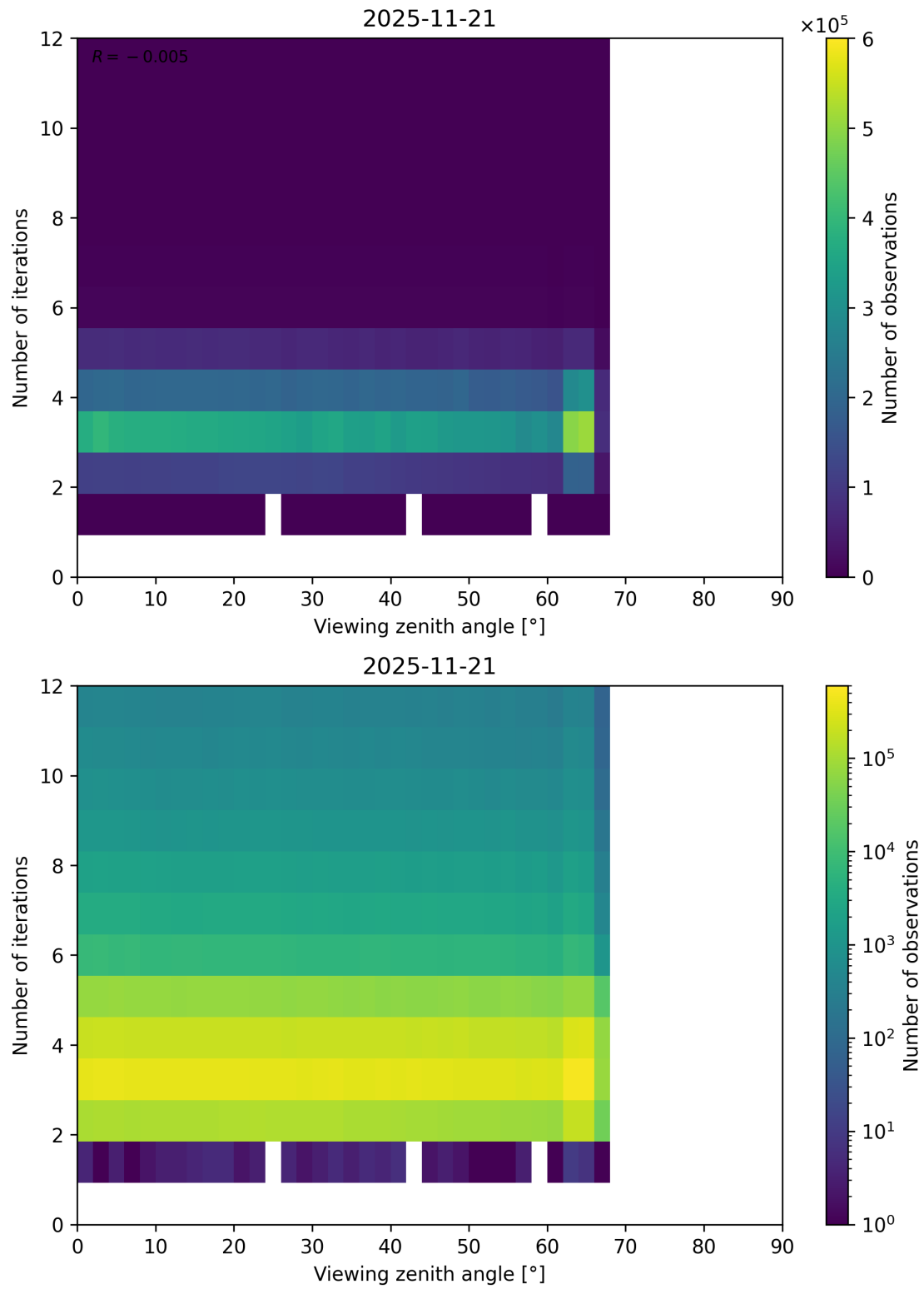
Figure 124: Scatter density plot of “Viewing zenith angle” against “Number of iterations” for 2025-11-20 to 2025-11-22.
