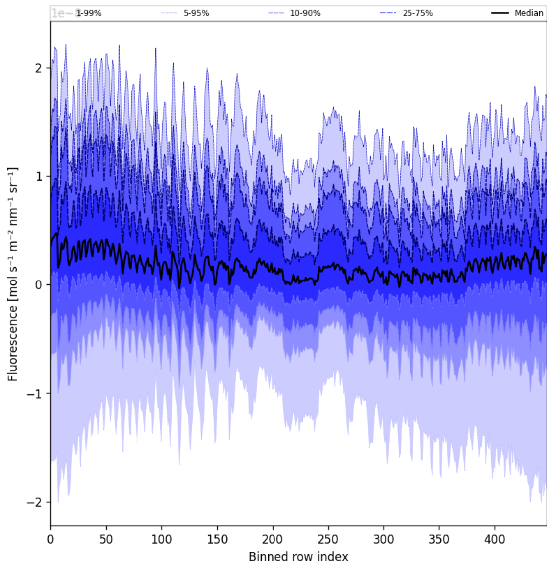
Figure 57: Along track statistics of “Fluorescence” for 2025-11-20 to 2025-11-22
