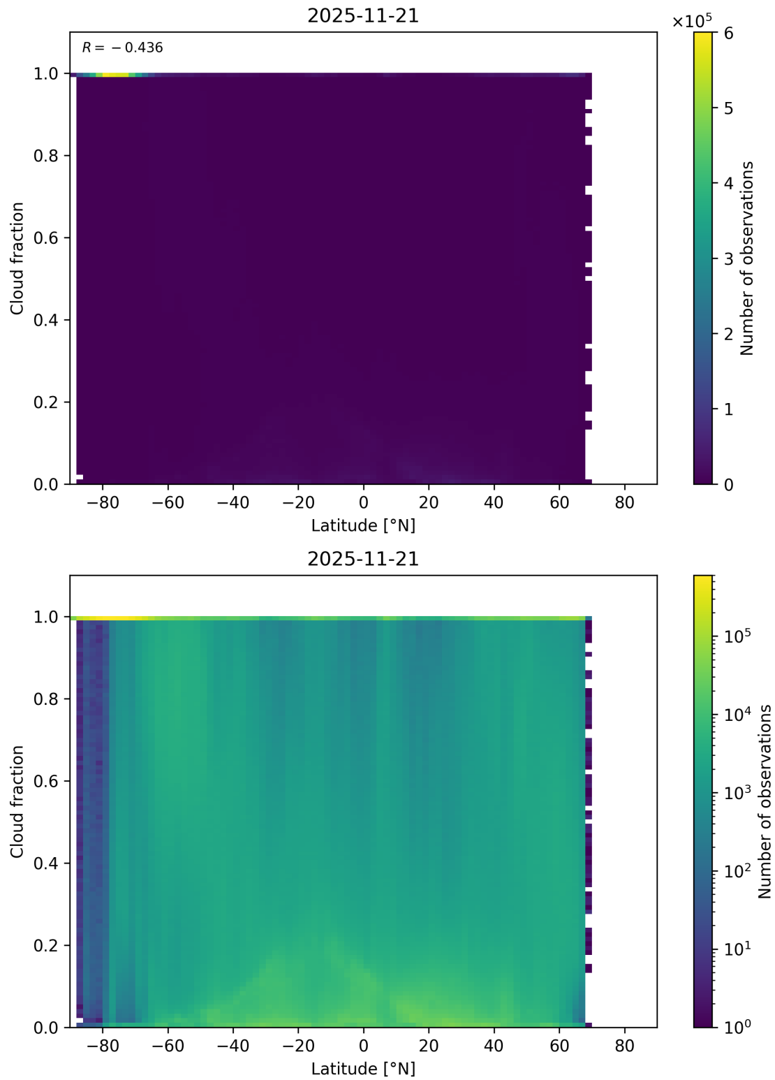
Figure 90: Scatter density plot of “Latitude” against “Cloud fraction” for 2025-11-20 to 2025-11-22.
