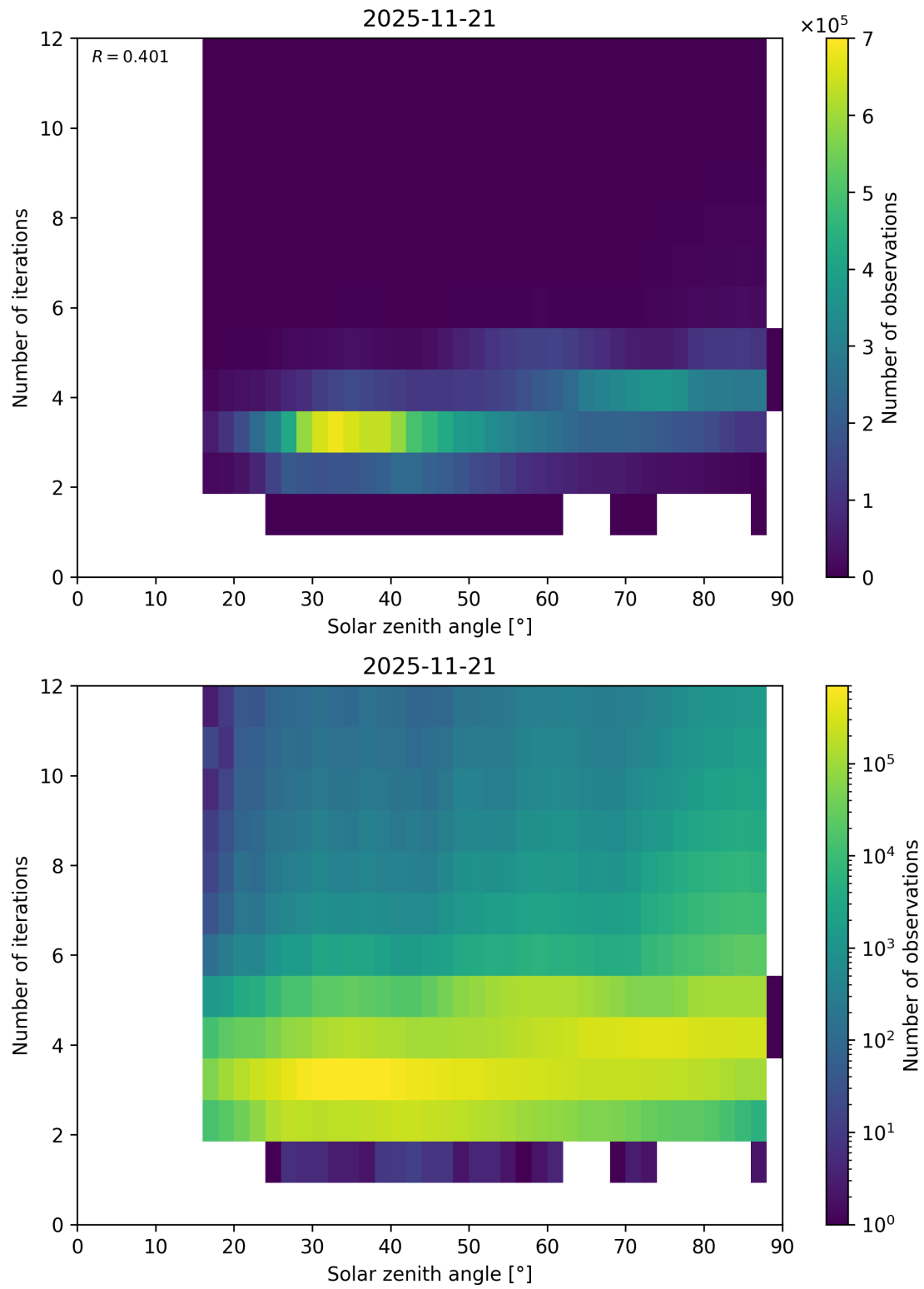
Figure 114: Scatter density plot of “Solar zenith angle” against “Number of iterations” for 2025-11-20 to 2025-11-22.
