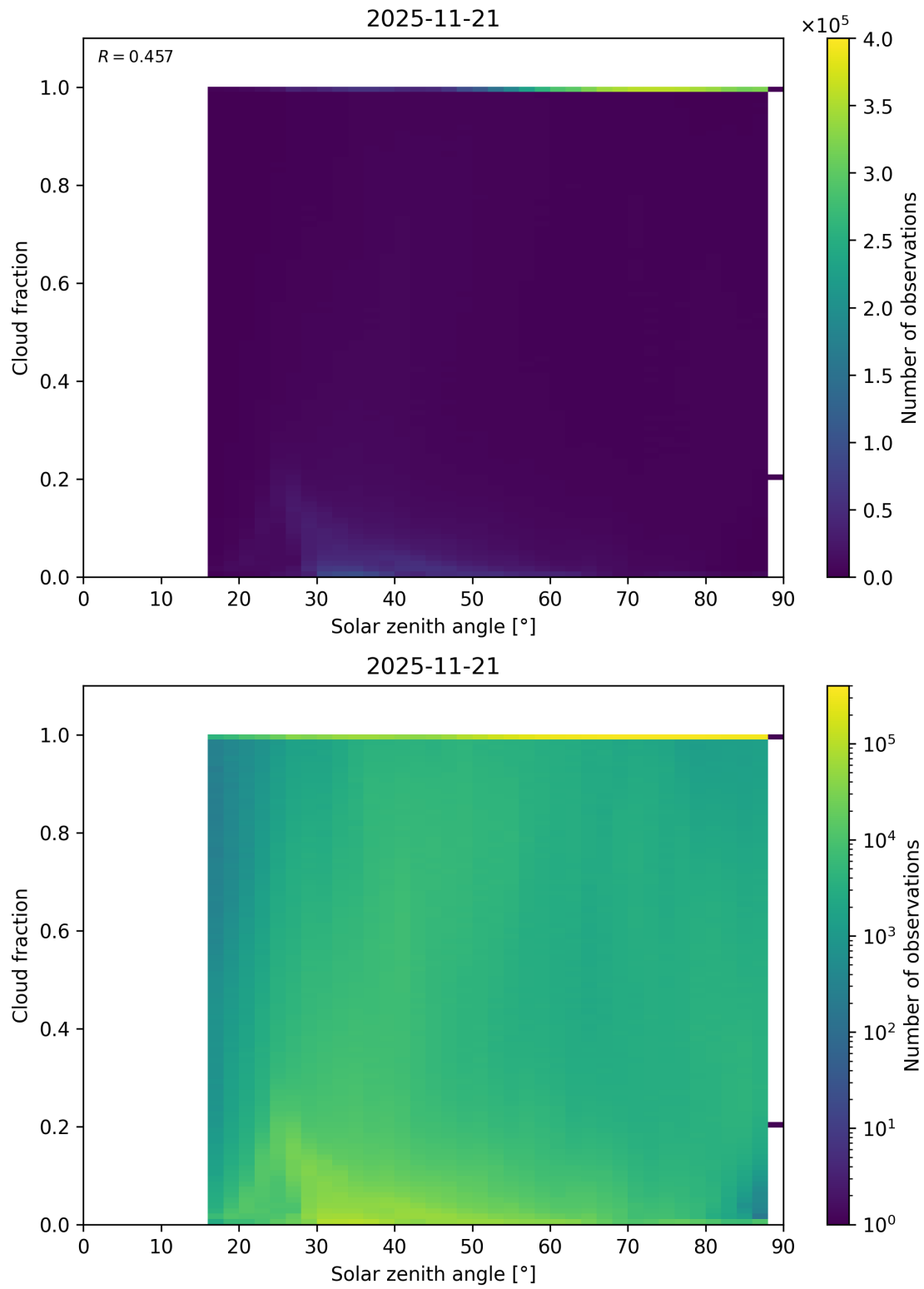
Figure 110: Scatter density plot of “Solar zenith angle” against “Cloud fraction” for 2025-11-20 to 2025-11-22.
