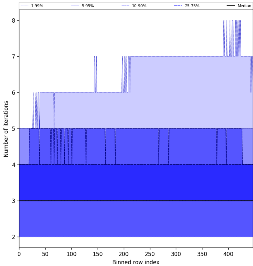
Figure 56: Along track statistics of “Number of iterations” for 2025-11-20 to 2025-11-22
