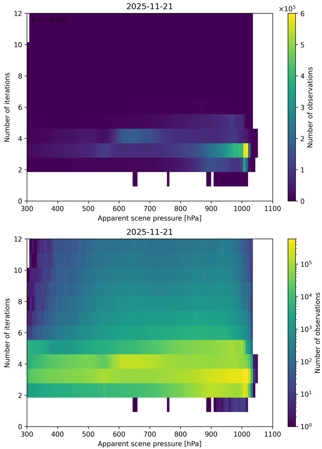
Figure 65: Scatter density plot of “Apparent scene pressure” against “Number of iterations” for 2025-11-20 to 2025-11-22.
