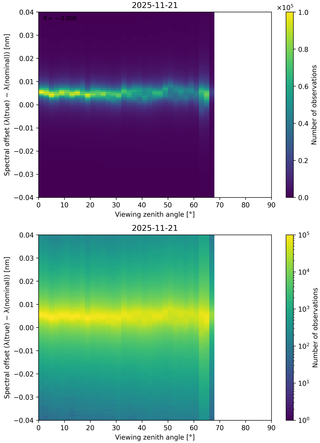
Figure 128: Scatter density plot of “Viewing zenith angle” against “Spectral offset ( \lambda_{\text{true}} - \lambda_{\text{nominal}} )” for 2025-11-20 to 2025-11-22.
