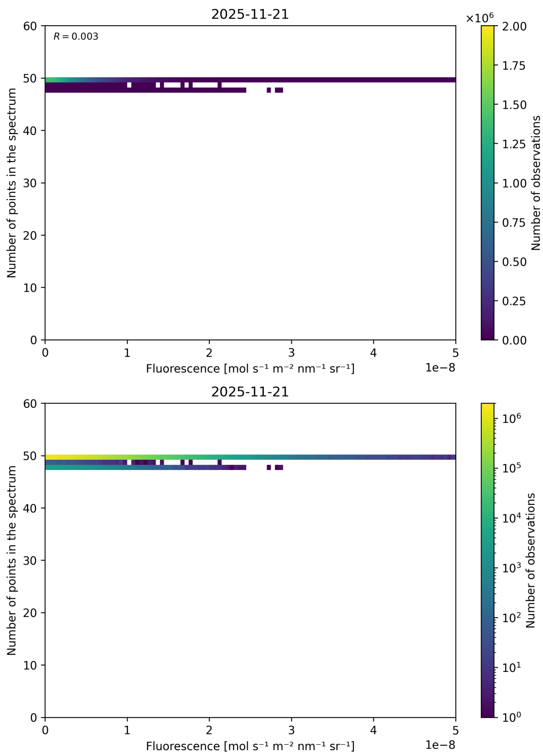
Figure 86: Scatter density plot of “Fluorescence” against “Number of points in the spectrum” for 2025-11-20 to 2025-11-22.
