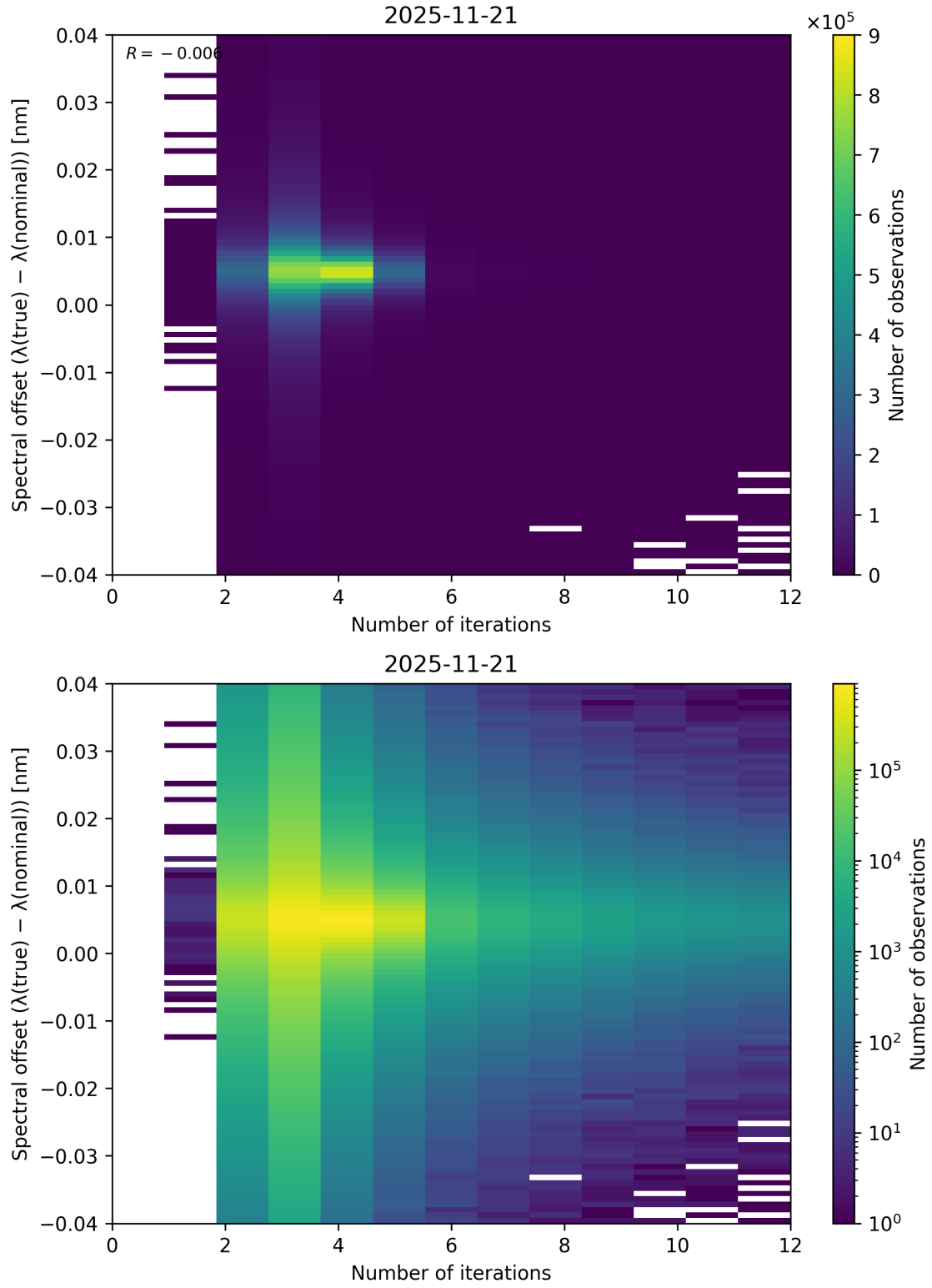
Figure 100: Scatter density plot of “Number of iterations” against “Spectral offset ( \lambda_{\text{true}} - \lambda_{\text{nominal}} )” for 2025-11-20 to 2025-11-22.
