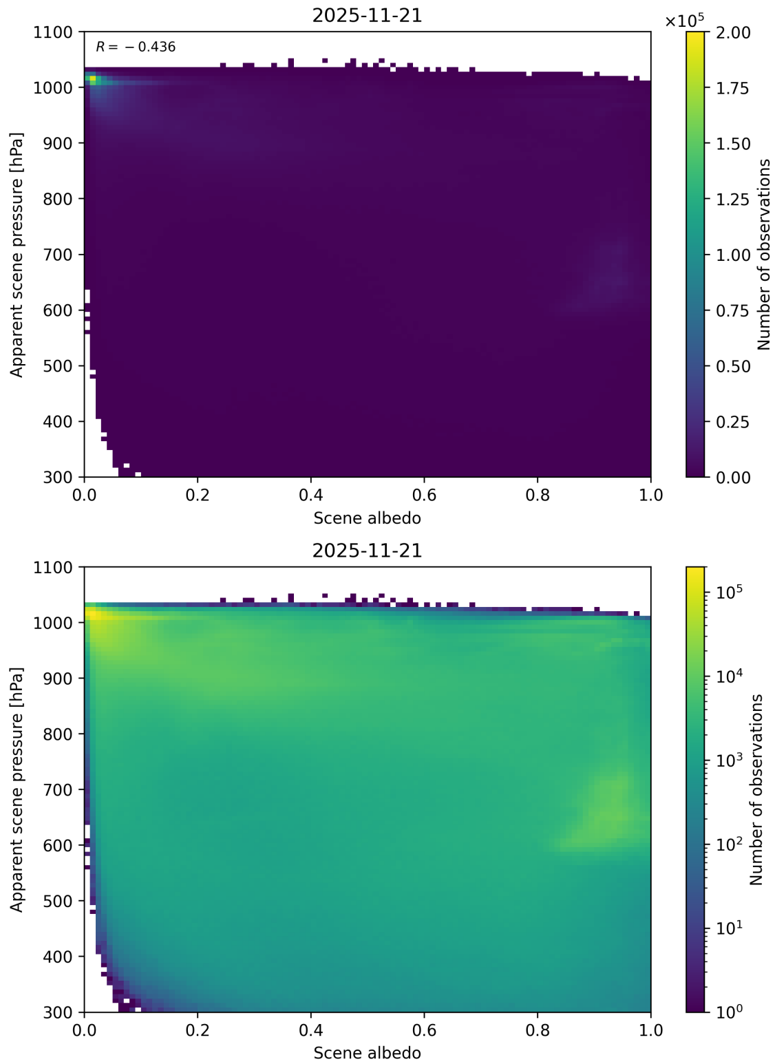
Figure 102: Scatter density plot of “Scene albedo” against “Apparent scene pressure” for 2025-11-20 to 2025-11-22.
