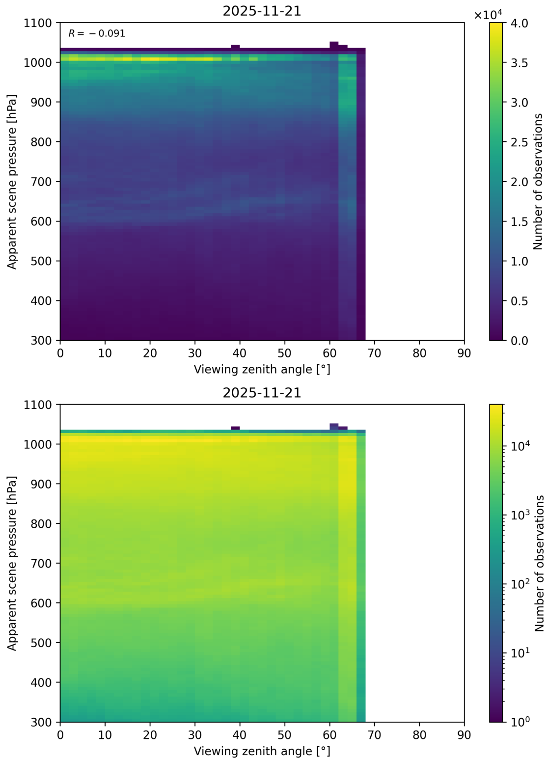
Figure 118: Scatter density plot of “Viewing zenith angle” against “Apparent scene pressure” for 2025-11-20 to 2025-11-22.
