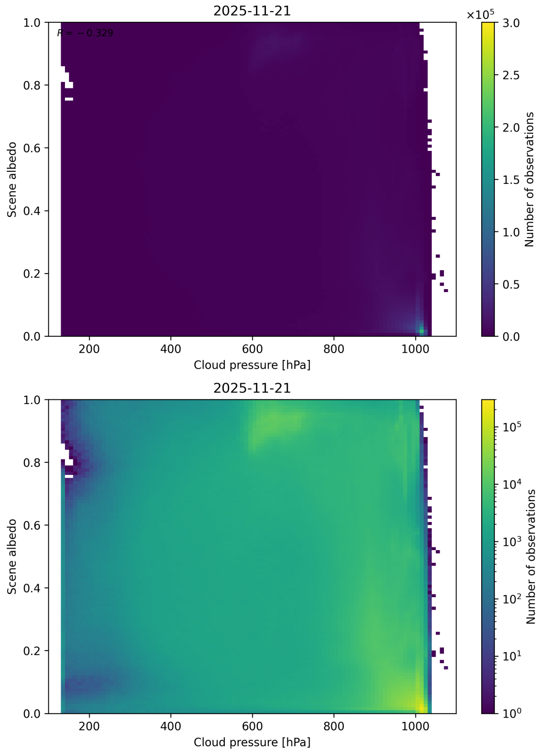
Figure 83: Scatter density plot of “Cloud pressure” against “Scene albedo” for 2025-11-20 to 2025-11-22.
