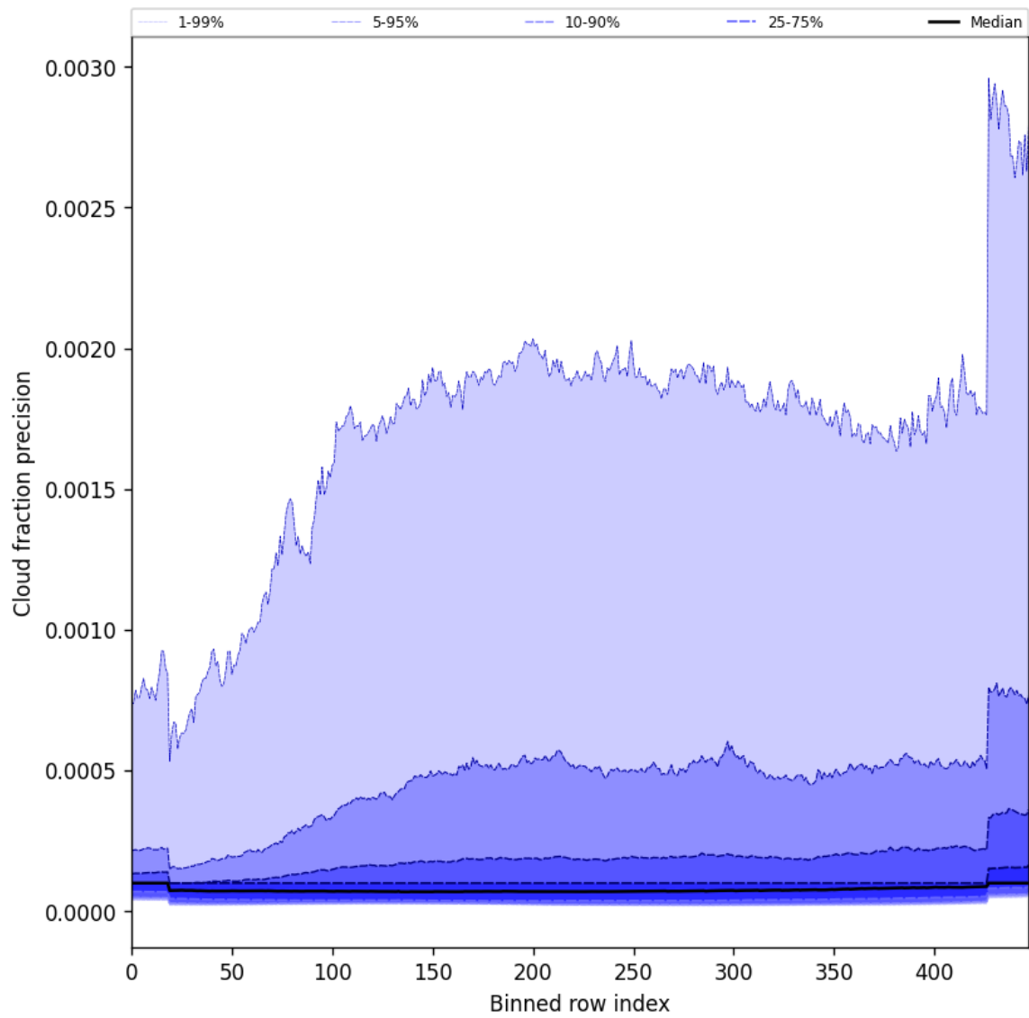
Figure 50: Along track statistics of “Cloud fraction precision” for 2025-11-20 to 2025-11-22
