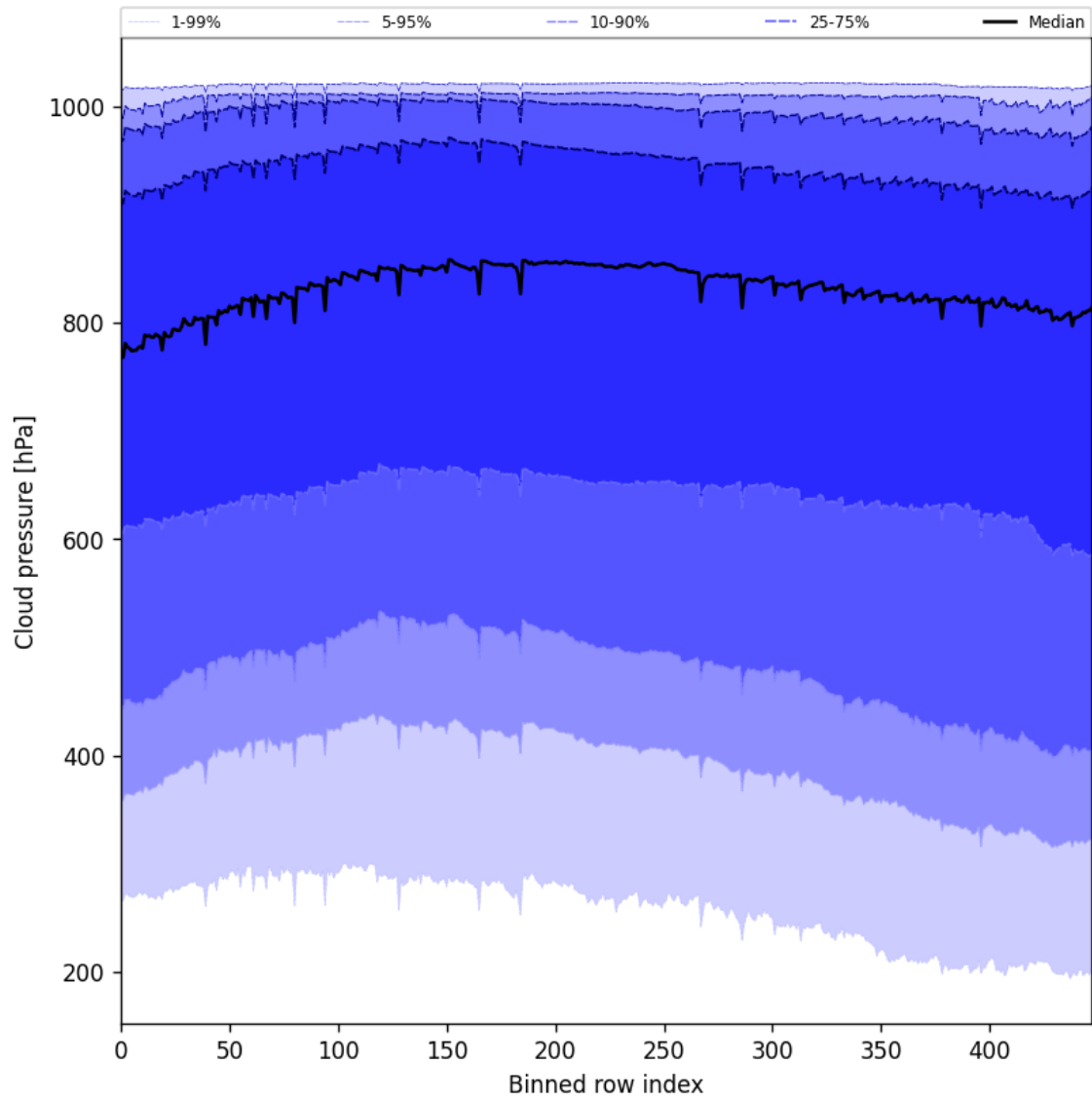
Figure 47: Along track statistics of “Cloud pressure” for 2025-11-20 to 2025-11-22
