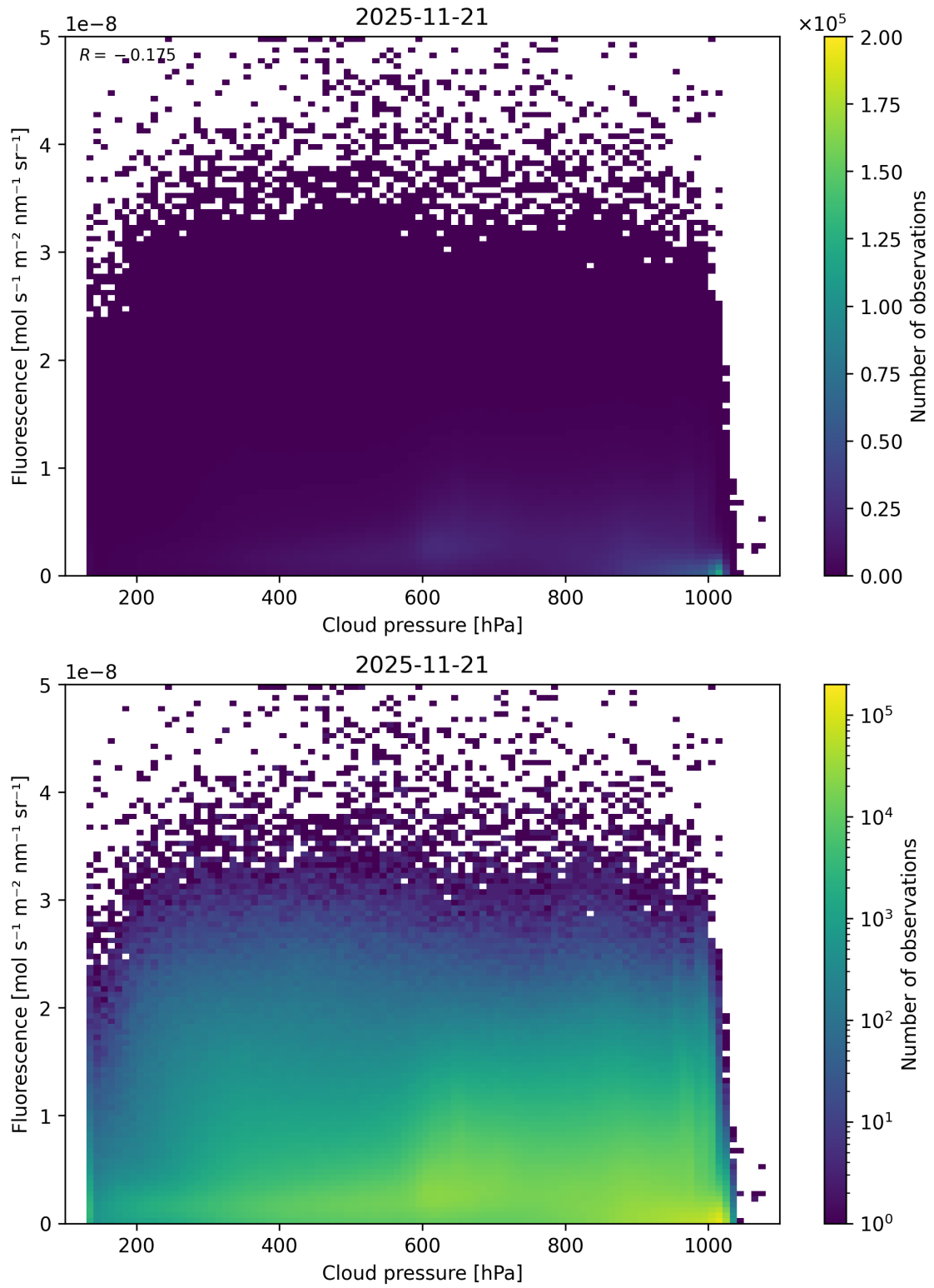
Figure 80: Scatter density plot of “Cloud pressure” against “Fluorescence” for 2025-11-20 to 2025-11-22.
