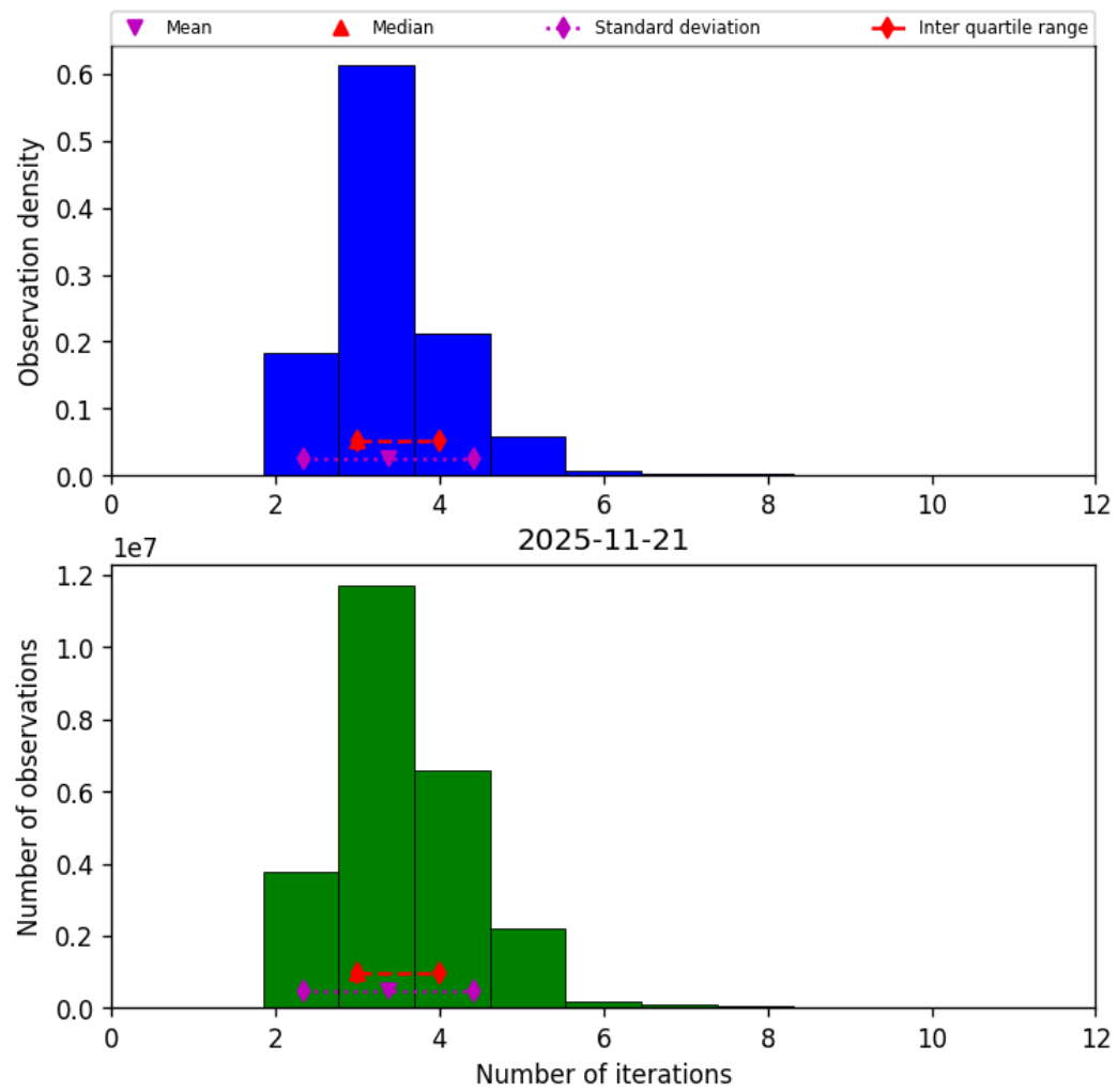
Figure 39: Histogram of “Number of iterations” for 2025-11-20 to 2025-11-22
