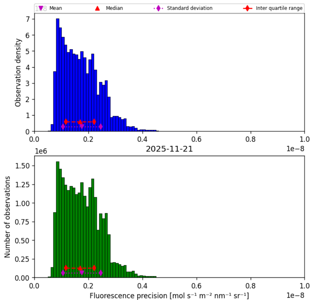
Figure 41: Histogram of “Fluorescence precision” for 2025-11-20 to 2025-11-22
