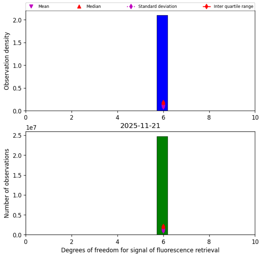
Figure 43: Histogram of "Degrees of freedom for signal of fluorescence retrieval" for 2025-11-20 to 2025-11-22
