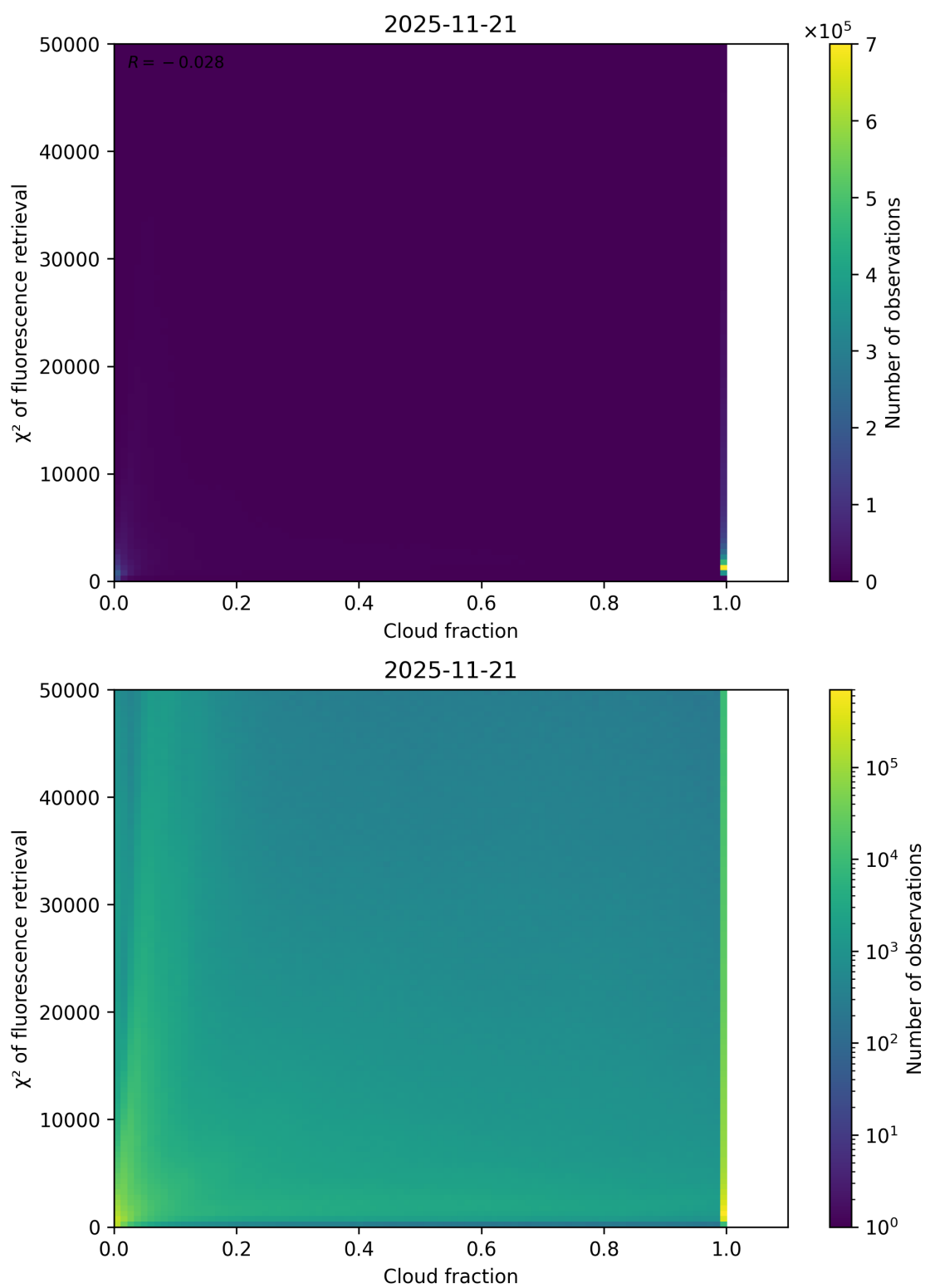
Figure 71: Scatter density plot of “Cloud fraction” against “ \chi^2 of fluorescence retrieval” for 2025-11-20 to 2025-11-22.
