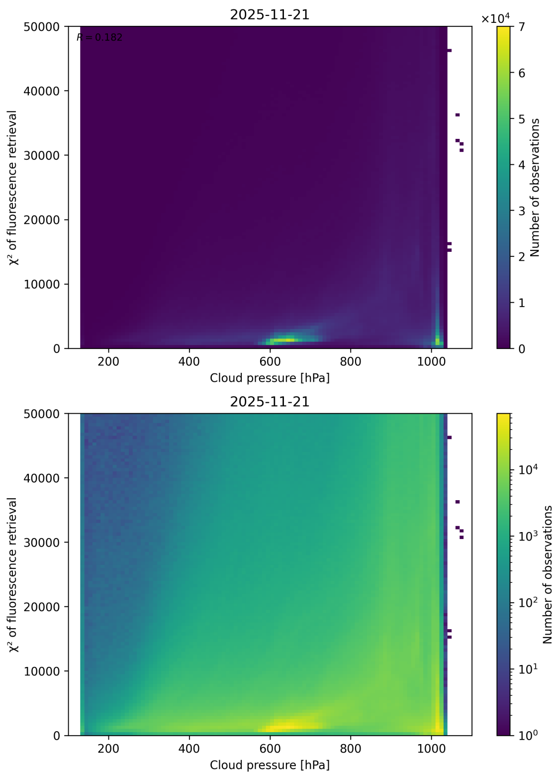
Figure 78: Scatter density plot of “Cloud pressure” against “ \chi^2 of fluorescence retrieval” for 2025-11-20 to 2025-11-22.
