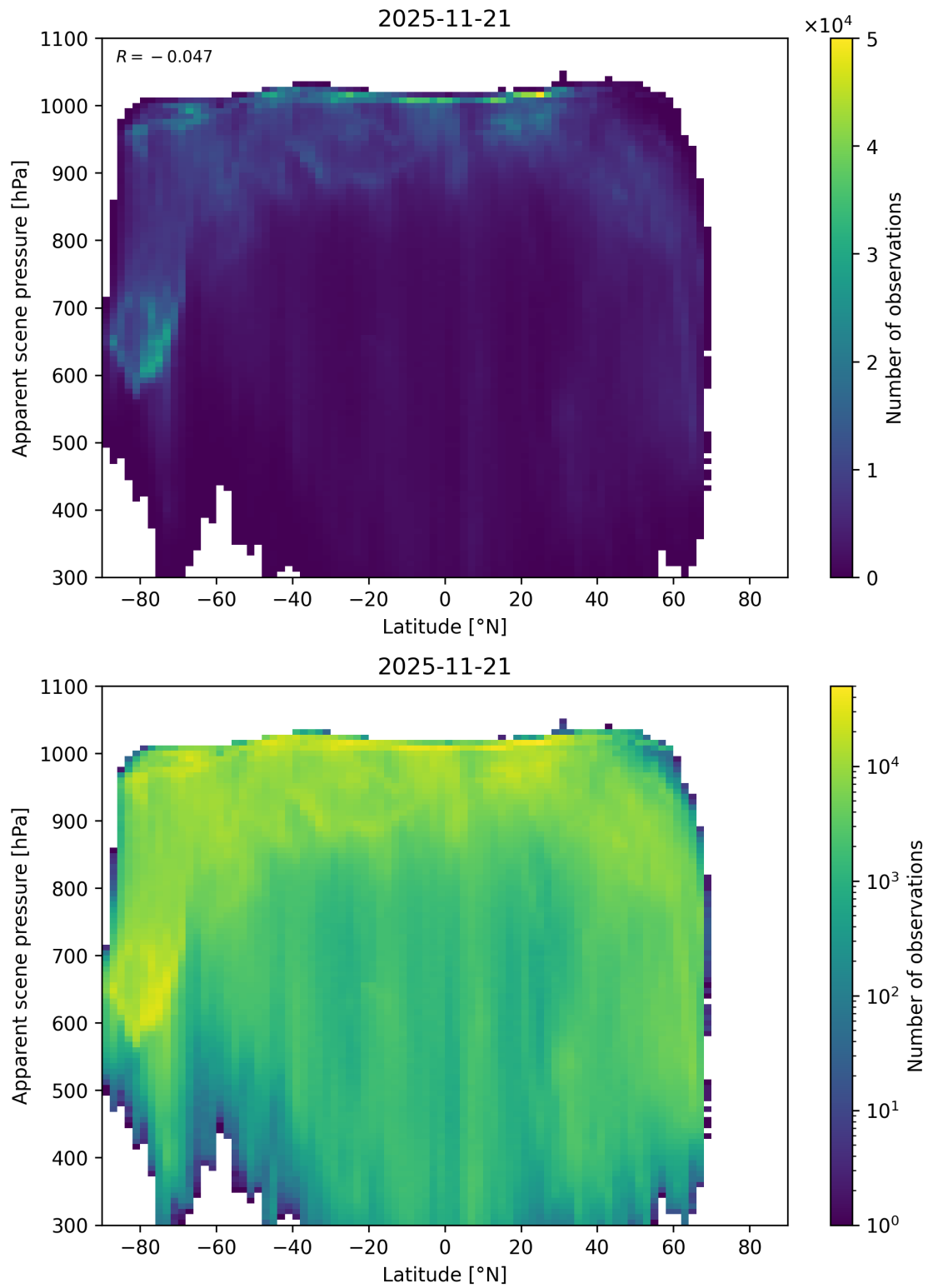
Figure 88: Scatter density plot of “Latitude” against “Apparent scene pressure” for 2025-11-20 to 2025-11-22.
