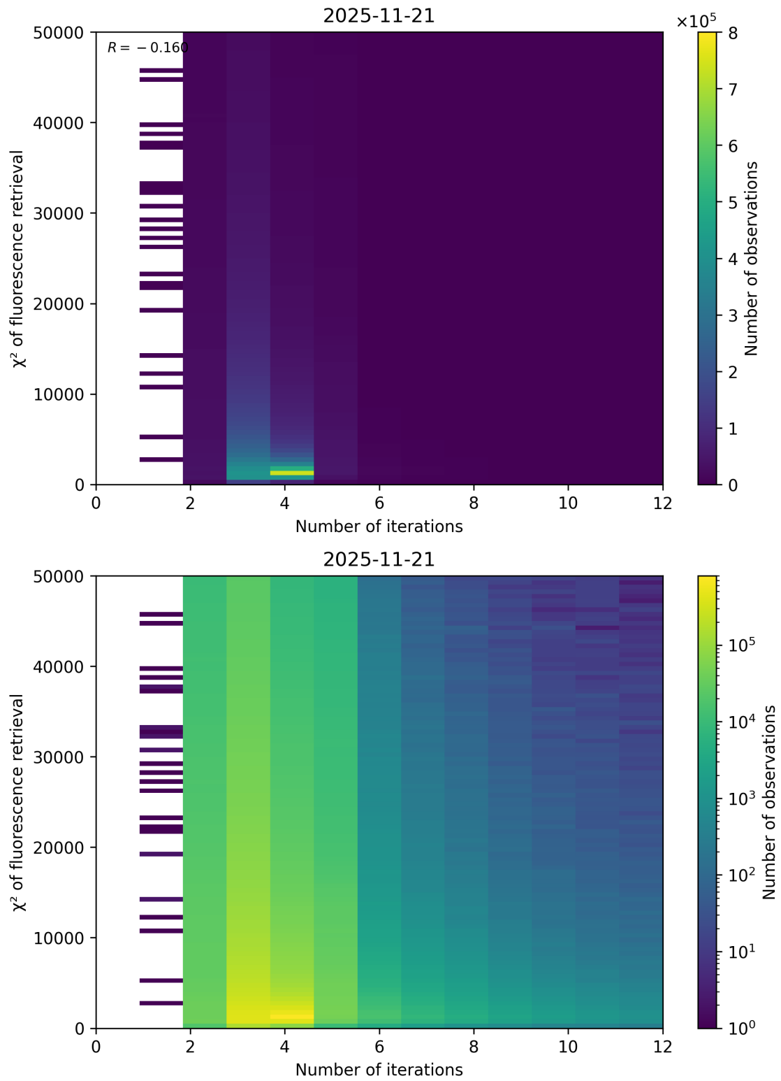
Figure 97: Scatter density plot of “Number of iterations” against “ \chi^2 of fluorescence retrieval” for 2025-11-20 to 2025-11-22.
