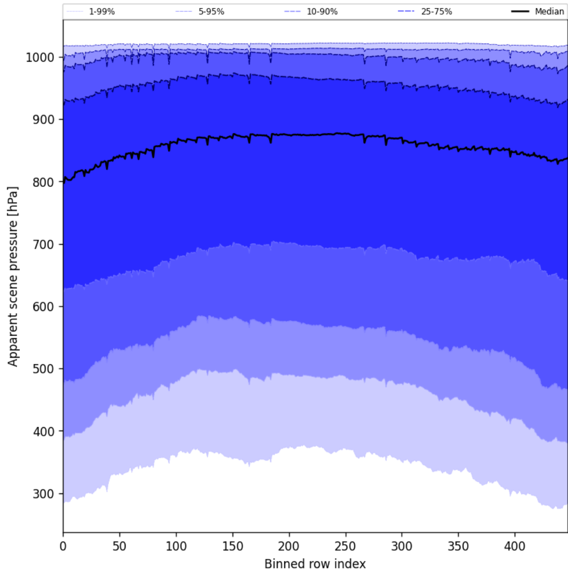
Figure 53: Along track statistics of “Apparent scene pressure” for 2025-11-20 to 2025-11-22
