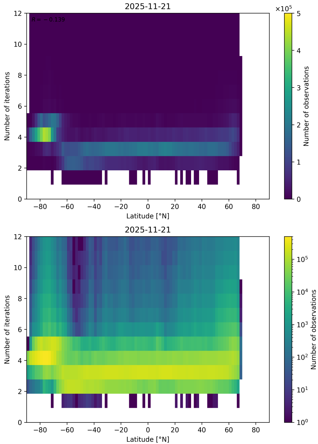
Figure 93: Scatter density plot of “Latitude” against “Number of iterations” for 2025-11-20 to 2025-11-22.
