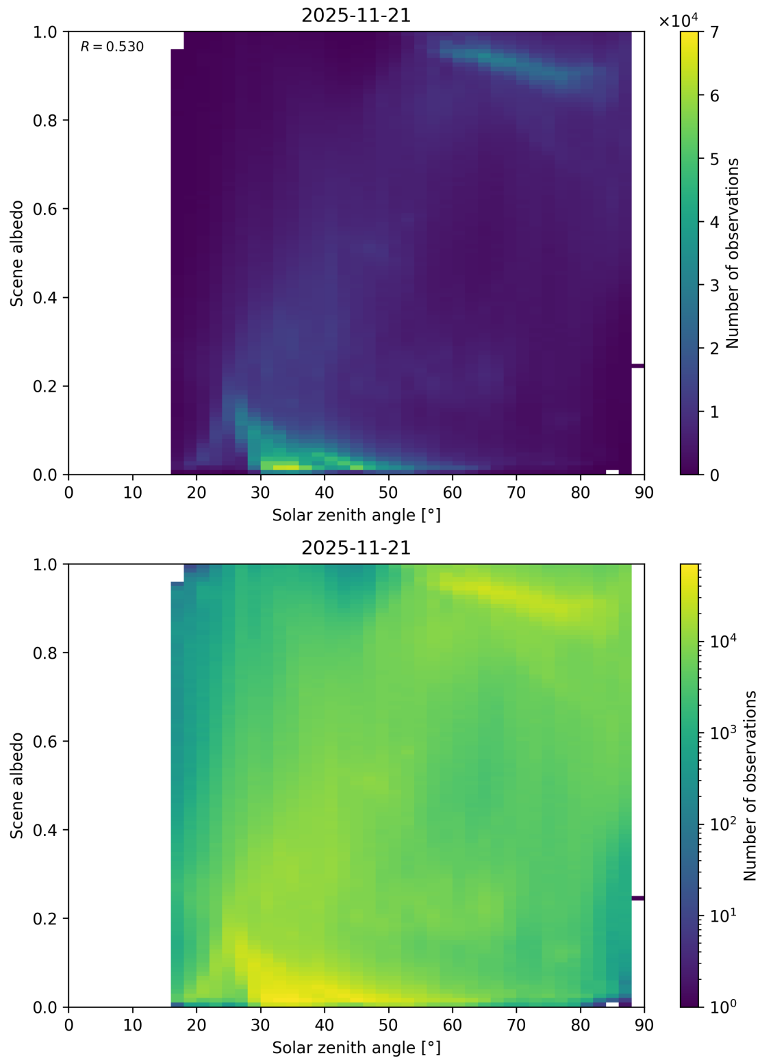
Figure 116: Scatter density plot of “Solar zenith angle” against “Scene albedo” for 2025-11-20 to 2025-11-22.
