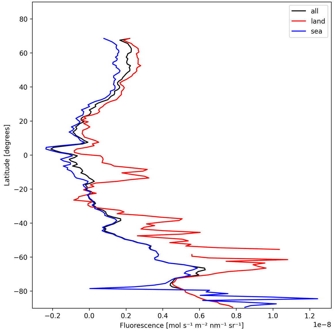
Figure 23: Zonal average of “Fluorescence” for 2025-11-20 to 2025-11-22.
