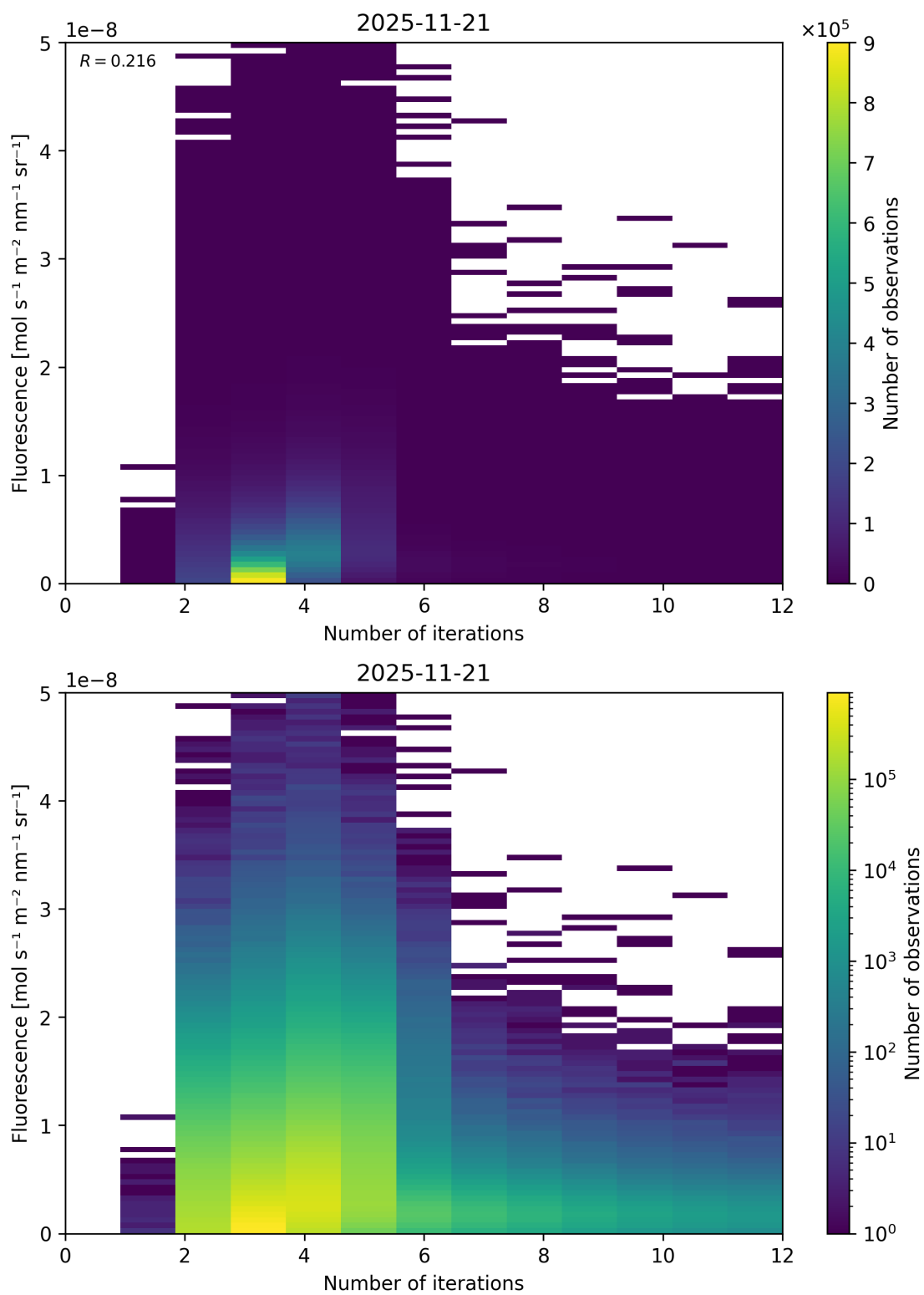
Figure 98: Scatter density plot of “Number of iterations” against “Fluorescence” for 2025-11-20 to 2025-11-22.
