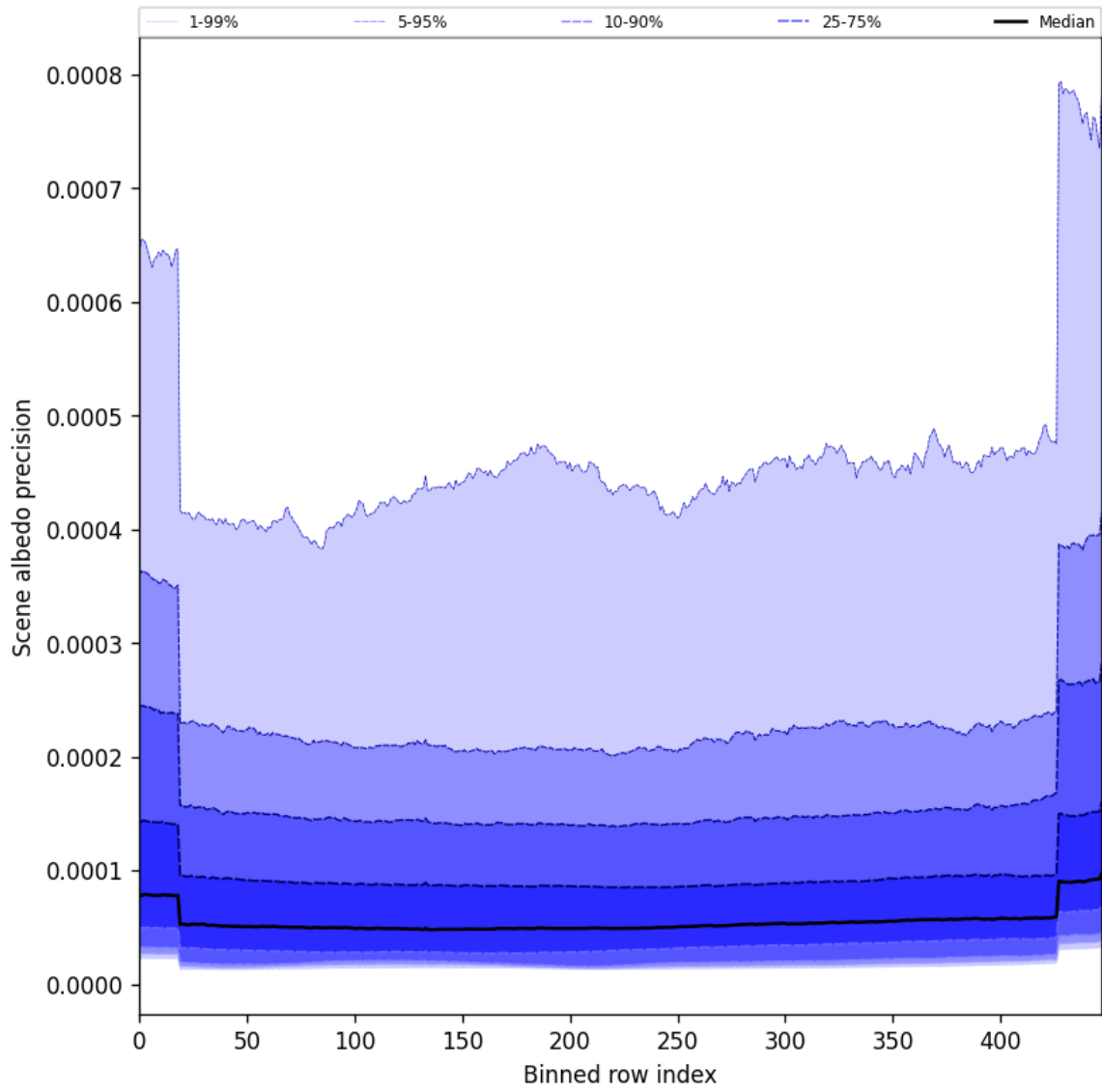
Figure 52: Along track statistics of “Scene albedo precision” for 2025-11-20 to 2025-11-22
