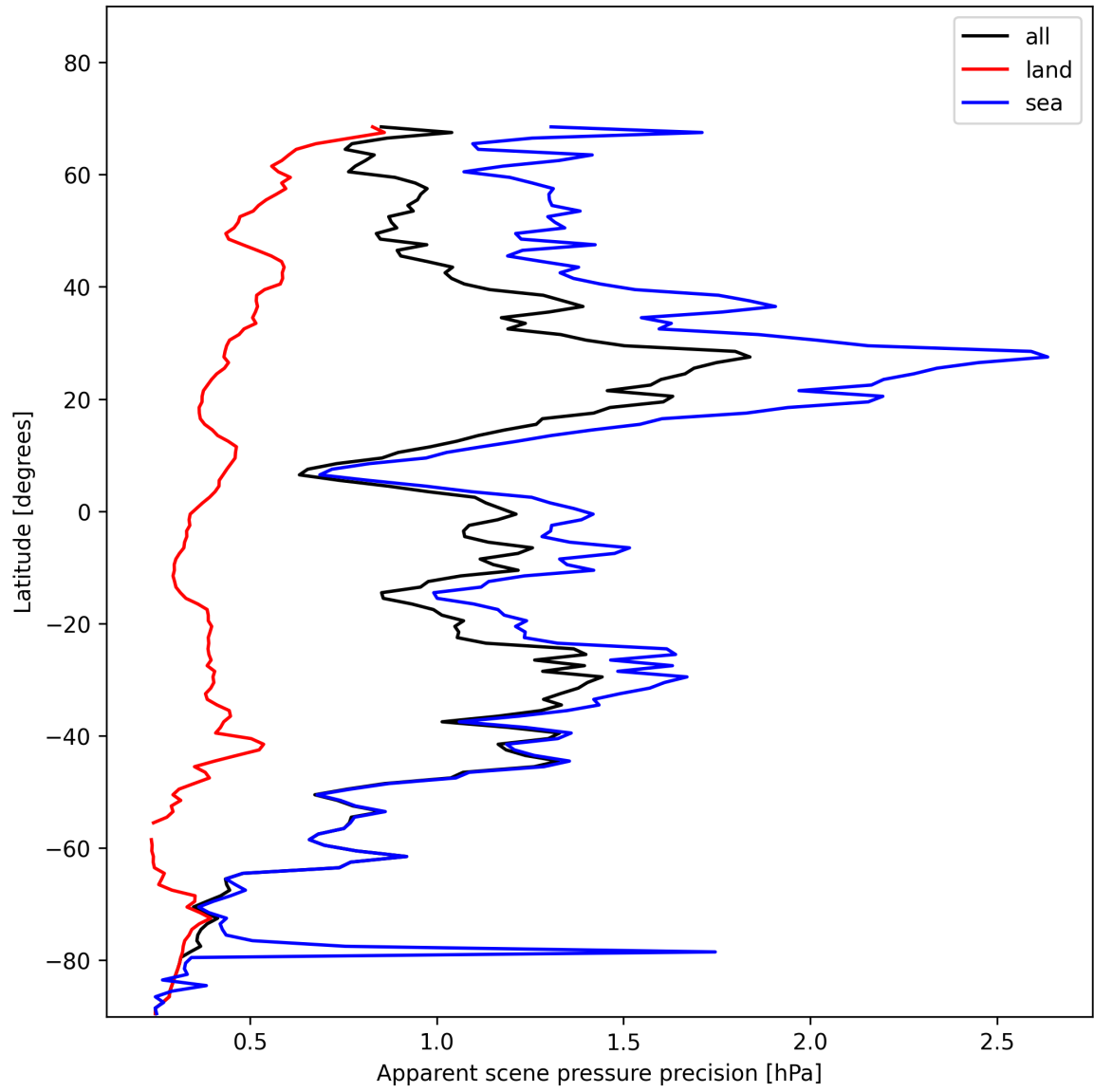
Figure 20: Zonal average of “Apparent scene pressure precision” for 2025-11-20 to 2025-11-22.
