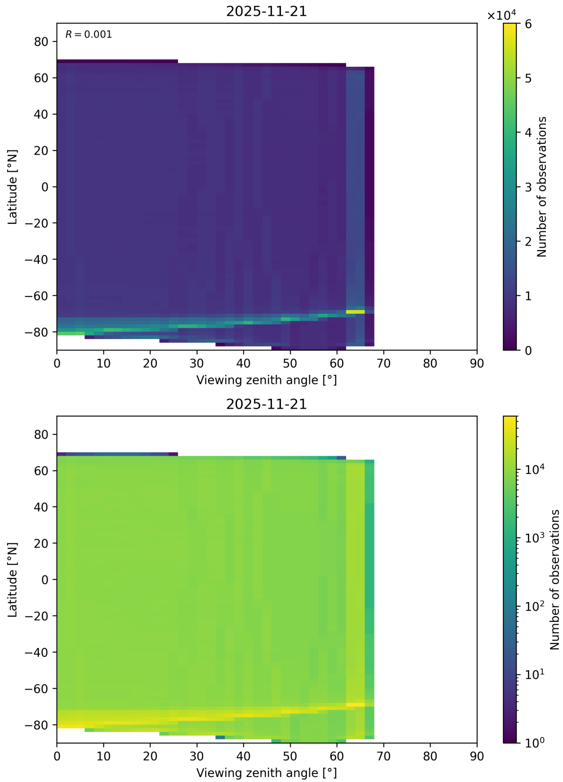
Figure 123: Scatter density plot of “Viewing zenith angle” against “Latitude” for 2025-11-20 to 2025-11-22.
