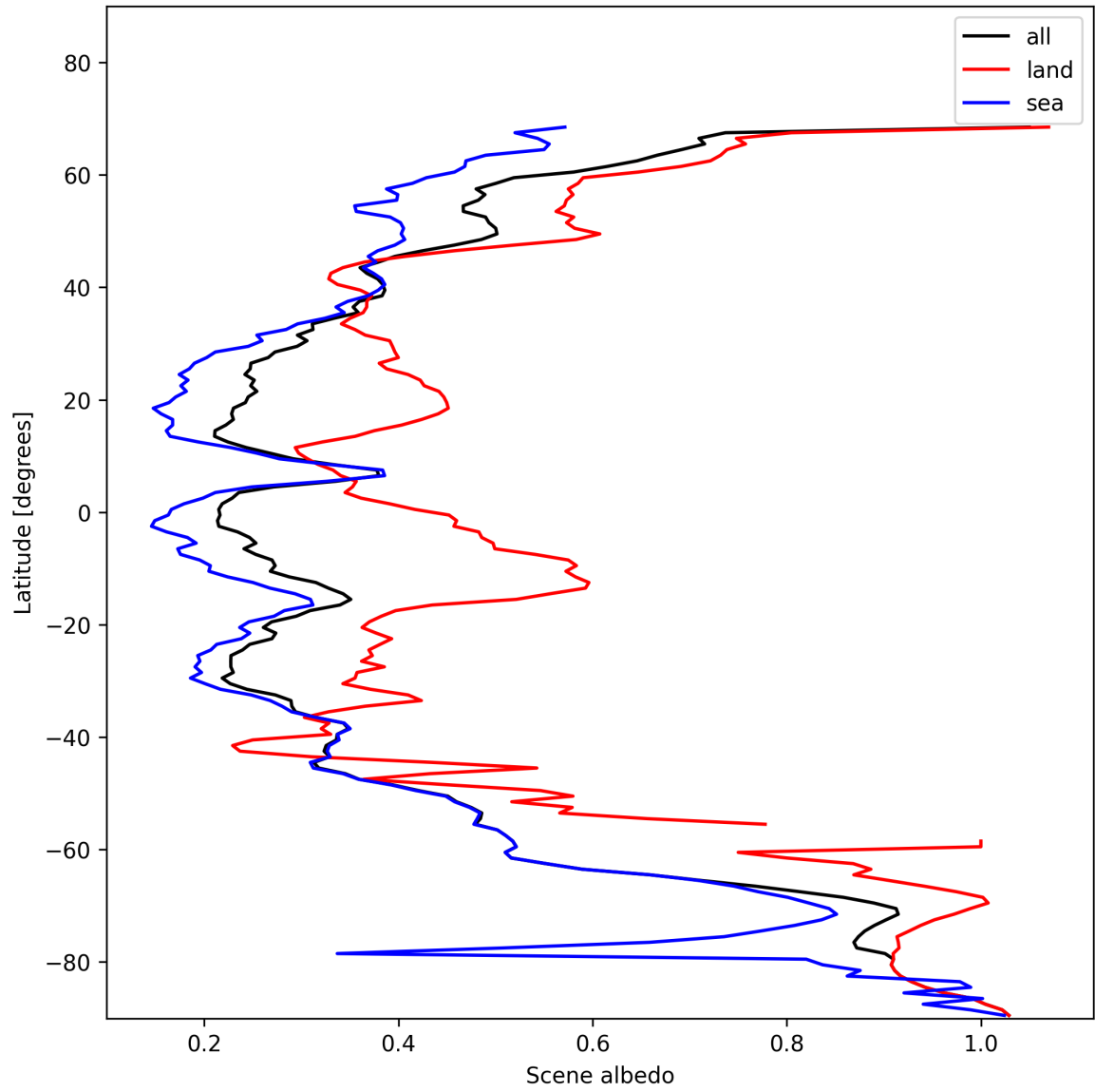
Figure 17: Zonal average of “Scene albedo” for 2025-11-20 to 2025-11-22.
