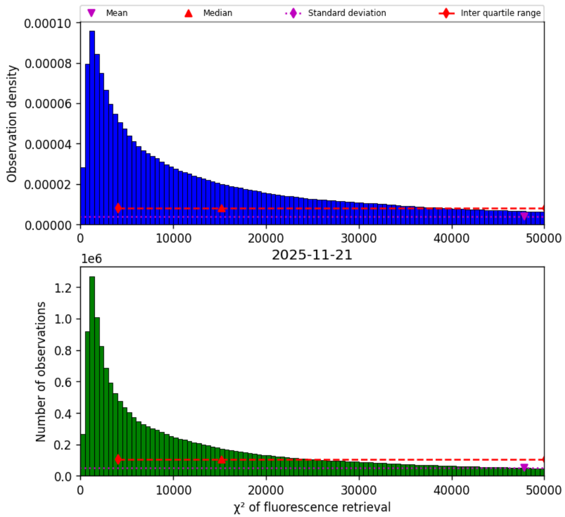
Figure 42: Histogram of “ \chi^2 of fluorescence retrieval” for 2025-11-20 to 2025-11-22
