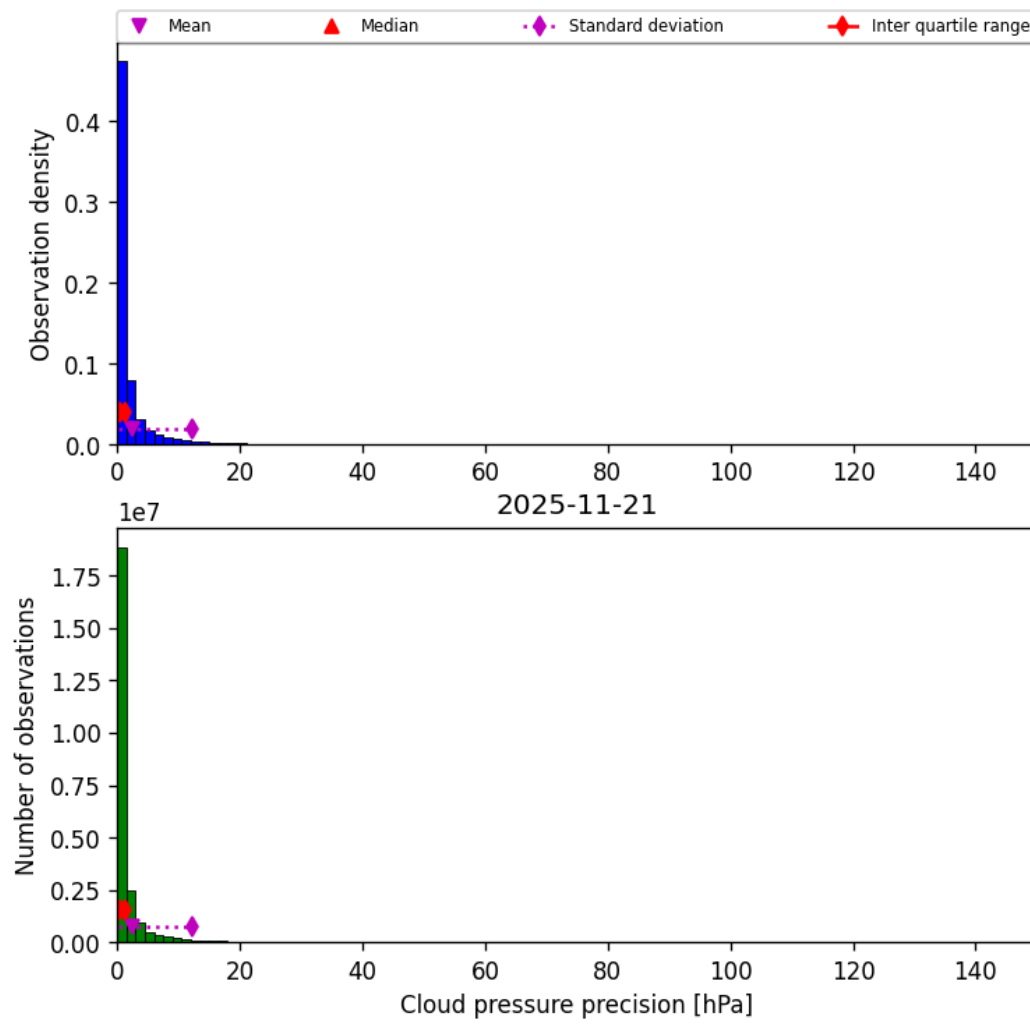
Figure 31: Histogram of “Cloud pressure precision” for 2025-11-20 to 2025-11-22
