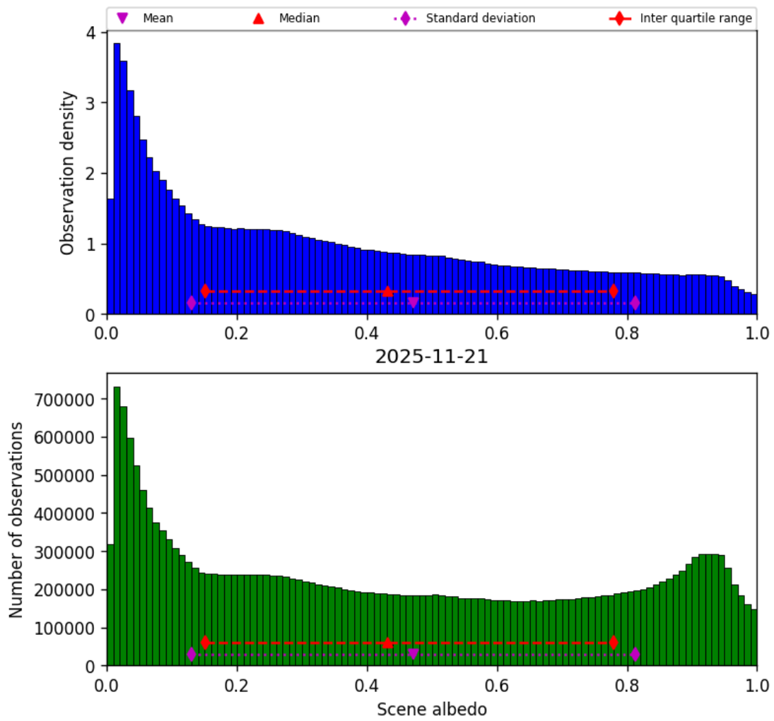
Figure 34: Histogram of “Scene albedo” for 2025-11-20 to 2025-11-22
