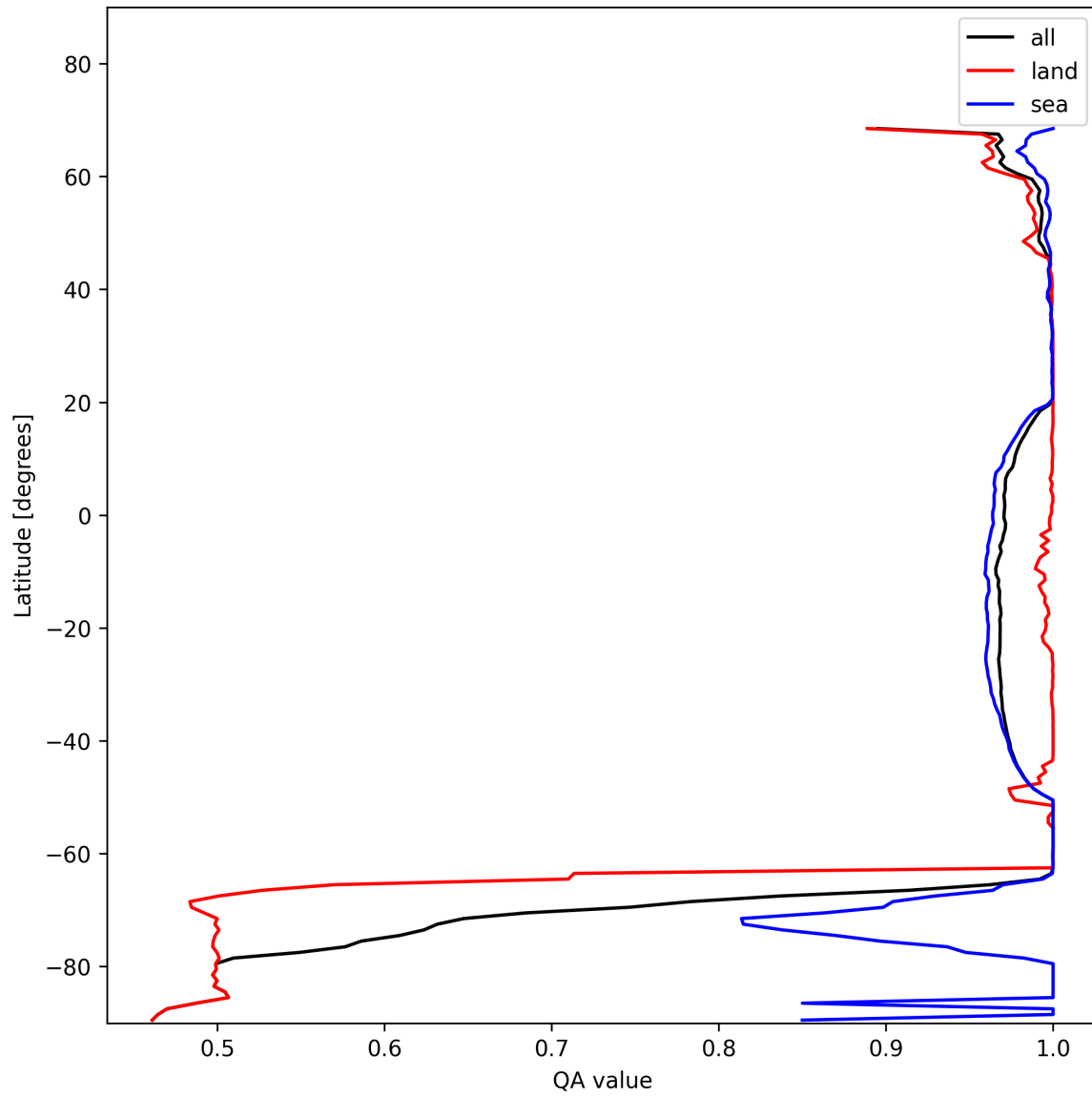
Figure 12: Zonal average of “QA value” for 2025-11-20 to 2025-11-22.
