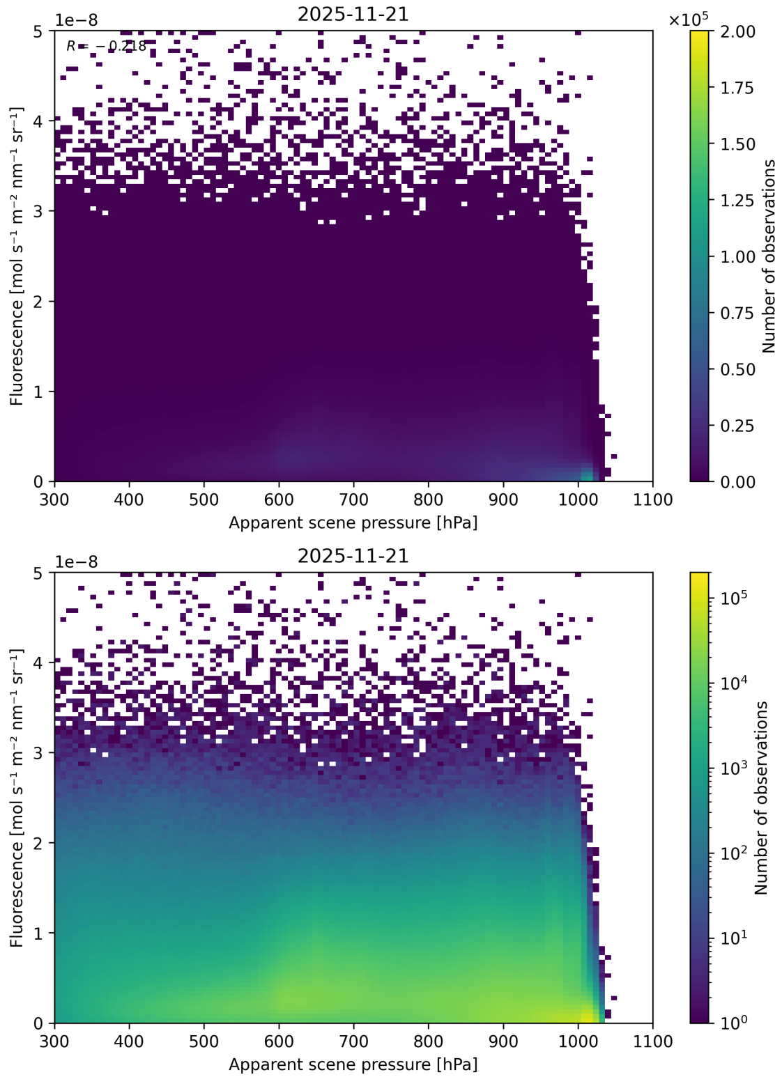
Figure 64: Scatter density plot of “Apparent scene pressure” against “Fluorescence” for 2025-11-20 to 2025-11-22.
