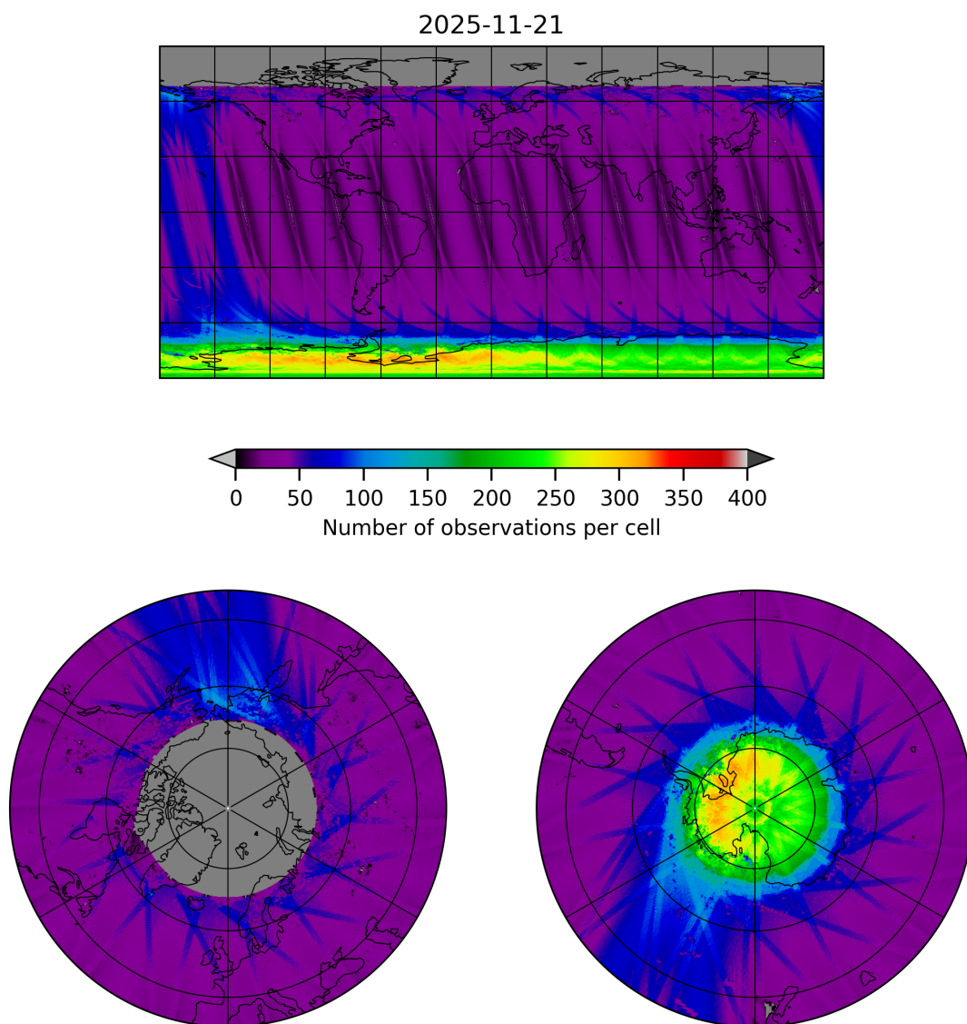
Figure 11: Map of the number of observations for 2025-11-20 to 2025-11-22
