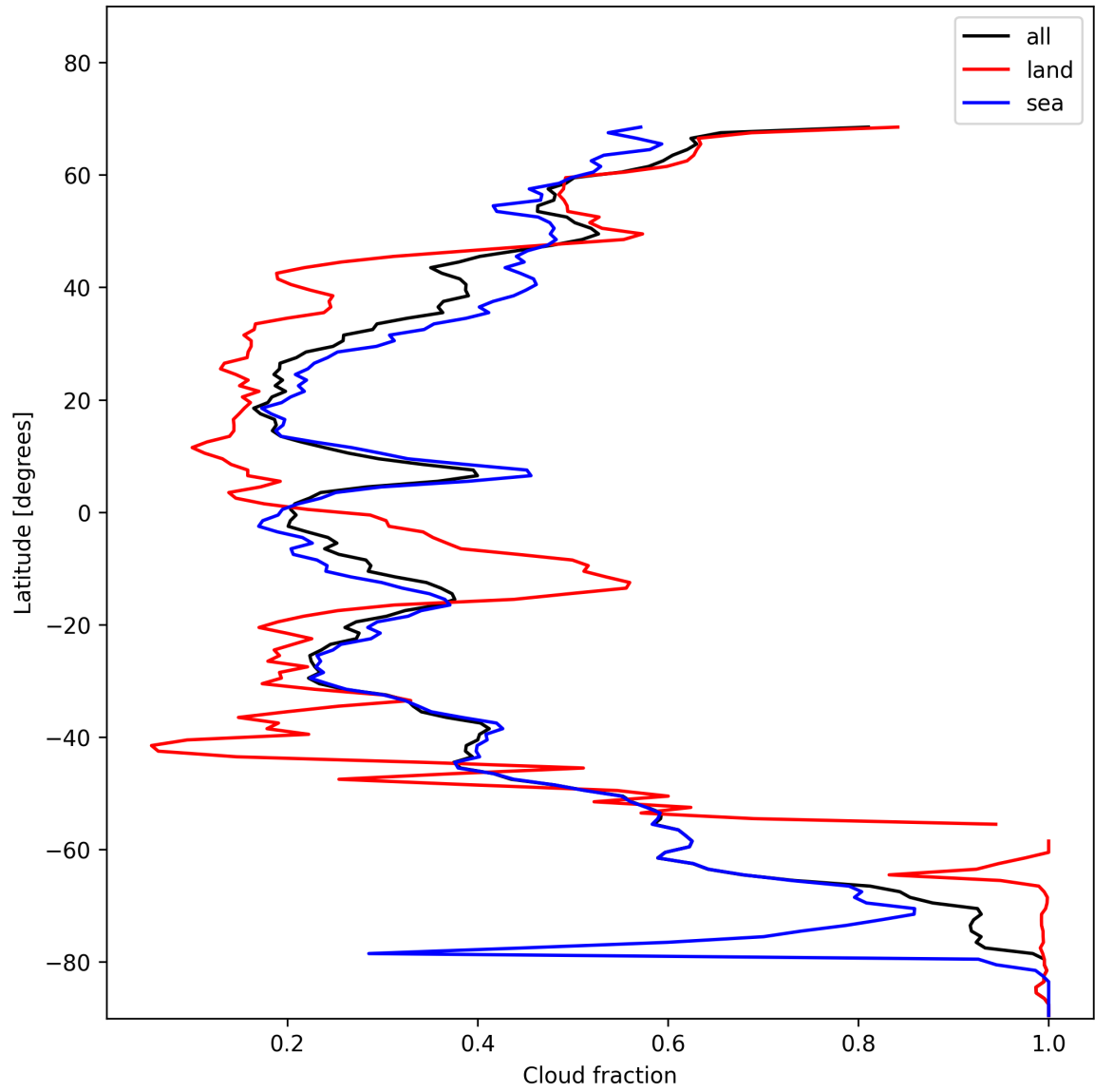
Figure 15: Zonal average of “Cloud fraction” for 2025-11-20 to 2025-11-22.
