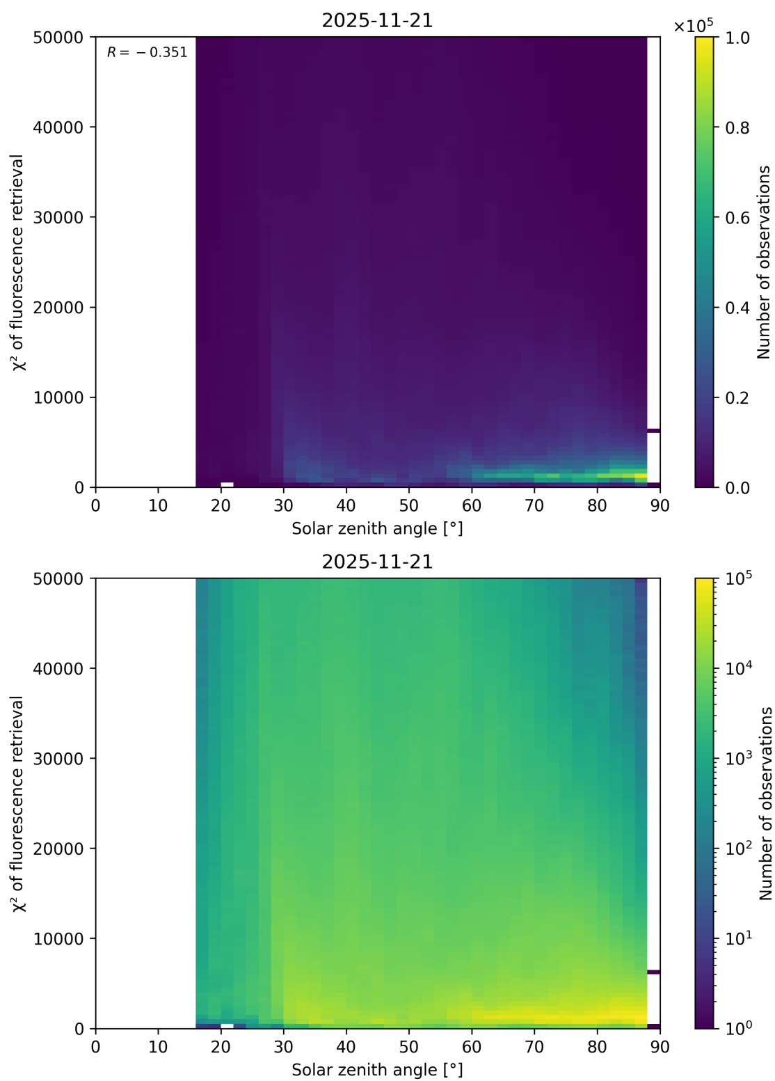
Figure 109: Scatter density plot of “Solar zenith angle” against “ \chi^2 of fluorescence retrieval” for 2025-11-20 to 2025-11-22.
