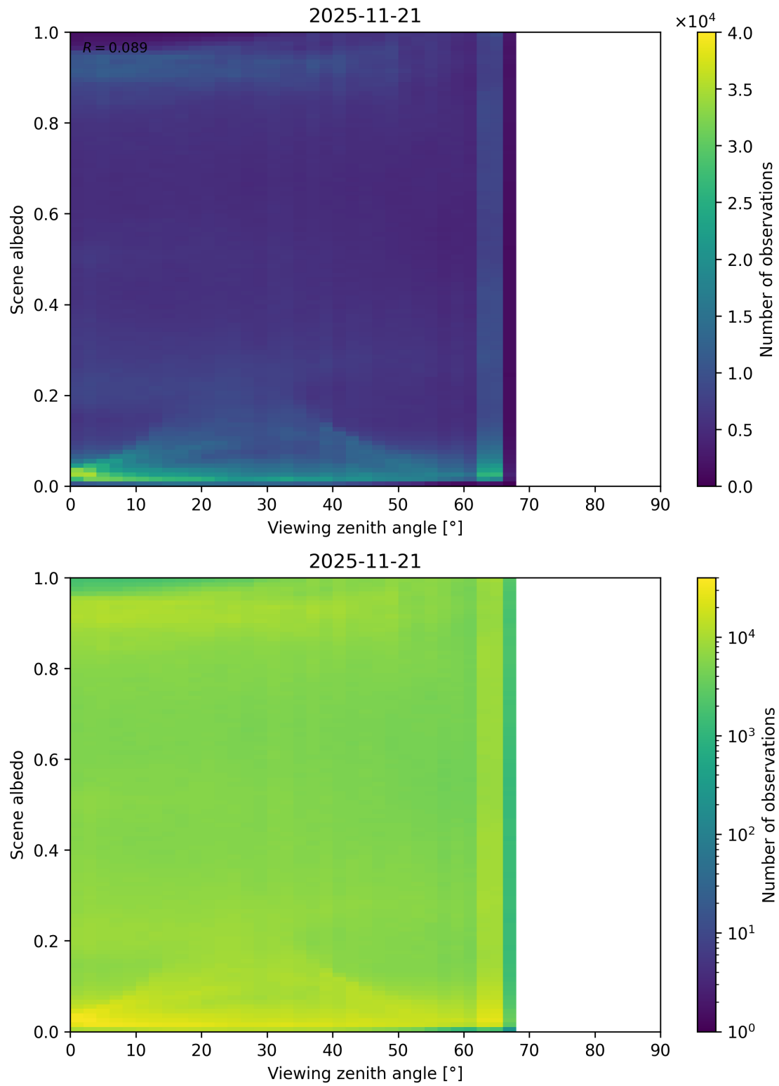
Figure 126: Scatter density plot of “Viewing zenith angle” against “Scene albedo” for 2025-11-20 to 2025-11-22.
