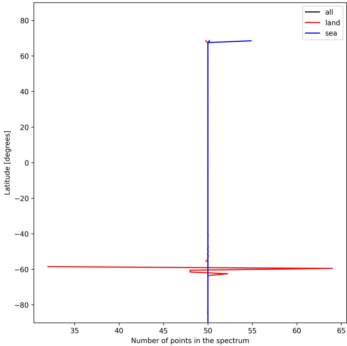
Figure 27: Zonal average of “Number of points in the spectrum” for 2025-11-20 to 2025-11-22.
