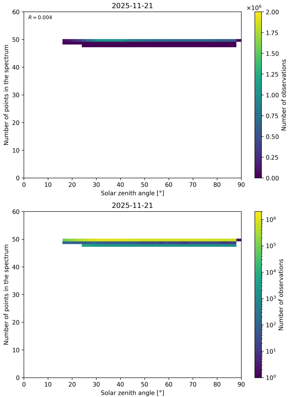
Figure 115: Scatter density plot of “Solar zenith angle” against “Number of points in the spectrum” for 2025-11-20 to 2025-11-22.
