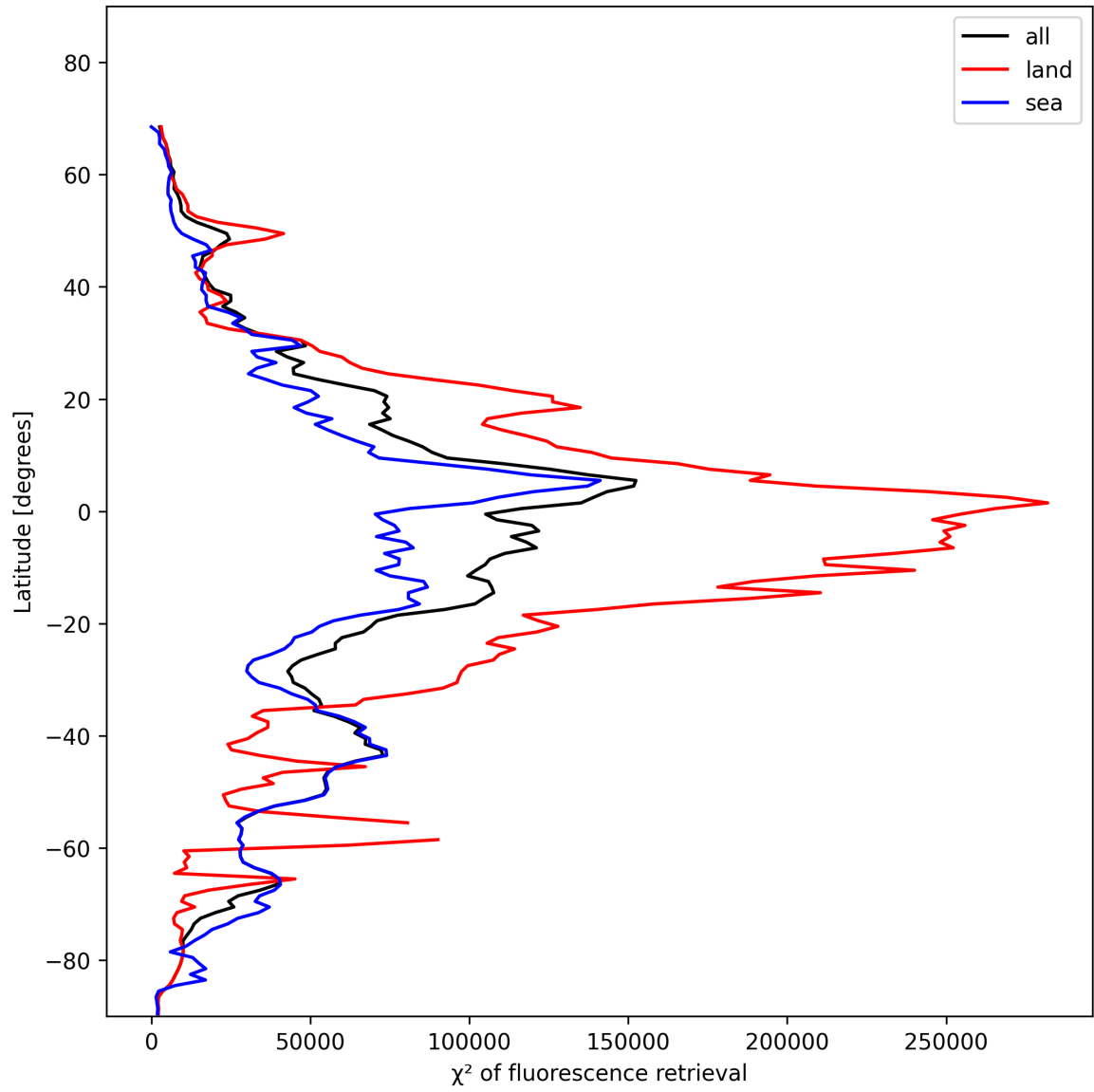
Figure 25: Zonal average of “ \chi^2 of fluorescence retrieval” for 2025-11-20 to 2025-11-22.
