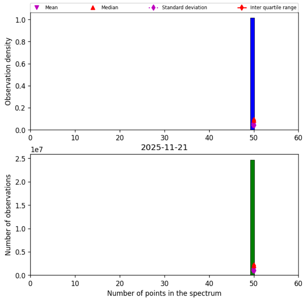
Figure 44: Histogram of “Number of points in the spectrum” for 2025-11-20 to 2025-11-22
