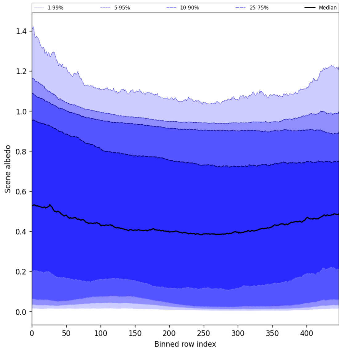
Figure 51: Along track statistics of “Scene albedo” for 2025-11-20 to 2025-11-22
