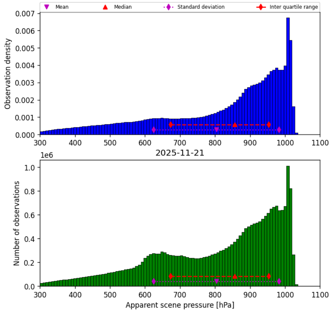
Figure 36: Histogram of “Apparent scene pressure” for 2025-11-20 to 2025-11-22
