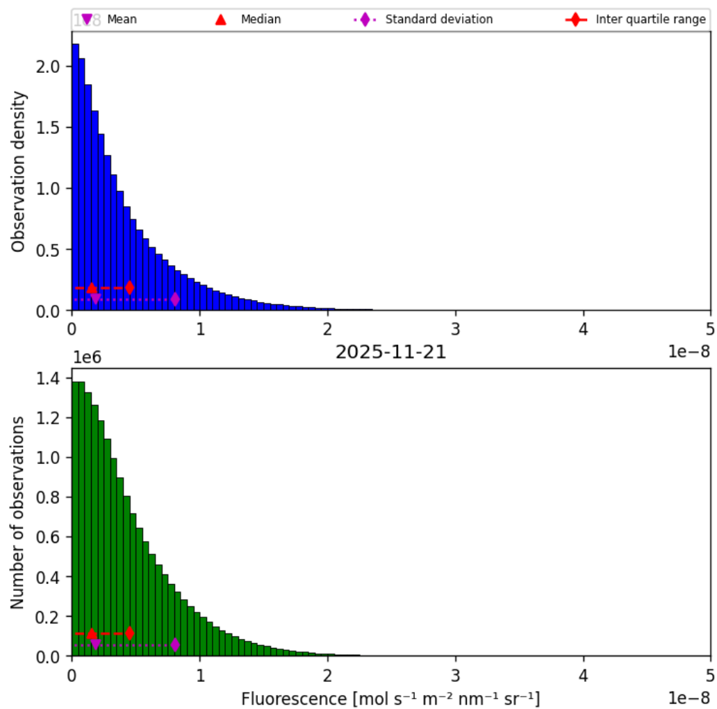
Figure 40: Histogram of “Fluorescence” for 2025-11-20 to 2025-11-22
