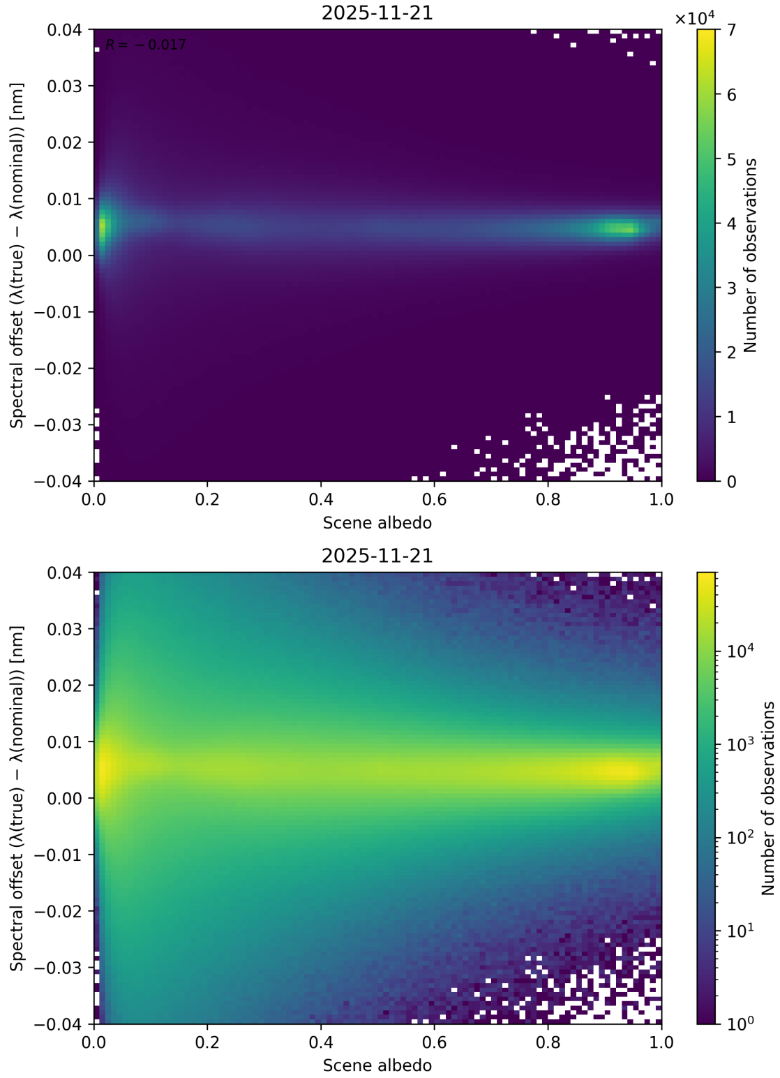
Figure 107: Scatter density plot of “Scene albedo” against “Spectral offset ( \lambda_{\text{true}} - \lambda_{\text{nominal}} )” for 2025-11-20 to 2025-11-22.
