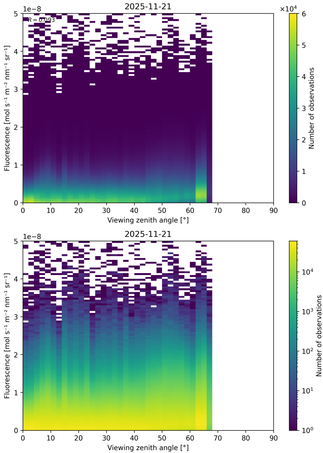
Figure 122: Scatter density plot of “Viewing zenith angle” against “Fluorescence” for 2025-11-20 to 2025-11-22.
