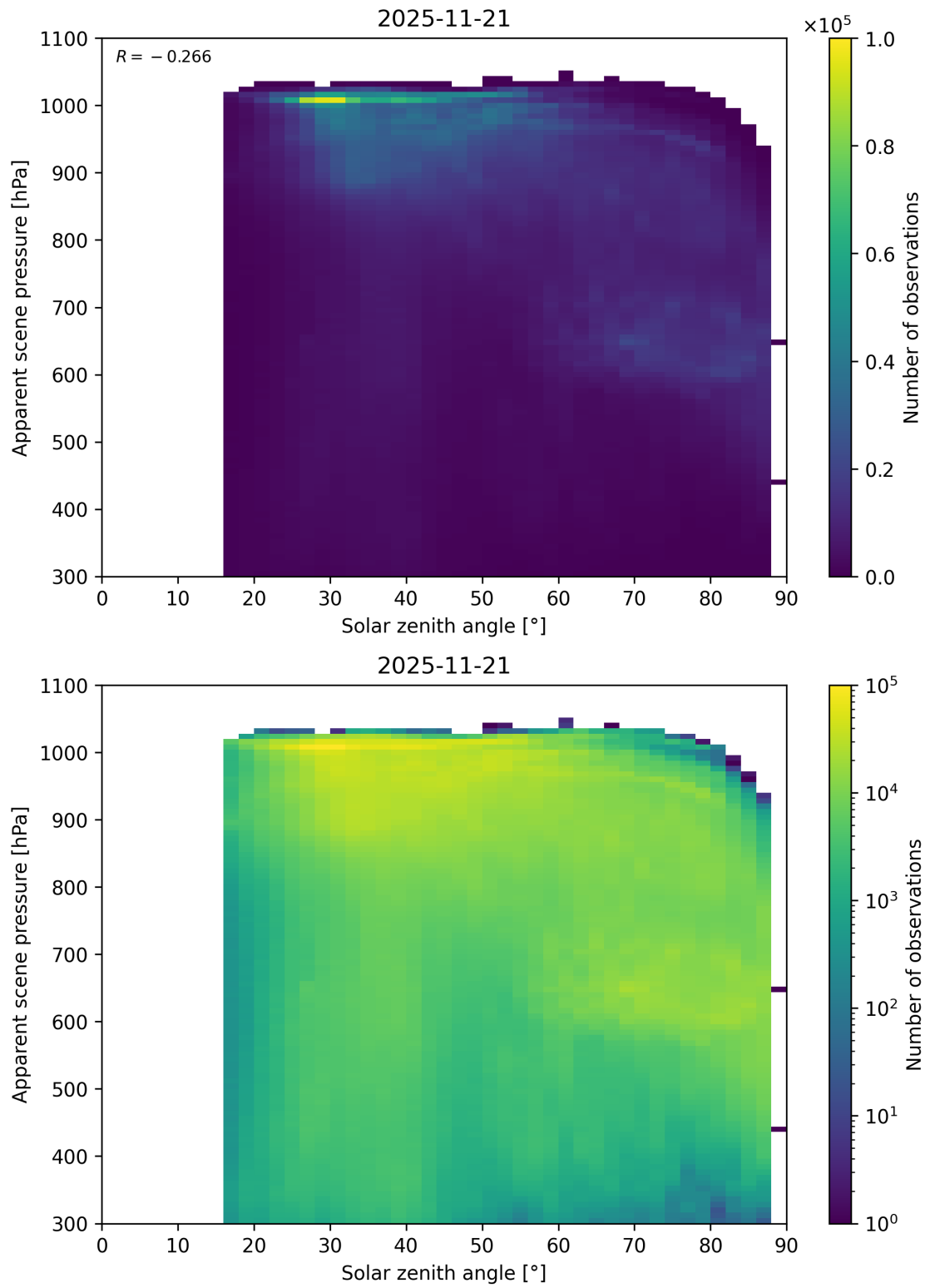
Figure 108: Scatter density plot of “Solar zenith angle” against “Apparent scene pressure” for 2025-11-20 to 2025-11-22.
