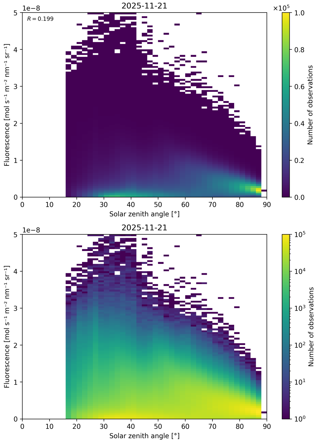
Figure 112: Scatter density plot of “Solar zenith angle” against “Fluorescence” for 2025-11-20 to 2025-11-22.
