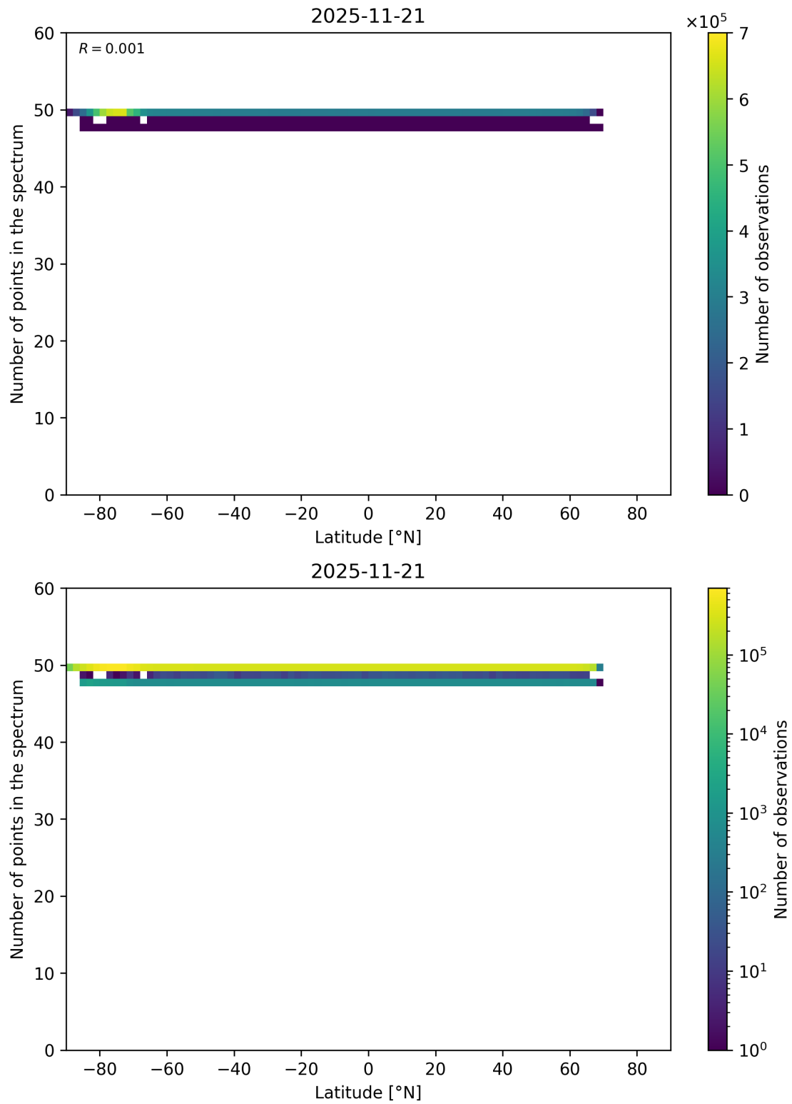
Figure 94: Scatter density plot of “Latitude” against “Number of points in the spectrum” for 2025-11-20 to 2025-11-22.
