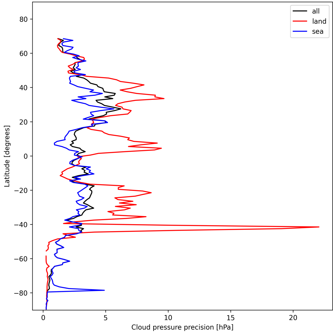
Figure 14: Zonal average of “Cloud pressure precision” for 2025-11-20 to 2025-11-22.
