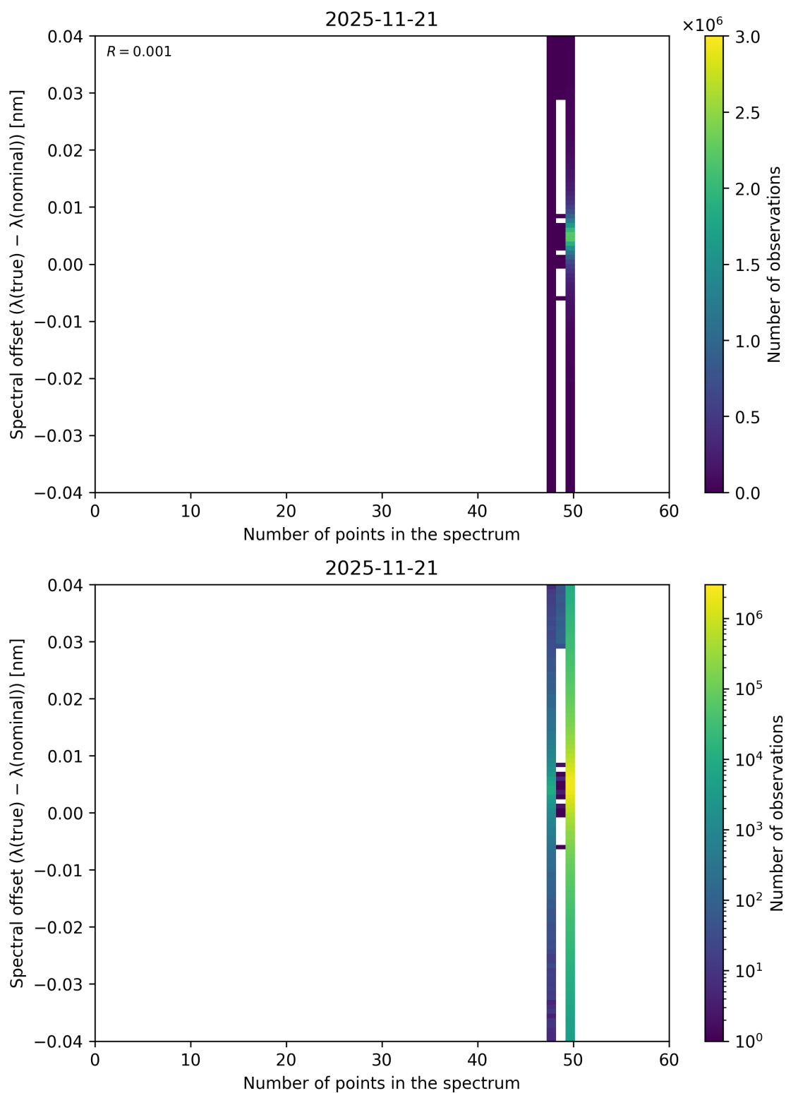
Figure 101: Scatter density plot of “Number of points in the spectrum” against “Spectral offset ( \lambda_{\text{true}} - \lambda_{\text{nominal}} )” for 2025-11-20 to 2025-11-22.
