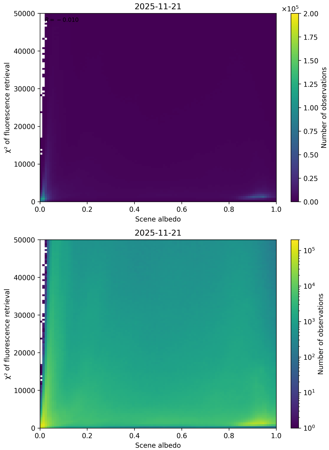
Figure 103: Scatter density plot of “Scene albedo” against “ \chi^2 of fluorescence retrieval” for 2025-11-20 to 2025-11-22.
