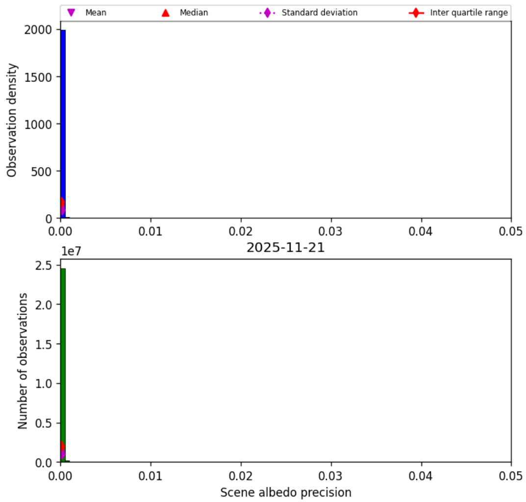
Figure 35: Histogram of “Scene albedo precision” for 2025-11-20 to 2025-11-22
