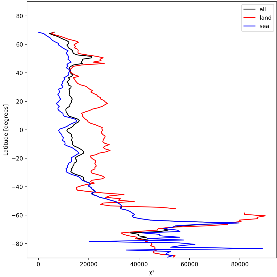
Figure 21: Zonal average of “ \chi^2 ” for 2025-11-20 to 2025-11-22.
