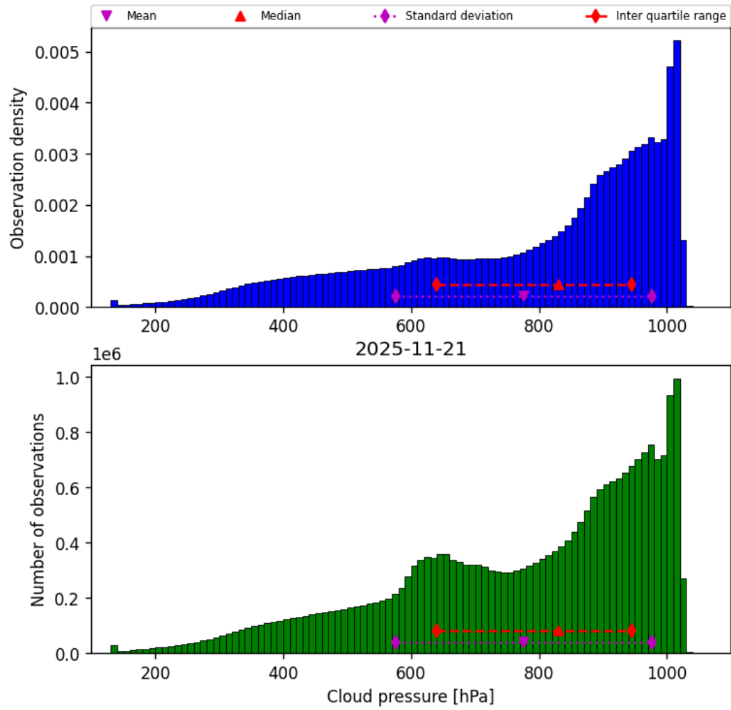
Figure 30: Histogram of “Cloud pressure” for 2025-11-20 to 2025-11-22
