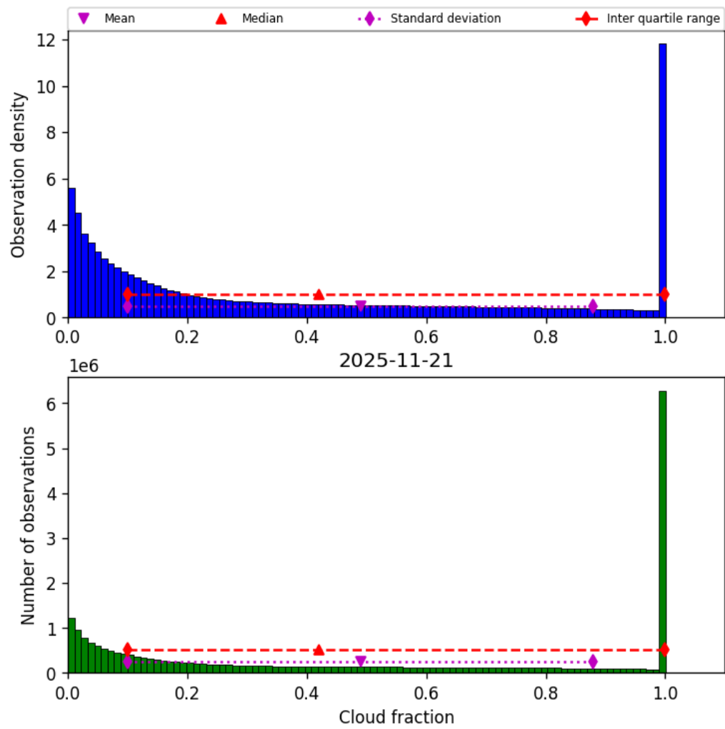
Figure 32: Histogram of “Cloud fraction” for 2025-11-20 to 2025-11-22
