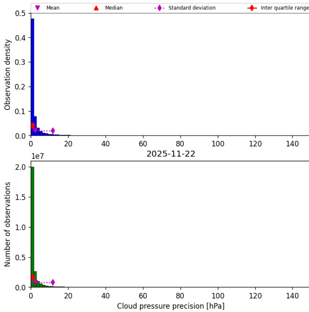
Figure 31: Histogram of “Cloud pressure precision” for 2025-11-21 to 2025-11-23
