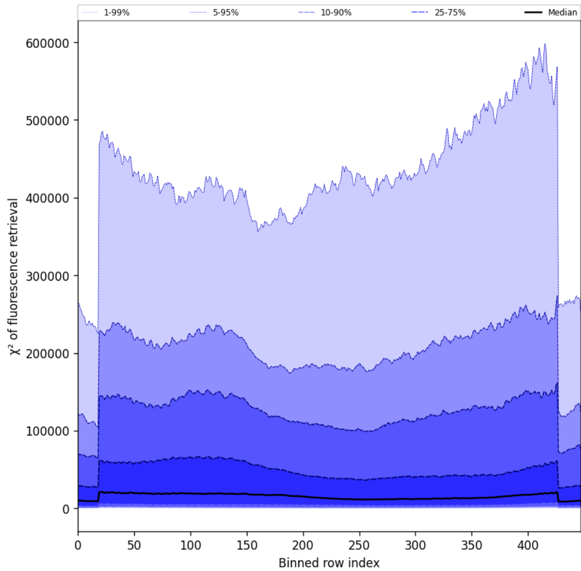
Figure 59: Along track statistics of “ \chi^2 of fluorescence retrieval” for 2025-11-21 to 2025-11-23
