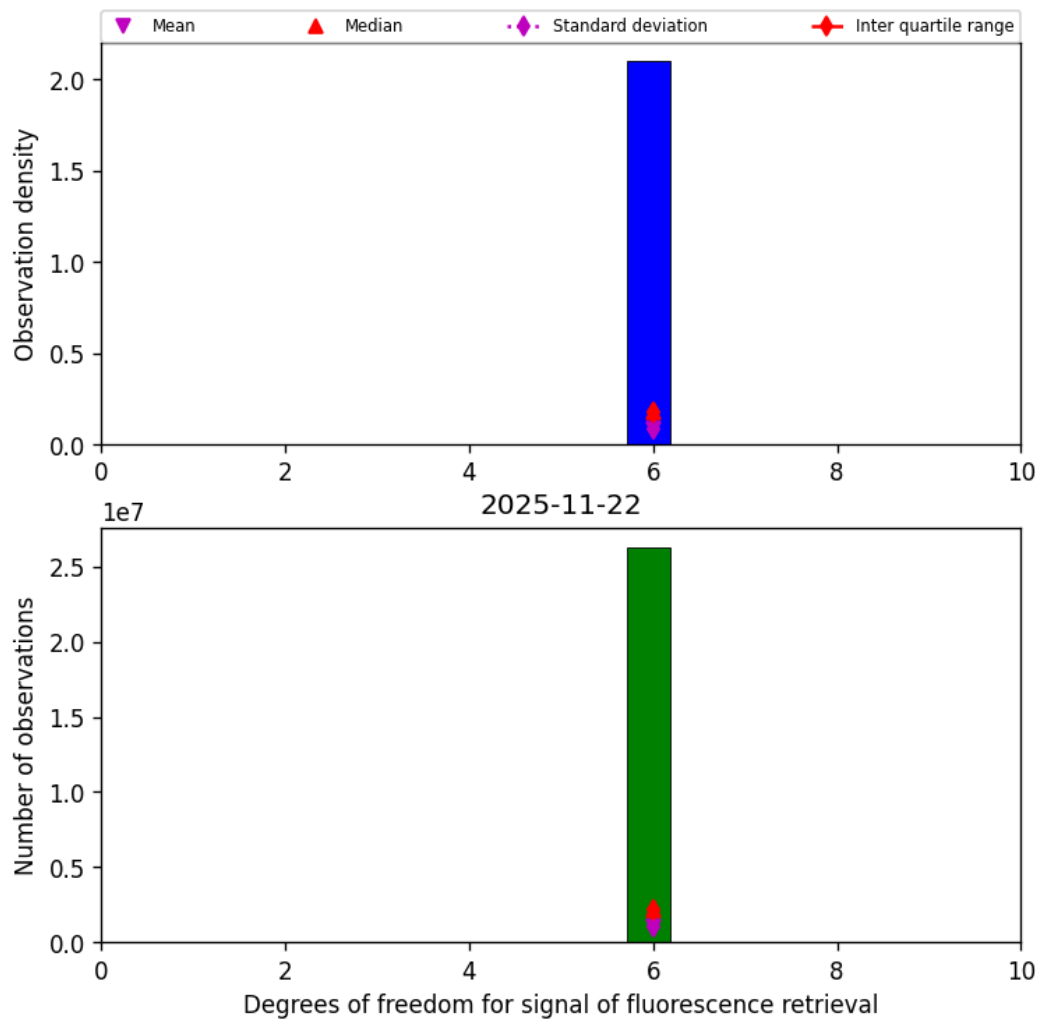
Figure 43: Histogram of "Degrees of freedom for signal of fluorescence retrieval" for 2025-11-21 to 2025-11-23
