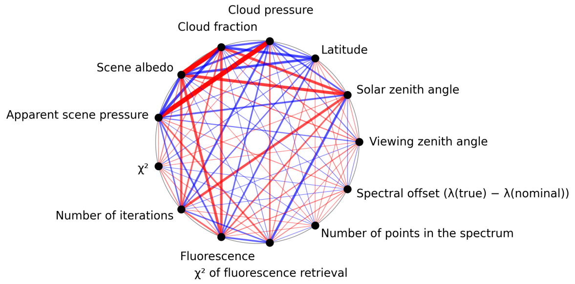
Figure 1: Map of correlation graph for 2025-11-21 to 2025-11-23.
