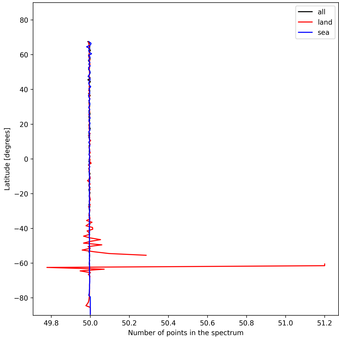
Figure 27: Zonal average of “Number of points in the spectrum” for 2025-11-21 to 2025-11-23.
