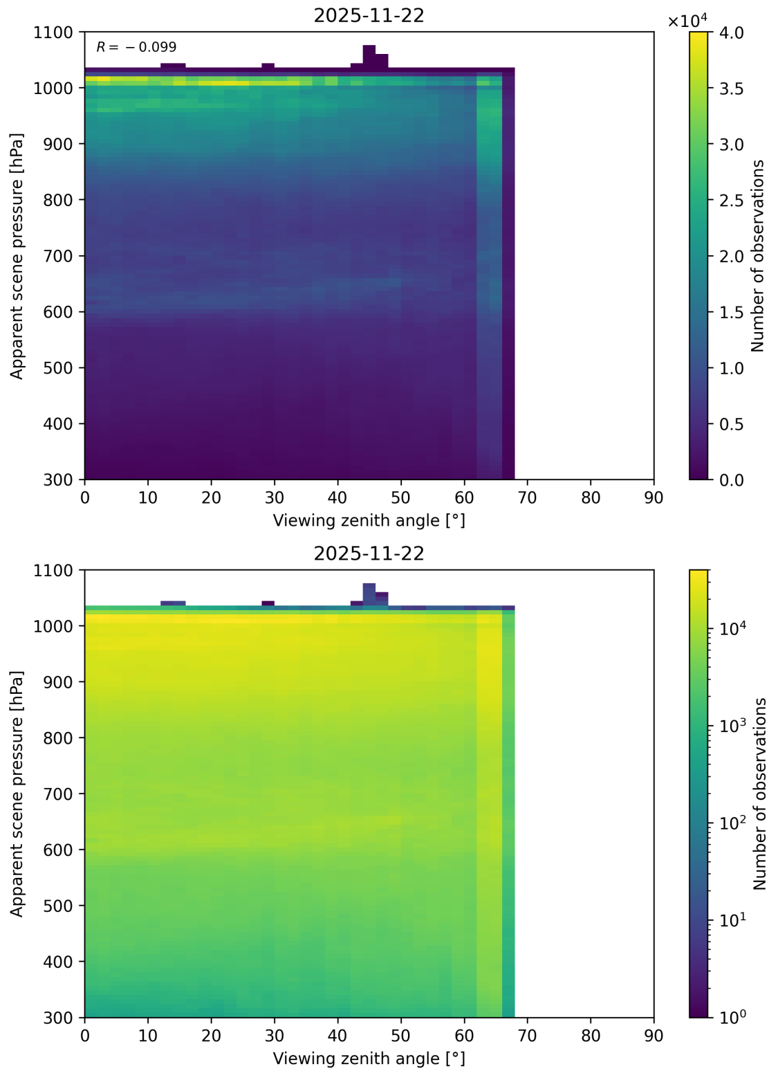
Figure 118: Scatter density plot of “Viewing zenith angle” against “Apparent scene pressure” for 2025-11-21 to 2025-11-23.
