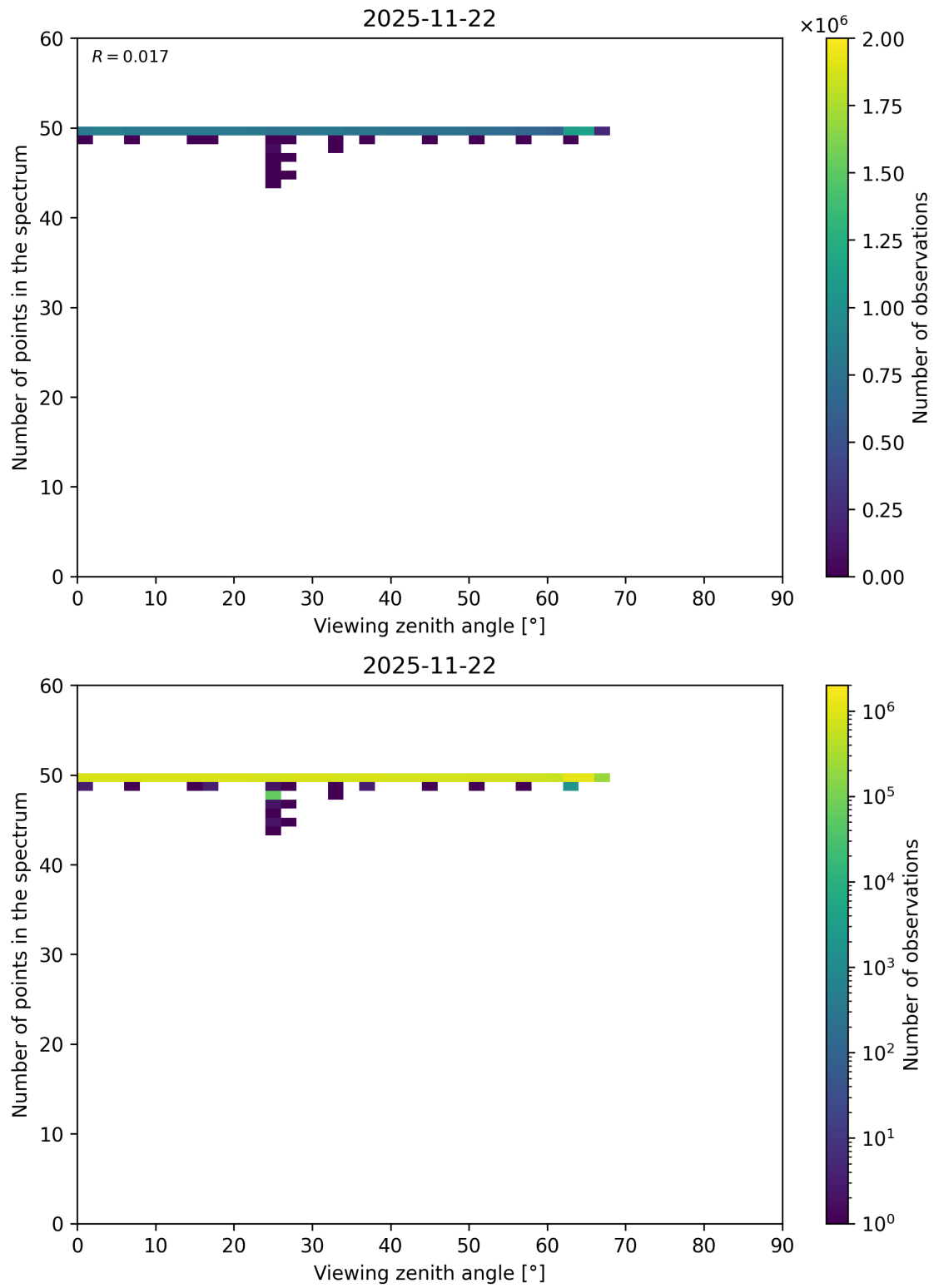
Figure 125: Scatter density plot of “Viewing zenith angle” against “Number of points in the spectrum” for 2025-11-21 to 2025-11-23.
