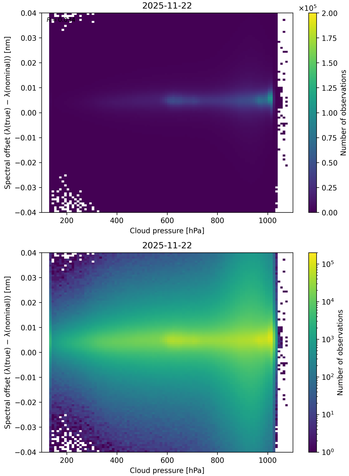
Figure 84: Scatter density plot of “Cloud pressure” against “Spectral offset ( \lambda_{\text{true}} - \lambda_{\text{nominal}} )” for 2025-11-21 to 2025-11-23.
