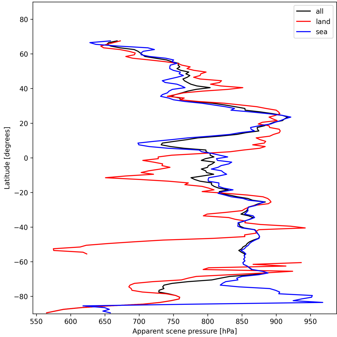
Figure 19: Zonal average of “Apparent scene pressure” for 2025-11-21 to 2025-11-23.
