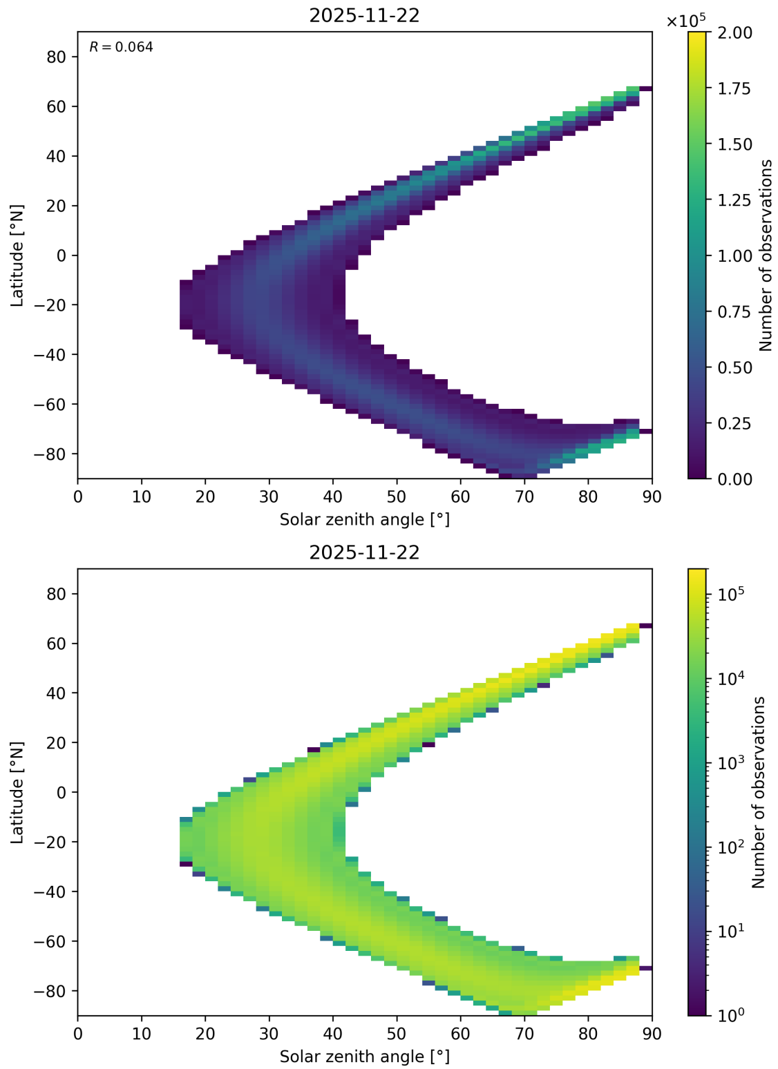
Figure 113: Scatter density plot of “Solar zenith angle” against “Latitude” for 2025-11-21 to 2025-11-23.
