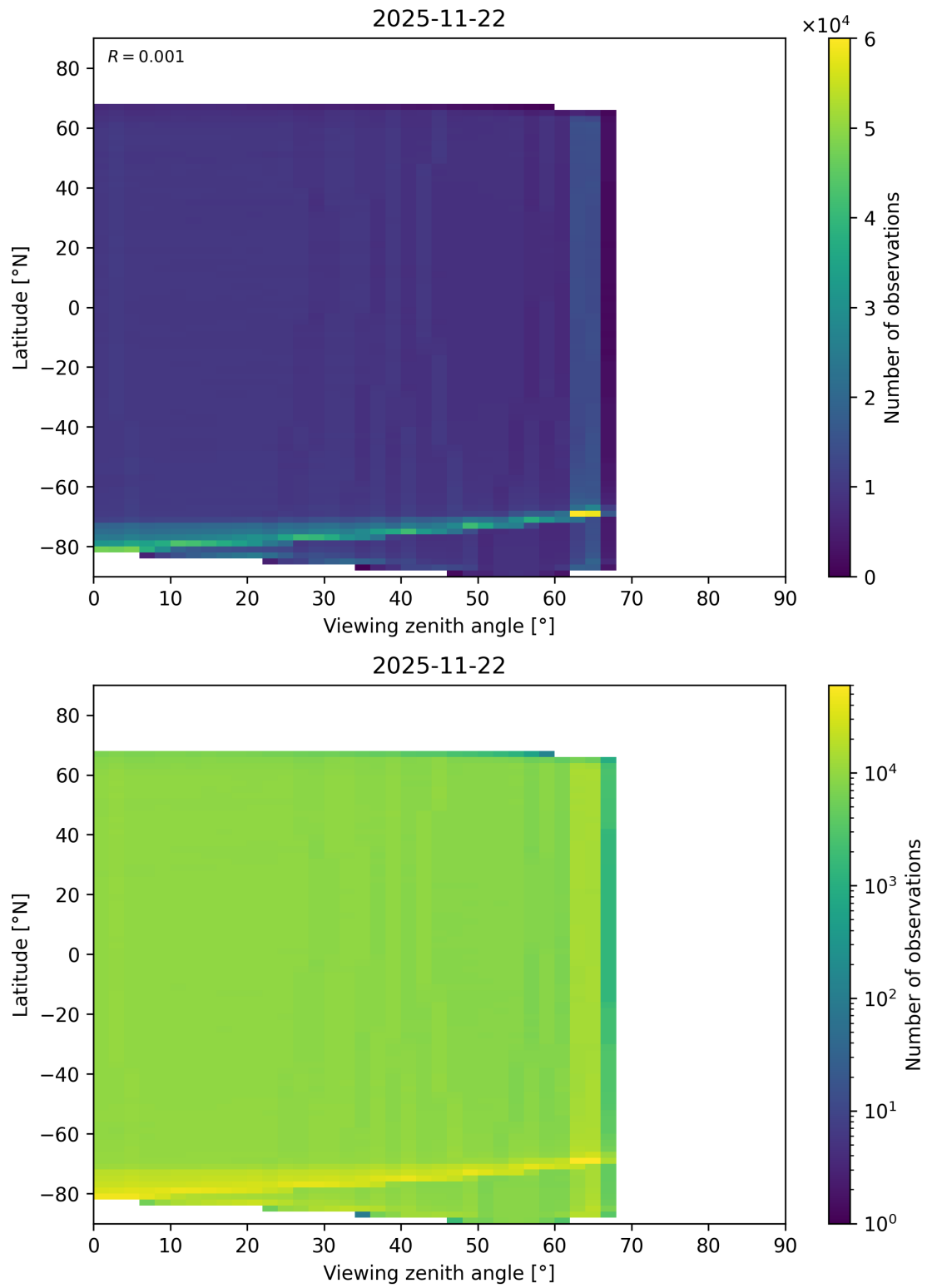
Figure 123: Scatter density plot of “Viewing zenith angle” against “Latitude” for 2025-11-21 to 2025-11-23.
