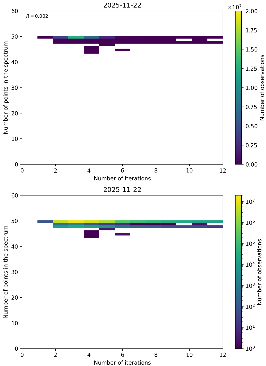
Figure 99: Scatter density plot of “Number of iterations” against “Number of points in the spectrum” for 2025-11-21 to 2025-11-23.
