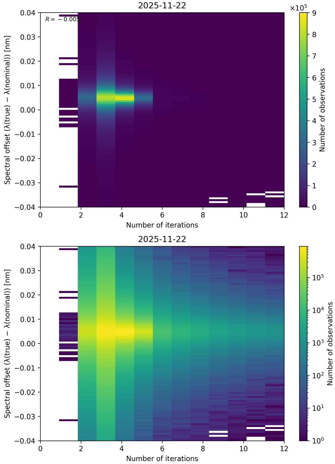
Figure 100: Scatter density plot of “Number of iterations” against “Spectral offset ( \lambda_{\text{true}} - \lambda_{\text{nominal}} )” for 2025-11-21 to 2025-11-23.
