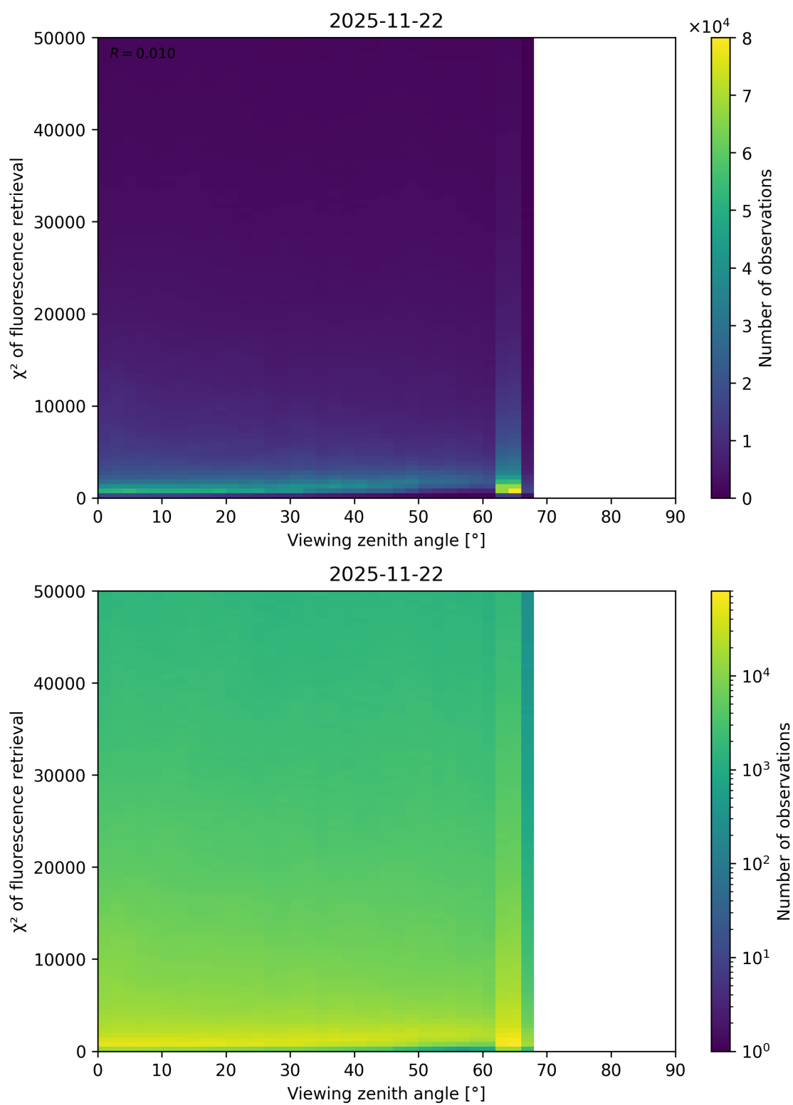
Figure 119: Scatter density plot of “Viewing zenith angle” against “ \chi^2 of fluorescence retrieval” for 2025-11-21 to 2025-11-23.
