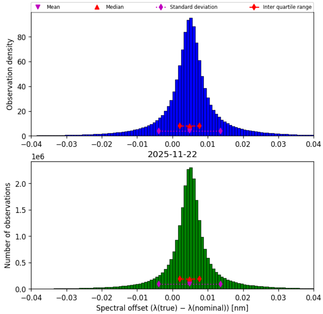
Figure 45: Histogram of “Spectral offset ( \lambda_{\text{true}} - \lambda_{\text{nominal}} )” for 2025-11-21 to 2025-11-23
