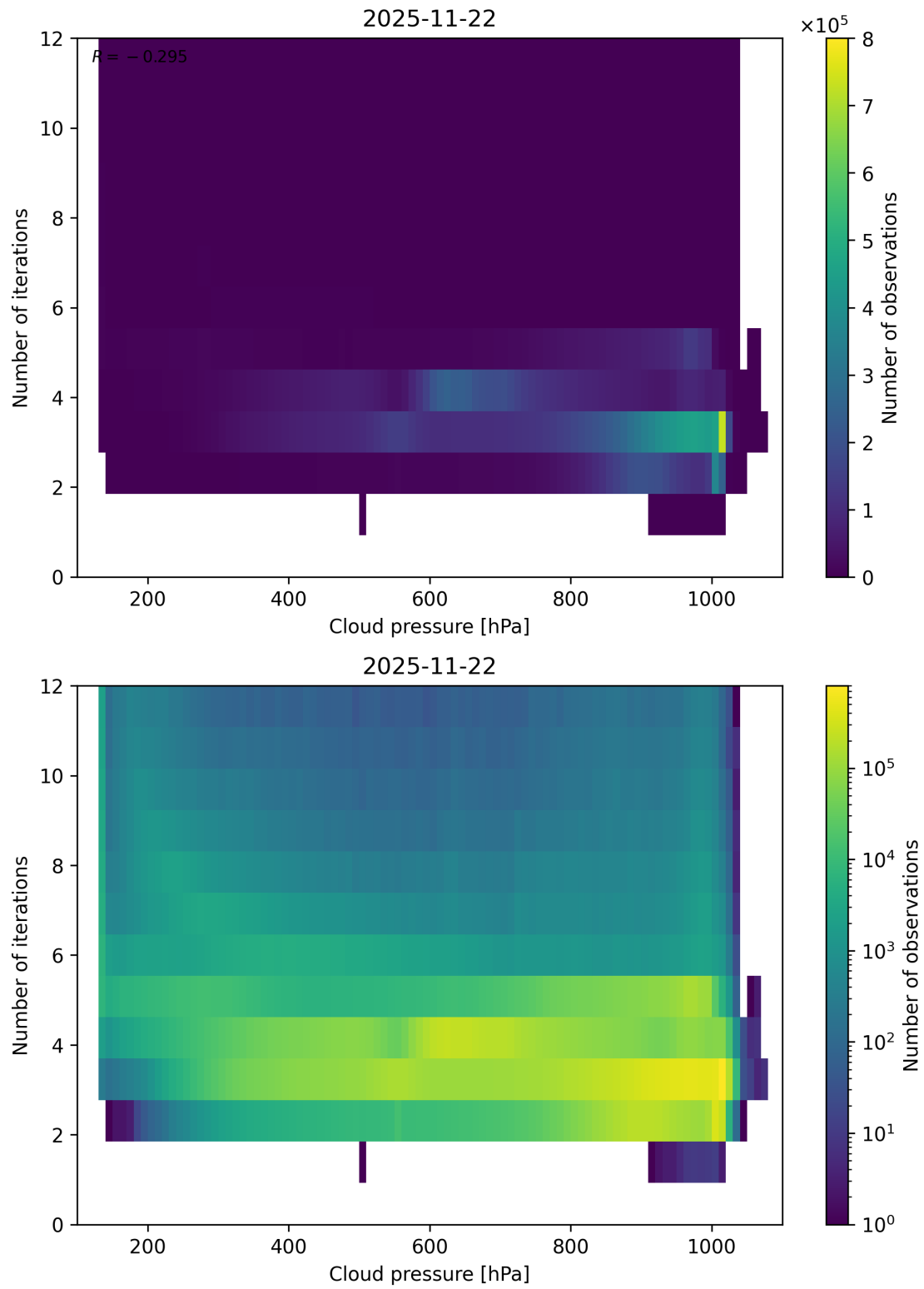
Figure 81: Scatter density plot of “Cloud pressure” against “Number of iterations” for 2025-11-21 to 2025-11-23.
