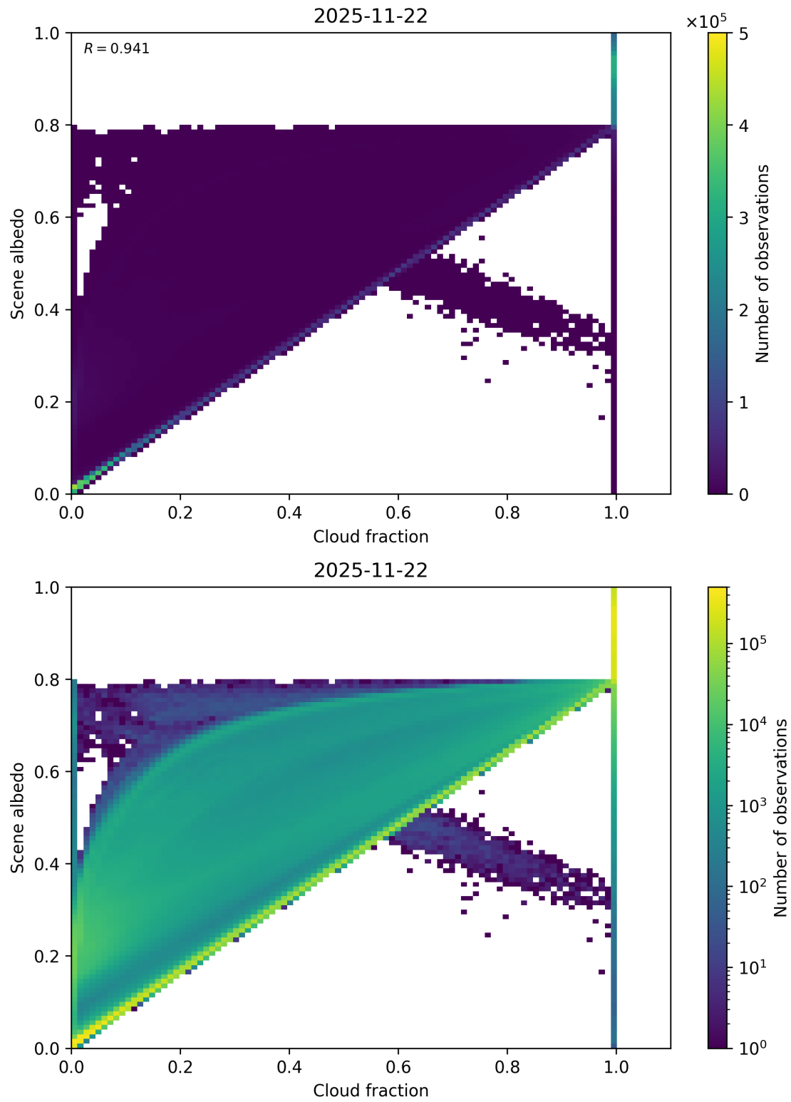
Figure 75: Scatter density plot of “Cloud fraction” against “Scene albedo” for 2025-11-21 to 2025-11-23.
