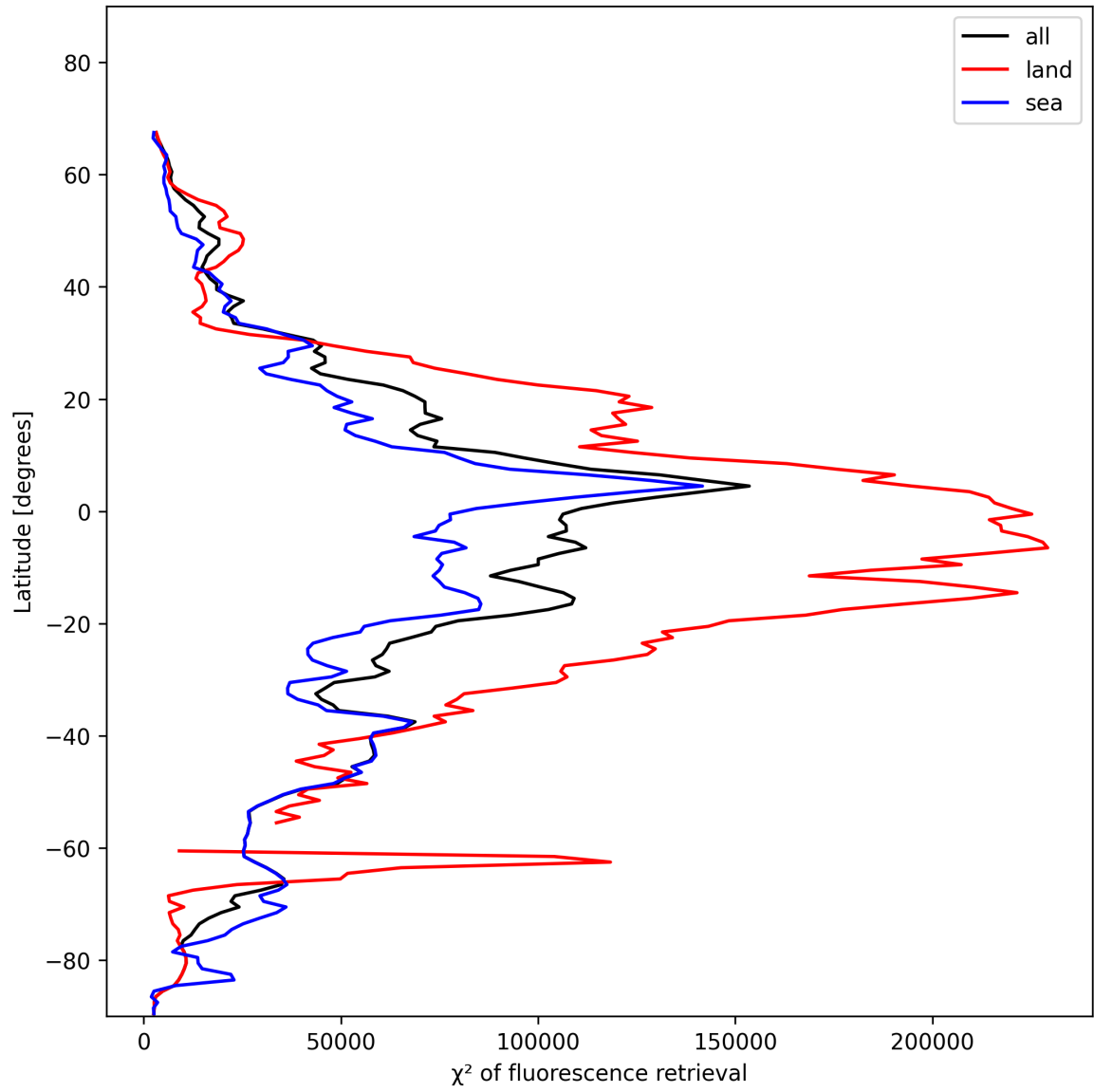
Figure 25: Zonal average of “ \chi^2 of fluorescence retrieval” for 2025-11-21 to 2025-11-23.
