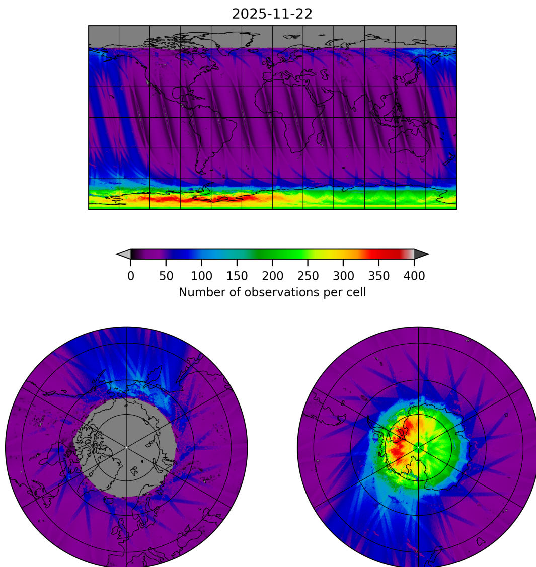
Figure 11: Map of the number of observations for 2025-11-21 to 2025-11-23
