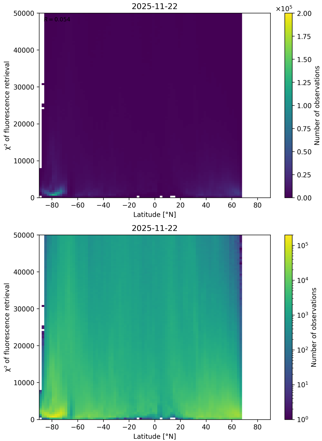
Figure 89: Scatter density plot of “Latitude” against “ \chi^2 of fluorescence retrieval” for 2025-11-21 to 2025-11-23.
