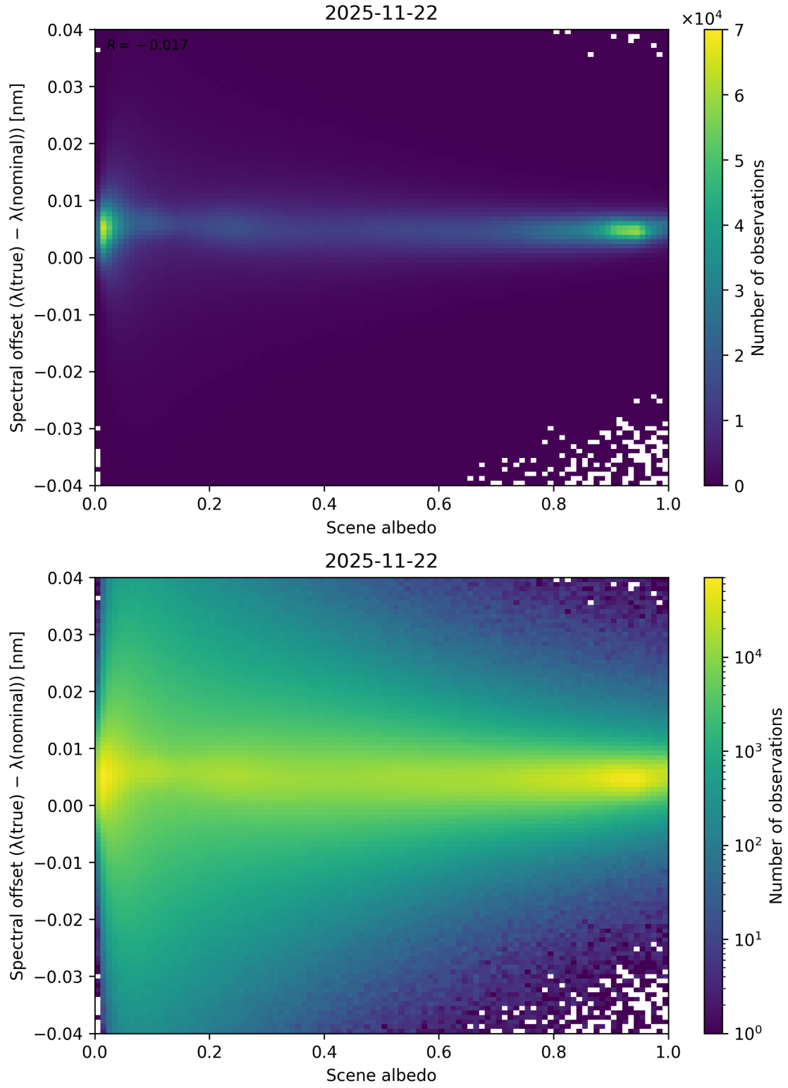
Figure 107: Scatter density plot of “Scene albedo” against “Spectral offset ( \lambda_{\text{true}} - \lambda_{\text{nominal}} )” for 2025-11-21 to 2025-11-23.
