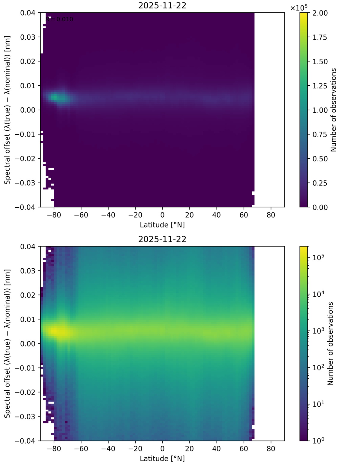
Figure 96: Scatter density plot of “Latitude” against “Spectral offset ( \lambda_{\text{true}} - \lambda_{\text{nominal}} )” for 2025-11-21 to 2025-11-23.
