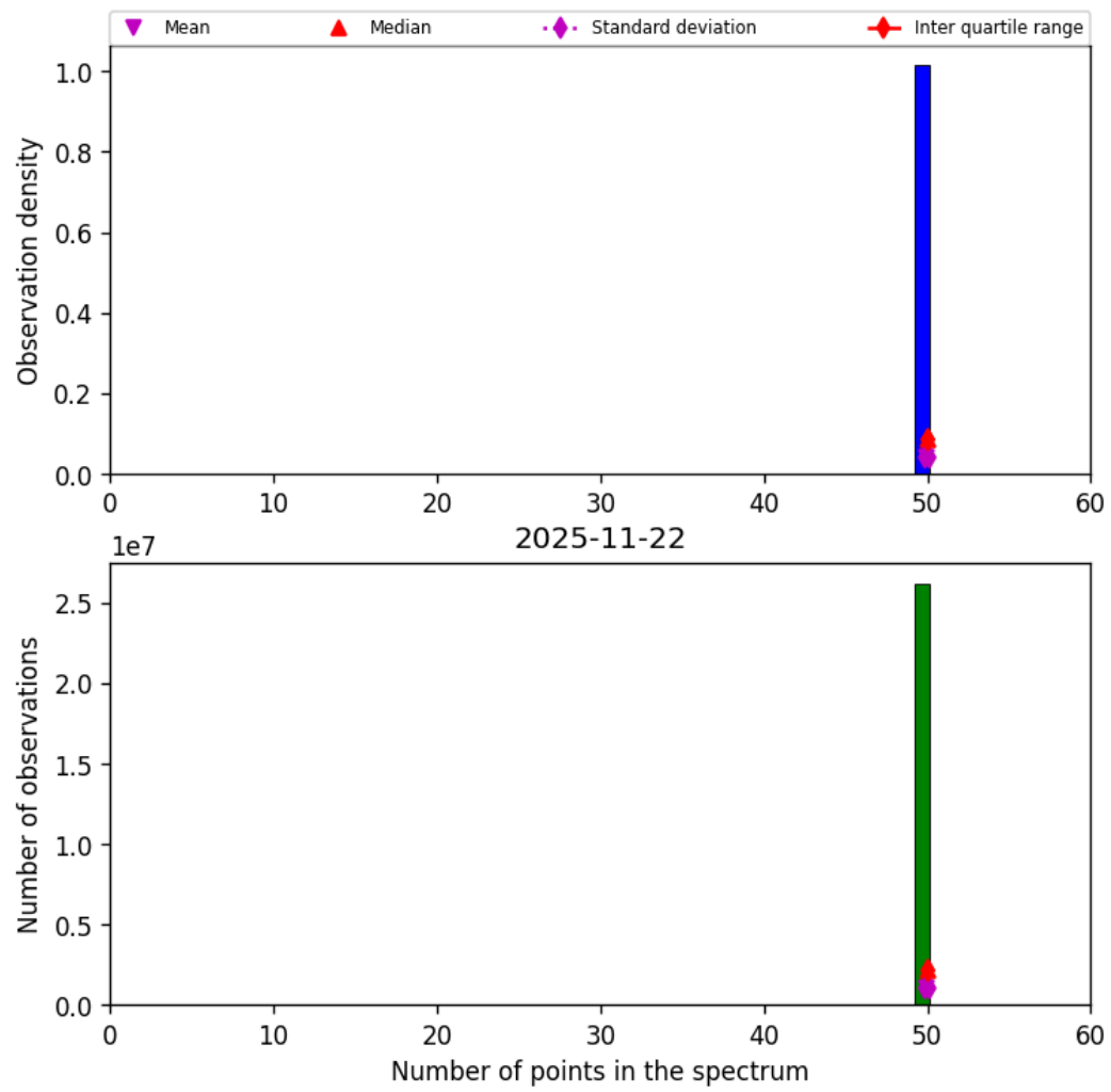
Figure 44: Histogram of "Number of points in the spectrum" for 2025-11-21 to 2025-11-23
