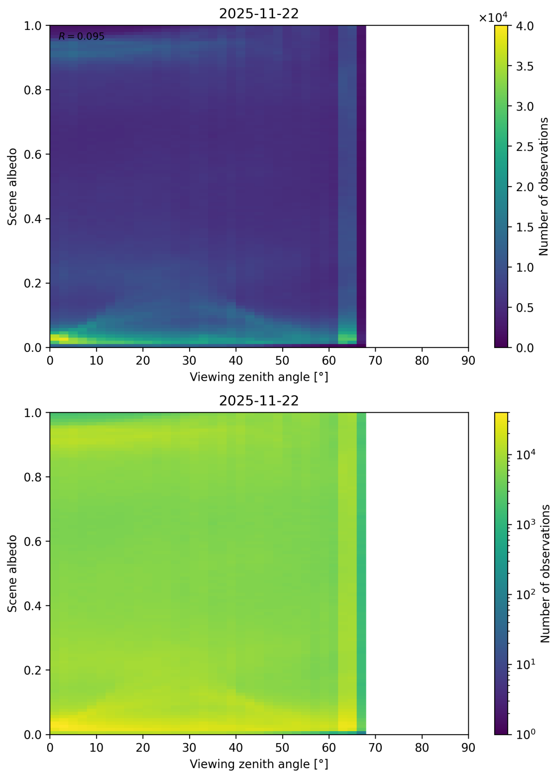
Figure 126: Scatter density plot of “Viewing zenith angle” against “Scene albedo” for 2025-11-21 to 2025-11-23.
