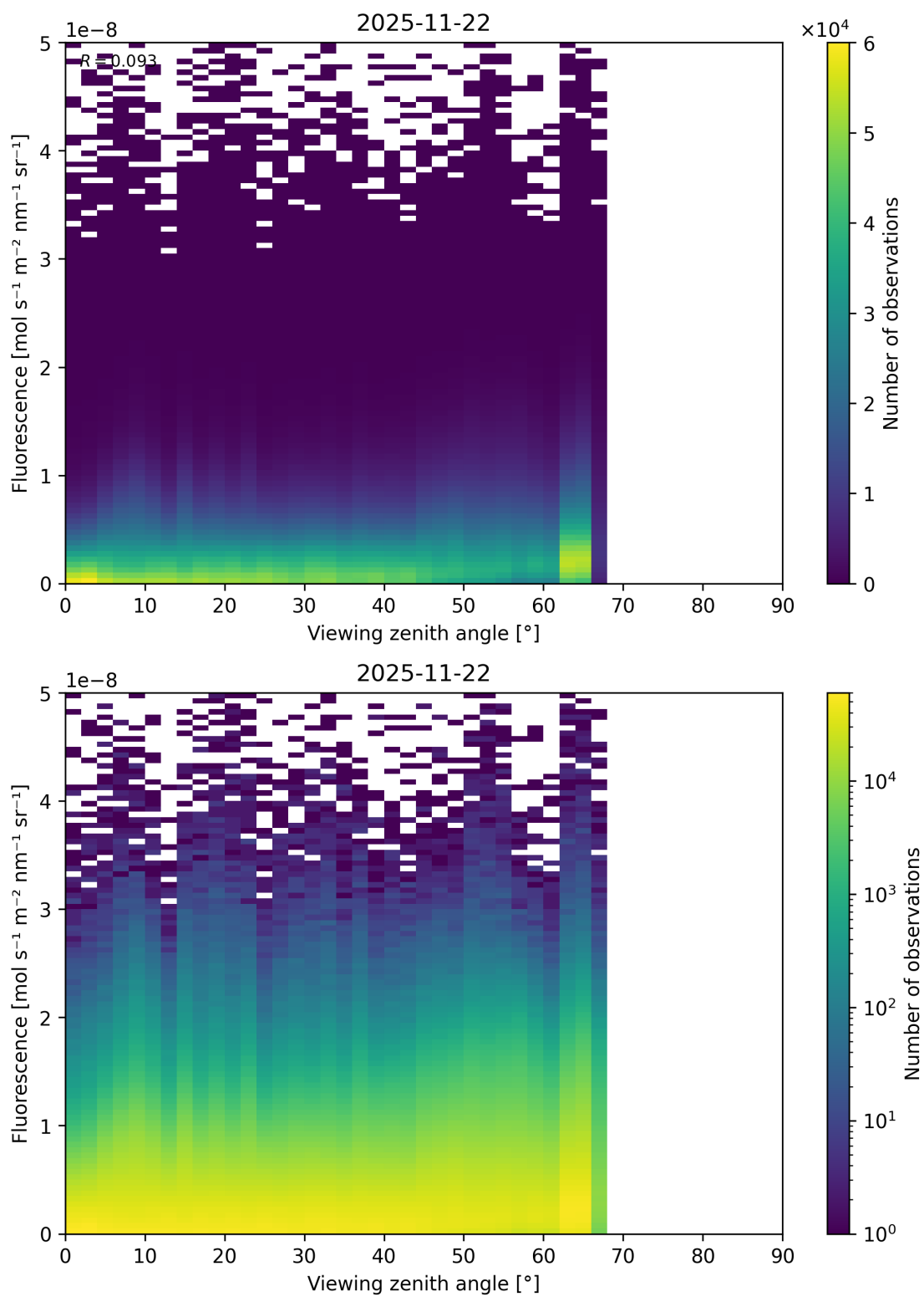
Figure 122: Scatter density plot of “Viewing zenith angle” against “Fluorescence” for 2025-11-21 to 2025-11-23.
