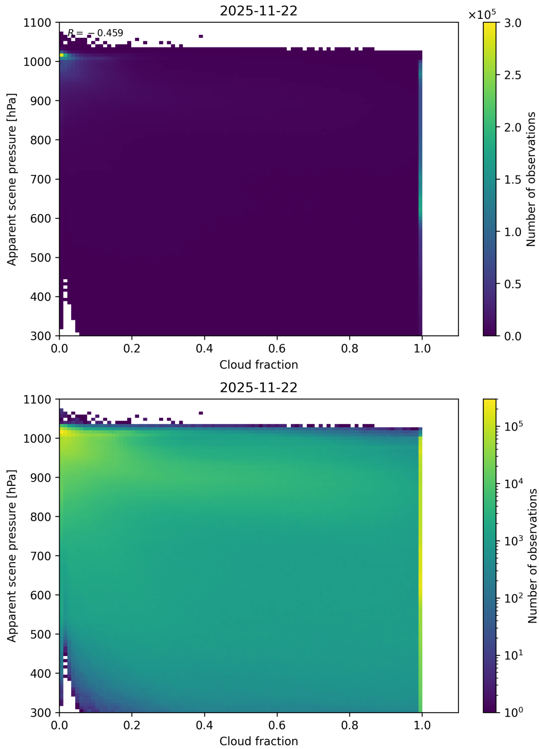
Figure 70: Scatter density plot of “Cloud fraction” against “Apparent scene pressure” for 2025-11-21 to 2025-11-23.
