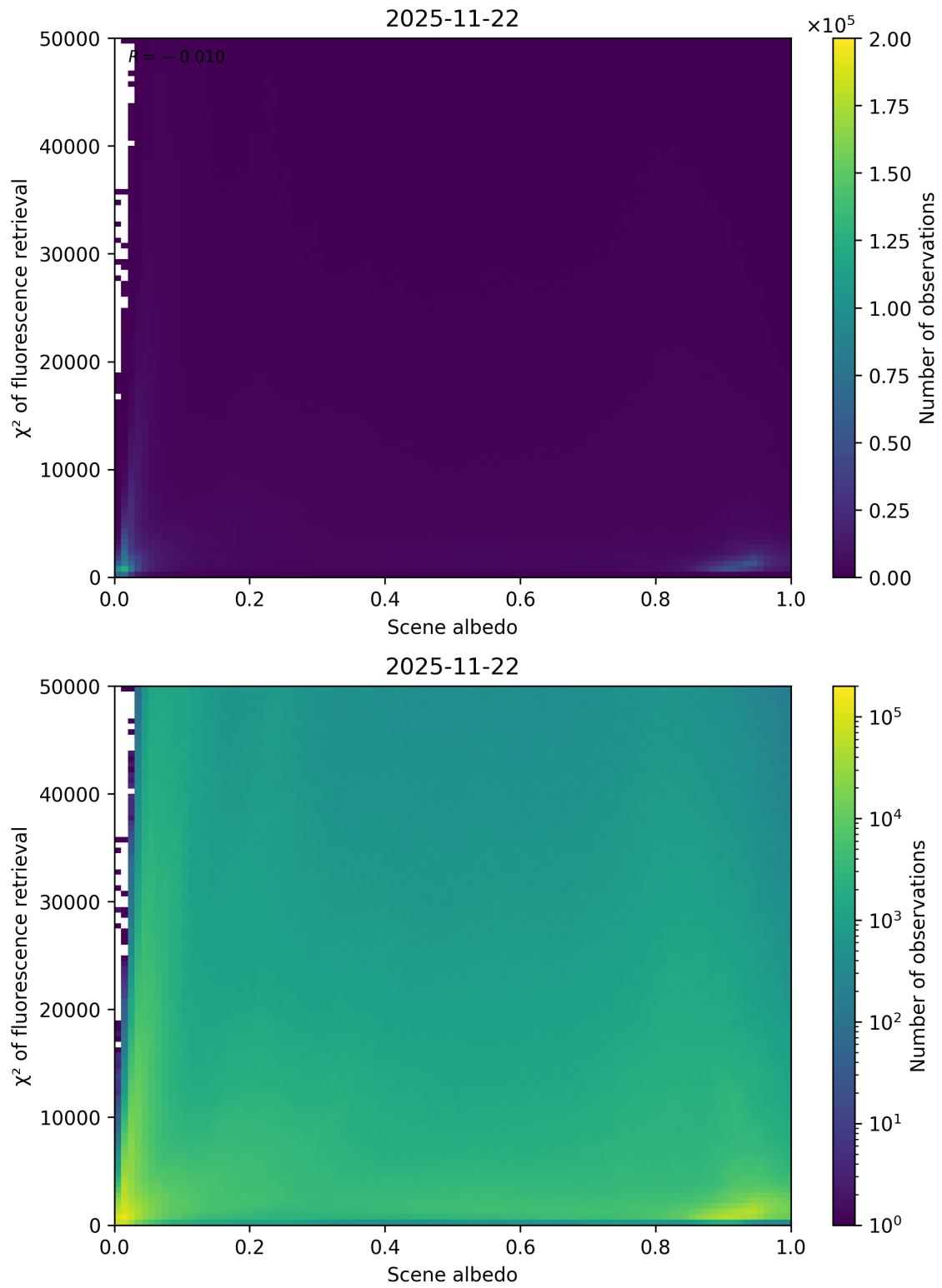
Figure 103: Scatter density plot of “Scene albedo” against “ \chi^2 of fluorescence retrieval” for 2025-11-21 to 2025-11-23.
