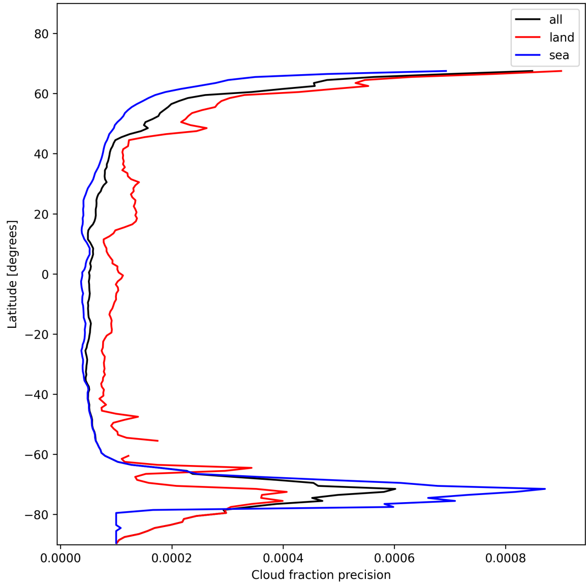
Figure 16: Zonal average of “Cloud fraction precision” for 2025-11-21 to 2025-11-23.
