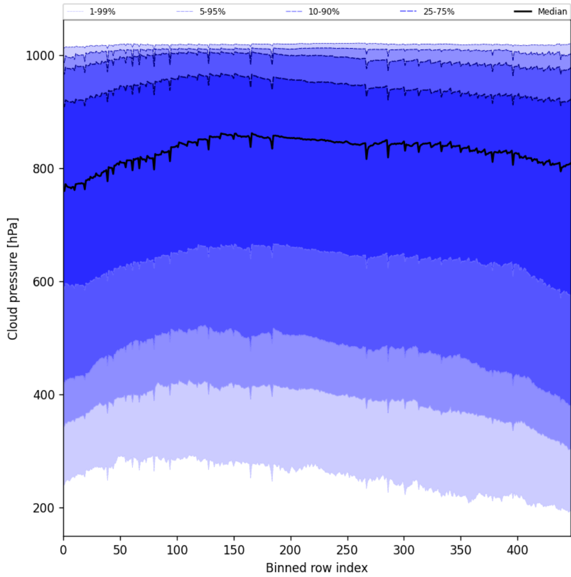
Figure 47: Along track statistics of “Cloud pressure” for 2025-11-21 to 2025-11-23
