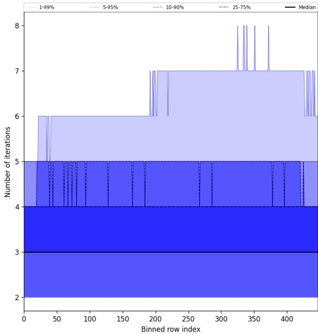
Figure 56: Along track statistics of “Number of iterations” for 2025-11-21 to 2025-11-23
