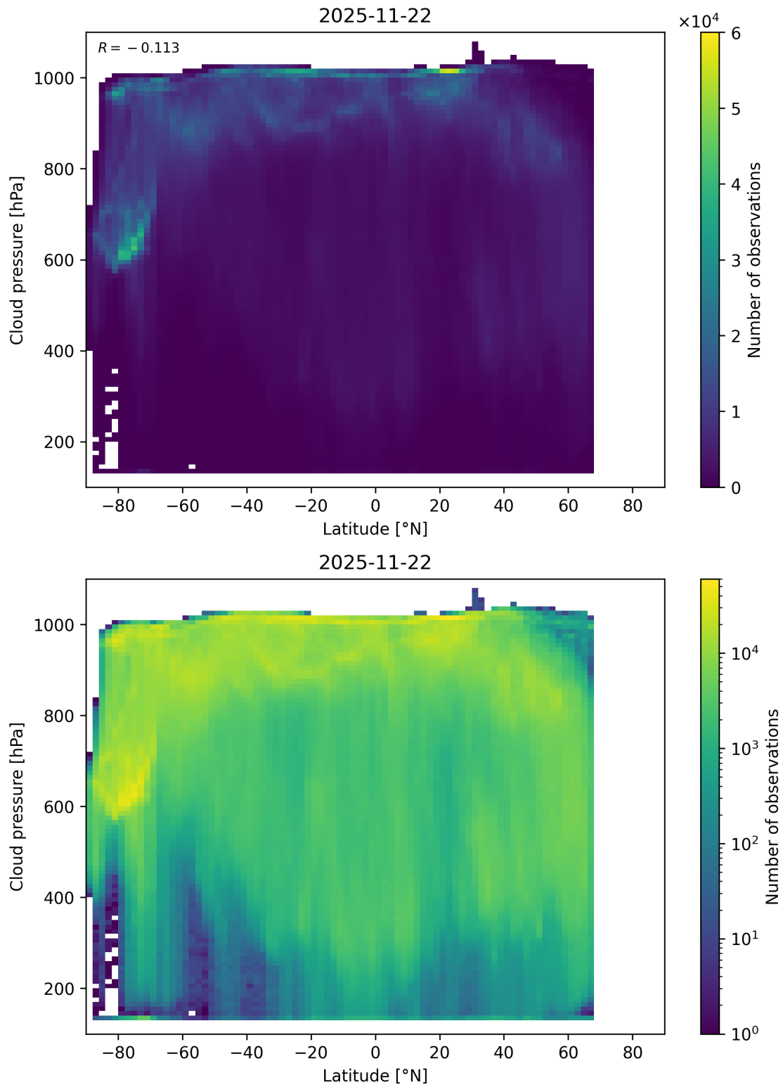
Figure 91: Scatter density plot of “Latitude” against “Cloud pressure” for 2025-11-21 to 2025-11-23.
