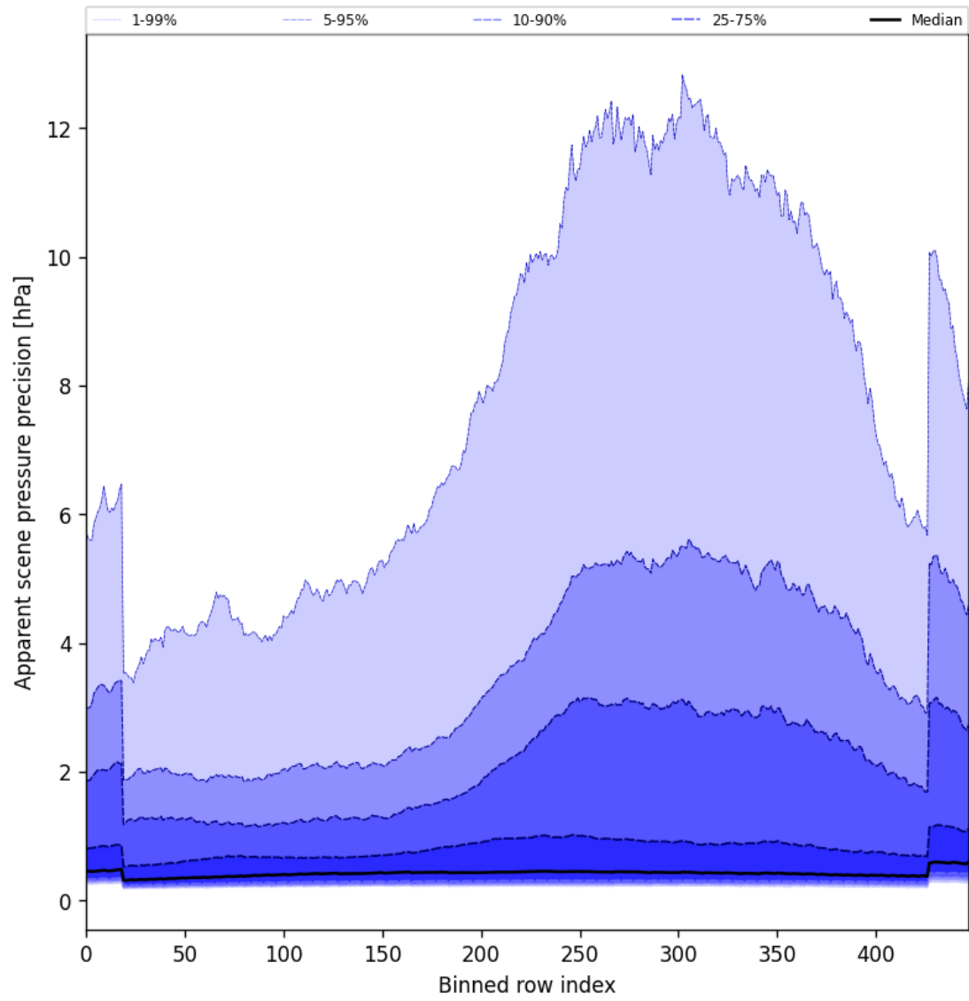
Figure 54: Along track statistics of “Apparent scene pressure precision” for 2025-11-21 to 2025-11-23
