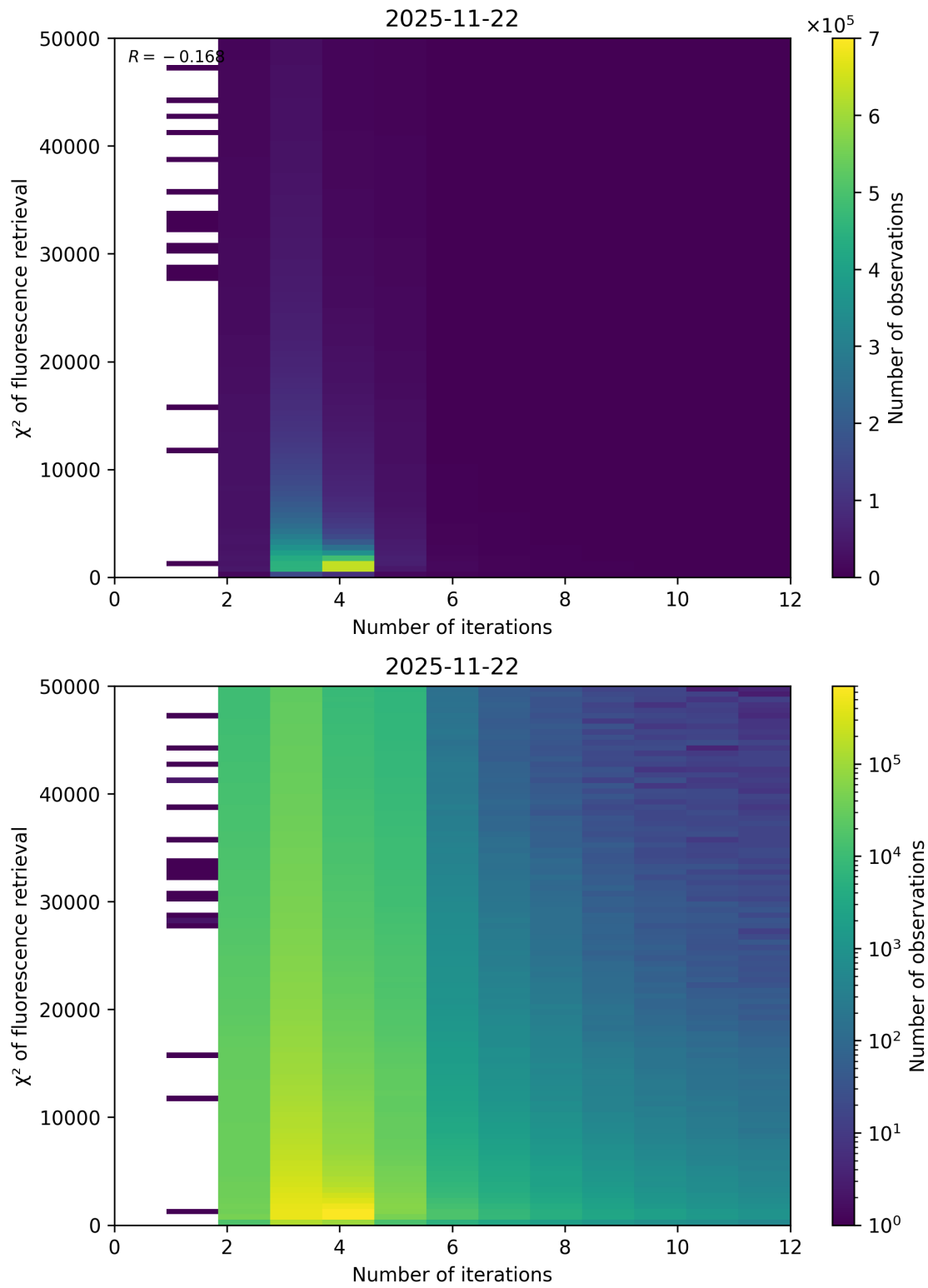
Figure 97: Scatter density plot of “Number of iterations” against “ \chi^2 of fluorescence retrieval” for 2025-11-21 to 2025-11-23.
