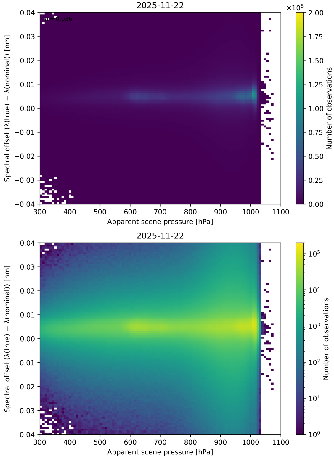
Figure 67: Scatter density plot of “Apparent scene pressure” against “Spectral offset ( \lambda_{\text{true}} - \lambda_{\text{nominal}} )” for 2025-11-21 to 2025-11-23.
