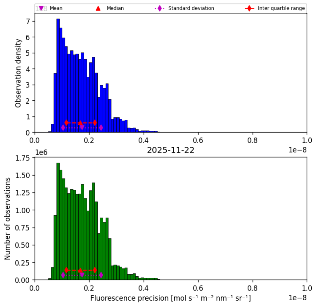
Figure 41: Histogram of “Fluorescence precision” for 2025-11-21 to 2025-11-23
