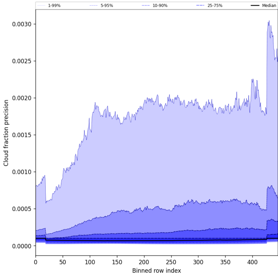
Figure 50: Along track statistics of “Cloud fraction precision” for 2025-11-21 to 2025-11-23
