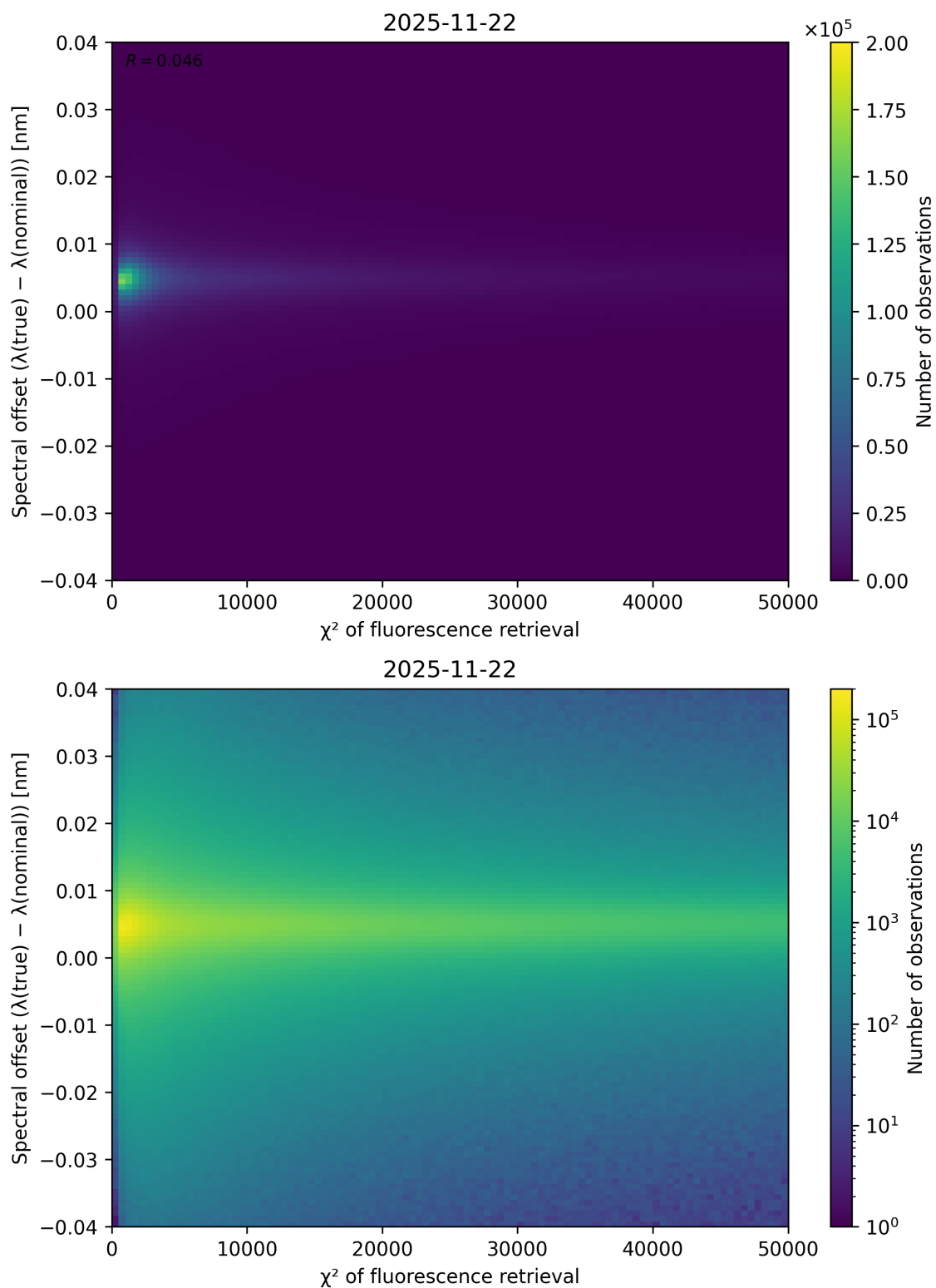
Figure 69: Scatter density plot of “ \chi^2 of fluorescence retrieval” against “Spectral offset ( \lambda_{\text{true}} - \lambda_{\text{nominal}} )” for 2025-11-21 to 2025-11-23.
