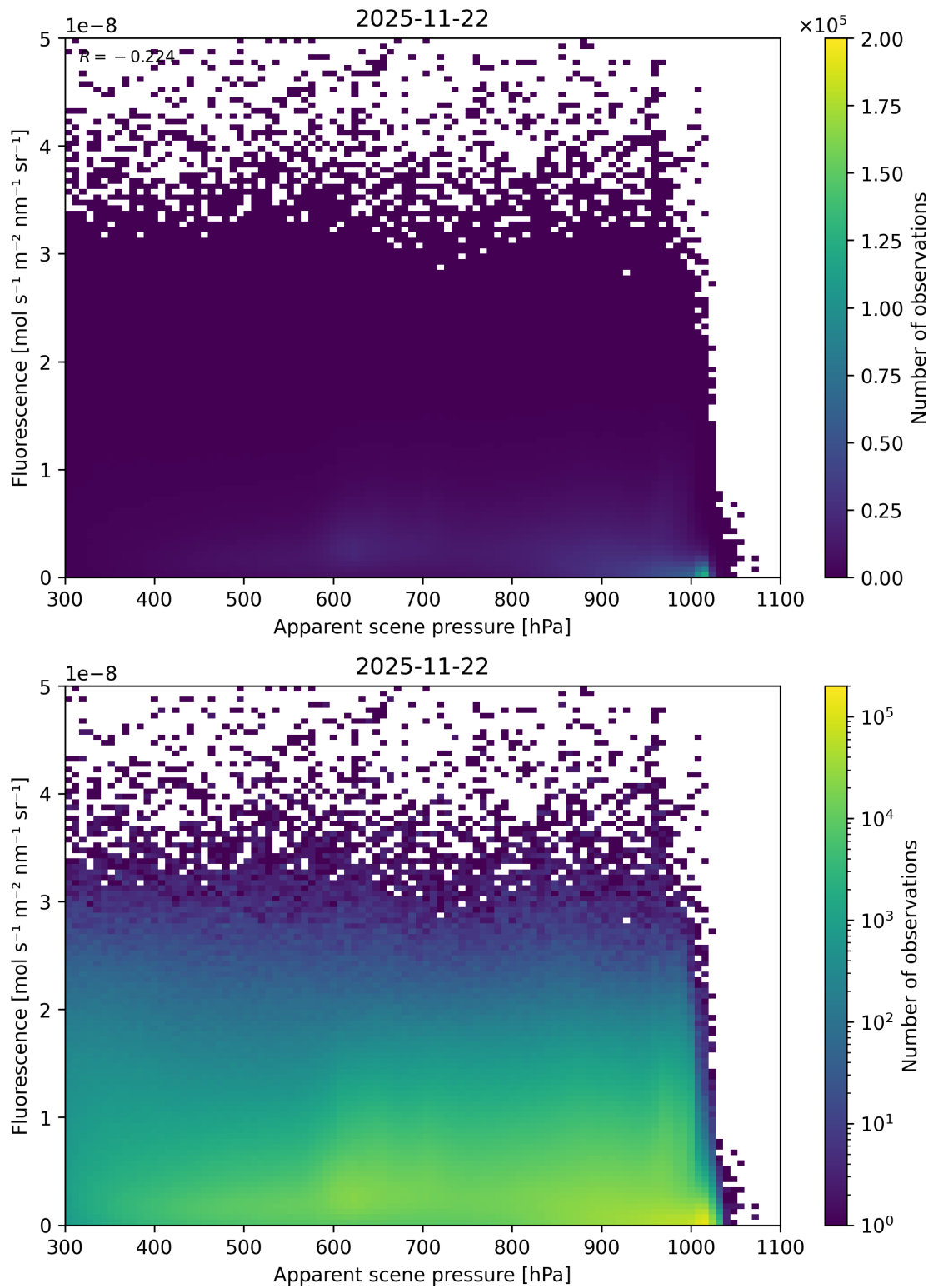
Figure 64: Scatter density plot of “Apparent scene pressure” against “Fluorescence” for 2025-11-21 to 2025-11-23.
