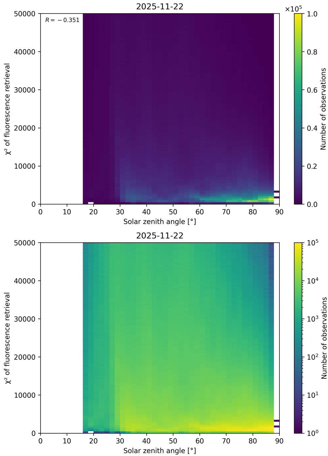
Figure 109: Scatter density plot of “Solar zenith angle” against “ \chi^2 of fluorescence retrieval” for 2025-11-21 to 2025-11-23.
