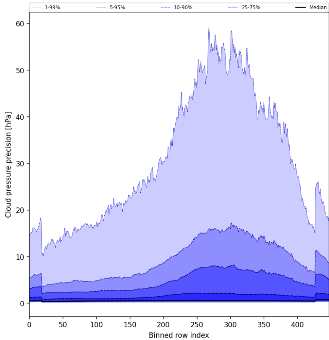
Figure 48: Along track statistics of “Cloud pressure precision” for 2025-11-21 to 2025-11-23
