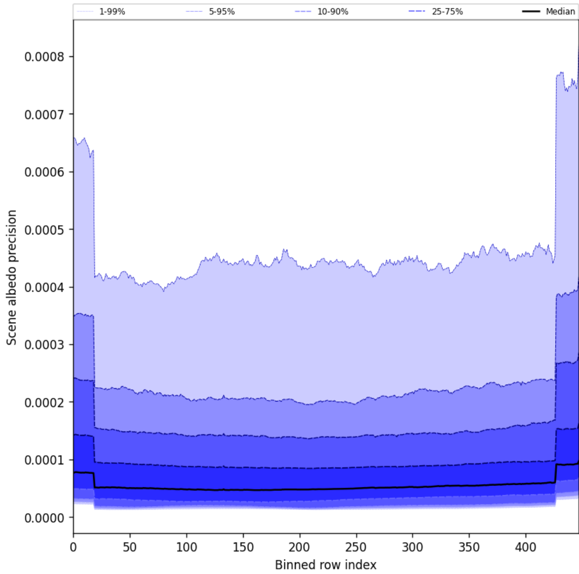
Figure 52: Along track statistics of “Scene albedo precision” for 2025-11-21 to 2025-11-23
