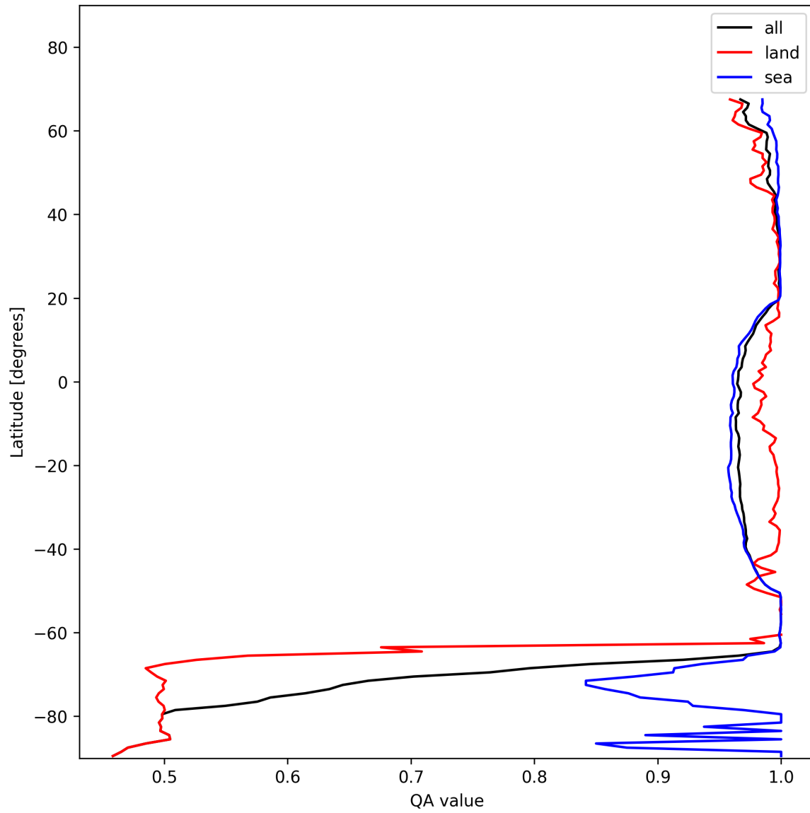
Figure 12: Zonal average of “QA value” for 2025-11-21 to 2025-11-23.
