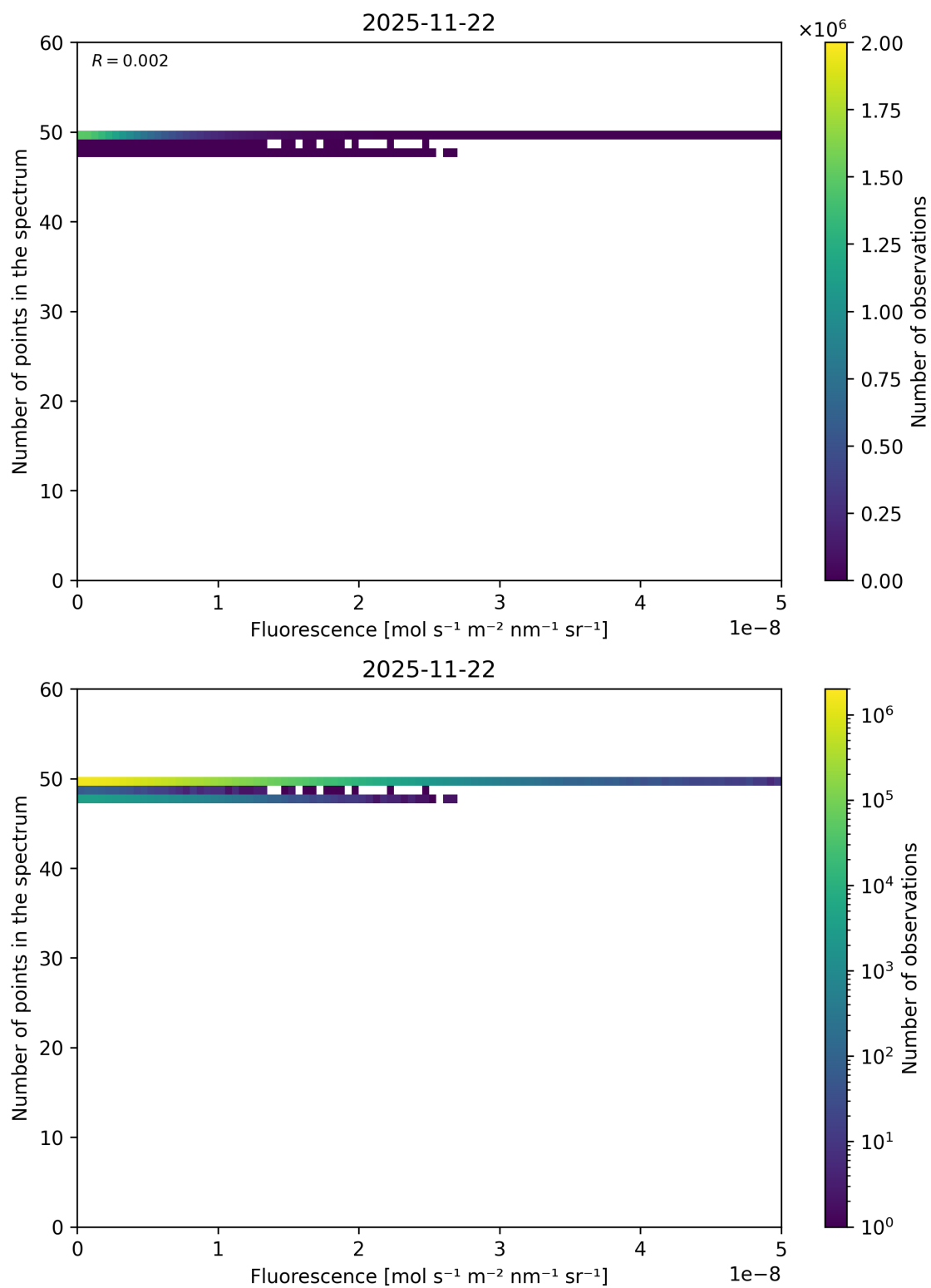
Figure 86: Scatter density plot of “Fluorescence” against “Number of points in the spectrum” for 2025-11-21 to 2025-11-23.
