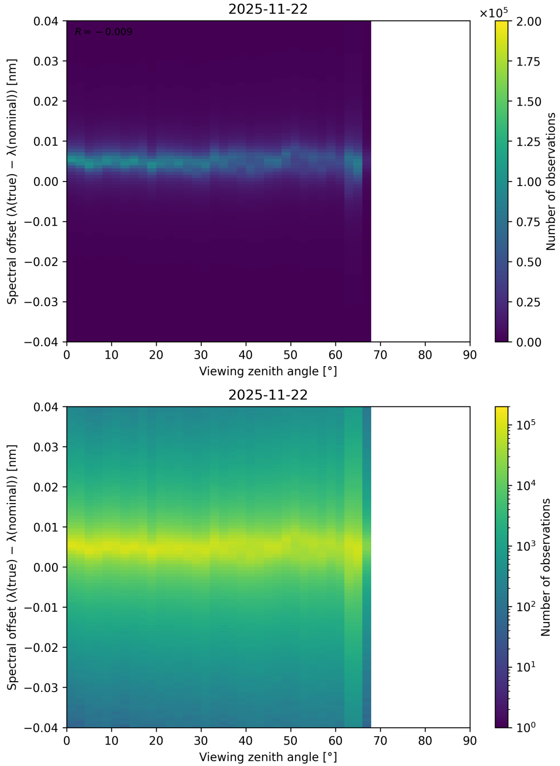
Figure 128: Scatter density plot of “Viewing zenith angle” against “Spectral offset ( \lambda_{\text{true}} - \lambda_{\text{nominal}} )” for 2025-11-21 to 2025-11-23.
