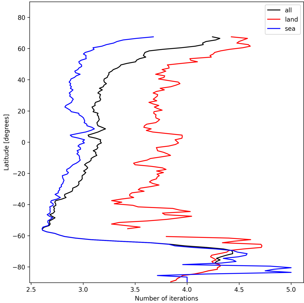
Figure 22: Zonal average of “Number of iterations” for 2025-11-21 to 2025-11-23.
