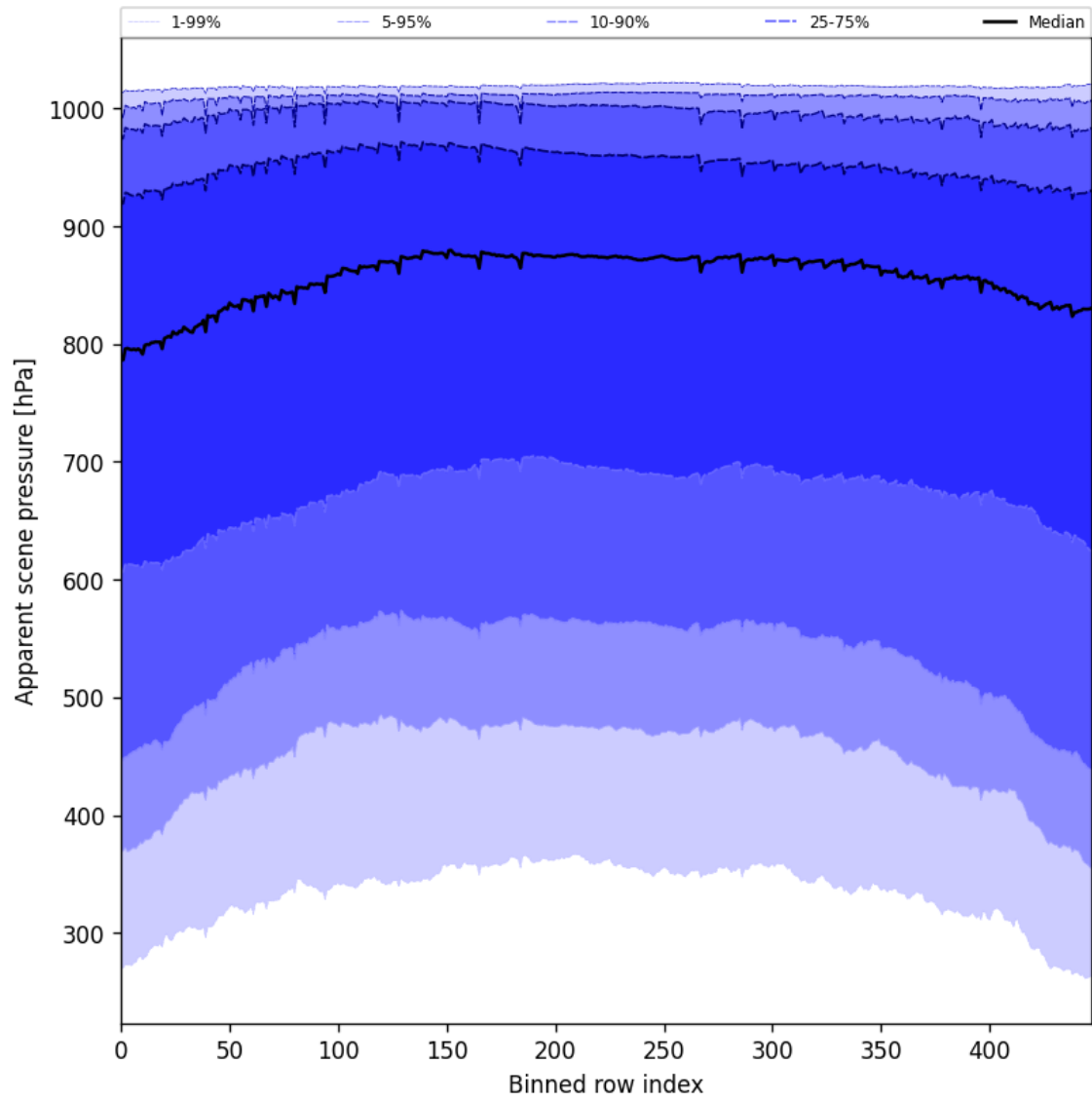
Figure 53: Along track statistics of “Apparent scene pressure” for 2025-11-21 to 2025-11-23
