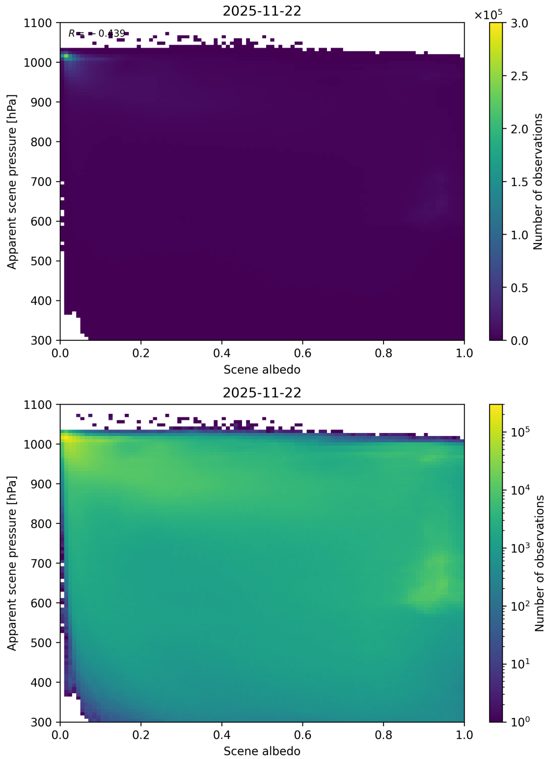
Figure 102: Scatter density plot of “Scene albedo” against “Apparent scene pressure” for 2025-11-21 to 2025-11-23.
