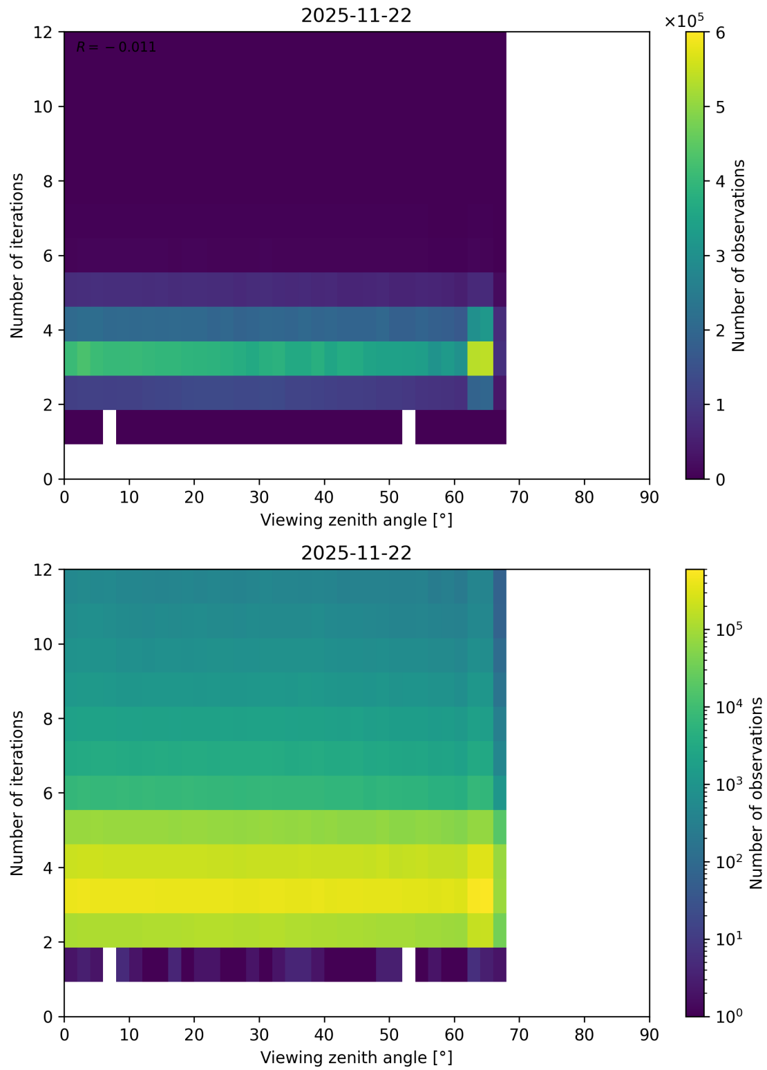
Figure 124: Scatter density plot of “Viewing zenith angle” against “Number of iterations” for 2025-11-21 to 2025-11-23.
