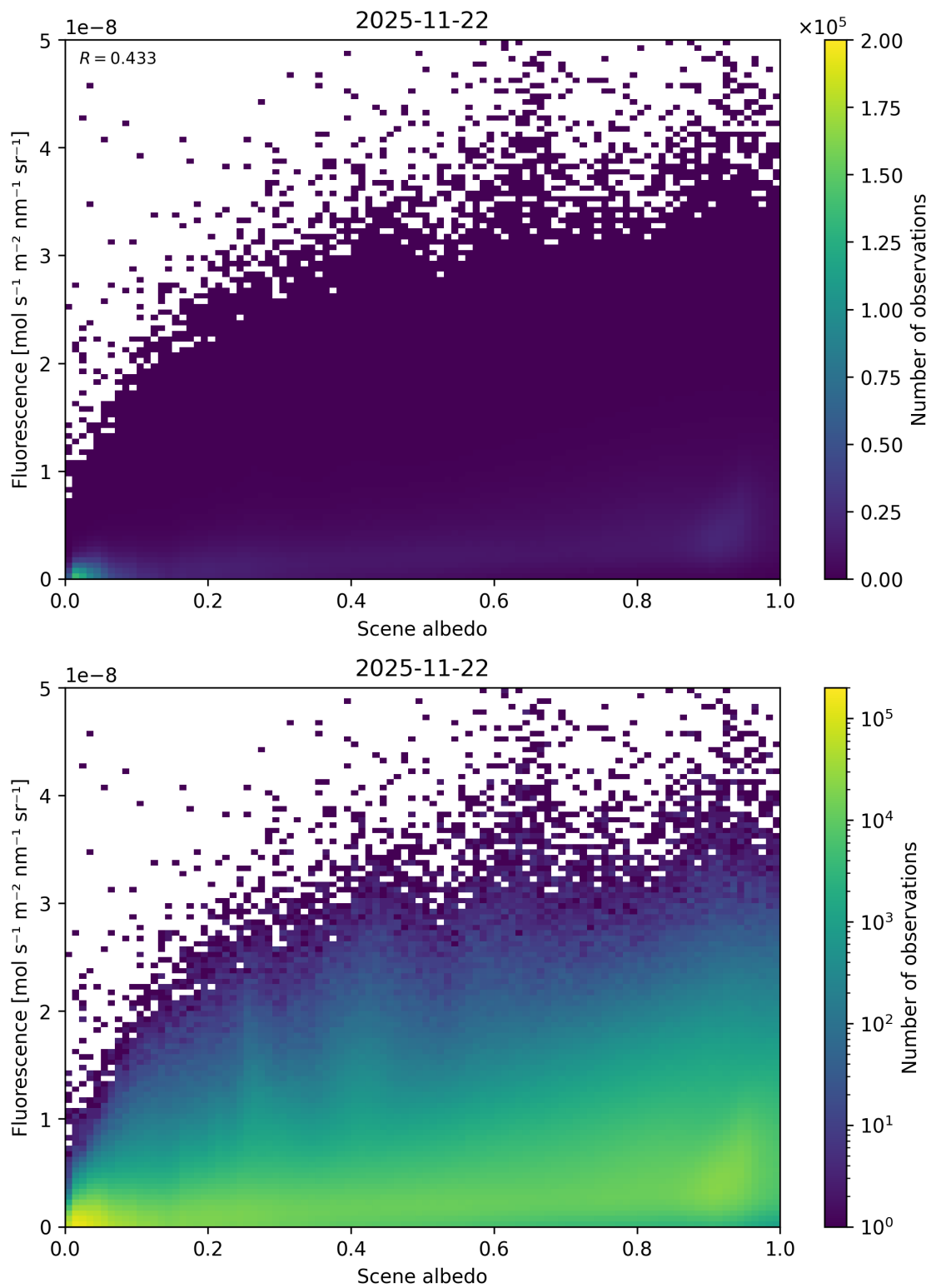
Figure 104: Scatter density plot of “Scene albedo” against “Fluorescence” for 2025-11-21 to 2025-11-23.
