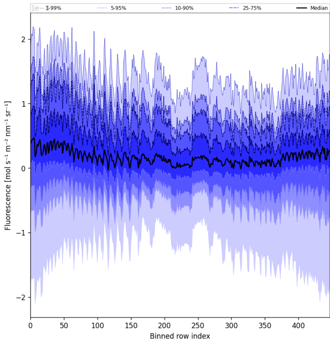
Figure 57: Along track statistics of “Fluorescence” for 2025-11-21 to 2025-11-23
