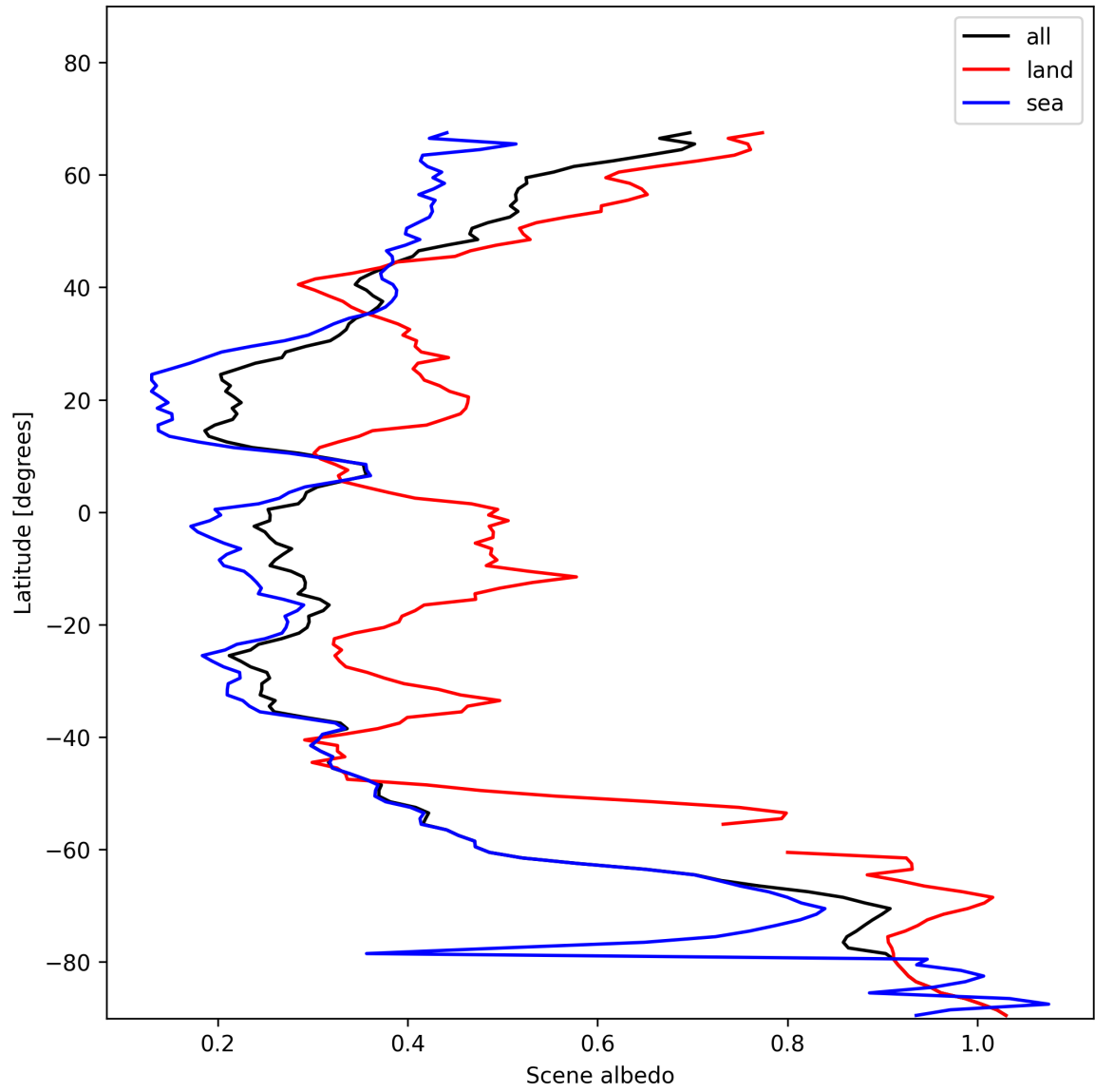
Figure 17: Zonal average of “Scene albedo” for 2025-11-21 to 2025-11-23.
