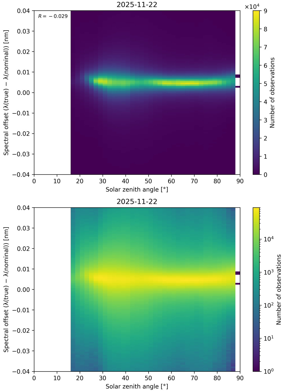
Figure 117: Scatter density plot of “Solar zenith angle” against “Spectral offset ( \lambda_{\text{true}} - \lambda_{\text{nominal}} )” for 2025-11-21 to 2025-11-23.
