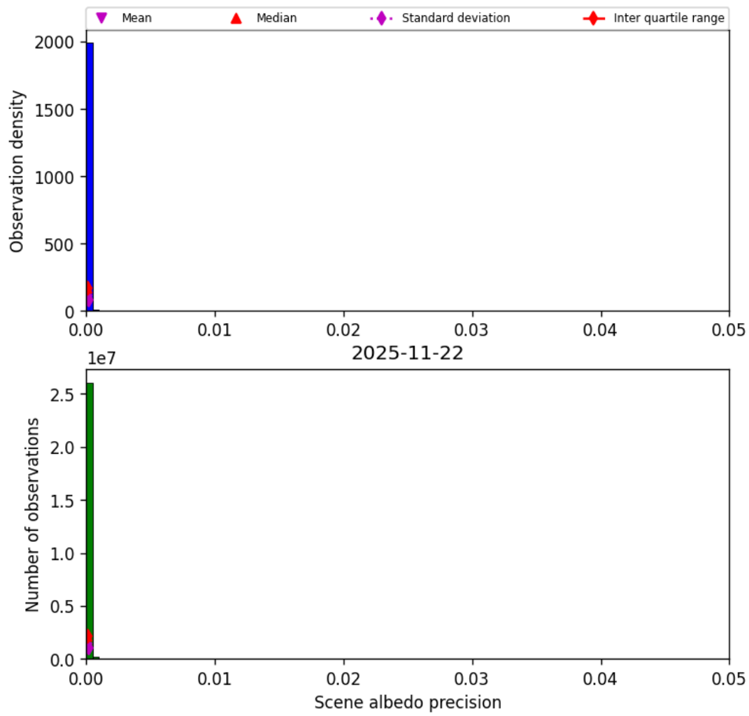
Figure 35: Histogram of “Scene albedo precision” for 2025-11-21 to 2025-11-23
