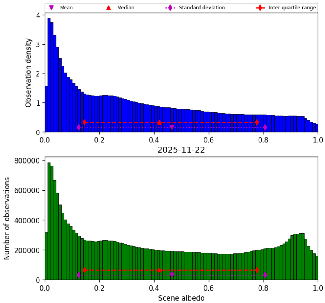
Figure 34: Histogram of “Scene albedo” for 2025-11-21 to 2025-11-23
