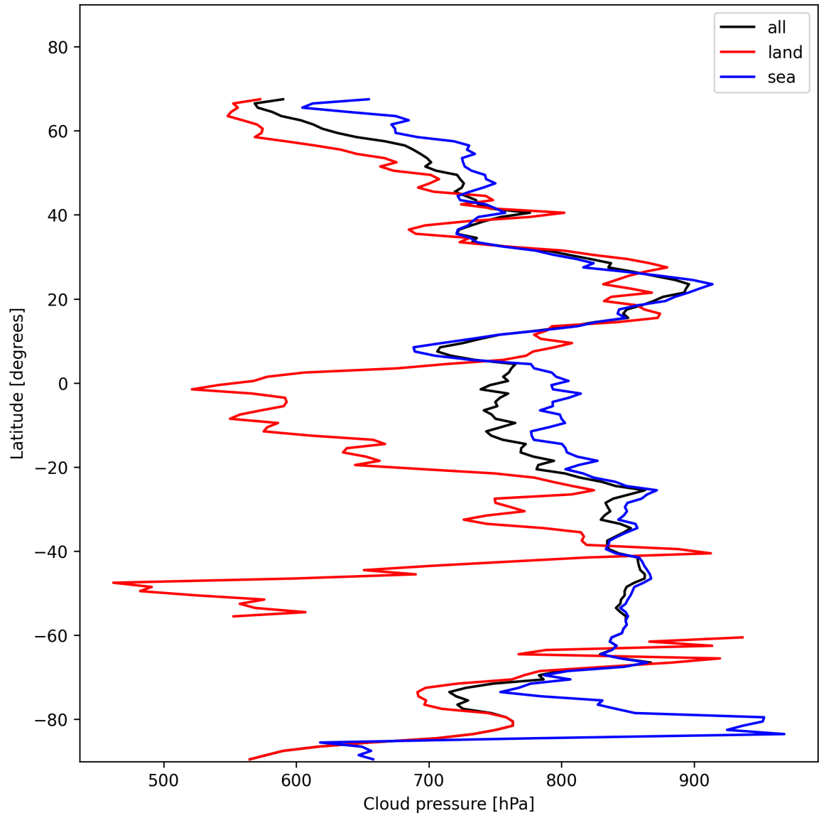
Figure 13: Zonal average of “Cloud pressure” for 2025-11-21 to 2025-11-23.
