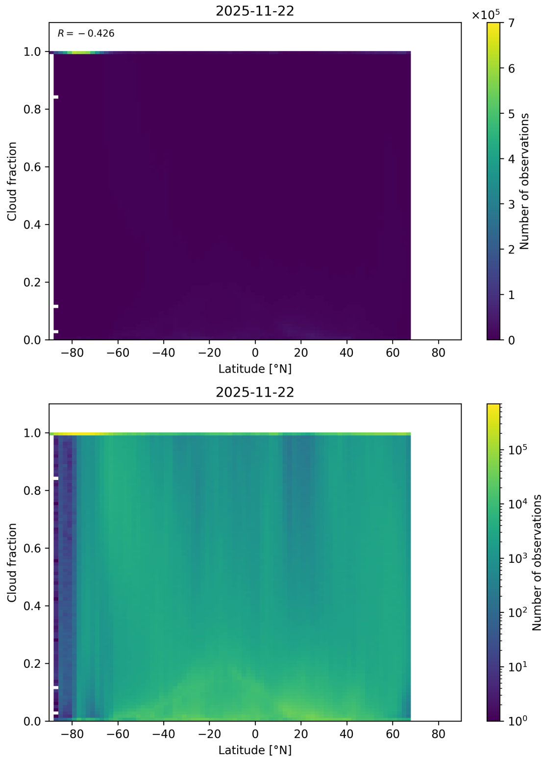
Figure 90: Scatter density plot of “Latitude” against “Cloud fraction” for 2025-11-21 to 2025-11-23.
