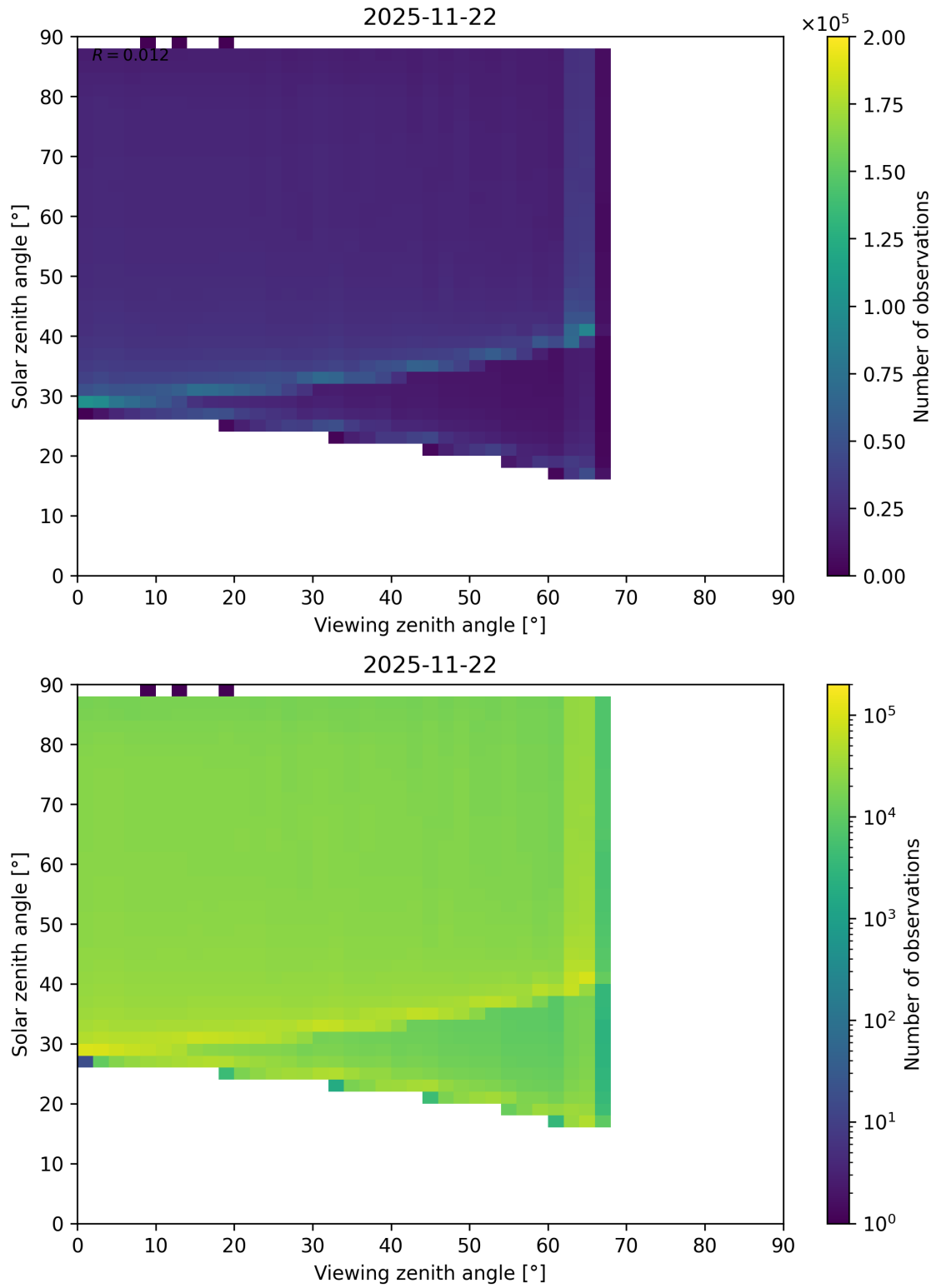
Figure 127: Scatter density plot of “Viewing zenith angle” against “Solar zenith angle” for 2025-11-21 to 2025-11-23.
