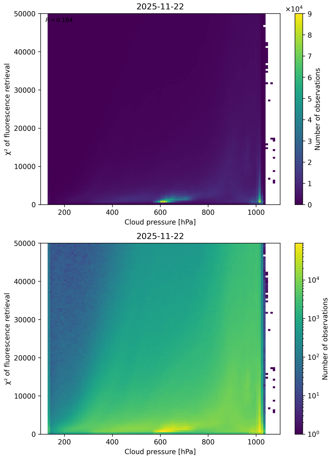
Figure 78: Scatter density plot of “Cloud pressure” against “ \chi^2 of fluorescence retrieval” for 2025-11-21 to 2025-11-23.
