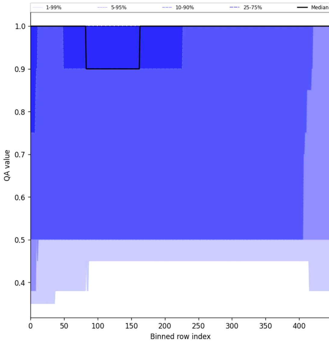
Figure 46: Along track statistics of “QA value” for 2025-11-21 to 2025-11-23
