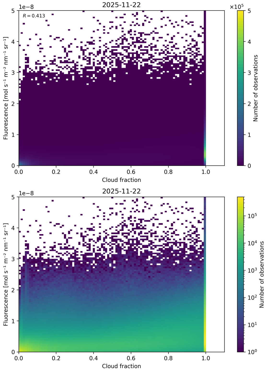
Figure 72: Scatter density plot of “Cloud fraction” against “Fluorescence” for 2025-11-21 to 2025-11-23.
