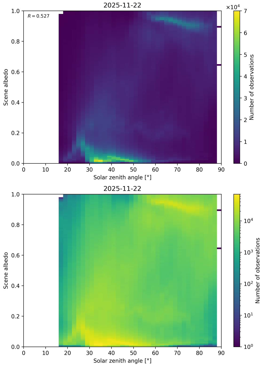
Figure 116: Scatter density plot of “Solar zenith angle” against “Scene albedo” for 2025-11-21 to 2025-11-23.
