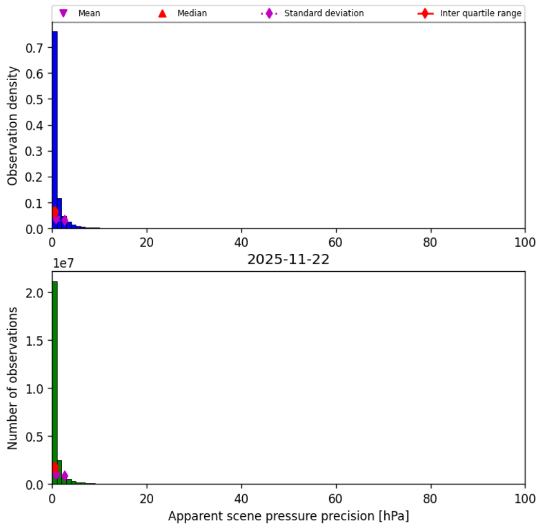
Figure 37: Histogram of “Apparent scene pressure precision” for 2025-11-21 to 2025-11-23
