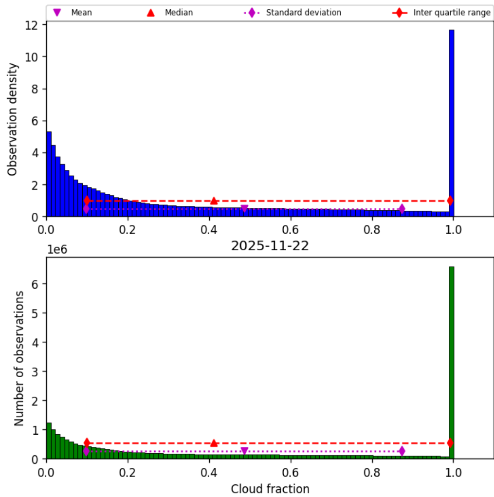
Figure 32: Histogram of "Cloud fraction" for 2025-11-21 to 2025-11-23
