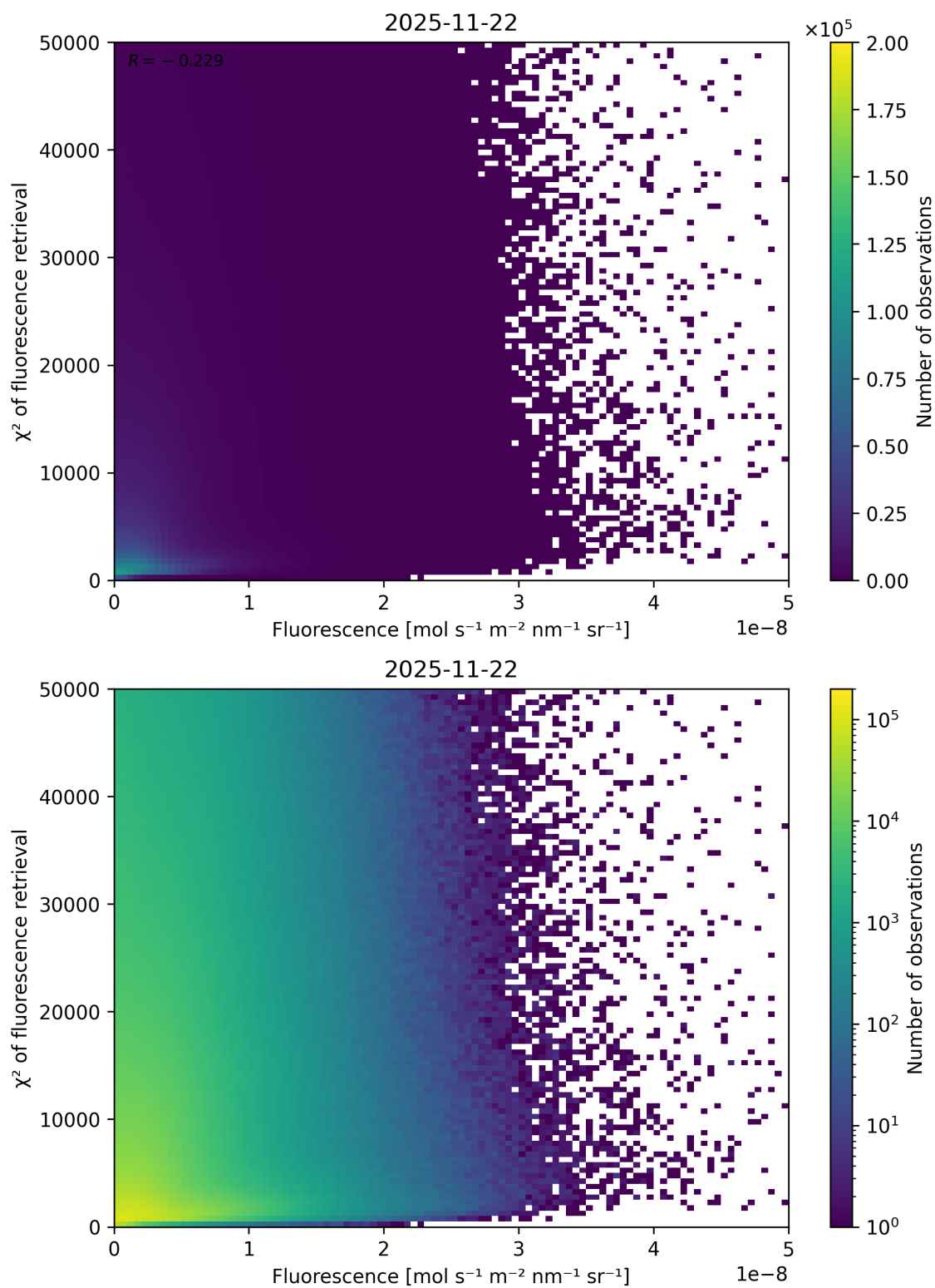
Figure 85: Scatter density plot of “Fluorescence” against “ \chi^2 of fluorescence retrieval” for 2025-11-21 to 2025-11-23.
