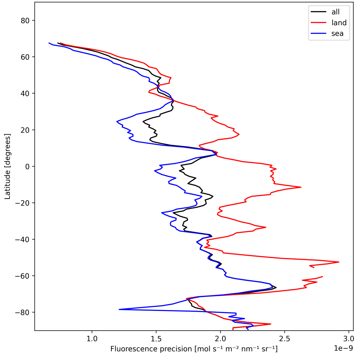
Figure 24: Zonal average of “Fluorescence precision” for 2025-11-21 to 2025-11-23.
