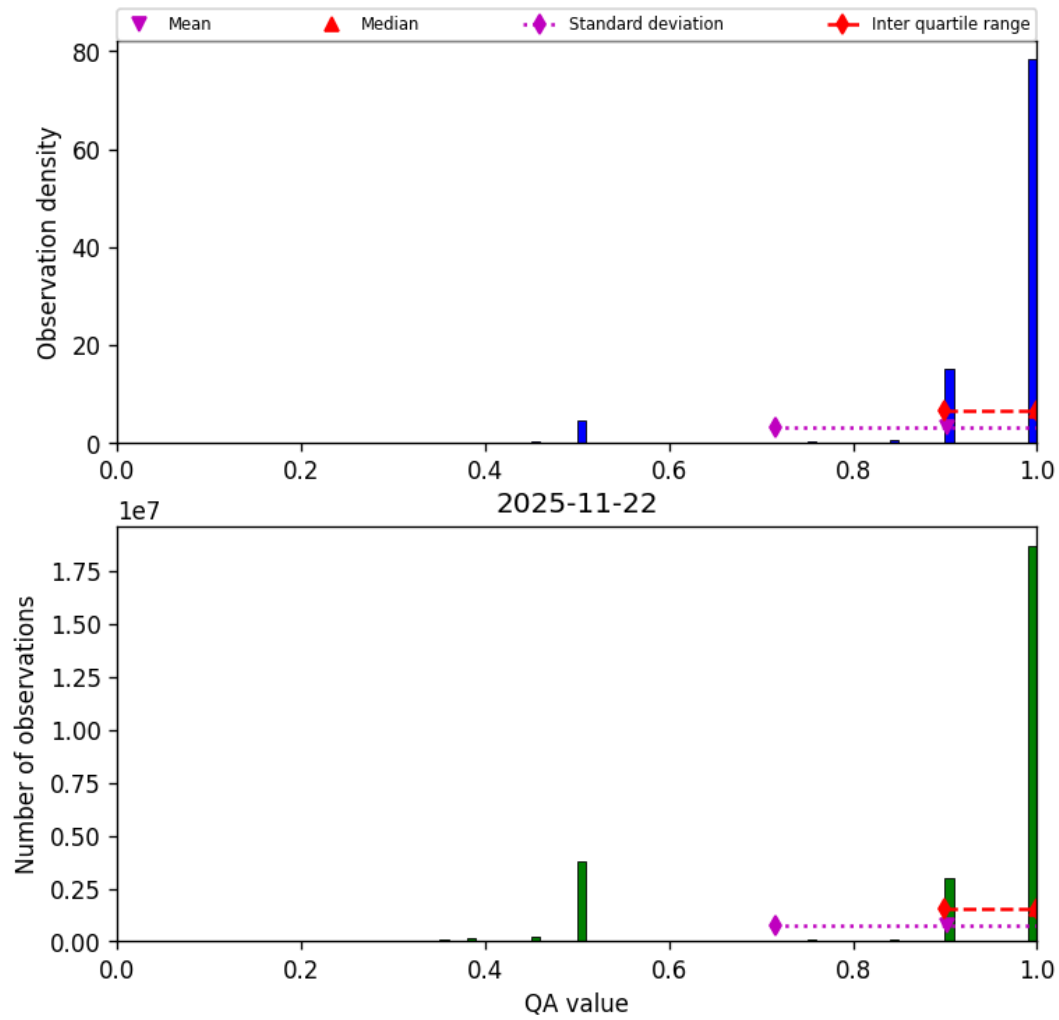
Figure 29: Histogram of “QA value” for 2025-11-21 to 2025-11-23
