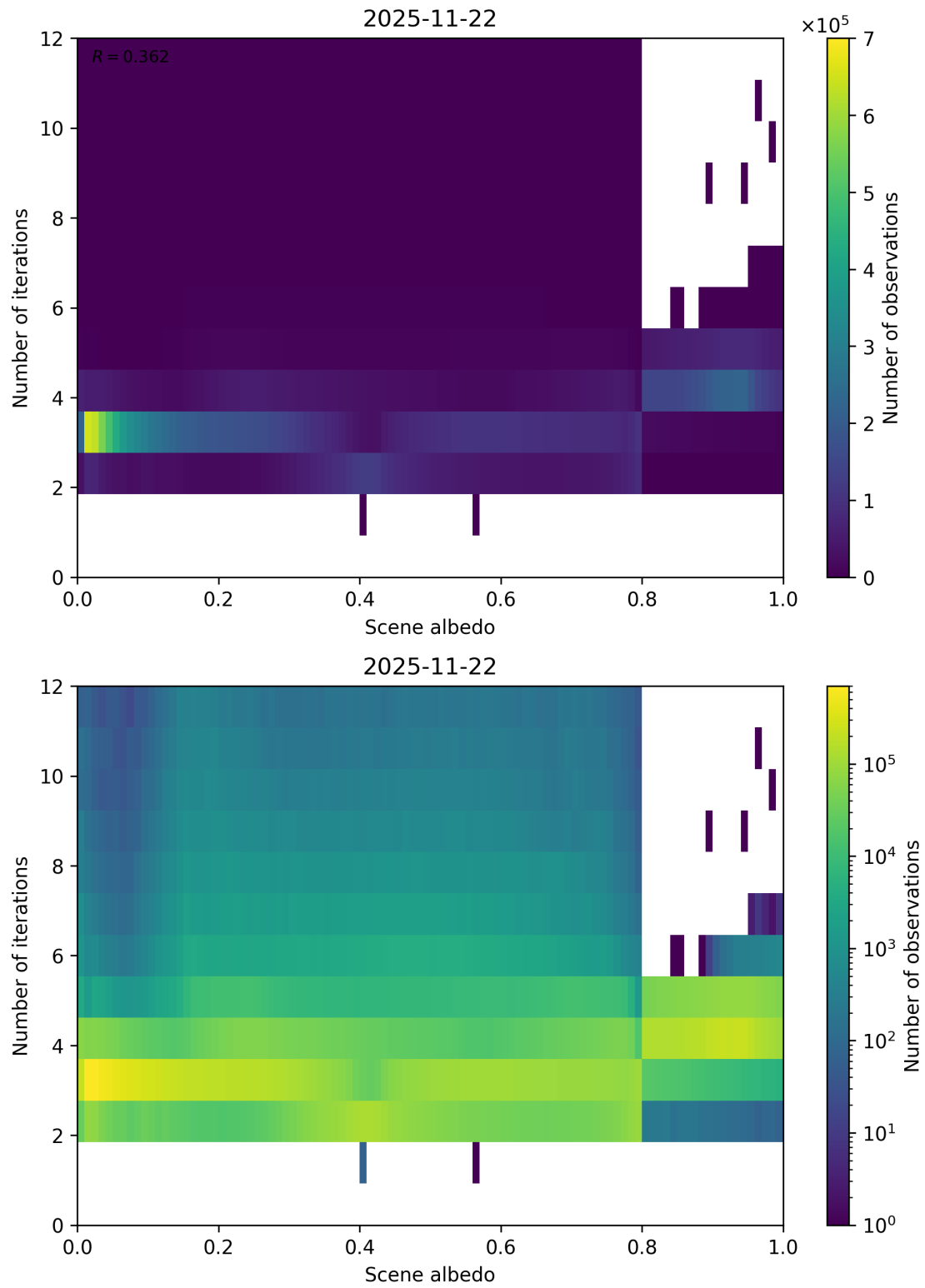
Figure 105: Scatter density plot of “Scene albedo” against “Number of iterations” for 2025-11-21 to 2025-11-23.
