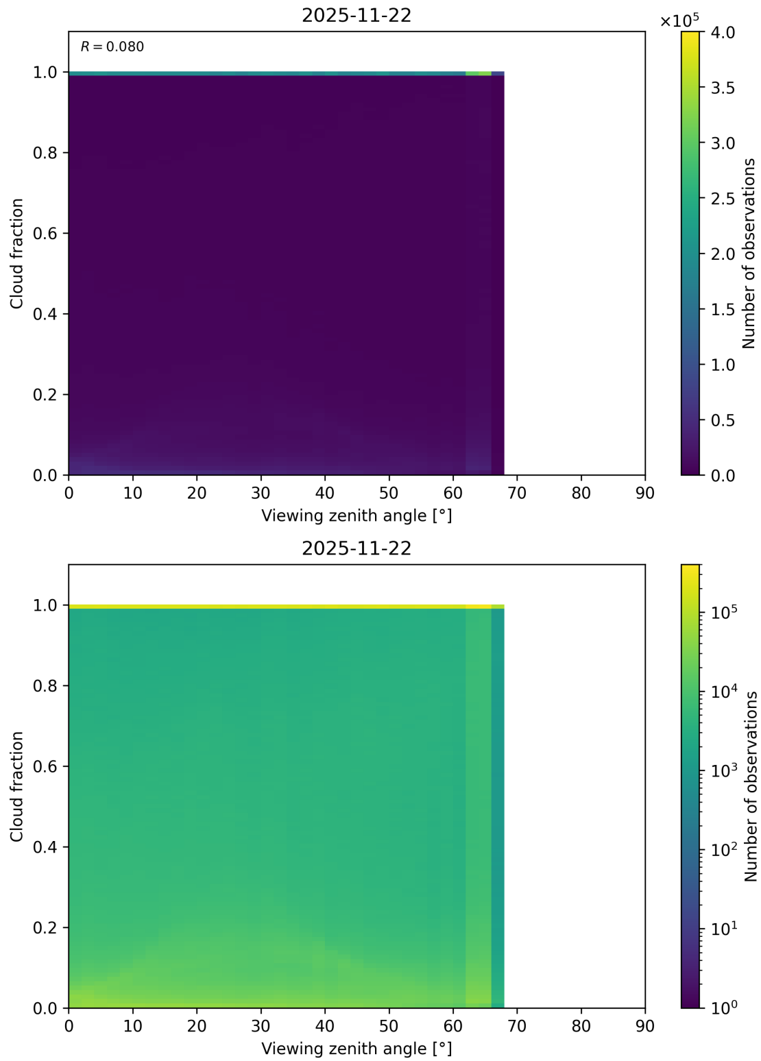
Figure 120: Scatter density plot of “Viewing zenith angle” against “Cloud fraction” for 2025-11-21 to 2025-11-23.
