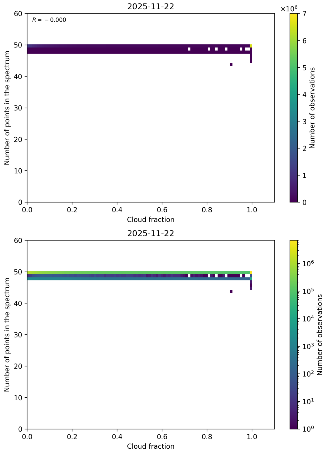
Figure 74: Scatter density plot of “Cloud fraction” against “Number of points in the spectrum” for 2025-11-21 to 2025-11-23.
