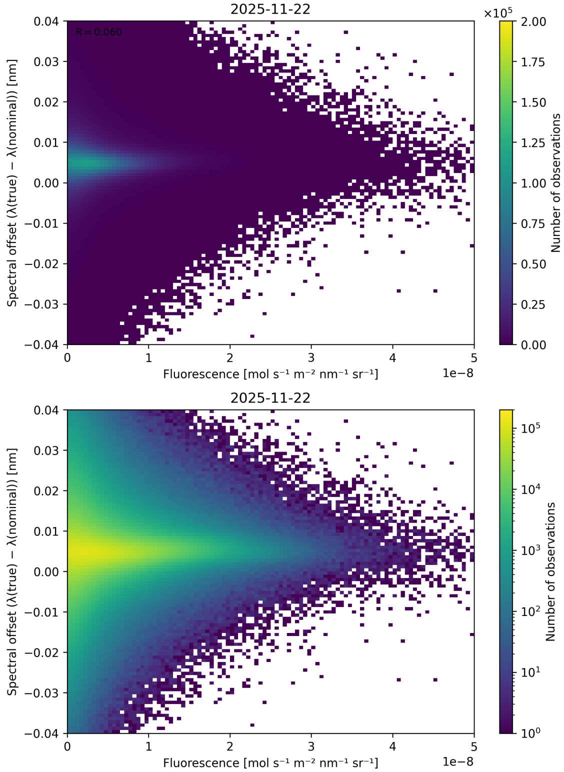
Figure 87: Scatter density plot of “Fluorescence” against “Spectral offset ( \lambda_{\text{true}} - \lambda_{\text{nominal}} )” for 2025-11-21 to 2025-11-23.
