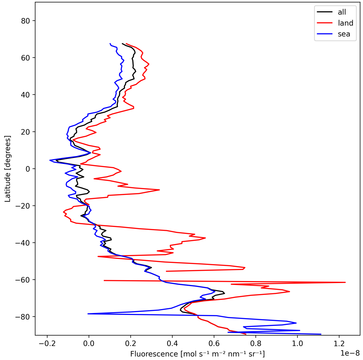
Figure 23: Zonal average of “Fluorescence” for 2025-11-21 to 2025-11-23.
