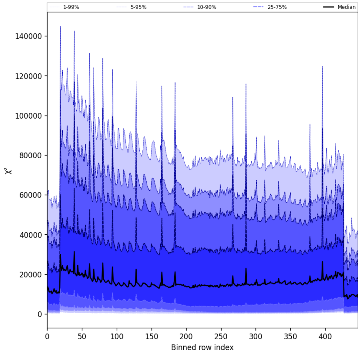
Figure 55: Along track statistics of “ \chi^2 ” for 2025-11-21 to 2025-11-23
