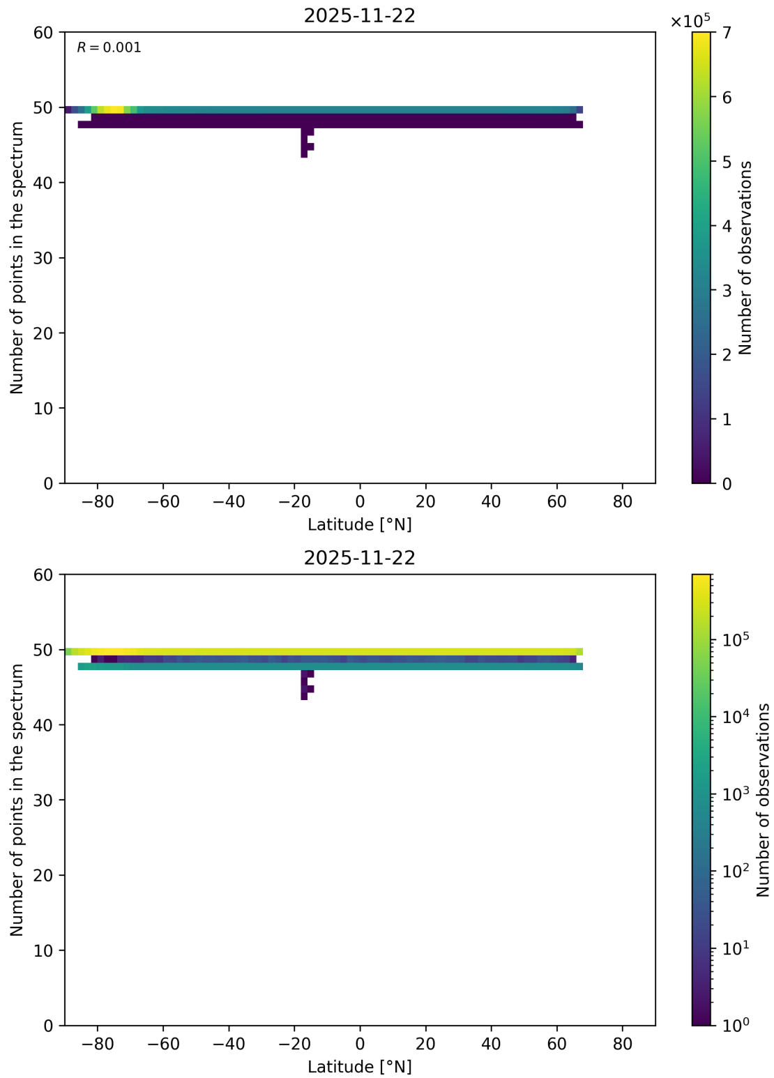
Figure 94: Scatter density plot of “Latitude” against “Number of points in the spectrum” for 2025-11-21 to 2025-11-23.
