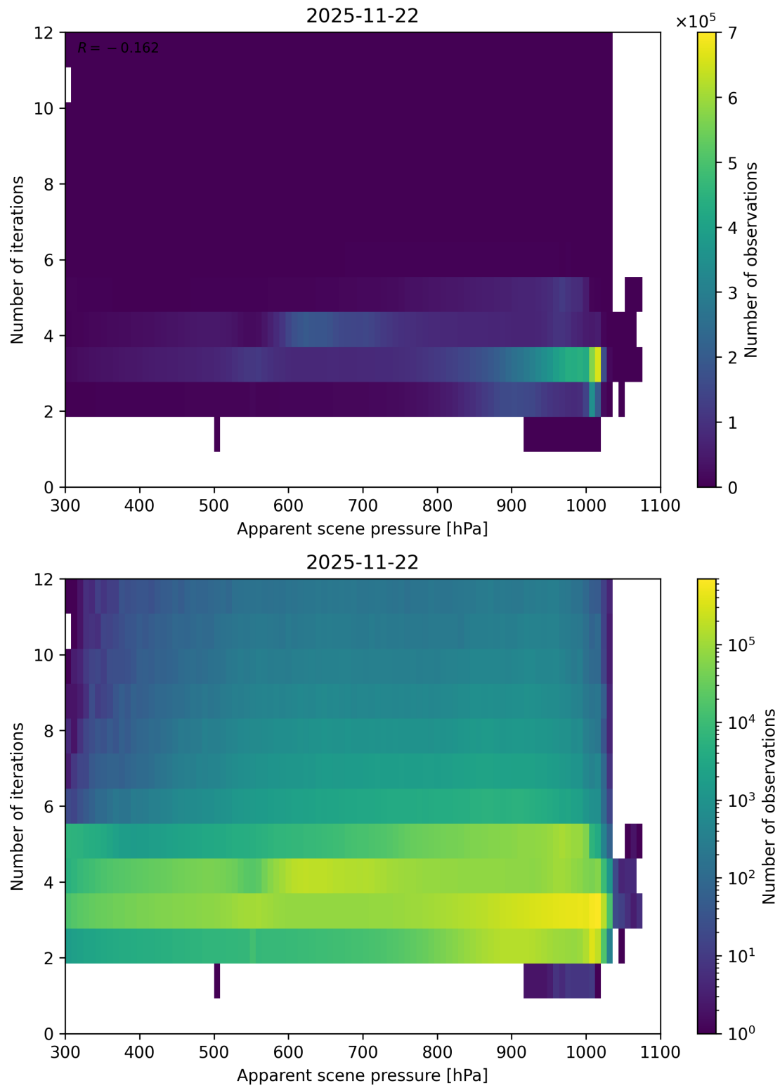
Figure 65: Scatter density plot of “Apparent scene pressure” against “Number of iterations” for 2025-11-21 to 2025-11-23.
