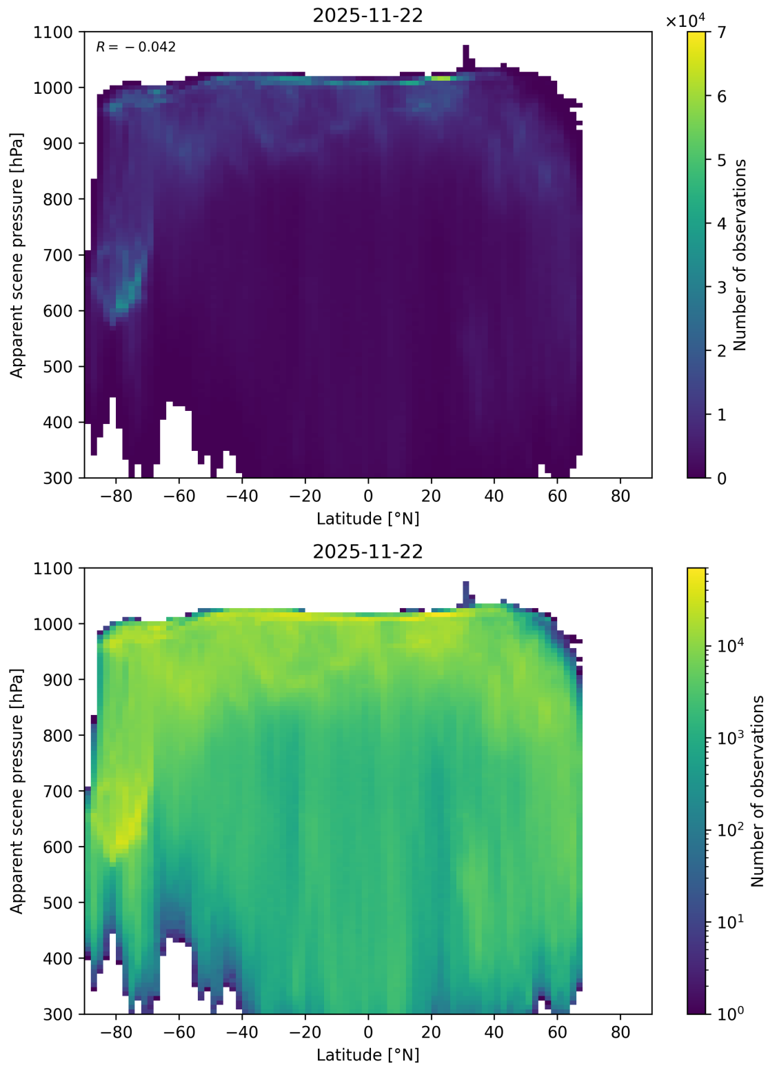
Figure 88: Scatter density plot of “Latitude” against “Apparent scene pressure” for 2025-11-21 to 2025-11-23.
