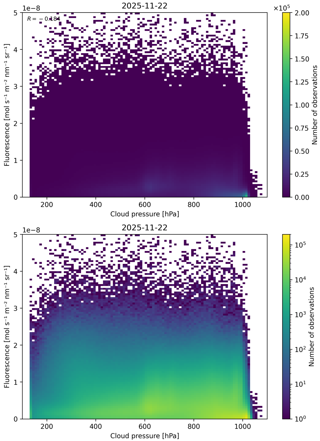
Figure 80: Scatter density plot of “Cloud pressure” against “Fluorescence” for 2025-11-21 to 2025-11-23.
