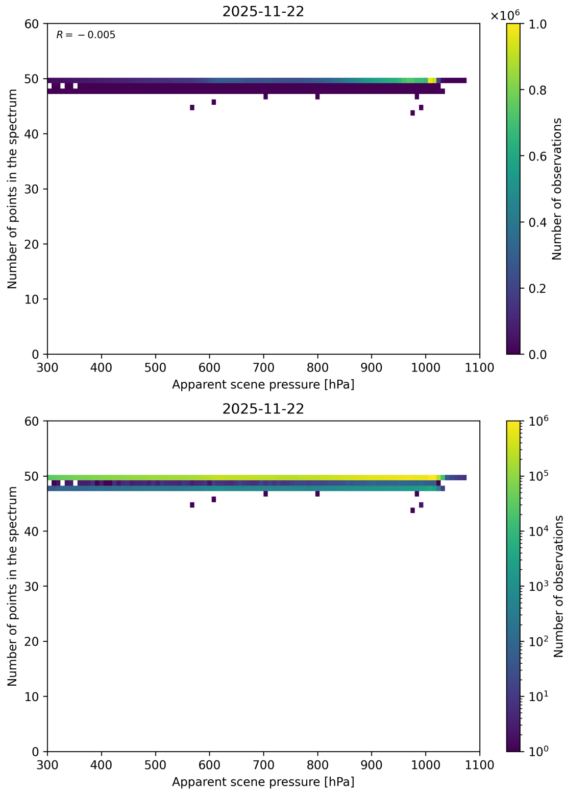
Figure 66: Scatter density plot of “Apparent scene pressure” against “Number of points in the spectrum” for 2025-11-21 to 2025-11-23.
