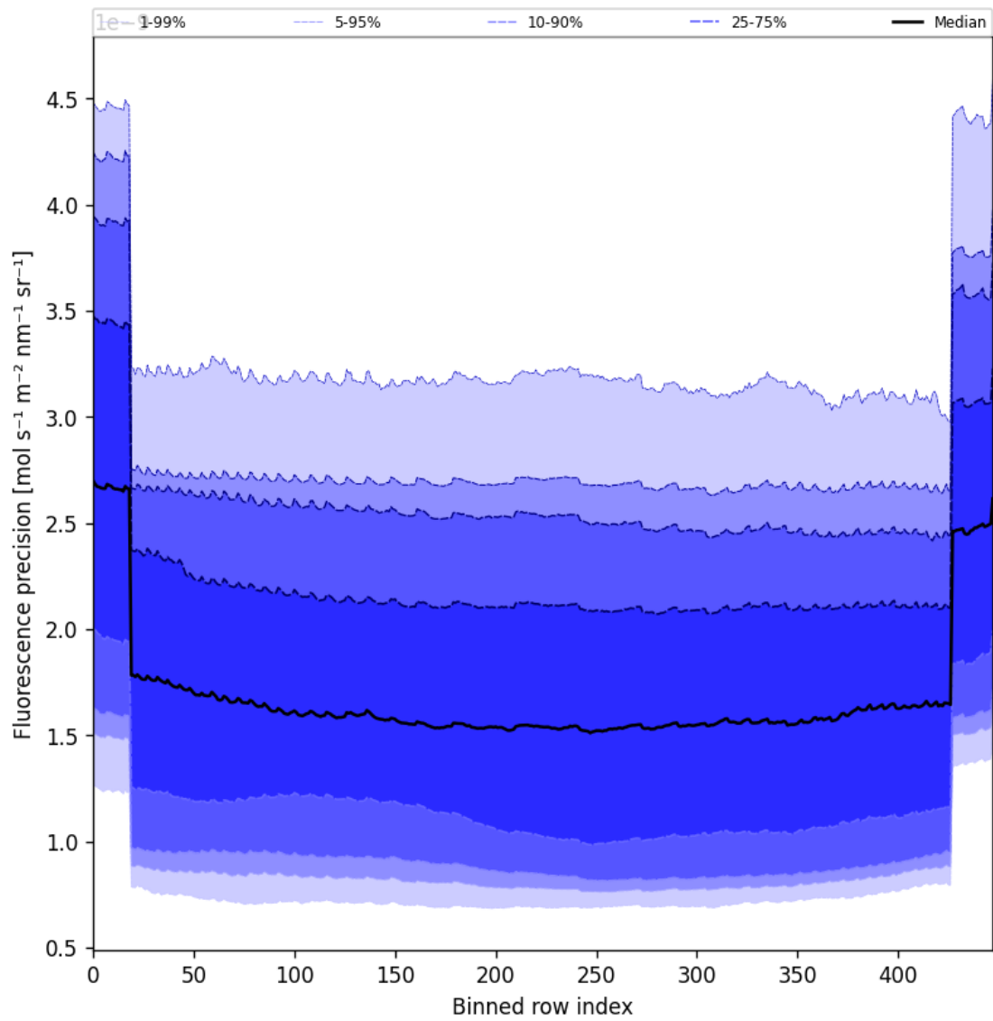
Figure 58: Along track statistics of “Fluorescence precision” for 2025-11-21 to 2025-11-23
