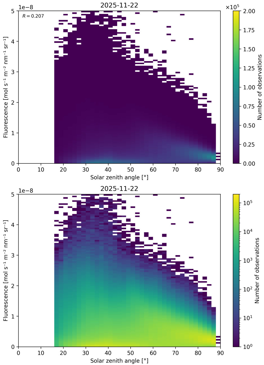
Figure 112: Scatter density plot of “Solar zenith angle” against “Fluorescence” for 2025-11-21 to 2025-11-23.
