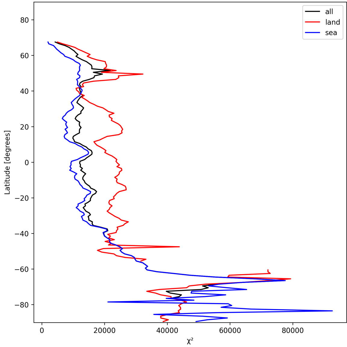
Figure 21: Zonal average of “ \chi^2 ” for 2025-11-21 to 2025-11-23.
