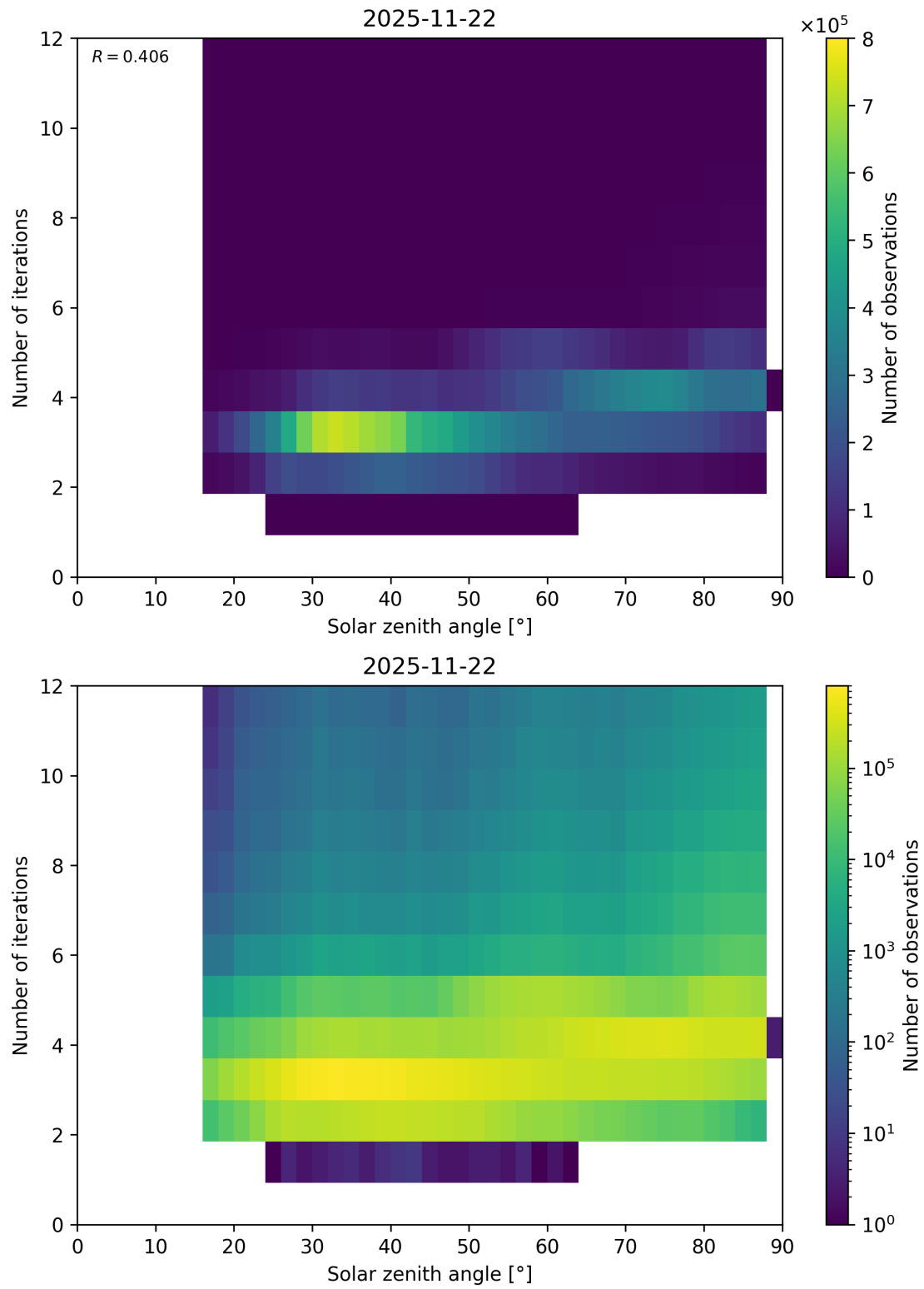
Figure 114: Scatter density plot of “Solar zenith angle” against “Number of iterations” for 2025-11-21 to 2025-11-23.
