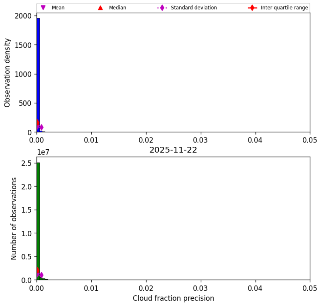
Figure 33: Histogram of “Cloud fraction precision” for 2025-11-21 to 2025-11-23
