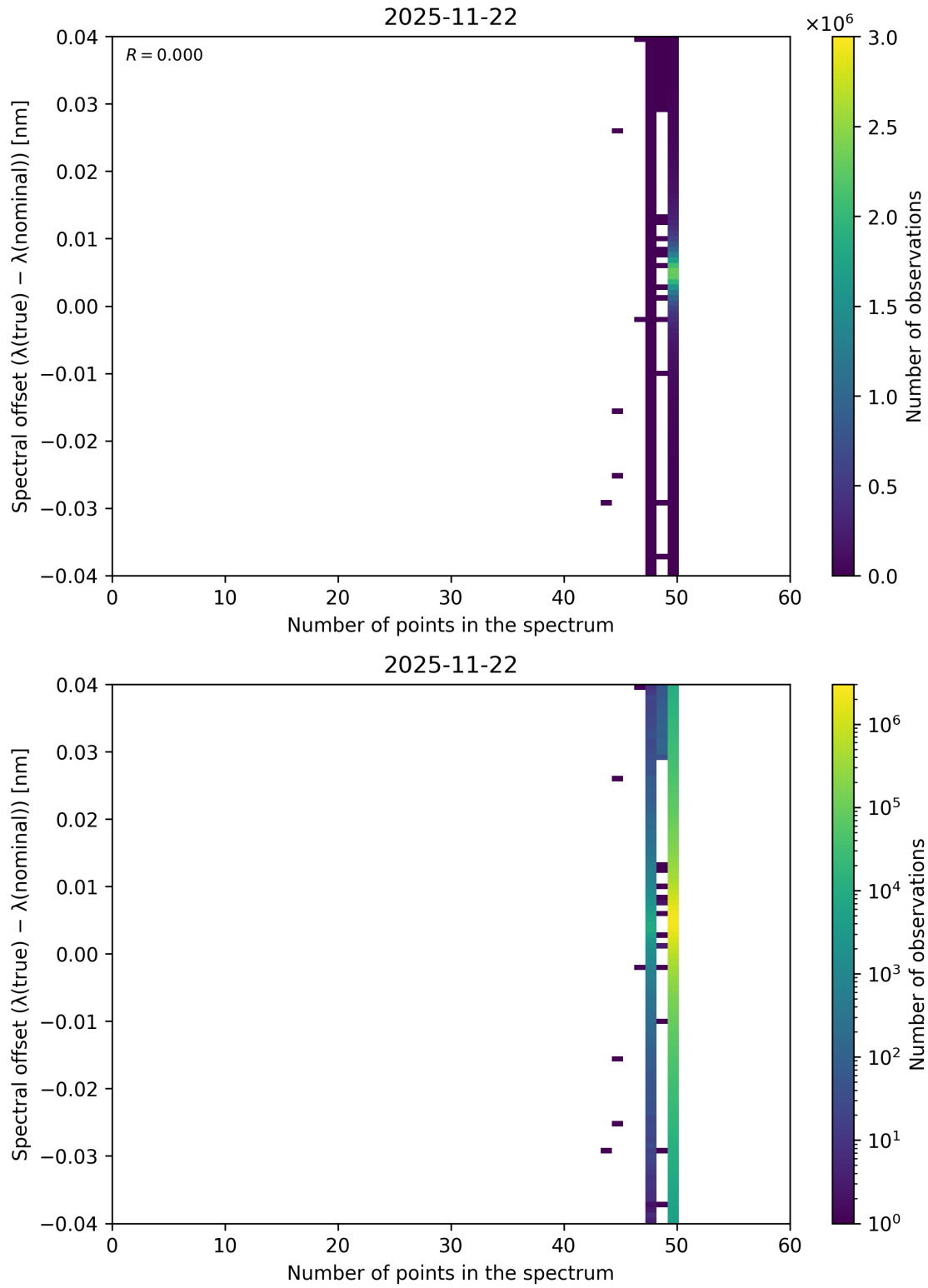
Figure 101: Scatter density plot of “Number of points in the spectrum” against “Spectral offset ( \lambda_{\text{true}} - \lambda_{\text{nominal}} )” for 2025-11-21 to 2025-11-23.
