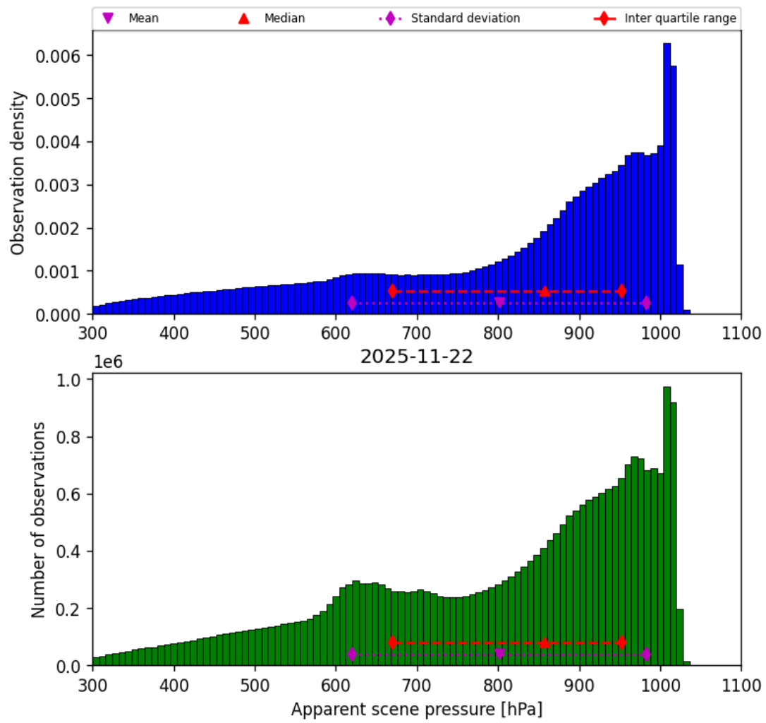
Figure 36: Histogram of “Apparent scene pressure” for 2025-11-21 to 2025-11-23
