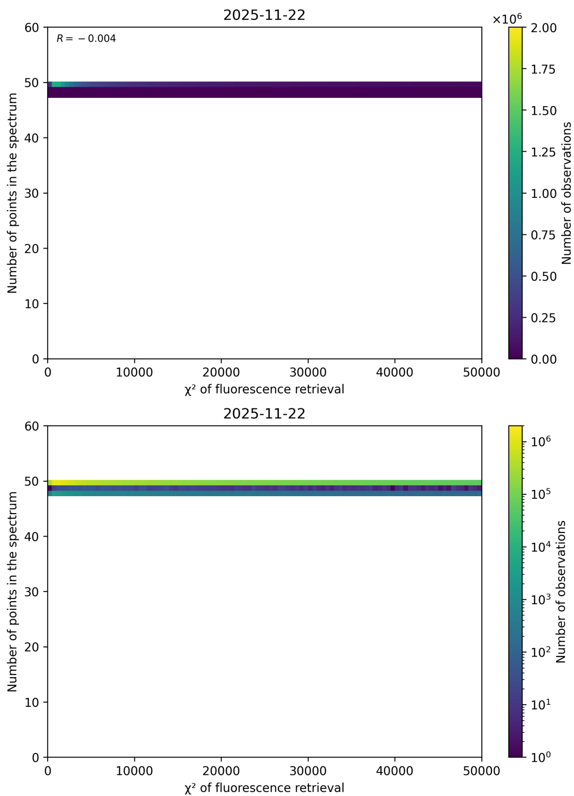
Figure 68: Scatter density plot of “ \chi^2 of fluorescence retrieval” against “Number of points in the spectrum” for 2025-11-21 to 2025-11-23.
