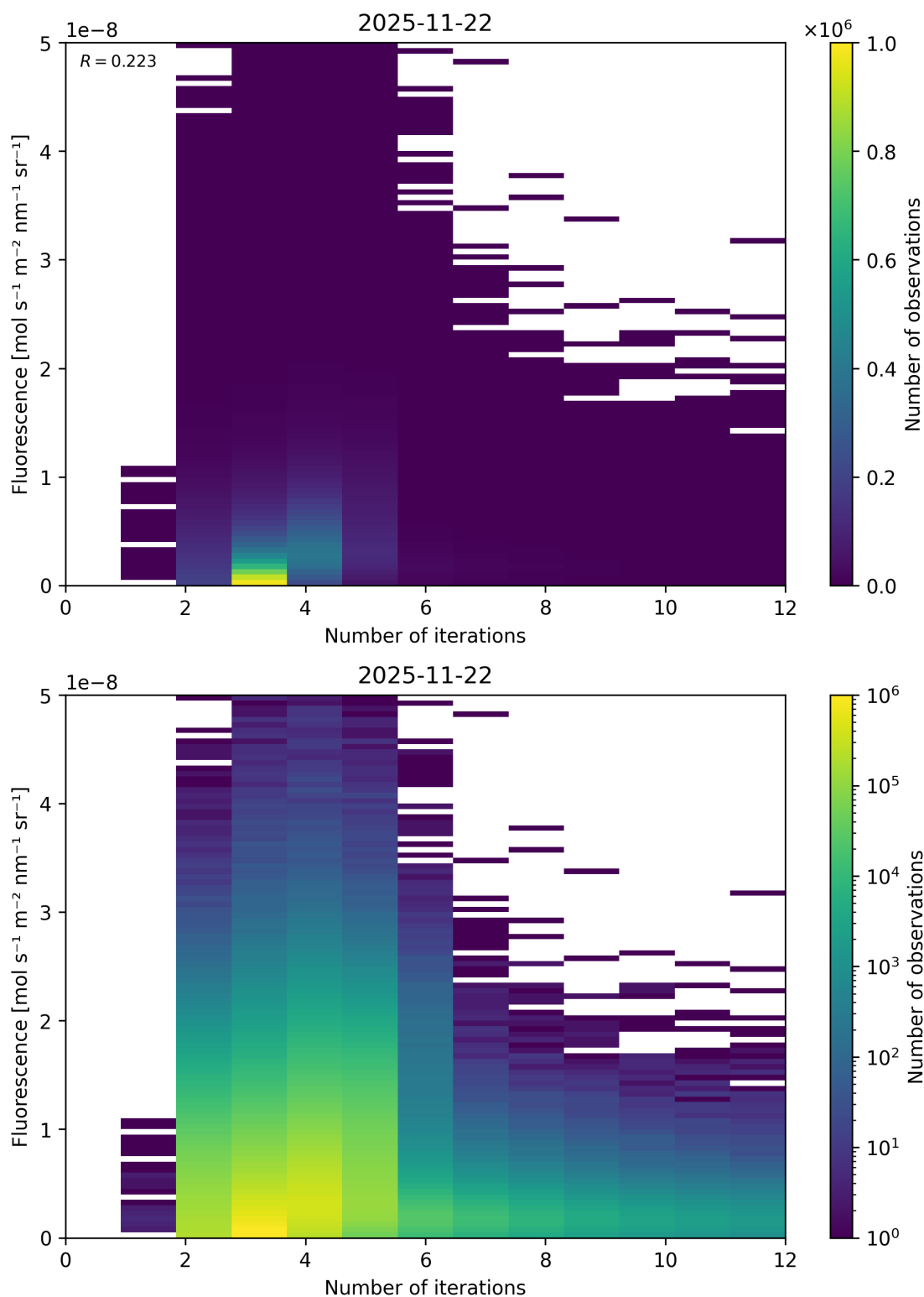
Figure 98: Scatter density plot of “Number of iterations” against “Fluorescence” for 2025-11-21 to 2025-11-23.
