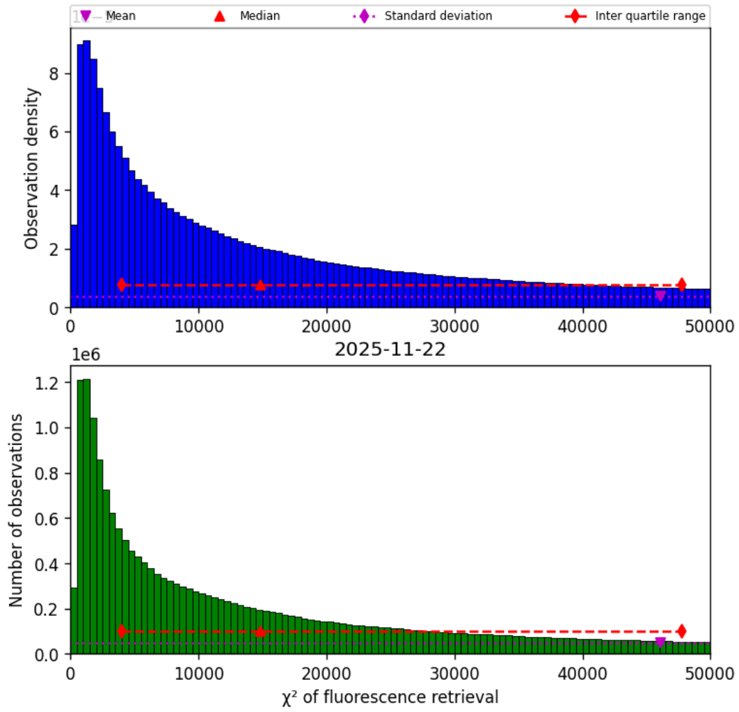
Figure 42: Histogram of “ \chi^2 of fluorescence retrieval” for 2025-11-21 to 2025-11-23
