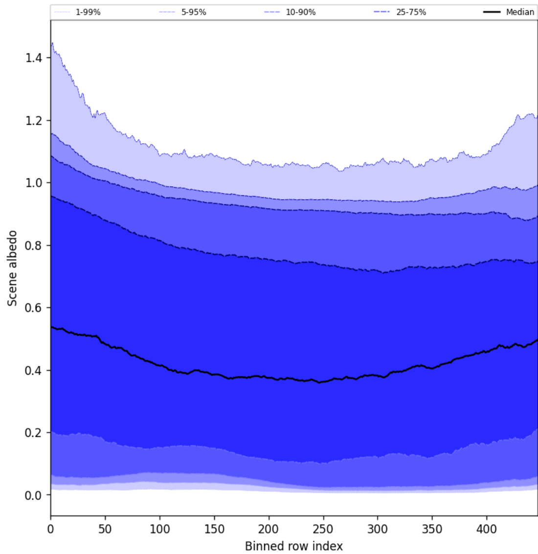
Figure 51: Along track statistics of “Scene albedo” for 2025-11-21 to 2025-11-23
