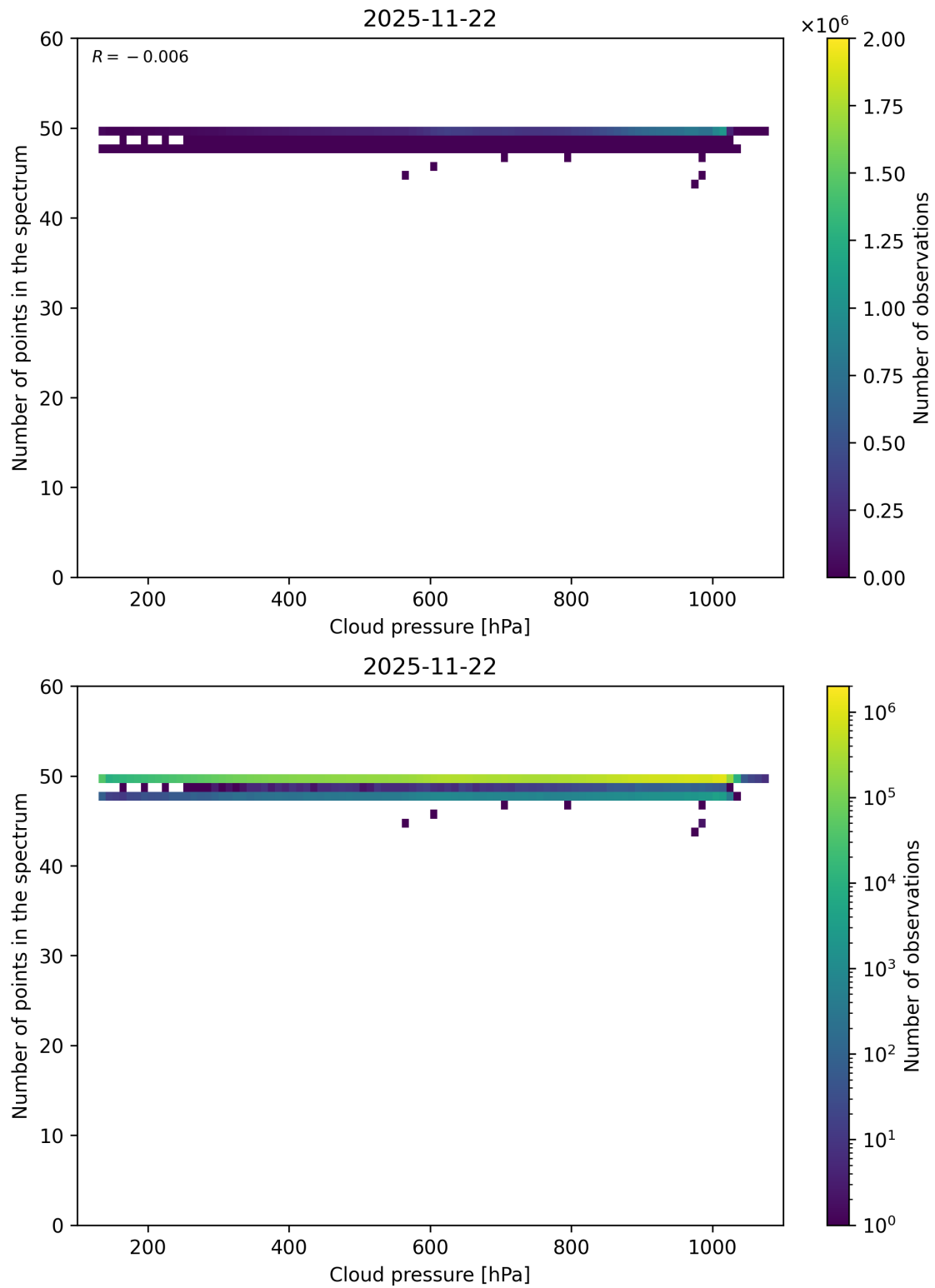
Figure 82: Scatter density plot of “Cloud pressure” against “Number of points in the spectrum” for 2025-11-21 to 2025-11-23.
