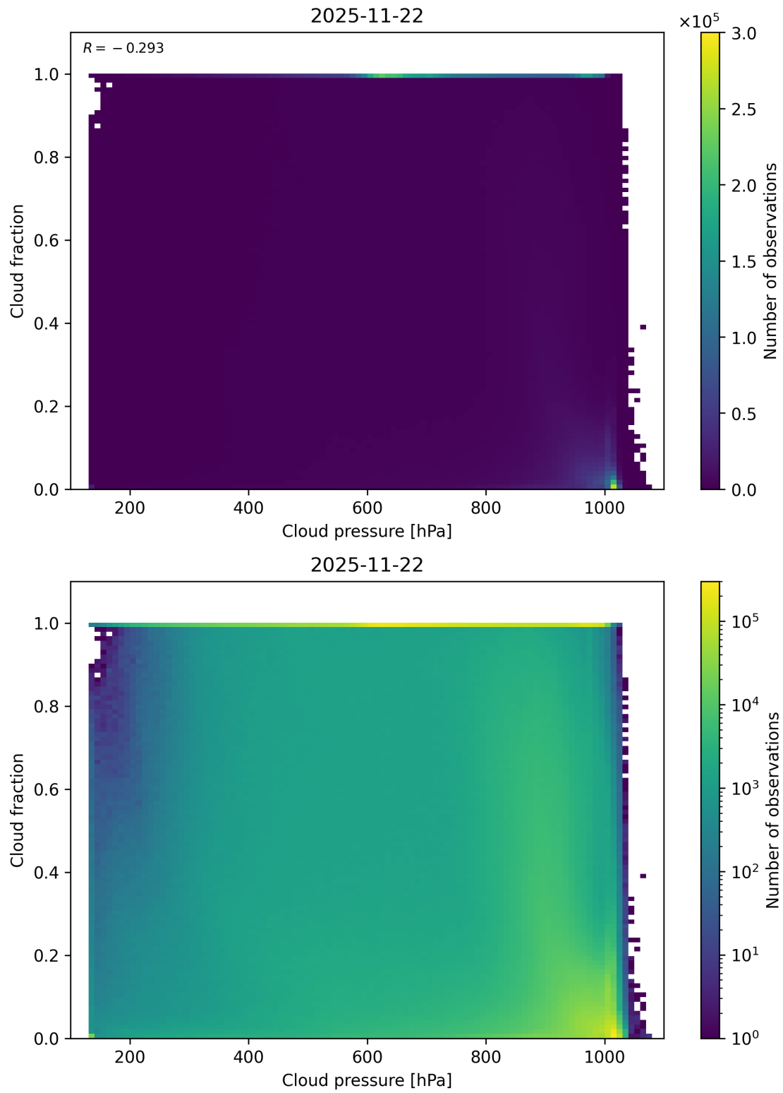
Figure 79: Scatter density plot of “Cloud pressure” against “Cloud fraction” for 2025-11-21 to 2025-11-23.
