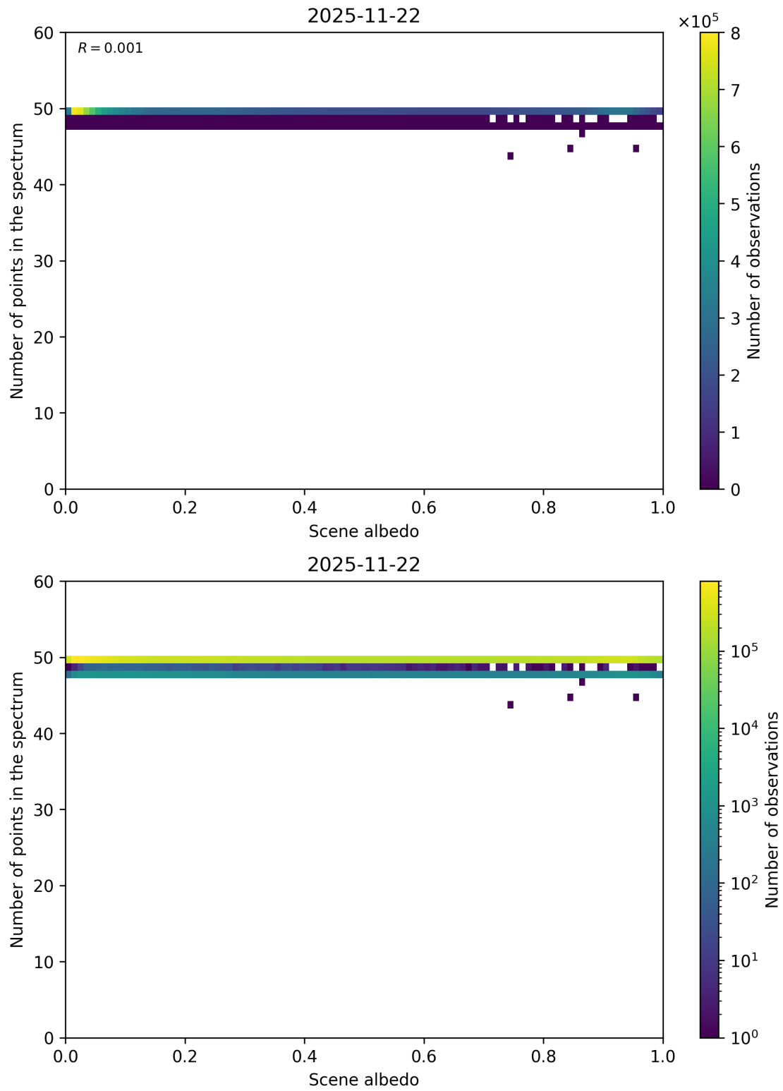
Figure 106: Scatter density plot of “Scene albedo” against “Number of points in the spectrum” for 2025-11-21 to 2025-11-23.
