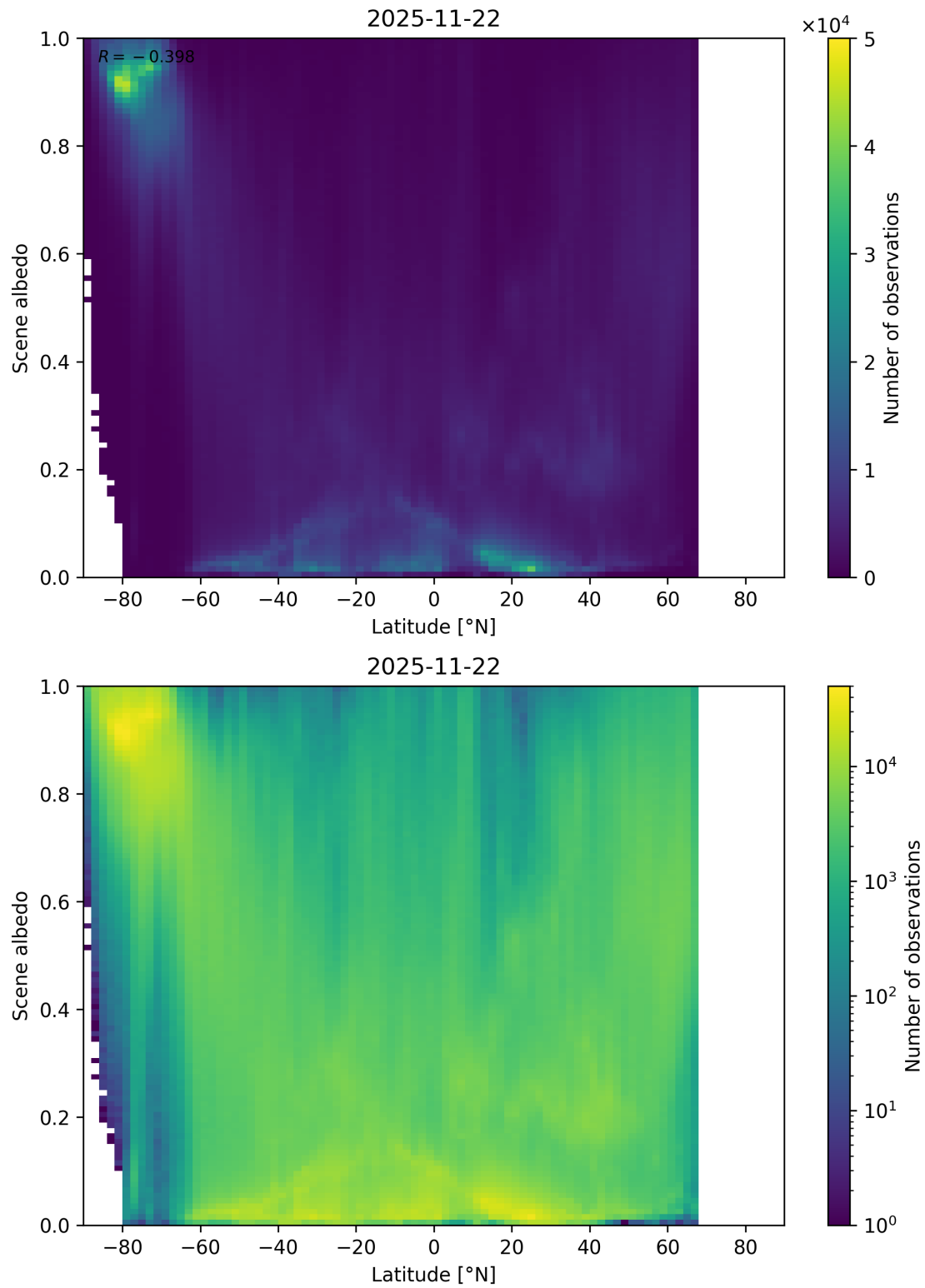
Figure 95: Scatter density plot of “Latitude” against “Scene albedo” for 2025-11-21 to 2025-11-23.
