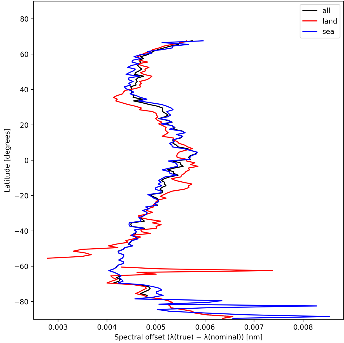
Figure 28: Zonal average of “Spectral offset ( \lambda_{\text{true}} - \lambda_{\text{nominal}} )” for 2025-11-21 to 2025-11-23.
