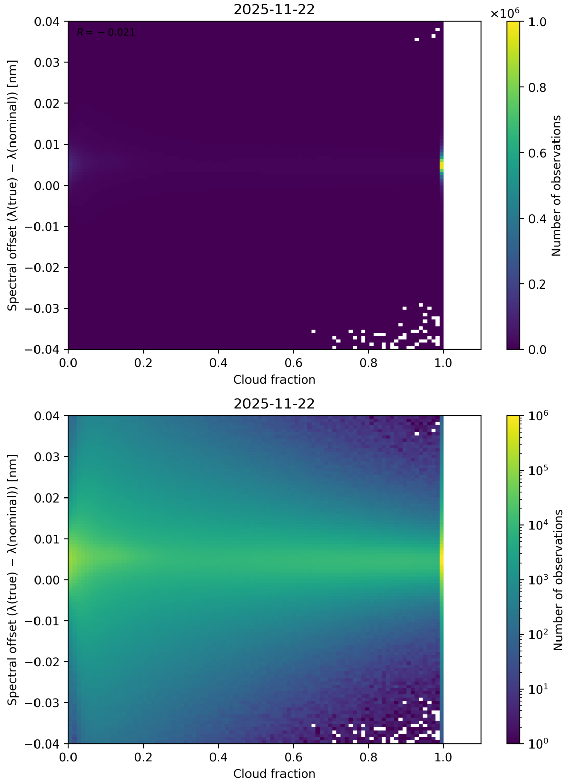
Figure 76: Scatter density plot of “Cloud fraction” against “Spectral offset ( \lambda_{\text{true}} - \lambda_{\text{nominal}} )” for 2025-11-21 to 2025-11-23.
