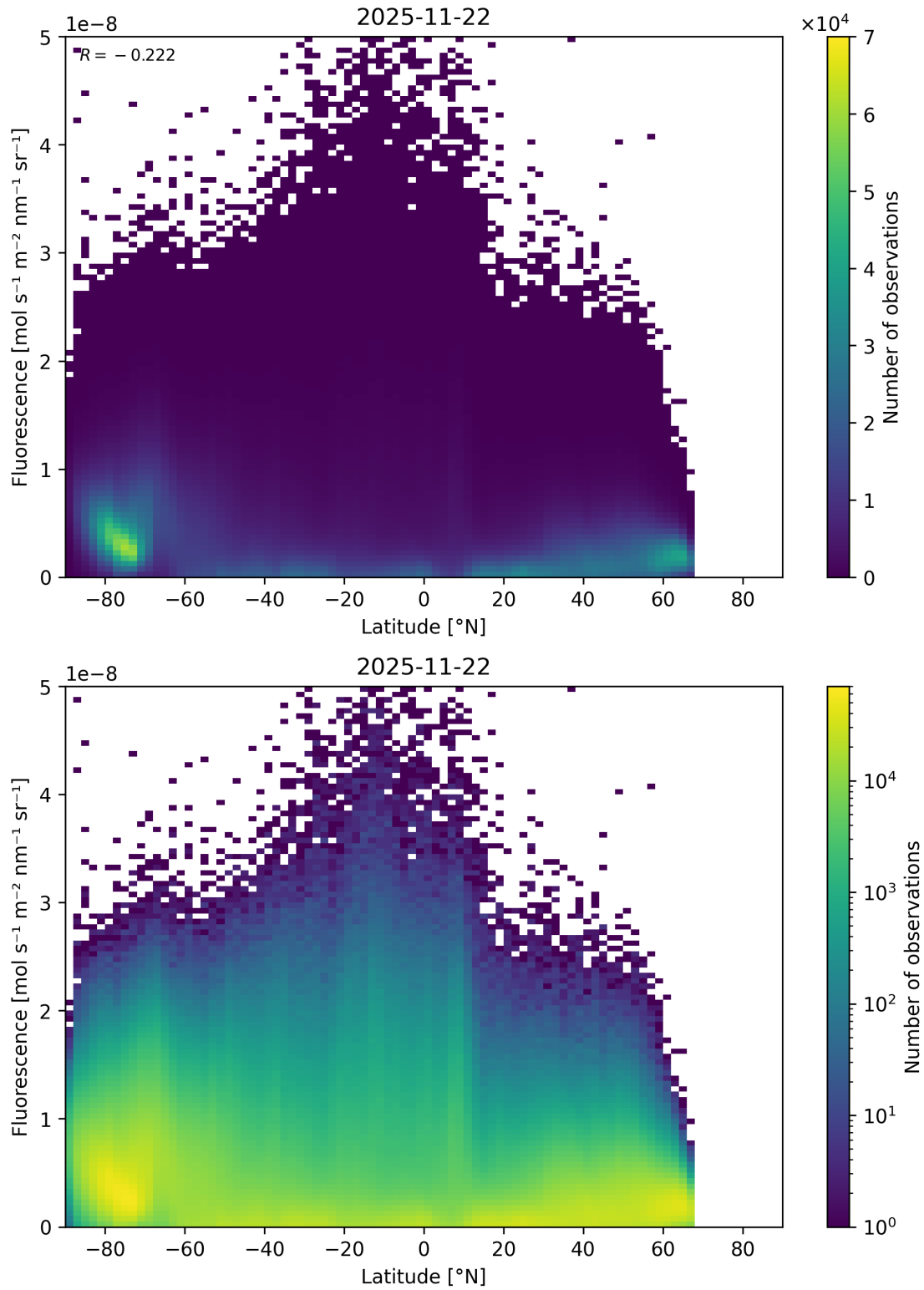
Figure 92: Scatter density plot of “Latitude” against “Fluorescence” for 2025-11-21 to 2025-11-23.
