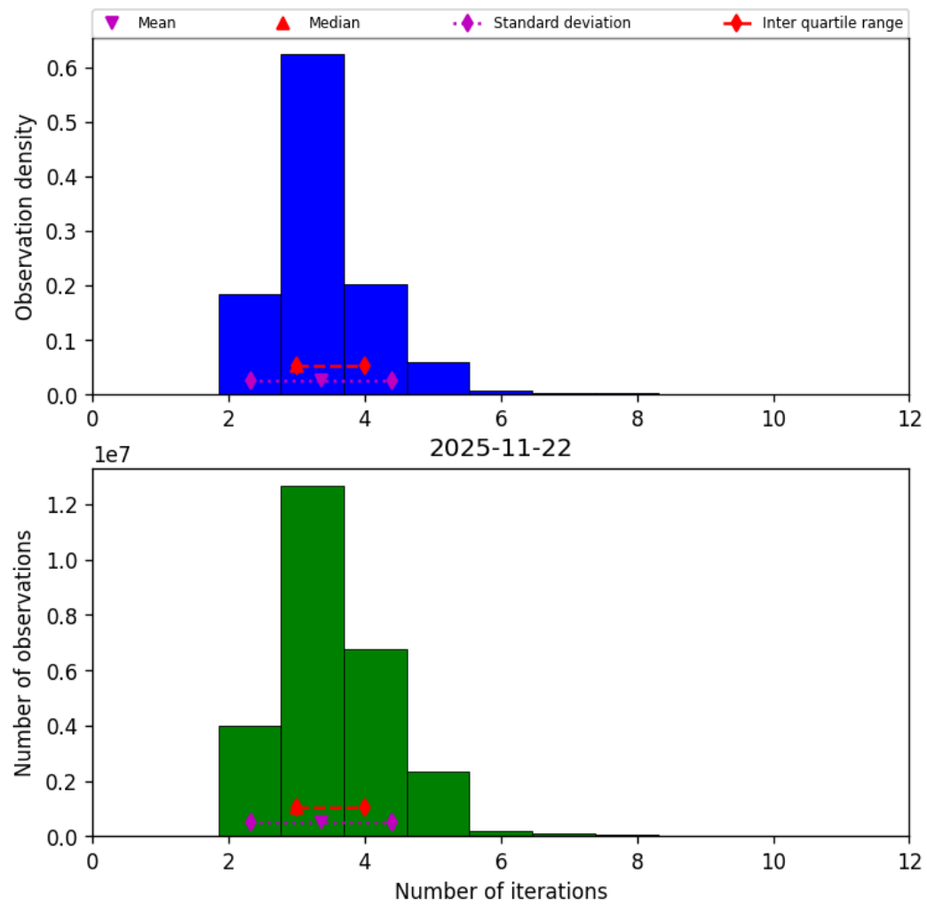
Figure 39: Histogram of “Number of iterations” for 2025-11-21 to 2025-11-23
