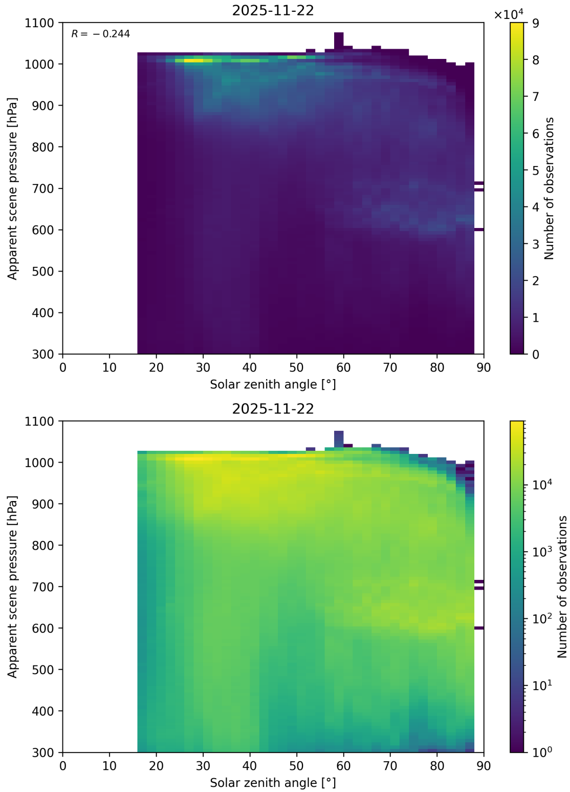
Figure 108: Scatter density plot of “Solar zenith angle” against “Apparent scene pressure” for 2025-11-21 to 2025-11-23.
