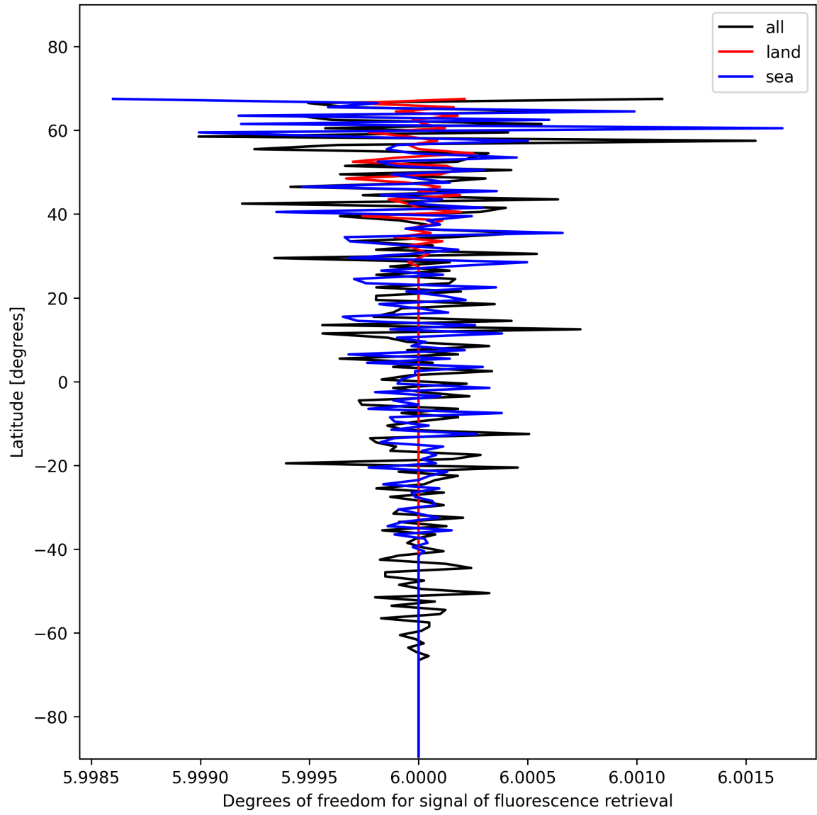
Figure 26: Zonal average of “Degrees of freedom for signal of fluorescence retrieval” for 2025-11-21 to 2025-11-23.
