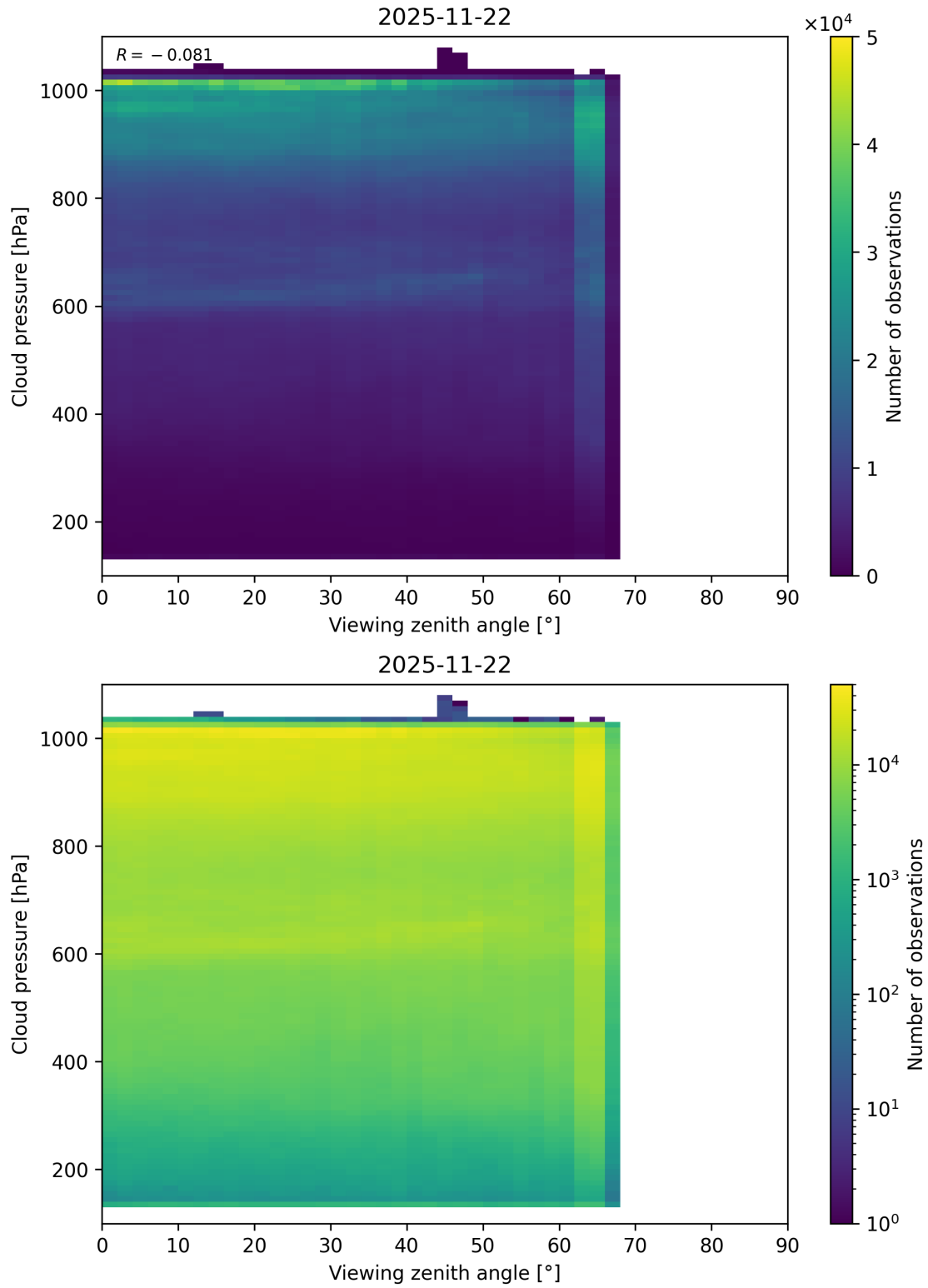
Figure 121: Scatter density plot of “Viewing zenith angle” against “Cloud pressure” for 2025-11-21 to 2025-11-23.
