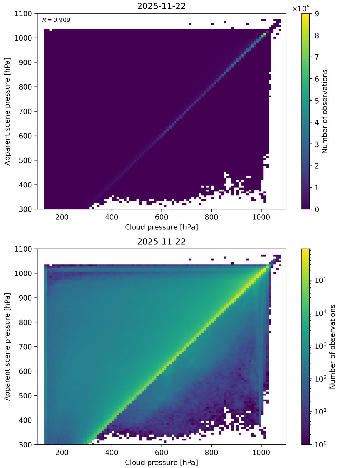
Figure 77: Scatter density plot of “Cloud pressure” against “Apparent scene pressure” for 2025-11-21 to 2025-11-23.
