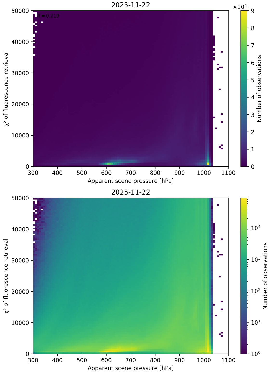
Figure 63: Scatter density plot of “Apparent scene pressure” against “ \chi^2 of fluorescence retrieval” for 2025-11-21 to 2025-11-23.
