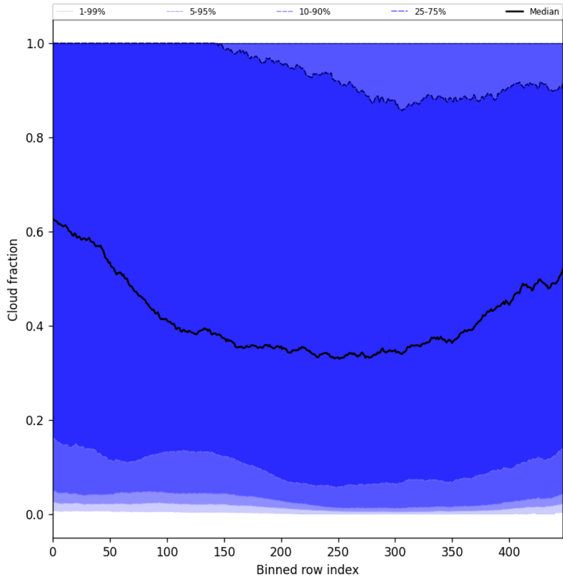
Figure 49: Along track statistics of “Cloud fraction” for 2025-11-21 to 2025-11-23
