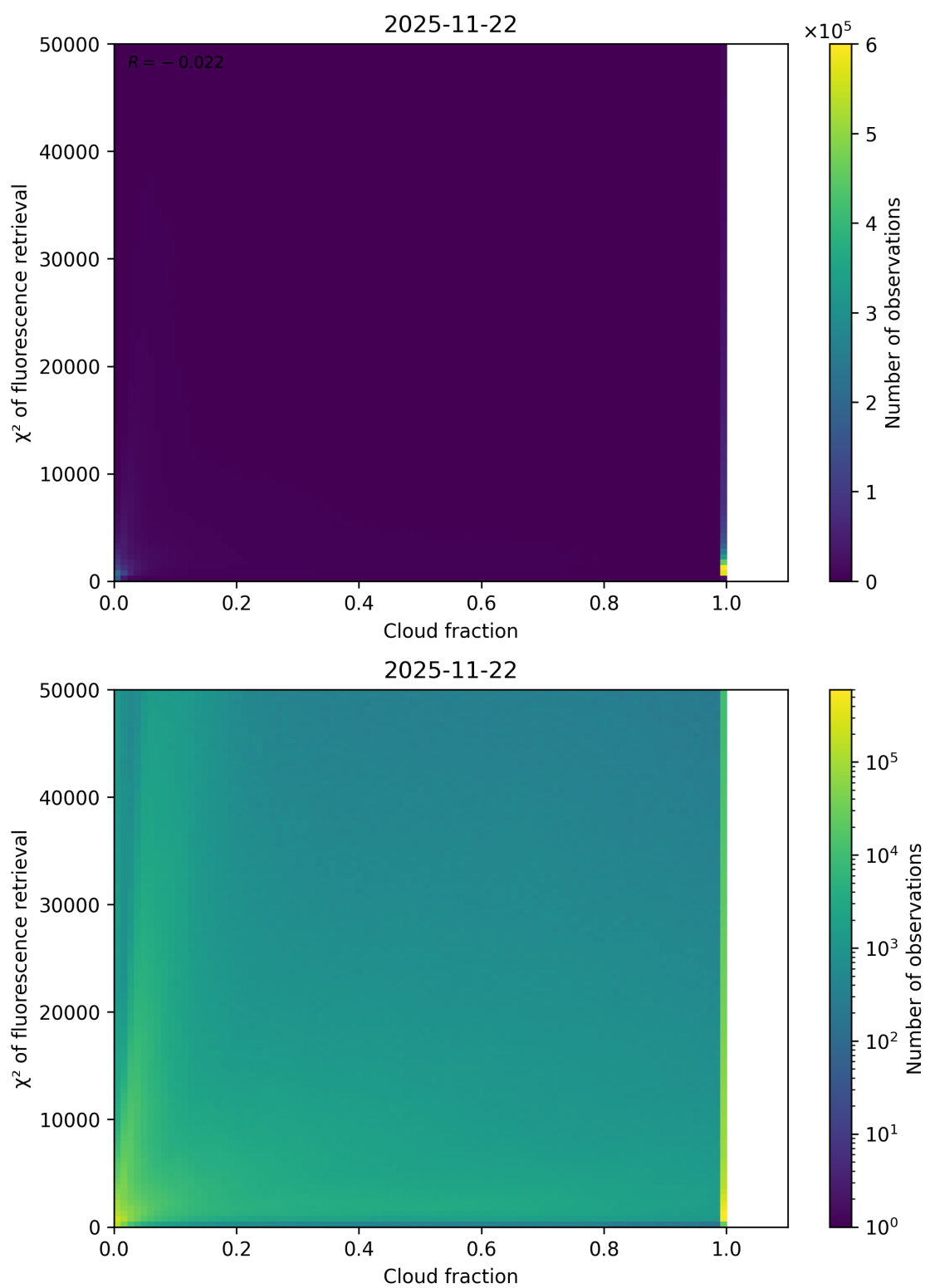
Figure 71: Scatter density plot of “Cloud fraction” against “ \chi^2 of fluorescence retrieval” for 2025-11-21 to 2025-11-23.
