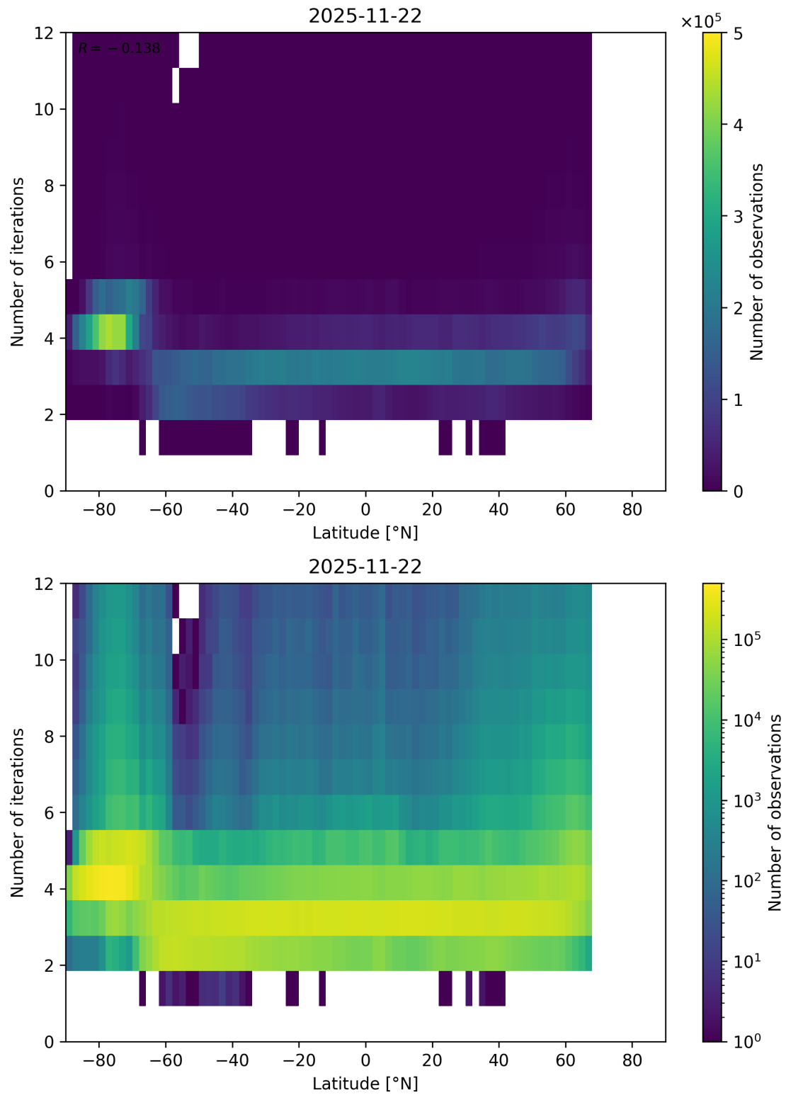
Figure 93: Scatter density plot of “Latitude” against “Number of iterations” for 2025-11-21 to 2025-11-23.
