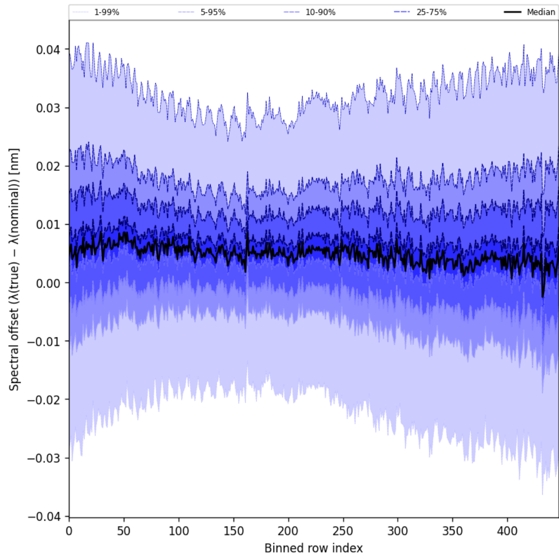
Figure 62: Along track statistics of “Spectral offset ( \lambda_{\text{true}} - \lambda_{\text{nominal}} )” for 2025-11-21 to 2025-11-23
