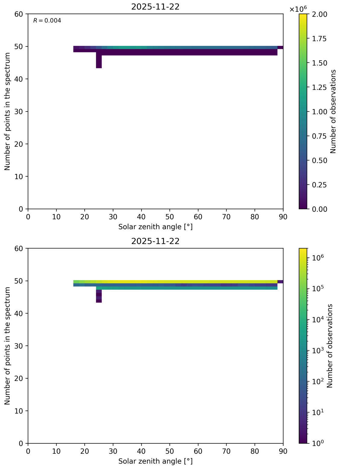
Figure 115: Scatter density plot of “Solar zenith angle” against “Number of points in the spectrum” for 2025-11-21 to 2025-11-23.
