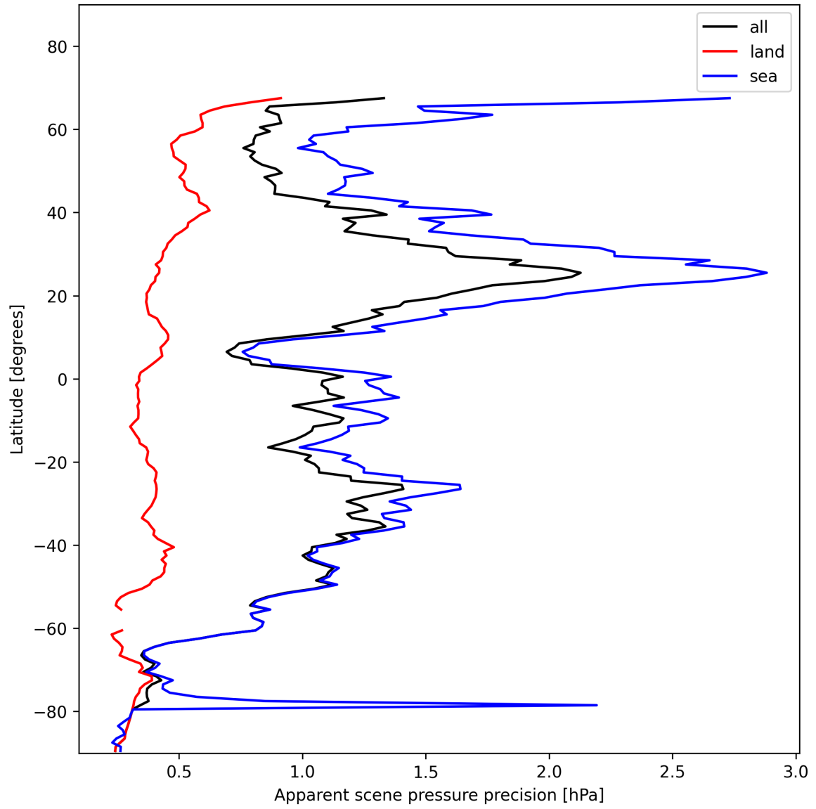
Figure 20: Zonal average of “Apparent scene pressure precision” for 2025-11-21 to 2025-11-23.
