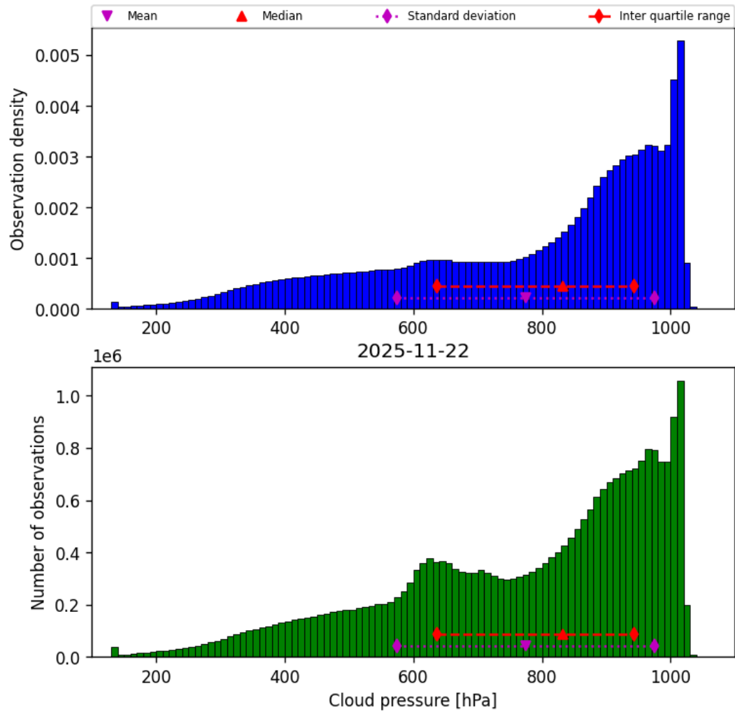
Figure 30: Histogram of “Cloud pressure” for 2025-11-21 to 2025-11-23
