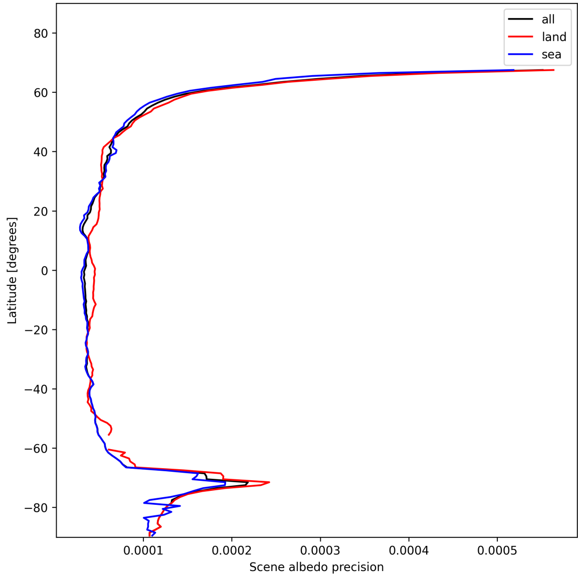
Figure 18: Zonal average of “Scene albedo precision” for 2025-11-21 to 2025-11-23.
