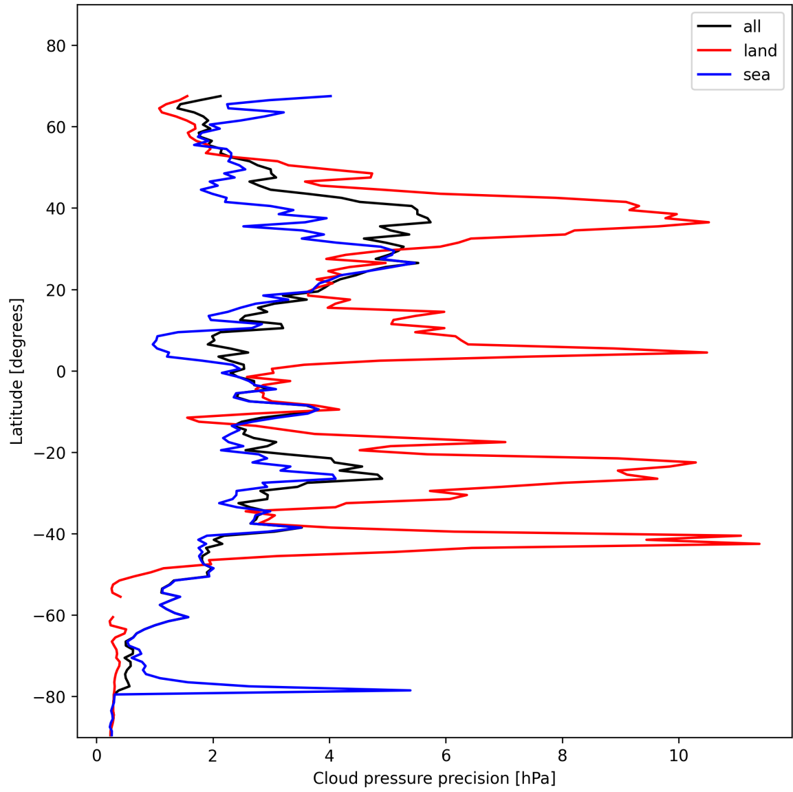
Figure 14: Zonal average of “Cloud pressure precision” for 2025-11-21 to 2025-11-23.
