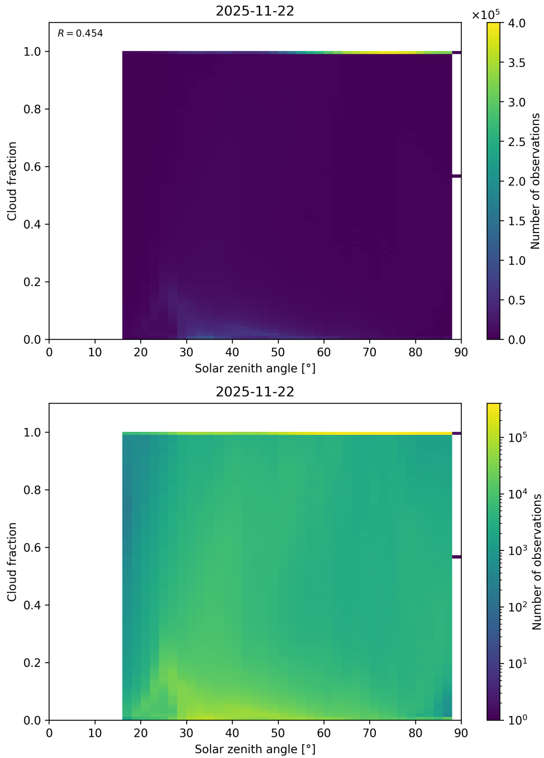
Figure 110: Scatter density plot of “Solar zenith angle” against “Cloud fraction” for 2025-11-21 to 2025-11-23.
