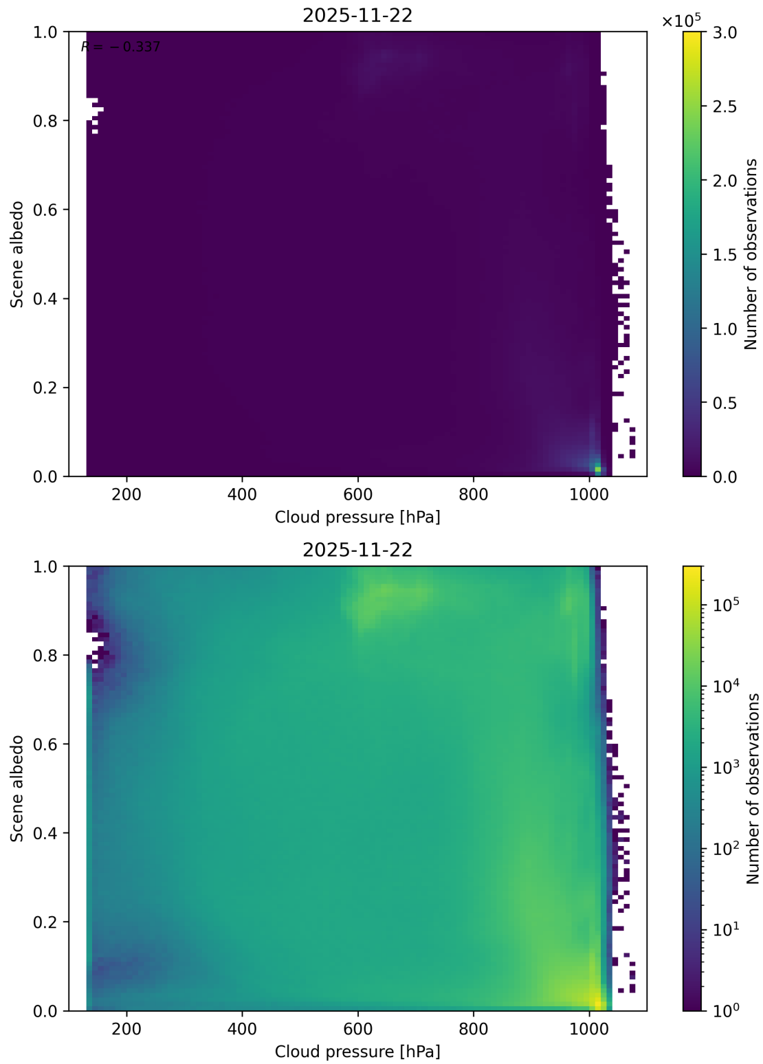
Figure 83: Scatter density plot of “Cloud pressure” against “Scene albedo” for 2025-11-21 to 2025-11-23.
