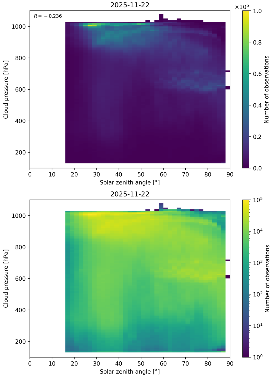
Figure 111: Scatter density plot of “Solar zenith angle” against “Cloud pressure” for 2025-11-21 to 2025-11-23.
