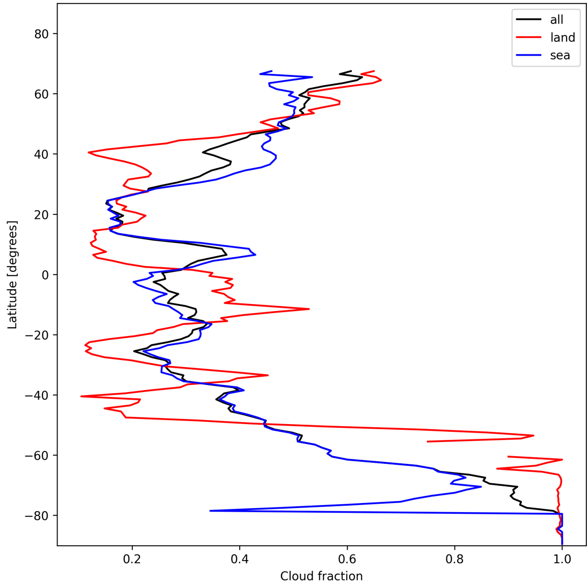
Figure 15: Zonal average of “Cloud fraction” for 2025-11-21 to 2025-11-23.
