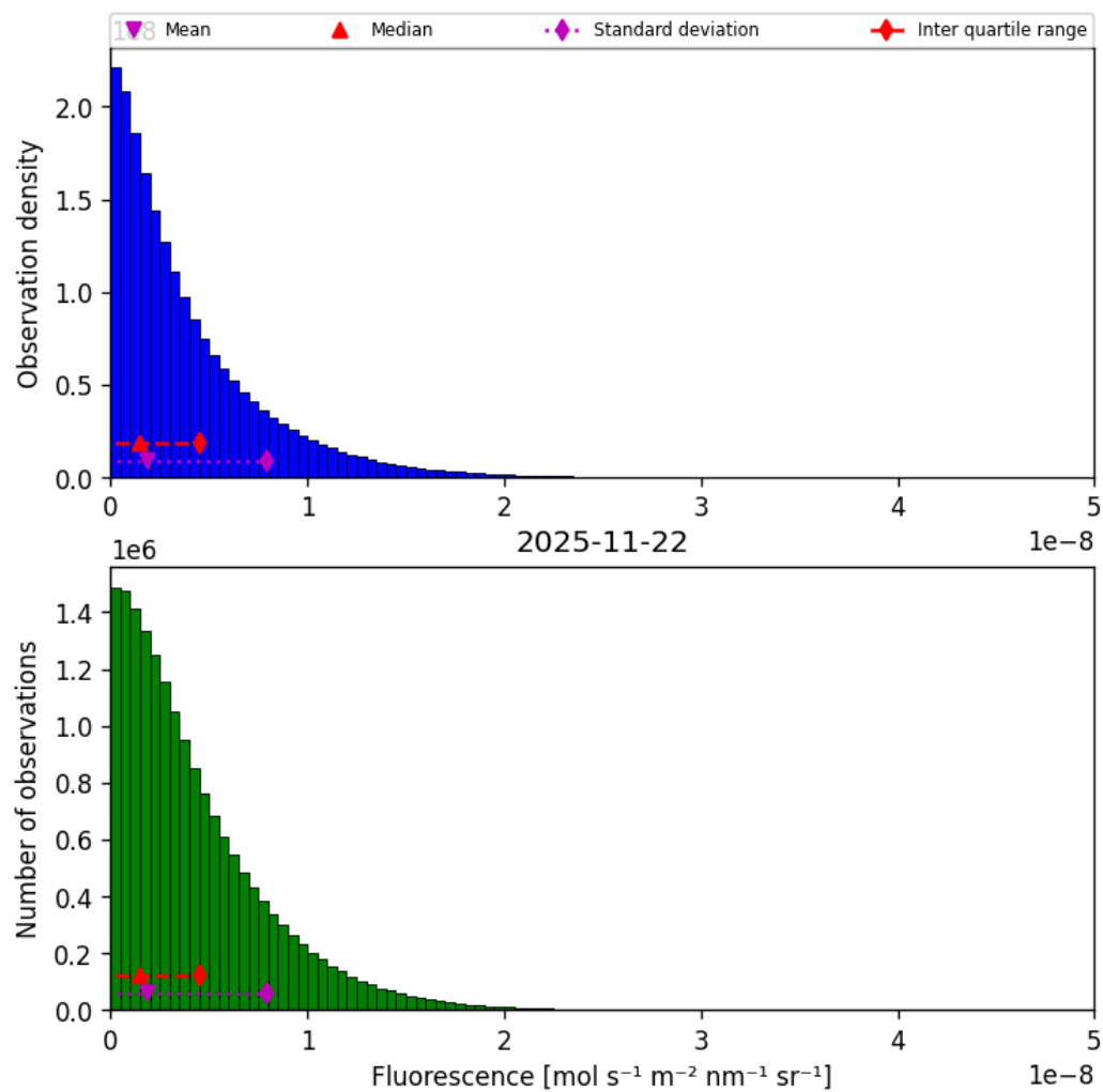
Figure 40: Histogram of “Fluorescence” for 2025-11-21 to 2025-11-23
