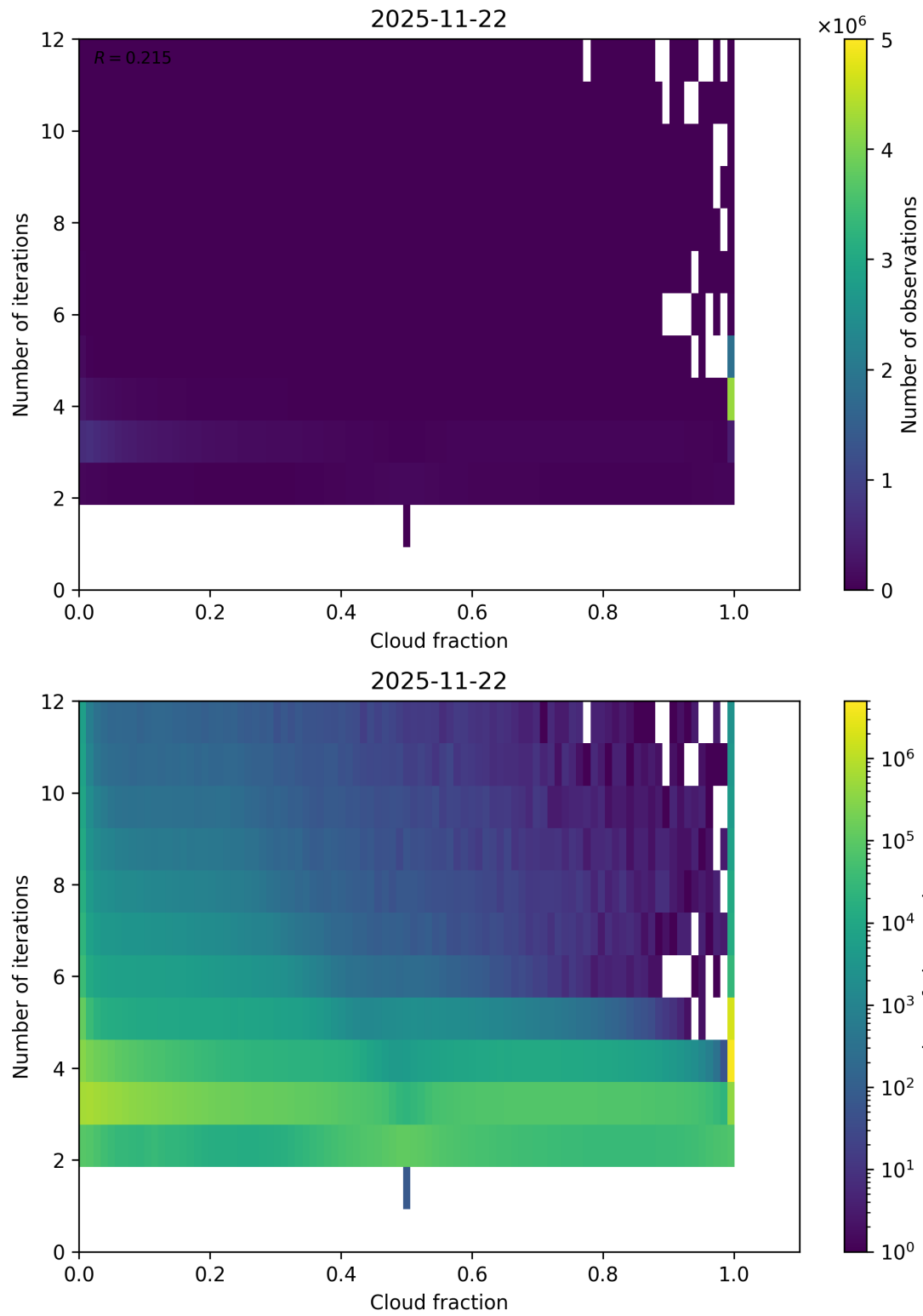
Figure 73: Scatter density plot of “Cloud fraction” against “Number of iterations” for 2025-11-21 to 2025-11-23.
