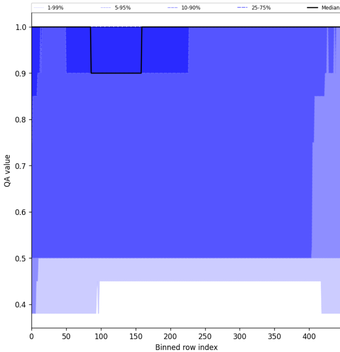
Figure 46: Along track statistics of “QA value” for 2025-11-23 to 2025-11-24
