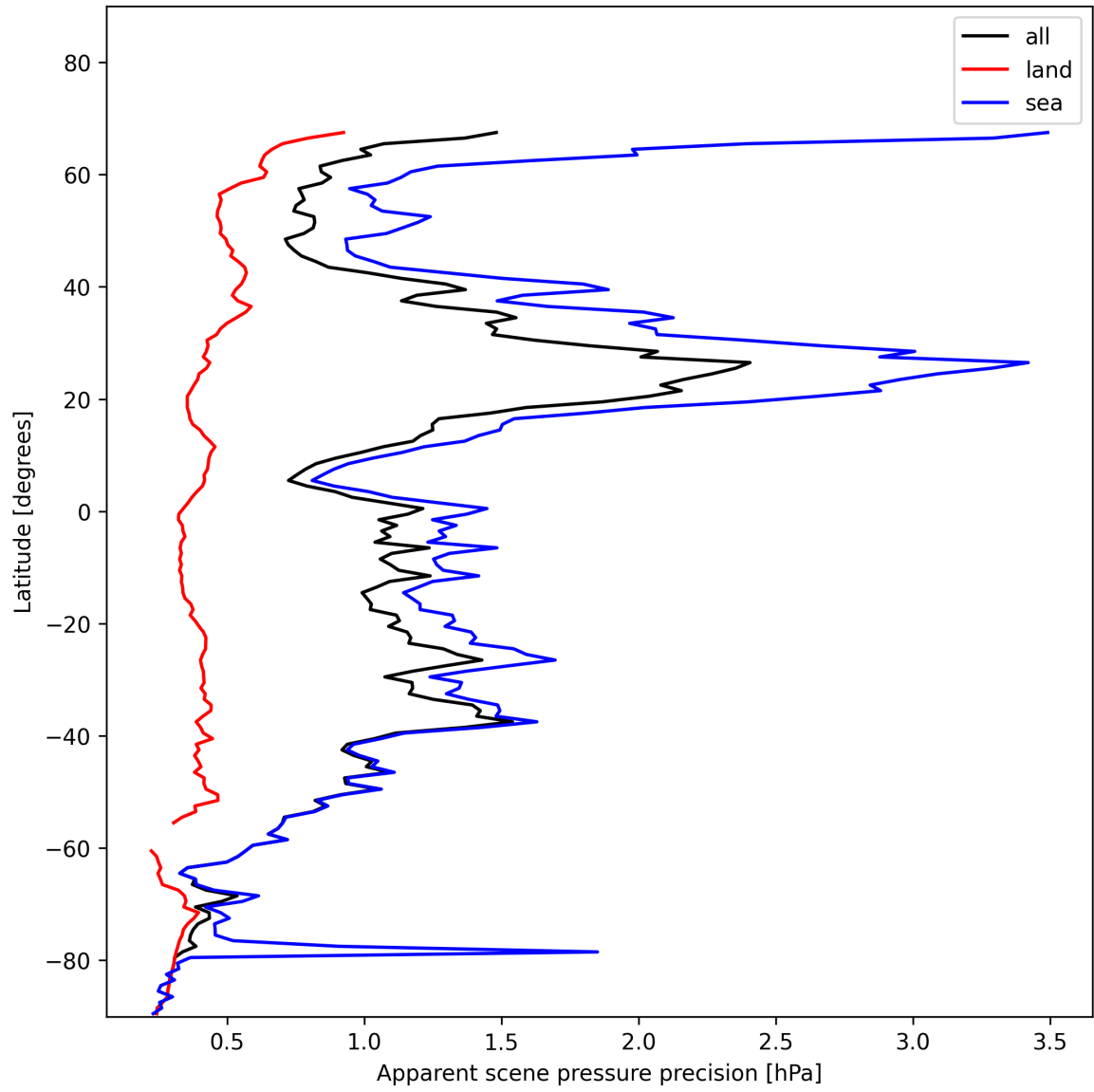
Figure 20: Zonal average of “Apparent scene pressure precision” for 2025-11-23 to 2025-11-24.
