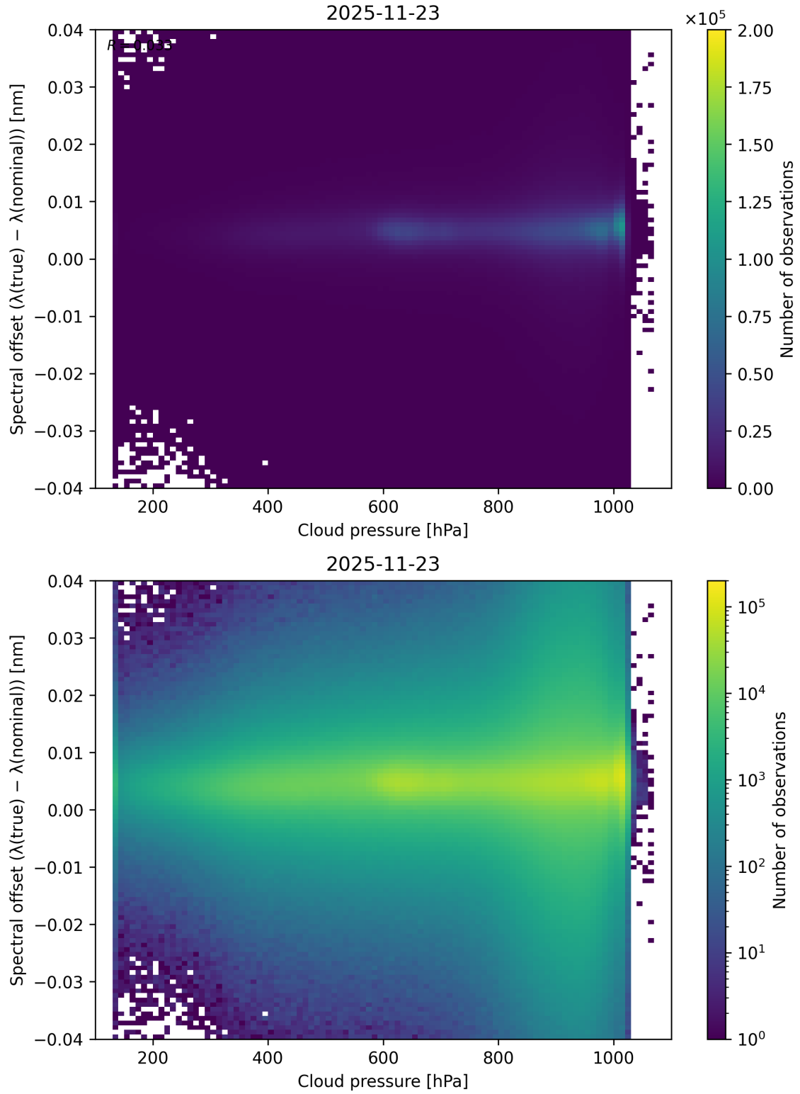
Figure 84: Scatter density plot of “Cloud pressure” against “Spectral offset ( \lambda_{\text{true}} - \lambda_{\text{nominal}} )” for 2025-11-23 to 2025-11-24.
