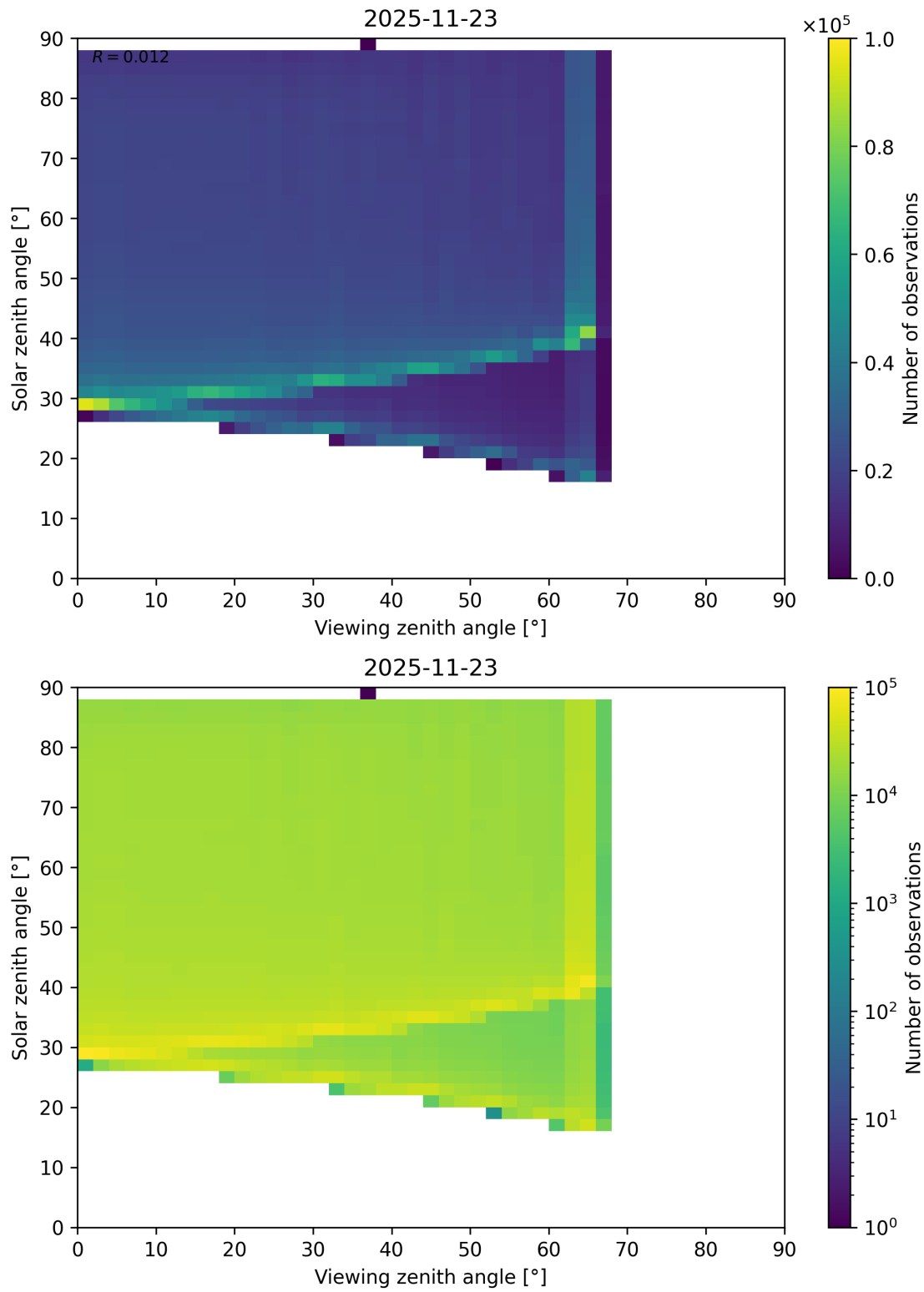
Figure 127: Scatter density plot of “Viewing zenith angle” against “Solar zenith angle” for 2025-11-23 to 2025-11-24.
