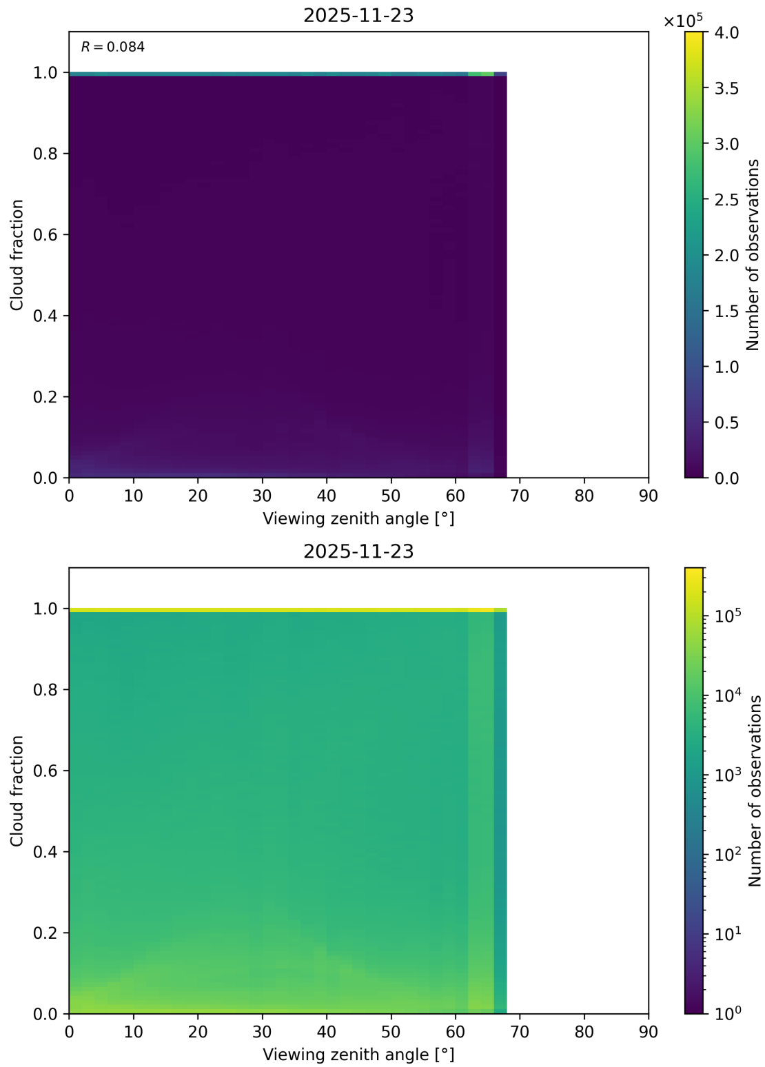
Figure 120: Scatter density plot of “Viewing zenith angle” against “Cloud fraction” for 2025-11-23 to 2025-11-24.
