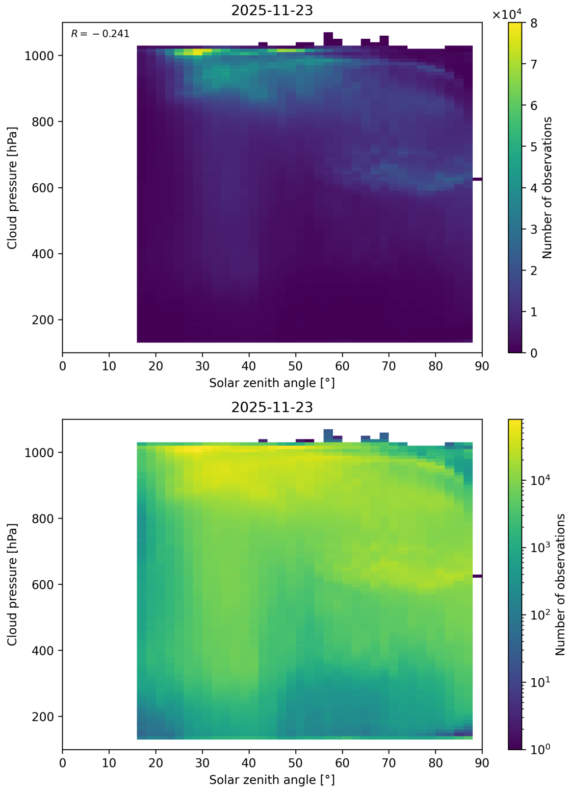
Figure 111: Scatter density plot of “Solar zenith angle” against “Cloud pressure” for 2025-11-23 to 2025-11-24.
