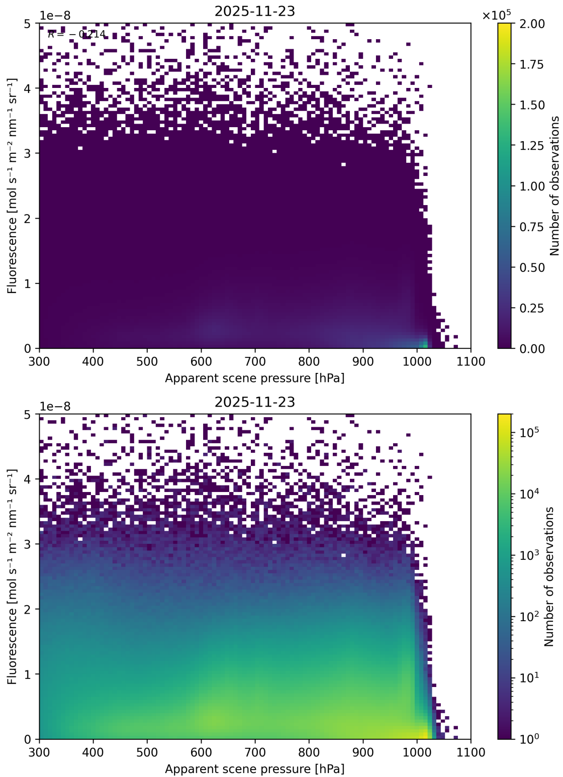
Figure 64: Scatter density plot of “Apparent scene pressure” against “Fluorescence” for 2025-11-23 to 2025-11-24.
