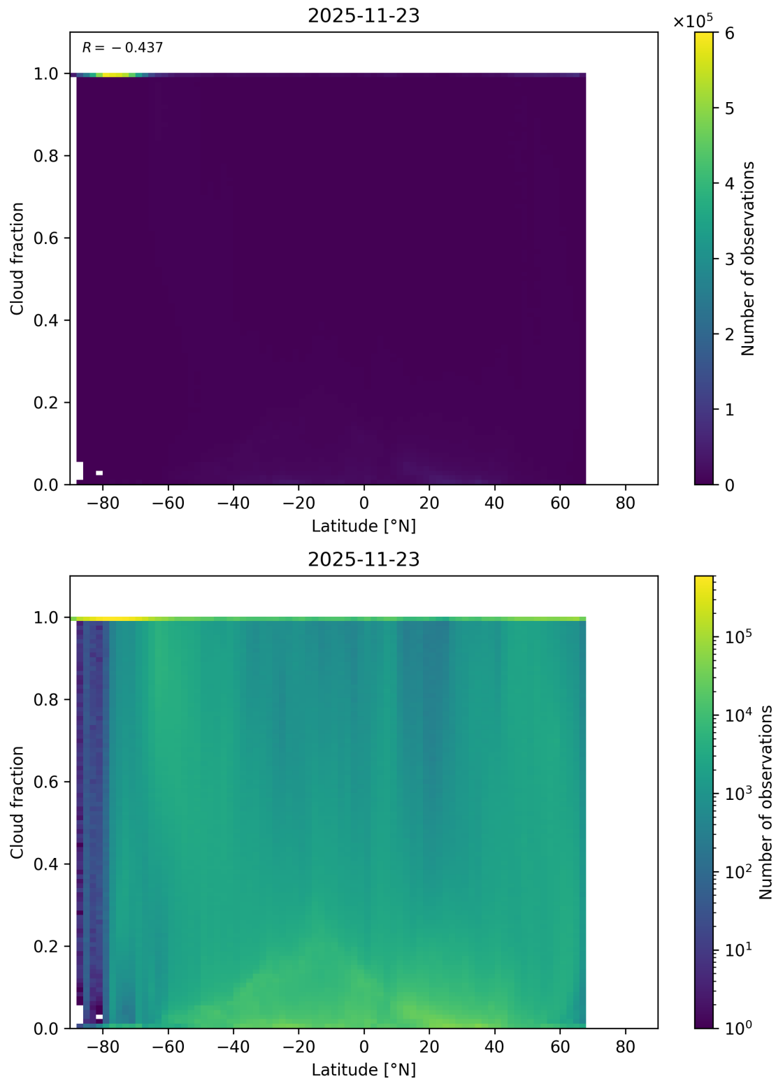
Figure 90: Scatter density plot of “Latitude” against “Cloud fraction” for 2025-11-23 to 2025-11-24.
