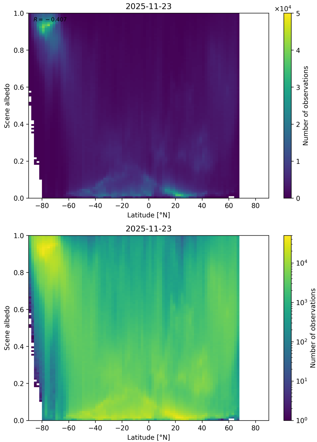
Figure 95: Scatter density plot of “Latitude” against “Scene albedo” for 2025-11-23 to 2025-11-24.
