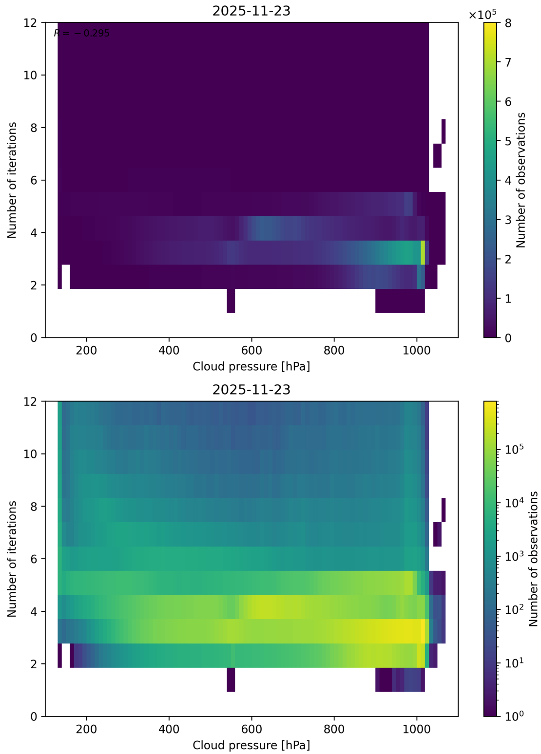
Figure 81: Scatter density plot of “Cloud pressure” against “Number of iterations” for 2025-11-23 to 2025-11-24.
