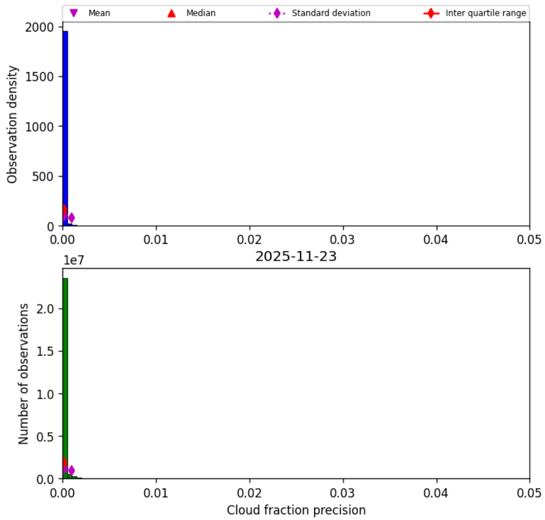
Figure 33: Histogram of “Cloud fraction precision” for 2025-11-23 to 2025-11-24
