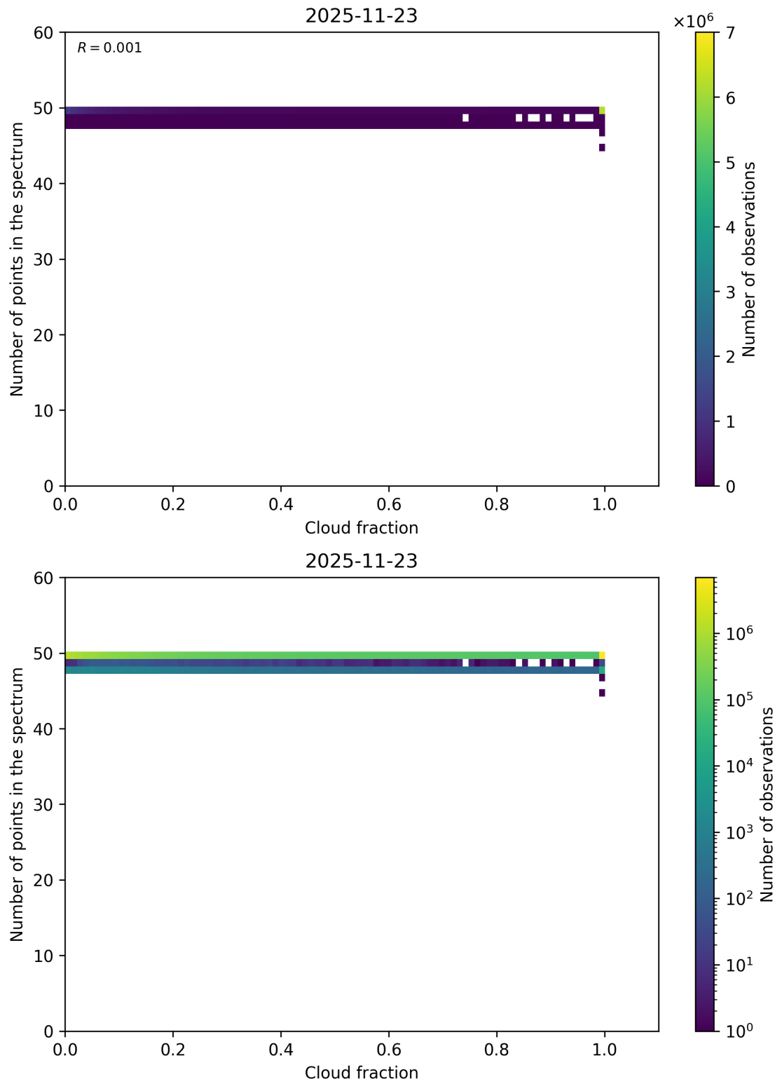
Figure 74: Scatter density plot of “Cloud fraction” against “Number of points in the spectrum” for 2025-11-23 to 2025-11-24.
