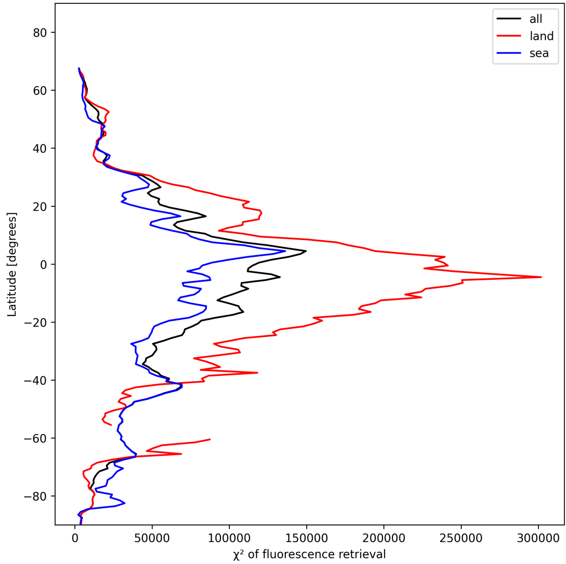
Figure 25: Zonal average of “ \chi^2 of fluorescence retrieval” for 2025-11-23 to 2025-11-24.
