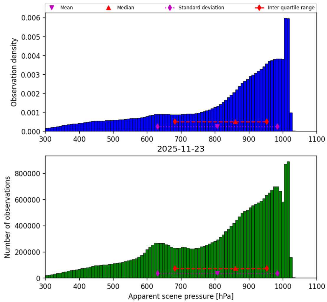
Figure 36: Histogram of “Apparent scene pressure” for 2025-11-23 to 2025-11-24
