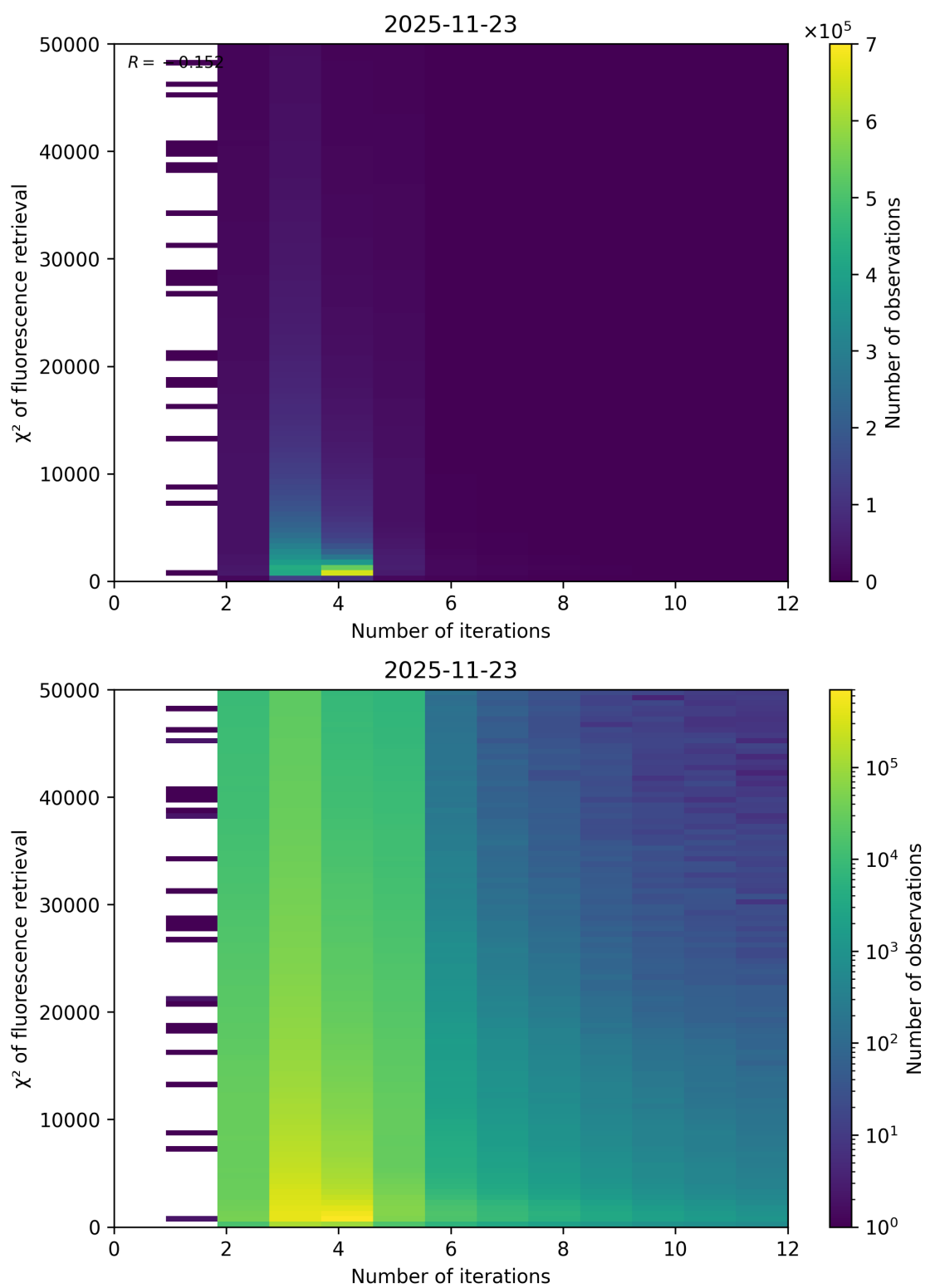
Figure 97: Scatter density plot of “Number of iterations” against “ \chi^2 of fluorescence retrieval” for 2025-11-23 to 2025-11-24.
