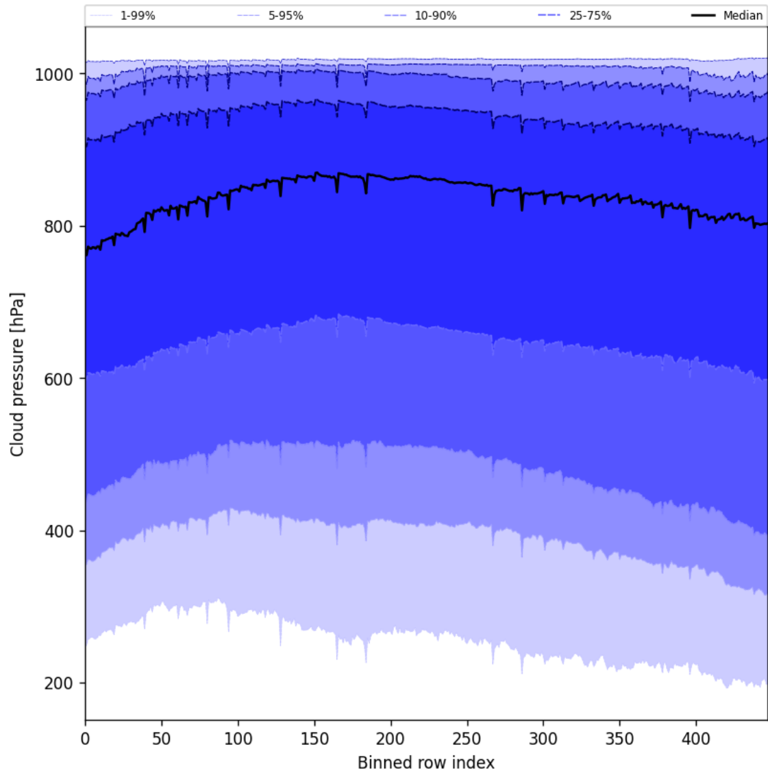
Figure 47: Along track statistics of “Cloud pressure” for 2025-11-23 to 2025-11-24
