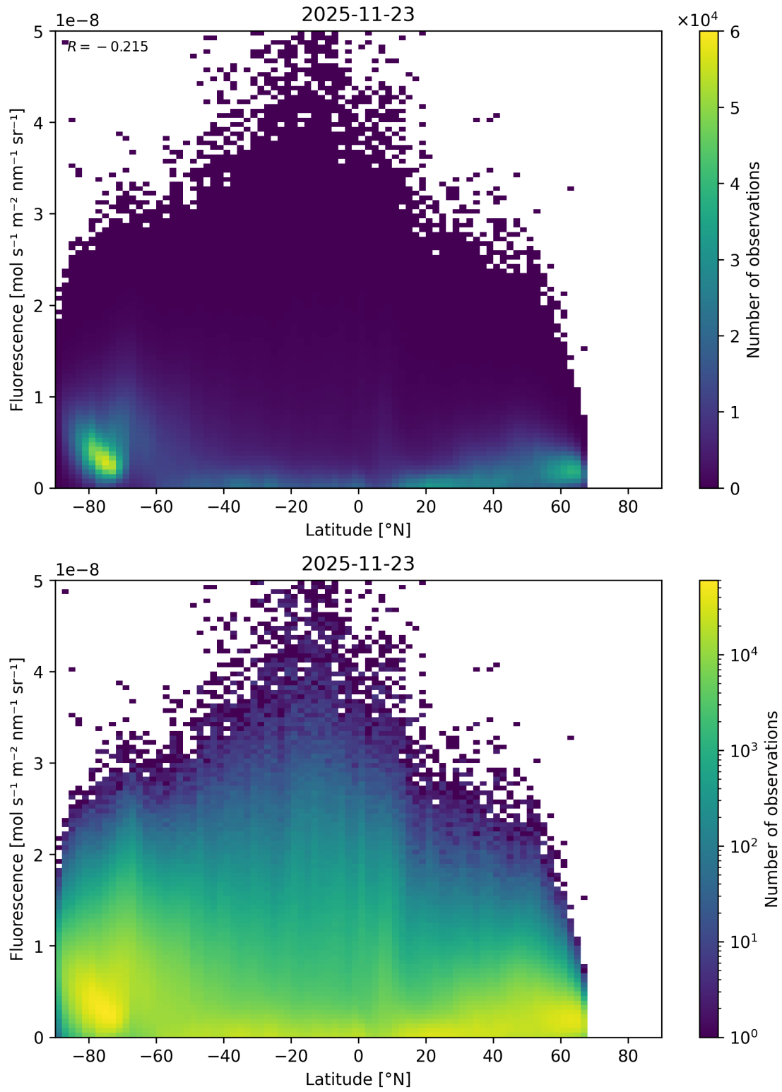
Figure 92: Scatter density plot of “Latitude” against “Fluorescence” for 2025-11-23 to 2025-11-24.
