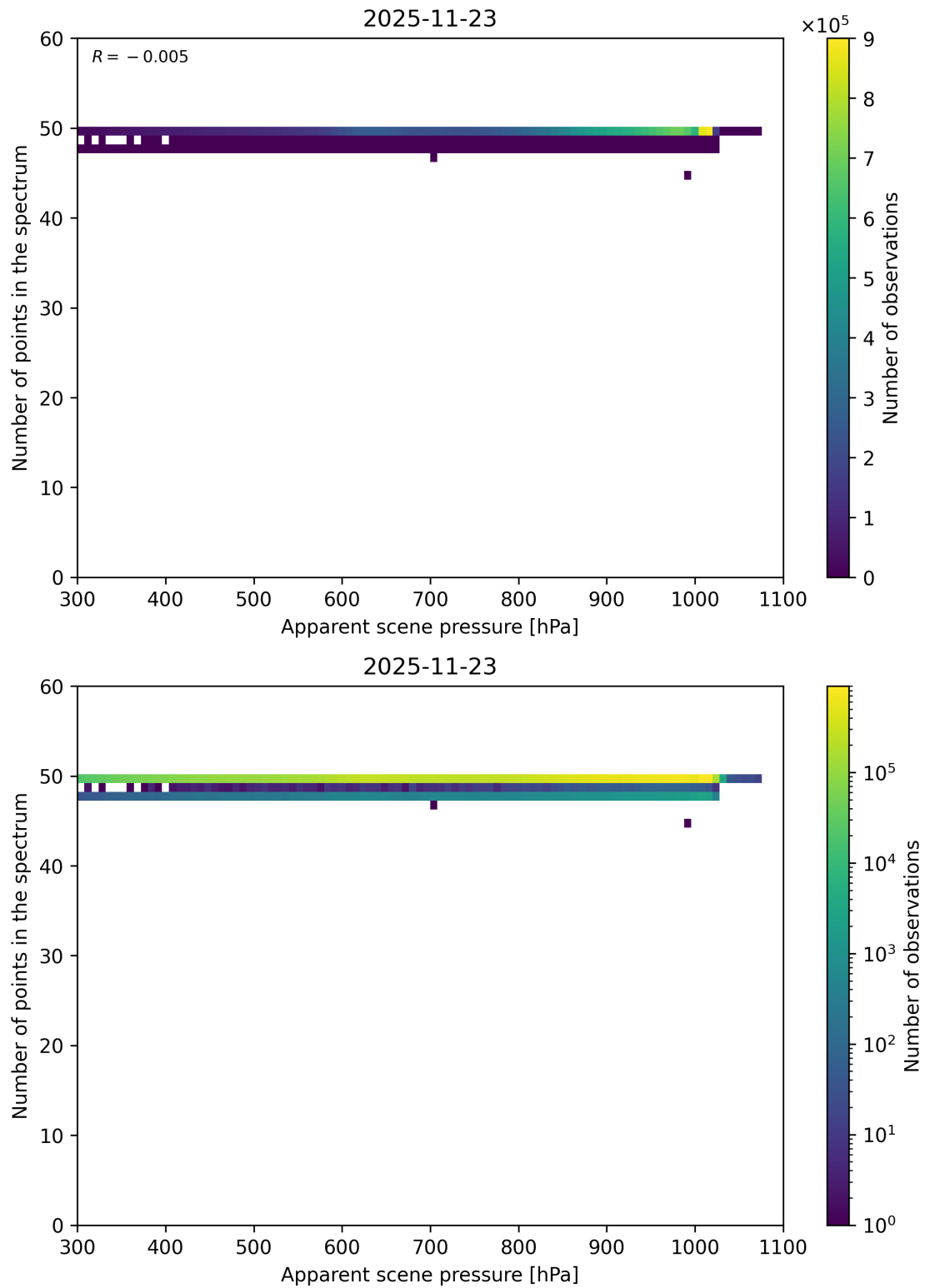
Figure 66: Scatter density plot of “Apparent scene pressure” against “Number of points in the spectrum” for 2025-11-23 to 2025-11-24.
