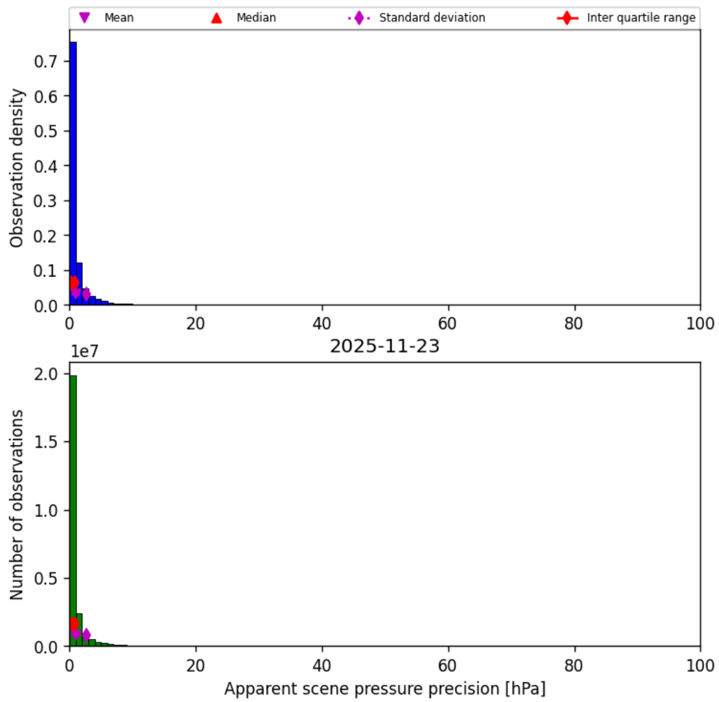
Figure 37: Histogram of “Apparent scene pressure precision” for 2025-11-23 to 2025-11-24
