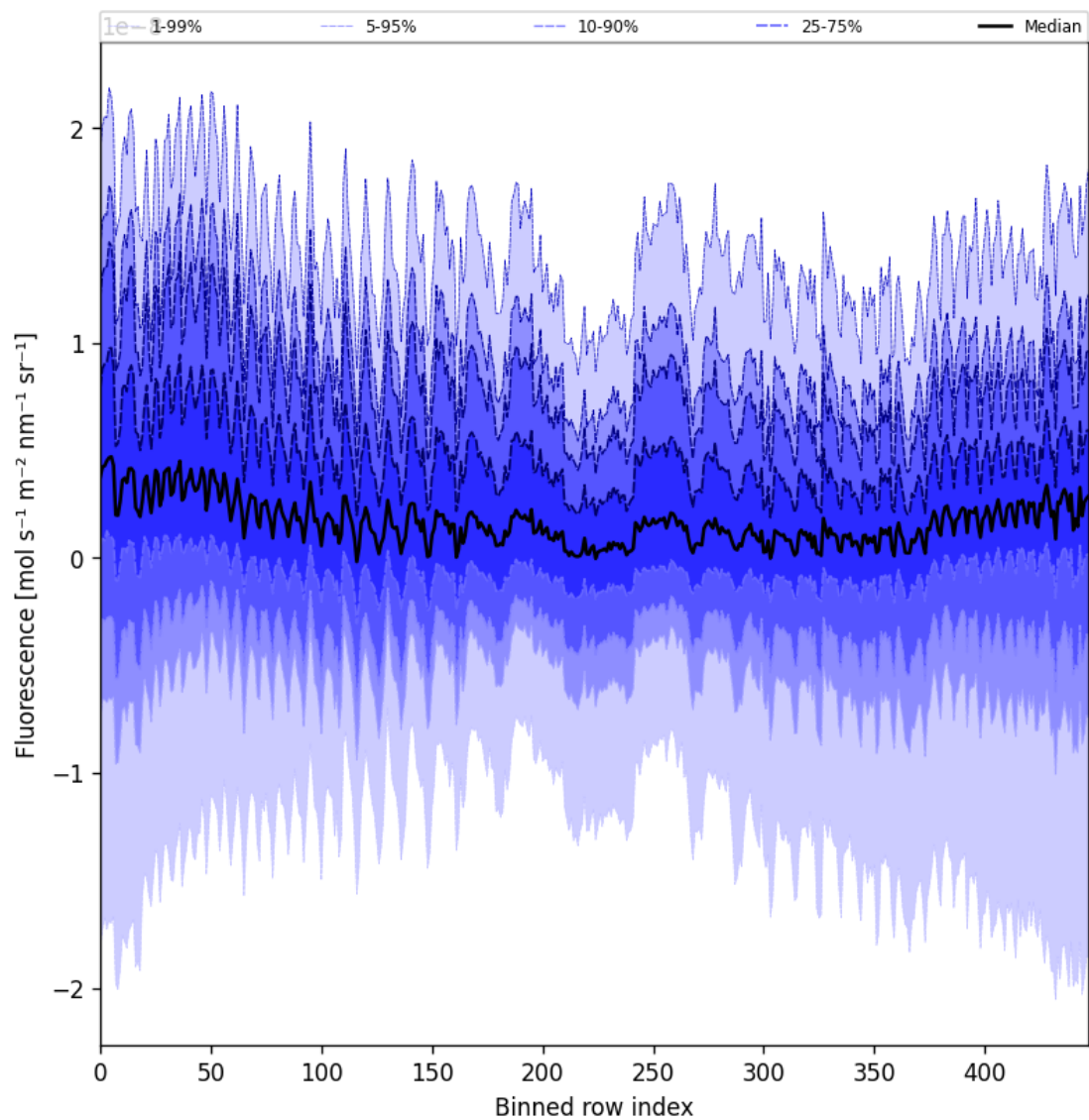
Figure 57: Along track statistics of “Fluorescence” for 2025-11-23 to 2025-11-24
