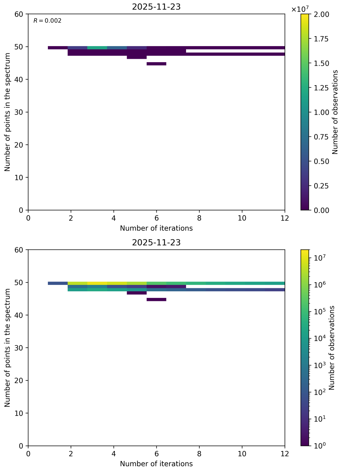
Figure 99: Scatter density plot of “Number of iterations” against “Number of points in the spectrum” for 2025-11-23 to 2025-11-24.
