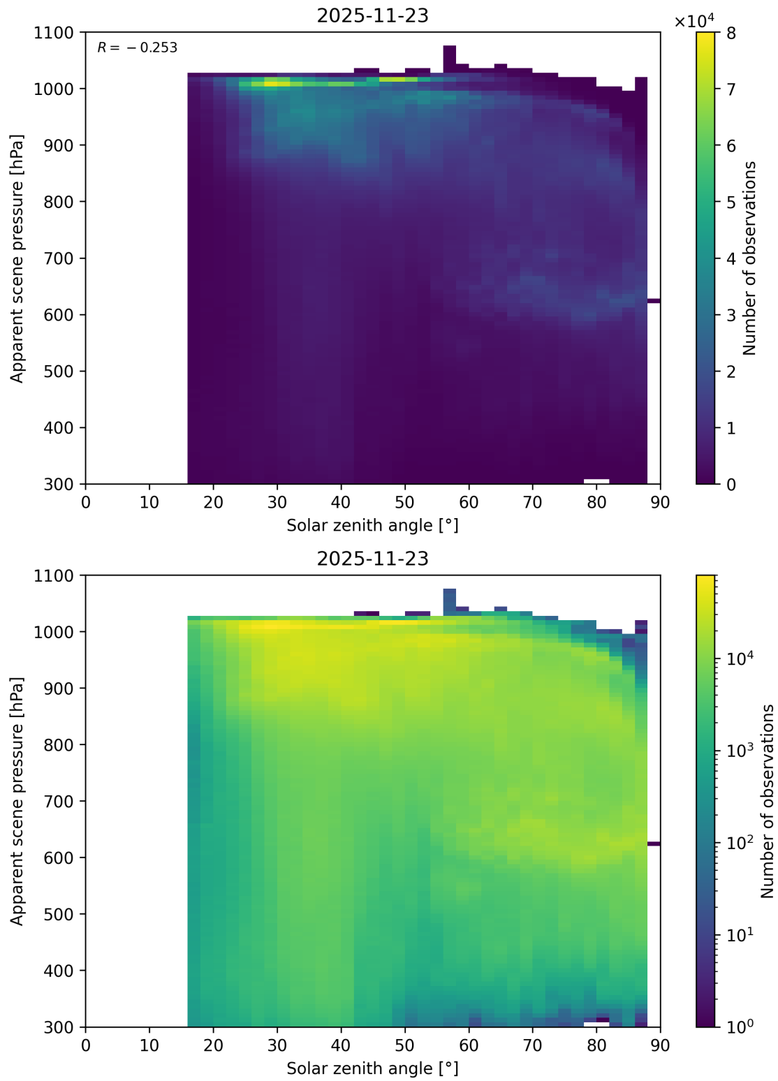
Figure 108: Scatter density plot of “Solar zenith angle” against “Apparent scene pressure” for 2025-11-23 to 2025-11-24.
