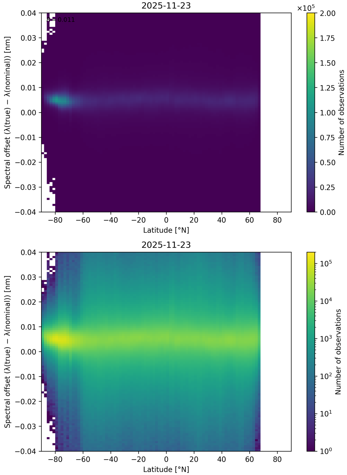
Figure 96: Scatter density plot of “Latitude” against “Spectral offset ( \lambda_{\text{true}} - \lambda_{\text{nominal}} )” for 2025-11-23 to 2025-11-24.
