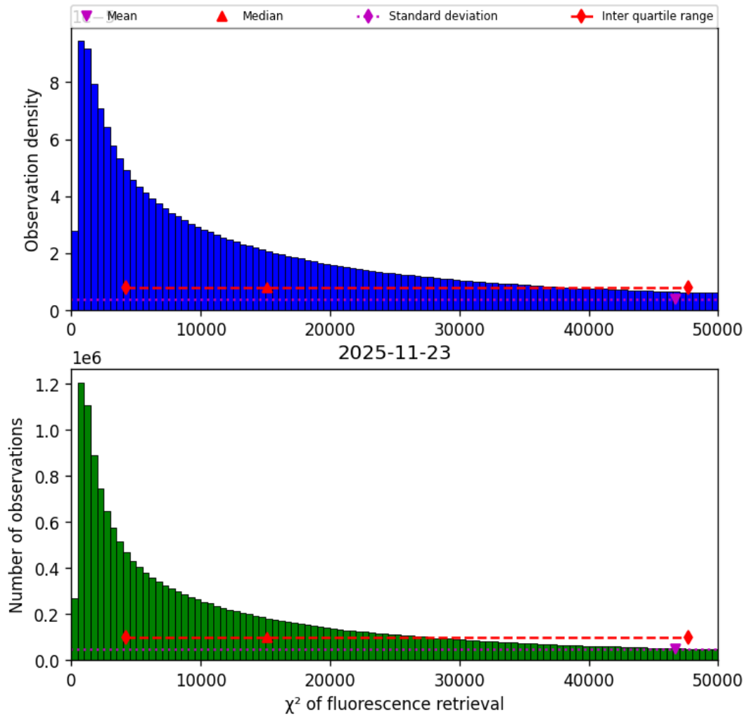
Figure 42: Histogram of “ \chi^2 of fluorescence retrieval” for 2025-11-23 to 2025-11-24
