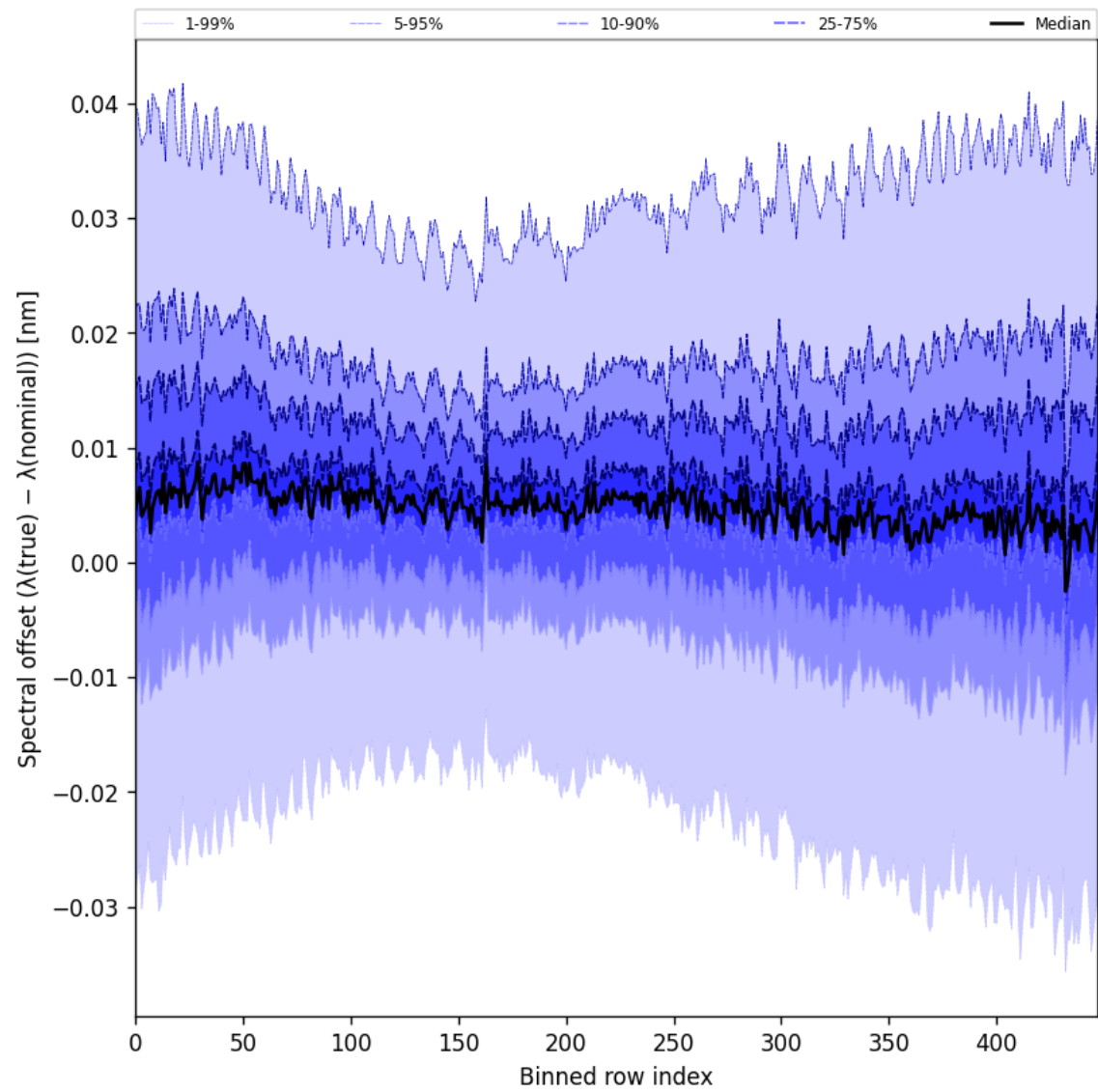
Figure 62: Along track statistics of “Spectral offset ( \lambda_{\text{true}} - \lambda_{\text{nominal}} )” for 2025-11-23 to 2025-11-24
