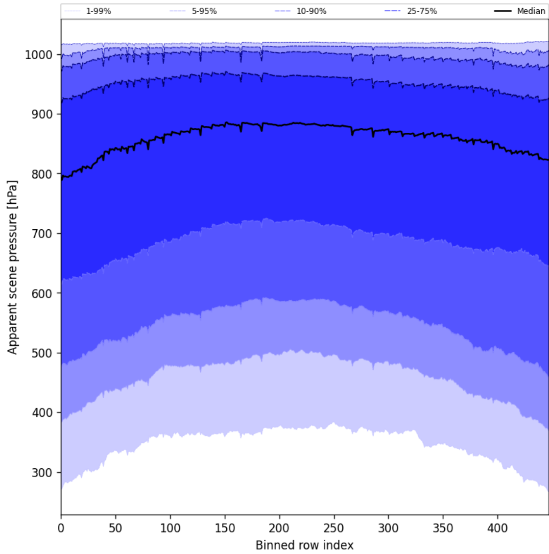
Figure 53: Along track statistics of “Apparent scene pressure” for 2025-11-23 to 2025-11-24
