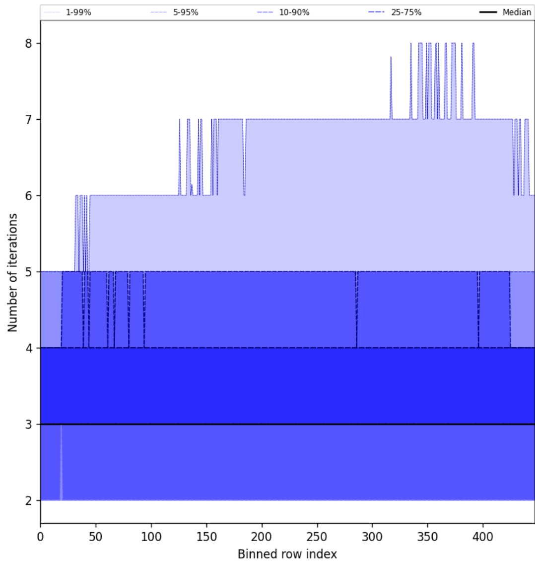
Figure 56: Along track statistics of “Number of iterations” for 2025-11-23 to 2025-11-24
