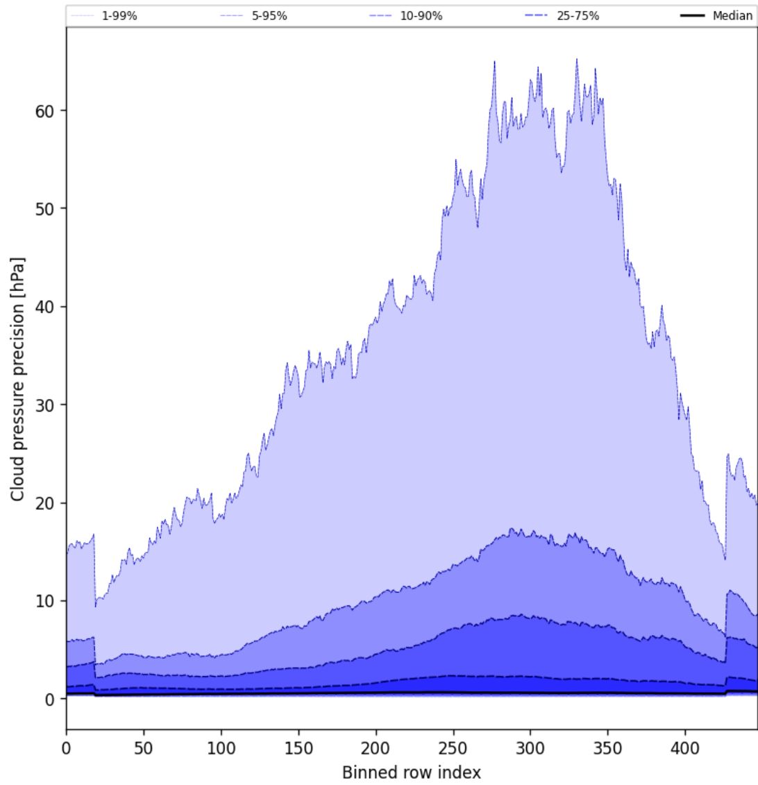
Figure 48: Along track statistics of “Cloud pressure precision” for 2025-11-23 to 2025-11-24
