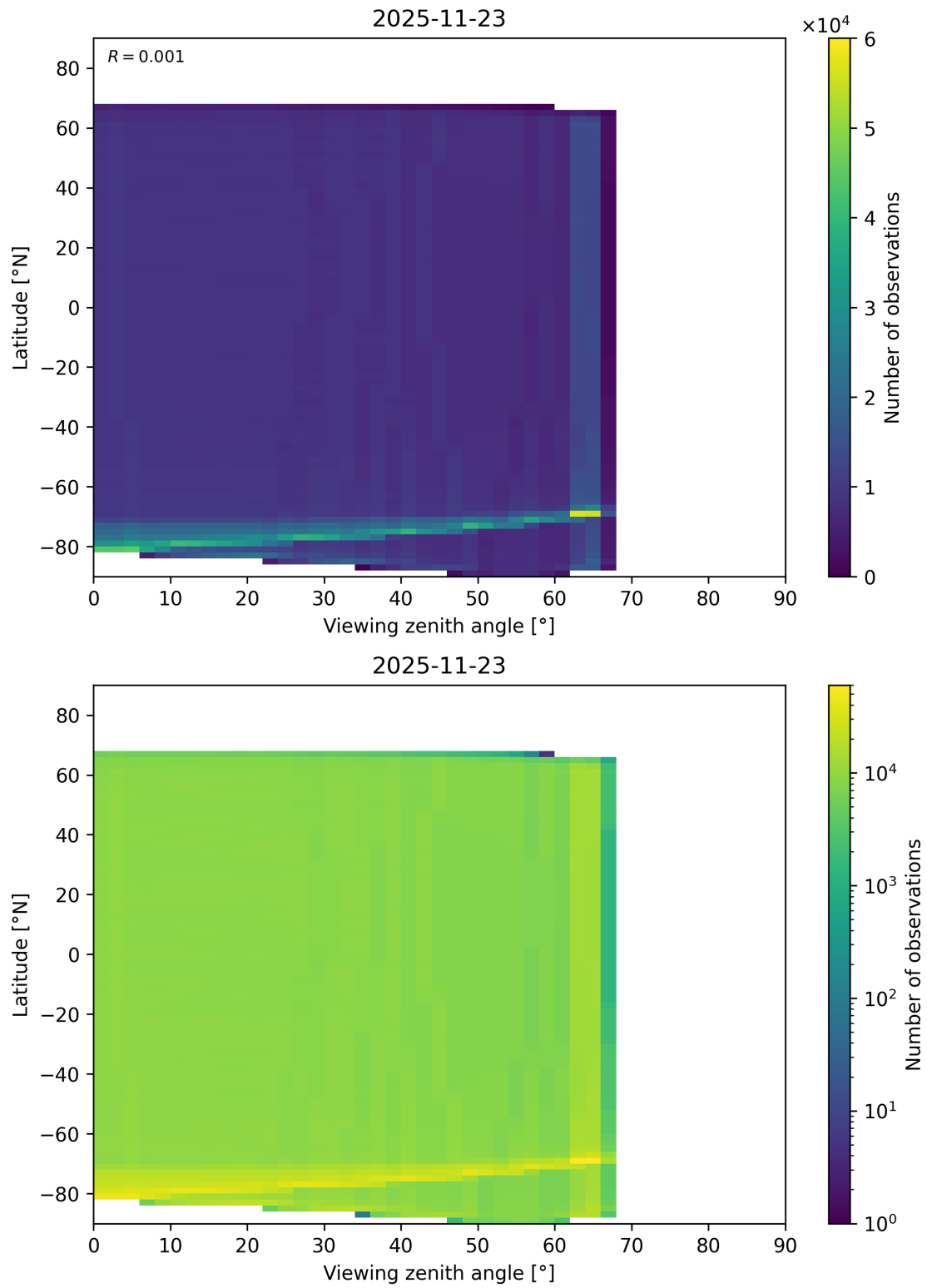
Figure 123: Scatter density plot of “Viewing zenith angle” against “Latitude” for 2025-11-23 to 2025-11-24.
