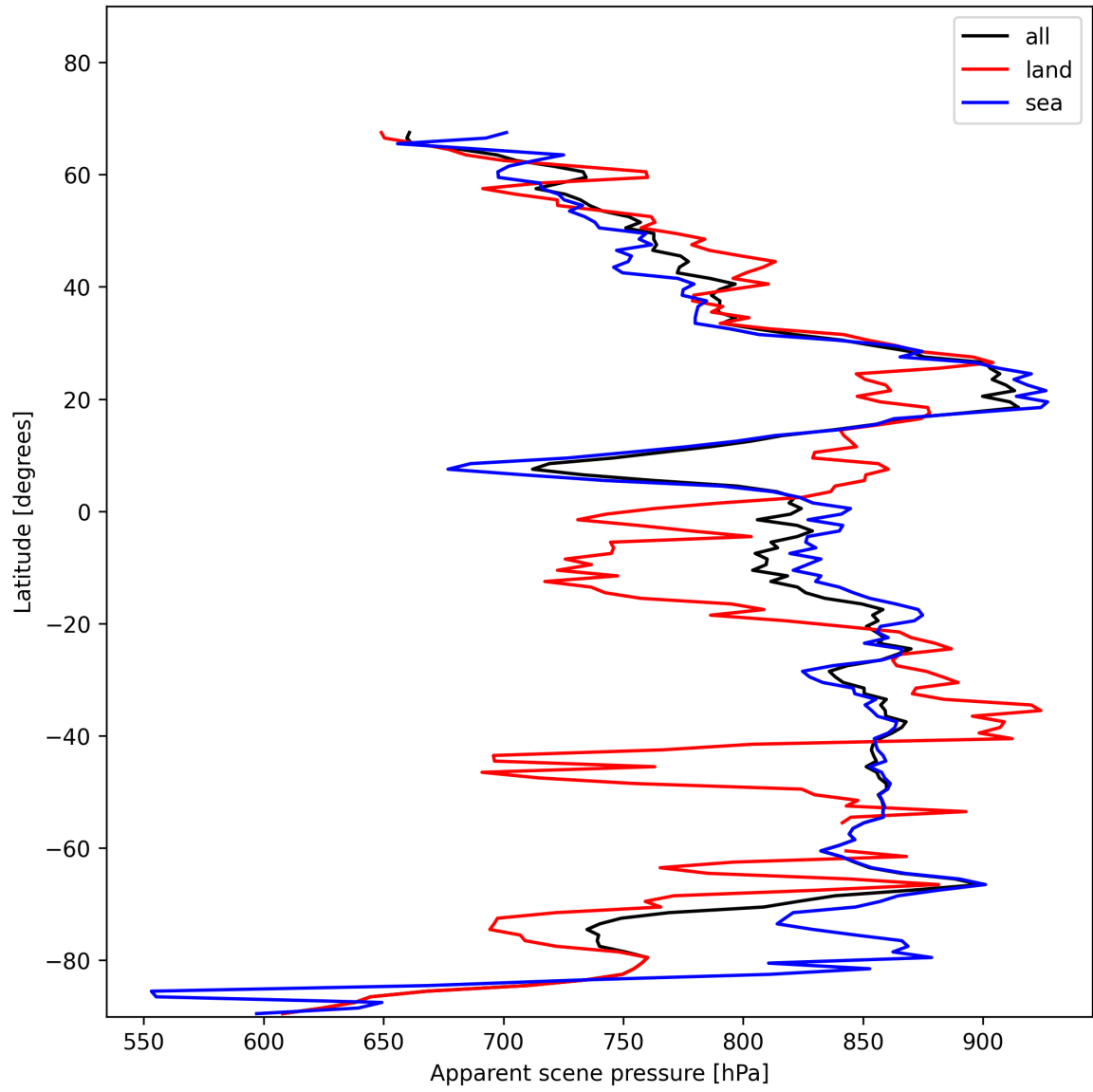
Figure 19: Zonal average of “Apparent scene pressure” for 2025-11-23 to 2025-11-24.
