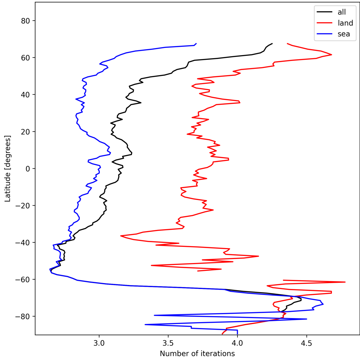
Figure 22: Zonal average of “Number of iterations” for 2025-11-23 to 2025-11-24.
