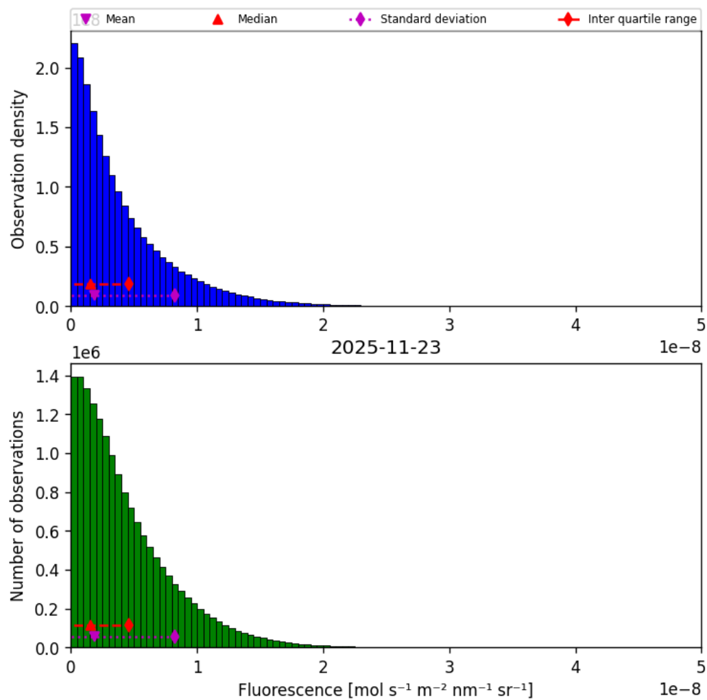
Figure 40: Histogram of “Fluorescence” for 2025-11-23 to 2025-11-24
