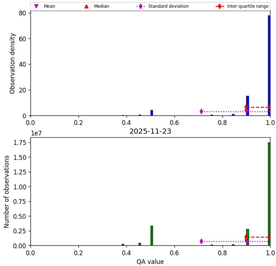
Figure 29: Histogram of “QA value” for 2025-11-23 to 2025-11-24
