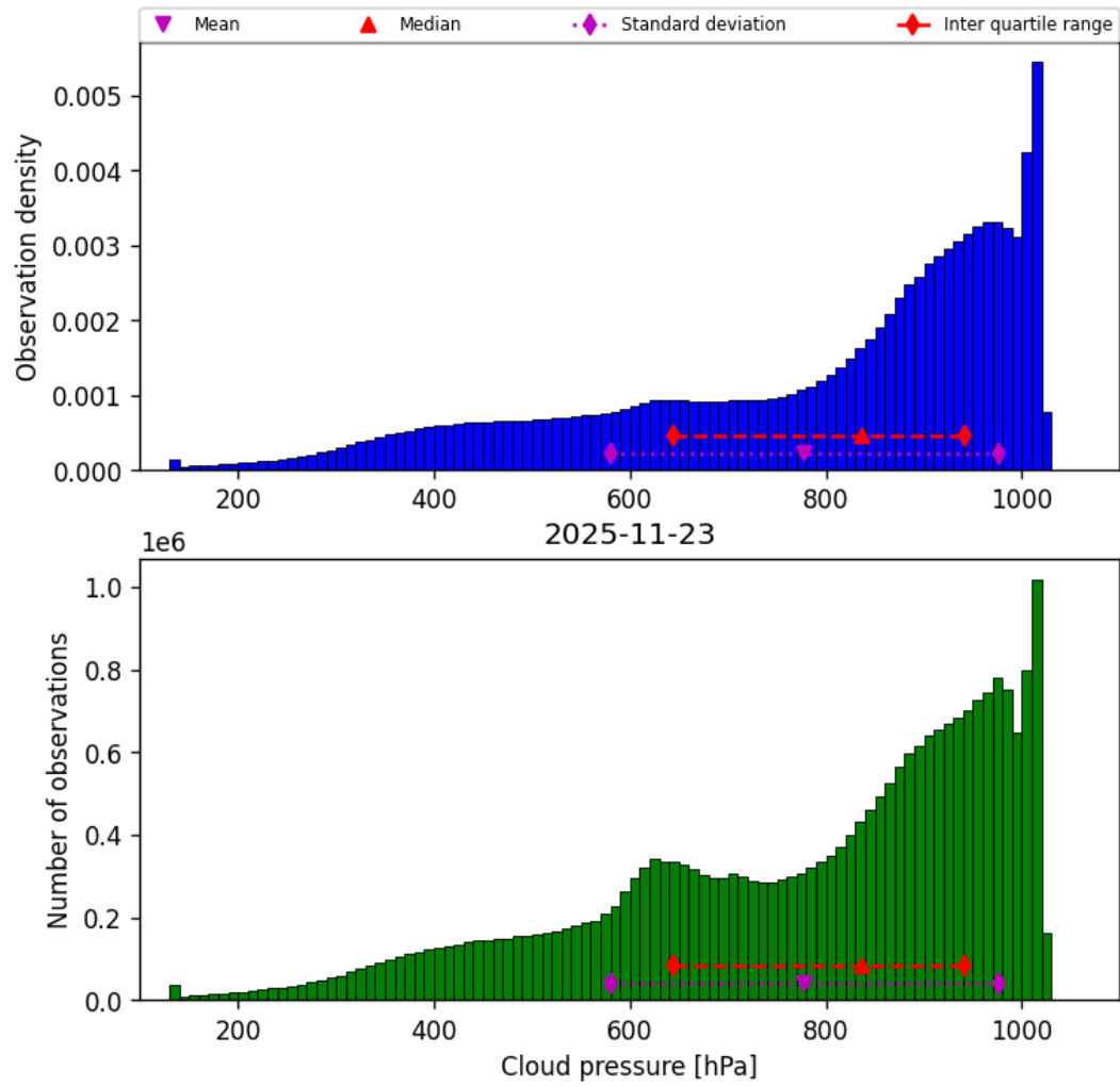
Figure 30: Histogram of “Cloud pressure” for 2025-11-23 to 2025-11-24
