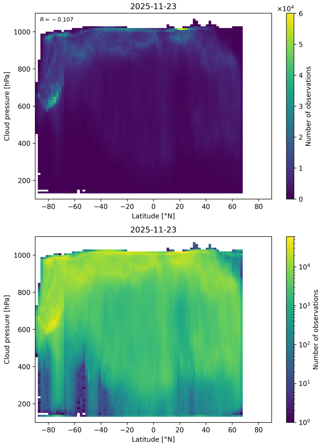
Figure 91: Scatter density plot of “Latitude” against “Cloud pressure” for 2025-11-23 to 2025-11-24.
