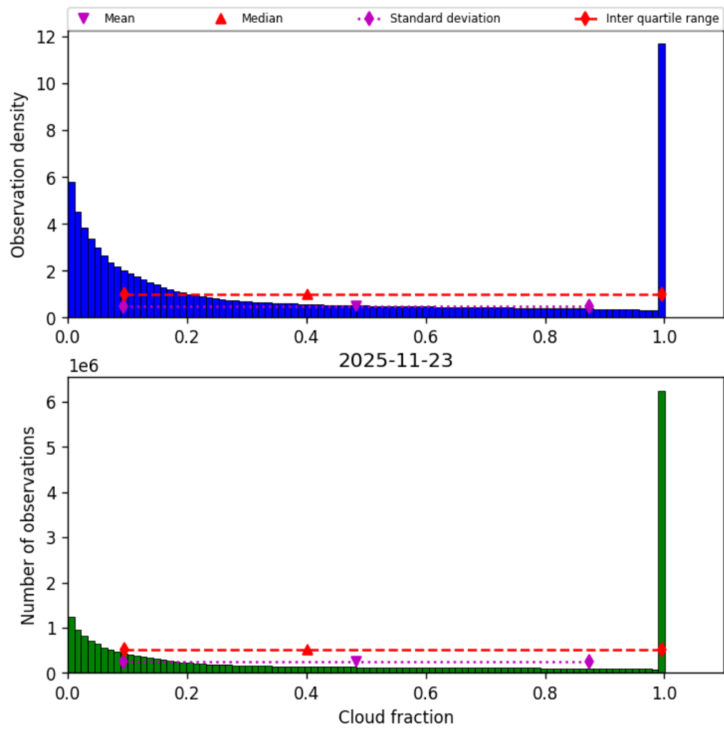
Figure 32: Histogram of “Cloud fraction” for 2025-11-23 to 2025-11-24
