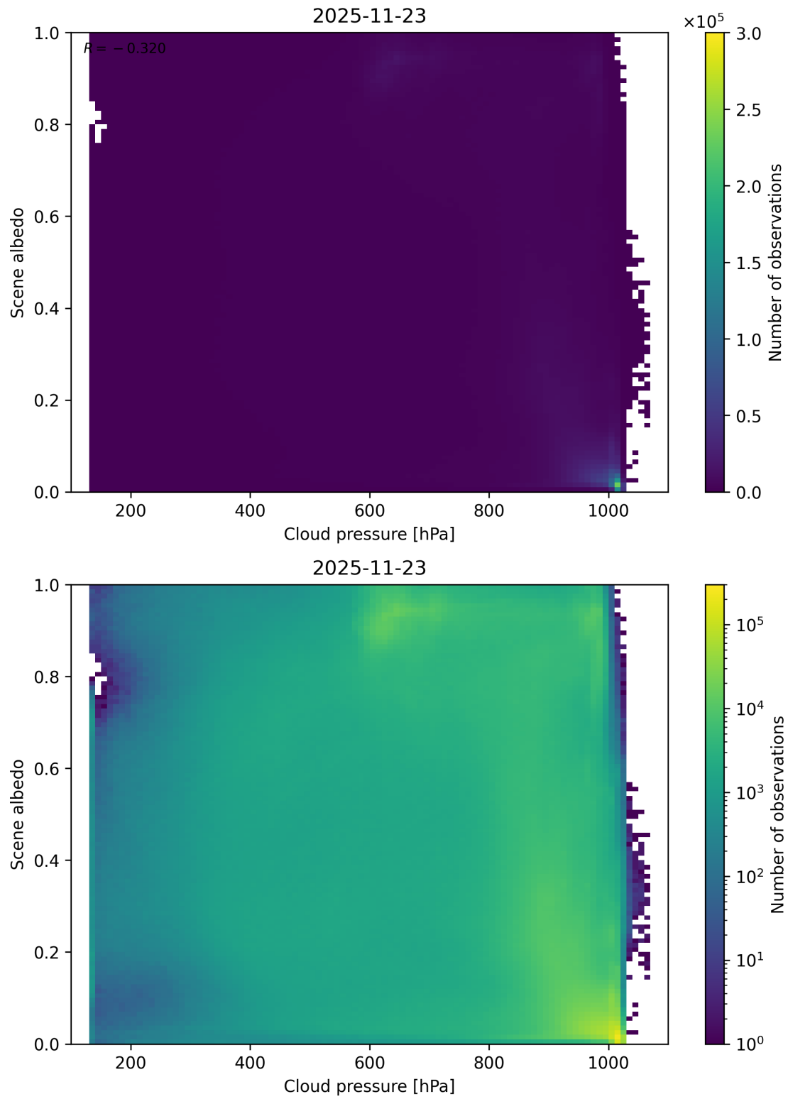
Figure 83: Scatter density plot of “Cloud pressure” against “Scene albedo” for 2025-11-23 to 2025-11-24.
