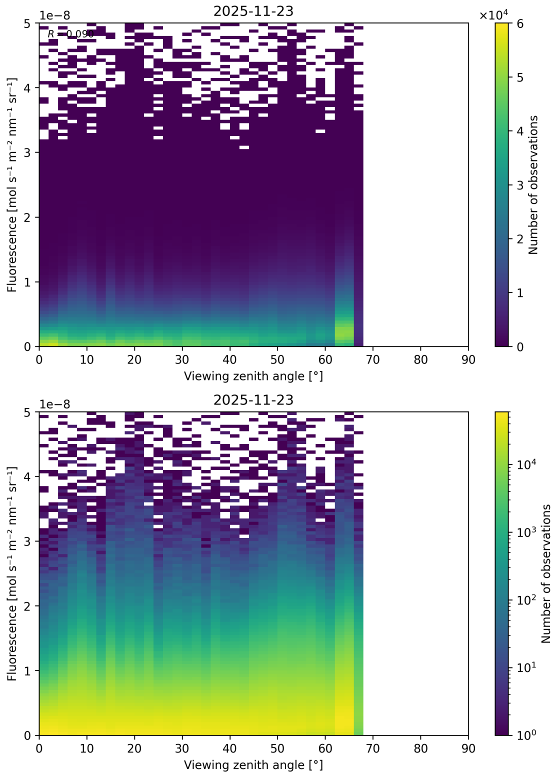
Figure 122: Scatter density plot of “Viewing zenith angle” against “Fluorescence” for 2025-11-23 to 2025-11-24.
