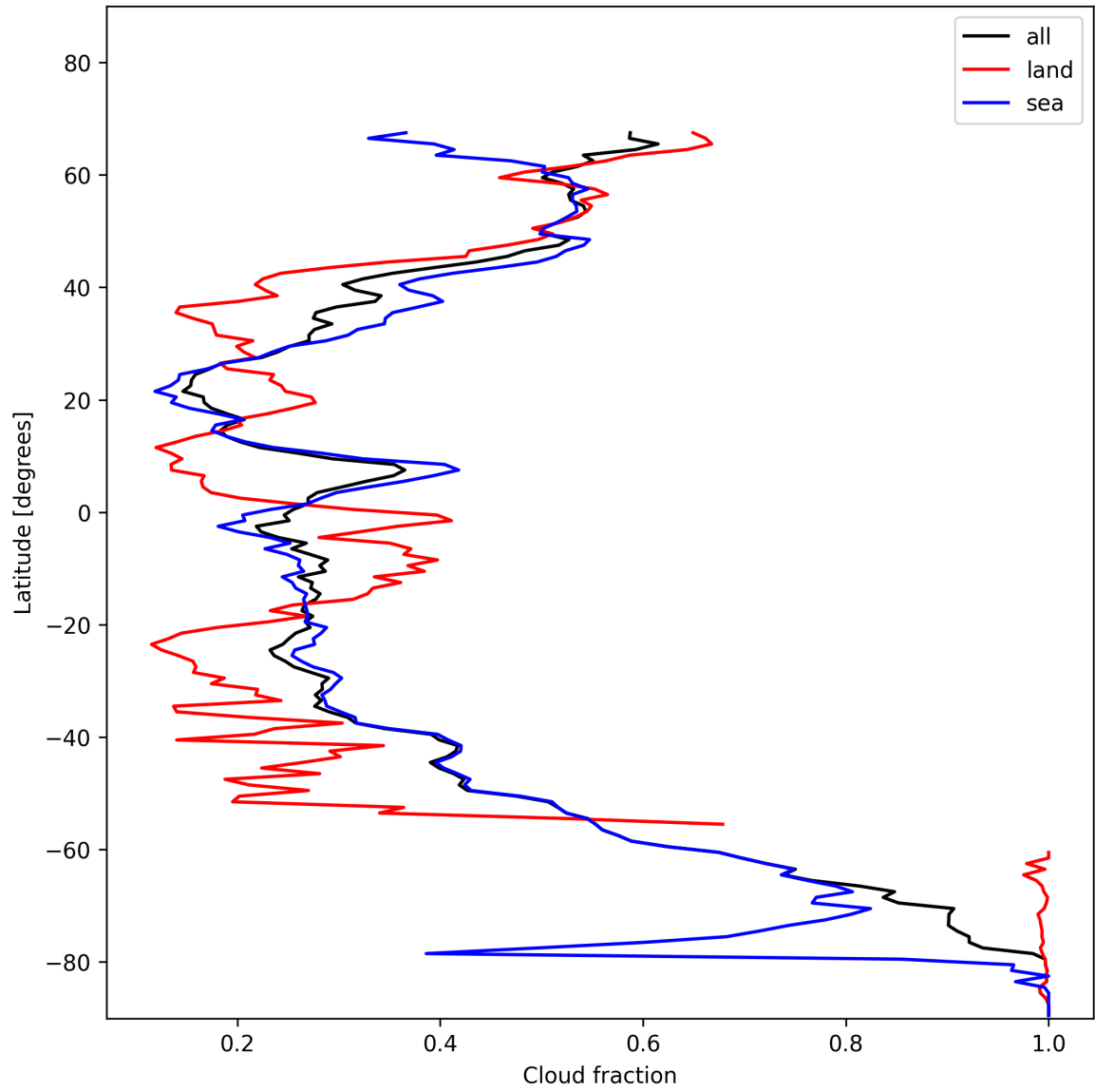
Figure 15: Zonal average of “Cloud fraction” for 2025-11-23 to 2025-11-24.
