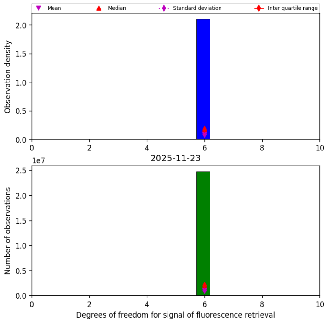
Figure 43: Histogram of “Degrees of freedom for signal of fluorescence retrieval” for 2025-11-23 to 2025-11-24
