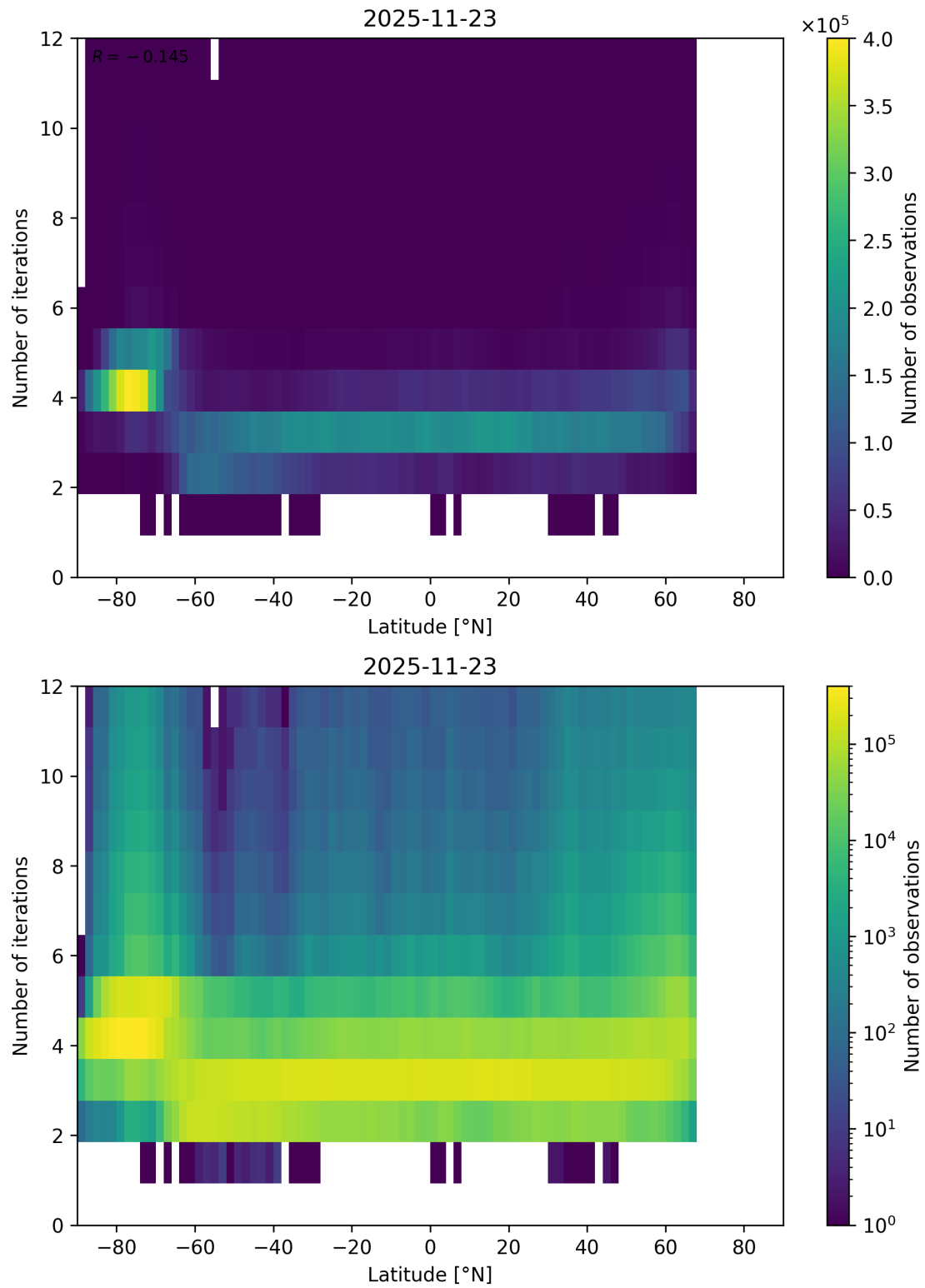
Figure 93: Scatter density plot of “Latitude” against “Number of iterations” for 2025-11-23 to 2025-11-24.
