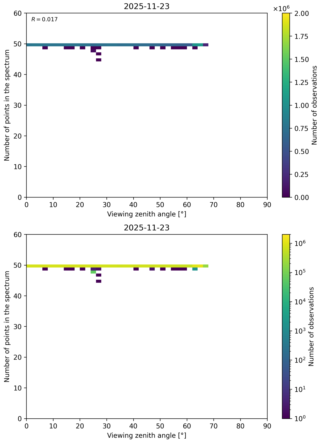
Figure 125: Scatter density plot of “Viewing zenith angle” against “Number of points in the spectrum” for 2025-11-23 to 2025-11-24.
