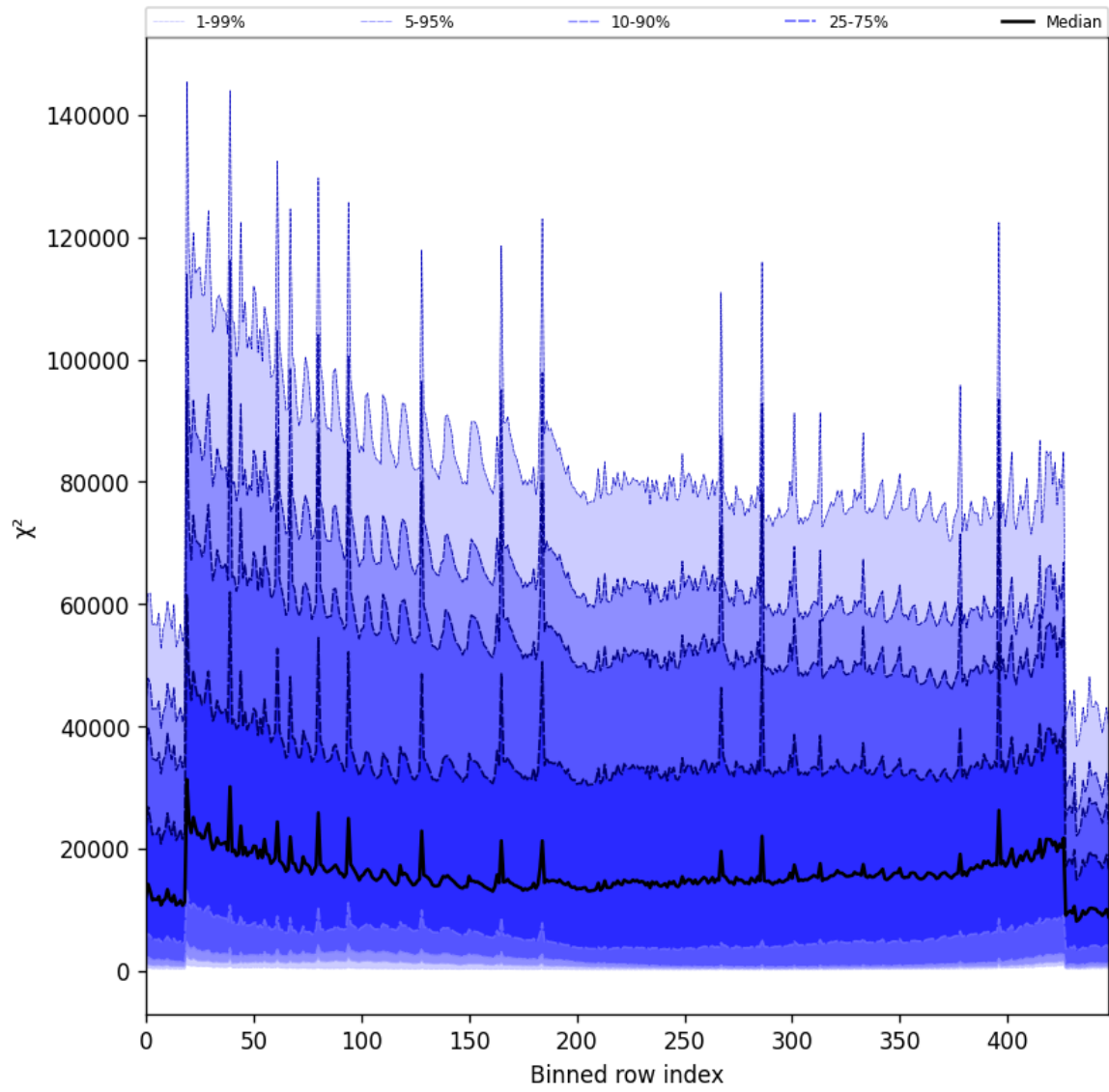
Figure 55: Along track statistics of “ \chi^2 ” for 2025-11-23 to 2025-11-24
