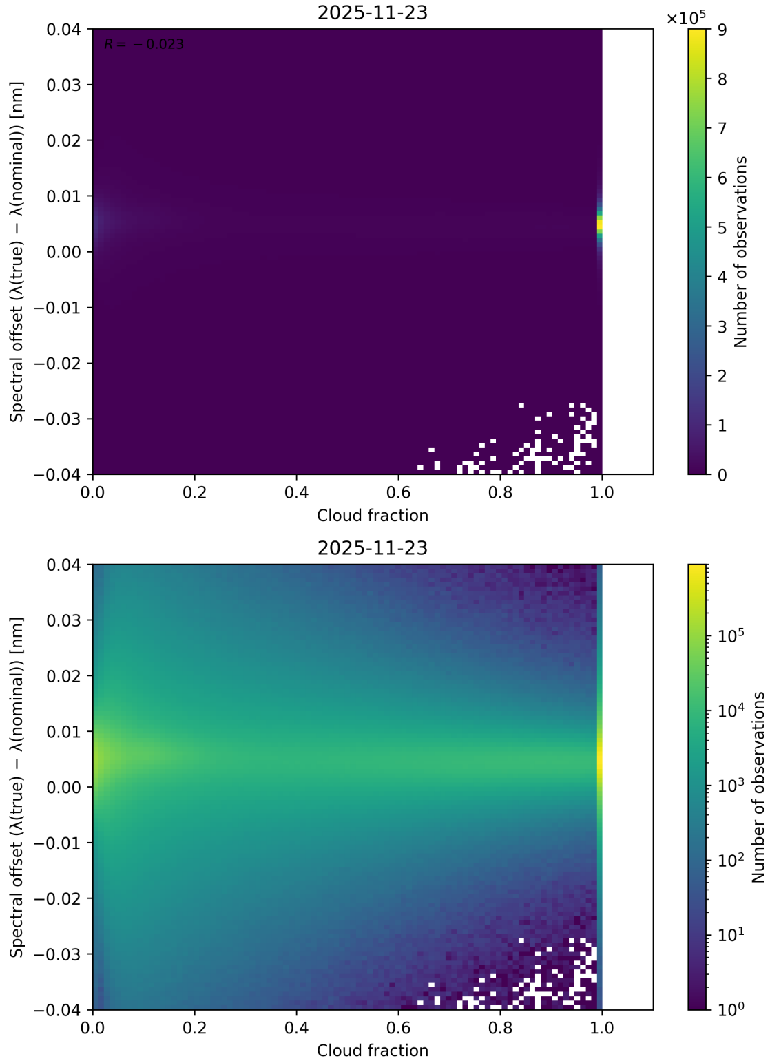
Figure 76: Scatter density plot of “Cloud fraction” against “Spectral offset ( \lambda_{\text{true}} - \lambda_{\text{nominal}} )” for 2025-11-23 to 2025-11-24.
