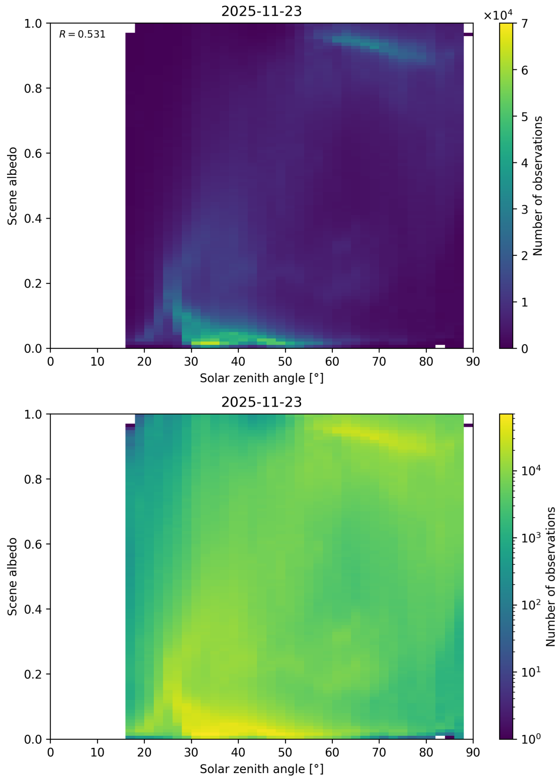
Figure 116: Scatter density plot of “Solar zenith angle” against “Scene albedo” for 2025-11-23 to 2025-11-24.
