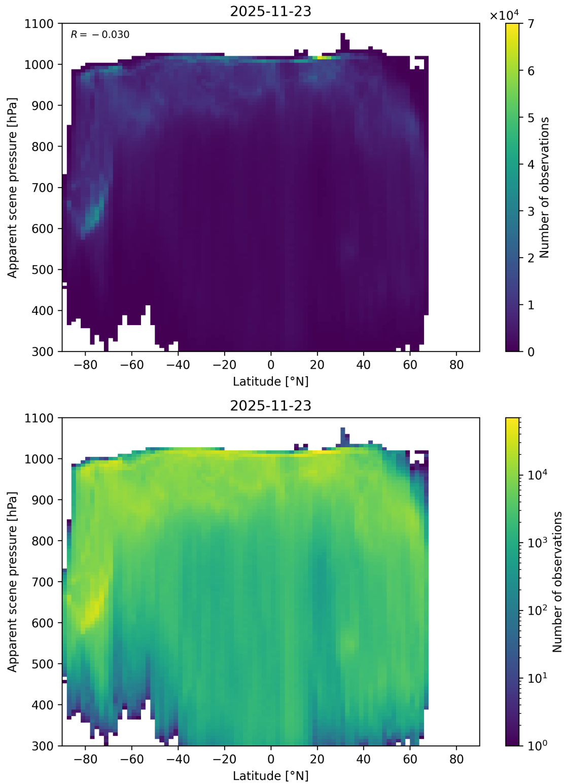
Figure 88: Scatter density plot of “Latitude” against “Apparent scene pressure” for 2025-11-23 to 2025-11-24.
