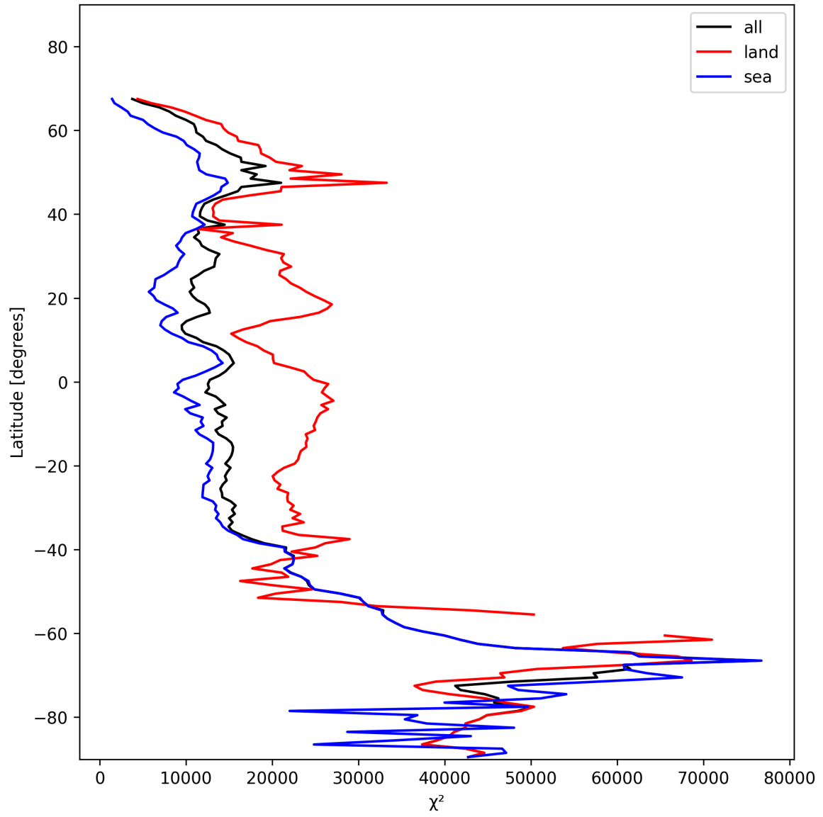
Figure 21: Zonal average of “ \chi^2 ” for 2025-11-23 to 2025-11-24.
