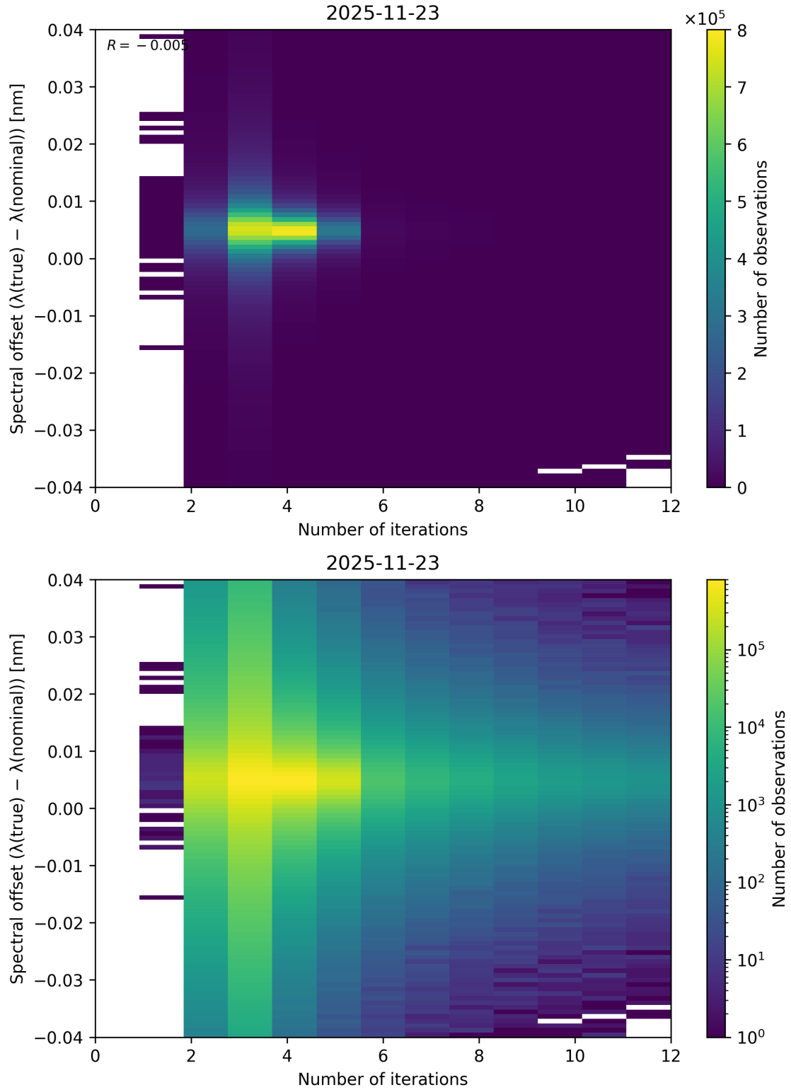
Figure 100: Scatter density plot of “Number of iterations” against “Spectral offset ( \lambda_{\text{true}} - \lambda_{\text{nominal}} )” for 2025-11-23 to 2025-11-24.
