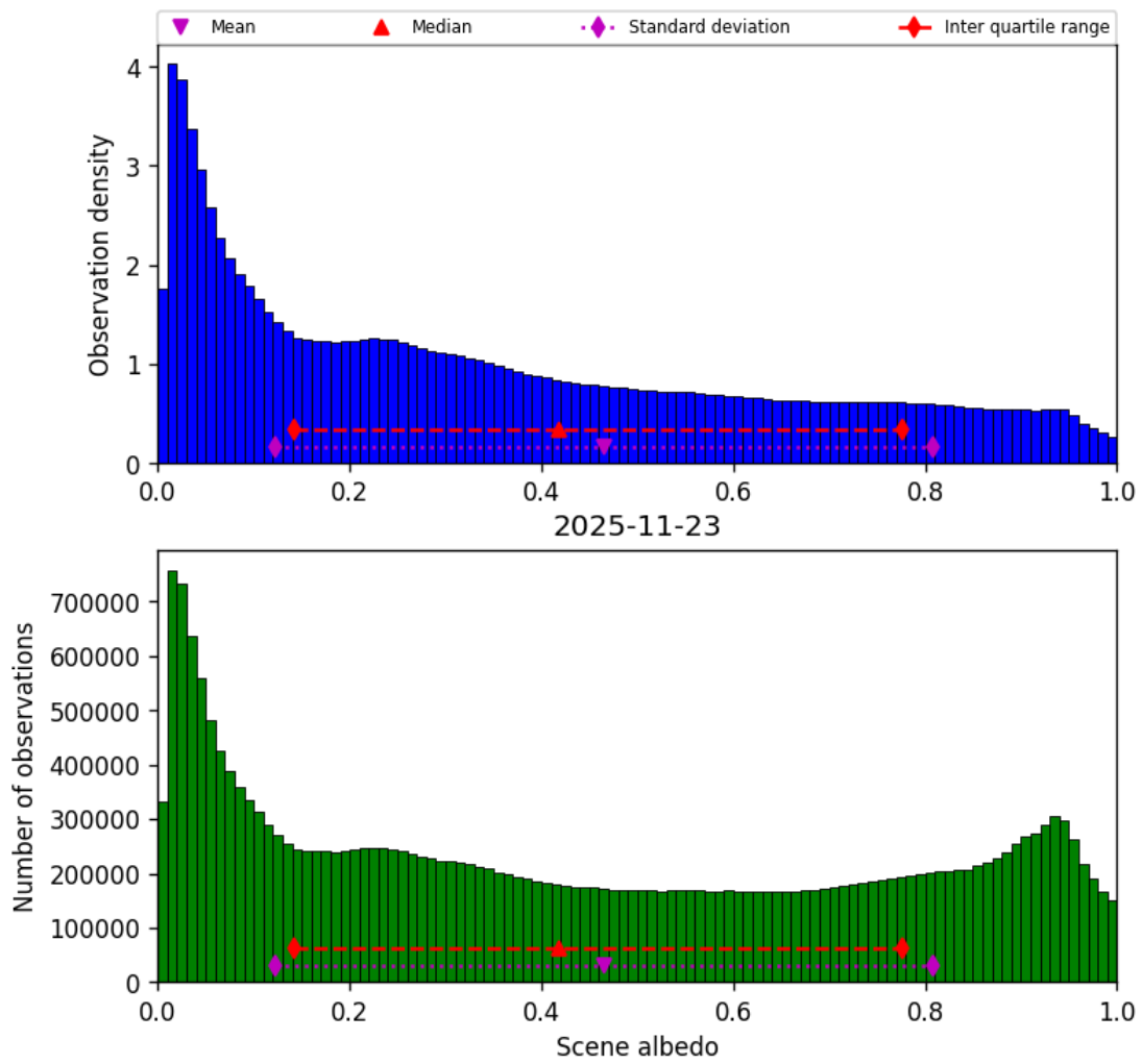
Figure 34: Histogram of “Scene albedo” for 2025-11-23 to 2025-11-24
