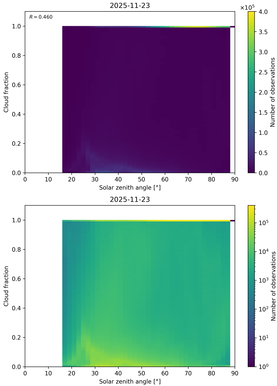
Figure 110: Scatter density plot of “Solar zenith angle” against “Cloud fraction” for 2025-11-23 to 2025-11-24.
