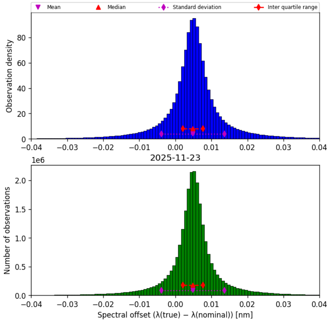
Figure 45: Histogram of “Spectral offset ( \lambda_{\text{true}} - \lambda_{\text{nominal}} )” for 2025-11-23 to 2025-11-24
