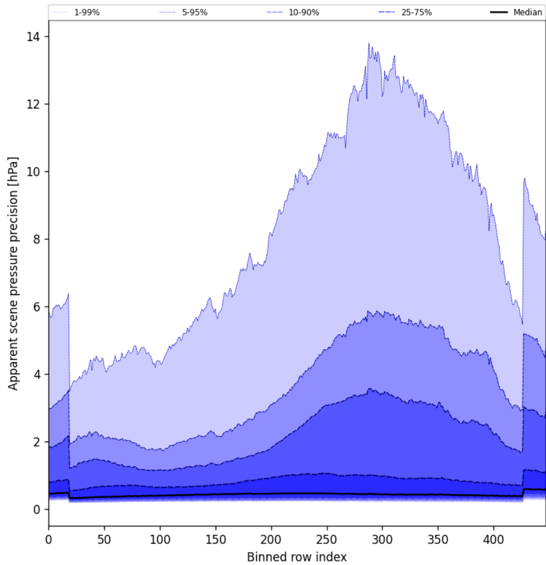
Figure 54: Along track statistics of “Apparent scene pressure precision” for 2025-11-23 to 2025-11-24
