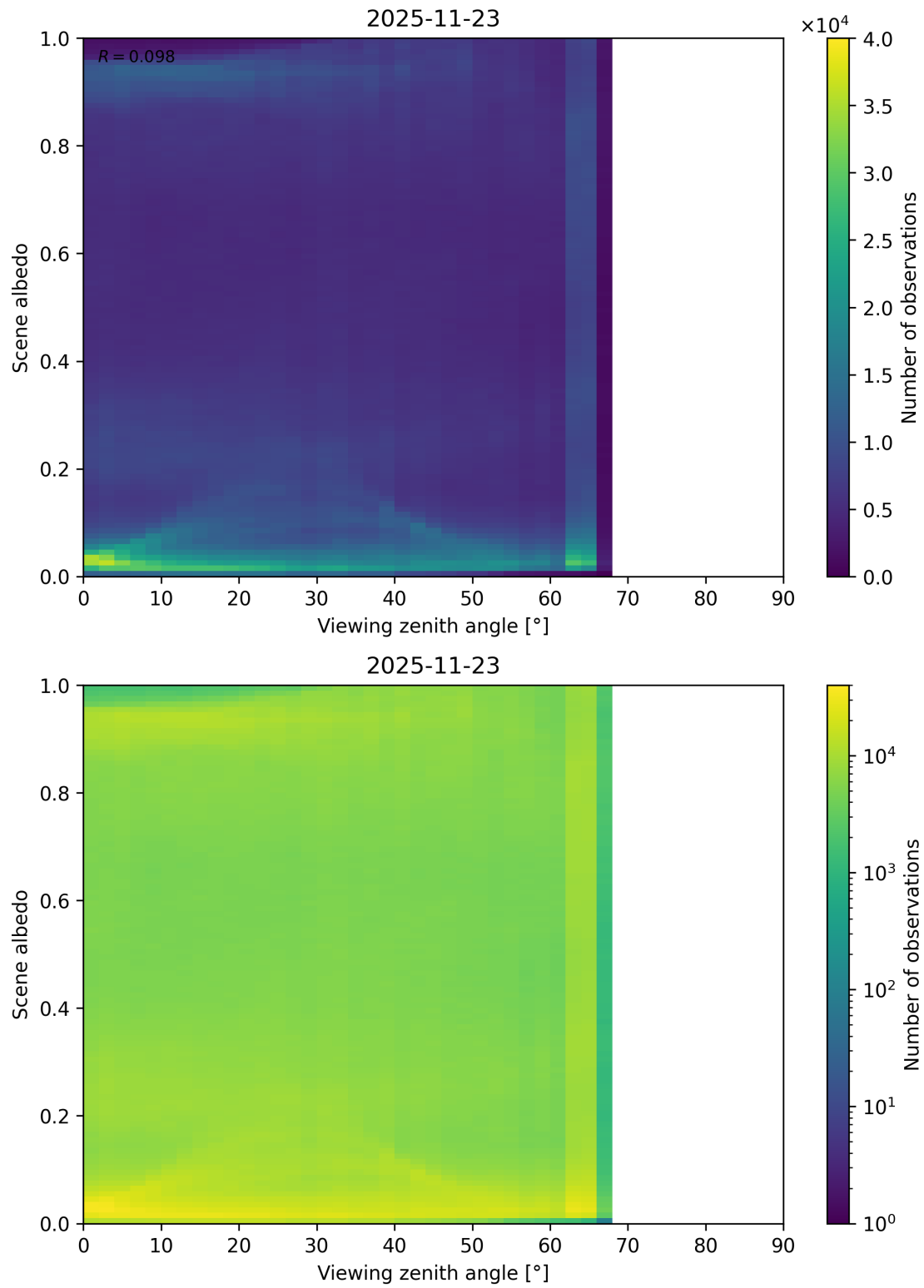
Figure 126: Scatter density plot of “Viewing zenith angle” against “Scene albedo” for 2025-11-23 to 2025-11-24.
