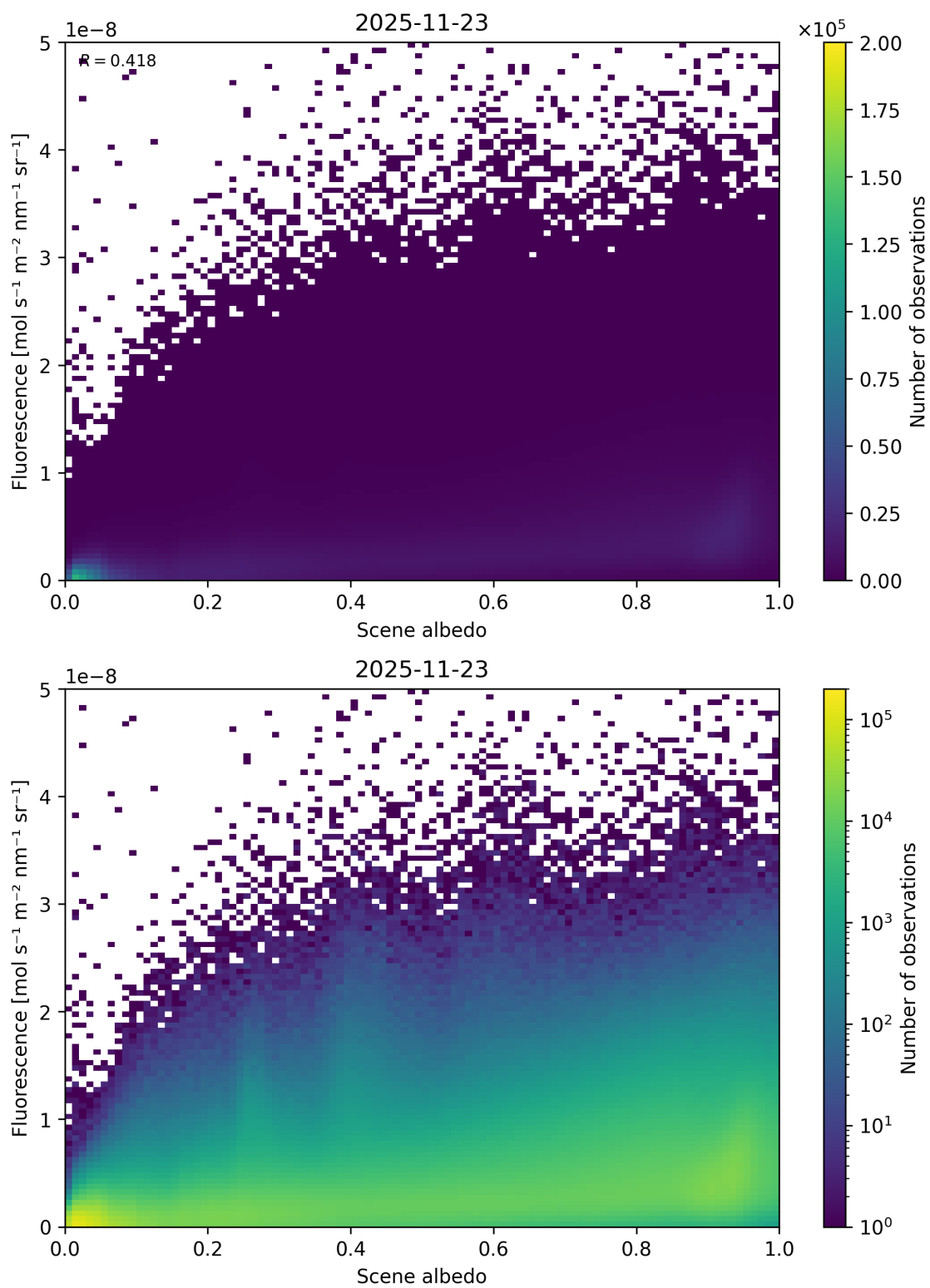
Figure 104: Scatter density plot of “Scene albedo” against “Fluorescence” for 2025-11-23 to 2025-11-24.
