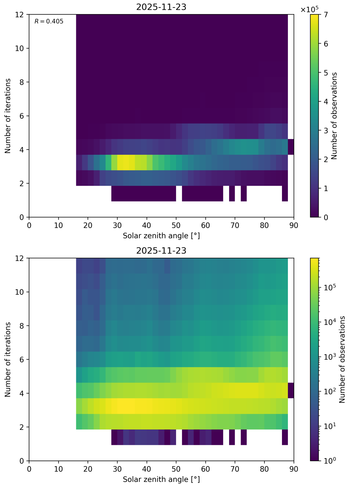
Figure 114: Scatter density plot of “Solar zenith angle” against “Number of iterations” for 2025-11-23 to 2025-11-24.
