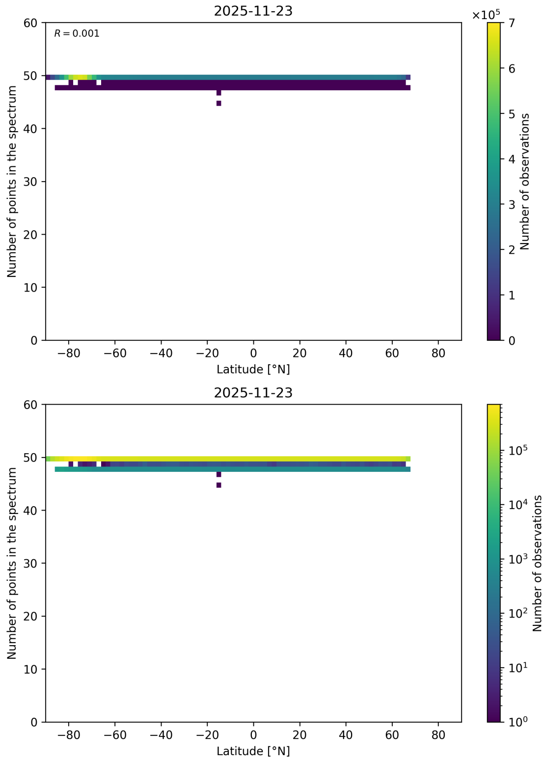
Figure 94: Scatter density plot of “Latitude” against “Number of points in the spectrum” for 2025-11-23 to 2025-11-24.
