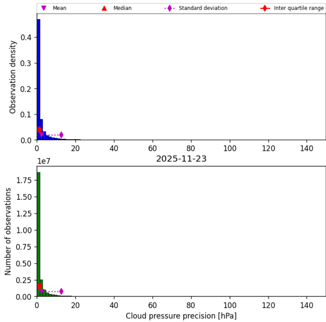
Figure 31: Histogram of “Cloud pressure precision” for 2025-11-23 to 2025-11-24
