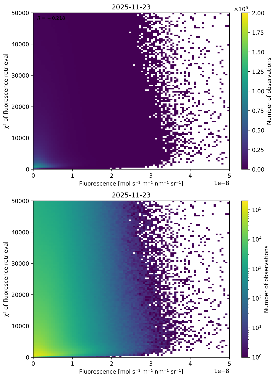
Figure 85: Scatter density plot of “Fluorescence” against “ \chi^2 of fluorescence retrieval” for 2025-11-23 to 2025-11-24.
