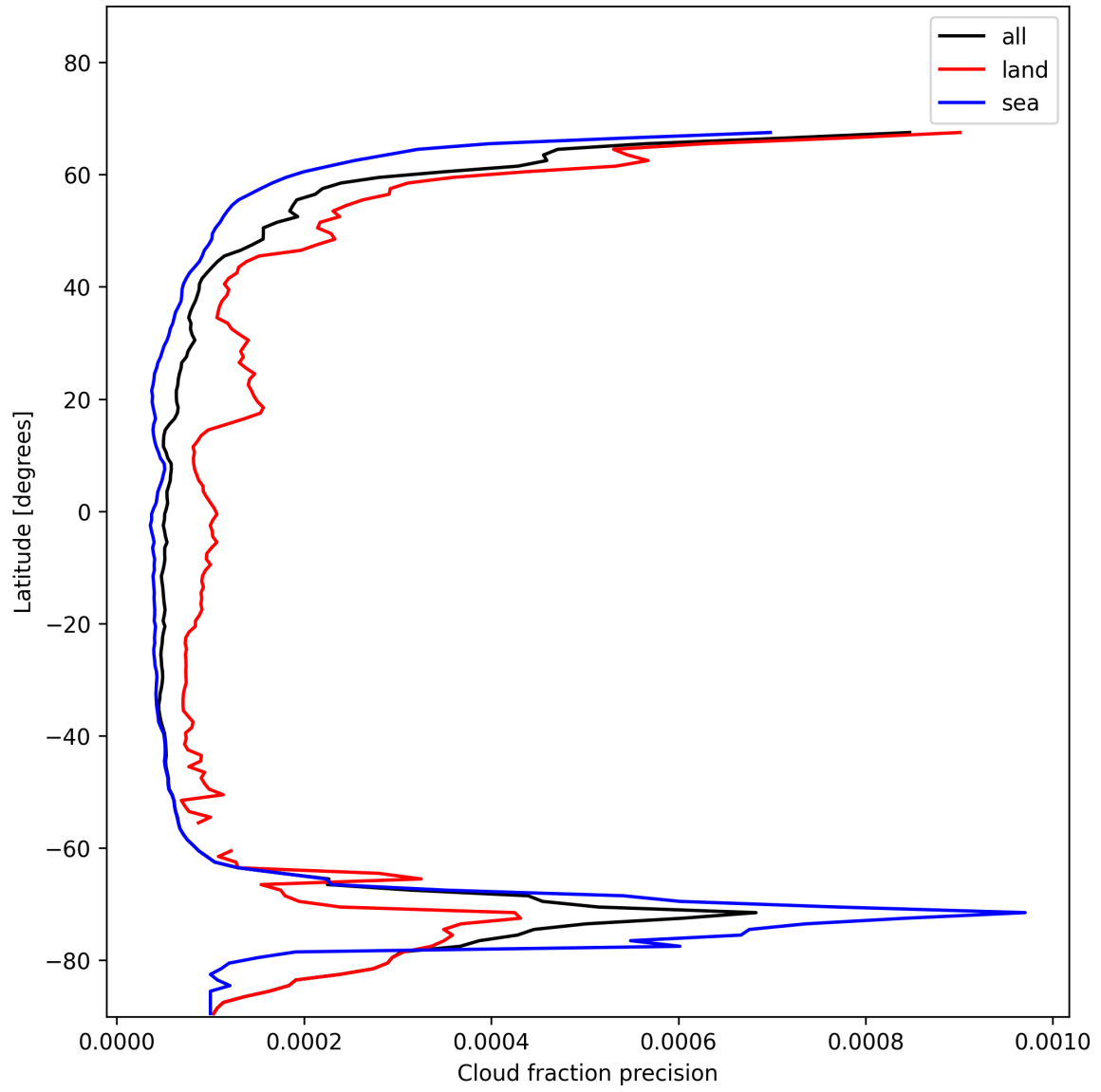
Figure 16: Zonal average of “Cloud fraction precision” for 2025-11-23 to 2025-11-24.
