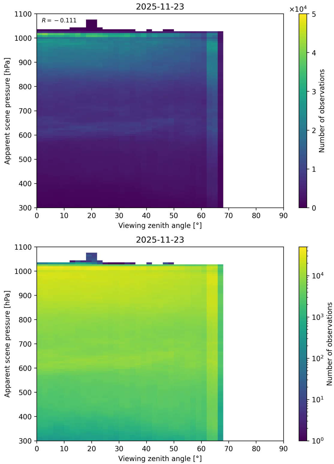
Figure 118: Scatter density plot of “Viewing zenith angle” against “Apparent scene pressure” for 2025-11-23 to 2025-11-24.
