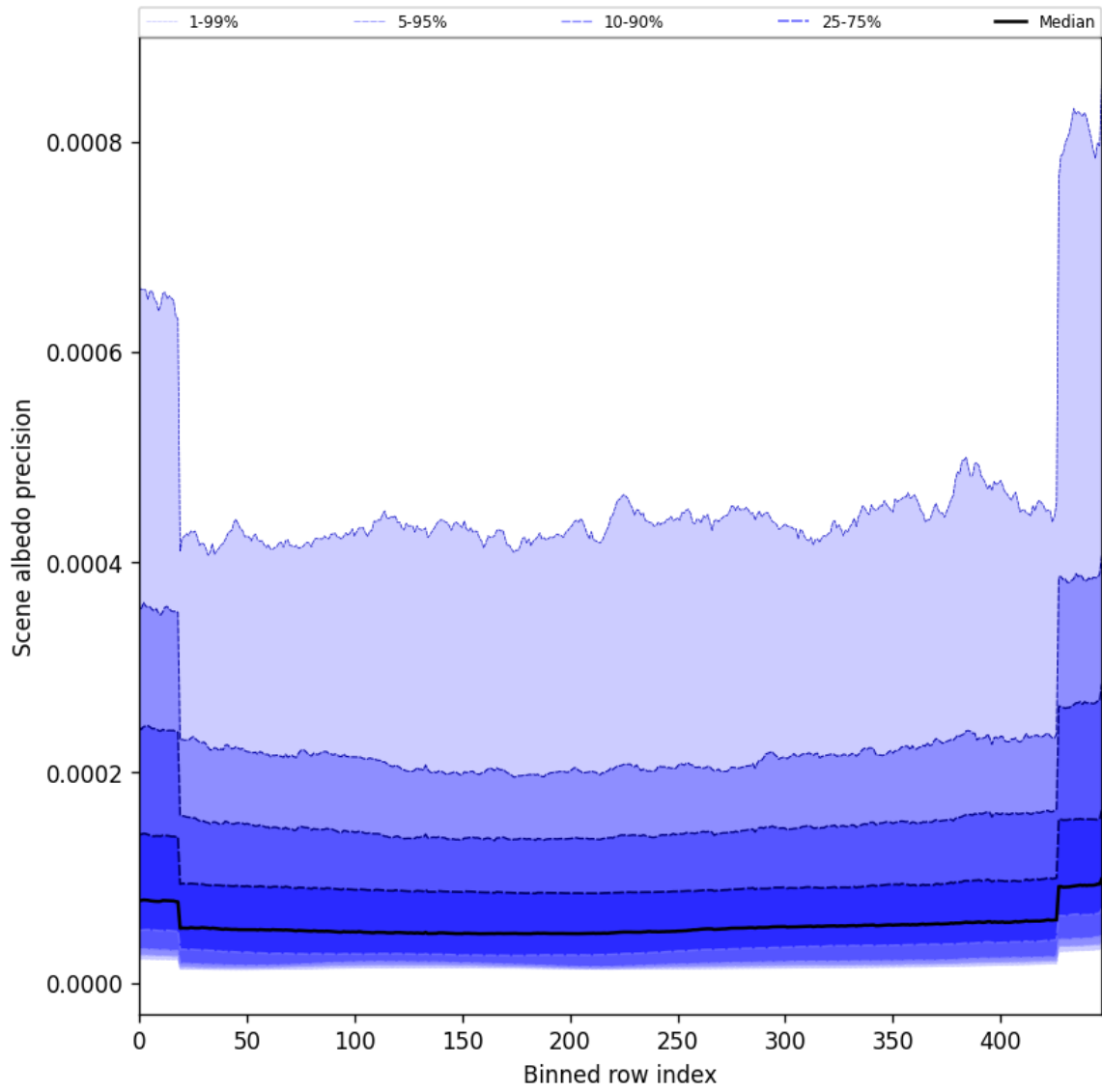
Figure 52: Along track statistics of “Scene albedo precision” for 2025-11-23 to 2025-11-24
