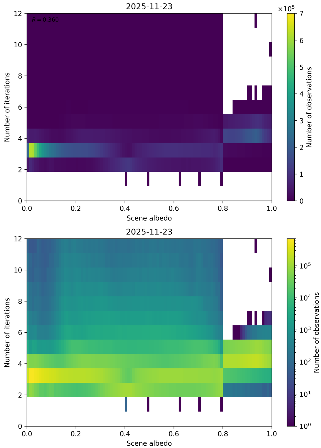
Figure 105: Scatter density plot of “Scene albedo” against “Number of iterations” for 2025-11-23 to 2025-11-24.
