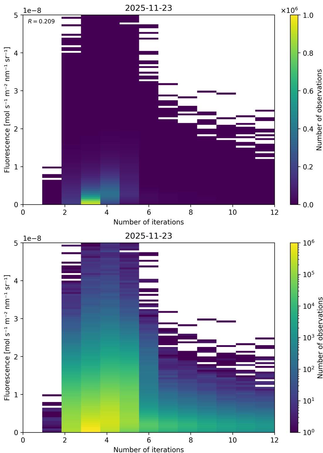
Figure 98: Scatter density plot of “Number of iterations” against “Fluorescence” for 2025-11-23 to 2025-11-24.
