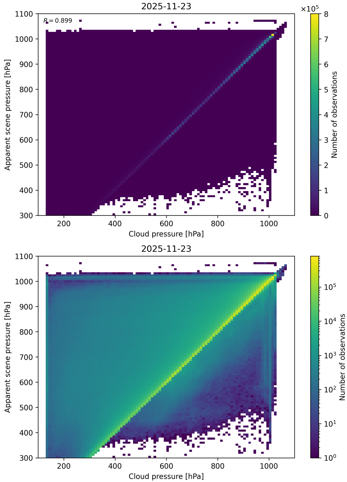
Figure 77: Scatter density plot of “Cloud pressure” against “Apparent scene pressure” for 2025-11-23 to 2025-11-24.
