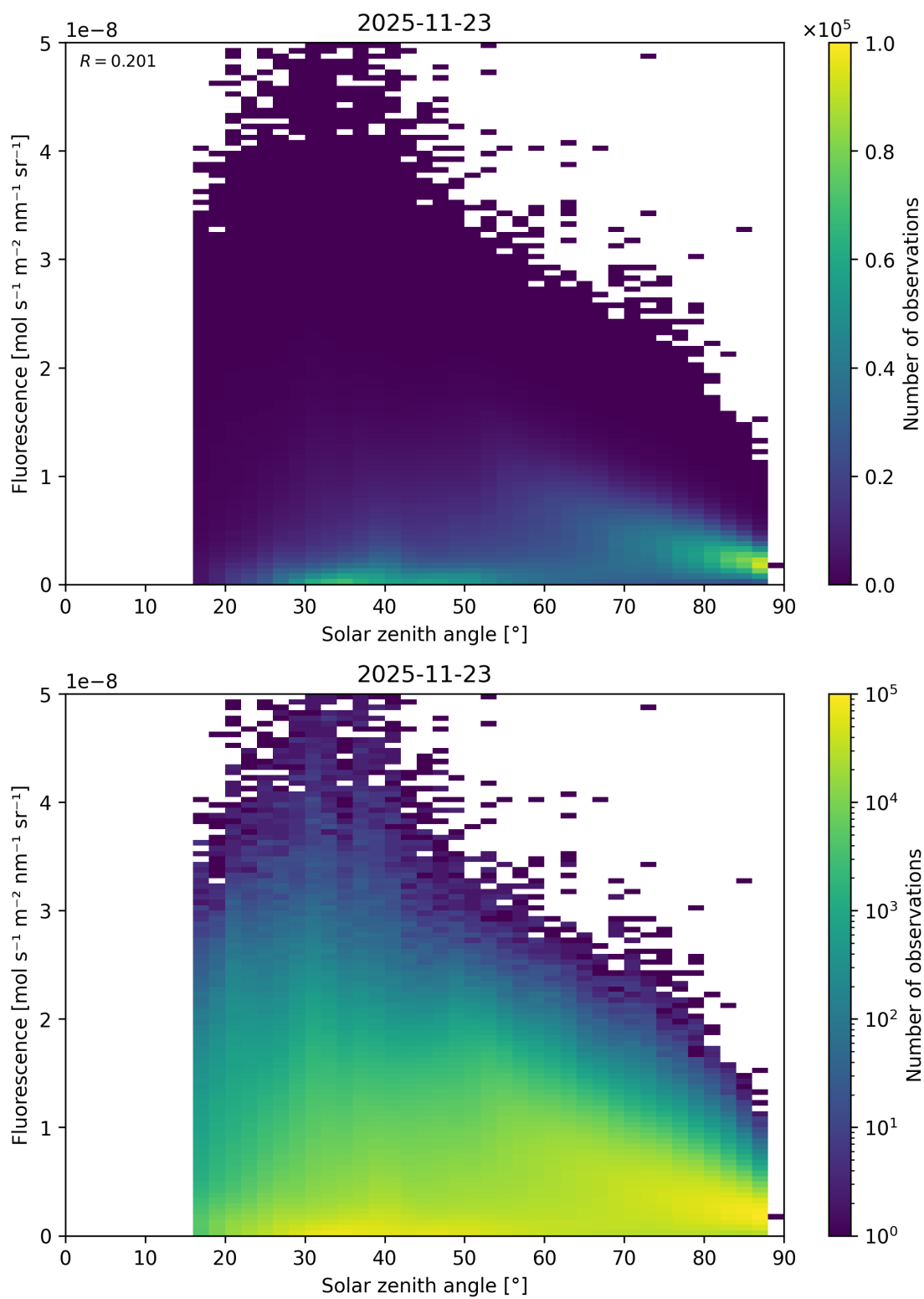
Figure 112: Scatter density plot of “Solar zenith angle” against “Fluorescence” for 2025-11-23 to 2025-11-24.
