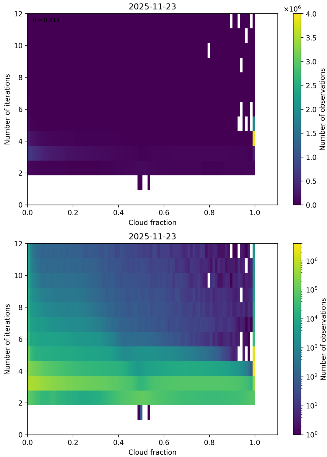
Figure 73: Scatter density plot of “Cloud fraction” against “Number of iterations” for 2025-11-23 to 2025-11-24.
