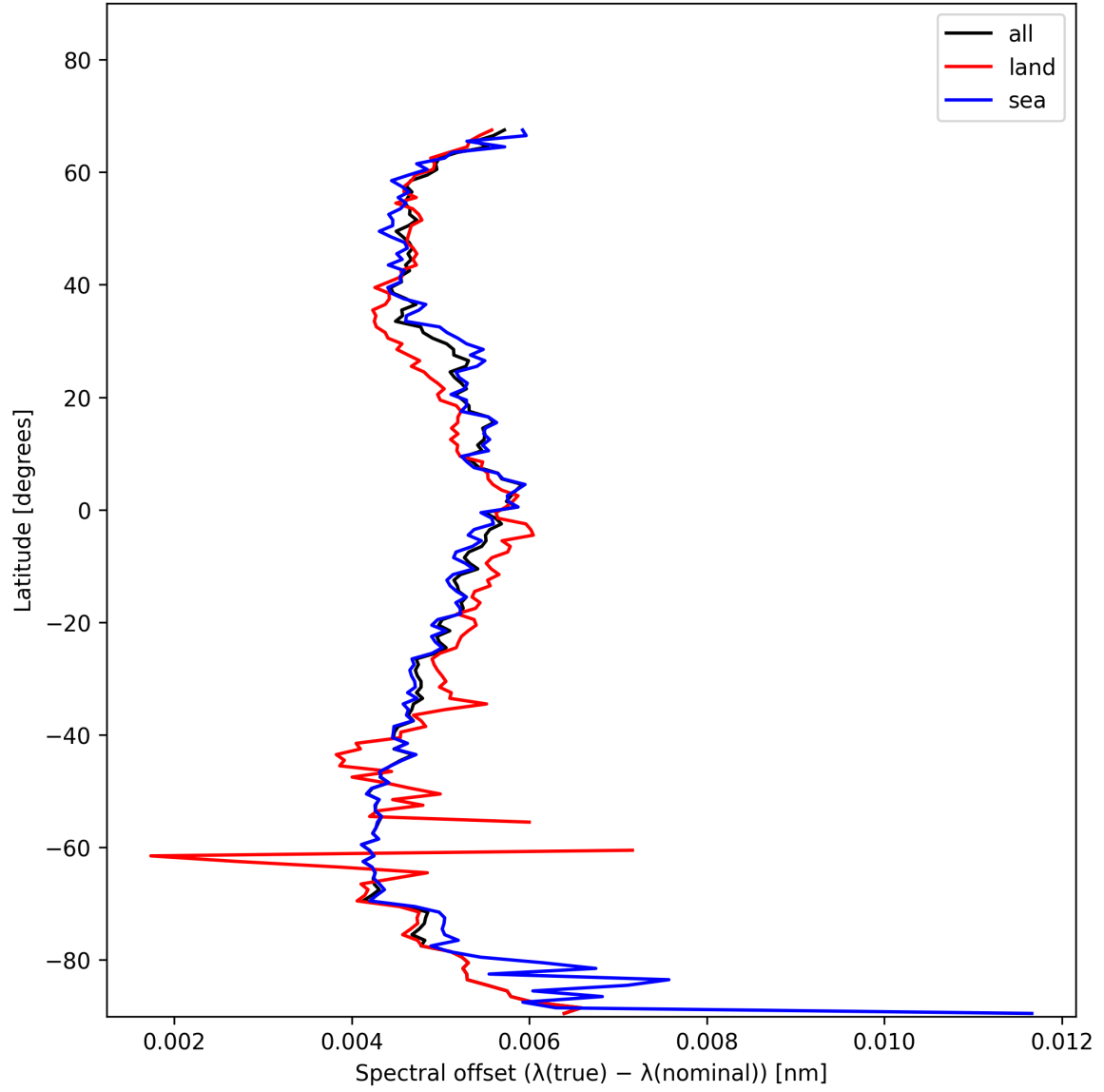
Figure 28: Zonal average of “Spectral offset ( \lambda_{\text{true}} - \lambda_{\text{nominal}} )” for 2025-11-23 to 2025-11-24.
