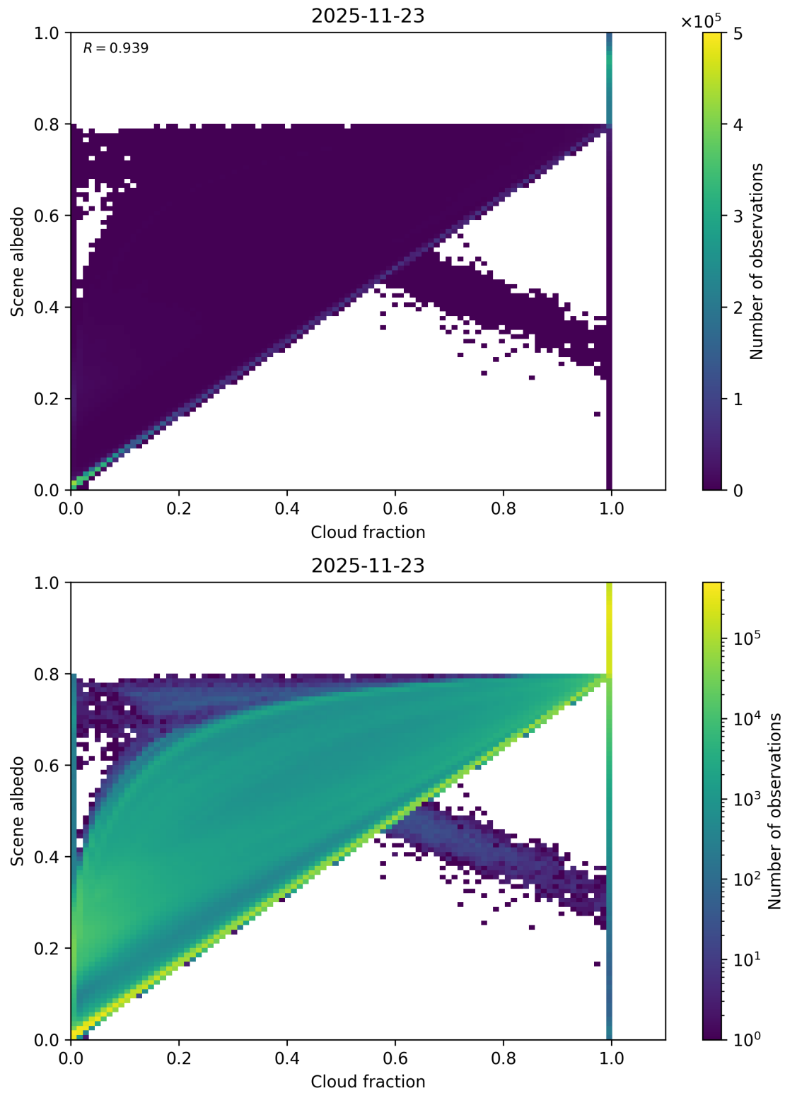
Figure 75: Scatter density plot of “Cloud fraction” against “Scene albedo” for 2025-11-23 to 2025-11-24.
