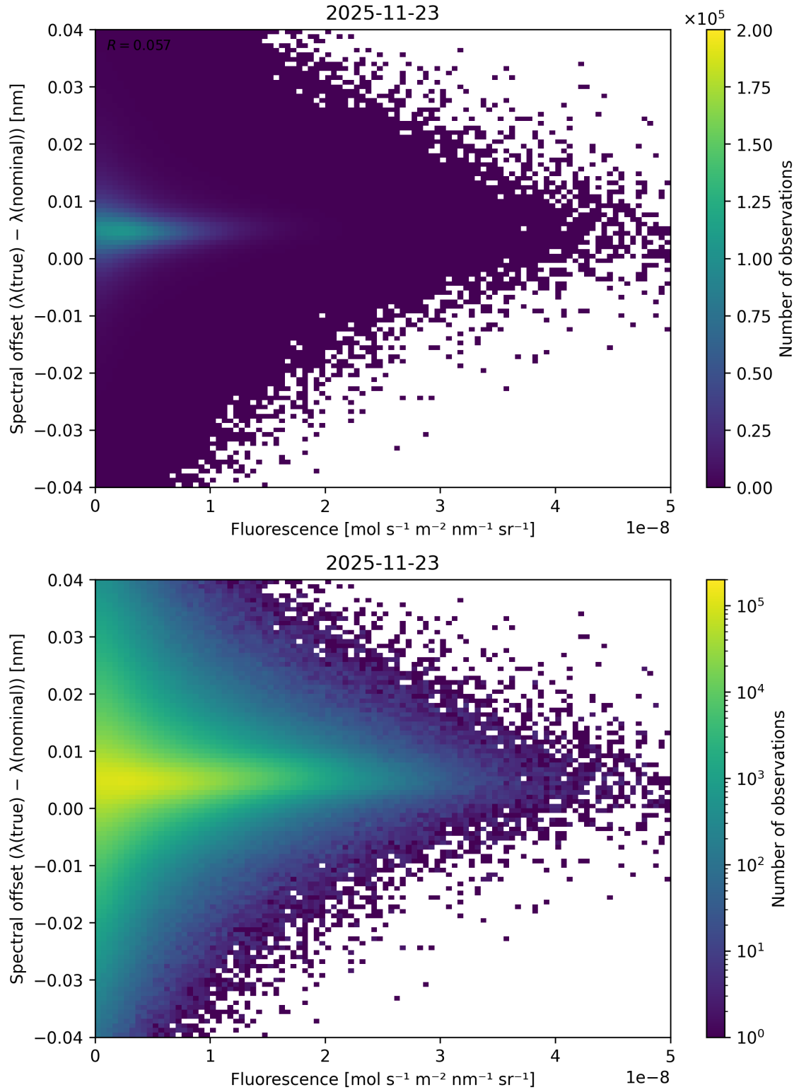
Figure 87: Scatter density plot of “Fluorescence” against “Spectral offset ( \lambda_{\text{true}} - \lambda_{\text{nominal}} )” for 2025-11-23 to 2025-11-24.
