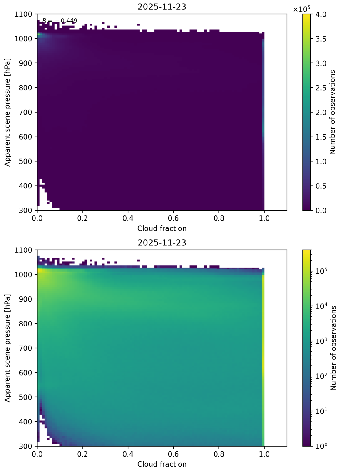
Figure 70: Scatter density plot of “Cloud fraction” against “Apparent scene pressure” for 2025-11-23 to 2025-11-24.
