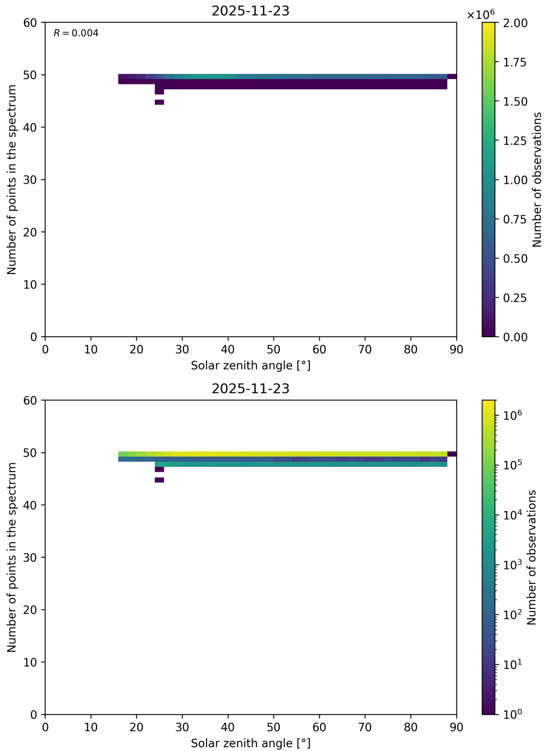
Figure 115: Scatter density plot of “Solar zenith angle” against “Number of points in the spectrum” for 2025-11-23 to 2025-11-24.
