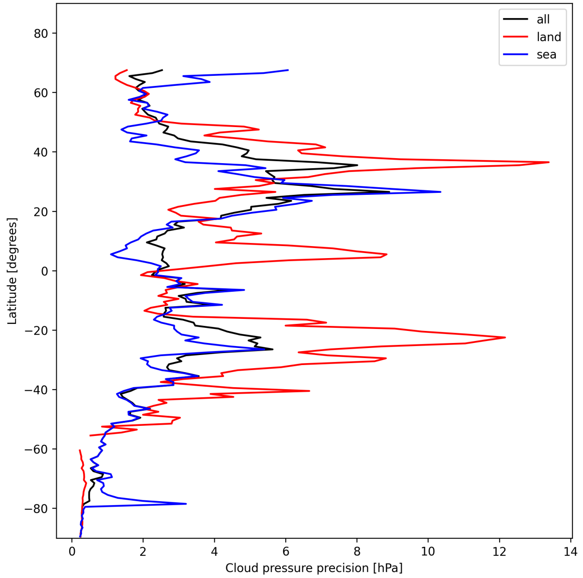
Figure 14: Zonal average of “Cloud pressure precision” for 2025-11-23 to 2025-11-24.
