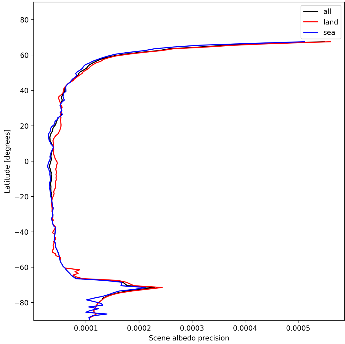
Figure 18: Zonal average of “Scene albedo precision” for 2025-11-23 to 2025-11-24.
