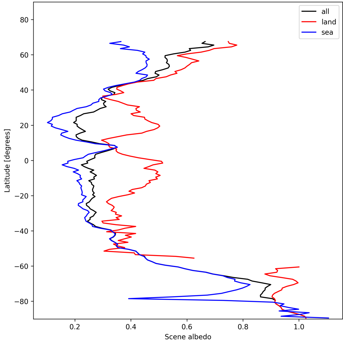
Figure 17: Zonal average of “Scene albedo” for 2025-11-23 to 2025-11-24.
