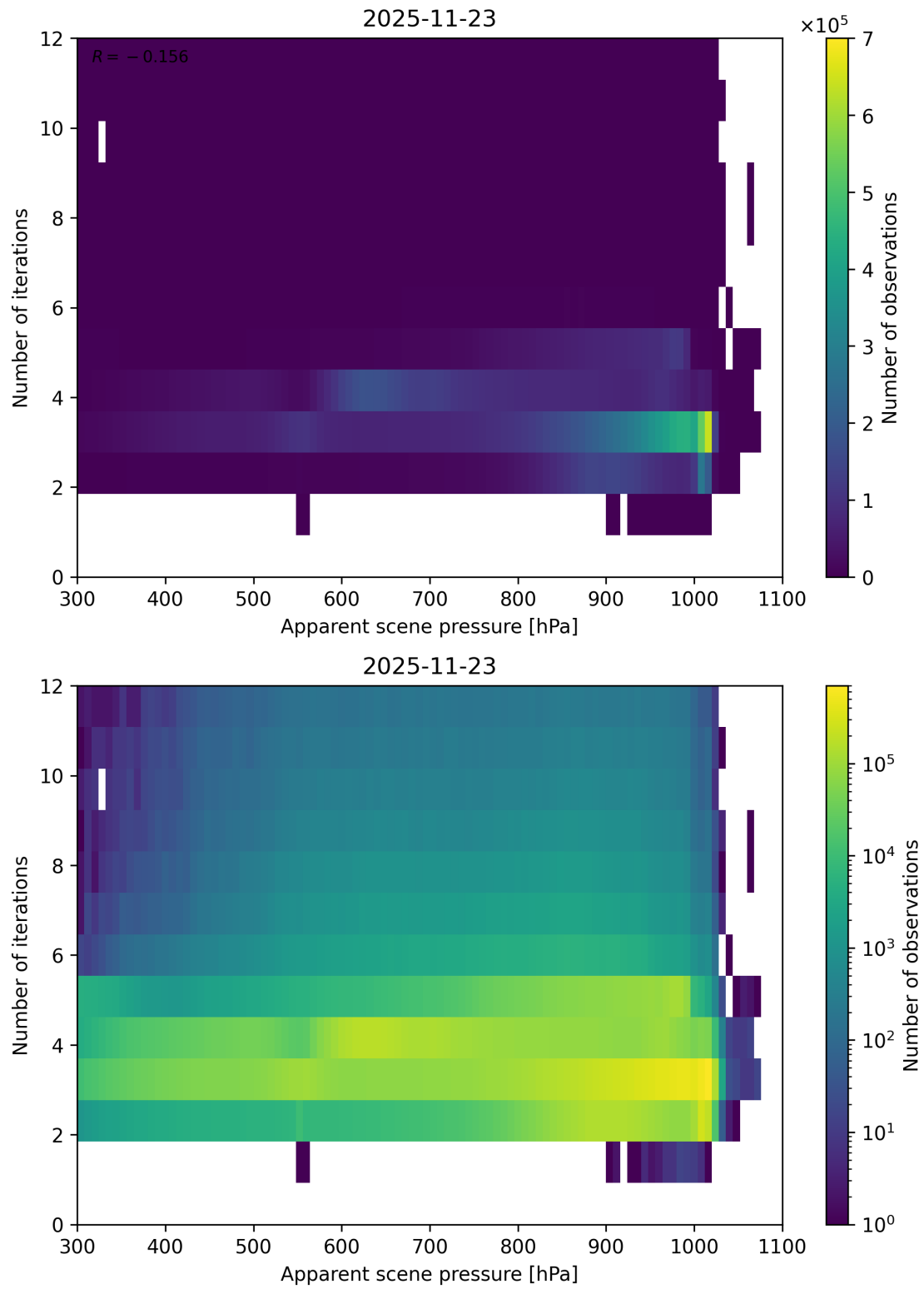
Figure 65: Scatter density plot of “Apparent scene pressure” against “Number of iterations” for 2025-11-23 to 2025-11-24.
