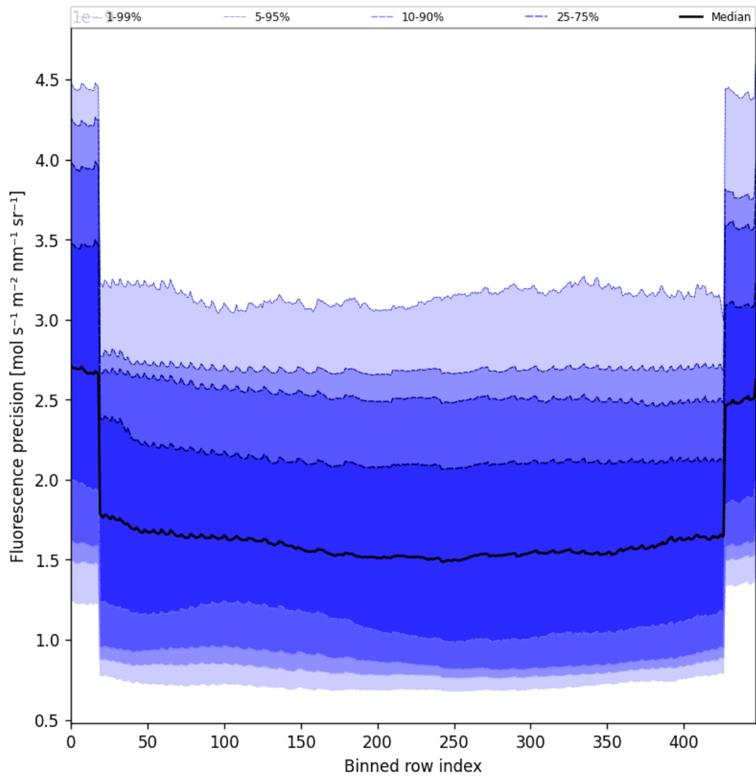
Figure 58: Along track statistics of “Fluorescence precision” for 2025-11-23 to 2025-11-24
