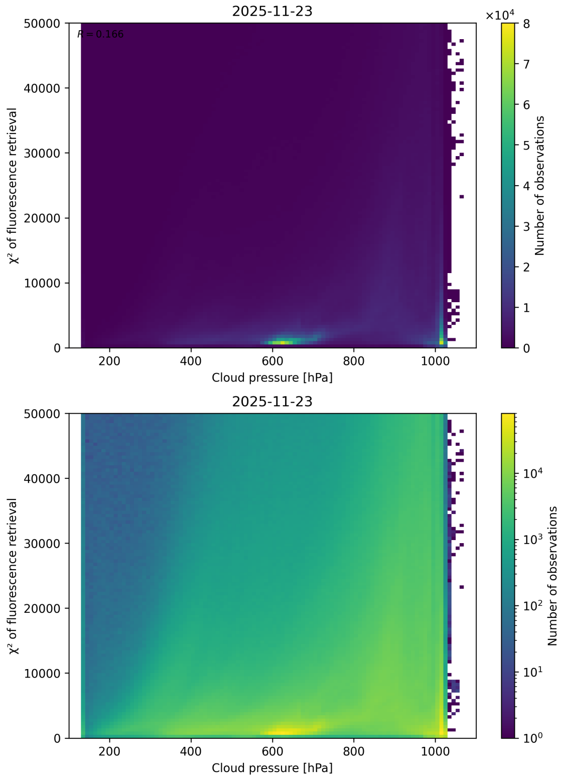
Figure 78: Scatter density plot of “Cloud pressure” against “ \chi^2 of fluorescence retrieval” for 2025-11-23 to 2025-11-24.
