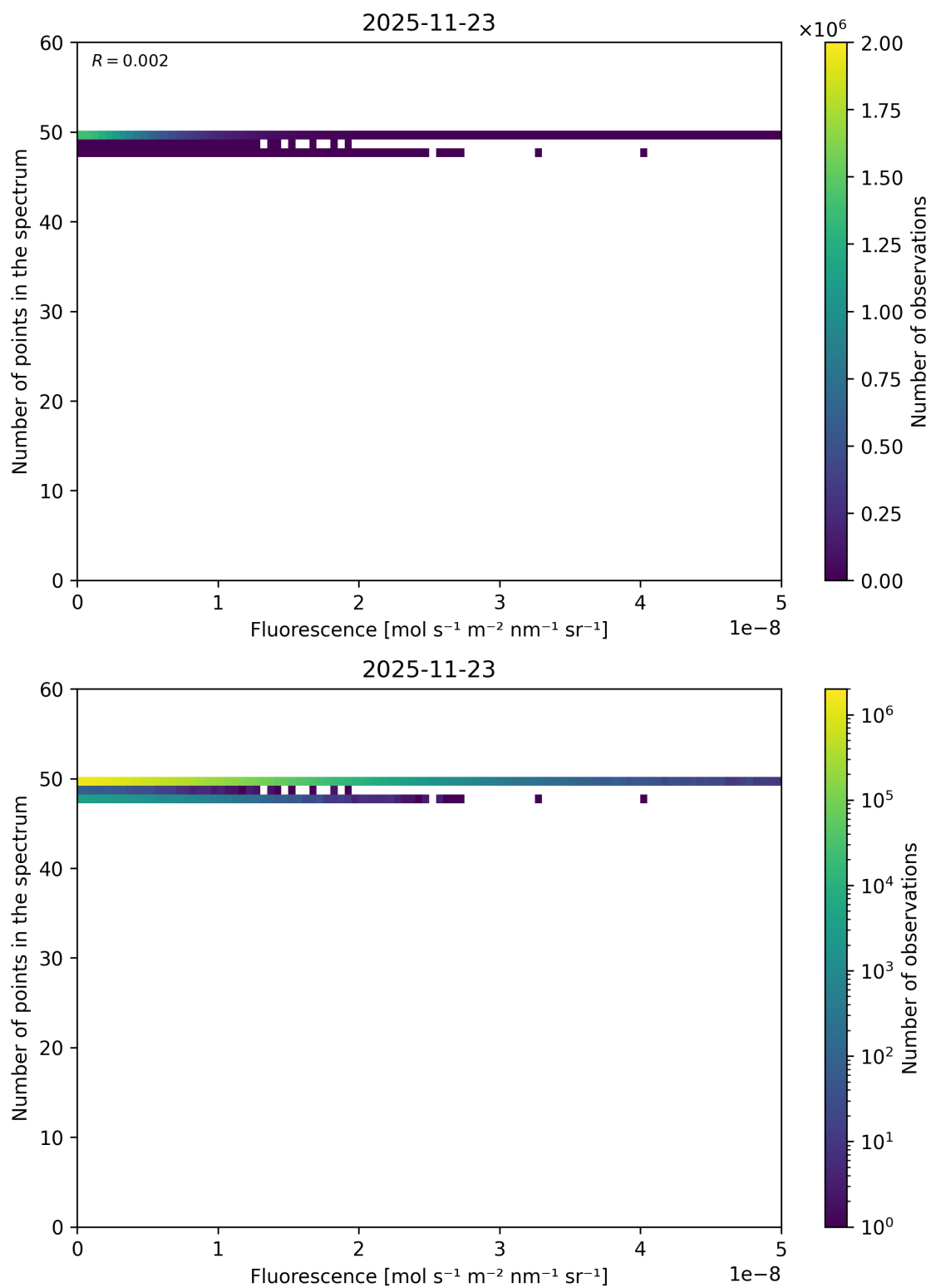
Figure 86: Scatter density plot of “Fluorescence” against “Number of points in the spectrum” for 2025-11-23 to 2025-11-24.
