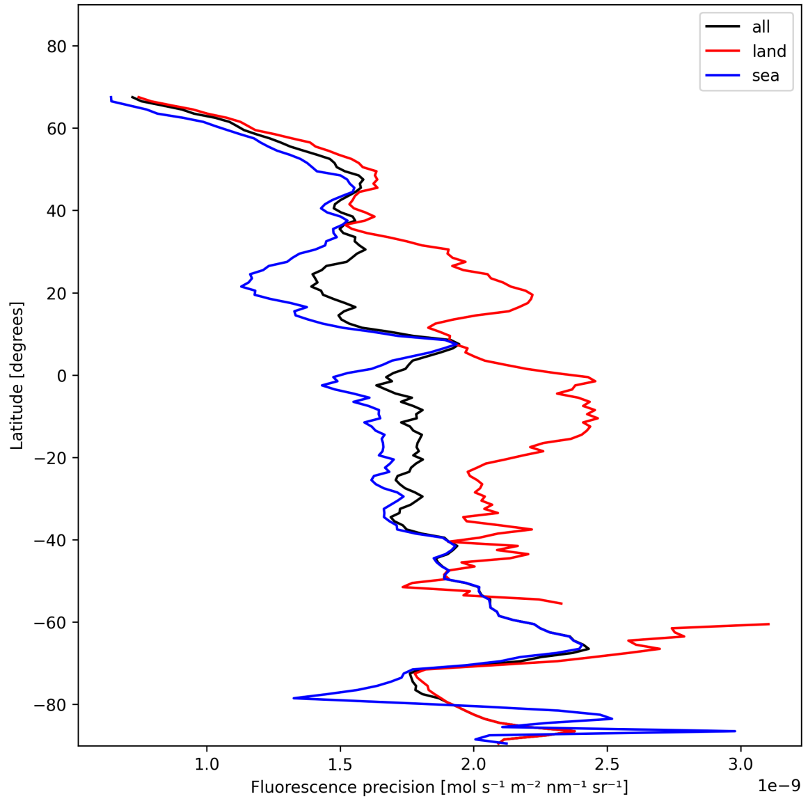
Figure 24: Zonal average of “Fluorescence precision” for 2025-11-23 to 2025-11-24.
