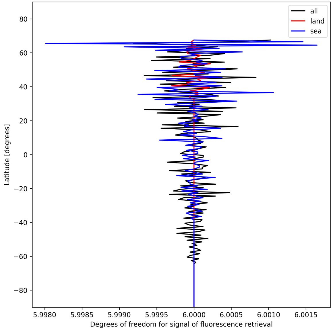
Figure 26: Zonal average of “Degrees of freedom for signal of fluorescence retrieval” for 2025-11-23 to 2025-11-24.
