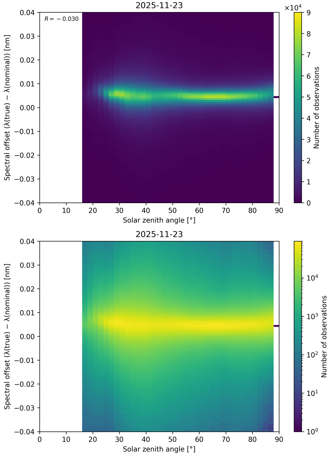
Figure 117: Scatter density plot of “Solar zenith angle” against “Spectral offset ( \lambda_{\text{true}} - \lambda_{\text{nominal}} )” for 2025-11-23 to 2025-11-24.
