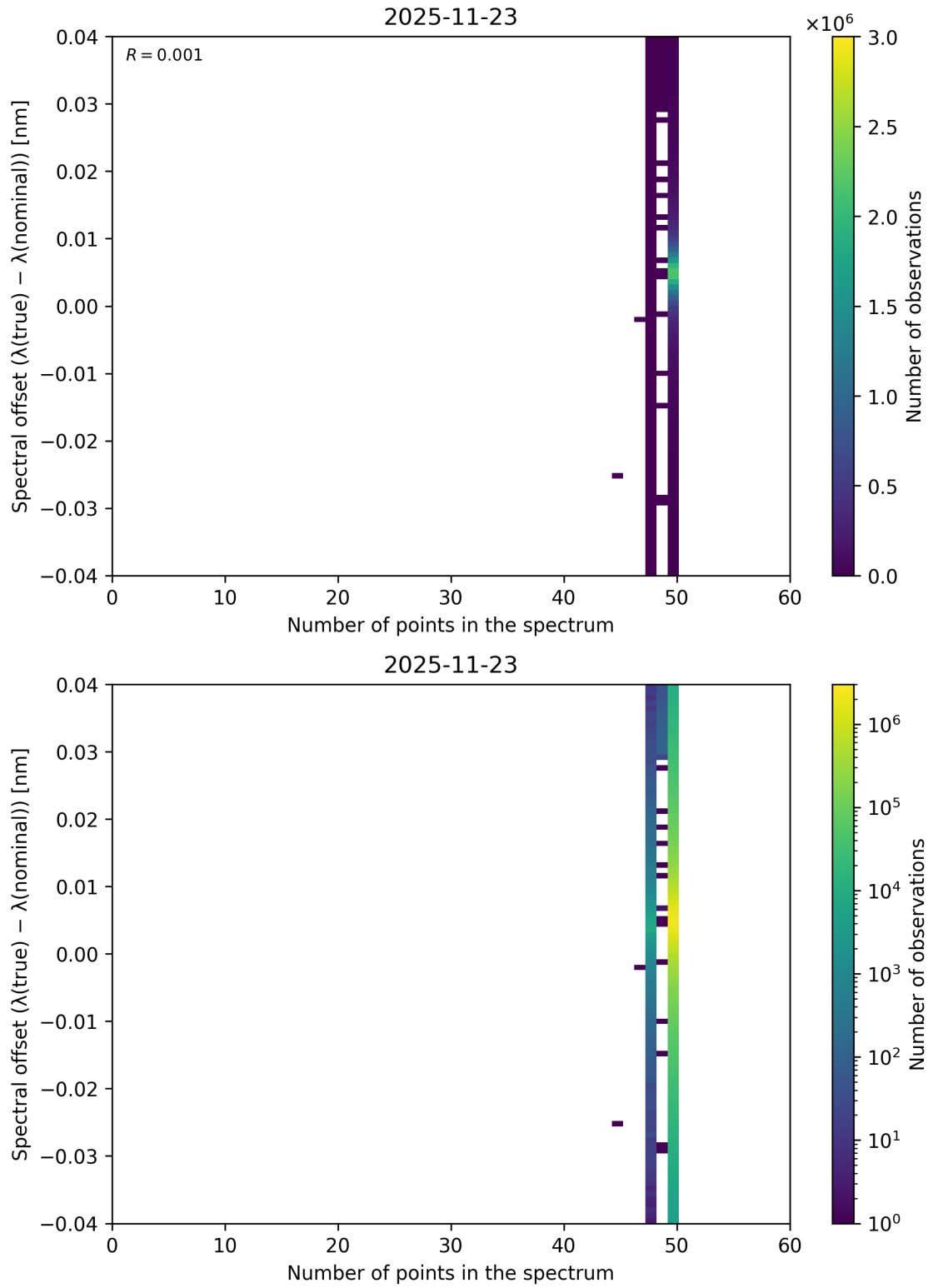
Figure 101: Scatter density plot of “Number of points in the spectrum” against “Spectral offset ( \lambda_{\text{true}} - \lambda_{\text{nominal}} )” for 2025-11-23 to 2025-11-24.
