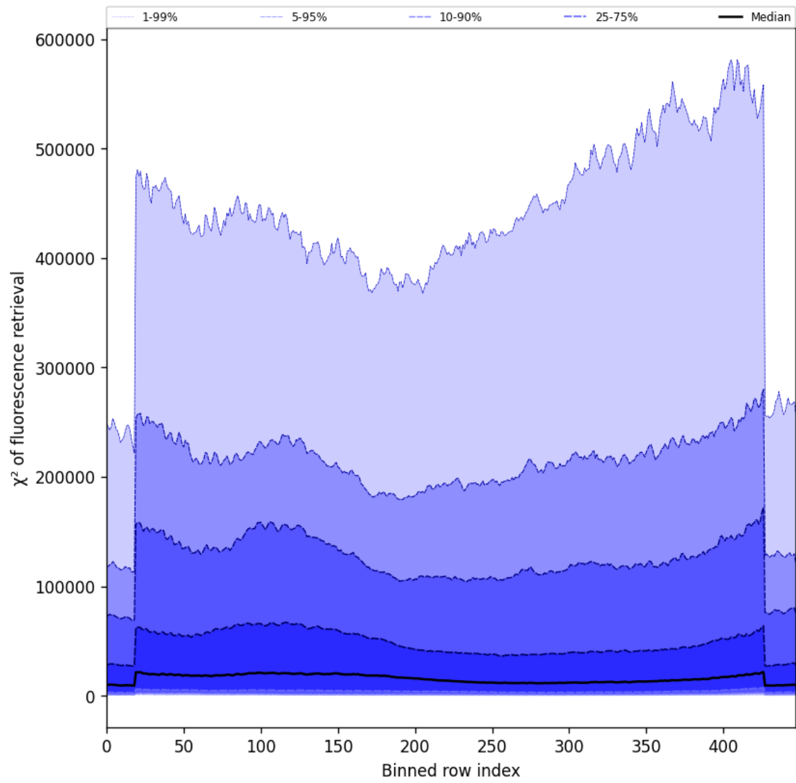
Figure 59: Along track statistics of “ \chi^2 of fluorescence retrieval” for 2025-11-23 to 2025-11-24
