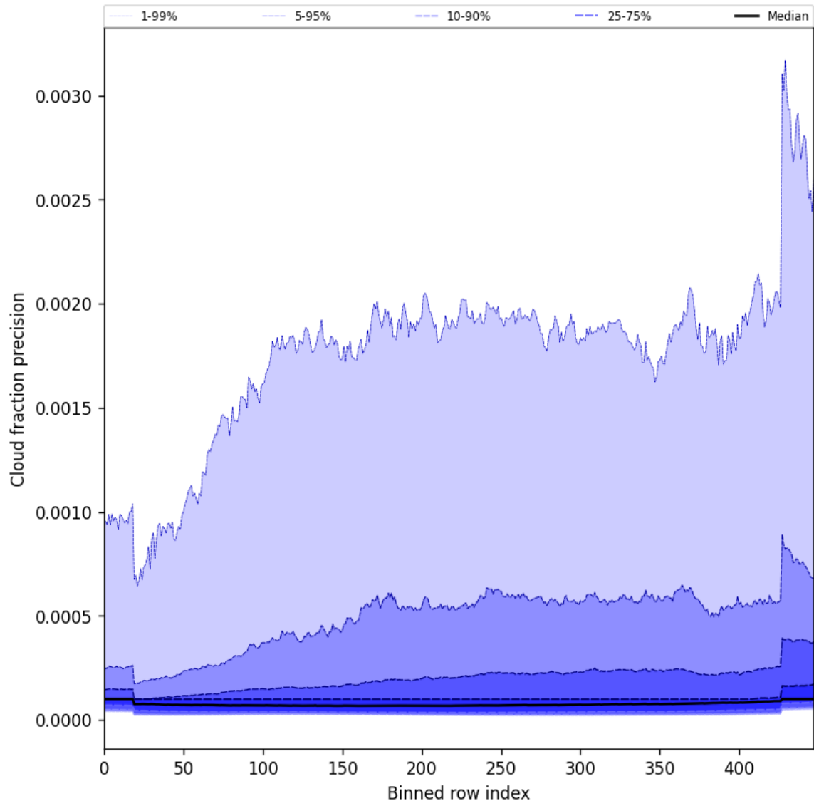
Figure 50: Along track statistics of “Cloud fraction precision” for 2025-11-23 to 2025-11-24
