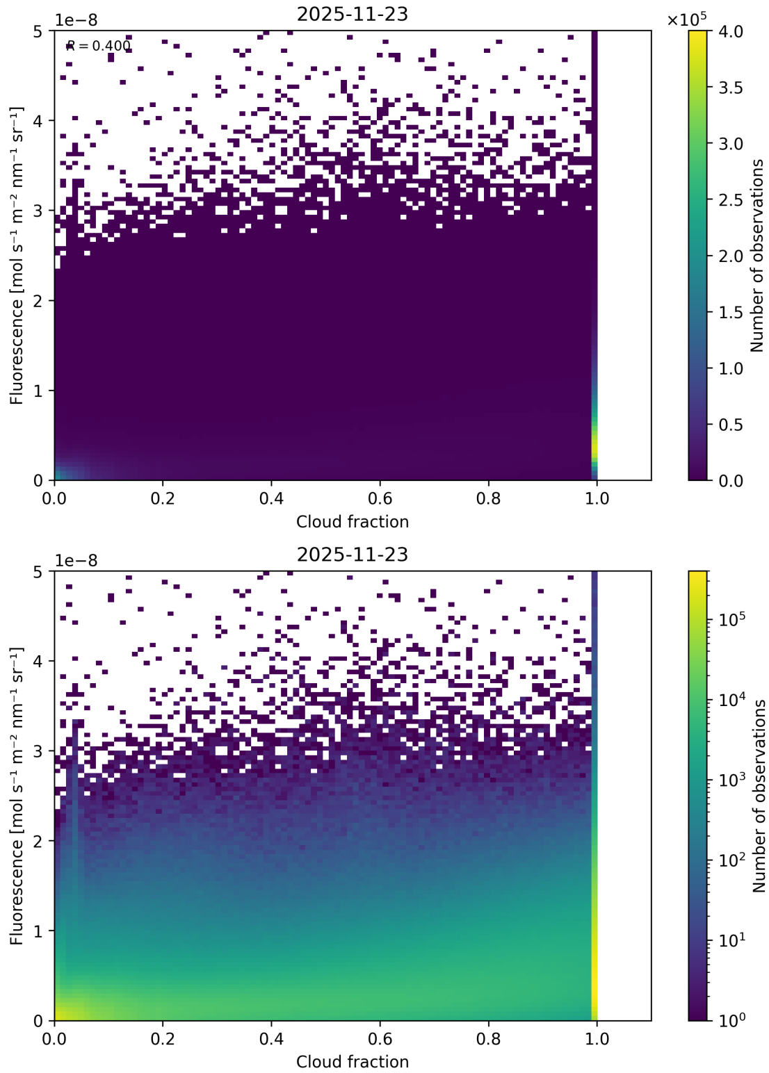
Figure 72: Scatter density plot of “Cloud fraction” against “Fluorescence” for 2025-11-23 to 2025-11-24.
