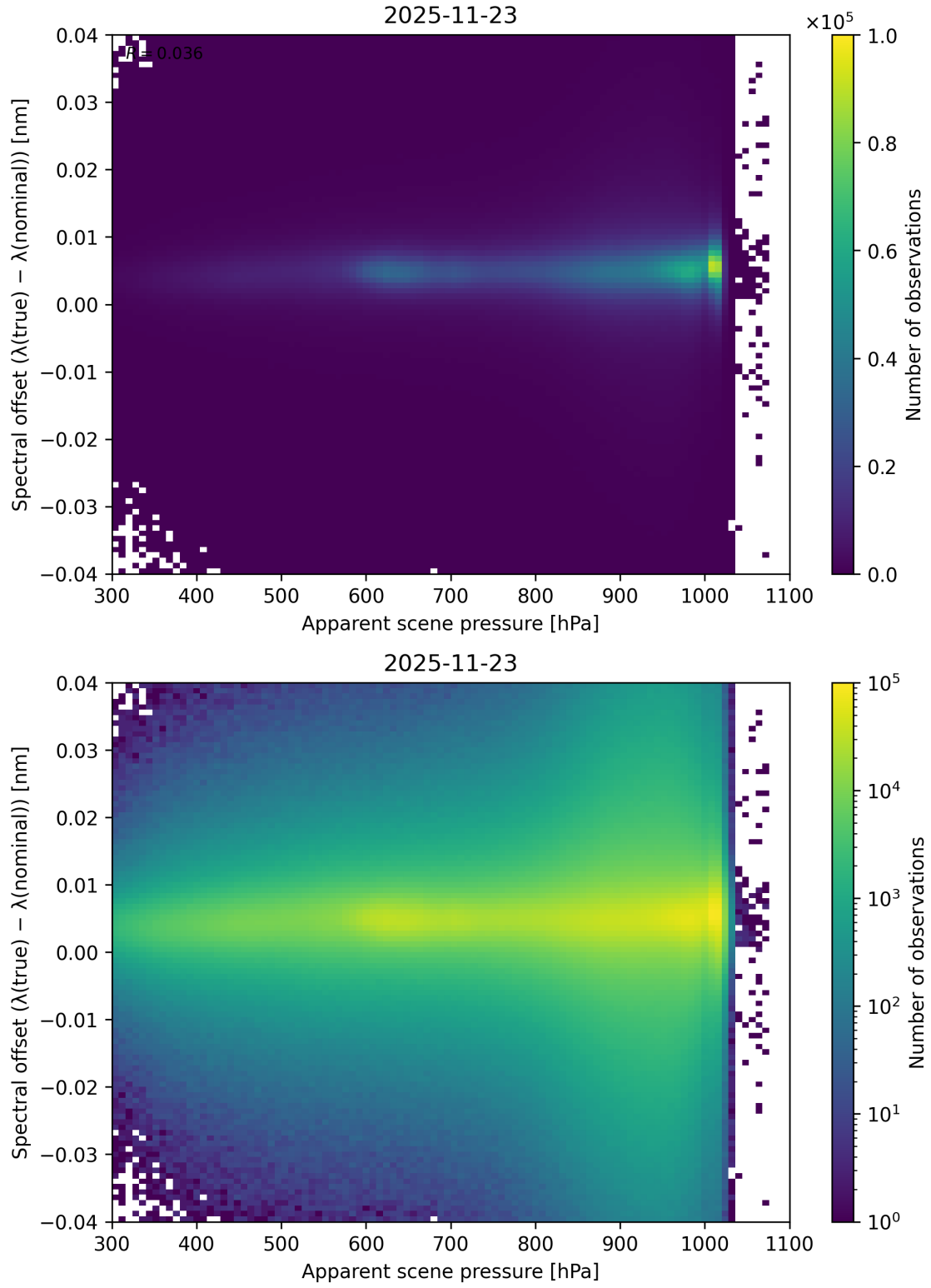
Figure 67: Scatter density plot of “Apparent scene pressure” against “Spectral offset ( \lambda_{\text{true}} - \lambda_{\text{nominal}} )” for 2025-11-23 to 2025-11-24.
