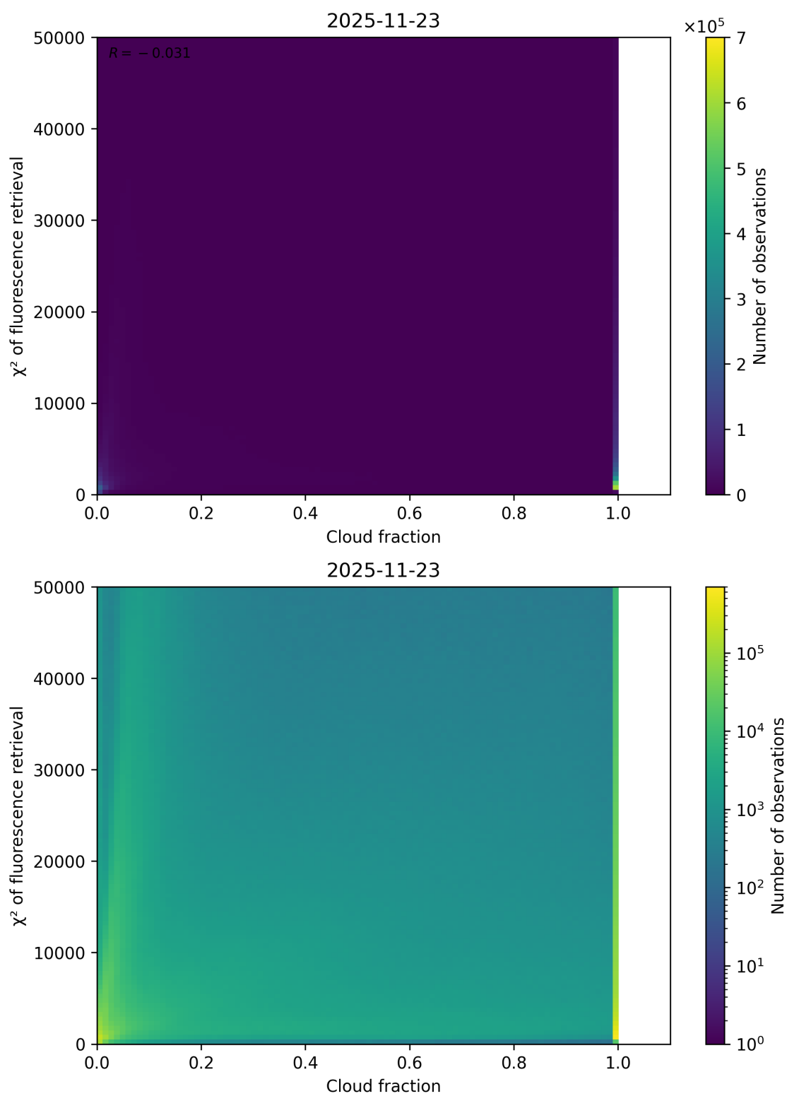
Figure 71: Scatter density plot of “Cloud fraction” against “ \chi^2 of fluorescence retrieval” for 2025-11-23 to 2025-11-24.
