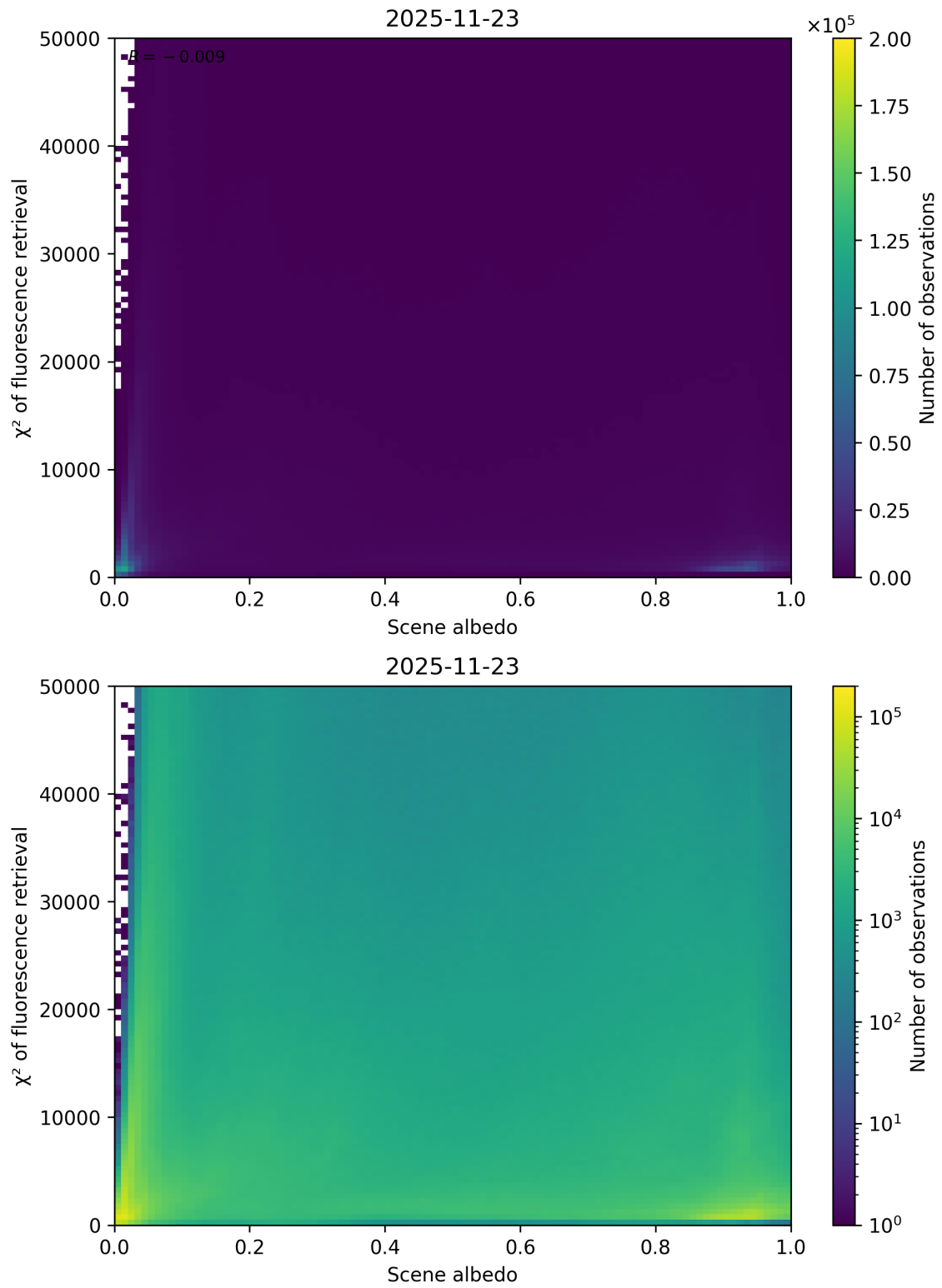
Figure 103: Scatter density plot of “Scene albedo” against “ \chi^2 of fluorescence retrieval” for 2025-11-23 to 2025-11-24.
