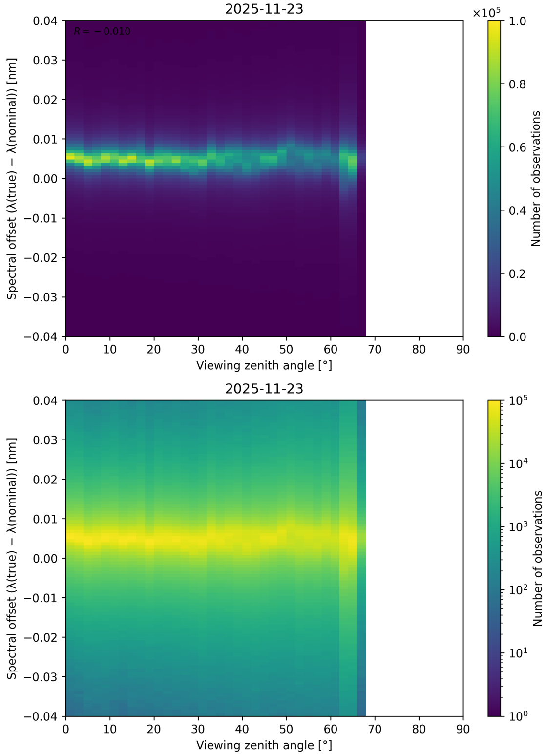
Figure 128: Scatter density plot of “Viewing zenith angle” against “Spectral offset ( \lambda_{\text{true}} - \lambda_{\text{nominal}} )” for 2025-11-23 to 2025-11-24.
