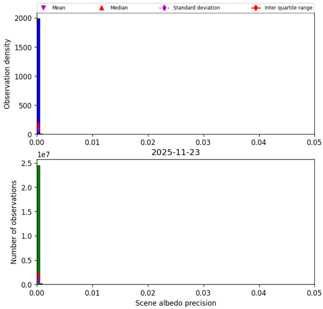
Figure 35: Histogram of “Scene albedo precision” for 2025-11-23 to 2025-11-24
