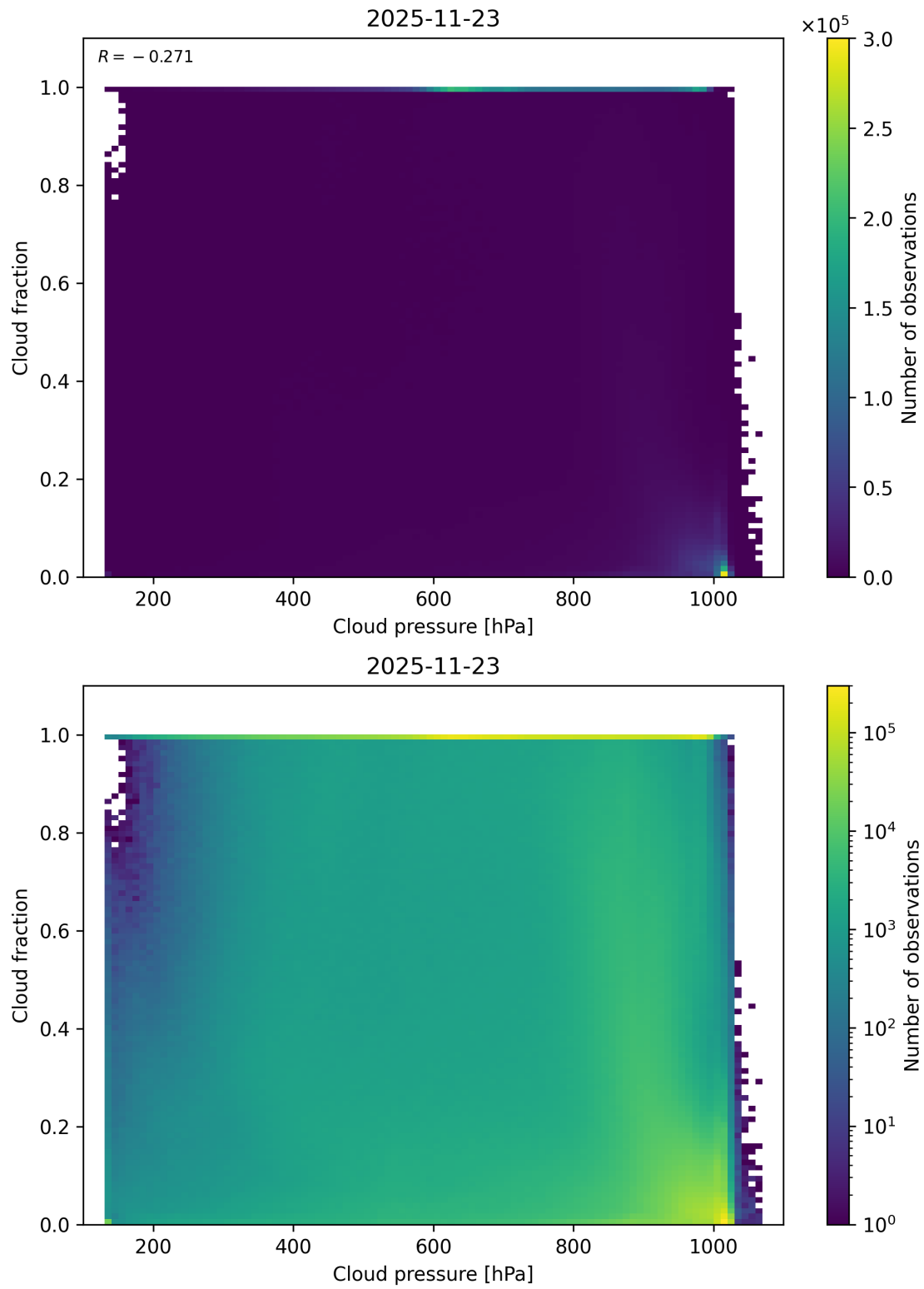
Figure 79: Scatter density plot of “Cloud pressure” against “Cloud fraction” for 2025-11-23 to 2025-11-24.
