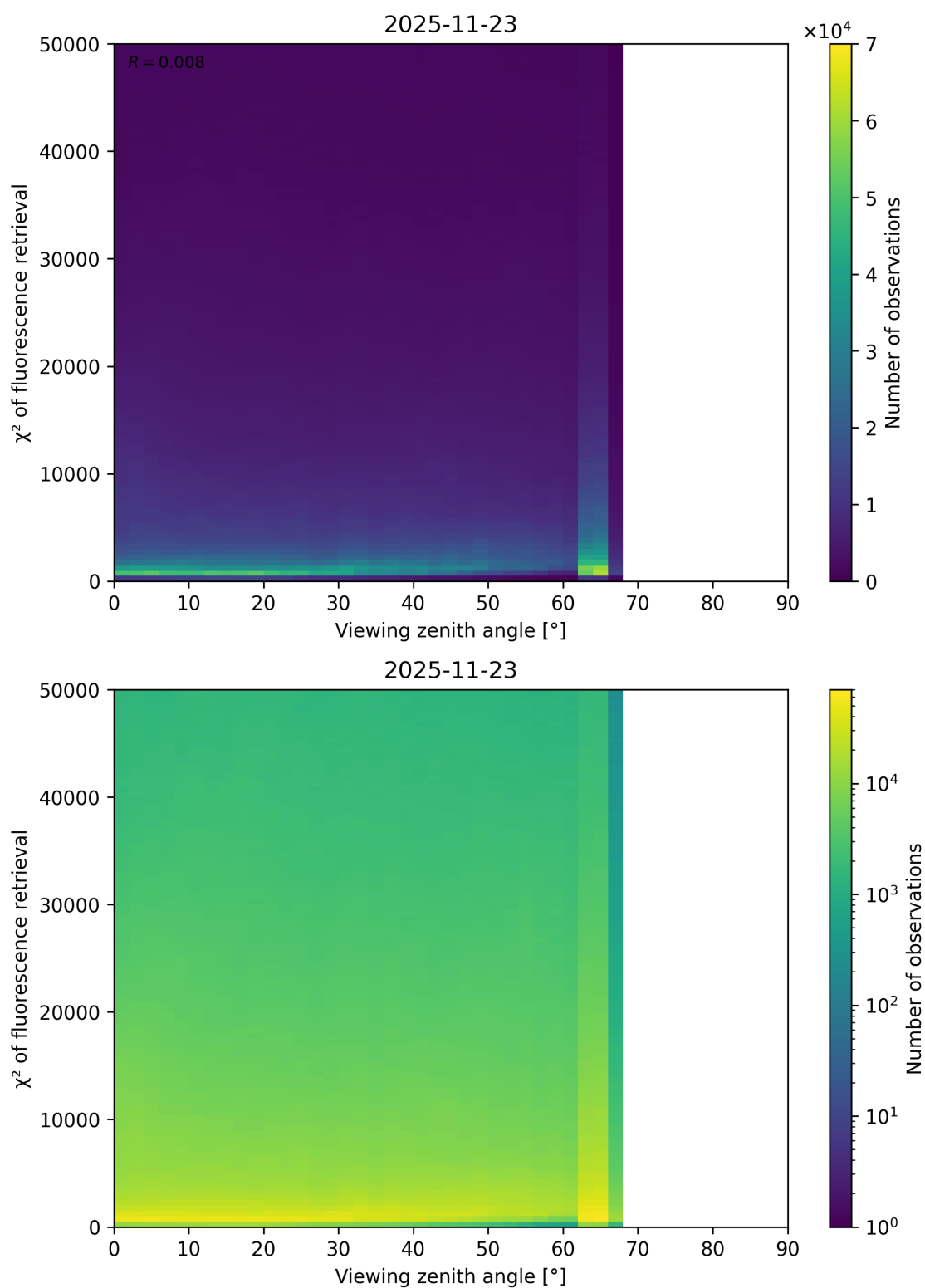
Figure 119: Scatter density plot of “Viewing zenith angle” against “ \chi^2 of fluorescence retrieval” for 2025-11-23 to 2025-11-24.
