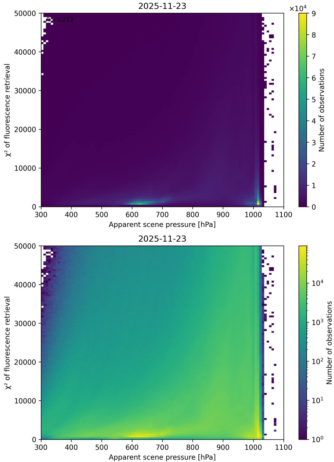
Figure 63: Scatter density plot of “Apparent scene pressure” against “ \chi^2 of fluorescence retrieval” for 2025-11-23 to 2025-11-24.
