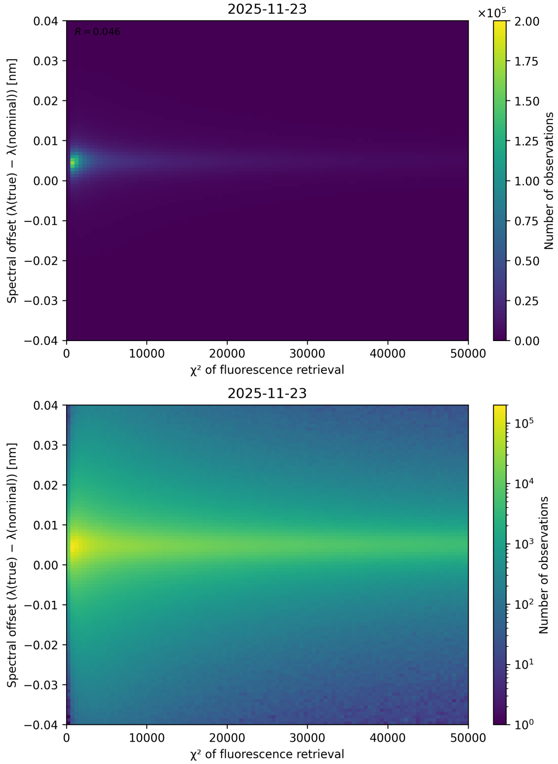
Figure 69: Scatter density plot of “ \chi^2 of fluorescence retrieval” against “Spectral offset ( \lambda_{\text{true}} - \lambda_{\text{nominal}} )” for 2025-11-23 to 2025-11-24.
