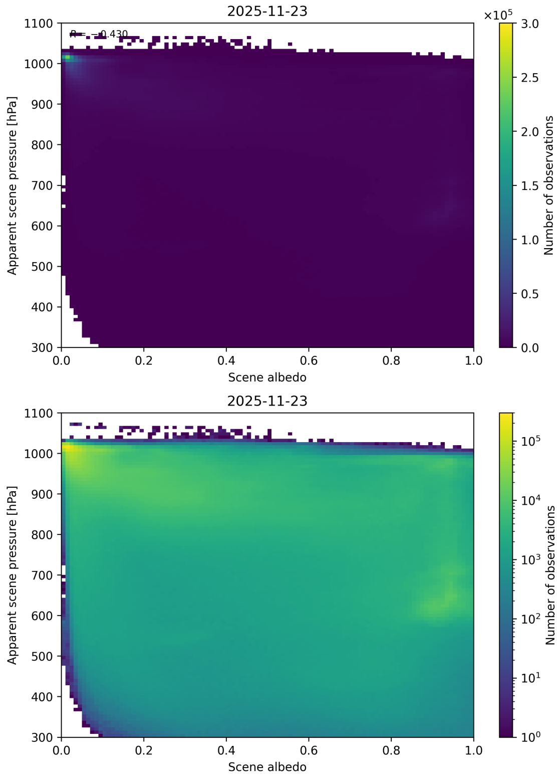
Figure 102: Scatter density plot of “Scene albedo” against “Apparent scene pressure” for 2025-11-23 to 2025-11-24.
