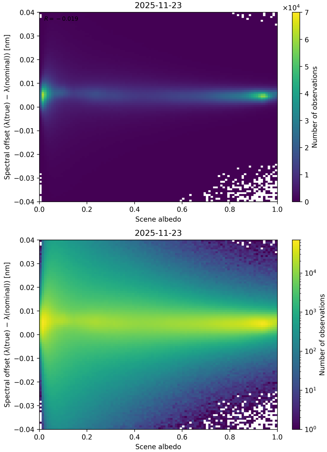
Figure 107: Scatter density plot of “Scene albedo” against “Spectral offset ( \lambda_{\text{true}} - \lambda_{\text{nominal}} )” for 2025-11-23 to 2025-11-24.
