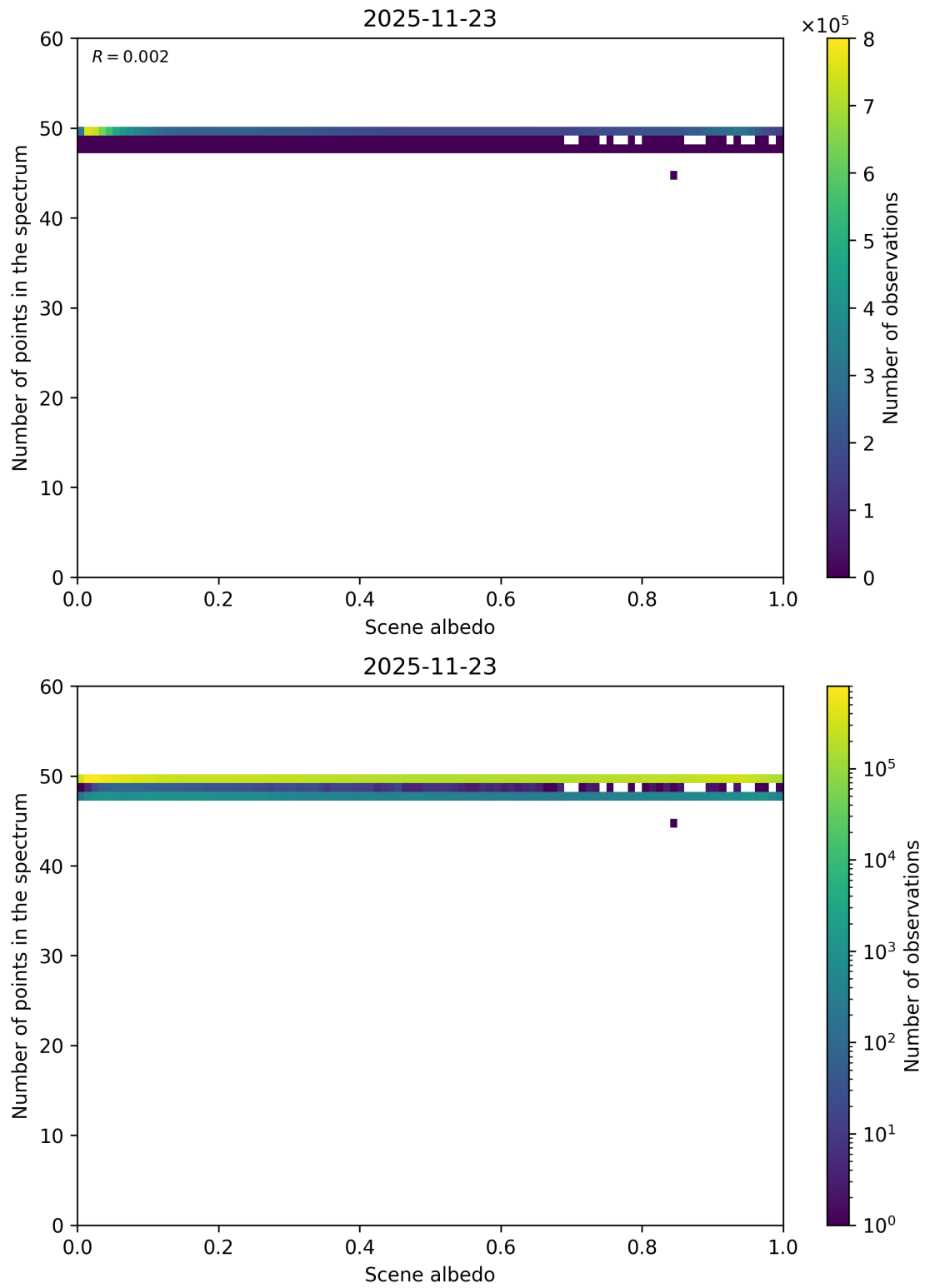
Figure 106: Scatter density plot of “Scene albedo” against “Number of points in the spectrum” for 2025-11-23 to 2025-11-24.
