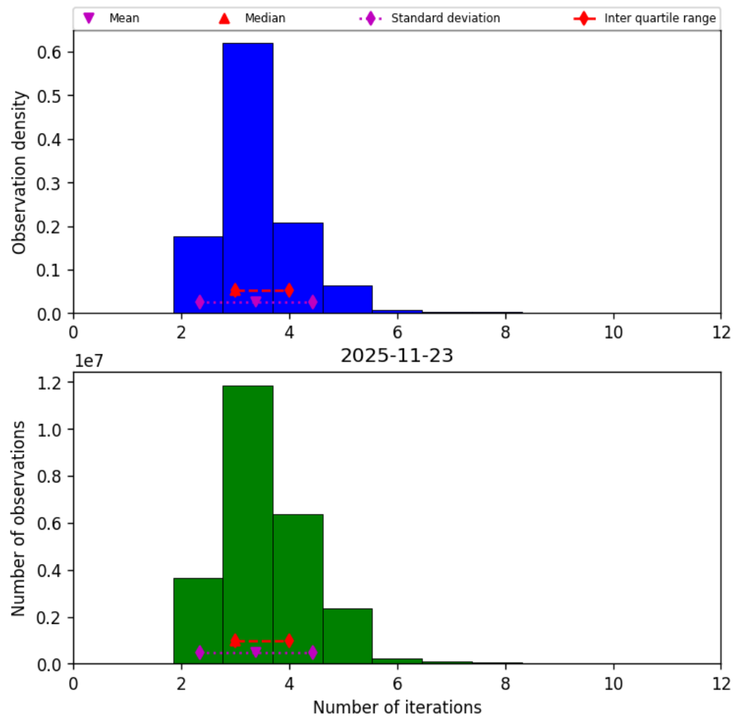
Figure 39: Histogram of “Number of iterations” for 2025-11-23 to 2025-11-24
