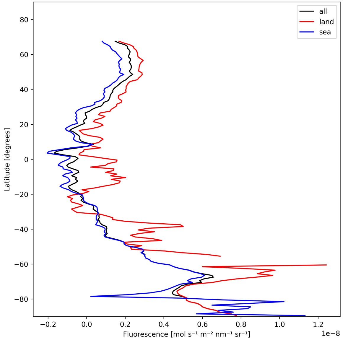
Figure 23: Zonal average of “Fluorescence” for 2025-11-23 to 2025-11-24.
