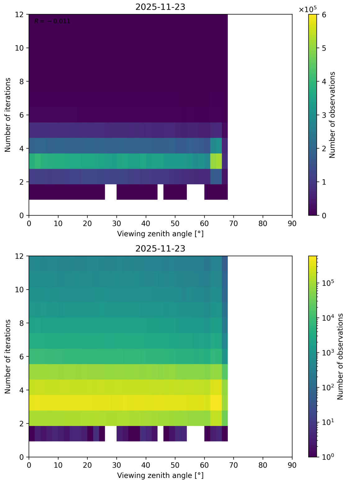
Figure 124: Scatter density plot of “Viewing zenith angle” against “Number of iterations” for 2025-11-23 to 2025-11-24.
