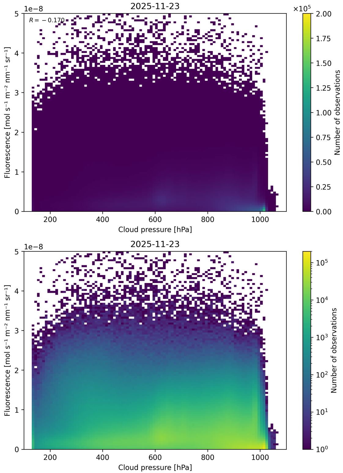
Figure 80: Scatter density plot of “Cloud pressure” against “Fluorescence” for 2025-11-23 to 2025-11-24.
