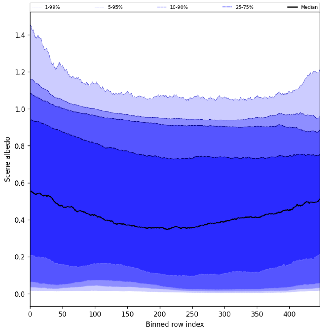
Figure 51: Along track statistics of “Scene albedo” for 2025-11-23 to 2025-11-24
