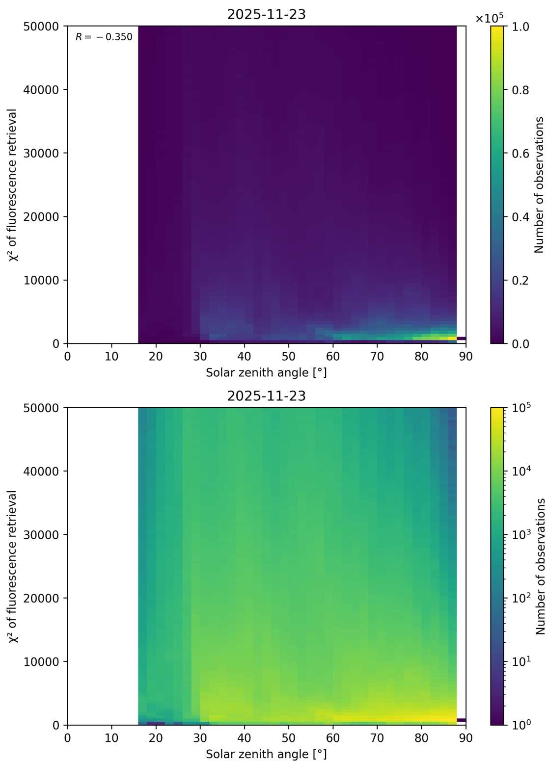
Figure 109: Scatter density plot of “Solar zenith angle” against “ \chi^2 of fluorescence retrieval” for 2025-11-23 to 2025-11-24.
