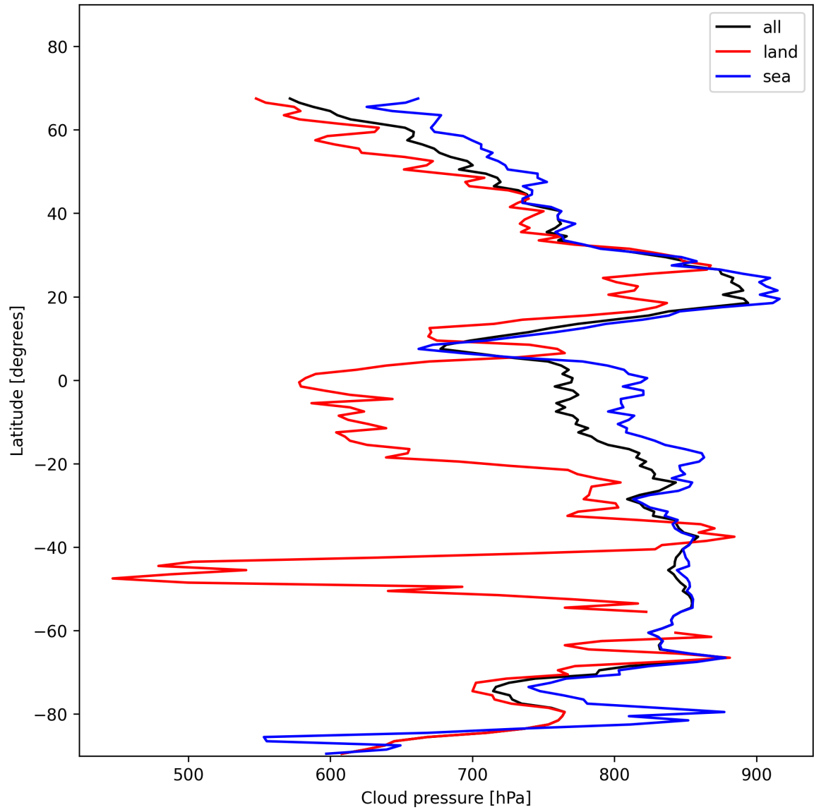
Figure 13: Zonal average of “Cloud pressure” for 2025-11-23 to 2025-11-24.
