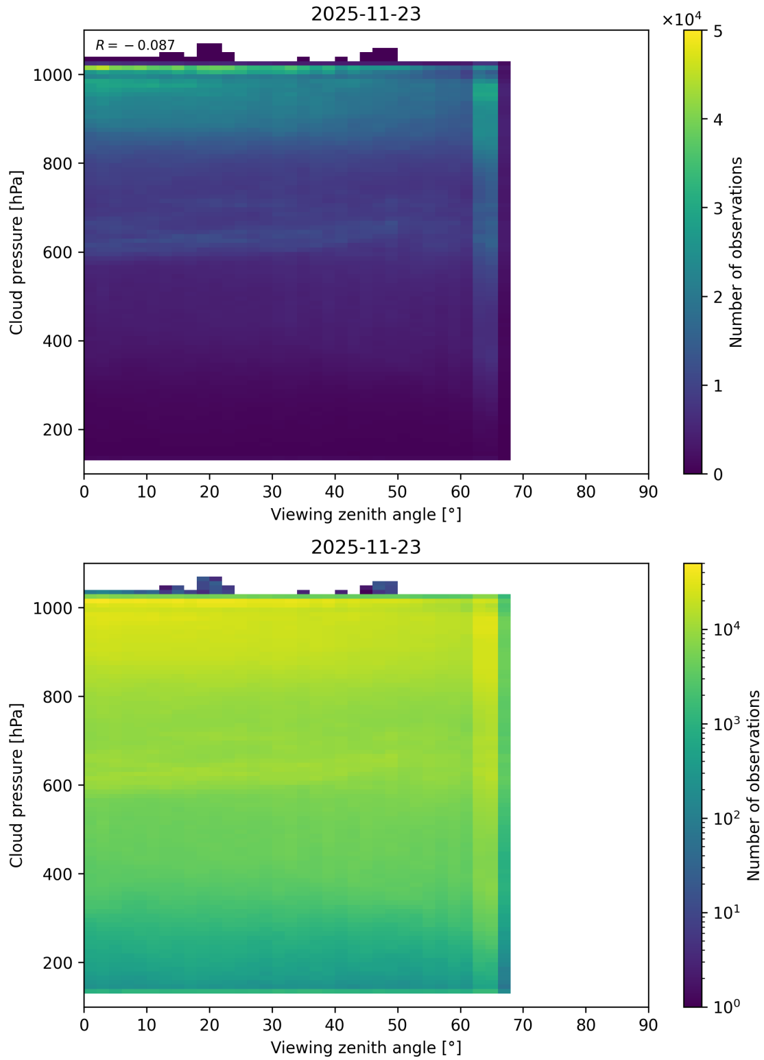
Figure 121: Scatter density plot of “Viewing zenith angle” against “Cloud pressure” for 2025-11-23 to 2025-11-24.
