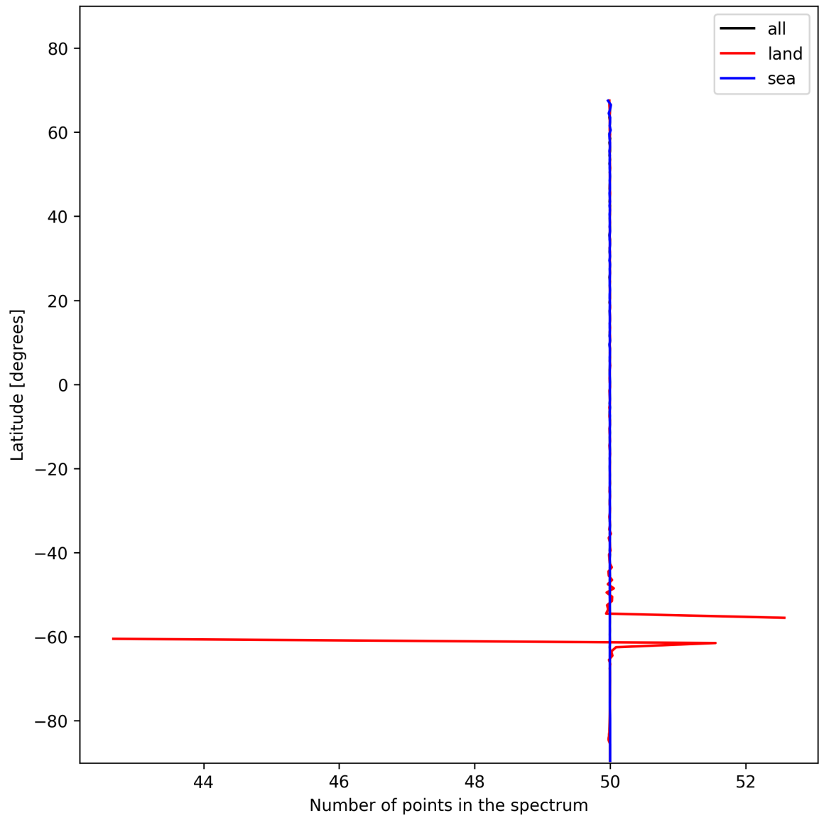
Figure 27: Zonal average of “Number of points in the spectrum” for 2025-11-23 to 2025-11-24.
