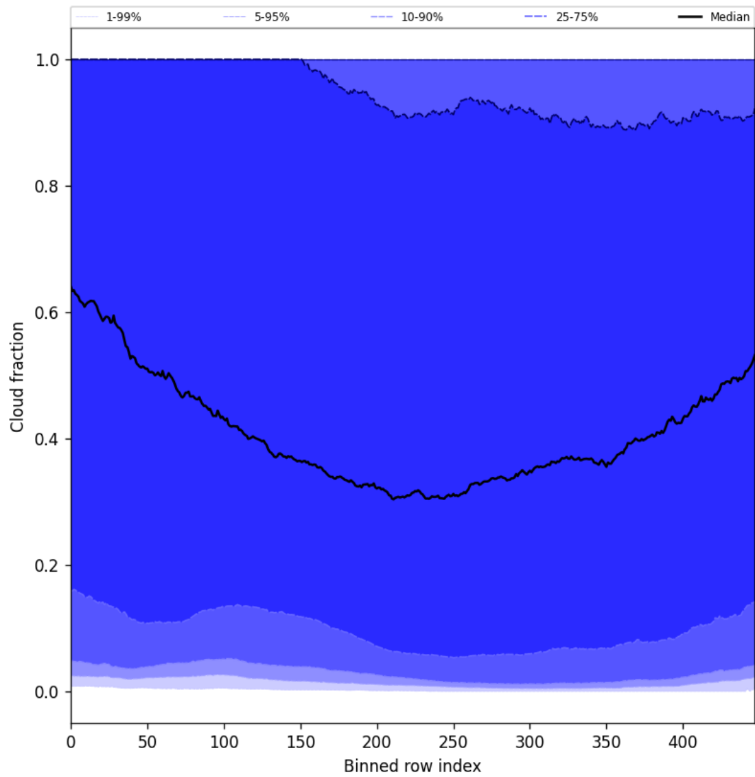
Figure 49: Along track statistics of “Cloud fraction” for 2025-11-23 to 2025-11-24
