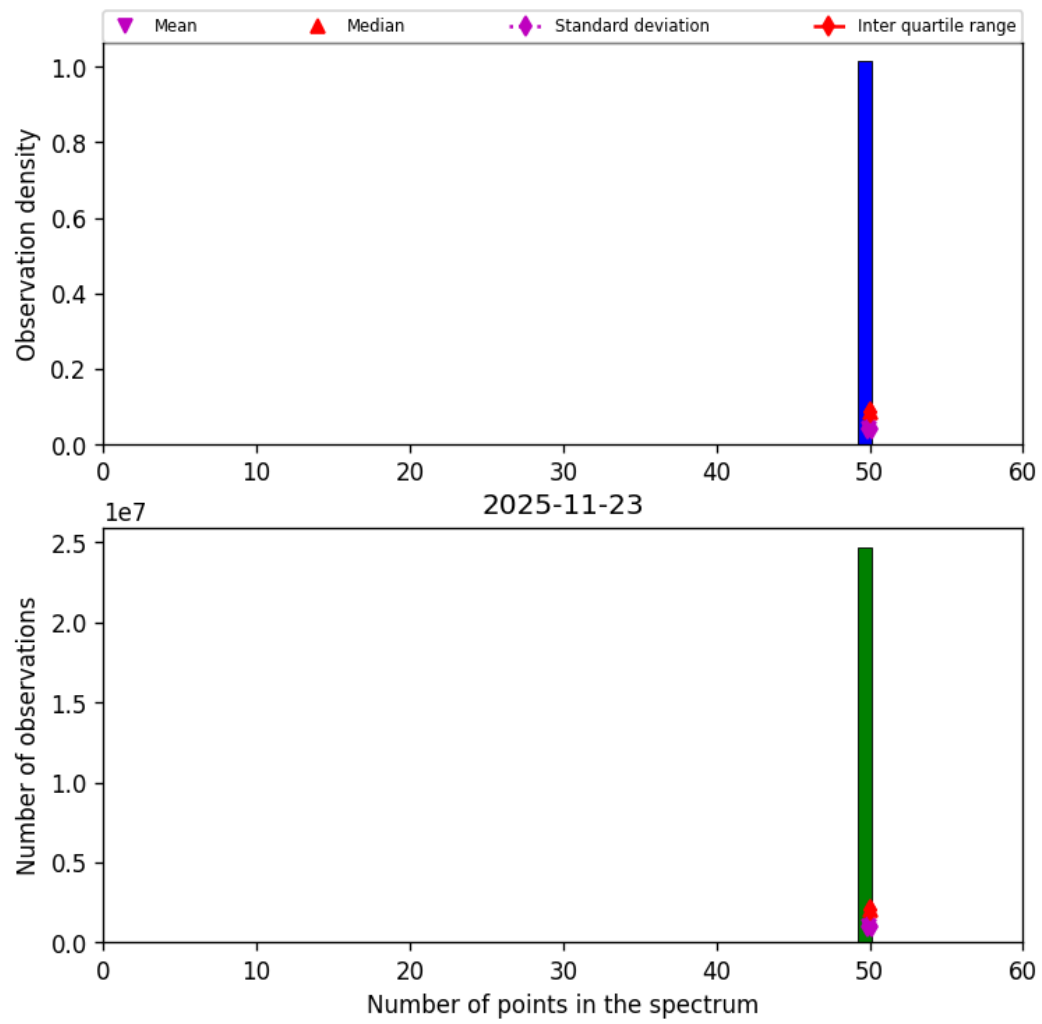
Figure 44: Histogram of “Number of points in the spectrum” for 2025-11-23 to 2025-11-24
