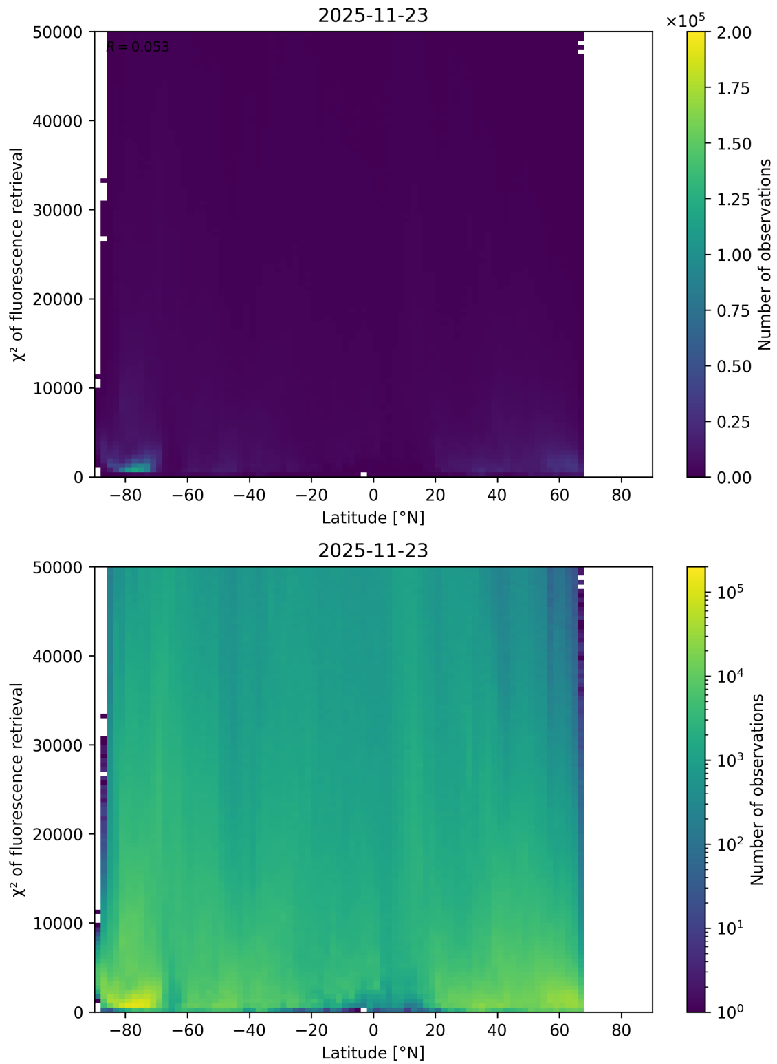
Figure 89: Scatter density plot of “Latitude” against “ \chi^2 of fluorescence retrieval” for 2025-11-23 to 2025-11-24.
