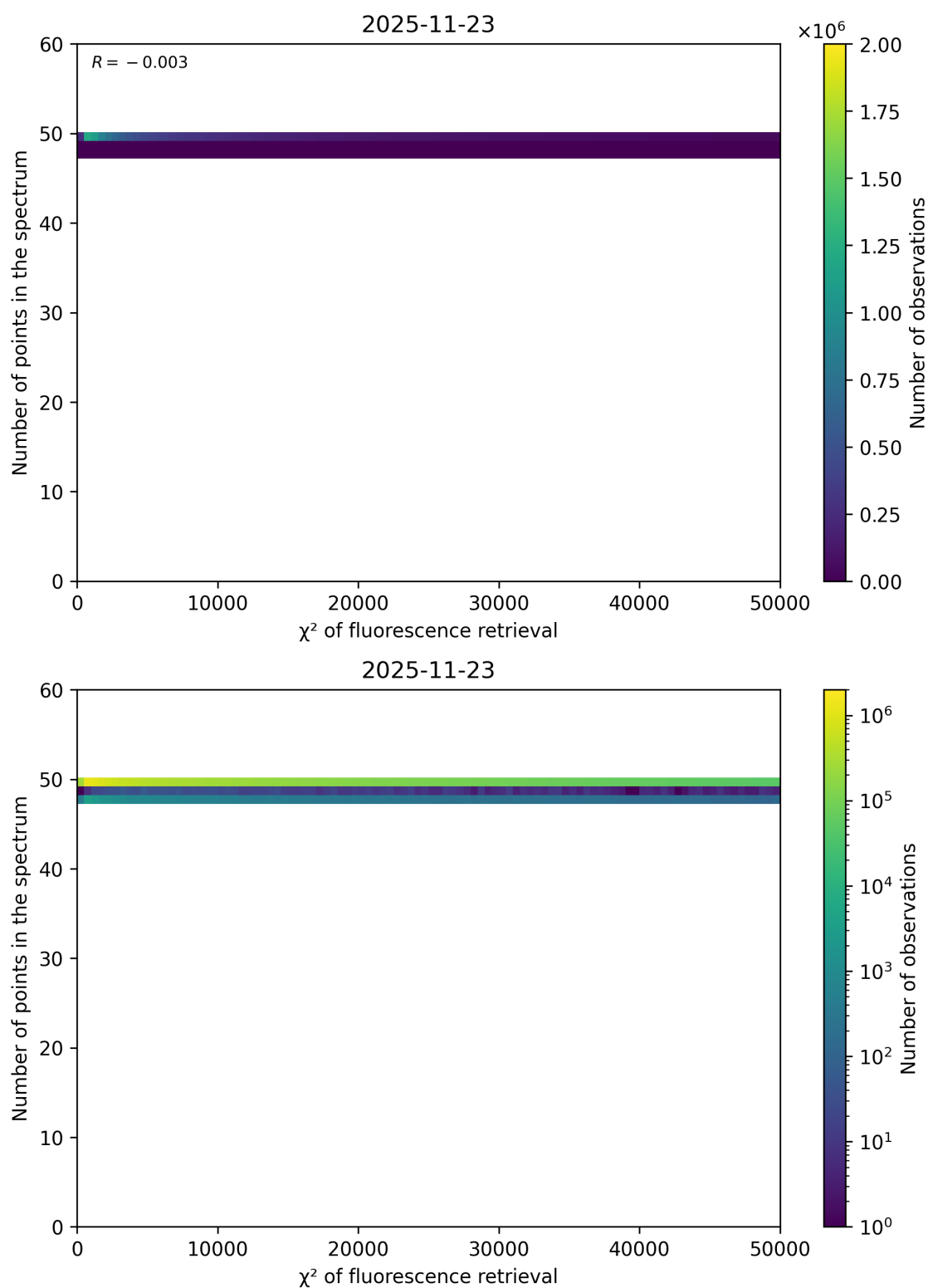
Figure 68: Scatter density plot of “ \chi^2 of fluorescence retrieval” against “Number of points in the spectrum” for 2025-11-23 to 2025-11-24.
