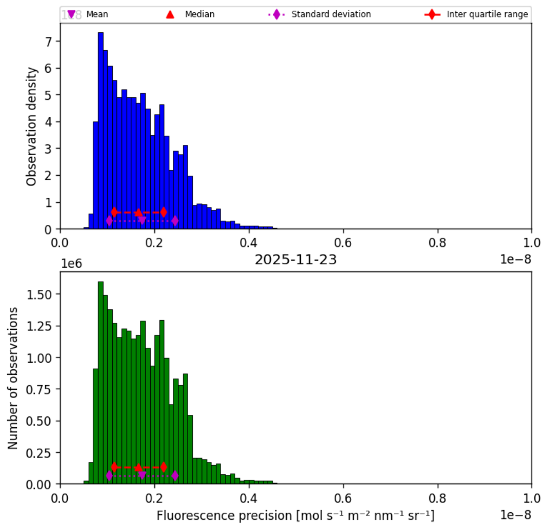
Figure 41: Histogram of “Fluorescence precision” for 2025-11-23 to 2025-11-24
