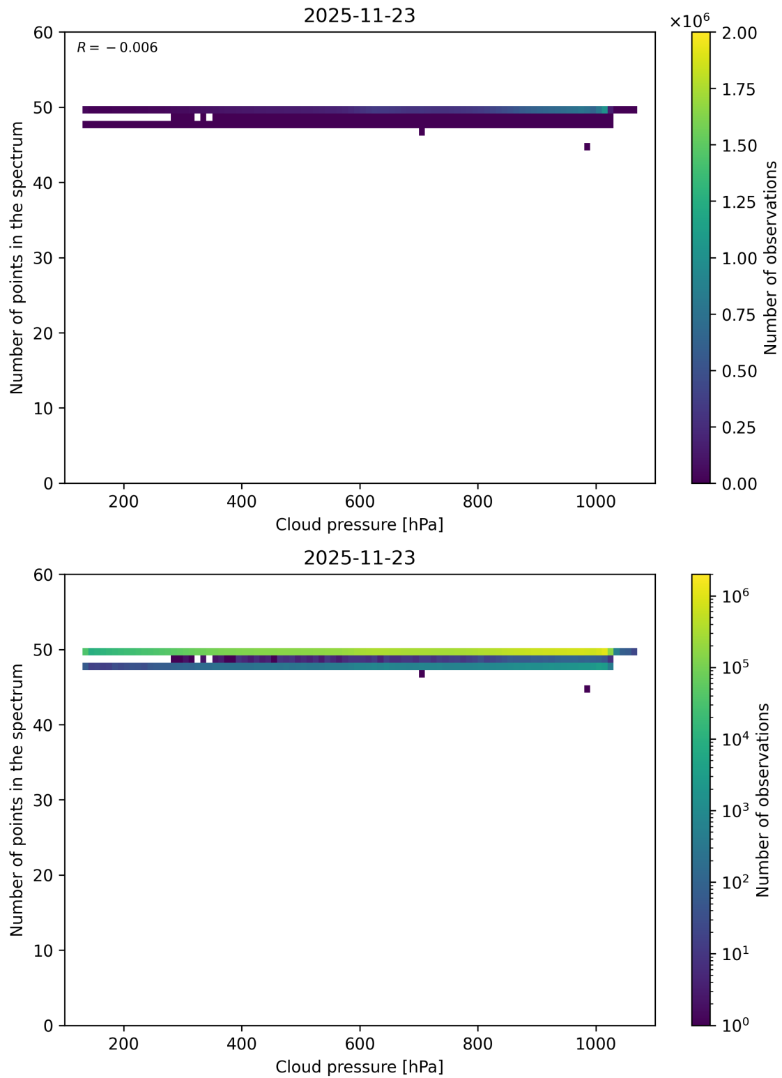
Figure 82: Scatter density plot of “Cloud pressure” against “Number of points in the spectrum” for 2025-11-23 to 2025-11-24.
