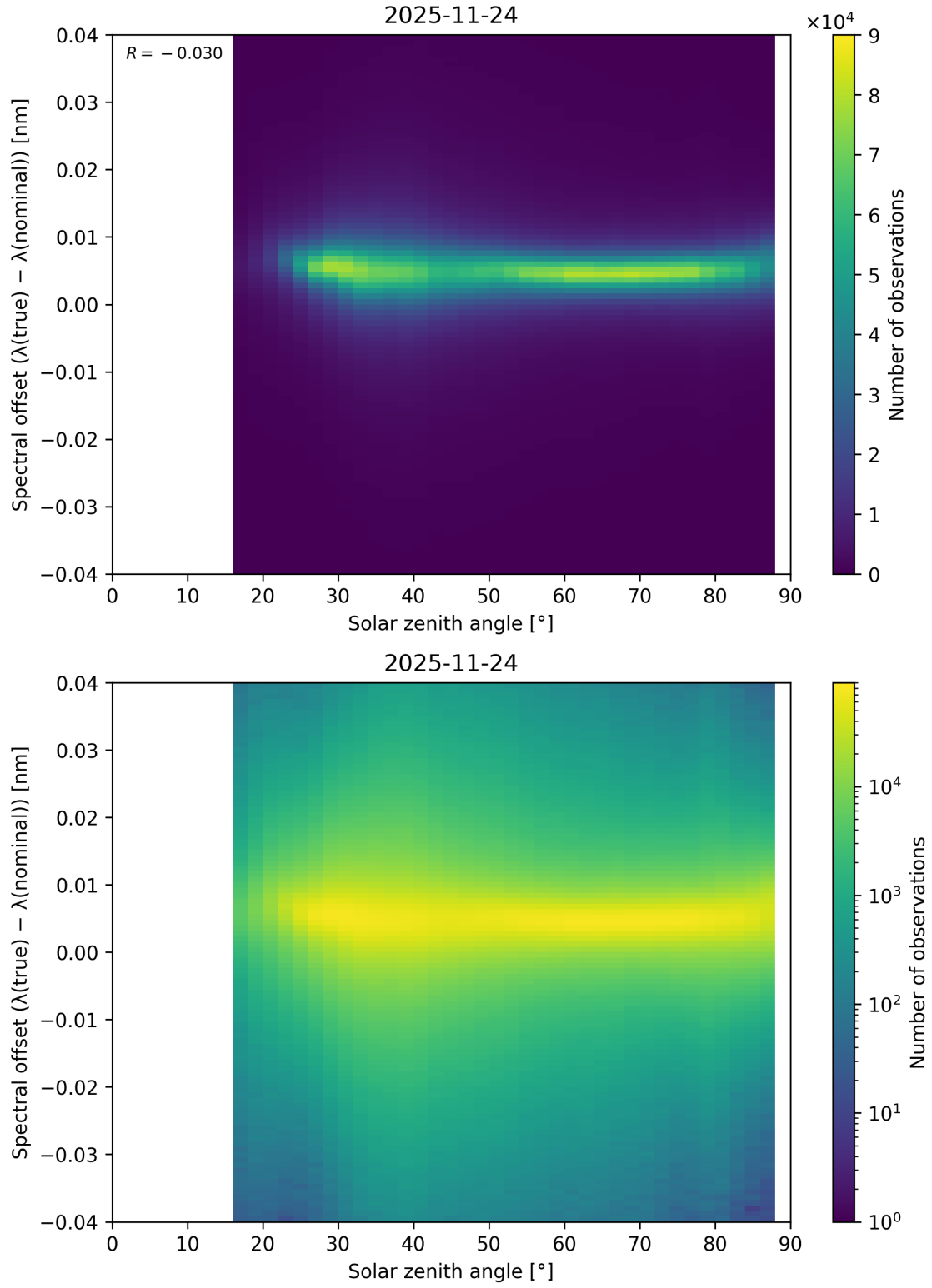
Figure 117: Scatter density plot of “Solar zenith angle” against “Spectral offset ( \lambda_{\text{true}} - \lambda_{\text{nominal}} )” for 2025-11-23 to 2025-11-25.
