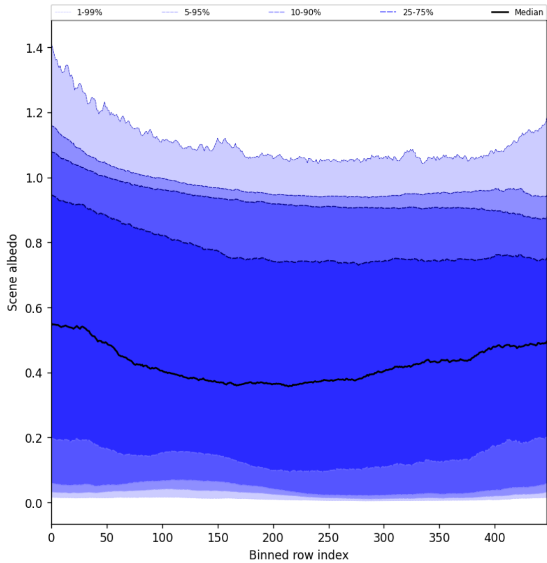
Figure 51: Along track statistics of “Scene albedo” for 2025-11-23 to 2025-11-25
