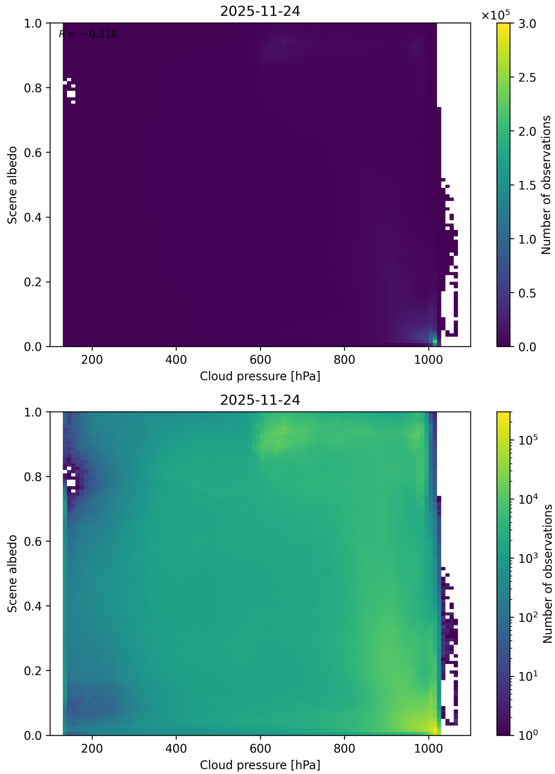
Figure 83: Scatter density plot of “Cloud pressure” against “Scene albedo” for 2025-11-23 to 2025-11-25.
