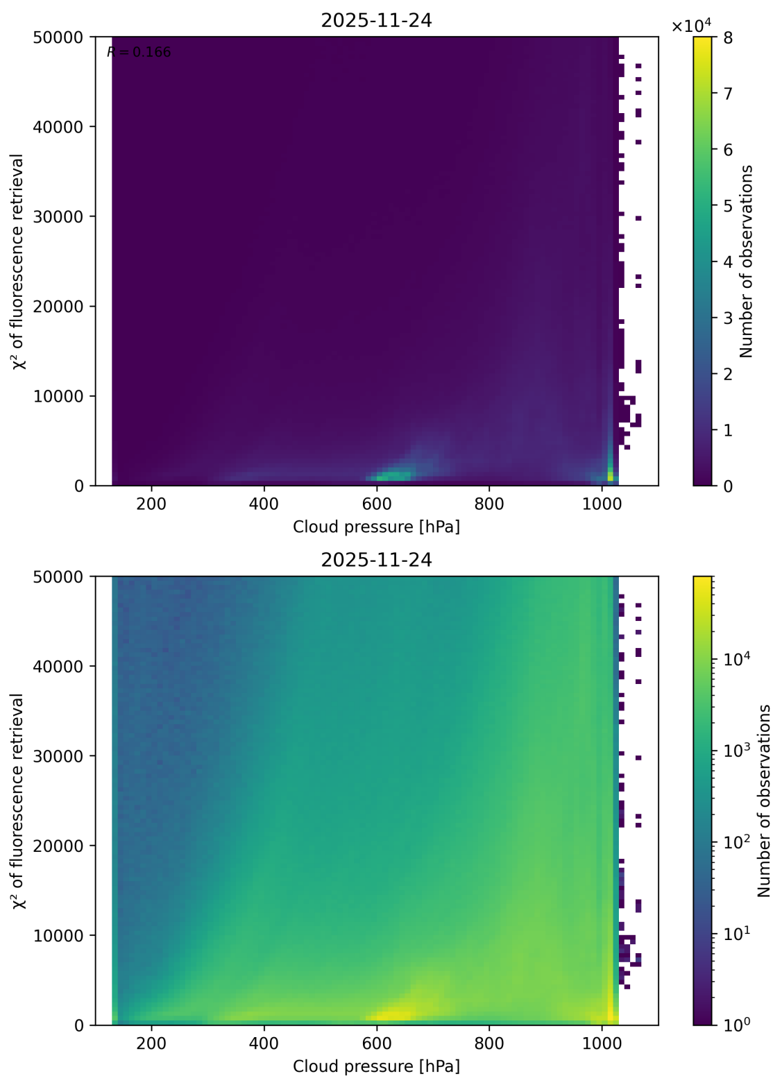
Figure 78: Scatter density plot of “Cloud pressure” against “ \chi^2 of fluorescence retrieval” for 2025-11-23 to 2025-11-25.
