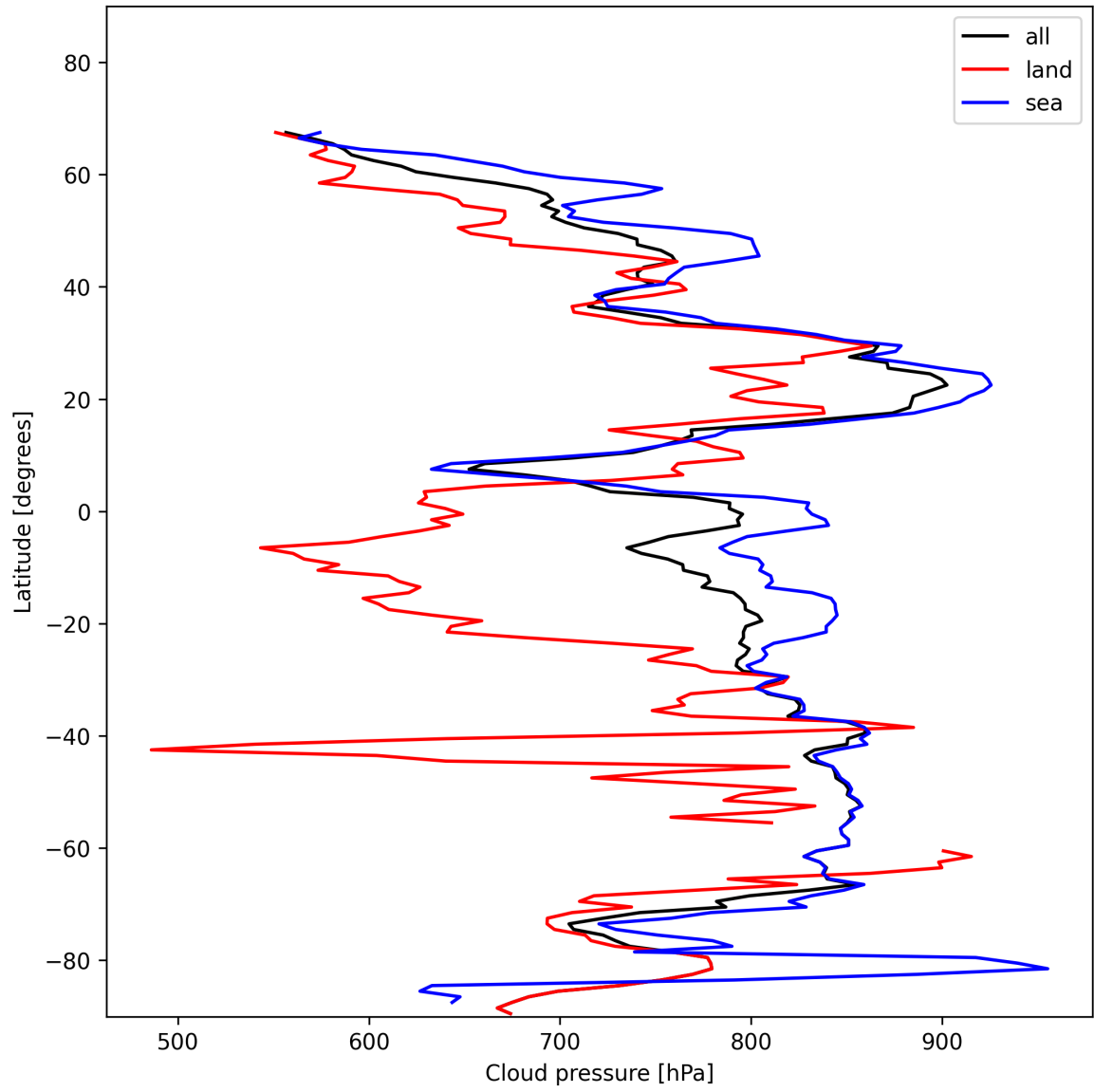
Figure 13: Zonal average of “Cloud pressure” for 2025-11-23 to 2025-11-25.
