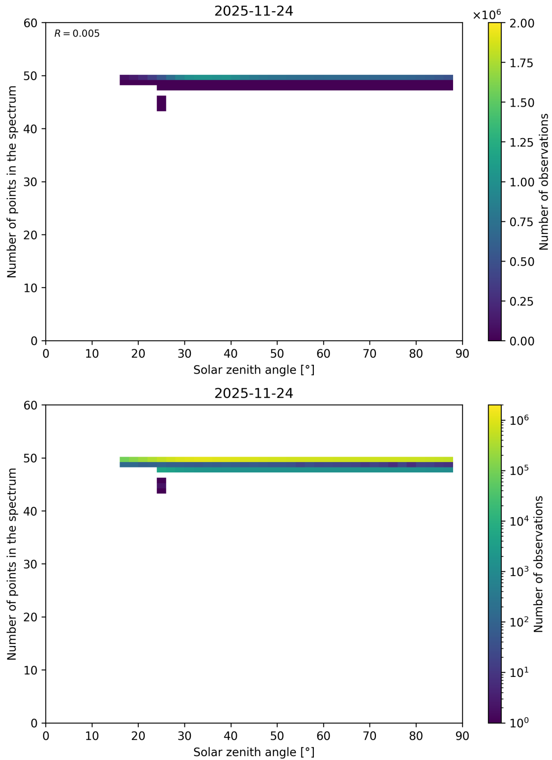
Figure 115: Scatter density plot of “Solar zenith angle” against “Number of points in the spectrum” for 2025-11-23 to 2025-11-25.
