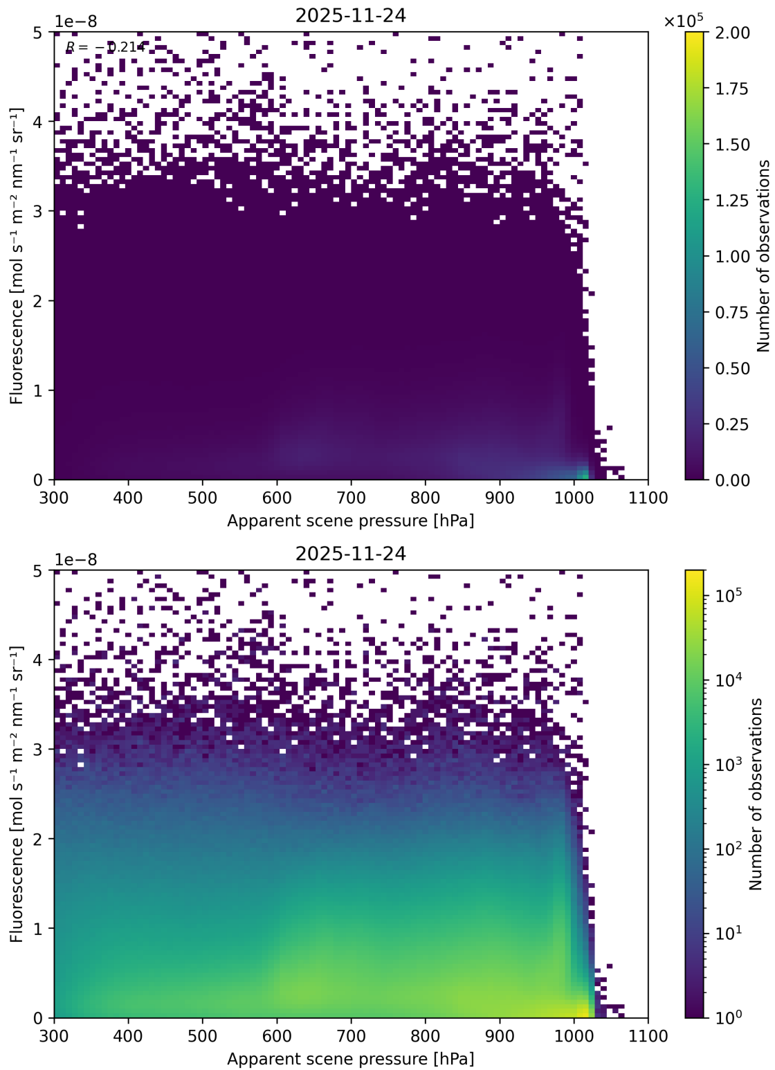
Figure 64: Scatter density plot of “Apparent scene pressure” against “Fluorescence” for 2025-11-23 to 2025-11-25.
