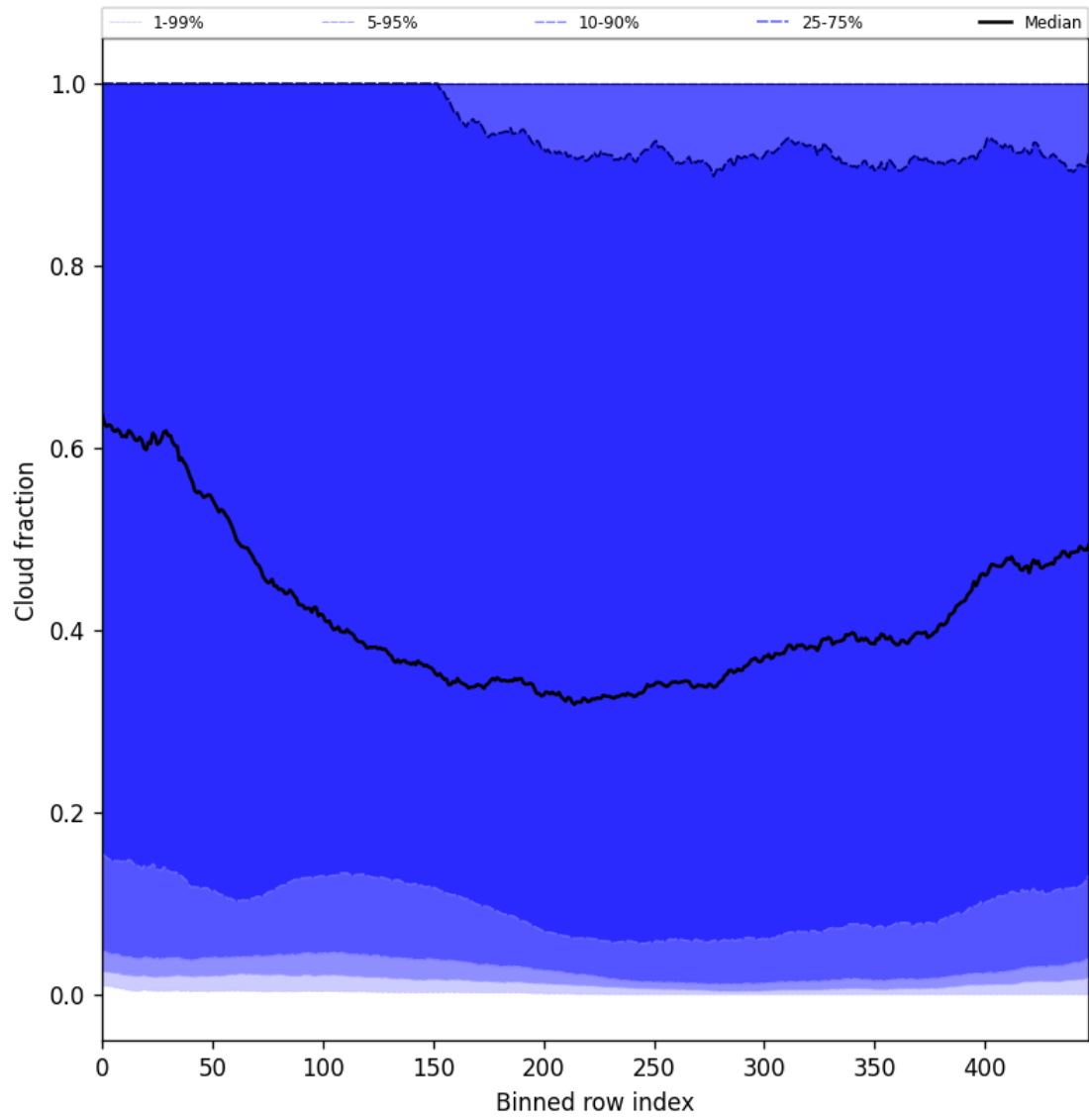
Figure 49: Along track statistics of “Cloud fraction” for 2025-11-23 to 2025-11-25
