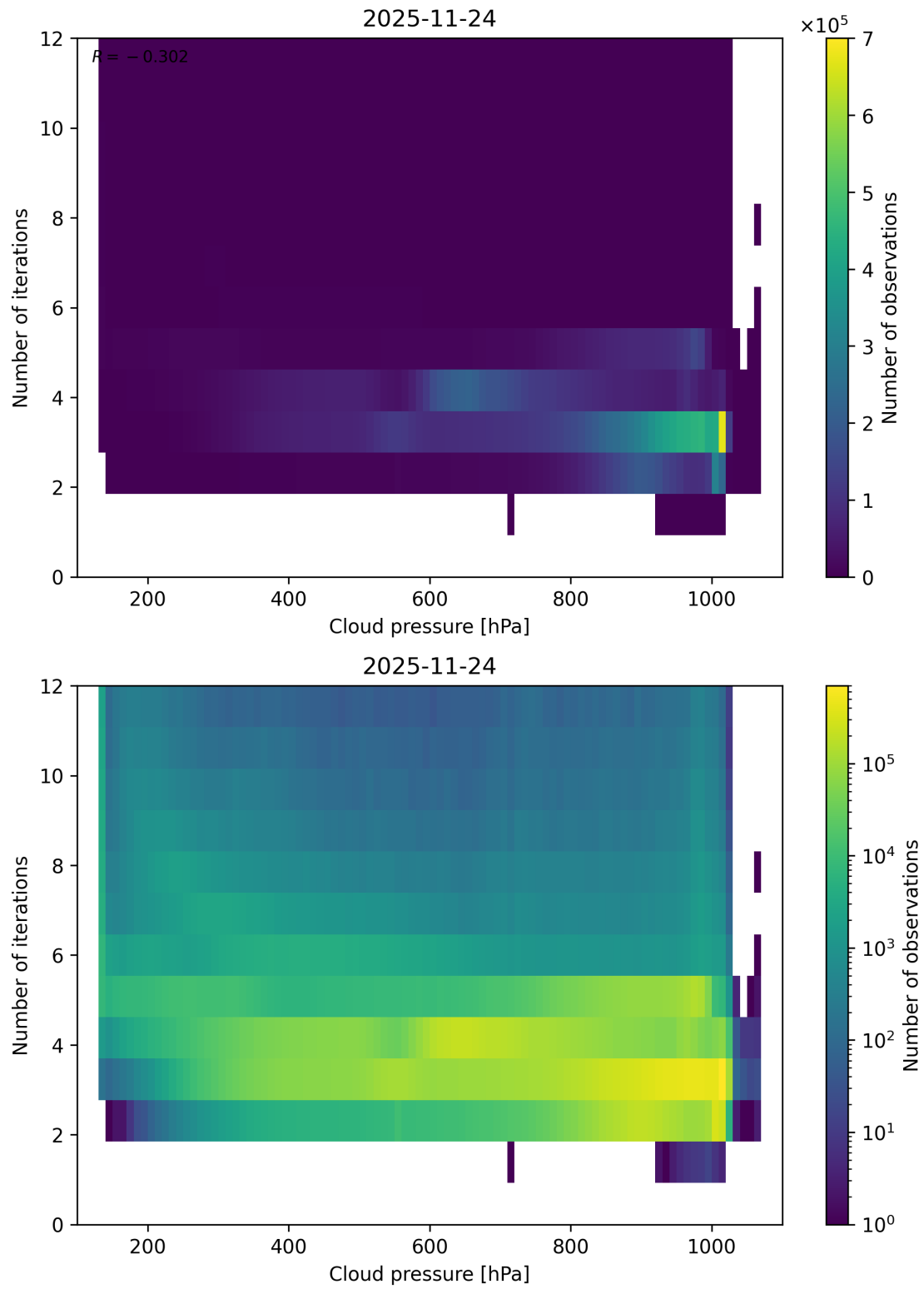
Figure 81: Scatter density plot of “Cloud pressure” against “Number of iterations” for 2025-11-23 to 2025-11-25.
