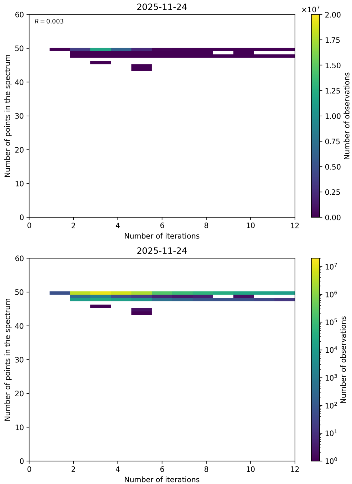
Figure 99: Scatter density plot of “Number of iterations” against “Number of points in the spectrum” for 2025-11-23 to 2025-11-25.
