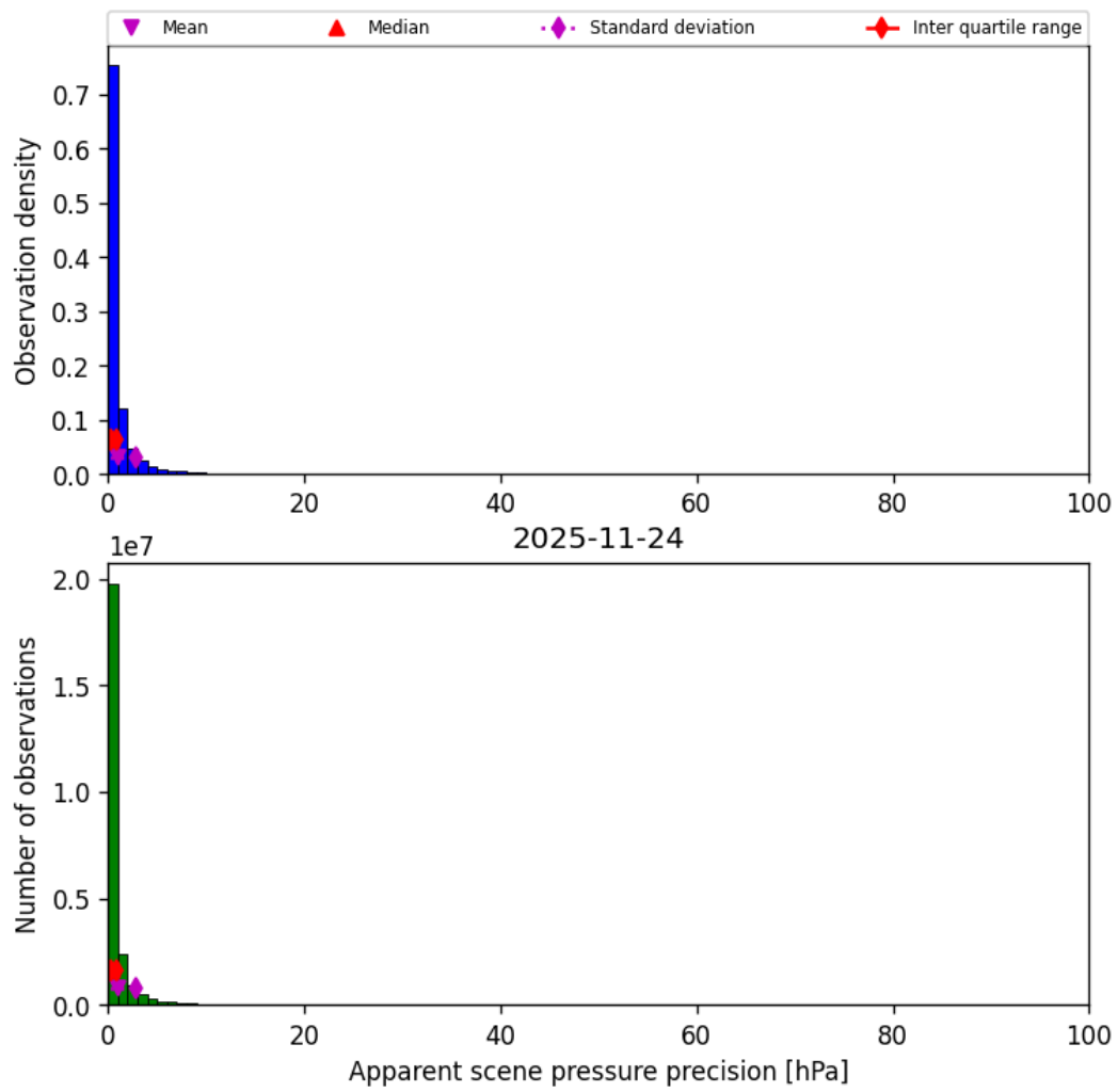
Figure 37: Histogram of “Apparent scene pressure precision” for 2025-11-23 to 2025-11-25
