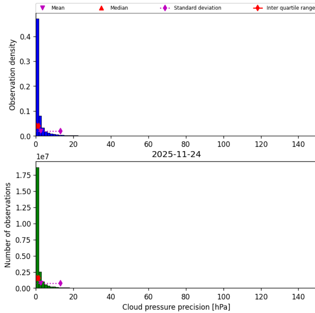
Figure 31: Histogram of “Cloud pressure precision” for 2025-11-23 to 2025-11-25
