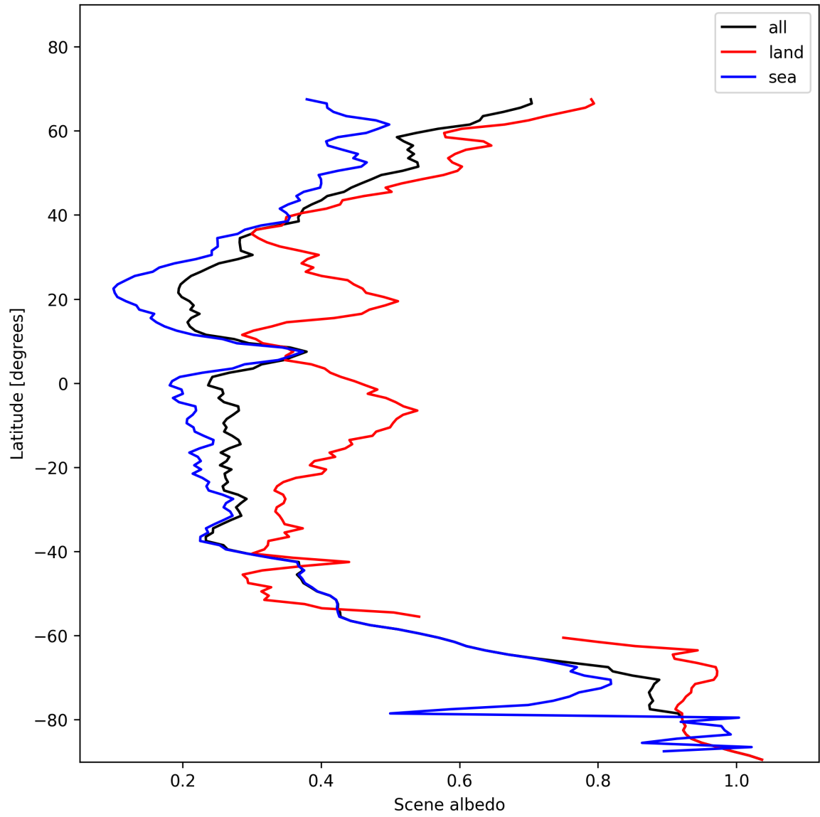
Figure 17: Zonal average of “Scene albedo” for 2025-11-23 to 2025-11-25.
