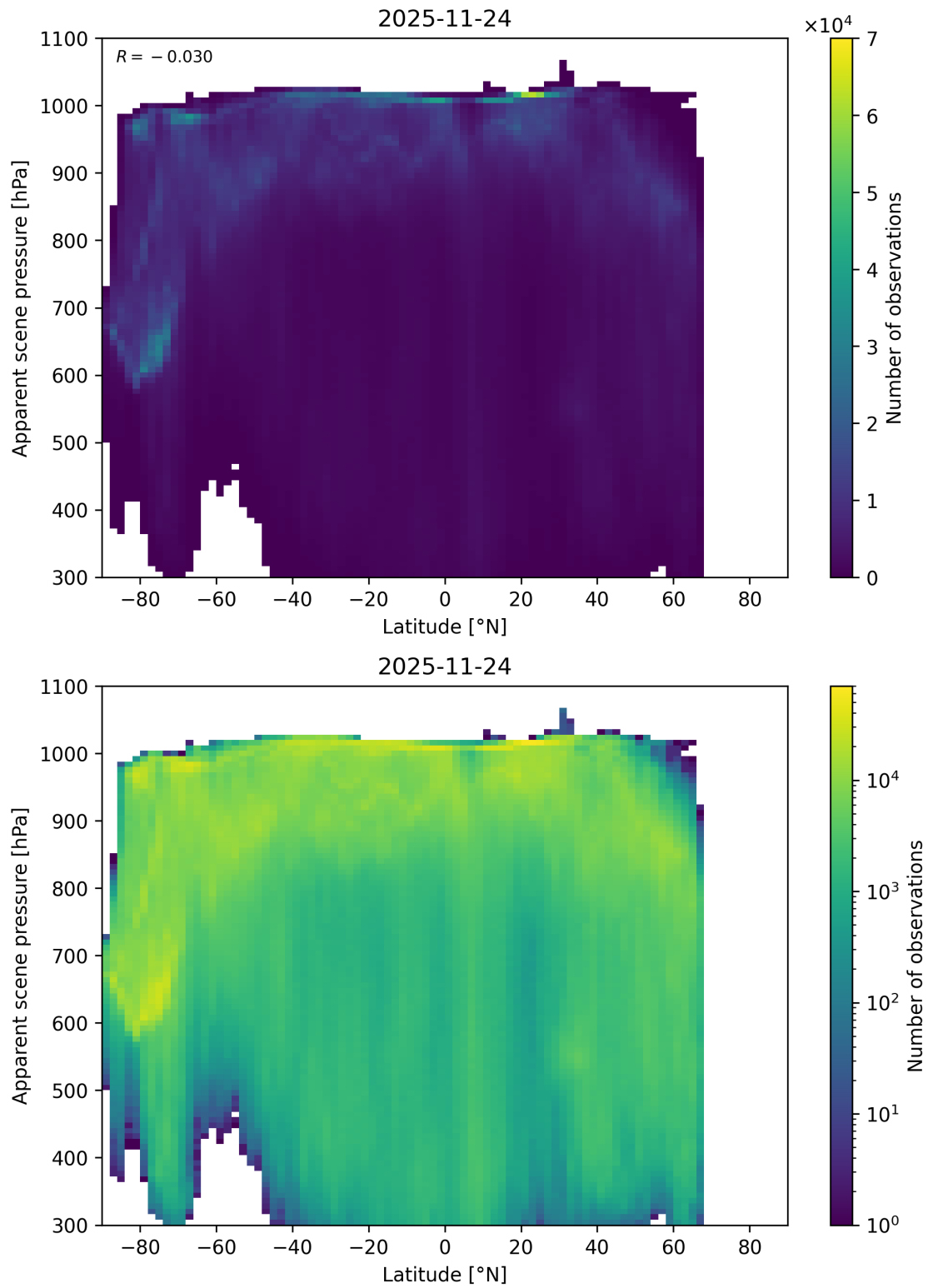
Figure 88: Scatter density plot of “Latitude” against “Apparent scene pressure” for 2025-11-23 to 2025-11-25.
