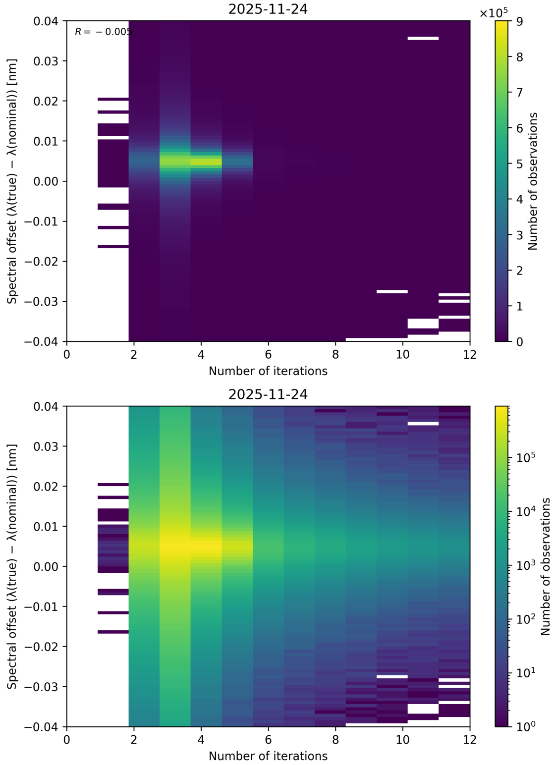
Figure 100: Scatter density plot of “Number of iterations” against “Spectral offset ( \lambda_{\text{true}} - \lambda_{\text{nominal}} )” for 2025-11-23 to 2025-11-25.
