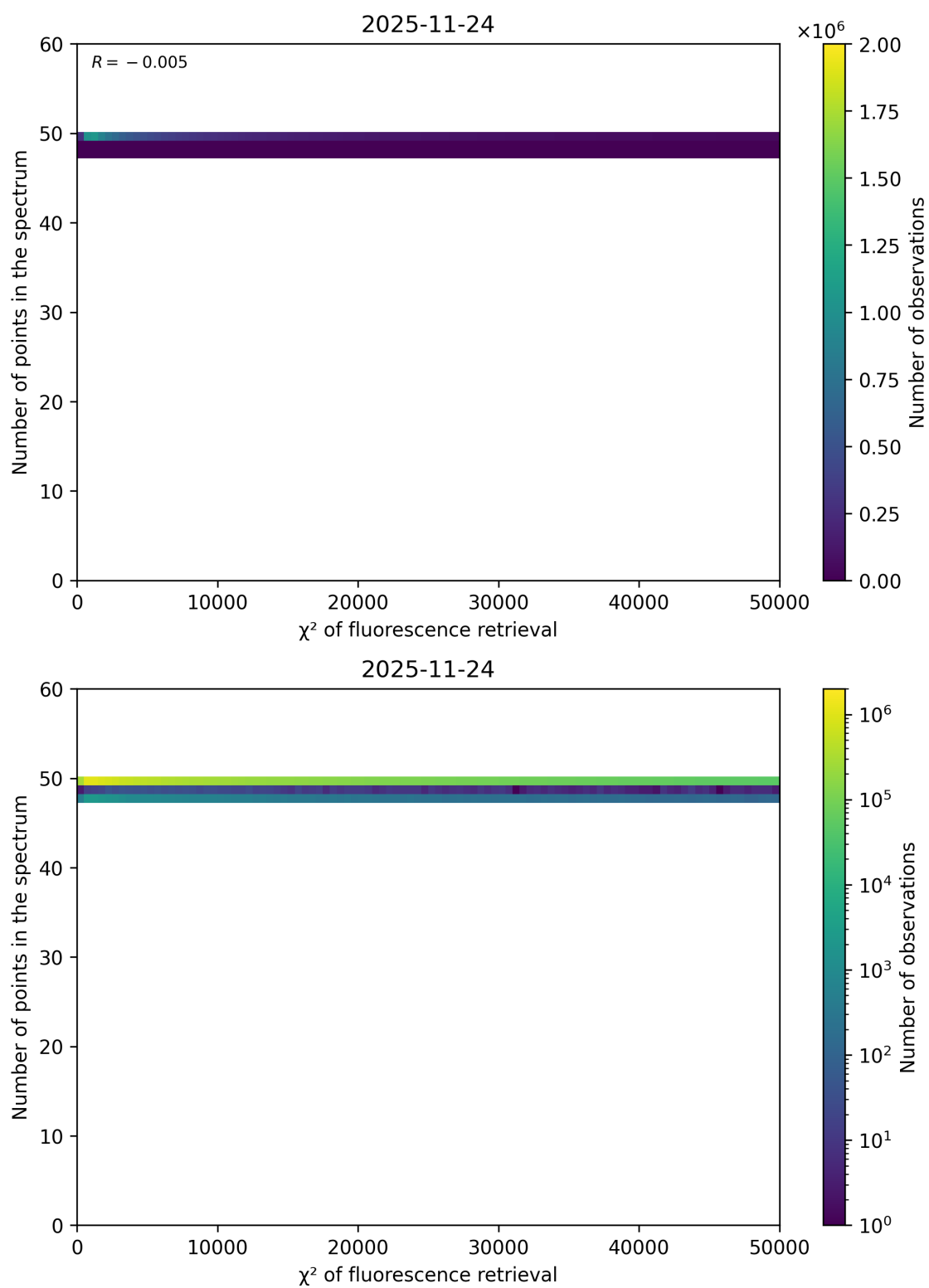
Figure 68: Scatter density plot of " \chi^2 of fluorescence retrieval" against "Number of points in the spectrum" for 2025-11-23 to 2025-11-25.
