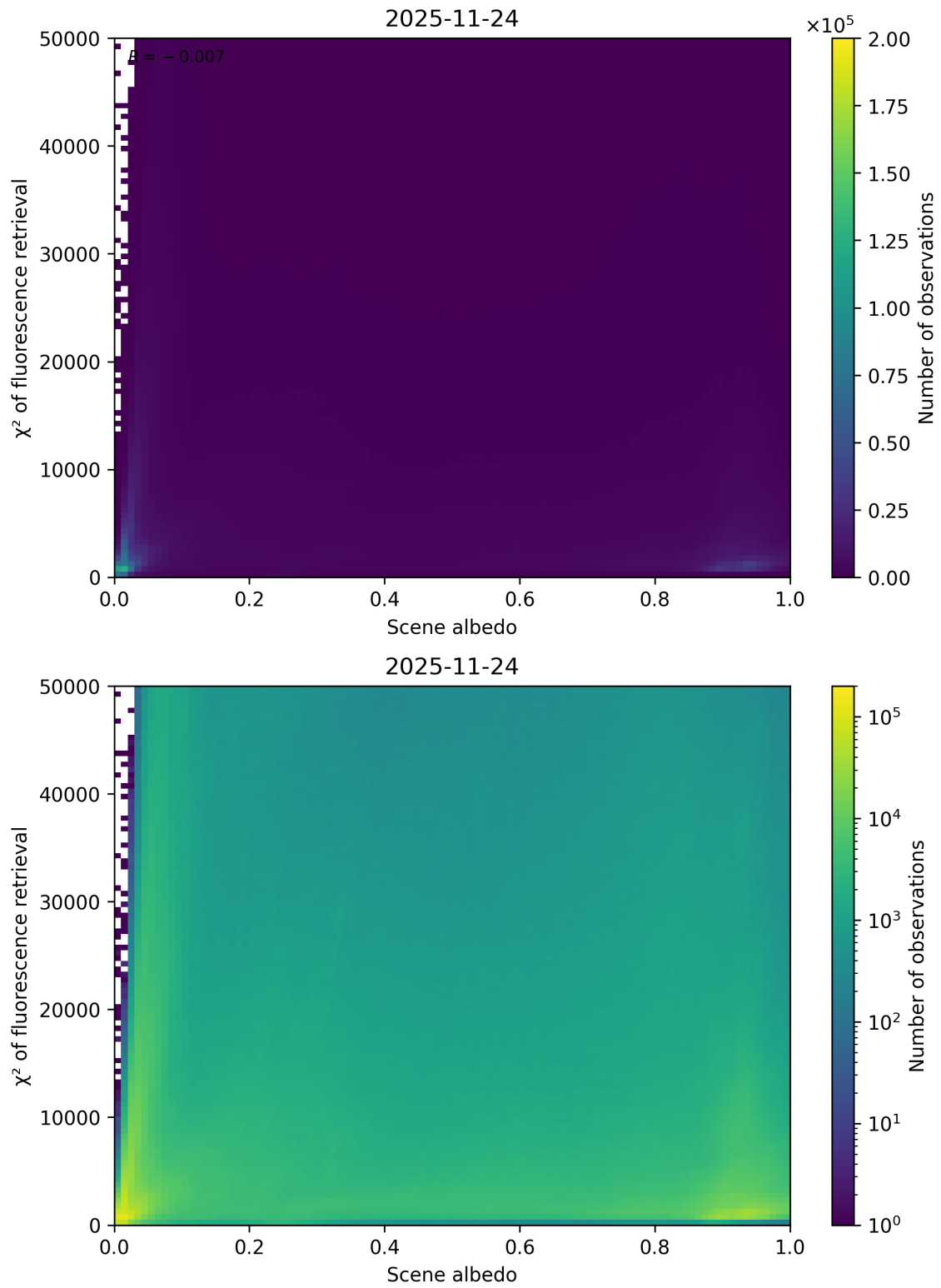
Figure 103: Scatter density plot of “Scene albedo” against “ \chi^2 of fluorescence retrieval” for 2025-11-23 to 2025-11-25.
