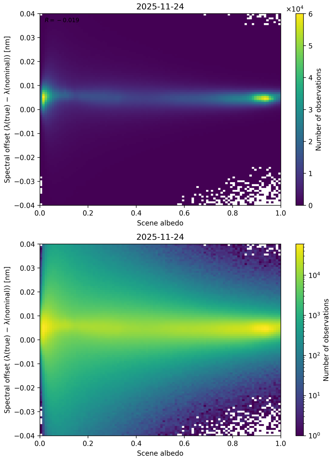
Figure 107: Scatter density plot of “Scene albedo” against “Spectral offset ( \lambda_{\text{true}} - \lambda_{\text{nominal}} )” for 2025-11-23 to 2025-11-25.
