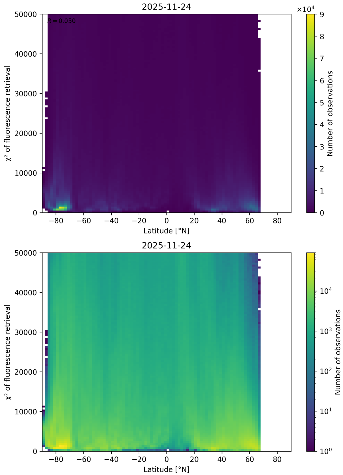
Figure 89: Scatter density plot of “Latitude” against “ \chi^2 of fluorescence retrieval” for 2025-11-23 to 2025-11-25.
