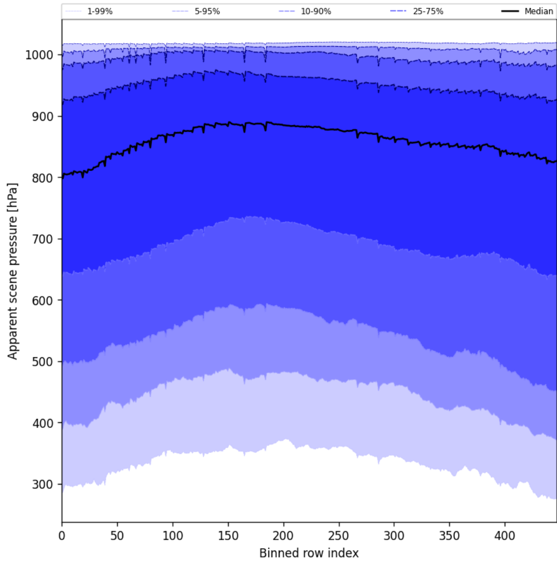
Figure 53: Along track statistics of “Apparent scene pressure” for 2025-11-23 to 2025-11-25
