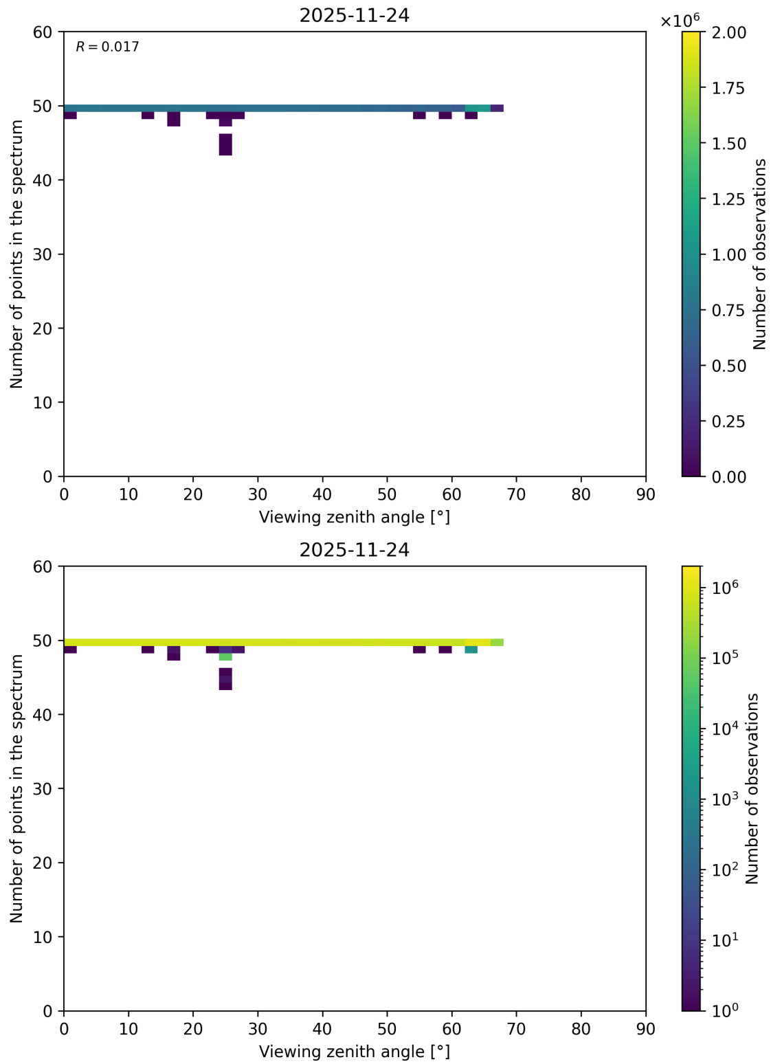
Figure 125: Scatter density plot of “Viewing zenith angle” against “Number of points in the spectrum” for 2025-11-23 to 2025-11-25.
