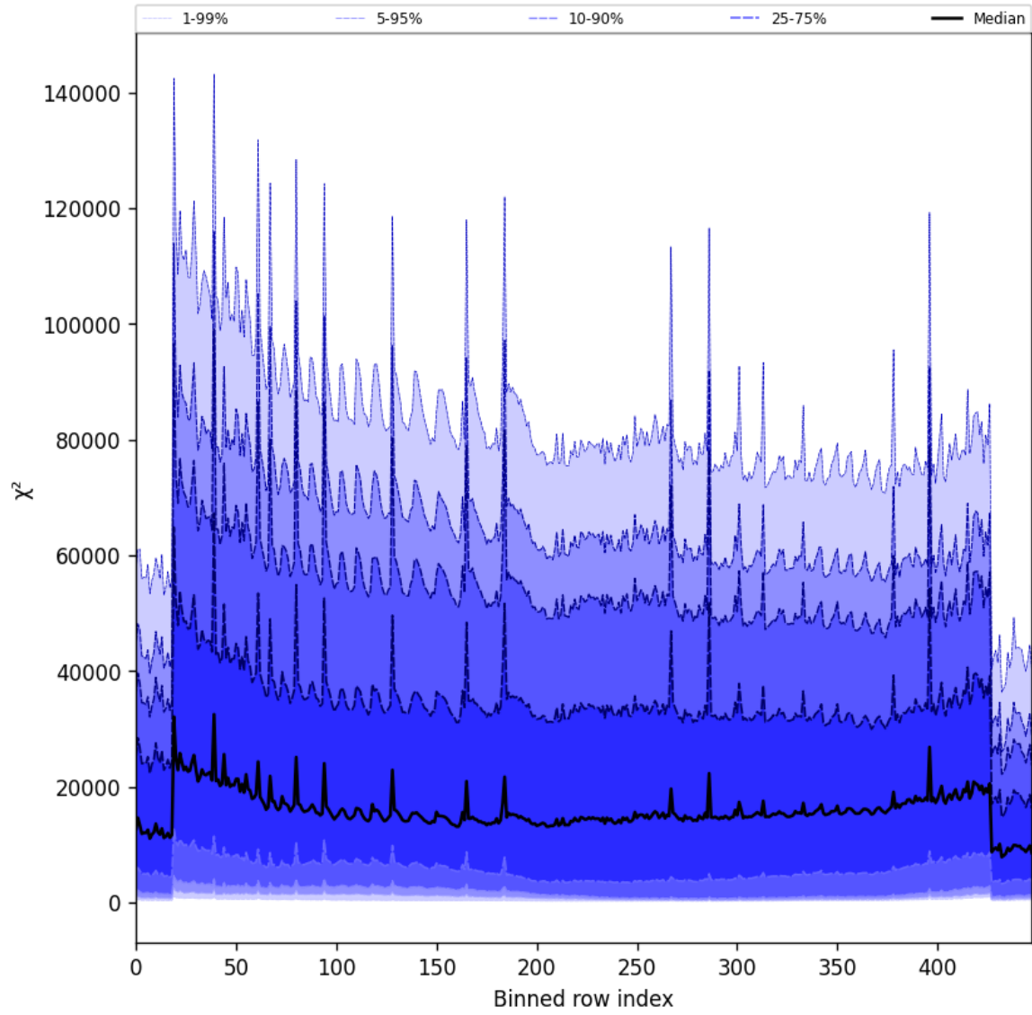
Figure 55: Along track statistics of “ \chi^2 ” for 2025-11-23 to 2025-11-25
