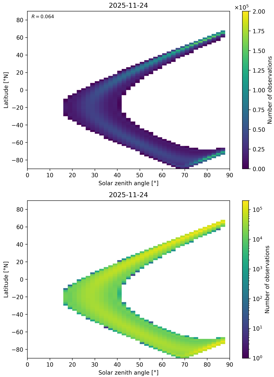
Figure 113: Scatter density plot of “Solar zenith angle” against “Latitude” for 2025-11-23 to 2025-11-25.
