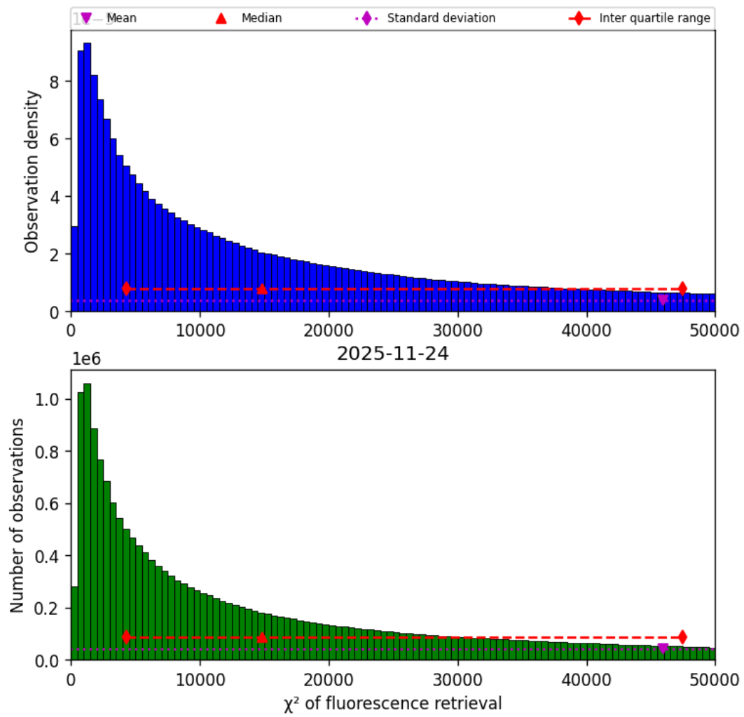
Figure 42: Histogram of “ \chi^2 of fluorescence retrieval” for 2025-11-23 to 2025-11-25
