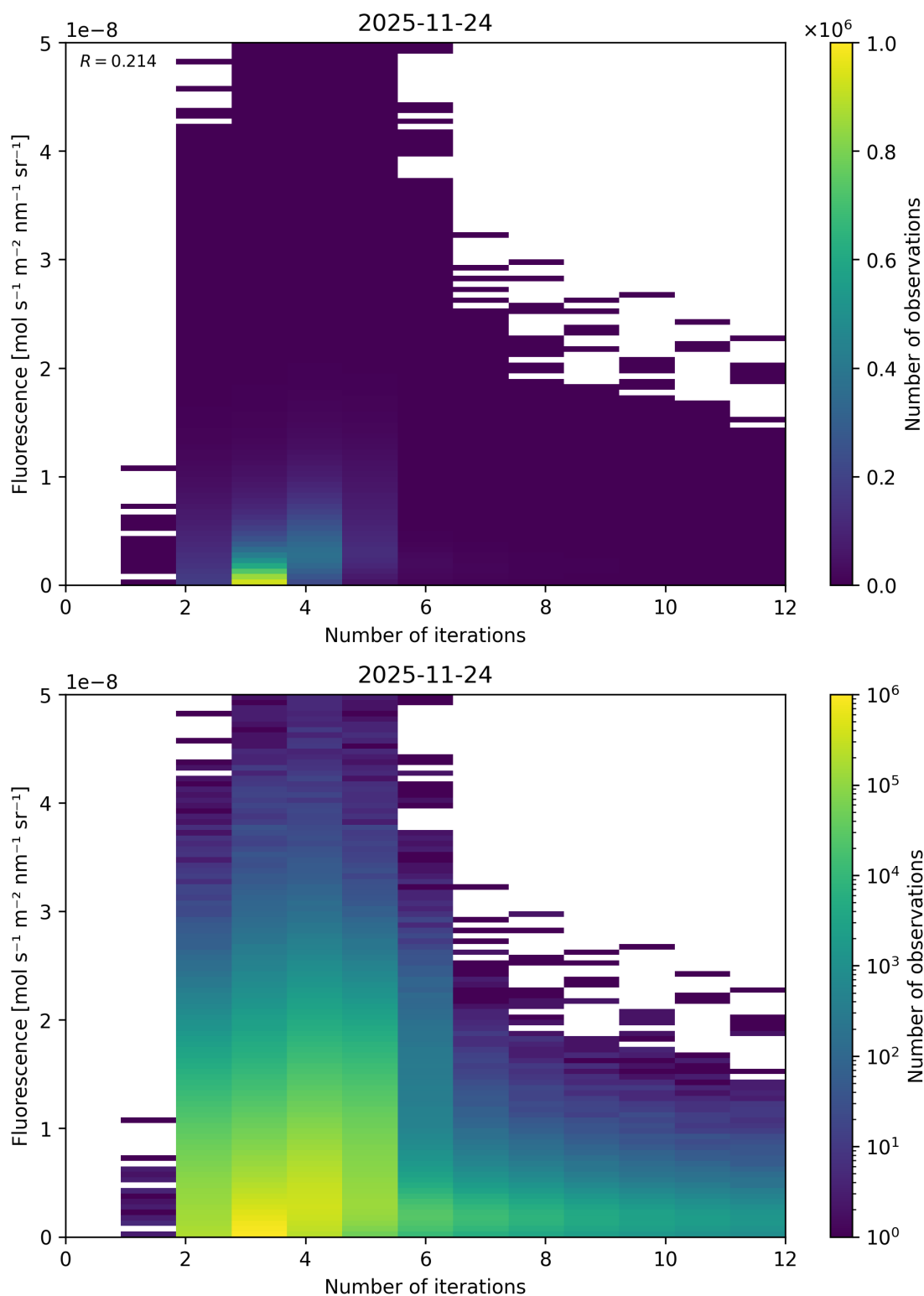
Figure 98: Scatter density plot of “Number of iterations” against “Fluorescence” for 2025-11-23 to 2025-11-25.
