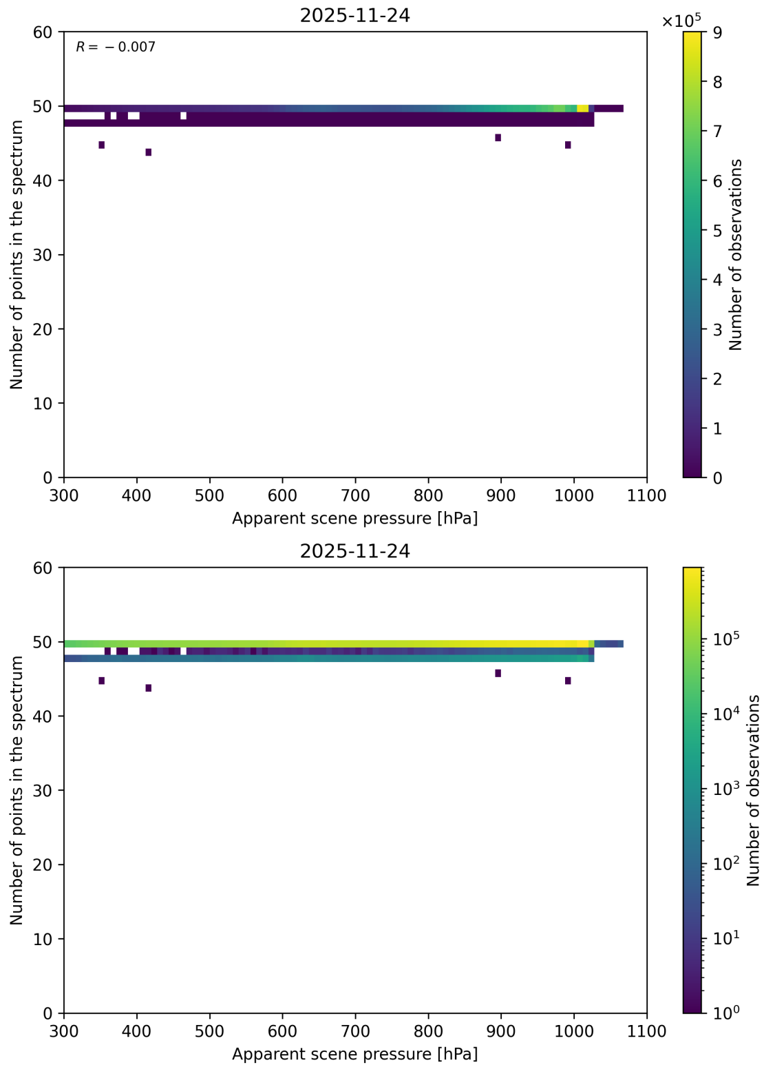
Figure 66: Scatter density plot of “Apparent scene pressure” against “Number of points in the spectrum” for 2025-11-23 to 2025-11-25.
