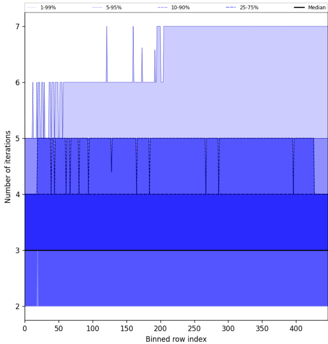
Figure 56: Along track statistics of “Number of iterations” for 2025-11-23 to 2025-11-25
