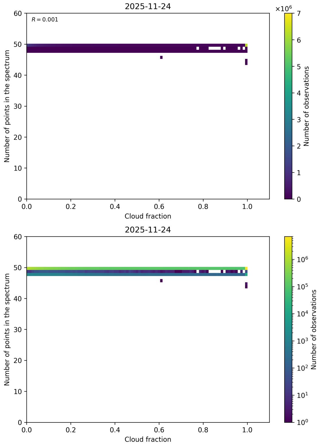
Figure 74: Scatter density plot of “Cloud fraction” against “Number of points in the spectrum” for 2025-11-23 to 2025-11-25.
