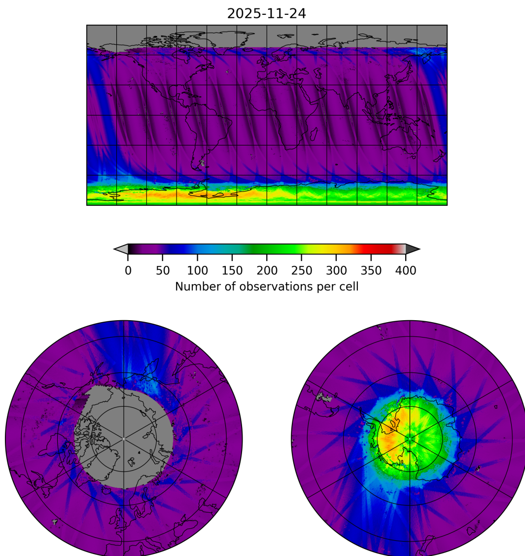
Figure 11: Map of the number of observations for 2025-11-23 to 2025-11-25
