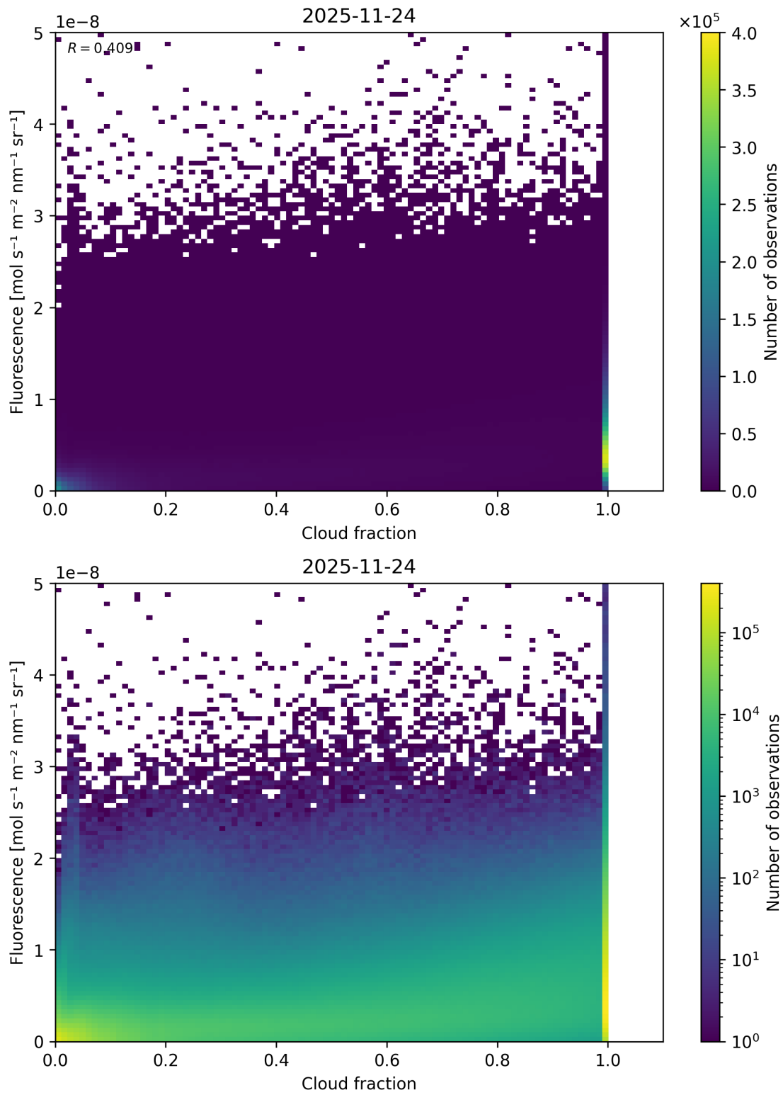
Figure 72: Scatter density plot of “Cloud fraction” against “Fluorescence” for 2025-11-23 to 2025-11-25.
