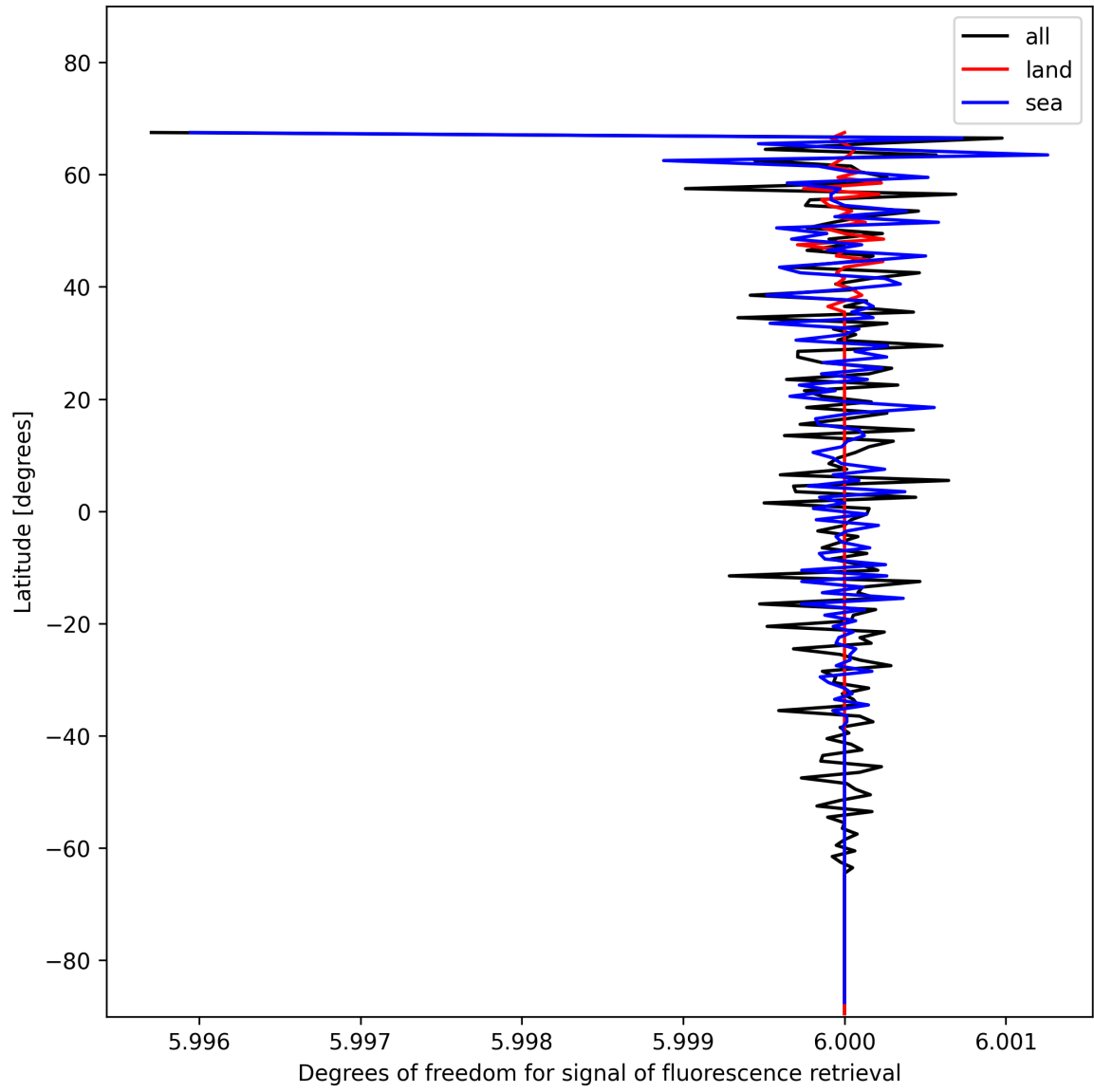
Figure 26: Zonal average of “Degrees of freedom for signal of fluorescence retrieval” for 2025-11-23 to 2025-11-25.
