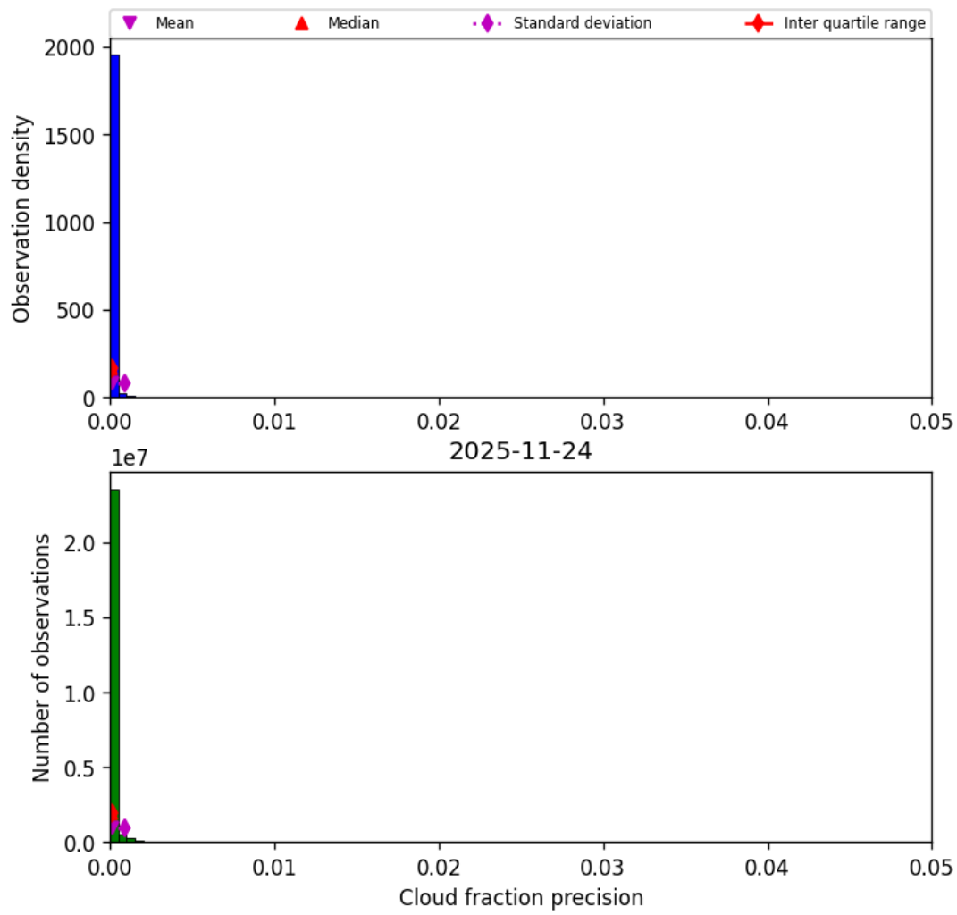
Figure 33: Histogram of “Cloud fraction precision” for 2025-11-23 to 2025-11-25
