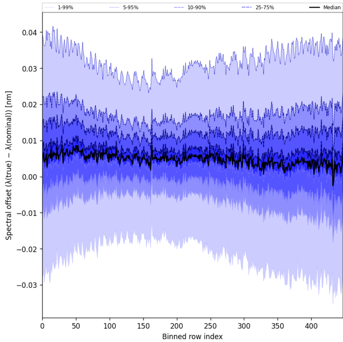
Figure 62: Along track statistics of “Spectral offset ( \lambda_{\text{true}} - \lambda_{\text{nominal}} )” for 2025-11-23 to 2025-11-25
