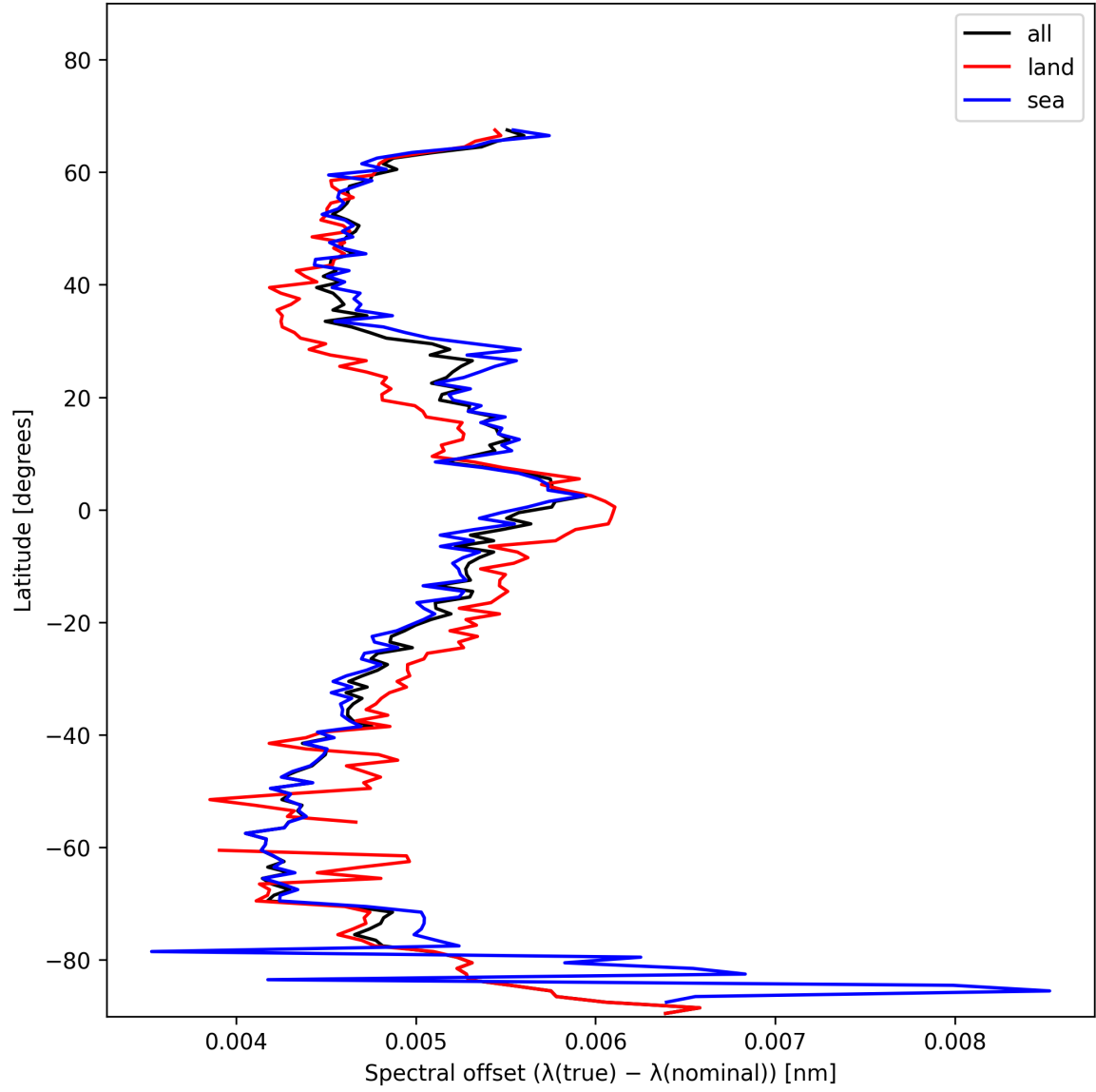
Figure 28: Zonal average of “Spectral offset ( \lambda_{\text{true}} - \lambda_{\text{nominal}} )” for 2025-11-23 to 2025-11-25.
