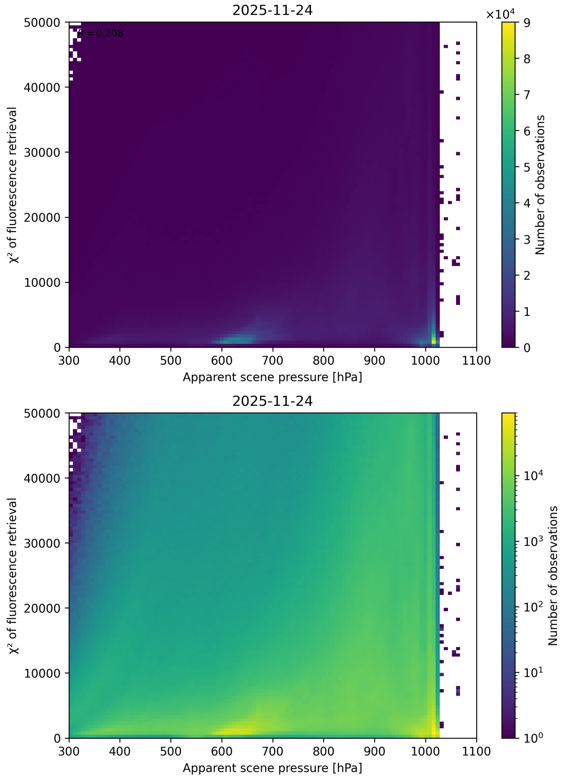
Figure 63: Scatter density plot of “Apparent scene pressure” against “ \chi^2 of fluorescence retrieval” for 2025-11-23 to 2025-11-25.
