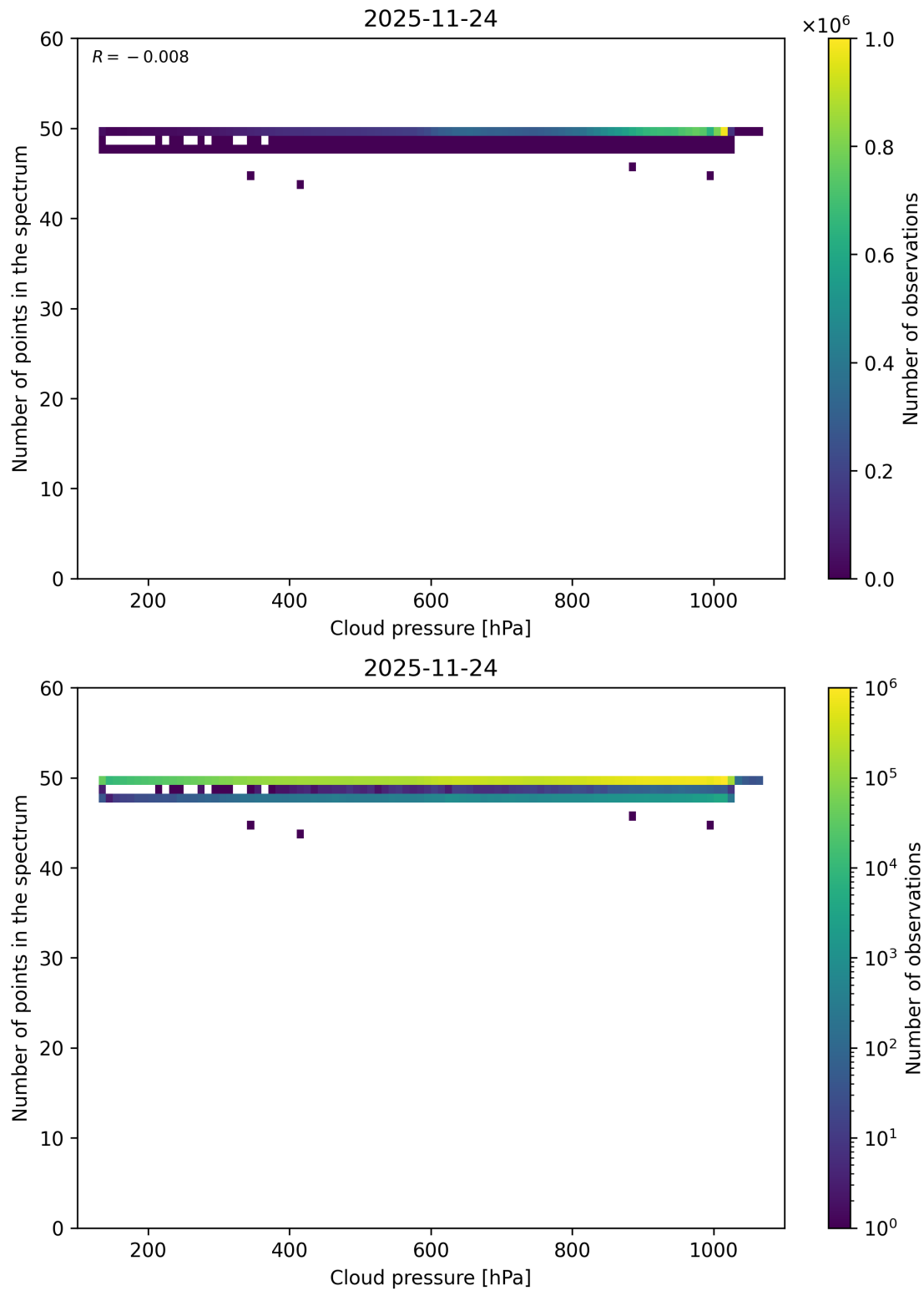
Figure 82: Scatter density plot of “Cloud pressure” against “Number of points in the spectrum” for 2025-11-23 to 2025-11-25.
