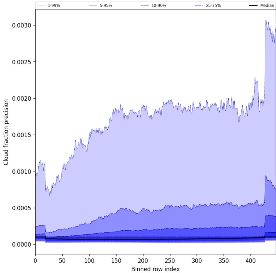
Figure 50: Along track statistics of “Cloud fraction precision” for 2025-11-23 to 2025-11-25
