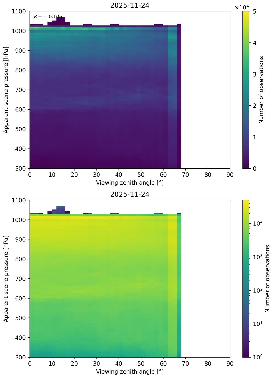
Figure 118: Scatter density plot of “Viewing zenith angle” against “Apparent scene pressure” for 2025-11-23 to 2025-11-25.
