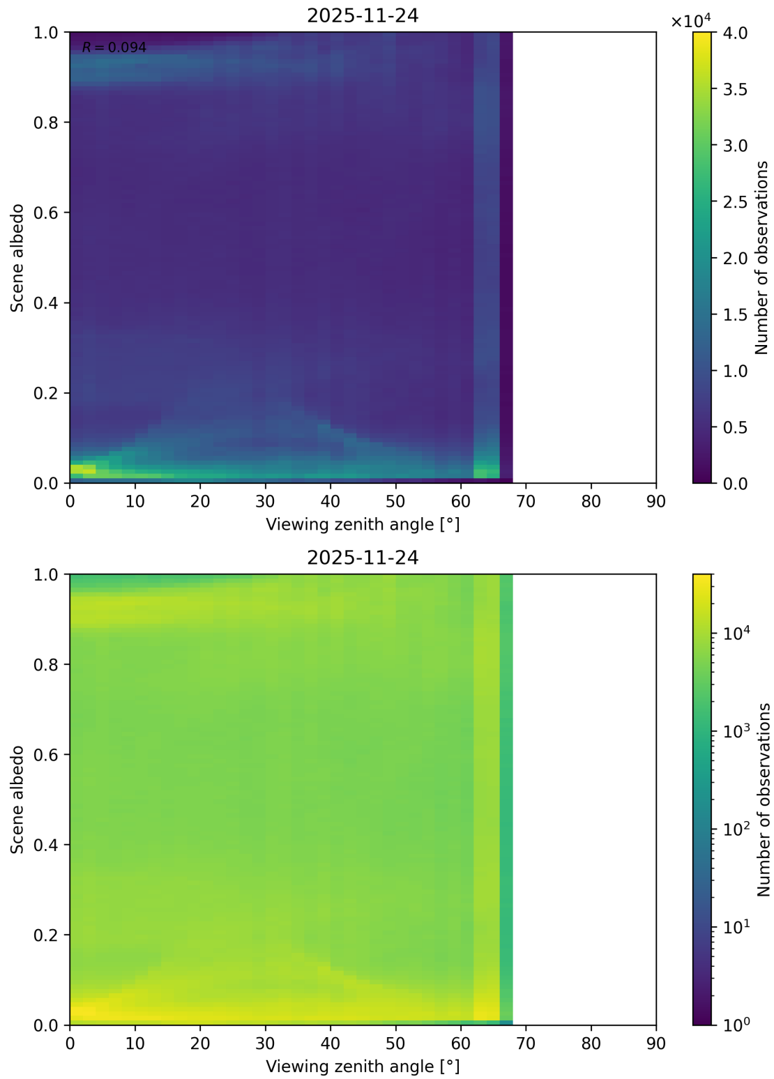
Figure 126: Scatter density plot of “Viewing zenith angle” against “Scene albedo” for 2025-11-23 to 2025-11-25.
