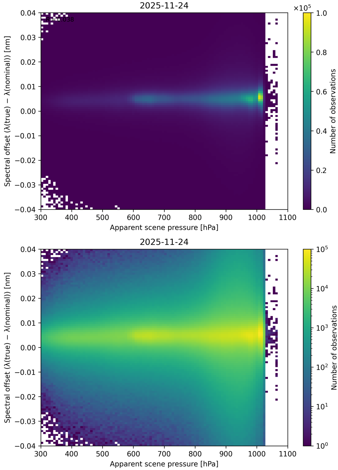
Figure 67: Scatter density plot of “Apparent scene pressure” against “Spectral offset ( \lambda_{\text{true}} - \lambda_{\text{nominal}} )” for 2025-11-23 to 2025-11-25.
