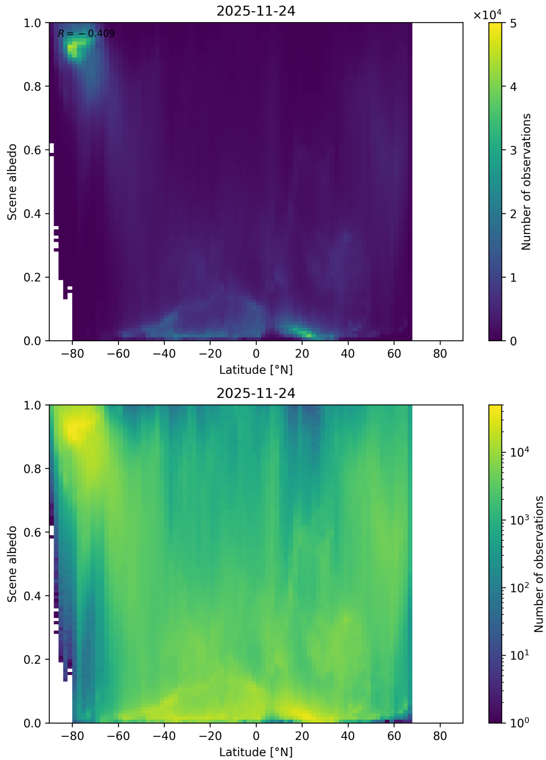
Figure 95: Scatter density plot of “Latitude” against “Scene albedo” for 2025-11-23 to 2025-11-25.
