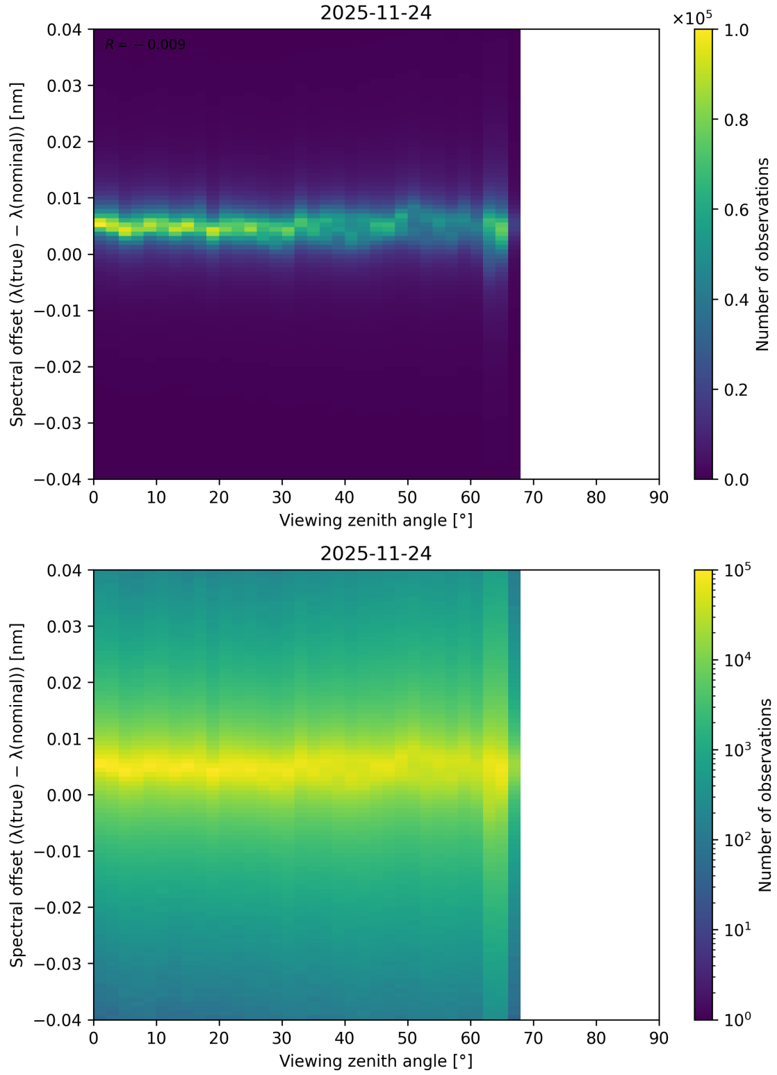
Figure 128: Scatter density plot of “Viewing zenith angle” against “Spectral offset ( \lambda_{\text{true}} - \lambda_{\text{nominal}} )” for 2025-11-23 to 2025-11-25.
