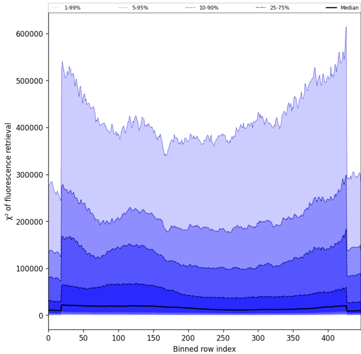
Figure 59: Along track statistics of “ \chi^2 of fluorescence retrieval” for 2025-11-23 to 2025-11-25
