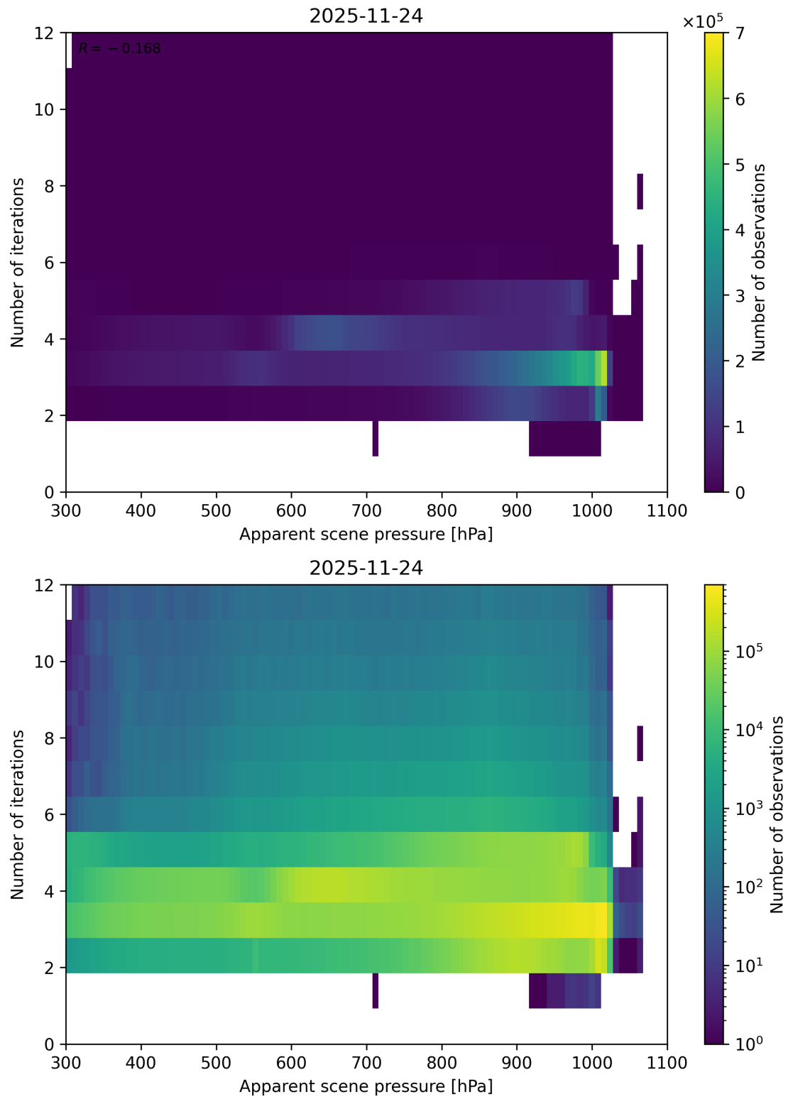
Figure 65: Scatter density plot of “Apparent scene pressure” against “Number of iterations” for 2025-11-23 to 2025-11-25.
