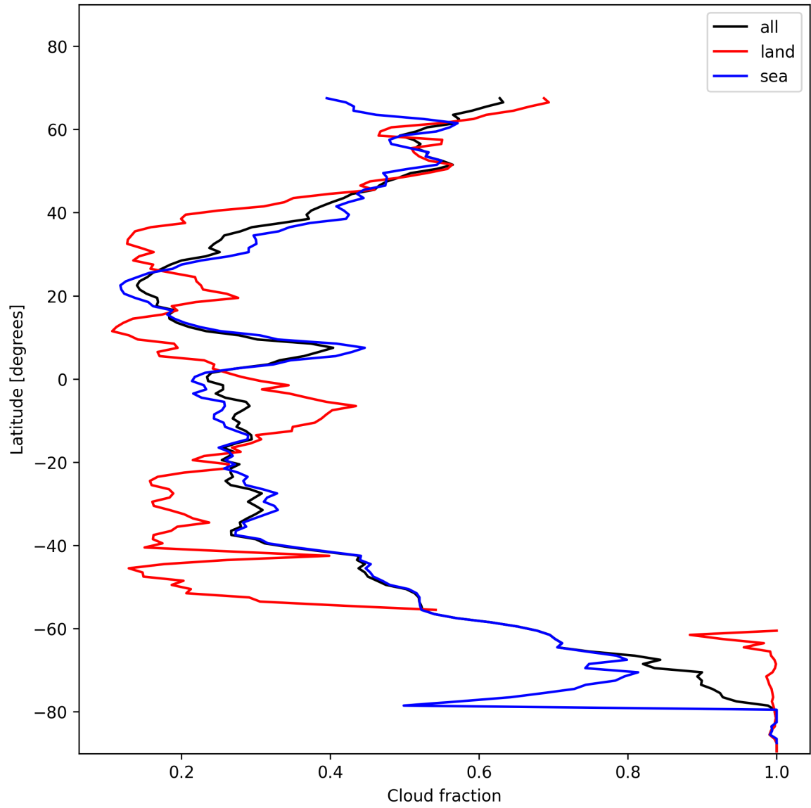
Figure 15: Zonal average of “Cloud fraction” for 2025-11-23 to 2025-11-25.
