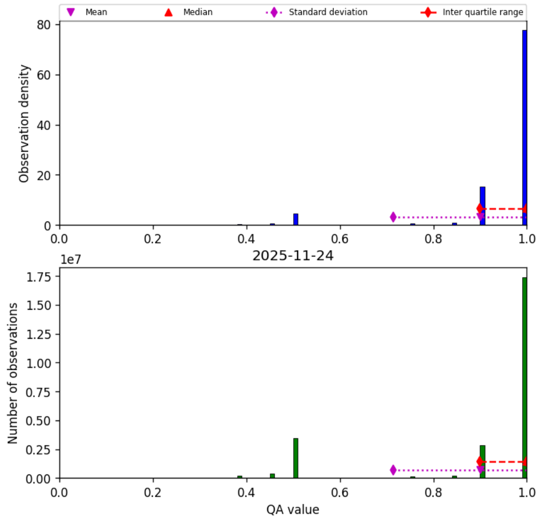
Figure 29: Histogram of “QA value” for 2025-11-23 to 2025-11-25
