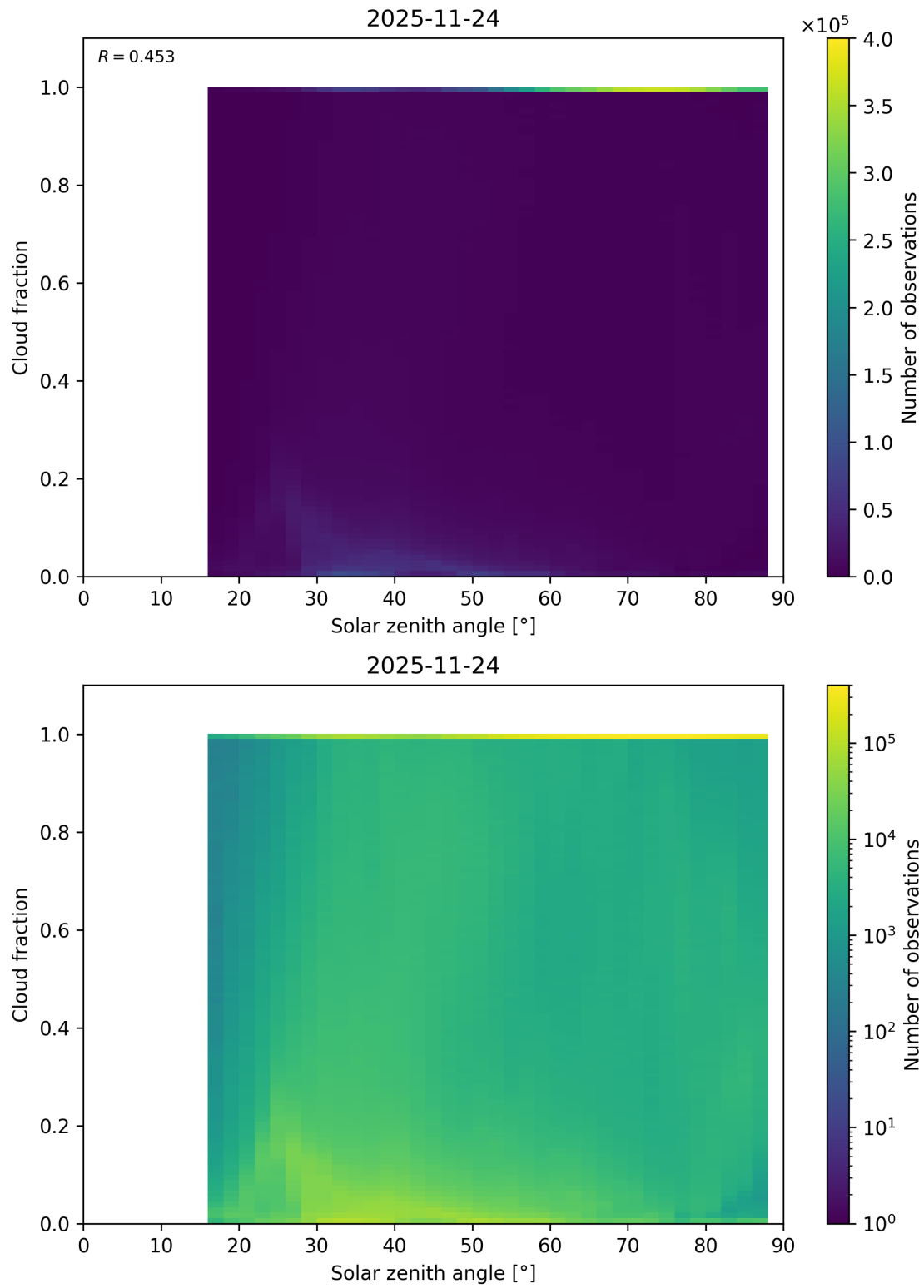
Figure 110: Scatter density plot of “Solar zenith angle” against “Cloud fraction” for 2025-11-23 to 2025-11-25.
