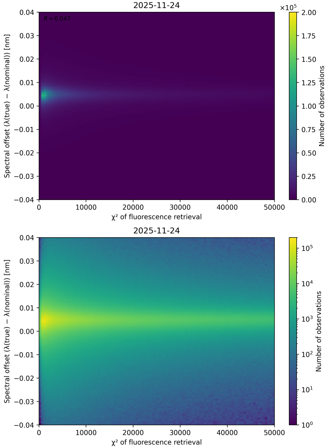
Figure 69: Scatter density plot of “ \chi^2 of fluorescence retrieval” against “Spectral offset ( \lambda_{\text{true}} - \lambda_{\text{nominal}} )” for 2025-11-23 to 2025-11-25.
