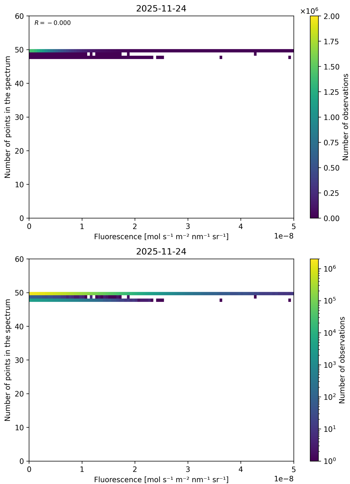
Figure 86: Scatter density plot of “Fluorescence” against “Number of points in the spectrum” for 2025-11-23 to 2025-11-25.
