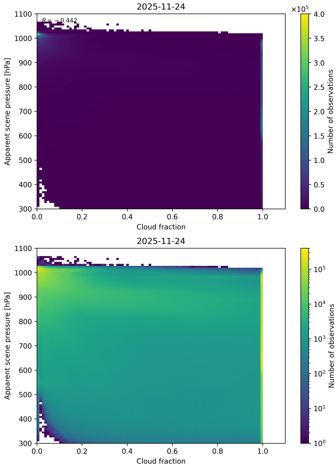
Figure 70: Scatter density plot of “Cloud fraction” against “Apparent scene pressure” for 2025-11-23 to 2025-11-25.
