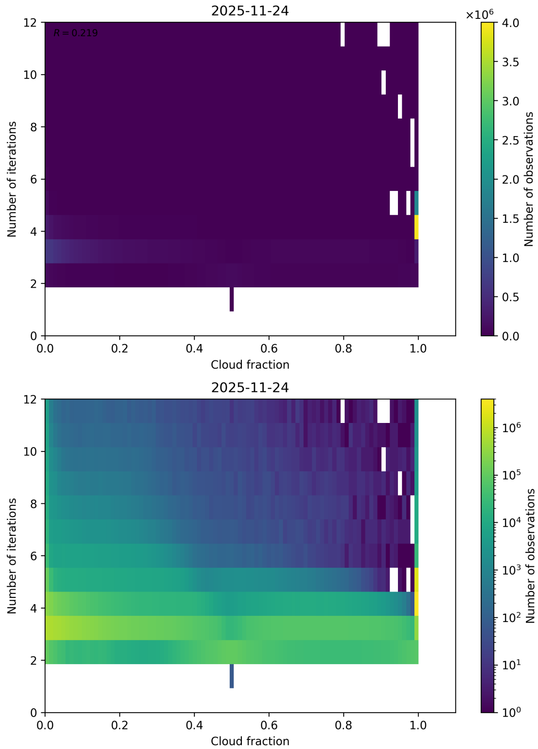
Figure 73: Scatter density plot of “Cloud fraction” against “Number of iterations” for 2025-11-23 to 2025-11-25.
