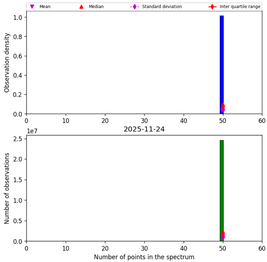
Figure 44: Histogram of “Number of points in the spectrum” for 2025-11-23 to 2025-11-25
