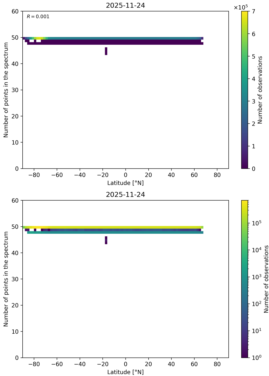
Figure 94: Scatter density plot of “Latitude” against “Number of points in the spectrum” for 2025-11-23 to 2025-11-25.
