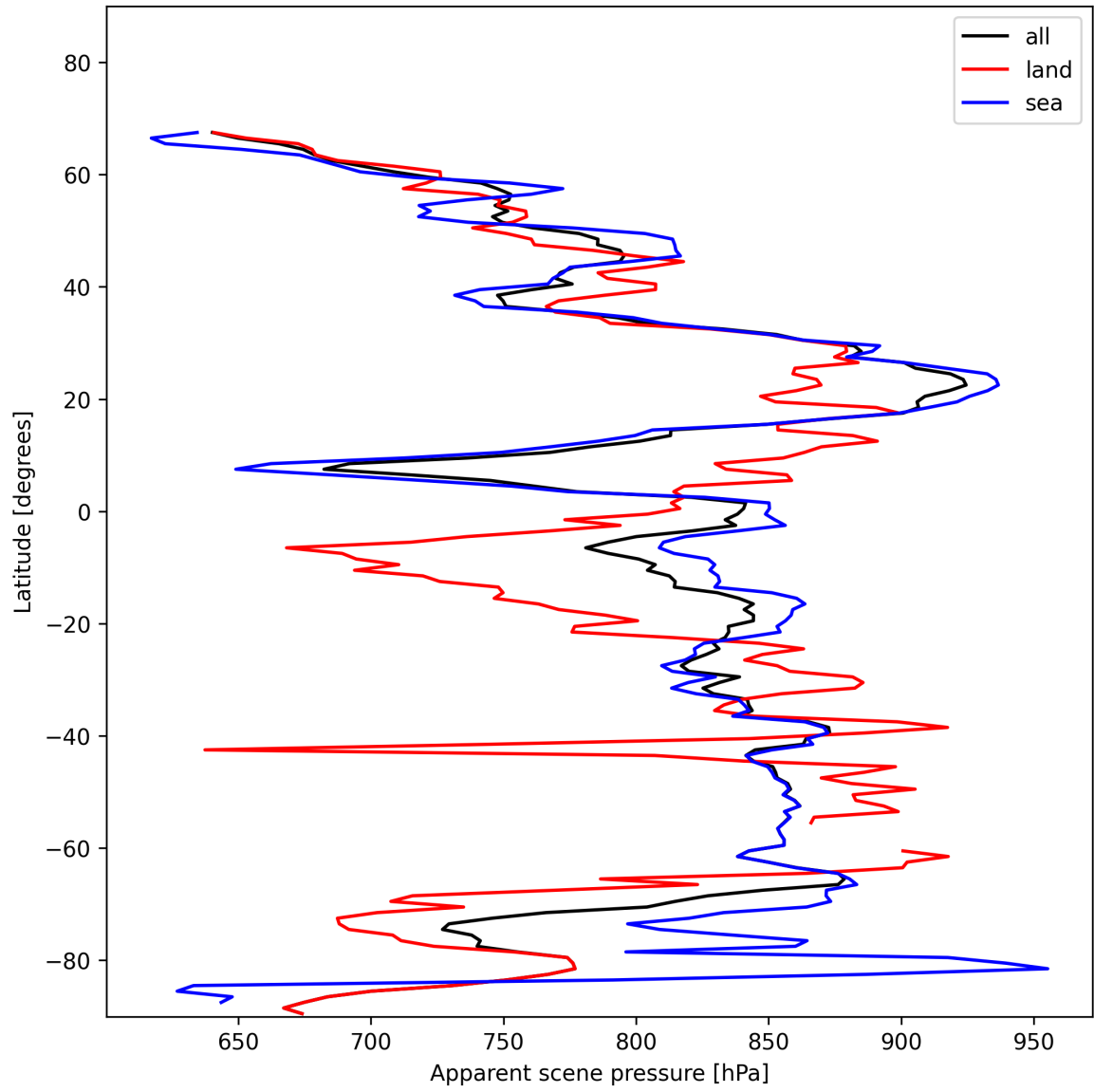
Figure 19: Zonal average of “Apparent scene pressure” for 2025-11-23 to 2025-11-25.
