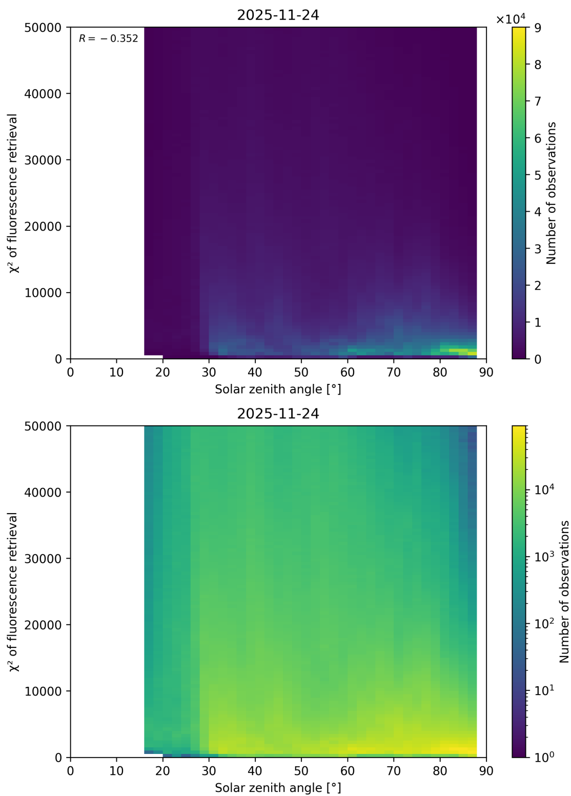
Figure 109: Scatter density plot of “Solar zenith angle” against “ \chi^2 of fluorescence retrieval” for 2025-11-23 to 2025-11-25.
