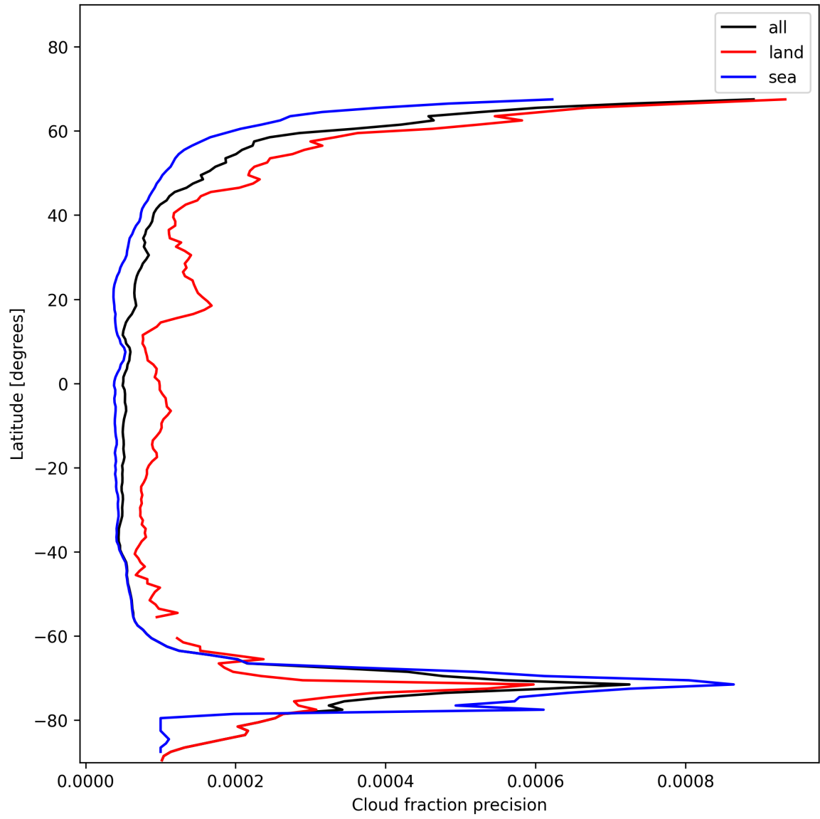
Figure 16: Zonal average of “Cloud fraction precision” for 2025-11-23 to 2025-11-25.
