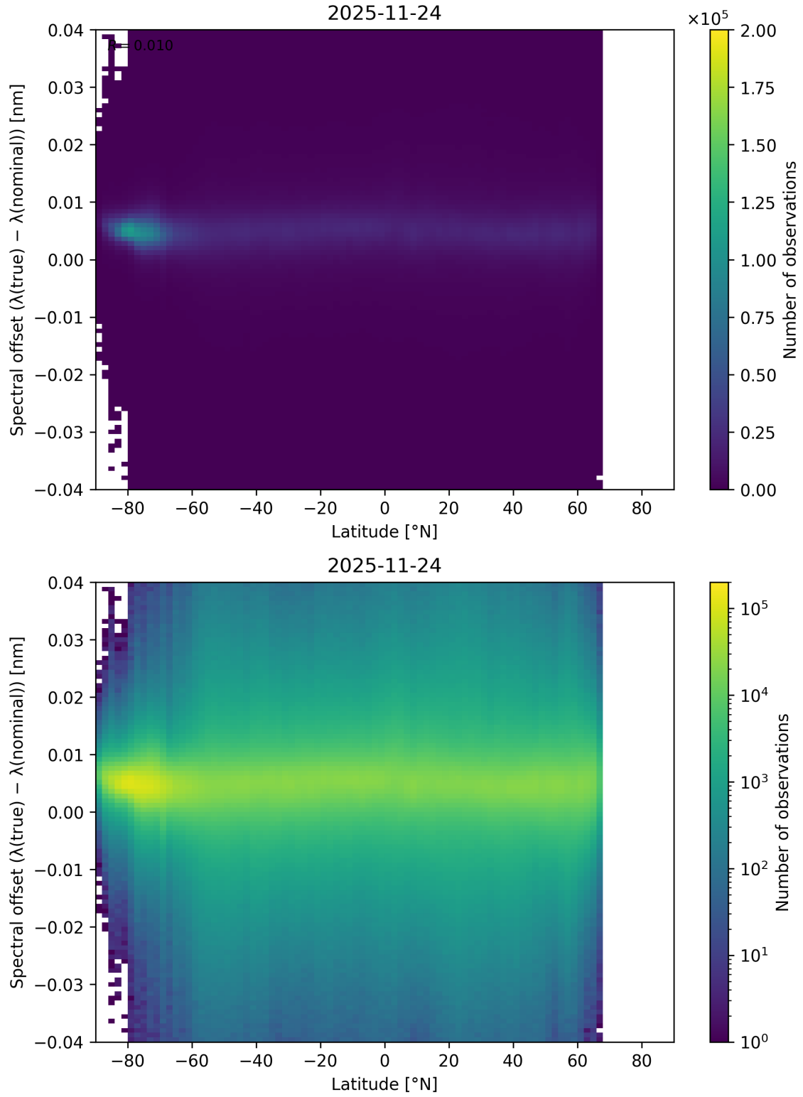
Figure 96: Scatter density plot of “Latitude” against “Spectral offset ( \lambda_{\text{true}} - \lambda_{\text{nominal}} )” for 2025-11-23 to 2025-11-25.
