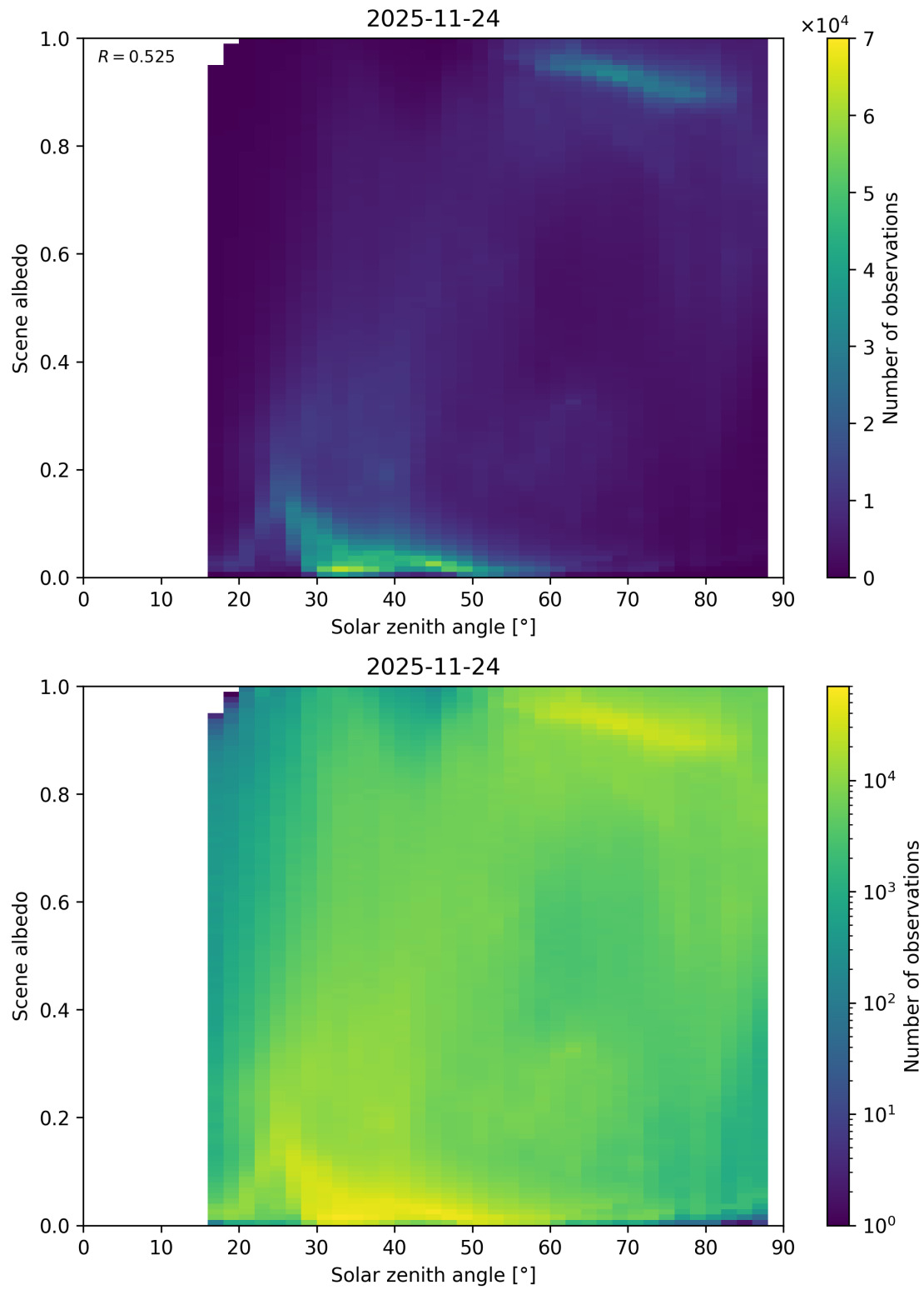
Figure 116: Scatter density plot of “Solar zenith angle” against “Scene albedo” for 2025-11-23 to 2025-11-25.
