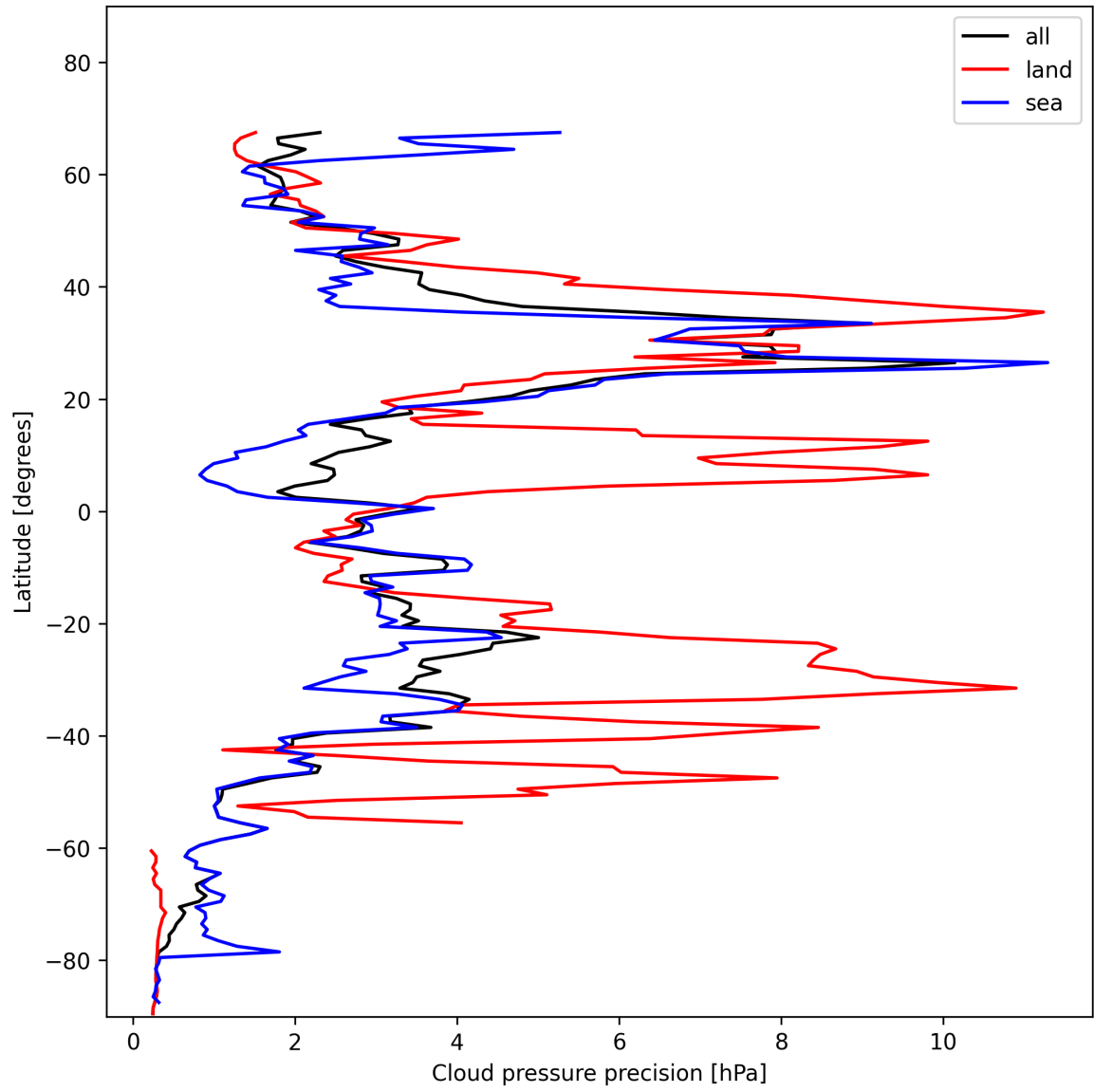
Figure 14: Zonal average of “Cloud pressure precision” for 2025-11-23 to 2025-11-25.
