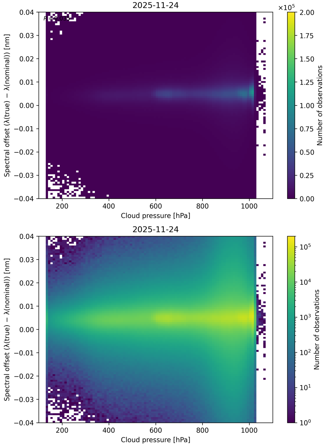
Figure 84: Scatter density plot of “Cloud pressure” against “Spectral offset ( \lambda_{\text{true}} - \lambda_{\text{nominal}} )” for 2025-11-23 to 2025-11-25.
