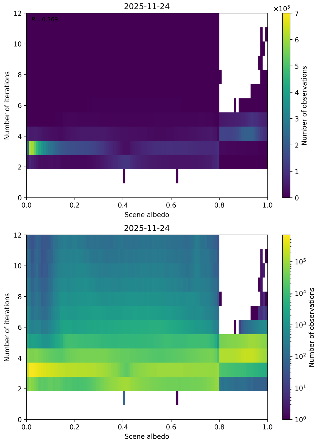
Figure 105: Scatter density plot of “Scene albedo” against “Number of iterations” for 2025-11-23 to 2025-11-25.
