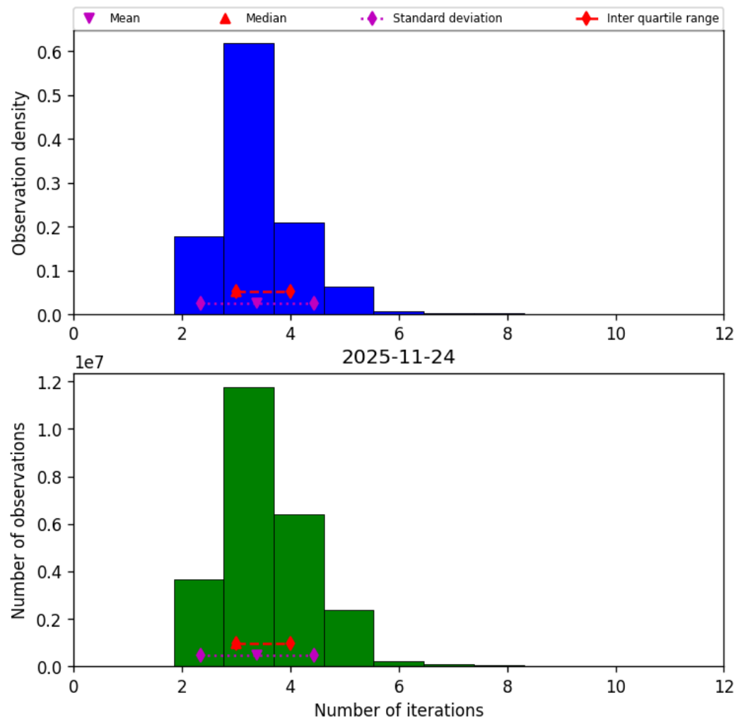
Figure 39: Histogram of “Number of iterations” for 2025-11-23 to 2025-11-25
