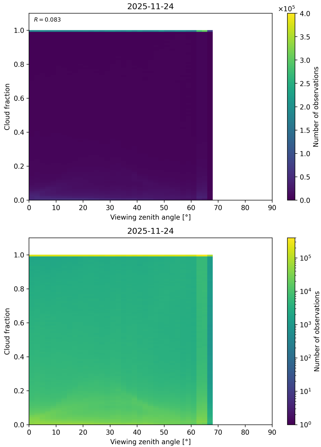
Figure 120: Scatter density plot of “Viewing zenith angle” against “Cloud fraction” for 2025-11-23 to 2025-11-25.
