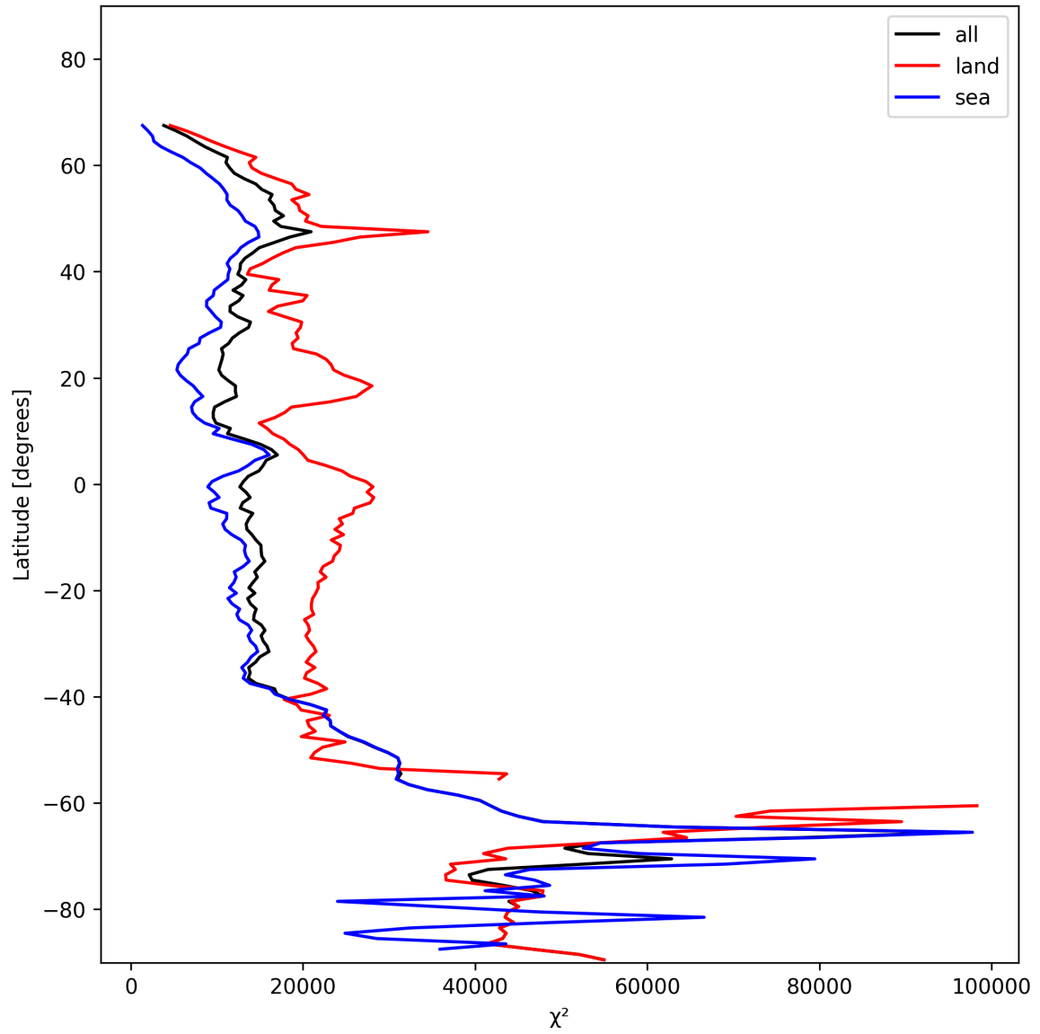
Figure 21: Zonal average of “ \chi^2 ” for 2025-11-23 to 2025-11-25.
