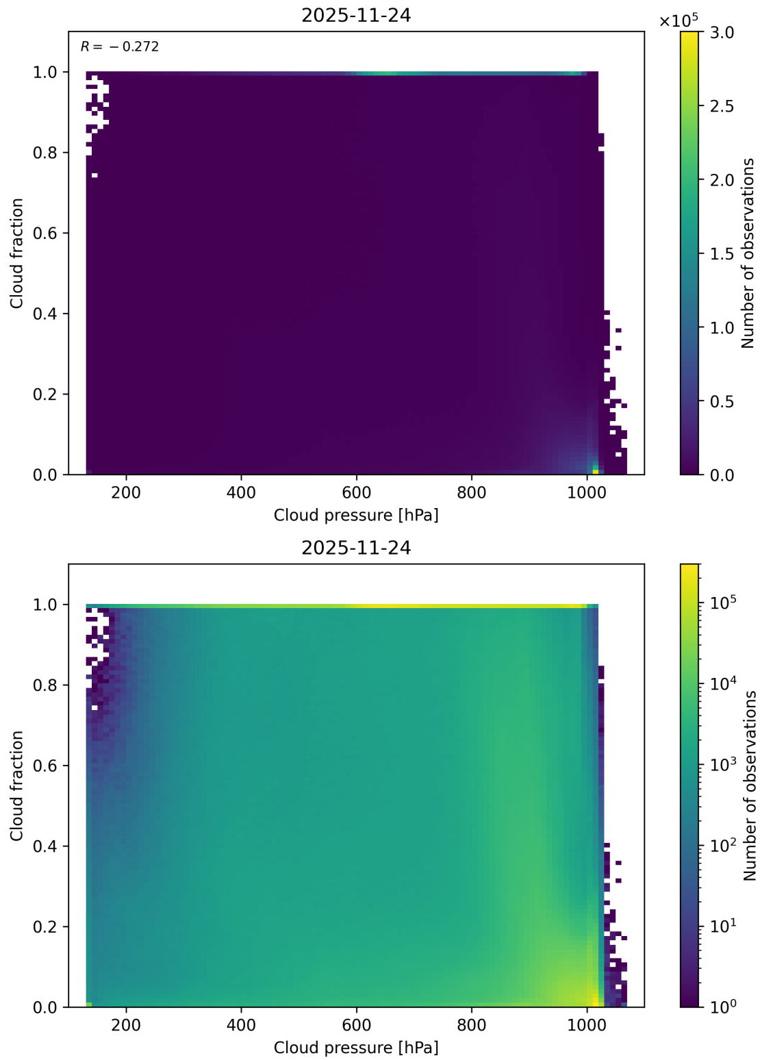
Figure 79: Scatter density plot of “Cloud pressure” against “Cloud fraction” for 2025-11-23 to 2025-11-25.
