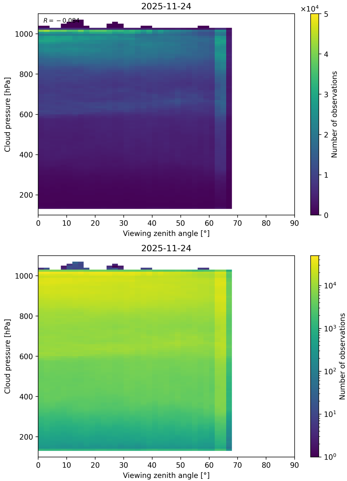
Figure 121: Scatter density plot of “Viewing zenith angle” against “Cloud pressure” for 2025-11-23 to 2025-11-25.
