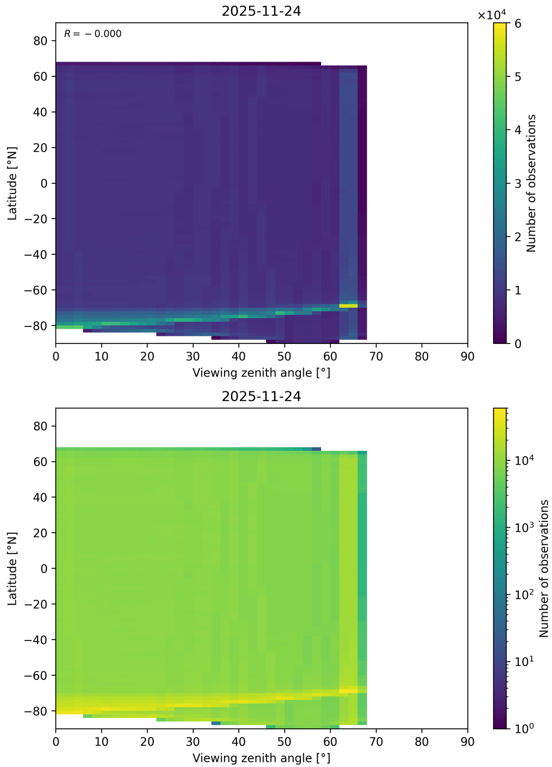
Figure 123: Scatter density plot of “Viewing zenith angle” against “Latitude” for 2025-11-23 to 2025-11-25.
