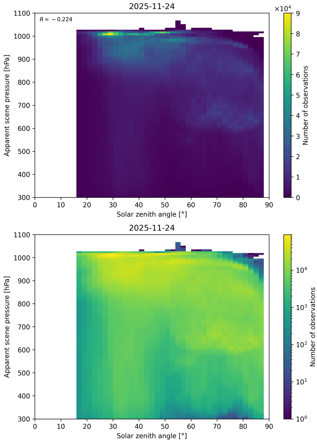
Figure 108: Scatter density plot of “Solar zenith angle” against “Apparent scene pressure” for 2025-11-23 to 2025-11-25.
