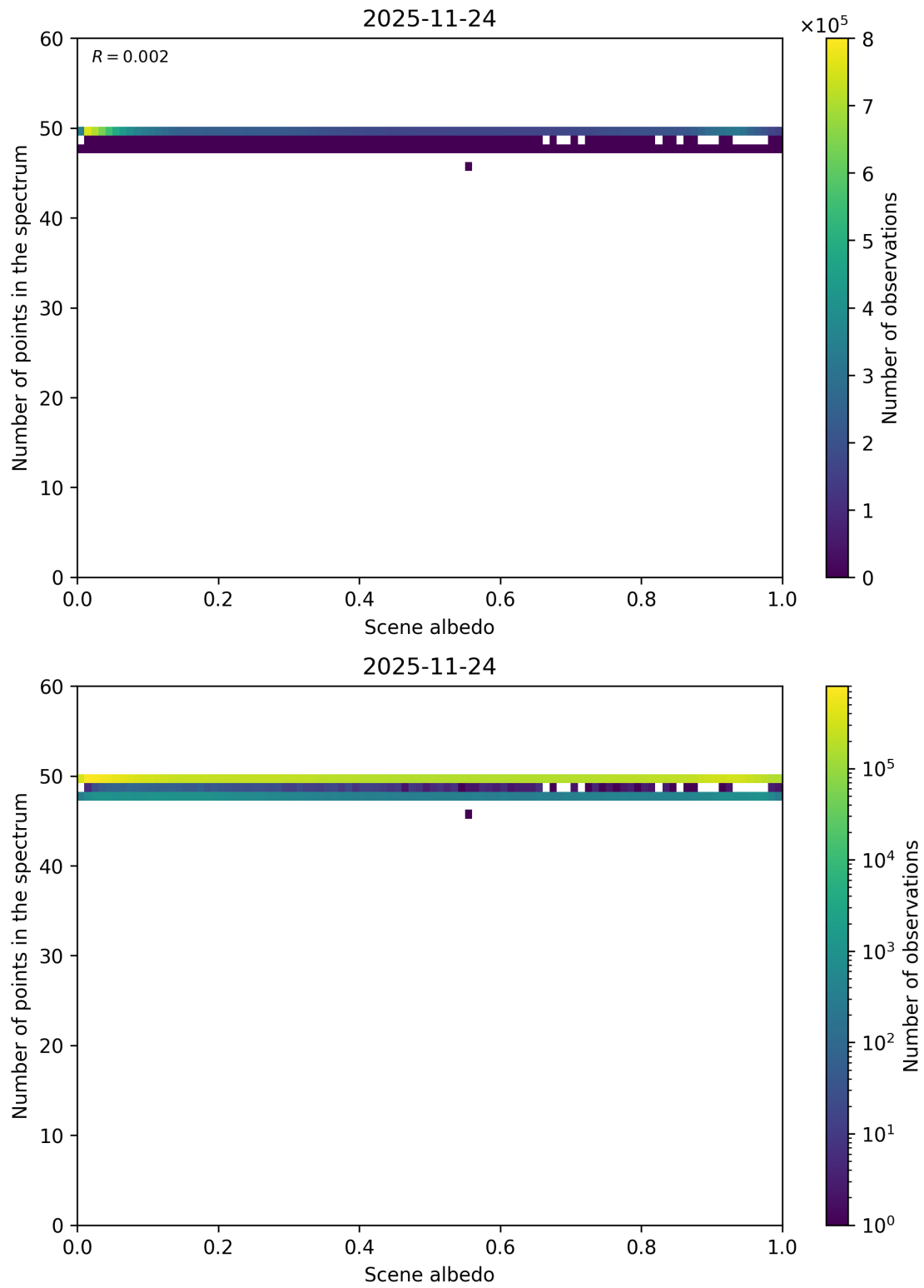
Figure 106: Scatter density plot of “Scene albedo” against “Number of points in the spectrum” for 2025-11-23 to 2025-11-25.
