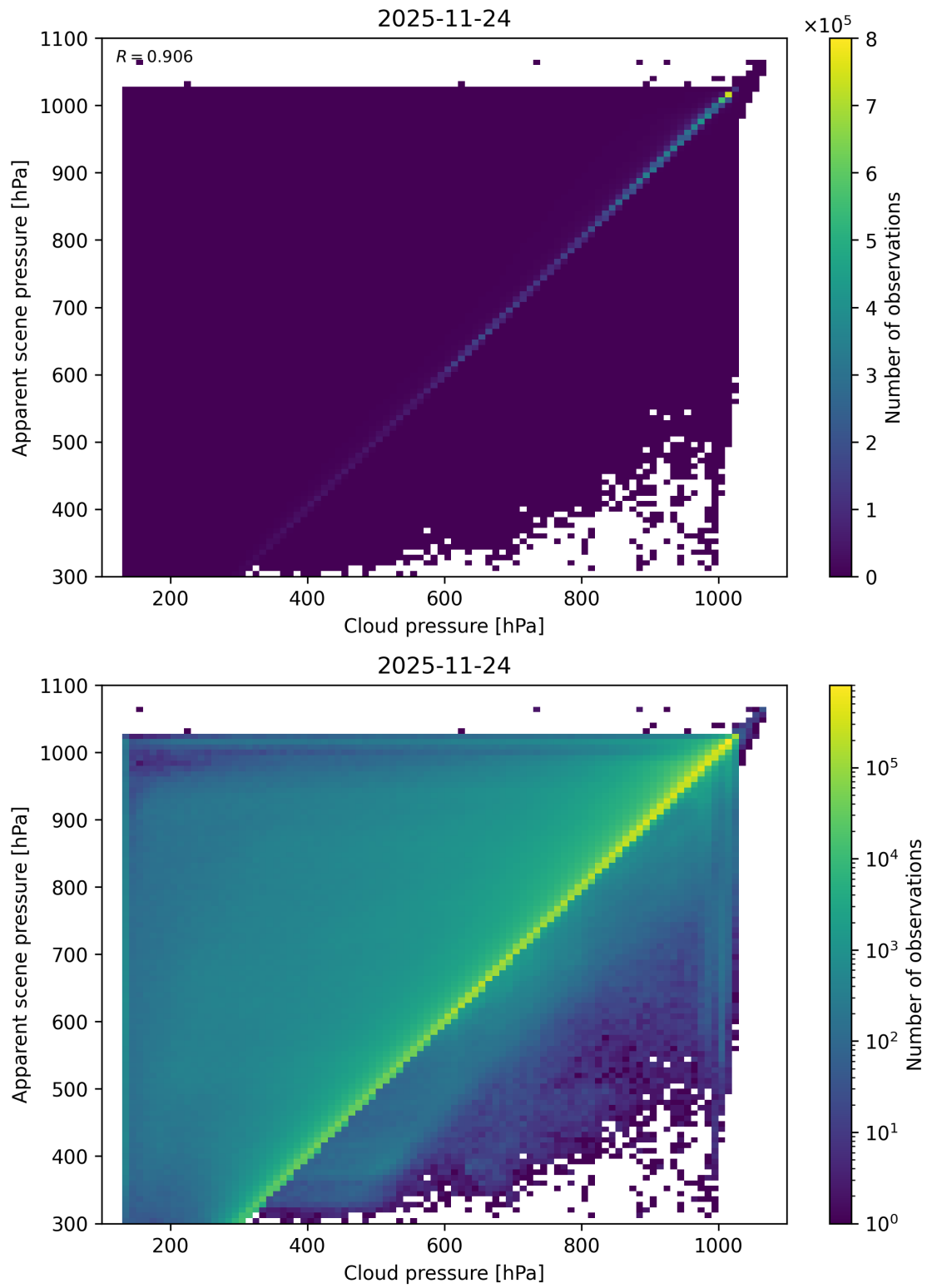
Figure 77: Scatter density plot of “Cloud pressure” against “Apparent scene pressure” for 2025-11-23 to 2025-11-25.
