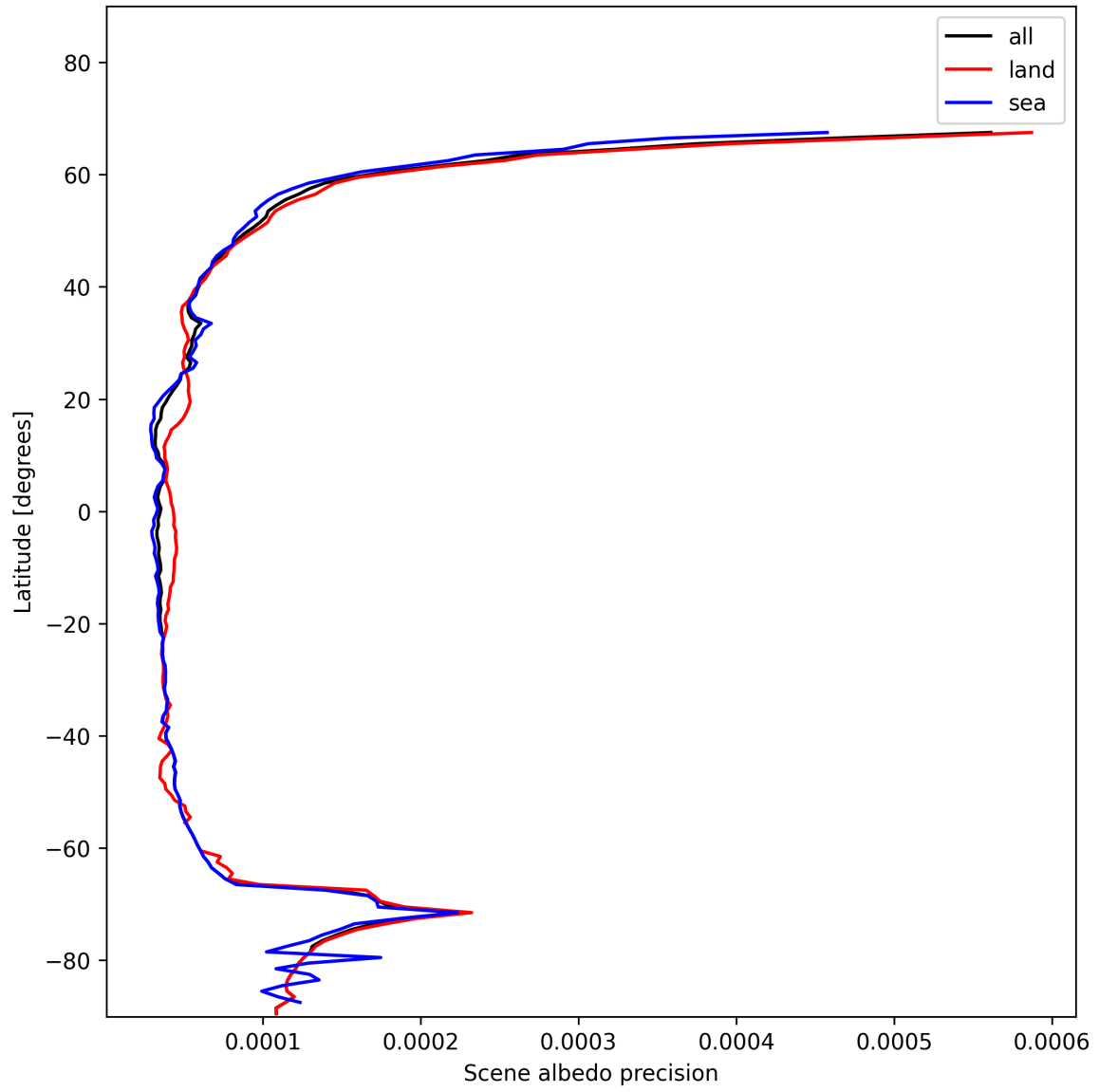
Figure 18: Zonal average of “Scene albedo precision” for 2025-11-23 to 2025-11-25.
