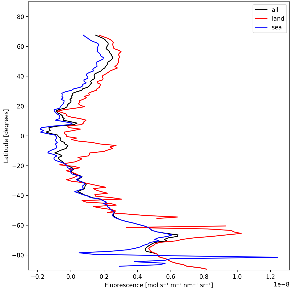
Figure 23: Zonal average of “Fluorescence” for 2025-11-23 to 2025-11-25.
