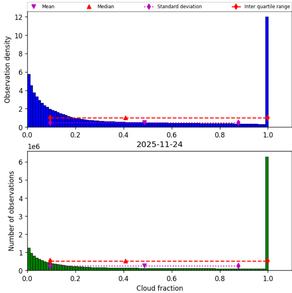
Figure 32: Histogram of “Cloud fraction” for 2025-11-23 to 2025-11-25
