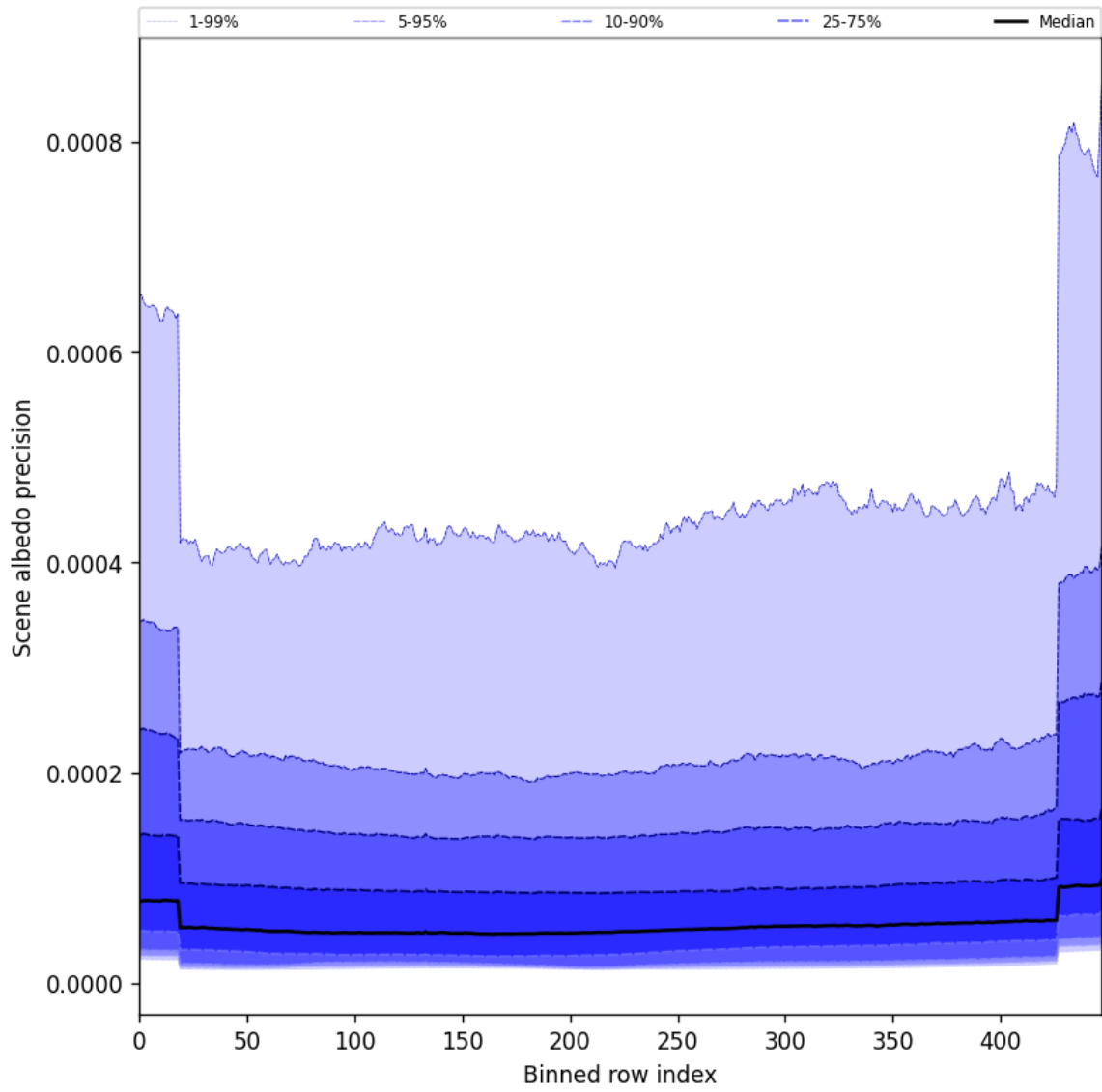
Figure 52: Along track statistics of “Scene albedo precision” for 2025-11-23 to 2025-11-25
