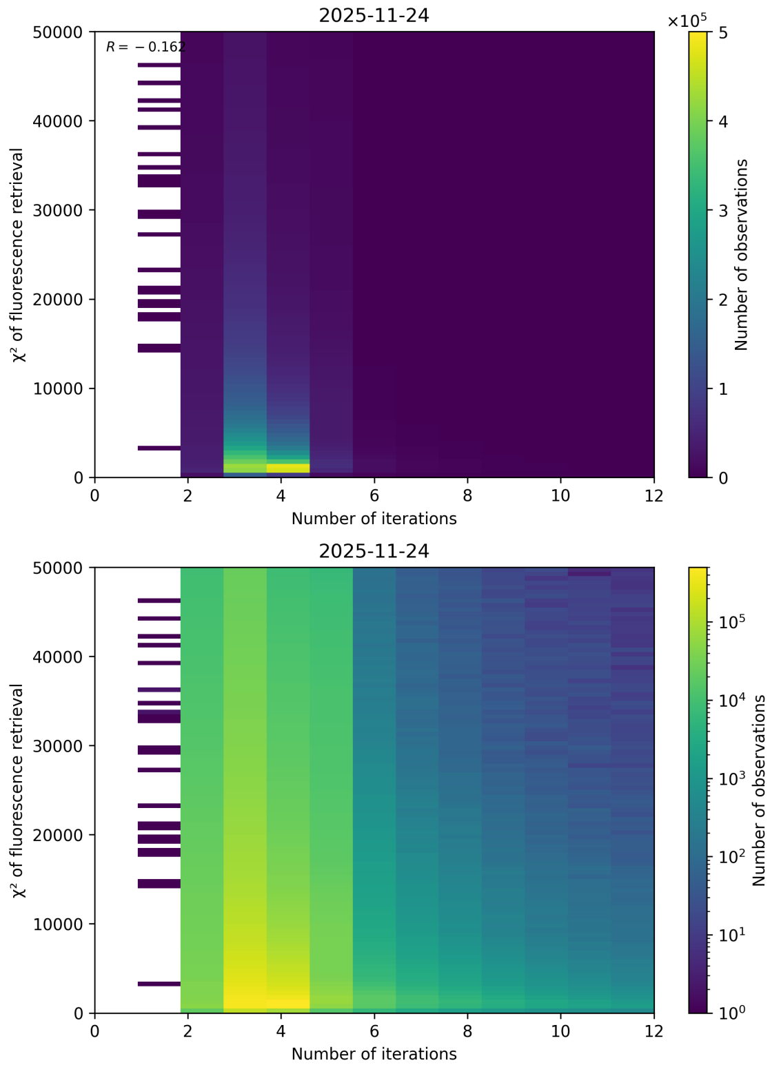
Figure 97: Scatter density plot of “Number of iterations” against “ \chi^2 of fluorescence retrieval” for 2025-11-23 to 2025-11-25.
