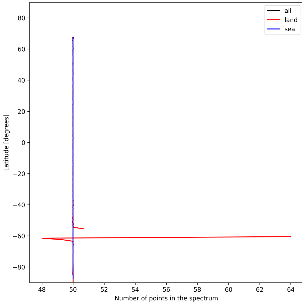
Figure 27: Zonal average of “Number of points in the spectrum” for 2025-11-23 to 2025-11-25.
