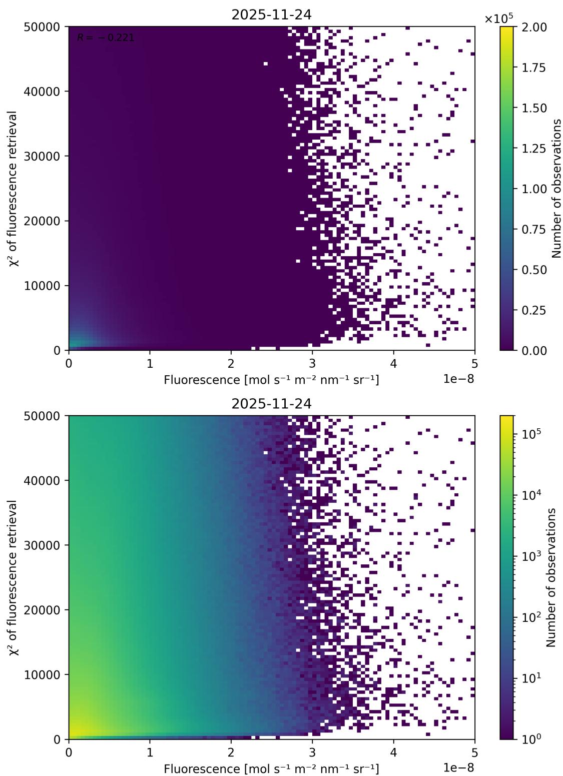
Figure 85: Scatter density plot of “Fluorescence” against “ \chi^2 of fluorescence retrieval” for 2025-11-23 to 2025-11-25.
