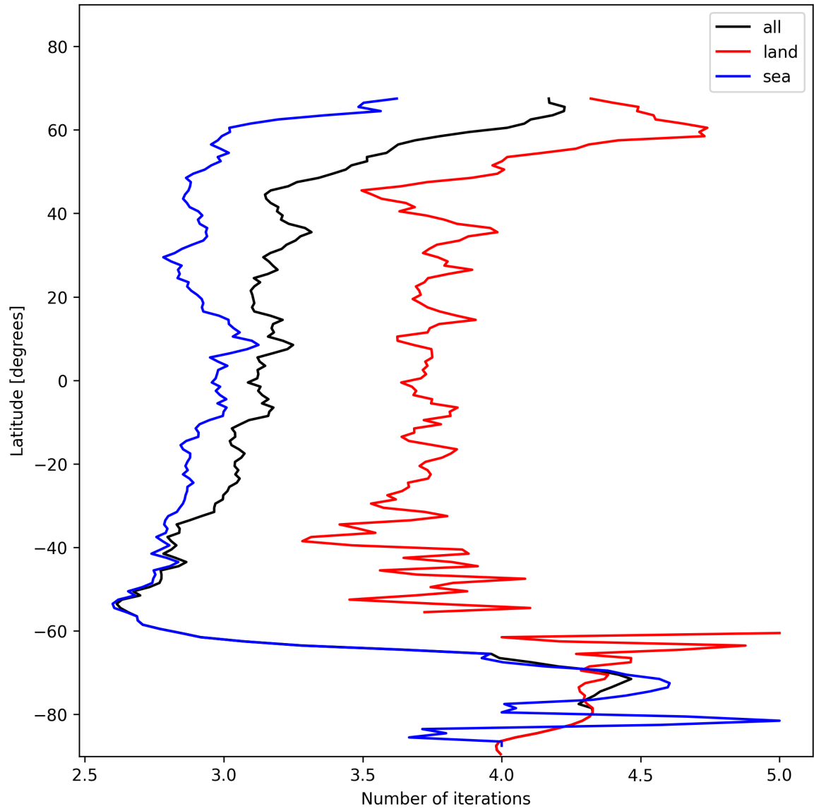
Figure 22: Zonal average of “Number of iterations” for 2025-11-23 to 2025-11-25.
