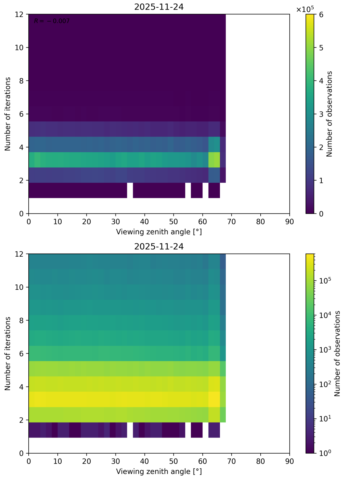
Figure 124: Scatter density plot of “Viewing zenith angle” against “Number of iterations” for 2025-11-23 to 2025-11-25.
