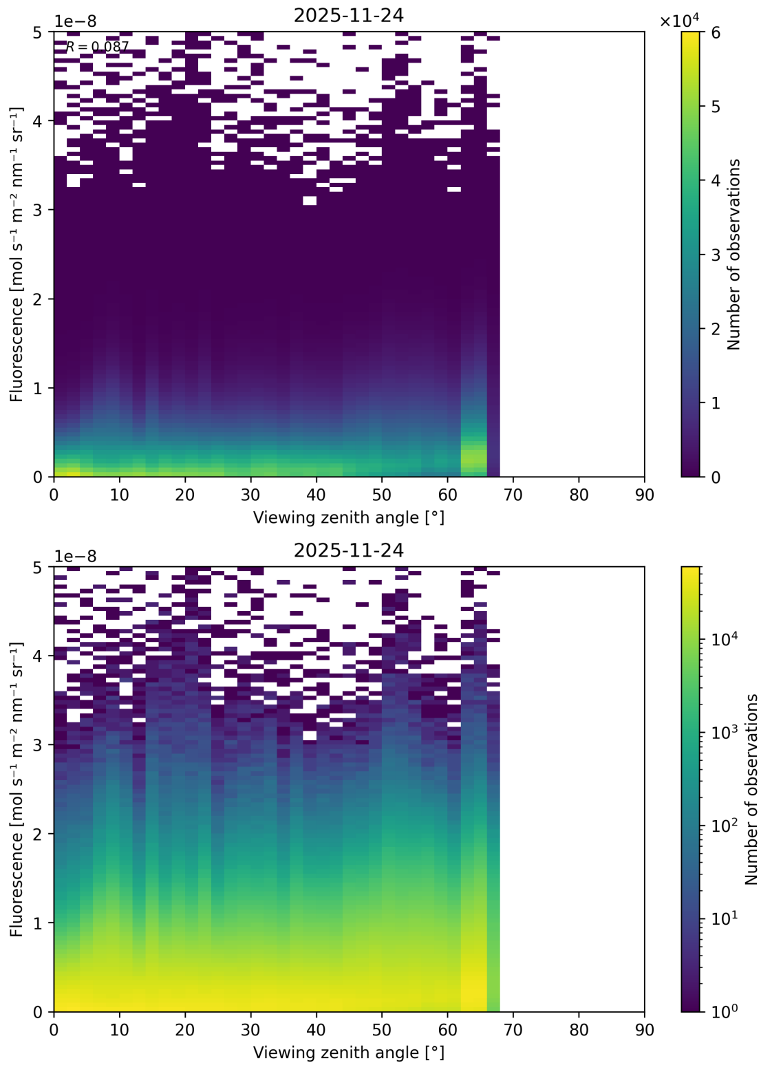
Figure 122: Scatter density plot of “Viewing zenith angle” against “Fluorescence” for 2025-11-23 to 2025-11-25.
