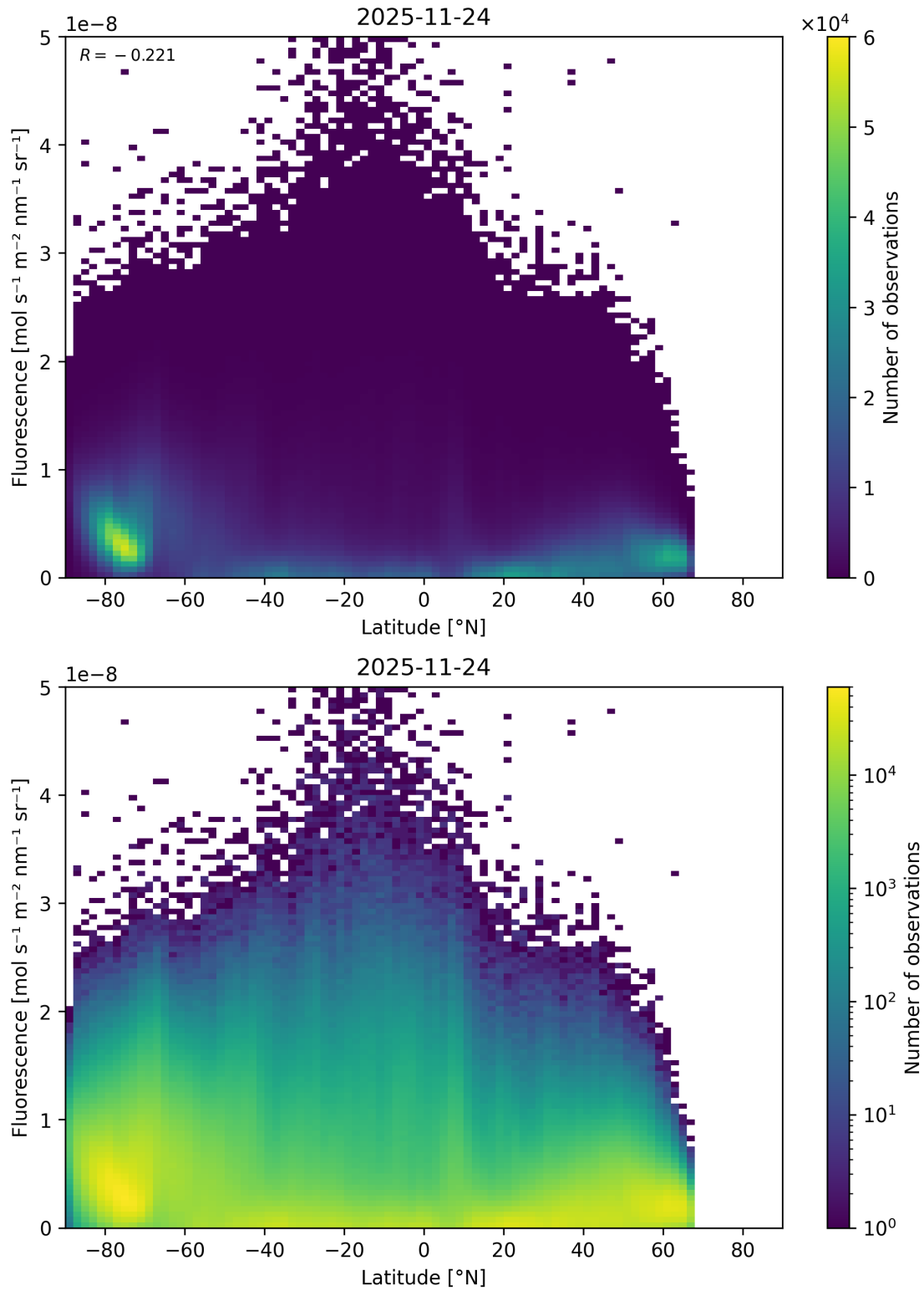
Figure 92: Scatter density plot of “Latitude” against “Fluorescence” for 2025-11-23 to 2025-11-25.
