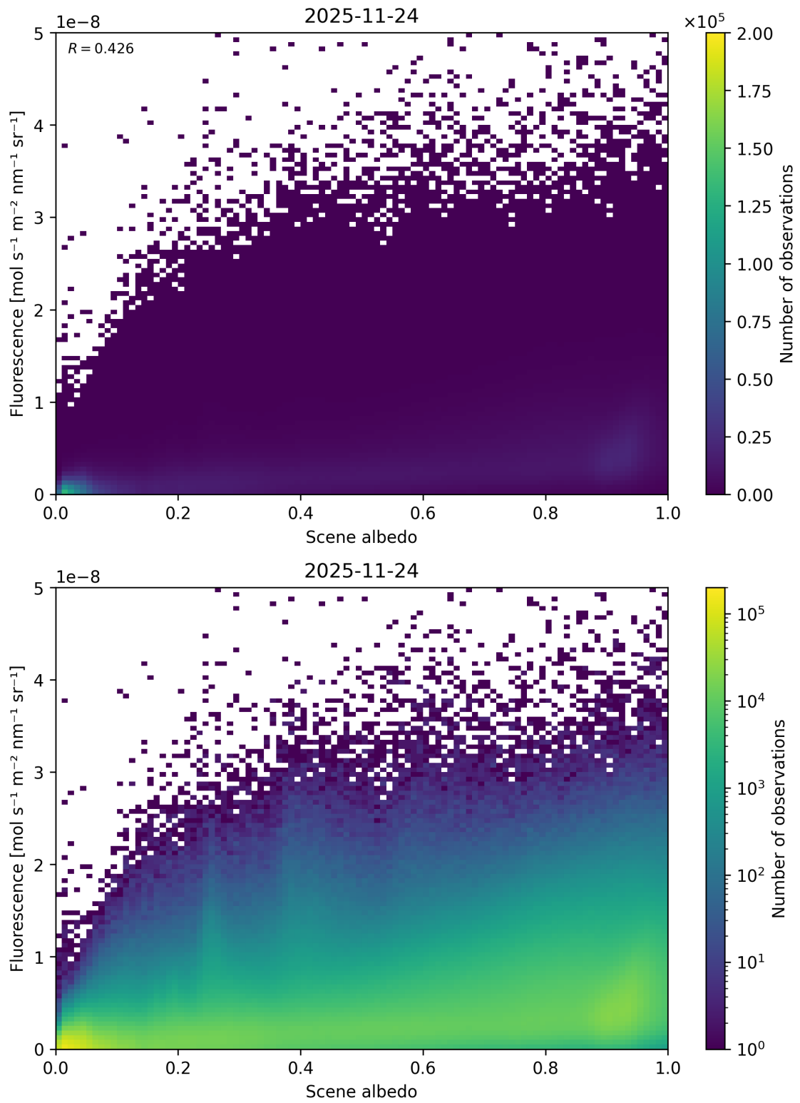
Figure 104: Scatter density plot of “Scene albedo” against “Fluorescence” for 2025-11-23 to 2025-11-25.
