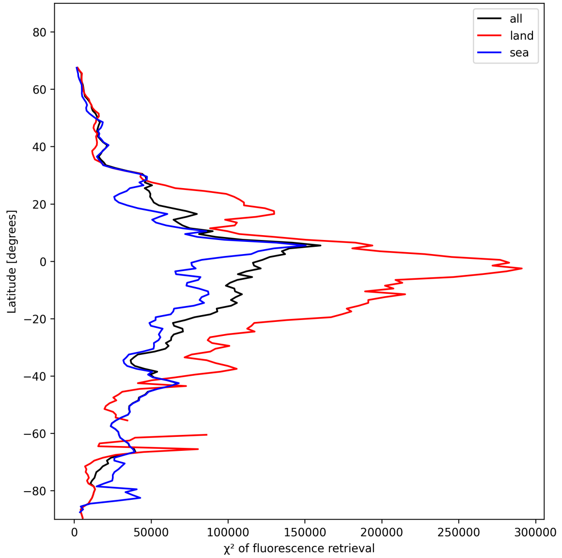
Figure 25: Zonal average of “ \chi^2 of fluorescence retrieval” for 2025-11-23 to 2025-11-25.
