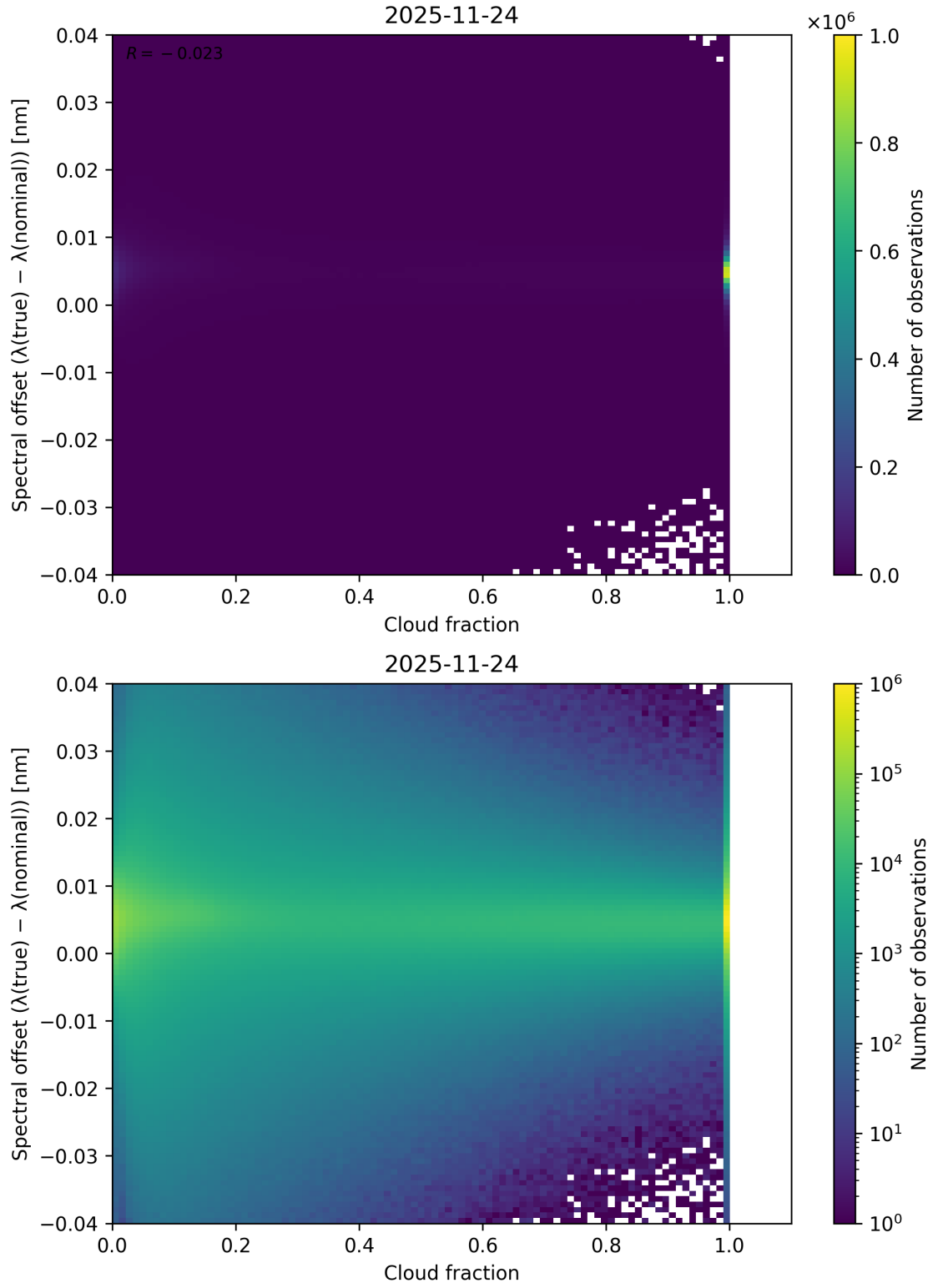
Figure 76: Scatter density plot of “Cloud fraction” against “Spectral offset ( \lambda_{\text{true}} - \lambda_{\text{nominal}} )” for 2025-11-23 to 2025-11-25.
