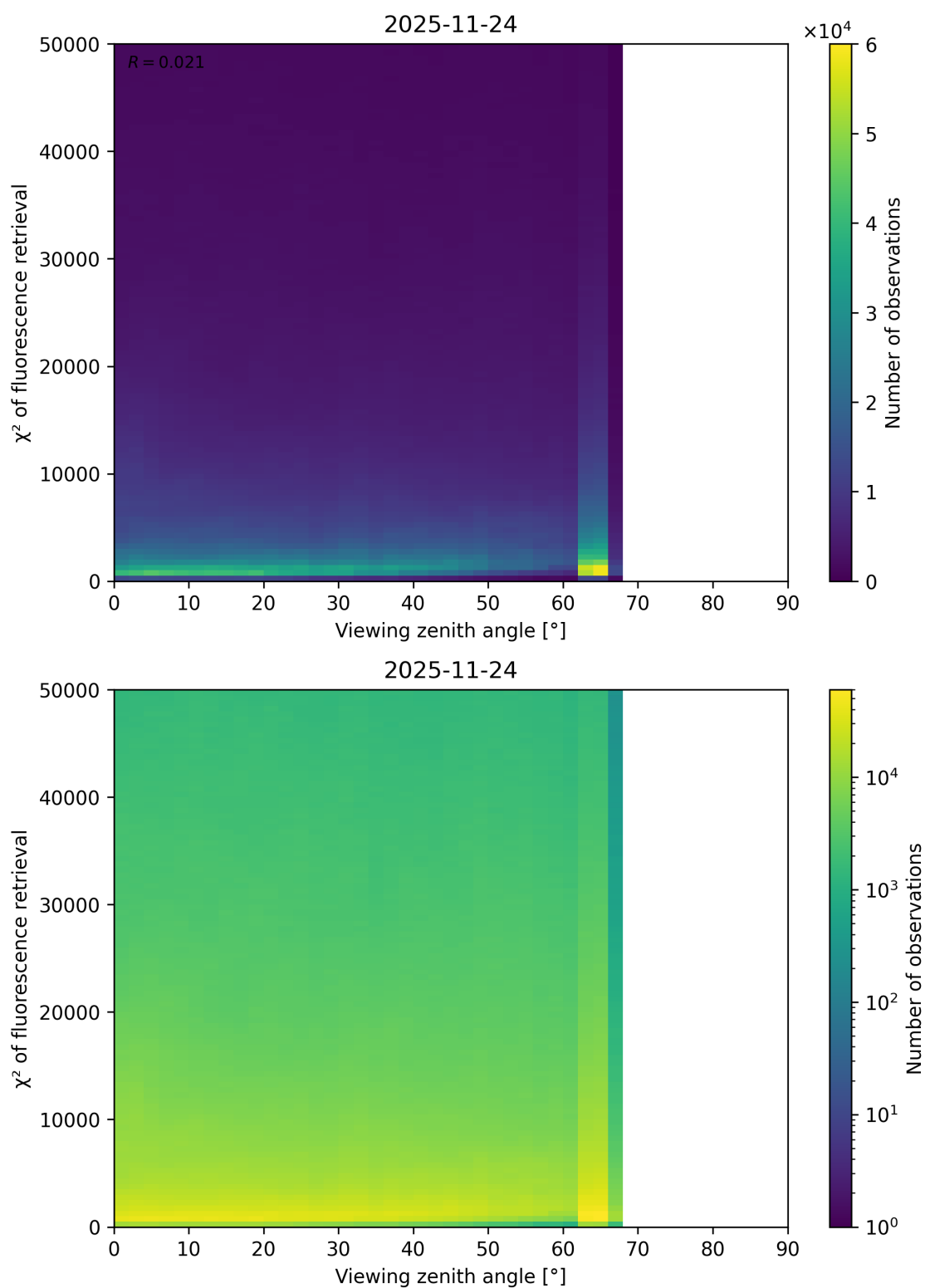
Figure 119: Scatter density plot of “Viewing zenith angle” against “ \chi^2 of fluorescence retrieval” for 2025-11-23 to 2025-11-25.
