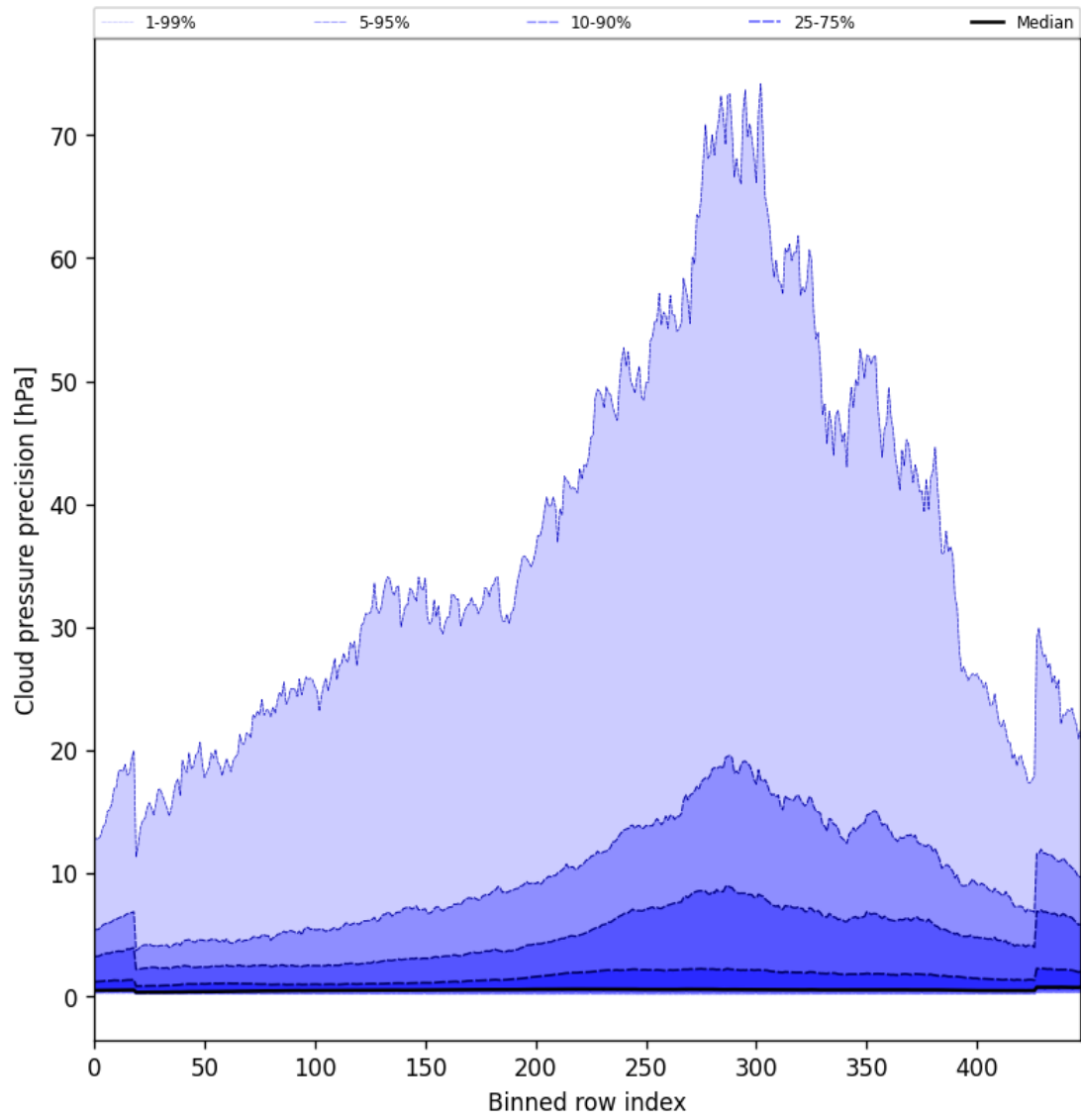
Figure 48: Along track statistics of “Cloud pressure precision” for 2025-11-23 to 2025-11-25
