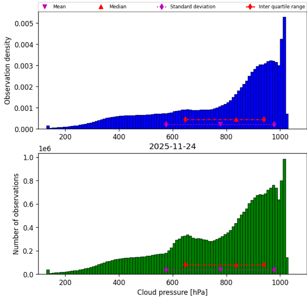
Figure 30: Histogram of “Cloud pressure” for 2025-11-23 to 2025-11-25
