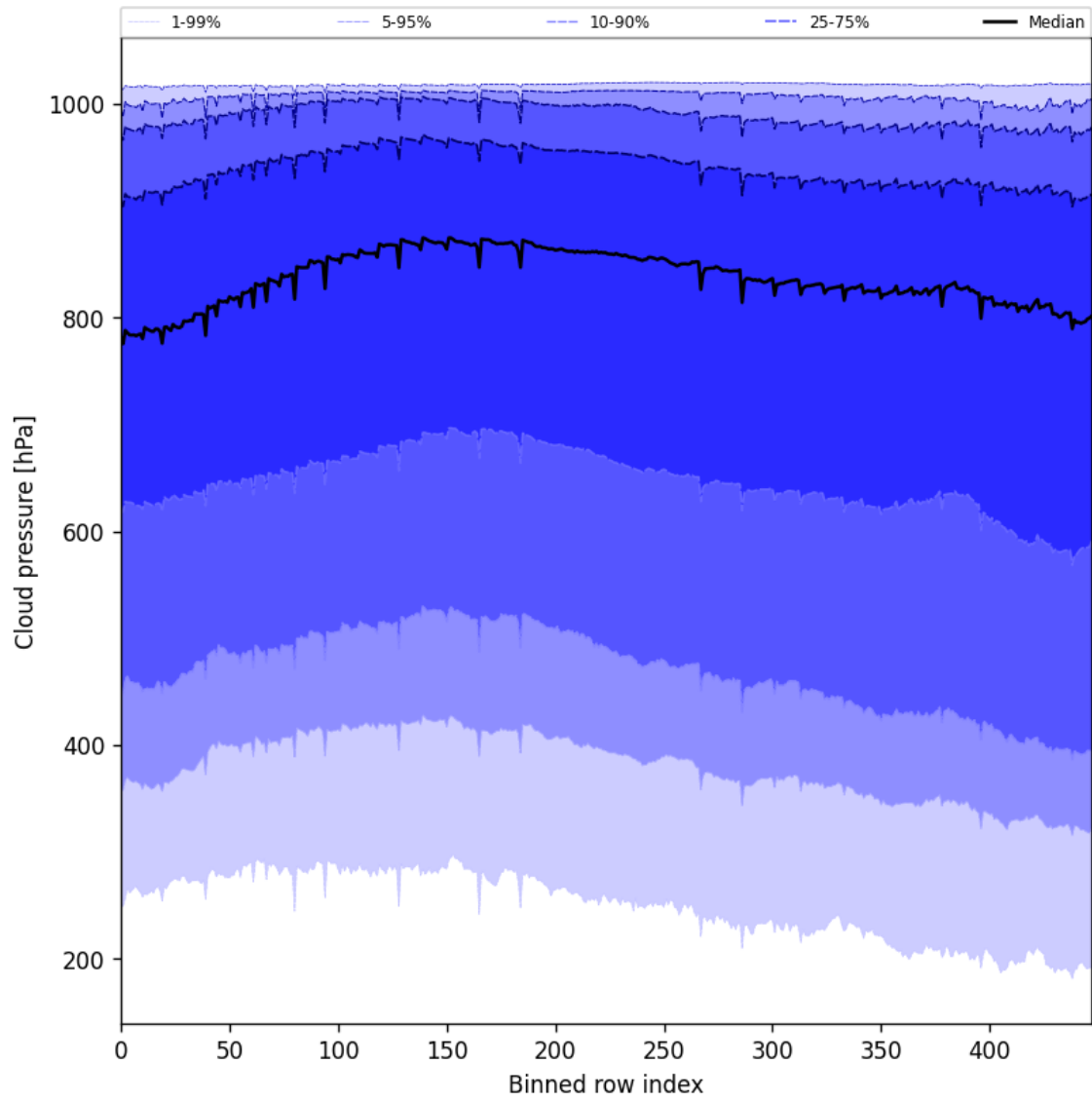
Figure 47: Along track statistics of “Cloud pressure” for 2025-11-23 to 2025-11-25
