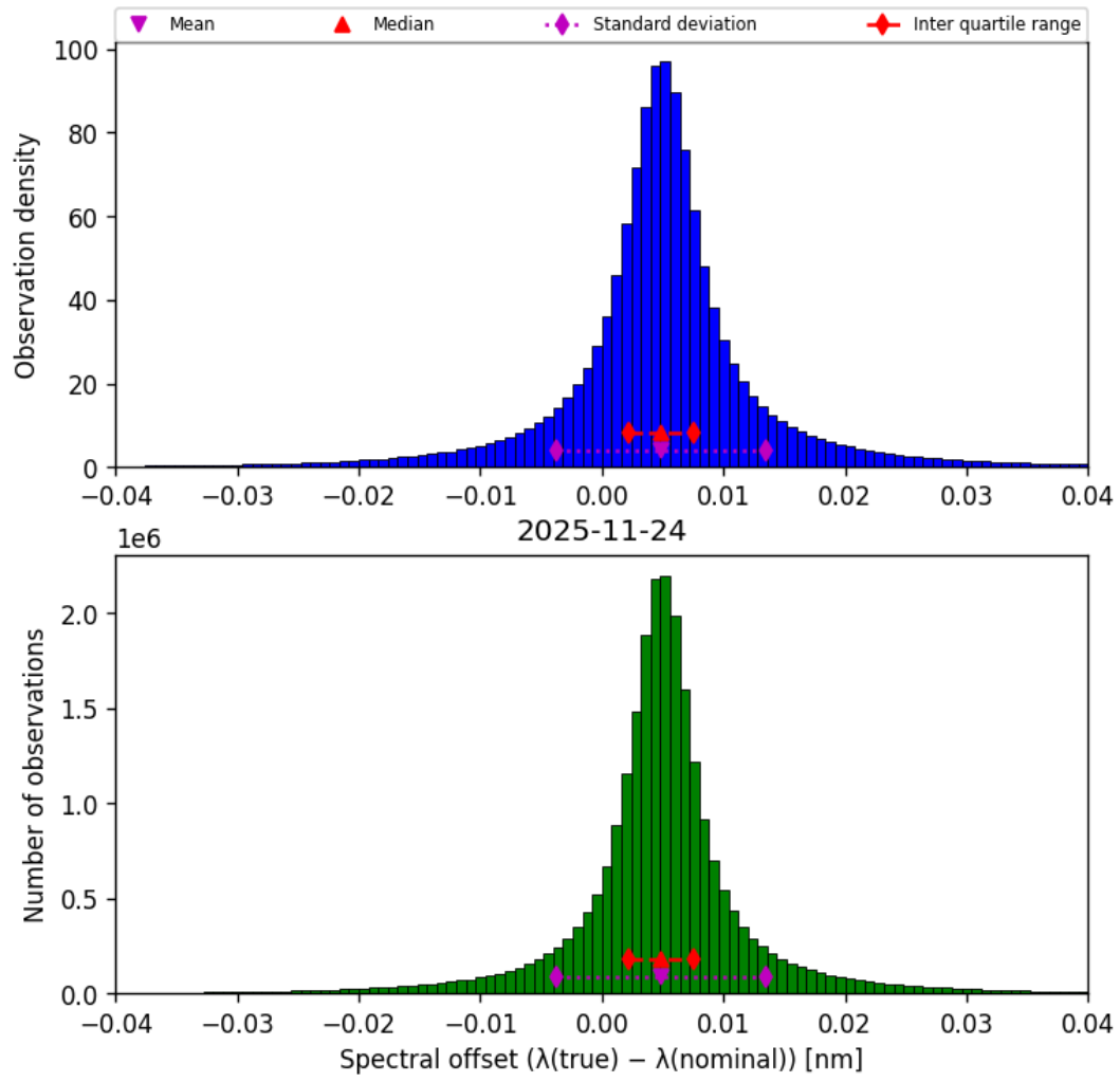
Figure 45: Histogram of “Spectral offset ( \lambda_{\text{true}} - \lambda_{\text{nominal}} )” for 2025-11-23 to 2025-11-25
