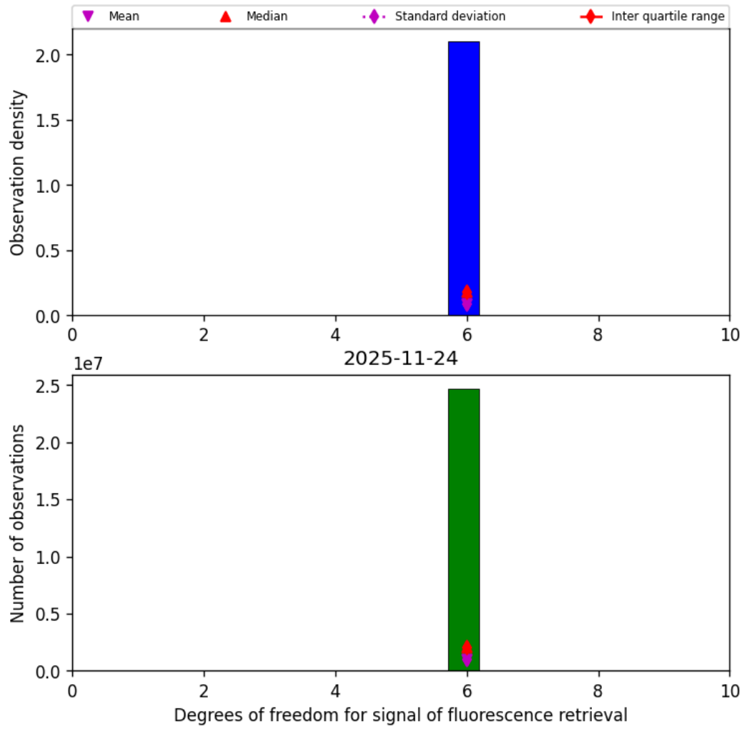
Figure 43: Histogram of "Degrees of freedom for signal of fluorescence retrieval" for 2025-11-23 to 2025-11-25
