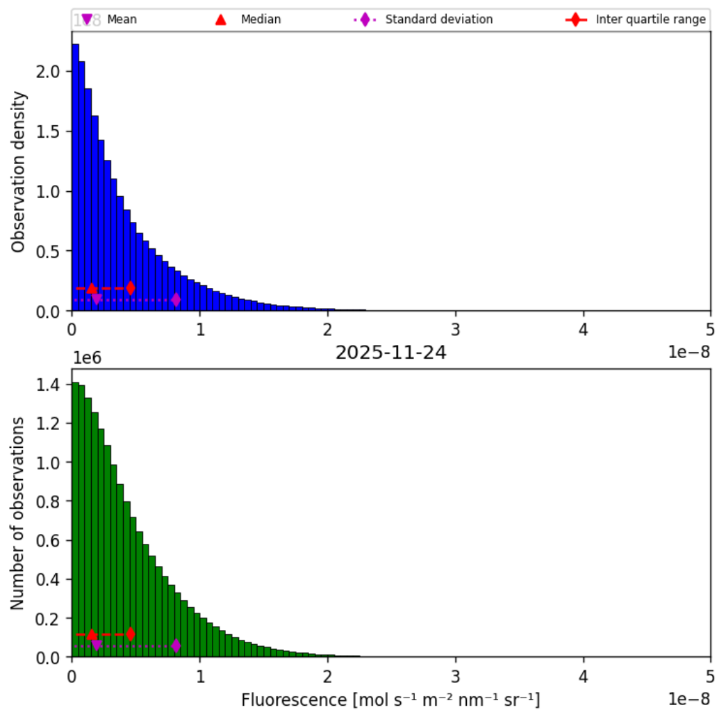
Figure 40: Histogram of “Fluorescence” for 2025-11-23 to 2025-11-25
