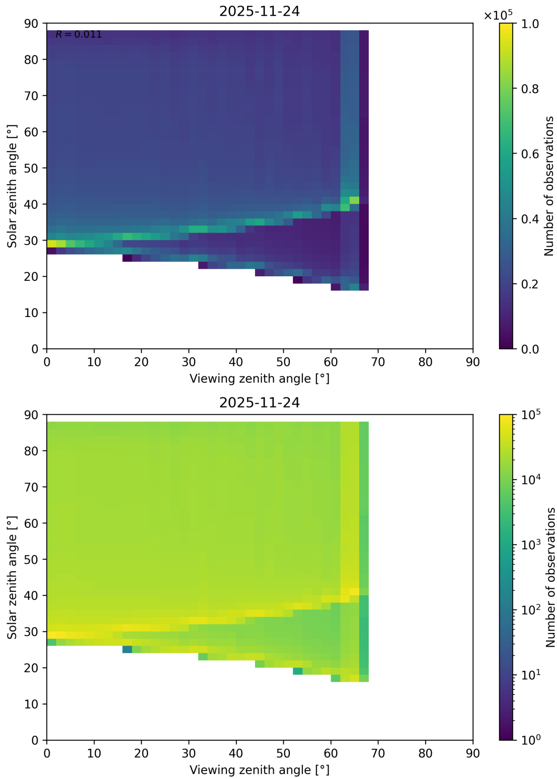
Figure 127: Scatter density plot of “Viewing zenith angle” against “Solar zenith angle” for 2025-11-23 to 2025-11-25.
