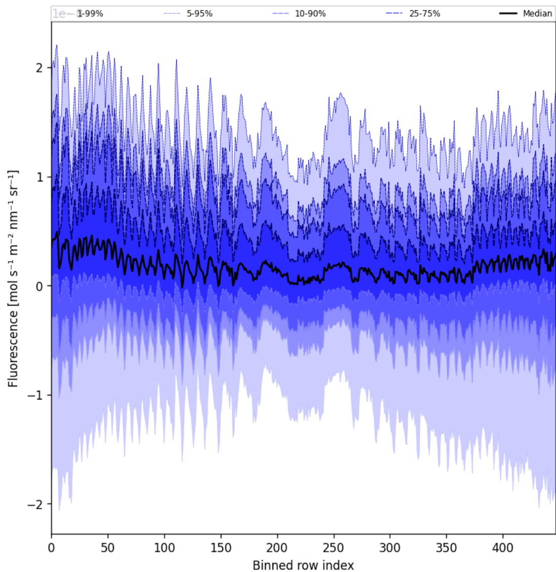
Figure 57: Along track statistics of “Fluorescence” for 2025-11-23 to 2025-11-25
