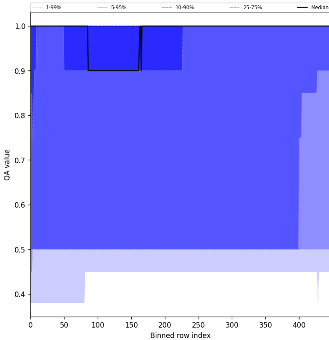
Figure 46: Along track statistics of “QA value” for 2025-11-23 to 2025-11-25
