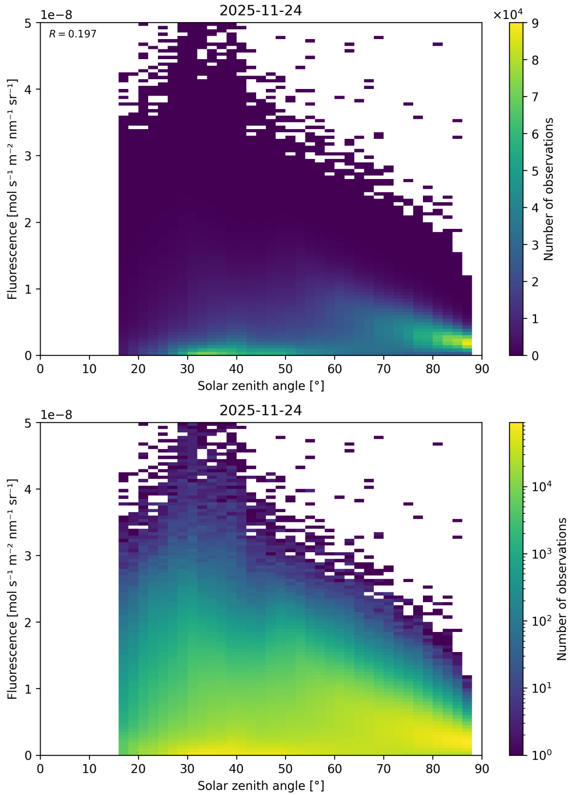
Figure 112: Scatter density plot of “Solar zenith angle” against “Fluorescence” for 2025-11-23 to 2025-11-25.
