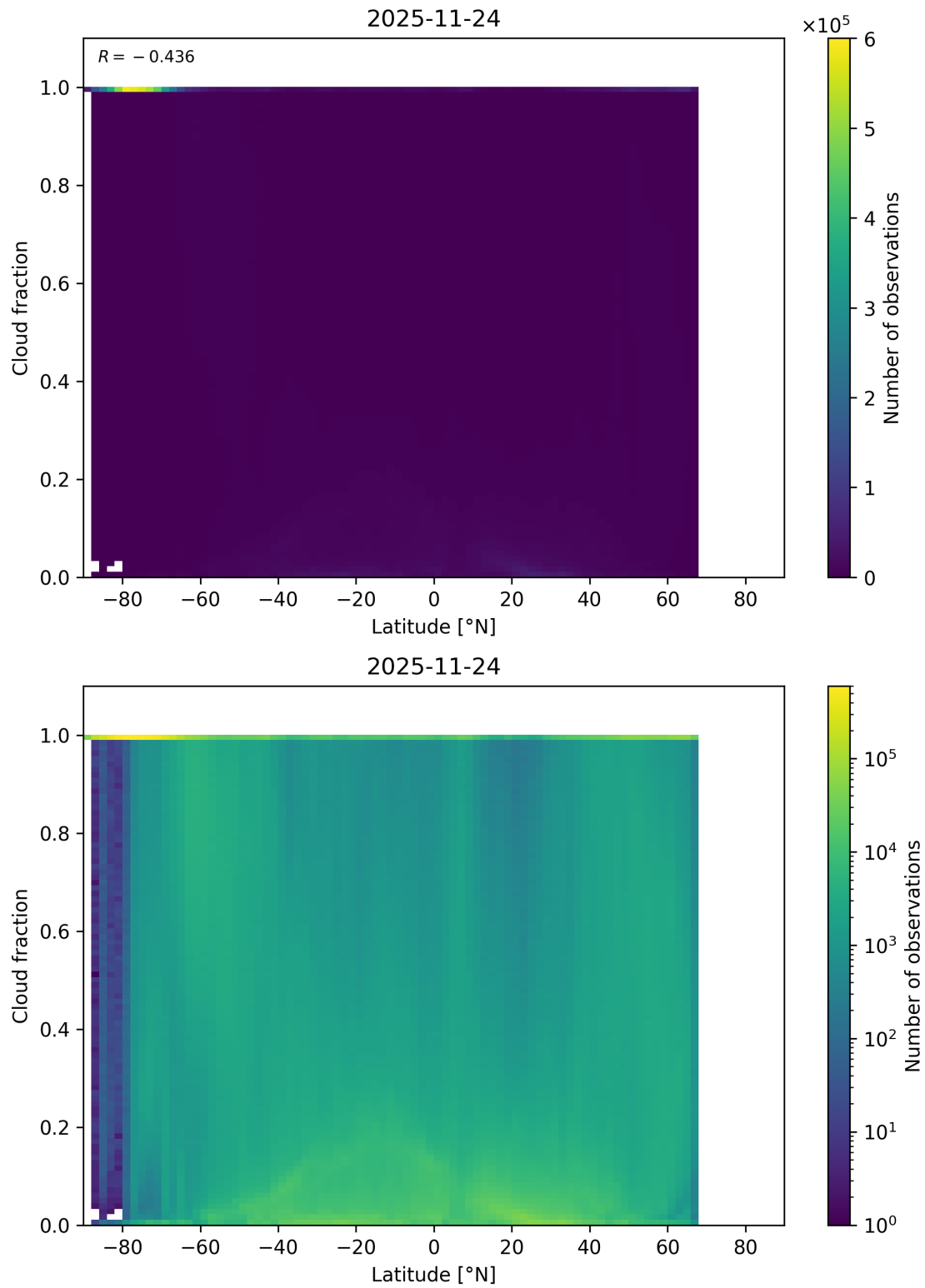
Figure 90: Scatter density plot of “Latitude” against “Cloud fraction” for 2025-11-23 to 2025-11-25.
