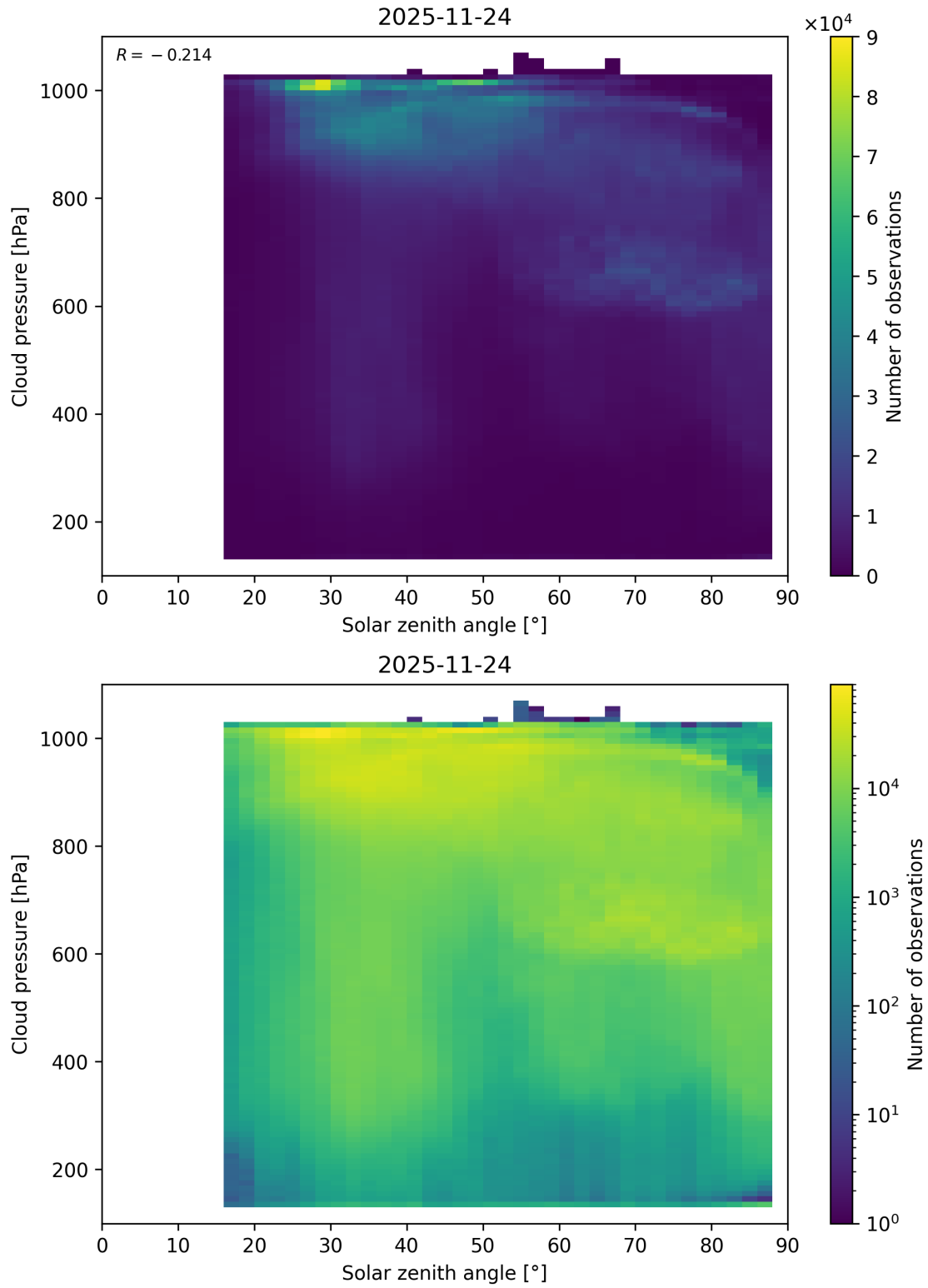
Figure 111: Scatter density plot of “Solar zenith angle” against “Cloud pressure” for 2025-11-23 to 2025-11-25.
