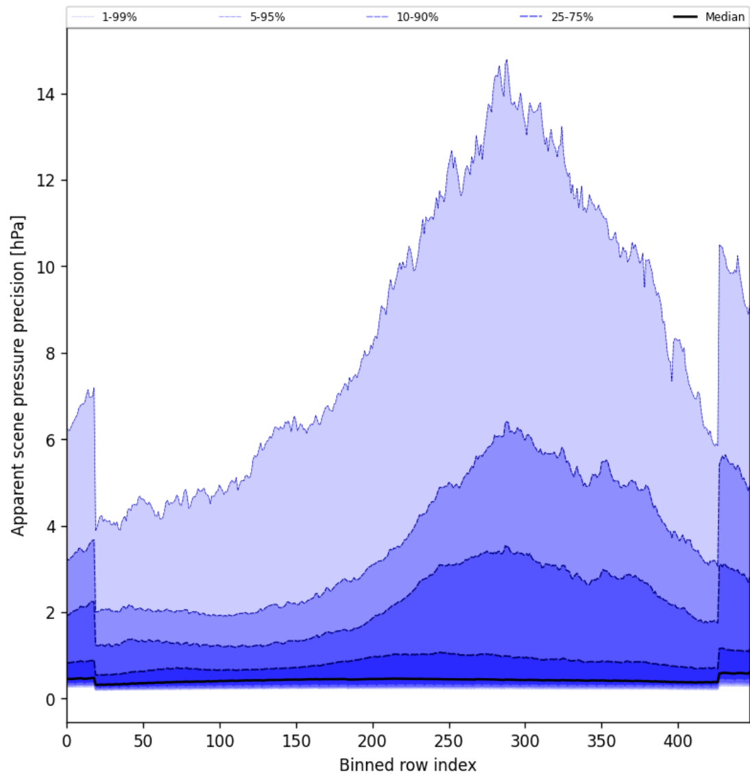
Figure 54: Along track statistics of “Apparent scene pressure precision” for 2025-11-23 to 2025-11-25
