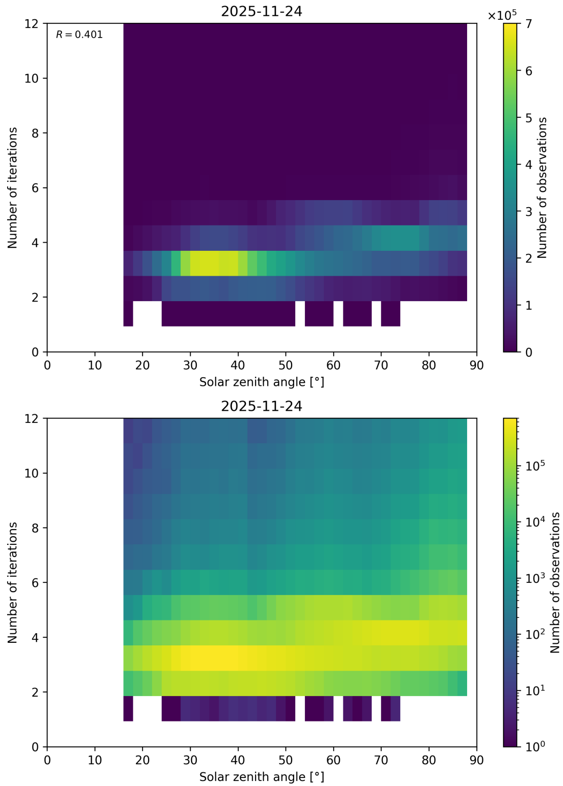
Figure 114: Scatter density plot of “Solar zenith angle” against “Number of iterations” for 2025-11-23 to 2025-11-25.
