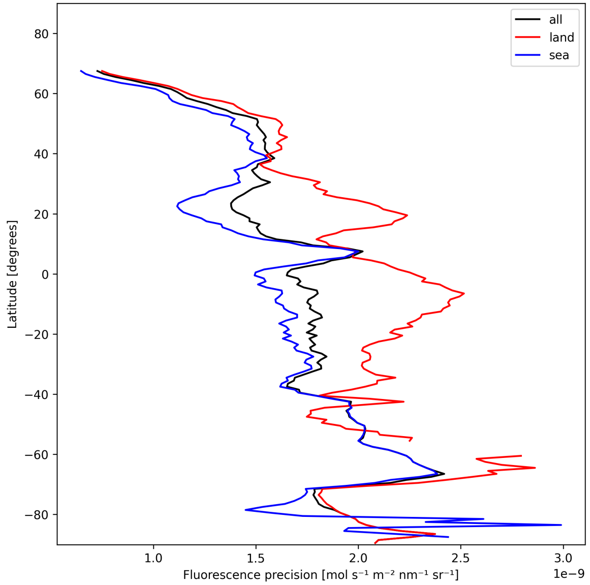
Figure 24: Zonal average of “Fluorescence precision” for 2025-11-23 to 2025-11-25.
