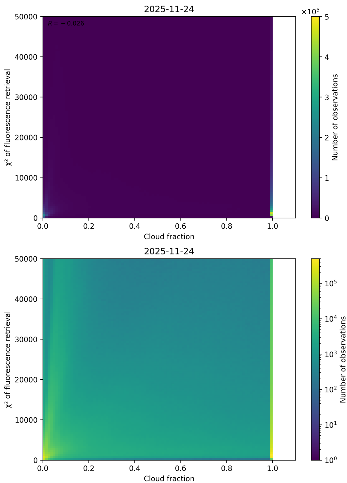
Figure 71: Scatter density plot of “Cloud fraction” against “ \chi^2 of fluorescence retrieval” for 2025-11-23 to 2025-11-25.
