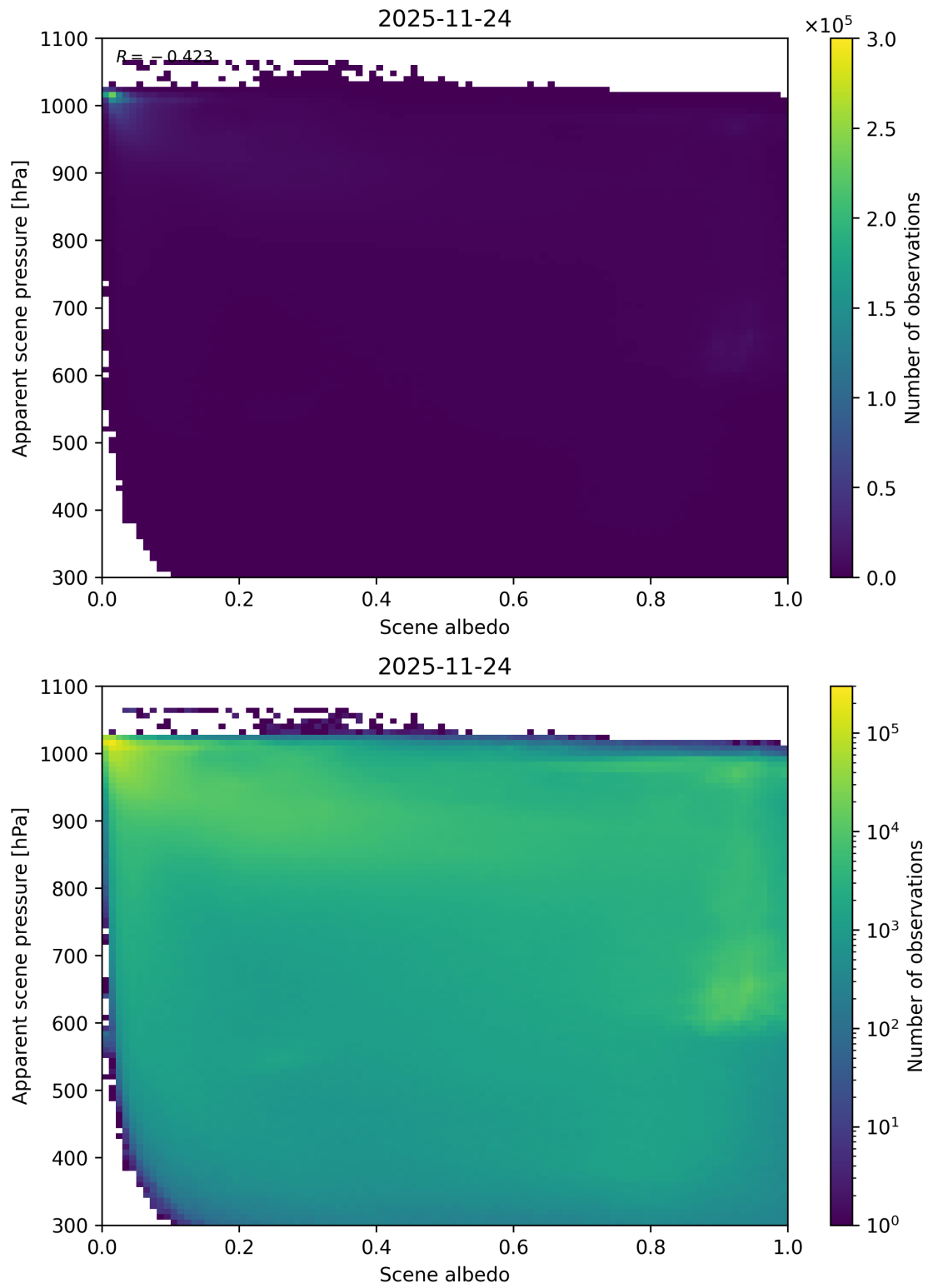
Figure 102: Scatter density plot of “Scene albedo” against “Apparent scene pressure” for 2025-11-23 to 2025-11-25.
