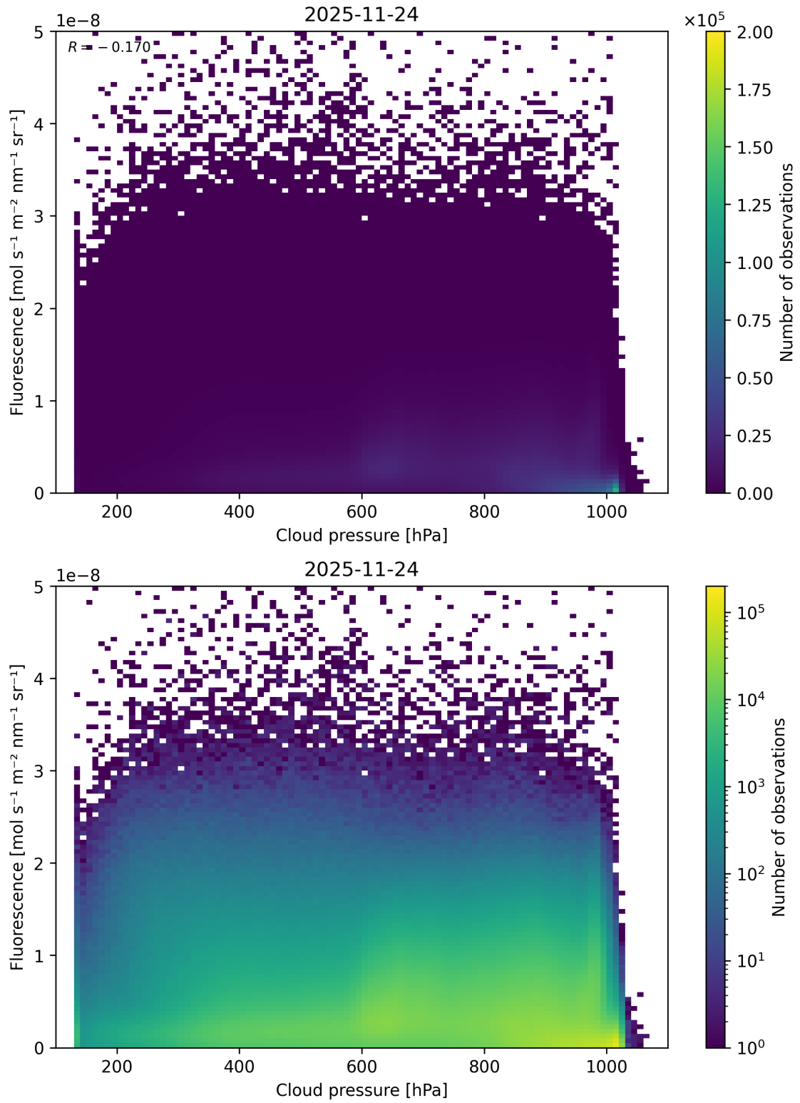
Figure 80: Scatter density plot of “Cloud pressure” against “Fluorescence” for 2025-11-23 to 2025-11-25.
