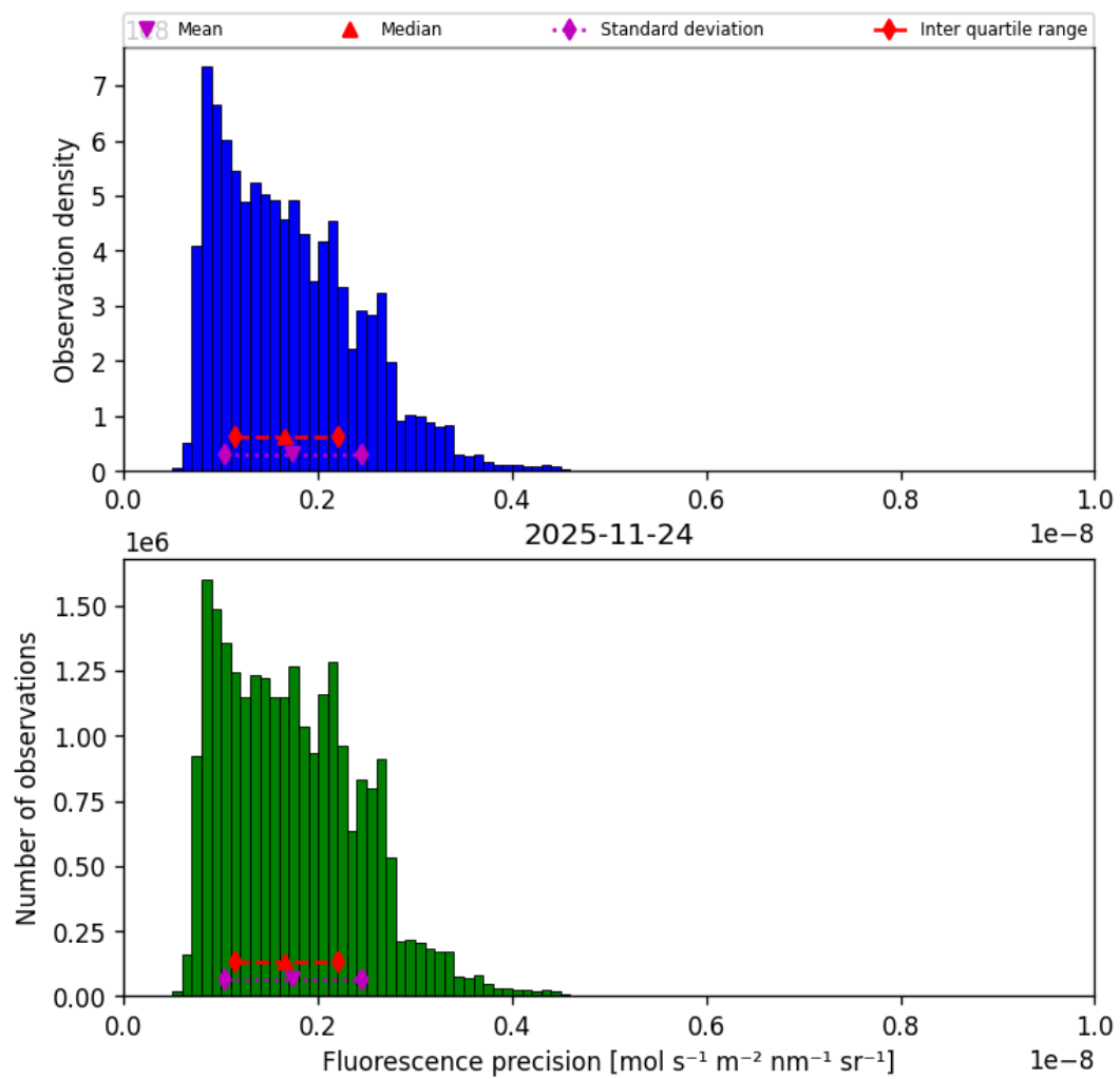
Figure 41: Histogram of “Fluorescence precision” for 2025-11-23 to 2025-11-25
