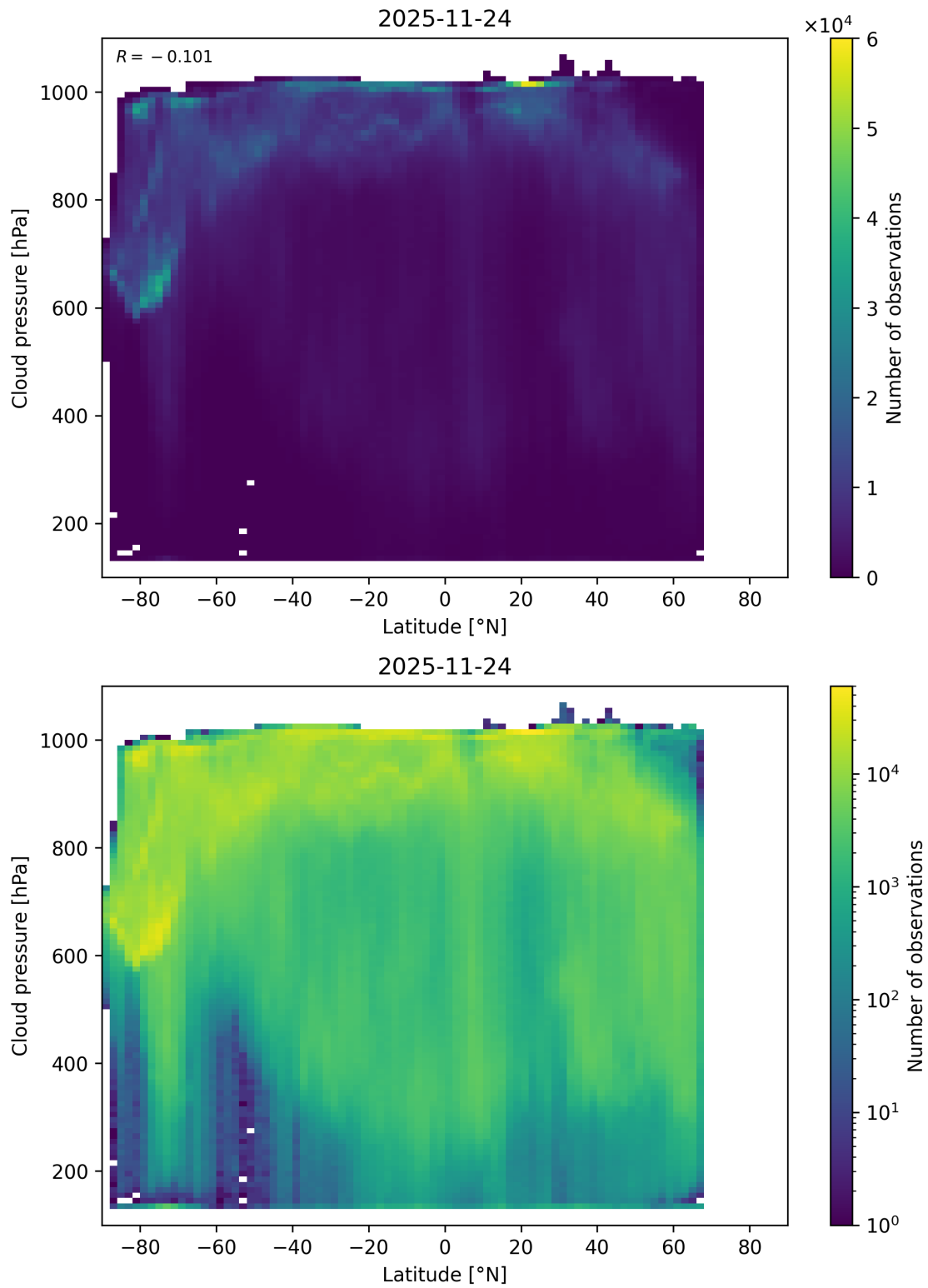
Figure 91: Scatter density plot of “Latitude” against “Cloud pressure” for 2025-11-23 to 2025-11-25.
