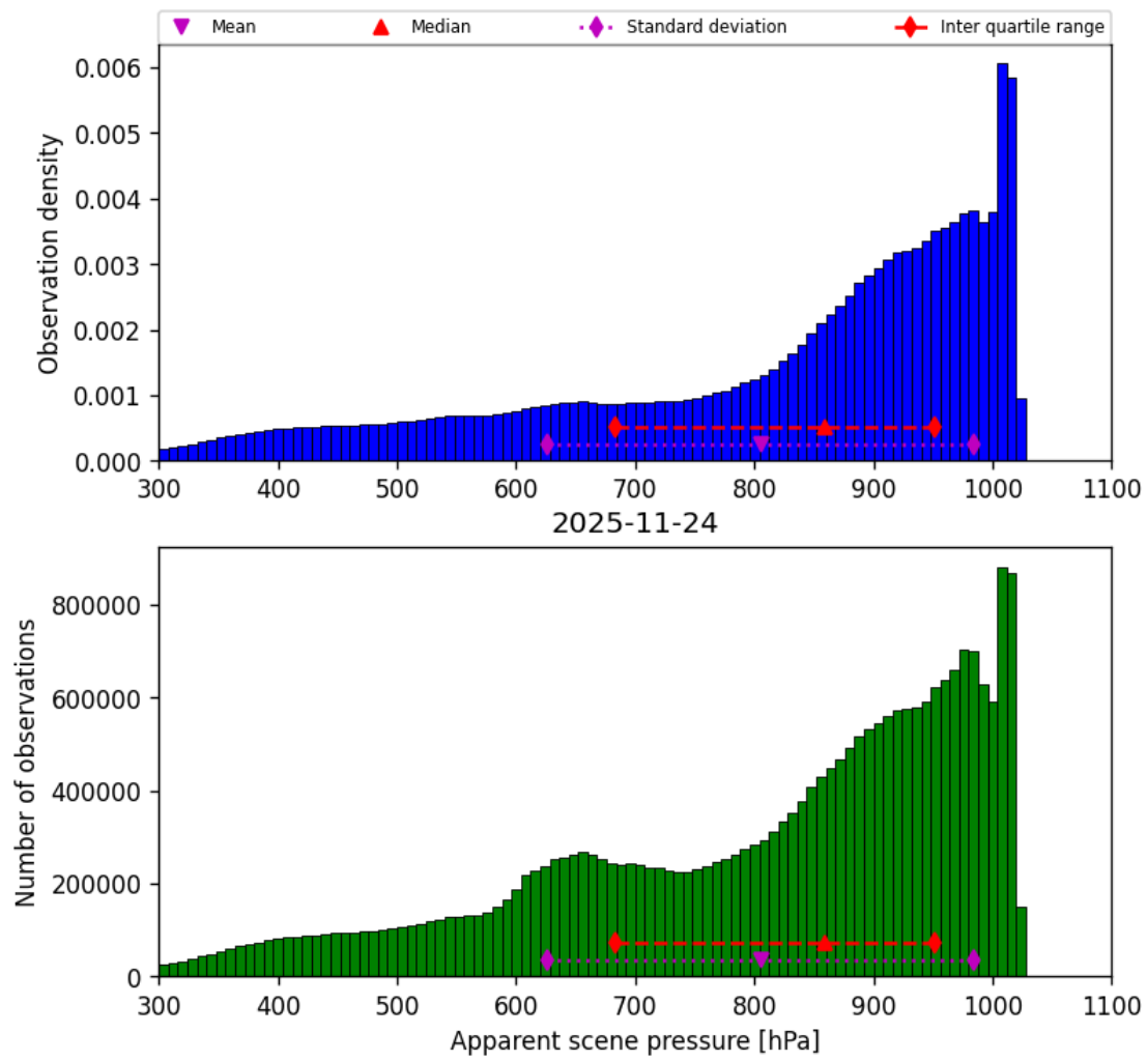
Figure 36: Histogram of “Apparent scene pressure” for 2025-11-23 to 2025-11-25
