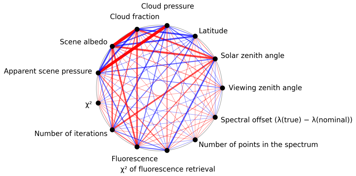
Figure 1: Map of correlation graph for 2025-11-23 to 2025-11-25.
