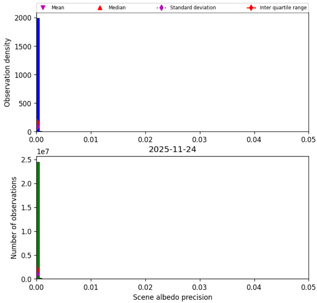
Figure 35: Histogram of “Scene albedo precision” for 2025-11-23 to 2025-11-25
