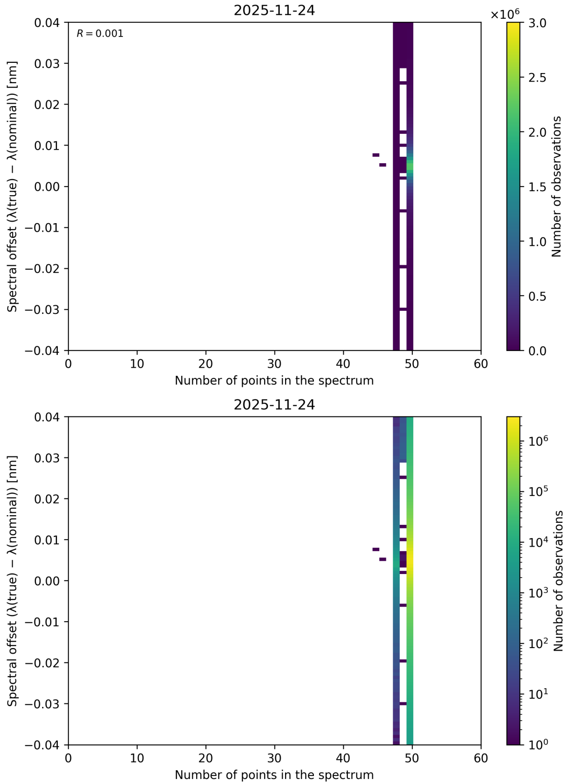
Figure 101: Scatter density plot of “Number of points in the spectrum” against “Spectral offset ( \lambda_{\text{true}} - \lambda_{\text{nominal}} )” for 2025-11-23 to 2025-11-25.
