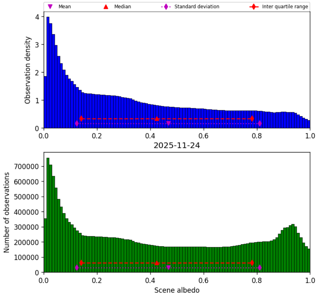
Figure 34: Histogram of “Scene albedo” for 2025-11-23 to 2025-11-25
