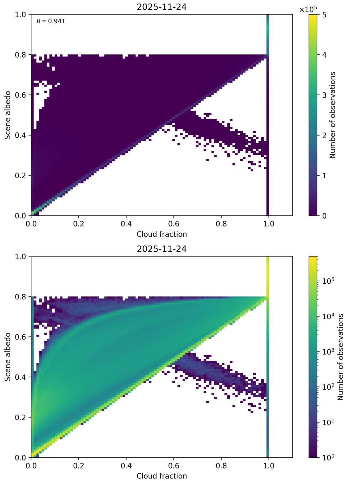
Figure 75: Scatter density plot of “Cloud fraction” against “Scene albedo” for 2025-11-23 to 2025-11-25.
