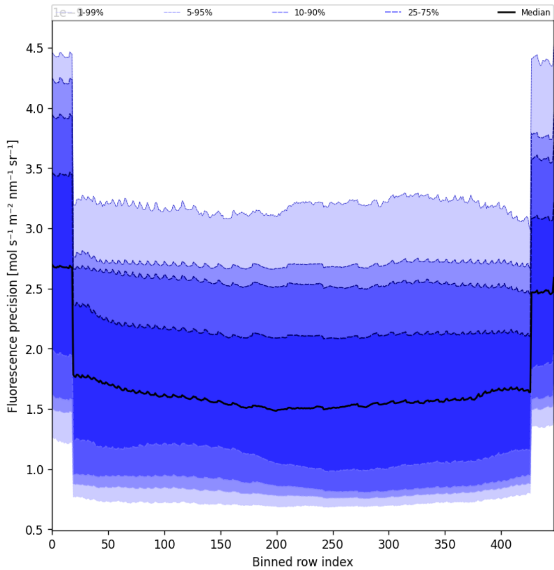
Figure 58: Along track statistics of “Fluorescence precision” for 2025-11-23 to 2025-11-25
