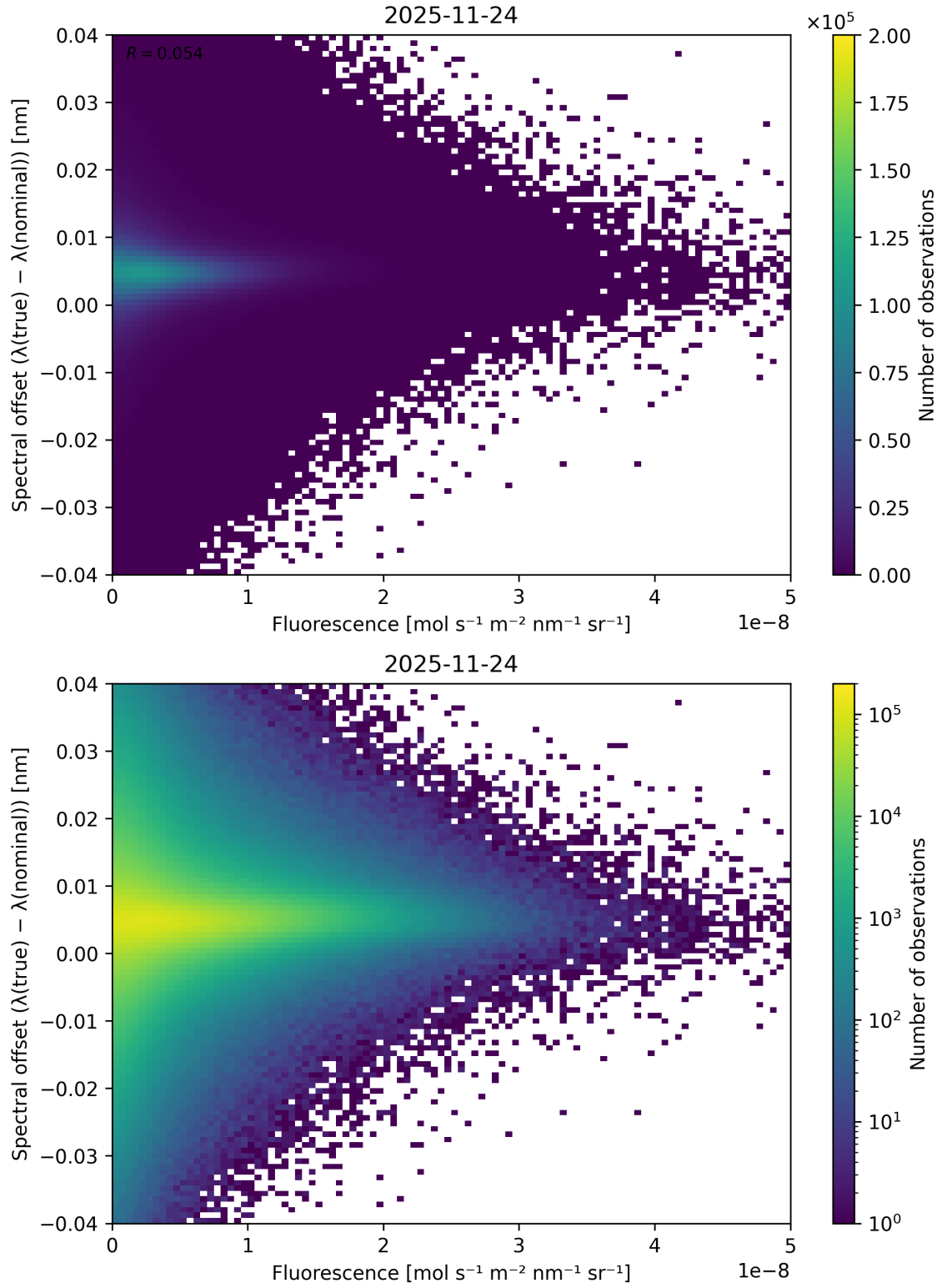
Figure 87: Scatter density plot of “Fluorescence” against “Spectral offset ( \lambda_{\text{true}} - \lambda_{\text{nominal}} )” for 2025-11-23 to 2025-11-25.
