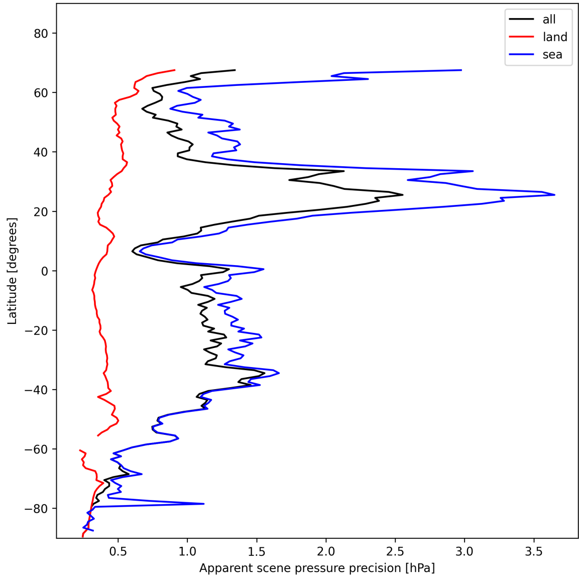
Figure 20: Zonal average of “Apparent scene pressure precision” for 2025-11-23 to 2025-11-25.
