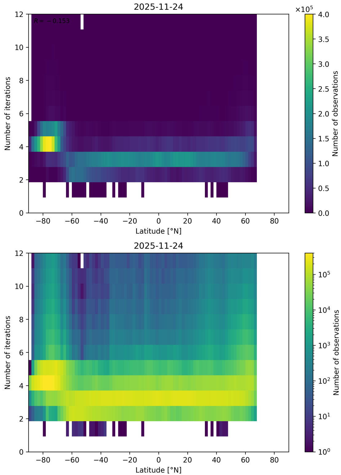
Figure 93: Scatter density plot of “Latitude” against “Number of iterations” for 2025-11-23 to 2025-11-25.
