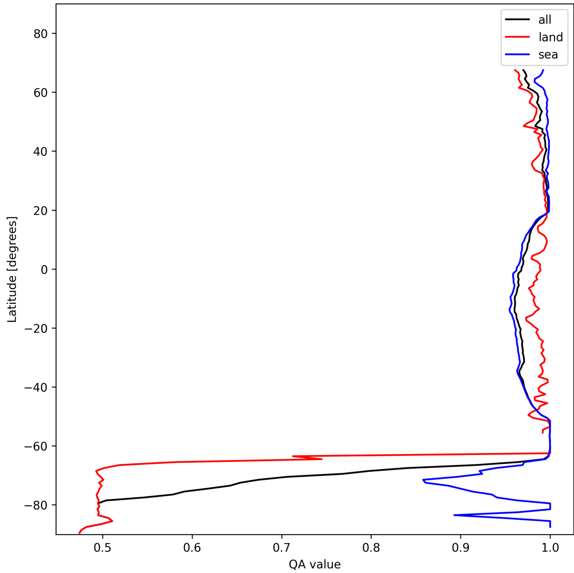
Figure 12: Zonal average of “QA value” for 2025-11-23 to 2025-11-25.
