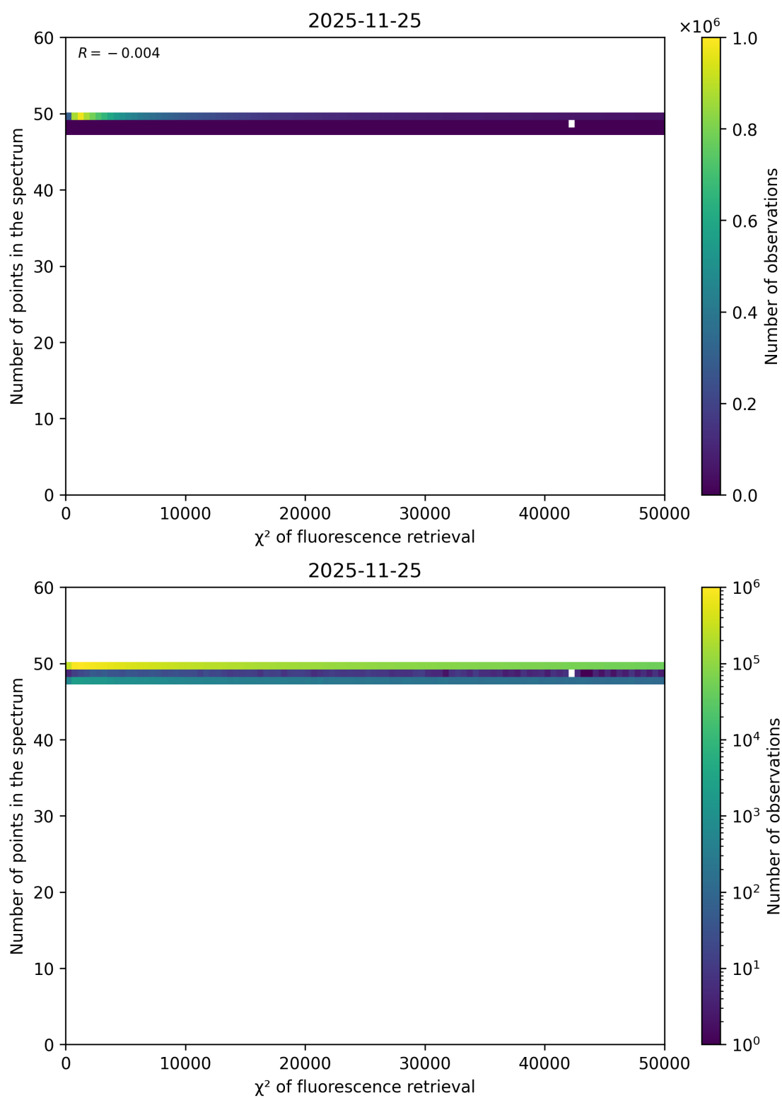
Figure 68: Scatter density plot of " \chi^2 of fluorescence retrieval" against "Number of points in the spectrum" for 2025-11-24 to 2025-11-26.
