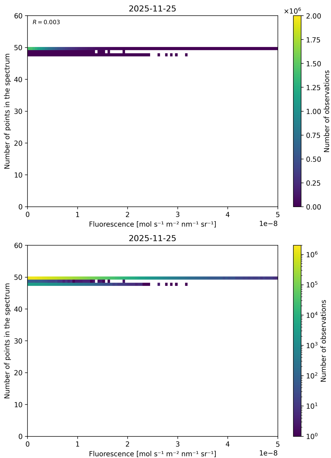
Figure 86: Scatter density plot of “Fluorescence” against “Number of points in the spectrum” for 2025-11-24 to 2025-11-26.
