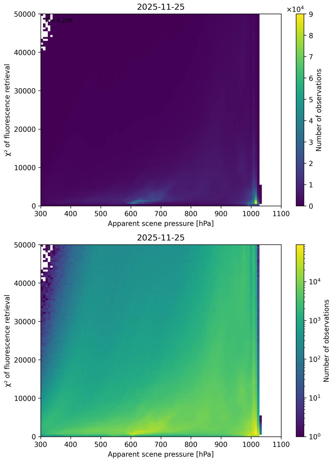
Figure 63: Scatter density plot of “Apparent scene pressure” against “ \chi^2 of fluorescence retrieval” for 2025-11-24 to 2025-11-26.
