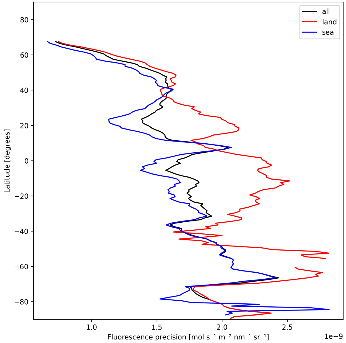
Figure 24: Zonal average of “Fluorescence precision” for 2025-11-24 to 2025-11-26.
