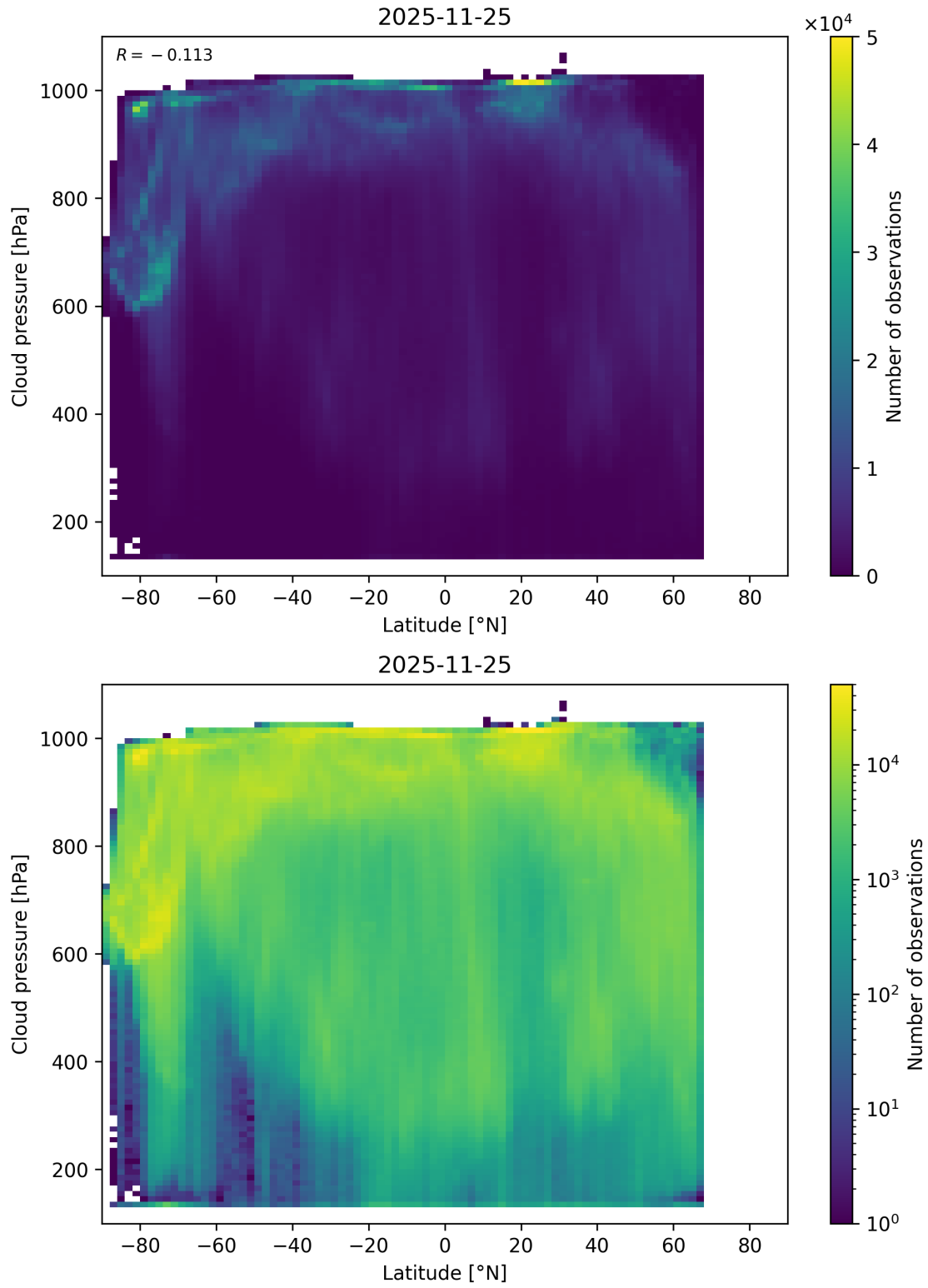
Figure 91: Scatter density plot of “Latitude” against “Cloud pressure” for 2025-11-24 to 2025-11-26.
