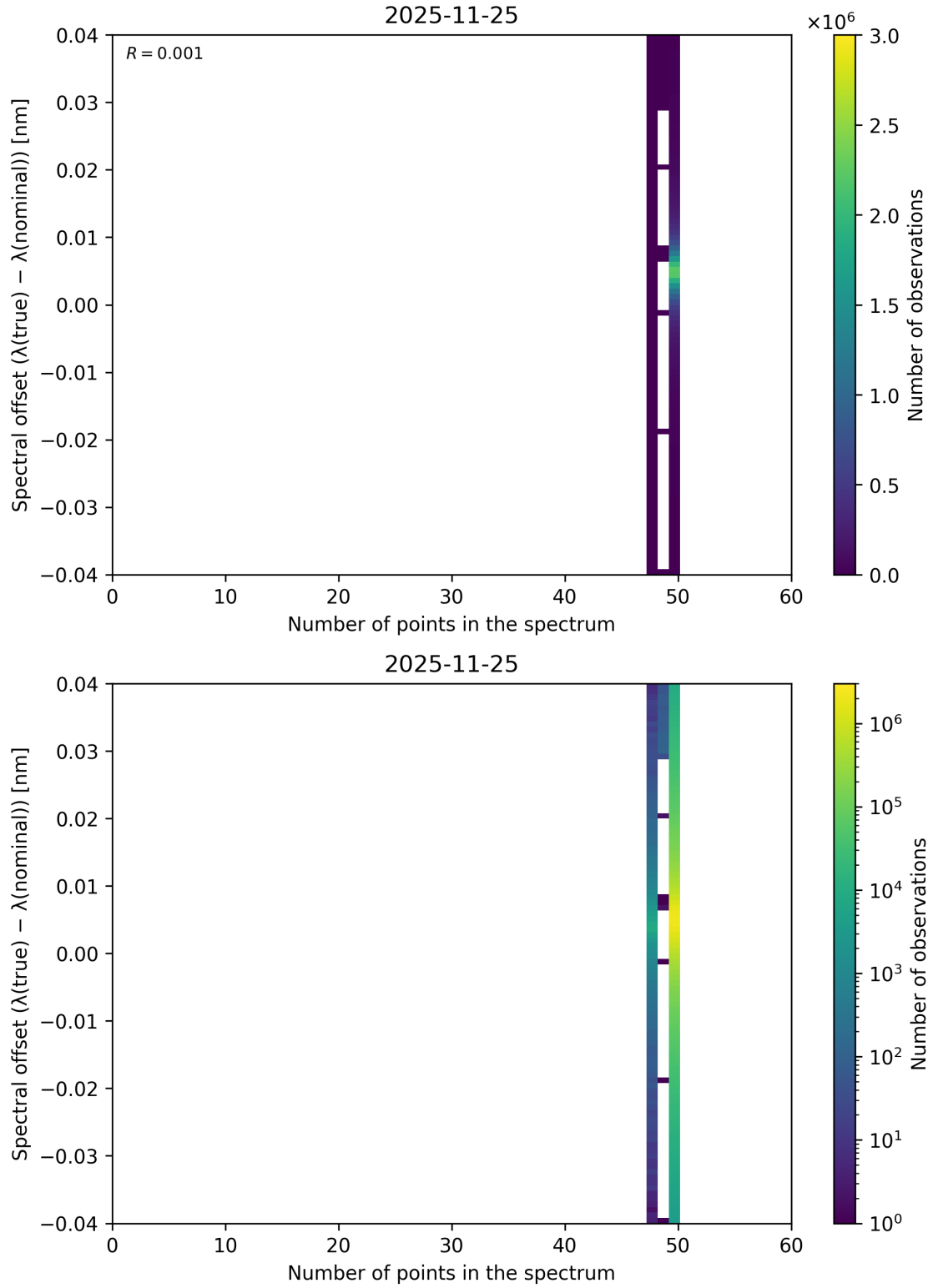
Figure 101: Scatter density plot of “Number of points in the spectrum” against “Spectral offset ( \lambda_{\text{true}} - \lambda_{\text{nominal}} )” for 2025-11-24 to 2025-11-26.
