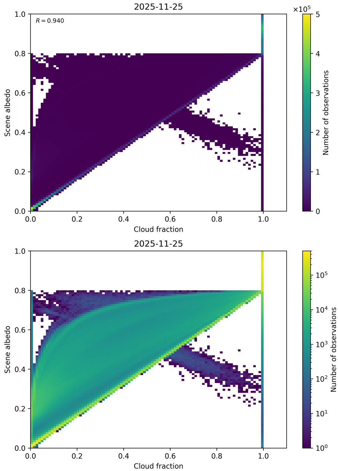
Figure 75: Scatter density plot of “Cloud fraction” against “Scene albedo” for 2025-11-24 to 2025-11-26.
