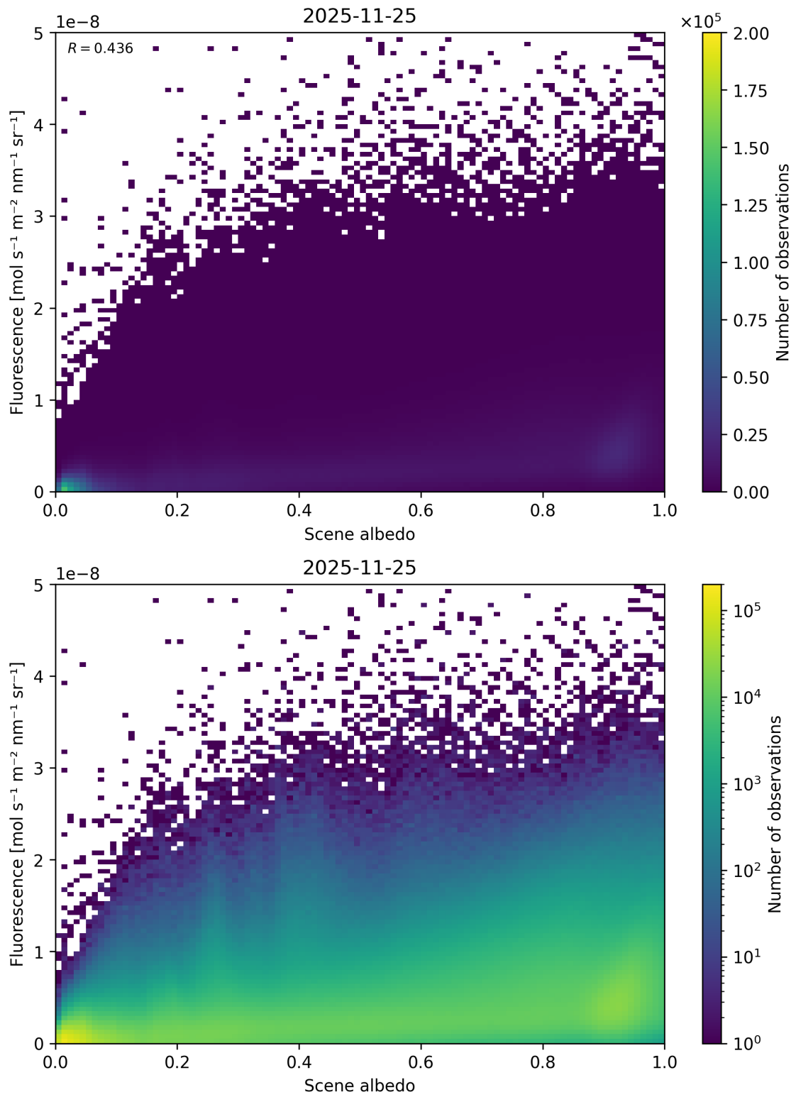
Figure 104: Scatter density plot of “Scene albedo” against “Fluorescence” for 2025-11-24 to 2025-11-26.
