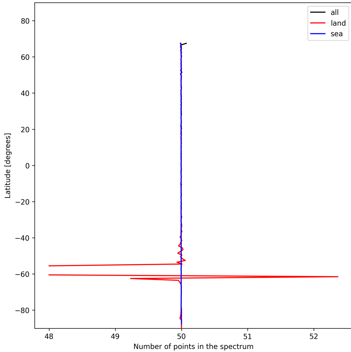
Figure 27: Zonal average of “Number of points in the spectrum” for 2025-11-24 to 2025-11-26.
