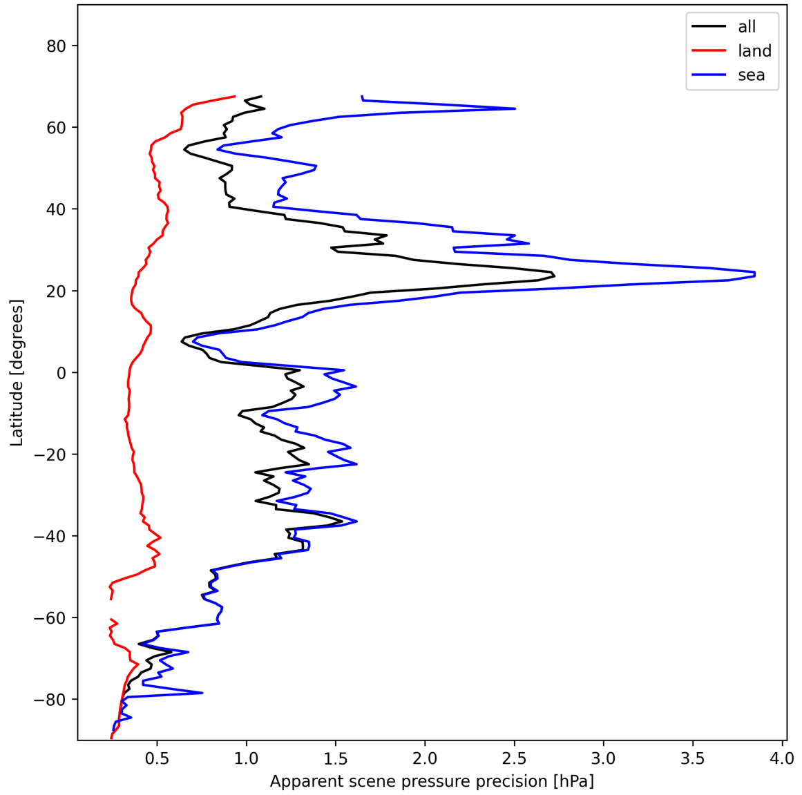
Figure 20: Zonal average of “Apparent scene pressure precision” for 2025-11-24 to 2025-11-26.
