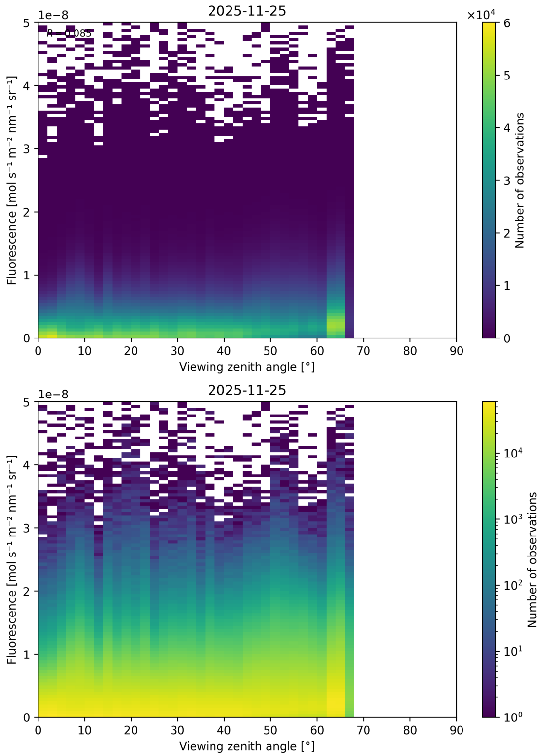
Figure 122: Scatter density plot of "Viewing zenith angle" against "Fluorescence" for 2025-11-24 to 2025-11-26.
