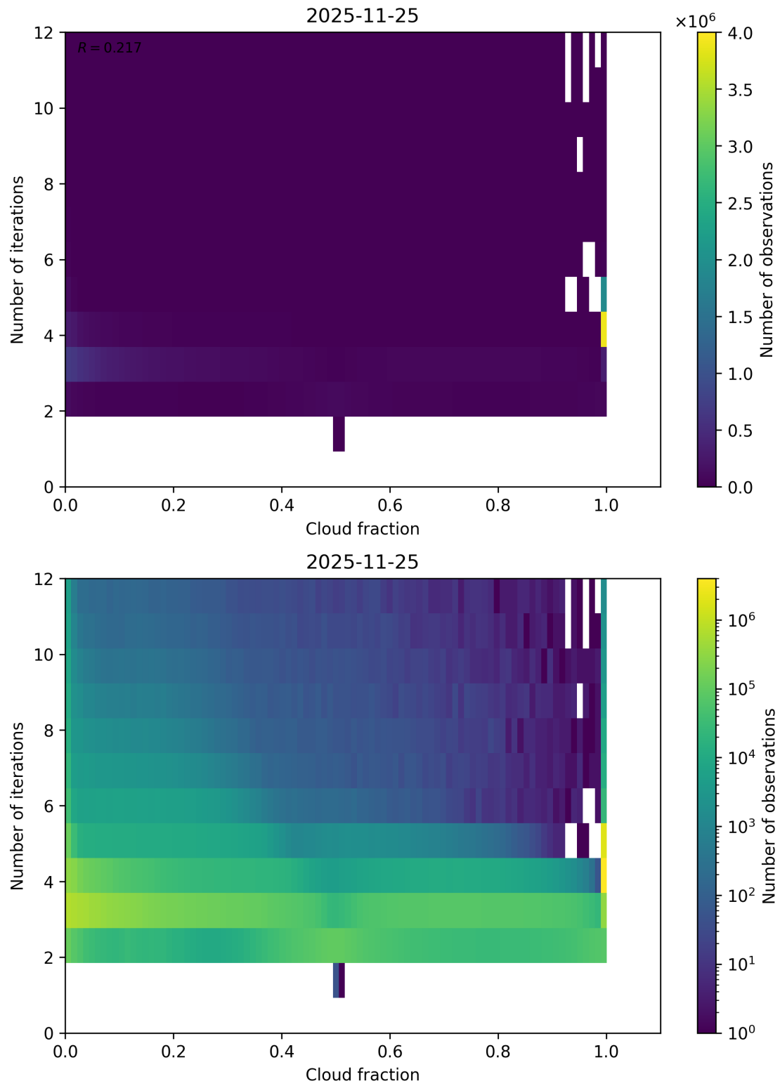
Figure 73: Scatter density plot of “Cloud fraction” against “Number of iterations” for 2025-11-24 to 2025-11-26.
