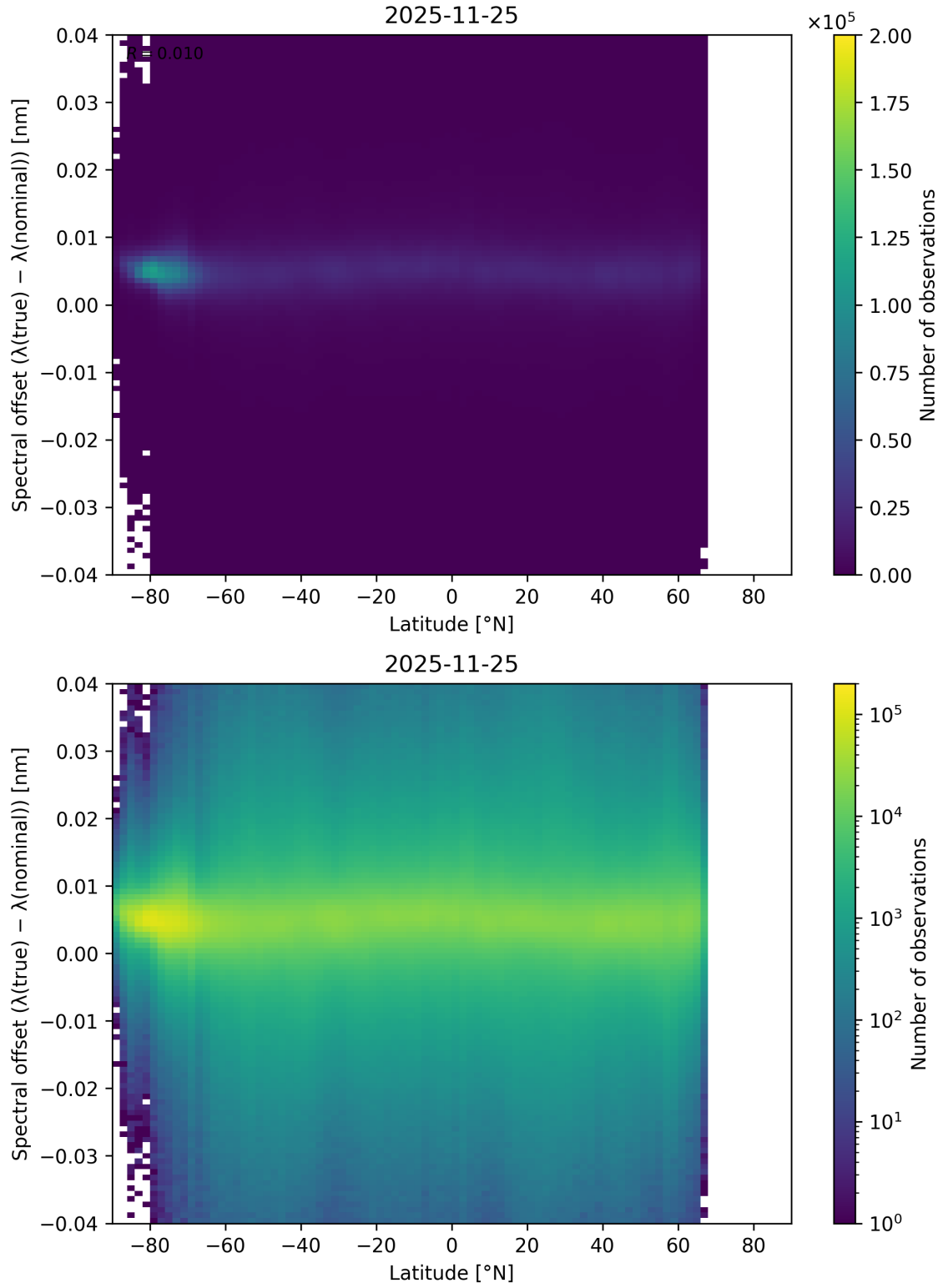
Figure 96: Scatter density plot of “Latitude” against “Spectral offset ( \lambda_{\text{true}} - \lambda_{\text{nominal}} )” for 2025-11-24 to 2025-11-26.
