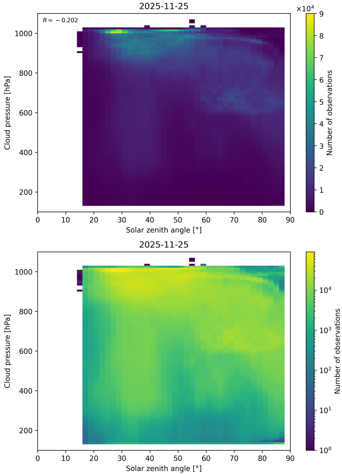
Figure 111: Scatter density plot of “Solar zenith angle” against “Cloud pressure” for 2025-11-24 to 2025-11-26.
