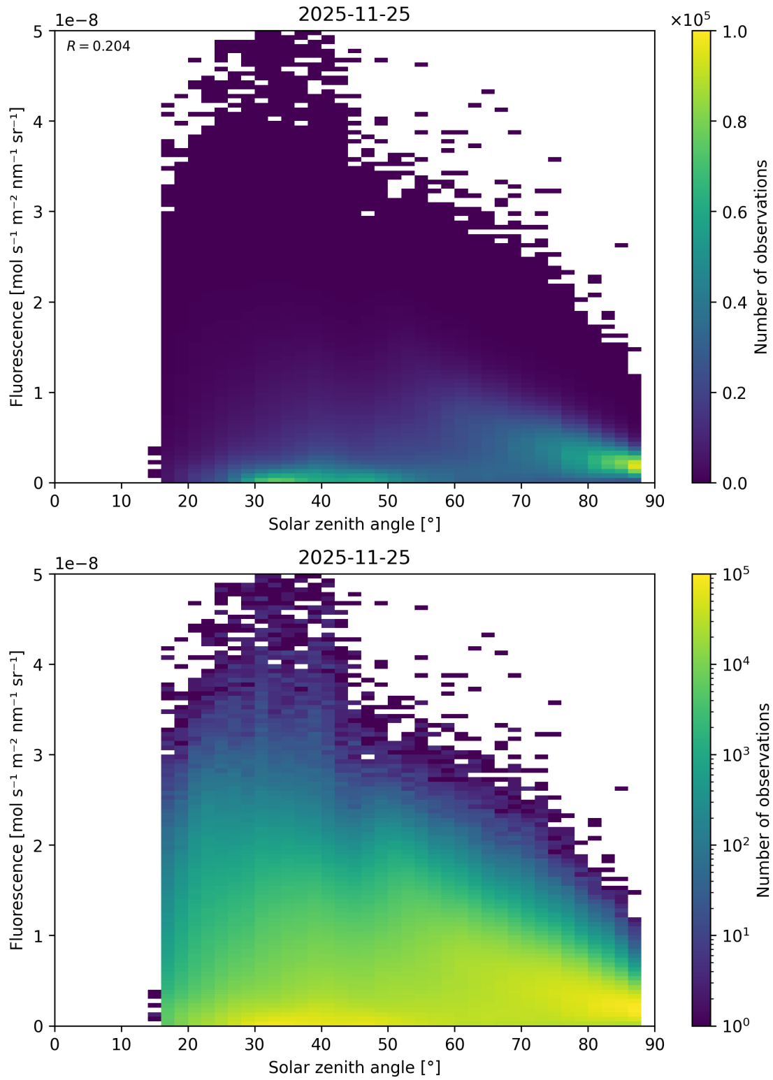
Figure 112: Scatter density plot of “Solar zenith angle” against “Fluorescence” for 2025-11-24 to 2025-11-26.
