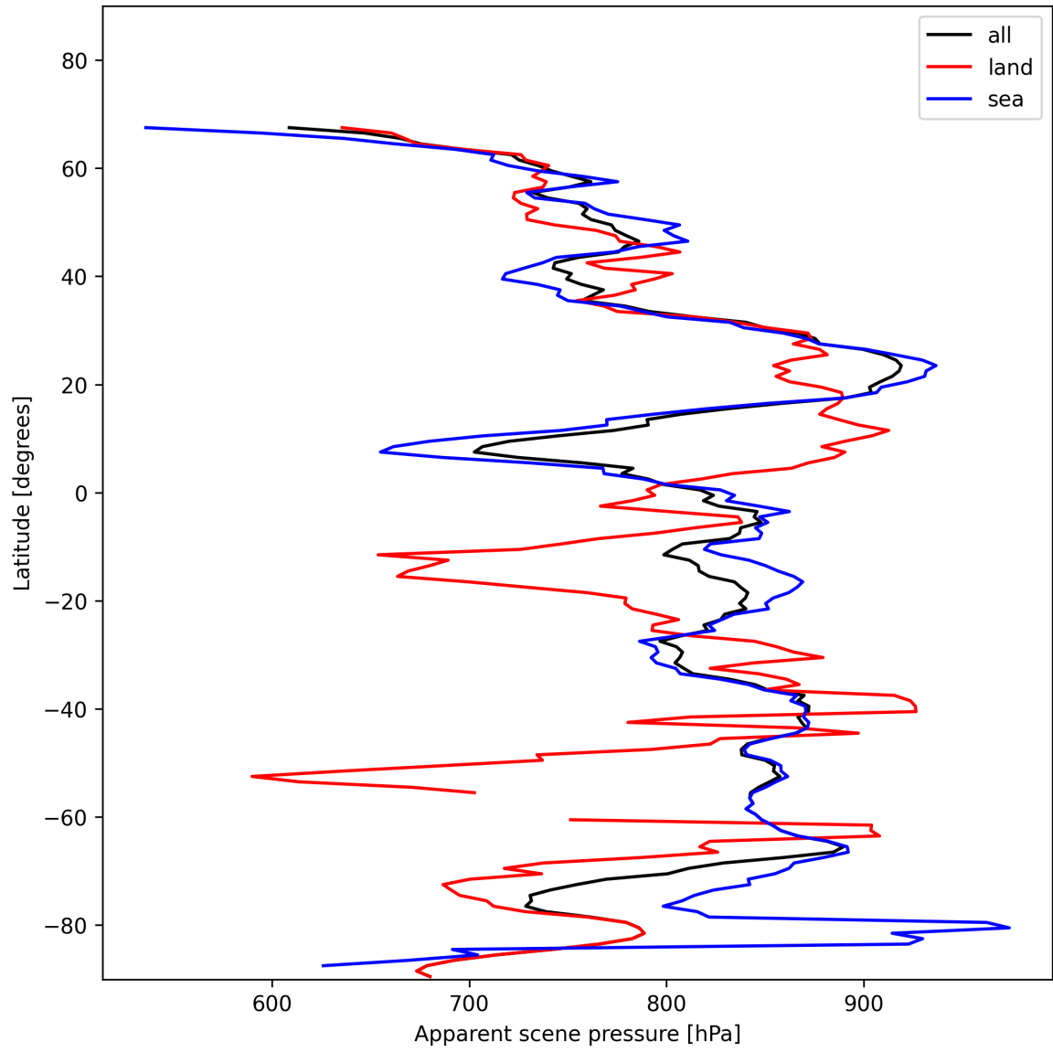
Figure 19: Zonal average of “Apparent scene pressure” for 2025-11-24 to 2025-11-26.
