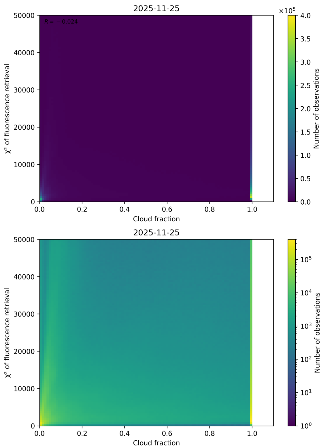
Figure 71: Scatter density plot of “Cloud fraction” against “ \chi^2 of fluorescence retrieval” for 2025-11-24 to 2025-11-26.
