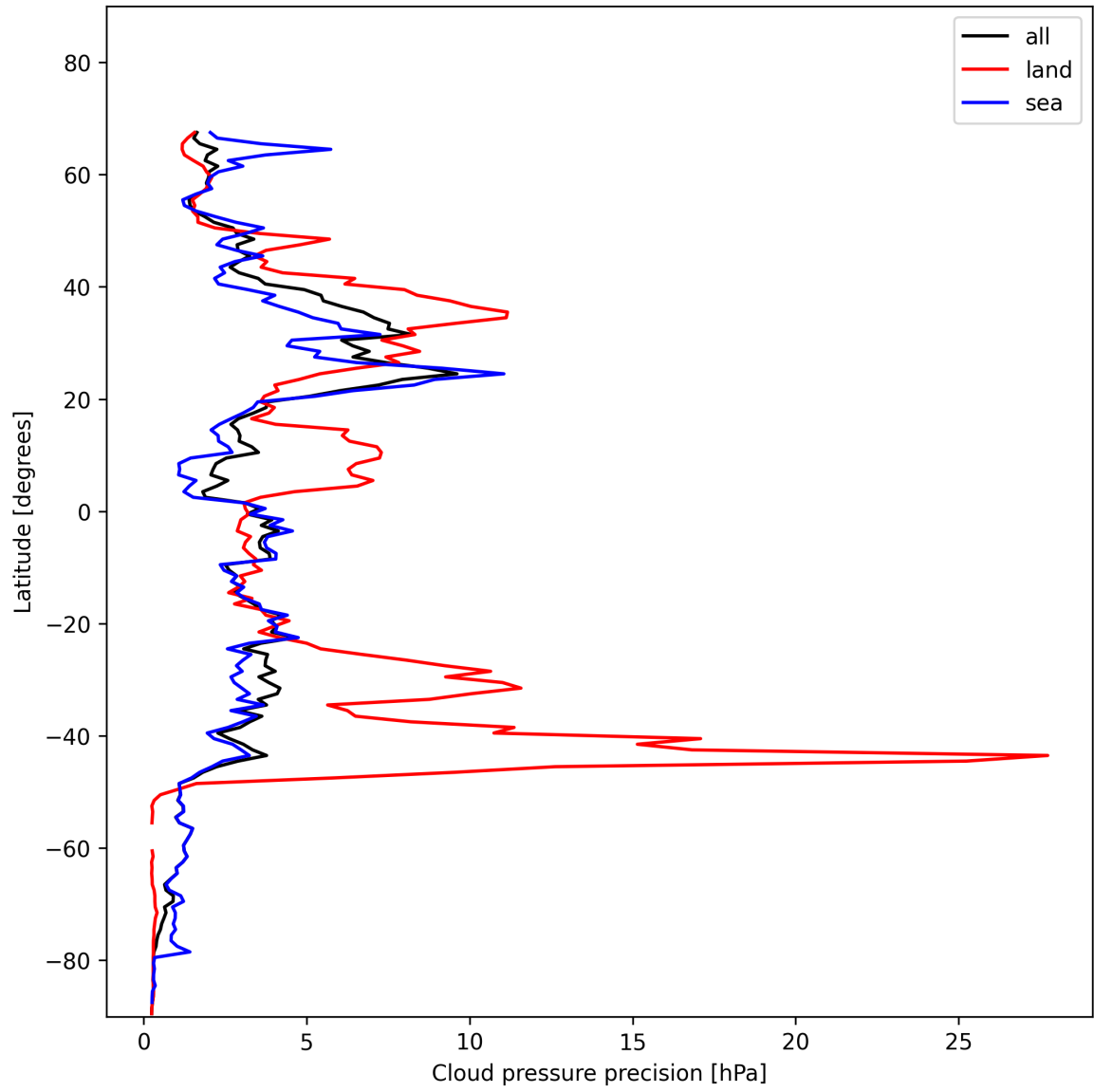
Figure 14: Zonal average of “Cloud pressure precision” for 2025-11-24 to 2025-11-26.
