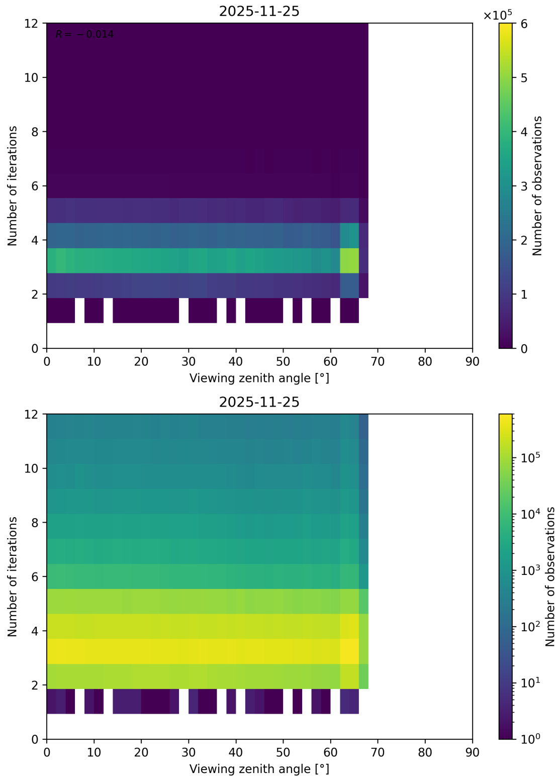
Figure 124: Scatter density plot of “Viewing zenith angle” against “Number of iterations” for 2025-11-24 to 2025-11-26.
