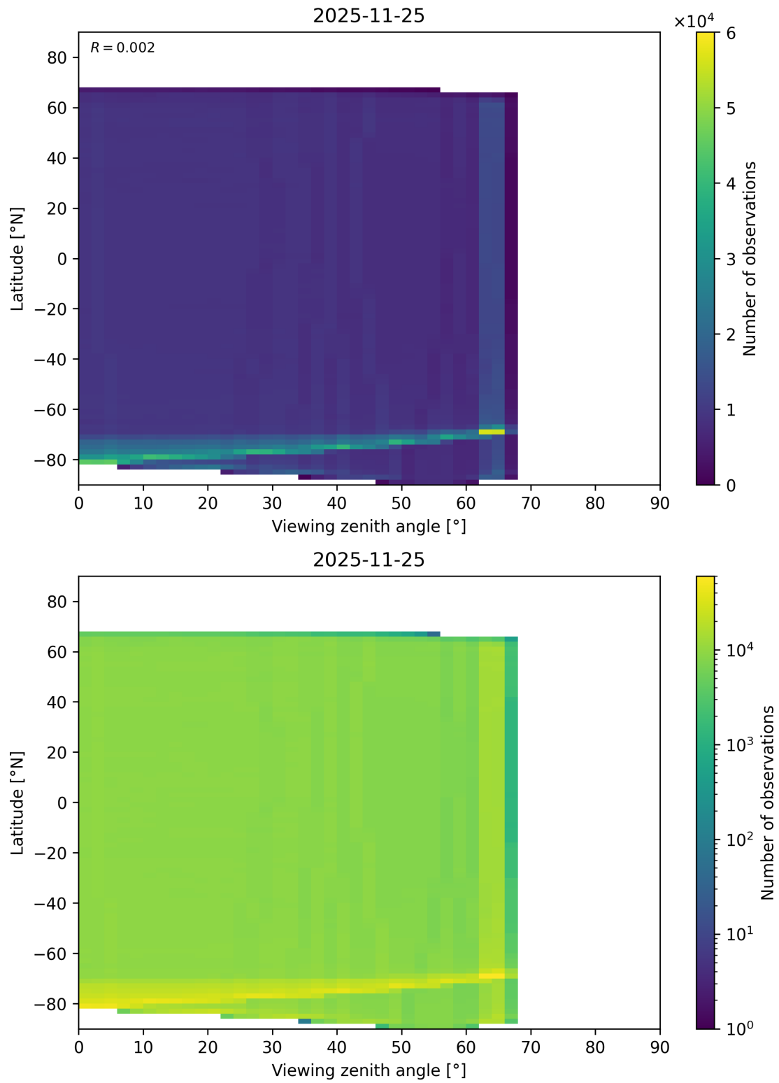
Figure 123: Scatter density plot of “Viewing zenith angle” against “Latitude” for 2025-11-24 to 2025-11-26.
