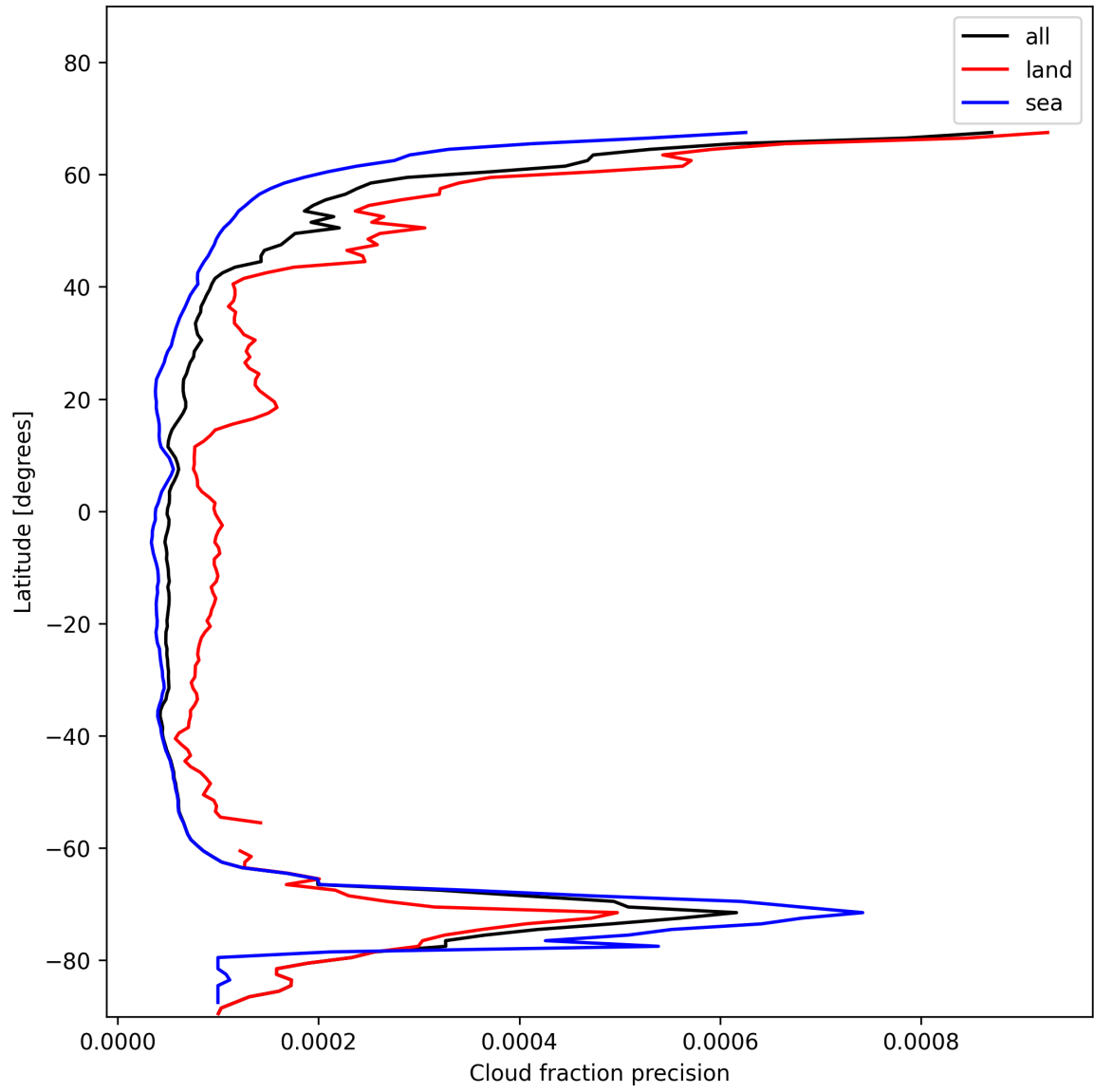
Figure 16: Zonal average of “Cloud fraction precision” for 2025-11-24 to 2025-11-26.
