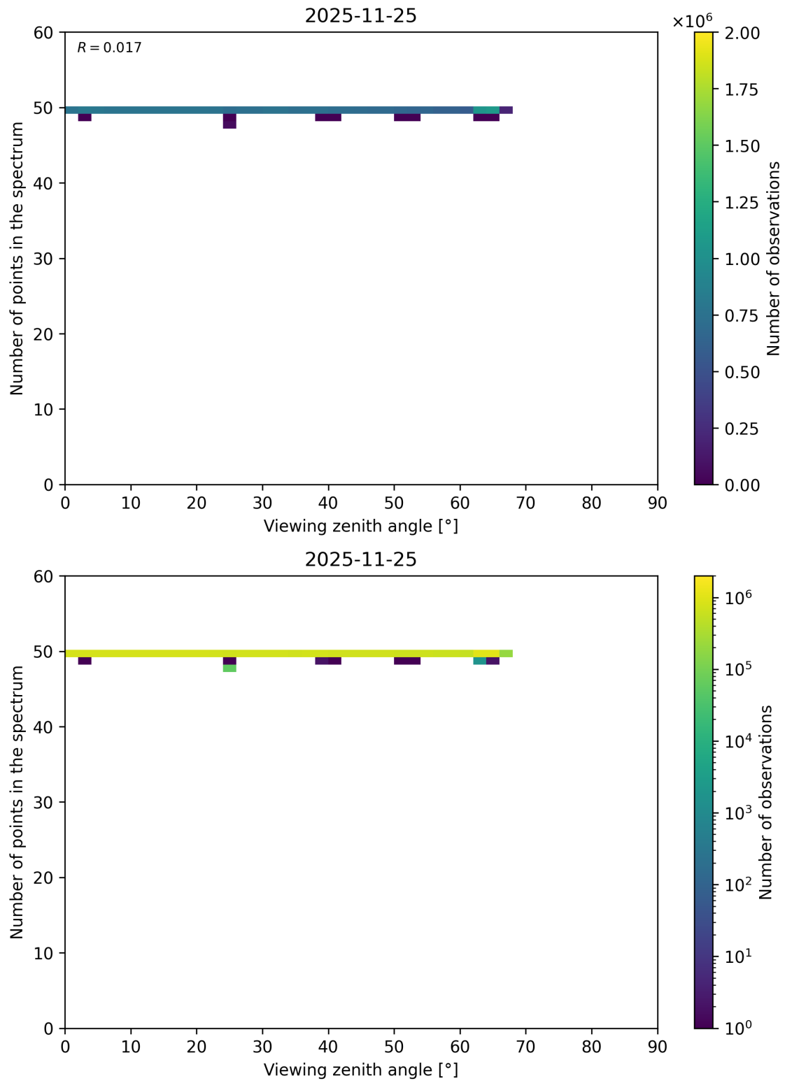
Figure 125: Scatter density plot of “Viewing zenith angle” against “Number of points in the spectrum” for 2025-11-24 to 2025-11-26.
