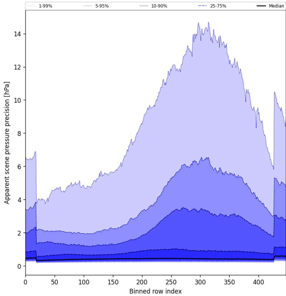
Figure 54: Along track statistics of “Apparent scene pressure precision” for 2025-11-24 to 2025-11-26
