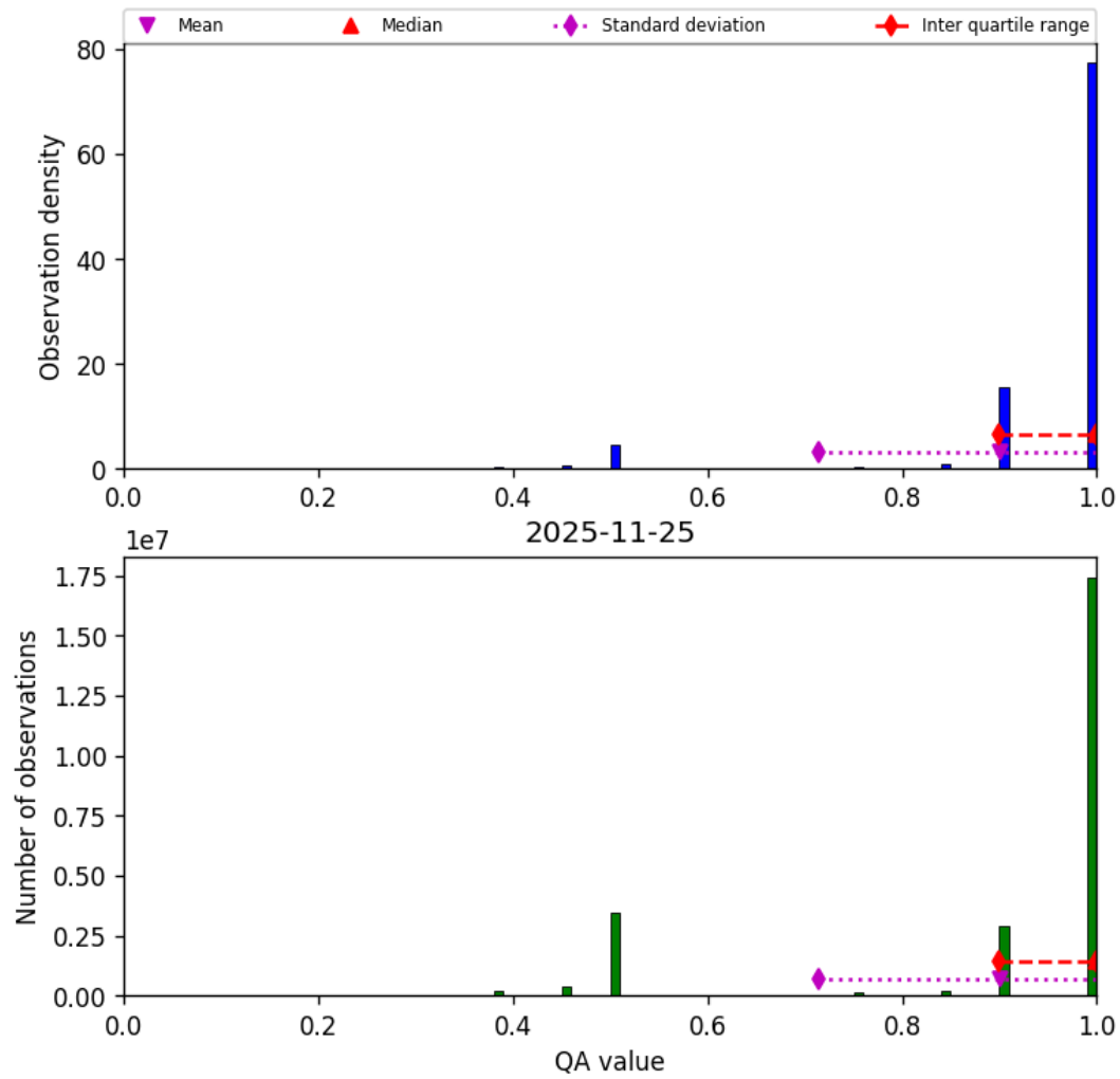
Figure 29: Histogram of “QA value” for 2025-11-24 to 2025-11-26
