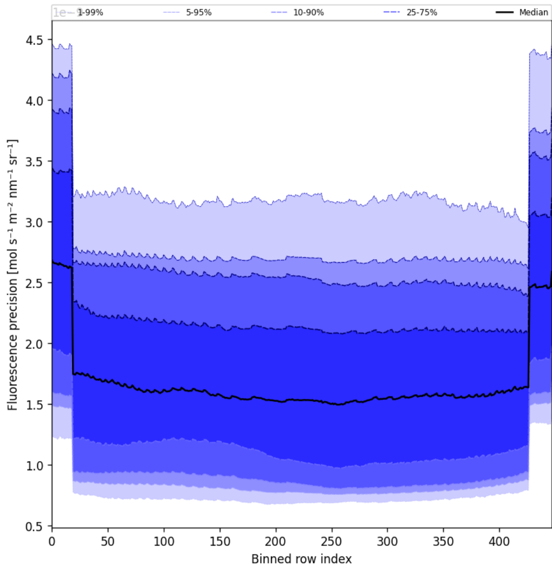
Figure 58: Along track statistics of “Fluorescence precision” for 2025-11-24 to 2025-11-26
