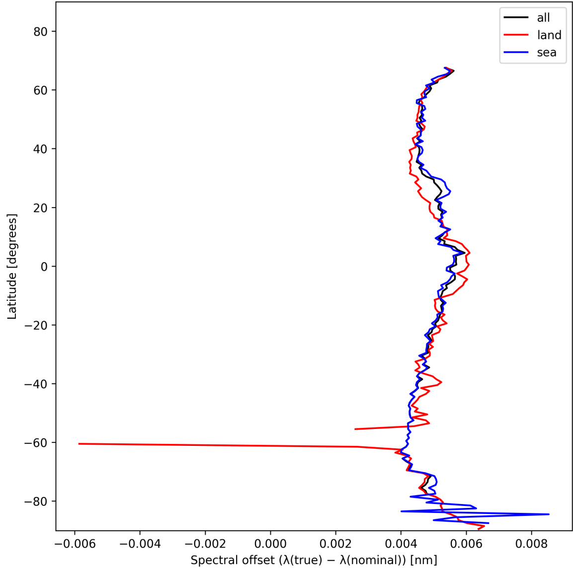
Figure 28: Zonal average of “Spectral offset ( \lambda_{\text{true}} - \lambda_{\text{nominal}} )” for 2025-11-24 to 2025-11-26.
