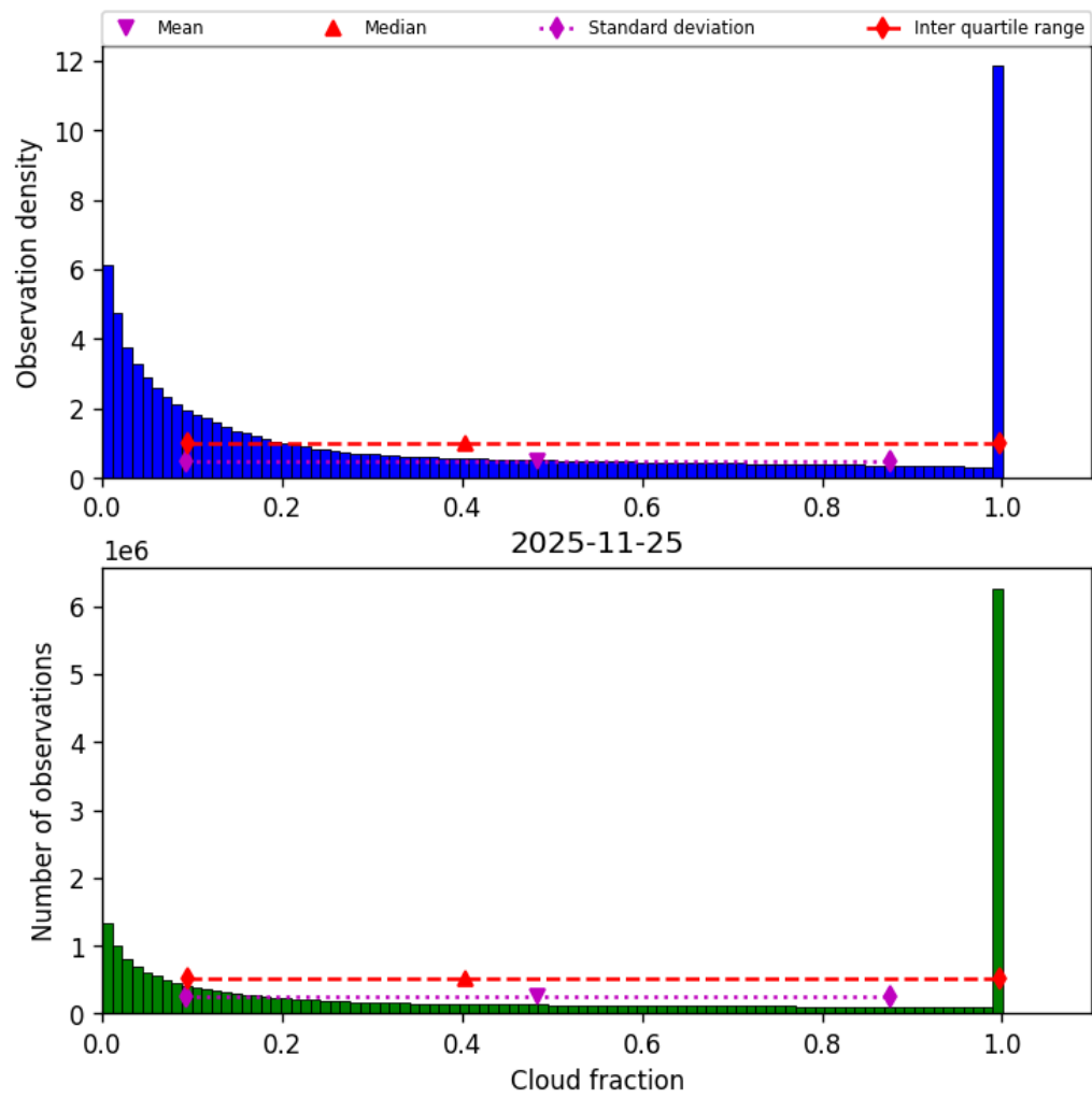
Figure 32: Histogram of “Cloud fraction” for 2025-11-24 to 2025-11-26
