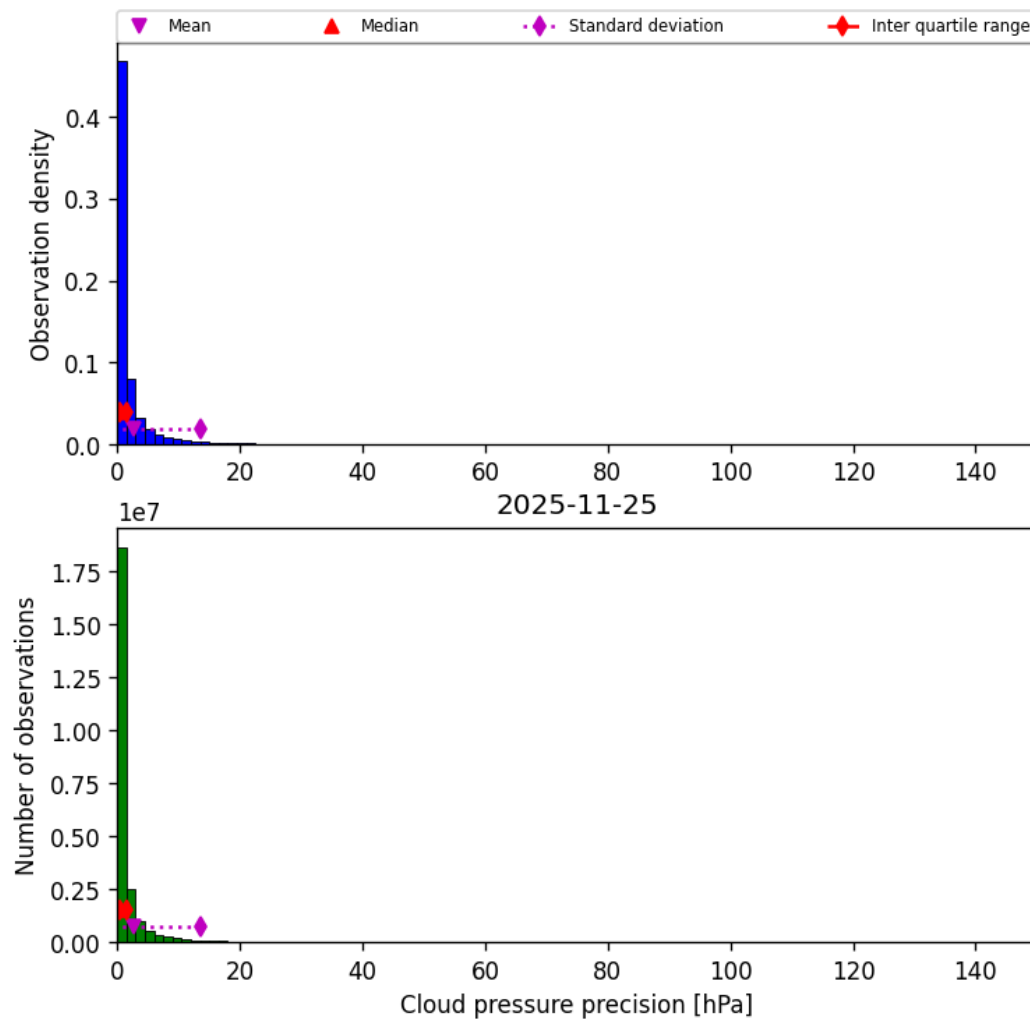
Figure 31: Histogram of “Cloud pressure precision” for 2025-11-24 to 2025-11-26
