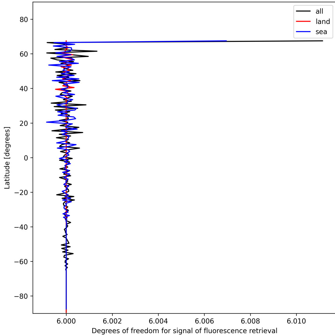
Figure 26: Zonal average of “Degrees of freedom for signal of fluorescence retrieval” for 2025-11-24 to 2025-11-26.
