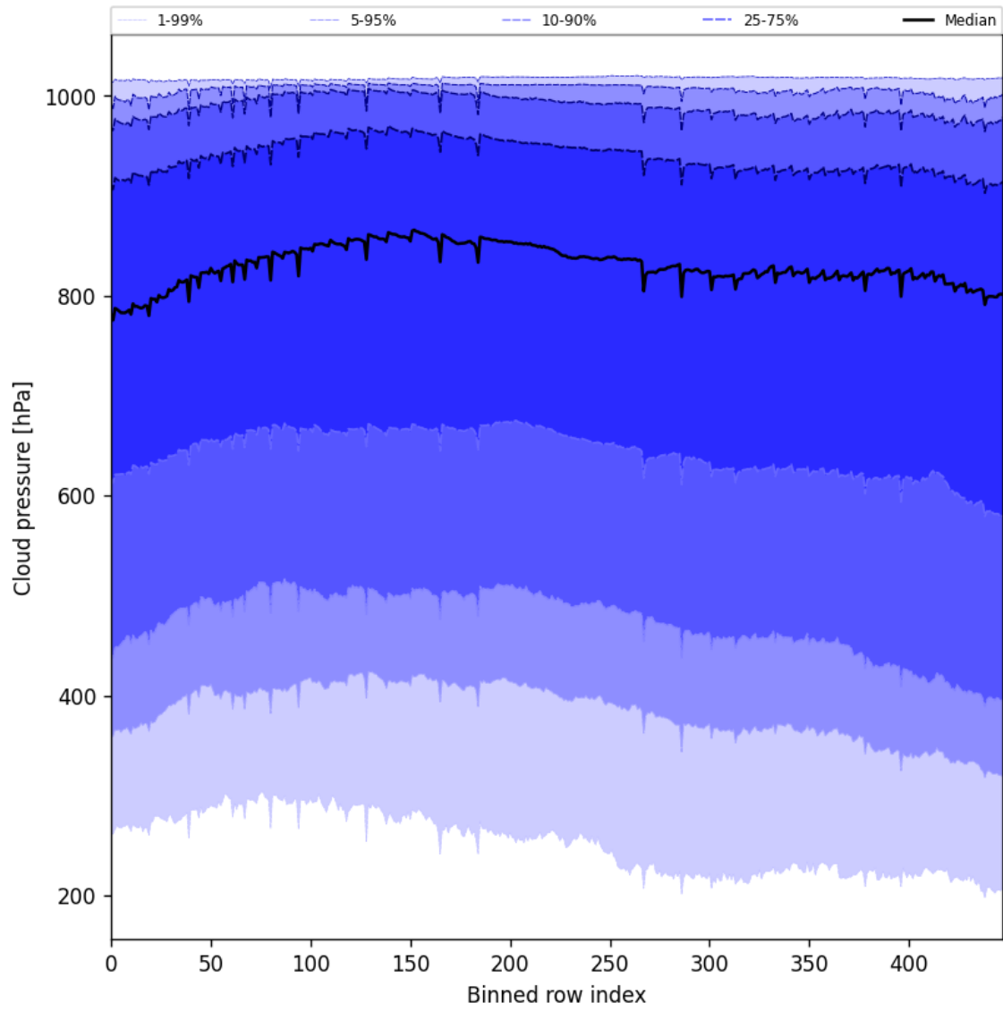
Figure 47: Along track statistics of “Cloud pressure” for 2025-11-24 to 2025-11-26
