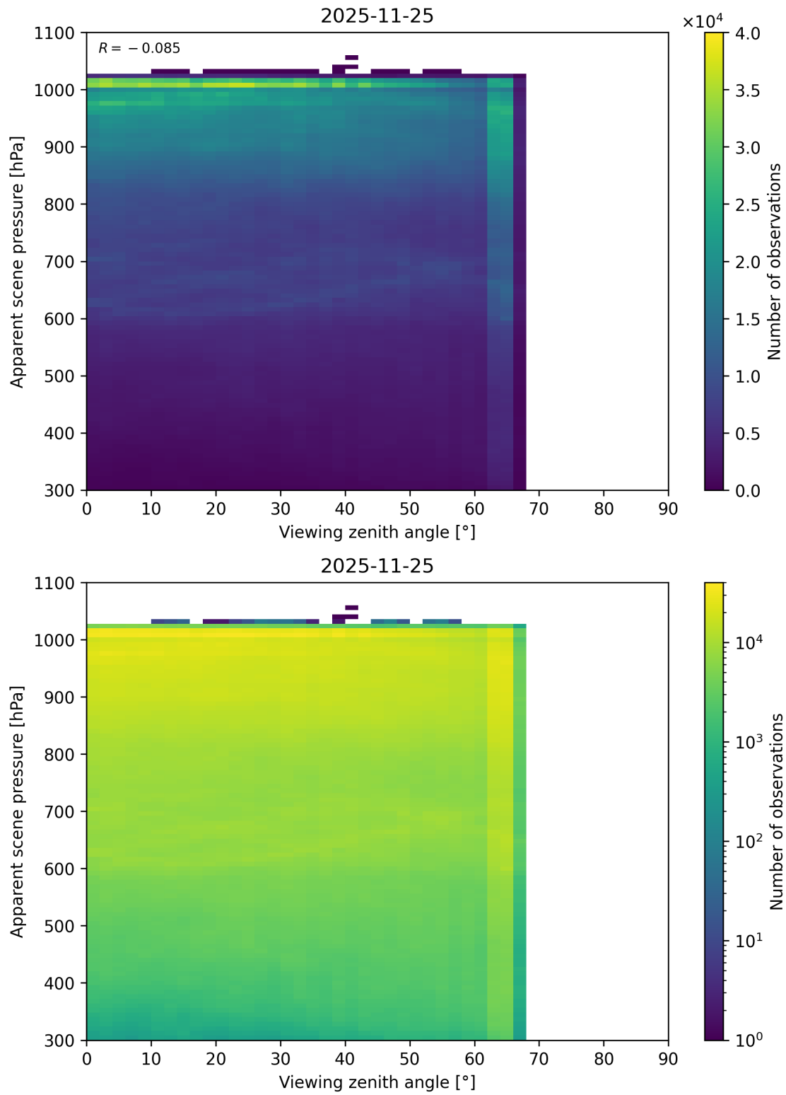
Figure 118: Scatter density plot of “Viewing zenith angle” against “Apparent scene pressure” for 2025-11-24 to 2025-11-26.
