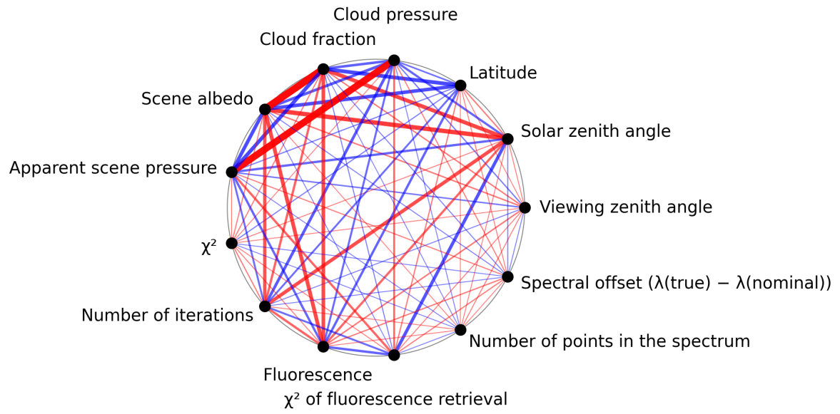
Figure 1: Map of correlation graph for 2025-11-24 to 2025-11-26.
