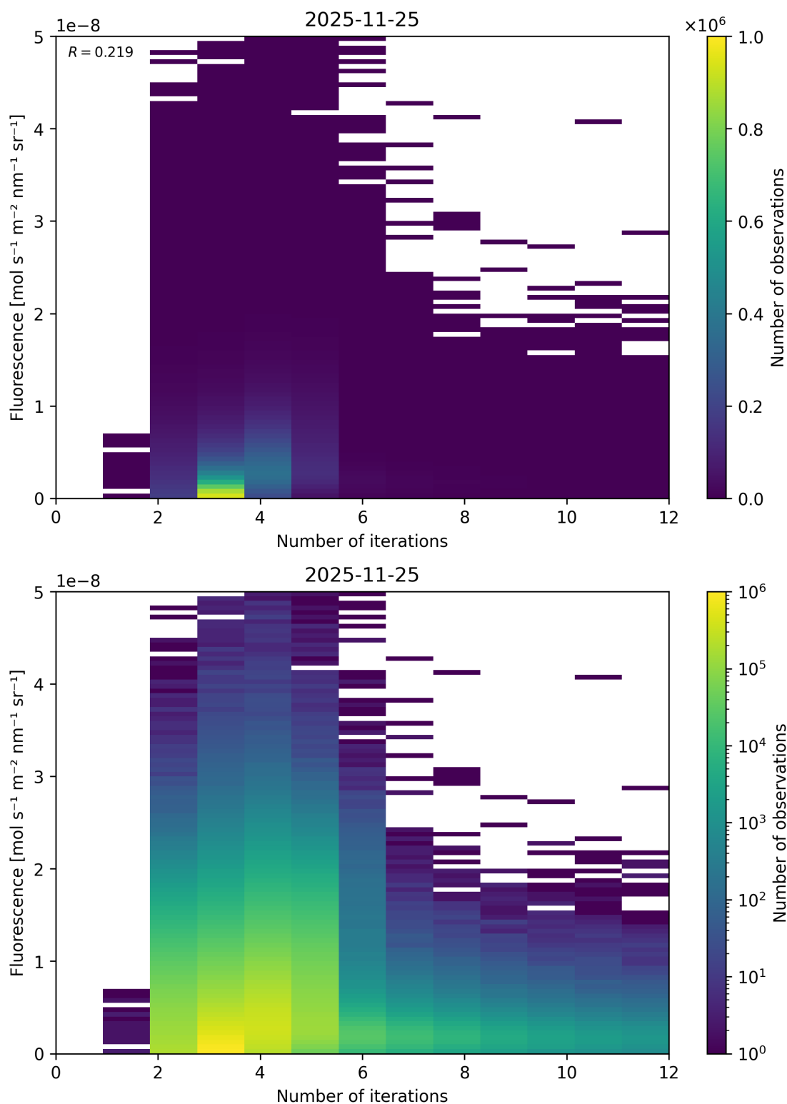
Figure 98: Scatter density plot of “Number of iterations” against “Fluorescence” for 2025-11-24 to 2025-11-26.
