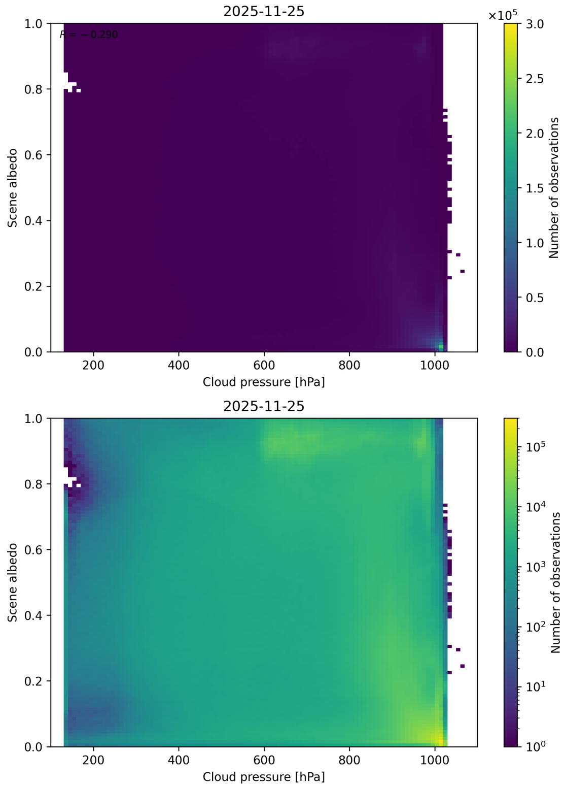
Figure 83: Scatter density plot of “Cloud pressure” against “Scene albedo” for 2025-11-24 to 2025-11-26.
