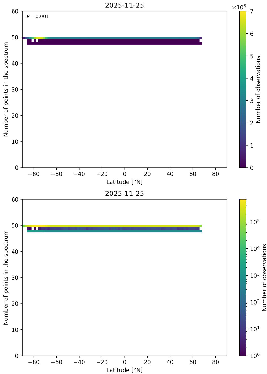
Figure 94: Scatter density plot of “Latitude” against “Number of points in the spectrum” for 2025-11-24 to 2025-11-26.
