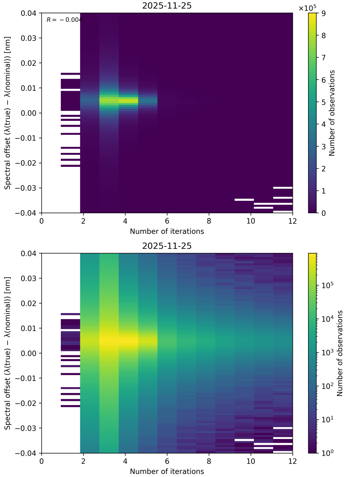
Figure 100: Scatter density plot of “Number of iterations” against “Spectral offset ( \lambda_{\text{true}} - \lambda_{\text{nominal}} )” for 2025-11-24 to 2025-11-26.
