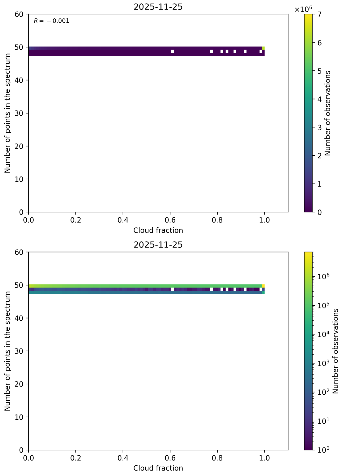
Figure 74: Scatter density plot of “Cloud fraction” against “Number of points in the spectrum” for 2025-11-24 to 2025-11-26.
