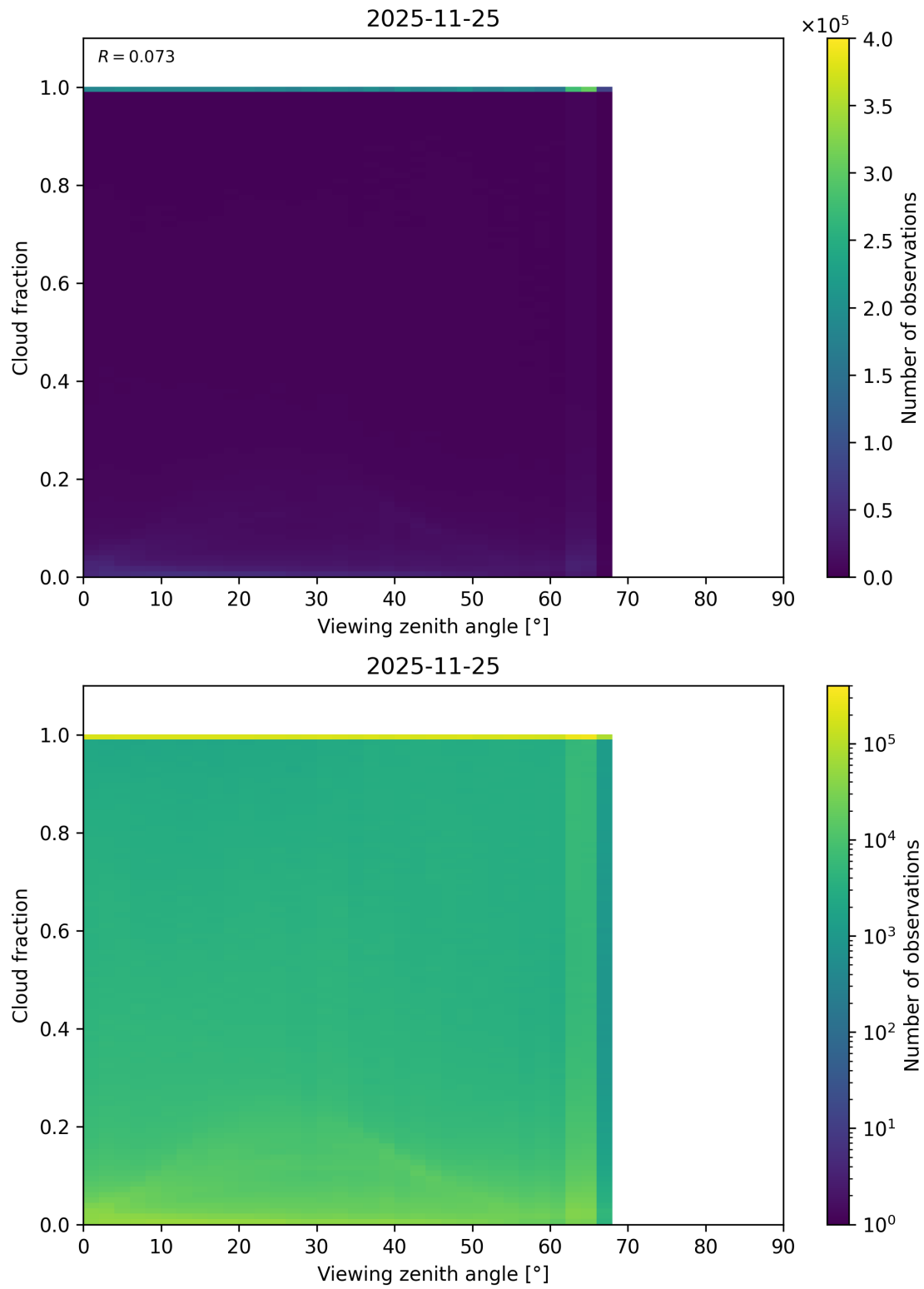
Figure 120: Scatter density plot of “Viewing zenith angle” against “Cloud fraction” for 2025-11-24 to 2025-11-26.
