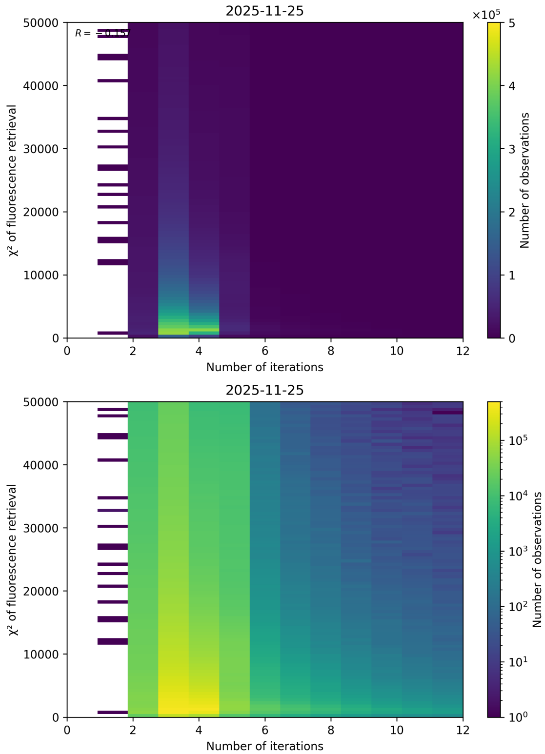
Figure 97: Scatter density plot of “Number of iterations” against “ \chi^2 of fluorescence retrieval” for 2025-11-24 to 2025-11-26.
