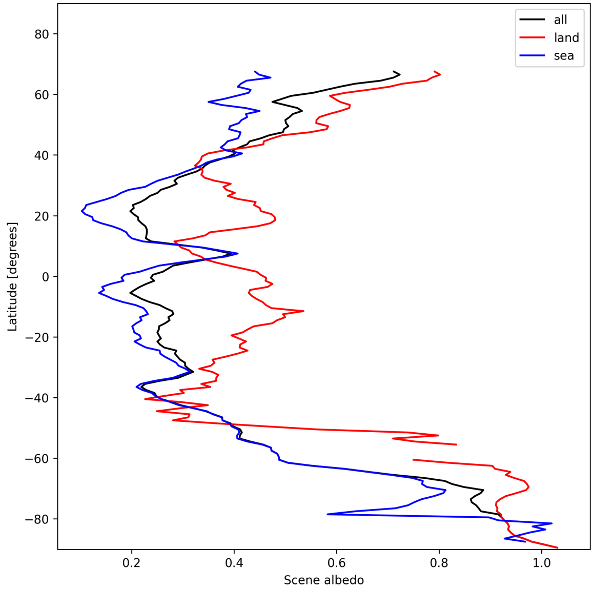
Figure 17: Zonal average of "Scene albedo" for 2025-11-24 to 2025-11-26.
