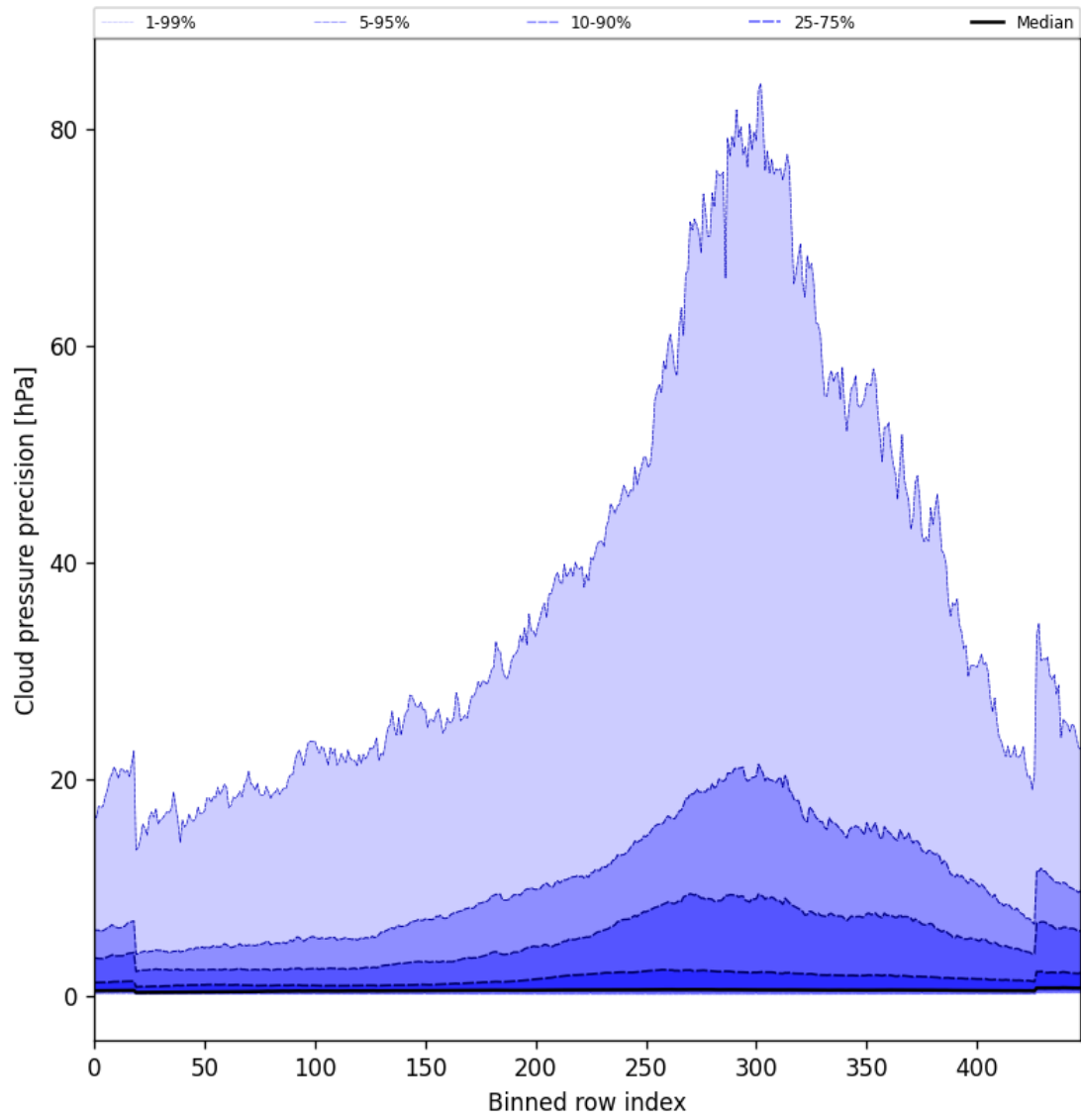
Figure 48: Along track statistics of “Cloud pressure precision” for 2025-11-24 to 2025-11-26
