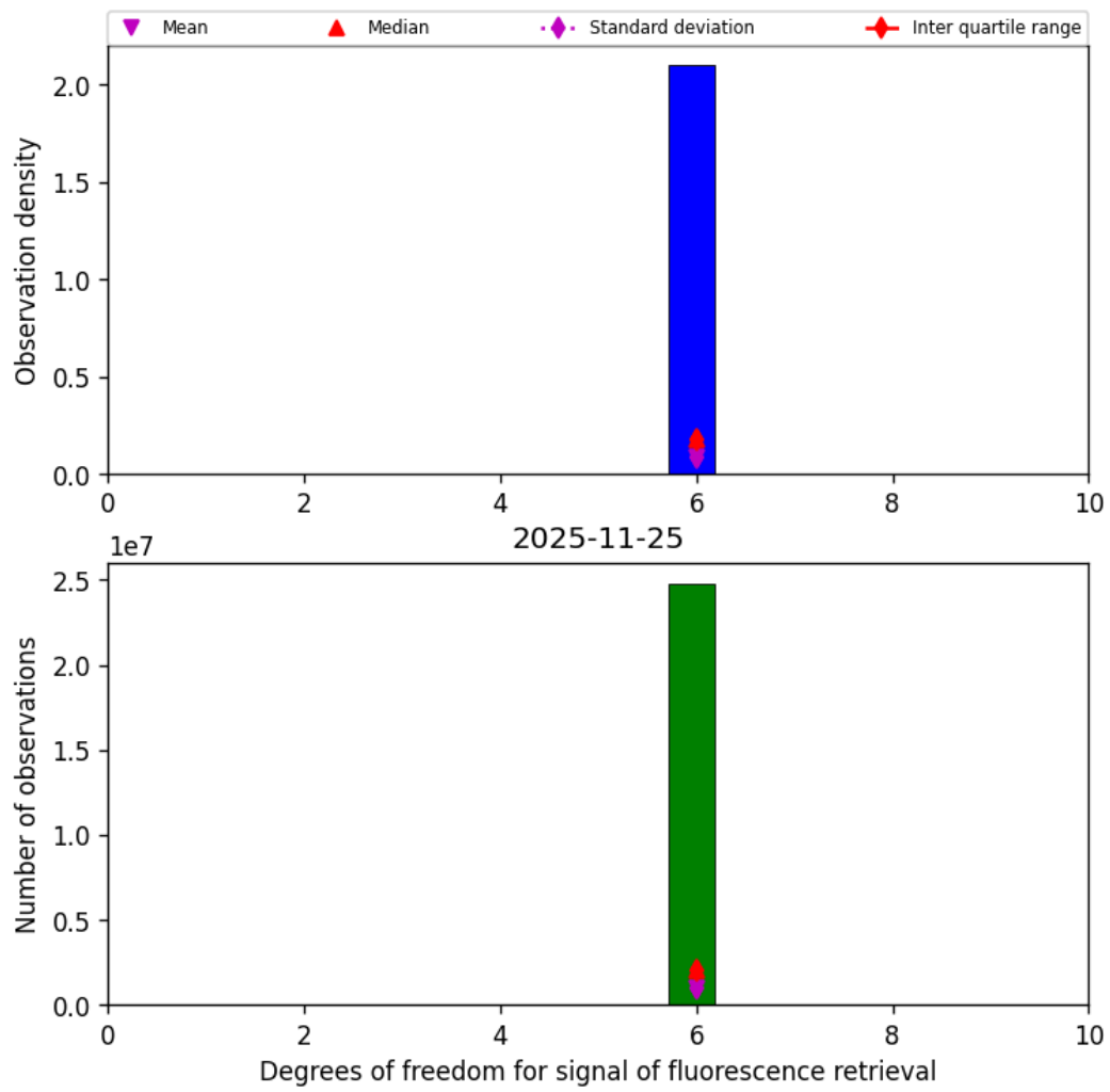
Figure 43: Histogram of "Degrees of freedom for signal of fluorescence retrieval" for 2025-11-24 to 2025-11-26
