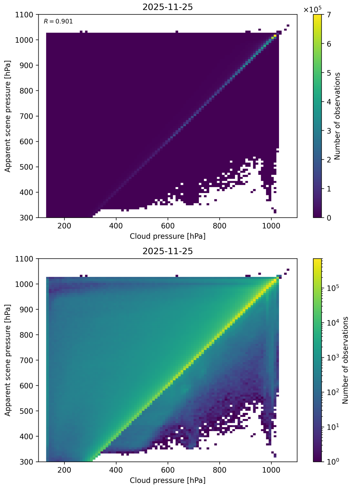
Figure 77: Scatter density plot of “Cloud pressure” against “Apparent scene pressure” for 2025-11-24 to 2025-11-26.
