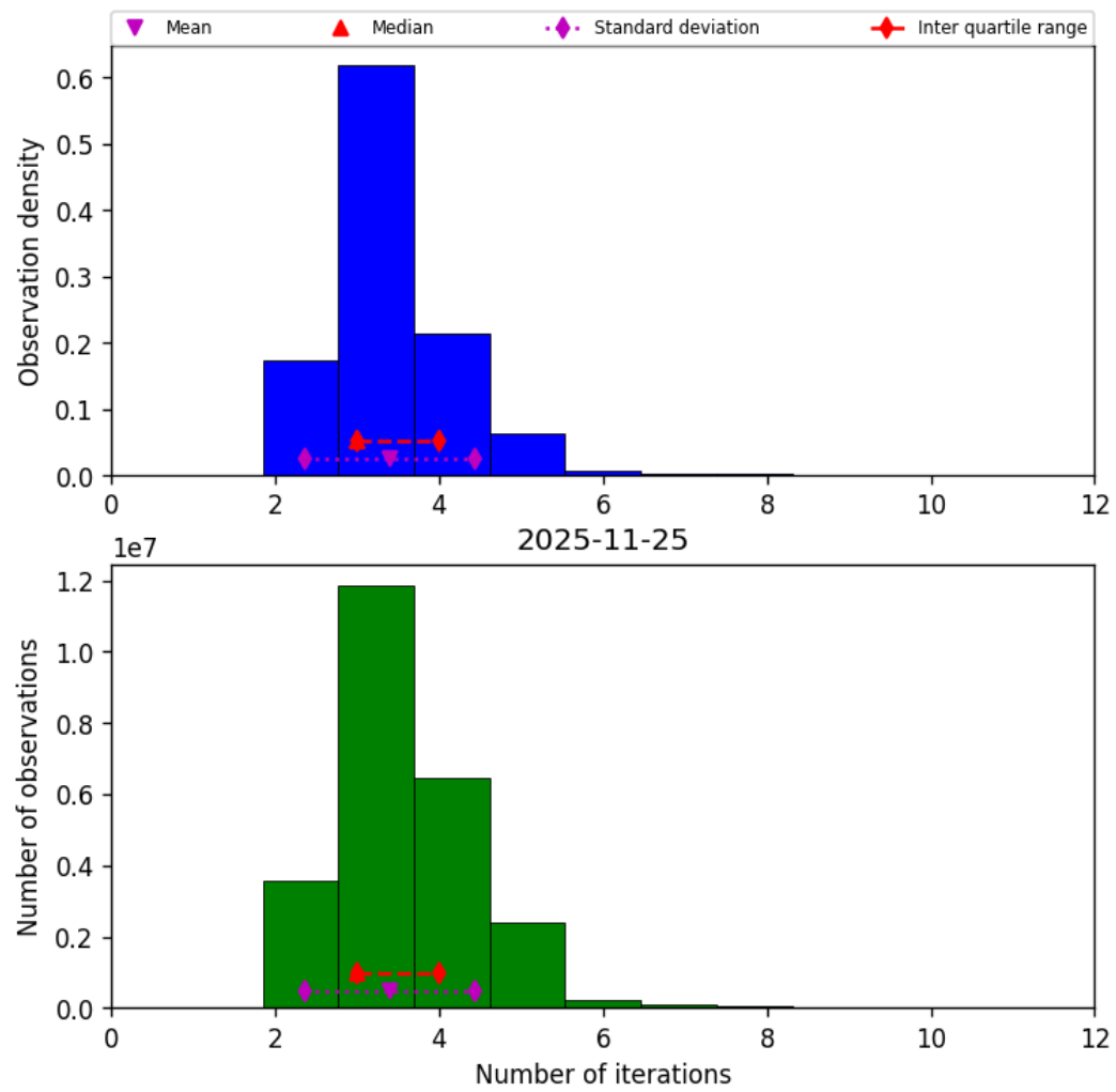
Figure 39: Histogram of “Number of iterations” for 2025-11-24 to 2025-11-26
