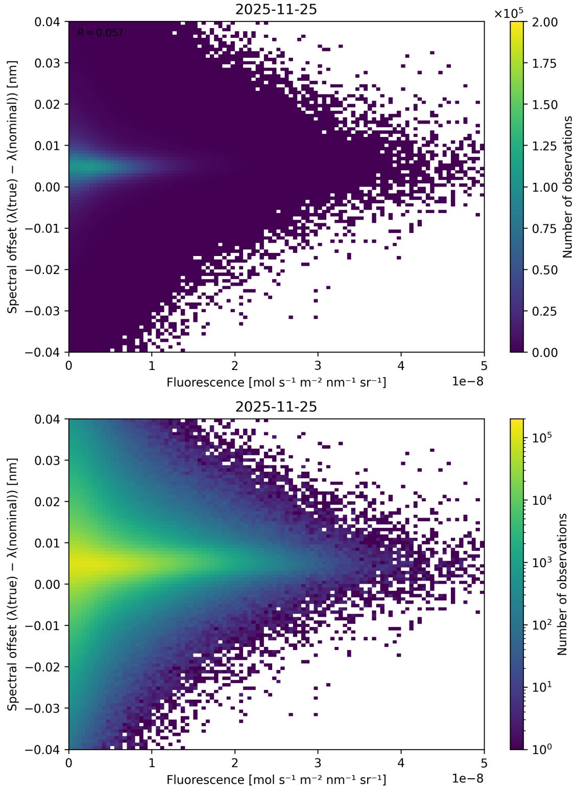
Figure 87: Scatter density plot of “Fluorescence” against “Spectral offset ( \lambda_{\text{true}} - \lambda_{\text{nominal}} )” for 2025-11-24 to 2025-11-26.
