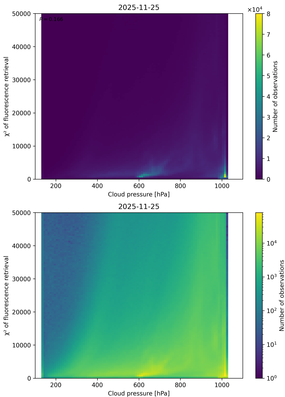
Figure 78: Scatter density plot of “Cloud pressure” against “ \chi^2 of fluorescence retrieval” for 2025-11-24 to 2025-11-26.
