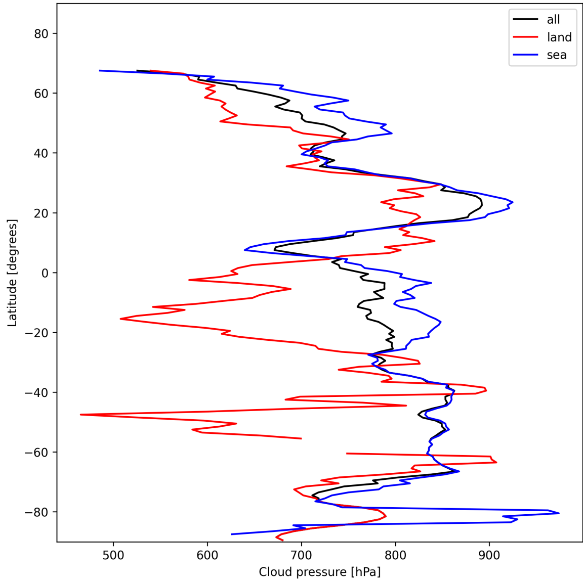
Figure 13: Zonal average of “Cloud pressure” for 2025-11-24 to 2025-11-26.
