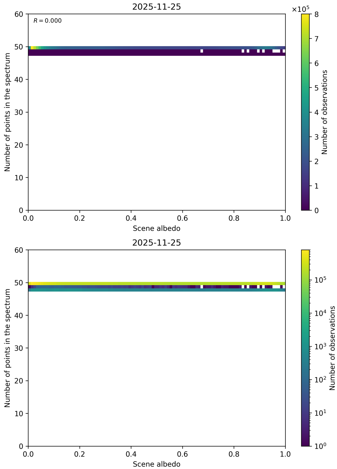
Figure 106: Scatter density plot of “Scene albedo” against “Number of points in the spectrum” for 2025-11-24 to 2025-11-26.
