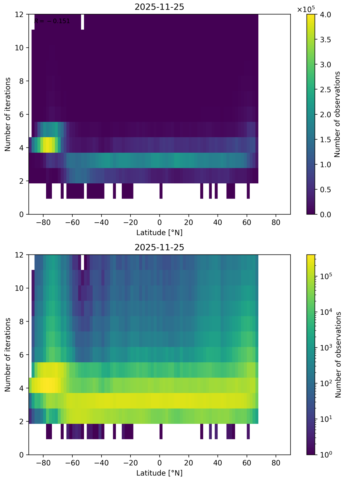
Figure 93: Scatter density plot of “Latitude” against “Number of iterations” for 2025-11-24 to 2025-11-26.
