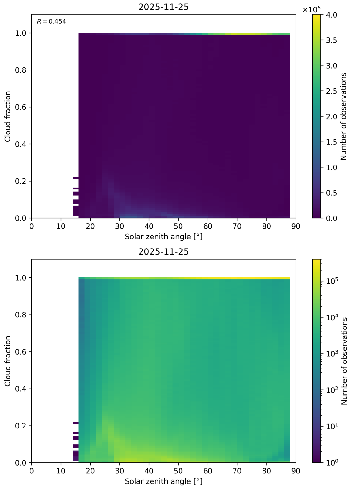
Figure 110: Scatter density plot of “Solar zenith angle” against “Cloud fraction” for 2025-11-24 to 2025-11-26.
