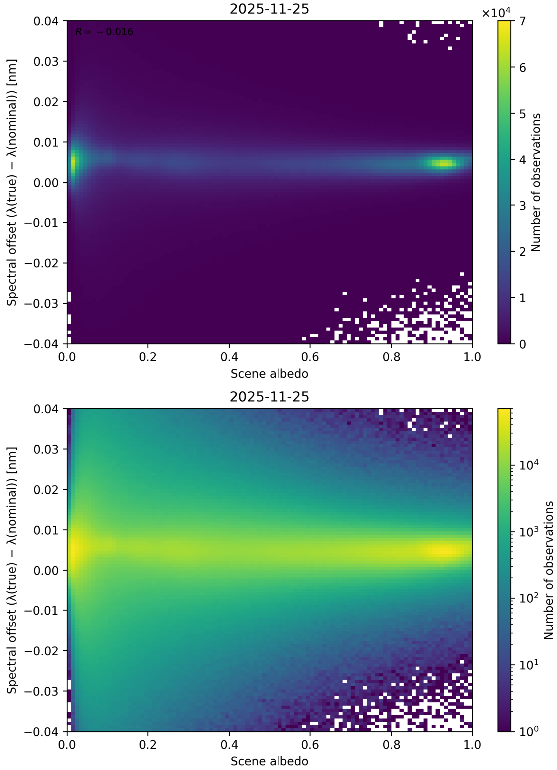
Figure 107: Scatter density plot of “Scene albedo” against “Spectral offset ( \lambda_{\text{true}} - \lambda_{\text{nominal}} )” for 2025-11-24 to 2025-11-26.
