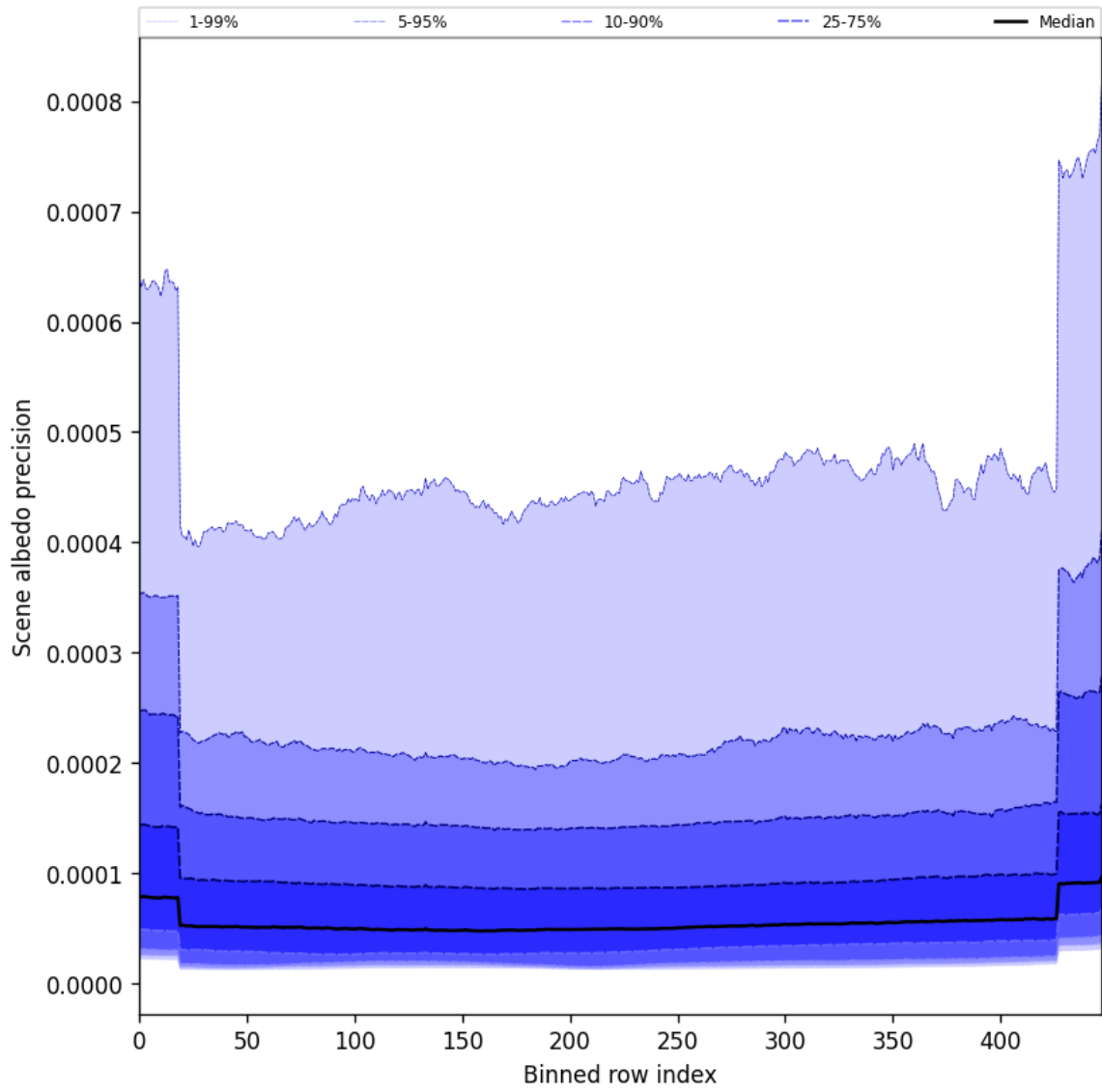
Figure 52: Along track statistics of “Scene albedo precision” for 2025-11-24 to 2025-11-26
