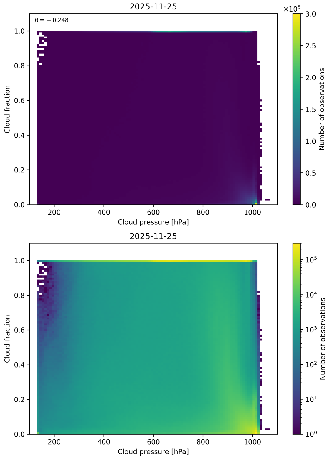
Figure 79: Scatter density plot of “Cloud pressure” against “Cloud fraction” for 2025-11-24 to 2025-11-26.
