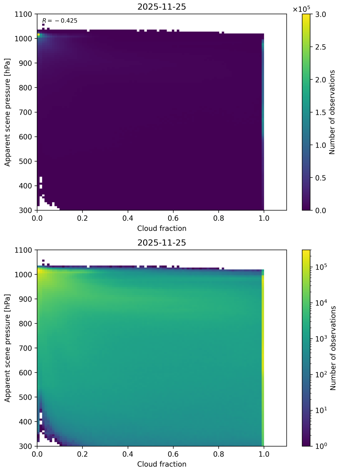
Figure 70: Scatter density plot of “Cloud fraction” against “Apparent scene pressure” for 2025-11-24 to 2025-11-26.
