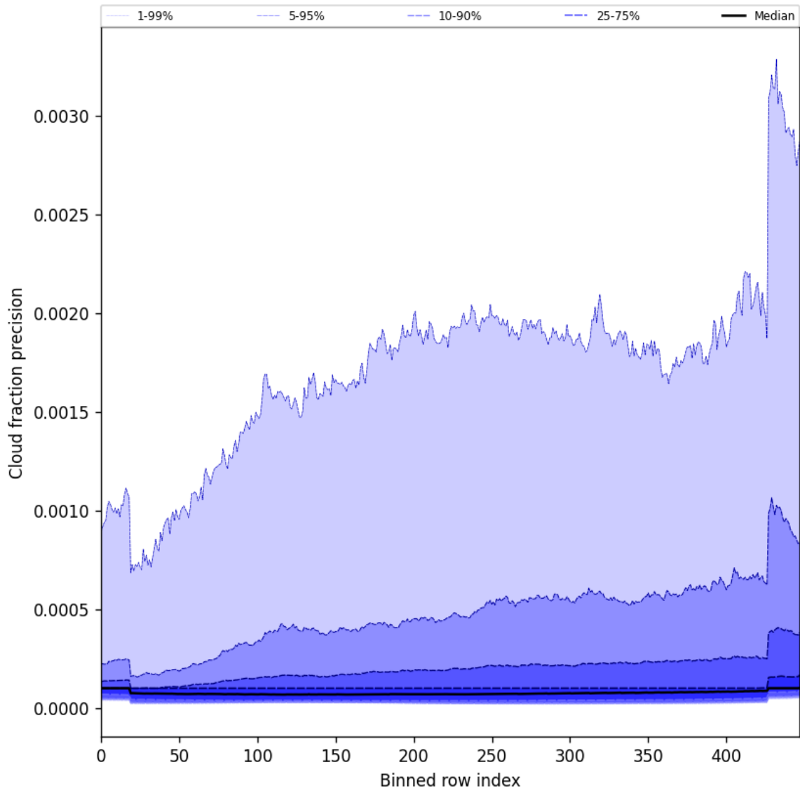
Figure 50: Along track statistics of “Cloud fraction precision” for 2025-11-24 to 2025-11-26
