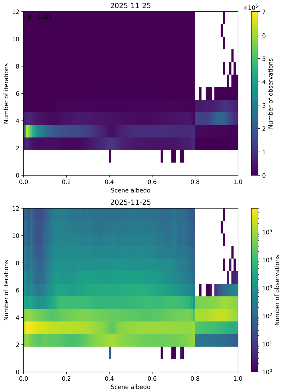
Figure 105: Scatter density plot of “Scene albedo” against “Number of iterations” for 2025-11-24 to 2025-11-26.
