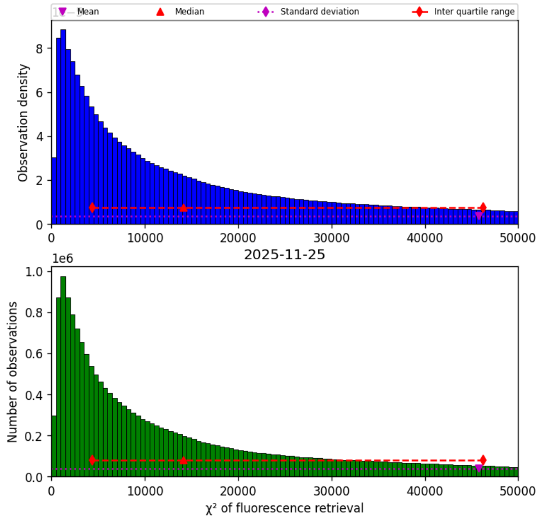
Figure 42: Histogram of “ \chi^2 of fluorescence retrieval” for 2025-11-24 to 2025-11-26
