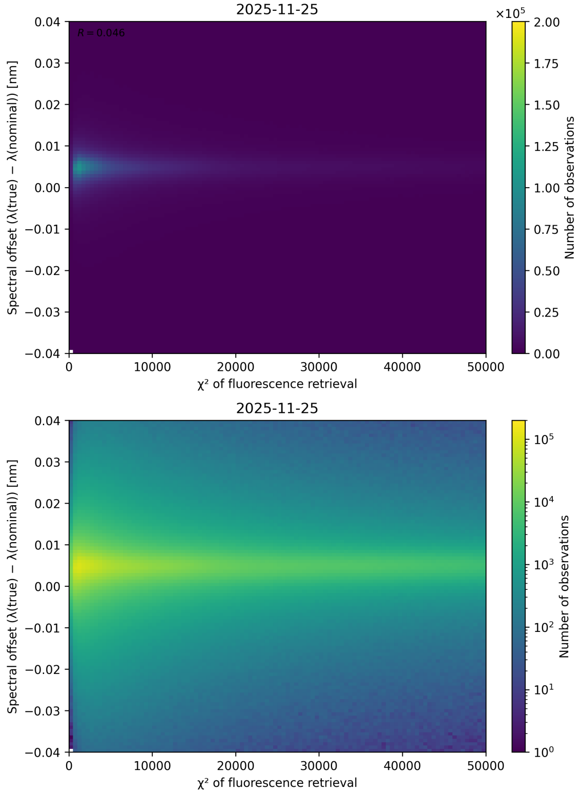
Figure 69: Scatter density plot of “ \chi^2 of fluorescence retrieval” against “Spectral offset ( \lambda_{\text{true}} - \lambda_{\text{nominal}} )” for 2025-11-24 to 2025-11-26.
