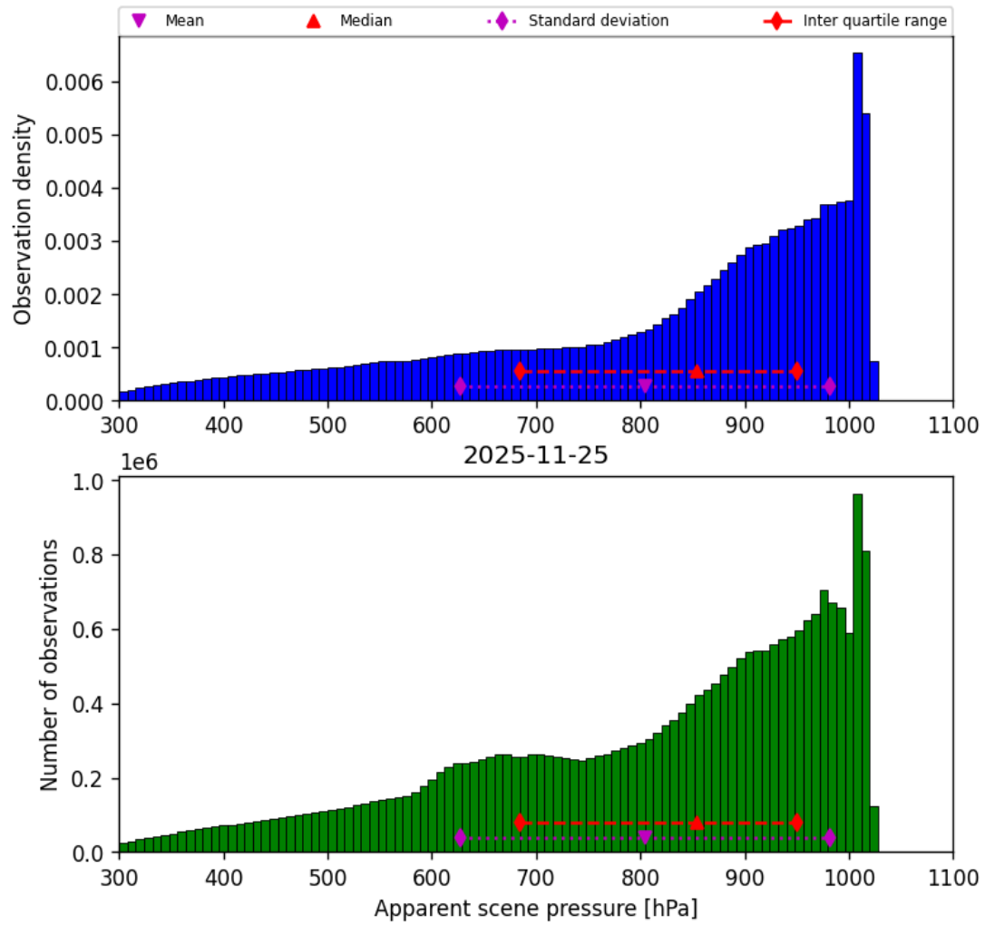
Figure 36: Histogram of “Apparent scene pressure” for 2025-11-24 to 2025-11-26
