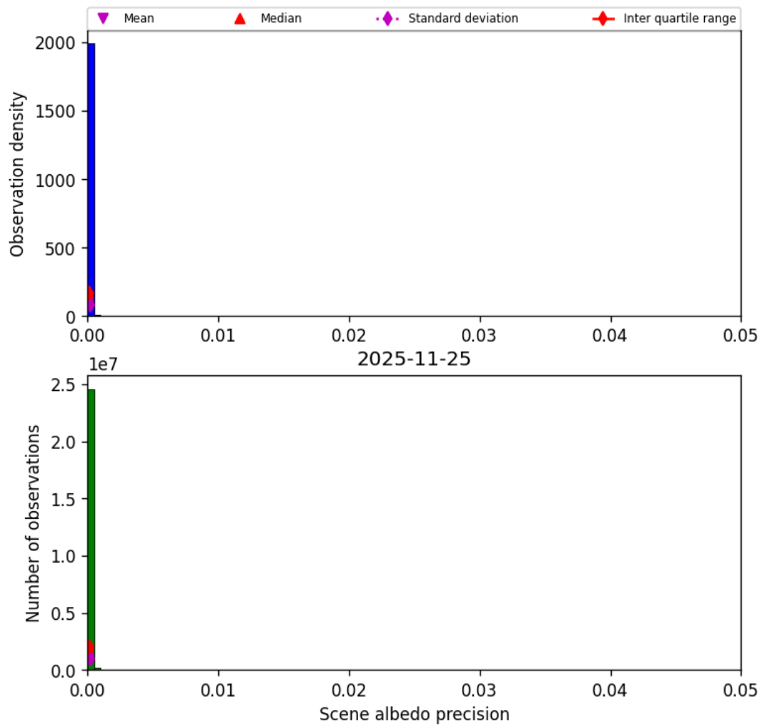
Figure 35: Histogram of “Scene albedo precision” for 2025-11-24 to 2025-11-26
