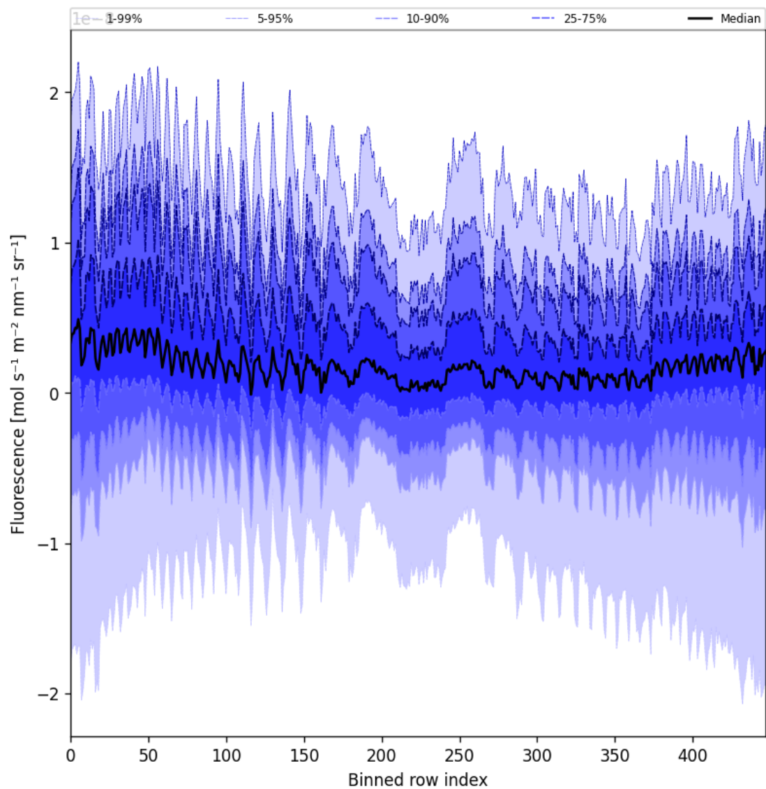
Figure 57: Along track statistics of “Fluorescence” for 2025-11-24 to 2025-11-26
