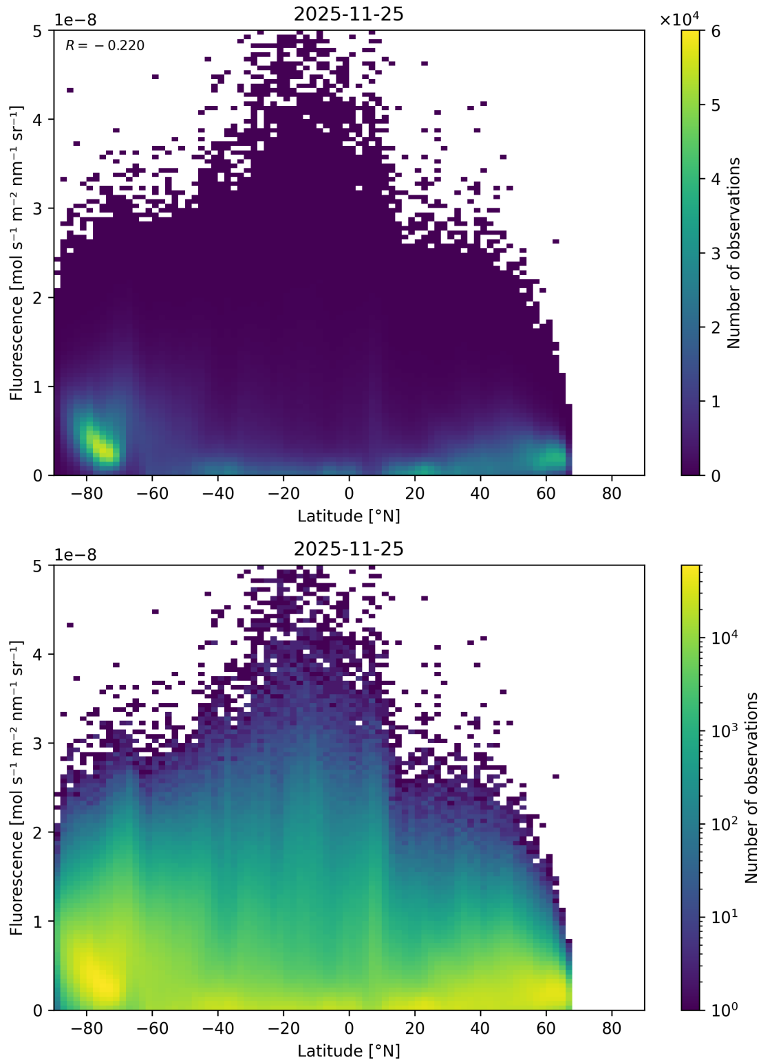
Figure 92: Scatter density plot of “Latitude” against “Fluorescence” for 2025-11-24 to 2025-11-26.
