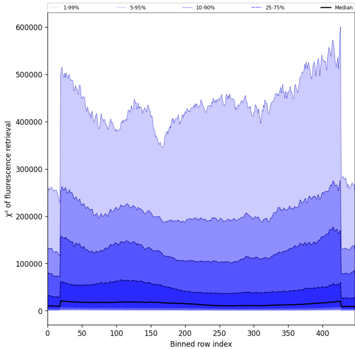
Figure 59: Along track statistics of “ \chi^2 of fluorescence retrieval” for 2025-11-24 to 2025-11-26
