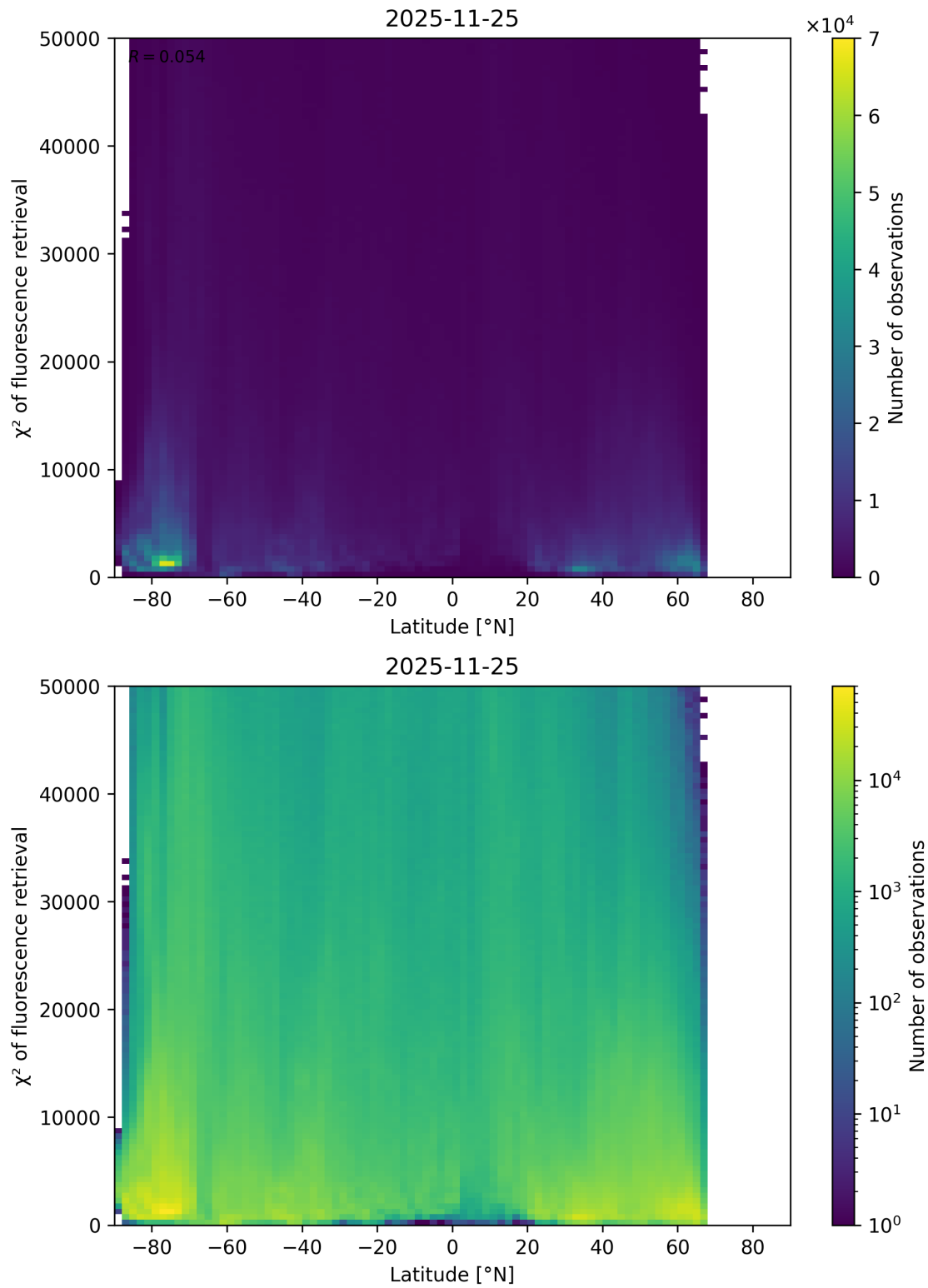
Figure 89: Scatter density plot of “Latitude” against “ \chi^2 of fluorescence retrieval” for 2025-11-24 to 2025-11-26.
