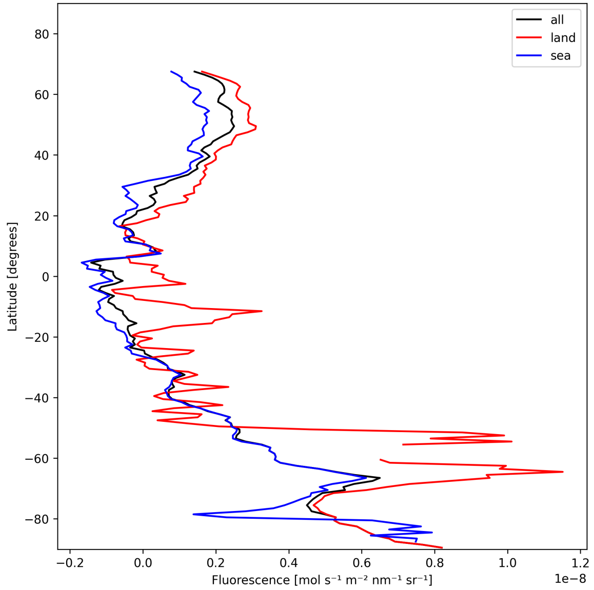
Figure 23: Zonal average of “Fluorescence” for 2025-11-24 to 2025-11-26.
