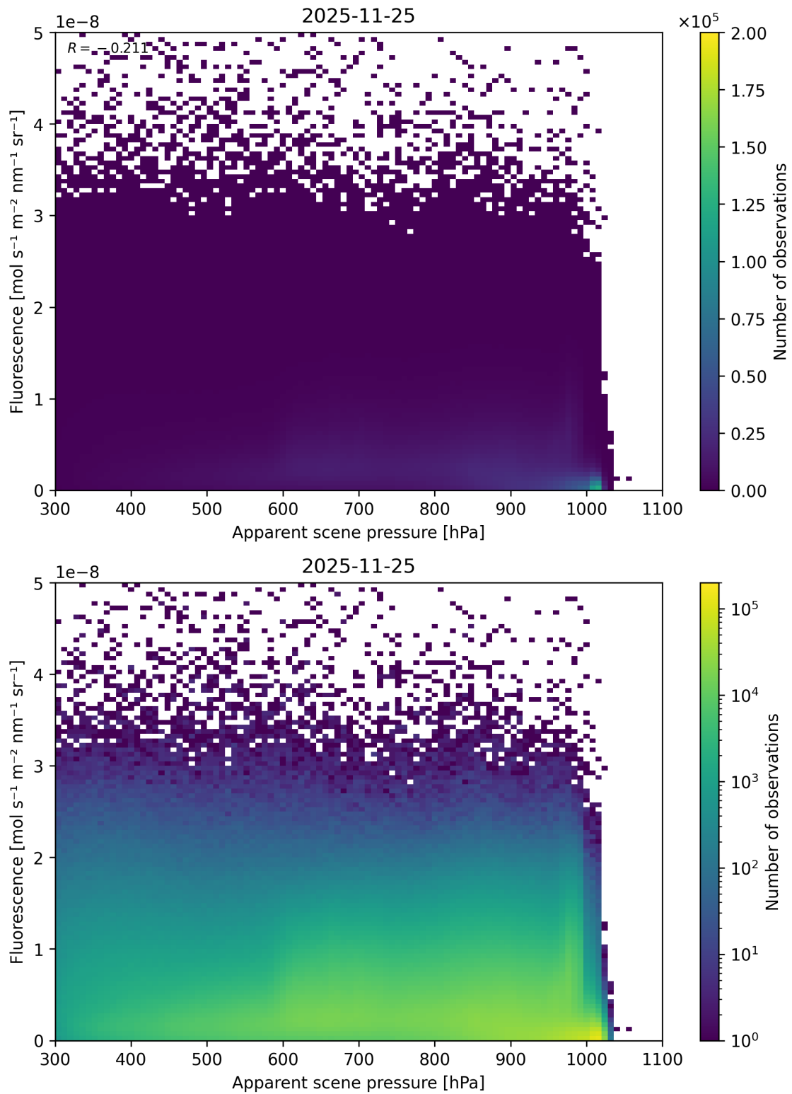
Figure 64: Scatter density plot of “Apparent scene pressure” against “Fluorescence” for 2025-11-24 to 2025-11-26.
