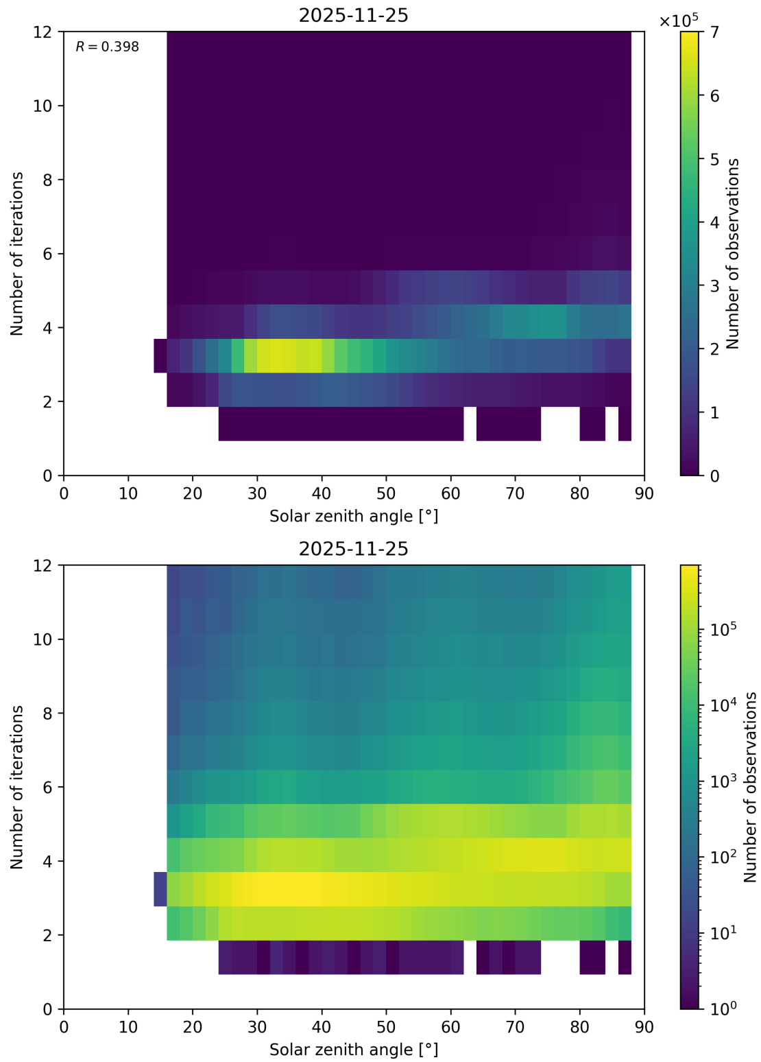
Figure 114: Scatter density plot of “Solar zenith angle” against “Number of iterations” for 2025-11-24 to 2025-11-26.
