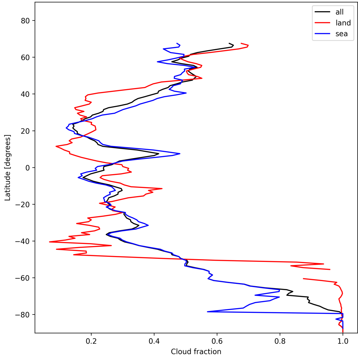
Figure 15: Zonal average of “Cloud fraction” for 2025-11-24 to 2025-11-26.
