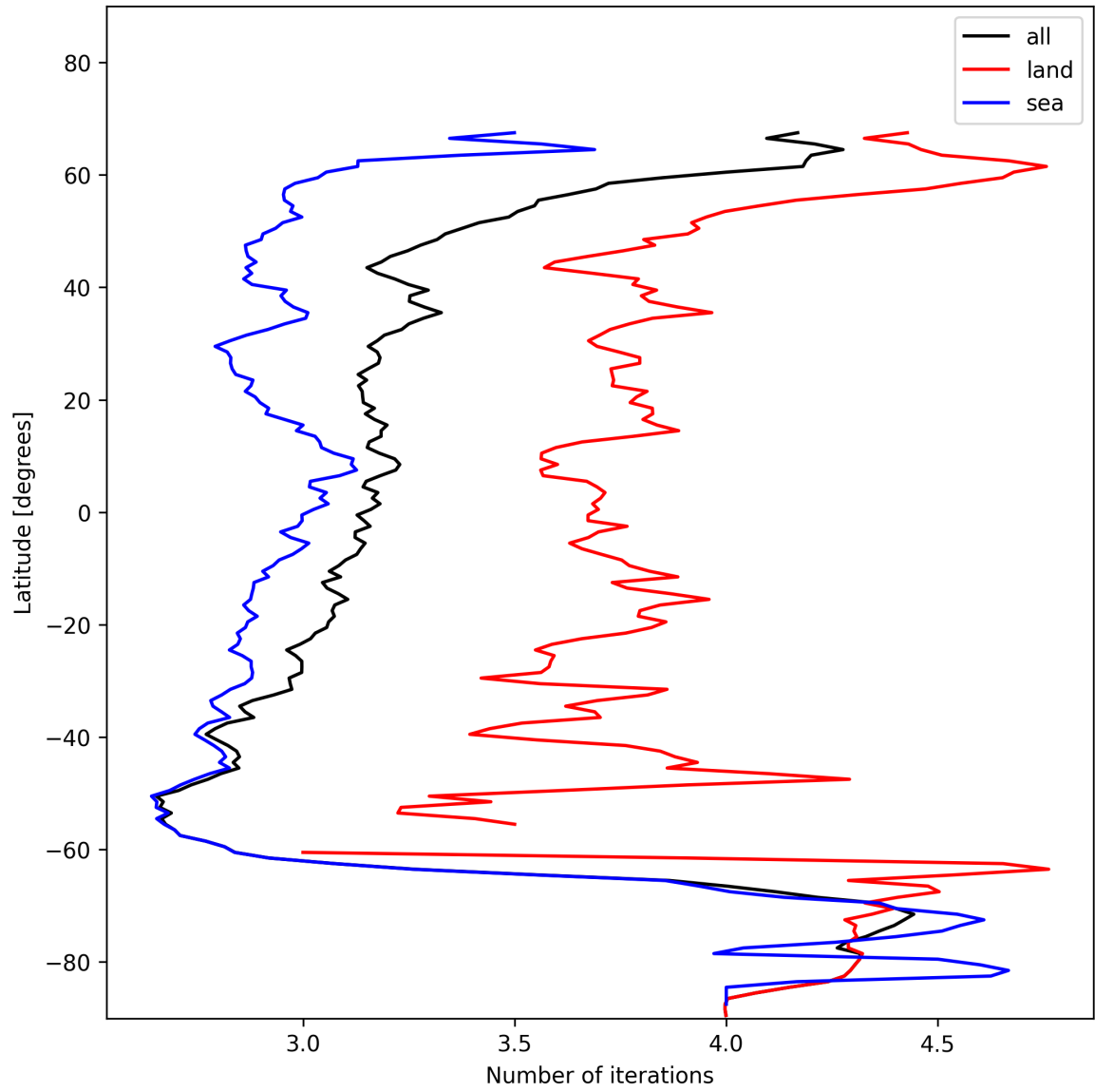
Figure 22: Zonal average of “Number of iterations” for 2025-11-24 to 2025-11-26.
