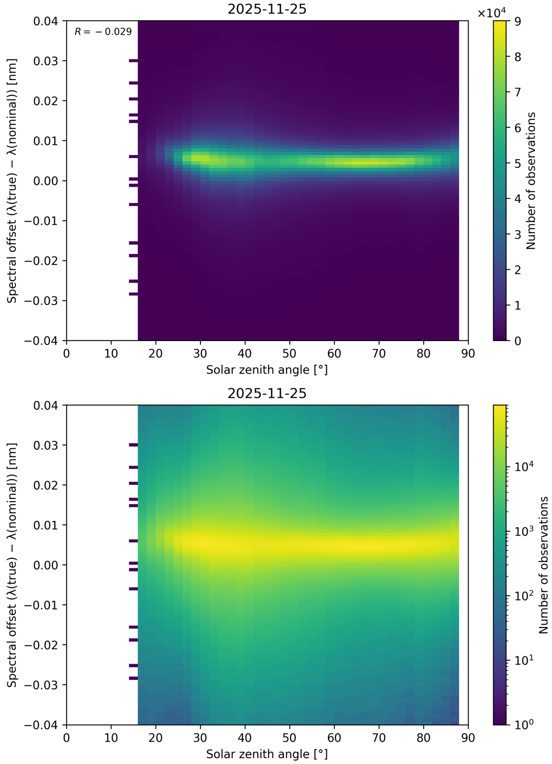
Figure 117: Scatter density plot of “Solar zenith angle” against “Spectral offset ( \lambda_{\text{true}} - \lambda_{\text{nominal}} )” for 2025-11-24 to 2025-11-26.
