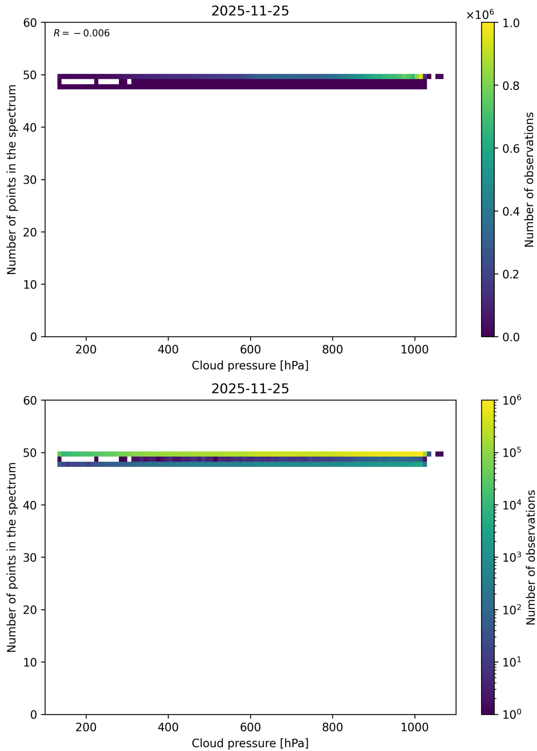
Figure 82: Scatter density plot of “Cloud pressure” against “Number of points in the spectrum” for 2025-11-24 to 2025-11-26.
