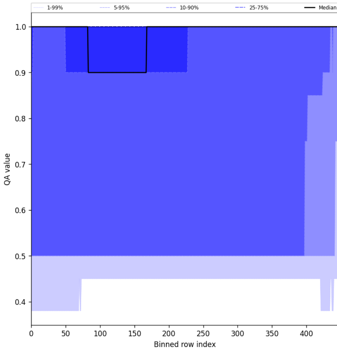
Figure 46: Along track statistics of “QA value” for 2025-11-24 to 2025-11-26
