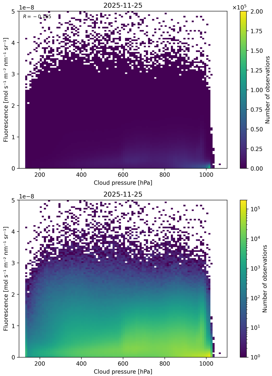
Figure 80: Scatter density plot of “Cloud pressure” against “Fluorescence” for 2025-11-24 to 2025-11-26.
