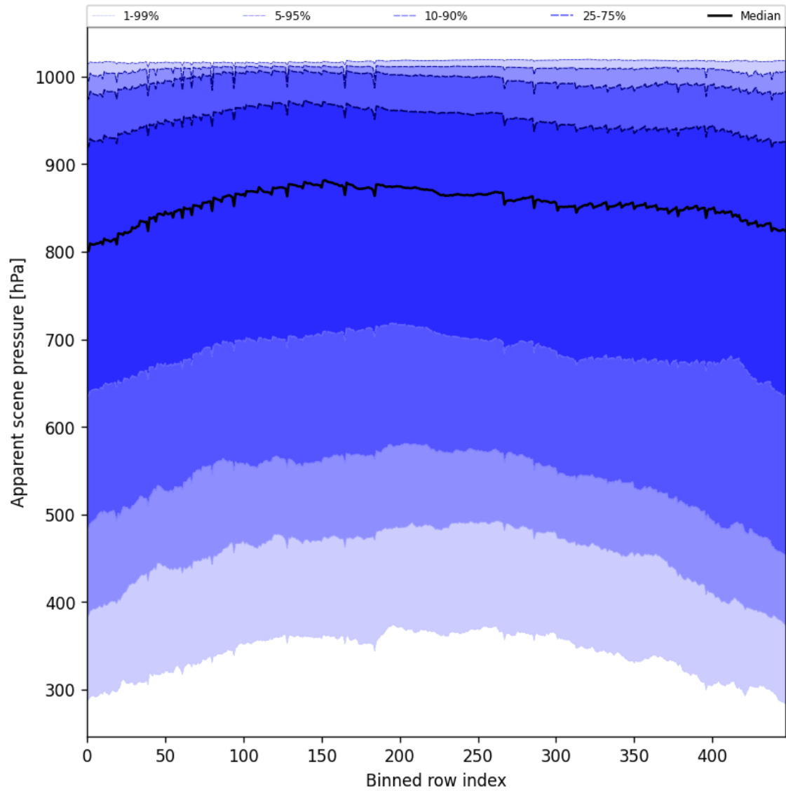
Figure 53: Along track statistics of “Apparent scene pressure” for 2025-11-24 to 2025-11-26
