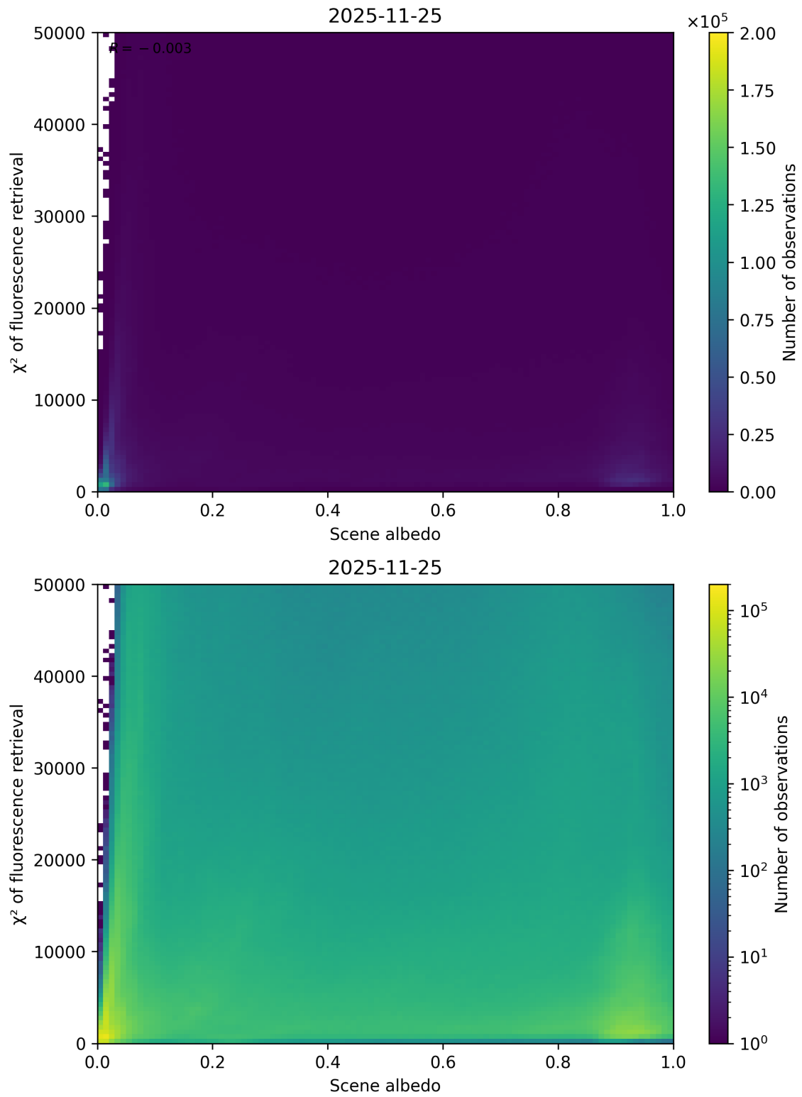
Figure 103: Scatter density plot of “Scene albedo” against “ \chi^2 of fluorescence retrieval” for 2025-11-24 to 2025-11-26.
