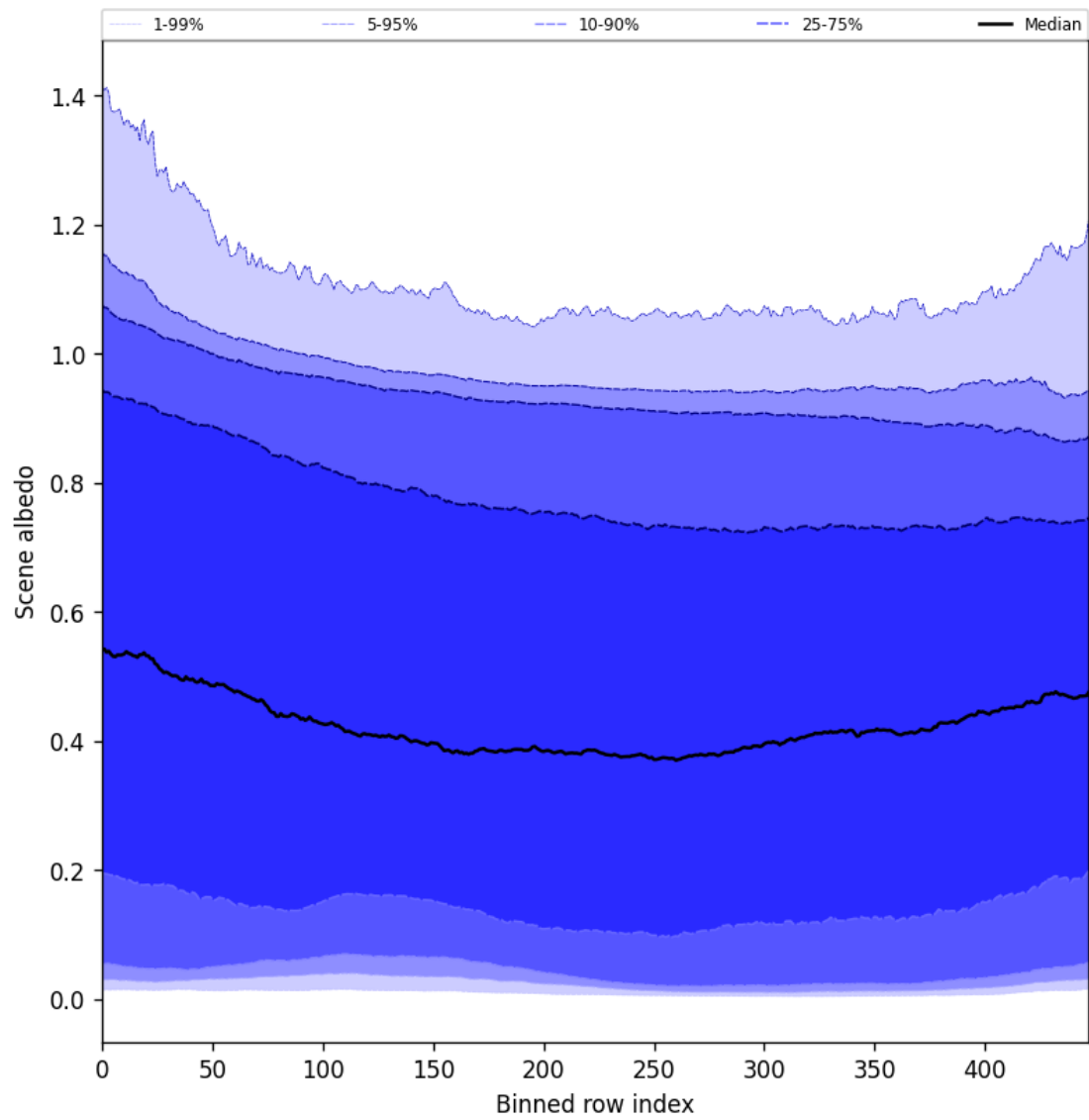
Figure 51: Along track statistics of “Scene albedo” for 2025-11-24 to 2025-11-26
