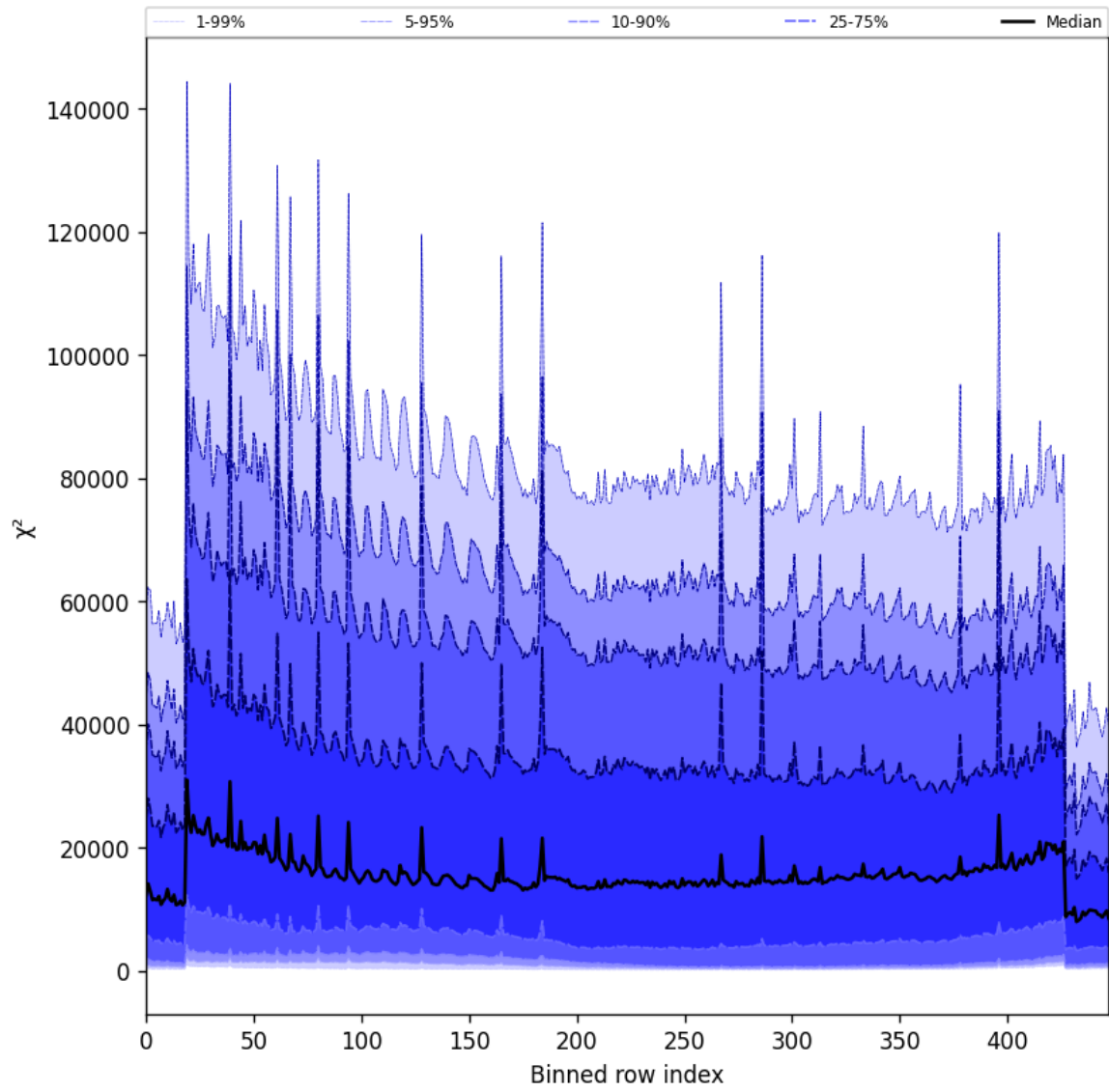
Figure 55: Along track statistics of “ \chi^2 ” for 2025-11-24 to 2025-11-26
