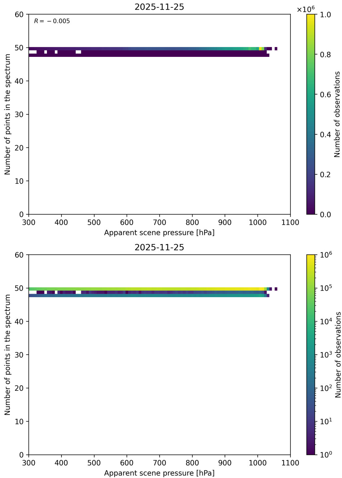
Figure 66: Scatter density plot of “Apparent scene pressure” against “Number of points in the spectrum” for 2025-11-24 to 2025-11-26.
