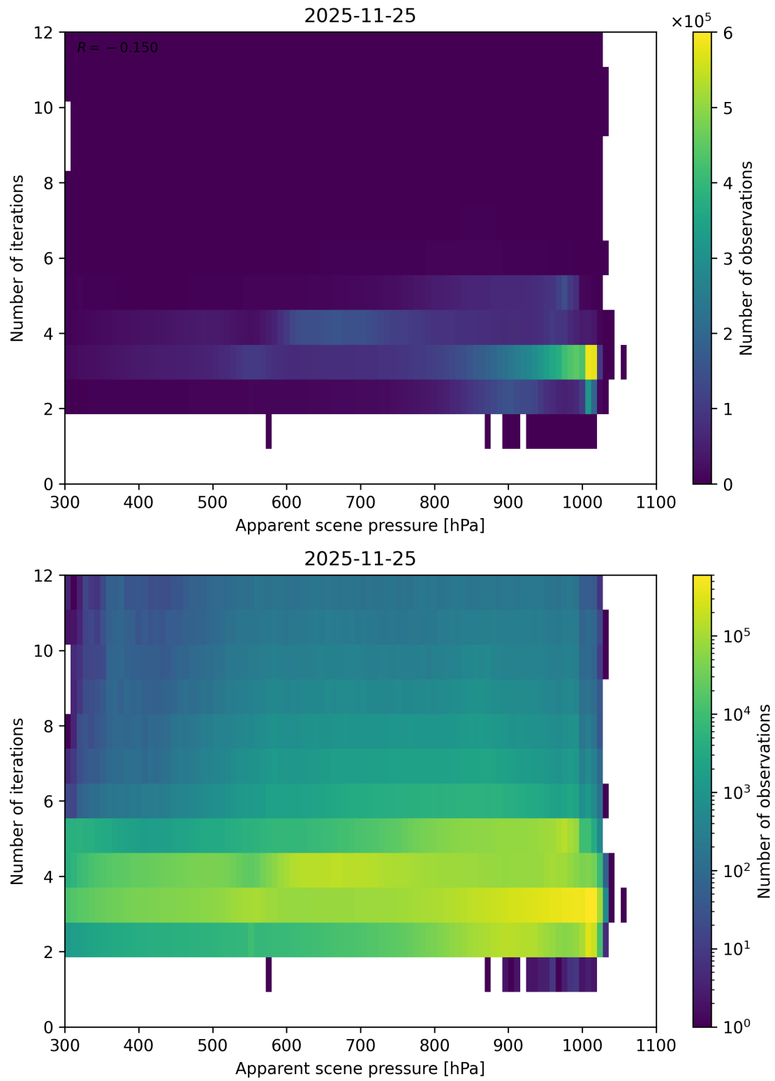
Figure 65: Scatter density plot of “Apparent scene pressure” against “Number of iterations” for 2025-11-24 to 2025-11-26.
