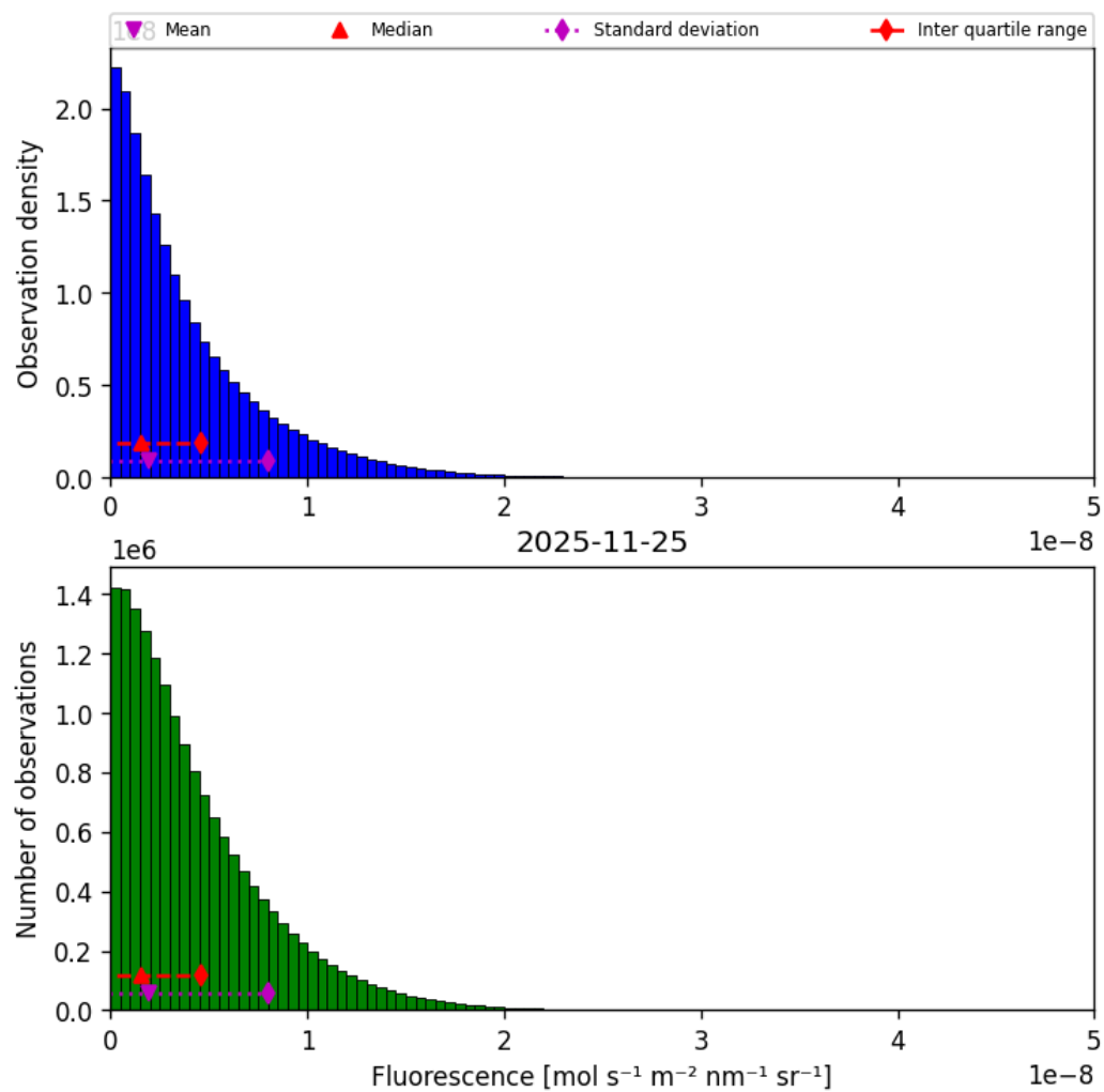
Figure 40: Histogram of “Fluorescence” for 2025-11-24 to 2025-11-26
