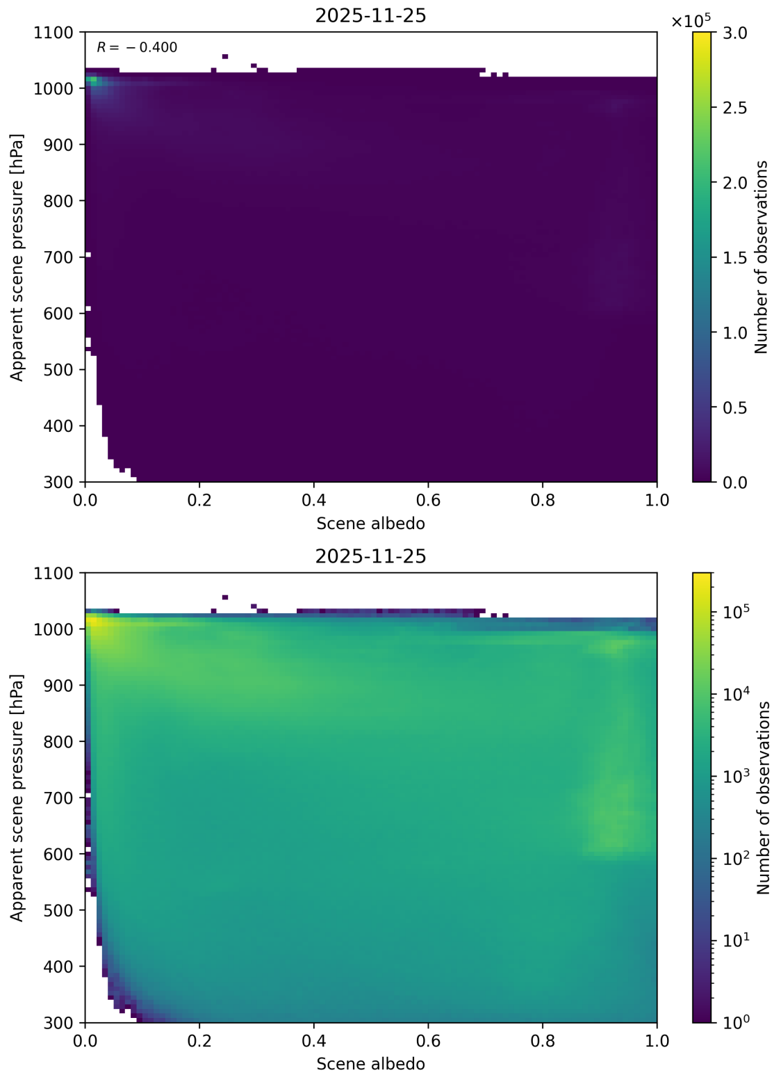
Figure 102: Scatter density plot of “Scene albedo” against “Apparent scene pressure” for 2025-11-24 to 2025-11-26.
