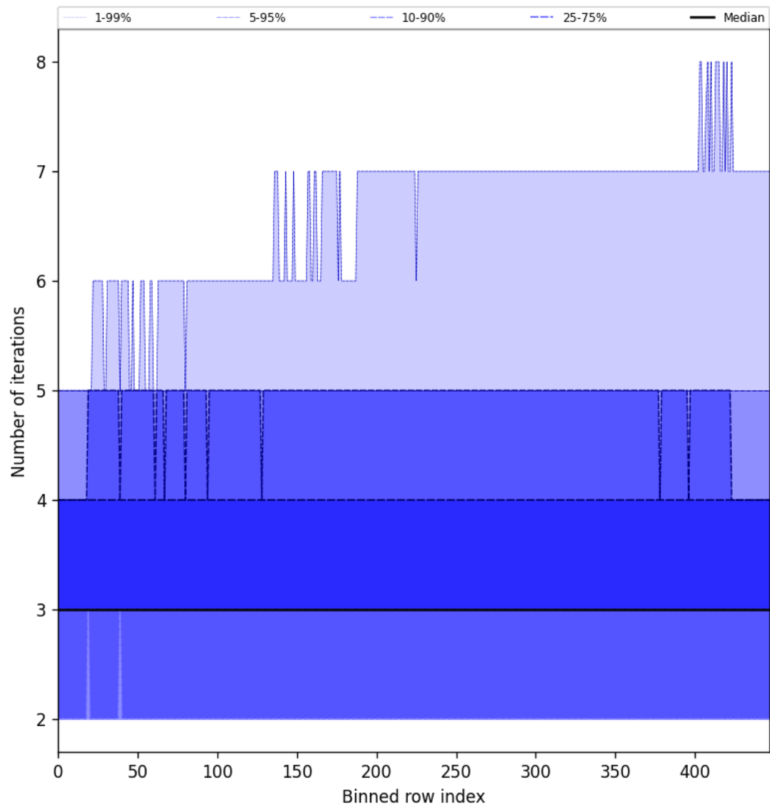
Figure 56: Along track statistics of “Number of iterations” for 2025-11-24 to 2025-11-26
