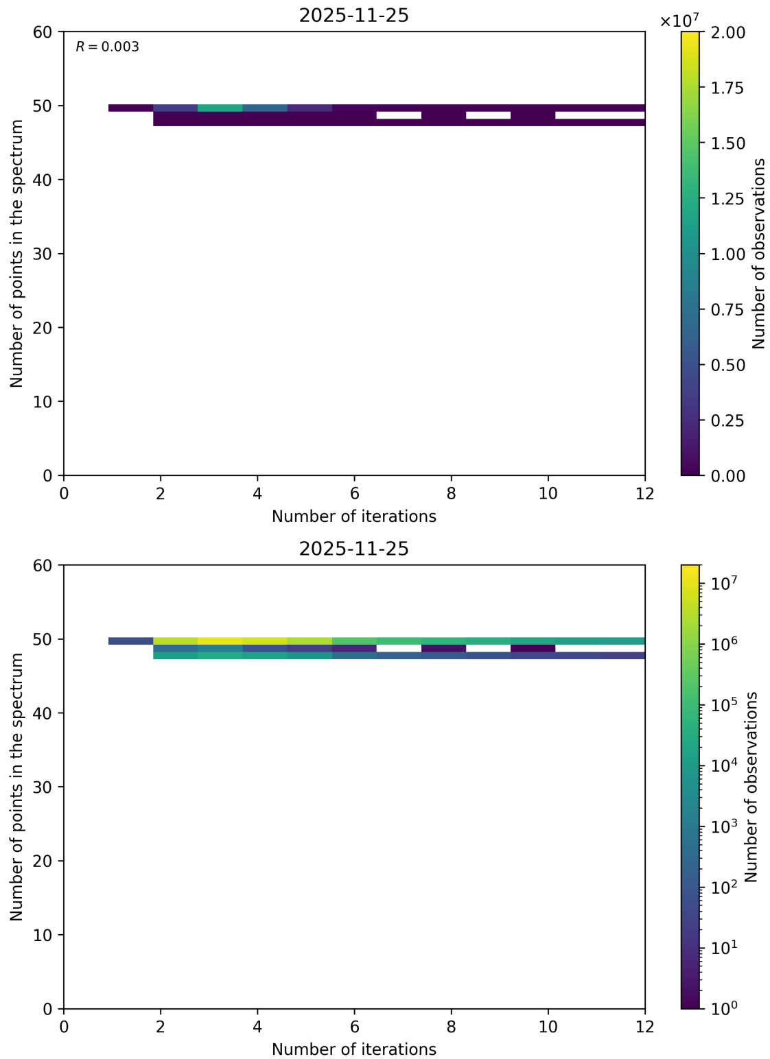
Figure 99: Scatter density plot of “Number of iterations” against “Number of points in the spectrum” for 2025-11-24 to 2025-11-26.
