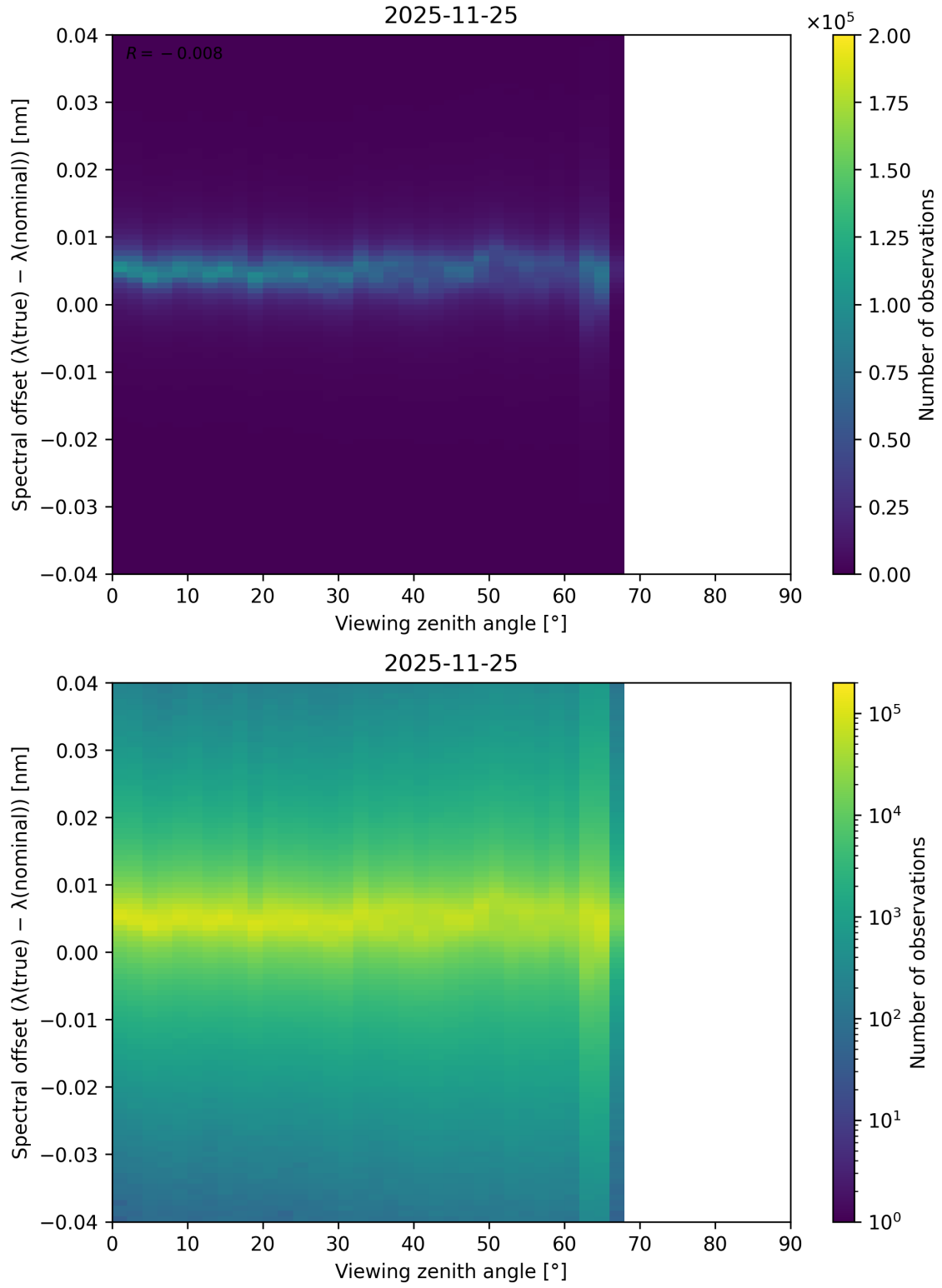
Figure 128: Scatter density plot of “Viewing zenith angle” against “Spectral offset ( \lambda_{\text{true}} - \lambda_{\text{nominal}} )” for 2025-11-24 to 2025-11-26.
