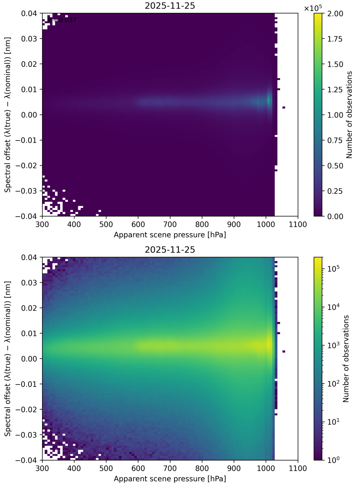
Figure 67: Scatter density plot of “Apparent scene pressure” against “Spectral offset ( \lambda_{\text{true}} - \lambda_{\text{nominal}} )” for 2025-11-24 to 2025-11-26.
