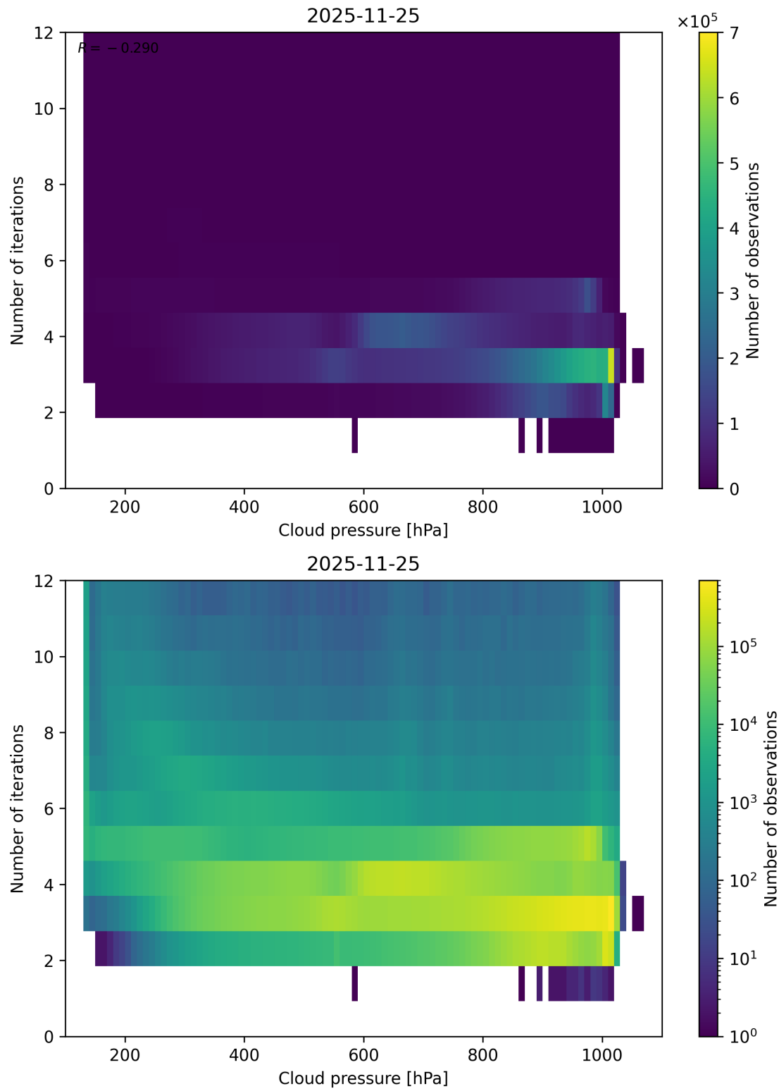
Figure 81: Scatter density plot of “Cloud pressure” against “Number of iterations” for 2025-11-24 to 2025-11-26.
