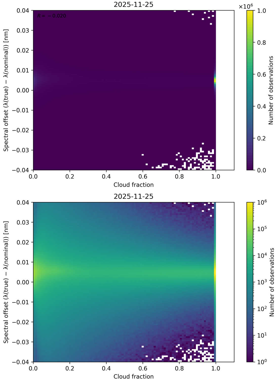
Figure 76: Scatter density plot of “Cloud fraction” against “Spectral offset ( \lambda_{\text{true}} - \lambda_{\text{nominal}} )” for 2025-11-24 to 2025-11-26.
