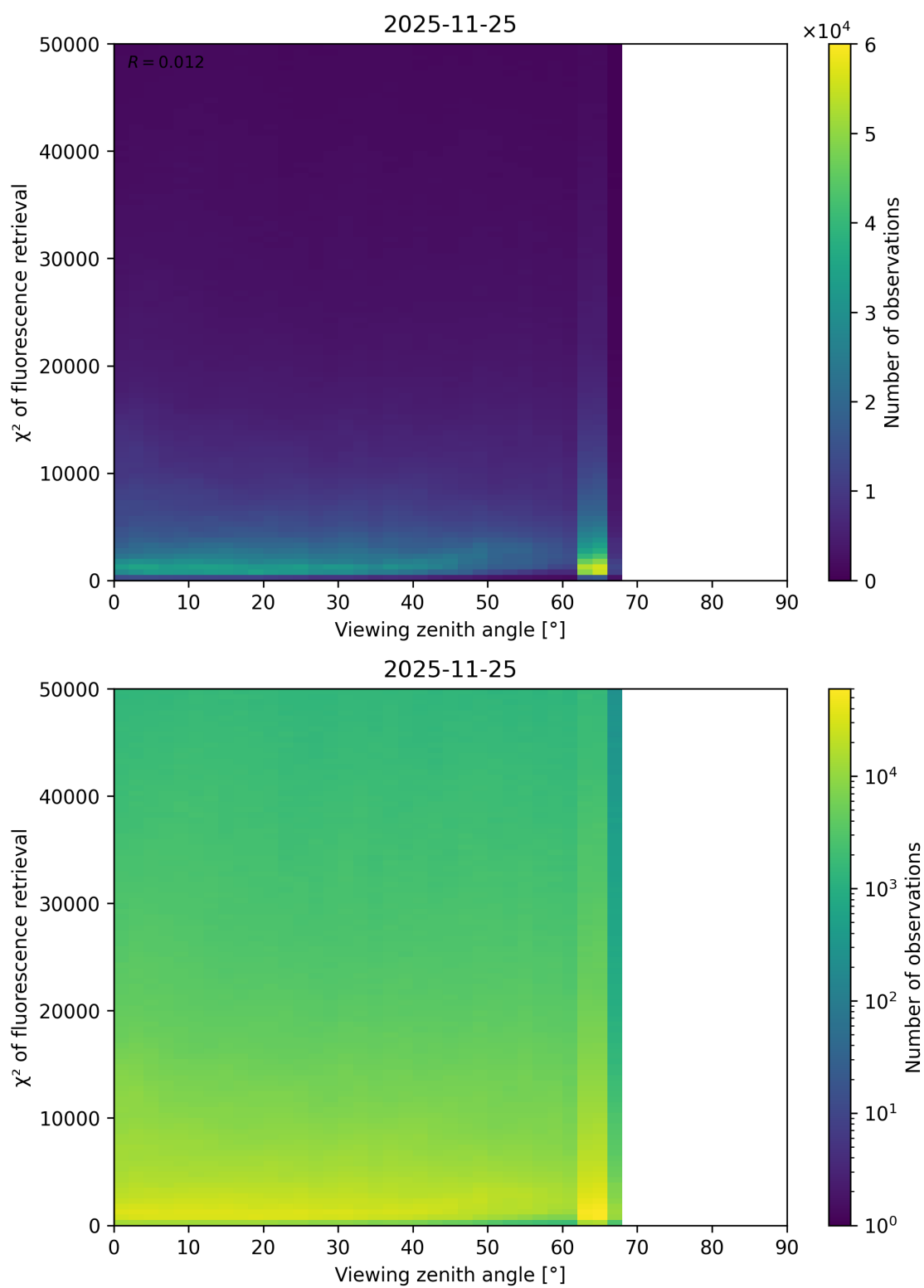
Figure 119: Scatter density plot of “Viewing zenith angle” against “ \chi^2 of fluorescence retrieval” for 2025-11-24 to 2025-11-26.
