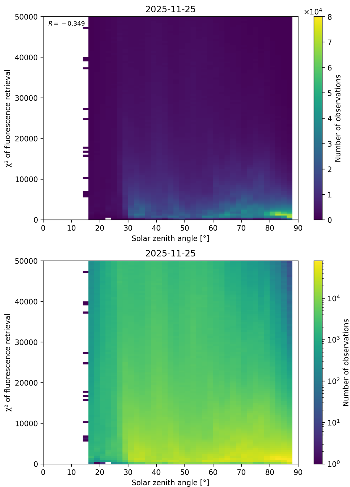
Figure 109: Scatter density plot of “Solar zenith angle” against “ \chi^2 of fluorescence retrieval” for 2025-11-24 to 2025-11-26.
