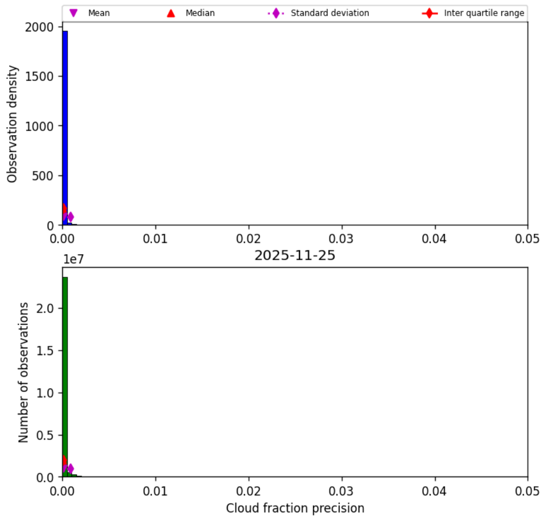
Figure 33: Histogram of “Cloud fraction precision” for 2025-11-24 to 2025-11-26
