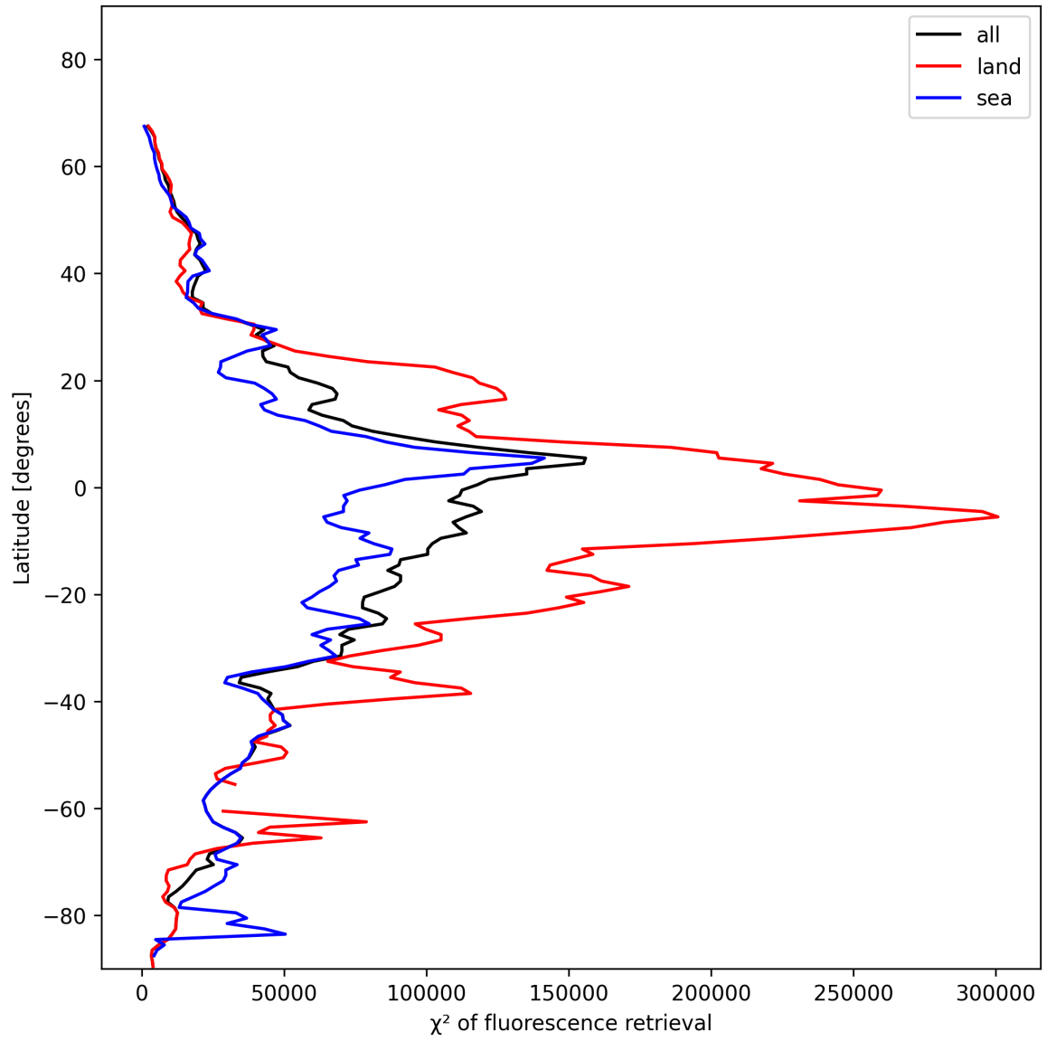
Figure 25: Zonal average of “ \chi^2 of fluorescence retrieval” for 2025-11-24 to 2025-11-26.
