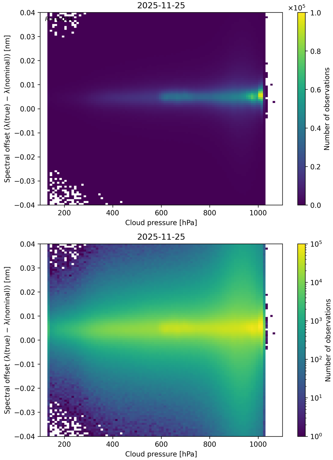
Figure 84: Scatter density plot of “Cloud pressure” against “Spectral offset ( \lambda_{\text{true}} - \lambda_{\text{nominal}} )” for 2025-11-24 to 2025-11-26.
