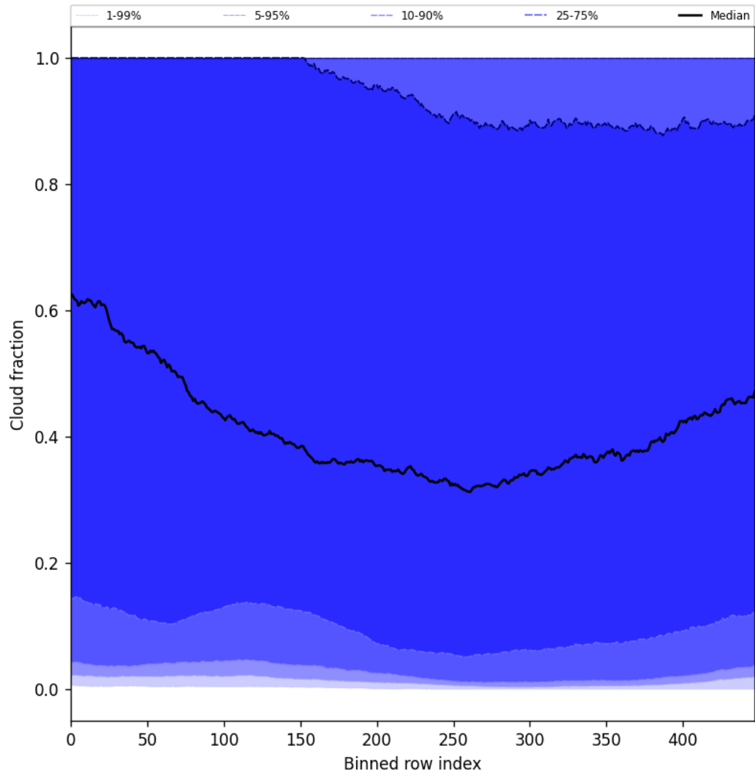
Figure 49: Along track statistics of “Cloud fraction” for 2025-11-24 to 2025-11-26
