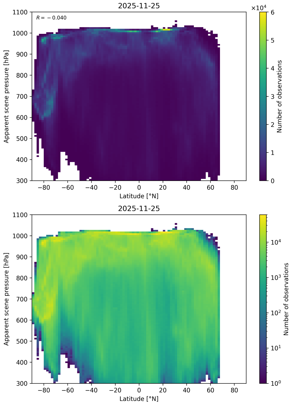
Figure 88: Scatter density plot of “Latitude” against “Apparent scene pressure” for 2025-11-24 to 2025-11-26.
