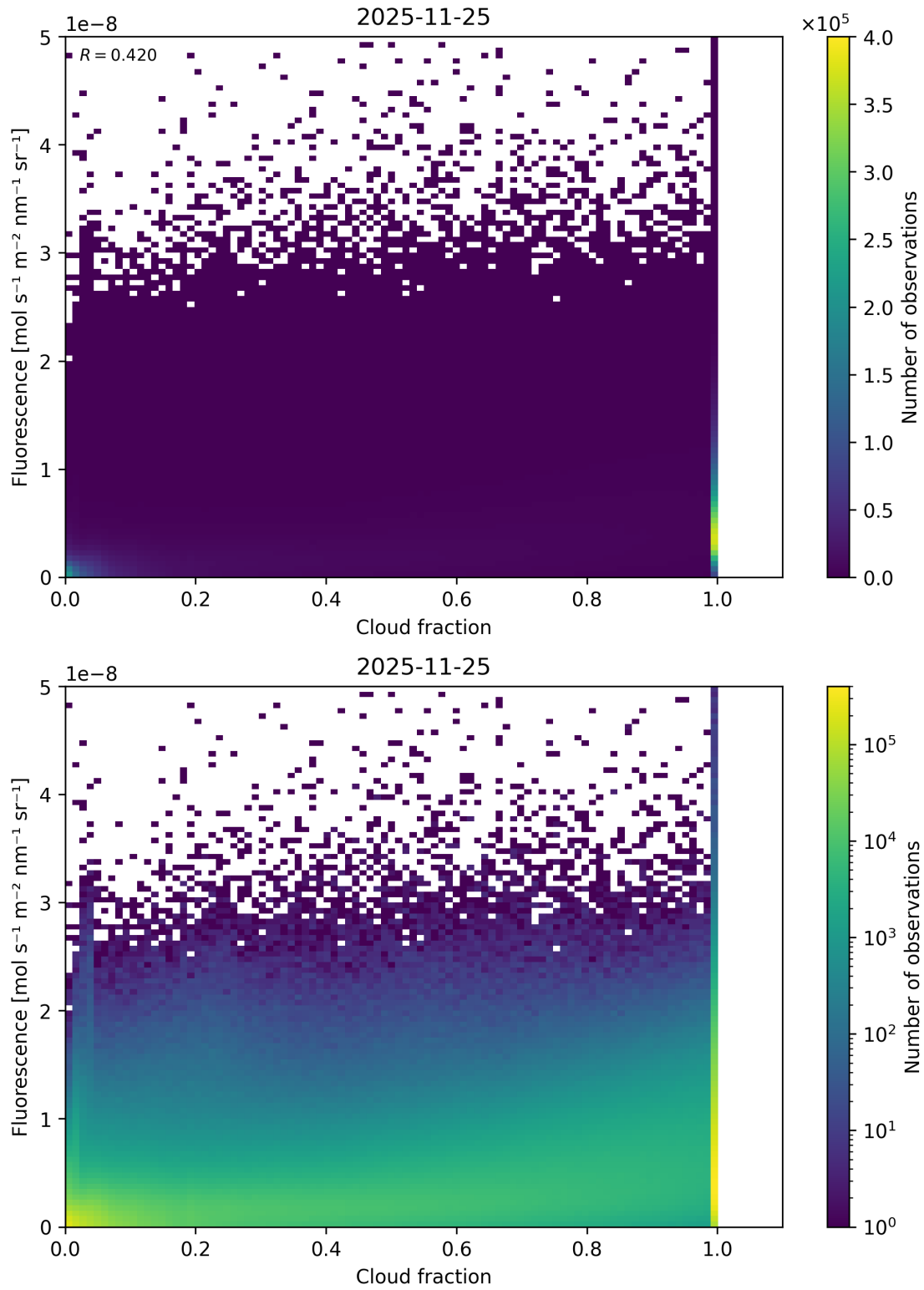
Figure 72: Scatter density plot of “Cloud fraction” against “Fluorescence” for 2025-11-24 to 2025-11-26.
