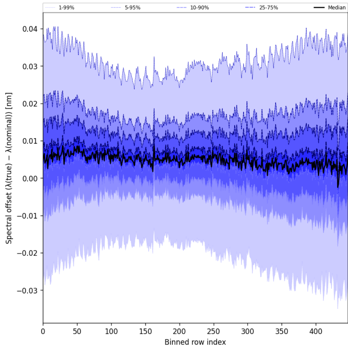
Figure 62: Along track statistics of “Spectral offset ( \lambda_{\text{true}} - \lambda_{\text{nominal}} )” for 2025-11-24 to 2025-11-26
