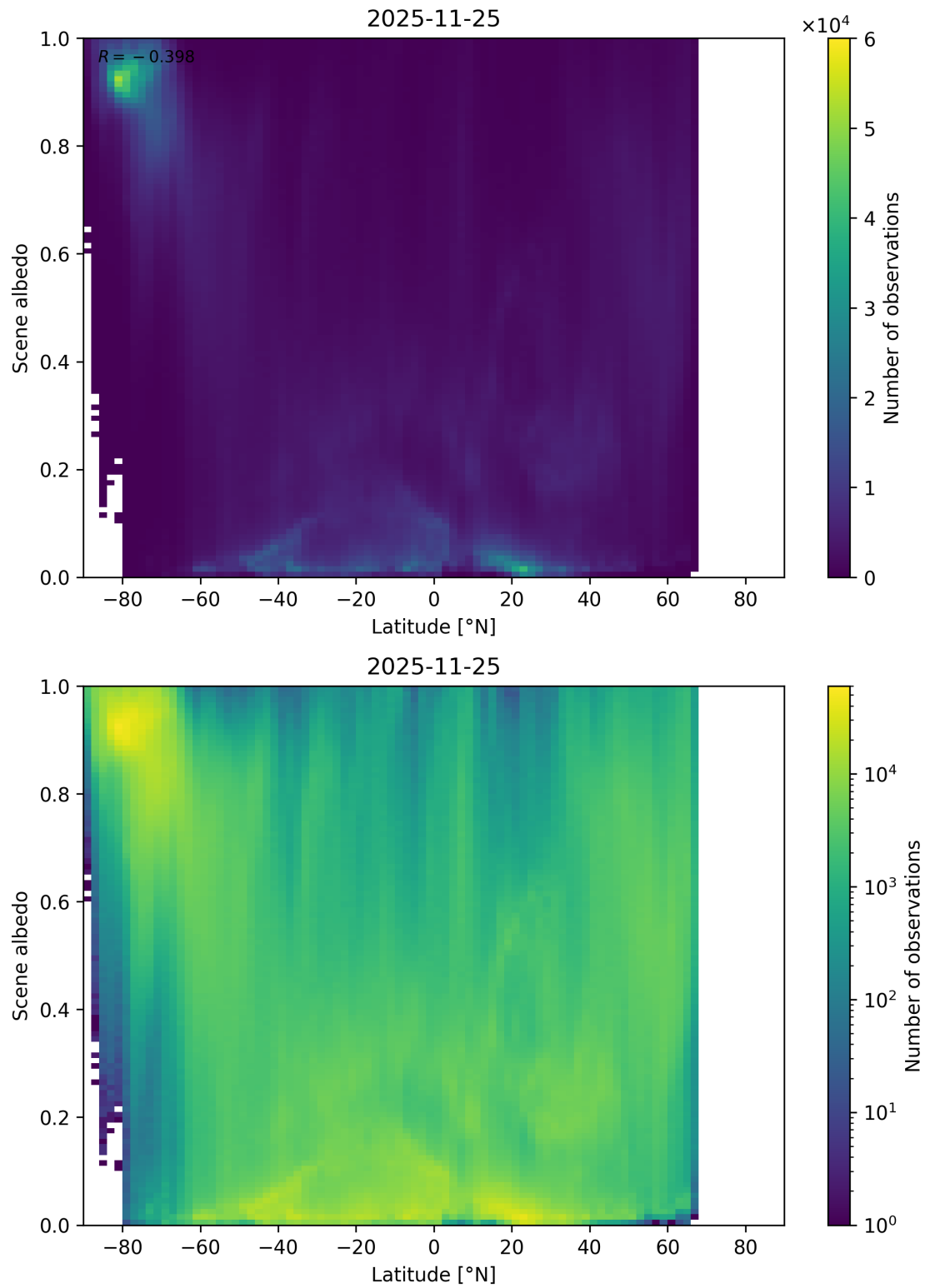
Figure 95: Scatter density plot of “Latitude” against “Scene albedo” for 2025-11-24 to 2025-11-26.
