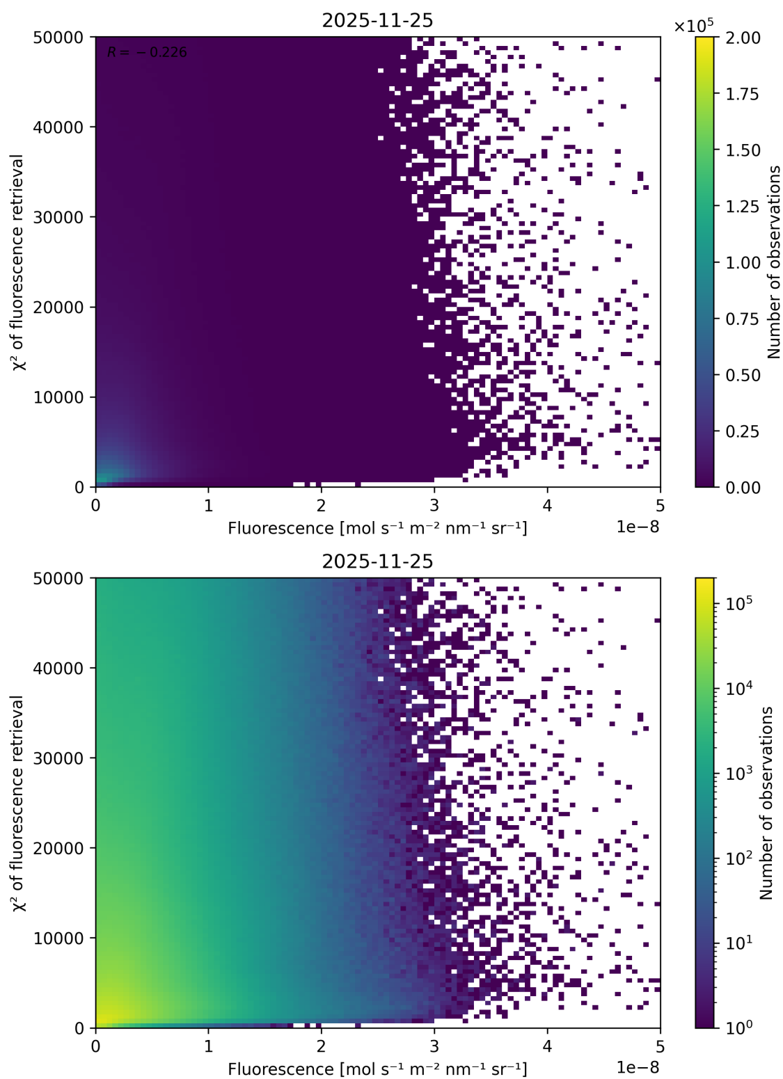
Figure 85: Scatter density plot of “Fluorescence” against “ \chi^2 of fluorescence retrieval” for 2025-11-24 to 2025-11-26.
