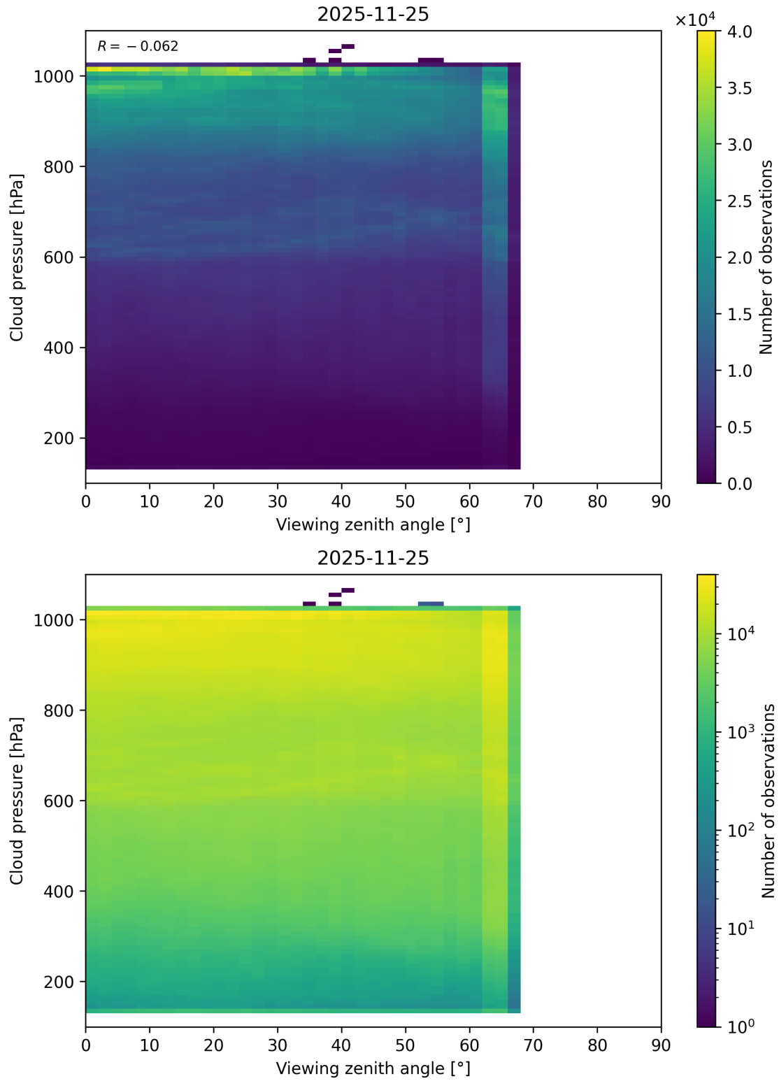
Figure 121: Scatter density plot of “Viewing zenith angle” against “Cloud pressure” for 2025-11-24 to 2025-11-26.
