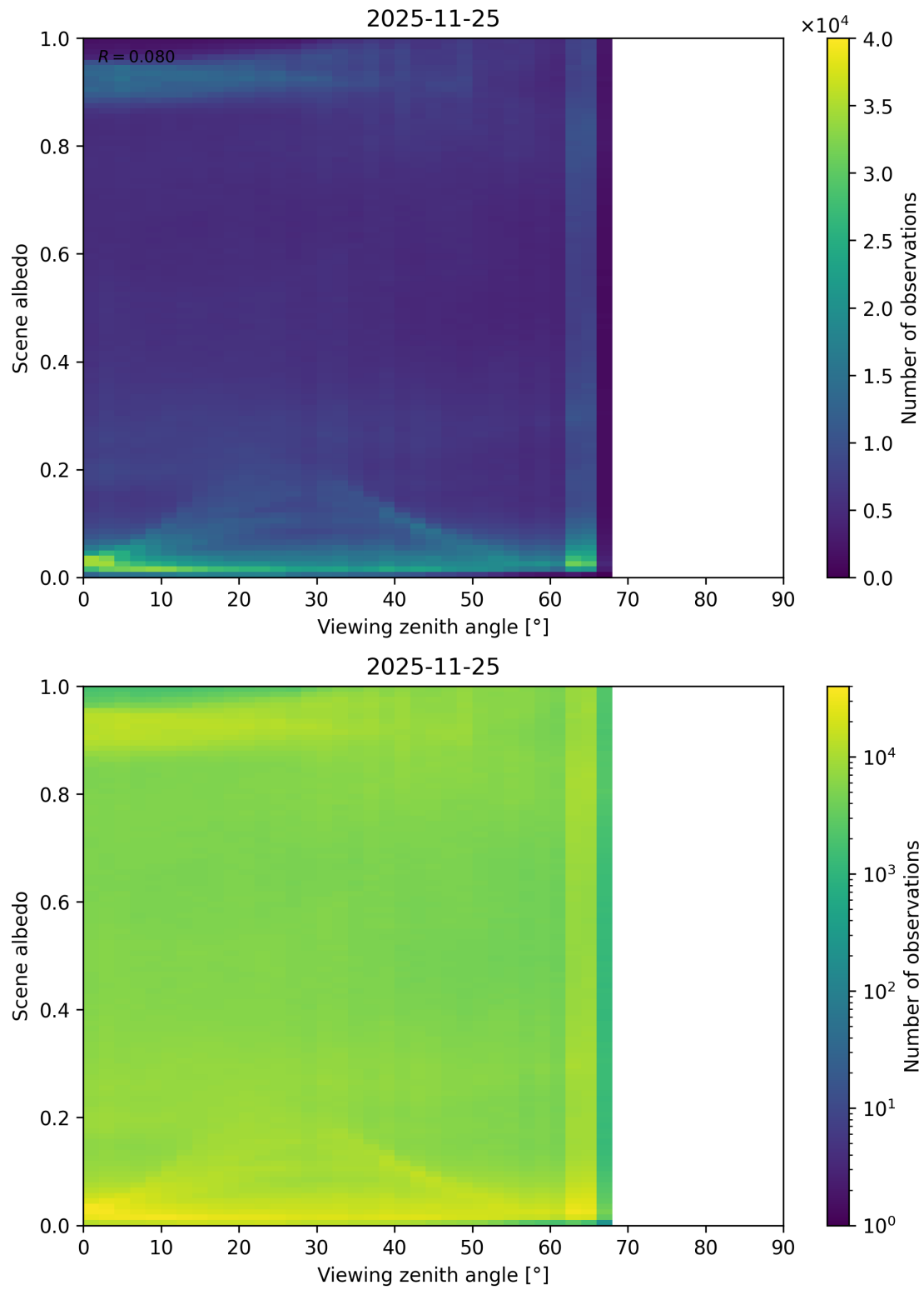
Figure 126: Scatter density plot of “Viewing zenith angle” against “Scene albedo” for 2025-11-24 to 2025-11-26.
