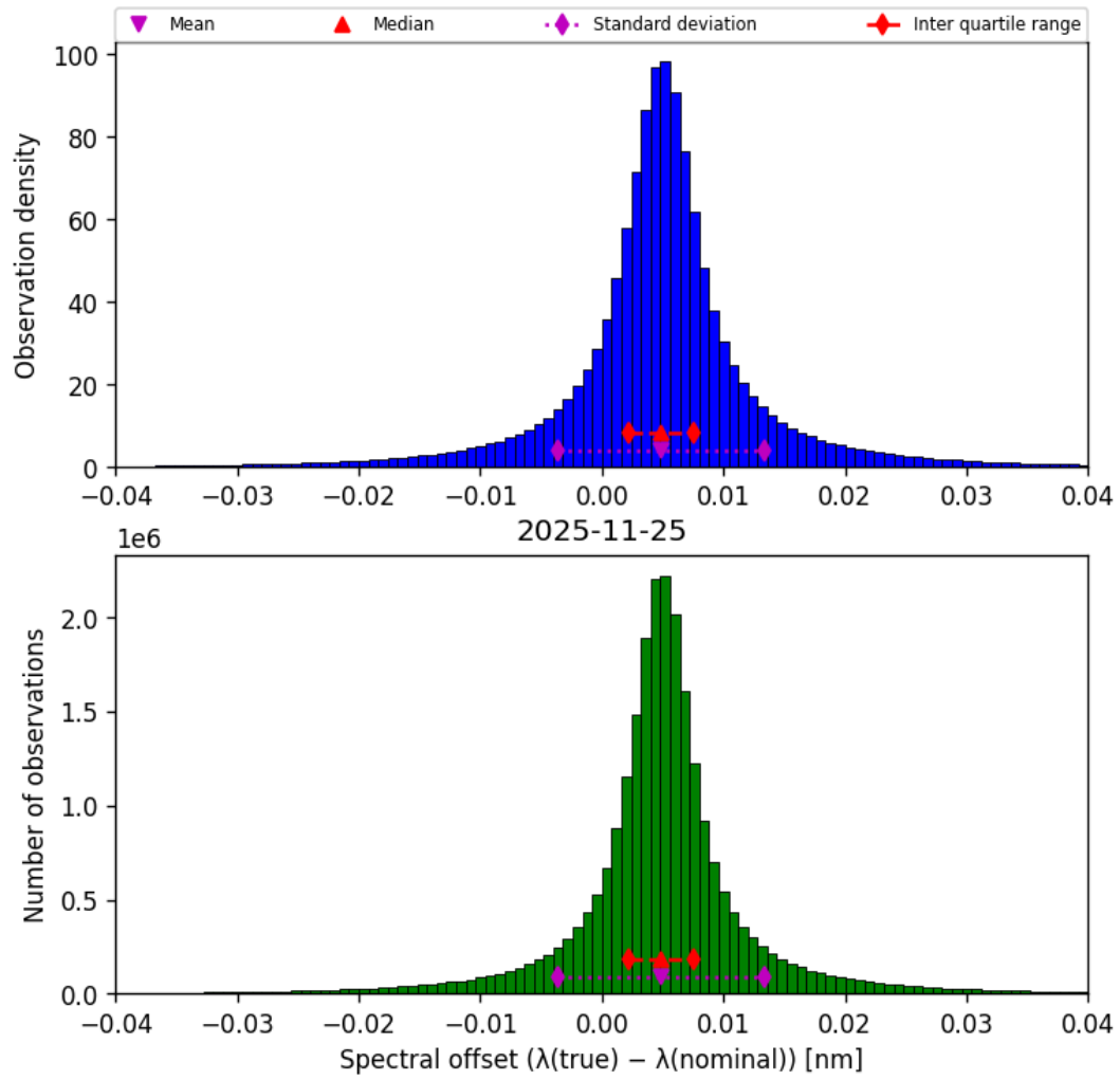
Figure 45: Histogram of “Spectral offset ( \lambda_{\text{true}} - \lambda_{\text{nominal}} )” for 2025-11-24 to 2025-11-26
