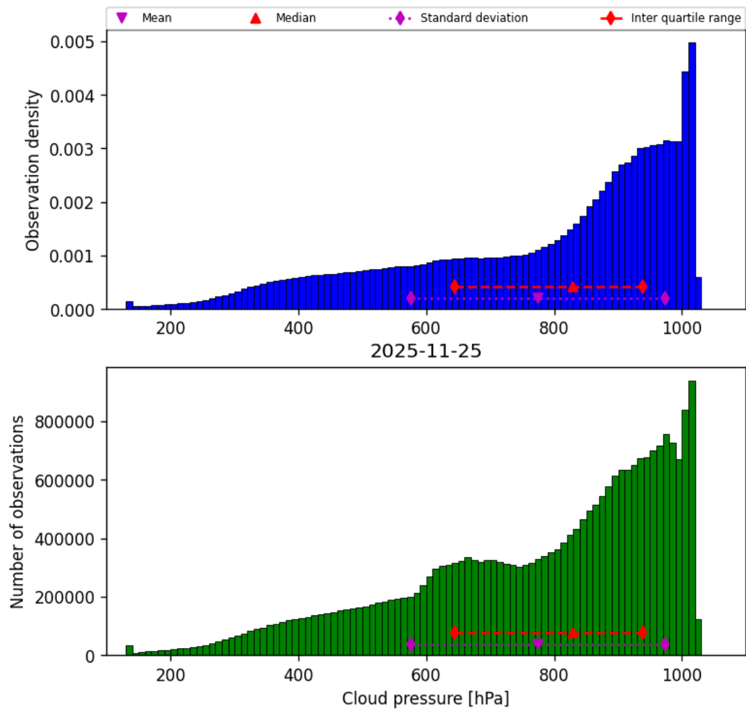
Figure 30: Histogram of “Cloud pressure” for 2025-11-24 to 2025-11-26
