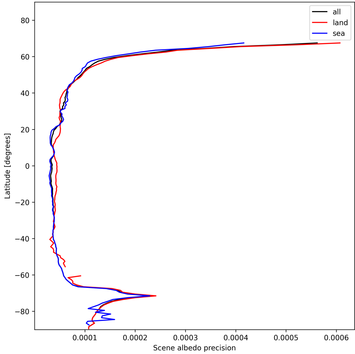
Figure 18: Zonal average of “Scene albedo precision” for 2025-11-24 to 2025-11-26.
