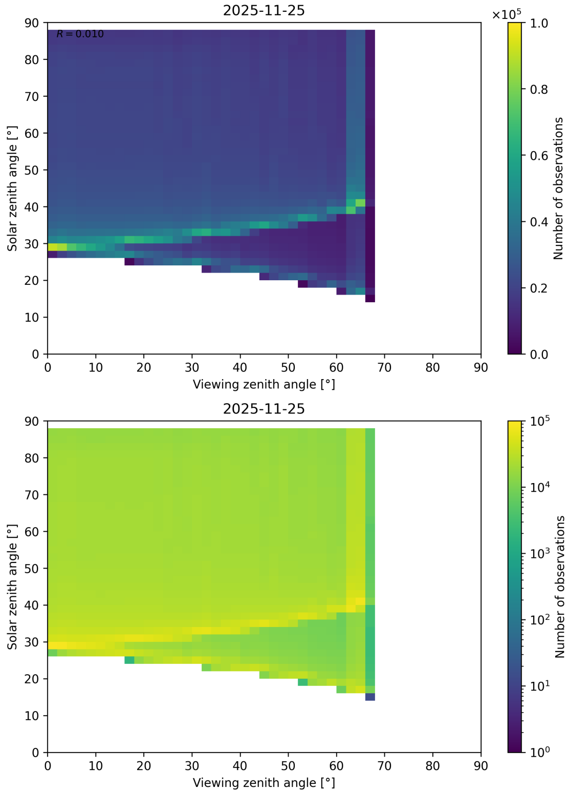
Figure 127: Scatter density plot of “Viewing zenith angle” against “Solar zenith angle” for 2025-11-24 to 2025-11-26.
