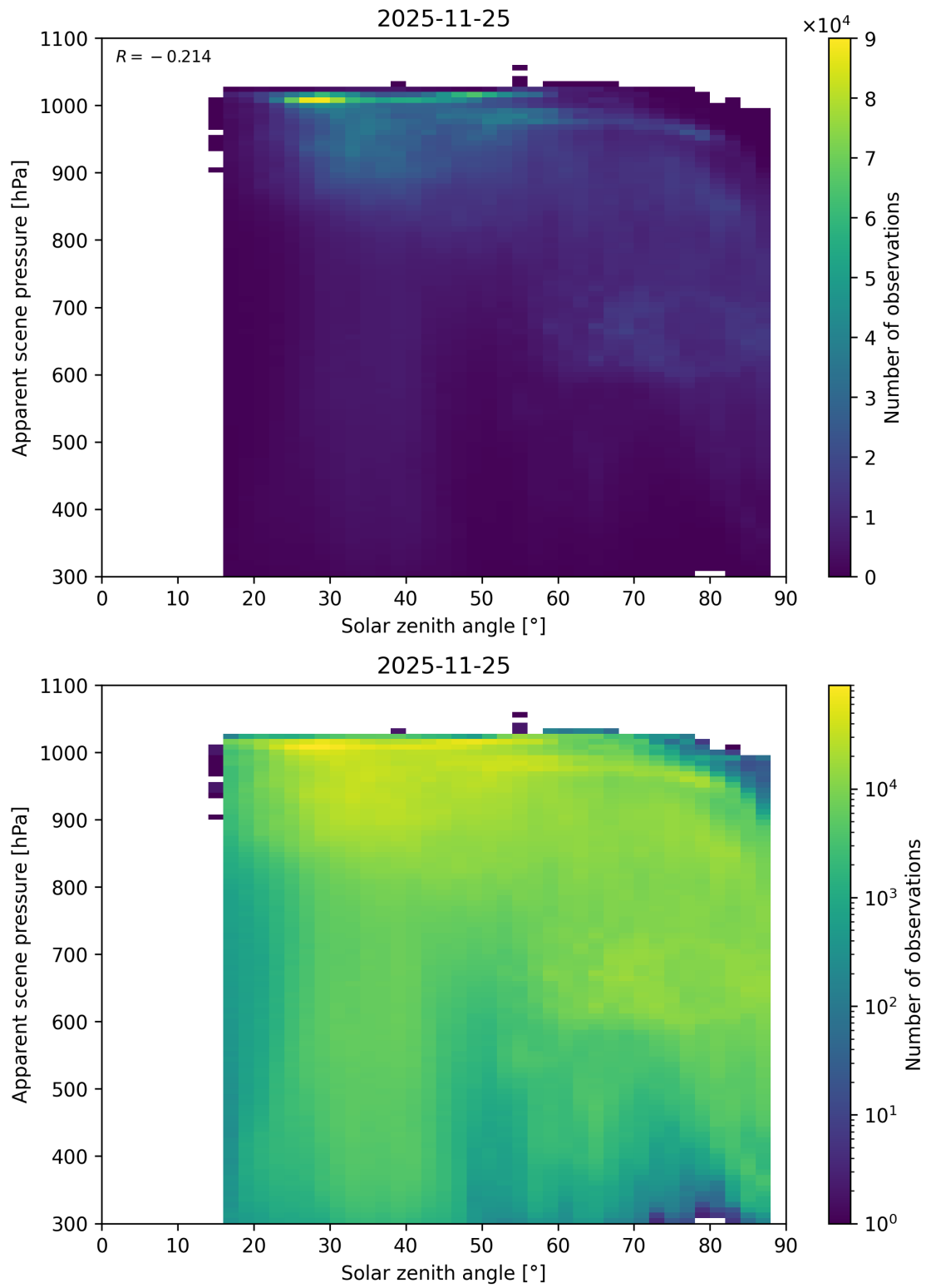
Figure 108: Scatter density plot of “Solar zenith angle” against “Apparent scene pressure” for 2025-11-24 to 2025-11-26.
