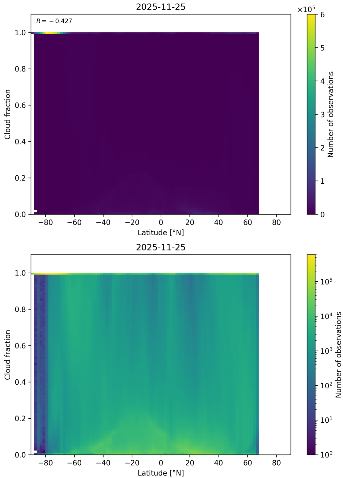
Figure 90: Scatter density plot of “Latitude” against “Cloud fraction” for 2025-11-24 to 2025-11-26.
