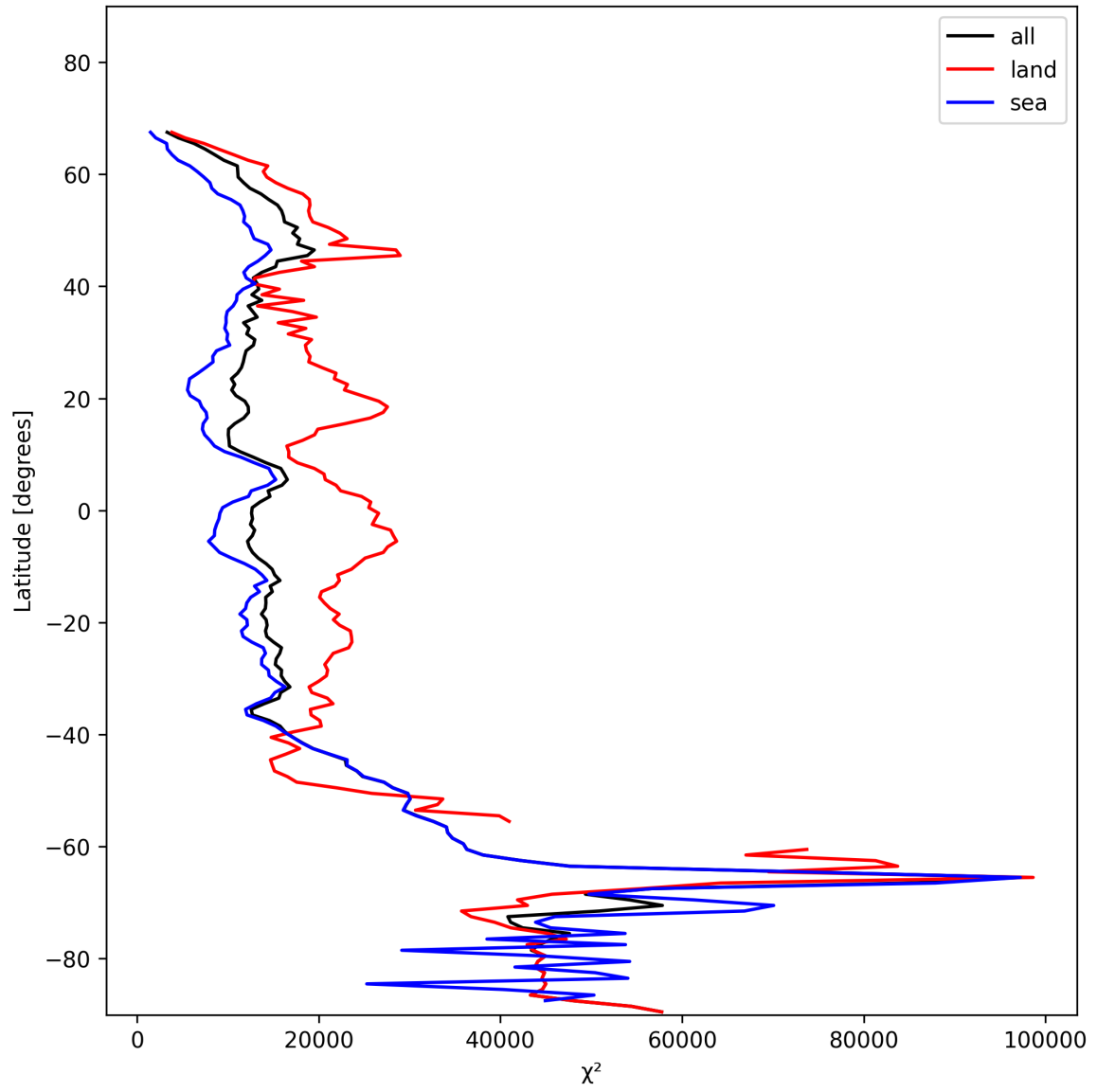
Figure 21: Zonal average of “ \chi^2 ” for 2025-11-24 to 2025-11-26.
