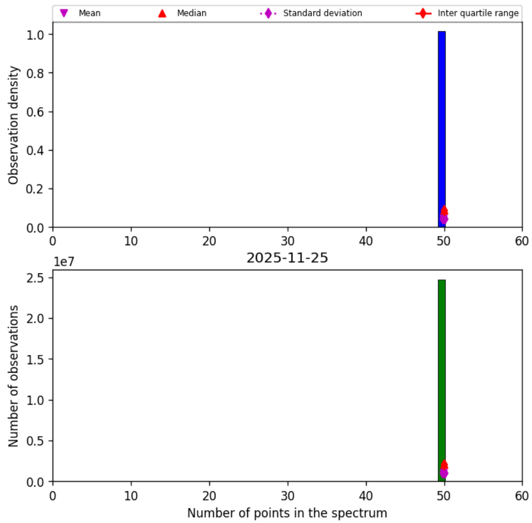
Figure 44: Histogram of “Number of points in the spectrum” for 2025-11-24 to 2025-11-26
