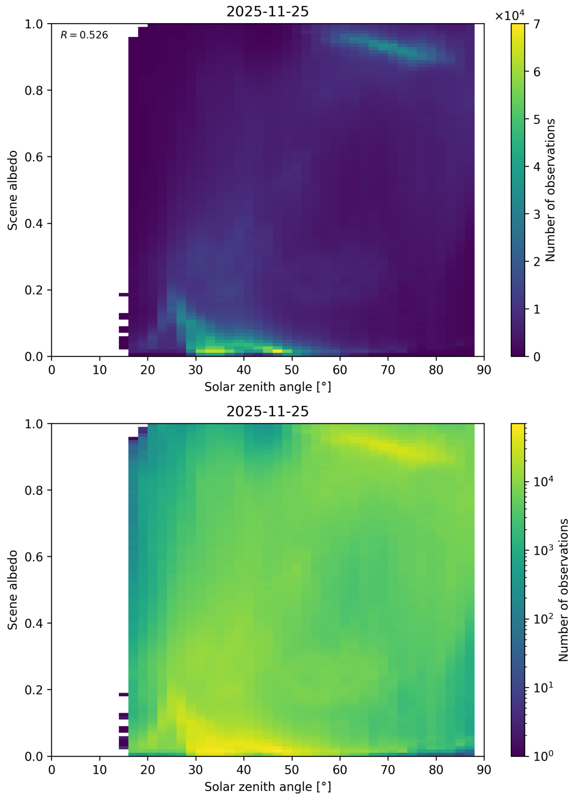
Figure 116: Scatter density plot of “Solar zenith angle” against “Scene albedo” for 2025-11-24 to 2025-11-26.
