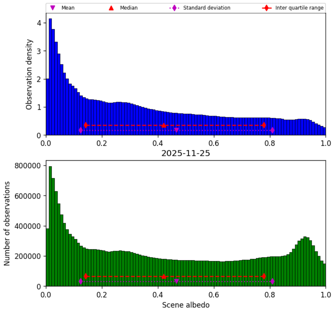
Figure 34: Histogram of “Scene albedo” for 2025-11-24 to 2025-11-26
