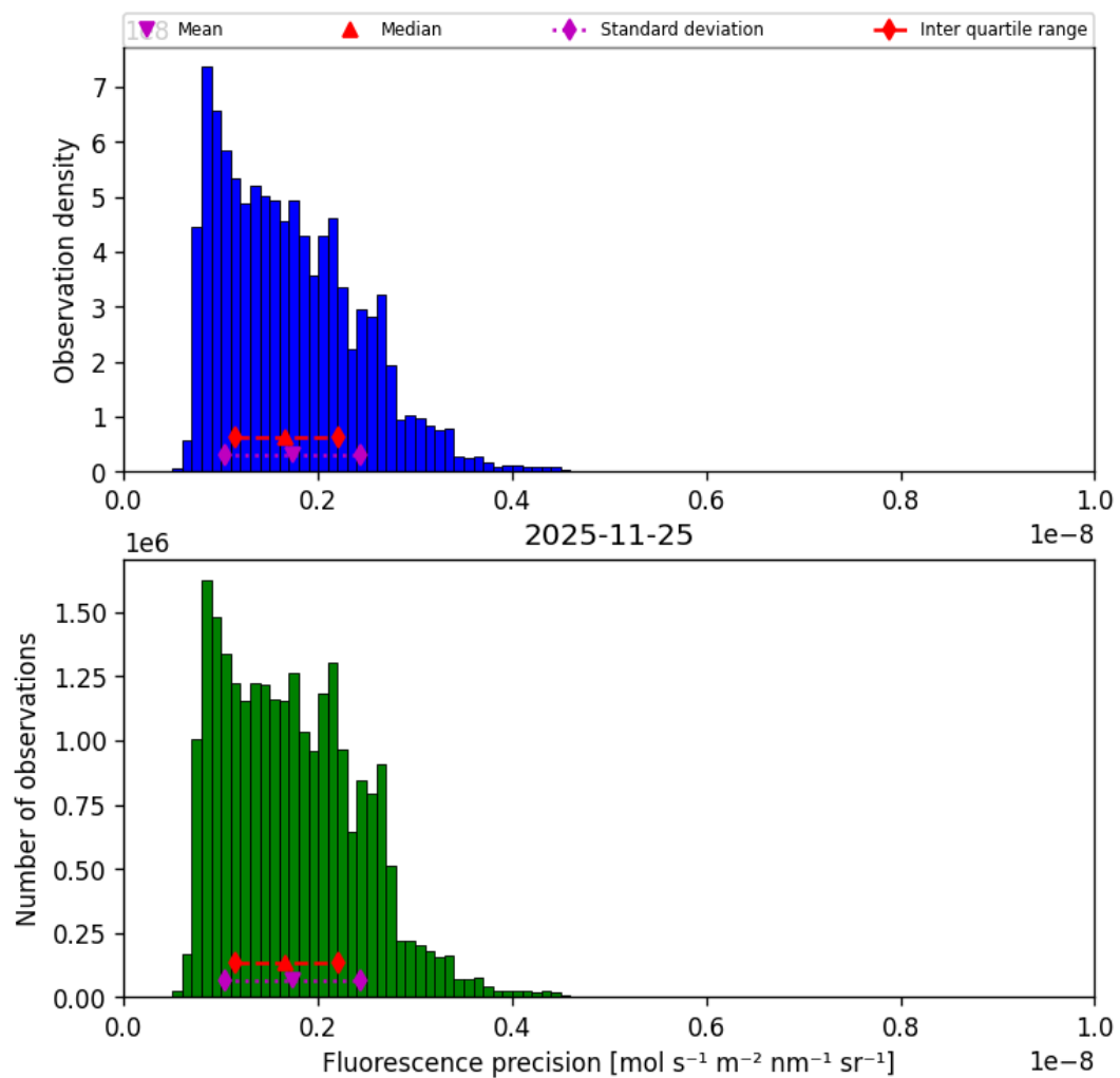
Figure 41: Histogram of “Fluorescence precision” for 2025-11-24 to 2025-11-26
