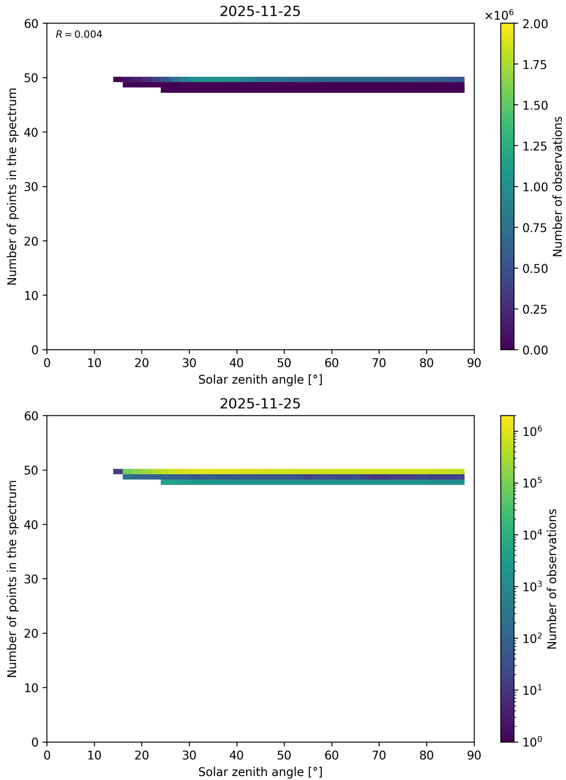
Figure 115: Scatter density plot of “Solar zenith angle” against “Number of points in the spectrum” for 2025-11-24 to 2025-11-26.
