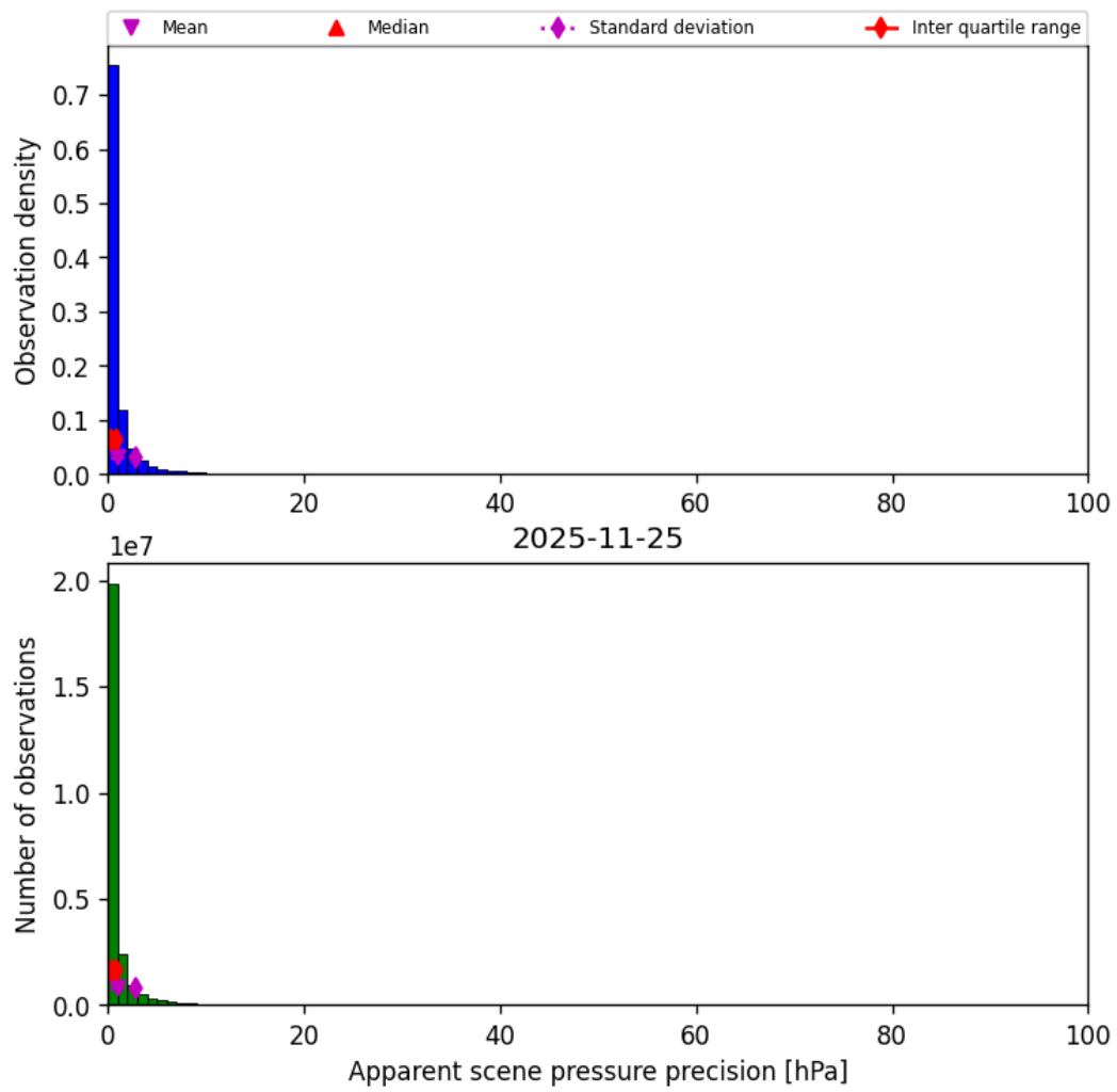
Figure 37: Histogram of “Apparent scene pressure precision” for 2025-11-24 to 2025-11-26
