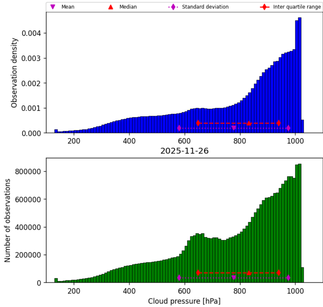
Figure 30: Histogram of “Cloud pressure” for 2025-11-25 to 2025-11-27
