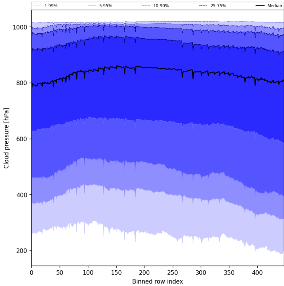
Figure 47: Along track statistics of “Cloud pressure” for 2025-11-25 to 2025-11-27
