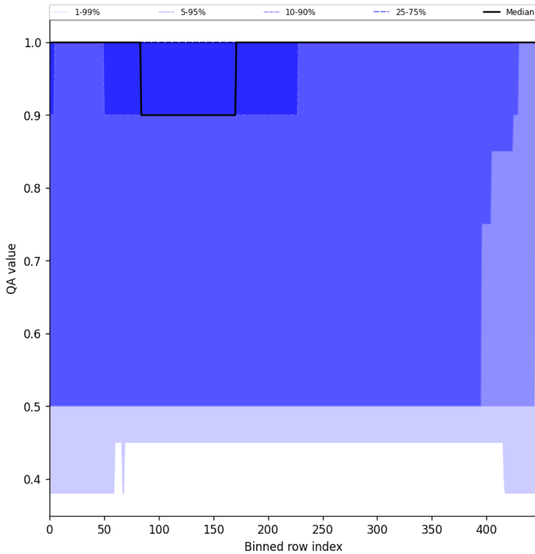
Figure 46: Along track statistics of “QA value” for 2025-11-25 to 2025-11-27
