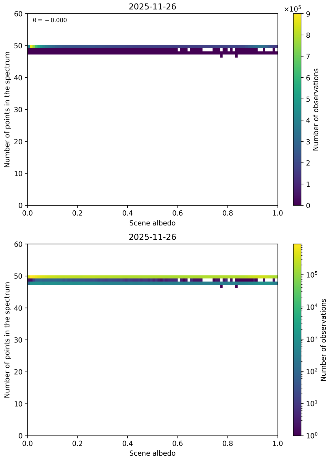
Figure 106: Scatter density plot of “Scene albedo” against “Number of points in the spectrum” for 2025-11-25 to 2025-11-27.
