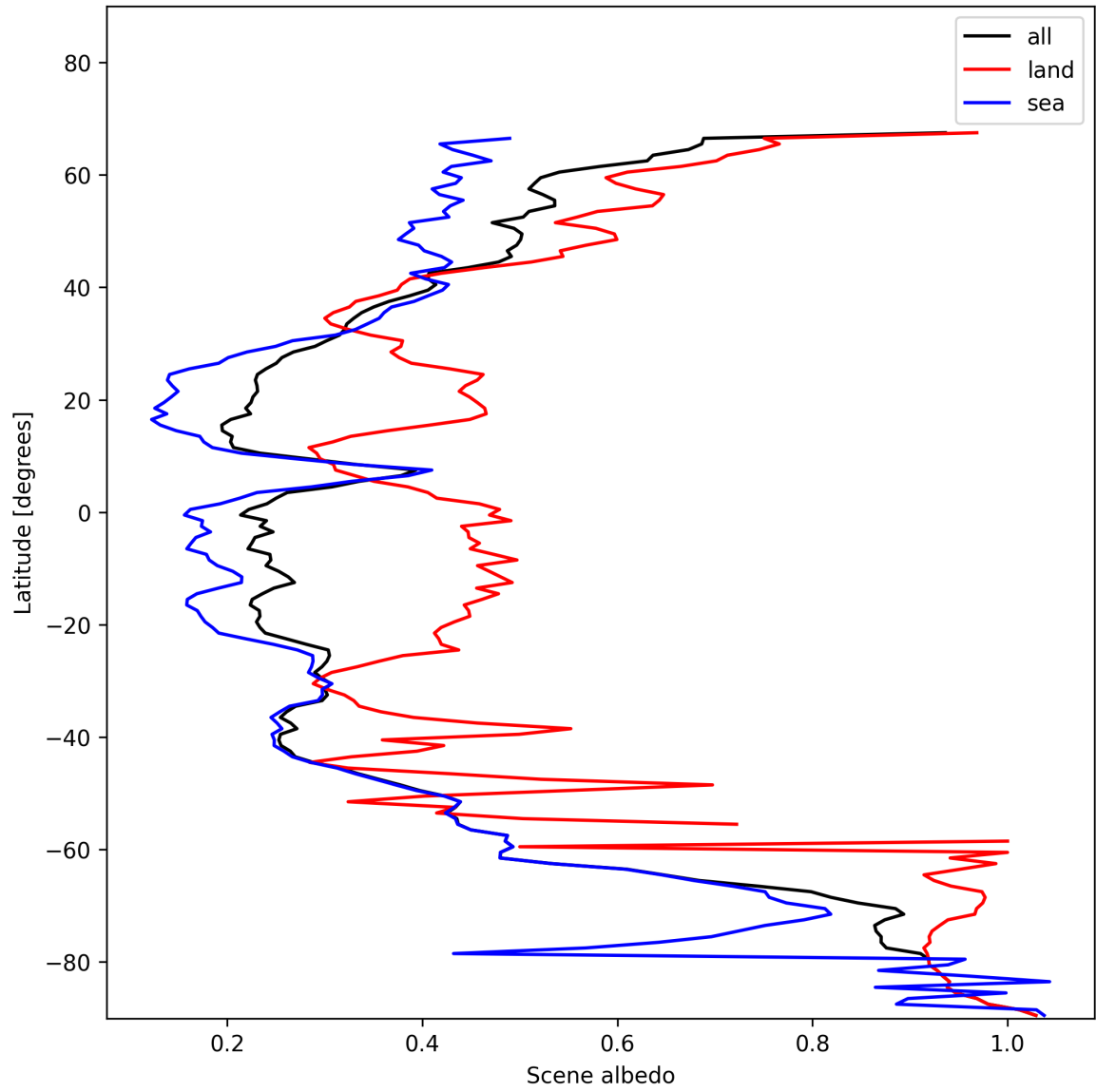
Figure 17: Zonal average of “Scene albedo” for 2025-11-25 to 2025-11-27.
