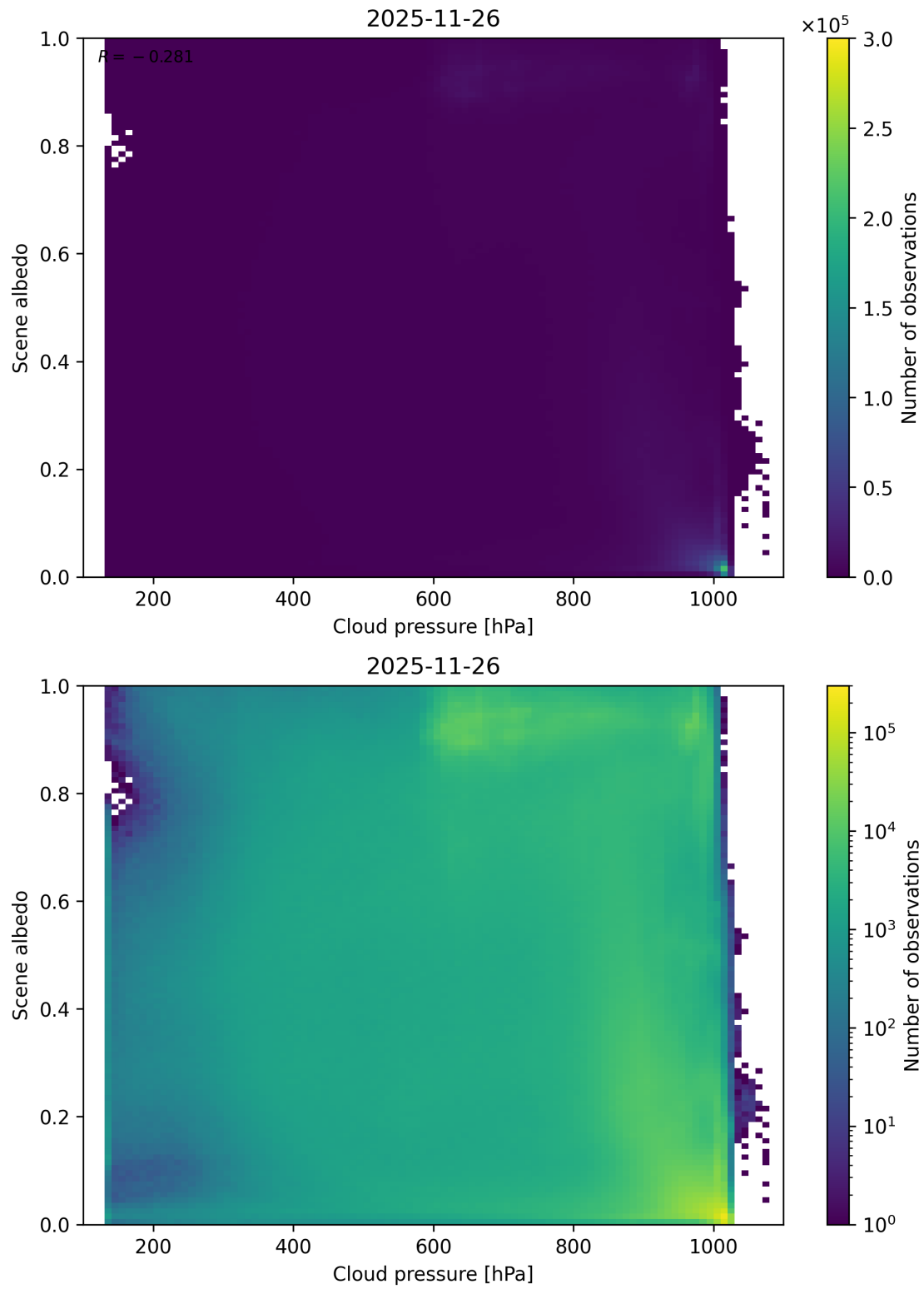
Figure 83: Scatter density plot of “Cloud pressure” against “Scene albedo” for 2025-11-25 to 2025-11-27.
