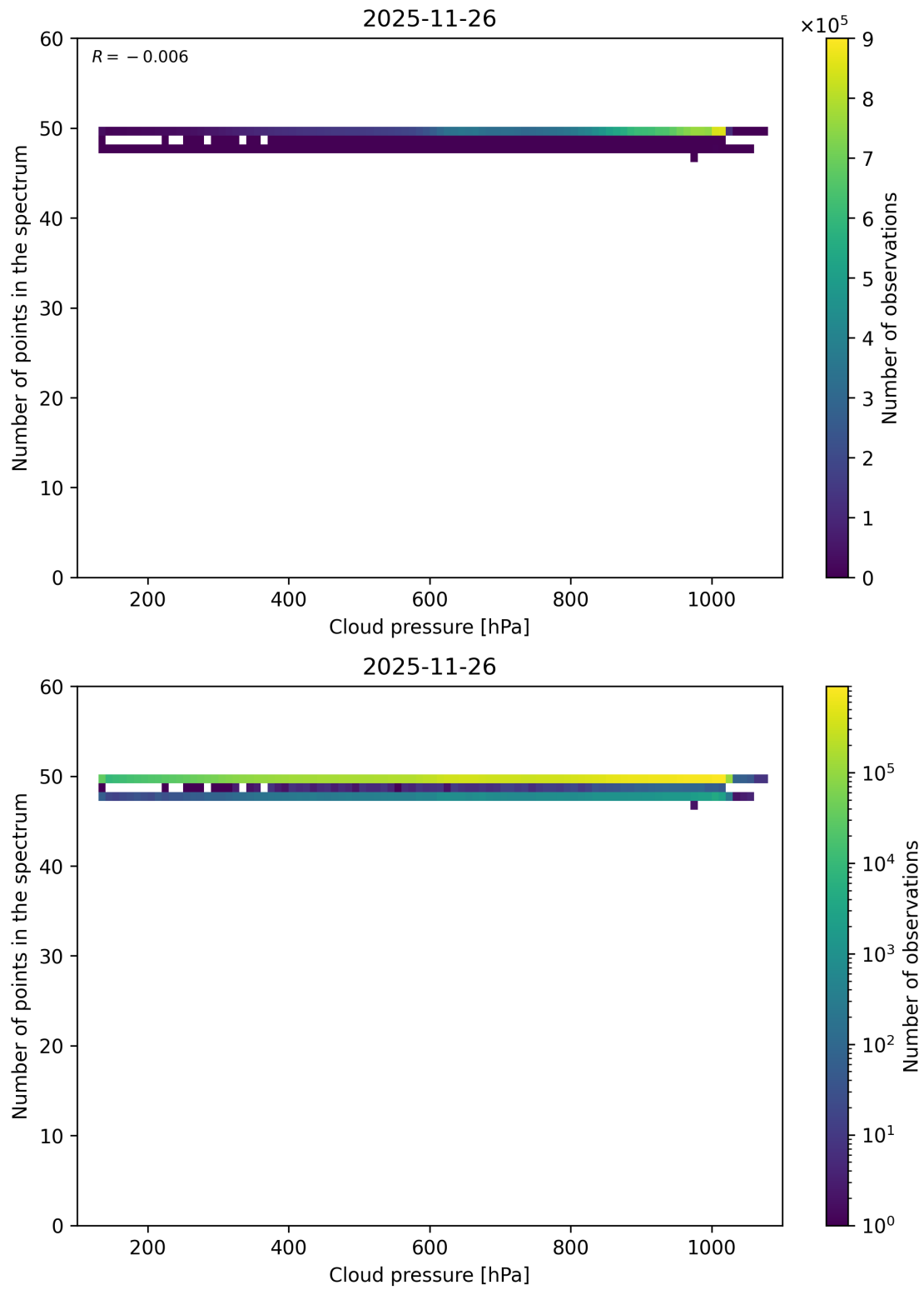
Figure 82: Scatter density plot of “Cloud pressure” against “Number of points in the spectrum” for 2025-11-25 to 2025-11-27.
