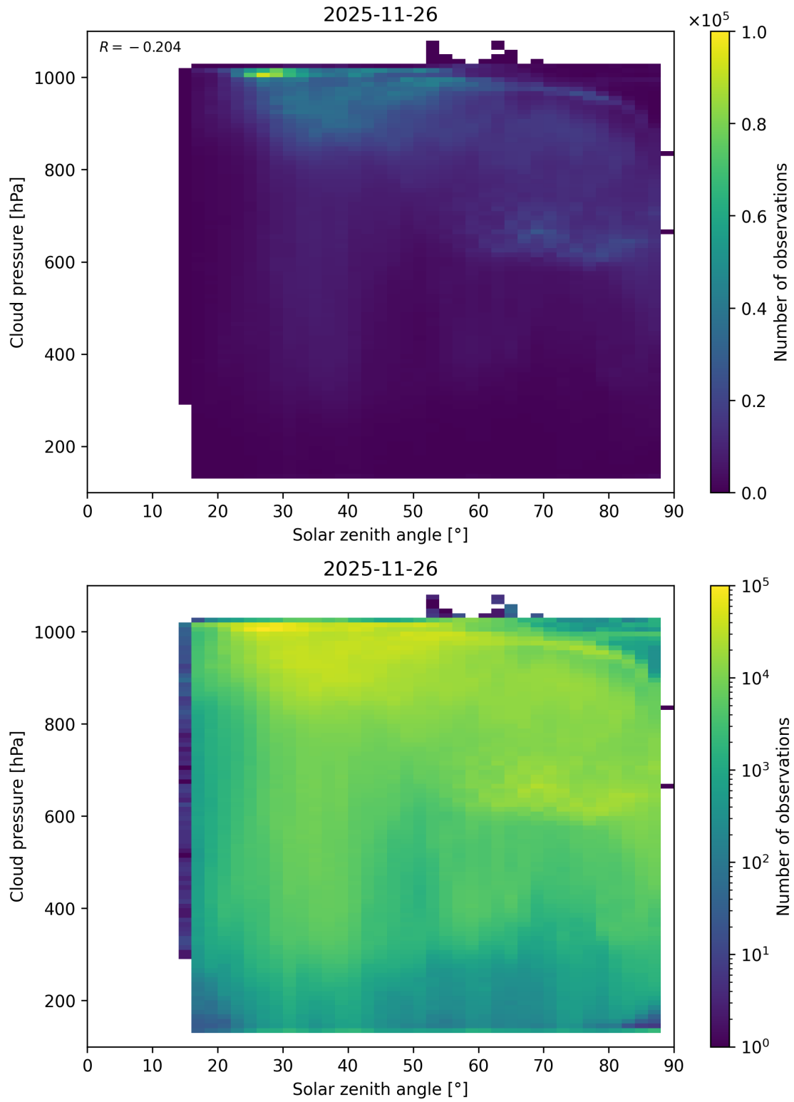
Figure 111: Scatter density plot of “Solar zenith angle” against “Cloud pressure” for 2025-11-25 to 2025-11-27.
