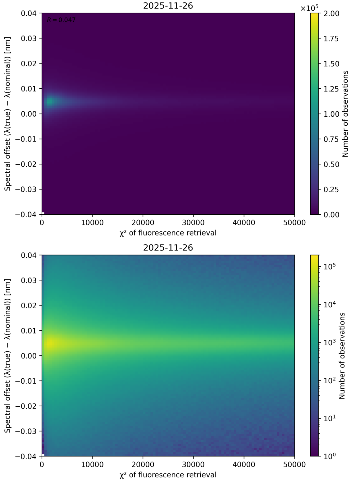
Figure 69: Scatter density plot of “ \chi^2 of fluorescence retrieval” against “Spectral offset ( \lambda_{\text{true}} - \lambda_{\text{nominal}} )” for 2025-11-25 to 2025-11-27.
