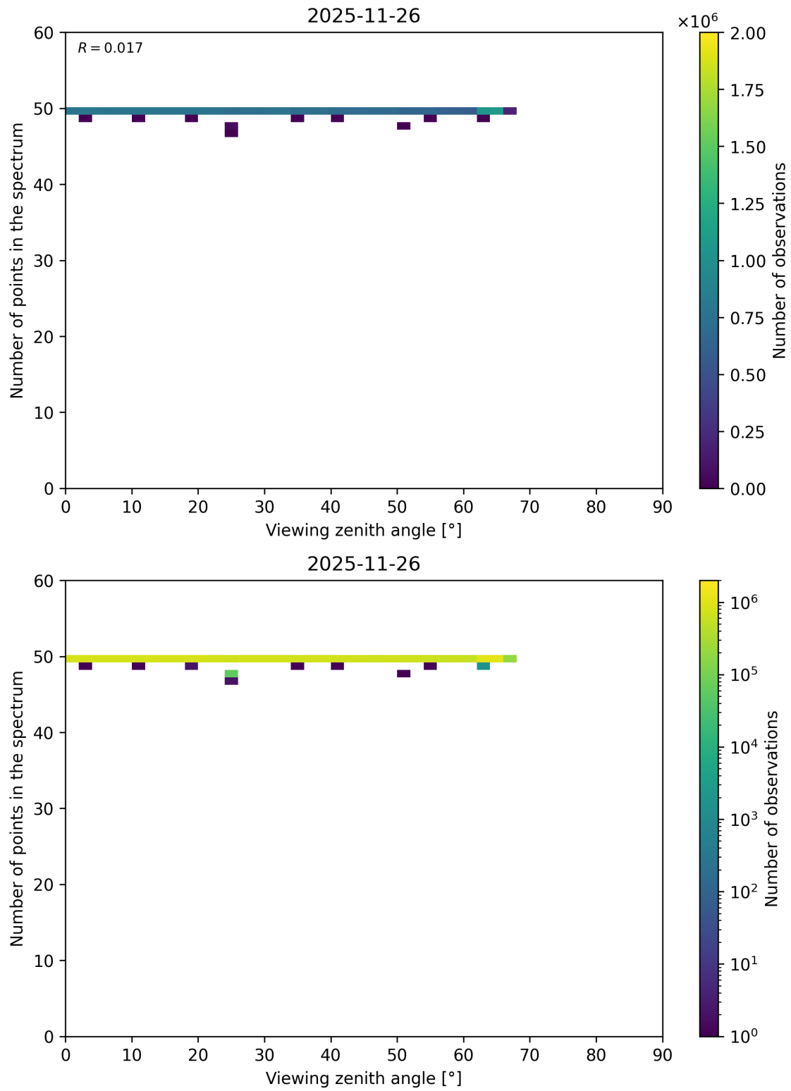
Figure 125: Scatter density plot of “Viewing zenith angle” against “Number of points in the spectrum” for 2025-11-25 to 2025-11-27.
