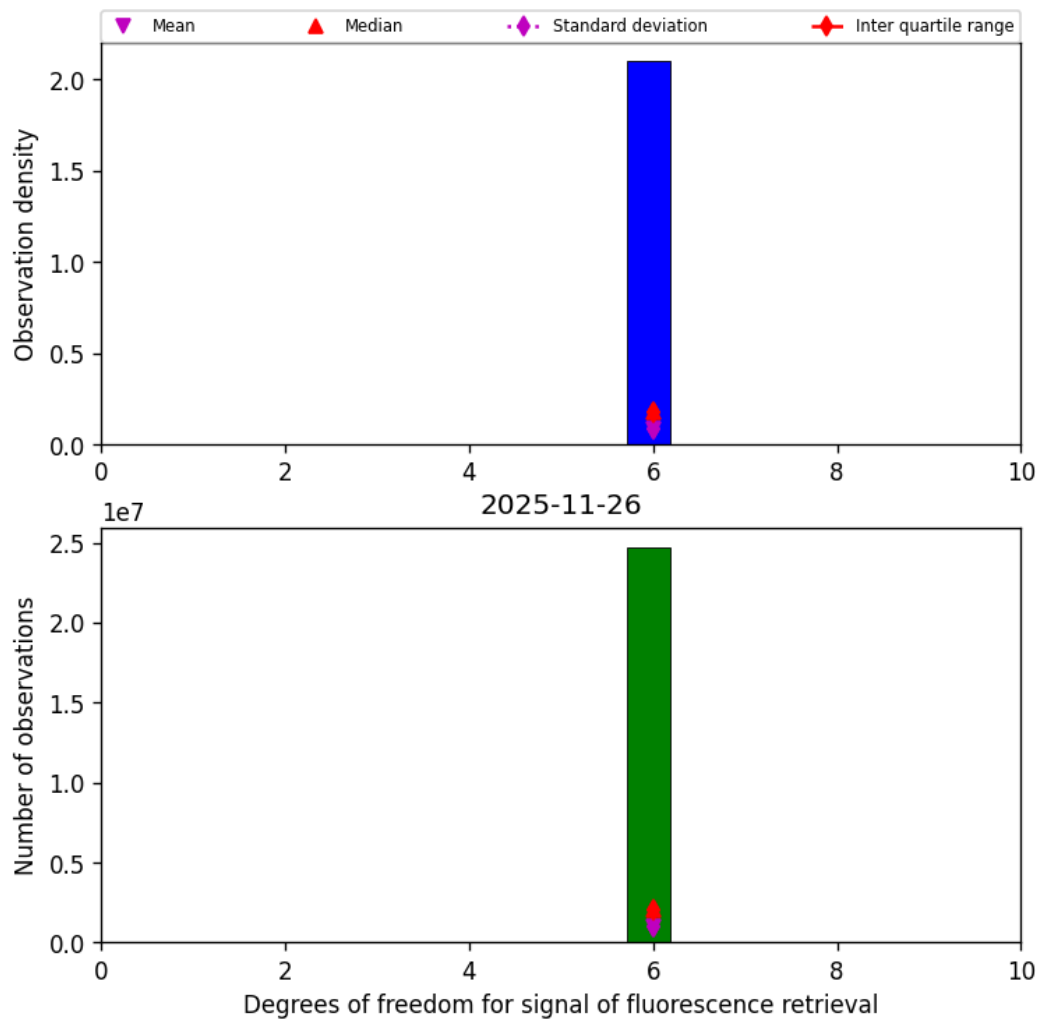
Figure 43: Histogram of “Degrees of freedom for signal of fluorescence retrieval” for 2025-11-25 to 2025-11-27
