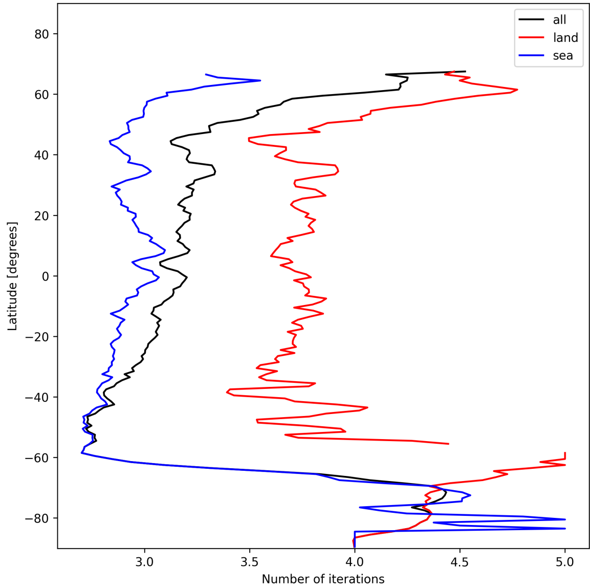
Figure 22: Zonal average of “Number of iterations” for 2025-11-25 to 2025-11-27.
