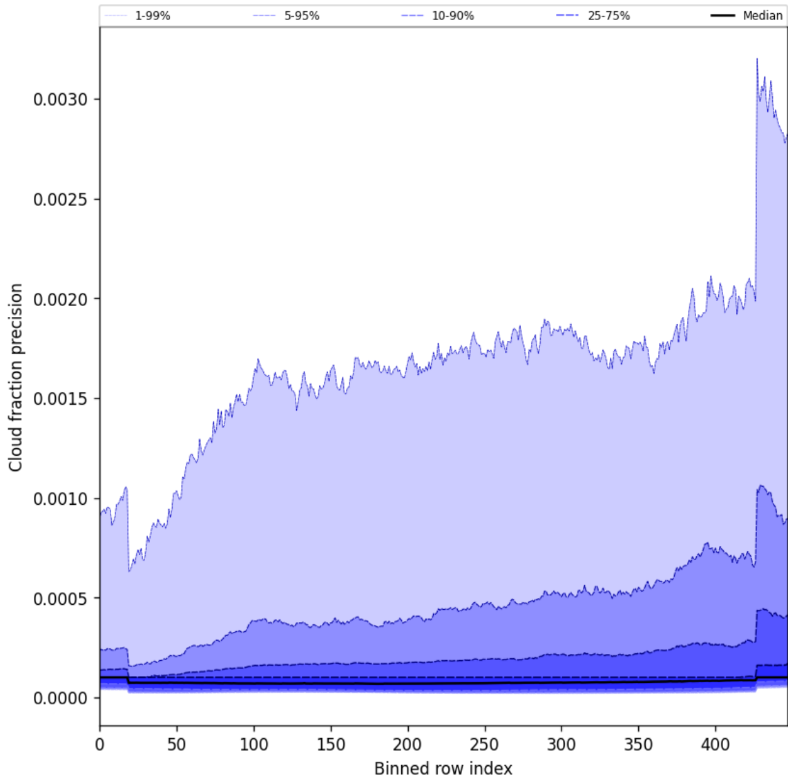
Figure 50: Along track statistics of “Cloud fraction precision” for 2025-11-25 to 2025-11-27
