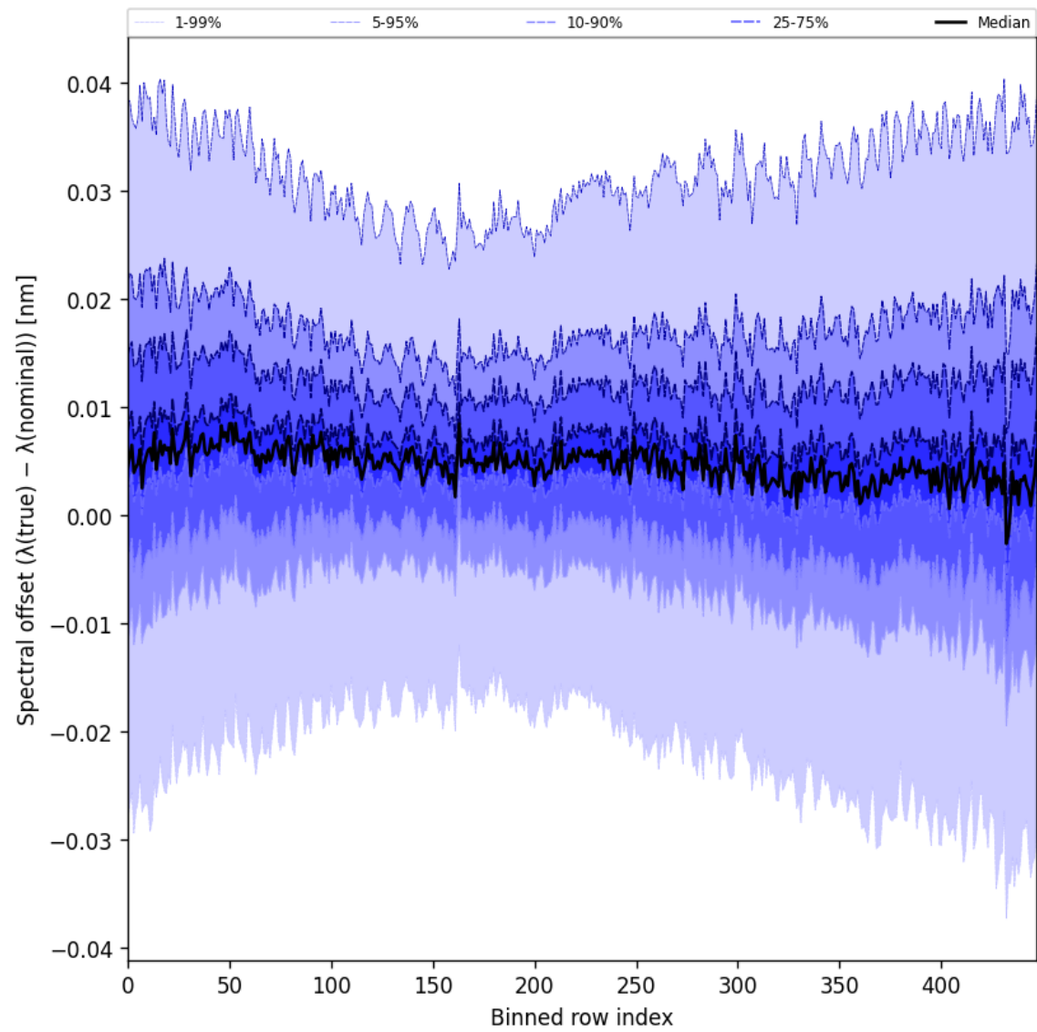
Figure 62: Along track statistics of “Spectral offset ( \lambda_{\text{true}} - \lambda_{\text{nominal}} )” for 2025-11-25 to 2025-11-27
