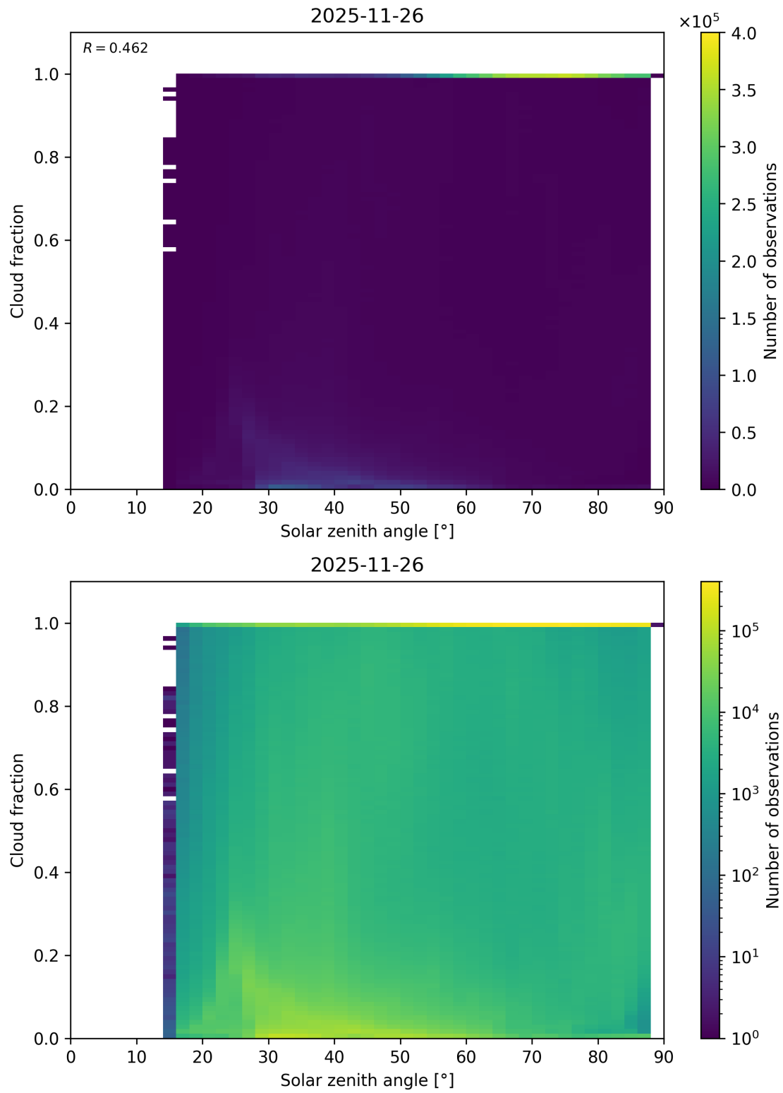
Figure 110: Scatter density plot of “Solar zenith angle” against “Cloud fraction” for 2025-11-25 to 2025-11-27.
