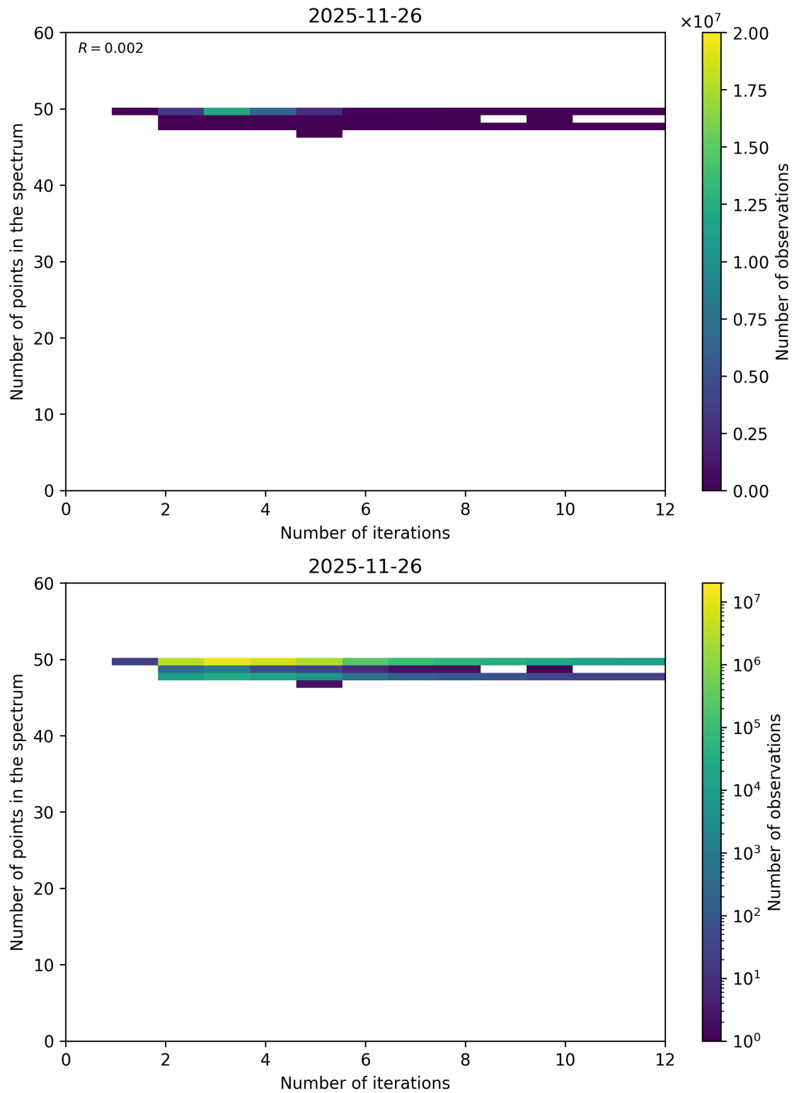
Figure 99: Scatter density plot of “Number of iterations” against “Number of points in the spectrum” for 2025-11-25 to 2025-11-27.
