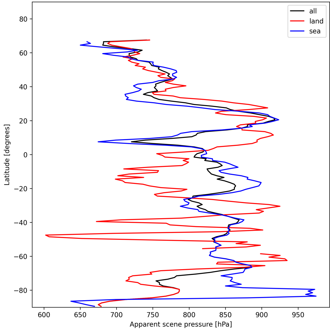
Figure 19: Zonal average of “Apparent scene pressure” for 2025-11-25 to 2025-11-27.
