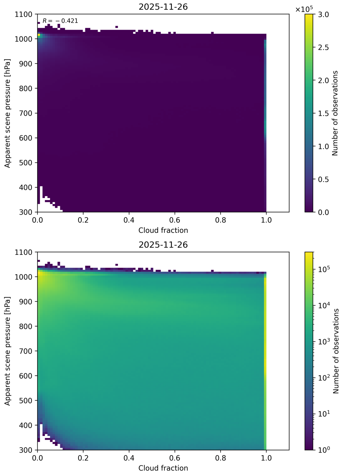
Figure 70: Scatter density plot of “Cloud fraction” against “Apparent scene pressure” for 2025-11-25 to 2025-11-27.
