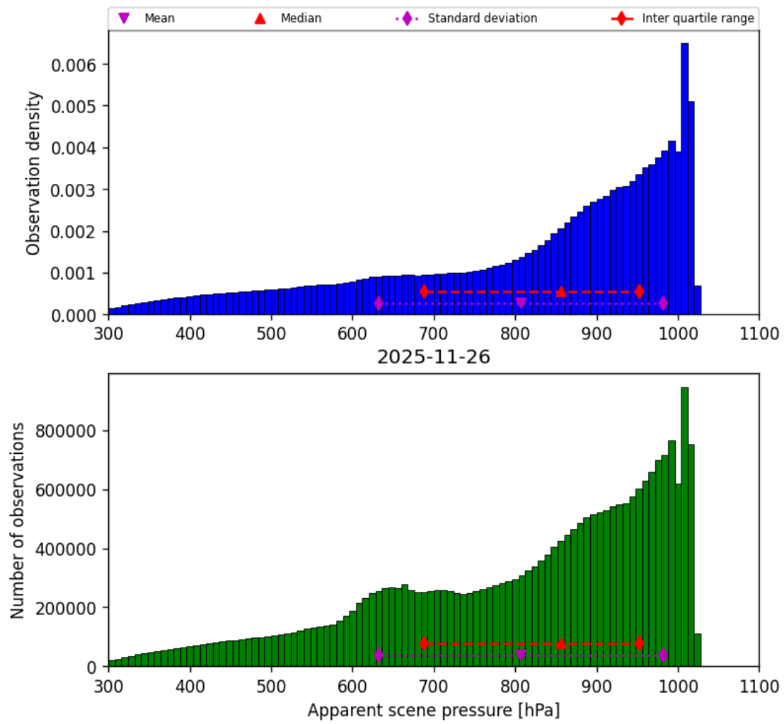
Figure 36: Histogram of “Apparent scene pressure” for 2025-11-25 to 2025-11-27
