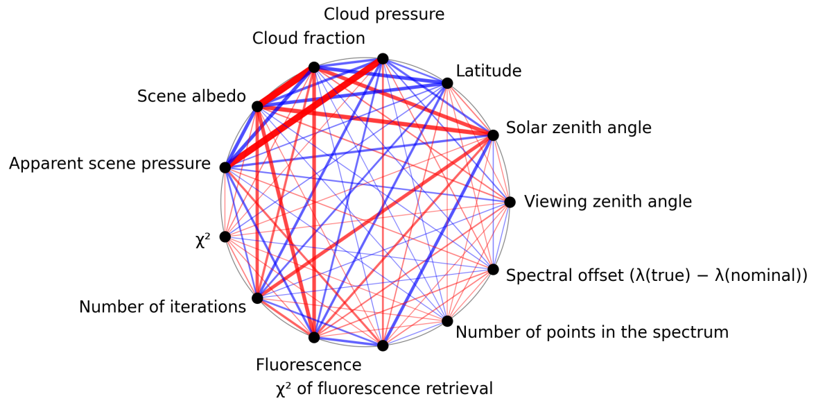
Figure 1: Map of correlation graph for 2025-11-25 to 2025-11-27.
