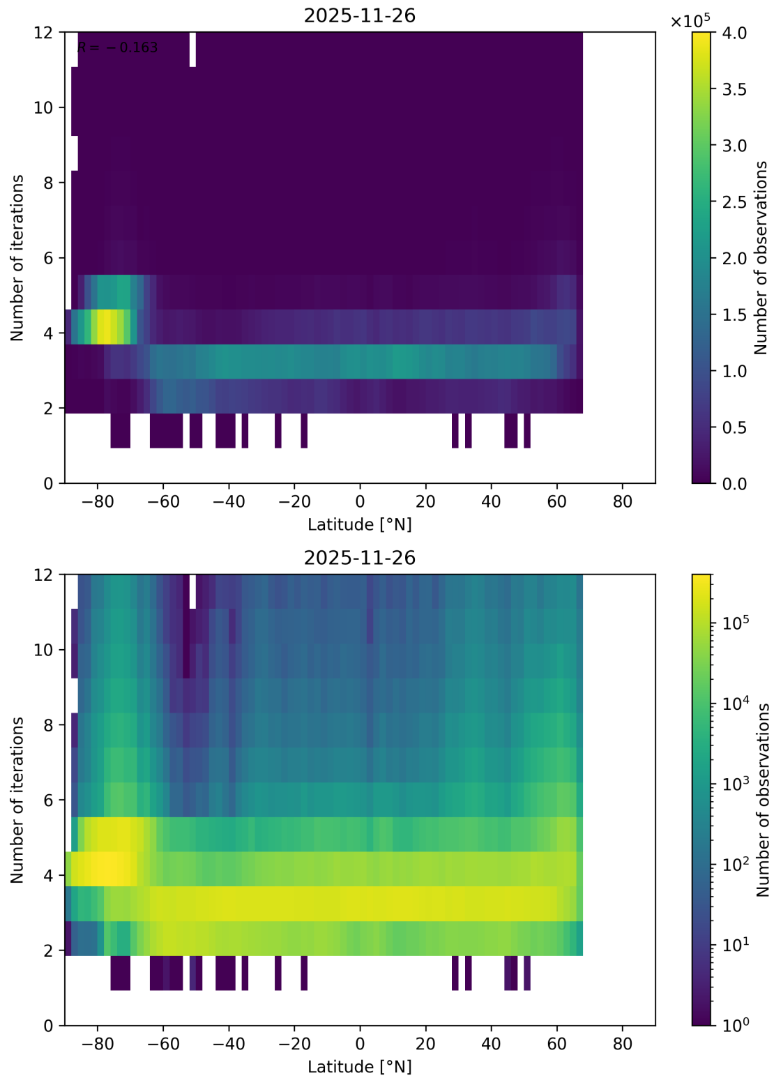
Figure 93: Scatter density plot of “Latitude” against “Number of iterations” for 2025-11-25 to 2025-11-27.
