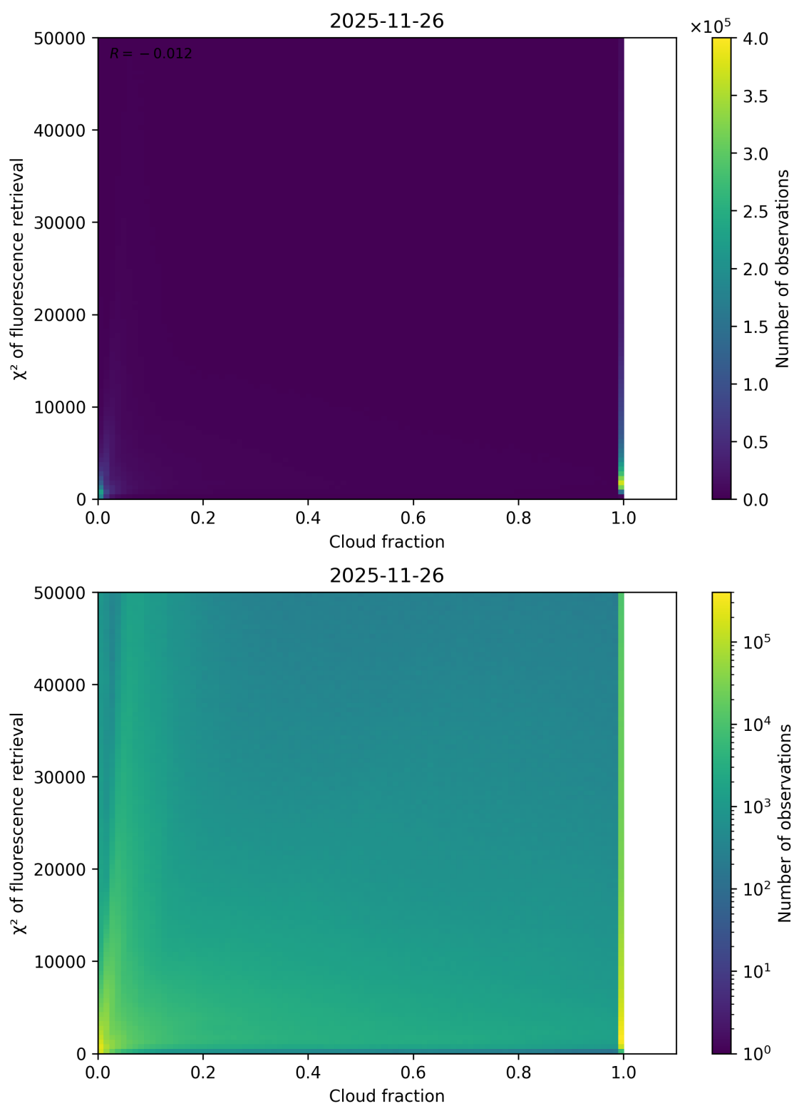
Figure 71: Scatter density plot of “Cloud fraction” against “ \chi^2 of fluorescence retrieval” for 2025-11-25 to 2025-11-27.
