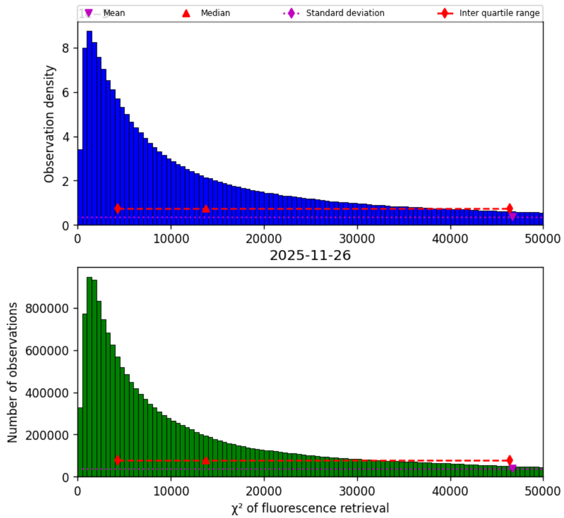
Figure 42: Histogram of “ \chi^2 of fluorescence retrieval” for 2025-11-25 to 2025-11-27
