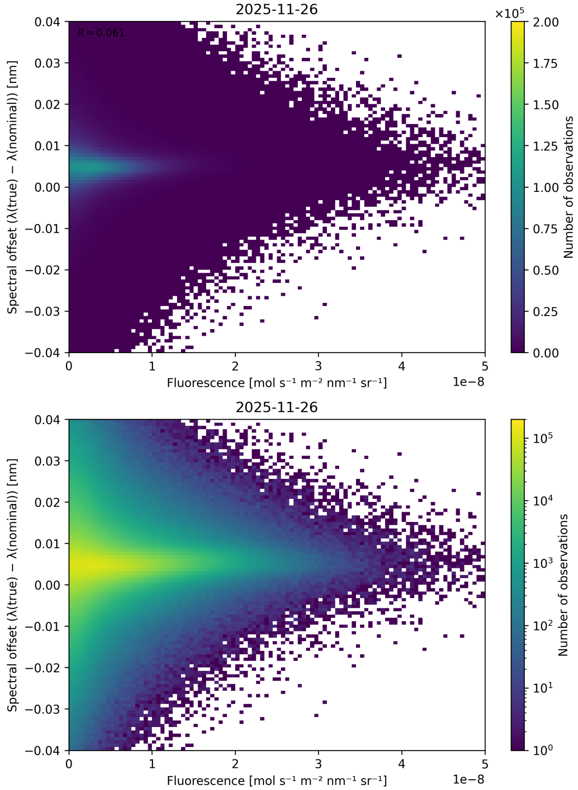
Figure 87: Scatter density plot of “Fluorescence” against “Spectral offset ( \lambda_{\text{true}} - \lambda_{\text{nominal}} )” for 2025-11-25 to 2025-11-27.
