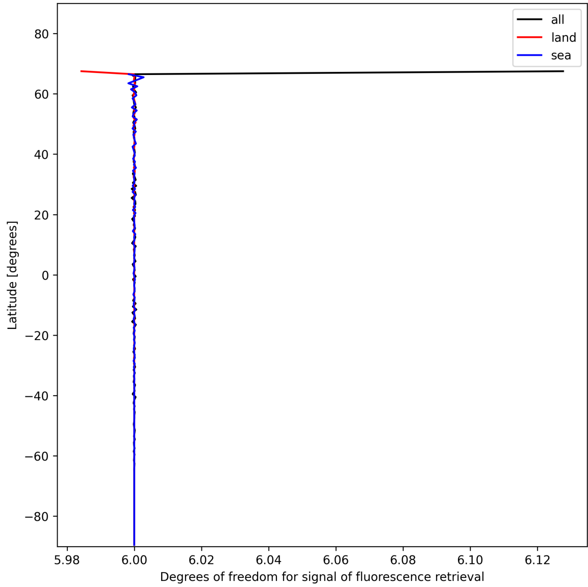
Figure 26: Zonal average of “Degrees of freedom for signal of fluorescence retrieval” for 2025-11-25 to 2025-11-27.
