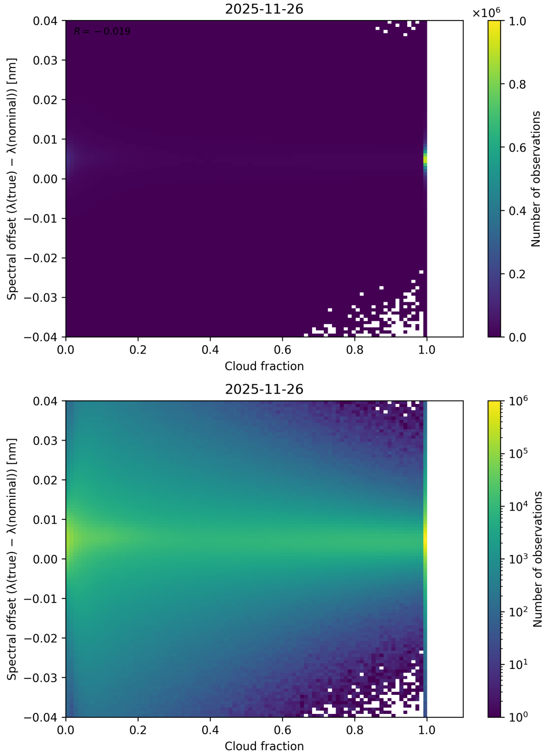
Figure 76: Scatter density plot of “Cloud fraction” against “Spectral offset ( \lambda_{\text{true}} - \lambda_{\text{nominal}} )” for 2025-11-25 to 2025-11-27.
