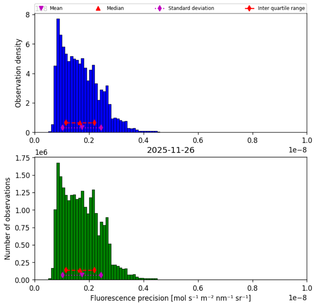
Figure 41: Histogram of “Fluorescence precision” for 2025-11-25 to 2025-11-27
