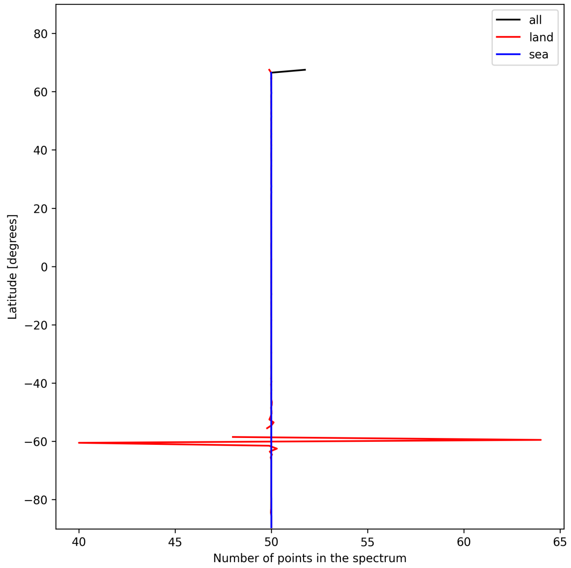
Figure 27: Zonal average of “Number of points in the spectrum” for 2025-11-25 to 2025-11-27.
