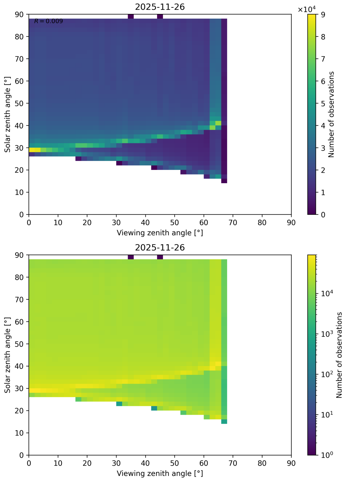
Figure 127: Scatter density plot of “Viewing zenith angle” against “Solar zenith angle” for 2025-11-25 to 2025-11-27.
