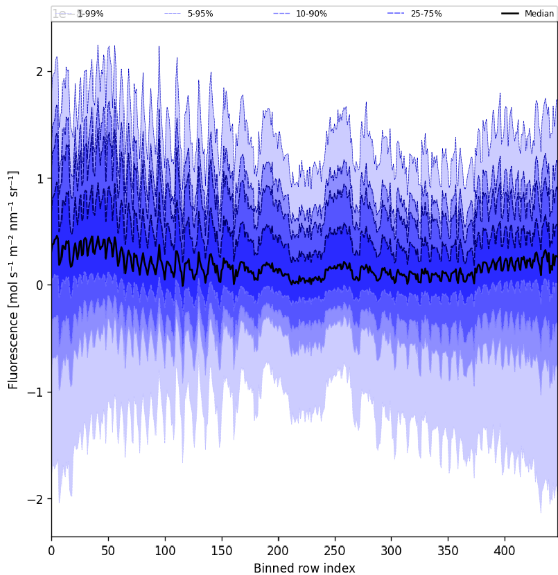
Figure 57: Along track statistics of “Fluorescence” for 2025-11-25 to 2025-11-27
