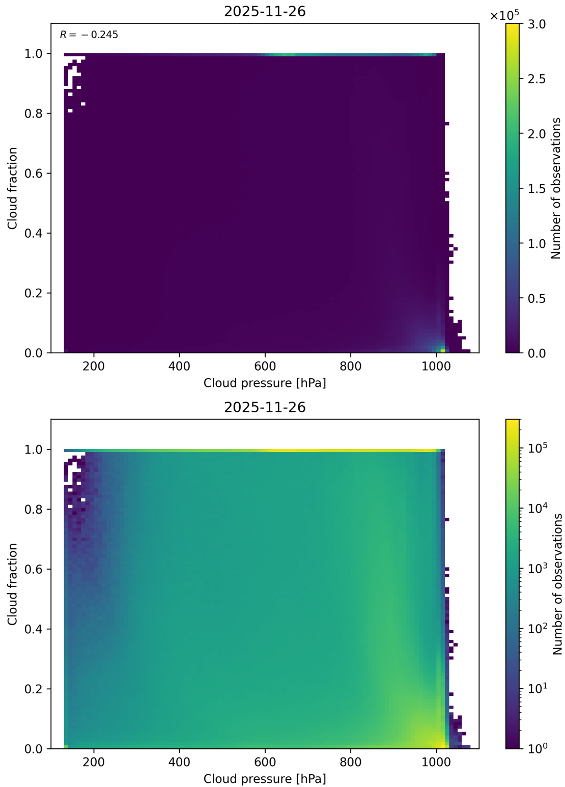
Figure 79: Scatter density plot of “Cloud pressure” against “Cloud fraction” for 2025-11-25 to 2025-11-27.
