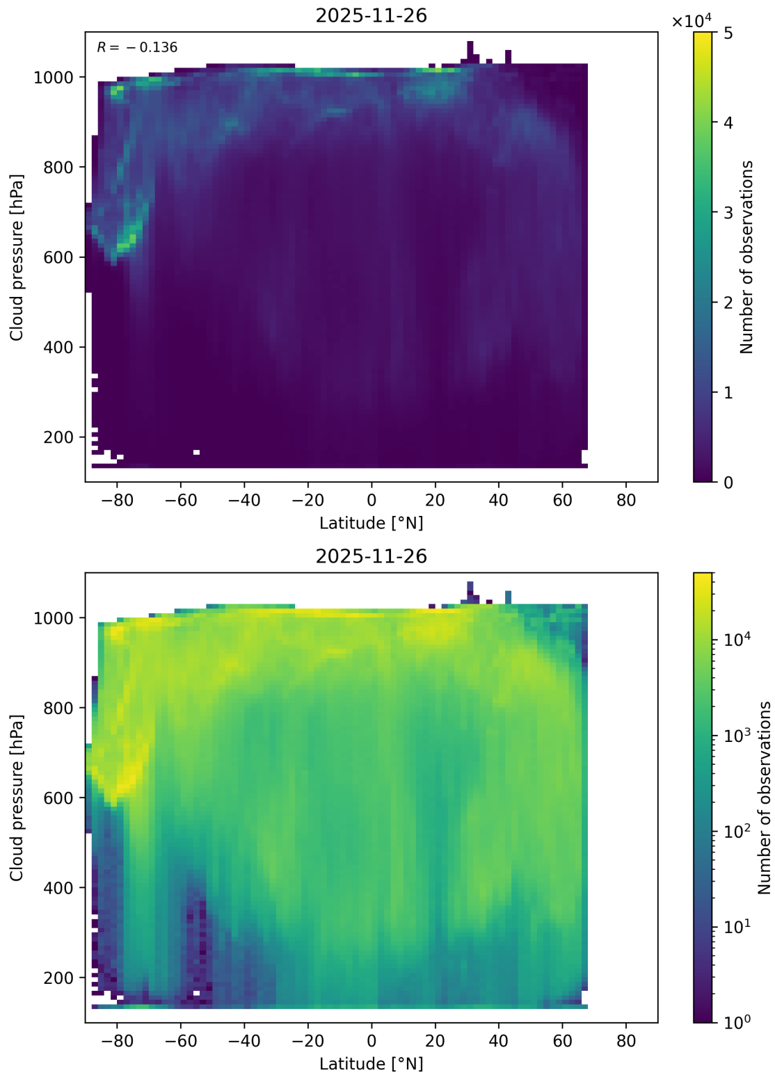
Figure 91: Scatter density plot of “Latitude” against “Cloud pressure” for 2025-11-25 to 2025-11-27.
