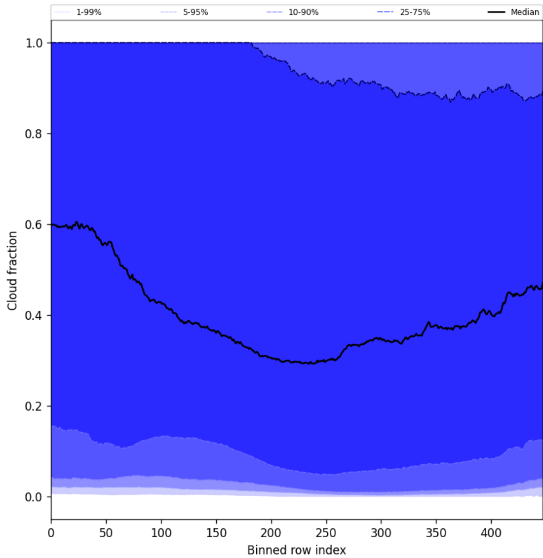
Figure 49: Along track statistics of “Cloud fraction” for 2025-11-25 to 2025-11-27
