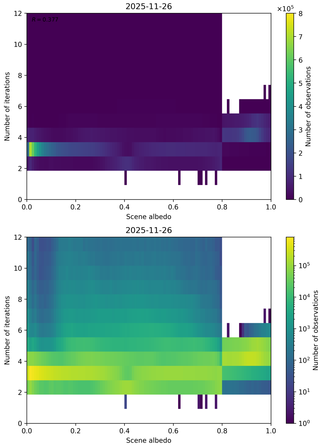
Figure 105: Scatter density plot of “Scene albedo” against “Number of iterations” for 2025-11-25 to 2025-11-27.
