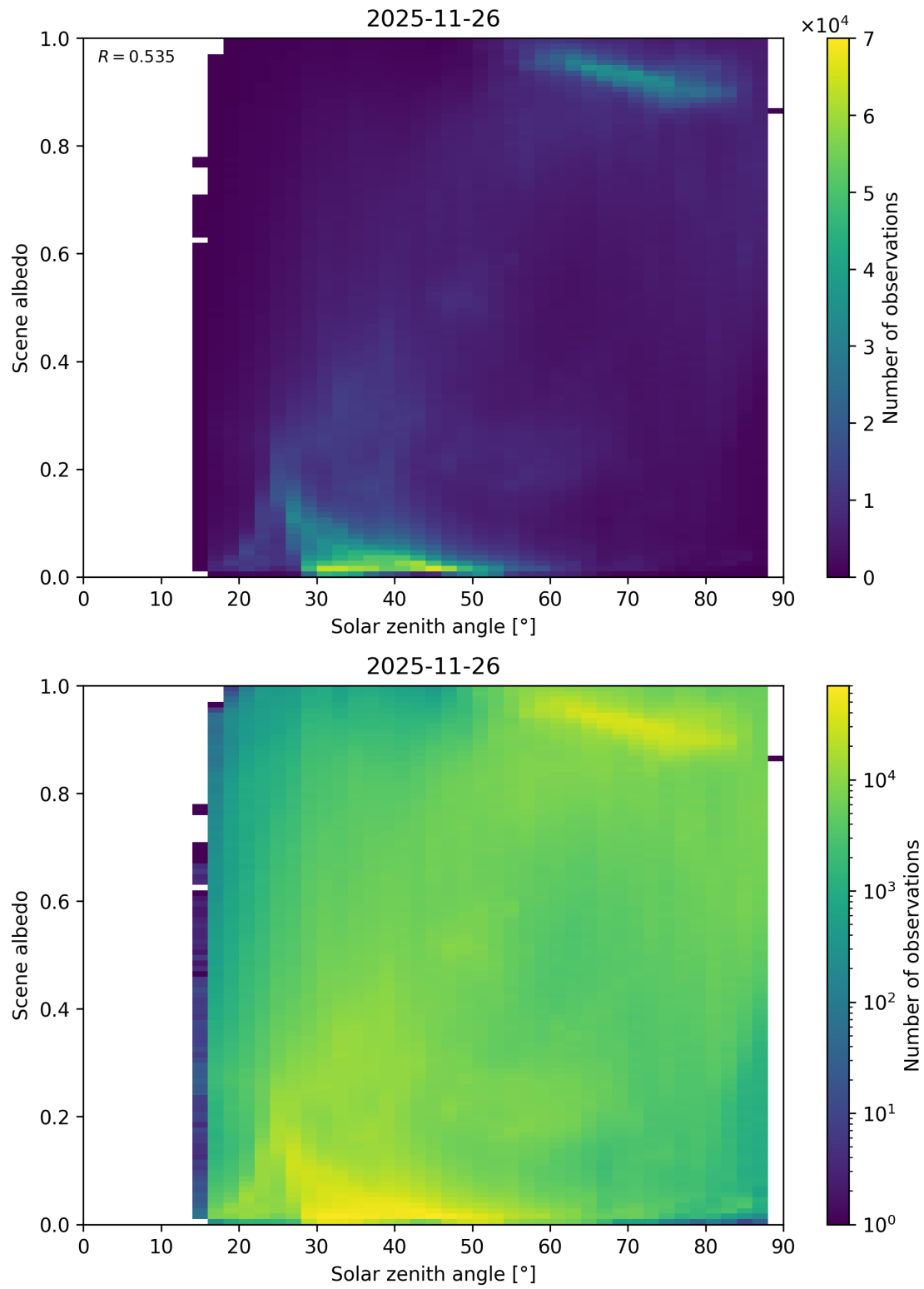
Figure 116: Scatter density plot of “Solar zenith angle” against “Scene albedo” for 2025-11-25 to 2025-11-27.
