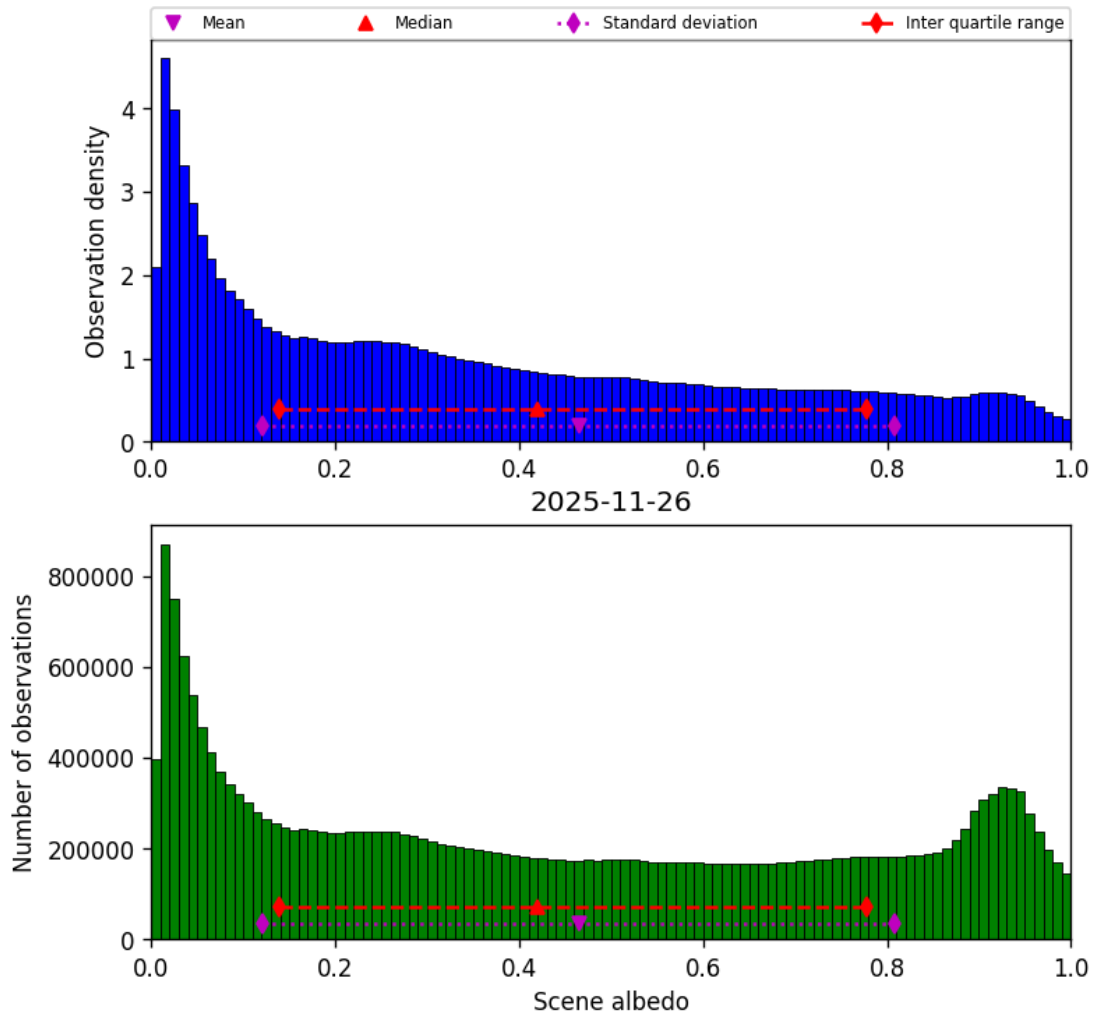
Figure 34: Histogram of “Scene albedo” for 2025-11-25 to 2025-11-27
