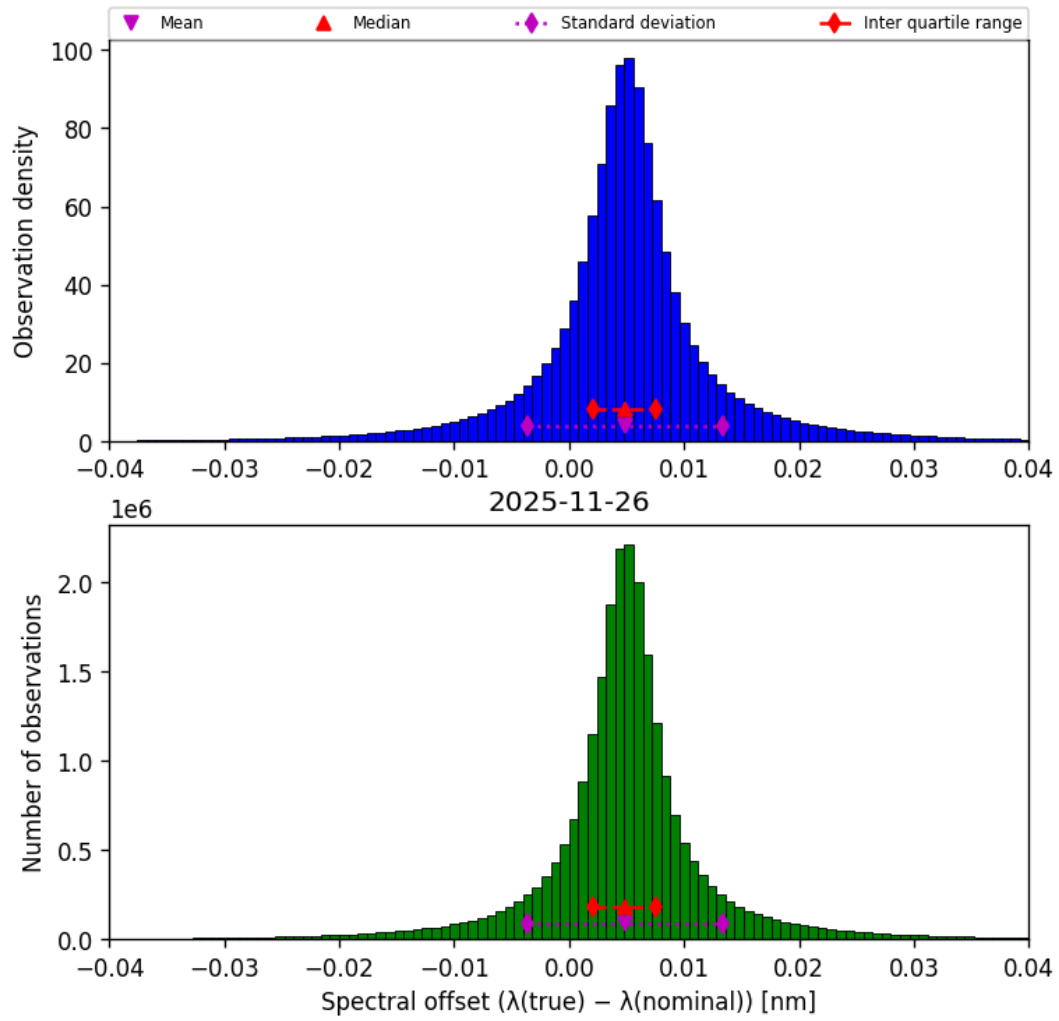
Figure 45: Histogram of “Spectral offset ( \lambda_{\text{true}} - \lambda_{\text{nominal}} )” for 2025-11-25 to 2025-11-27
