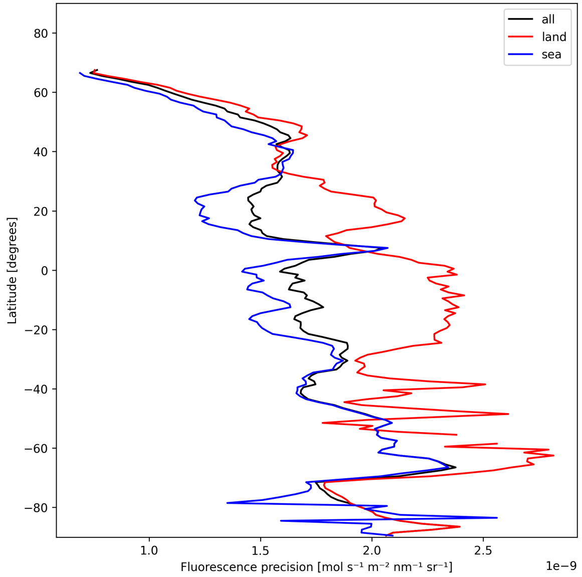
Figure 24: Zonal average of “Fluorescence precision” for 2025-11-25 to 2025-11-27.
