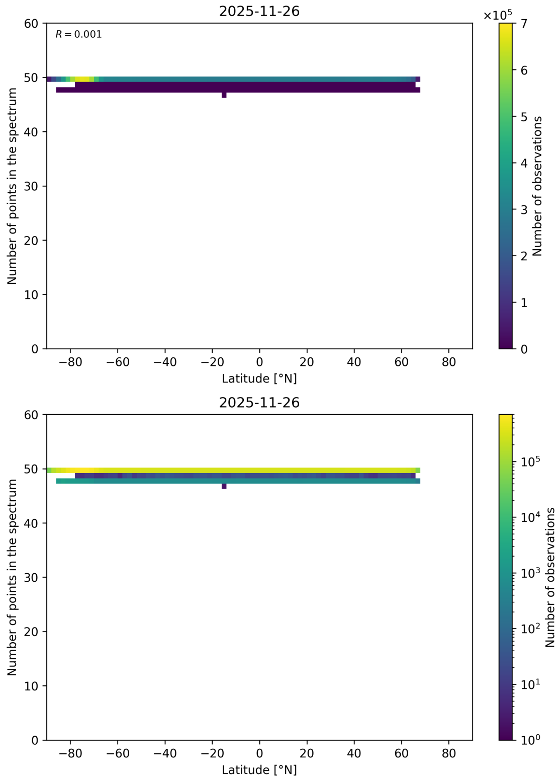
Figure 94: Scatter density plot of “Latitude” against “Number of points in the spectrum” for 2025-11-25 to 2025-11-27.
