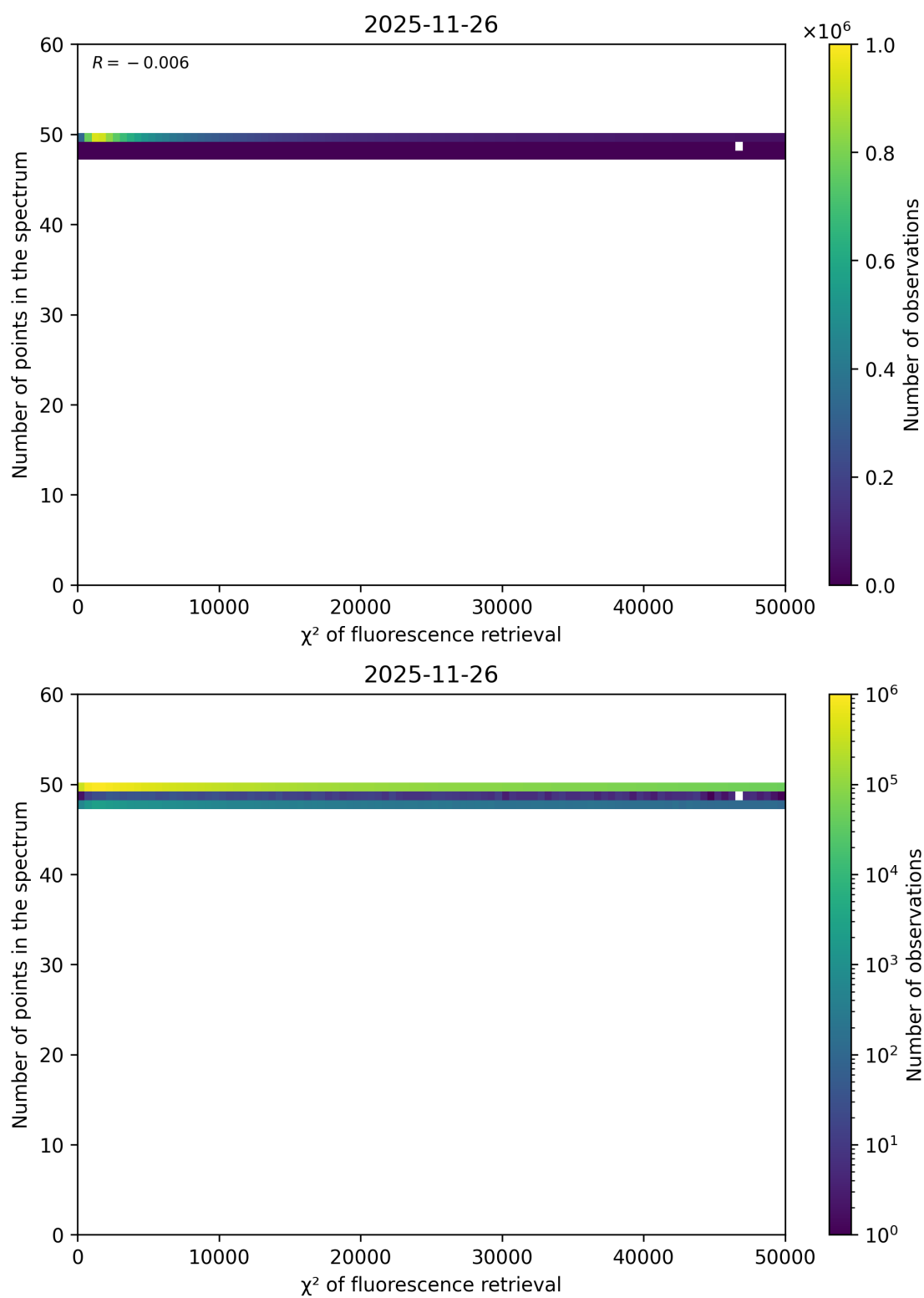
Figure 68: Scatter density plot of " \chi^2 of fluorescence retrieval" against "Number of points in the spectrum" for 2025-11-25 to 2025-11-27.
