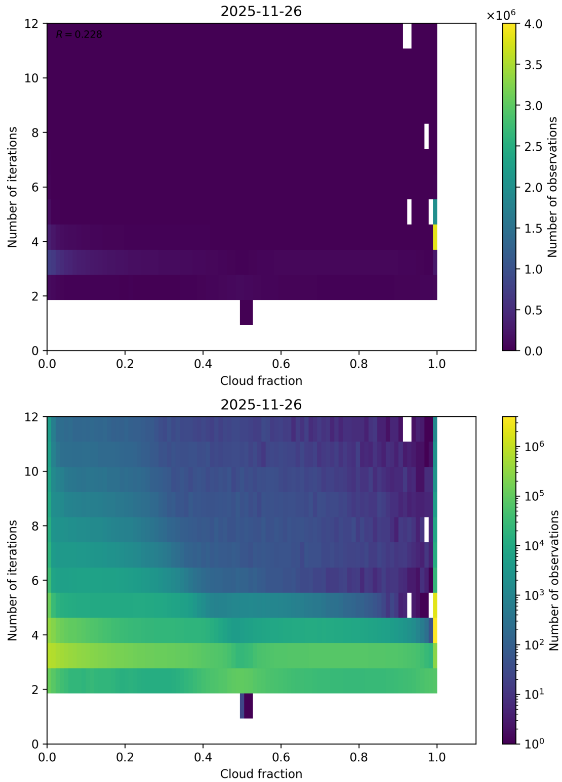
Figure 73: Scatter density plot of “Cloud fraction” against “Number of iterations” for 2025-11-25 to 2025-11-27.
