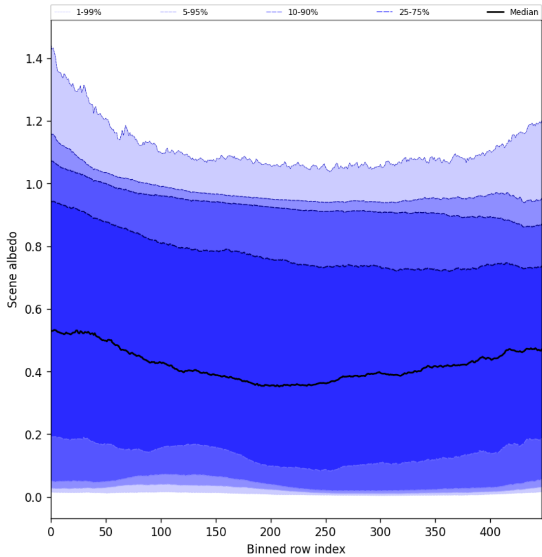
Figure 51: Along track statistics of “Scene albedo” for 2025-11-25 to 2025-11-27
