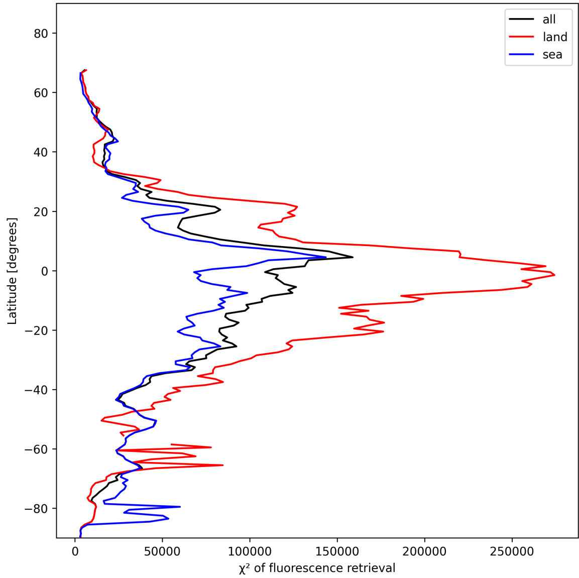
Figure 25: Zonal average of “ \chi^2 of fluorescence retrieval” for 2025-11-25 to 2025-11-27.
