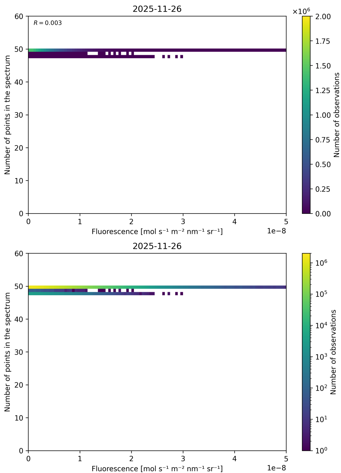
Figure 86: Scatter density plot of “Fluorescence” against “Number of points in the spectrum” for 2025-11-25 to 2025-11-27.
