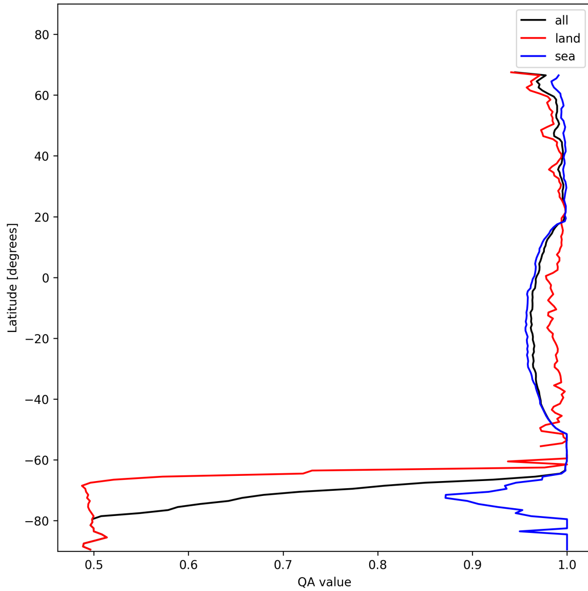
Figure 12: Zonal average of “QA value” for 2025-11-25 to 2025-11-27.
