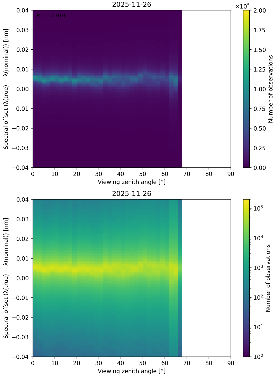
Figure 128: Scatter density plot of “Viewing zenith angle” against “Spectral offset ( \lambda_{\text{true}} - \lambda_{\text{nominal}} )” for 2025-11-25 to 2025-11-27.
