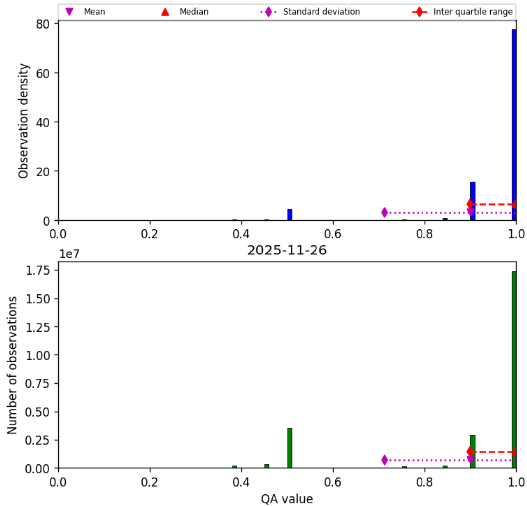
Figure 29: Histogram of “QA value” for 2025-11-25 to 2025-11-27
