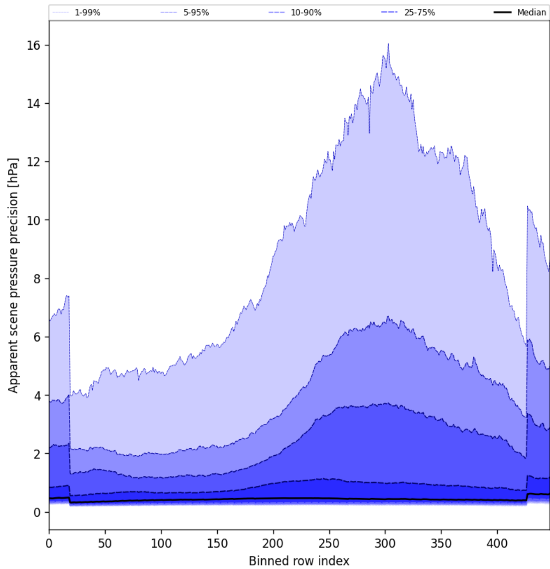
Figure 54: Along track statistics of “Apparent scene pressure precision” for 2025-11-25 to 2025-11-27
