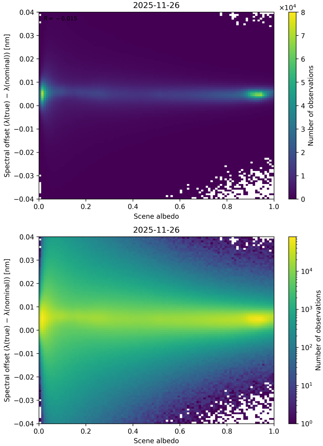
Figure 107: Scatter density plot of “Scene albedo” against “Spectral offset ( \lambda_{\text{true}} - \lambda_{\text{nominal}} )” for 2025-11-25 to 2025-11-27.
