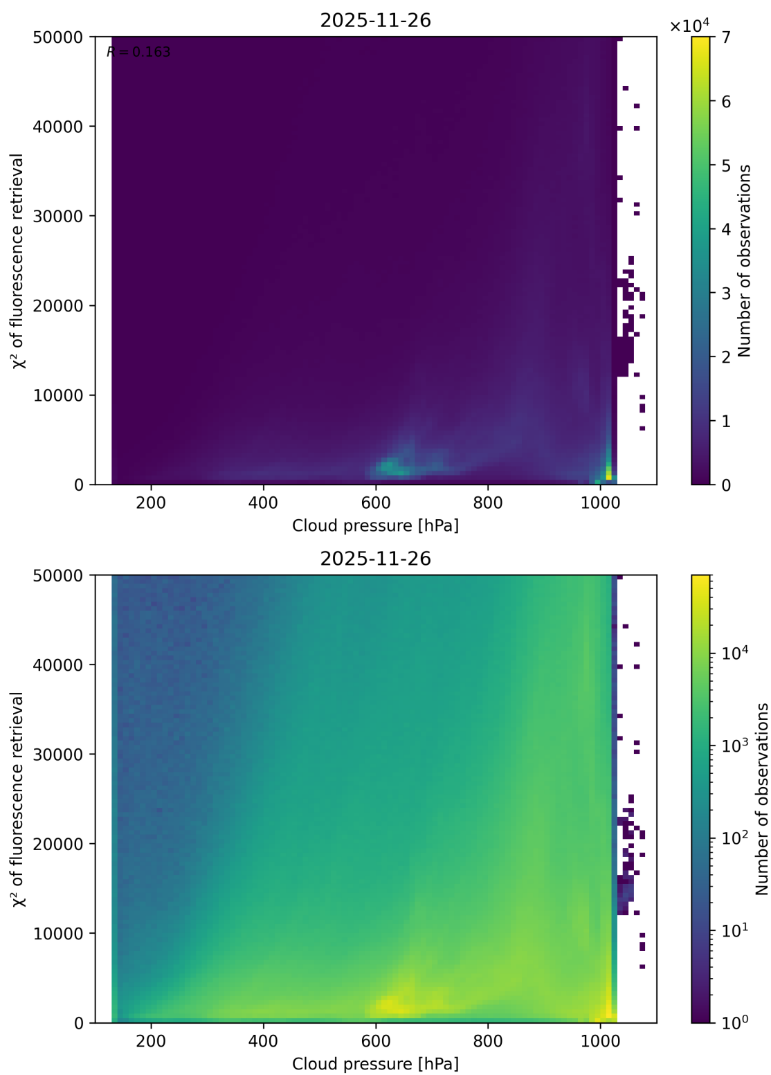
Figure 78: Scatter density plot of “Cloud pressure” against “ \chi^2 of fluorescence retrieval” for 2025-11-25 to 2025-11-27.
