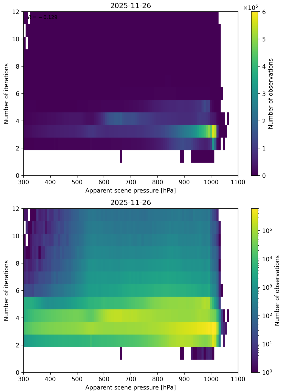
Figure 65: Scatter density plot of “Apparent scene pressure” against “Number of iterations” for 2025-11-25 to 2025-11-27.
