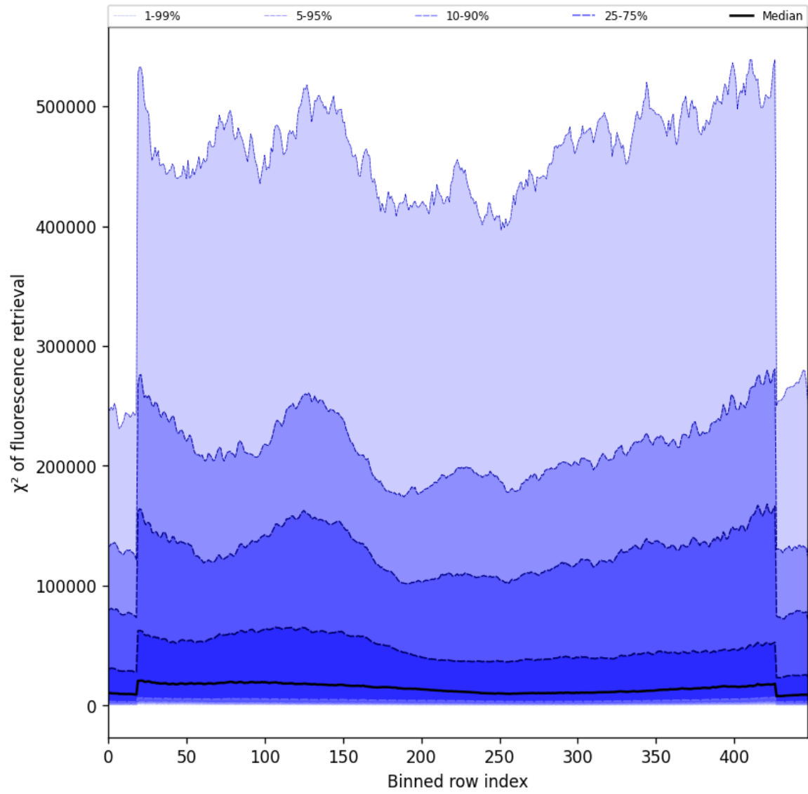
Figure 59: Along track statistics of “ \chi^2 of fluorescence retrieval” for 2025-11-25 to 2025-11-27
