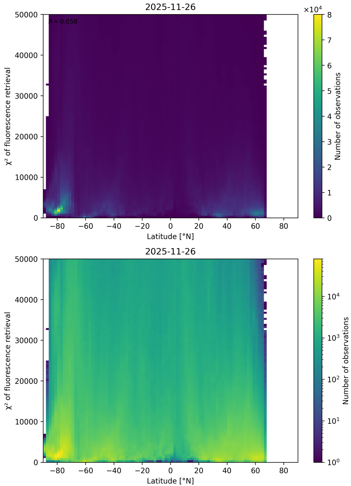
Figure 89: Scatter density plot of “Latitude” against “ \chi^2 of fluorescence retrieval” for 2025-11-25 to 2025-11-27.
