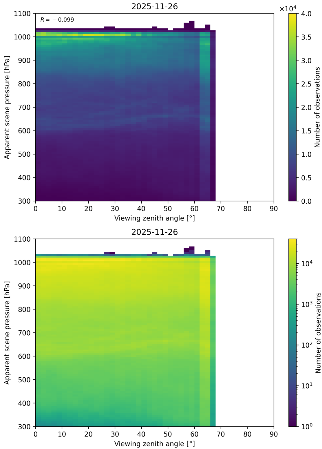
Figure 118: Scatter density plot of “Viewing zenith angle” against “Apparent scene pressure” for 2025-11-25 to 2025-11-27.
