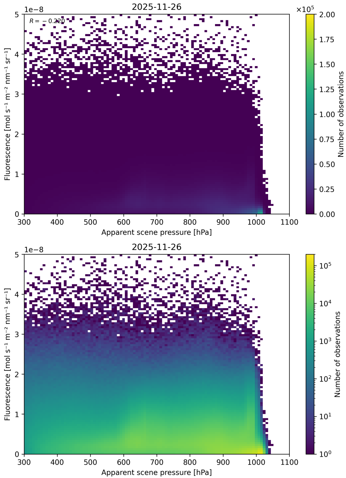
Figure 64: Scatter density plot of “Apparent scene pressure” against “Fluorescence” for 2025-11-25 to 2025-11-27.
