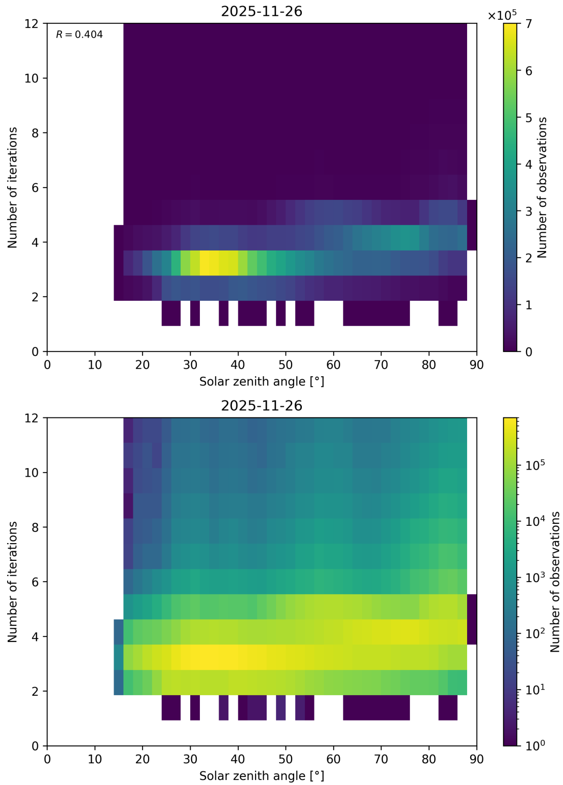
Figure 114: Scatter density plot of “Solar zenith angle” against “Number of iterations” for 2025-11-25 to 2025-11-27.
