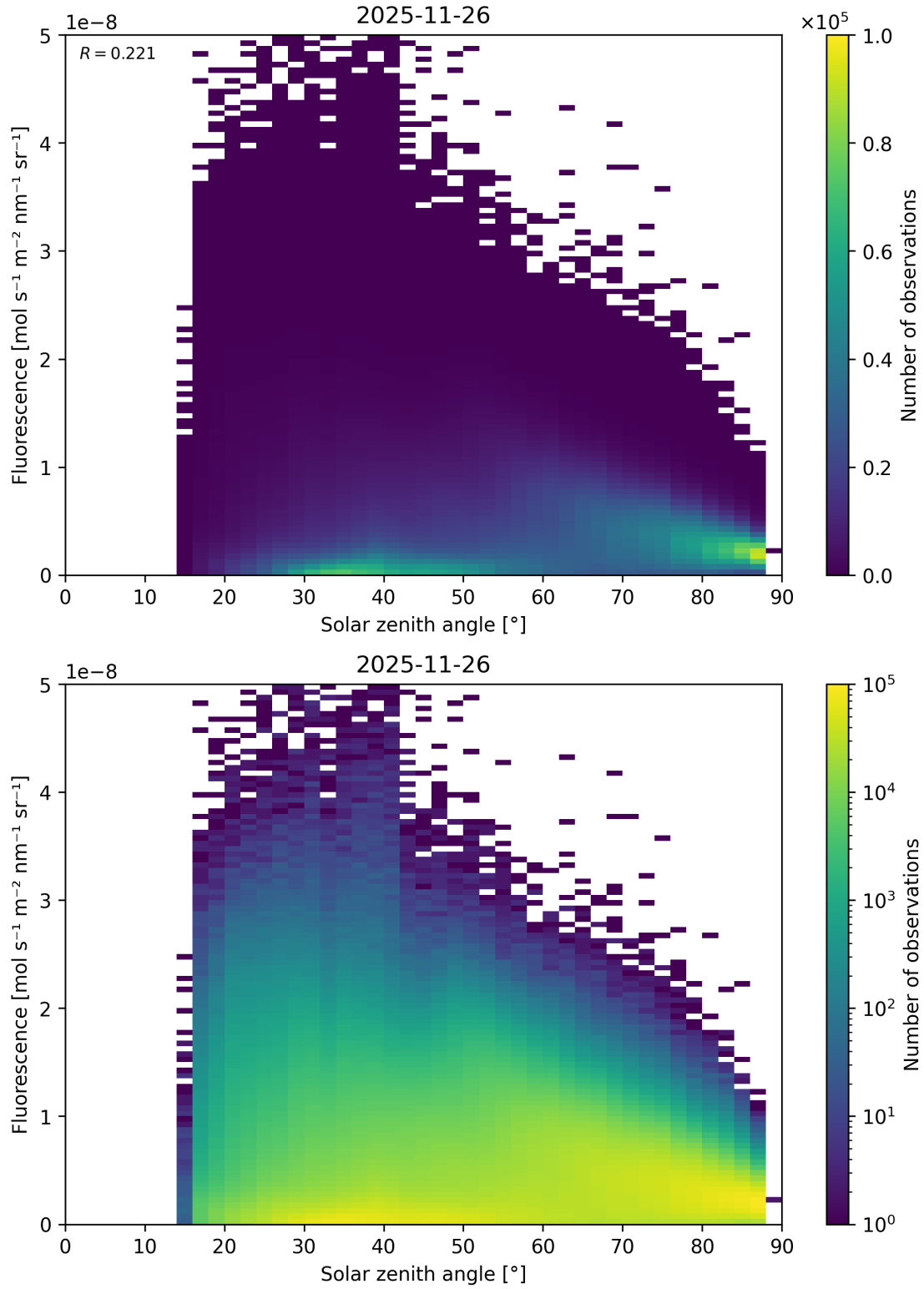
Figure 112: Scatter density plot of “Solar zenith angle” against “Fluorescence” for 2025-11-25 to 2025-11-27.
