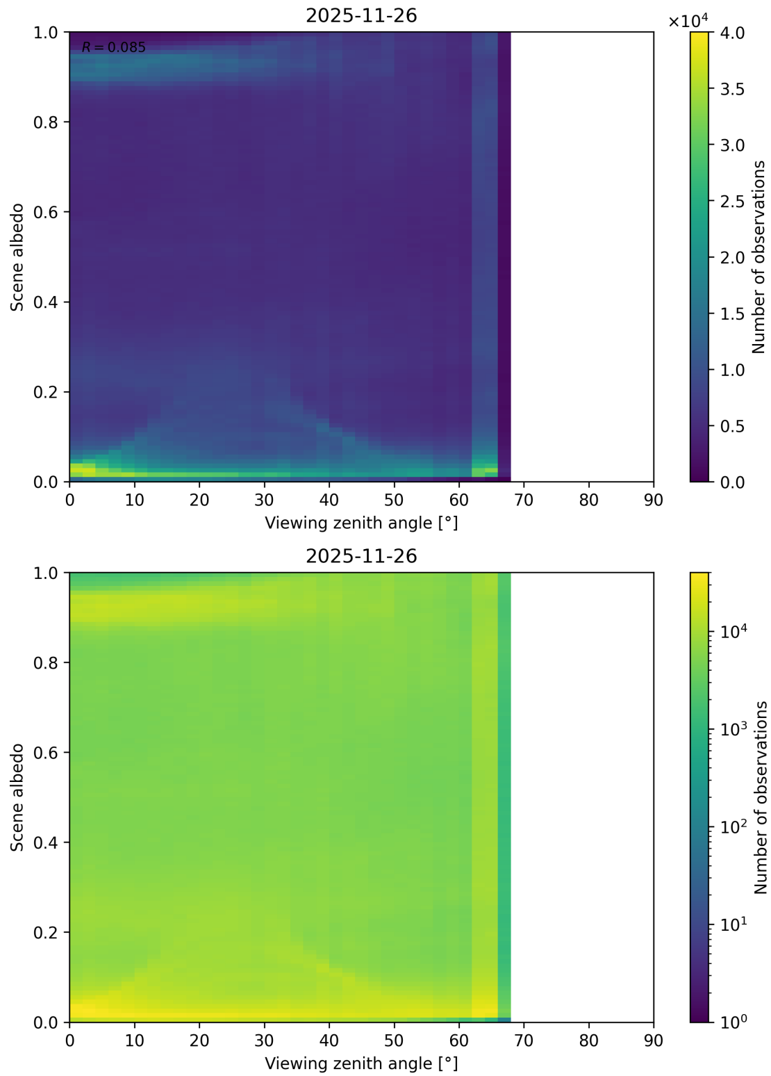
Figure 126: Scatter density plot of “Viewing zenith angle” against “Scene albedo” for 2025-11-25 to 2025-11-27.
