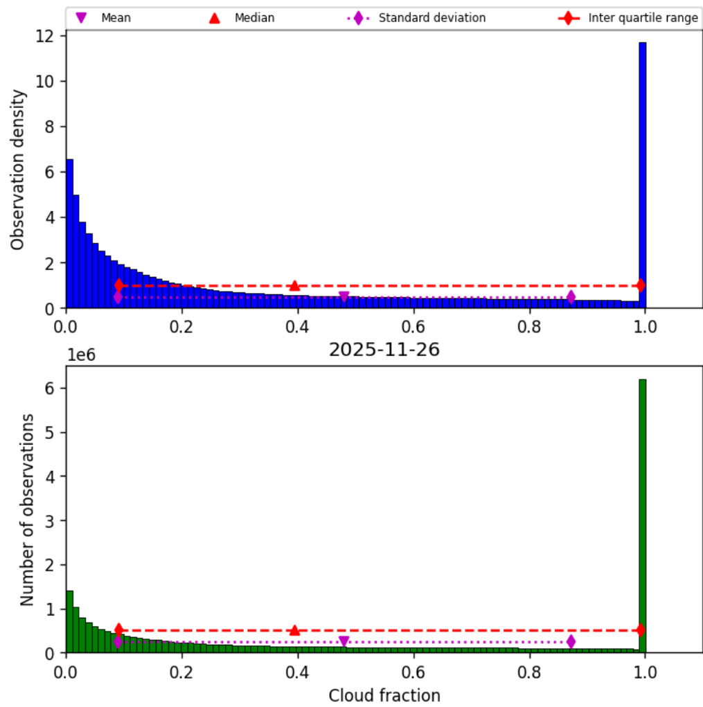
Figure 32: Histogram of “Cloud fraction” for 2025-11-25 to 2025-11-27
