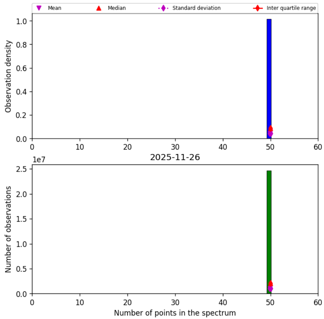
Figure 44: Histogram of “Number of points in the spectrum” for 2025-11-25 to 2025-11-27
