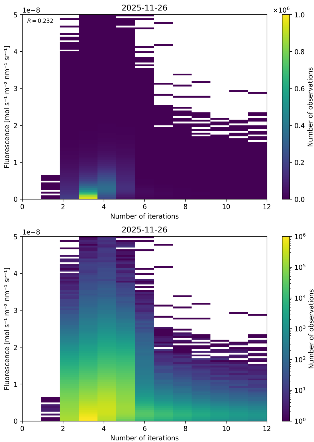
Figure 98: Scatter density plot of “Number of iterations” against “Fluorescence” for 2025-11-25 to 2025-11-27.
