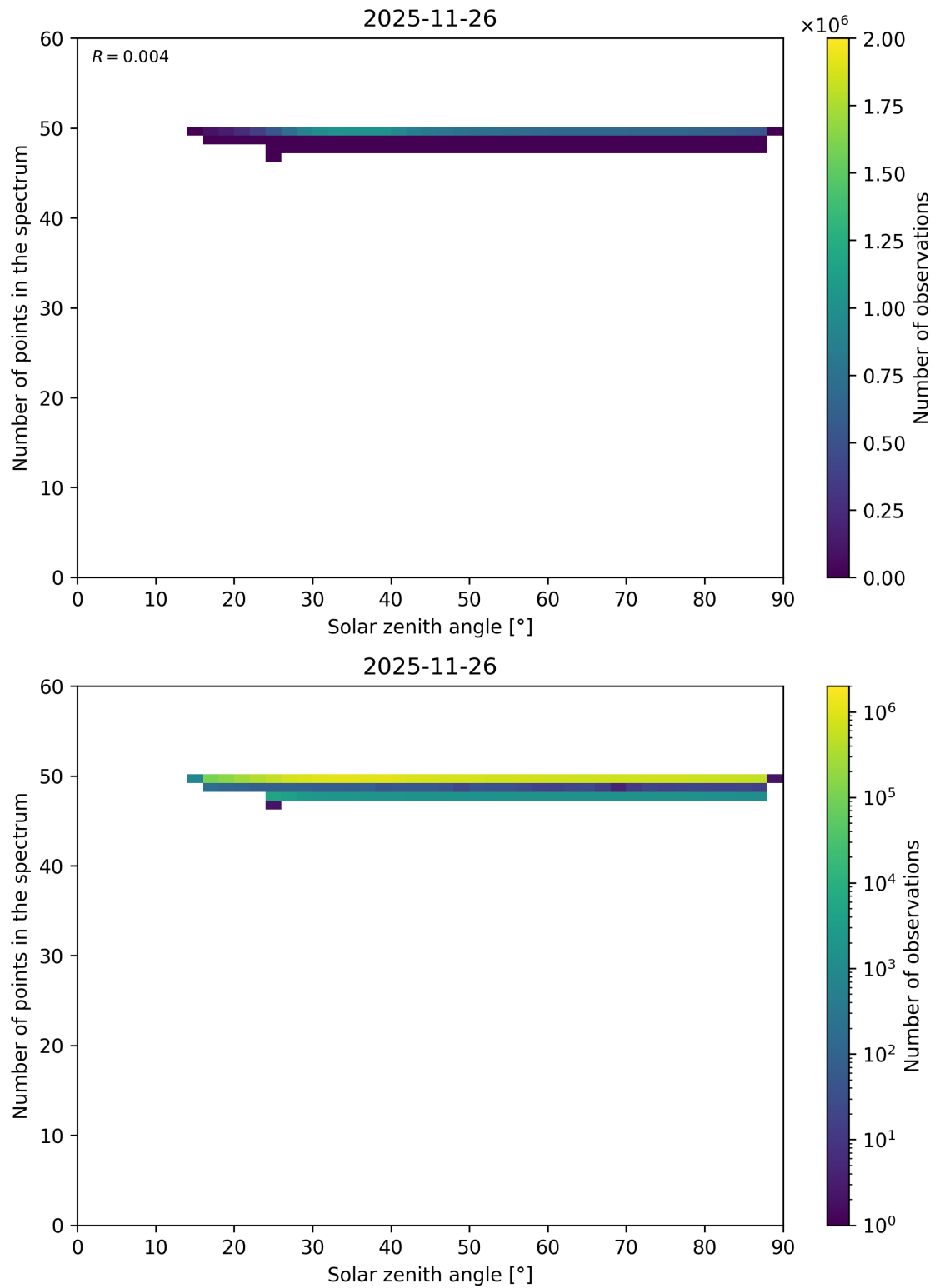
Figure 115: Scatter density plot of “Solar zenith angle” against “Number of points in the spectrum” for 2025-11-25 to 2025-11-27.
