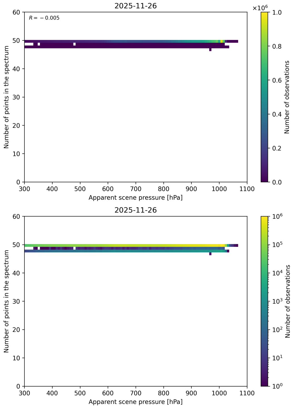
Figure 66: Scatter density plot of “Apparent scene pressure” against “Number of points in the spectrum” for 2025-11-25 to 2025-11-27.
