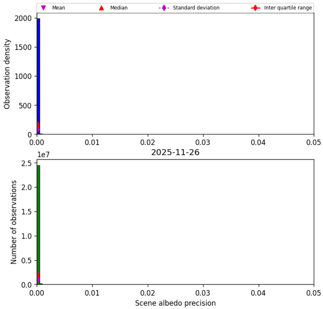
Figure 35: Histogram of “Scene albedo precision” for 2025-11-25 to 2025-11-27
