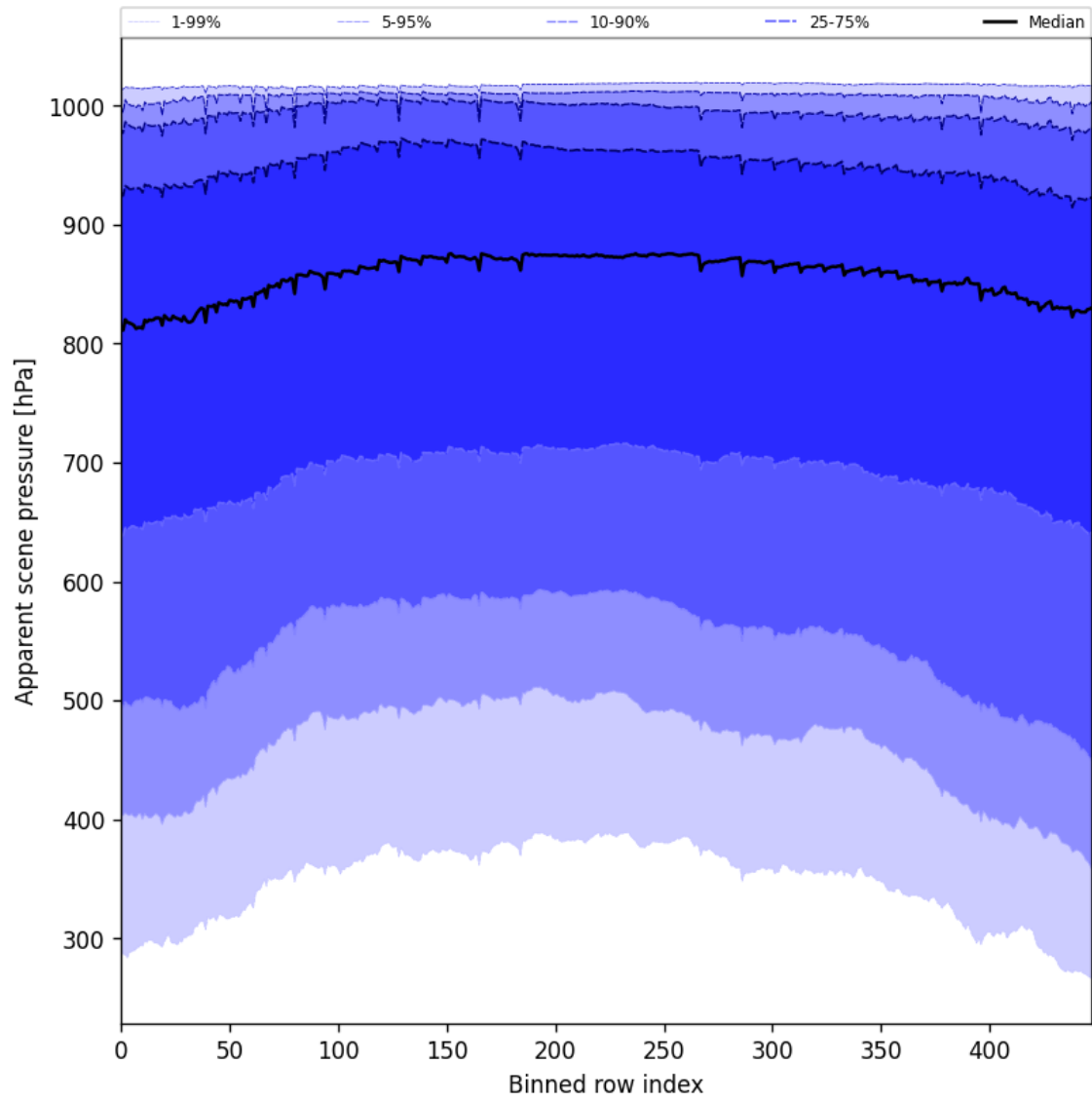
Figure 53: Along track statistics of “Apparent scene pressure” for 2025-11-25 to 2025-11-27
