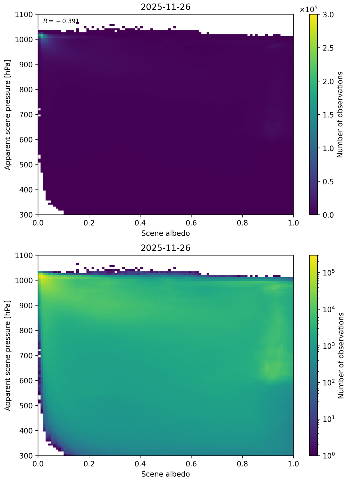
Figure 102: Scatter density plot of “Scene albedo” against “Apparent scene pressure” for 2025-11-25 to 2025-11-27.
