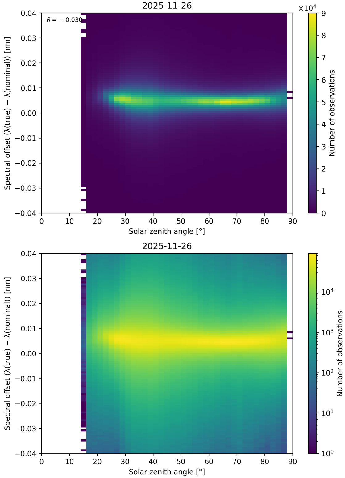
Figure 117: Scatter density plot of “Solar zenith angle” against “Spectral offset ( \lambda_{\text{true}} - \lambda_{\text{nominal}} )” for 2025-11-25 to 2025-11-27.
