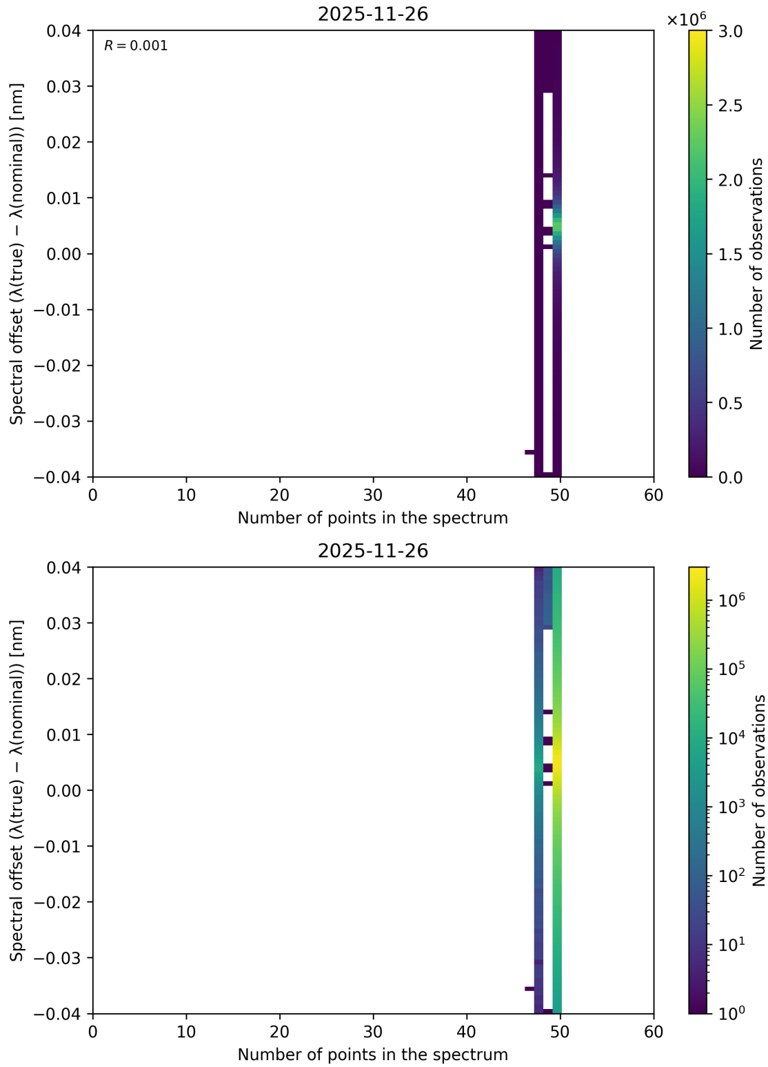
Figure 101: Scatter density plot of “Number of points in the spectrum” against “Spectral offset ( \lambda_{\text{true}} - \lambda_{\text{nominal}} )” for 2025-11-25 to 2025-11-27.
