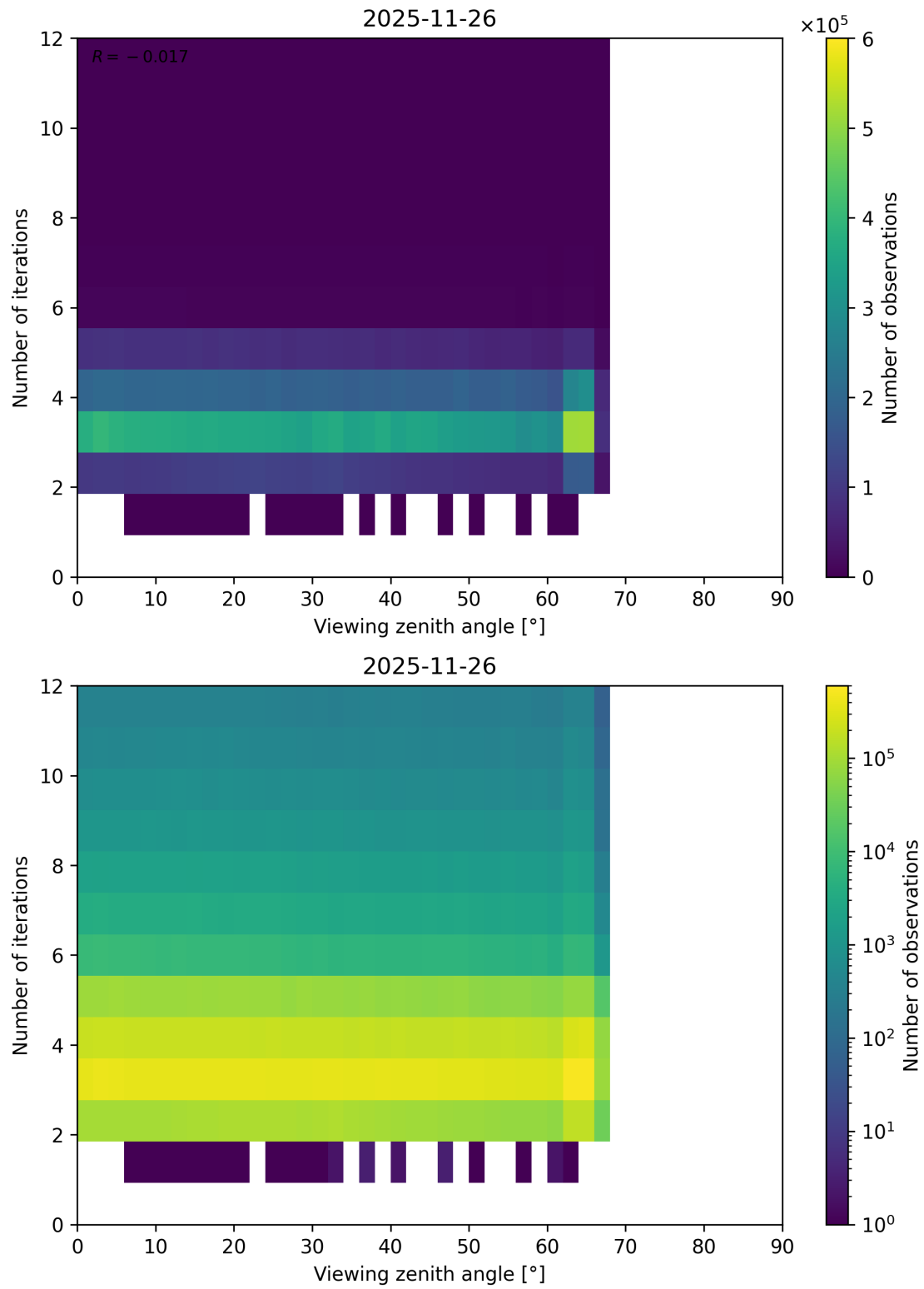
Figure 124: Scatter density plot of “Viewing zenith angle” against “Number of iterations” for 2025-11-25 to 2025-11-27.
