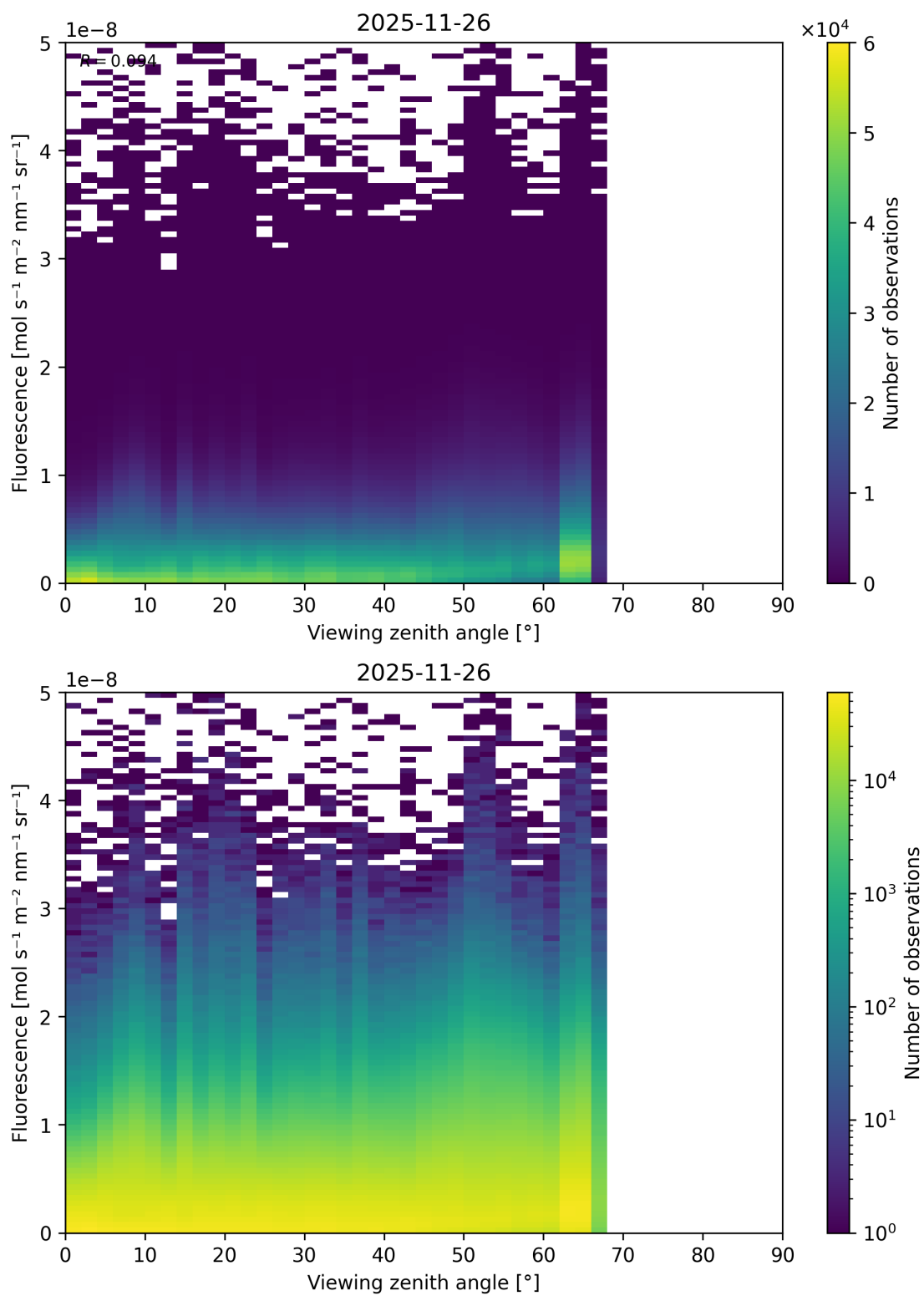
Figure 122: Scatter density plot of “Viewing zenith angle” against “Fluorescence” for 2025-11-25 to 2025-11-27.
