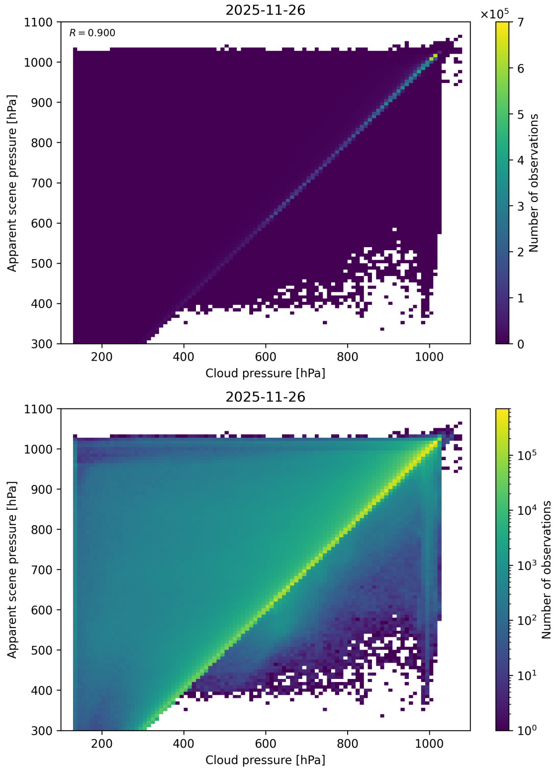
Figure 77: Scatter density plot of “Cloud pressure” against “Apparent scene pressure” for 2025-11-25 to 2025-11-27.
