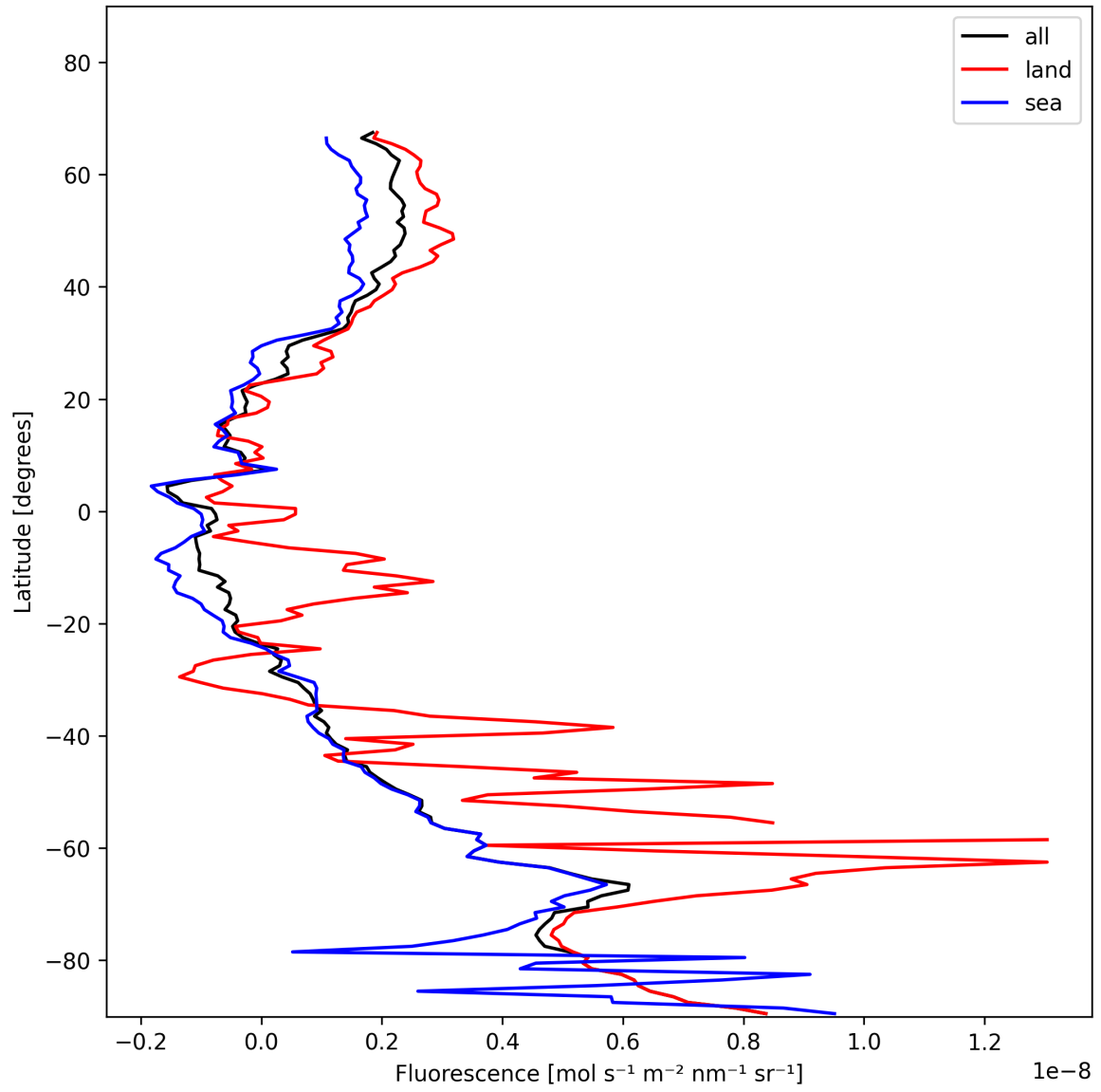
Figure 23: Zonal average of “Fluorescence” for 2025-11-25 to 2025-11-27.
