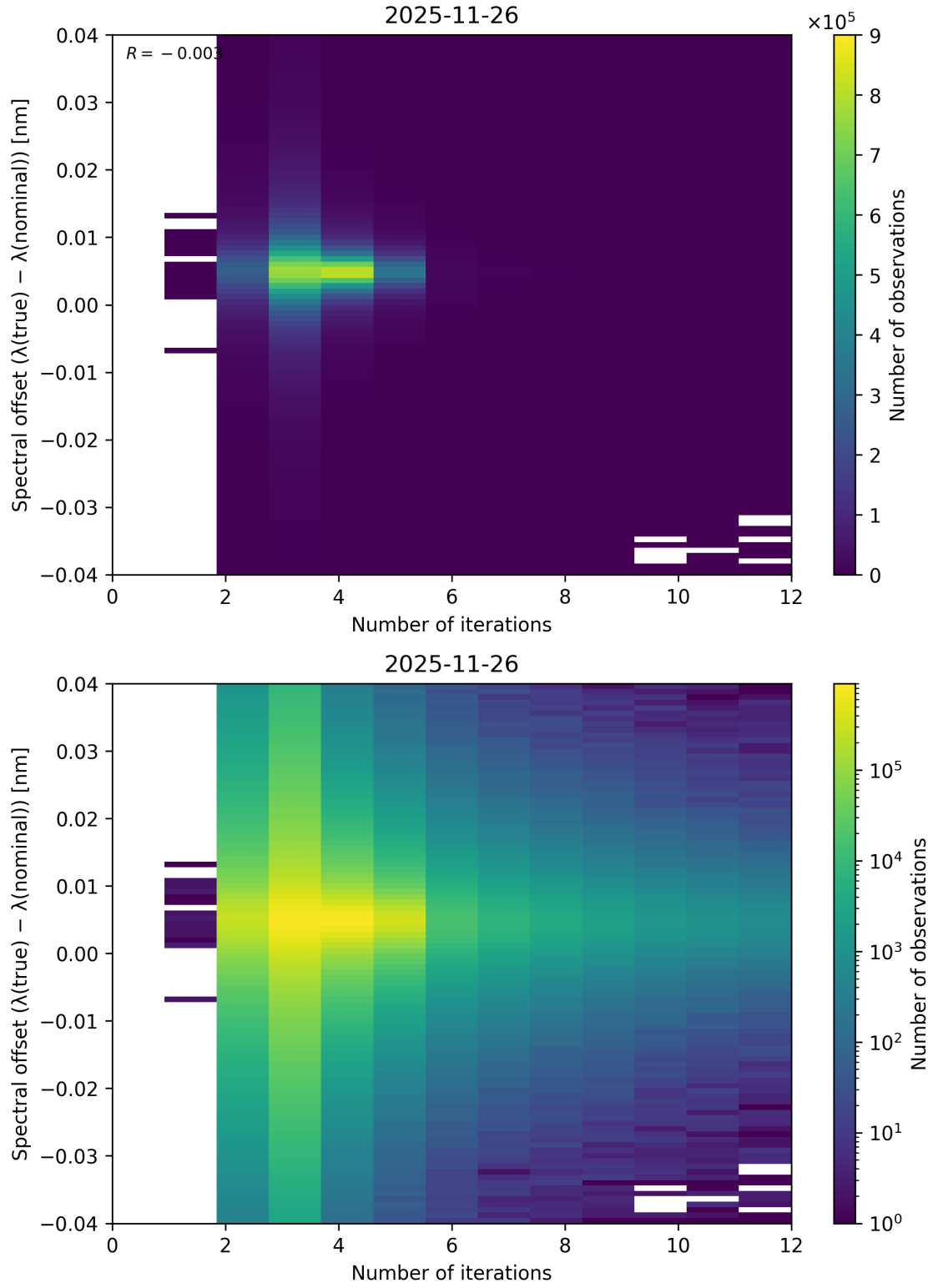
Figure 100: Scatter density plot of “Number of iterations” against “Spectral offset ( \lambda_{\text{true}} - \lambda_{\text{nominal}} )” for 2025-11-25 to 2025-11-27.
