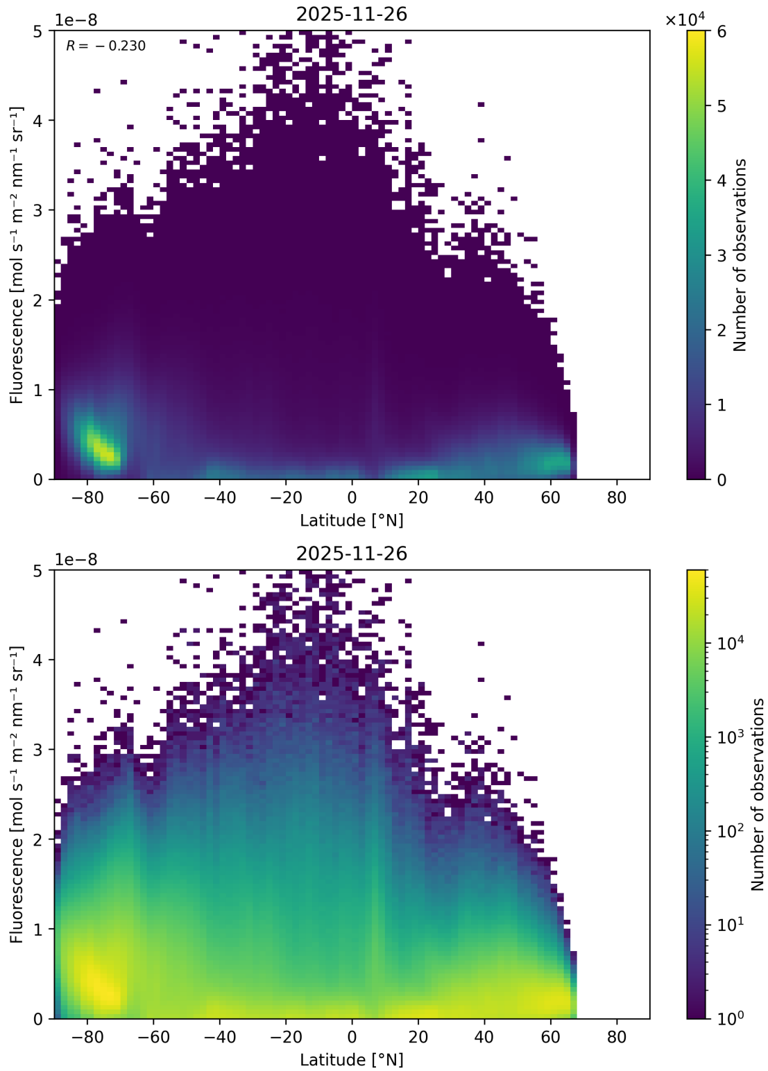
Figure 92: Scatter density plot of “Latitude” against “Fluorescence” for 2025-11-25 to 2025-11-27.
