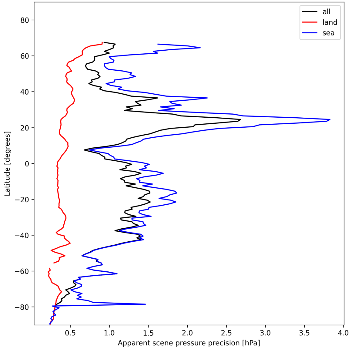
Figure 20: Zonal average of “Apparent scene pressure precision” for 2025-11-25 to 2025-11-27.
