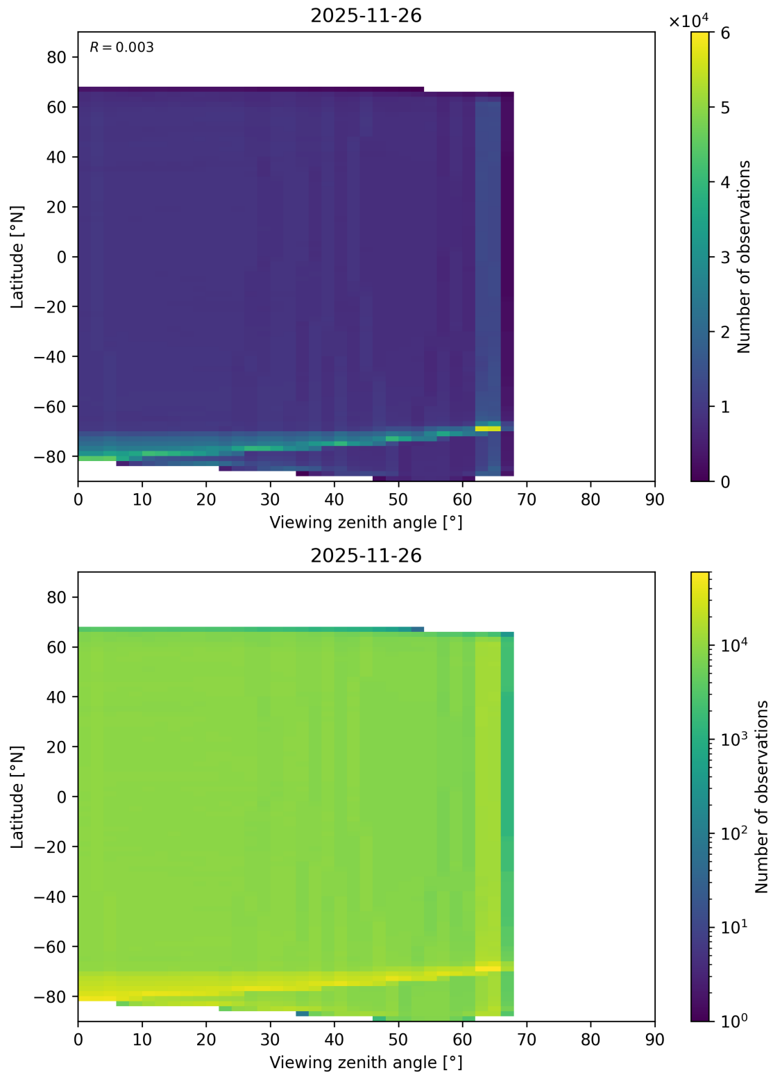
Figure 123: Scatter density plot of “Viewing zenith angle” against “Latitude” for 2025-11-25 to 2025-11-27.
