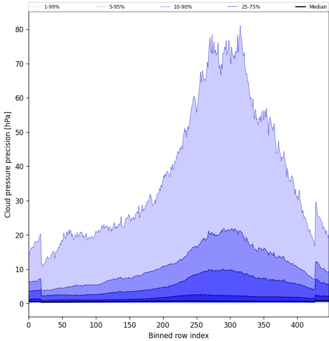
Figure 48: Along track statistics of “Cloud pressure precision” for 2025-11-25 to 2025-11-27
