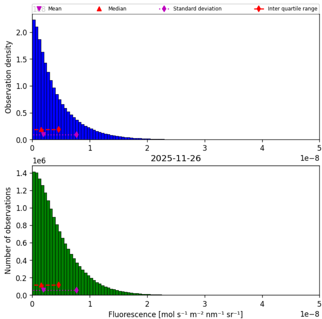
Figure 40: Histogram of “Fluorescence” for 2025-11-25 to 2025-11-27
