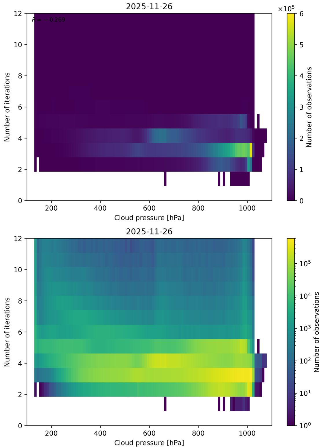
Figure 81: Scatter density plot of “Cloud pressure” against “Number of iterations” for 2025-11-25 to 2025-11-27.
