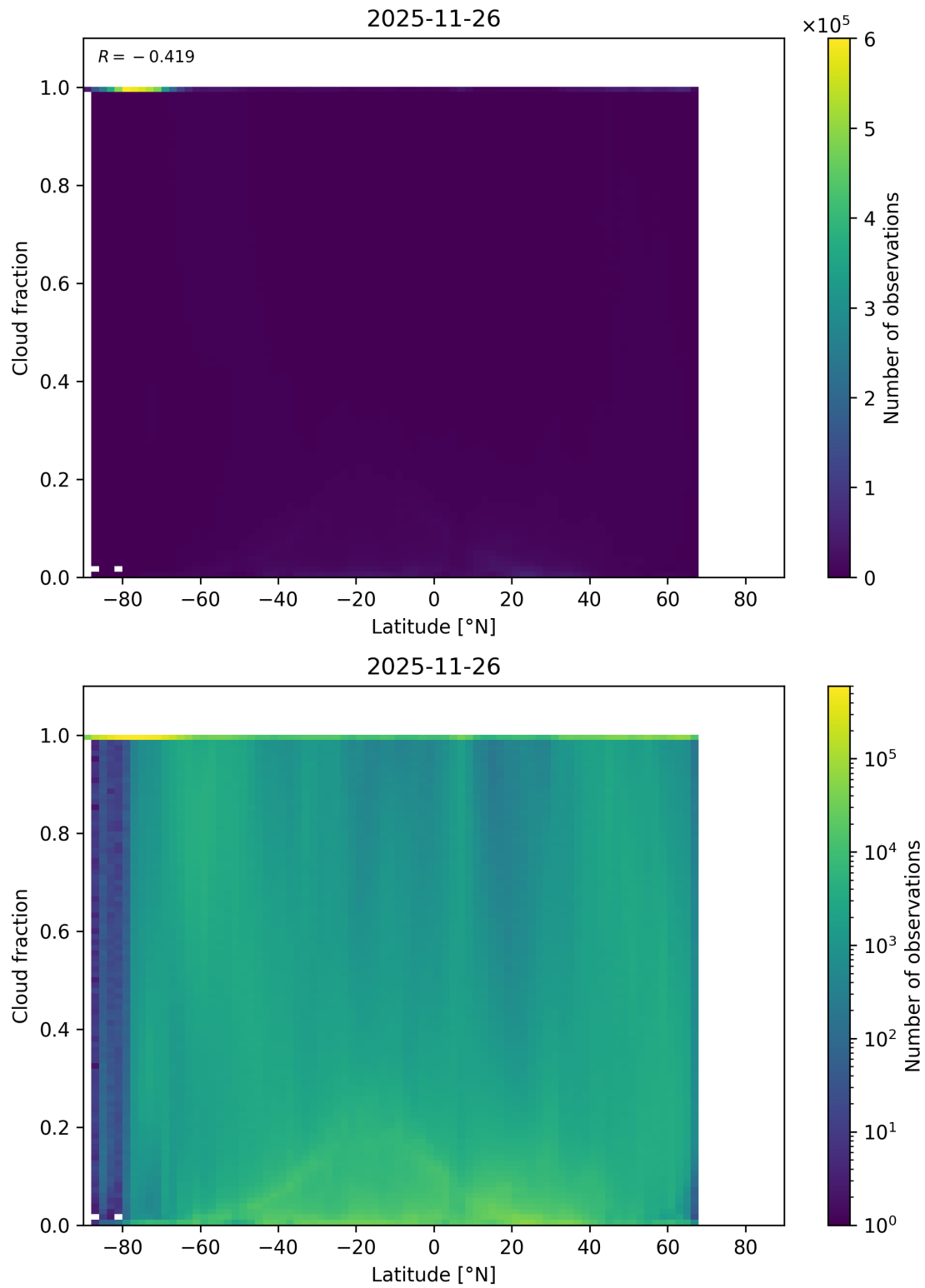
Figure 90: Scatter density plot of “Latitude” against “Cloud fraction” for 2025-11-25 to 2025-11-27.
