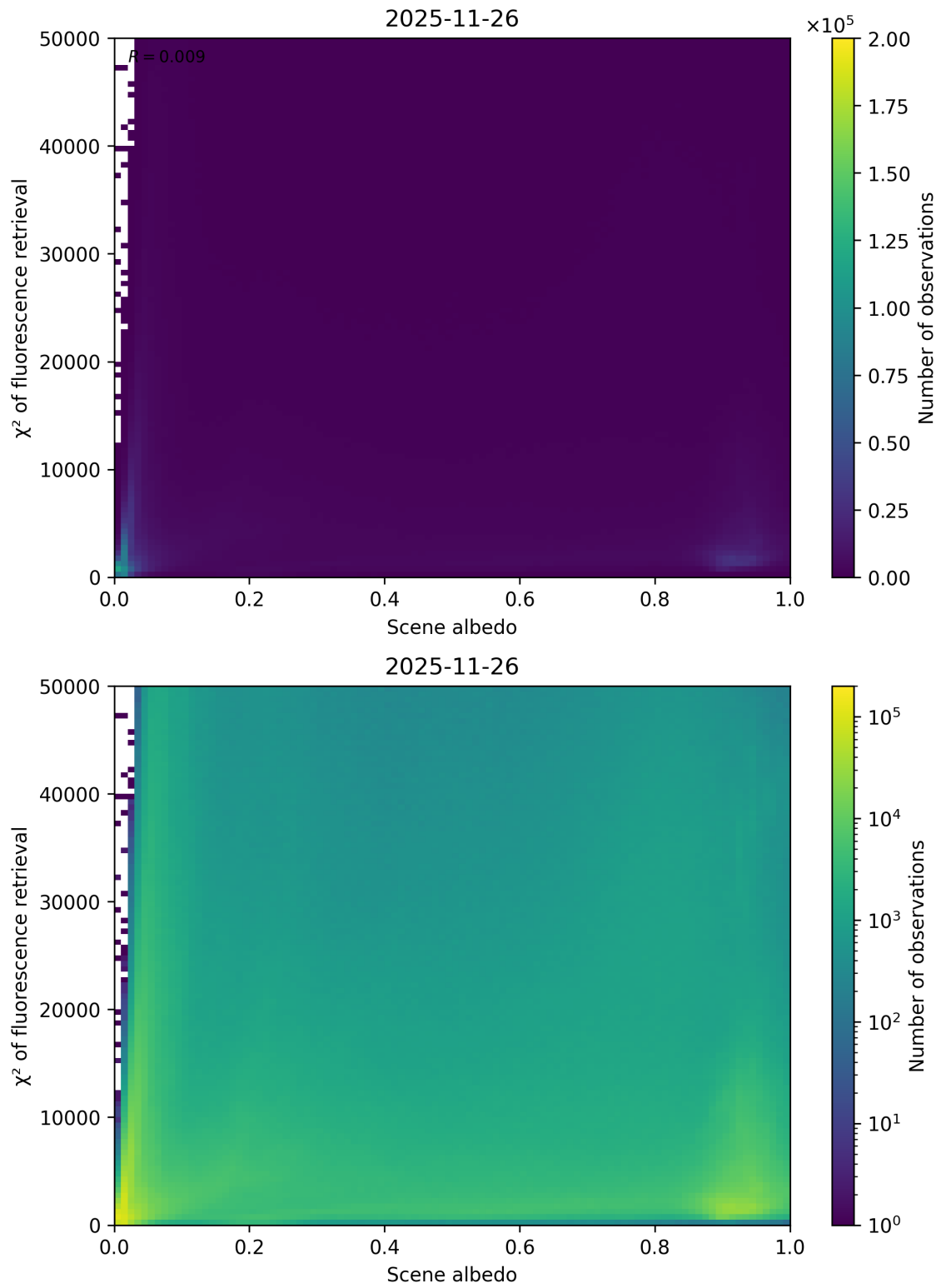
Figure 103: Scatter density plot of “Scene albedo” against “ \chi^2 of fluorescence retrieval” for 2025-11-25 to 2025-11-27.
