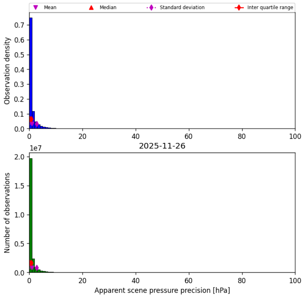
Figure 37: Histogram of “Apparent scene pressure precision” for 2025-11-25 to 2025-11-27
