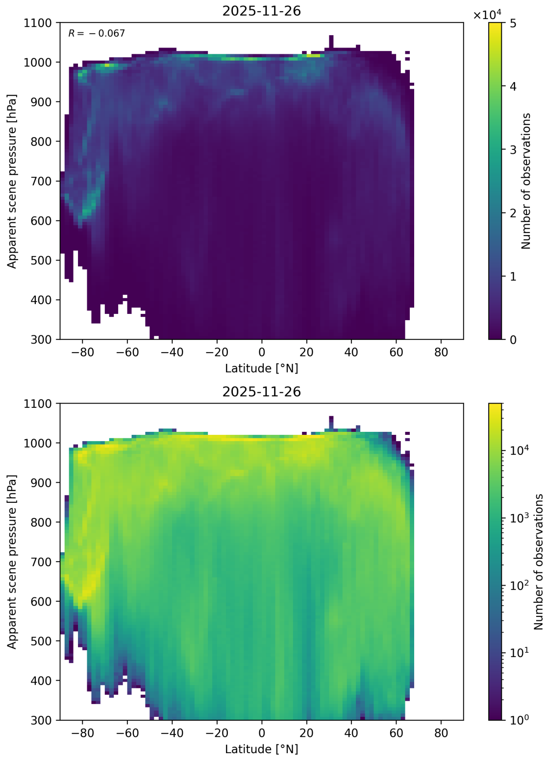
Figure 88: Scatter density plot of “Latitude” against “Apparent scene pressure” for 2025-11-25 to 2025-11-27.
