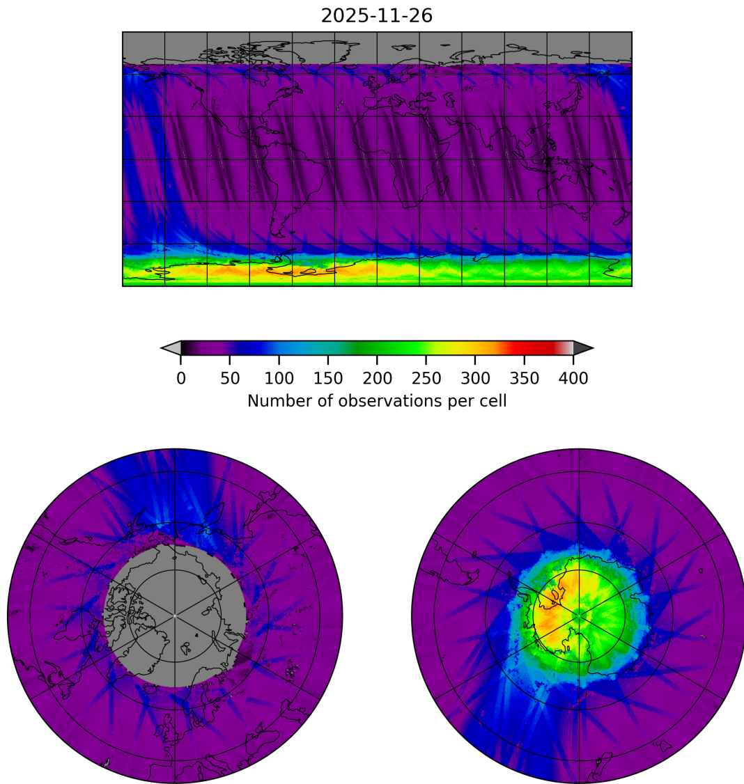
Figure 11: Map of the number of observations for 2025-11-25 to 2025-11-27
