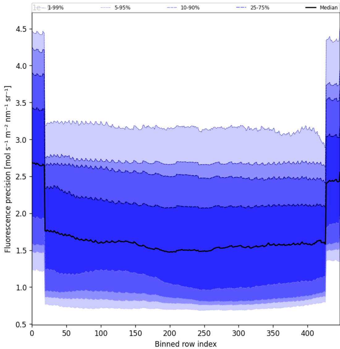
Figure 58: Along track statistics of “Fluorescence precision” for 2025-11-25 to 2025-11-27
