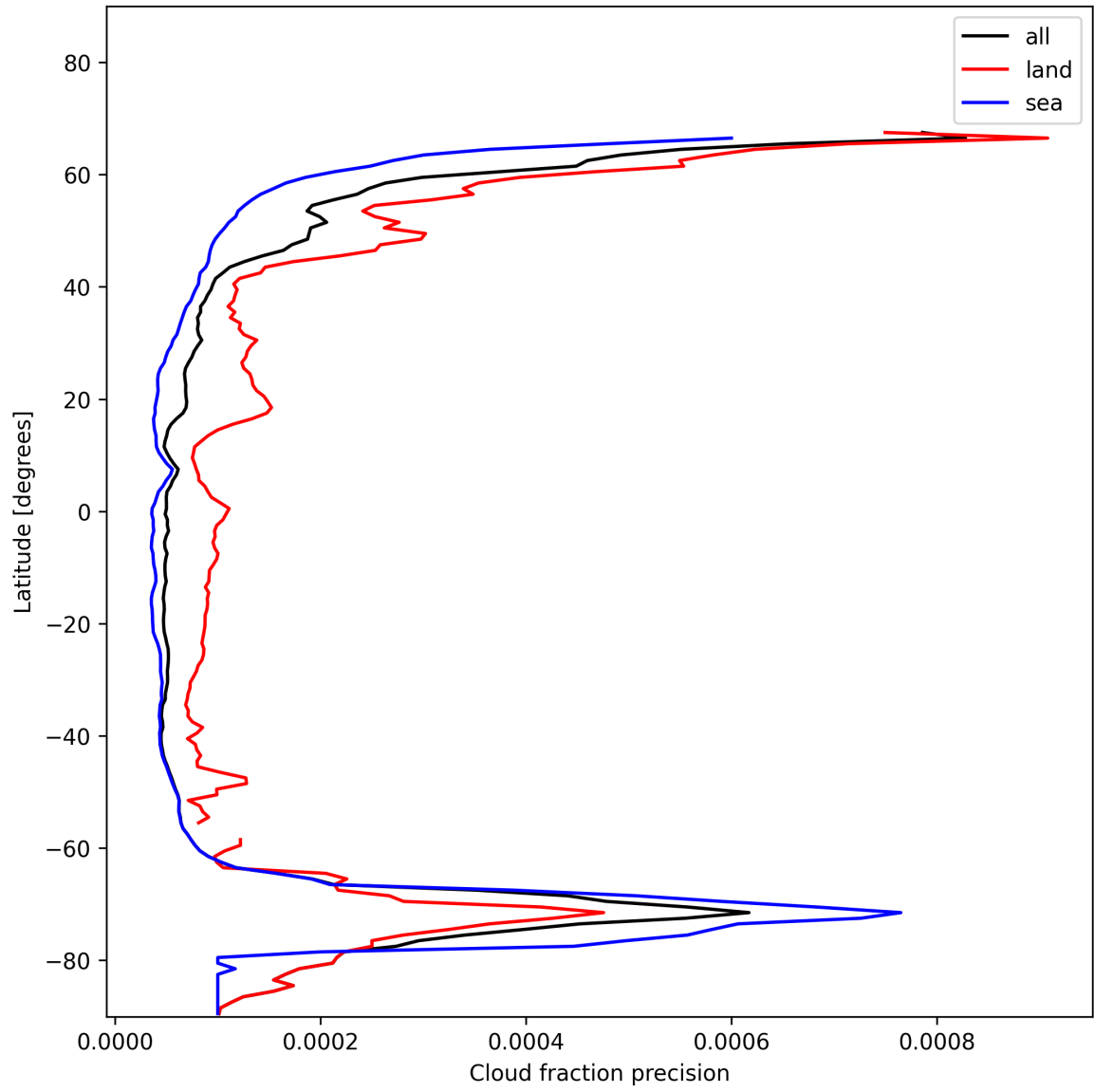
Figure 16: Zonal average of “Cloud fraction precision” for 2025-11-25 to 2025-11-27.
