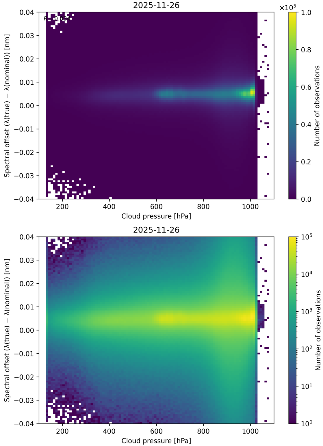
Figure 84: Scatter density plot of “Cloud pressure” against “Spectral offset ( \lambda_{\text{true}} - \lambda_{\text{nominal}} )” for 2025-11-25 to 2025-11-27.
