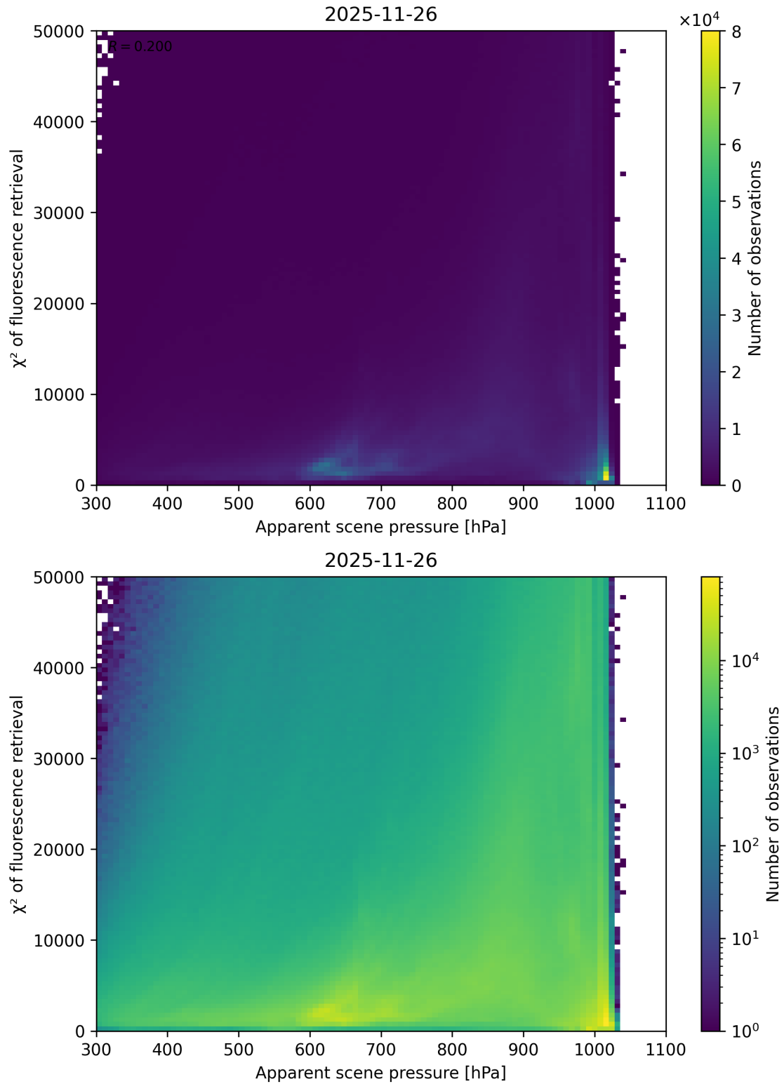
Figure 63: Scatter density plot of “Apparent scene pressure” against “ \chi^2 of fluorescence retrieval” for 2025-11-25 to 2025-11-27.
