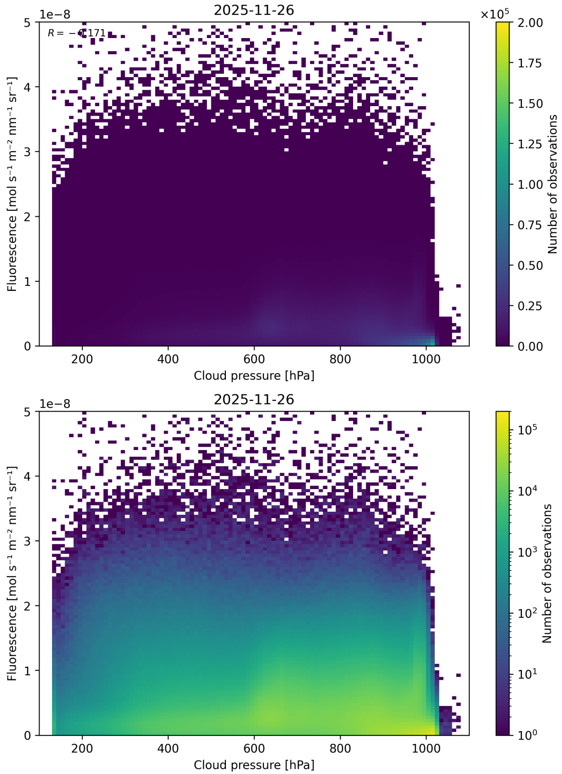
Figure 80: Scatter density plot of “Cloud pressure” against “Fluorescence” for 2025-11-25 to 2025-11-27.
