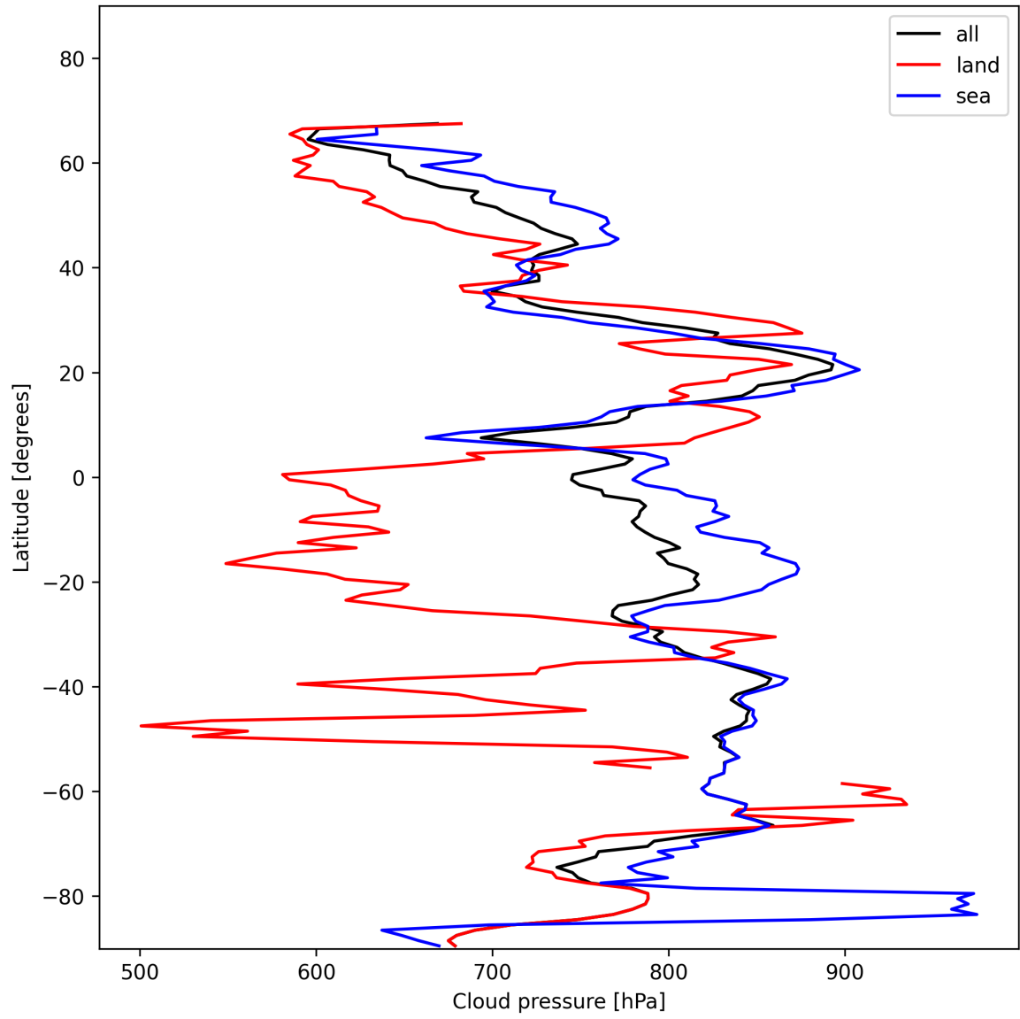
Figure 13: Zonal average of “Cloud pressure” for 2025-11-25 to 2025-11-27.
