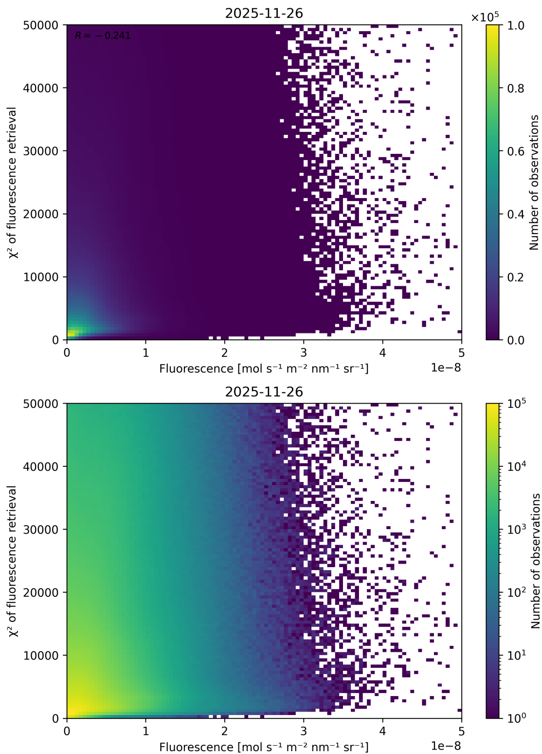
Figure 85: Scatter density plot of “Fluorescence” against “ \chi^2 of fluorescence retrieval” for 2025-11-25 to 2025-11-27.
