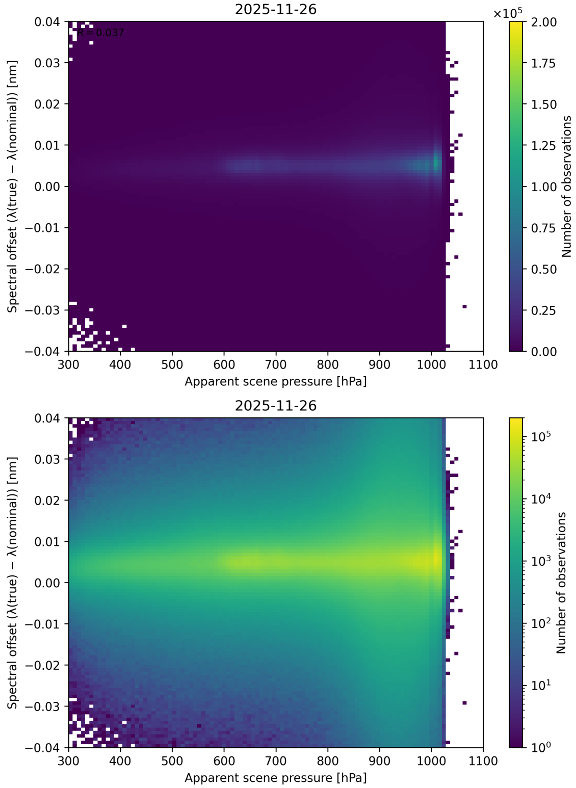
Figure 67: Scatter density plot of “Apparent scene pressure” against “Spectral offset ( \lambda_{\text{true}} - \lambda_{\text{nominal}} )” for 2025-11-25 to 2025-11-27.
