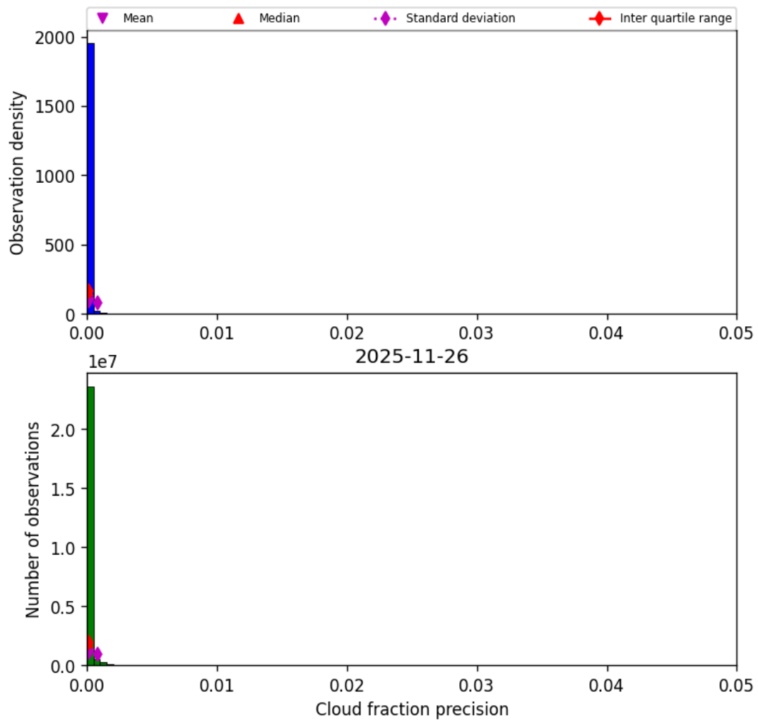
Figure 33: Histogram of “Cloud fraction precision” for 2025-11-25 to 2025-11-27
