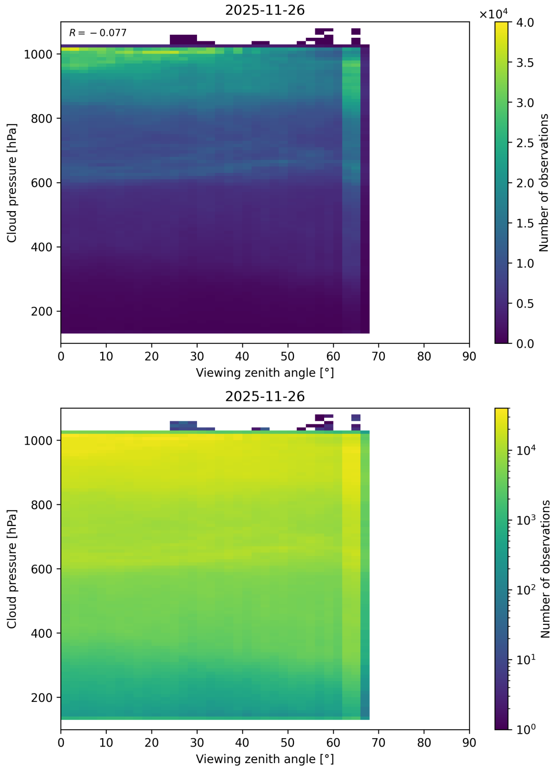
Figure 121: Scatter density plot of “Viewing zenith angle” against “Cloud pressure” for 2025-11-25 to 2025-11-27.
