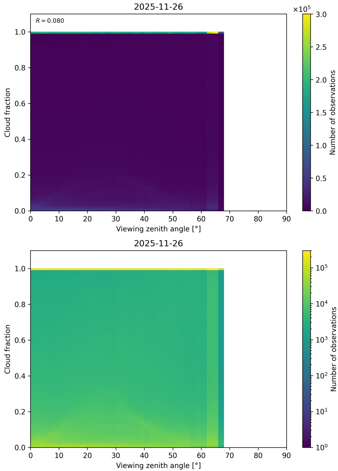
Figure 120: Scatter density plot of “Viewing zenith angle” against “Cloud fraction” for 2025-11-25 to 2025-11-27.
