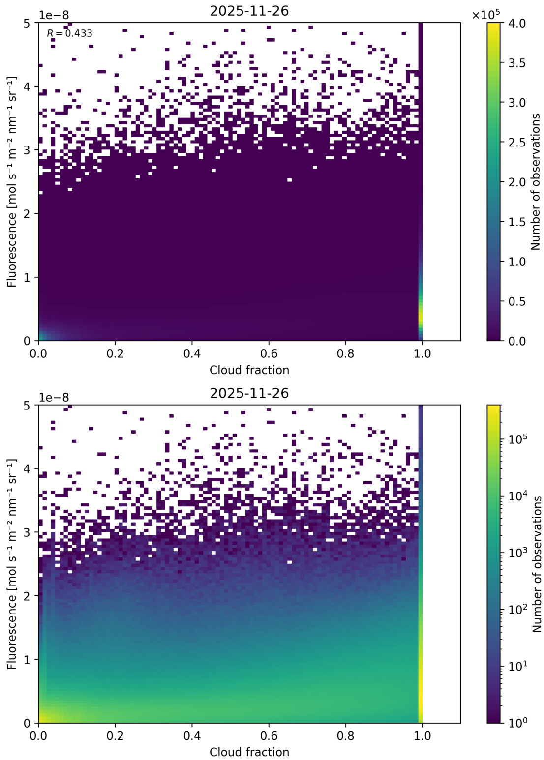
Figure 72: Scatter density plot of “Cloud fraction” against “Fluorescence” for 2025-11-25 to 2025-11-27.
