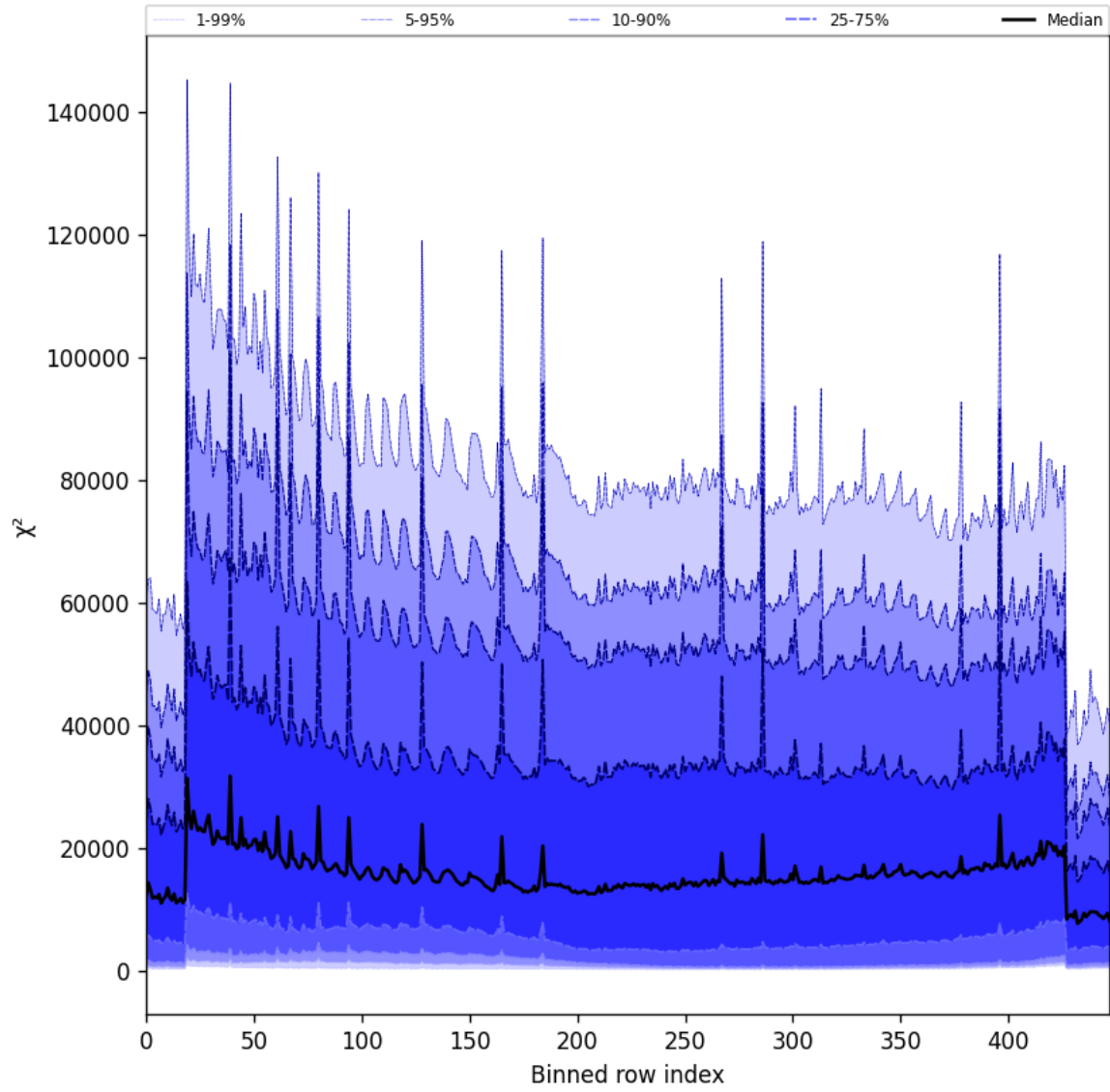
Figure 55: Along track statistics of “ \chi^2 ” for 2025-11-25 to 2025-11-27
