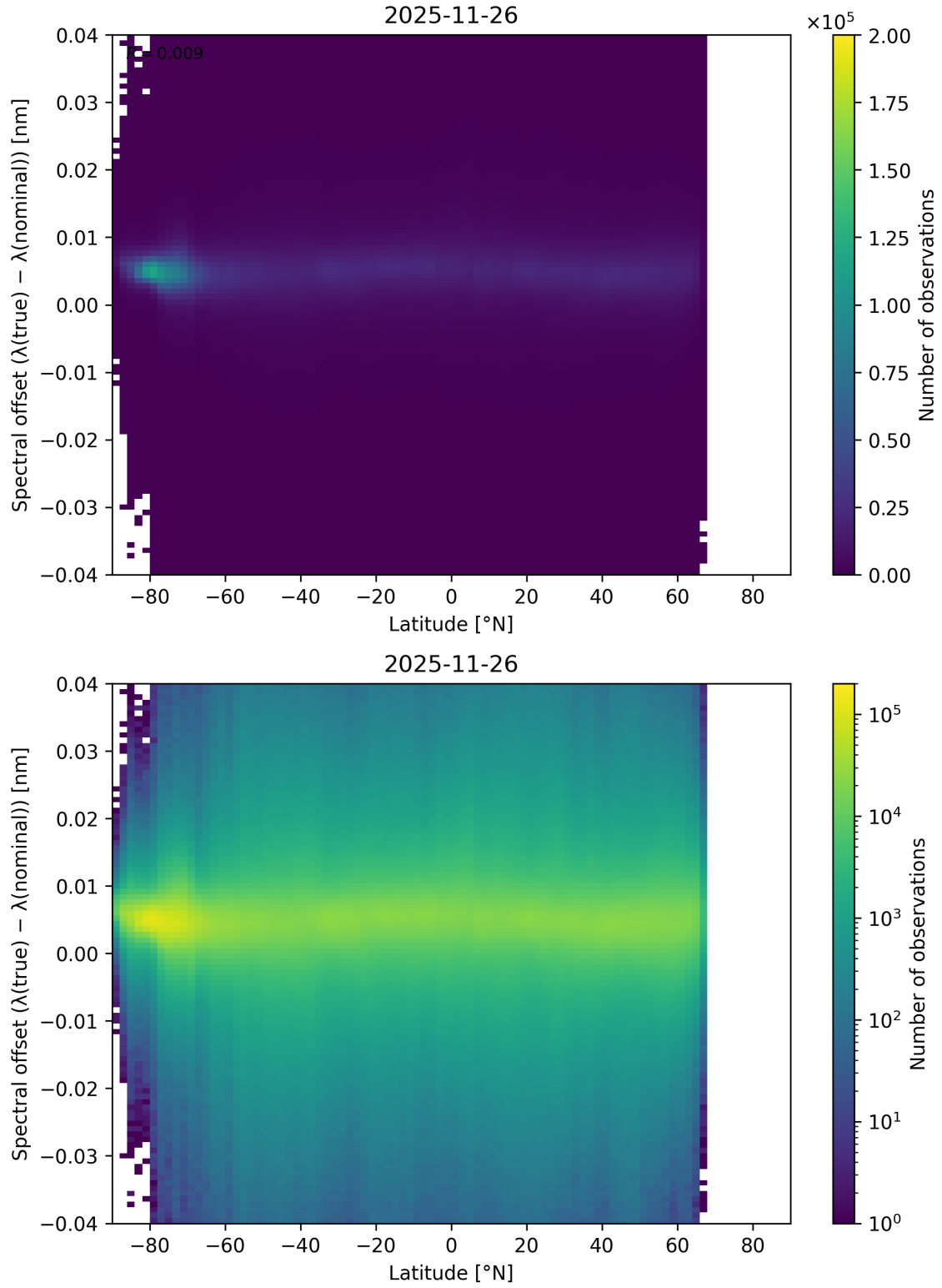
Figure 96: Scatter density plot of “Latitude” against “Spectral offset ( \lambda_{\text{true}} - \lambda_{\text{nominal}} )” for 2025-11-25 to 2025-11-27.
