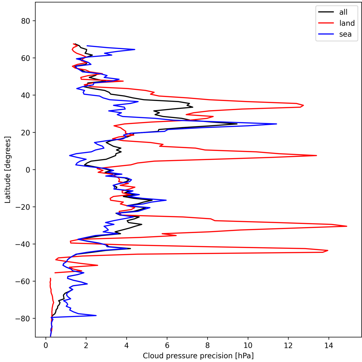
Figure 14: Zonal average of “Cloud pressure precision” for 2025-11-25 to 2025-11-27.
