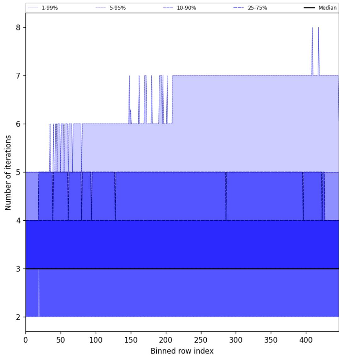
Figure 56: Along track statistics of “Number of iterations” for 2025-11-25 to 2025-11-27
