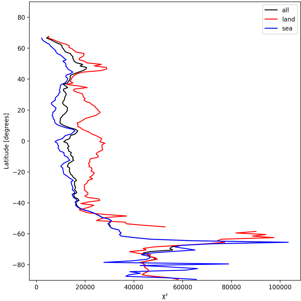
Figure 21: Zonal average of “ \chi^2 ” for 2025-11-25 to 2025-11-27.
