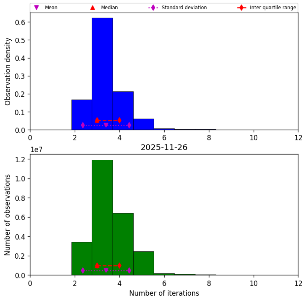
Figure 39: Histogram of “Number of iterations” for 2025-11-25 to 2025-11-27
