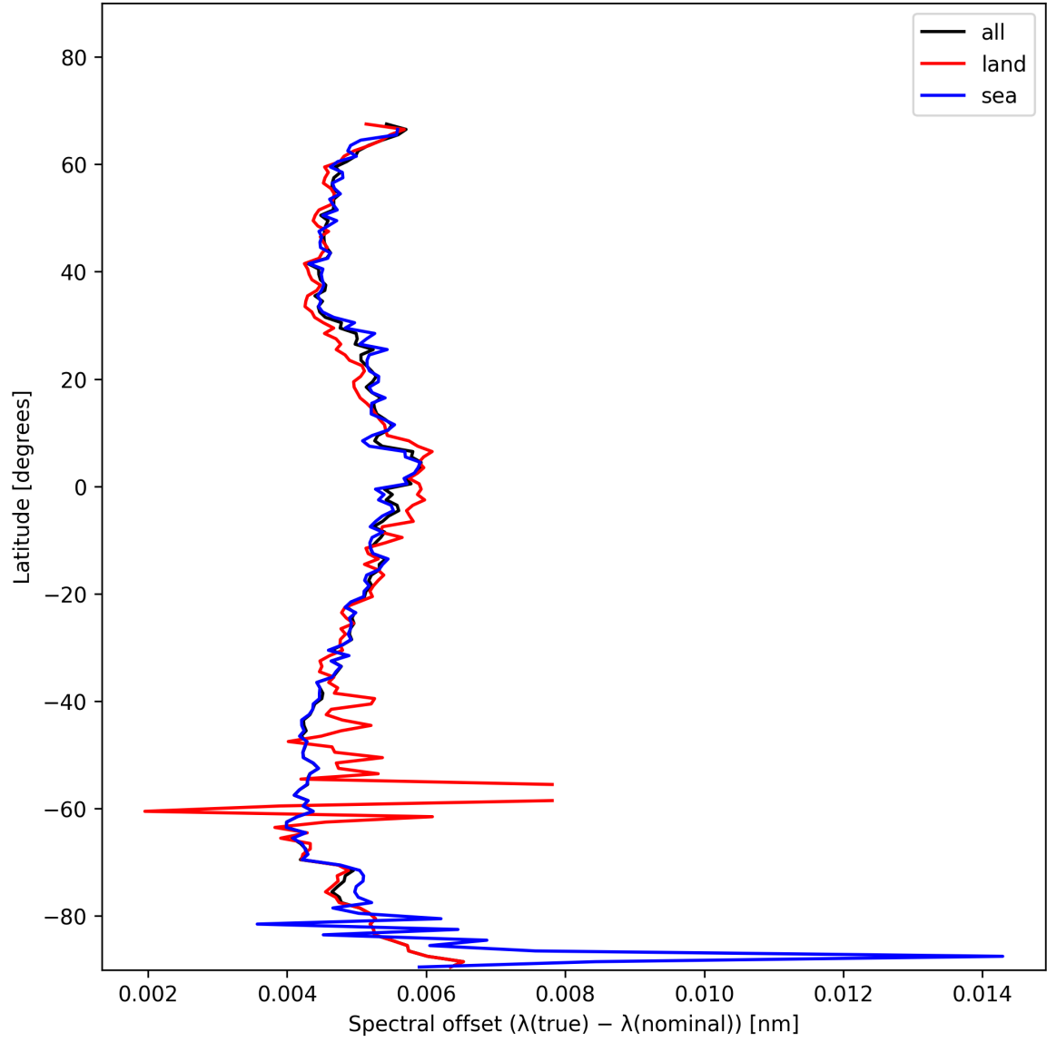
Figure 28: Zonal average of “Spectral offset ( \lambda_{\text{true}} - \lambda_{\text{nominal}} )” for 2025-11-25 to 2025-11-27.
