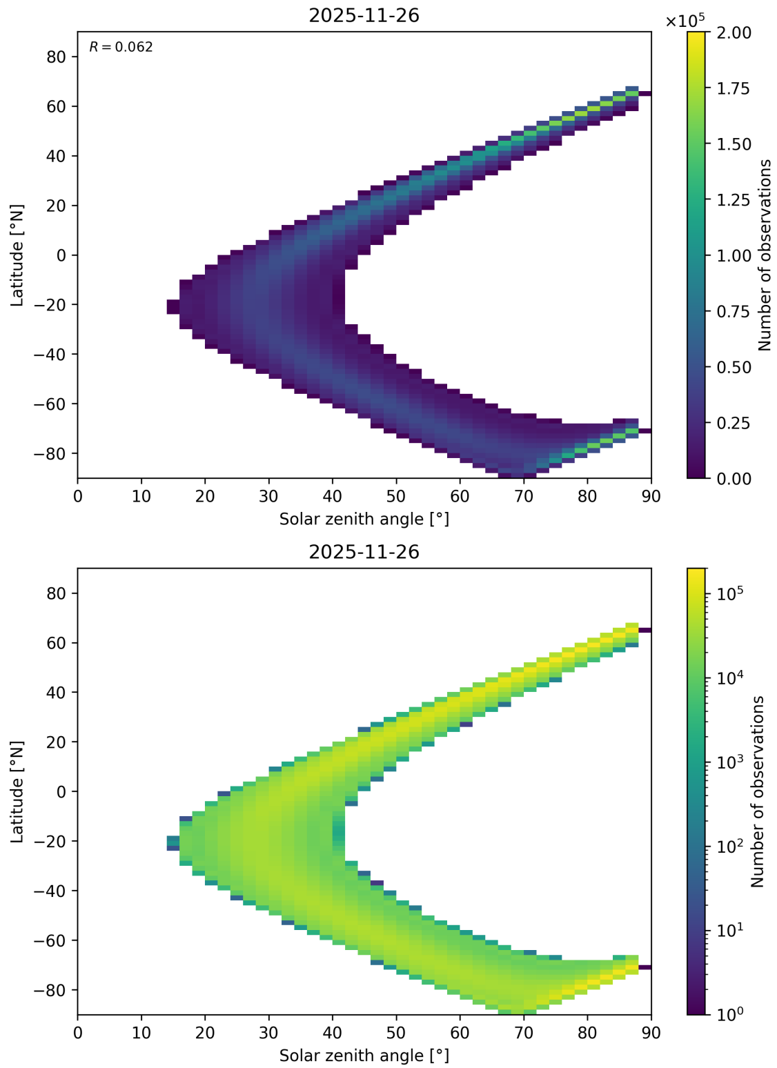
Figure 113: Scatter density plot of “Solar zenith angle” against “Latitude” for 2025-11-25 to 2025-11-27.
