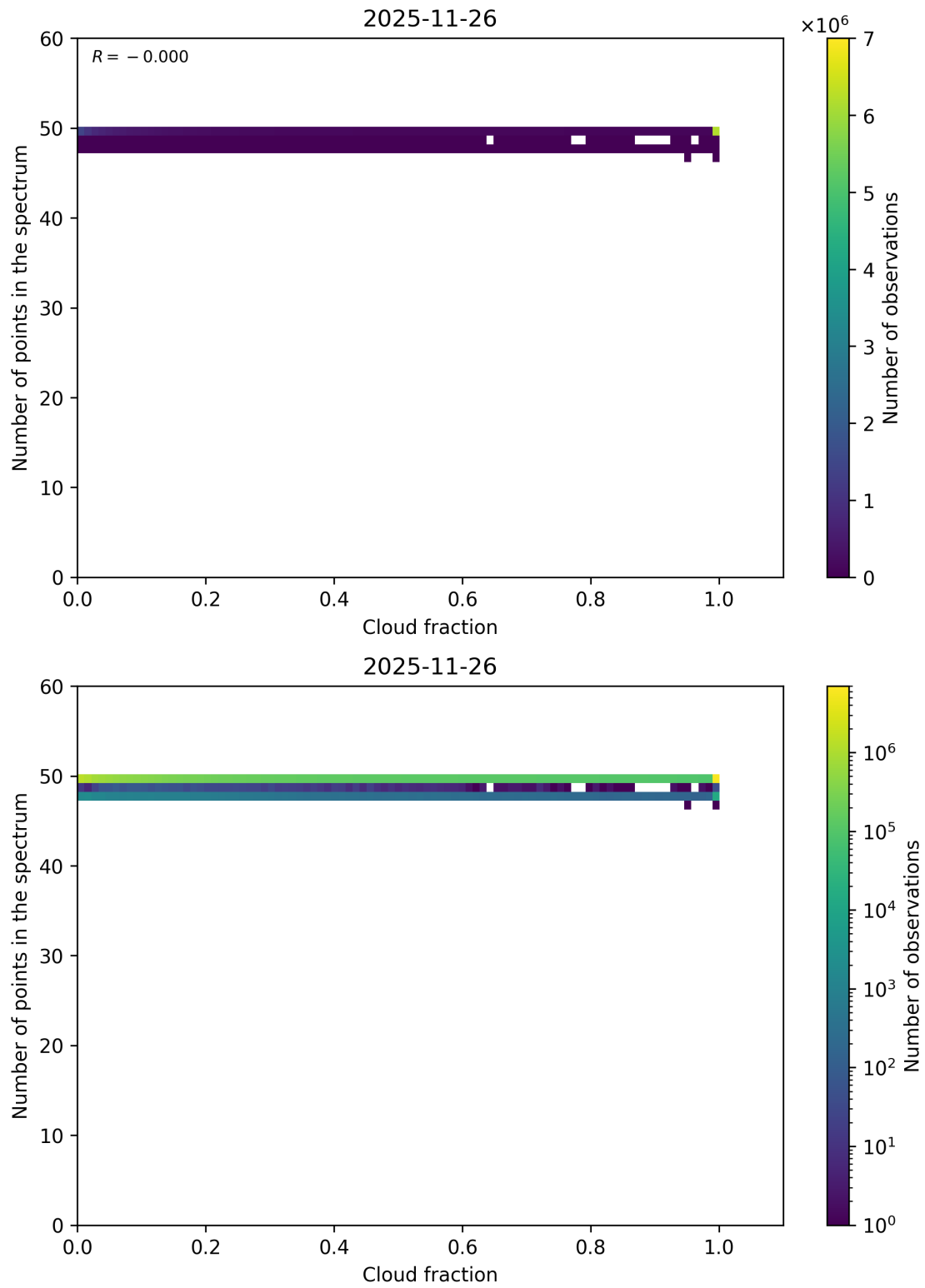
Figure 74: Scatter density plot of “Cloud fraction” against “Number of points in the spectrum” for 2025-11-25 to 2025-11-27.
