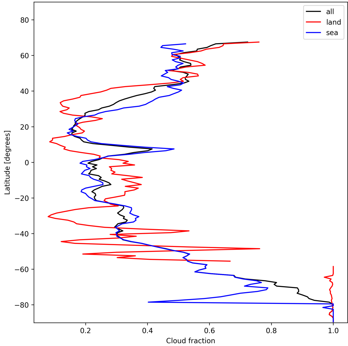
Figure 15: Zonal average of “Cloud fraction” for 2025-11-25 to 2025-11-27.
