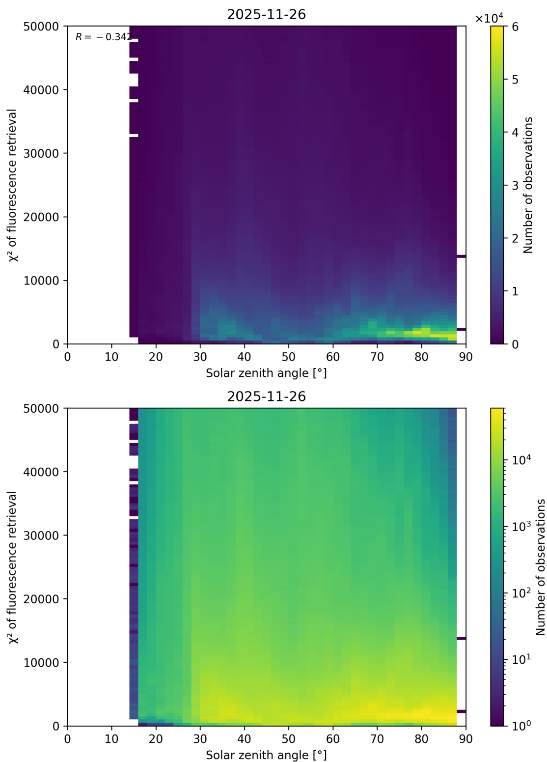
Figure 109: Scatter density plot of “Solar zenith angle” against “ \chi^2 of fluorescence retrieval” for 2025-11-25 to 2025-11-27.
