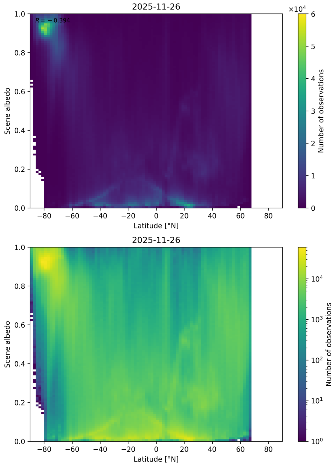
Figure 95: Scatter density plot of “Latitude” against “Scene albedo” for 2025-11-25 to 2025-11-27.
