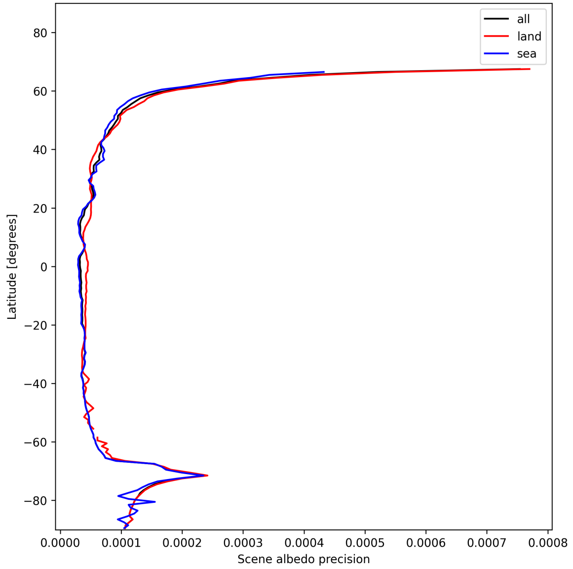
Figure 18: Zonal average of “Scene albedo precision” for 2025-11-25 to 2025-11-27.
