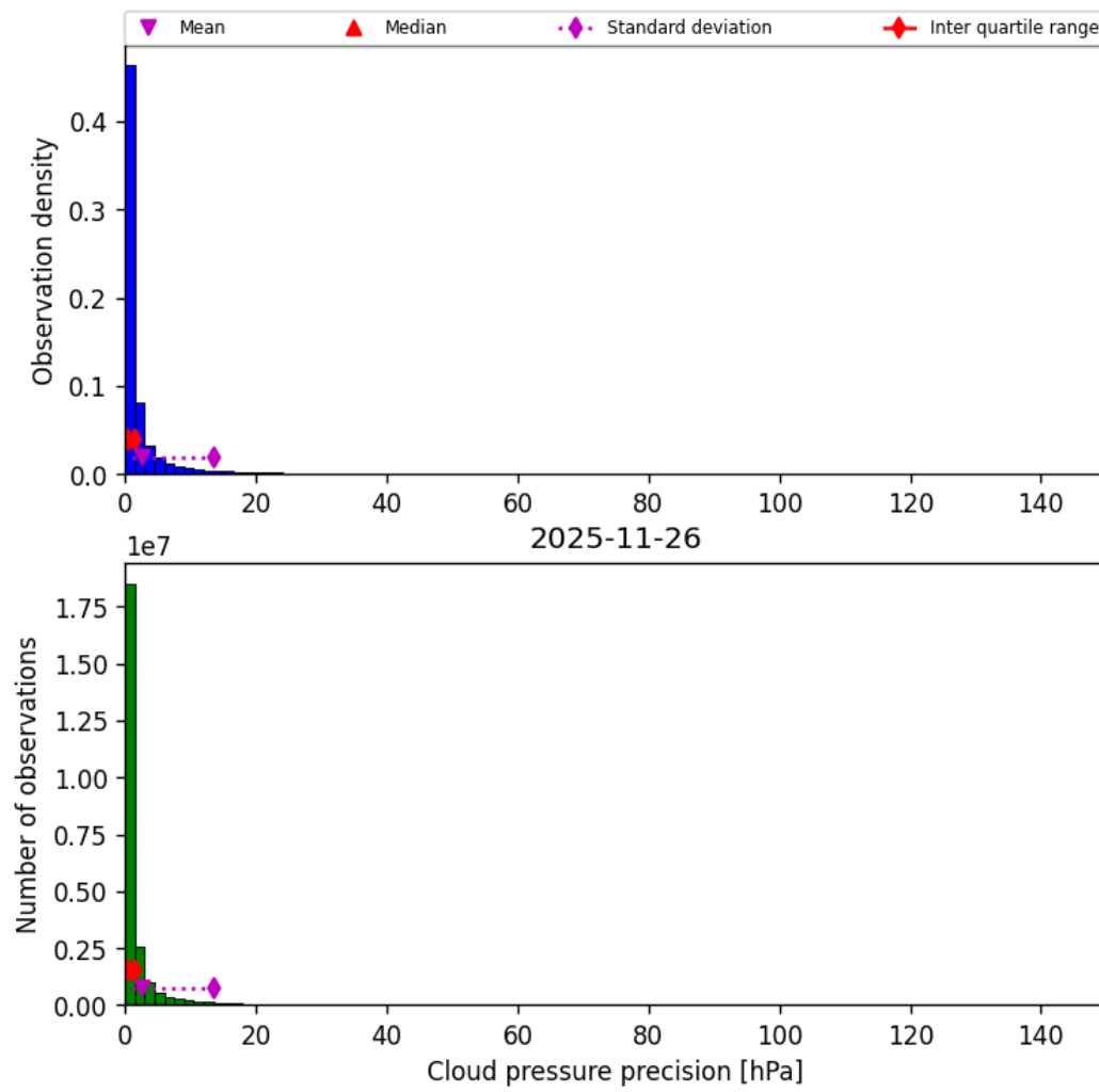
Figure 31: Histogram of “Cloud pressure precision” for 2025-11-25 to 2025-11-27
