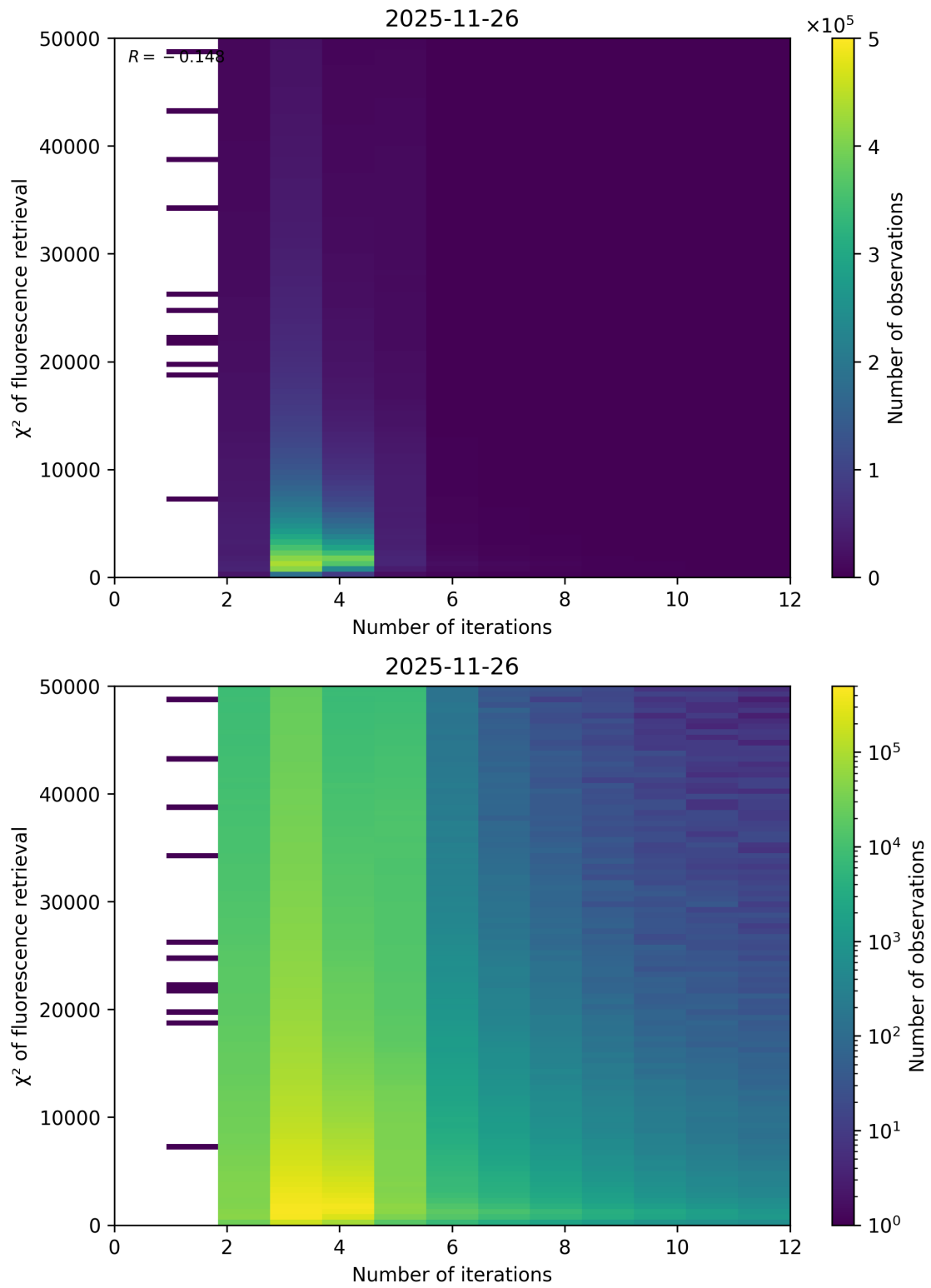
Figure 97: Scatter density plot of “Number of iterations” against “ \chi^2 of fluorescence retrieval” for 2025-11-25 to 2025-11-27.
