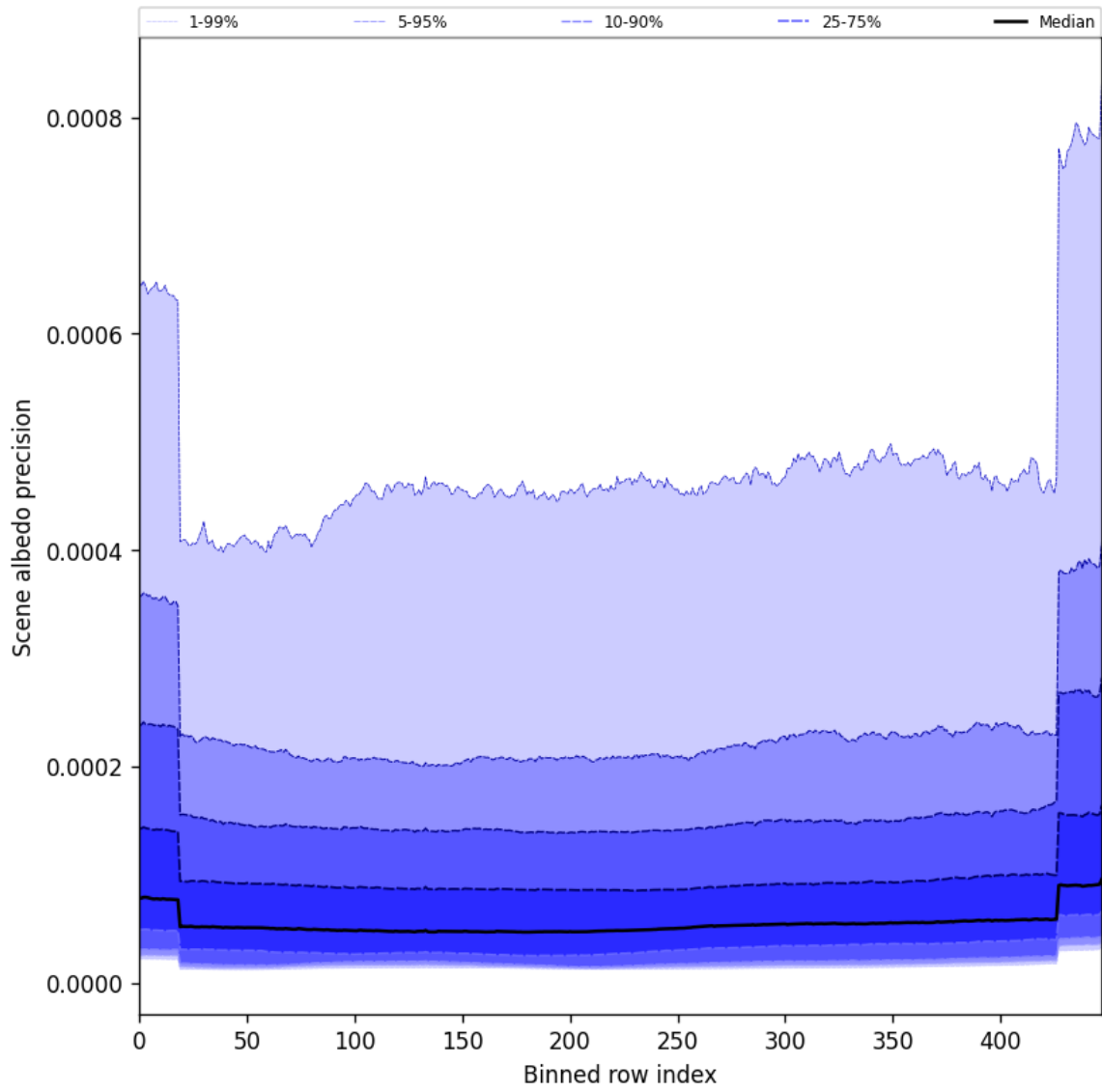
Figure 52: Along track statistics of “Scene albedo precision” for 2025-11-25 to 2025-11-27
