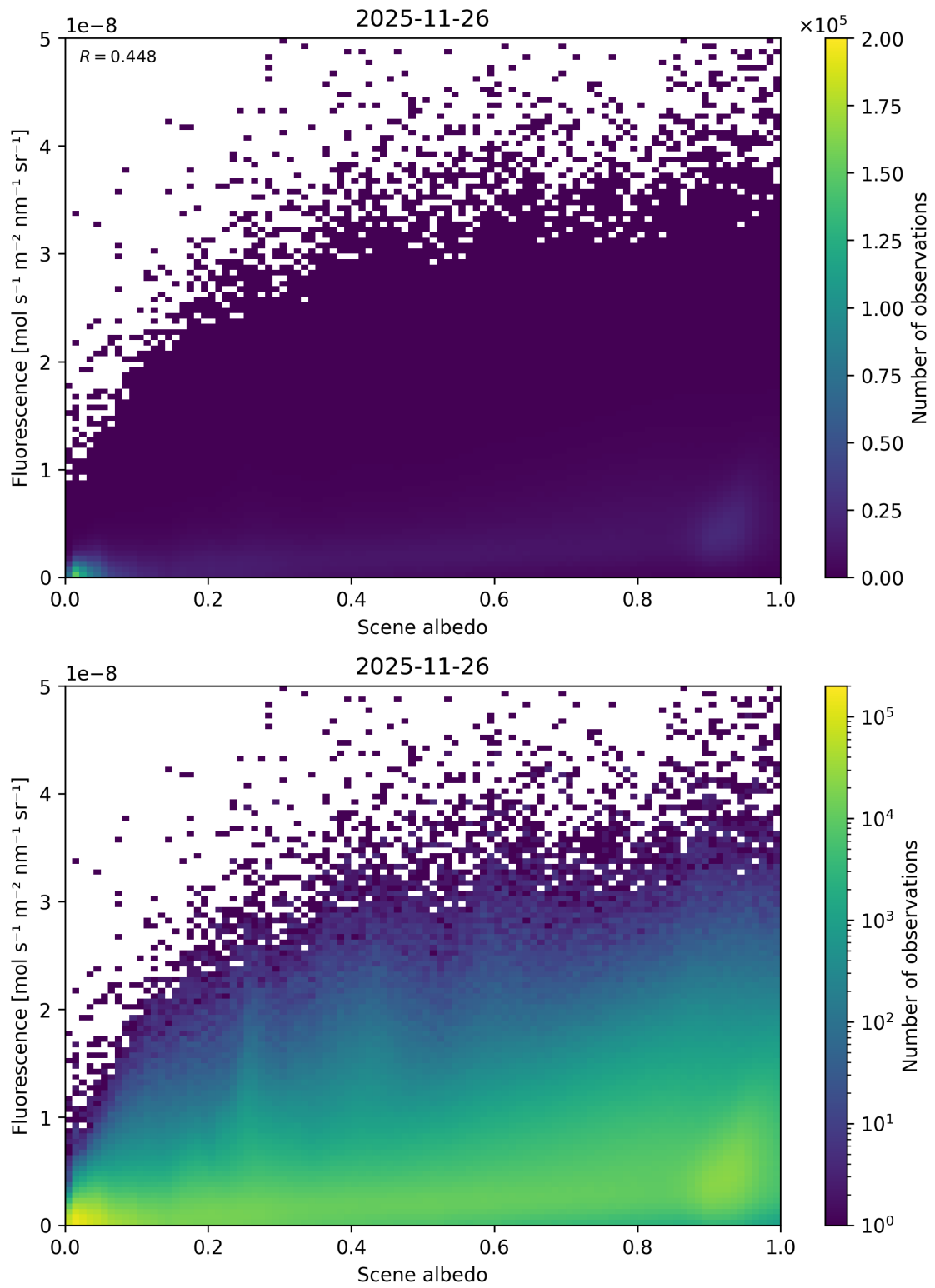
Figure 104: Scatter density plot of “Scene albedo” against “Fluorescence” for 2025-11-25 to 2025-11-27.
