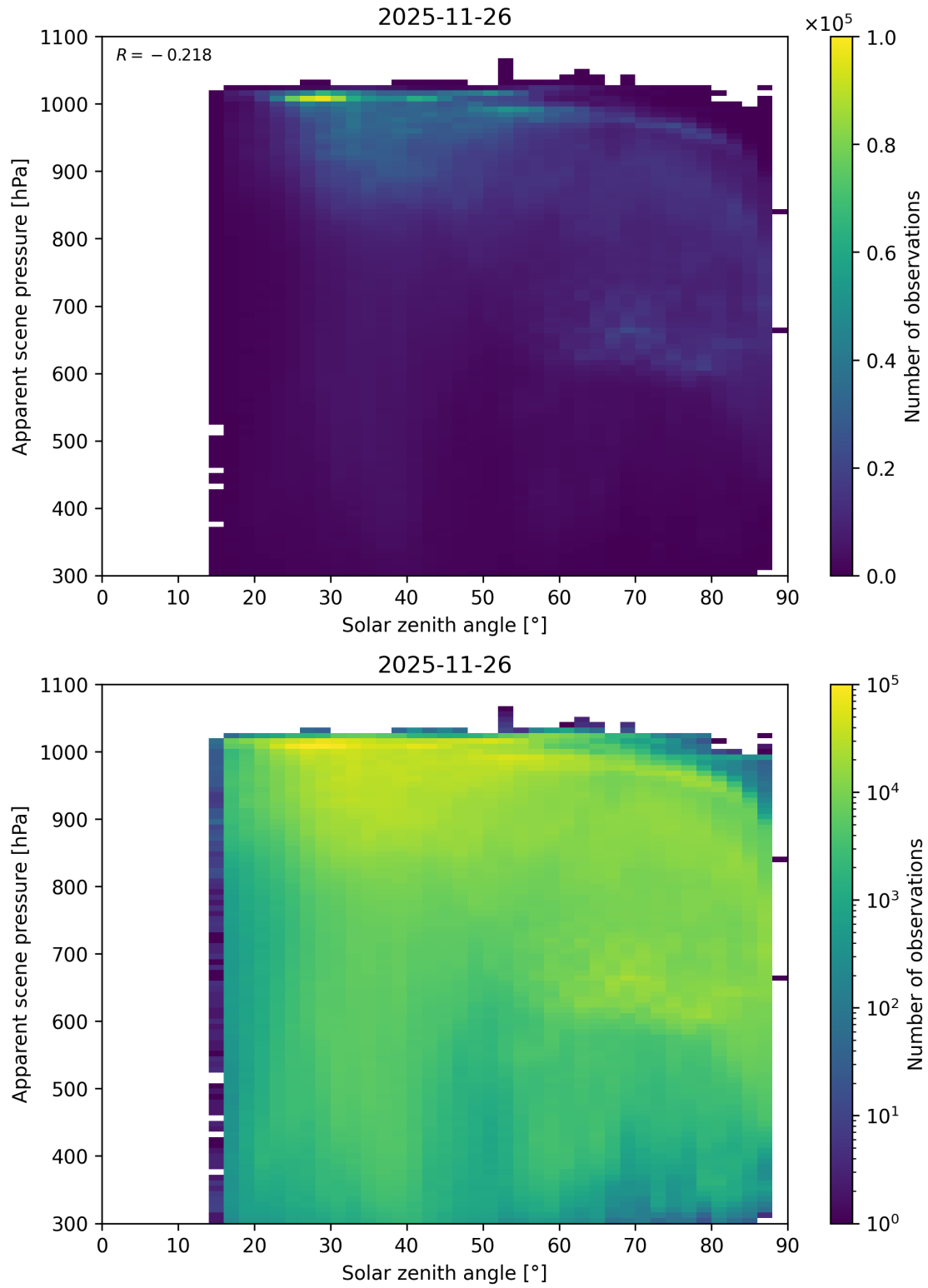
Figure 108: Scatter density plot of “Solar zenith angle” against “Apparent scene pressure” for 2025-11-25 to 2025-11-27.
