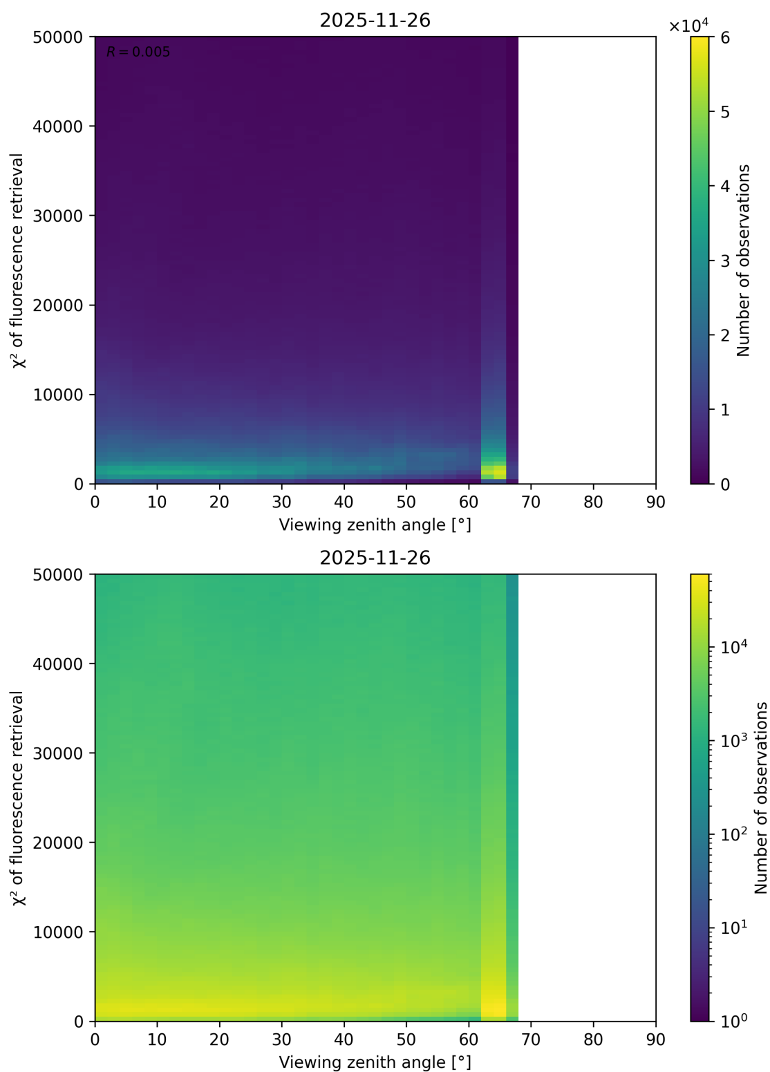
Figure 119: Scatter density plot of “Viewing zenith angle” against “ \chi^2 of fluorescence retrieval” for 2025-11-25 to 2025-11-27.
