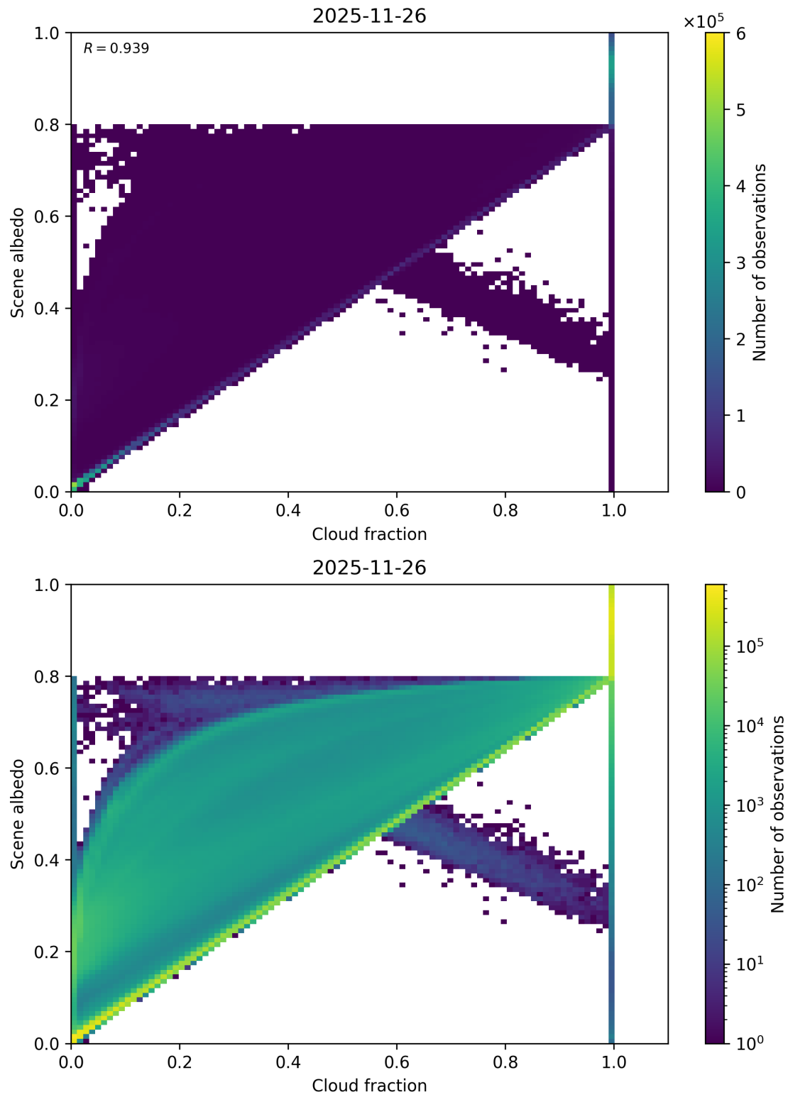
Figure 75: Scatter density plot of “Cloud fraction” against “Scene albedo” for 2025-11-25 to 2025-11-27.
