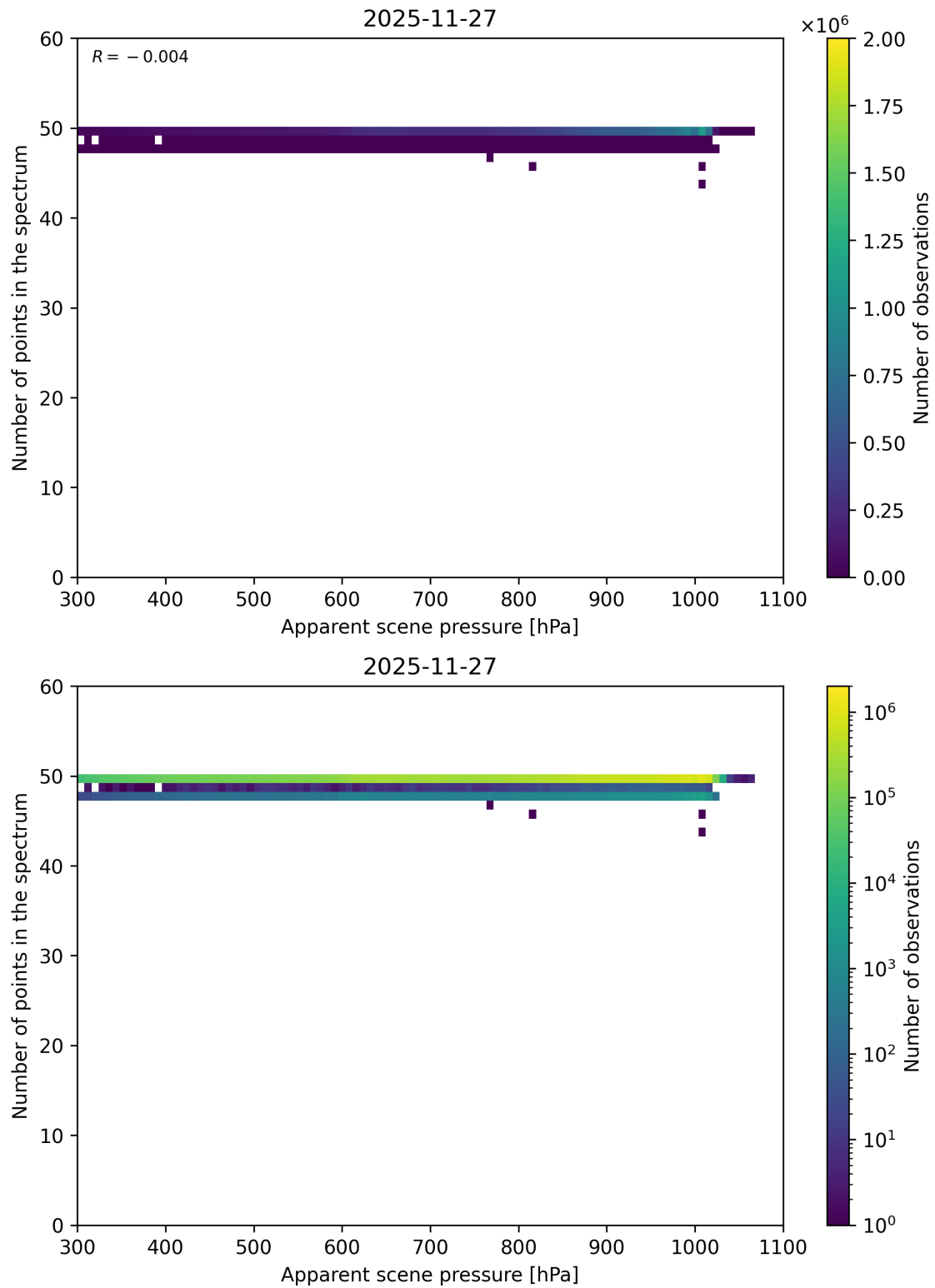
Figure 66: Scatter density plot of “Apparent scene pressure” against “Number of points in the spectrum” for 2025-11-26 to 2025-11-28.
