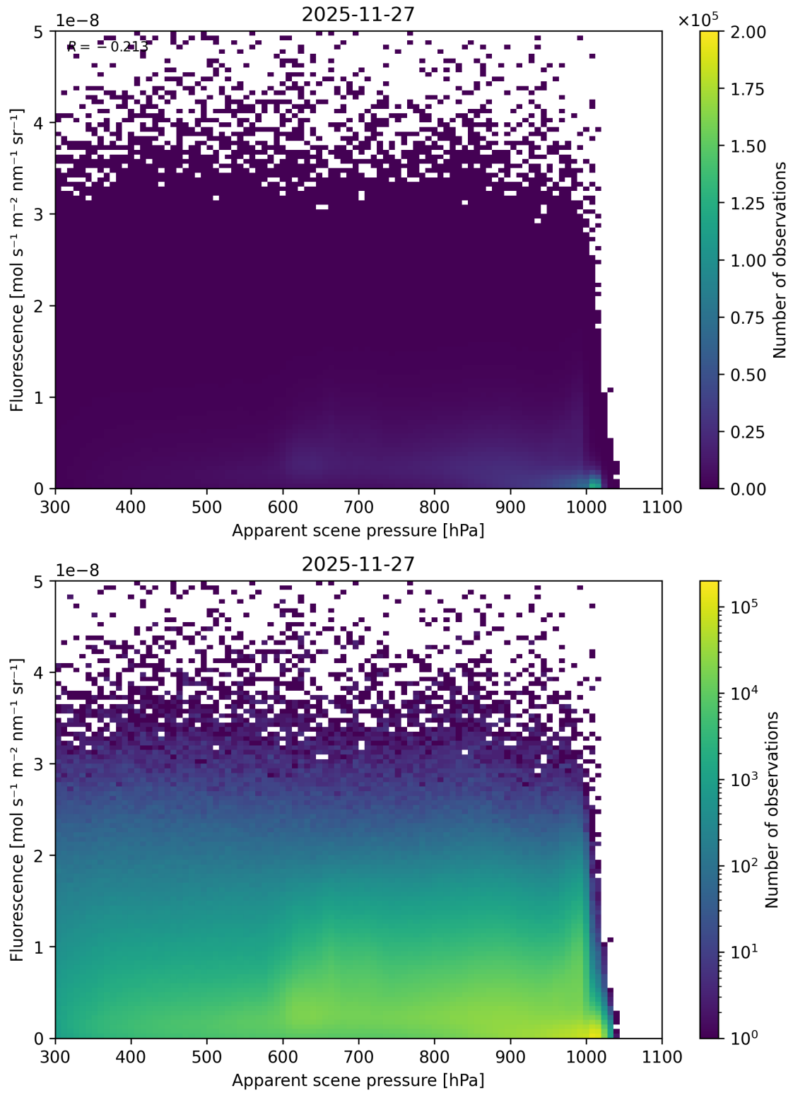
Figure 64: Scatter density plot of “Apparent scene pressure” against “Fluorescence” for 2025-11-26 to 2025-11-28.
