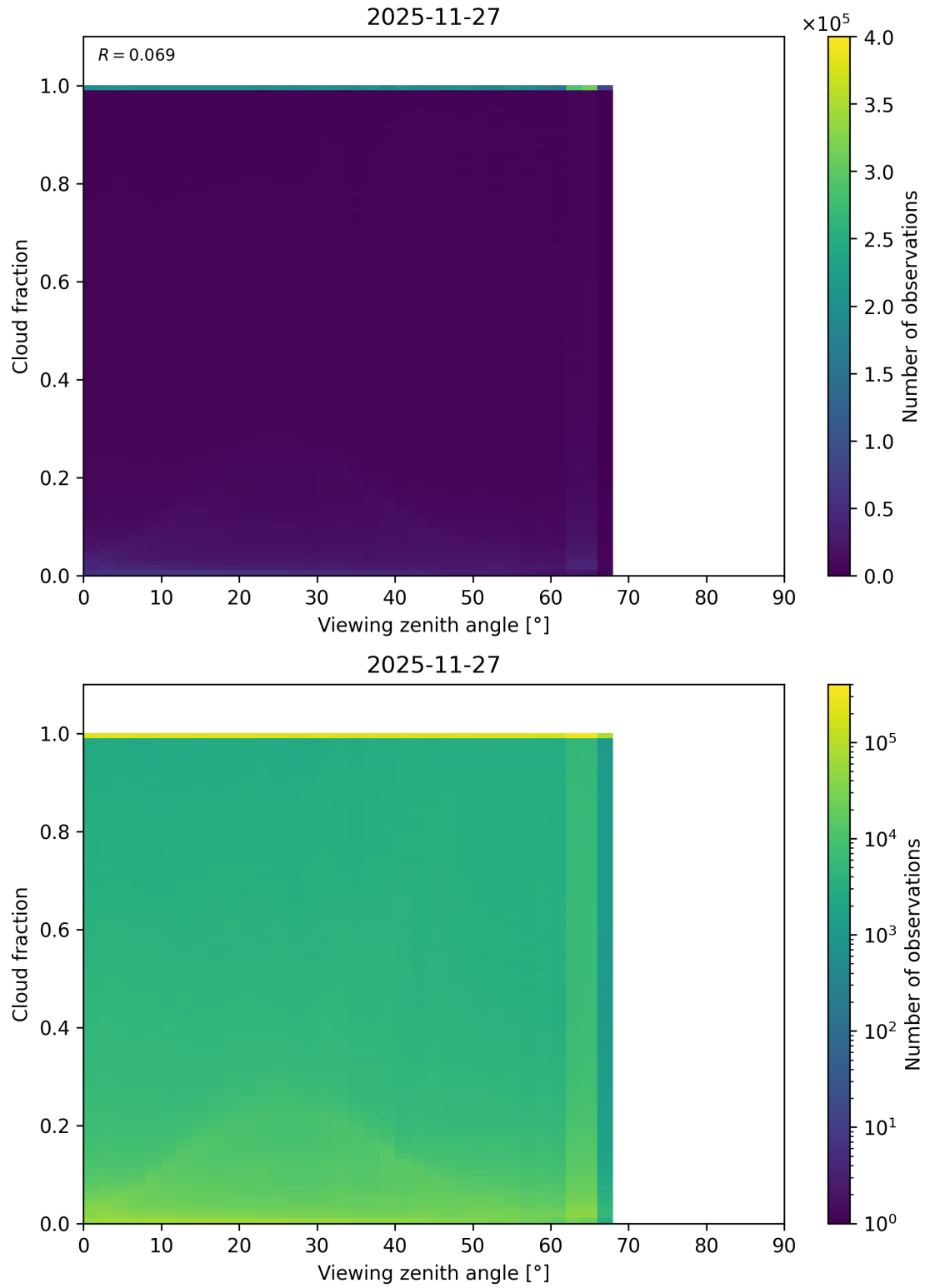
Figure 120: Scatter density plot of “Viewing zenith angle” against “Cloud fraction” for 2025-11-26 to 2025-11-28.
