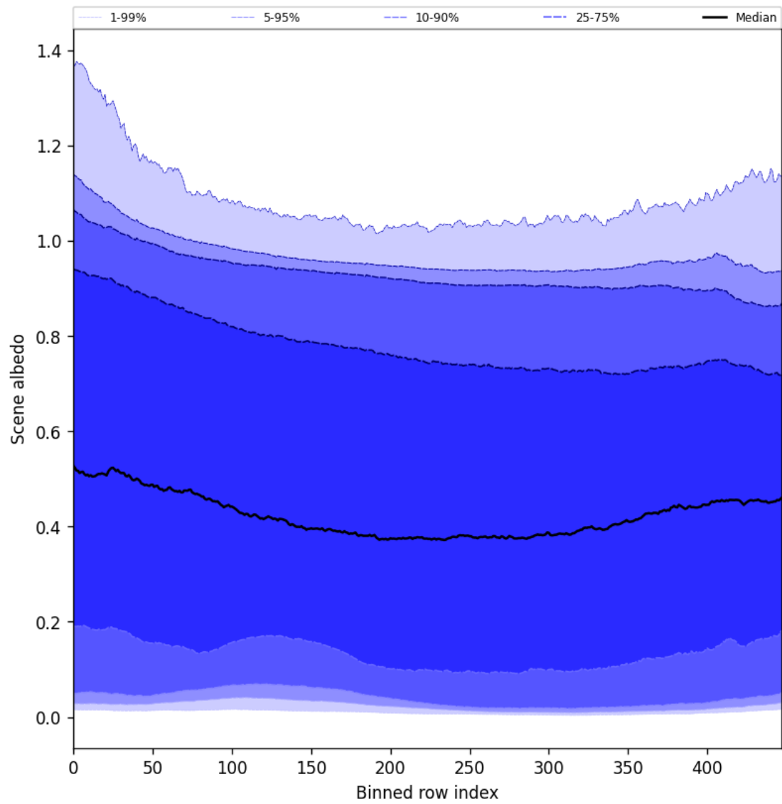
Figure 51: Along track statistics of “Scene albedo” for 2025-11-26 to 2025-11-28
