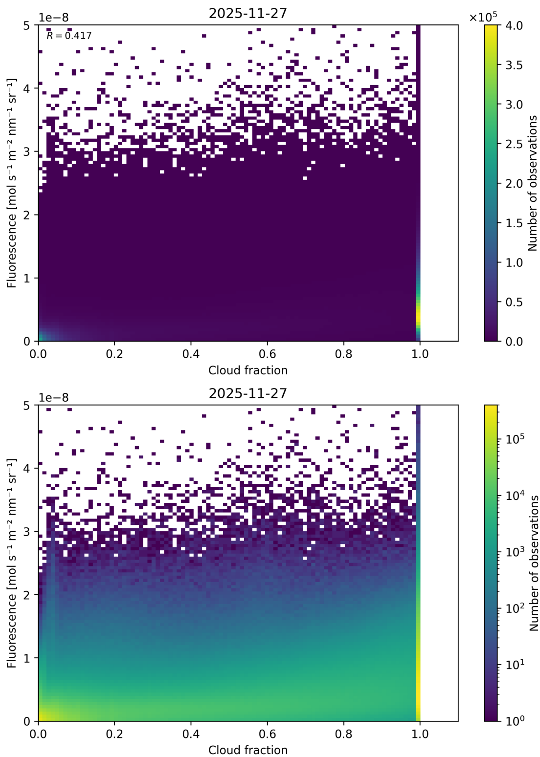
Figure 72: Scatter density plot of “Cloud fraction” against “Fluorescence” for 2025-11-26 to 2025-11-28.
