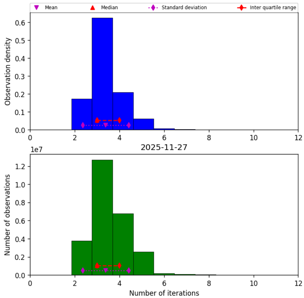
Figure 39: Histogram of “Number of iterations” for 2025-11-26 to 2025-11-28
