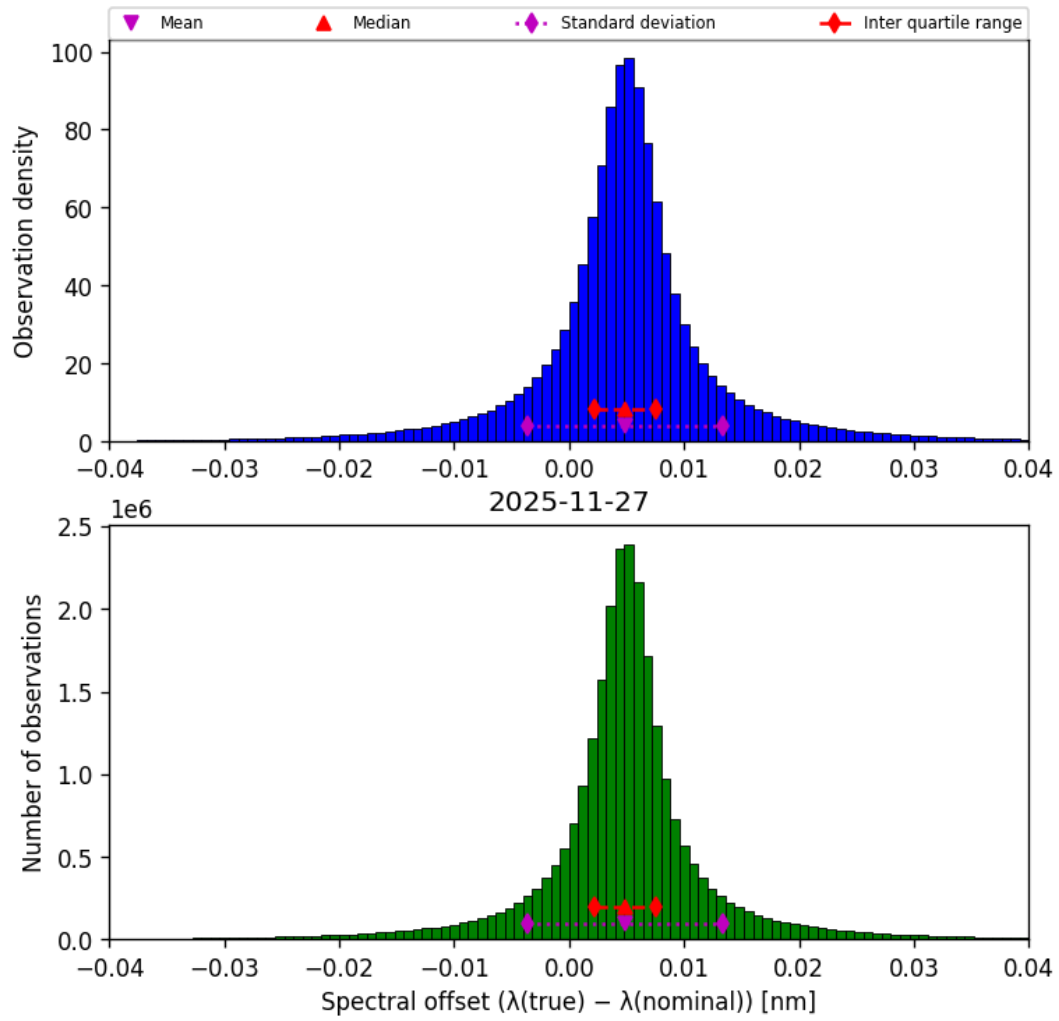
Figure 45: Histogram of “Spectral offset ( \lambda_{\text{true}} - \lambda_{\text{nominal}} )” for 2025-11-26 to 2025-11-28
