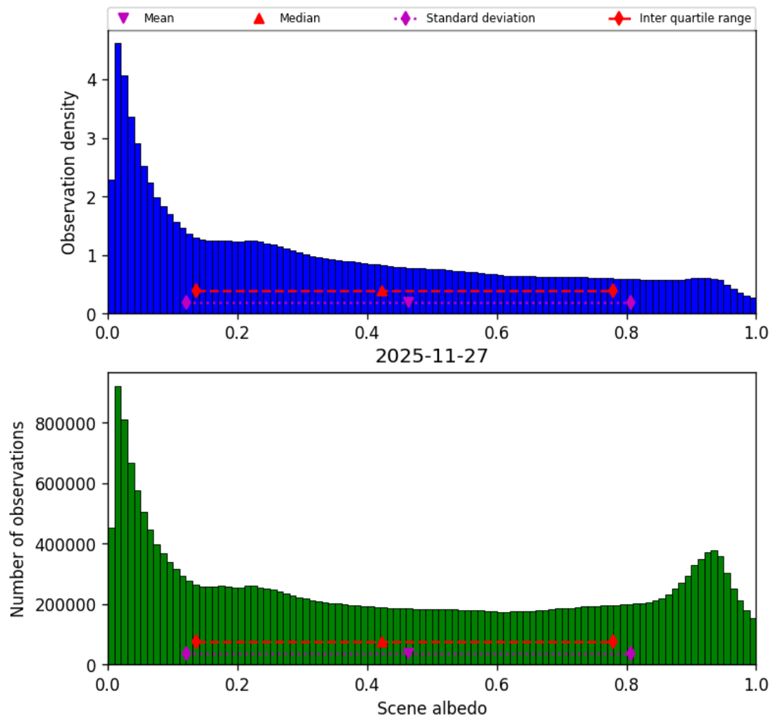
Figure 34: Histogram of “Scene albedo” for 2025-11-26 to 2025-11-28
