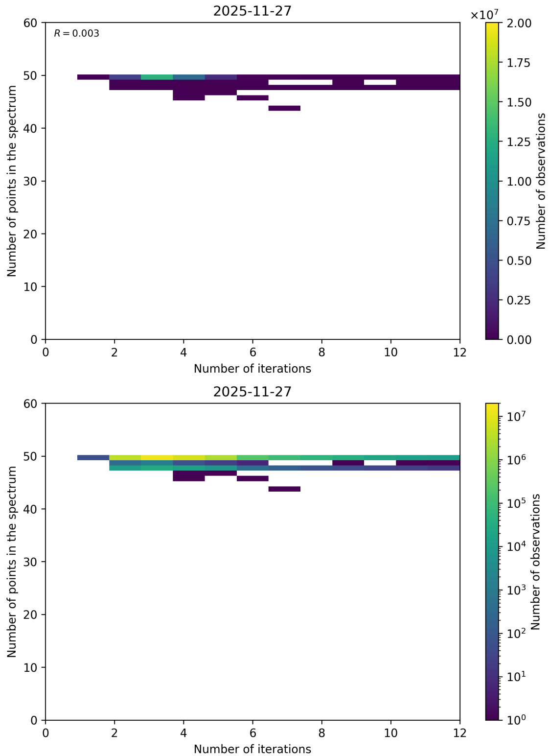
Figure 99: Scatter density plot of “Number of iterations” against “Number of points in the spectrum” for 2025-11-26 to 2025-11-28.
