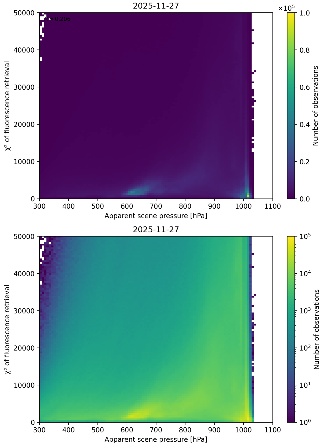
Figure 63: Scatter density plot of “Apparent scene pressure” against “ \chi^2 of fluorescence retrieval” for 2025-11-26 to 2025-11-28.
