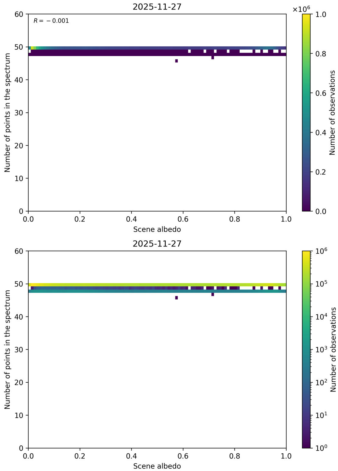
Figure 106: Scatter density plot of “Scene albedo” against “Number of points in the spectrum” for 2025-11-26 to 2025-11-28.
