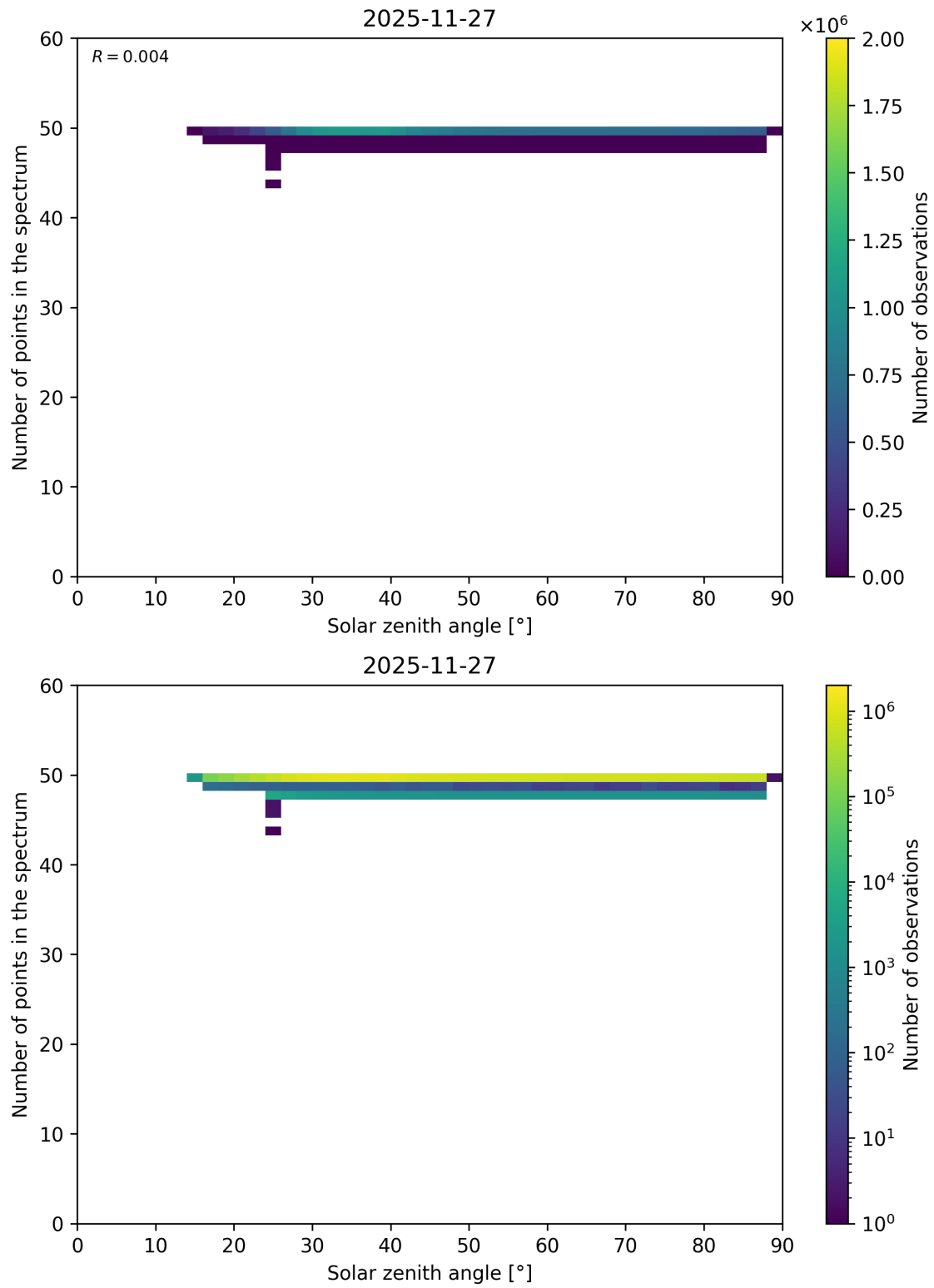
Figure 115: Scatter density plot of “Solar zenith angle” against “Number of points in the spectrum” for 2025-11-26 to 2025-11-28.
