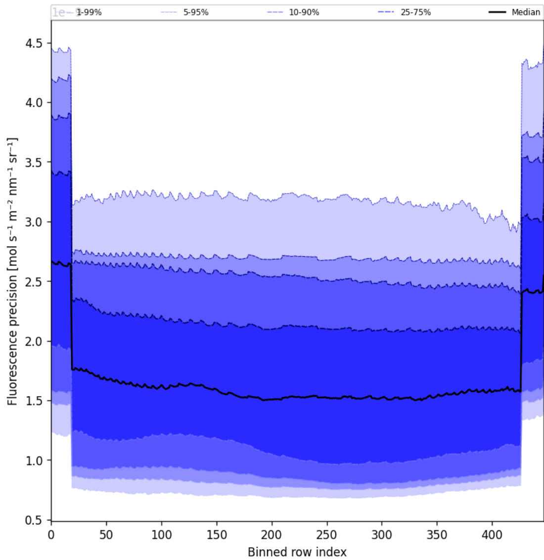
Figure 58: Along track statistics of “Fluorescence precision” for 2025-11-26 to 2025-11-28
