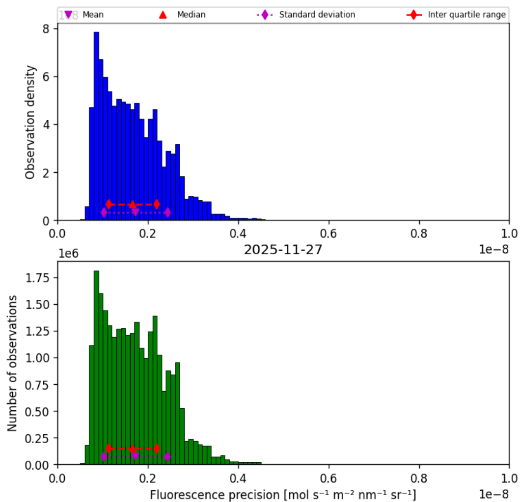
Figure 41: Histogram of “Fluorescence precision” for 2025-11-26 to 2025-11-28
