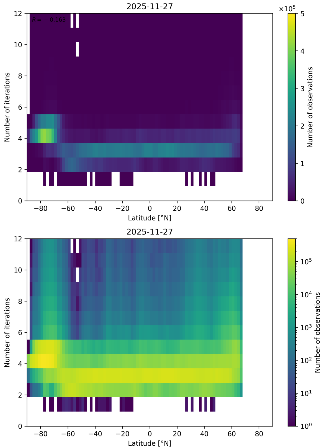
Figure 93: Scatter density plot of “Latitude” against “Number of iterations” for 2025-11-26 to 2025-11-28.
