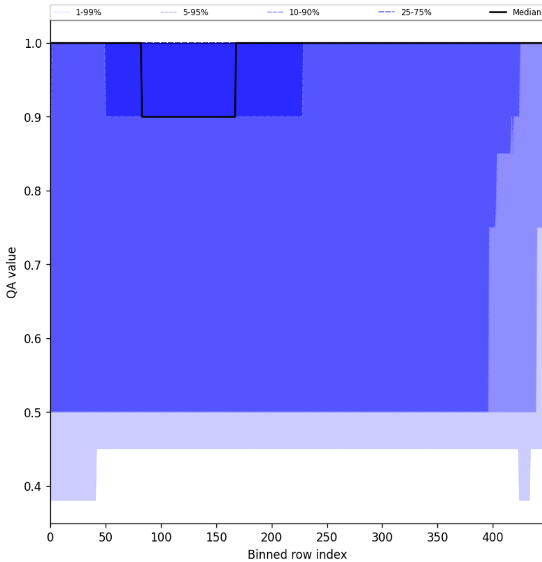
Figure 46: Along track statistics of “QA value” for 2025-11-26 to 2025-11-28
