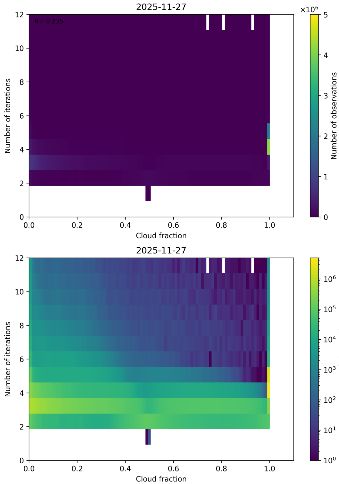
Figure 73: Scatter density plot of “Cloud fraction” against “Number of iterations” for 2025-11-26 to 2025-11-28.
