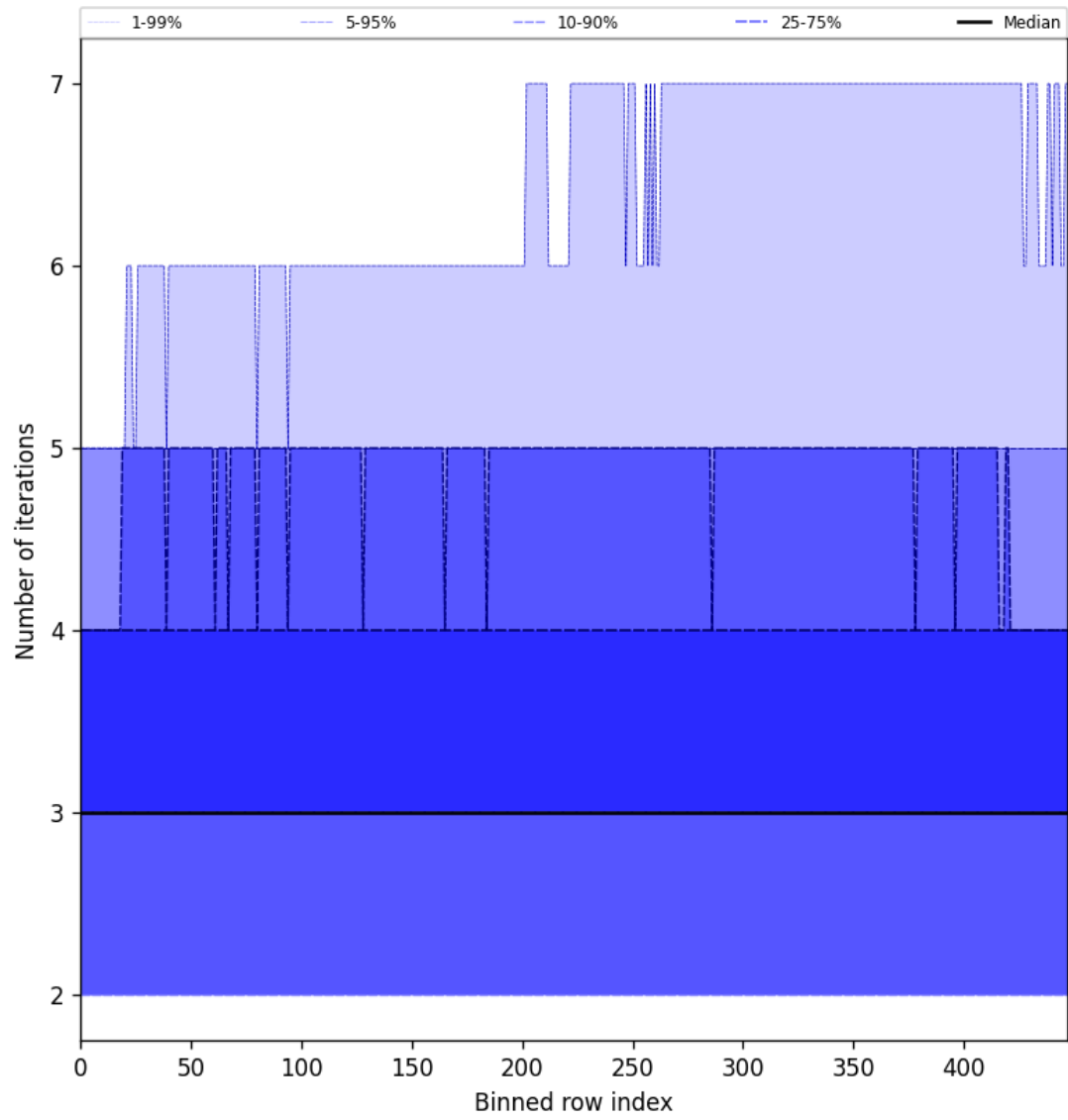
Figure 56: Along track statistics of “Number of iterations” for 2025-11-26 to 2025-11-28
