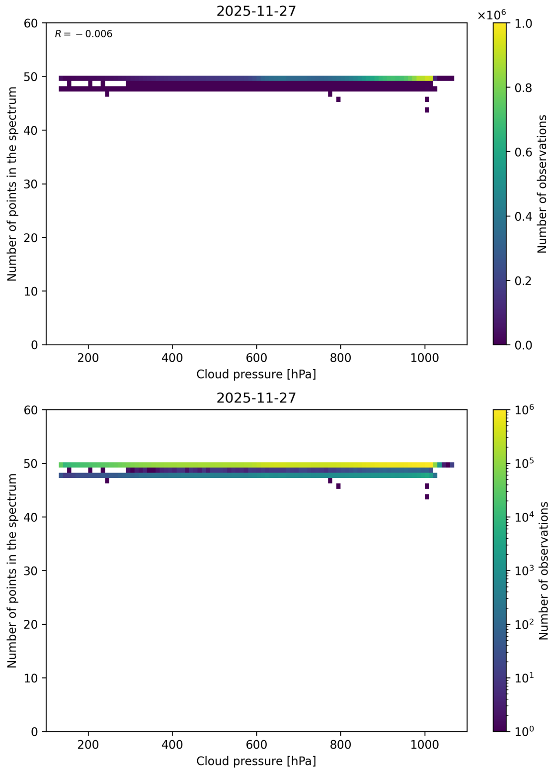
Figure 82: Scatter density plot of “Cloud pressure” against “Number of points in the spectrum” for 2025-11-26 to 2025-11-28.
