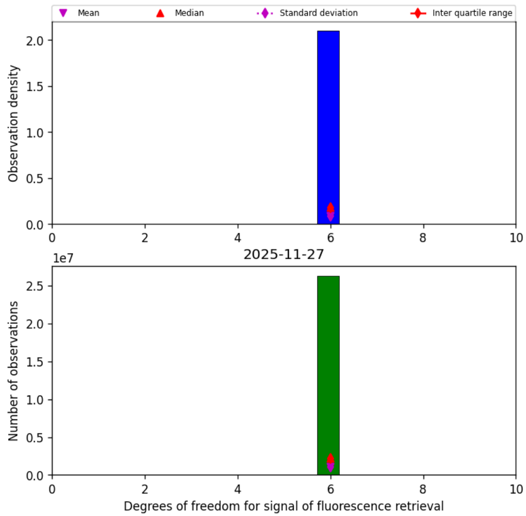
Figure 43: Histogram of “Degrees of freedom for signal of fluorescence retrieval” for 2025-11-26 to 2025-11-28
