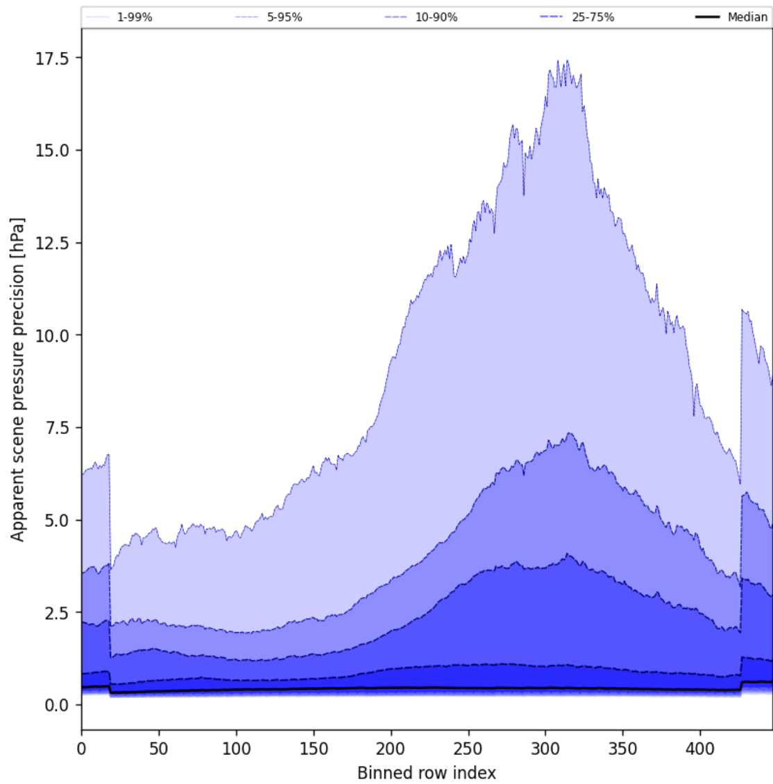
Figure 54: Along track statistics of “Apparent scene pressure precision” for 2025-11-26 to 2025-11-28
