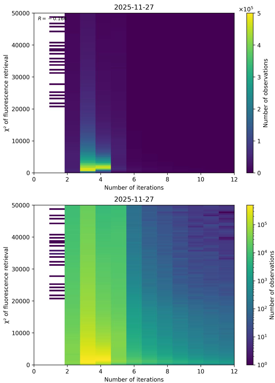
Figure 97: Scatter density plot of “Number of iterations” against “ \chi^2 of fluorescence retrieval” for 2025-11-26 to 2025-11-28.
