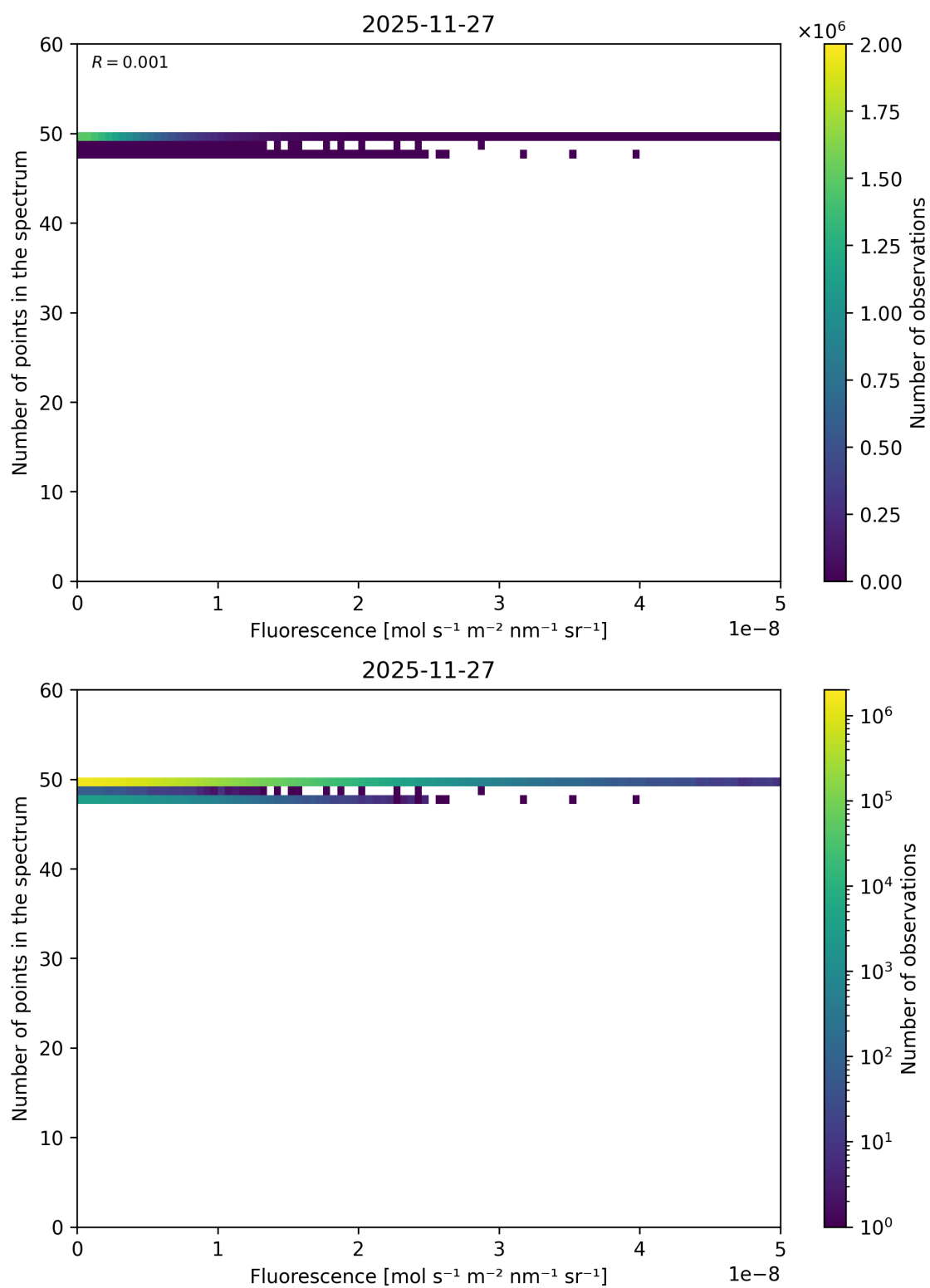
Figure 86: Scatter density plot of “Fluorescence” against “Number of points in the spectrum” for 2025-11-26 to 2025-11-28.
