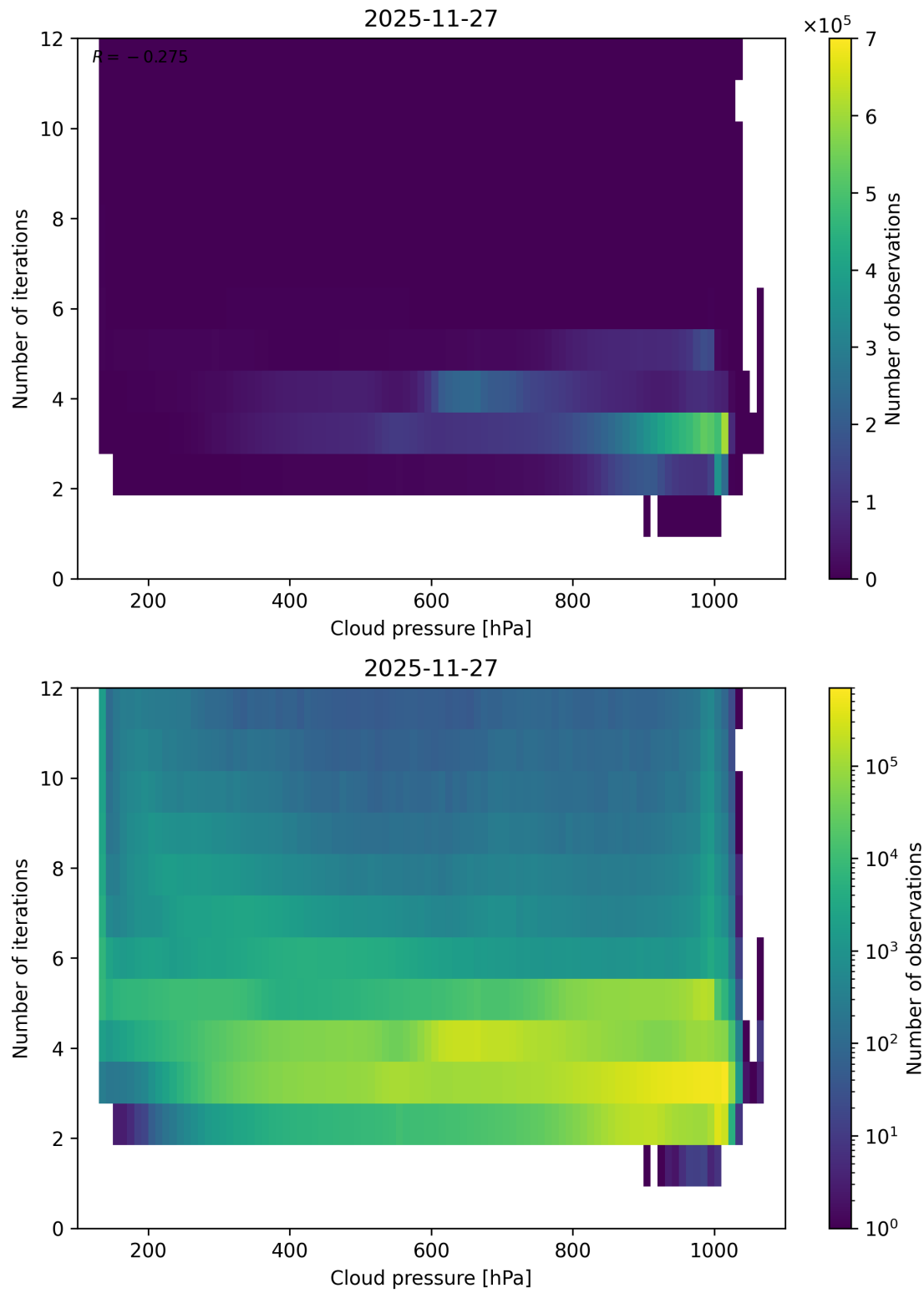
Figure 81: Scatter density plot of “Cloud pressure” against “Number of iterations” for 2025-11-26 to 2025-11-28.
