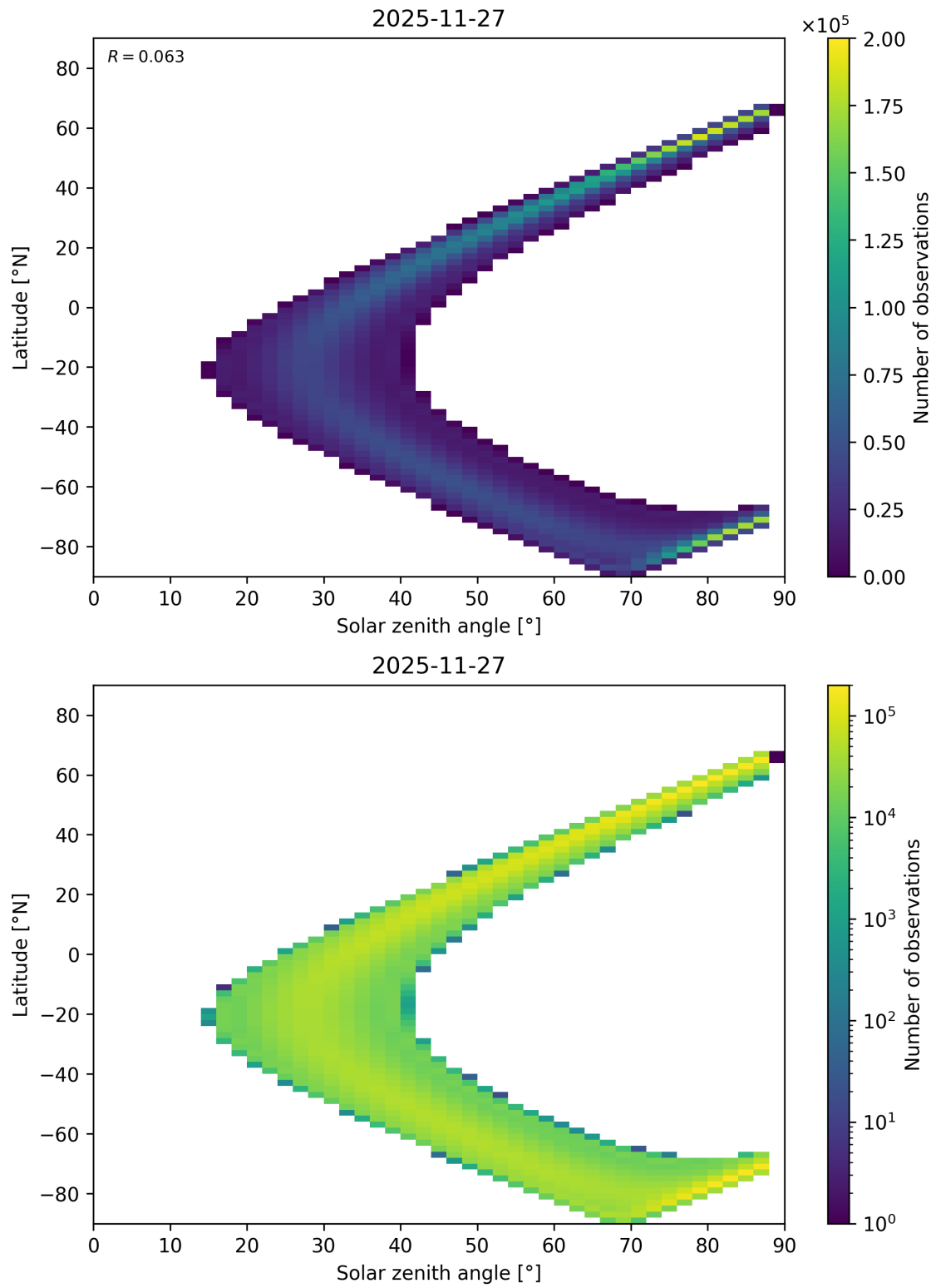
Figure 113: Scatter density plot of “Solar zenith angle” against “Latitude” for 2025-11-26 to 2025-11-28.
