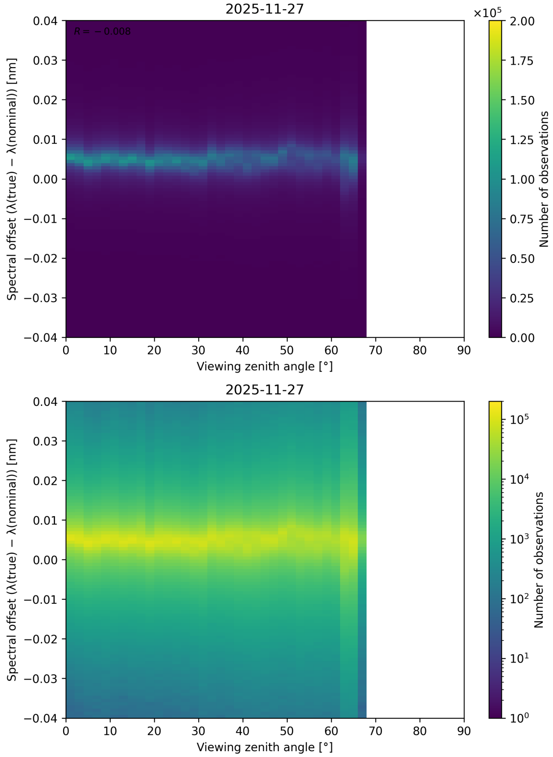
Figure 128: Scatter density plot of “Viewing zenith angle” against “Spectral offset ( \lambda_{\text{true}} - \lambda_{\text{nominal}} )” for 2025-11-26 to 2025-11-28.
