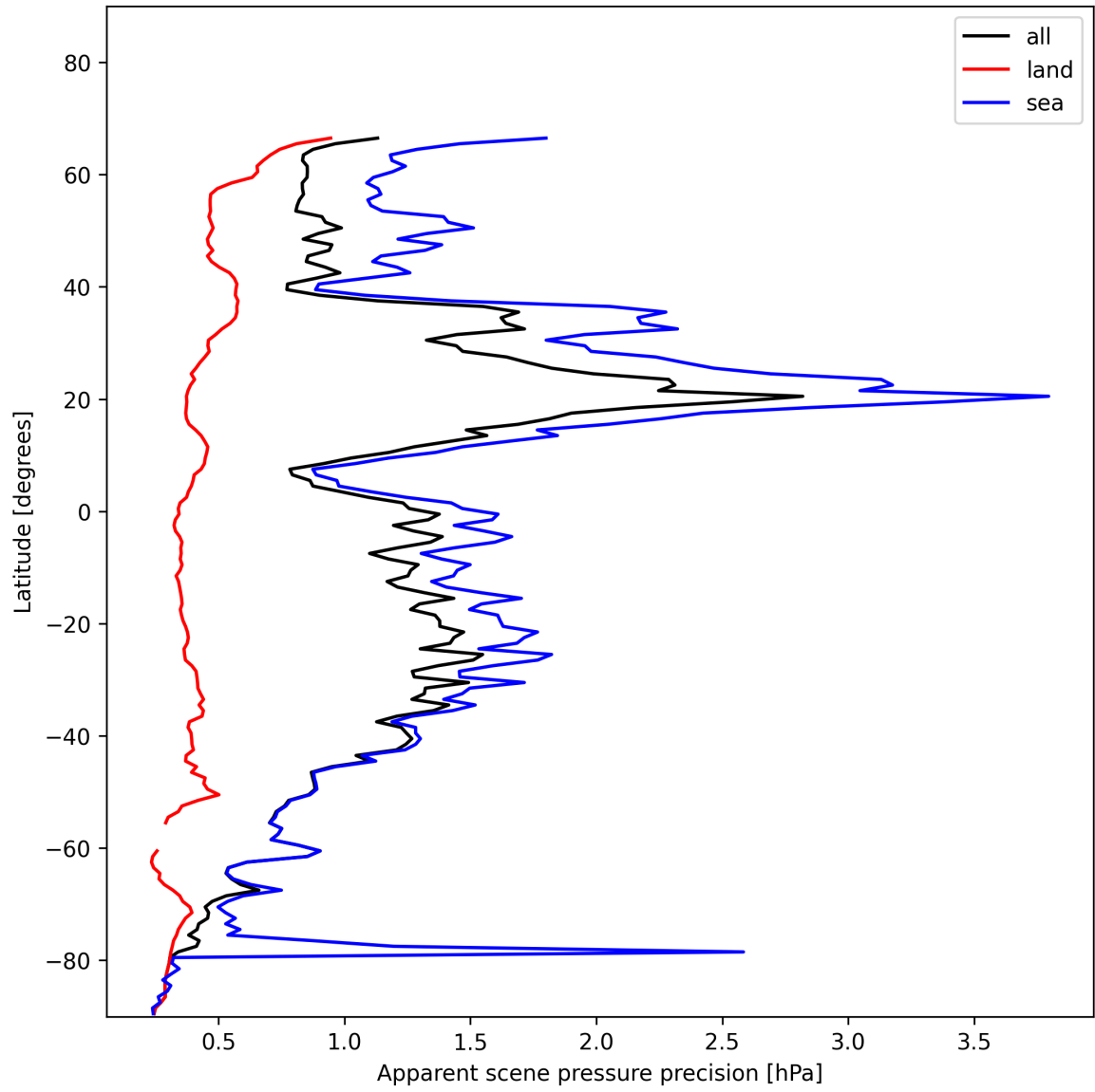
Figure 20: Zonal average of “Apparent scene pressure precision” for 2025-11-26 to 2025-11-28.
