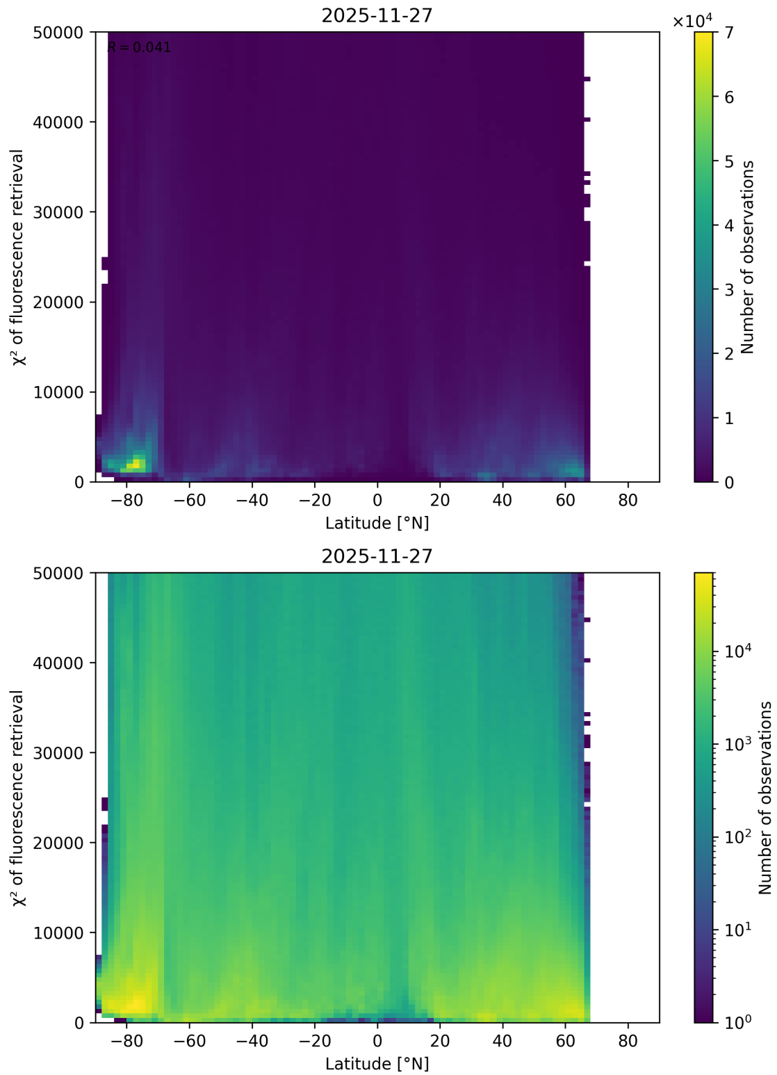
Figure 89: Scatter density plot of “Latitude” against “ \chi^2 of fluorescence retrieval” for 2025-11-26 to 2025-11-28.
