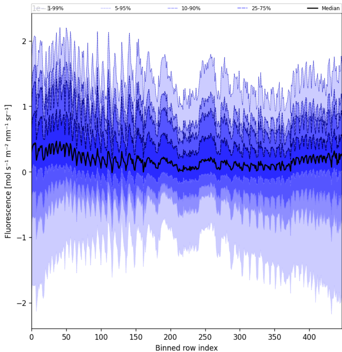
Figure 57: Along track statistics of “Fluorescence” for 2025-11-26 to 2025-11-28
