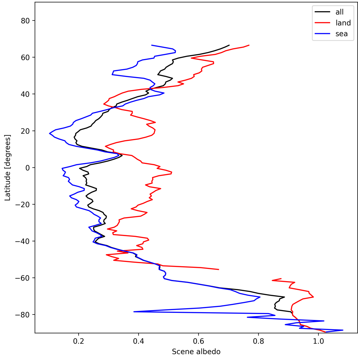
Figure 17: Zonal average of “Scene albedo” for 2025-11-26 to 2025-11-28.
