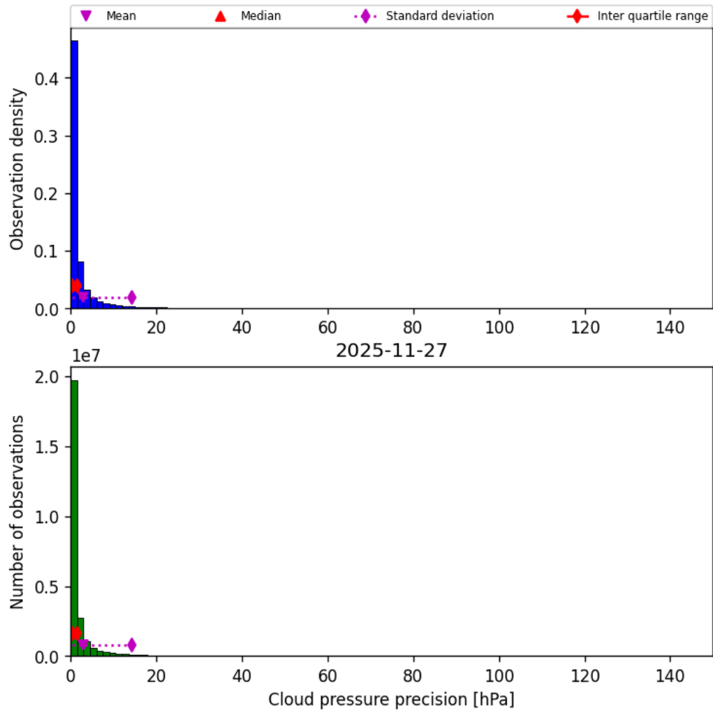
Figure 31: Histogram of “Cloud pressure precision” for 2025-11-26 to 2025-11-28
