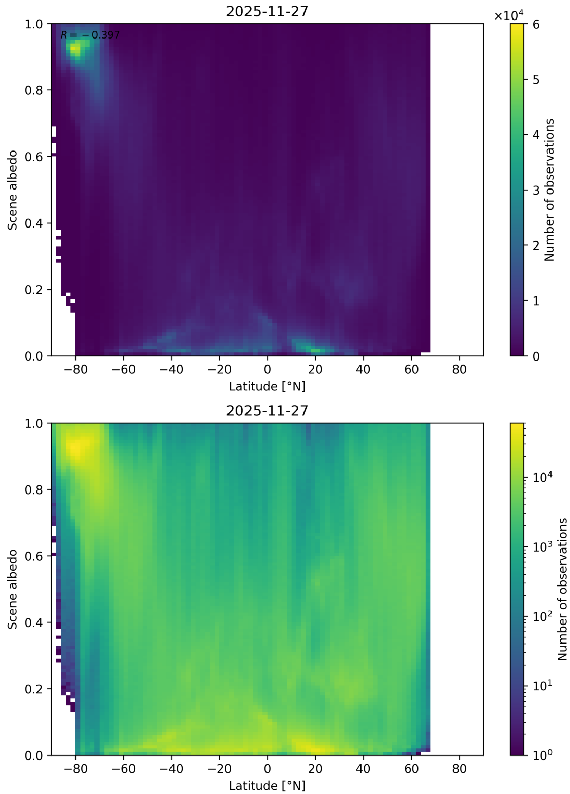
Figure 95: Scatter density plot of “Latitude” against “Scene albedo” for 2025-11-26 to 2025-11-28.
