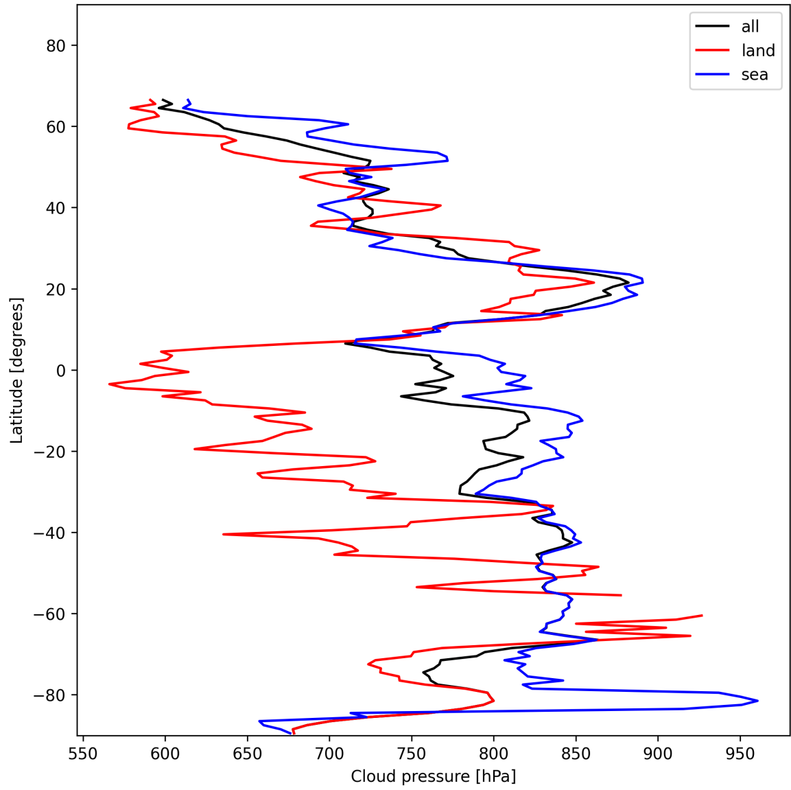
Figure 13: Zonal average of “Cloud pressure” for 2025-11-26 to 2025-11-28.
