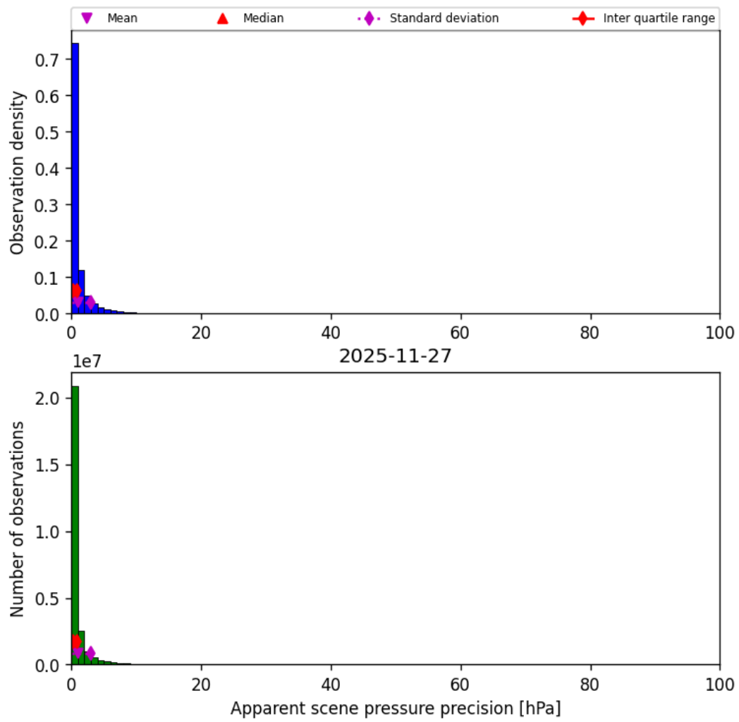
Figure 37: Histogram of “Apparent scene pressure precision” for 2025-11-26 to 2025-11-28
