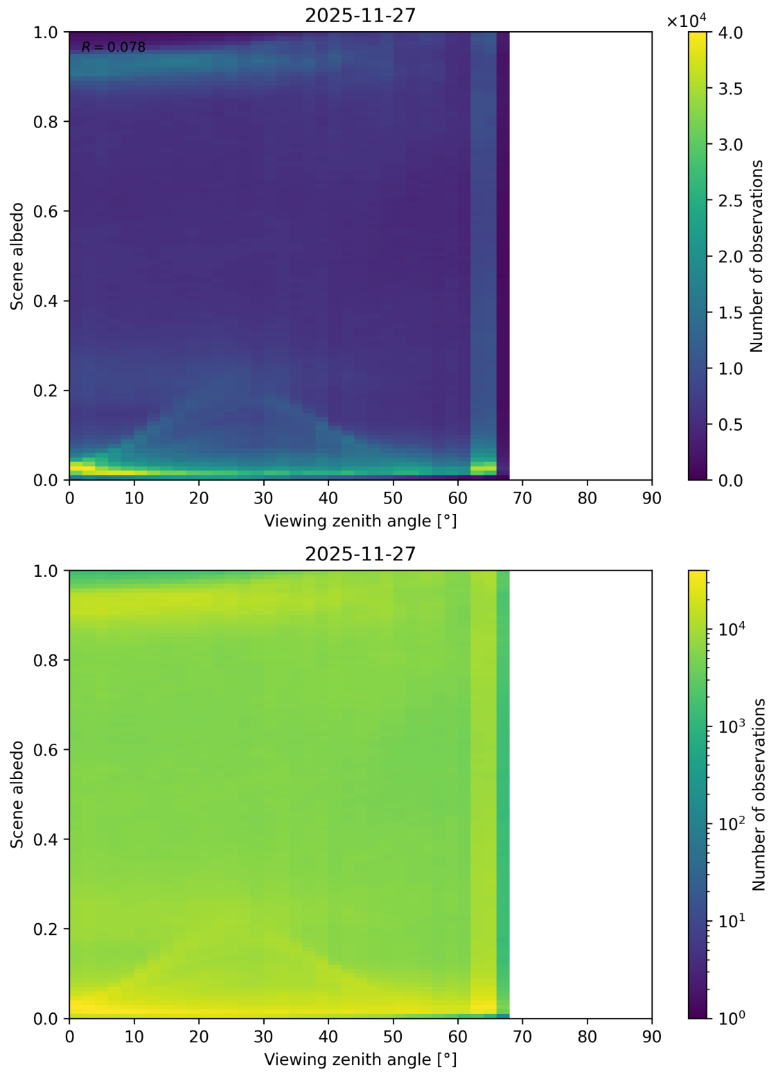
Figure 126: Scatter density plot of “Viewing zenith angle” against “Scene albedo” for 2025-11-26 to 2025-11-28.
