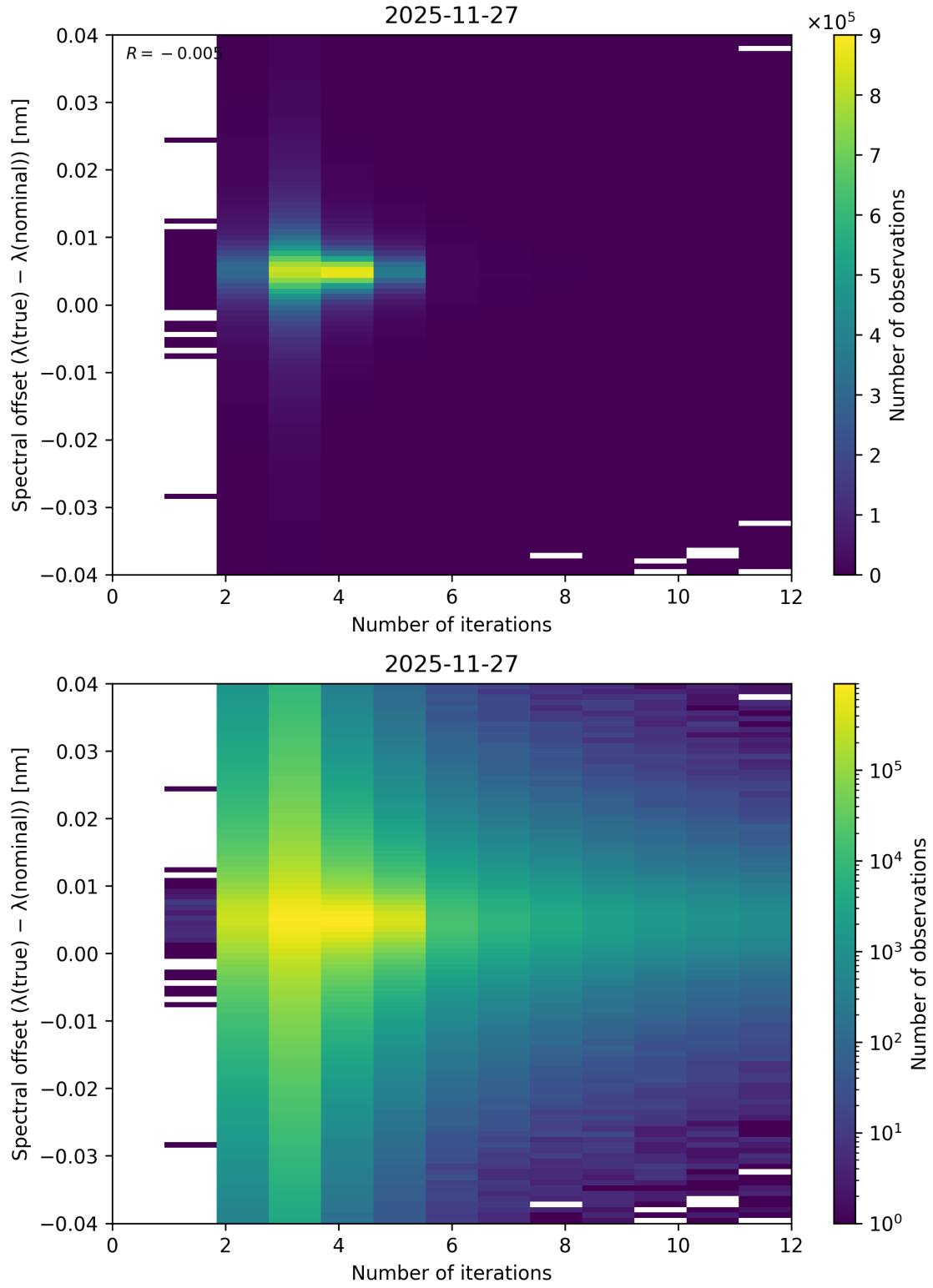
Figure 100: Scatter density plot of “Number of iterations” against “Spectral offset ( \lambda_{\text{true}} - \lambda_{\text{nominal}} )” for 2025-11-26 to 2025-11-28.
