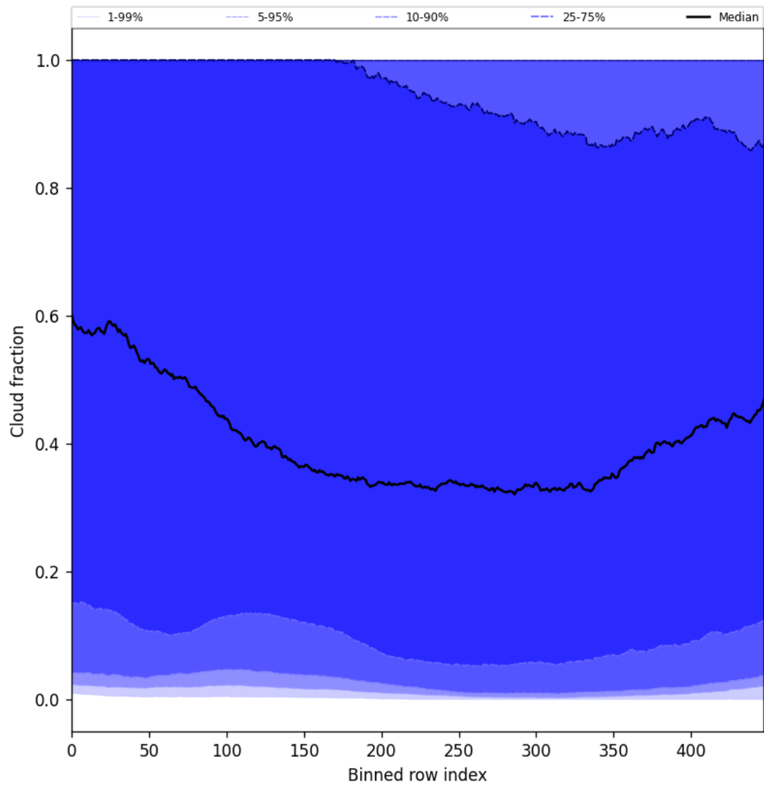
Figure 49: Along track statistics of “Cloud fraction” for 2025-11-26 to 2025-11-28
