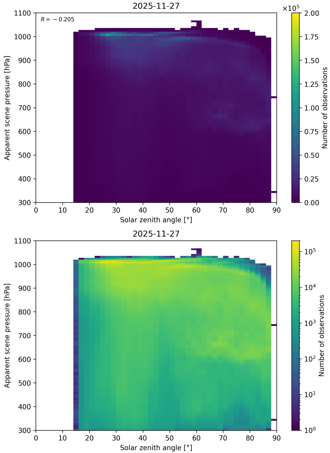
Figure 108: Scatter density plot of “Solar zenith angle” against “Apparent scene pressure” for 2025-11-26 to 2025-11-28.
