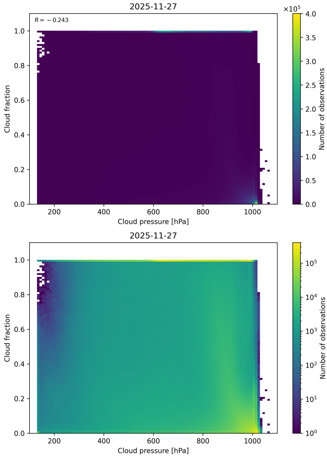
Figure 79: Scatter density plot of “Cloud pressure” against “Cloud fraction” for 2025-11-26 to 2025-11-28.
