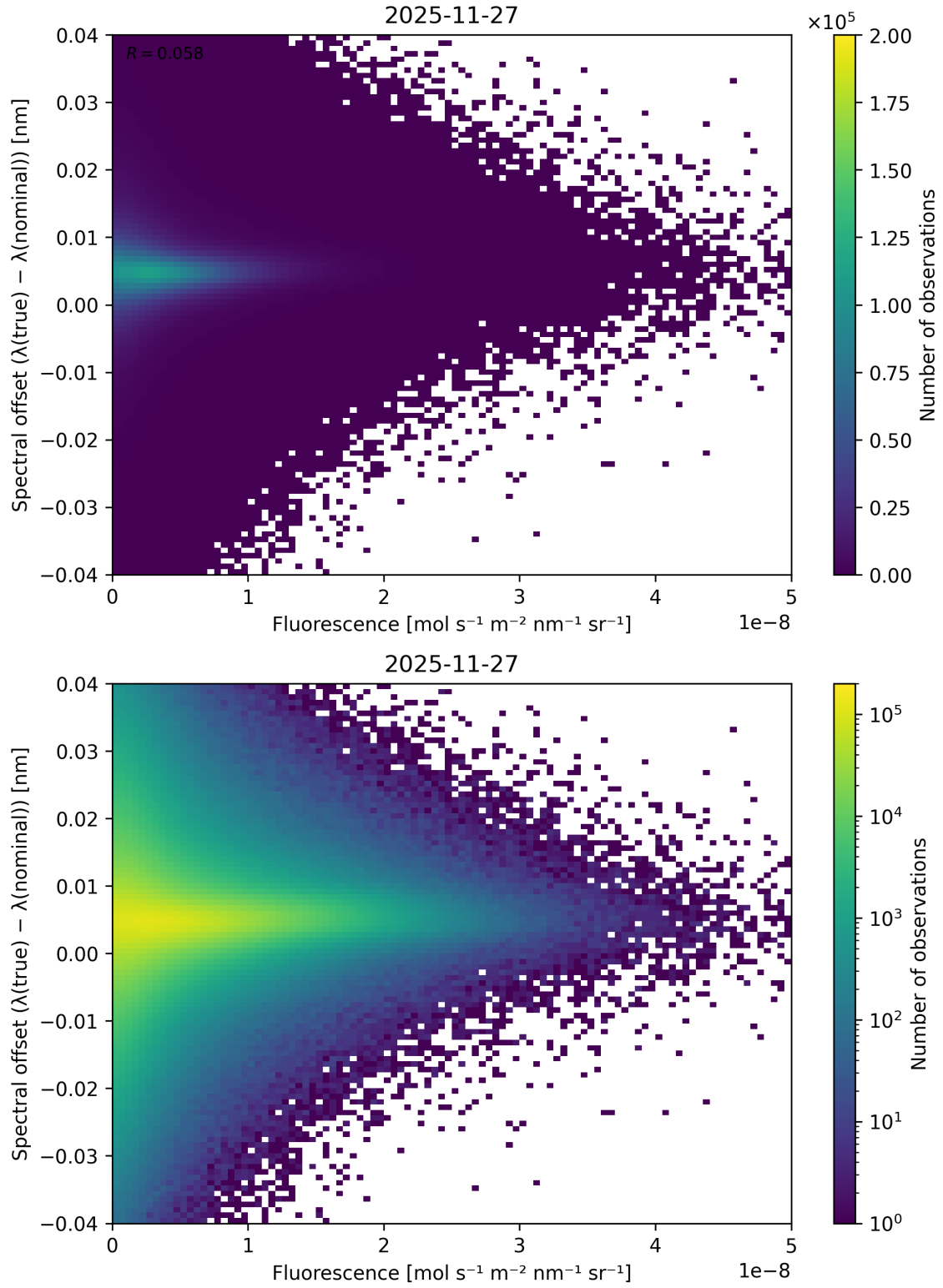
Figure 87: Scatter density plot of “Fluorescence” against “Spectral offset ( \lambda_{\text{true}} - \lambda_{\text{nominal}} )” for 2025-11-26 to 2025-11-28.
