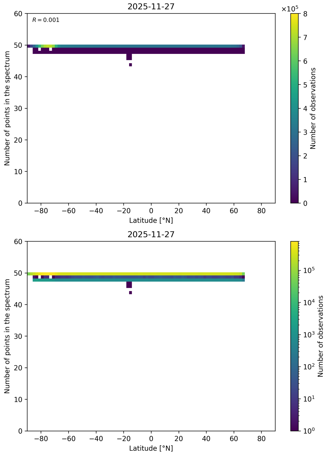
Figure 94: Scatter density plot of “Latitude” against “Number of points in the spectrum” for 2025-11-26 to 2025-11-28.
