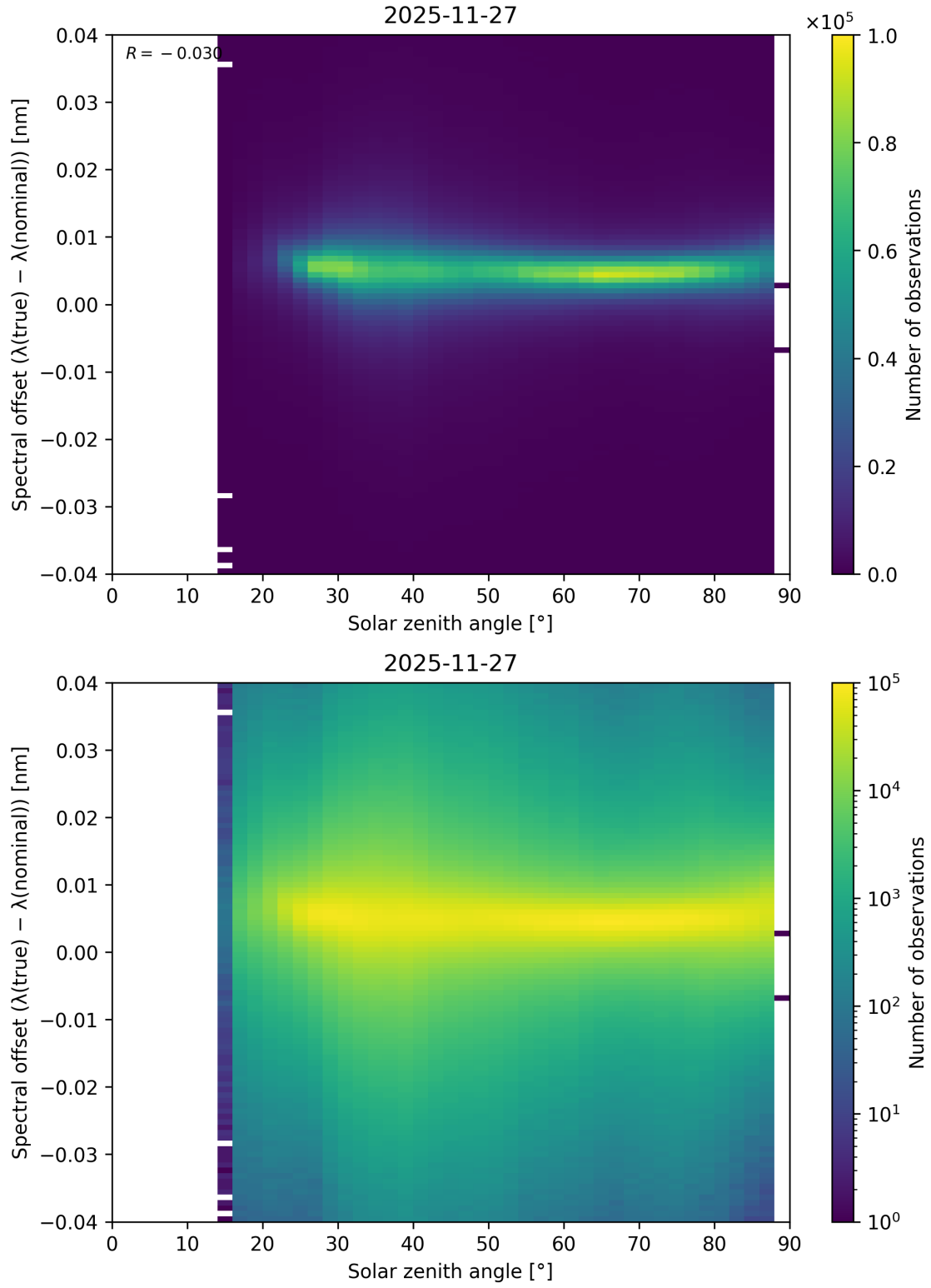
Figure 117: Scatter density plot of “Solar zenith angle” against “Spectral offset ( \lambda_{\text{true}} - \lambda_{\text{nominal}} )” for 2025-11-26 to 2025-11-28.
