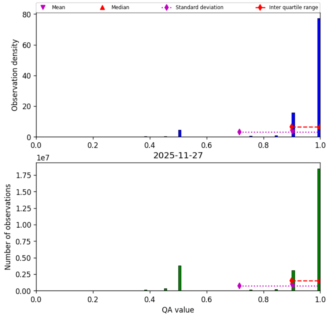
Figure 29: Histogram of “QA value” for 2025-11-26 to 2025-11-28
