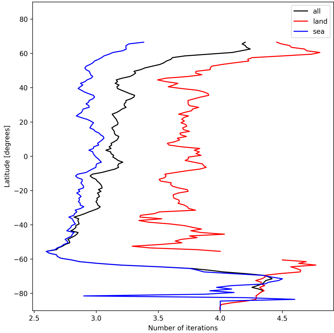
Figure 22: Zonal average of “Number of iterations” for 2025-11-26 to 2025-11-28.
