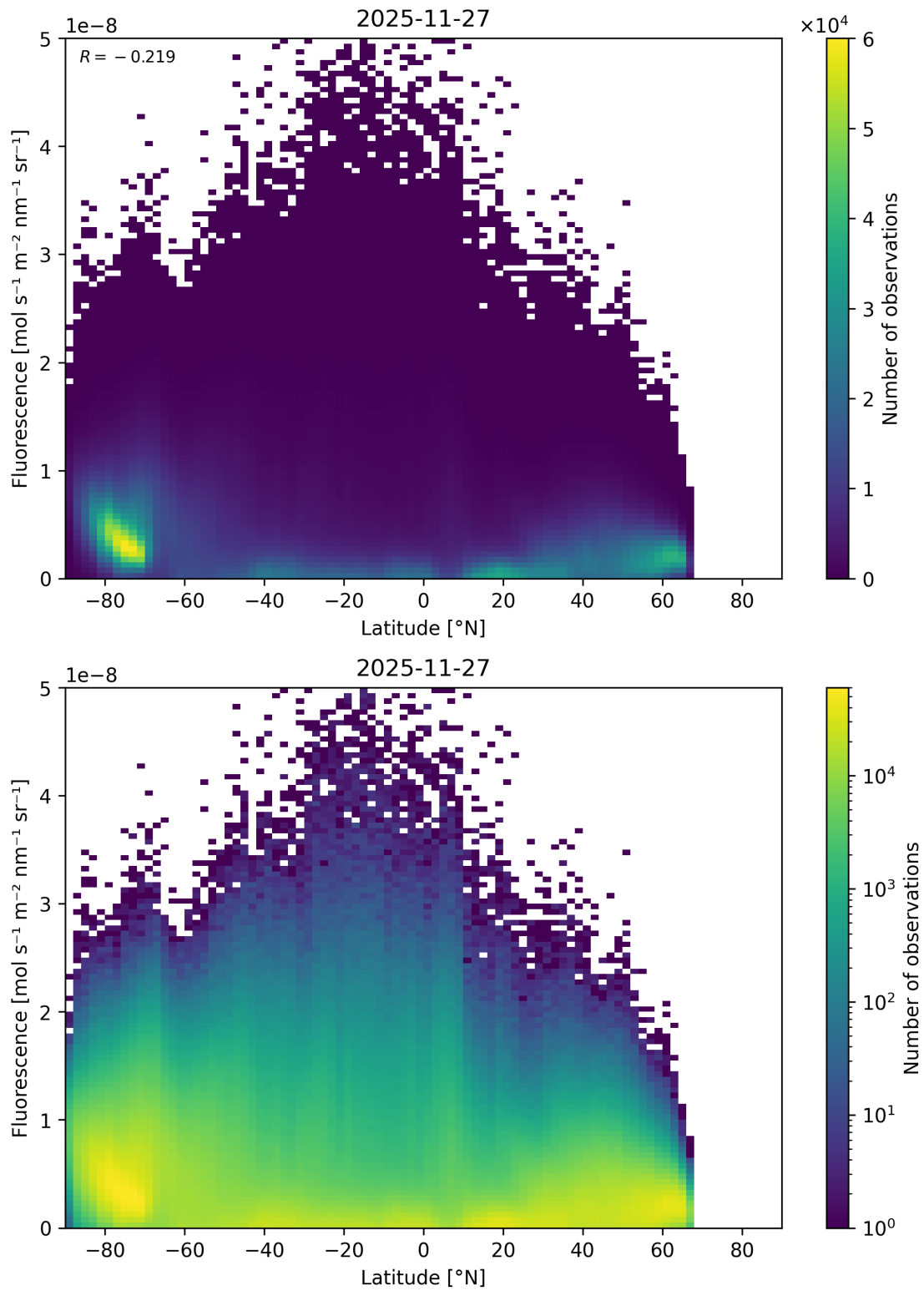
Figure 92: Scatter density plot of “Latitude” against “Fluorescence” for 2025-11-26 to 2025-11-28.
