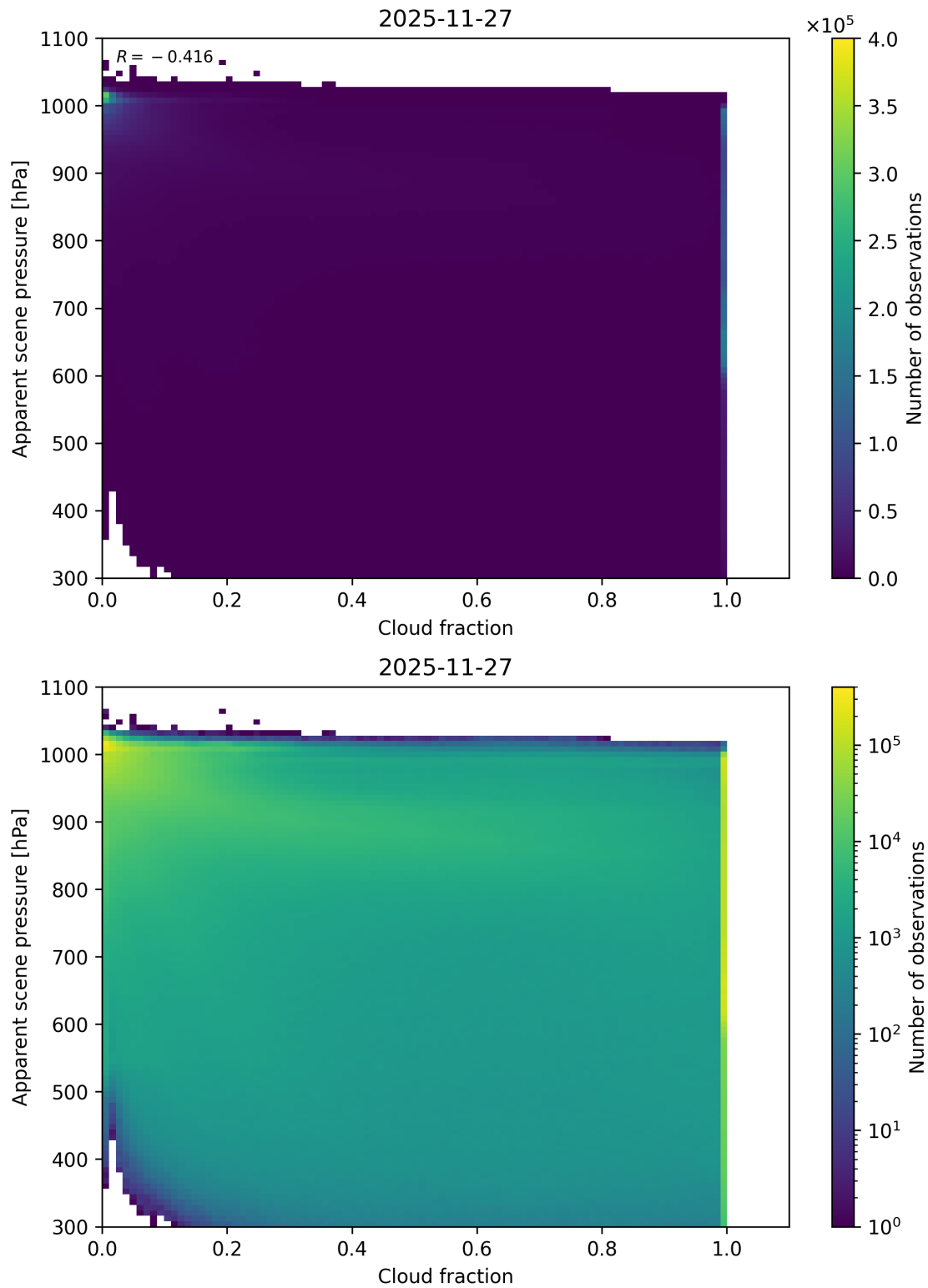
Figure 70: Scatter density plot of “Cloud fraction” against “Apparent scene pressure” for 2025-11-26 to 2025-11-28.
