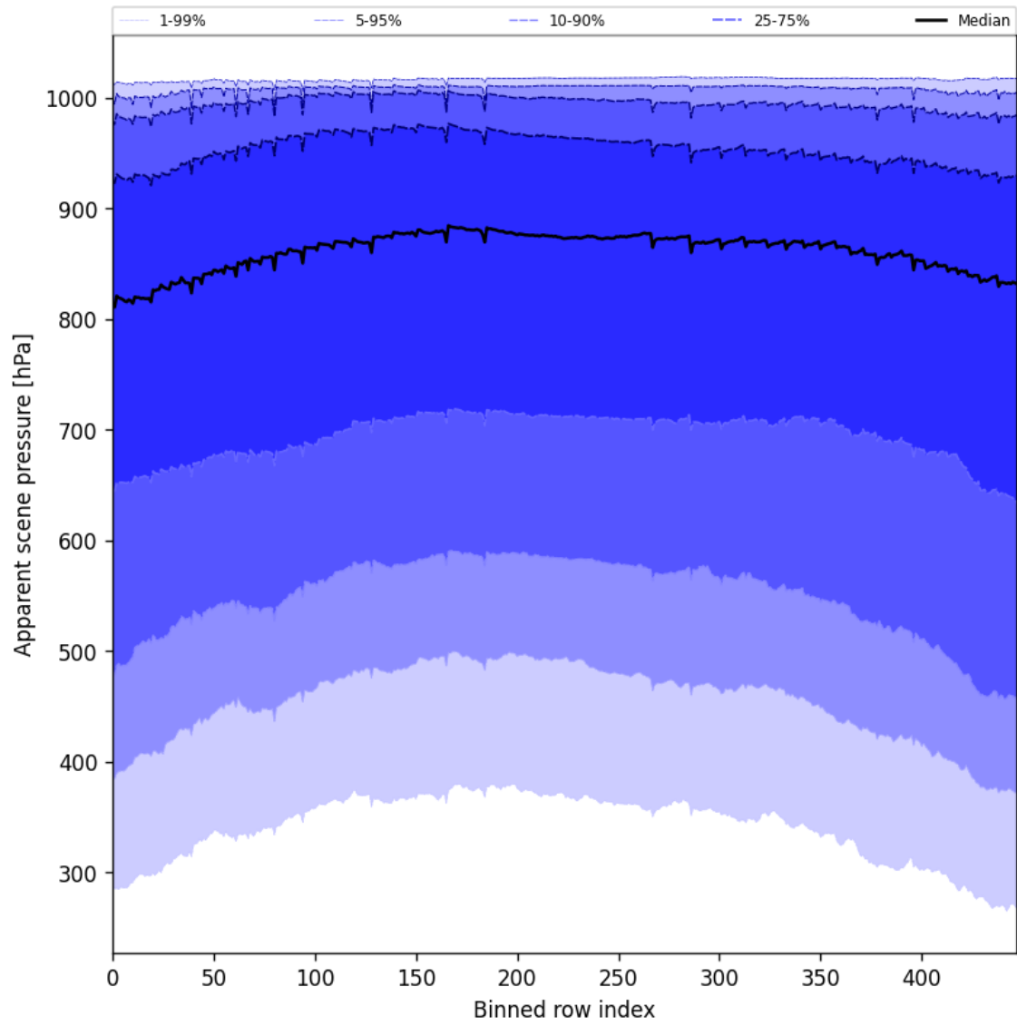
Figure 53: Along track statistics of “Apparent scene pressure” for 2025-11-26 to 2025-11-28
