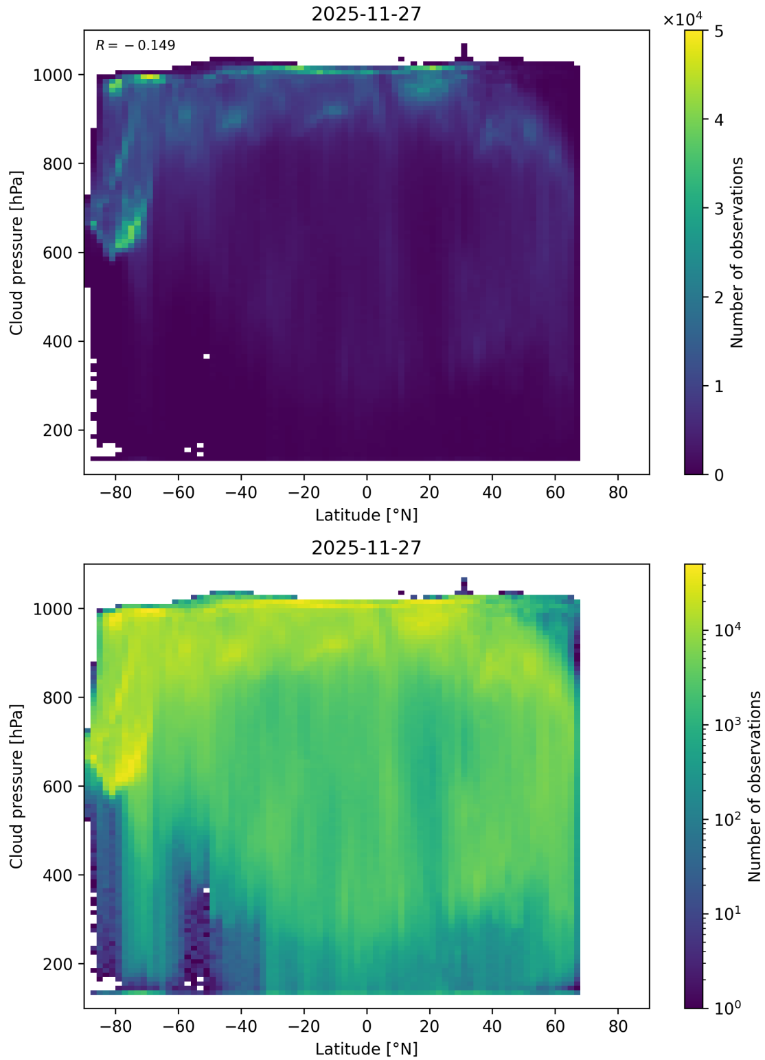
Figure 91: Scatter density plot of “Latitude” against “Cloud pressure” for 2025-11-26 to 2025-11-28.
