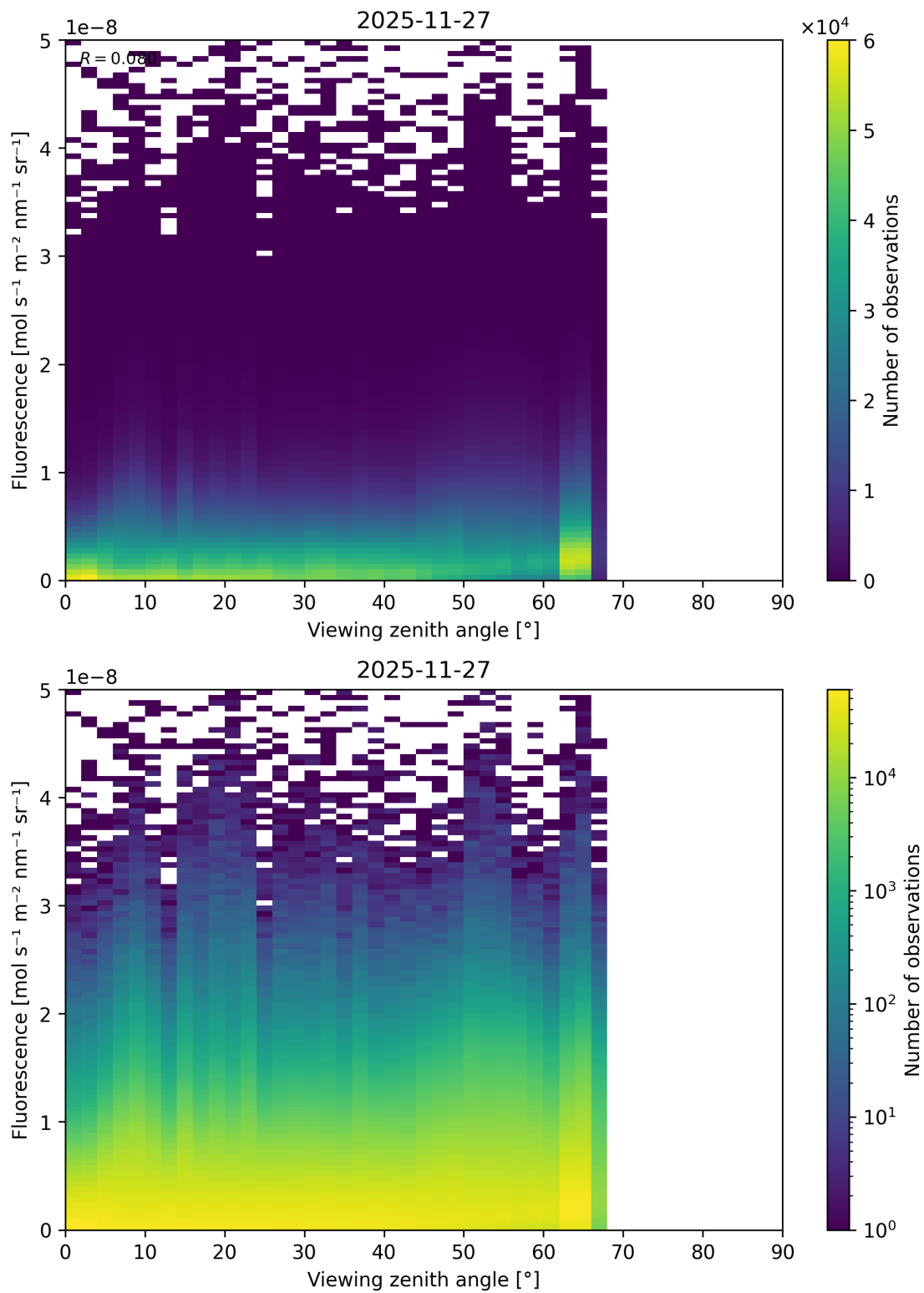
Figure 122: Scatter density plot of “Viewing zenith angle” against “Fluorescence” for 2025-11-26 to 2025-11-28.
