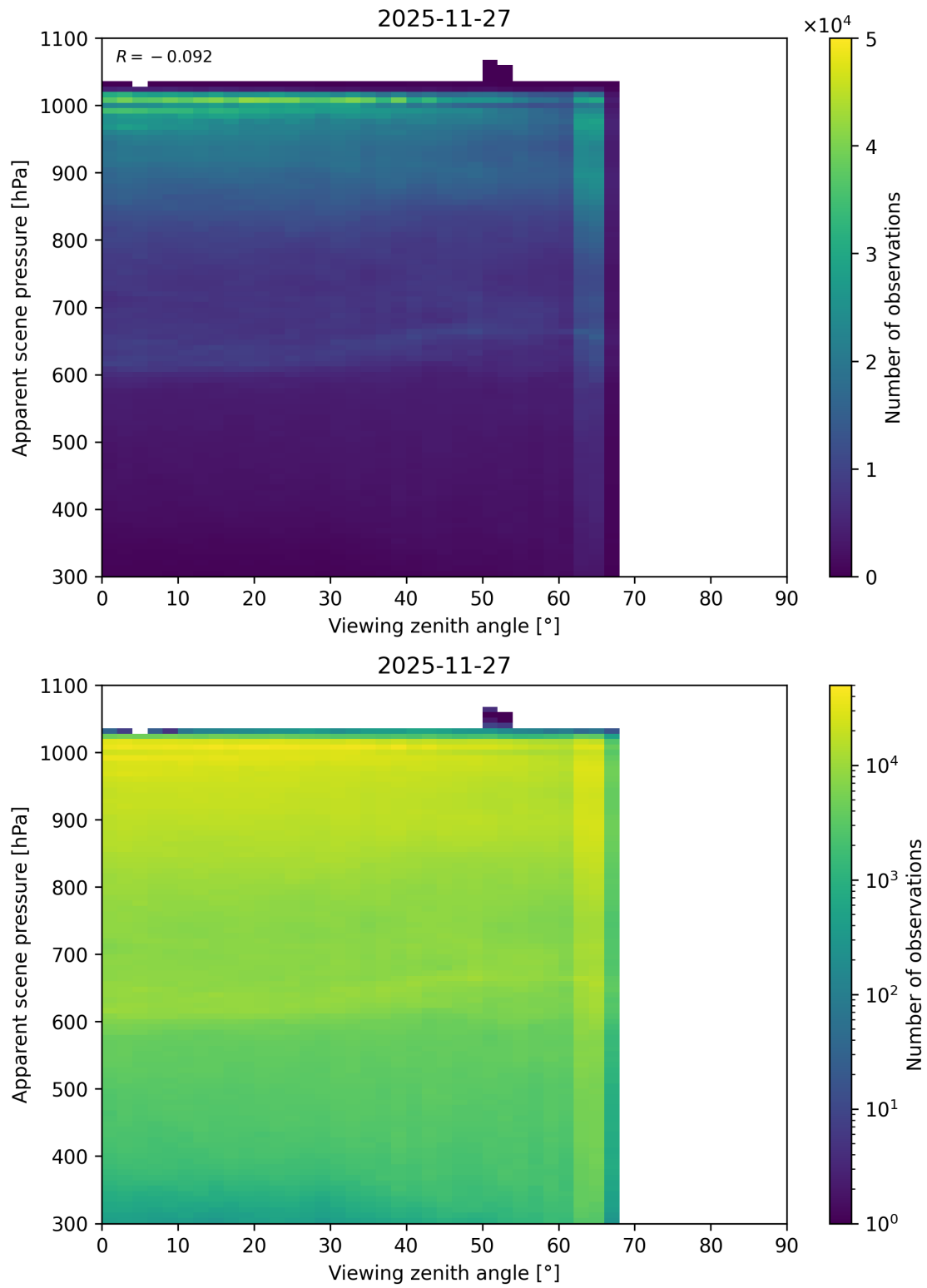
Figure 118: Scatter density plot of “Viewing zenith angle” against “Apparent scene pressure” for 2025-11-26 to 2025-11-28.
