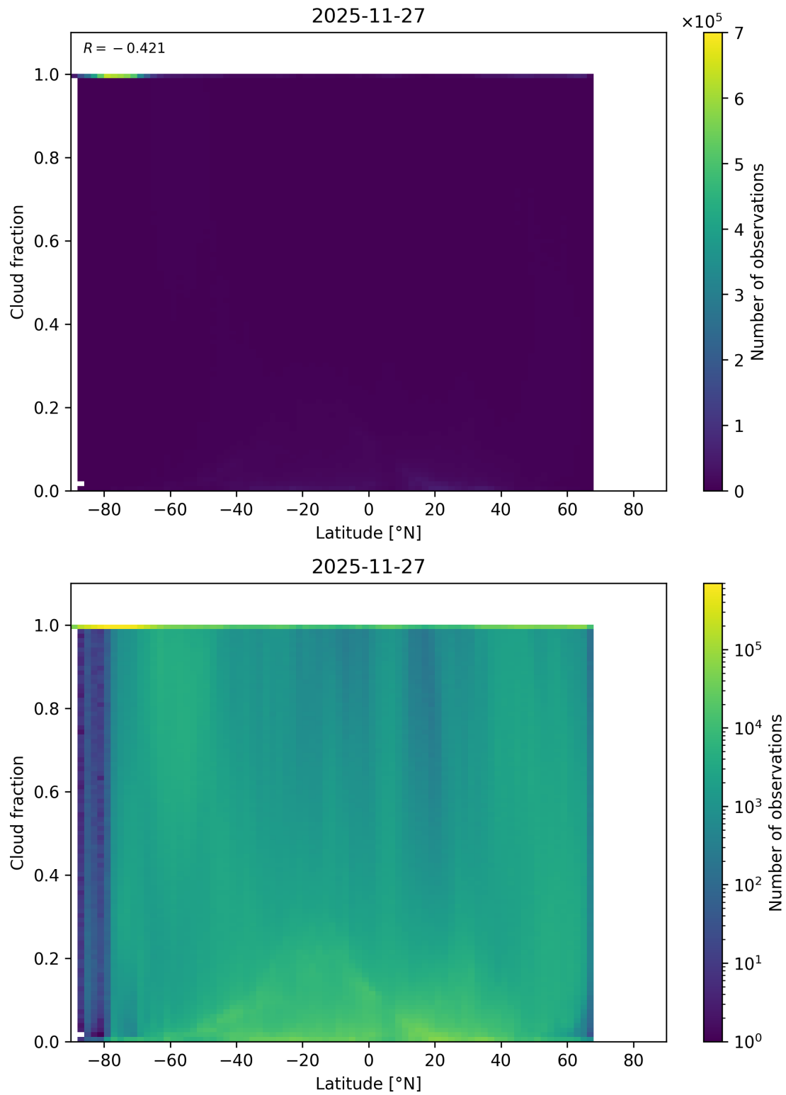
Figure 90: Scatter density plot of “Latitude” against “Cloud fraction” for 2025-11-26 to 2025-11-28.
