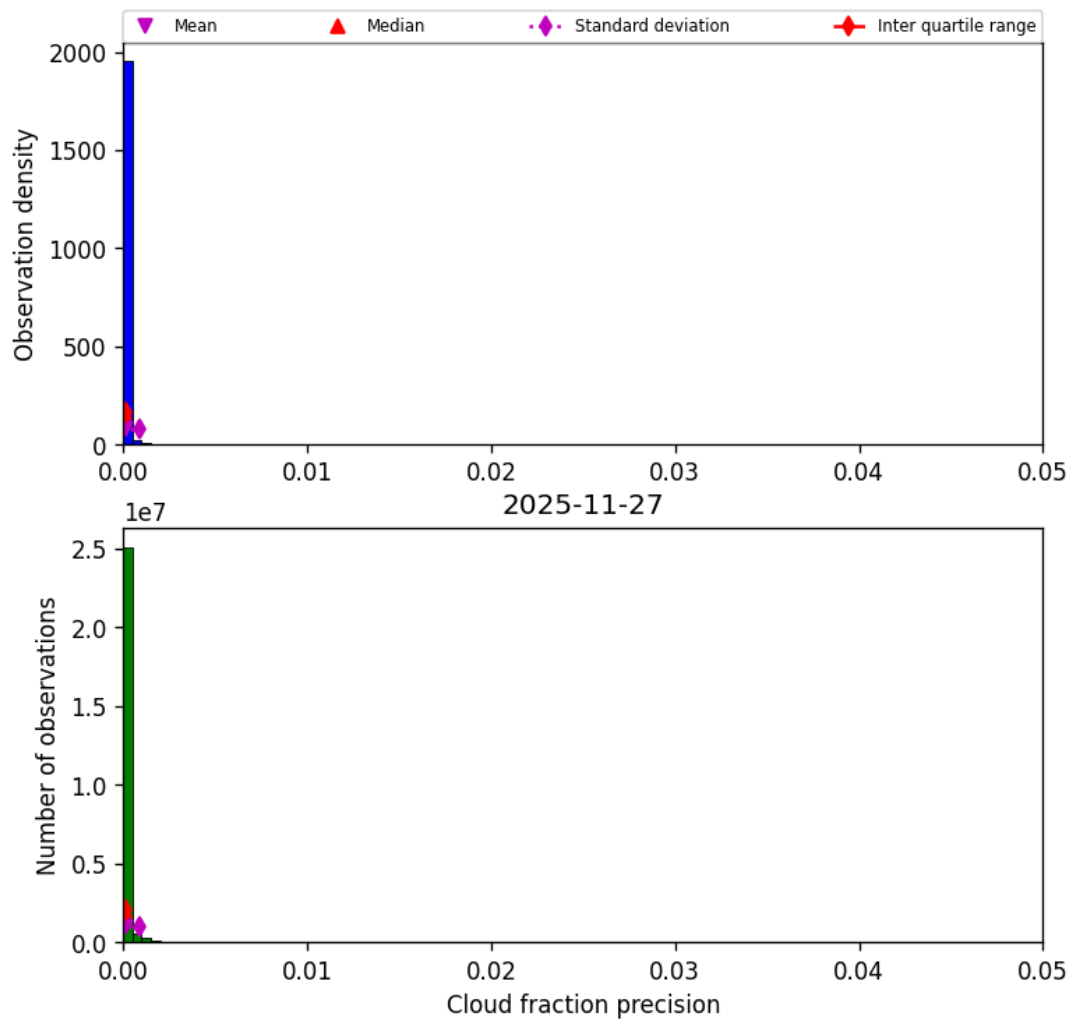
Figure 33: Histogram of “Cloud fraction precision” for 2025-11-26 to 2025-11-28
