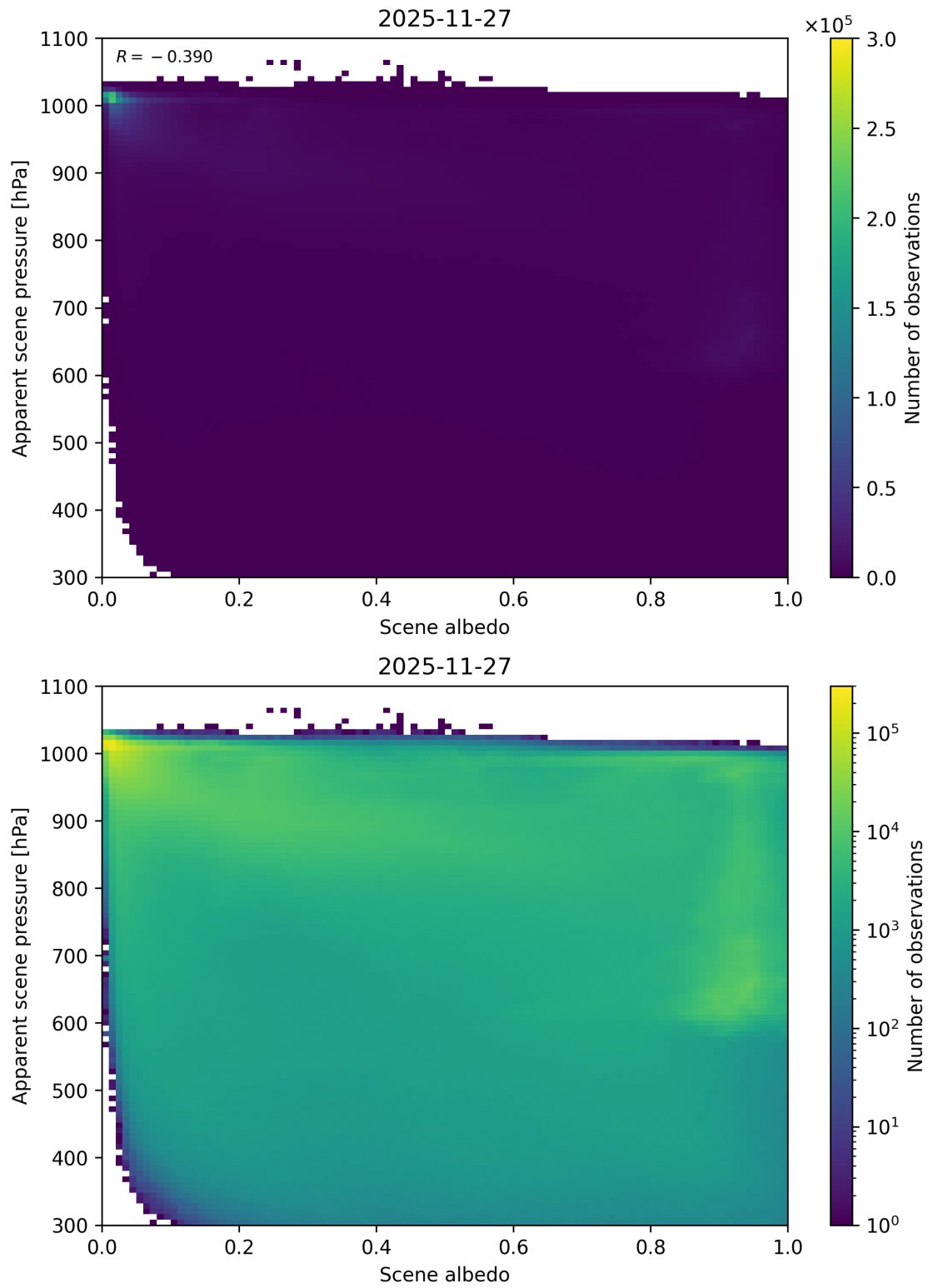
Figure 102: Scatter density plot of “Scene albedo” against “Apparent scene pressure” for 2025-11-26 to 2025-11-28.
