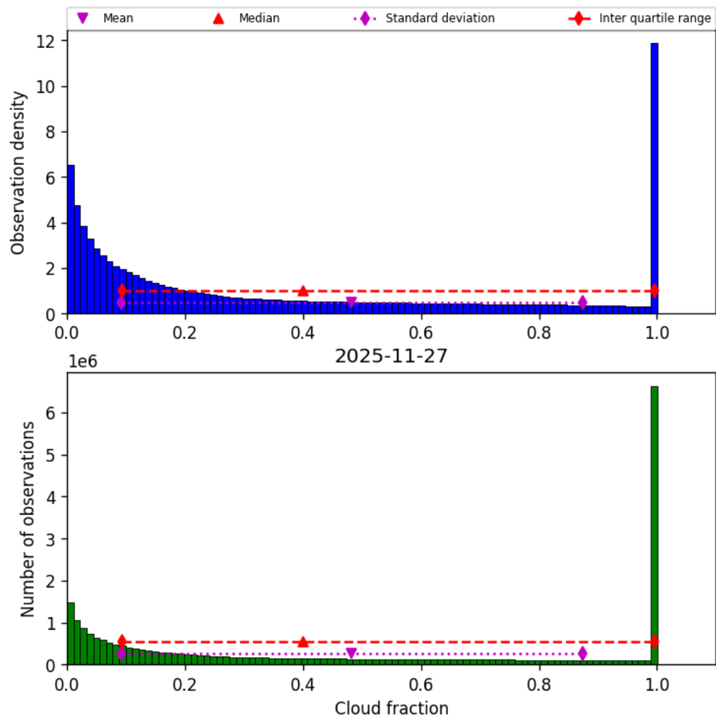
Figure 32: Histogram of “Cloud fraction” for 2025-11-26 to 2025-11-28
