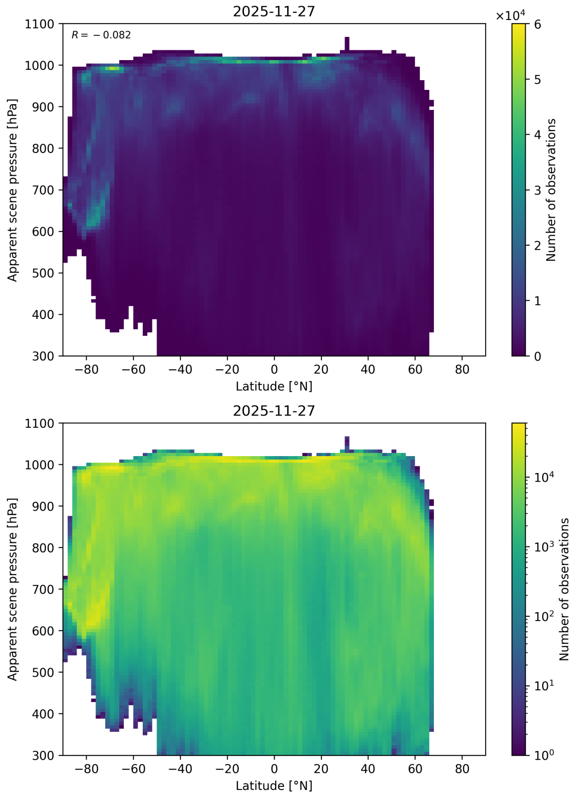
Figure 88: Scatter density plot of “Latitude” against “Apparent scene pressure” for 2025-11-26 to 2025-11-28.
