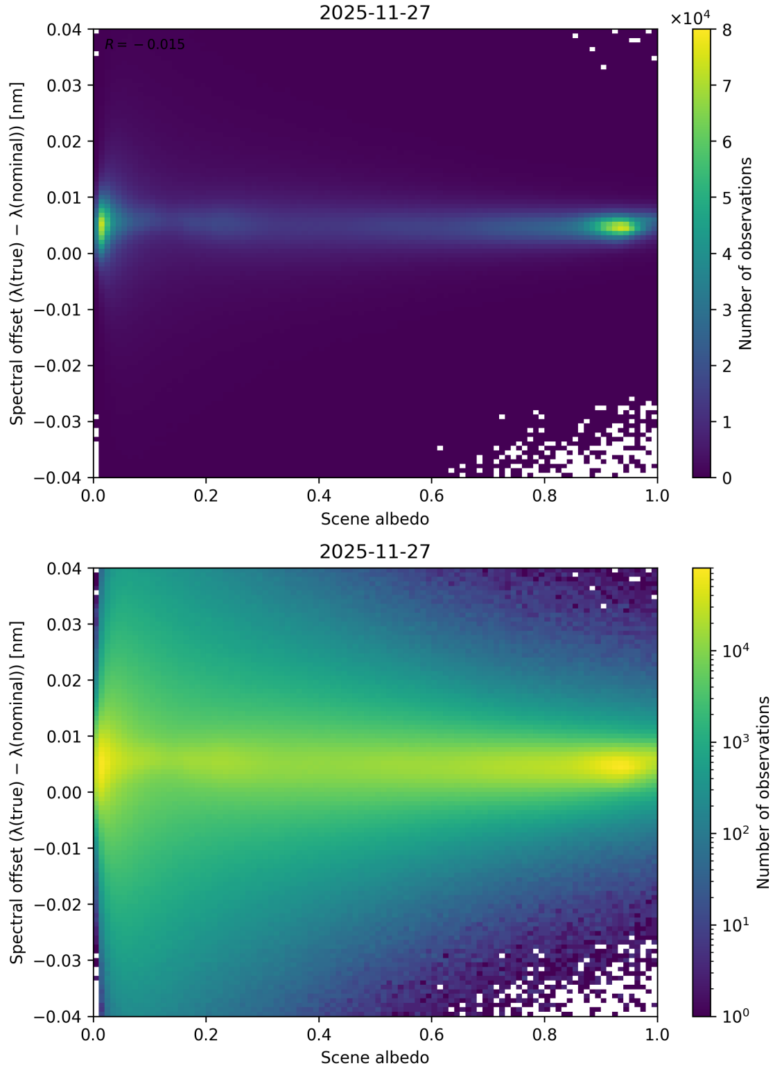
Figure 107: Scatter density plot of “Scene albedo” against “Spectral offset ( \lambda_{\text{true}} - \lambda_{\text{nominal}} )” for 2025-11-26 to 2025-11-28.
