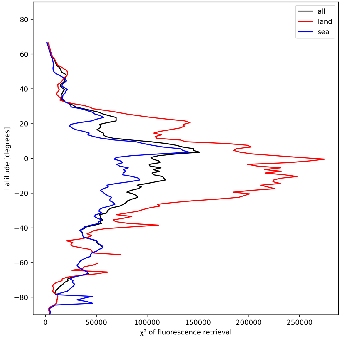
Figure 25: Zonal average of “ \chi^2 of fluorescence retrieval” for 2025-11-26 to 2025-11-28.
