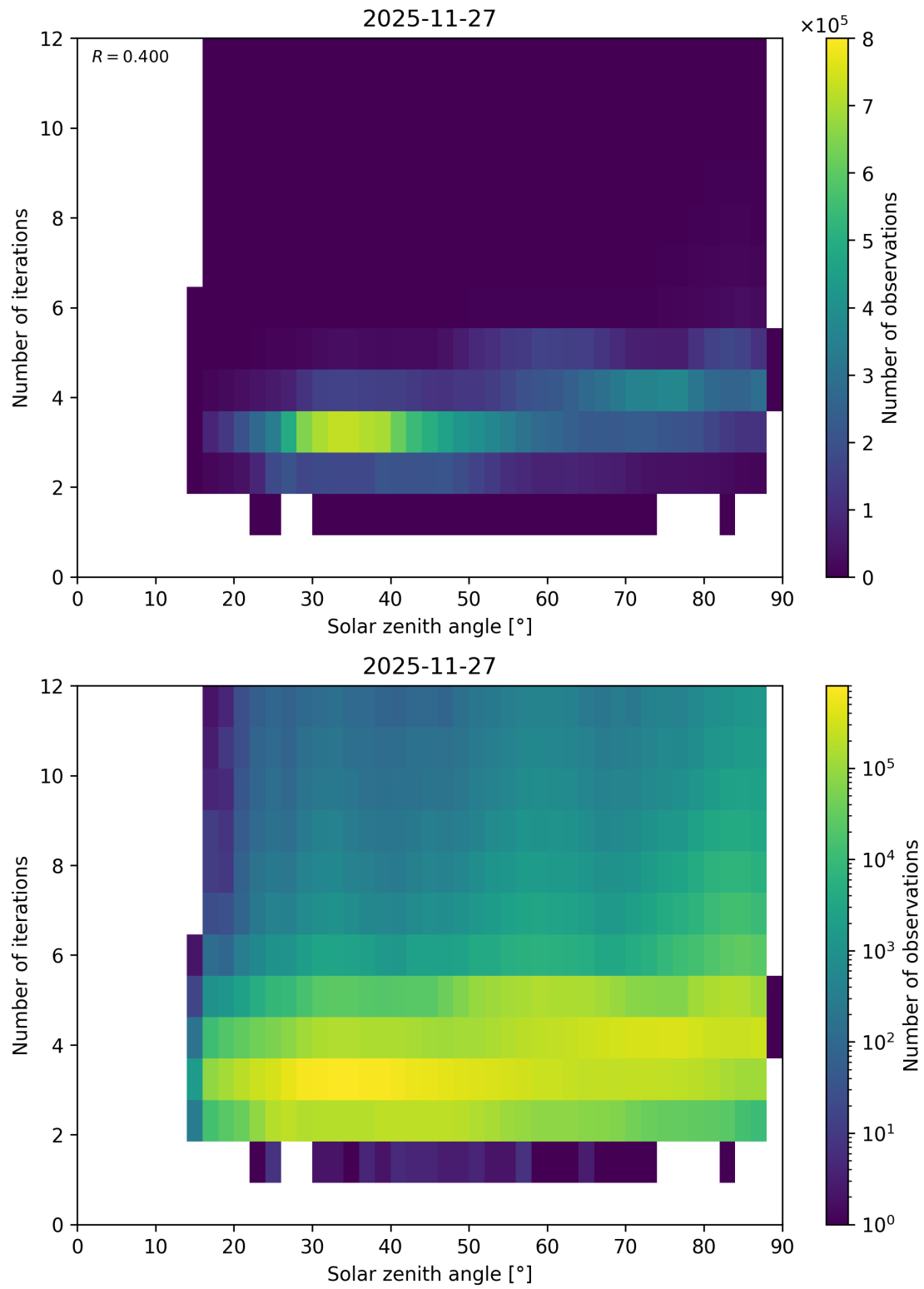
Figure 114: Scatter density plot of “Solar zenith angle” against “Number of iterations” for 2025-11-26 to 2025-11-28.
