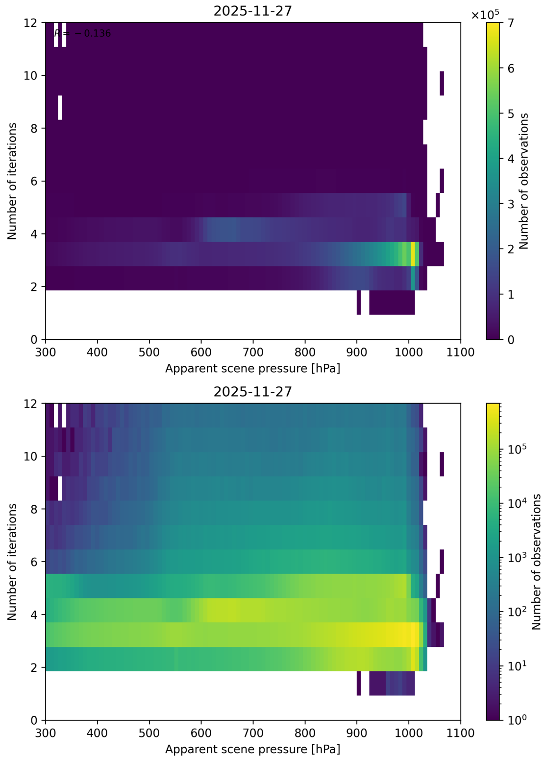
Figure 65: Scatter density plot of “Apparent scene pressure” against “Number of iterations” for 2025-11-26 to 2025-11-28.
