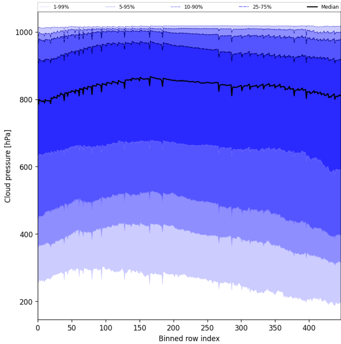
Figure 47: Along track statistics of “Cloud pressure” for 2025-11-26 to 2025-11-28
