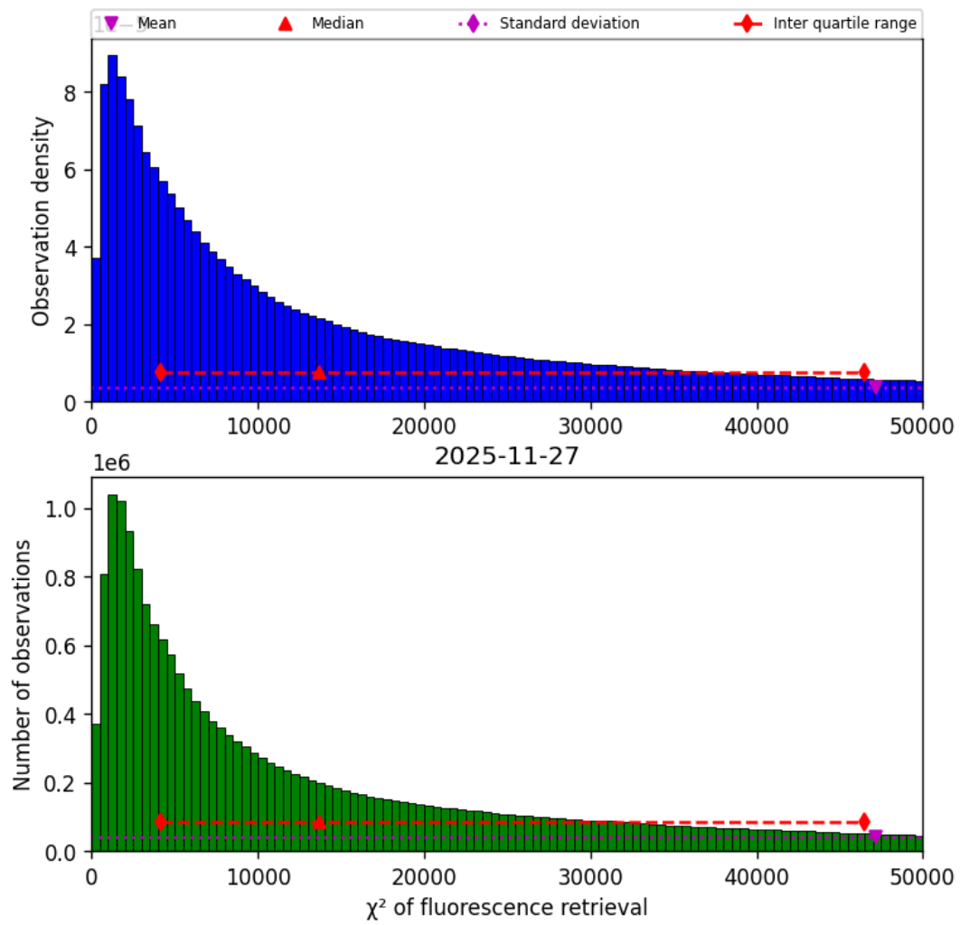
Figure 42: Histogram of “ \chi^2 of fluorescence retrieval” for 2025-11-26 to 2025-11-28
