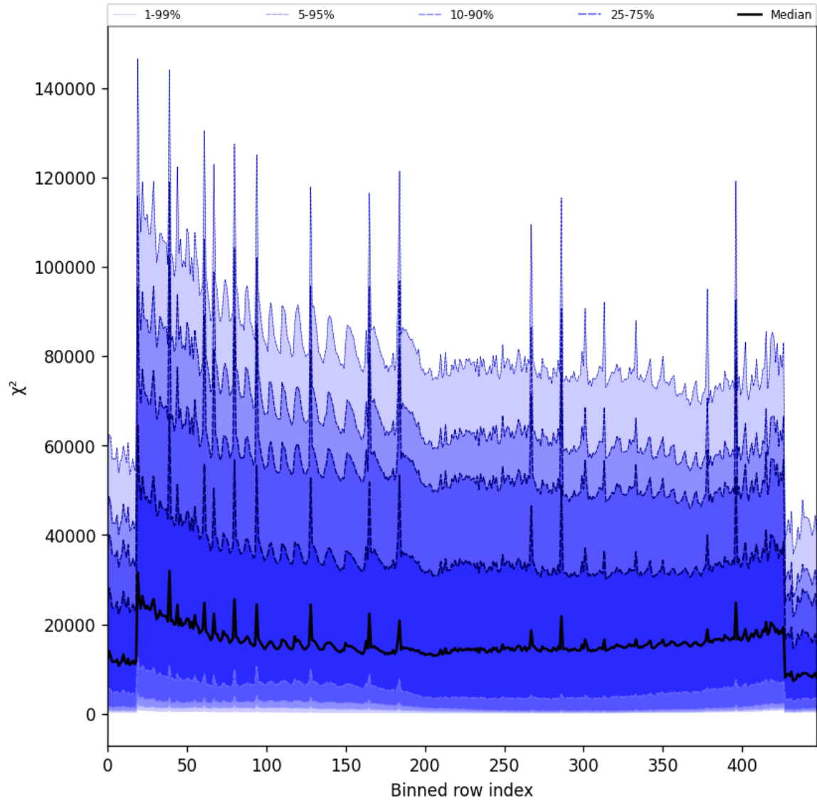
Figure 55: Along track statistics of “ \chi^2 ” for 2025-11-26 to 2025-11-28
