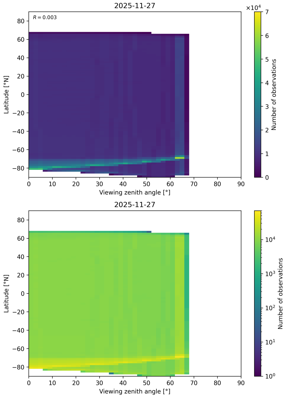
Figure 123: Scatter density plot of “Viewing zenith angle” against “Latitude” for 2025-11-26 to 2025-11-28.
