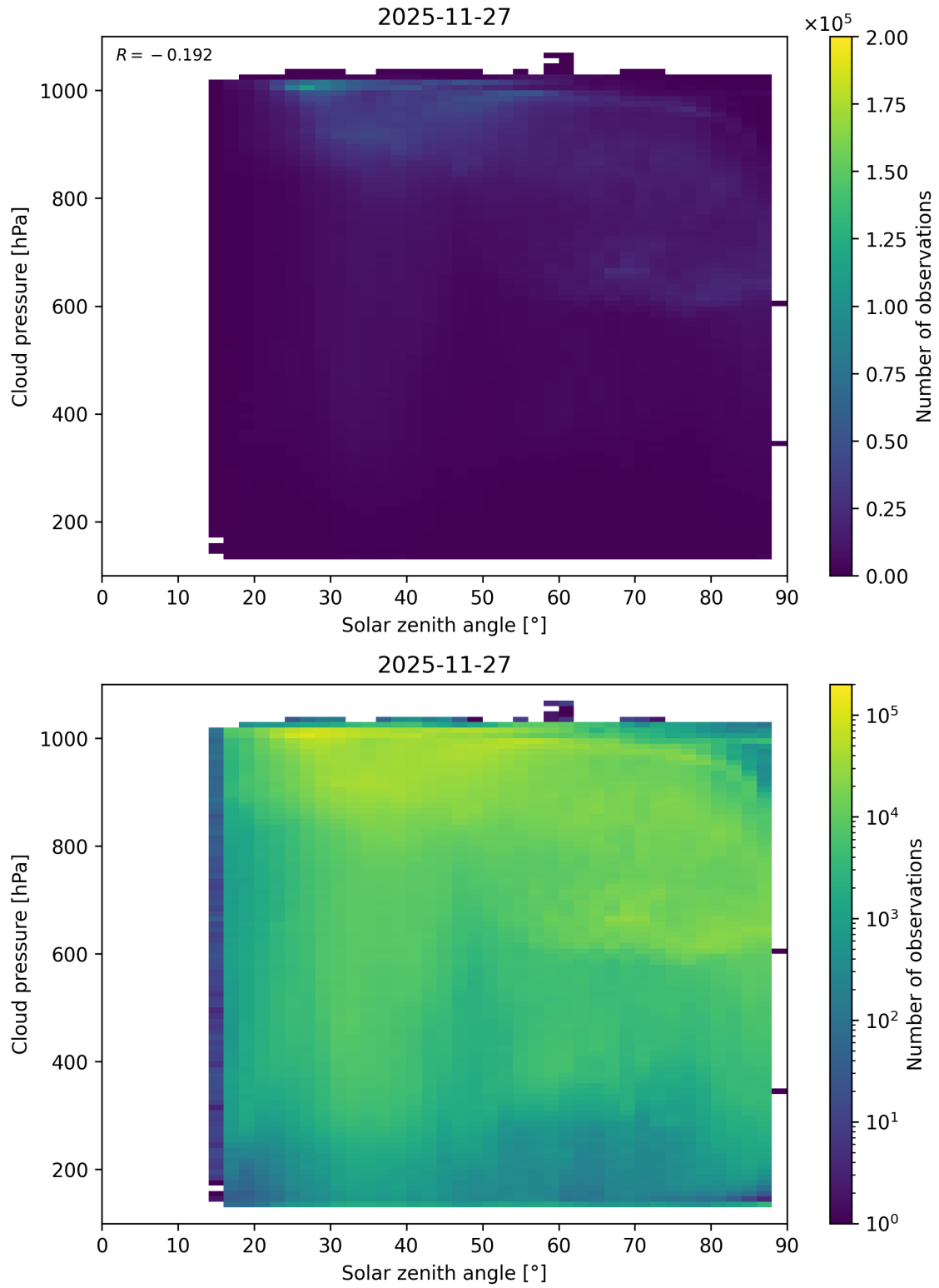
Figure 111: Scatter density plot of “Solar zenith angle” against “Cloud pressure” for 2025-11-26 to 2025-11-28.
