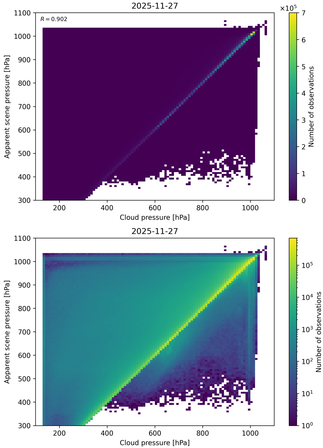
Figure 77: Scatter density plot of “Cloud pressure” against “Apparent scene pressure” for 2025-11-26 to 2025-11-28.
