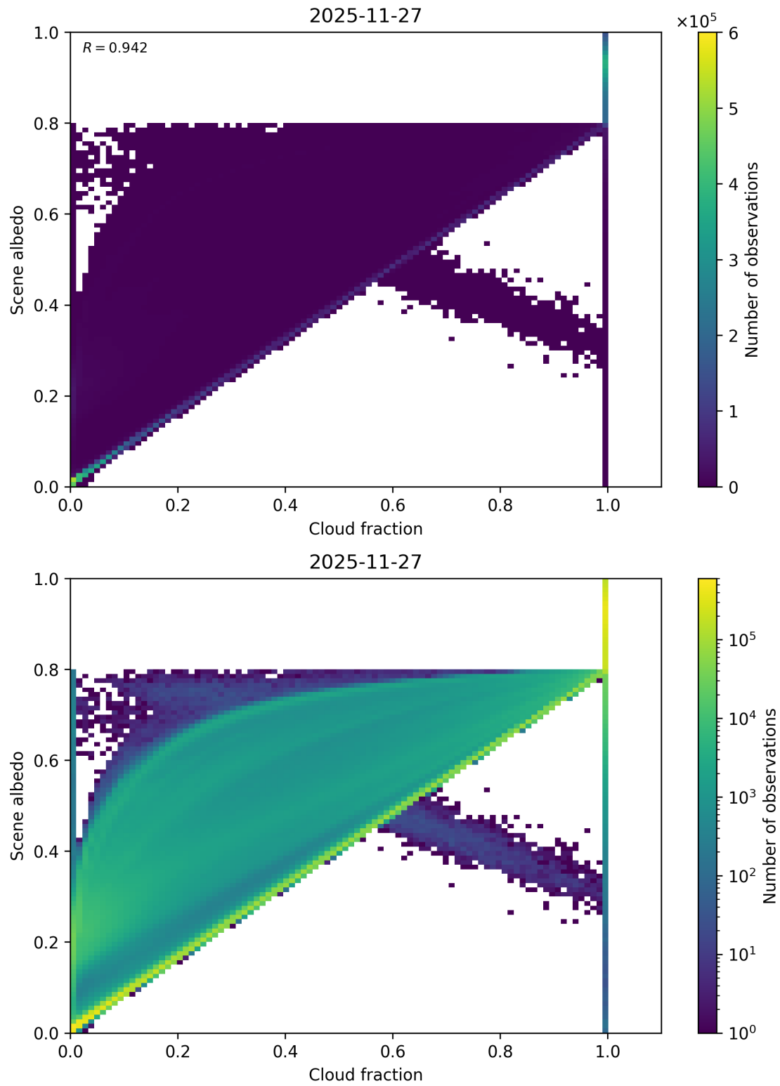
Figure 75: Scatter density plot of “Cloud fraction” against “Scene albedo” for 2025-11-26 to 2025-11-28.
