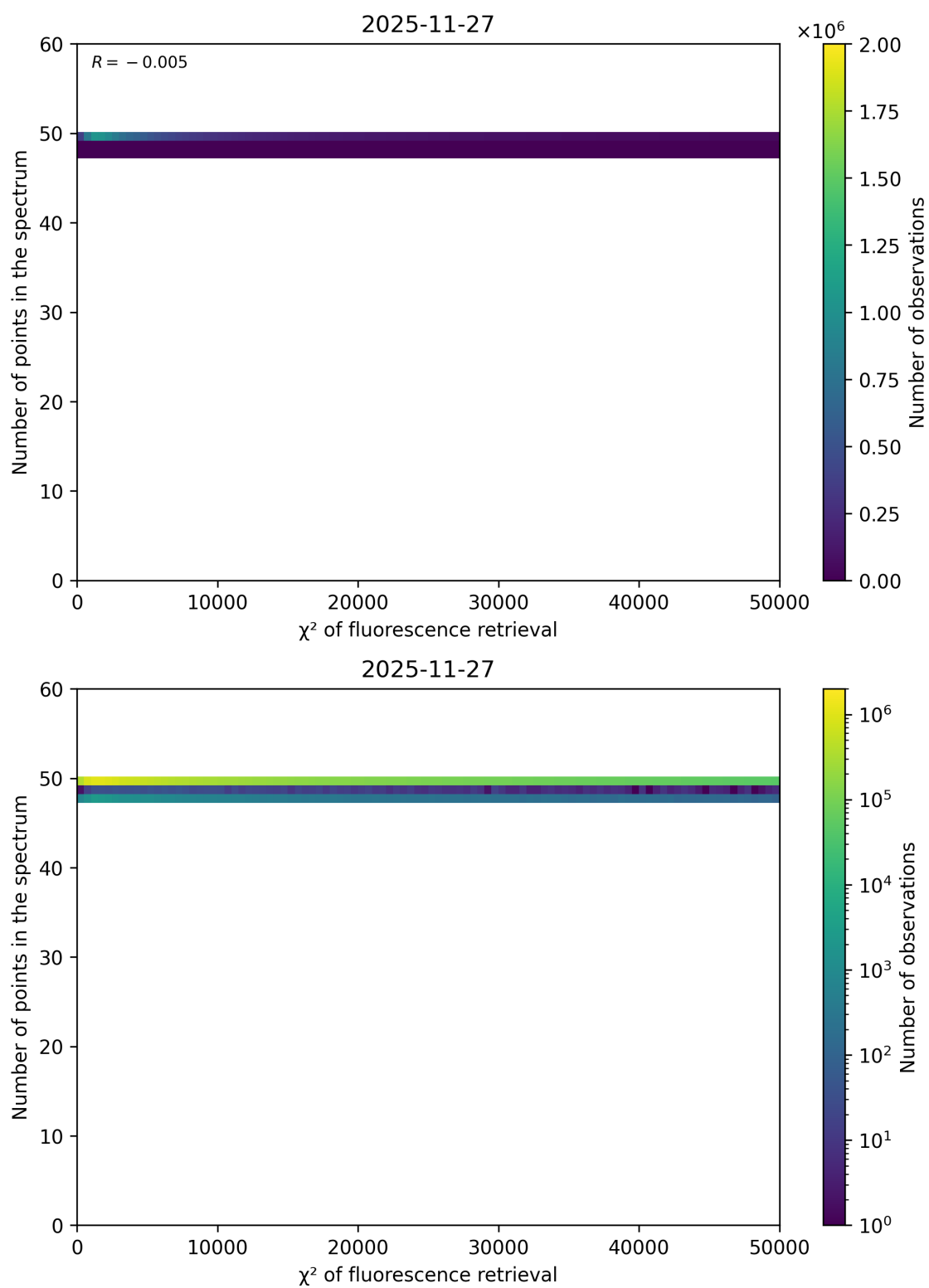
Figure 68: Scatter density plot of " \chi^2 of fluorescence retrieval" against "Number of points in the spectrum" for 2025-11-26 to 2025-11-28.
