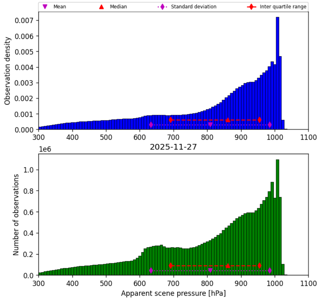
Figure 36: Histogram of “Apparent scene pressure” for 2025-11-26 to 2025-11-28
