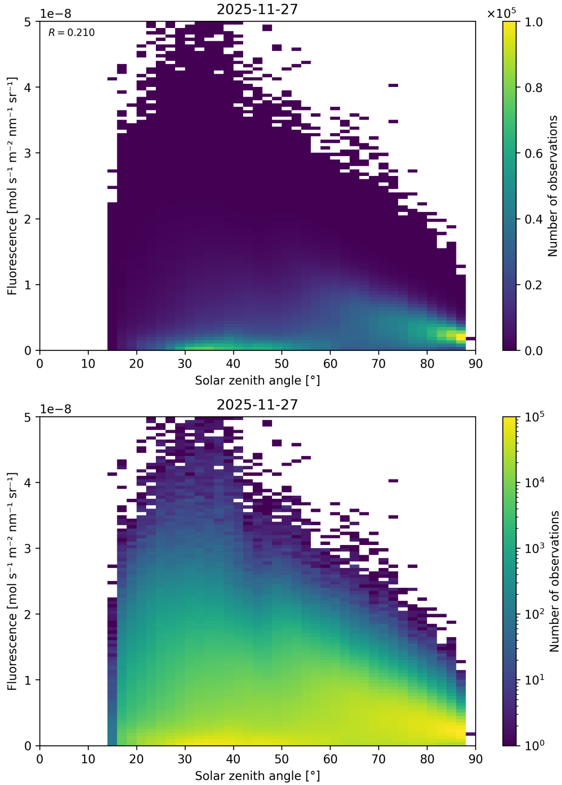
Figure 112: Scatter density plot of “Solar zenith angle” against “Fluorescence” for 2025-11-26 to 2025-11-28.
