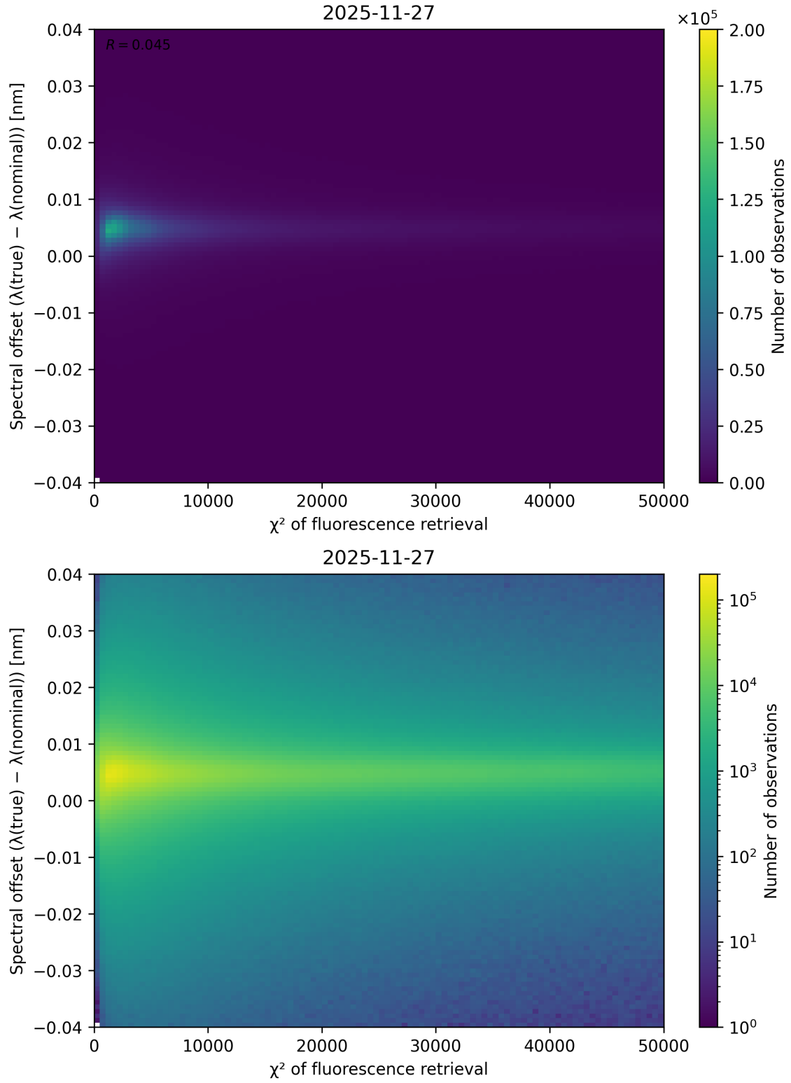
Figure 69: Scatter density plot of “ \chi^2 of fluorescence retrieval” against “Spectral offset ( \lambda_{\text{true}} - \lambda_{\text{nominal}} )” for 2025-11-26 to 2025-11-28.
