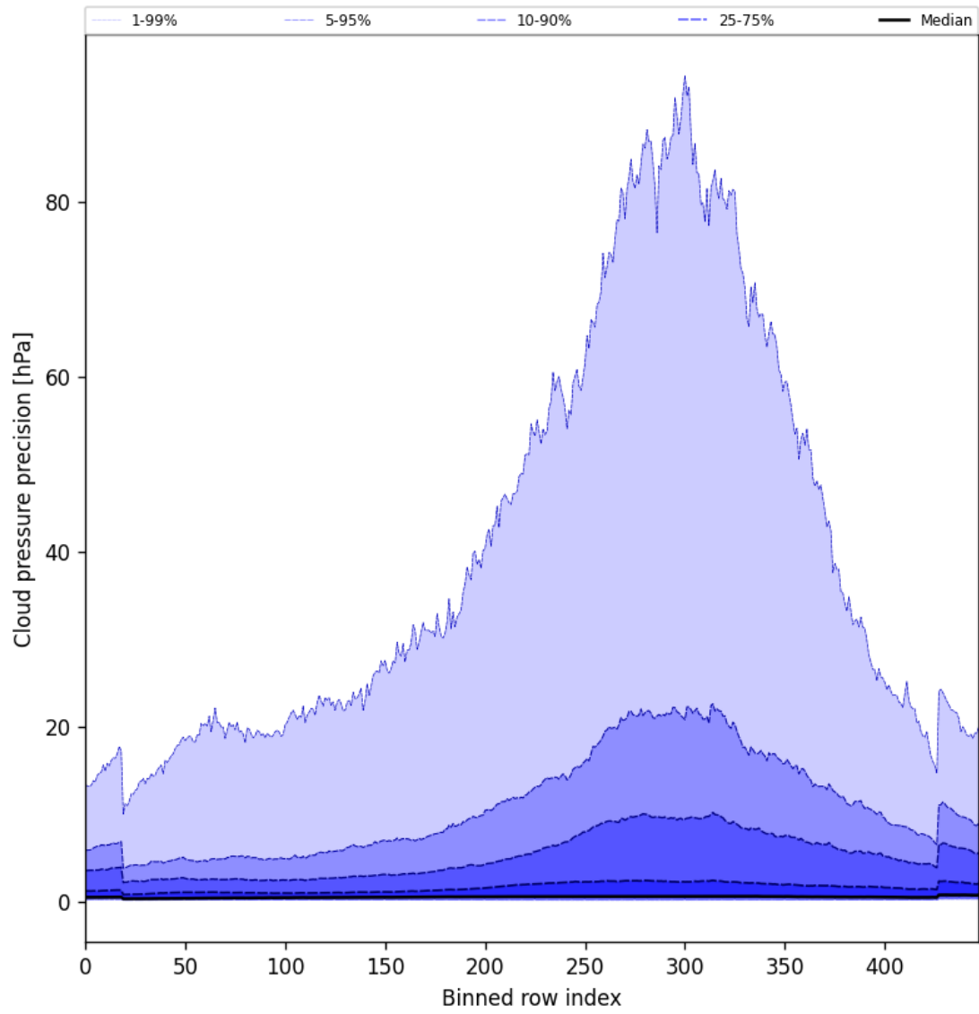
Figure 48: Along track statistics of “Cloud pressure precision” for 2025-11-26 to 2025-11-28
