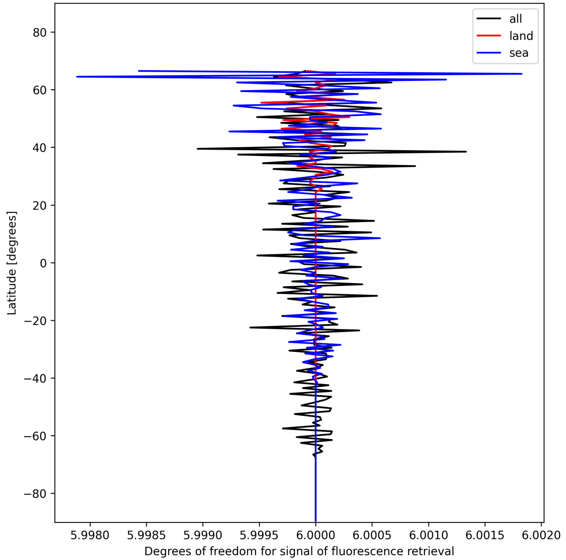
Figure 26: Zonal average of “Degrees of freedom for signal of fluorescence retrieval” for 2025-11-26 to 2025-11-28.
