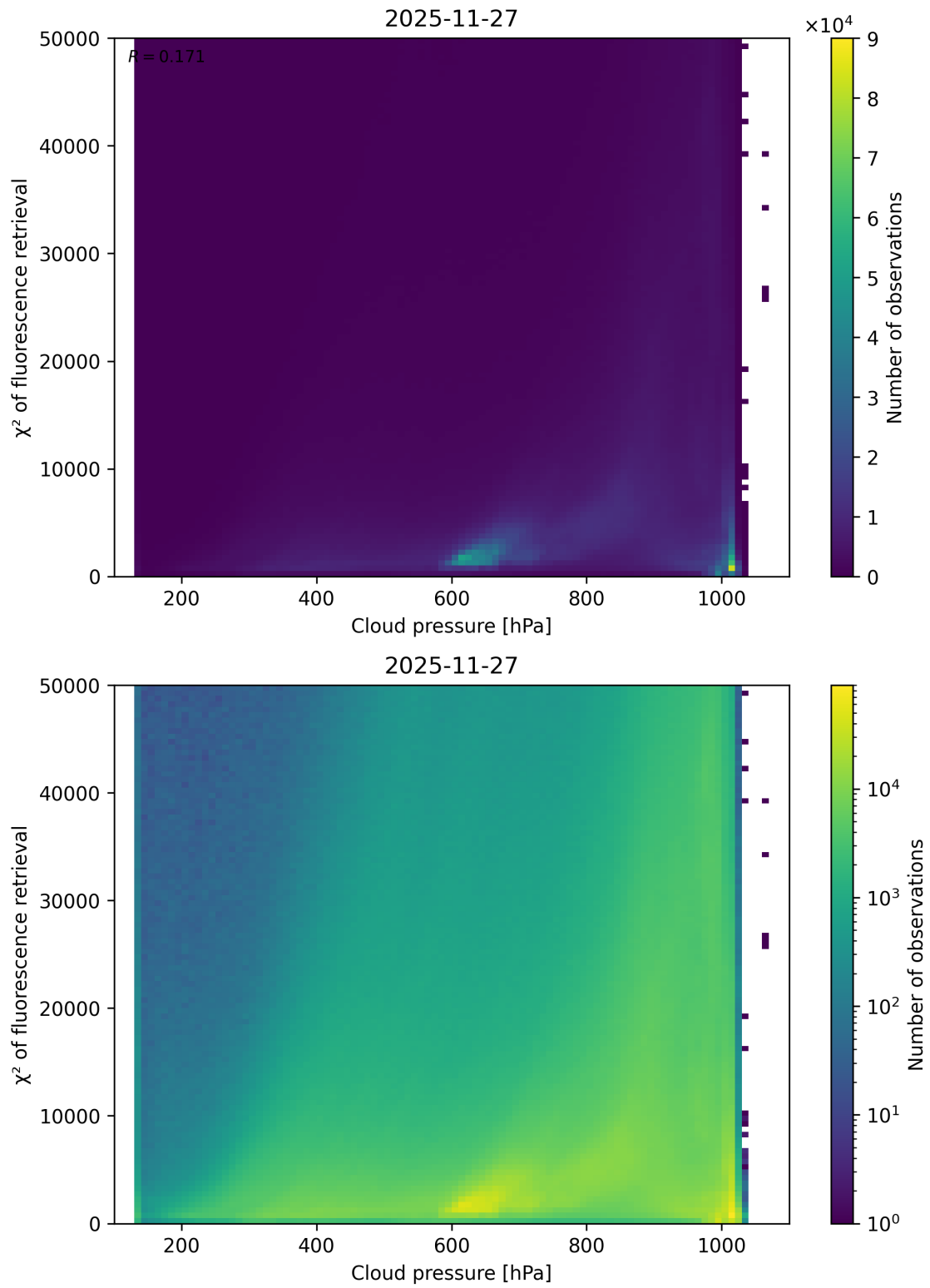
Figure 78: Scatter density plot of “Cloud pressure” against “ \chi^2 of fluorescence retrieval” for 2025-11-26 to 2025-11-28.
