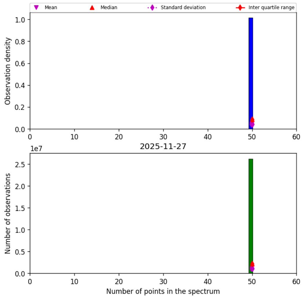
Figure 44: Histogram of "Number of points in the spectrum" for 2025-11-26 to 2025-11-28
