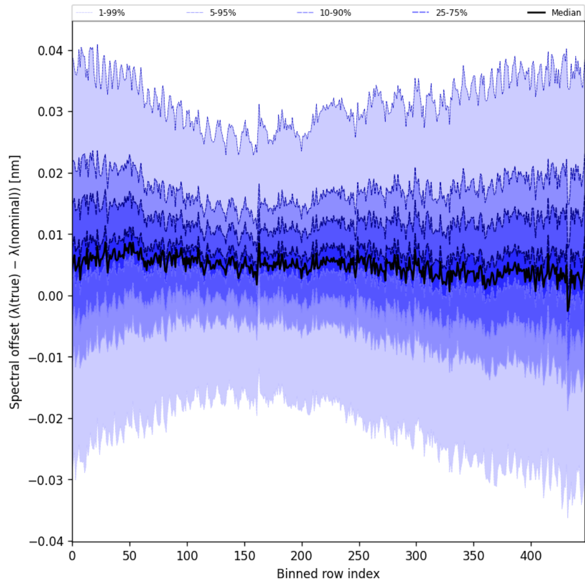
Figure 62: Along track statistics of “Spectral offset ( \lambda_{\text{true}} - \lambda_{\text{nominal}} )” for 2025-11-26 to 2025-11-28
