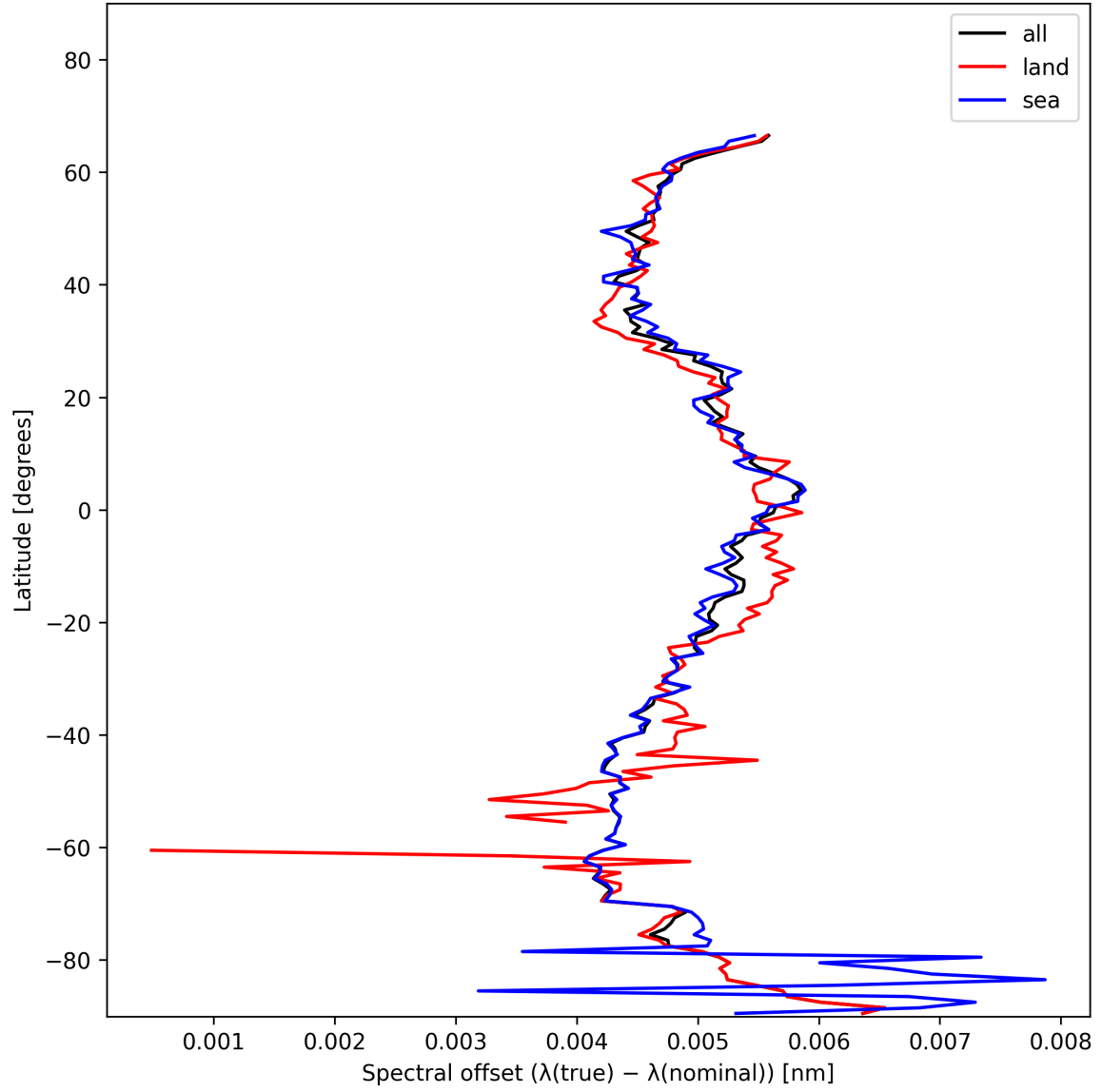
Figure 28: Zonal average of “Spectral offset ( \lambda_{\text{true}} - \lambda_{\text{nominal}} )” for 2025-11-26 to 2025-11-28.
