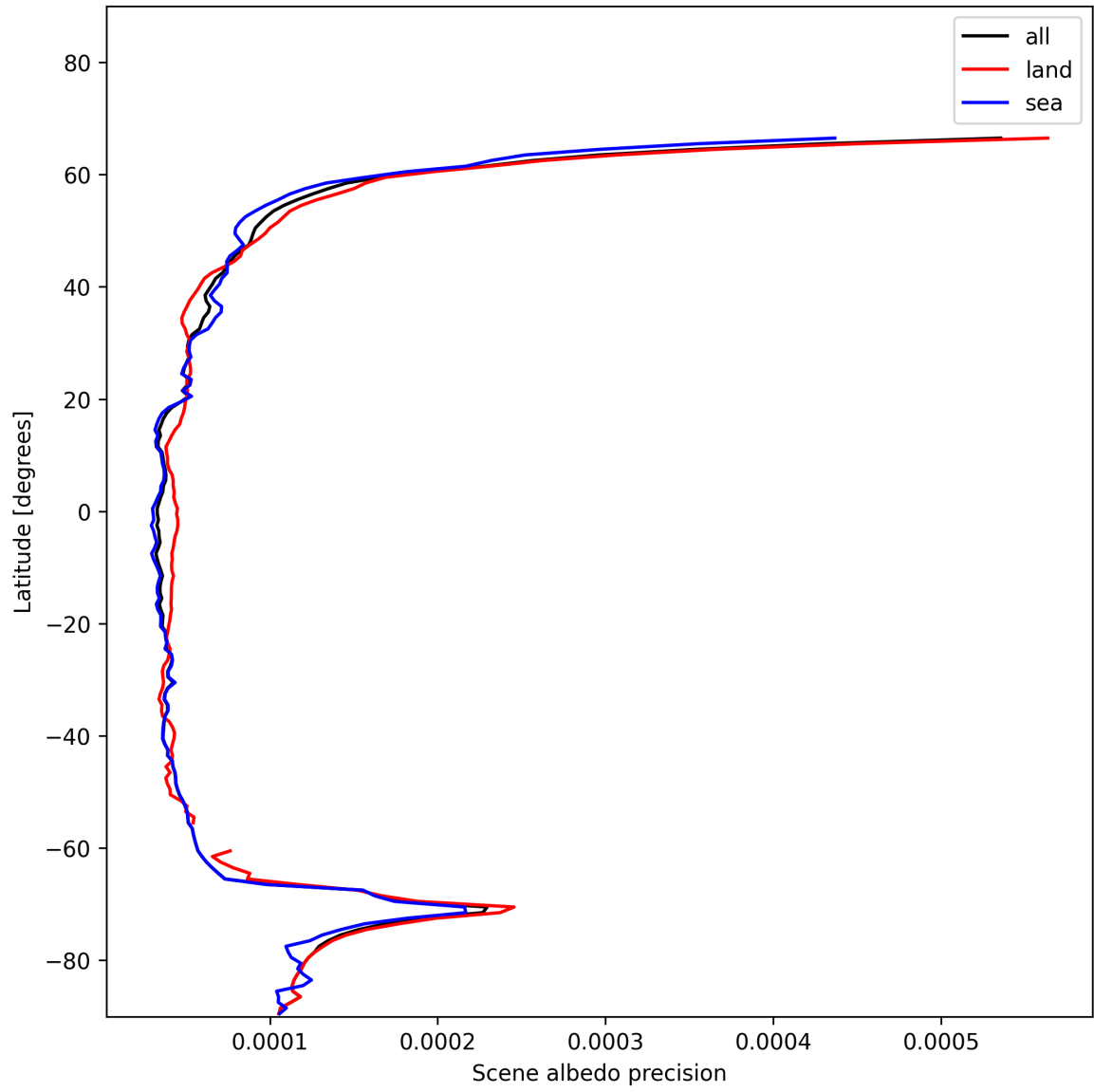
Figure 18: Zonal average of “Scene albedo precision” for 2025-11-26 to 2025-11-28.
