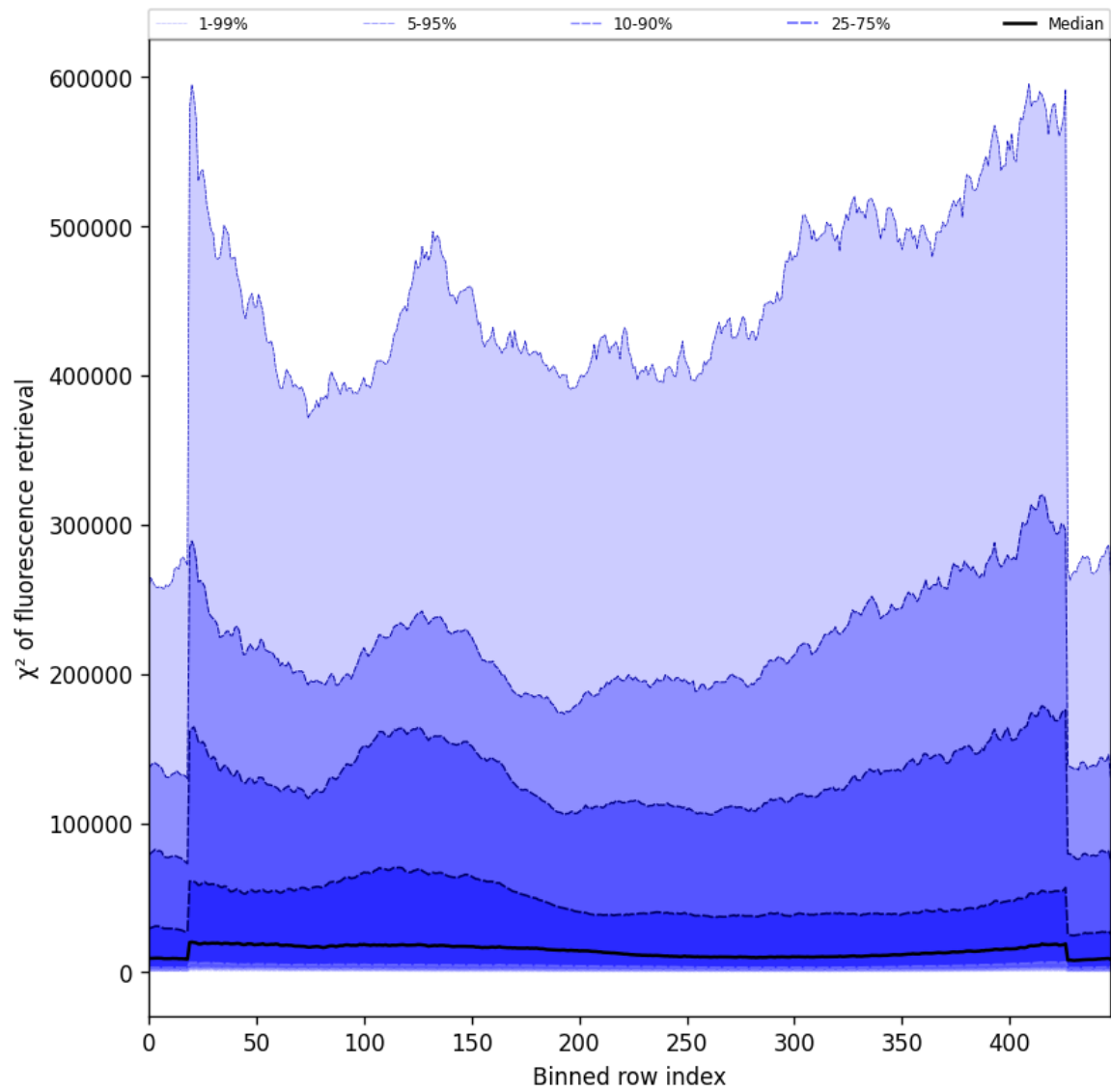
Figure 59: Along track statistics of “ \chi^2 of fluorescence retrieval” for 2025-11-26 to 2025-11-28
