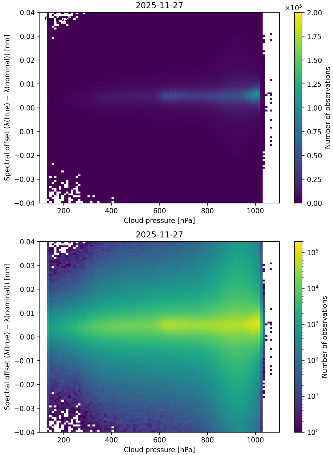
Figure 84: Scatter density plot of “Cloud pressure” against “Spectral offset ( \lambda_{\text{true}} - \lambda_{\text{nominal}} )” for 2025-11-26 to 2025-11-28.
