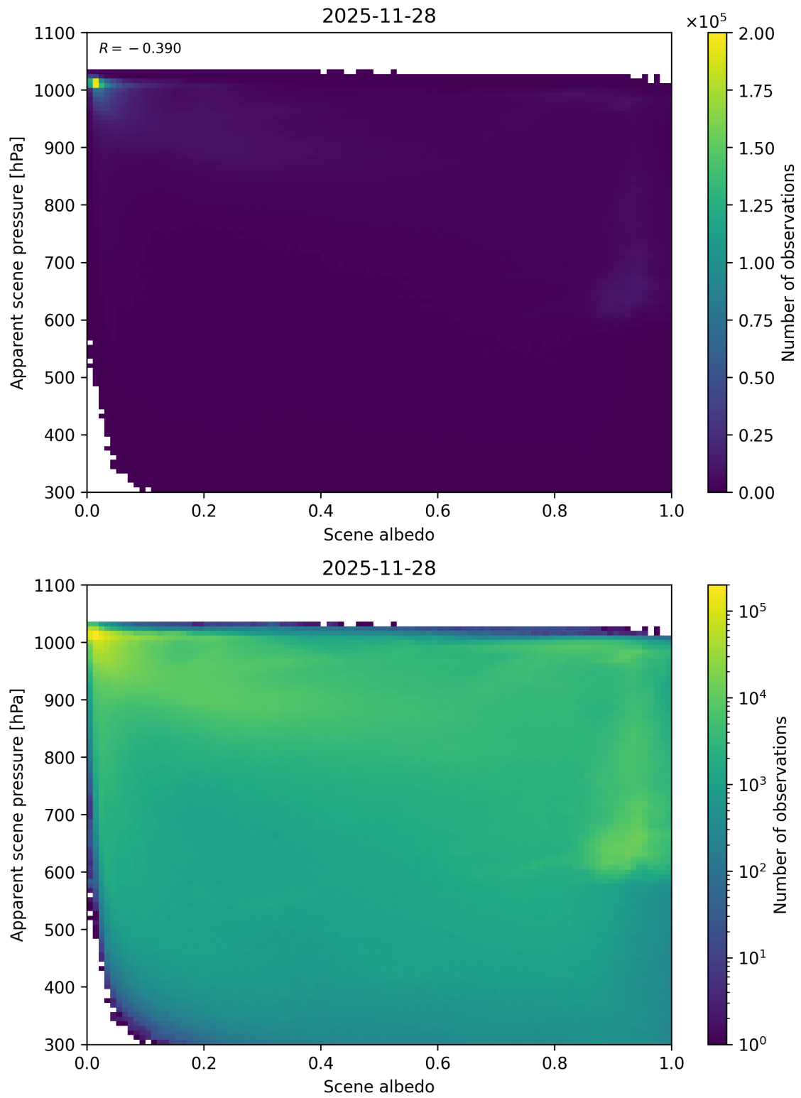
Figure 102: Scatter density plot of “Scene albedo” against “Apparent scene pressure” for 2025-11-28 to 2025-11-29.
