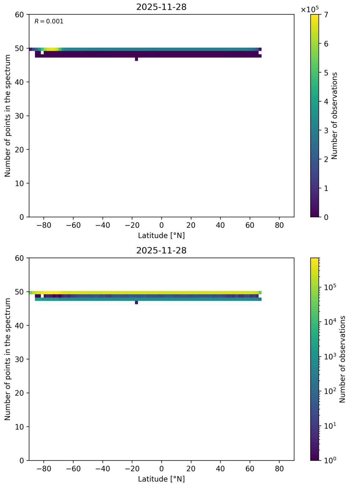
Figure 94: Scatter density plot of “Latitude” against “Number of points in the spectrum” for 2025-11-28 to 2025-11-29.
