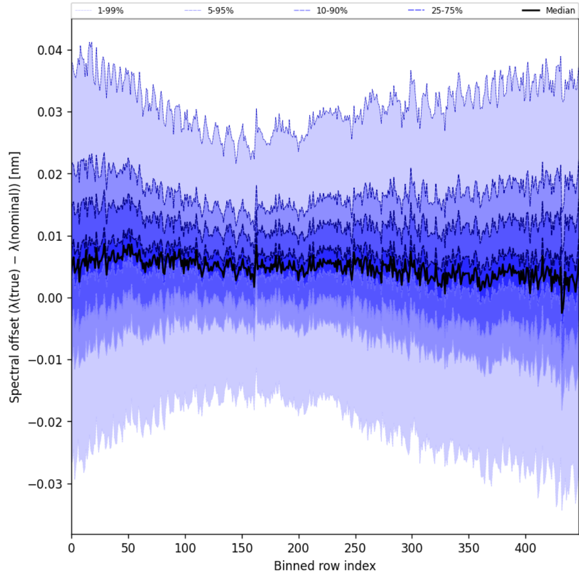
Figure 62: Along track statistics of “Spectral offset ( \lambda_{\text{true}} - \lambda_{\text{nominal}} )” for 2025-11-28 to 2025-11-29
