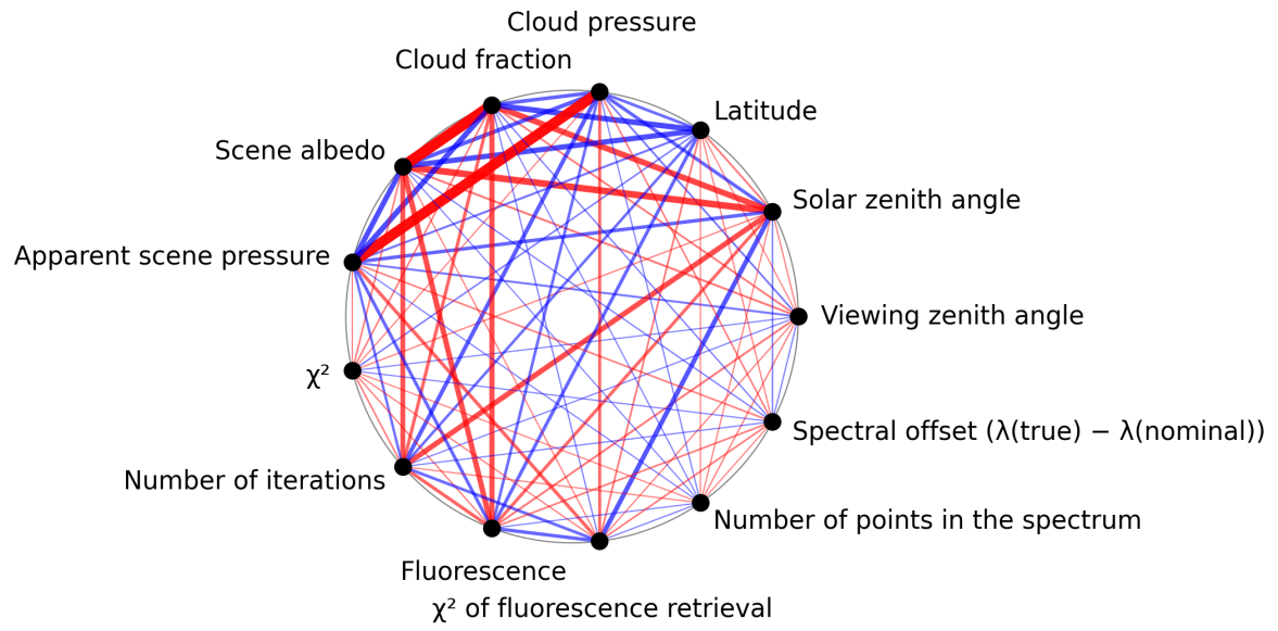
Figure 1: Map of correlation graph for 2025-11-28 to 2025-11-29.
