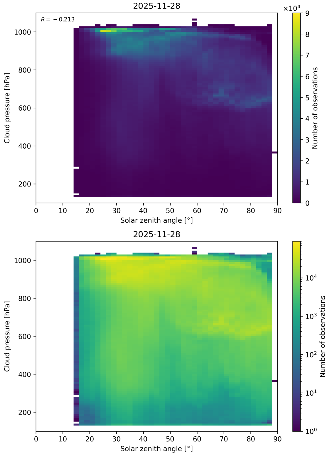
Figure 111: Scatter density plot of “Solar zenith angle” against “Cloud pressure” for 2025-11-28 to 2025-11-29.
