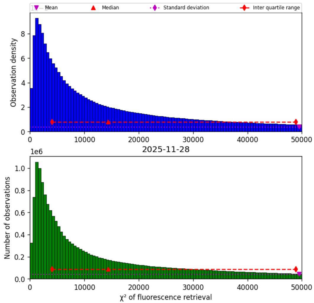
Figure 42: Histogram of “ \chi^2 of fluorescence retrieval” for 2025-11-28 to 2025-11-29
