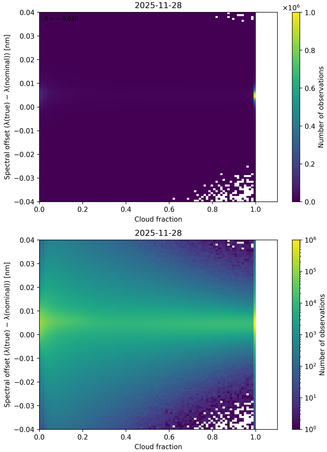
Figure 76: Scatter density plot of “Cloud fraction” against “Spectral offset ( \lambda_{\text{true}} - \lambda_{\text{nominal}} )” for 2025-11-28 to 2025-11-29.
