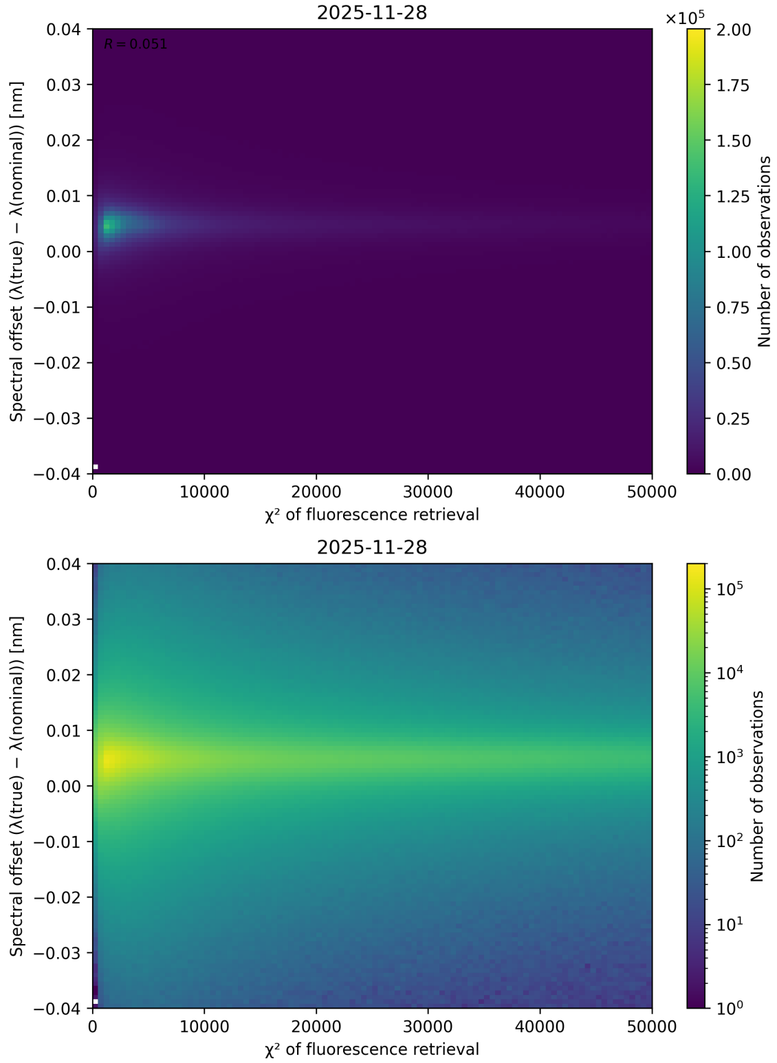
Figure 69: Scatter density plot of “ \chi^2 of fluorescence retrieval” against “Spectral offset ( \lambda_{\text{true}} - \lambda_{\text{nominal}} )” for 2025-11-28 to 2025-11-29.
