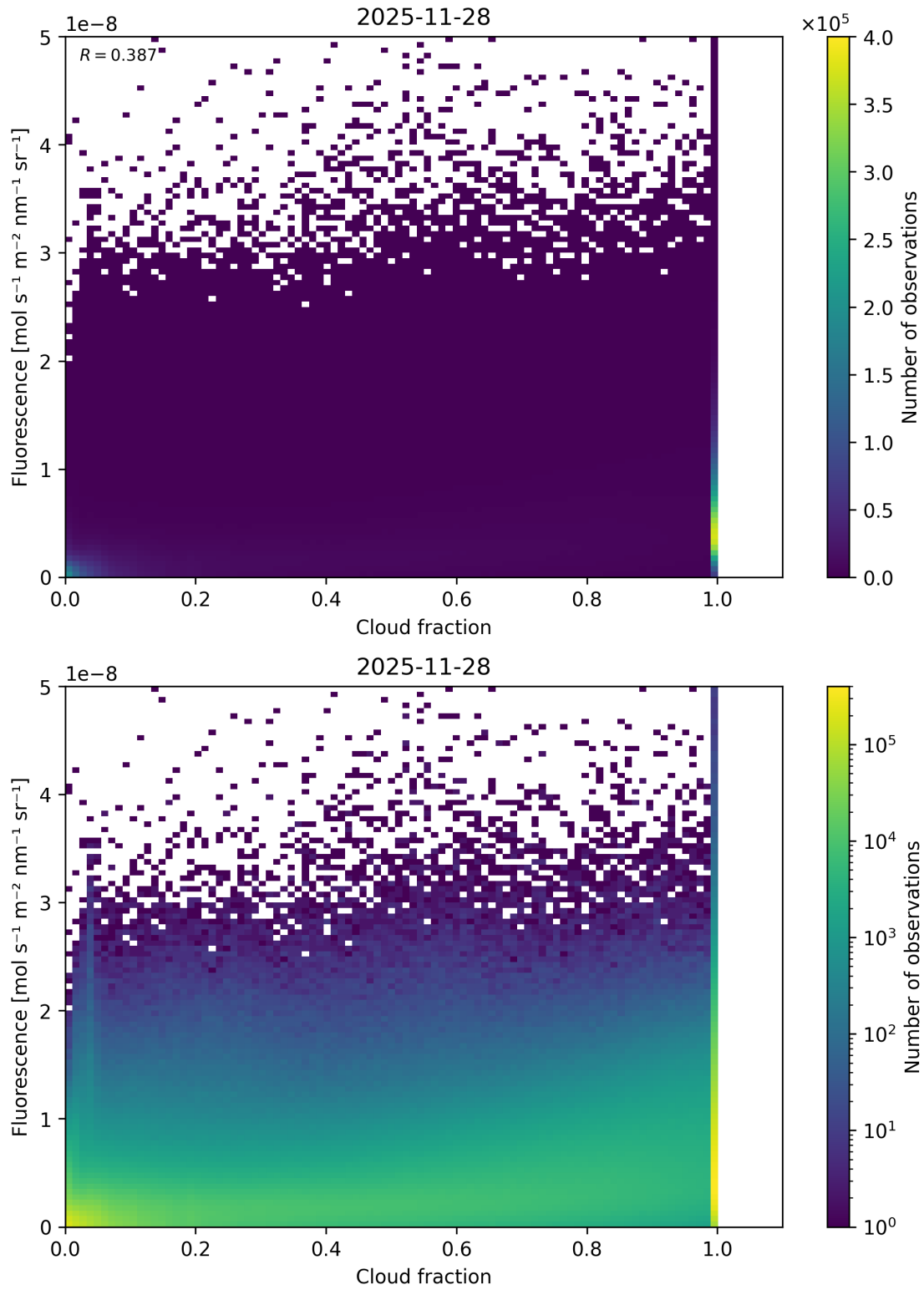
Figure 72: Scatter density plot of “Cloud fraction” against “Fluorescence” for 2025-11-28 to 2025-11-29.
