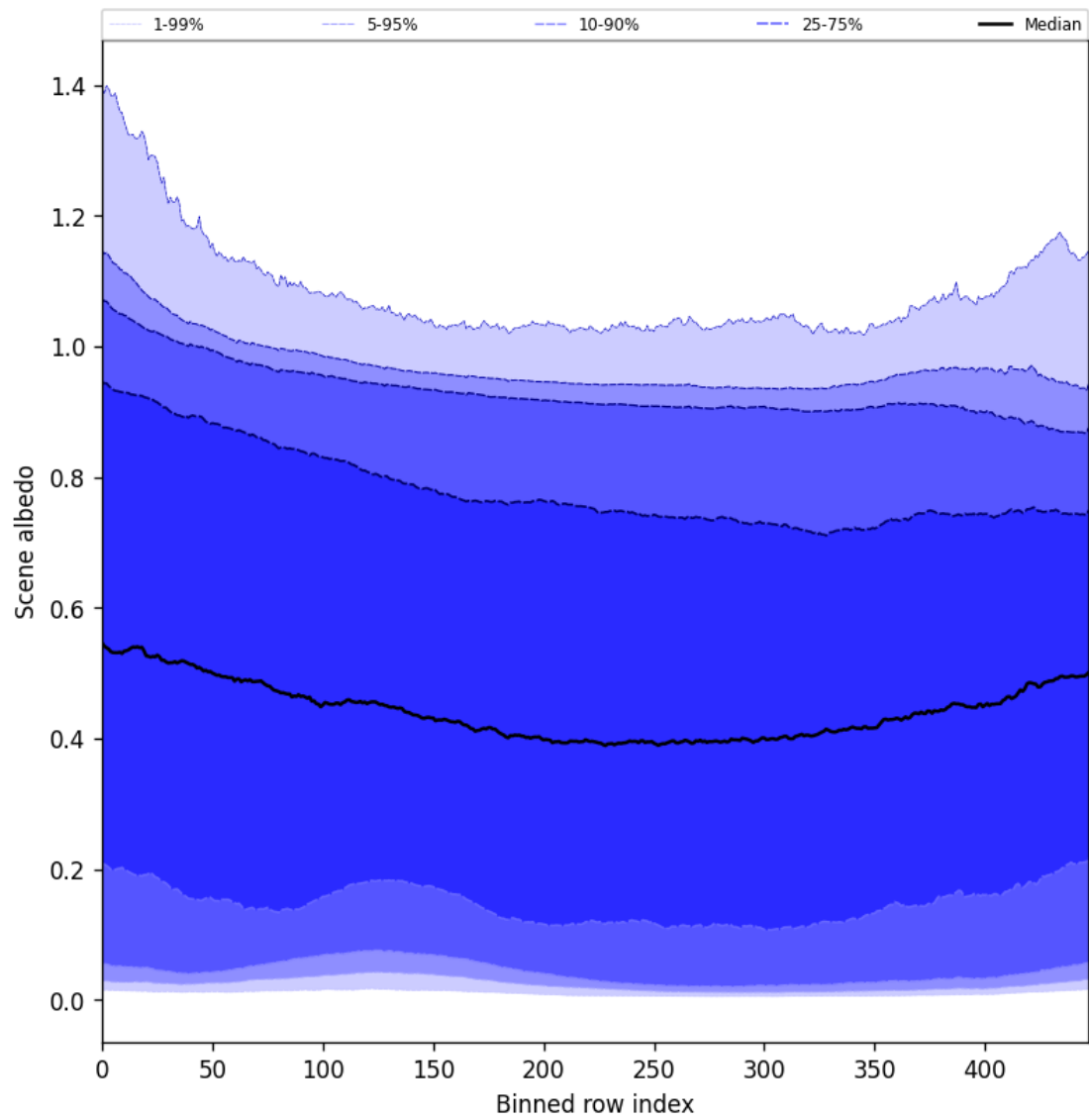
Figure 51: Along track statistics of “Scene albedo” for 2025-11-28 to 2025-11-29
