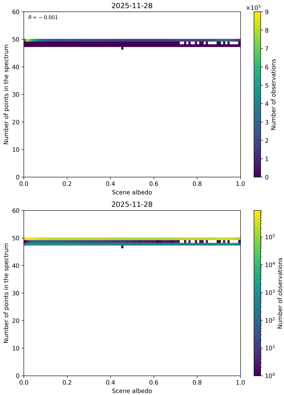
Figure 106: Scatter density plot of “Scene albedo” against “Number of points in the spectrum” for 2025-11-28 to 2025-11-29.
