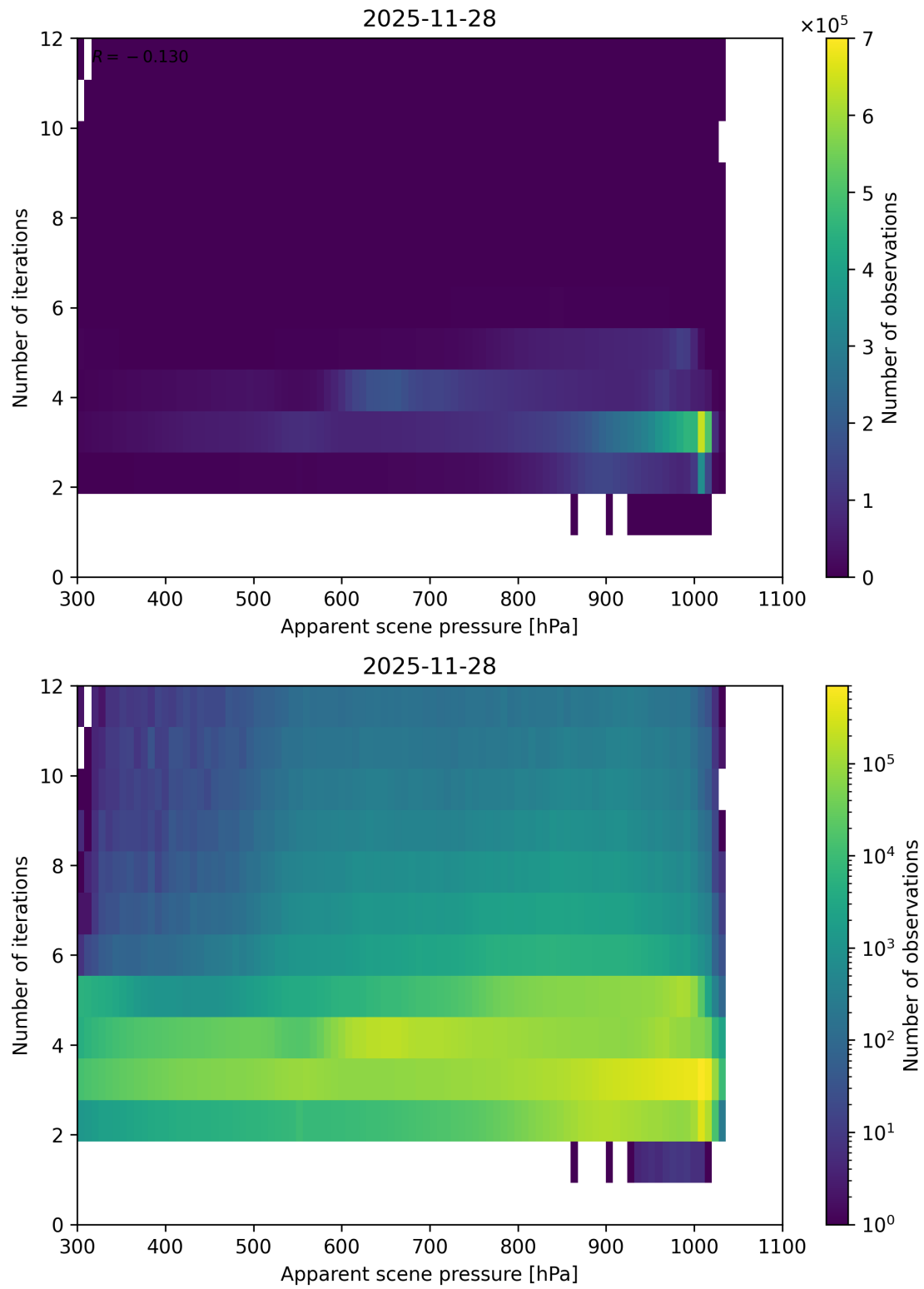
Figure 65: Scatter density plot of “Apparent scene pressure” against “Number of iterations” for 2025-11-28 to 2025-11-29.
