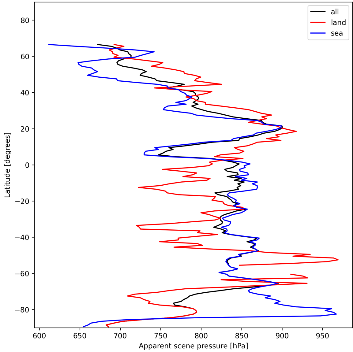
Figure 19: Zonal average of “Apparent scene pressure” for 2025-11-28 to 2025-11-29.
