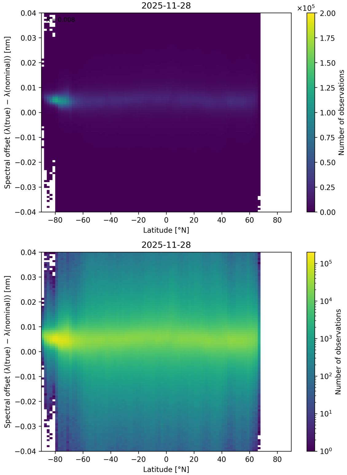
Figure 96: Scatter density plot of “Latitude” against “Spectral offset ( \lambda_{\text{true}} - \lambda_{\text{nominal}} )” for 2025-11-28 to 2025-11-29.
