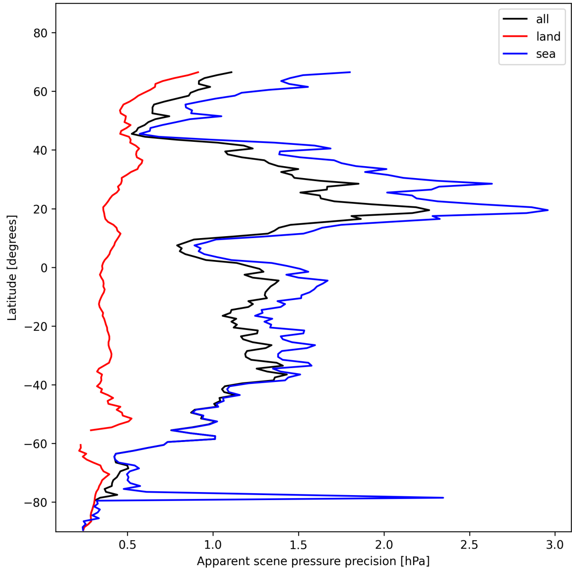
Figure 20: Zonal average of “Apparent scene pressure precision” for 2025-11-28 to 2025-11-29.
