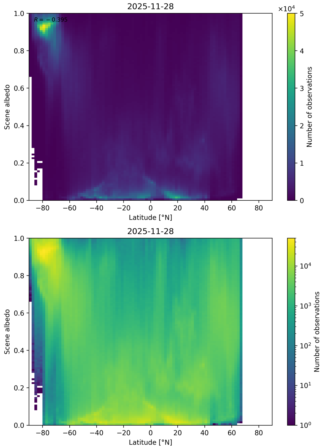
Figure 95: Scatter density plot of “Latitude” against “Scene albedo” for 2025-11-28 to 2025-11-29.
