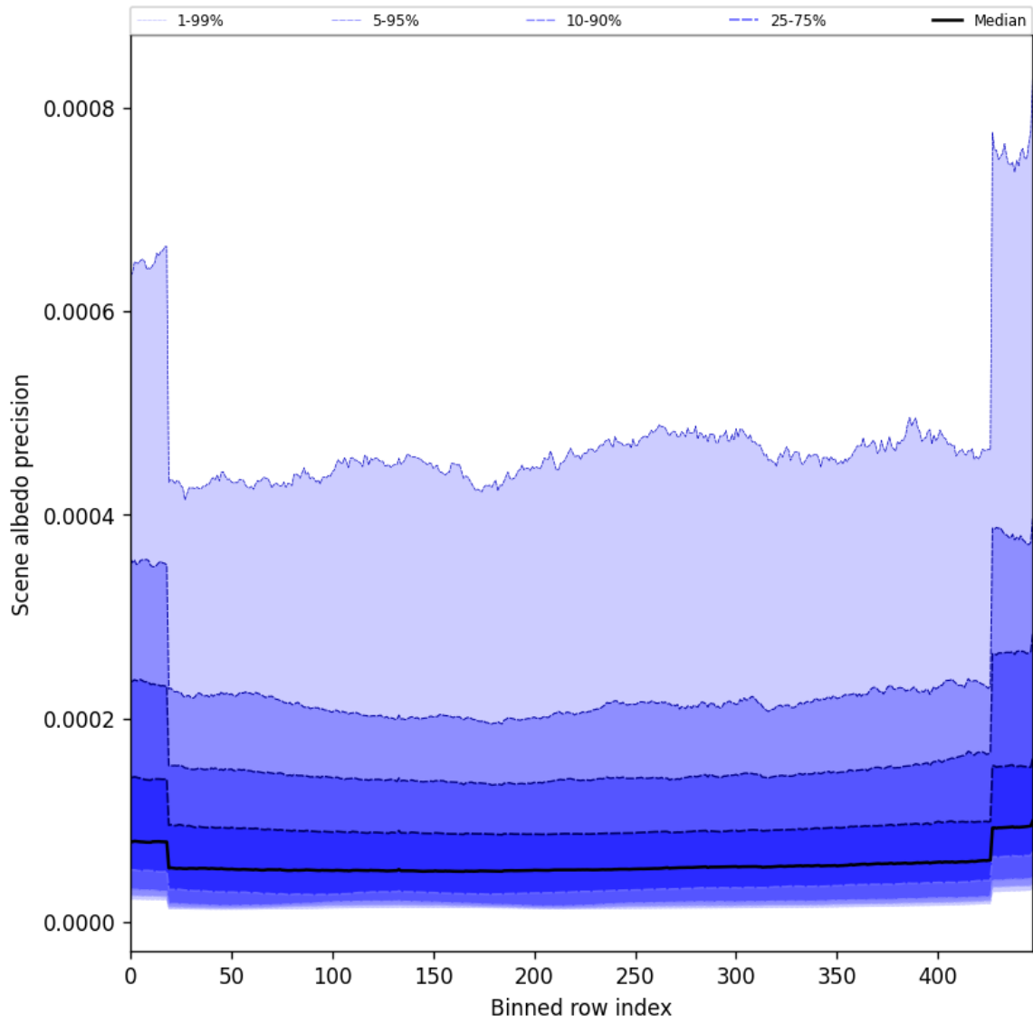
Figure 52: Along track statistics of “Scene albedo precision” for 2025-11-28 to 2025-11-29
