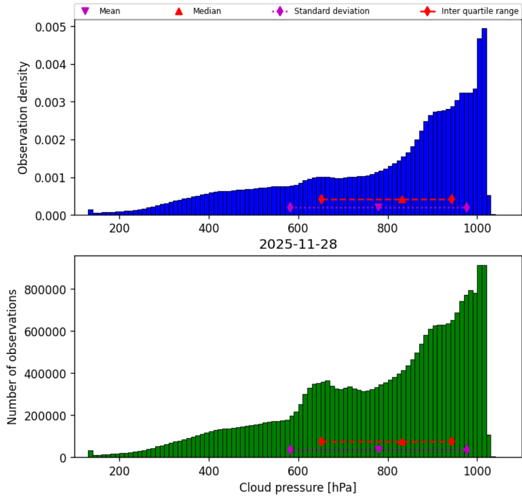
Figure 30: Histogram of “Cloud pressure” for 2025-11-28 to 2025-11-29
