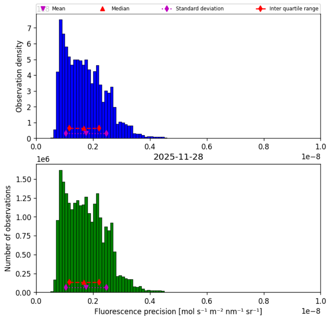
Figure 41: Histogram of “Fluorescence precision” for 2025-11-28 to 2025-11-29
