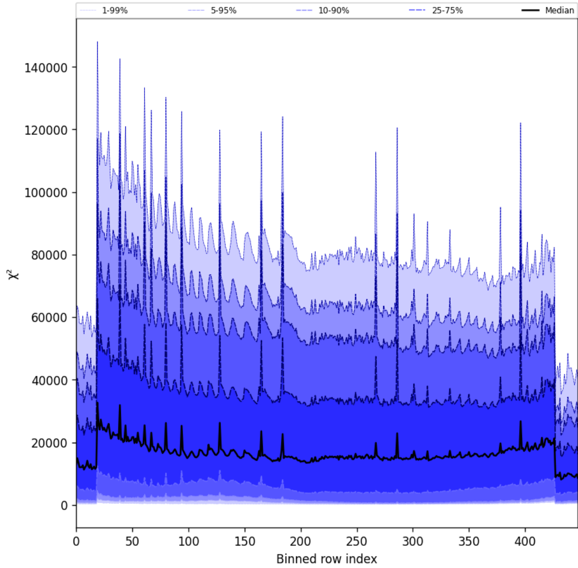
Figure 55: Along track statistics of “ \chi^2 ” for 2025-11-28 to 2025-11-29
