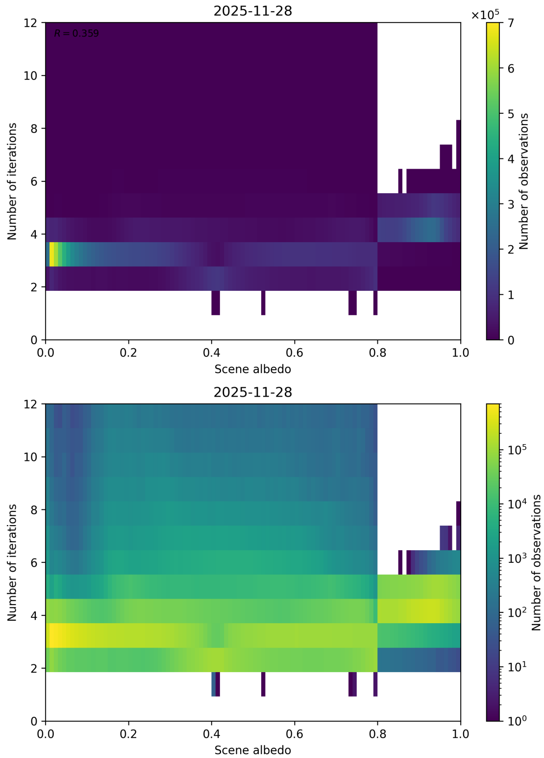
Figure 105: Scatter density plot of “Scene albedo” against “Number of iterations” for 2025-11-28 to 2025-11-29.
