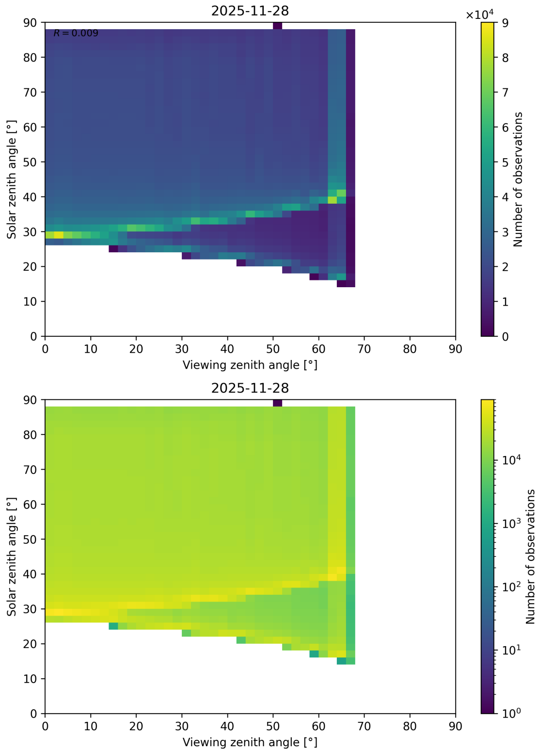
Figure 127: Scatter density plot of “Viewing zenith angle” against “Solar zenith angle” for 2025-11-28 to 2025-11-29.
