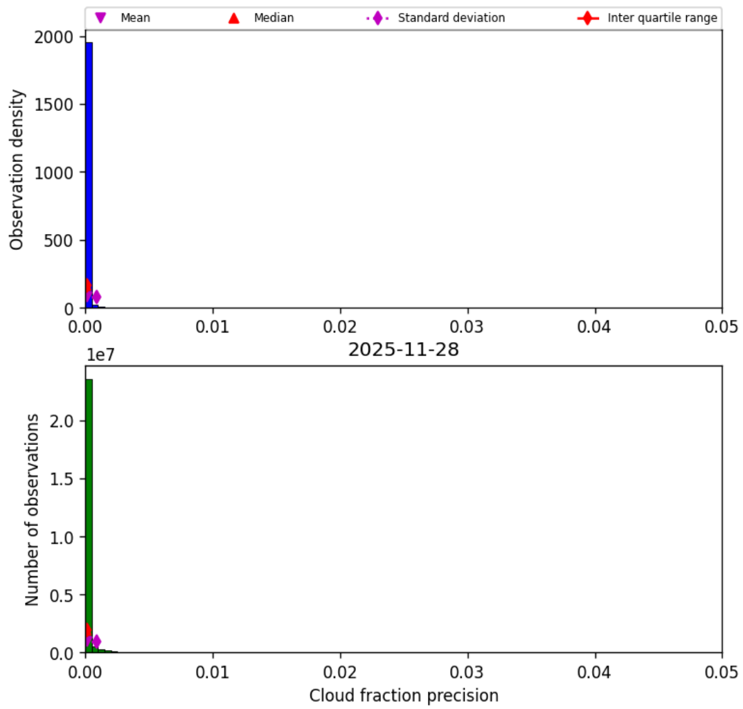
Figure 33: Histogram of “Cloud fraction precision” for 2025-11-28 to 2025-11-29
