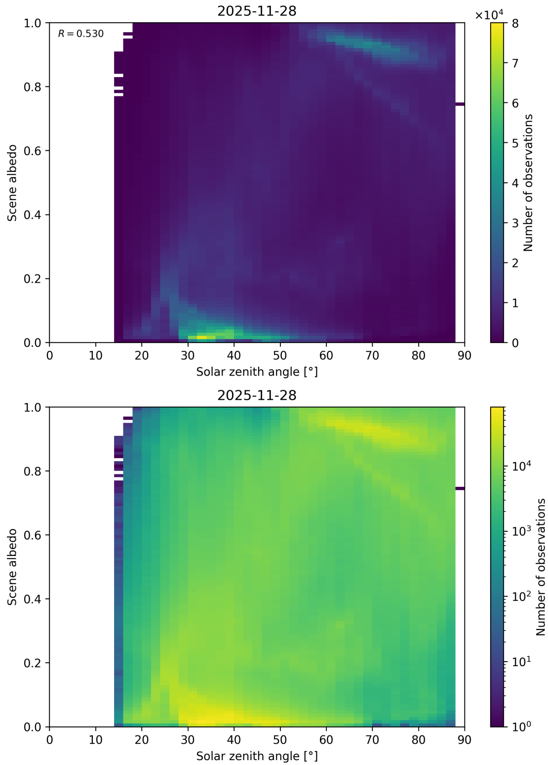
Figure 116: Scatter density plot of “Solar zenith angle” against “Scene albedo” for 2025-11-28 to 2025-11-29.
