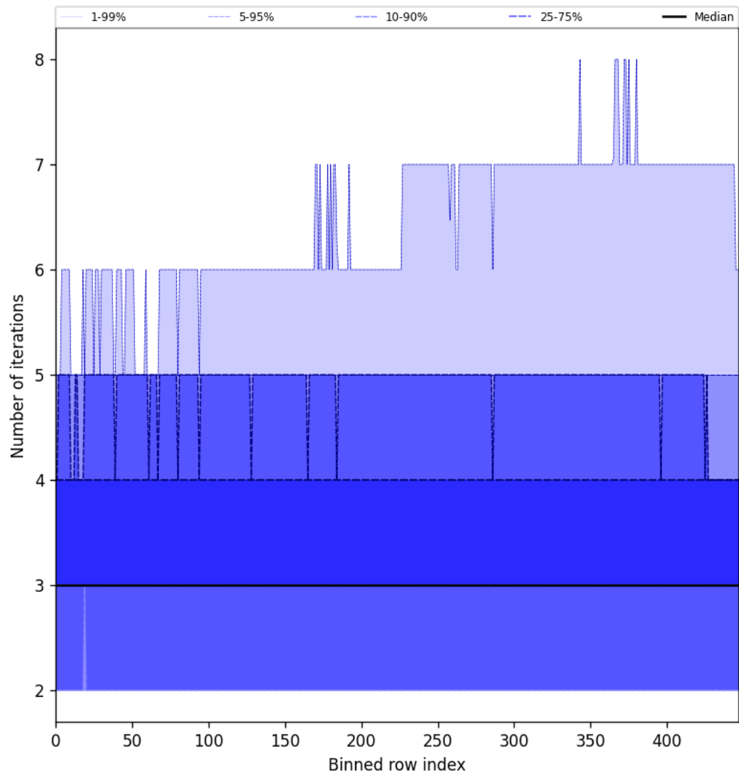
Figure 56: Along track statistics of “Number of iterations” for 2025-11-28 to 2025-11-29
