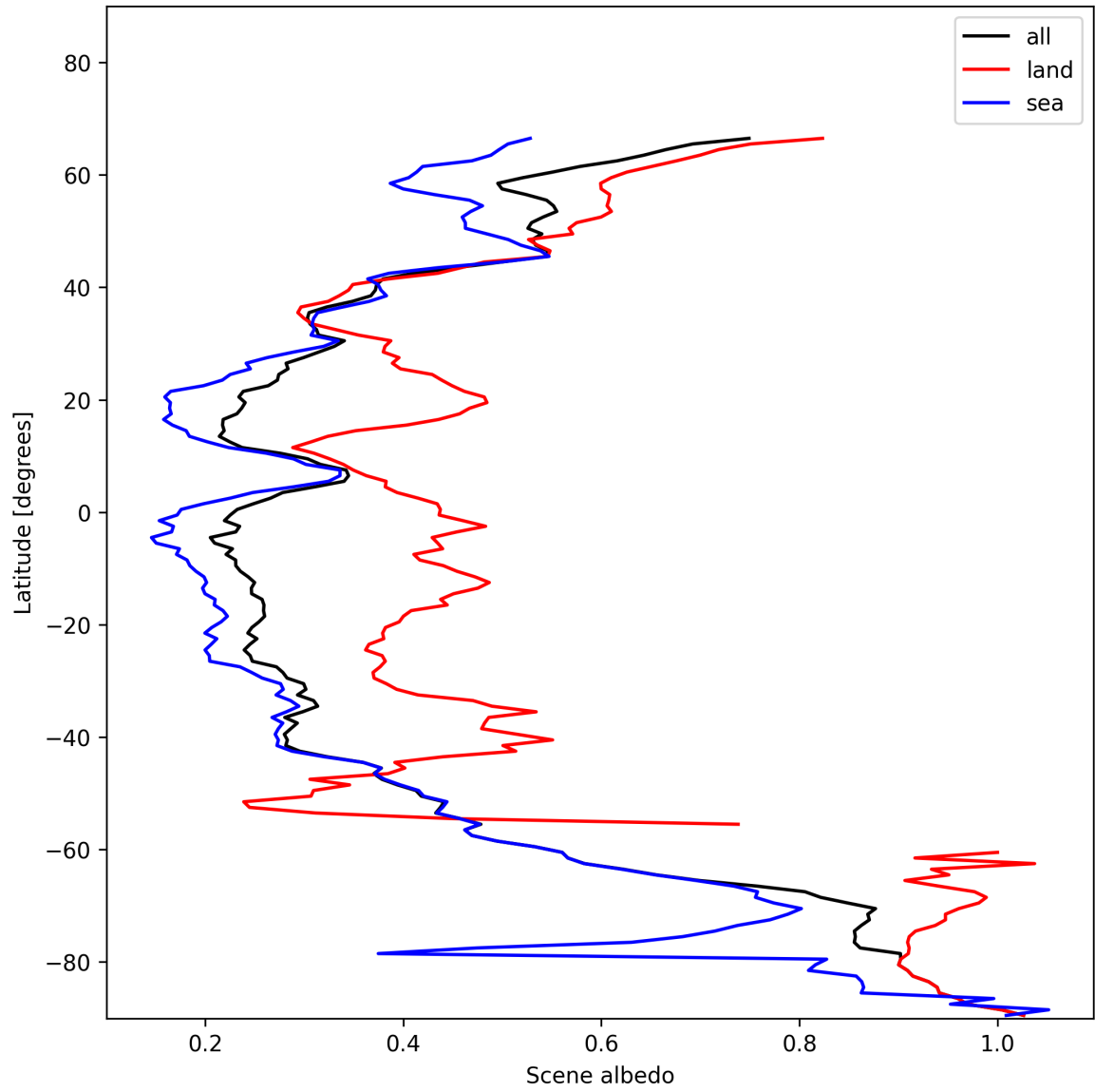
Figure 17: Zonal average of “Scene albedo” for 2025-11-28 to 2025-11-29.
