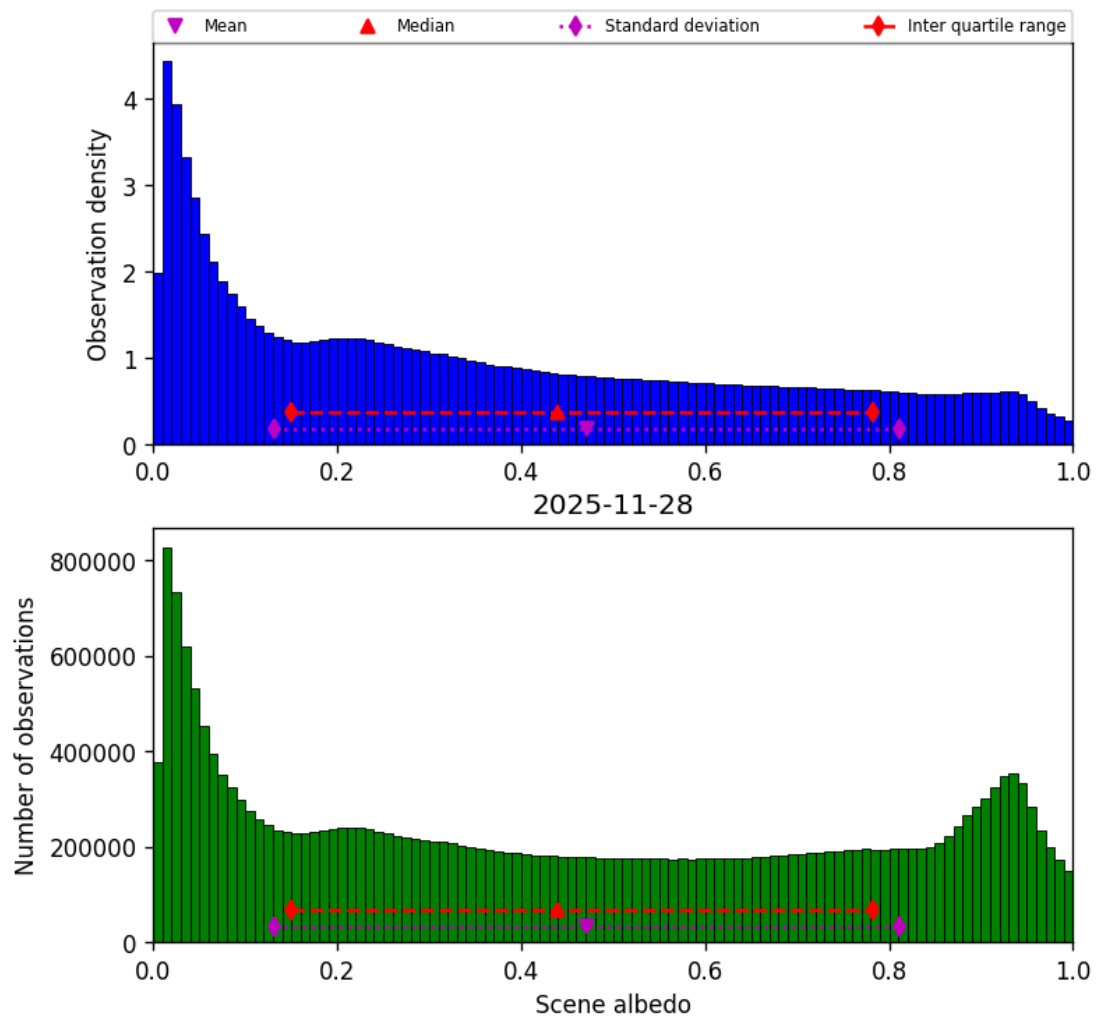
Figure 34: Histogram of “Scene albedo” for 2025-11-28 to 2025-11-29
