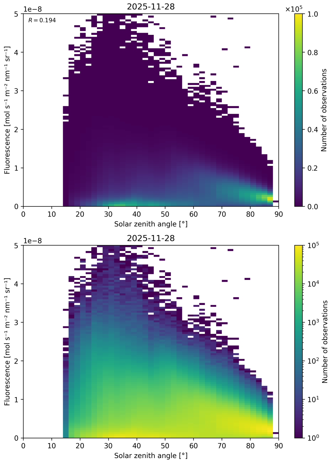
Figure 112: Scatter density plot of “Solar zenith angle” against “Fluorescence” for 2025-11-28 to 2025-11-29.
