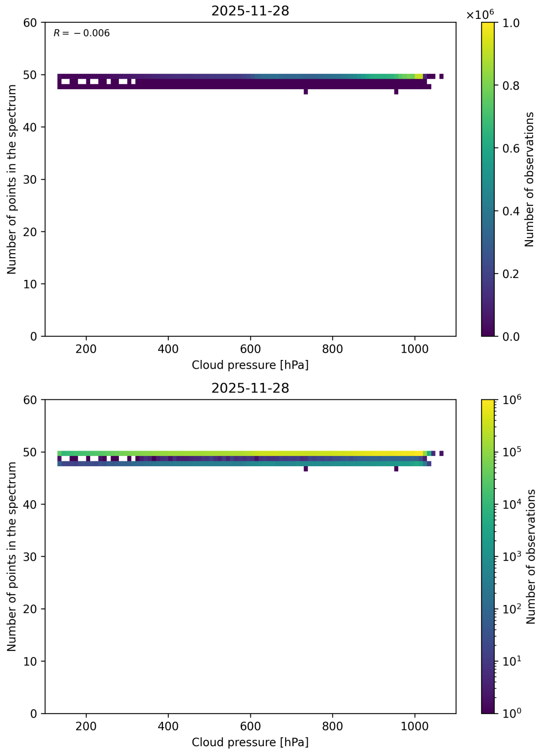
Figure 82: Scatter density plot of “Cloud pressure” against “Number of points in the spectrum” for 2025-11-28 to 2025-11-29.
