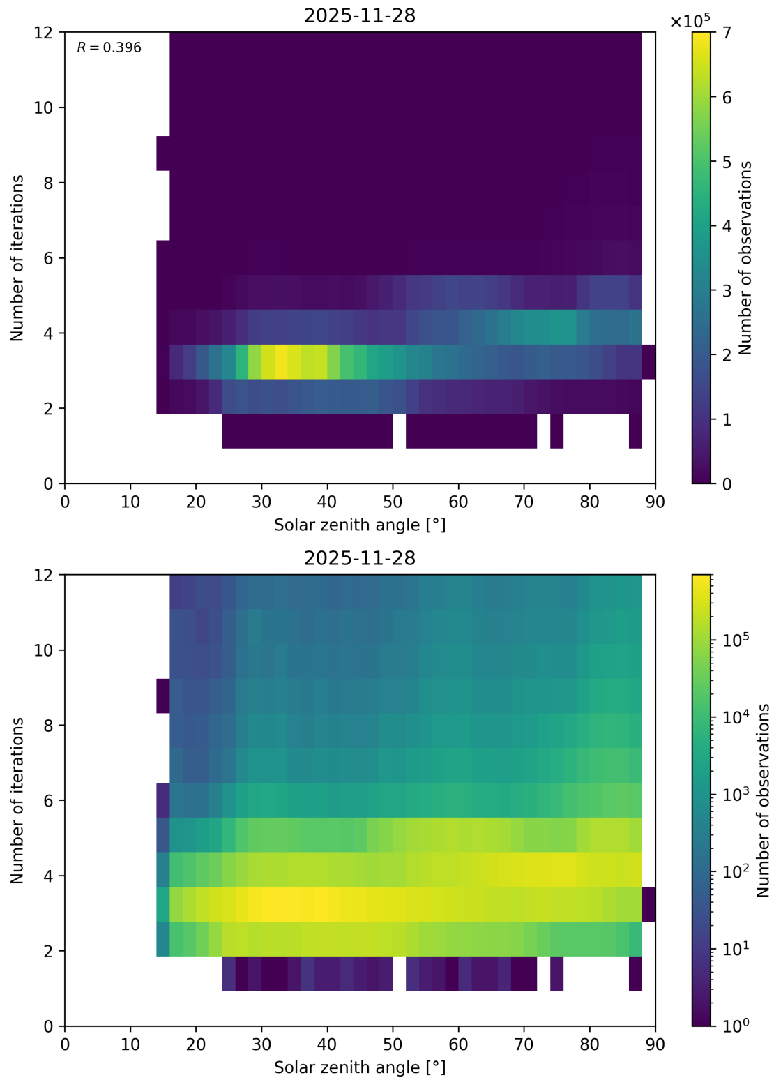
Figure 114: Scatter density plot of “Solar zenith angle” against “Number of iterations” for 2025-11-28 to 2025-11-29.
