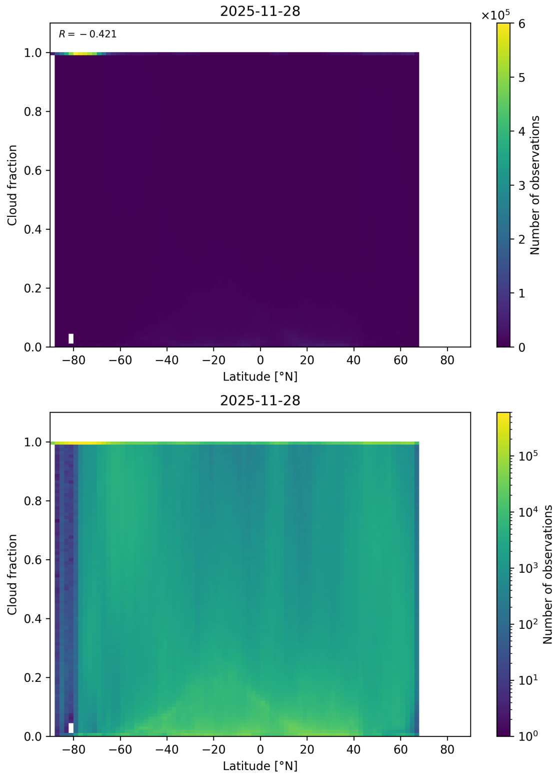
Figure 90: Scatter density plot of “Latitude” against “Cloud fraction” for 2025-11-28 to 2025-11-29.
