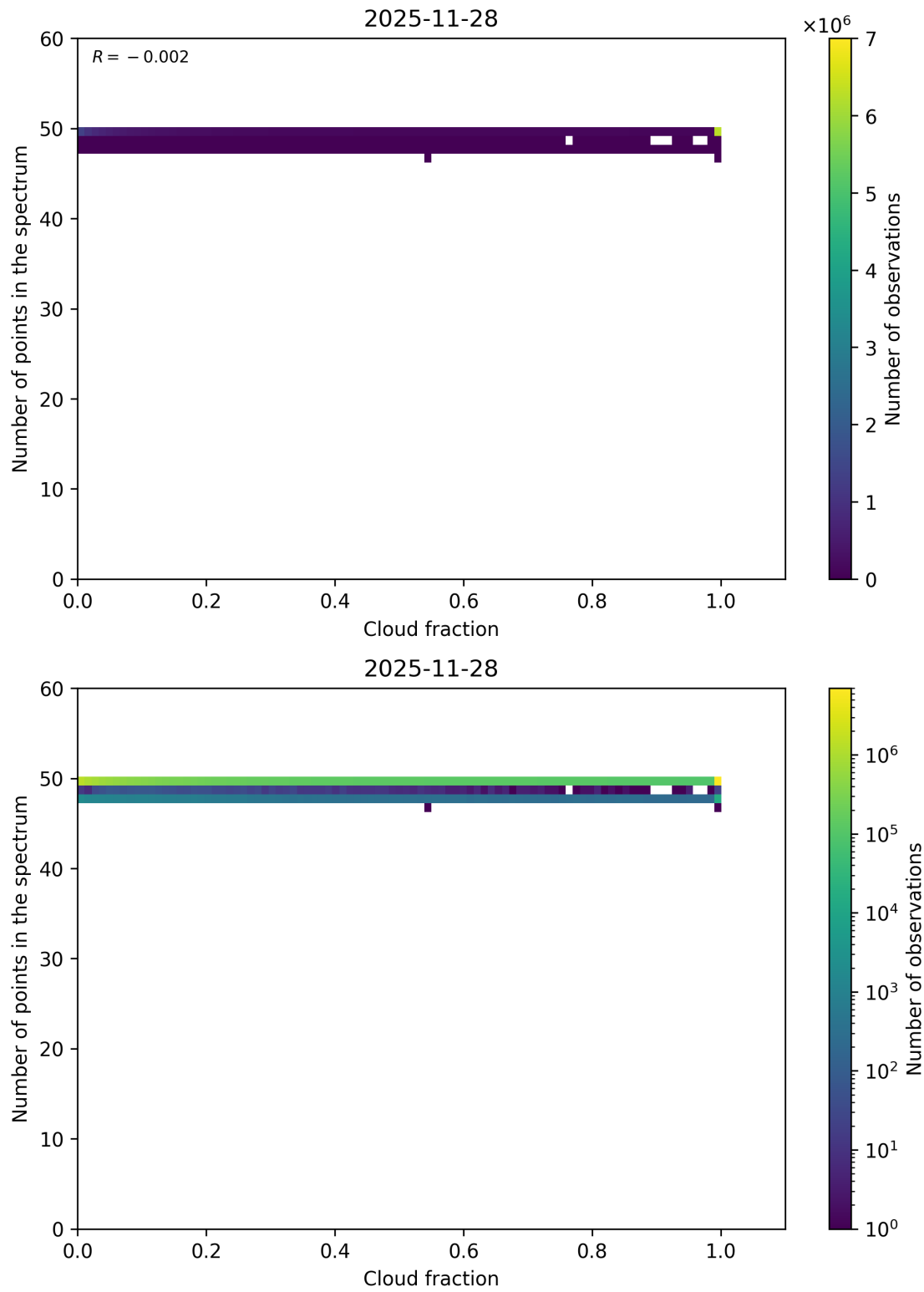
Figure 74: Scatter density plot of “Cloud fraction” against “Number of points in the spectrum” for 2025-11-28 to 2025-11-29.
