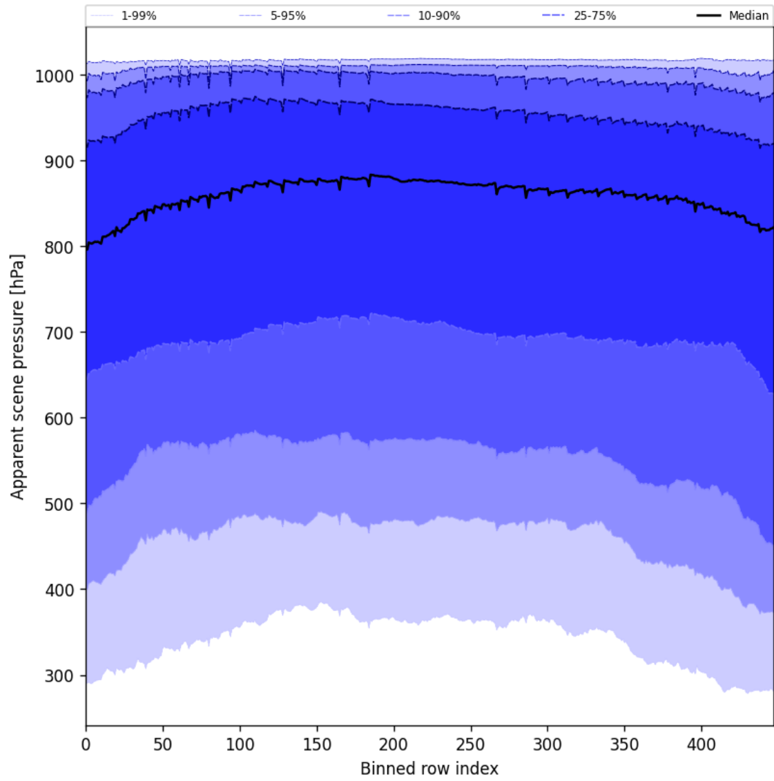
Figure 53: Along track statistics of “Apparent scene pressure” for 2025-11-28 to 2025-11-29
