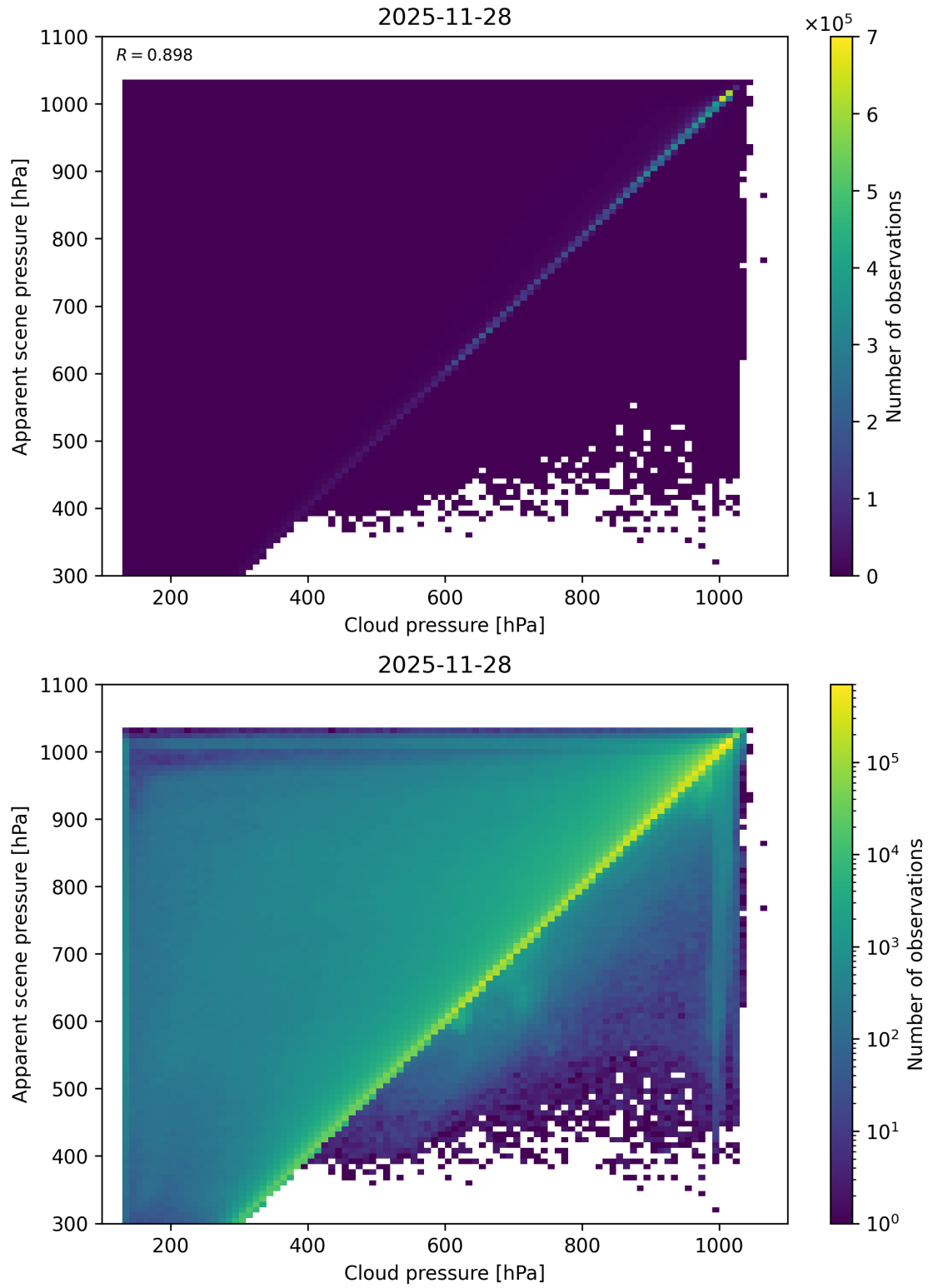
Figure 77: Scatter density plot of “Cloud pressure” against “Apparent scene pressure” for 2025-11-28 to 2025-11-29.
