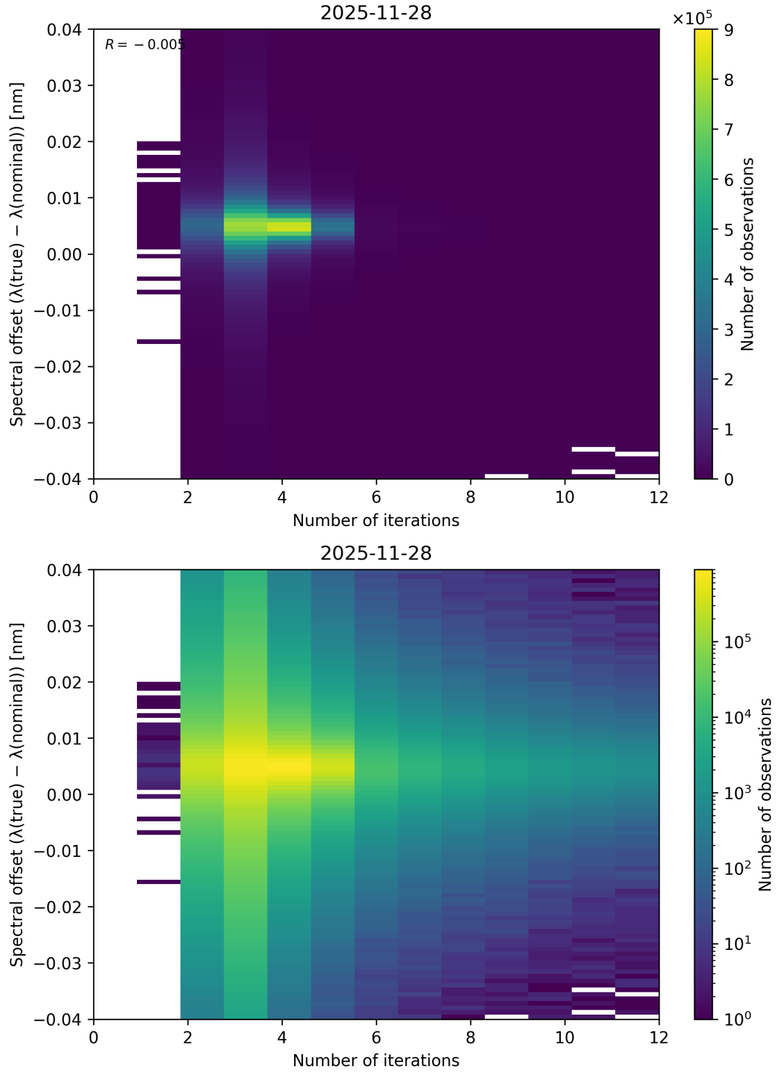
Figure 100: Scatter density plot of “Number of iterations” against “Spectral offset ( \lambda_{\text{true}} - \lambda_{\text{nominal}} )” for 2025-11-28 to 2025-11-29.
