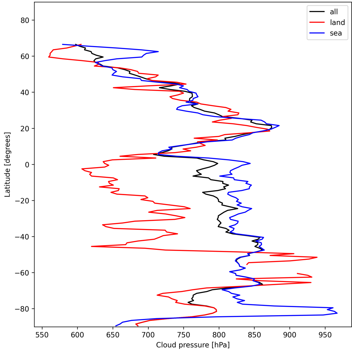
Figure 13: Zonal average of “Cloud pressure” for 2025-11-28 to 2025-11-29.
