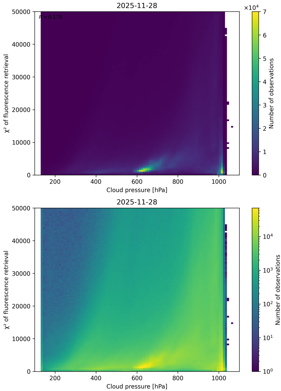
Figure 78: Scatter density plot of “Cloud pressure” against “ \chi^2 of fluorescence retrieval” for 2025-11-28 to 2025-11-29.
