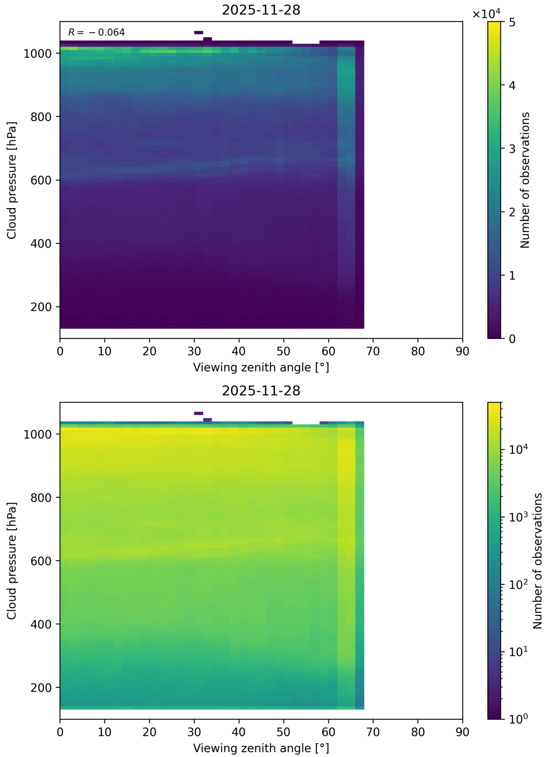
Figure 121: Scatter density plot of “Viewing zenith angle” against “Cloud pressure” for 2025-11-28 to 2025-11-29.
