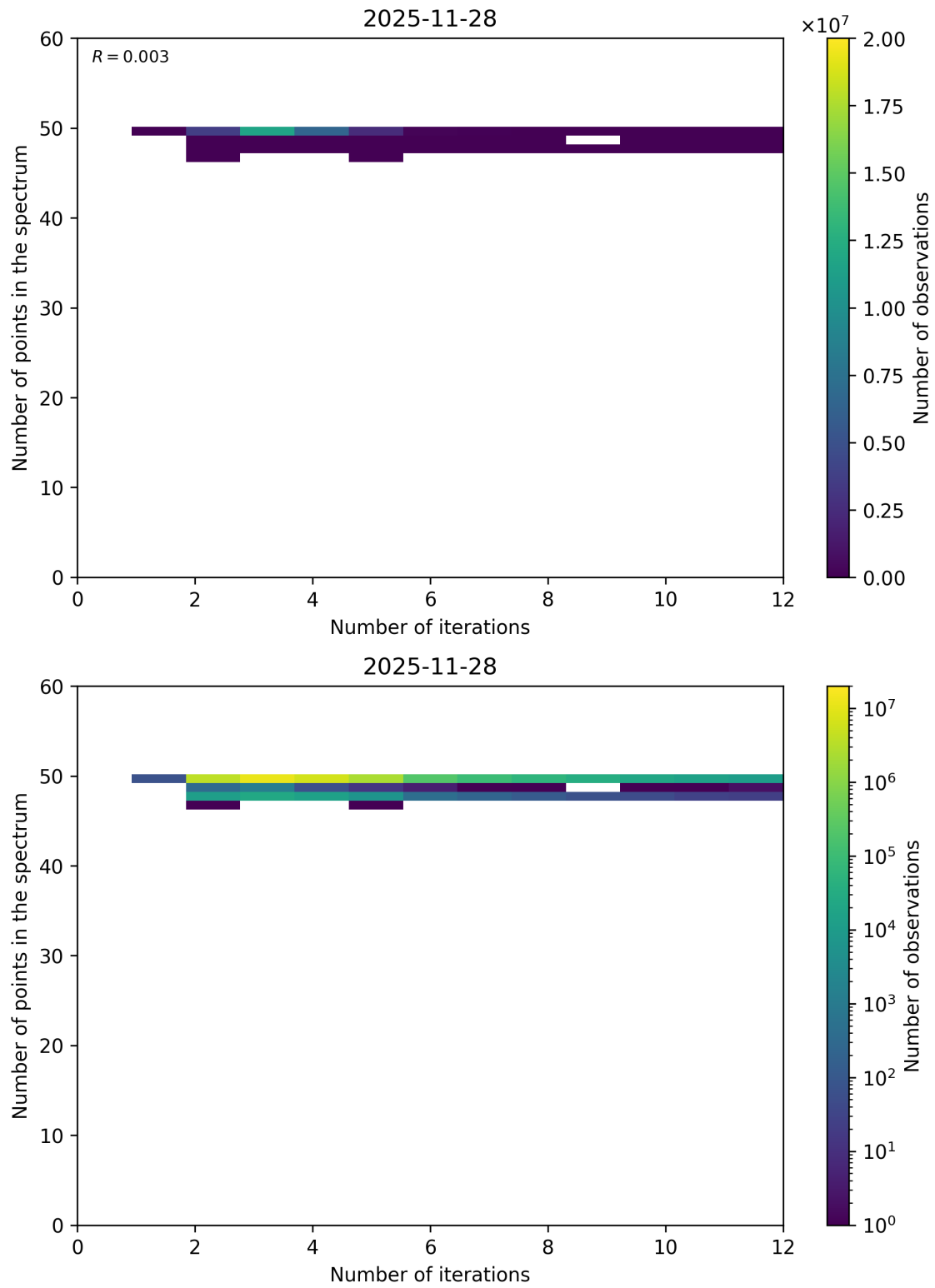
Figure 99: Scatter density plot of “Number of iterations” against “Number of points in the spectrum” for 2025-11-28 to 2025-11-29.
