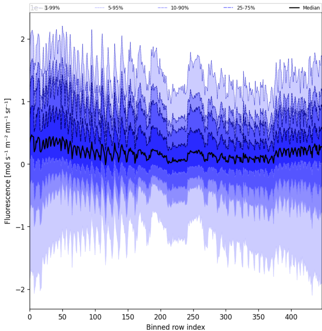
Figure 57: Along track statistics of “Fluorescence” for 2025-11-28 to 2025-11-29
