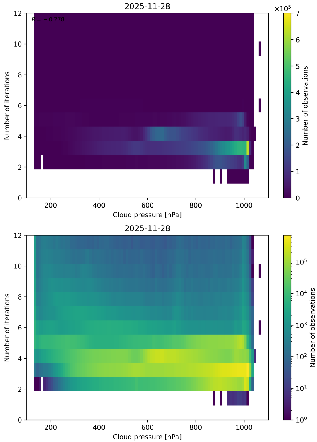
Figure 81: Scatter density plot of “Cloud pressure” against “Number of iterations” for 2025-11-28 to 2025-11-29.
