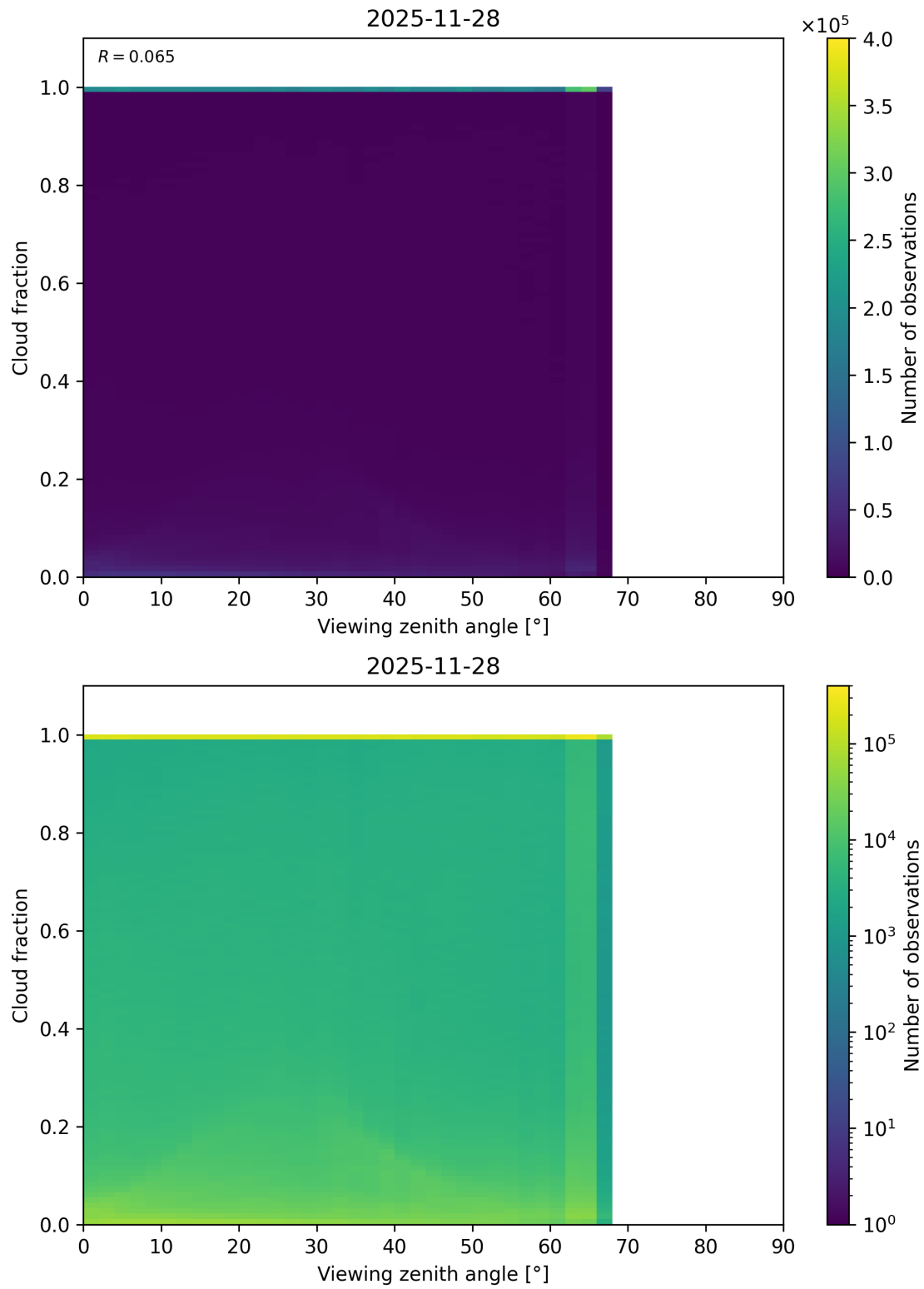
Figure 120: Scatter density plot of “Viewing zenith angle” against “Cloud fraction” for 2025-11-28 to 2025-11-29.
