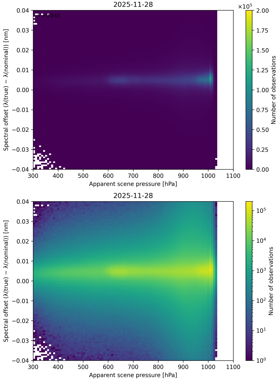
Figure 67: Scatter density plot of “Apparent scene pressure” against “Spectral offset ( \lambda_{\text{true}} - \lambda_{\text{nominal}} )” for 2025-11-28 to 2025-11-29.
