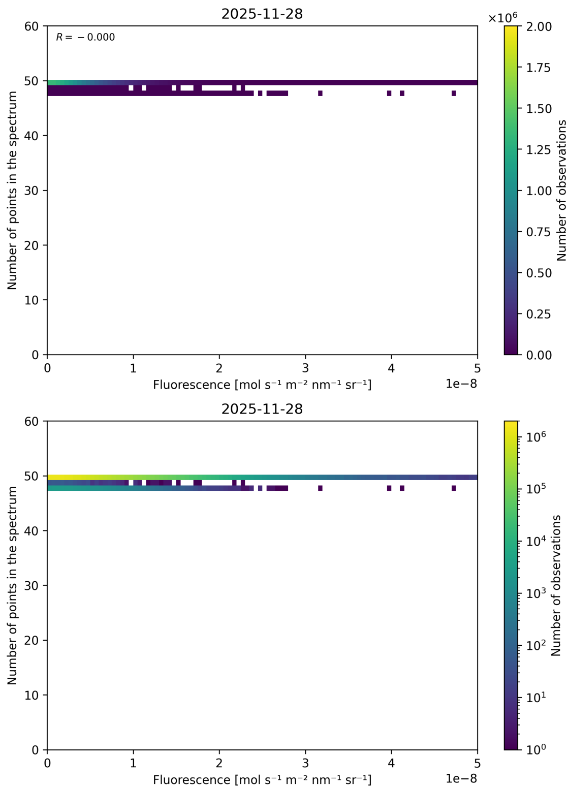
Figure 86: Scatter density plot of “Fluorescence” against “Number of points in the spectrum” for 2025-11-28 to 2025-11-29.
