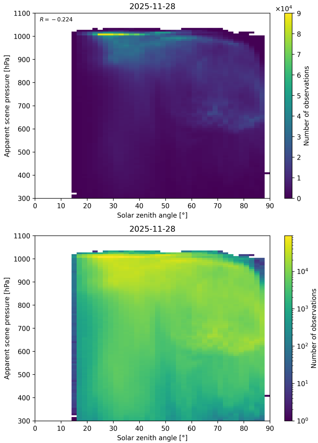
Figure 108: Scatter density plot of “Solar zenith angle” against “Apparent scene pressure” for 2025-11-28 to 2025-11-29.
