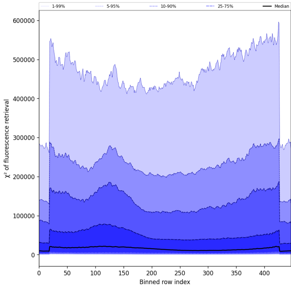
Figure 59: Along track statistics of “ \chi^2 of fluorescence retrieval” for 2025-11-28 to 2025-11-29
