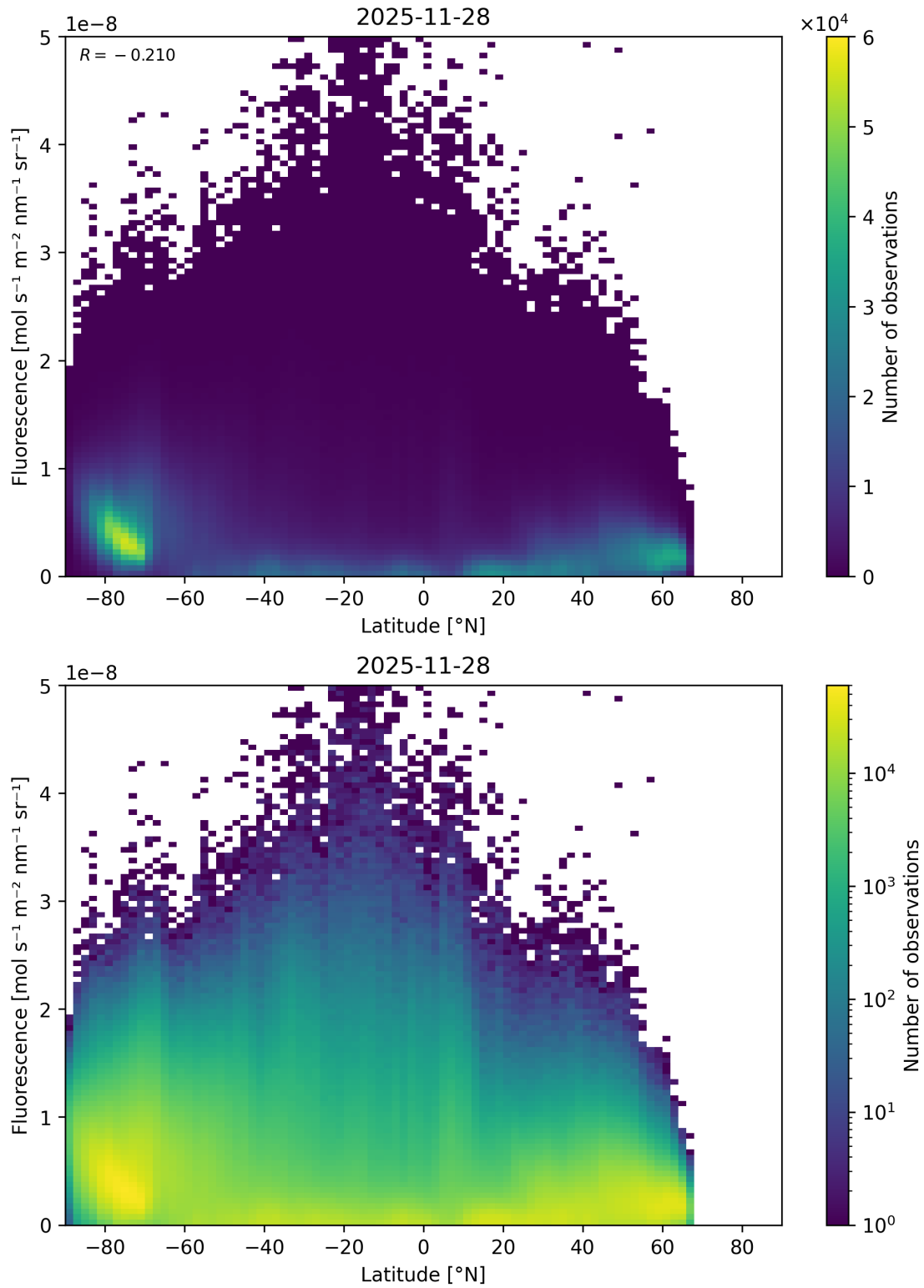
Figure 92: Scatter density plot of “Latitude” against “Fluorescence” for 2025-11-28 to 2025-11-29.
