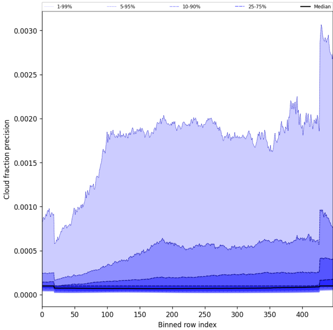
Figure 50: Along track statistics of “Cloud fraction precision” for 2025-11-28 to 2025-11-29
