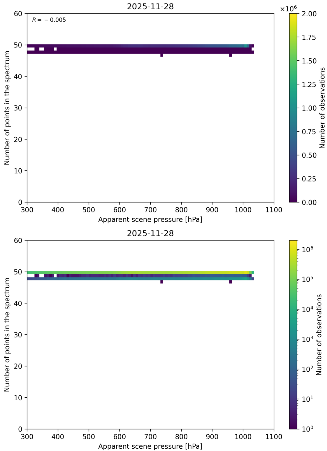
Figure 66: Scatter density plot of “Apparent scene pressure” against “Number of points in the spectrum” for 2025-11-28 to 2025-11-29.
