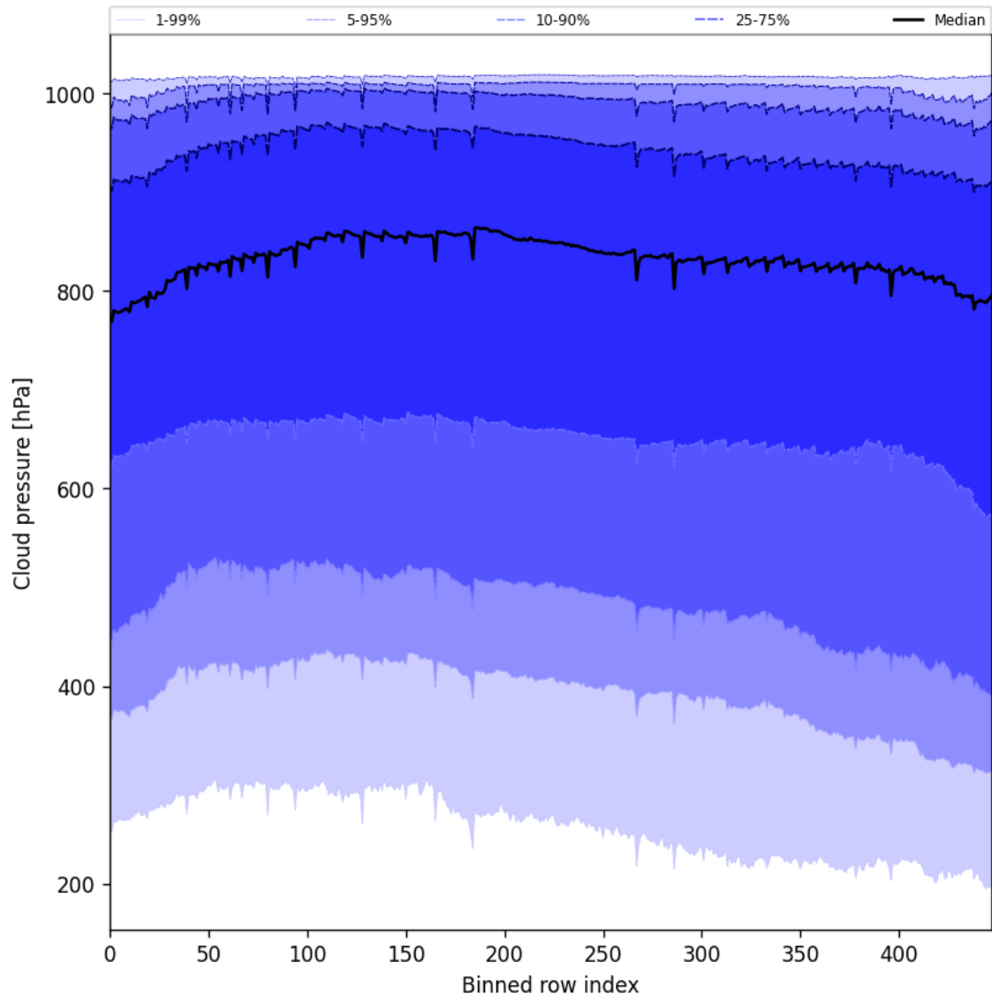
Figure 47: Along track statistics of “Cloud pressure” for 2025-11-28 to 2025-11-29
