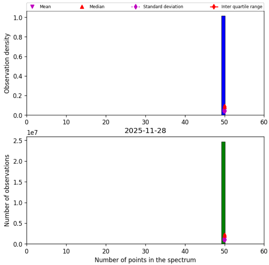
Figure 44: Histogram of “Number of points in the spectrum” for 2025-11-28 to 2025-11-29
