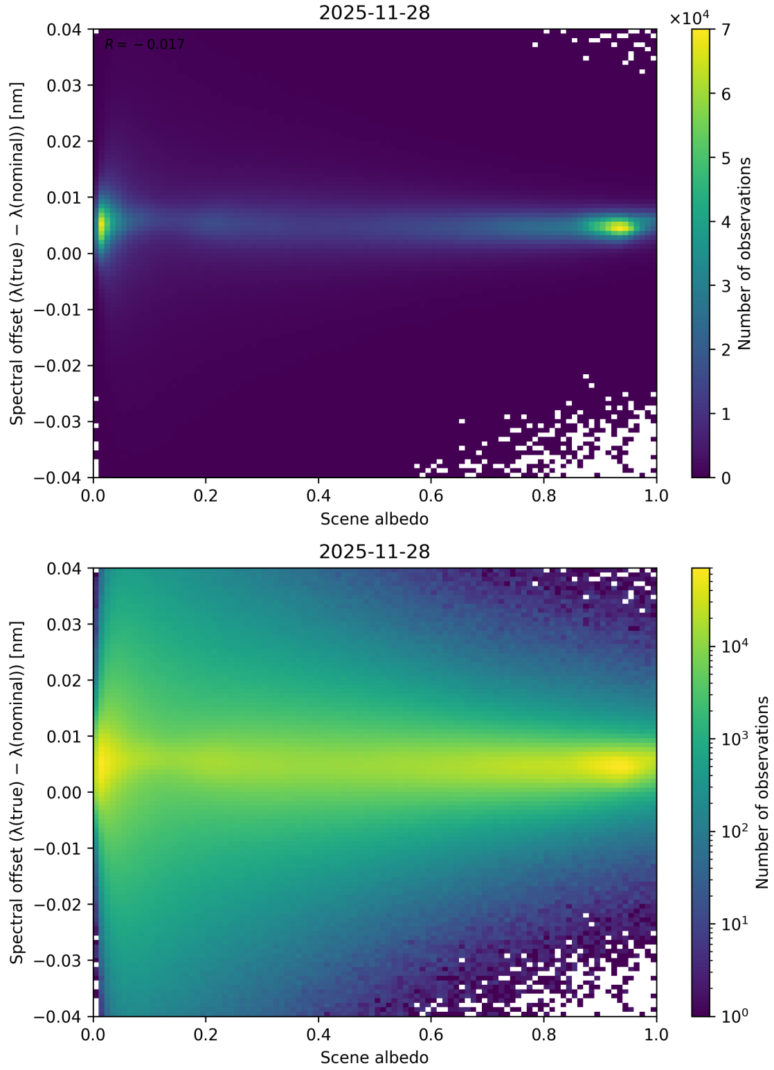
Figure 107: Scatter density plot of “Scene albedo” against “Spectral offset ( \lambda_{\text{true}} - \lambda_{\text{nominal}} )” for 2025-11-28 to 2025-11-29.
