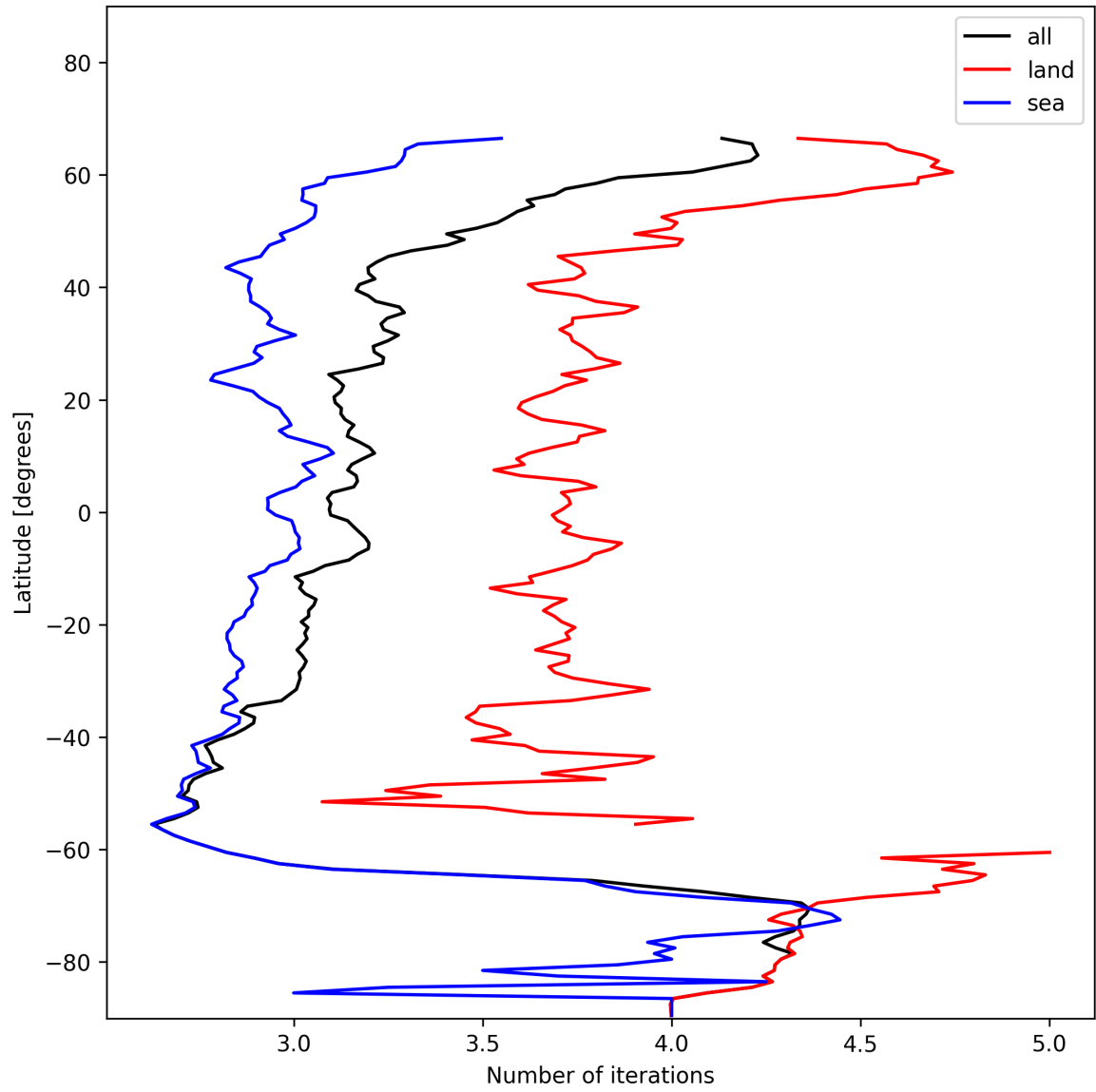
Figure 22: Zonal average of “Number of iterations” for 2025-11-28 to 2025-11-29.
