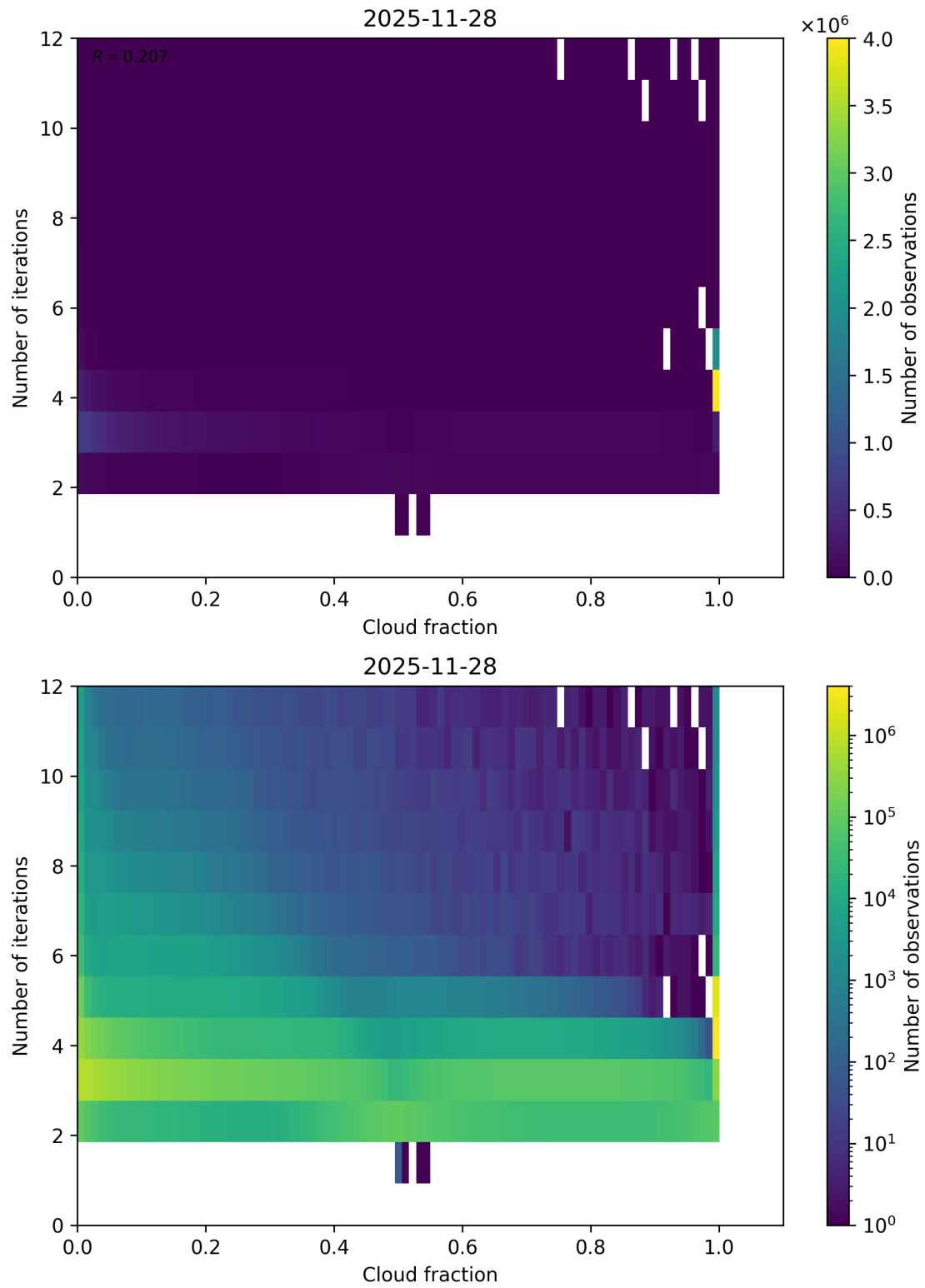
Figure 73: Scatter density plot of “Cloud fraction” against “Number of iterations” for 2025-11-28 to 2025-11-29.
