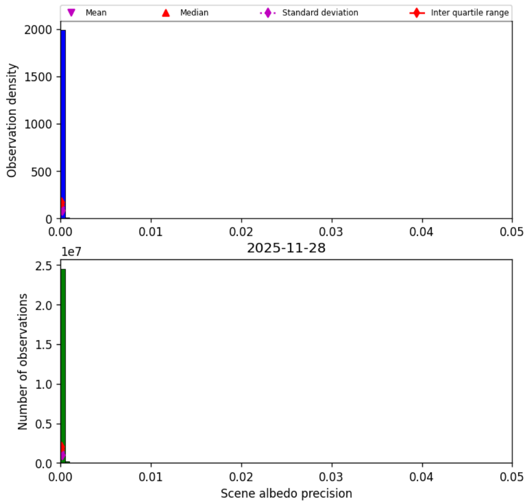
Figure 35: Histogram of “Scene albedo precision” for 2025-11-28 to 2025-11-29
