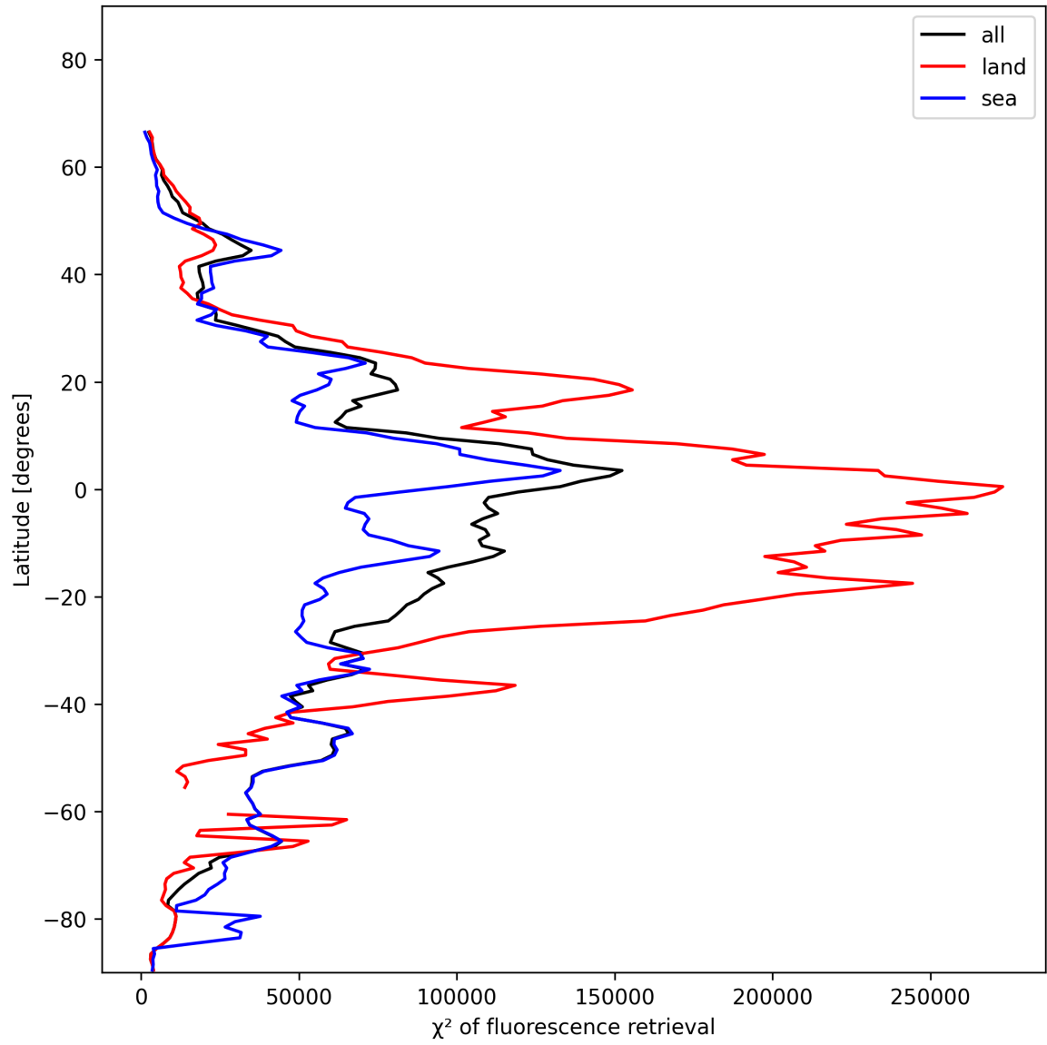
Figure 25: Zonal average of “ \chi^2 of fluorescence retrieval” for 2025-11-28 to 2025-11-29.
