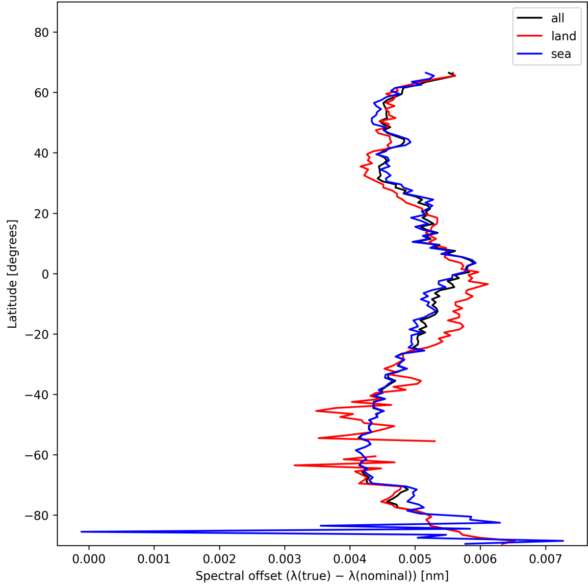
Figure 28: Zonal average of “Spectral offset ( \lambda_{\text{true}} - \lambda_{\text{nominal}} )” for 2025-11-28 to 2025-11-29.
