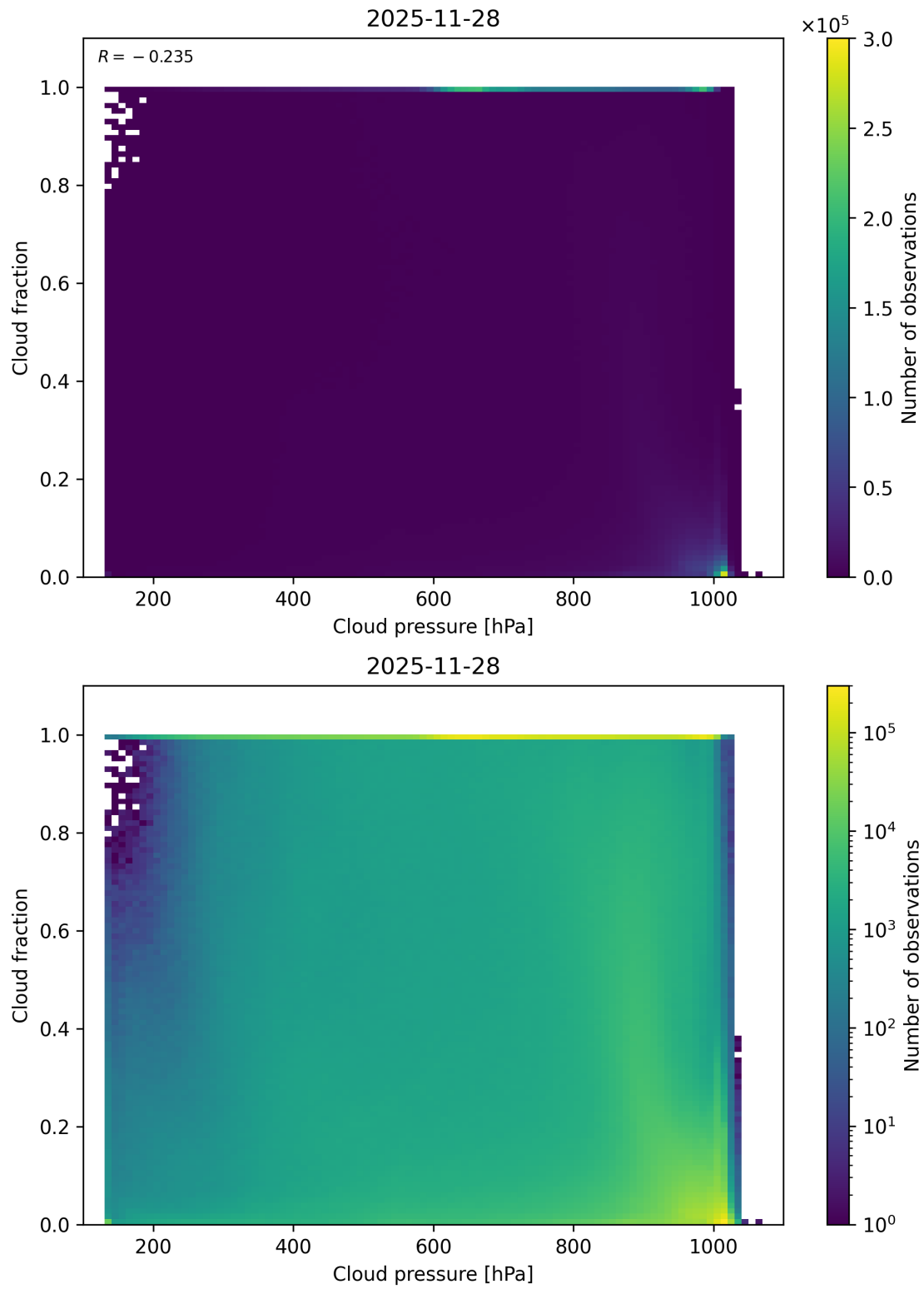
Figure 79: Scatter density plot of “Cloud pressure” against “Cloud fraction” for 2025-11-28 to 2025-11-29.
