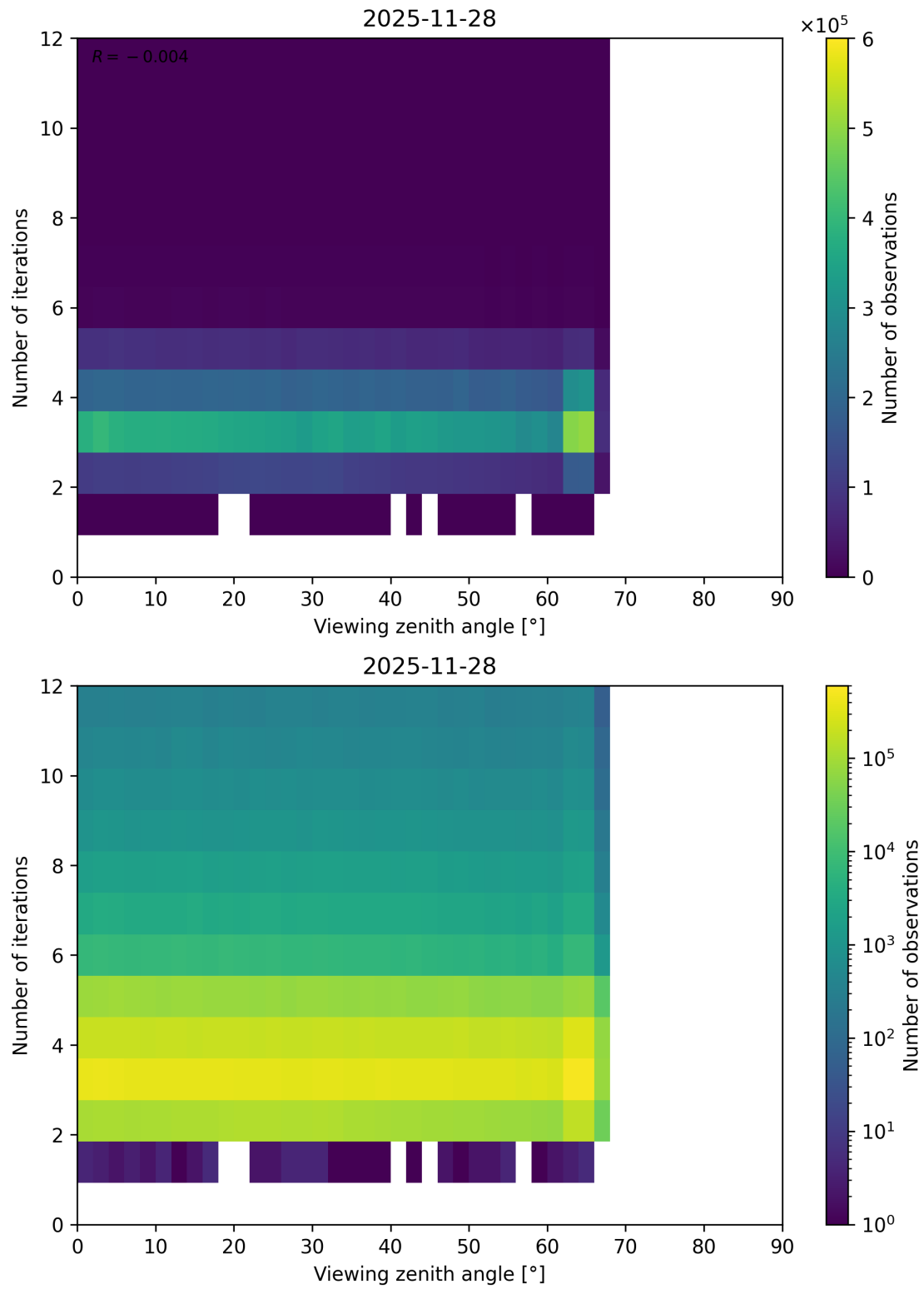
Figure 124: Scatter density plot of “Viewing zenith angle” against “Number of iterations” for 2025-11-28 to 2025-11-29.
