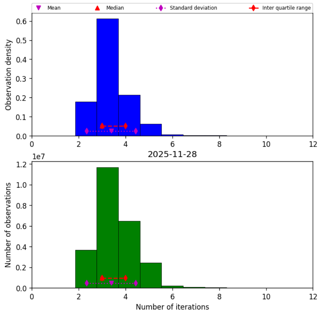
Figure 39: Histogram of “Number of iterations” for 2025-11-28 to 2025-11-29
