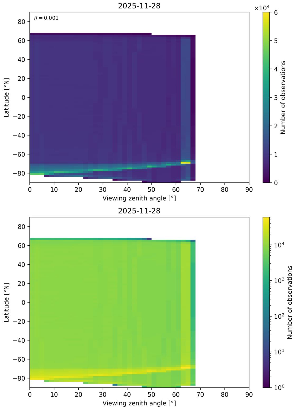
Figure 123: Scatter density plot of “Viewing zenith angle” against “Latitude” for 2025-11-28 to 2025-11-29.
