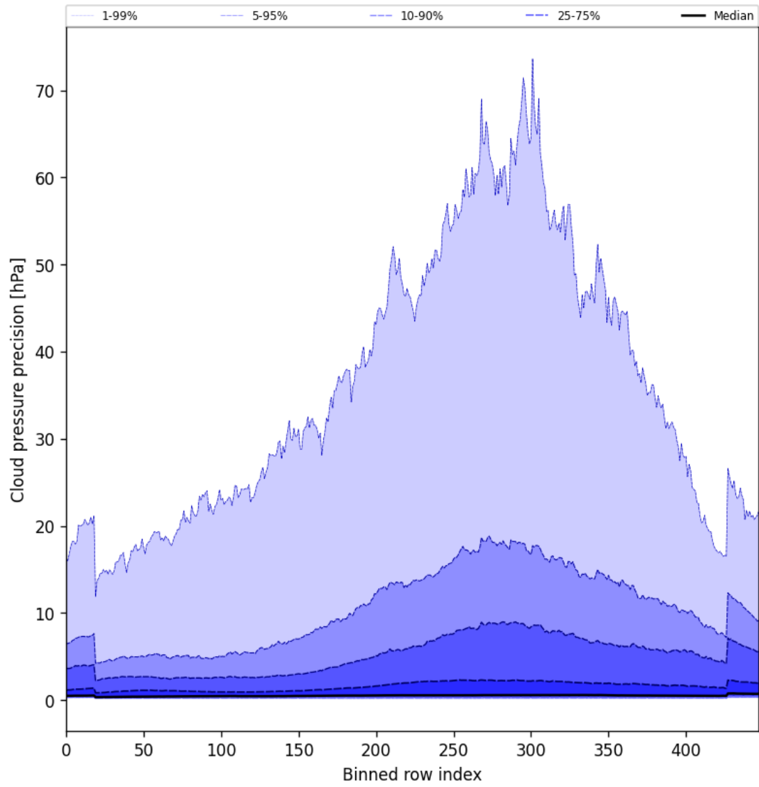
Figure 48: Along track statistics of “Cloud pressure precision” for 2025-11-28 to 2025-11-29
