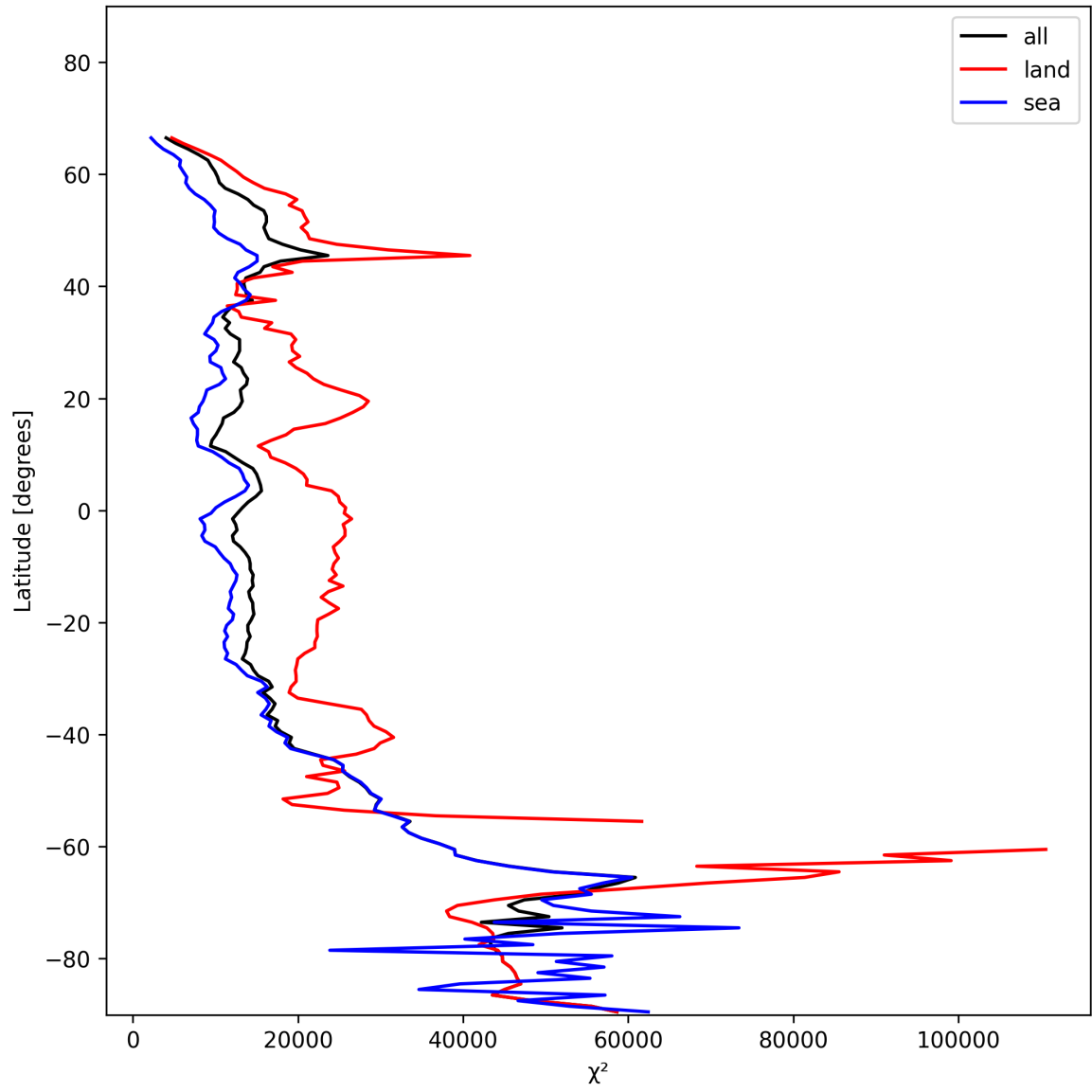
Figure 21: Zonal average of “ \chi^2 ” for 2025-11-28 to 2025-11-29.
