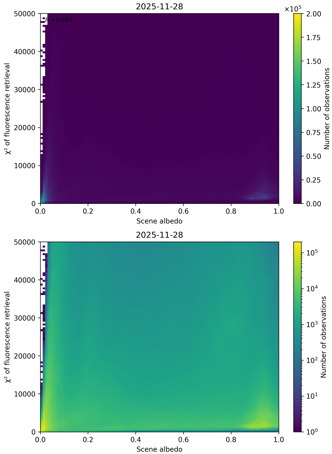
Figure 103: Scatter density plot of “Scene albedo” against “ \chi^2 of fluorescence retrieval” for 2025-11-28 to 2025-11-29.
