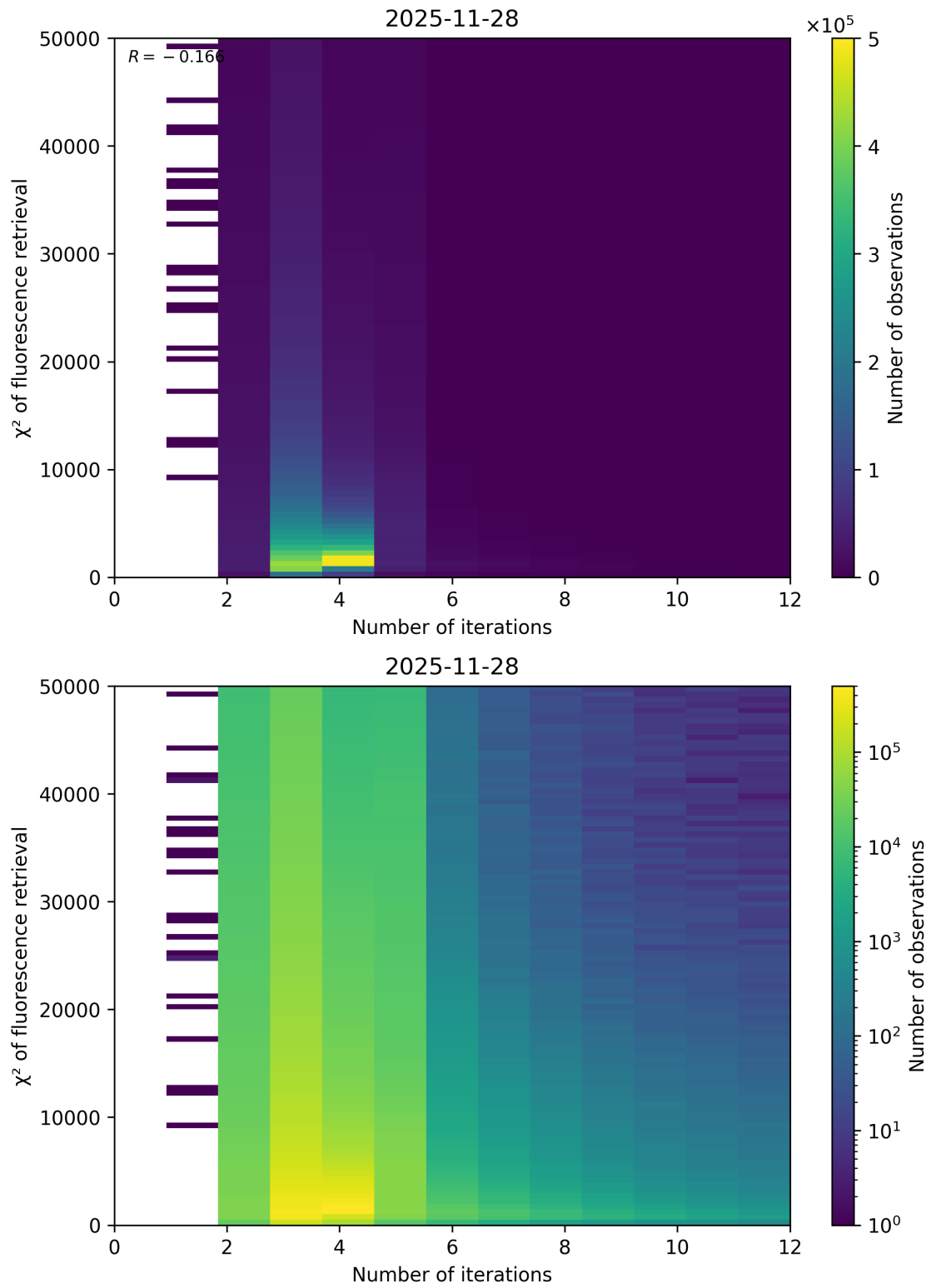
Figure 97: Scatter density plot of “Number of iterations” against “ \chi^2 of fluorescence retrieval” for 2025-11-28 to 2025-11-29.
