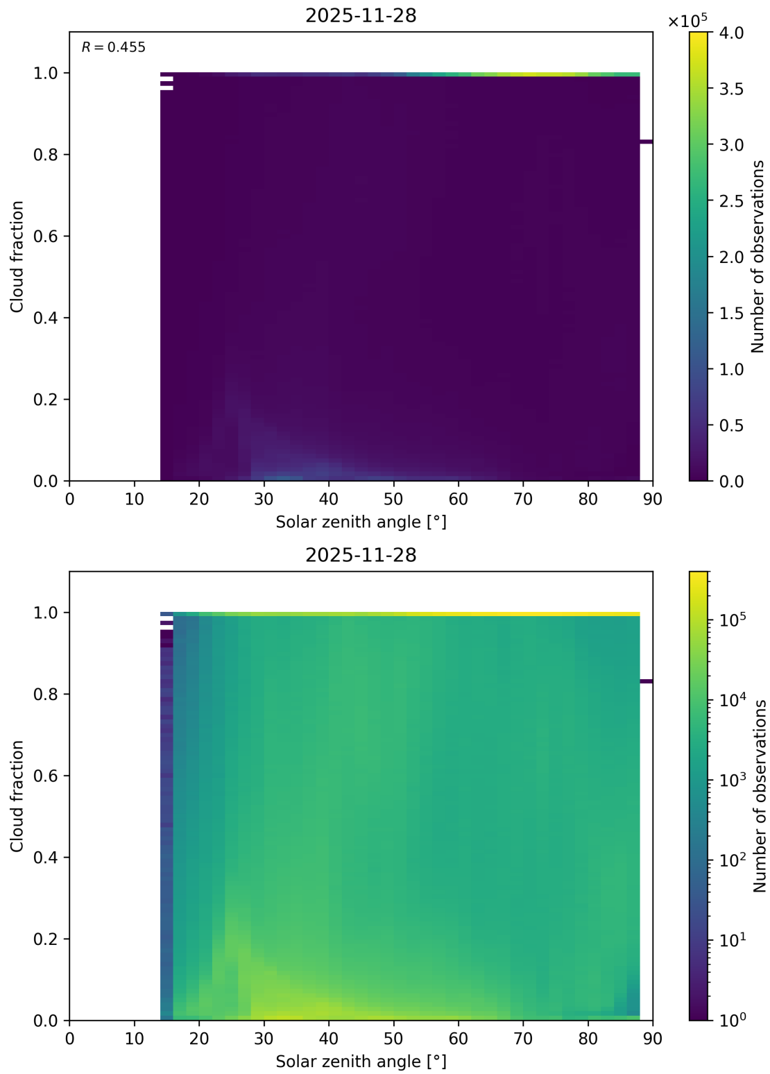
Figure 110: Scatter density plot of “Solar zenith angle” against “Cloud fraction” for 2025-11-28 to 2025-11-29.
