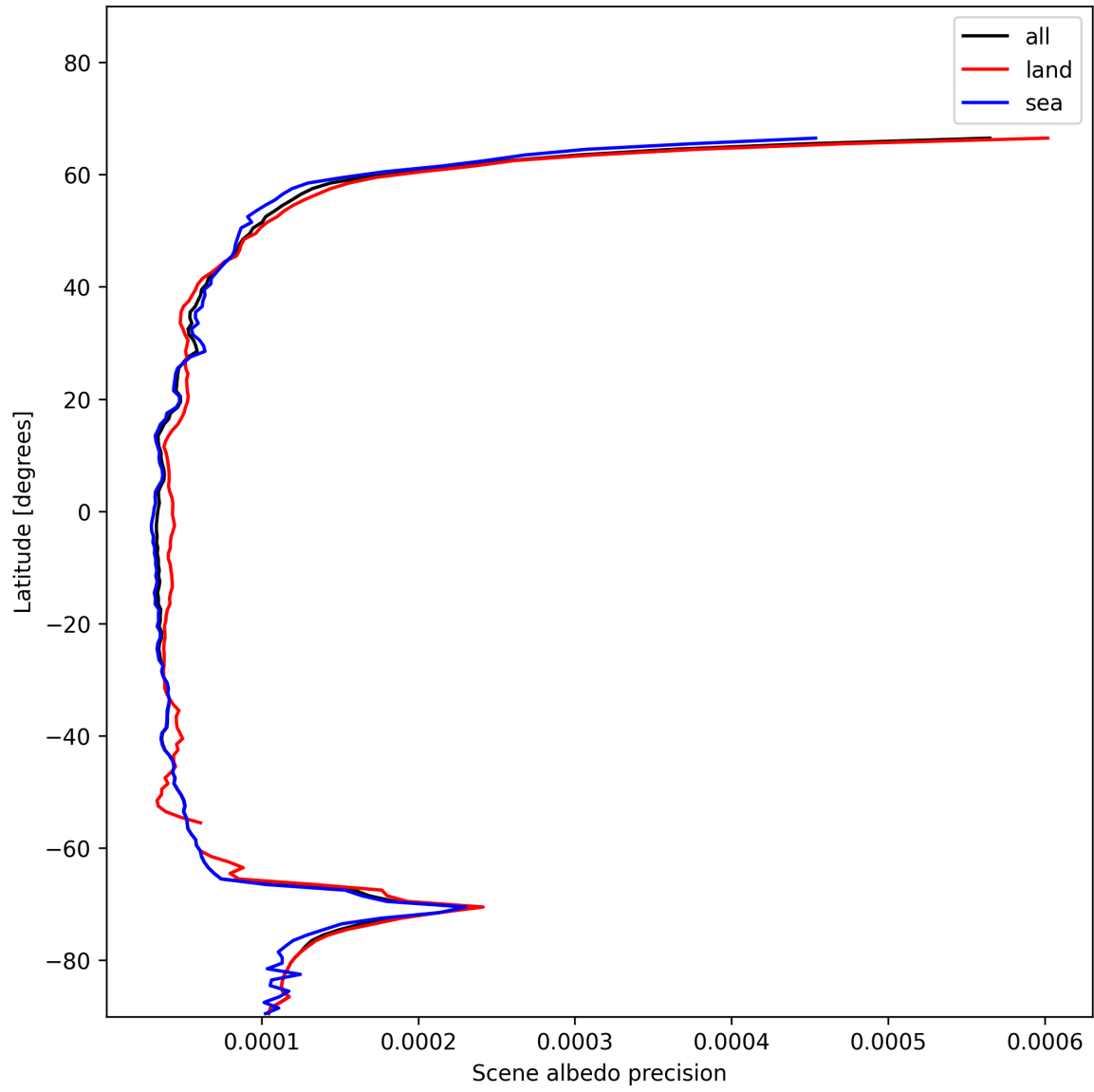
Figure 18: Zonal average of “Scene albedo precision” for 2025-11-28 to 2025-11-29.
