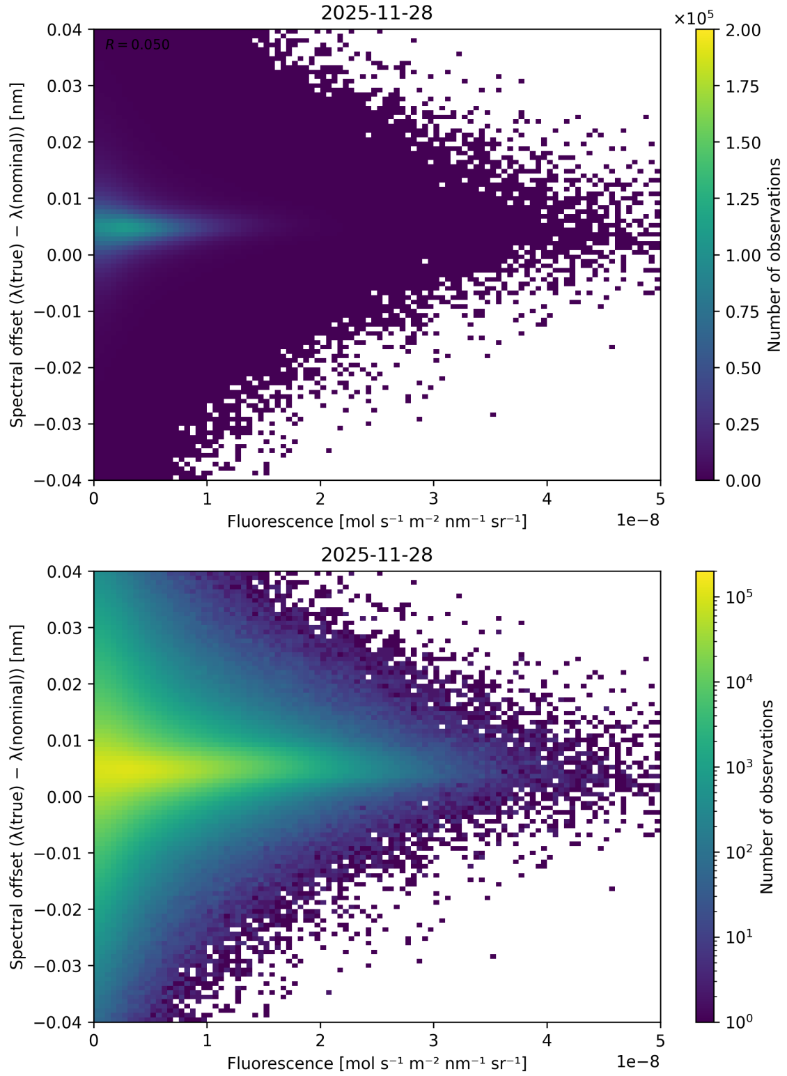
Figure 87: Scatter density plot of “Fluorescence” against “Spectral offset ( \lambda_{\text{true}} - \lambda_{\text{nominal}} )” for 2025-11-28 to 2025-11-29.
