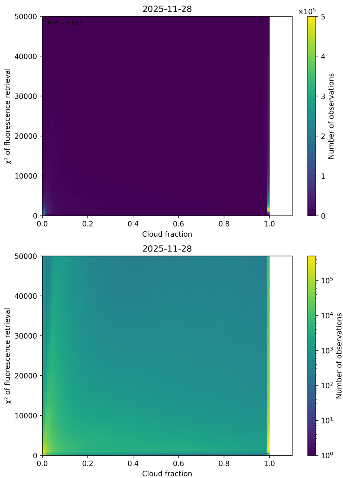
Figure 71: Scatter density plot of “Cloud fraction” against “ \chi^2 of fluorescence retrieval” for 2025-11-28 to 2025-11-29.
