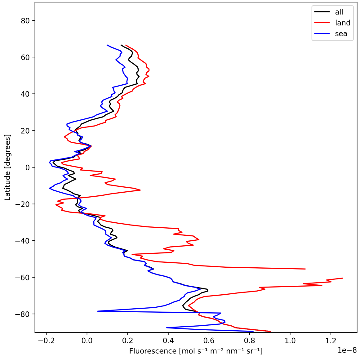
Figure 23: Zonal average of “Fluorescence” for 2025-11-28 to 2025-11-29.
