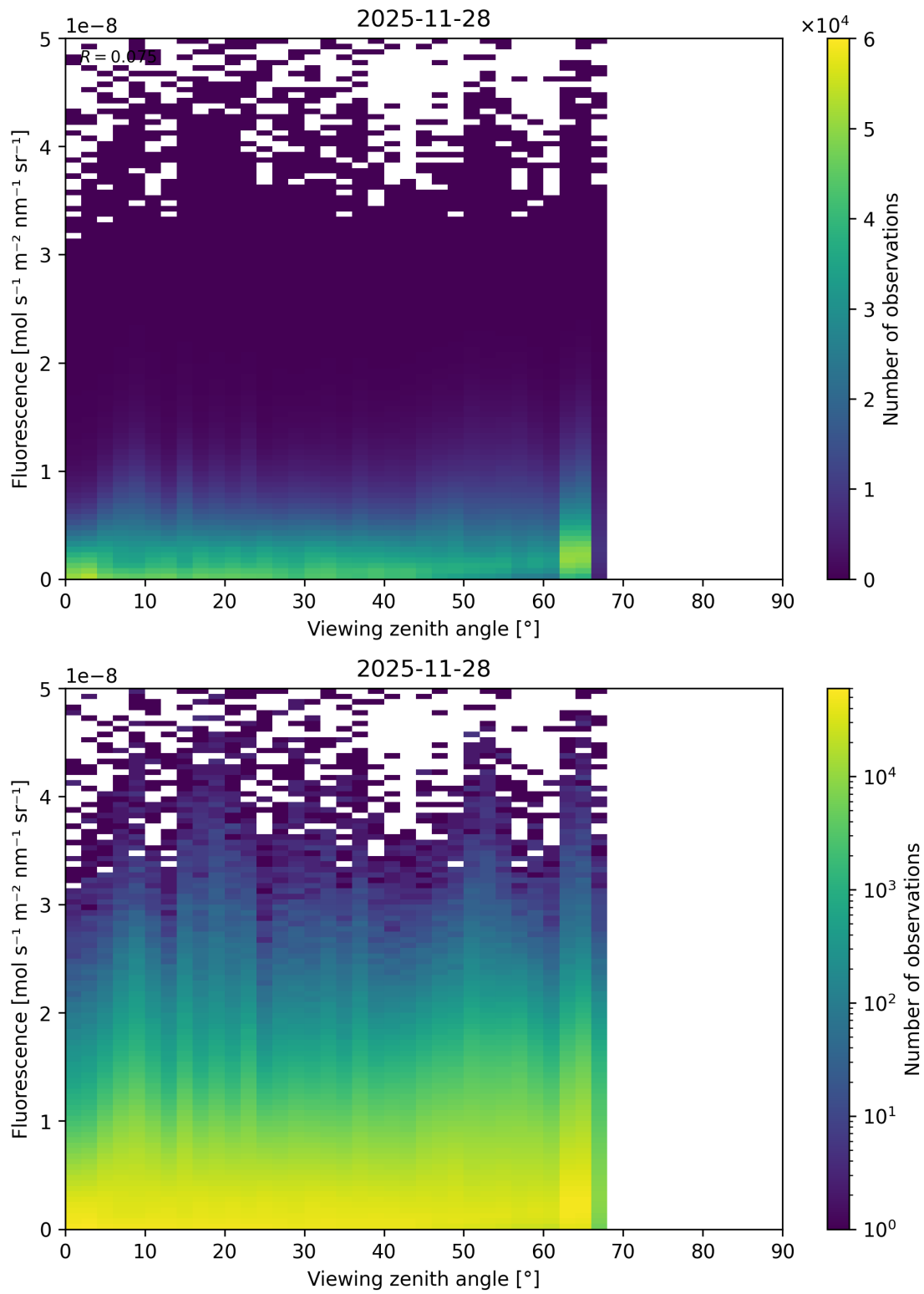
Figure 122: Scatter density plot of “Viewing zenith angle” against “Fluorescence” for 2025-11-28 to 2025-11-29.
