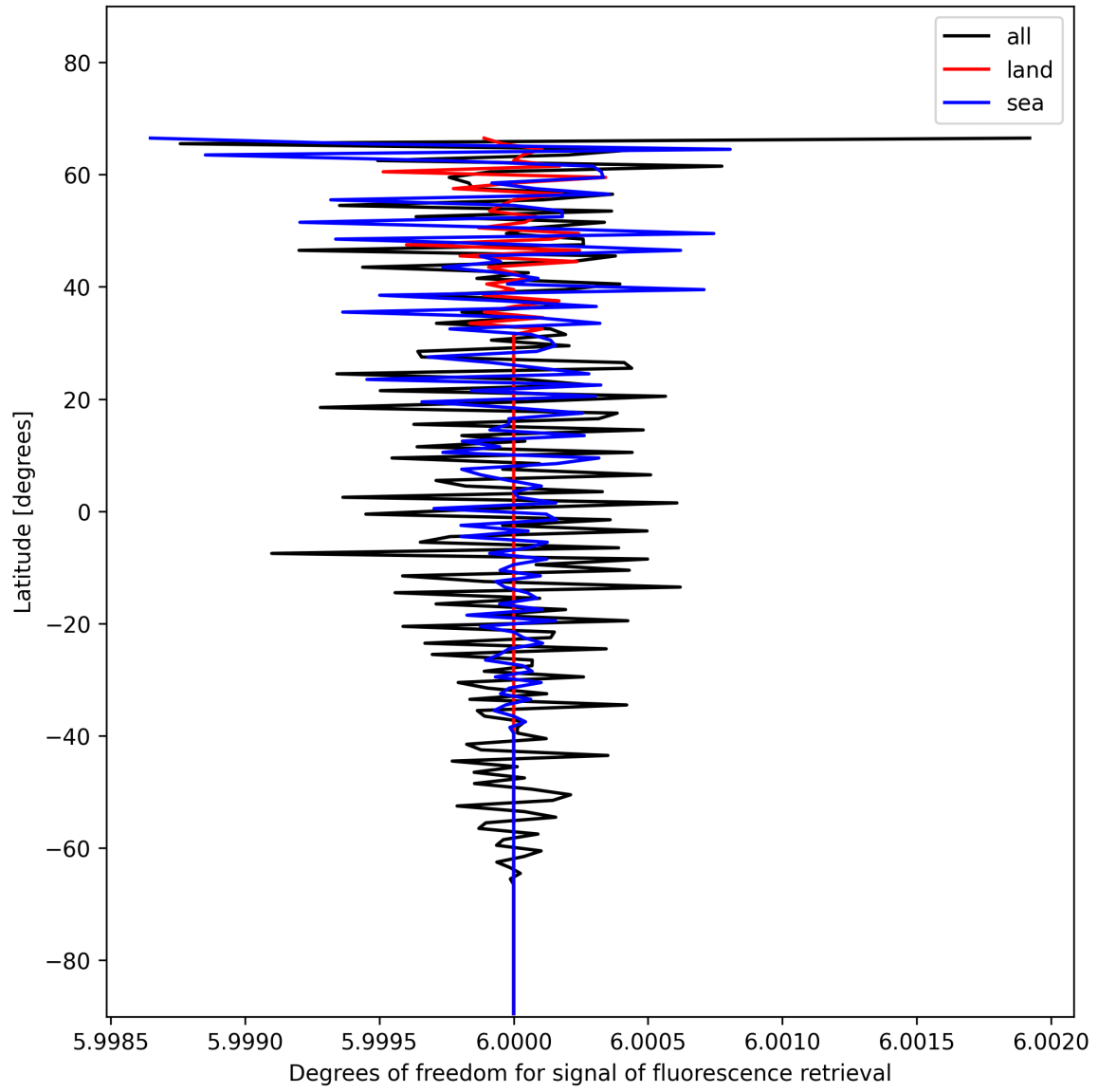
Figure 26: Zonal average of “Degrees of freedom for signal of fluorescence retrieval” for 2025-11-28 to 2025-11-29.
