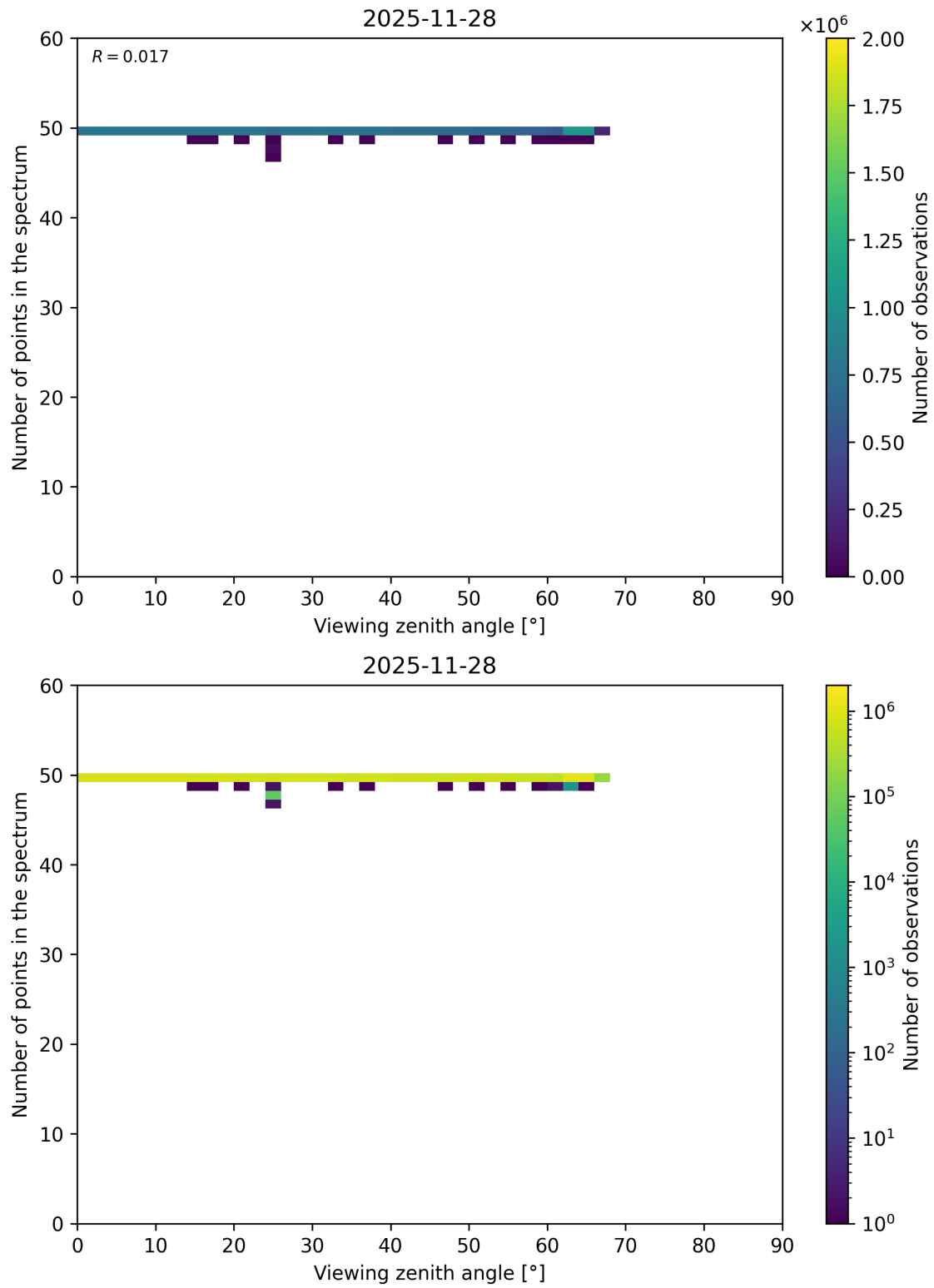
Figure 125: Scatter density plot of “Viewing zenith angle” against “Number of points in the spectrum” for 2025-11-28 to 2025-11-29.
