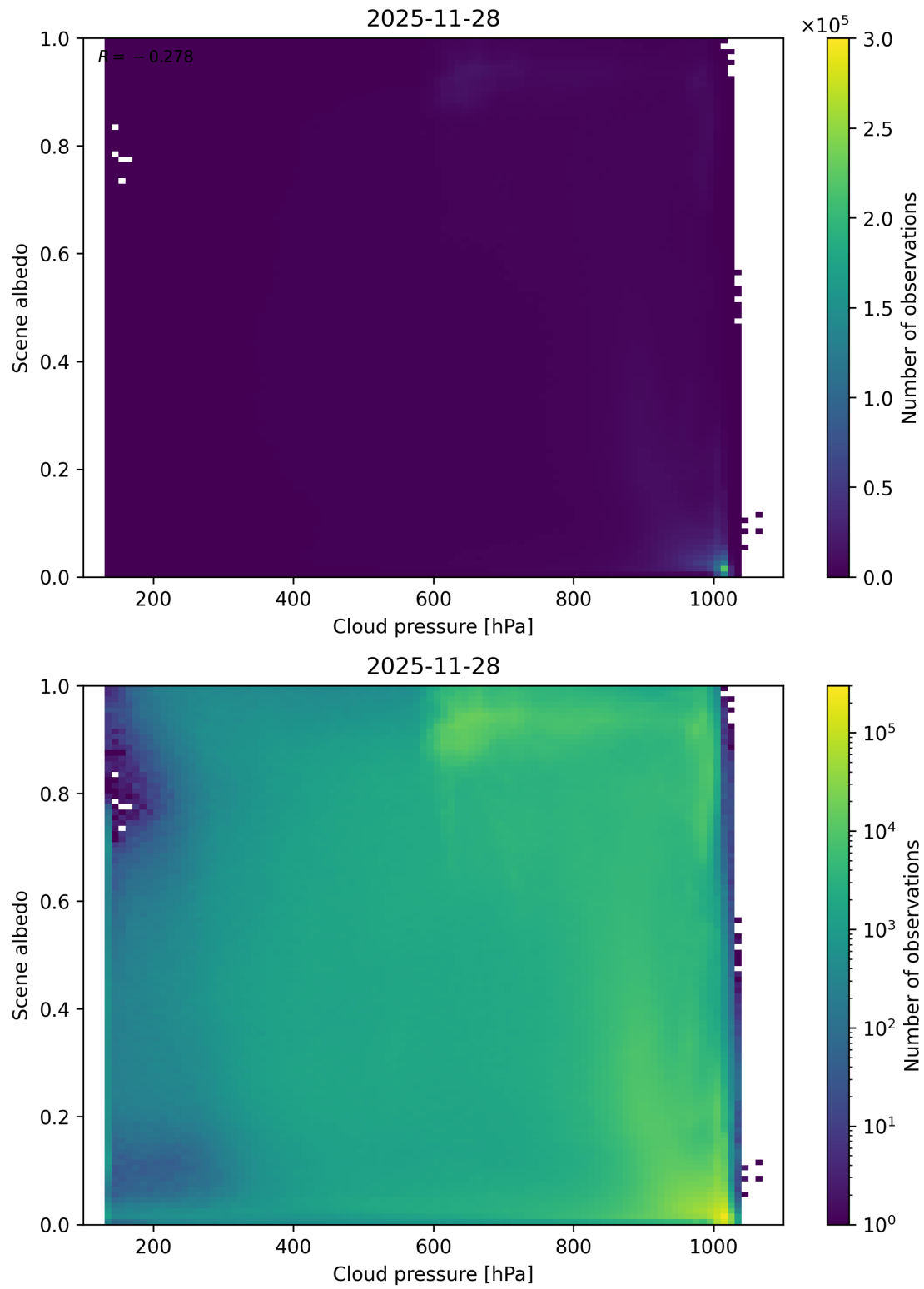
Figure 83: Scatter density plot of “Cloud pressure” against “Scene albedo” for 2025-11-28 to 2025-11-29.
