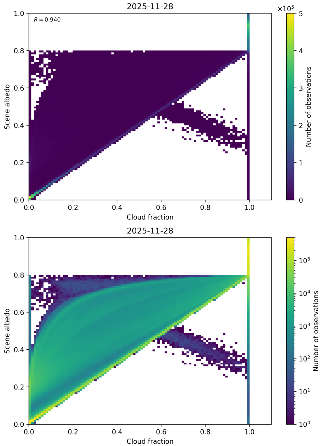
Figure 75: Scatter density plot of “Cloud fraction” against “Scene albedo” for 2025-11-28 to 2025-11-29.
