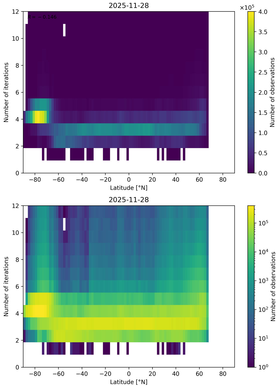
Figure 93: Scatter density plot of “Latitude” against “Number of iterations” for 2025-11-28 to 2025-11-29.
