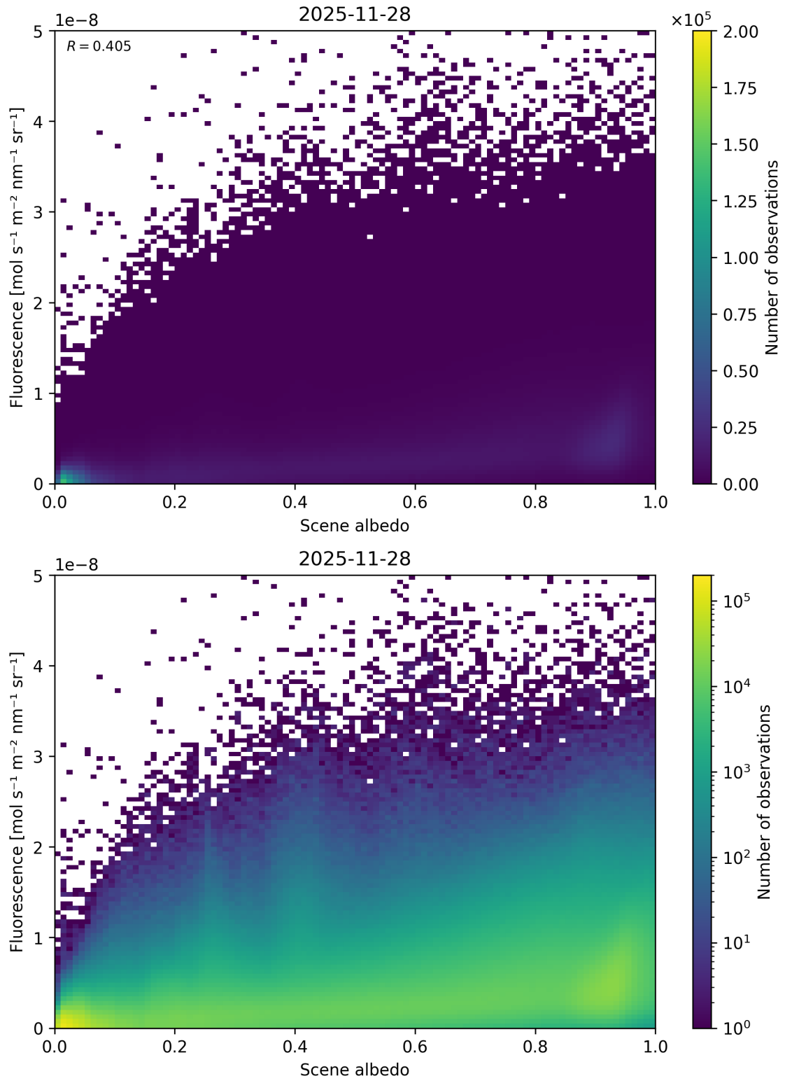
Figure 104: Scatter density plot of “Scene albedo” against “Fluorescence” for 2025-11-28 to 2025-11-29.
