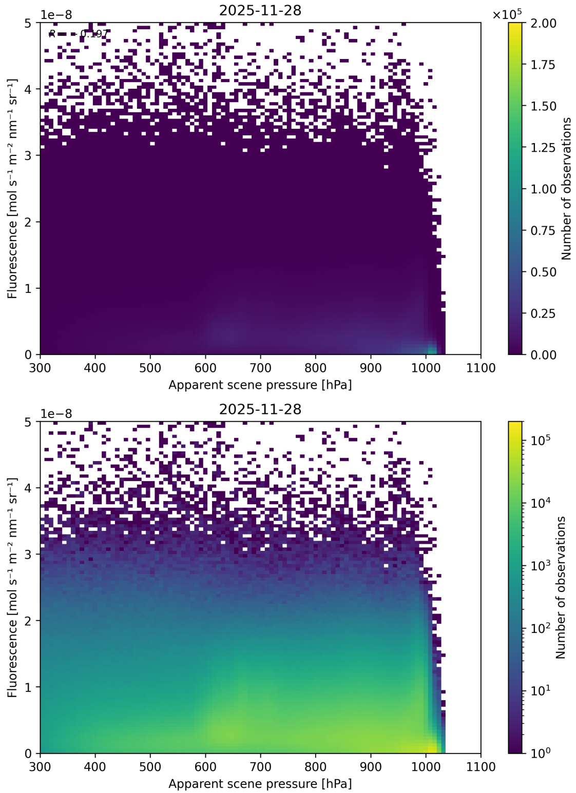
Figure 64: Scatter density plot of “Apparent scene pressure” against “Fluorescence” for 2025-11-28 to 2025-11-29.
