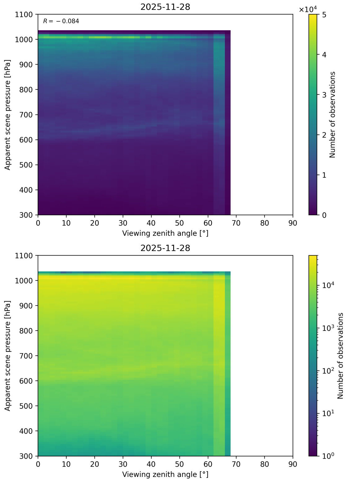
Figure 118: Scatter density plot of “Viewing zenith angle” against “Apparent scene pressure” for 2025-11-28 to 2025-11-29.
