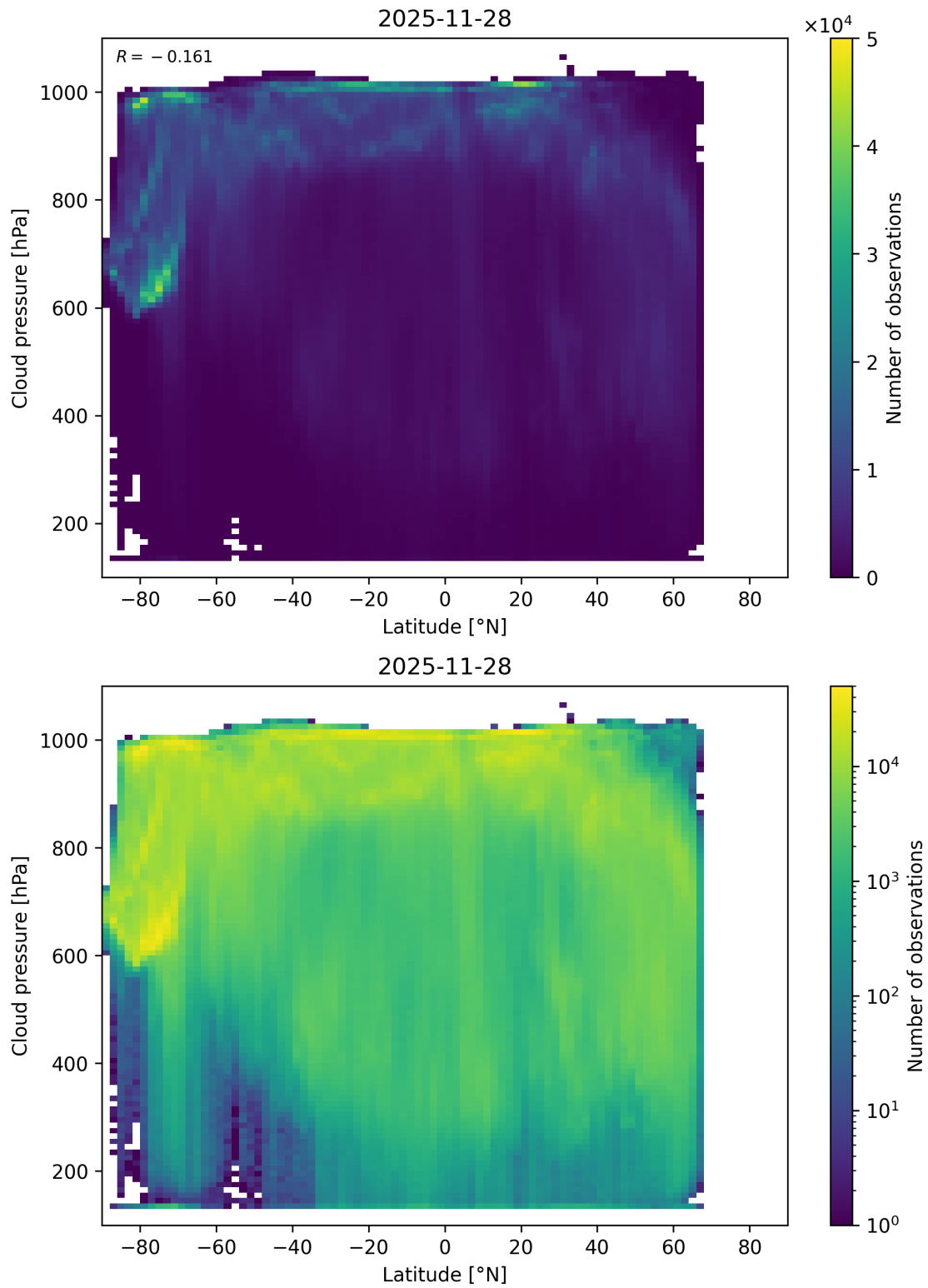
Figure 91: Scatter density plot of “Latitude” against “Cloud pressure” for 2025-11-28 to 2025-11-29.
