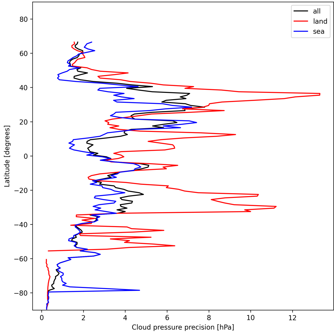
Figure 14: Zonal average of “Cloud pressure precision” for 2025-11-28 to 2025-11-29.
