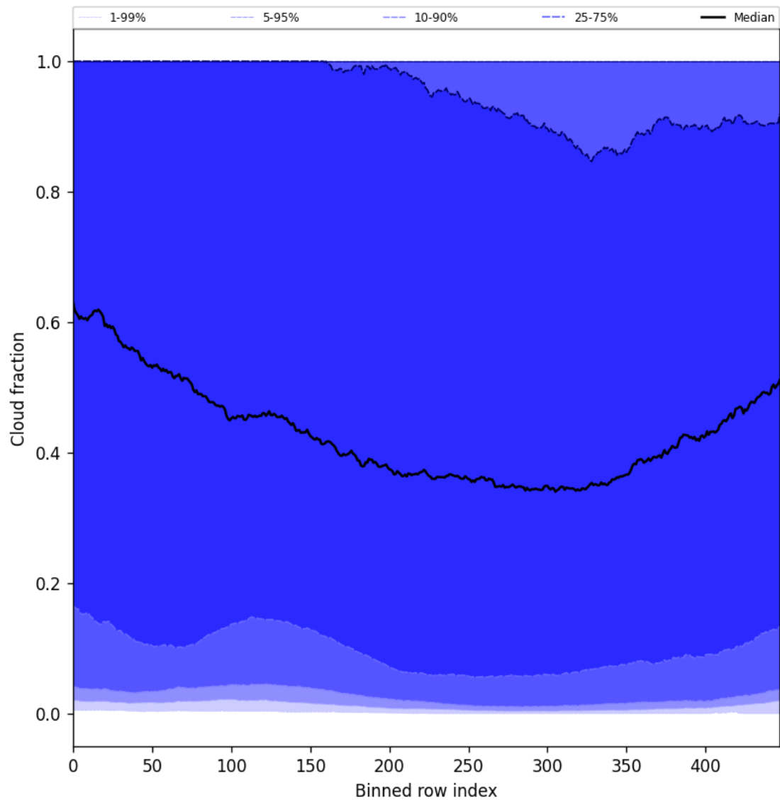
Figure 49: Along track statistics of “Cloud fraction” for 2025-11-28 to 2025-11-29
