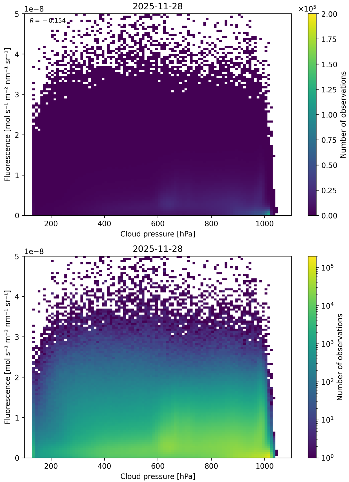
Figure 80: Scatter density plot of “Cloud pressure” against “Fluorescence” for 2025-11-28 to 2025-11-29.
