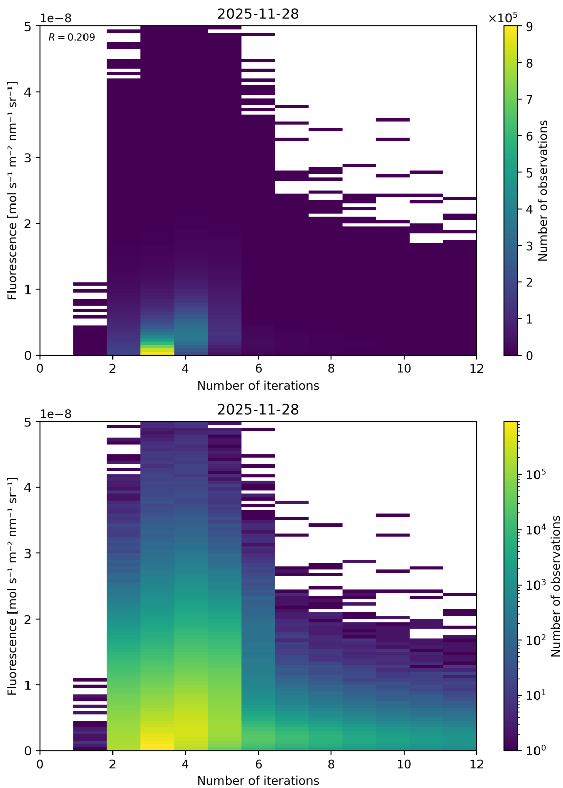
Figure 98: Scatter density plot of “Number of iterations” against “Fluorescence” for 2025-11-28 to 2025-11-29.
