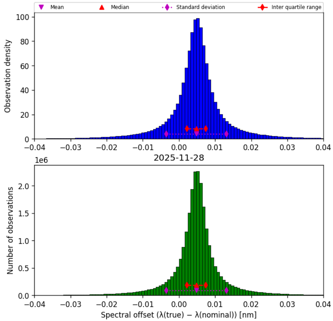
Figure 45: Histogram of “Spectral offset ( \lambda_{\text{true}} - \lambda_{\text{nominal}} )” for 2025-11-28 to 2025-11-29
