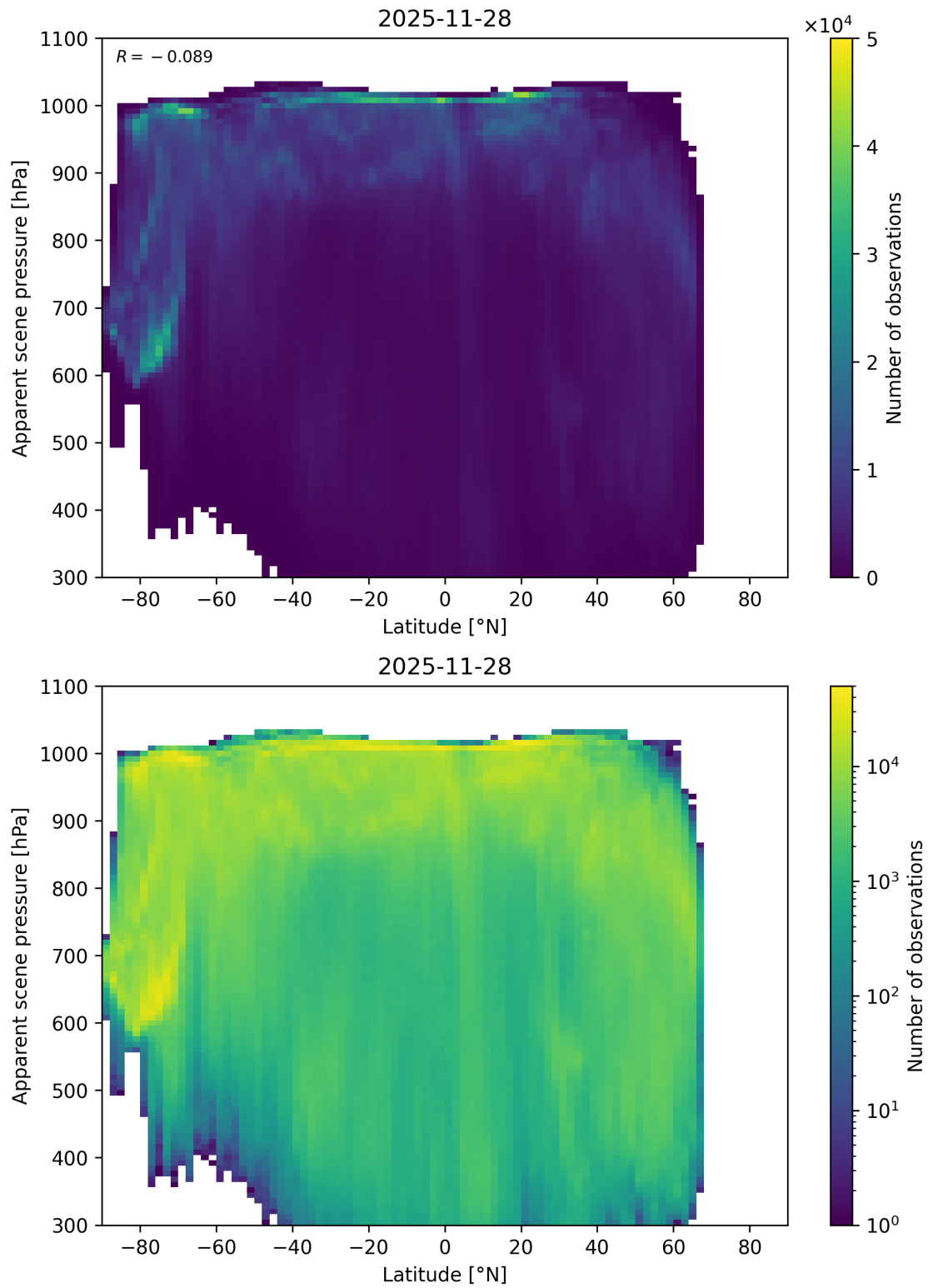
Figure 88: Scatter density plot of “Latitude” against “Apparent scene pressure” for 2025-11-28 to 2025-11-29.
