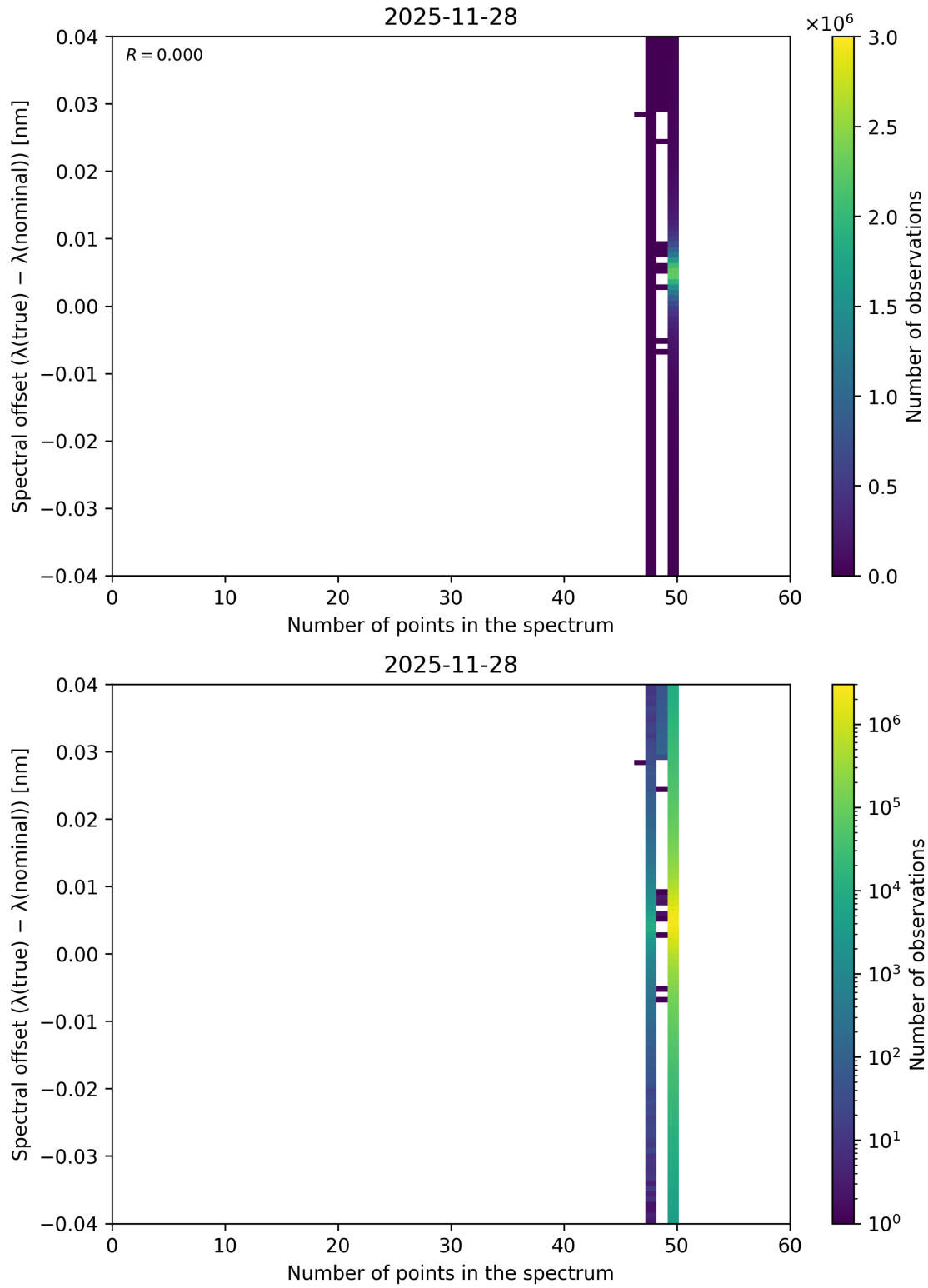
Figure 101: Scatter density plot of “Number of points in the spectrum” against “Spectral offset ( \lambda_{\text{true}} - \lambda_{\text{nominal}} )” for 2025-11-28 to 2025-11-29.
