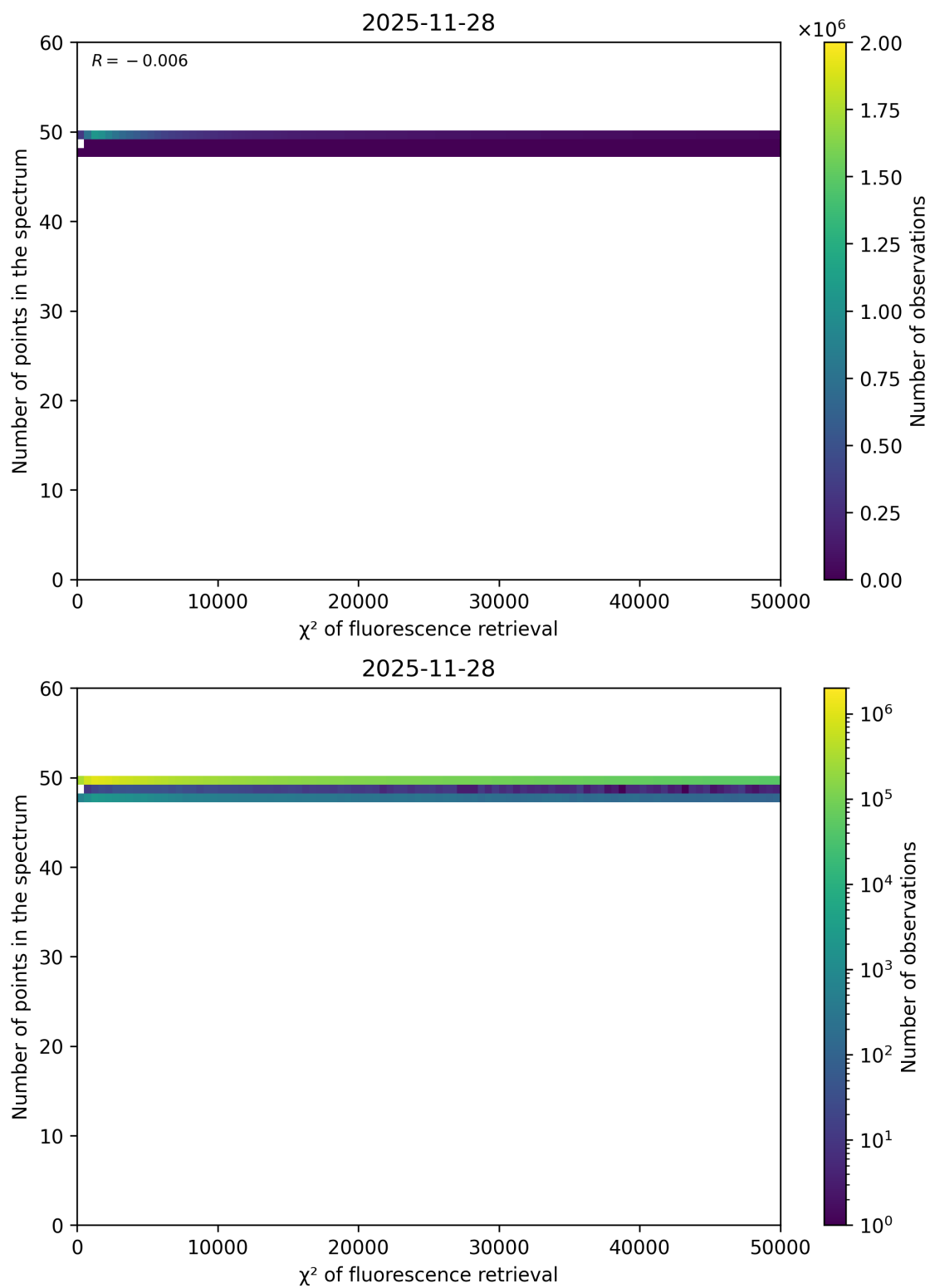
Figure 68: Scatter density plot of “ \chi^2 of fluorescence retrieval” against “Number of points in the spectrum” for 2025-11-28 to 2025-11-29.
