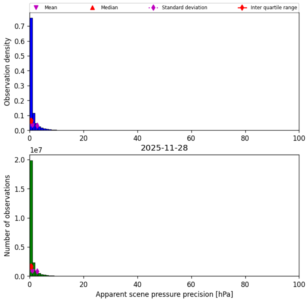
Figure 37: Histogram of “Apparent scene pressure precision” for 2025-11-28 to 2025-11-29
