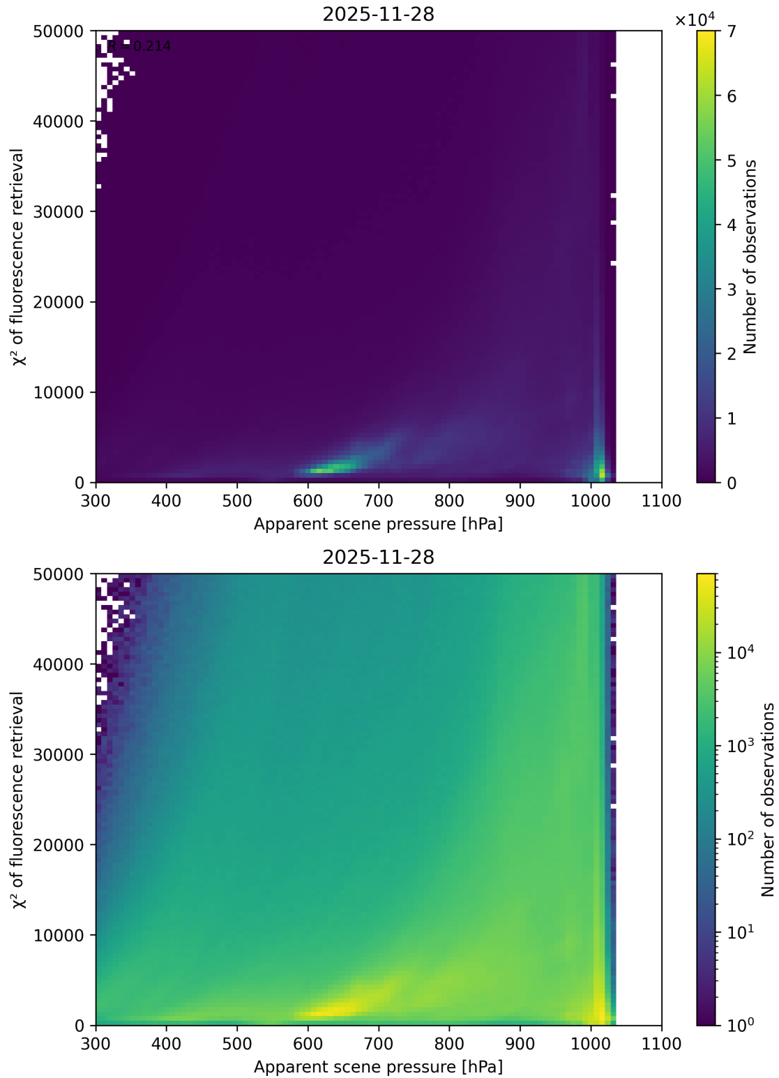
Figure 63: Scatter density plot of “Apparent scene pressure” against “ \chi^2 of fluorescence retrieval” for 2025-11-28 to 2025-11-29.
