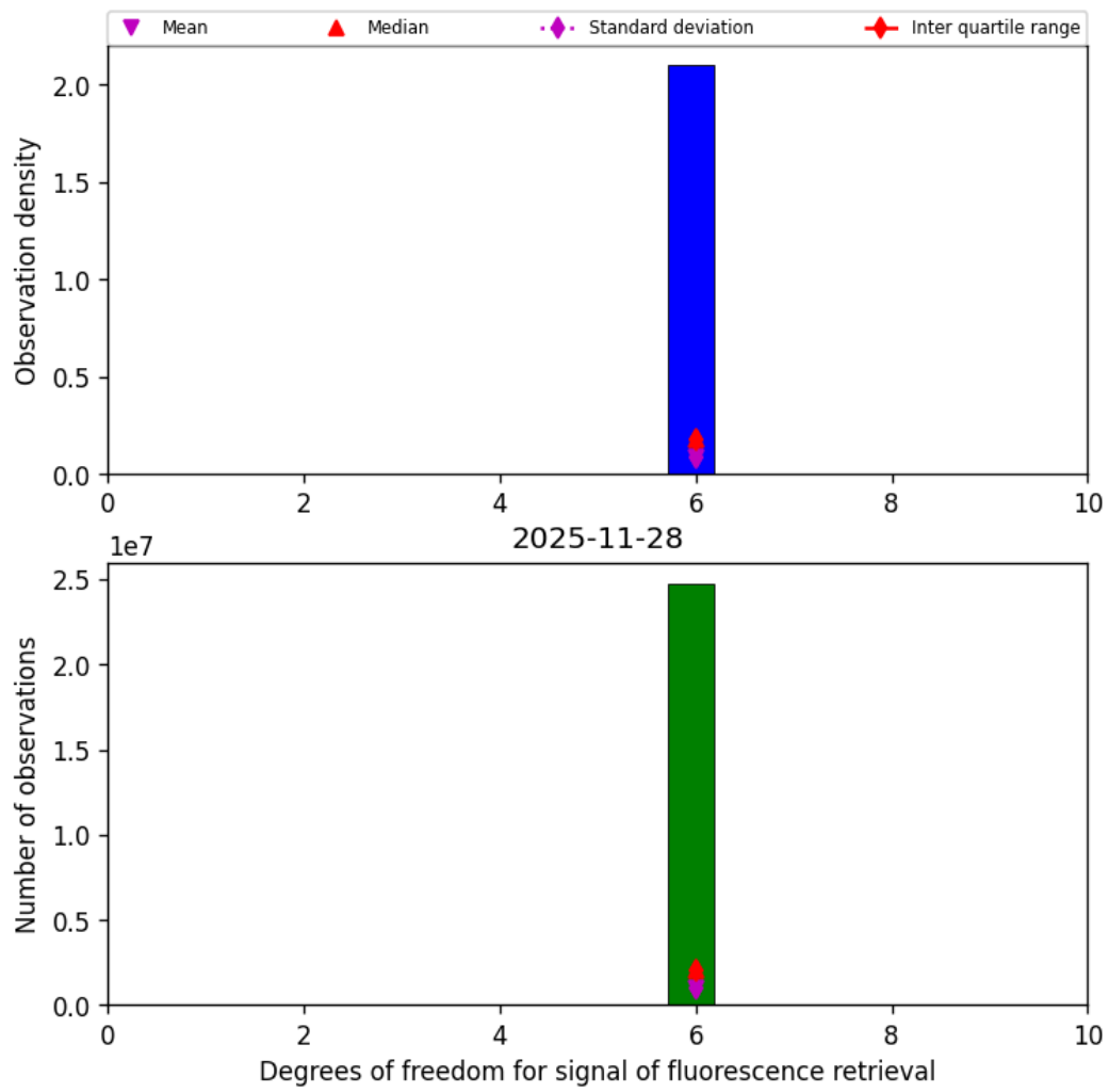
Figure 43: Histogram of “Degrees of freedom for signal of fluorescence retrieval” for 2025-11-28 to 2025-11-29
