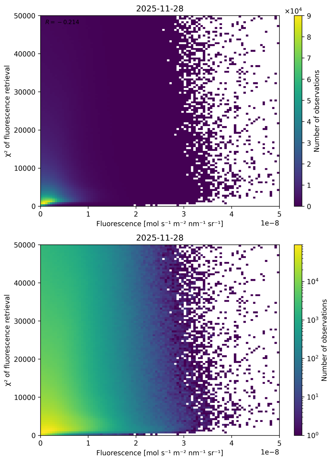
Figure 85: Scatter density plot of “Fluorescence” against “ \chi^2 of fluorescence retrieval” for 2025-11-28 to 2025-11-29.
