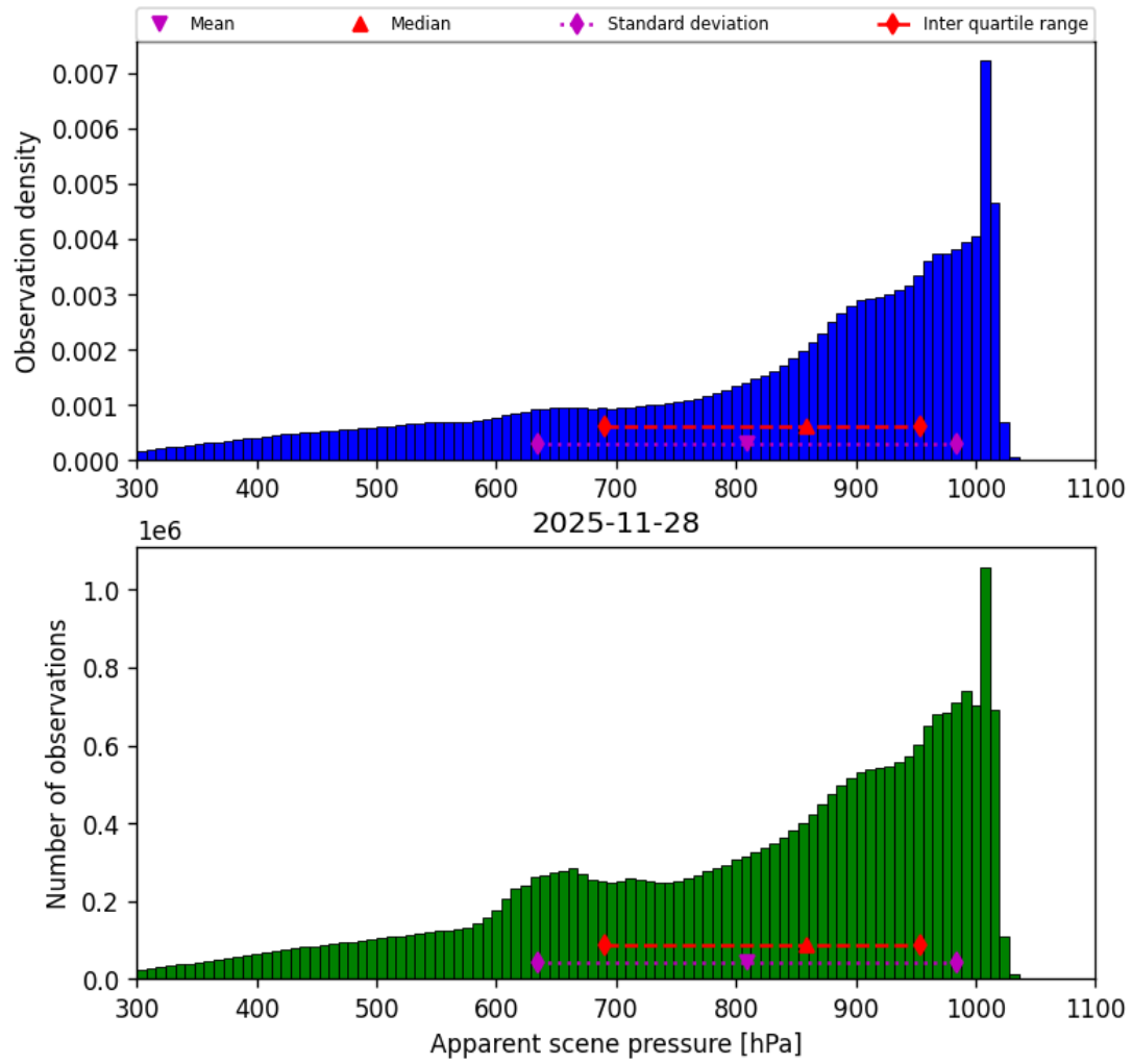
Figure 36: Histogram of “Apparent scene pressure” for 2025-11-28 to 2025-11-29
