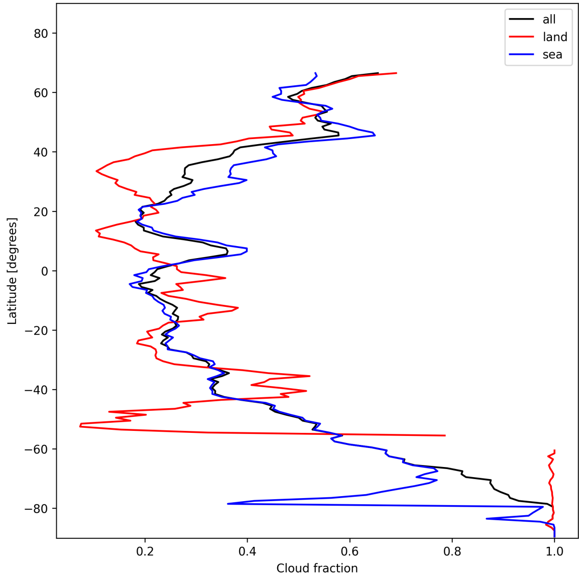
Figure 15: Zonal average of “Cloud fraction” for 2025-11-28 to 2025-11-29.
