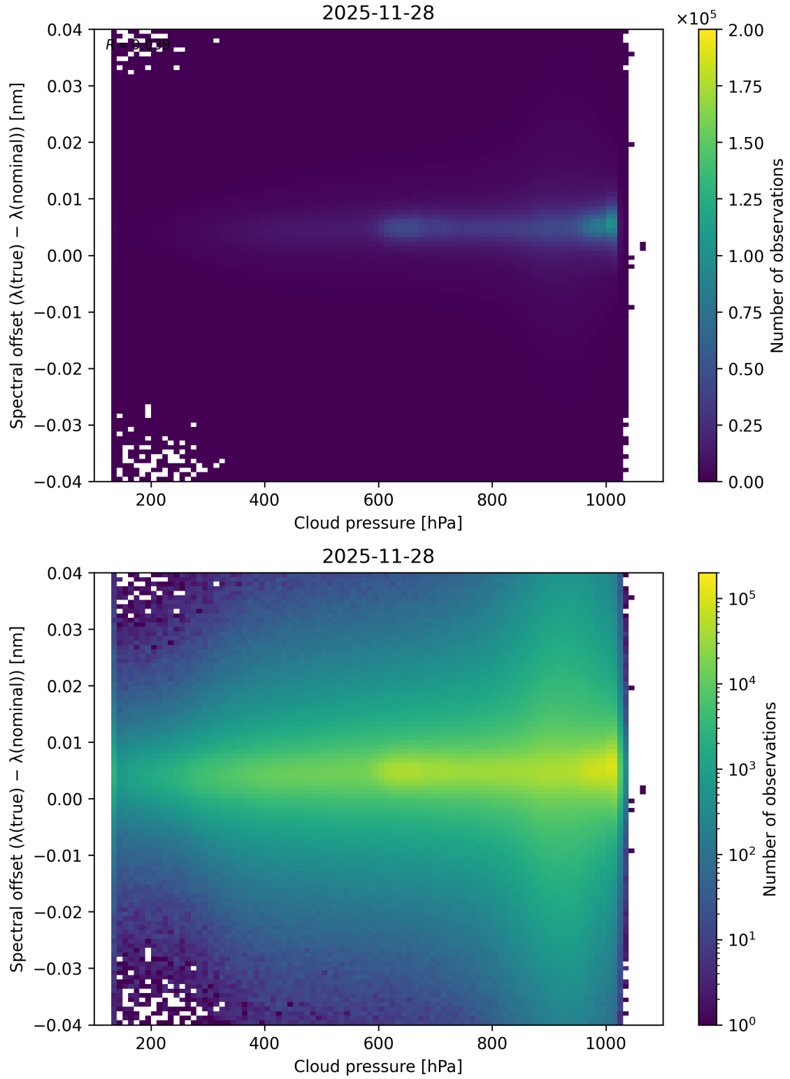
Figure 84: Scatter density plot of “Cloud pressure” against “Spectral offset ( \lambda_{\text{true}} - \lambda_{\text{nominal}} )” for 2025-11-28 to 2025-11-29.
