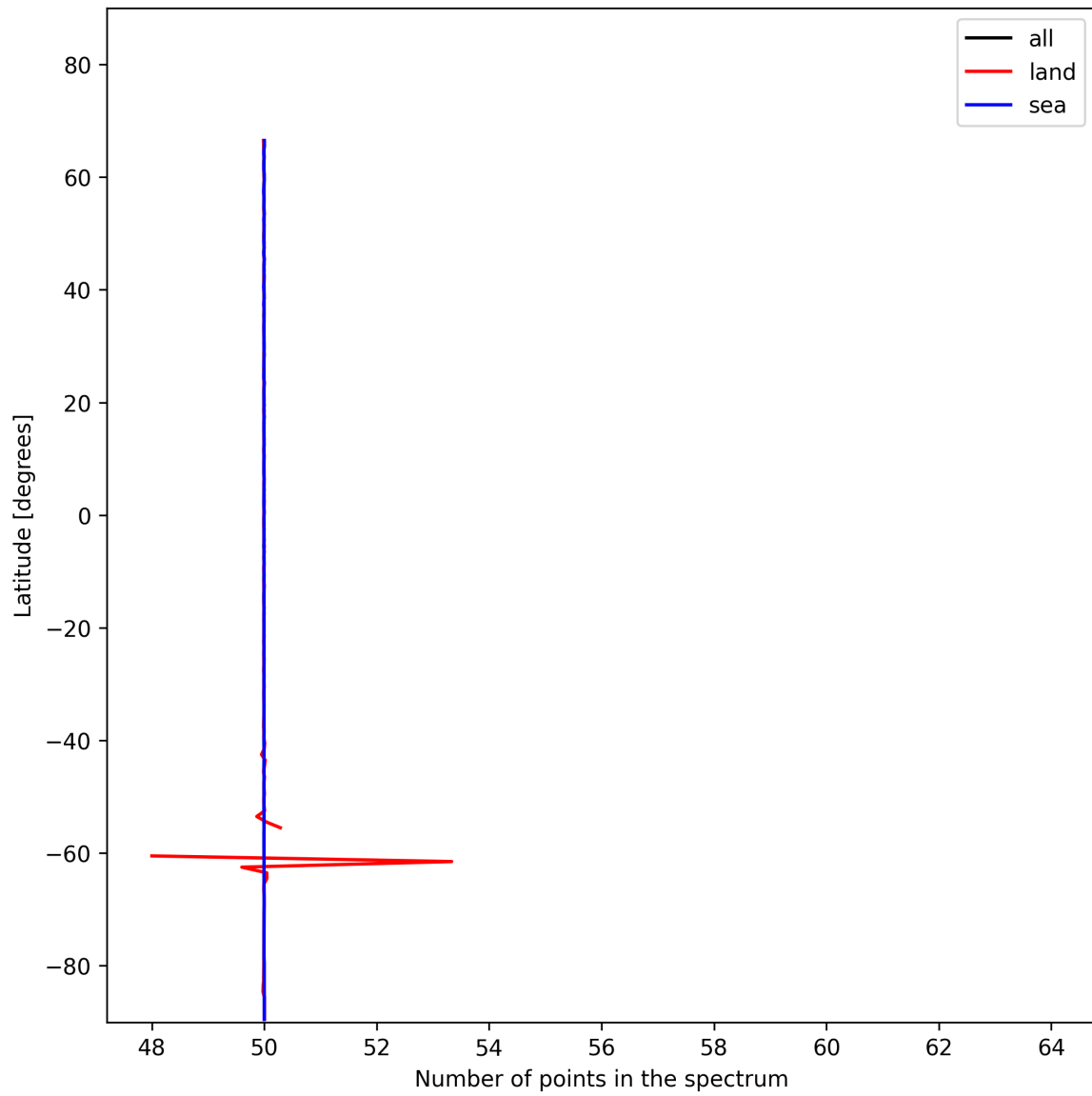
Figure 27: Zonal average of “Number of points in the spectrum” for 2025-11-28 to 2025-11-29.
