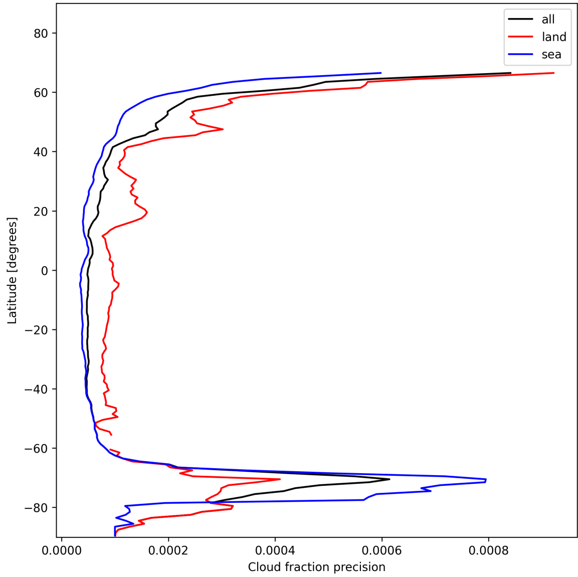
Figure 16: Zonal average of “Cloud fraction precision” for 2025-11-28 to 2025-11-29.
