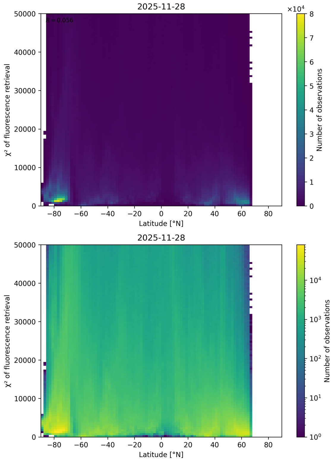
Figure 89: Scatter density plot of “Latitude” against “ \chi^2 of fluorescence retrieval” for 2025-11-28 to 2025-11-29.
