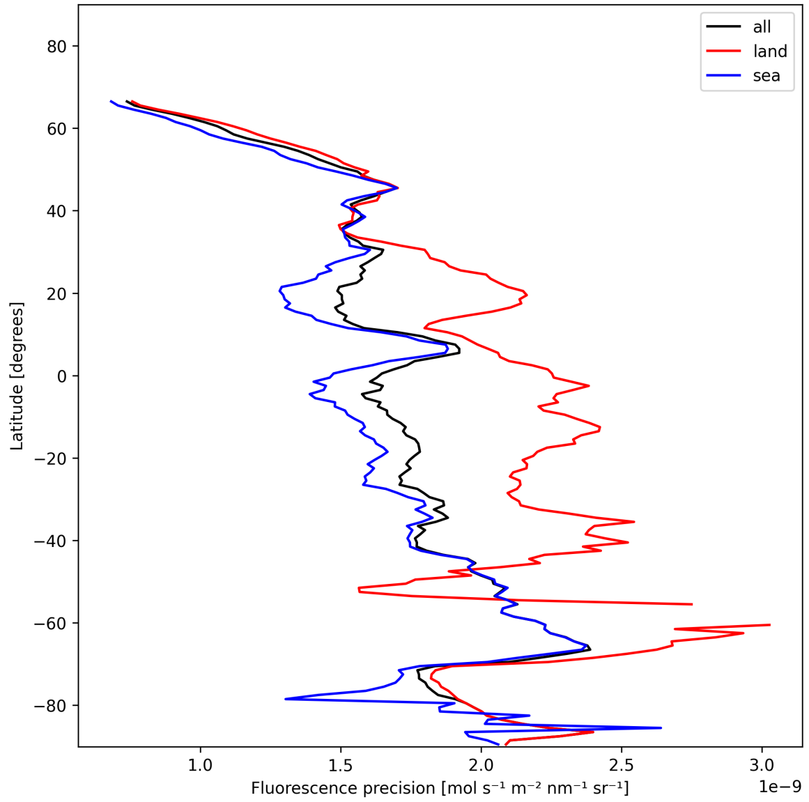
Figure 24: Zonal average of “Fluorescence precision” for 2025-11-28 to 2025-11-29.
