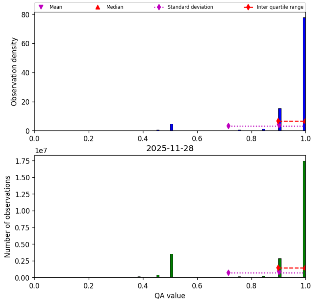
Figure 29: Histogram of “QA value” for 2025-11-28 to 2025-11-29
