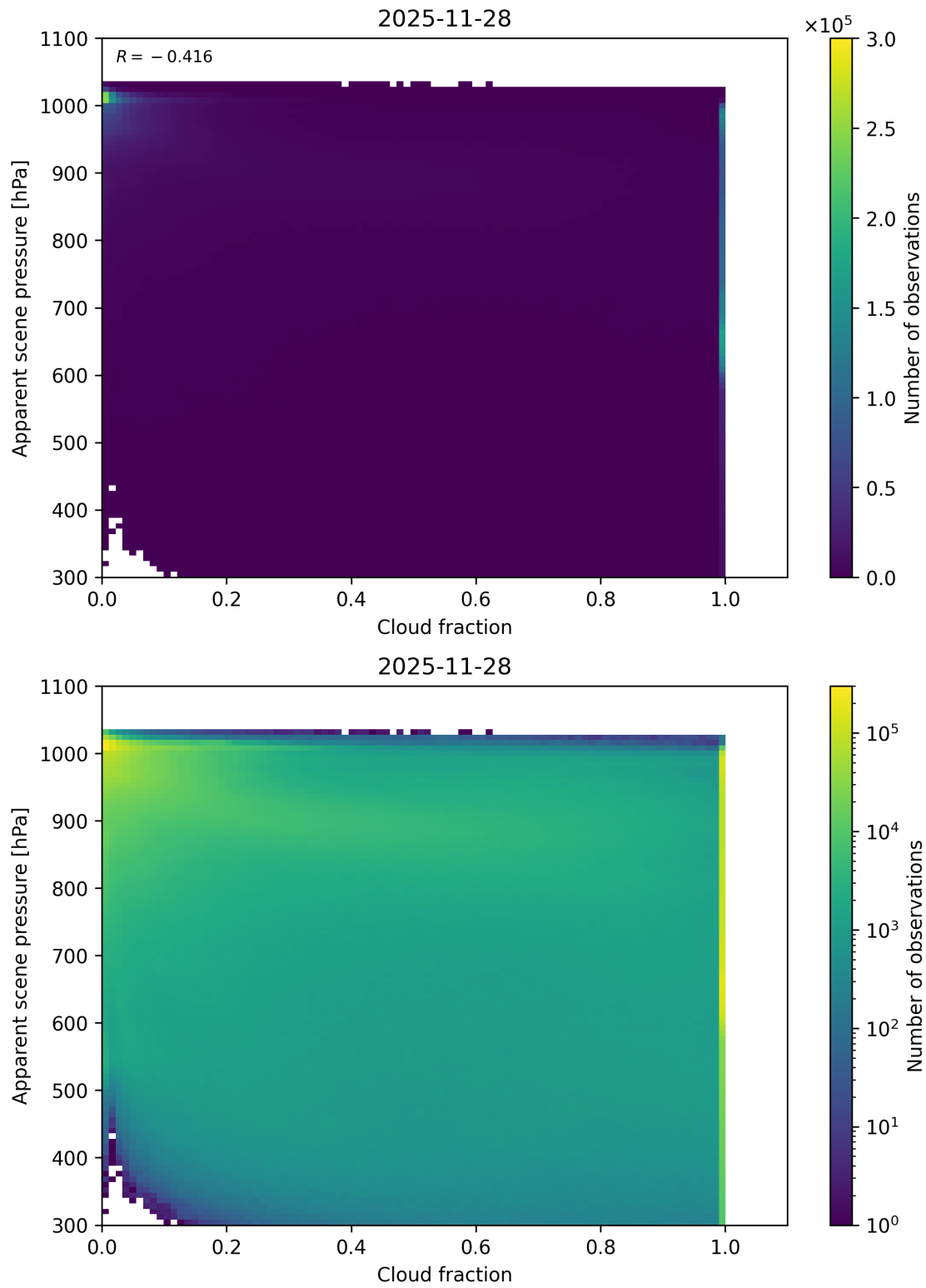
Figure 70: Scatter density plot of “Cloud fraction” against “Apparent scene pressure” for 2025-11-28 to 2025-11-29.
