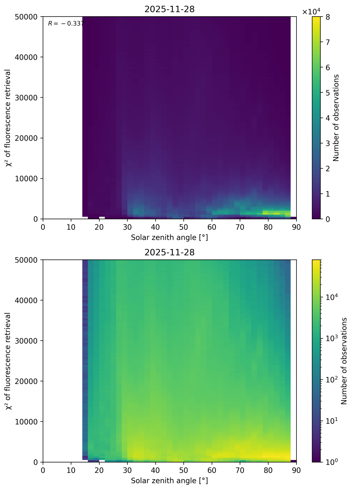
Figure 109: Scatter density plot of “Solar zenith angle” against “ \chi^2 of fluorescence retrieval” for 2025-11-28 to 2025-11-29.
