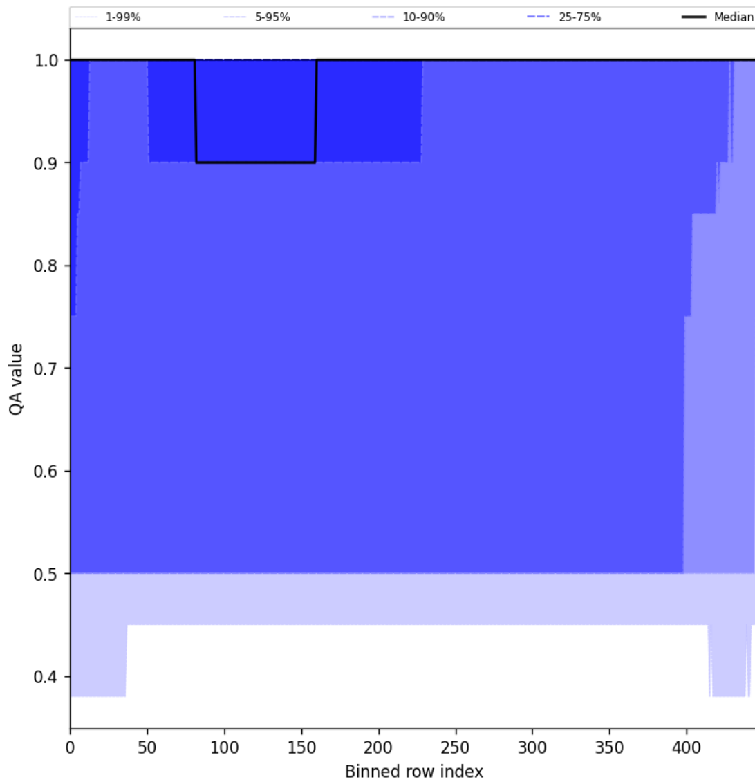
Figure 46: Along track statistics of “QA value” for 2025-11-28 to 2025-11-29
