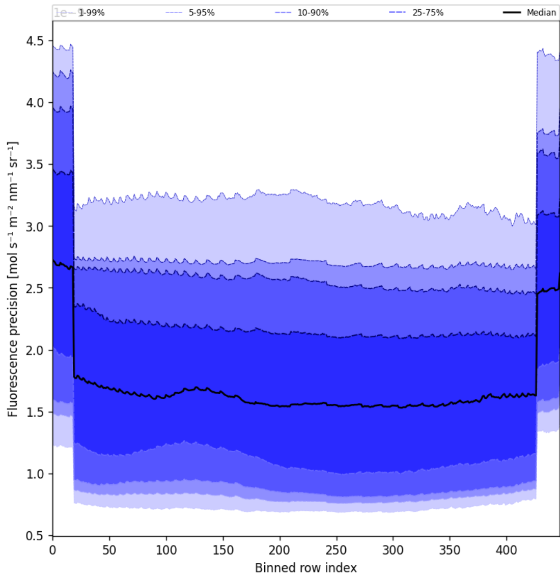
Figure 58: Along track statistics of “Fluorescence precision” for 2025-11-28 to 2025-11-29
