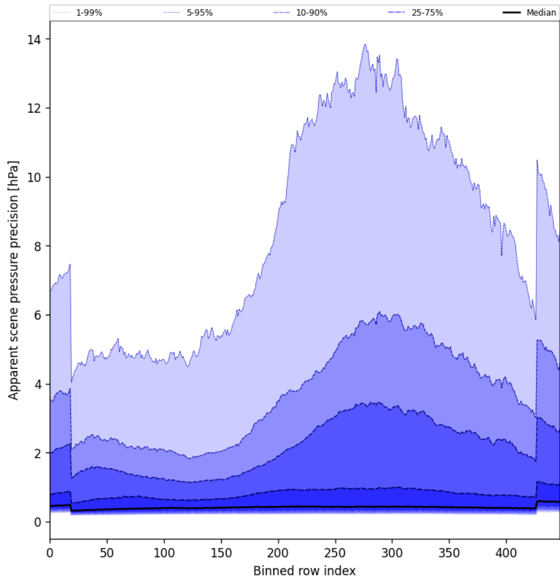
Figure 54: Along track statistics of “Apparent scene pressure precision” for 2025-11-28 to 2025-11-29
