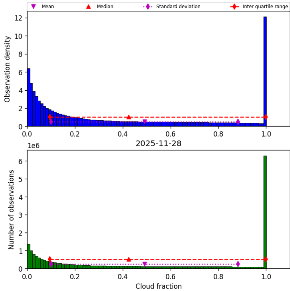
Figure 32: Histogram of “Cloud fraction” for 2025-11-28 to 2025-11-29
