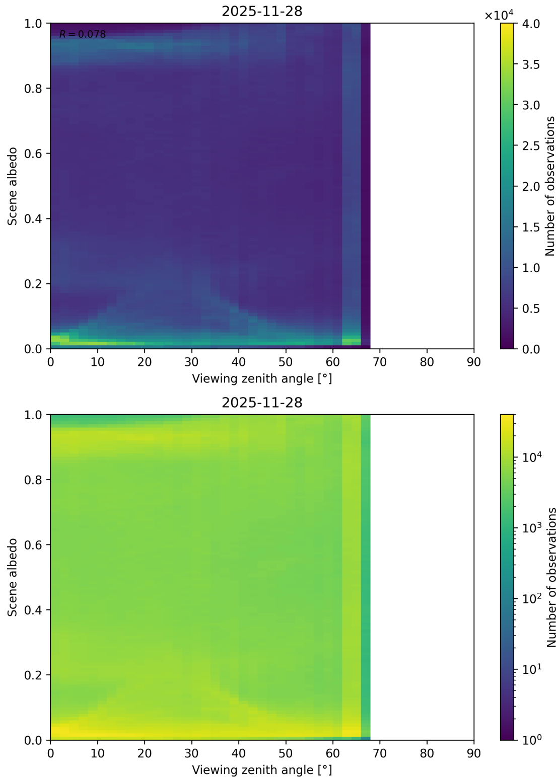
Figure 126: Scatter density plot of “Viewing zenith angle” against “Scene albedo” for 2025-11-28 to 2025-11-29.
