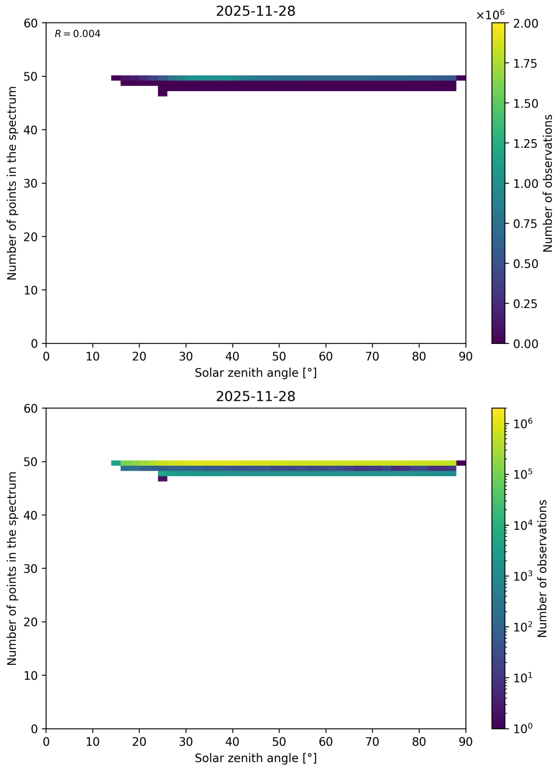
Figure 115: Scatter density plot of “Solar zenith angle” against “Number of points in the spectrum” for 2025-11-28 to 2025-11-29.
