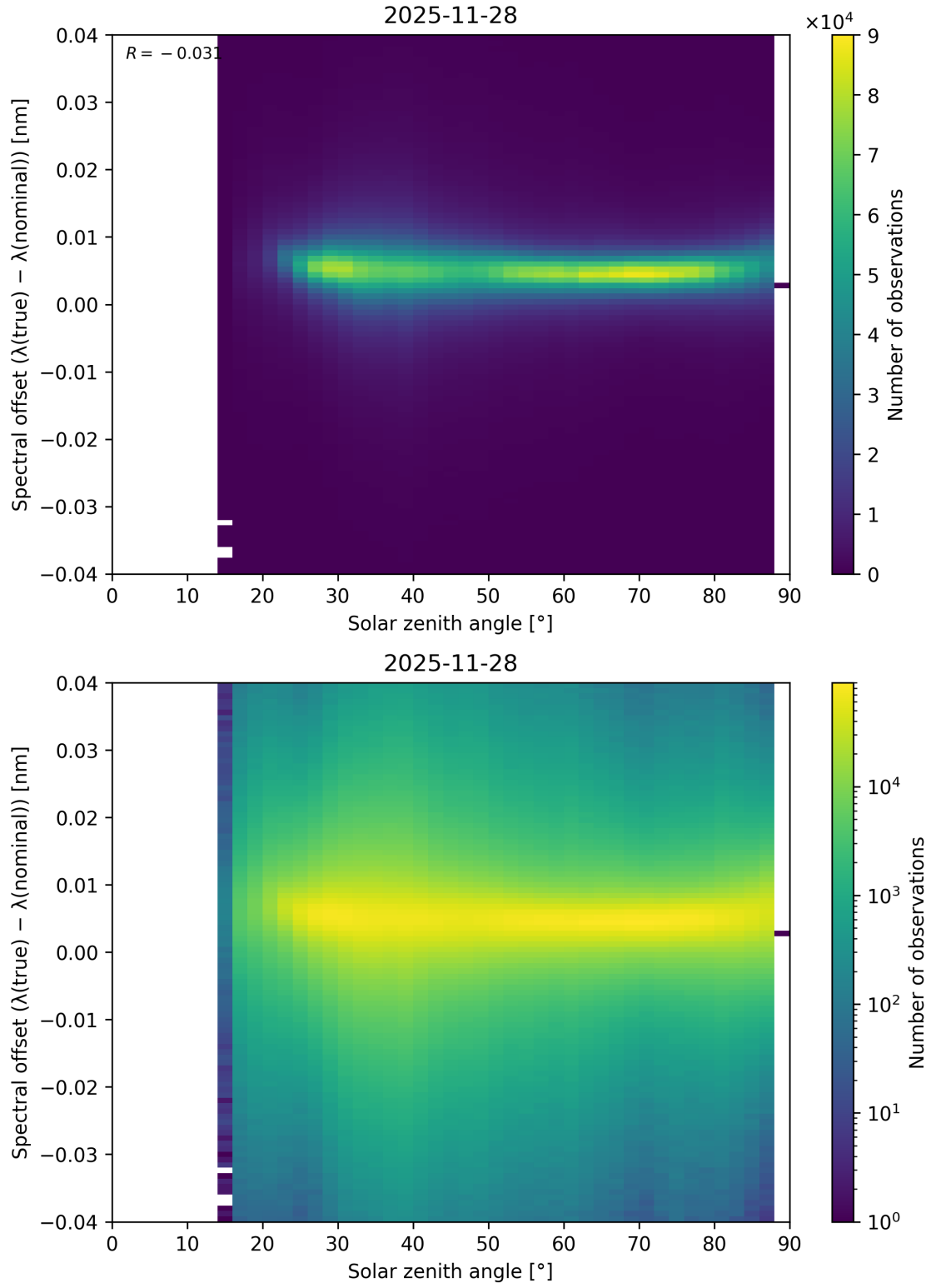
Figure 117: Scatter density plot of “Solar zenith angle” against “Spectral offset ( \lambda_{\text{true}} - \lambda_{\text{nominal}} )” for 2025-11-28 to 2025-11-29.
