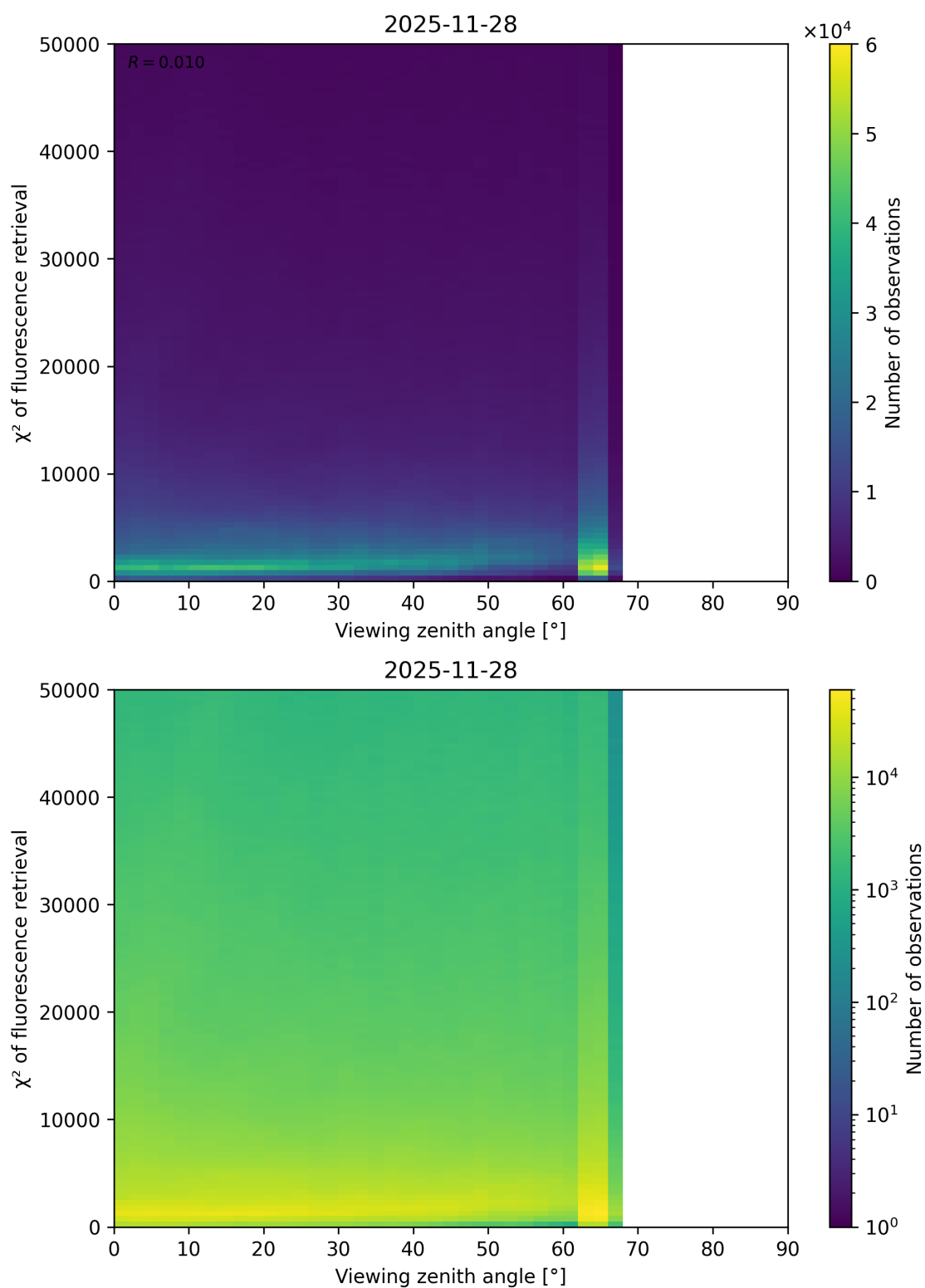
Figure 119: Scatter density plot of “Viewing zenith angle” against “ \chi^2 of fluorescence retrieval” for 2025-11-28 to 2025-11-29.
