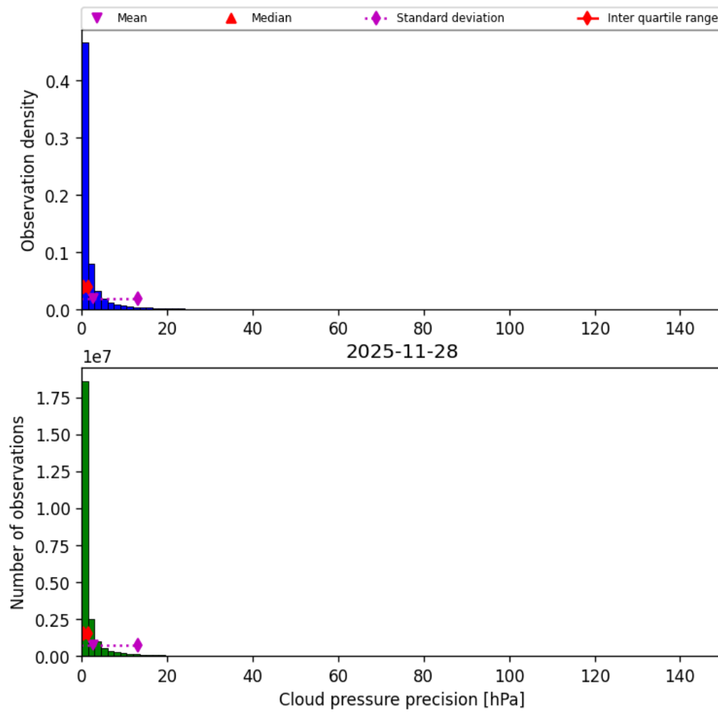
Figure 31: Histogram of “Cloud pressure precision” for 2025-11-28 to 2025-11-29
