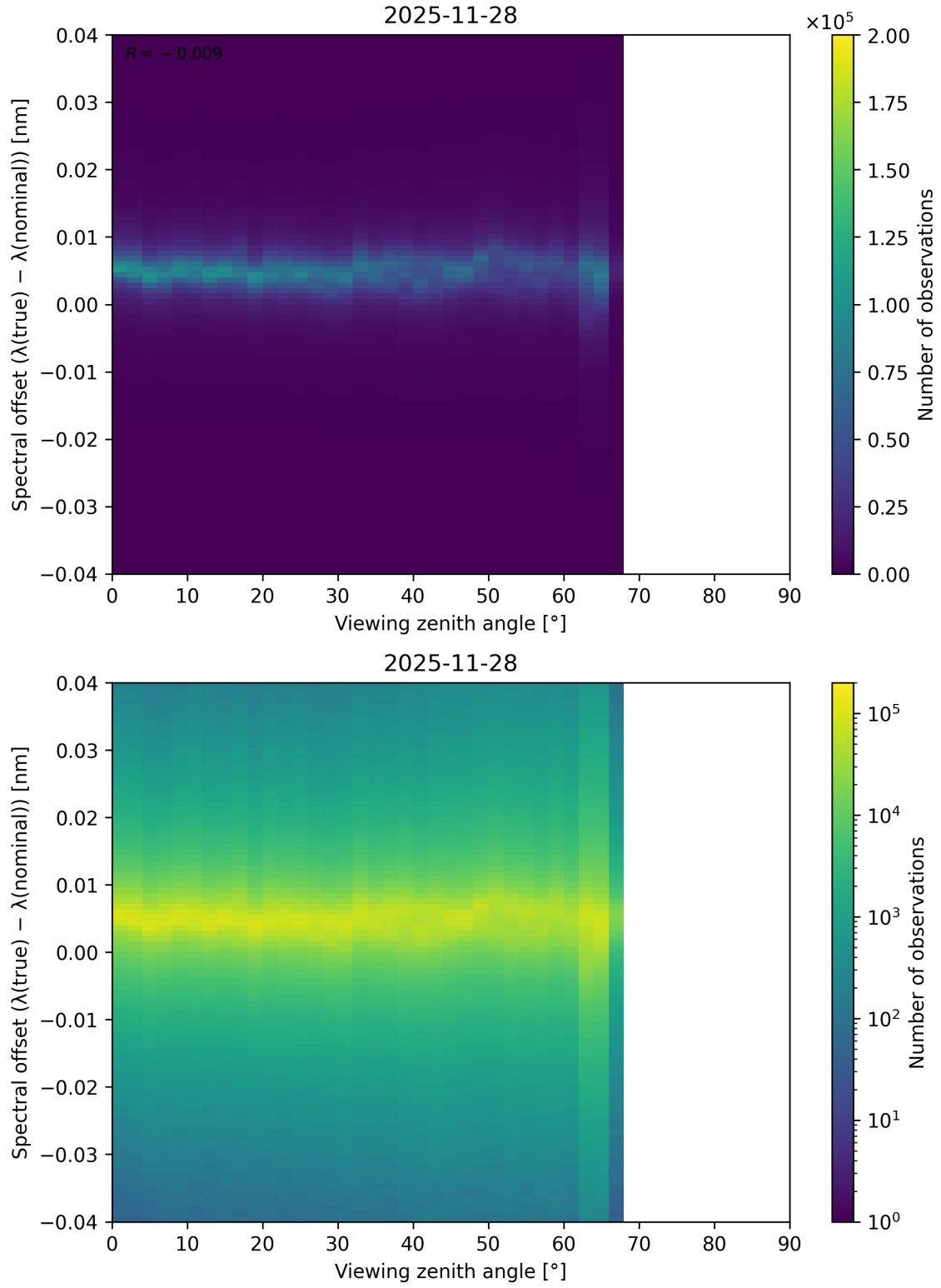
Figure 128: Scatter density plot of “Viewing zenith angle” against “Spectral offset ( \lambda_{\text{true}} - \lambda_{\text{nominal}} )” for 2025-11-28 to 2025-11-29.
