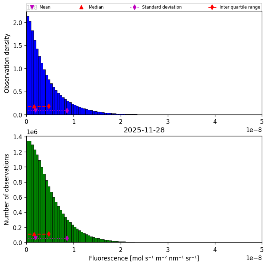
Figure 40: Histogram of “Fluorescence” for 2025-11-28 to 2025-11-29
