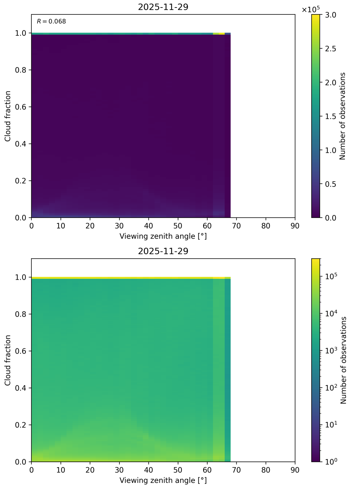
Figure 120: Scatter density plot of “Viewing zenith angle” against “Cloud fraction” for 2025-11-28 to 2025-11-30.
