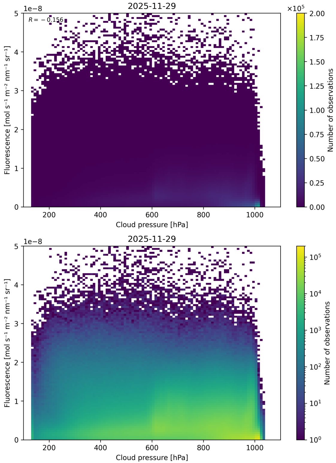
Figure 80: Scatter density plot of “Cloud pressure” against “Fluorescence” for 2025-11-28 to 2025-11-30.
