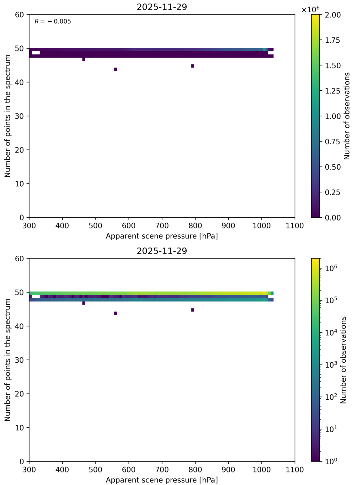
Figure 66: Scatter density plot of “Apparent scene pressure” against “Number of points in the spectrum” for 2025-11-28 to 2025-11-30.
