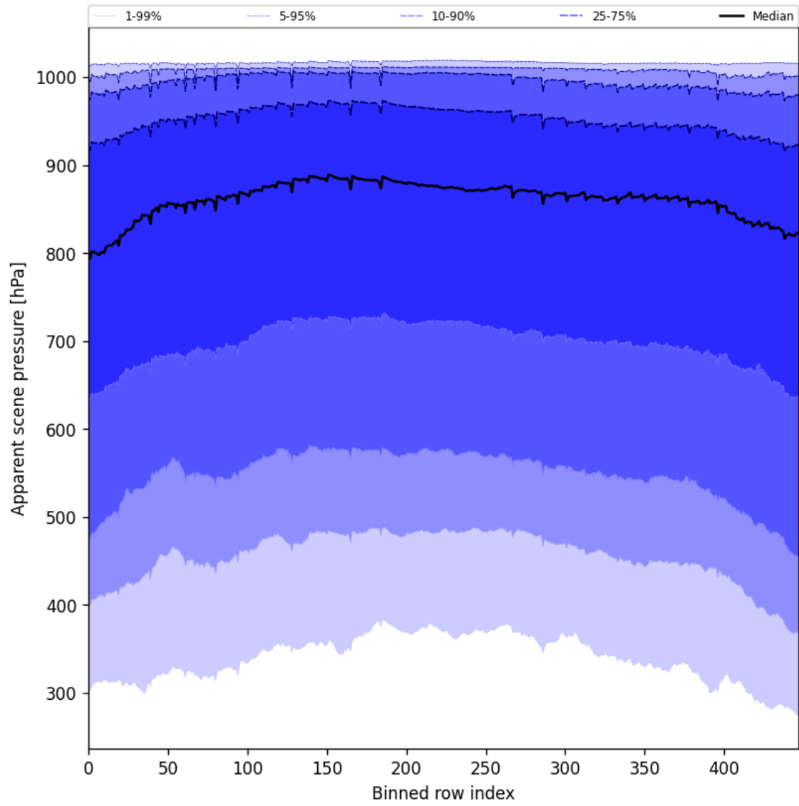
Figure 53: Along track statistics of “Apparent scene pressure” for 2025-11-28 to 2025-11-30
