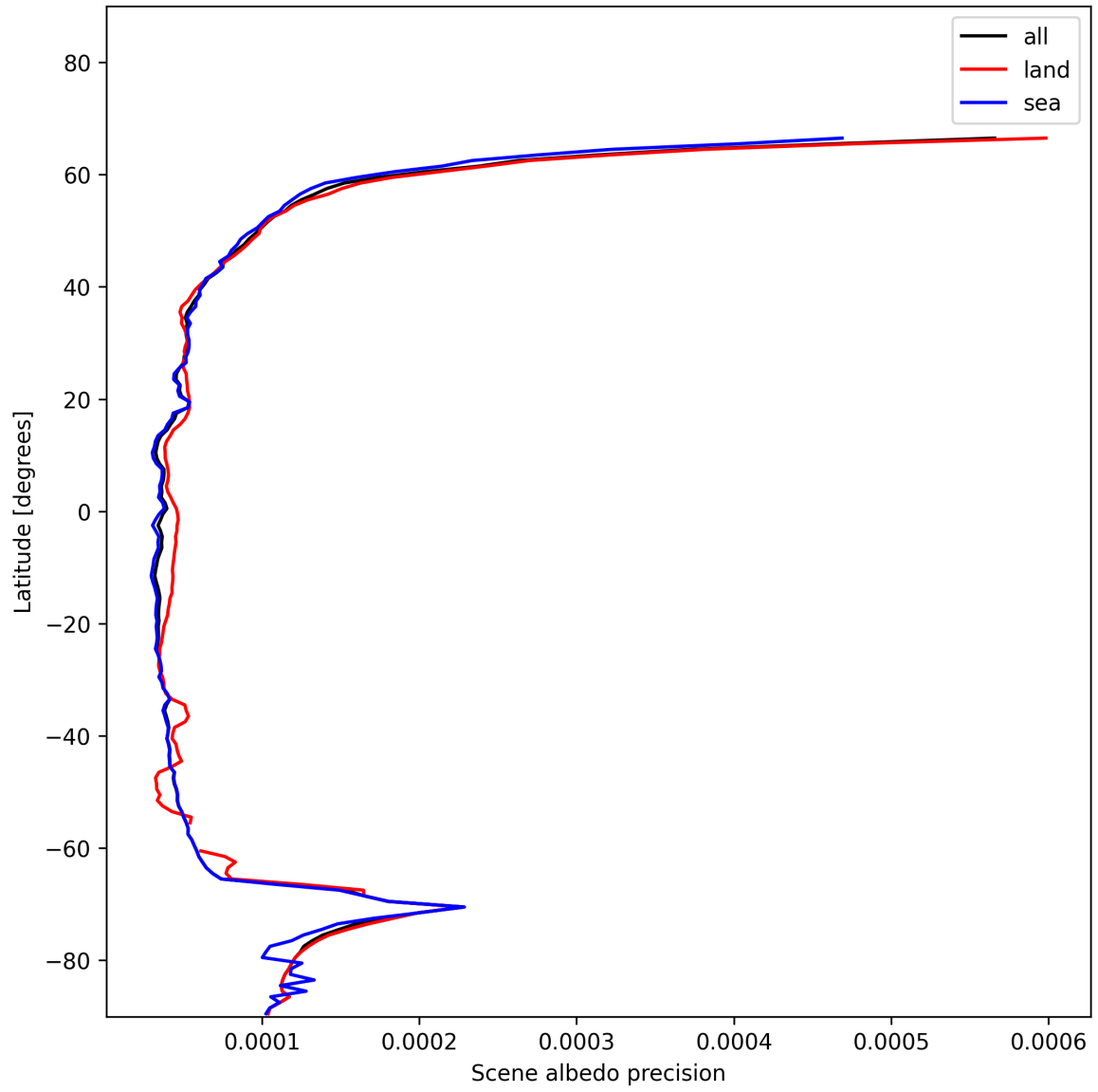
Figure 18: Zonal average of “Scene albedo precision” for 2025-11-28 to 2025-11-30.
