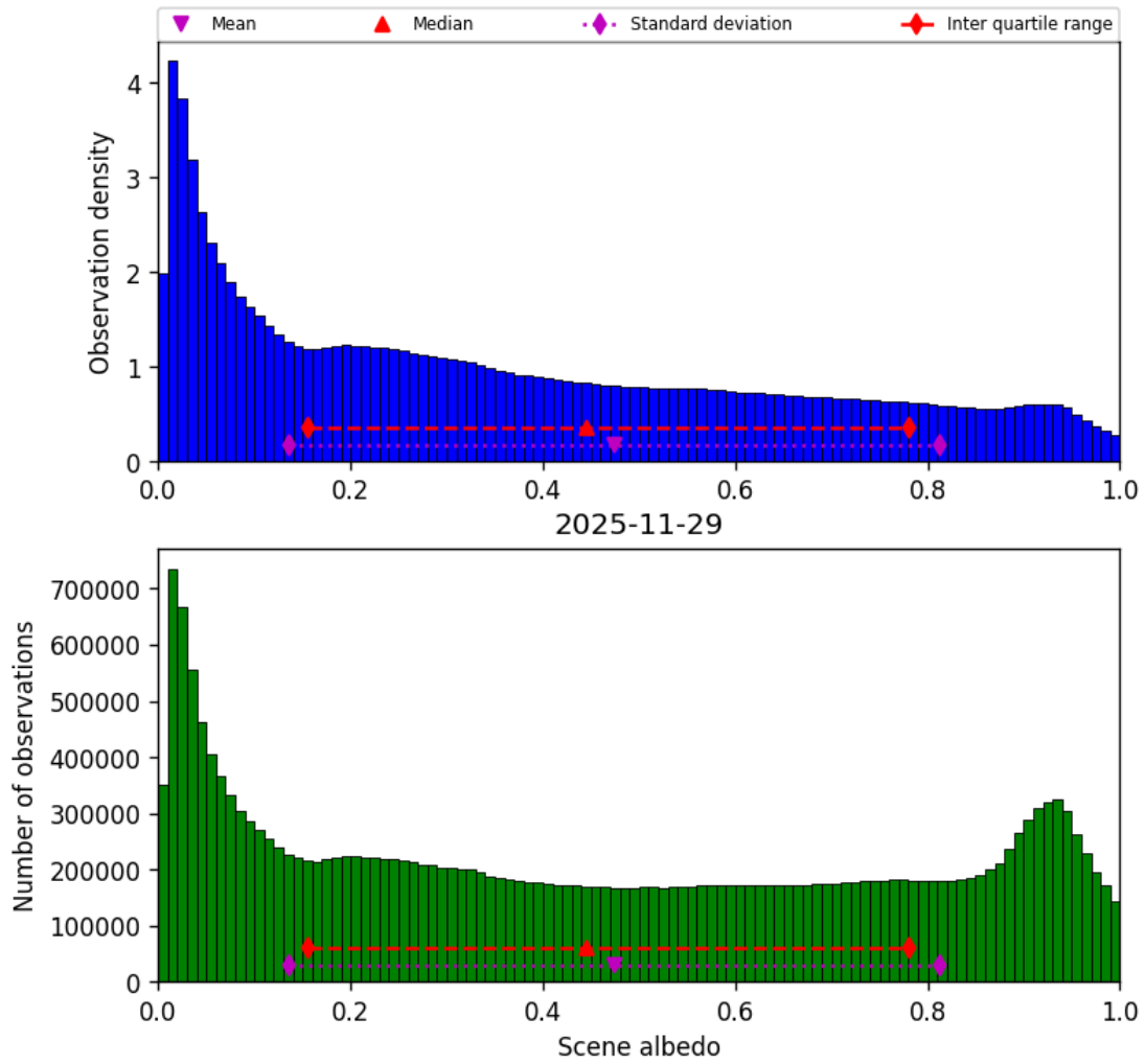
Figure 34: Histogram of “Scene albedo” for 2025-11-28 to 2025-11-30
