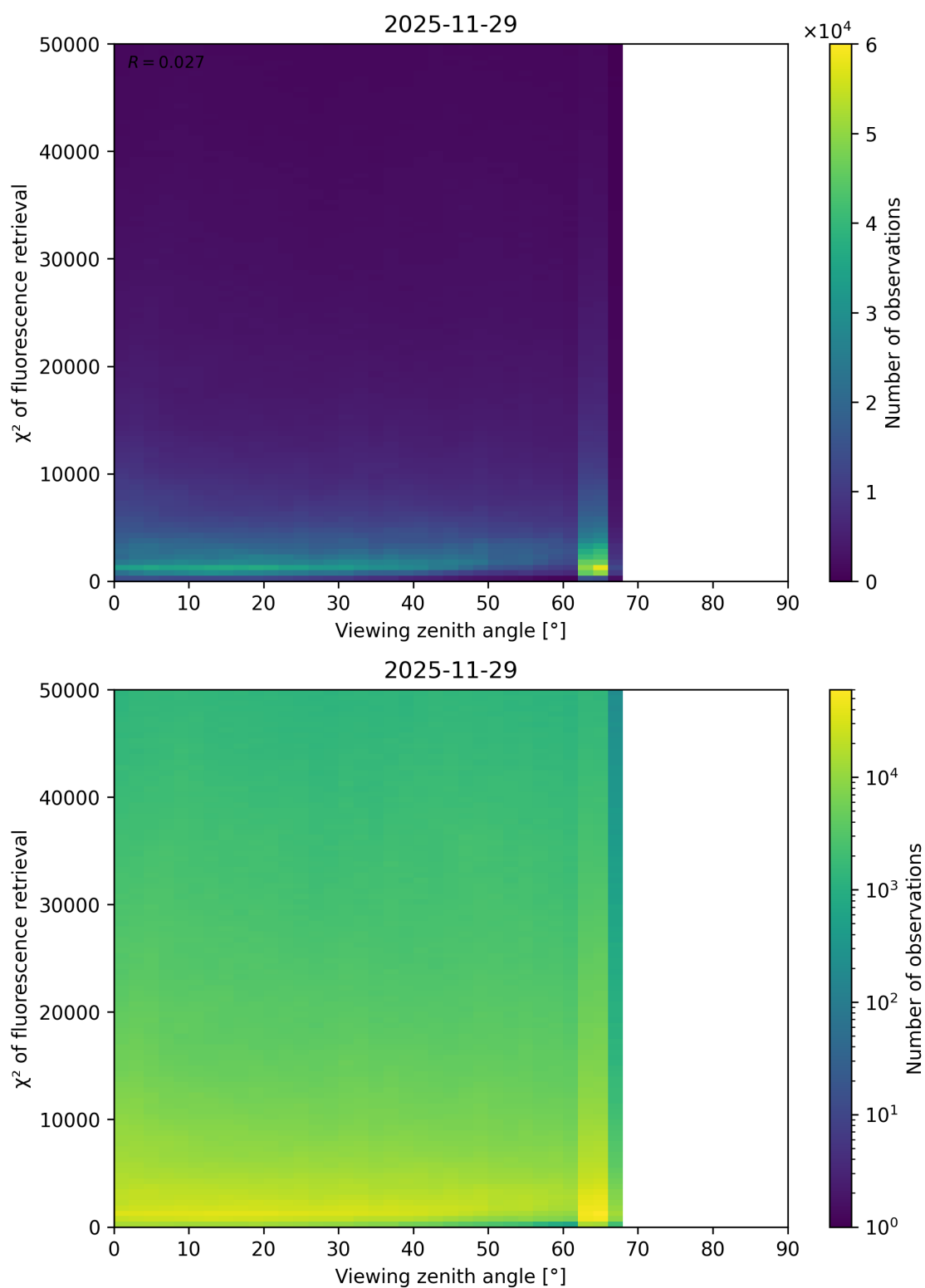
Figure 119: Scatter density plot of “Viewing zenith angle” against “ \chi^2 of fluorescence retrieval” for 2025-11-28 to 2025-11-30.
