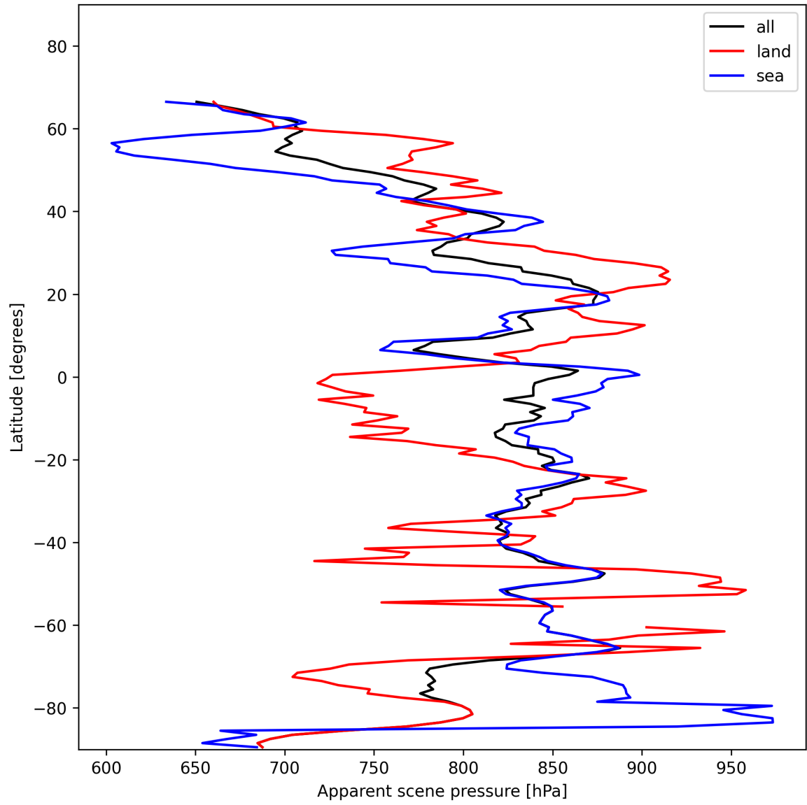
Figure 19: Zonal average of “Apparent scene pressure” for 2025-11-28 to 2025-11-30.
