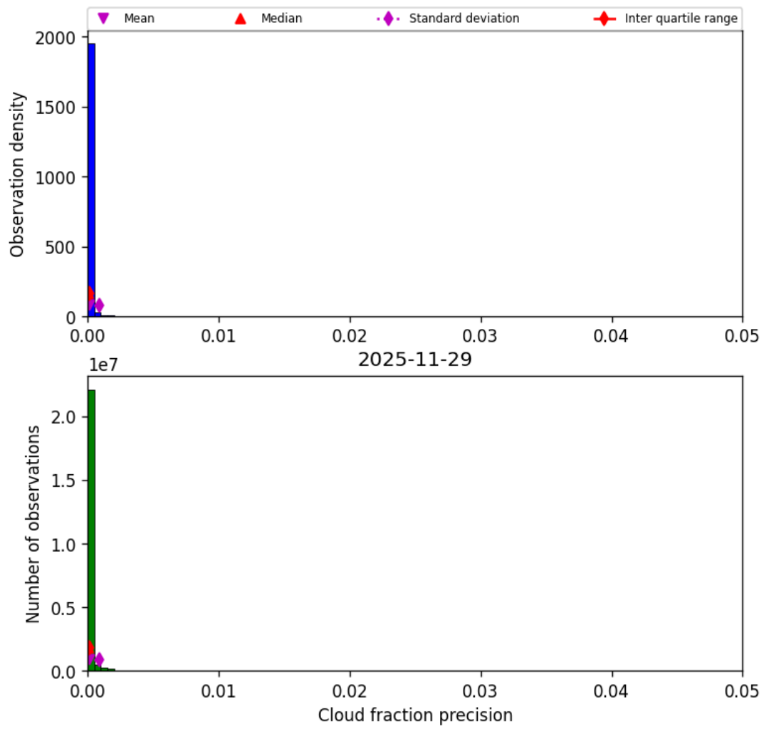
Figure 33: Histogram of “Cloud fraction precision” for 2025-11-28 to 2025-11-30
