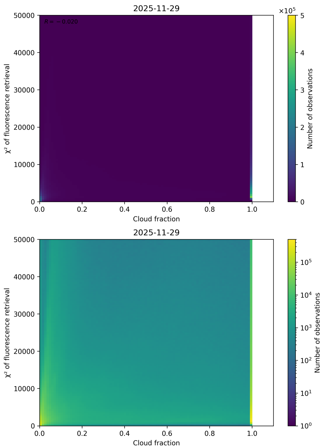
Figure 71: Scatter density plot of “Cloud fraction” against “ \chi^2 of fluorescence retrieval” for 2025-11-28 to 2025-11-30.
