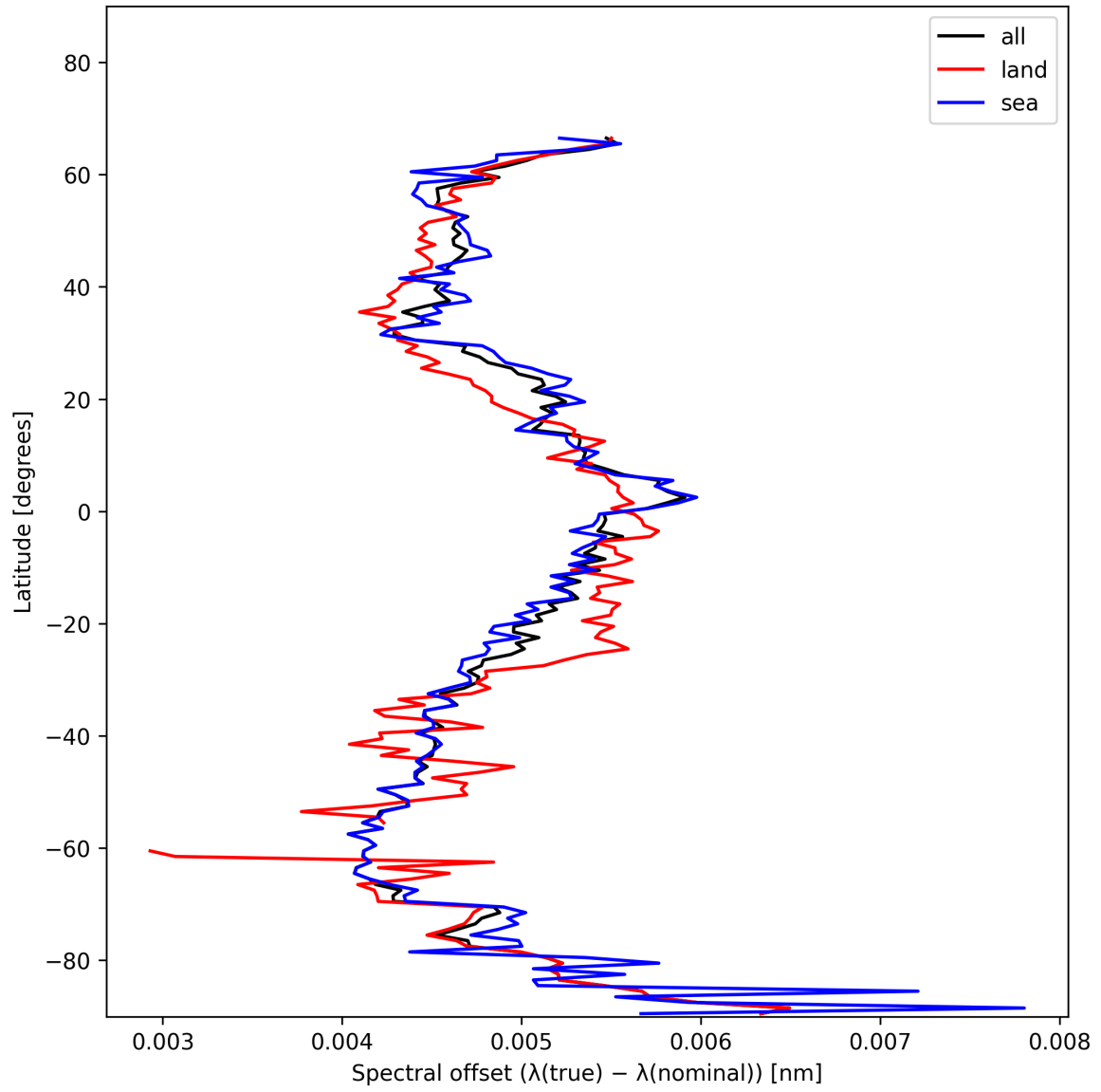
Figure 28: Zonal average of “Spectral offset ( \lambda_{\text{true}} - \lambda_{\text{nominal}} )” for 2025-11-28 to 2025-11-30.
