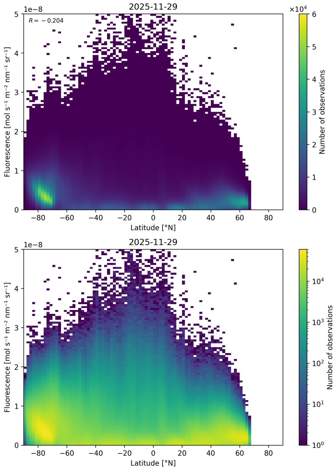
Figure 92: Scatter density plot of “Latitude” against “Fluorescence” for 2025-11-28 to 2025-11-30.
