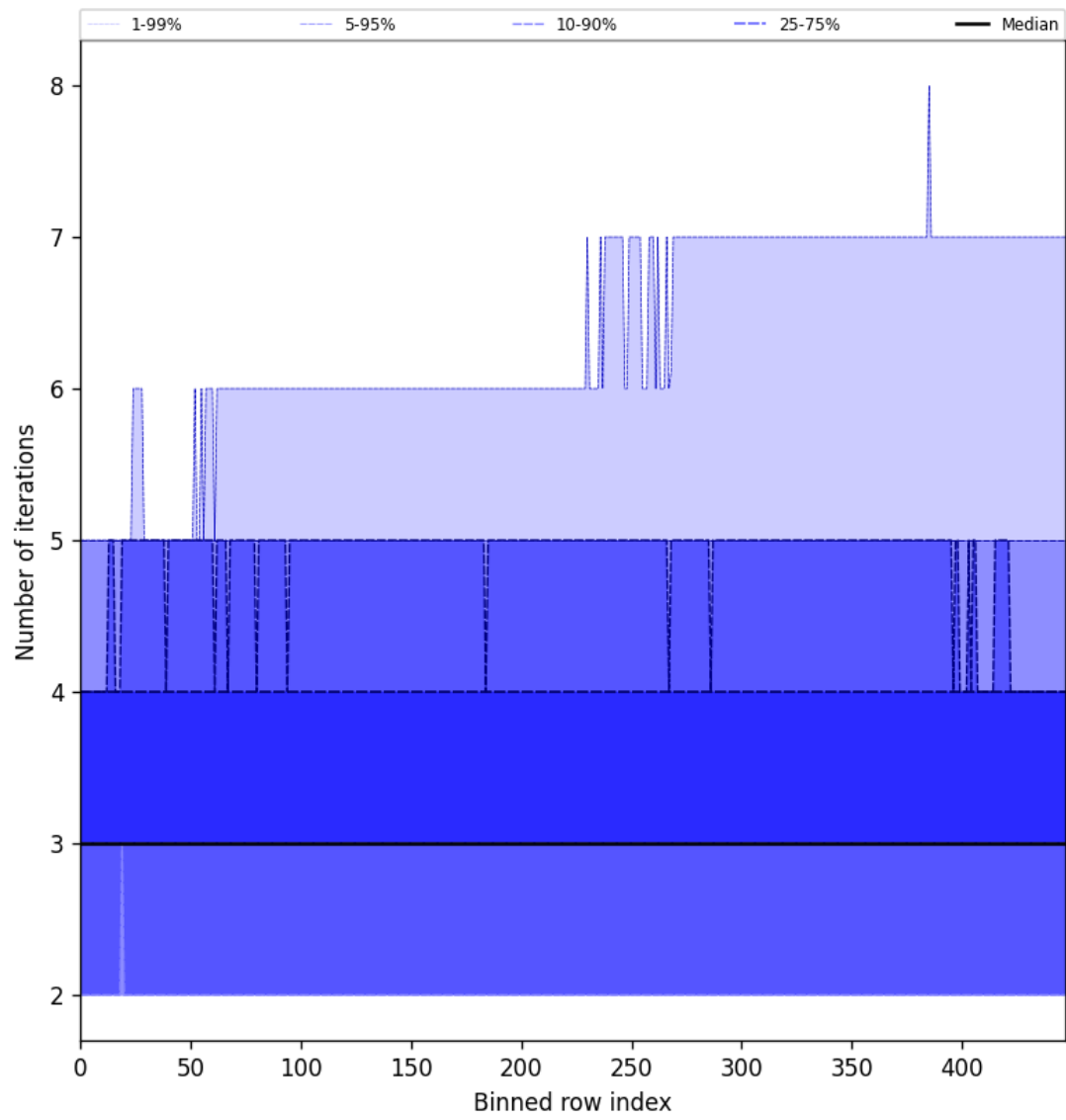
Figure 56: Along track statistics of “Number of iterations” for 2025-11-28 to 2025-11-30
