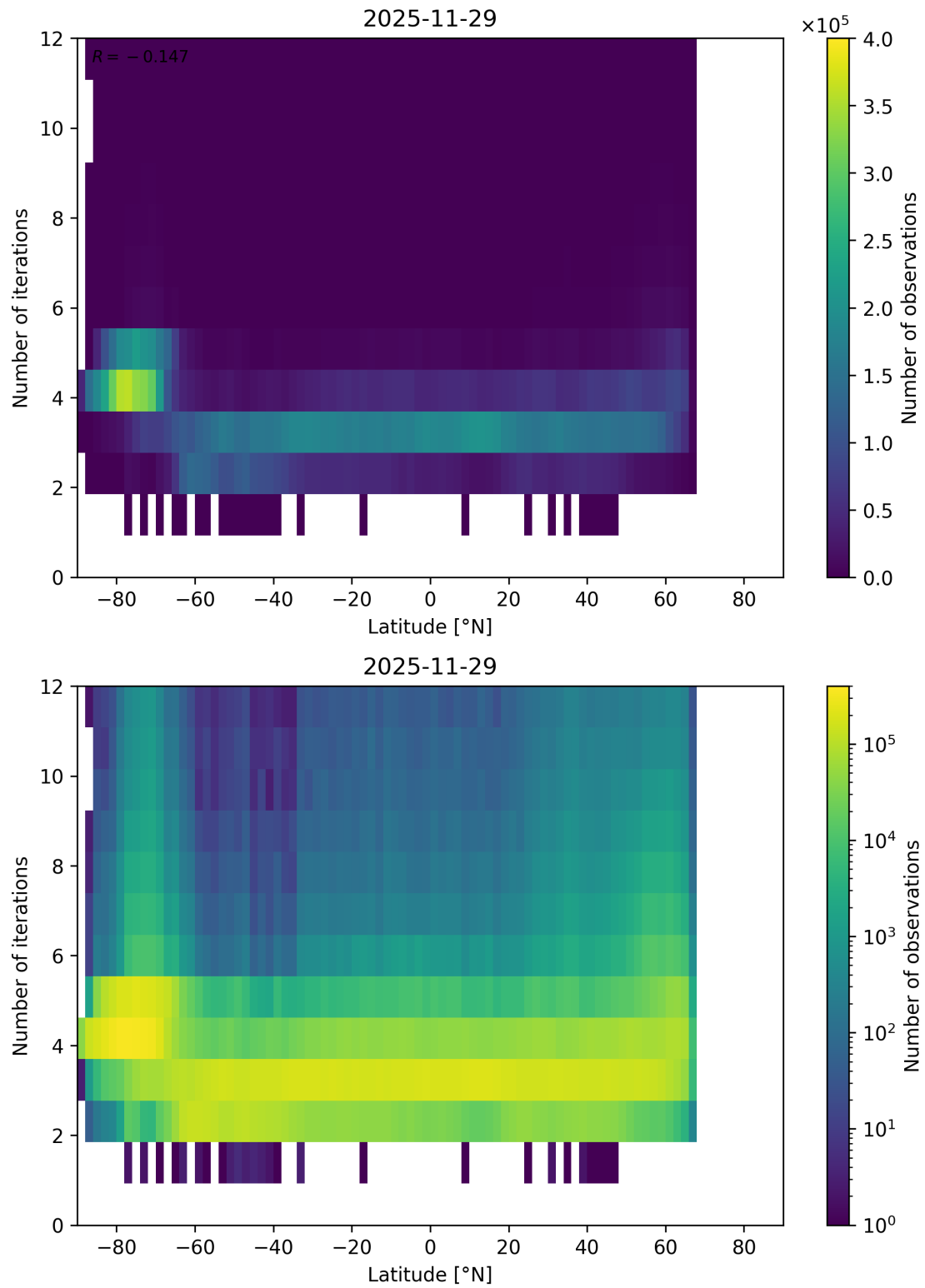
Figure 93: Scatter density plot of “Latitude” against “Number of iterations” for 2025-11-28 to 2025-11-30.
