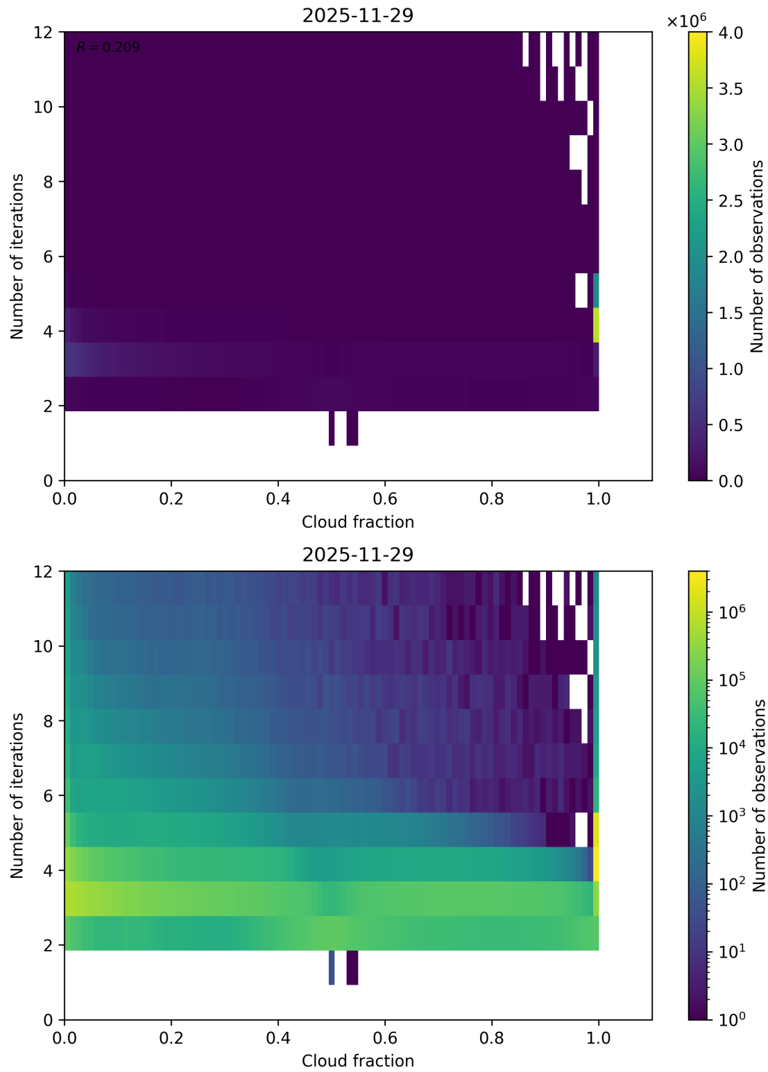
Figure 73: Scatter density plot of “Cloud fraction” against “Number of iterations” for 2025-11-28 to 2025-11-30.
