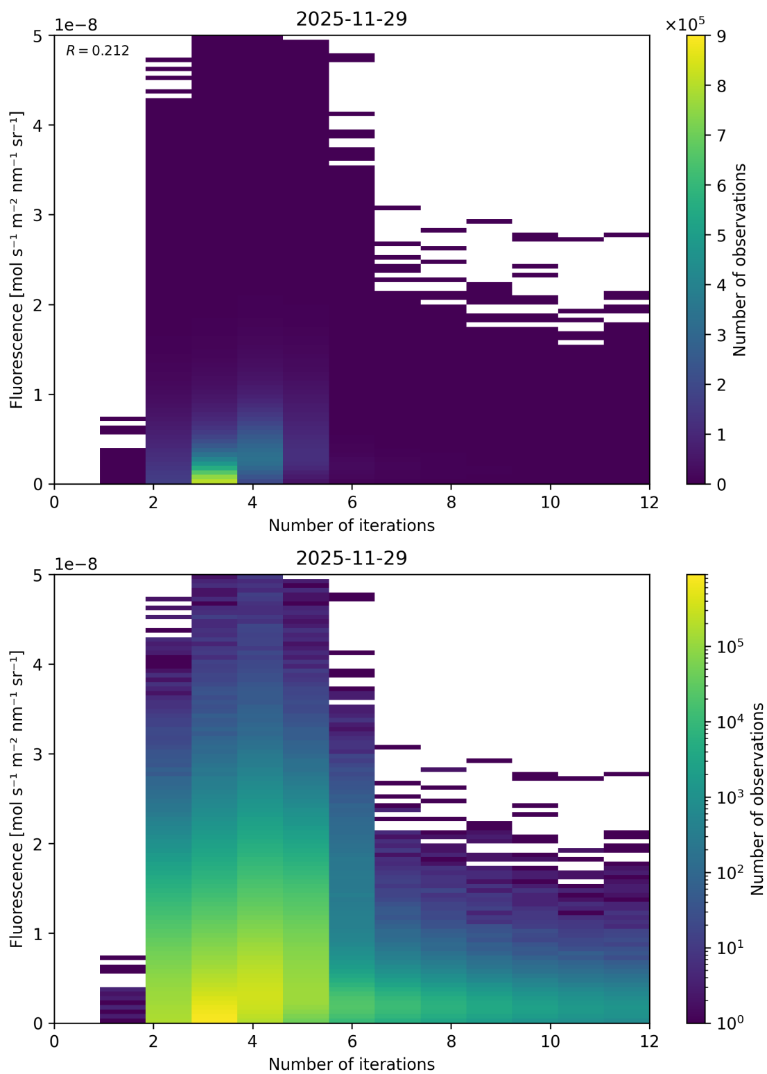
Figure 98: Scatter density plot of “Number of iterations” against “Fluorescence” for 2025-11-28 to 2025-11-30.
