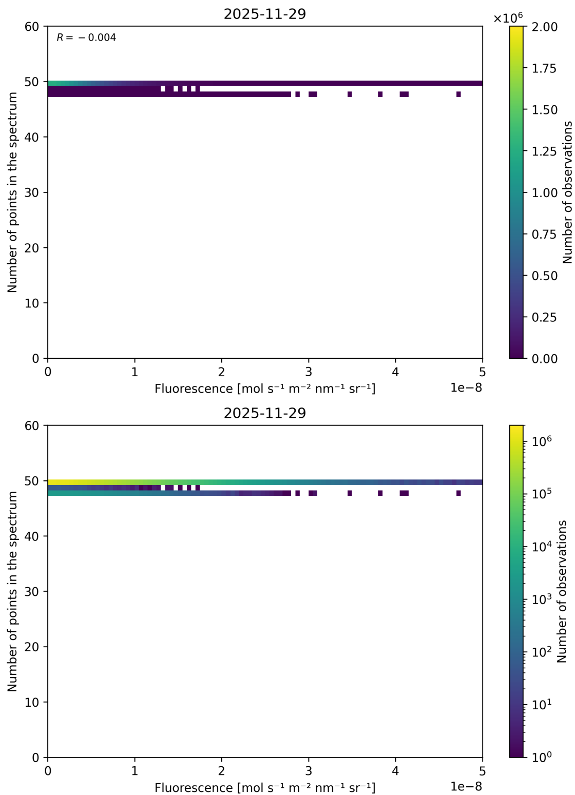
Figure 86: Scatter density plot of “Fluorescence” against “Number of points in the spectrum” for 2025-11-28 to 2025-11-30.
