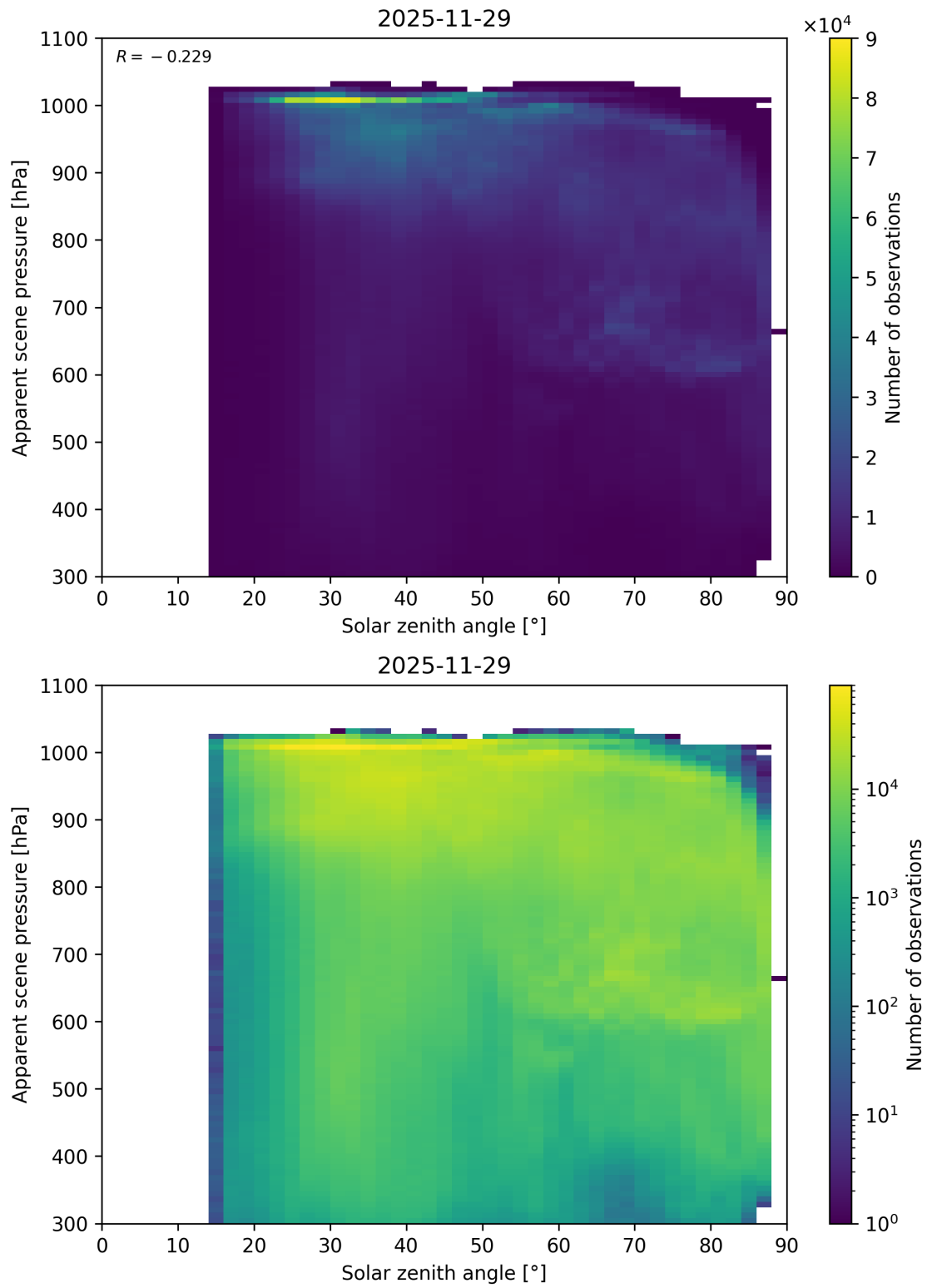
Figure 108: Scatter density plot of “Solar zenith angle” against “Apparent scene pressure” for 2025-11-28 to 2025-11-30.
