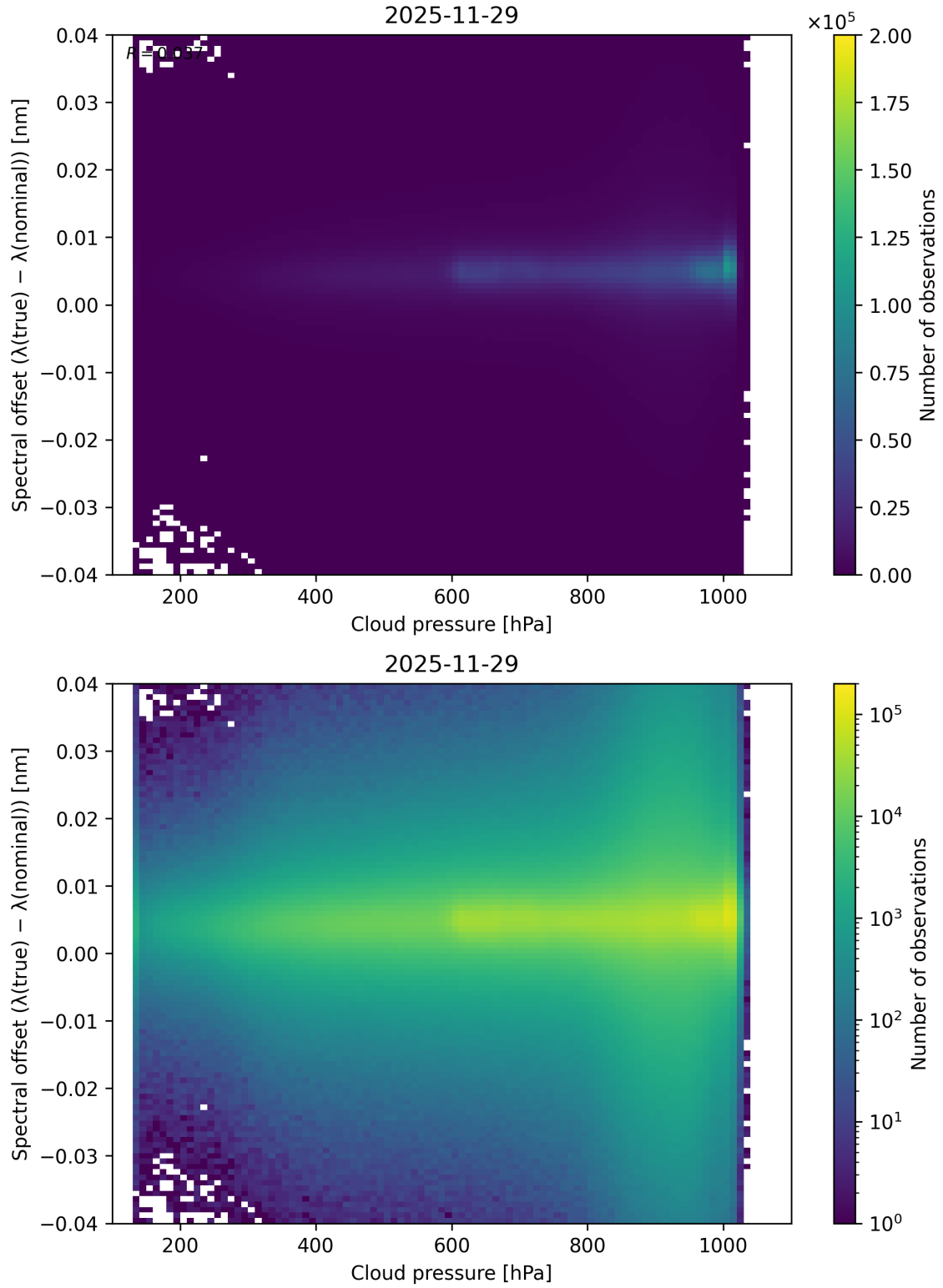
Figure 84: Scatter density plot of “Cloud pressure” against “Spectral offset ( \lambda_{\text{true}} - \lambda_{\text{nominal}} )” for 2025-11-28 to 2025-11-30.
