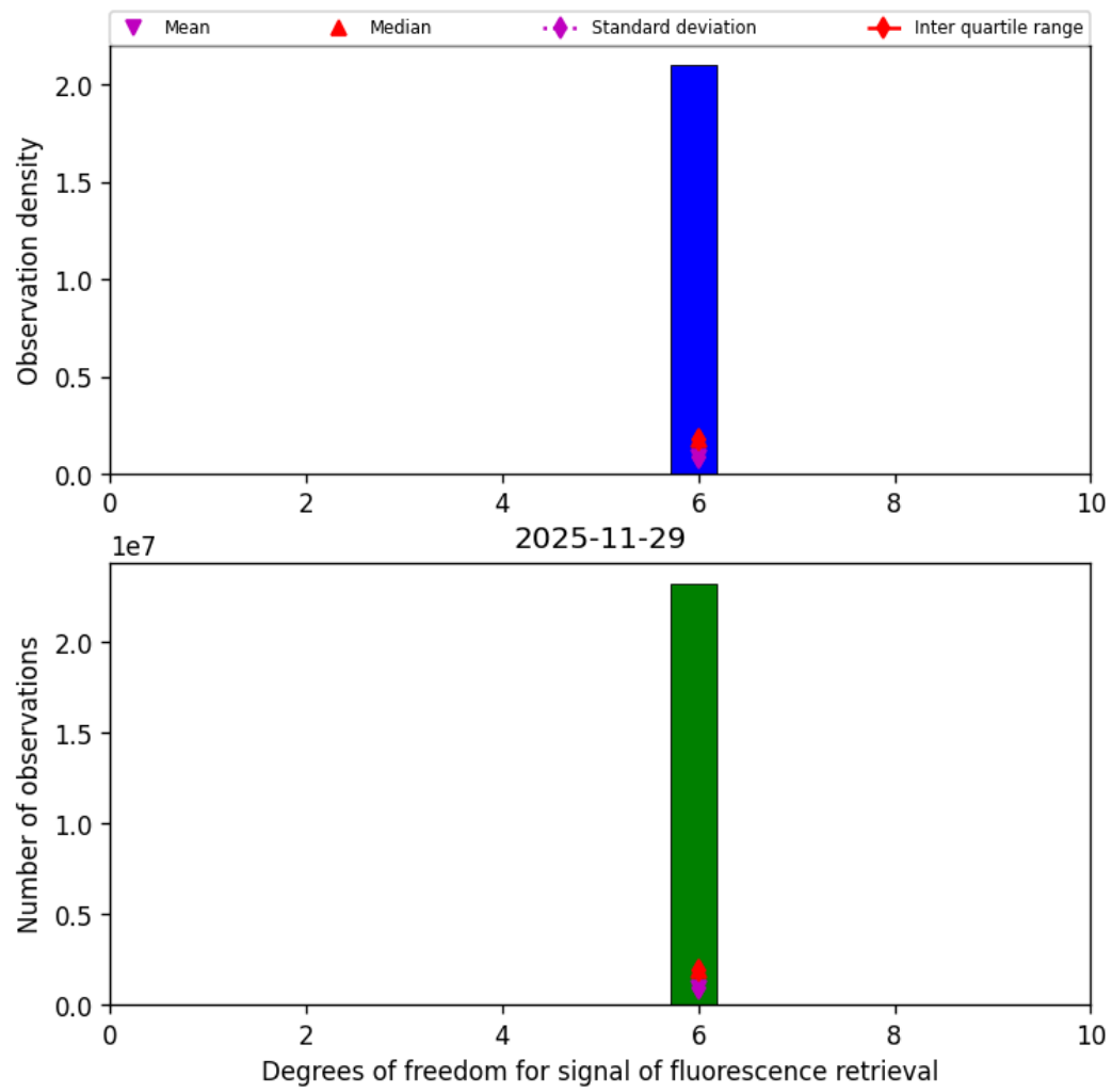
Figure 43: Histogram of "Degrees of freedom for signal of fluorescence retrieval" for 2025-11-28 to 2025-11-30
