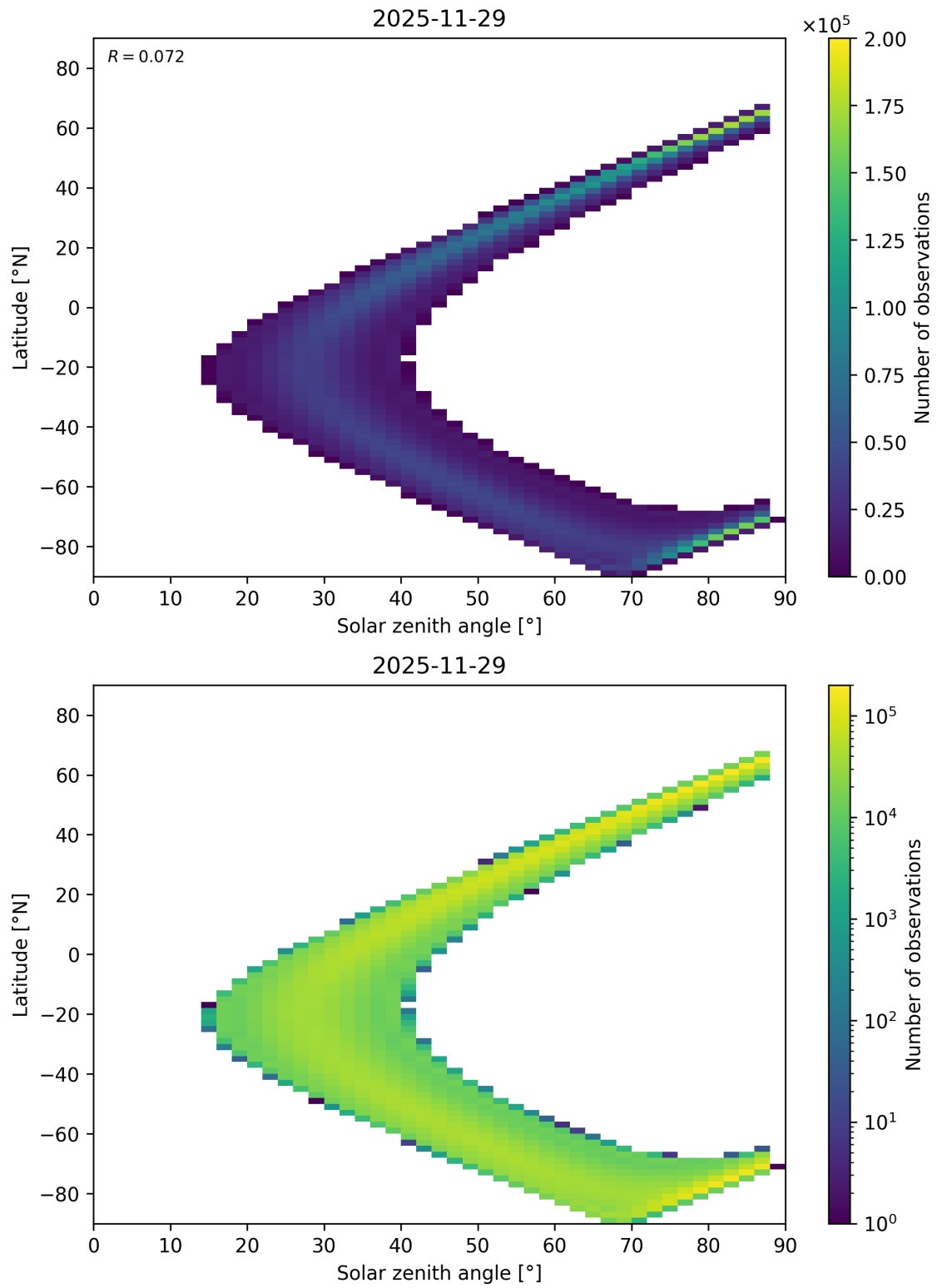
Figure 113: Scatter density plot of “Solar zenith angle” against “Latitude” for 2025-11-28 to 2025-11-30.
