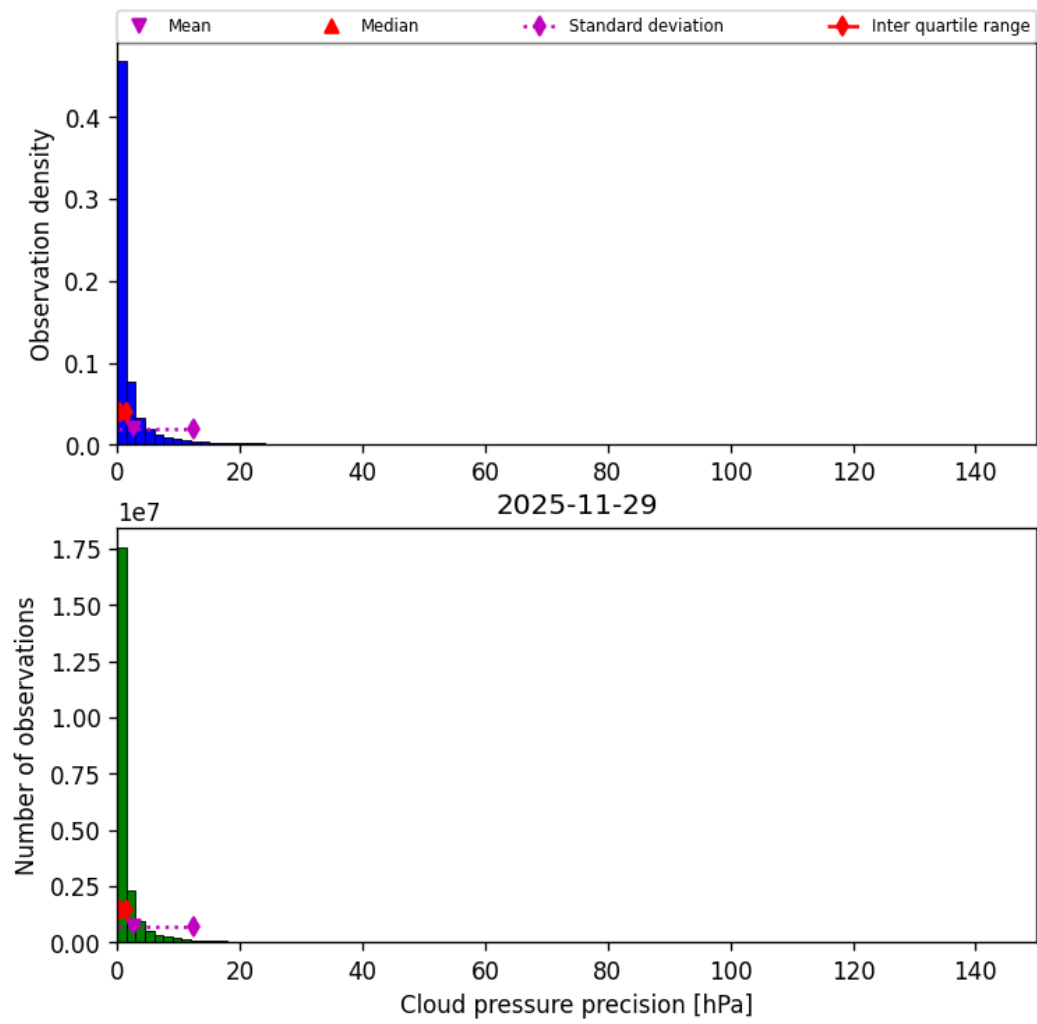
Figure 31: Histogram of “Cloud pressure precision” for 2025-11-28 to 2025-11-30
