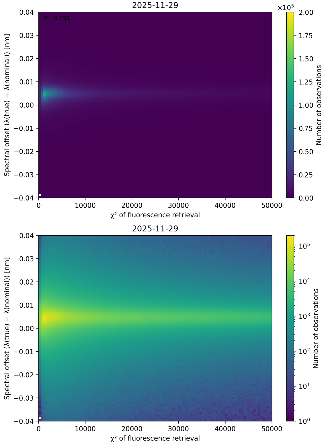
Figure 69: Scatter density plot of “ \chi^2 of fluorescence retrieval” against “Spectral offset ( \lambda_{\text{true}} - \lambda_{\text{nominal}} )” for 2025-11-28 to 2025-11-30.
