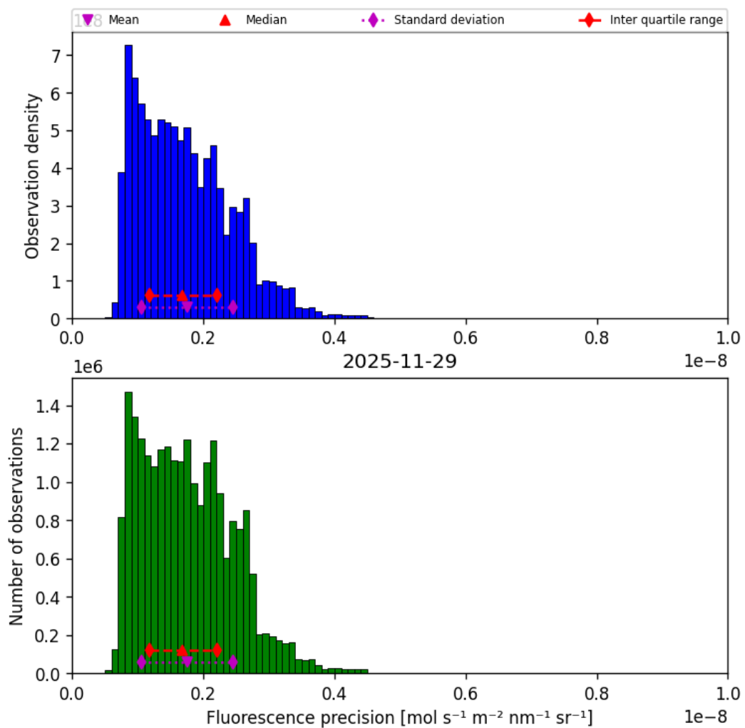
Figure 41: Histogram of “Fluorescence precision” for 2025-11-28 to 2025-11-30
