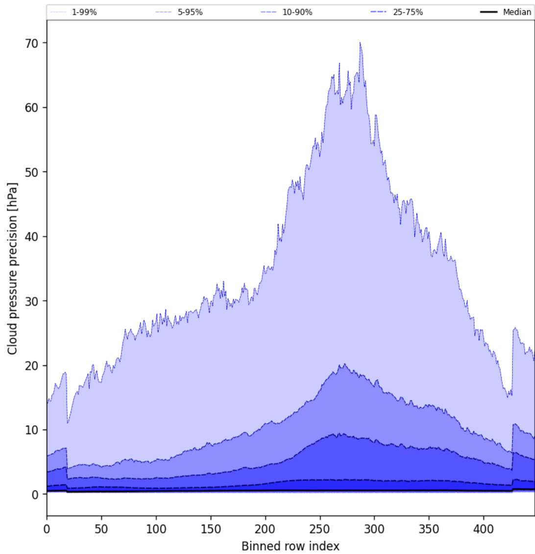
Figure 48: Along track statistics of “Cloud pressure precision” for 2025-11-28 to 2025-11-30
