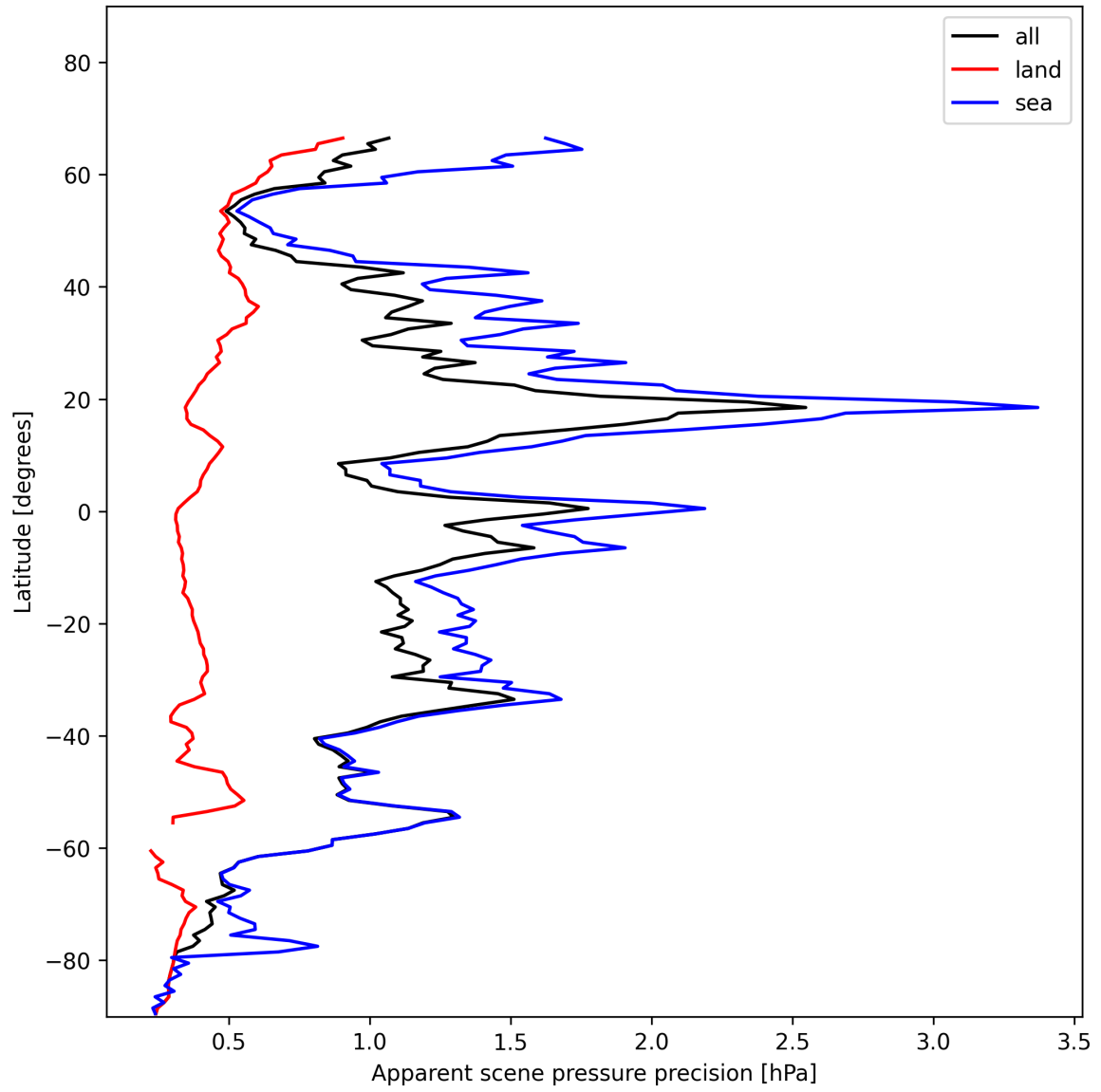
Figure 20: Zonal average of “Apparent scene pressure precision” for 2025-11-28 to 2025-11-30.
