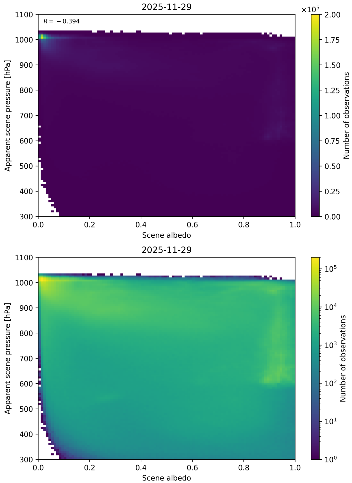
Figure 102: Scatter density plot of “Scene albedo” against “Apparent scene pressure” for 2025-11-28 to 2025-11-30.
