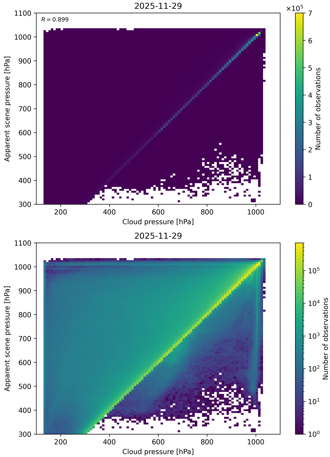
Figure 77: Scatter density plot of “Cloud pressure” against “Apparent scene pressure” for 2025-11-28 to 2025-11-30.
