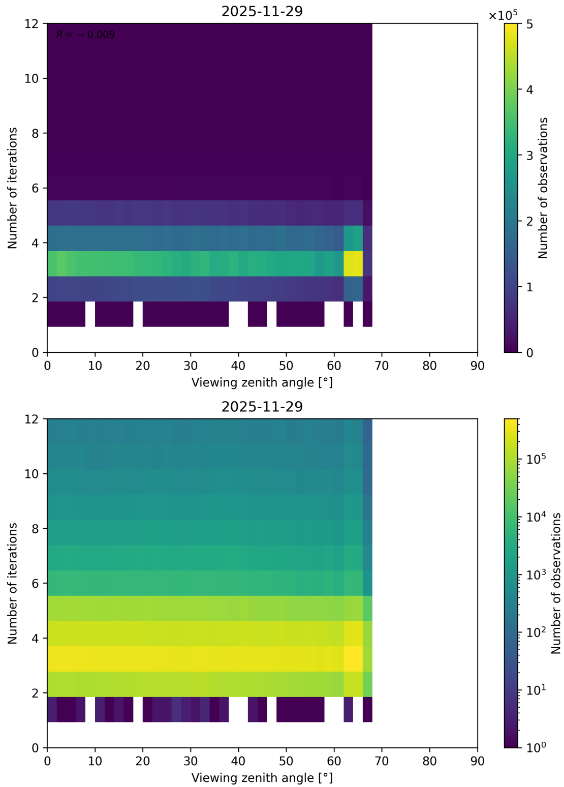
Figure 124: Scatter density plot of “Viewing zenith angle” against “Number of iterations” for 2025-11-28 to 2025-11-30.
