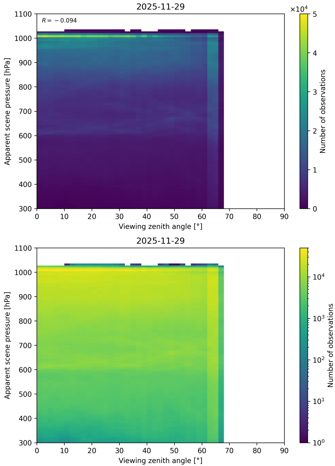
Figure 118: Scatter density plot of “Viewing zenith angle” against “Apparent scene pressure” for 2025-11-28 to 2025-11-30.
