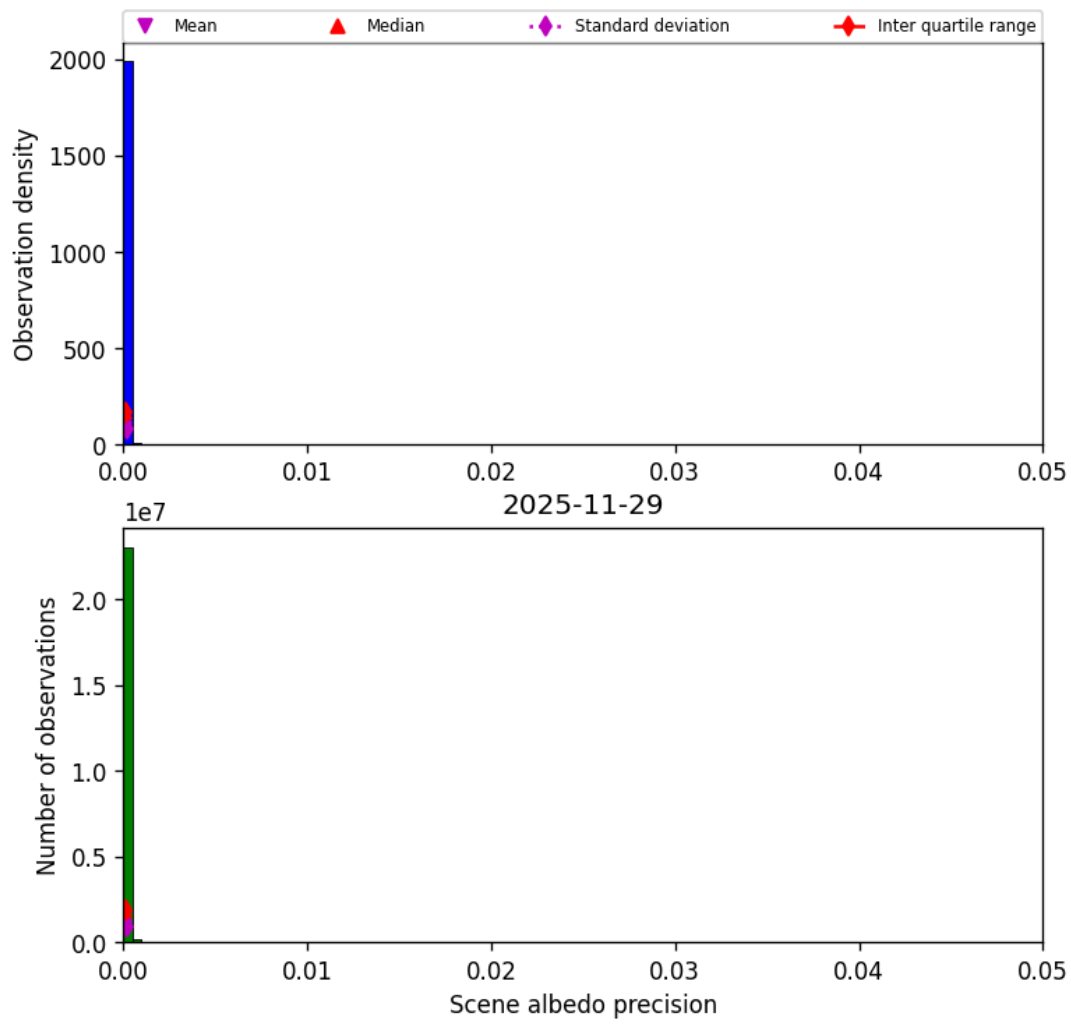
Figure 35: Histogram of “Scene albedo precision” for 2025-11-28 to 2025-11-30
