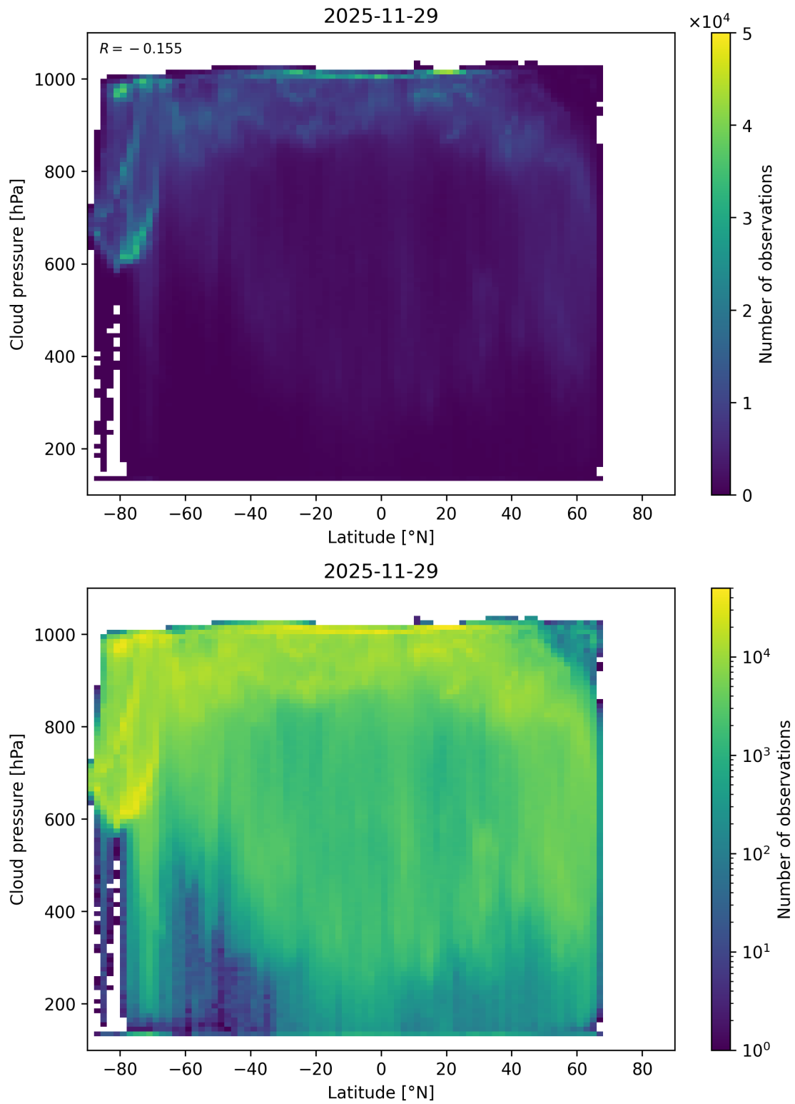
Figure 91: Scatter density plot of “Latitude” against “Cloud pressure” for 2025-11-28 to 2025-11-30.
