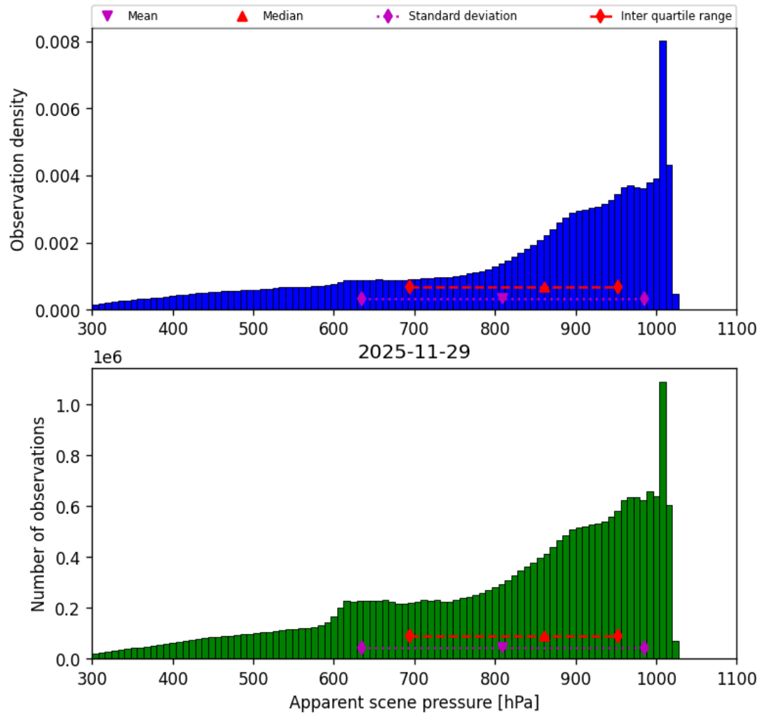
Figure 36: Histogram of “Apparent scene pressure” for 2025-11-28 to 2025-11-30
