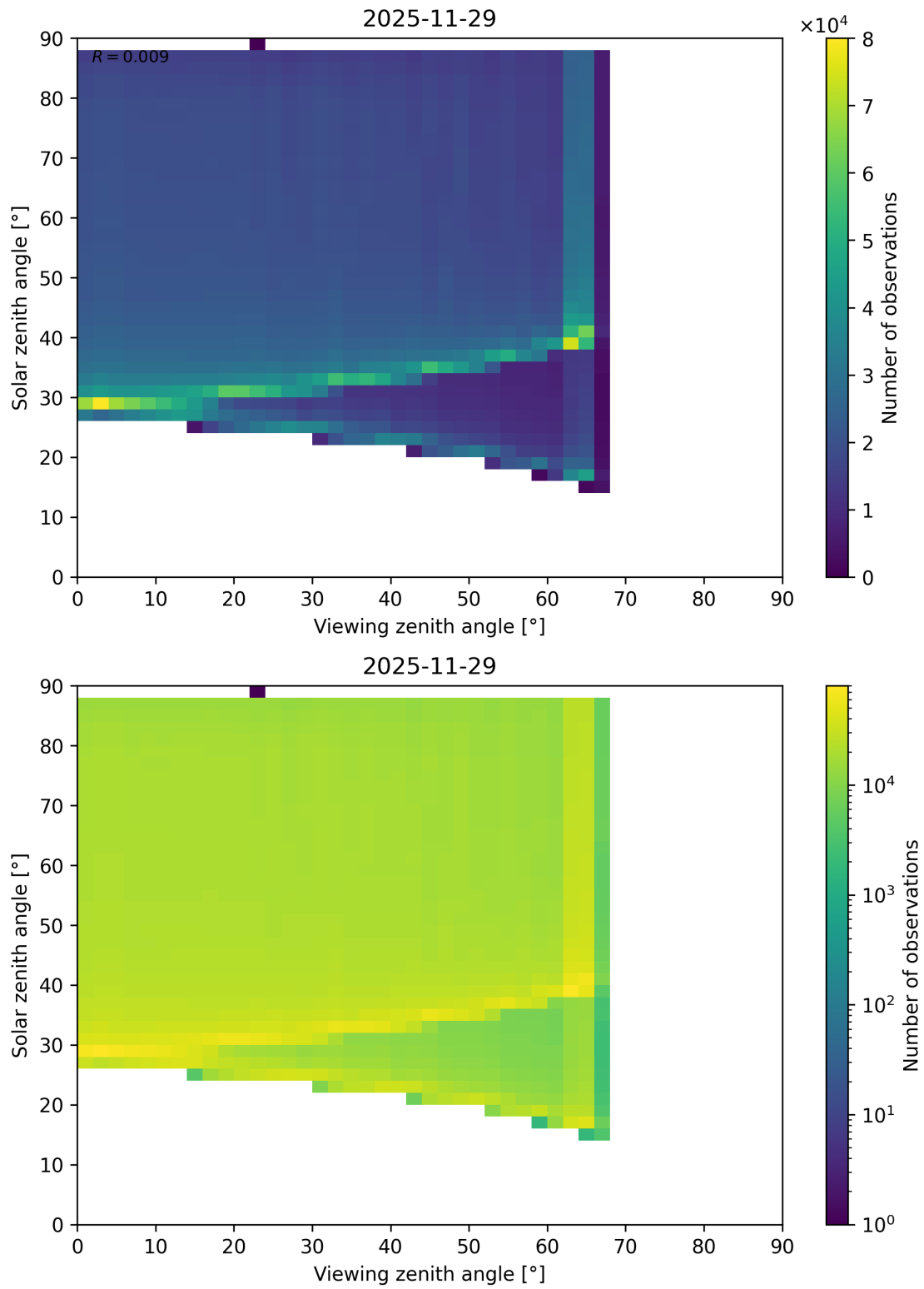
Figure 127: Scatter density plot of “Viewing zenith angle” against “Solar zenith angle” for 2025-11-28 to 2025-11-30.
