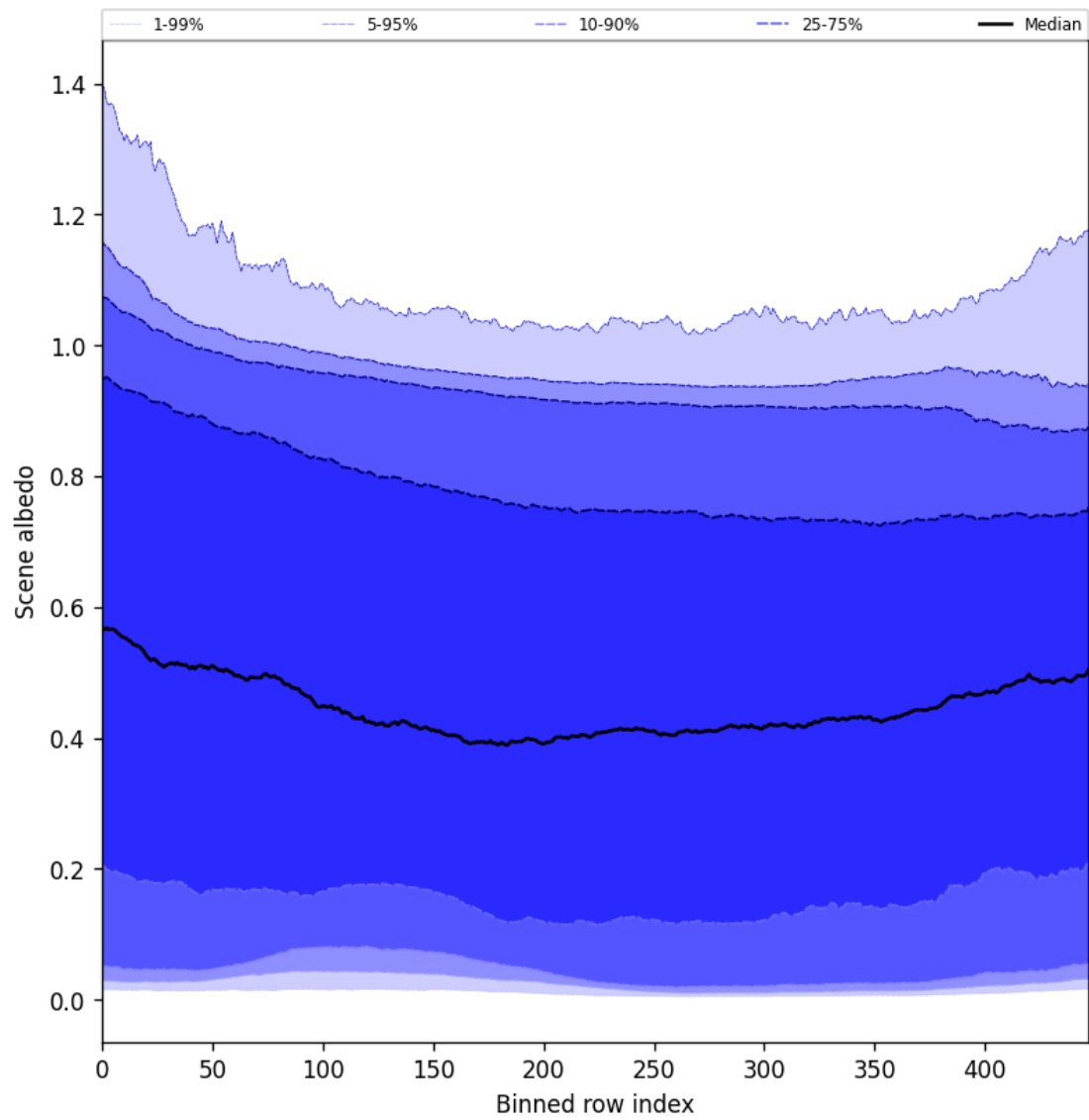
Figure 51: Along track statistics of “Scene albedo” for 2025-11-28 to 2025-11-30
