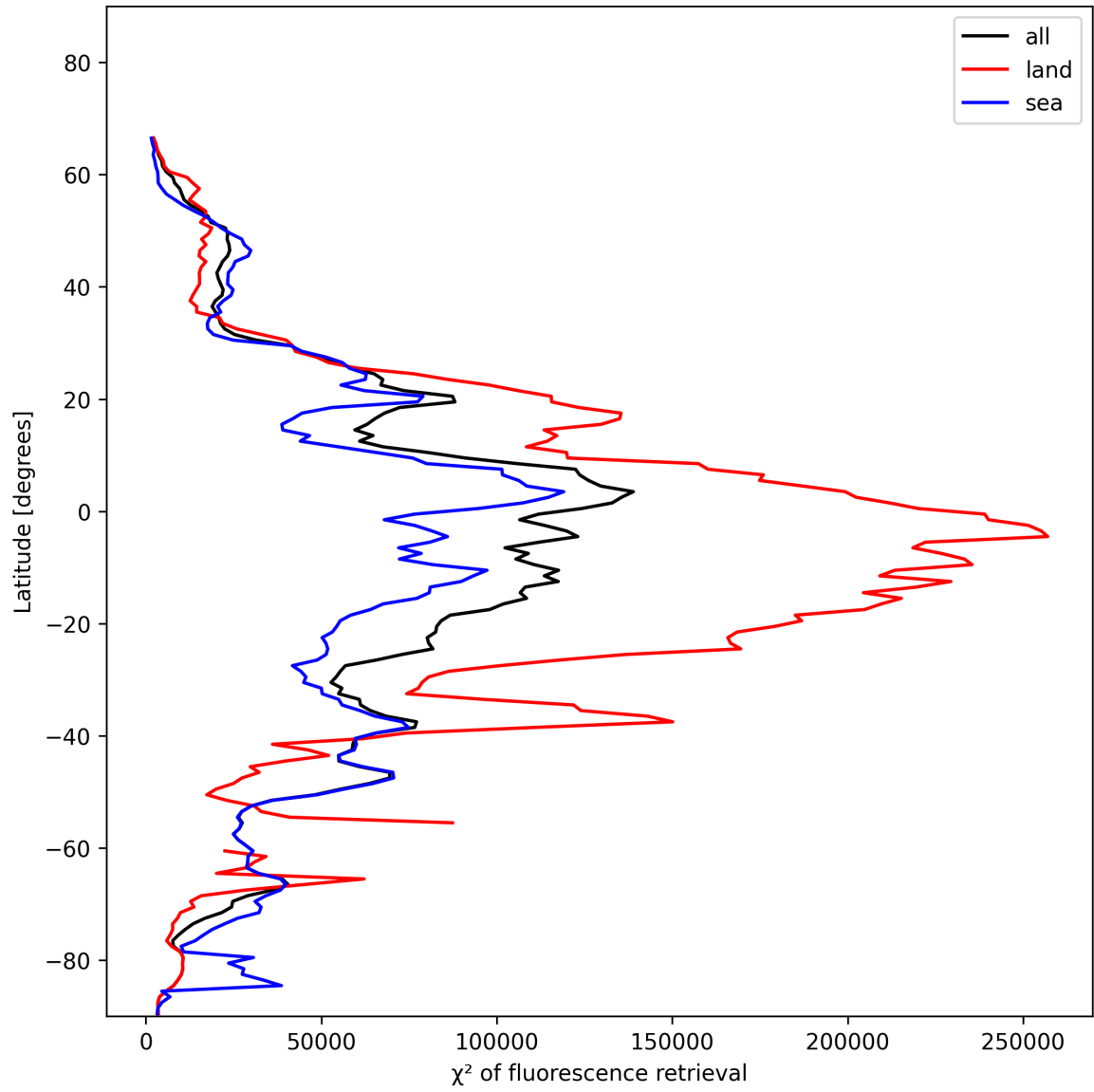
Figure 25: Zonal average of “ \chi^2 of fluorescence retrieval” for 2025-11-28 to 2025-11-30.
