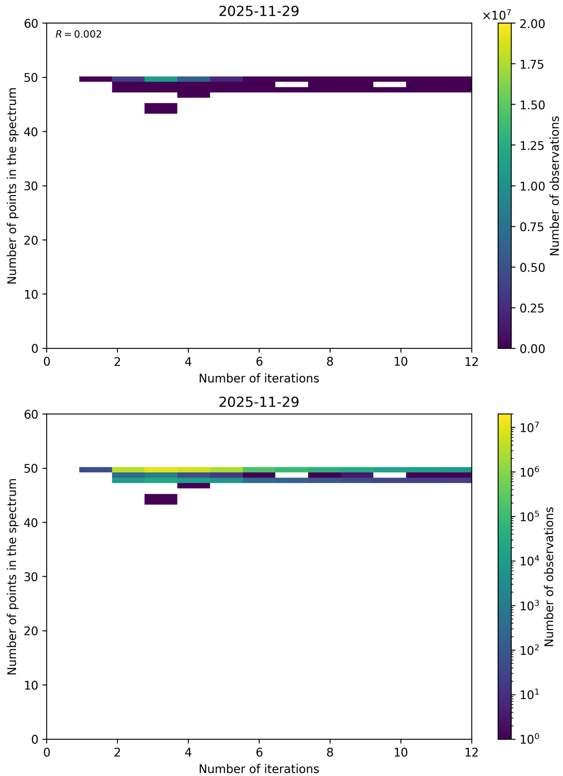
Figure 99: Scatter density plot of “Number of iterations” against “Number of points in the spectrum” for 2025-11-28 to 2025-11-30.
