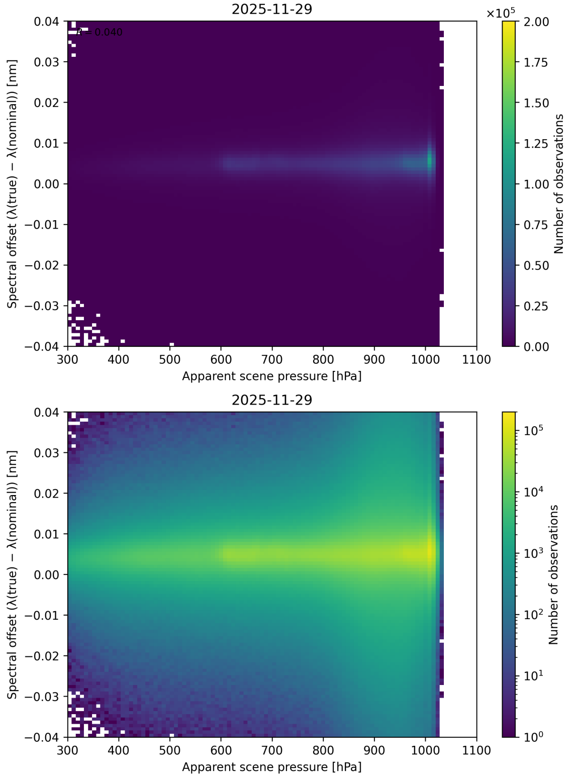
Figure 67: Scatter density plot of “Apparent scene pressure” against “Spectral offset ( \lambda_{\text{true}} - \lambda_{\text{nominal}} )” for 2025-11-28 to 2025-11-30.
