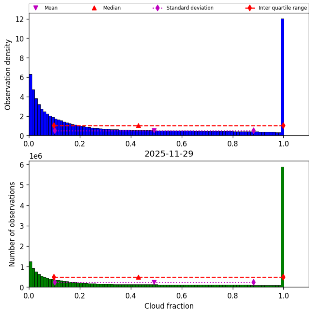
Figure 32: Histogram of “Cloud fraction” for 2025-11-28 to 2025-11-30
