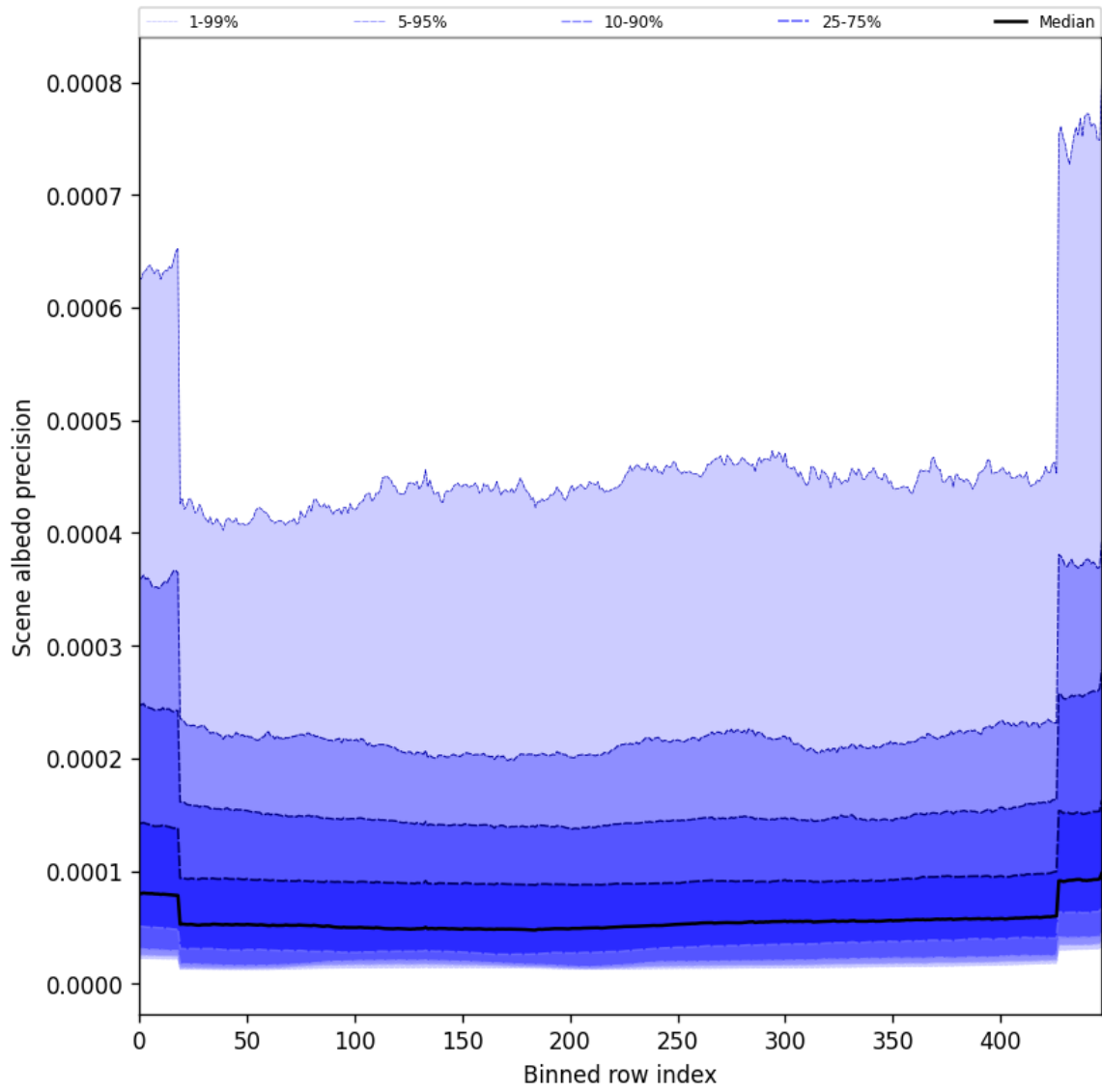
Figure 52: Along track statistics of “Scene albedo precision” for 2025-11-28 to 2025-11-30
