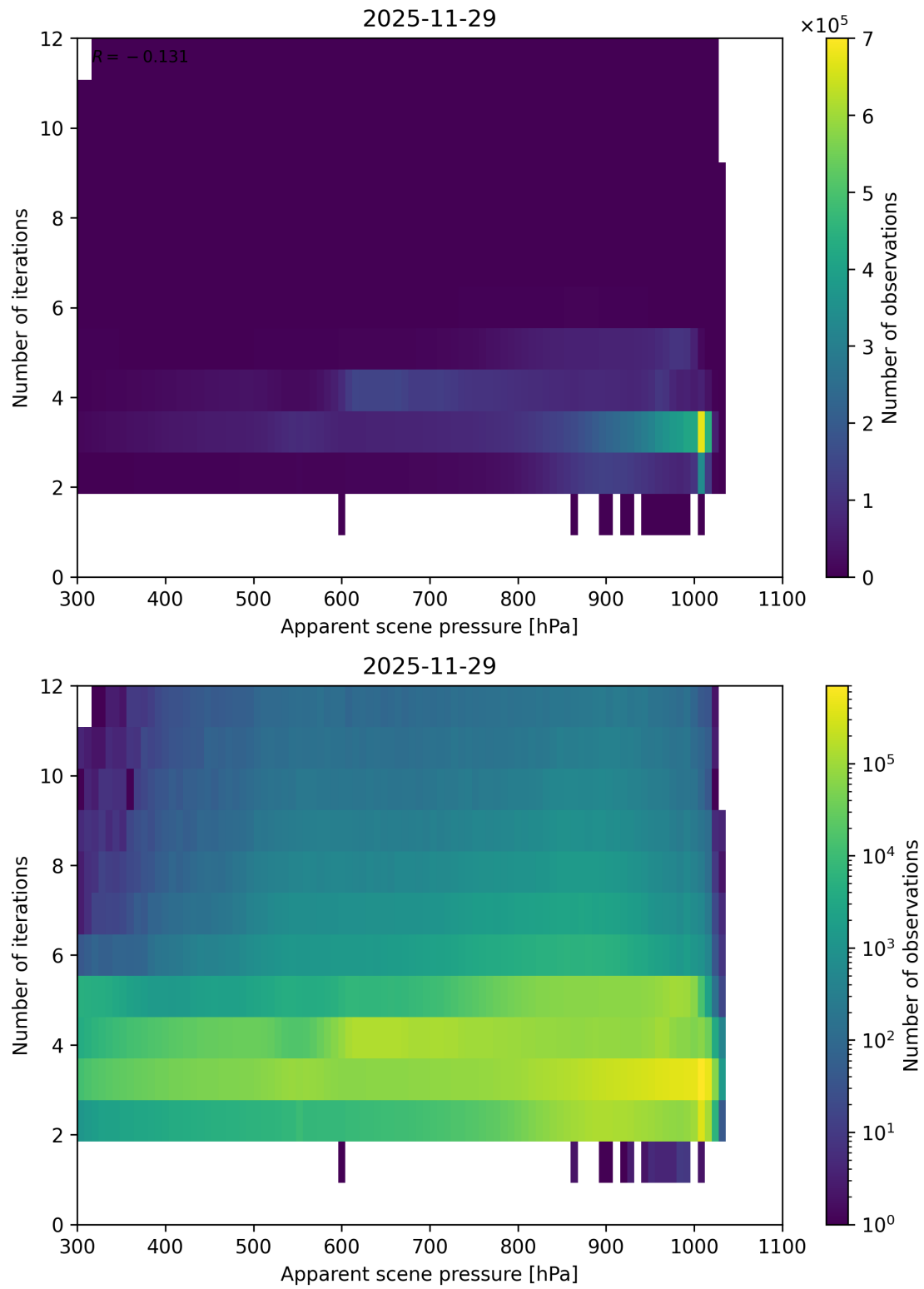
Figure 65: Scatter density plot of “Apparent scene pressure” against “Number of iterations” for 2025-11-28 to 2025-11-30.
