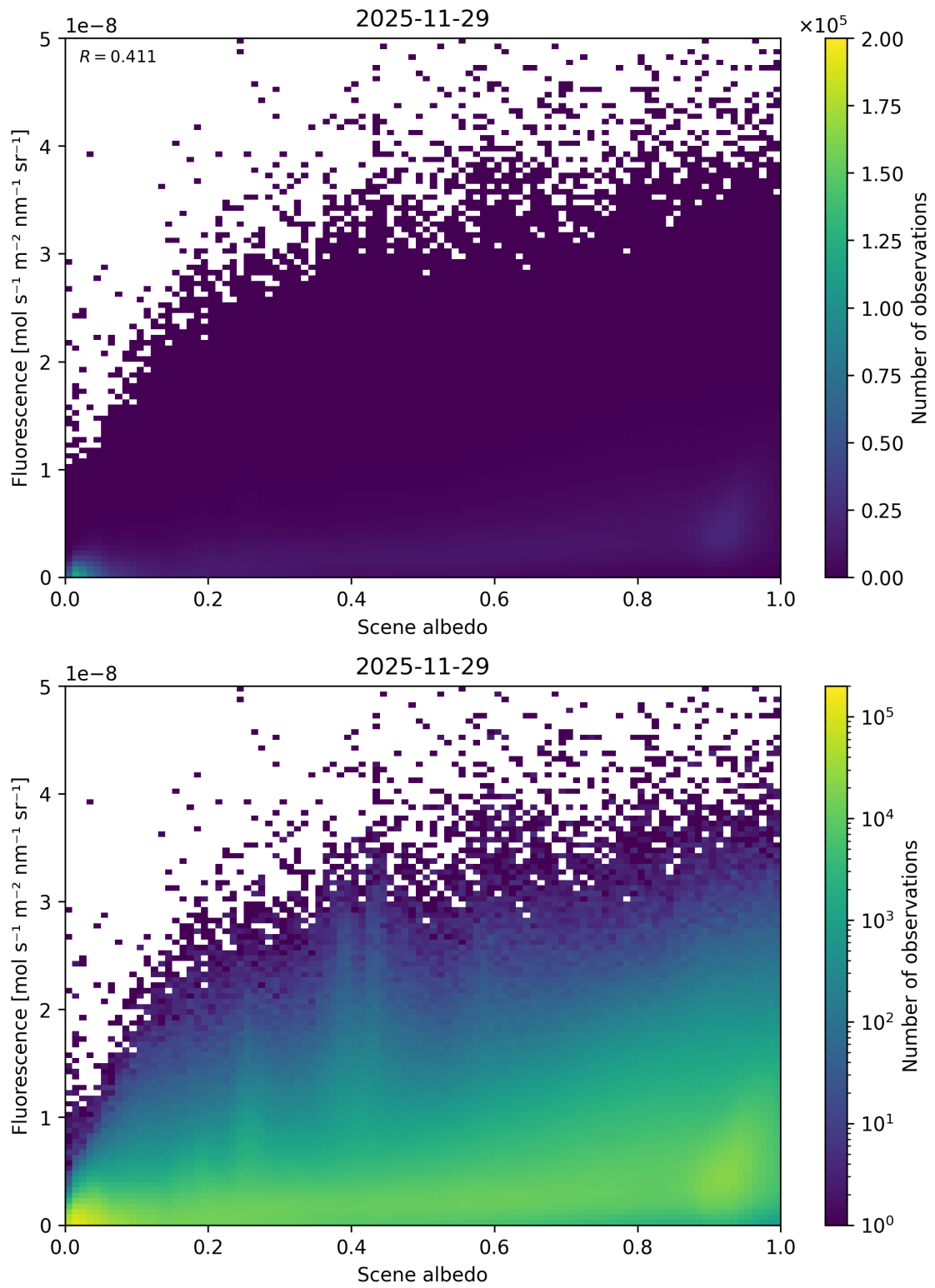
Figure 104: Scatter density plot of “Scene albedo” against “Fluorescence” for 2025-11-28 to 2025-11-30.
