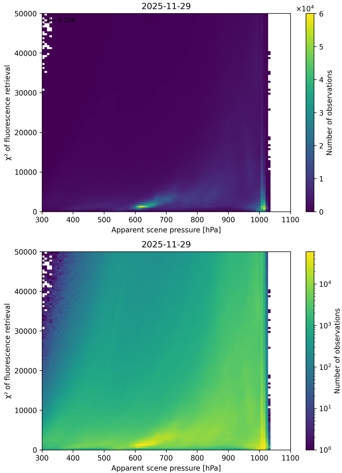
Figure 63: Scatter density plot of “Apparent scene pressure” against “ \chi^2 of fluorescence retrieval” for 2025-11-28 to 2025-11-30.
