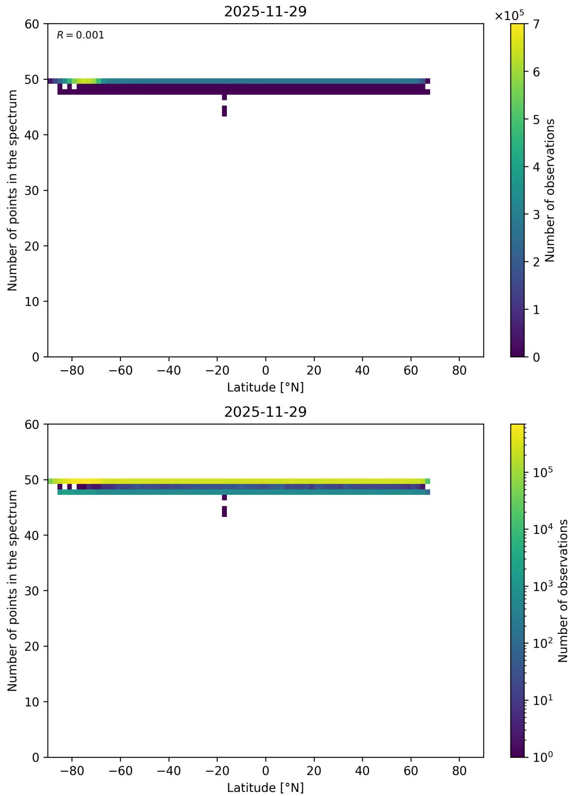
Figure 94: Scatter density plot of “Latitude” against “Number of points in the spectrum” for 2025-11-28 to 2025-11-30.
