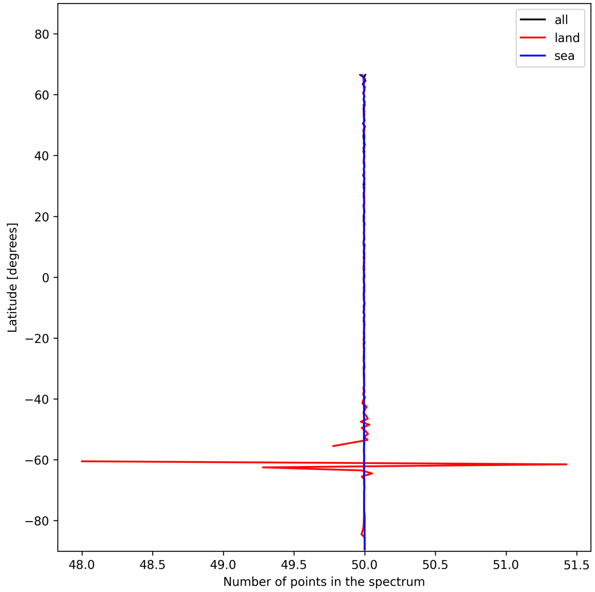
Figure 27: Zonal average of “Number of points in the spectrum” for 2025-11-28 to 2025-11-30.
