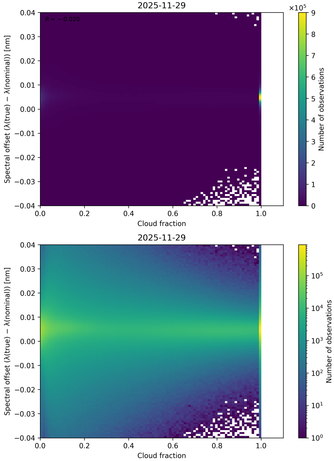
Figure 76: Scatter density plot of “Cloud fraction” against “Spectral offset ( \lambda_{\text{true}} - \lambda_{\text{nominal}} )” for 2025-11-28 to 2025-11-30.
