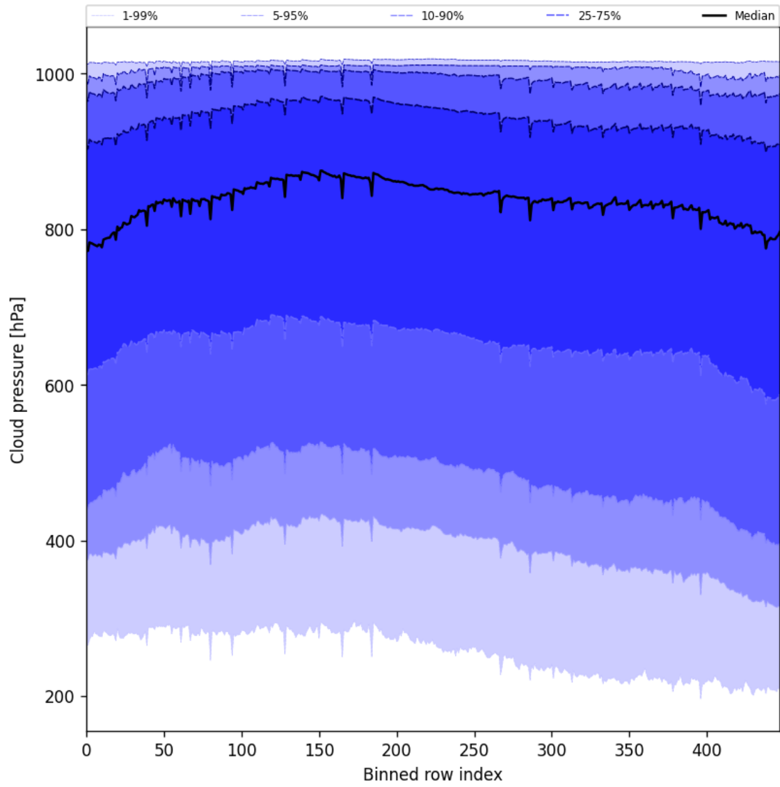
Figure 47: Along track statistics of “Cloud pressure” for 2025-11-28 to 2025-11-30
