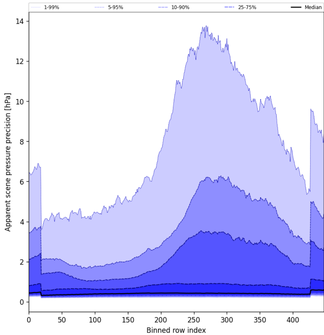
Figure 54: Along track statistics of “Apparent scene pressure precision” for 2025-11-28 to 2025-11-30
