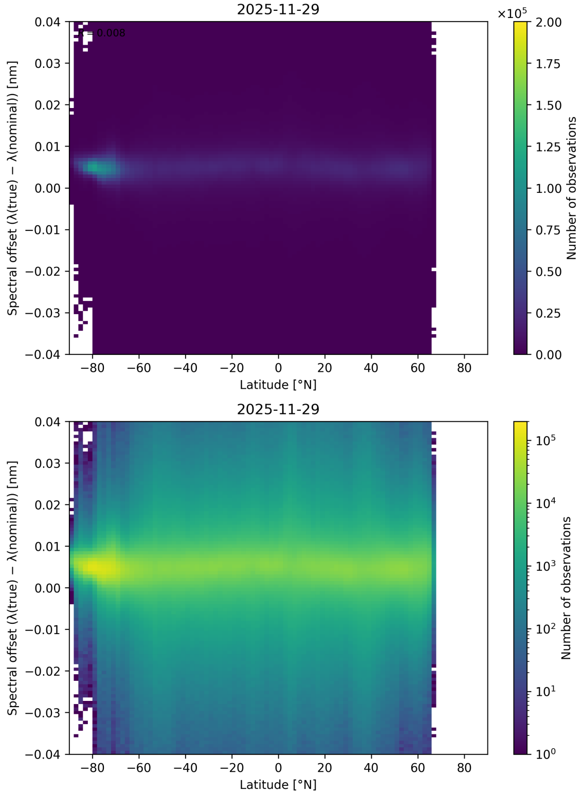
Figure 96: Scatter density plot of “Latitude” against “Spectral offset ( \lambda_{\text{true}} - \lambda_{\text{nominal}} )” for 2025-11-28 to 2025-11-30.
