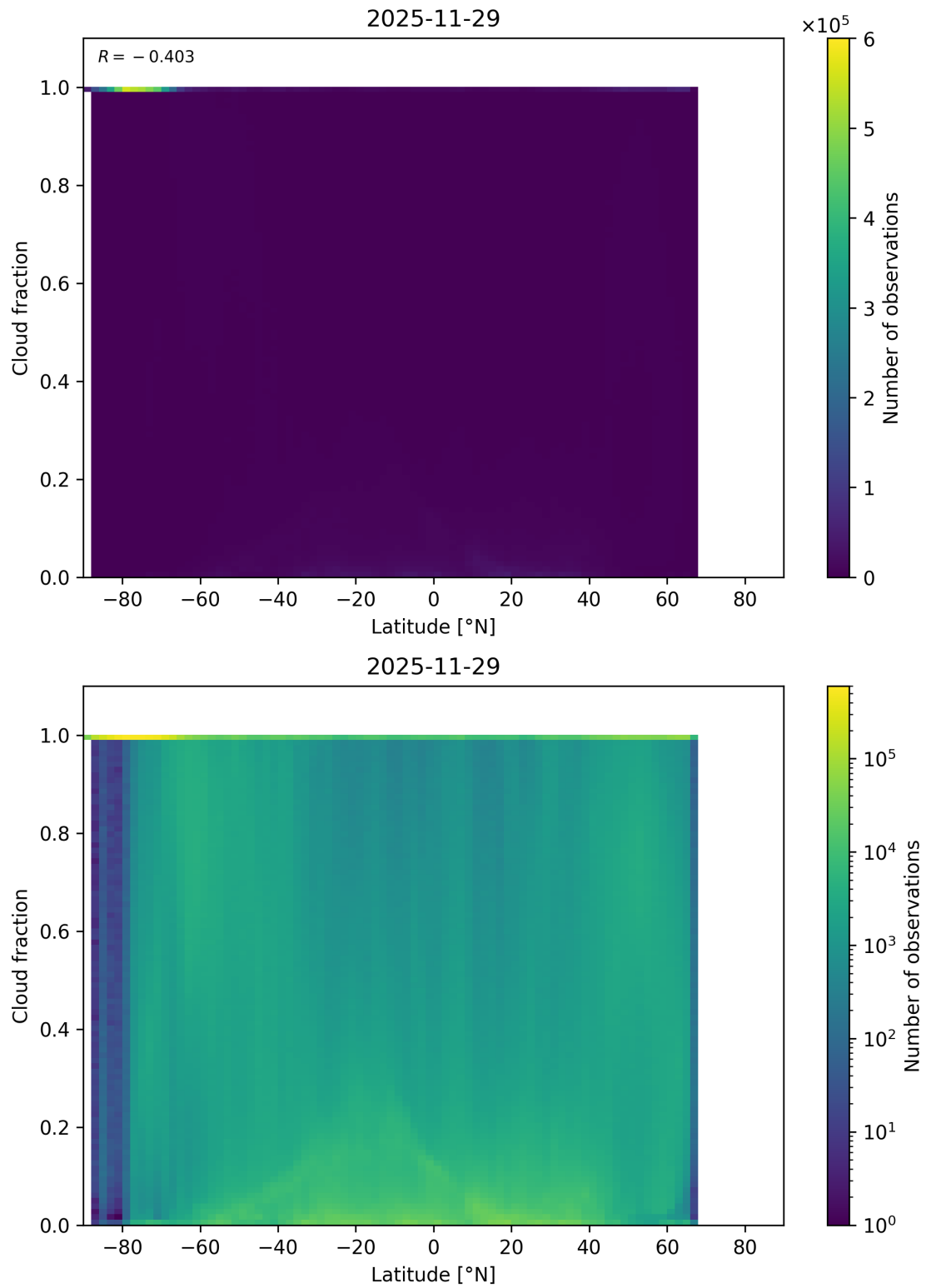
Figure 90: Scatter density plot of “Latitude” against “Cloud fraction” for 2025-11-28 to 2025-11-30.
