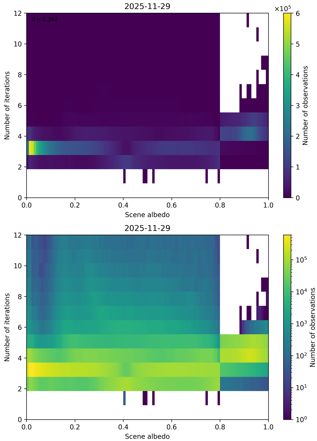
Figure 105: Scatter density plot of “Scene albedo” against “Number of iterations” for 2025-11-28 to 2025-11-30.
