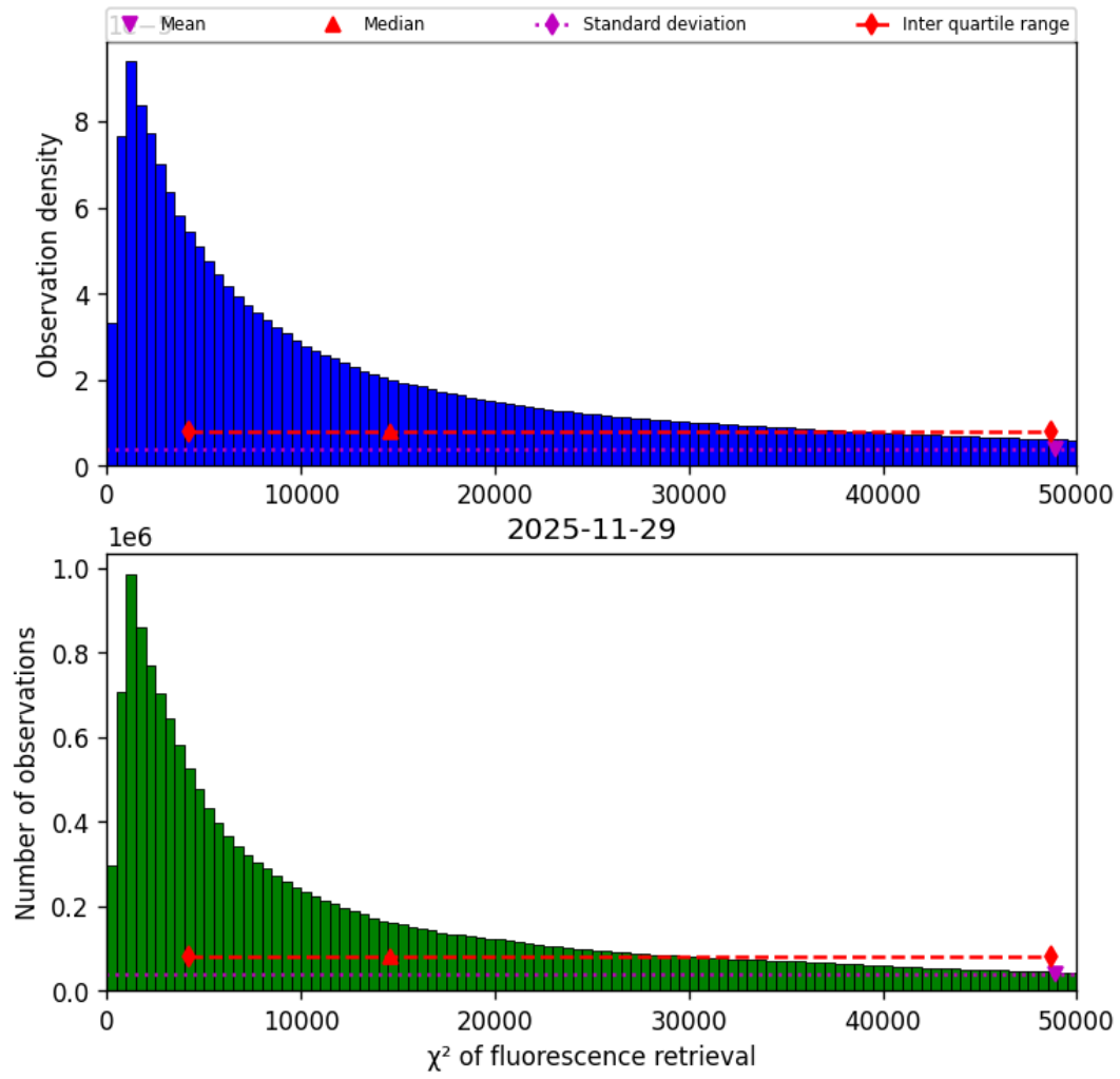
Figure 42: Histogram of “ \chi^2 of fluorescence retrieval” for 2025-11-28 to 2025-11-30
