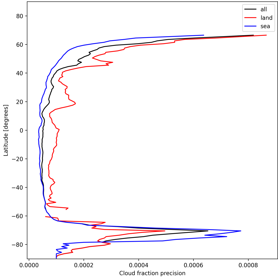
Figure 16: Zonal average of “Cloud fraction precision” for 2025-11-28 to 2025-11-30.
