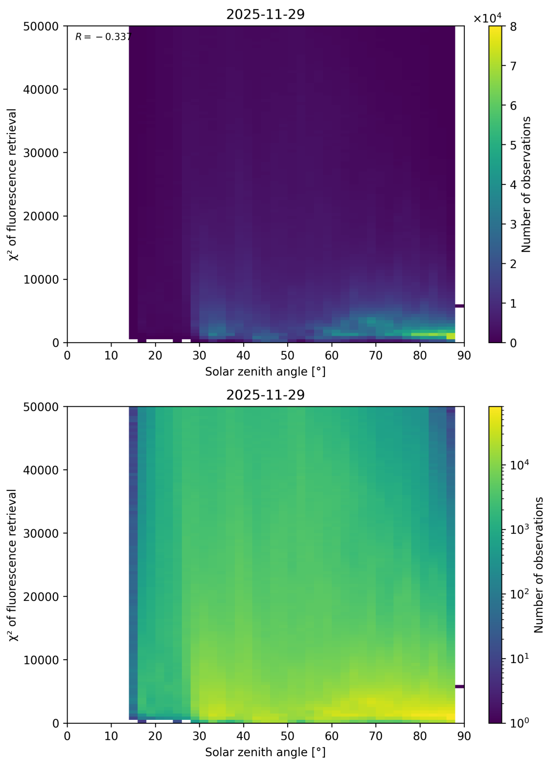
Figure 109: Scatter density plot of “Solar zenith angle” against “ \chi^2 of fluorescence retrieval” for 2025-11-28 to 2025-11-30.
