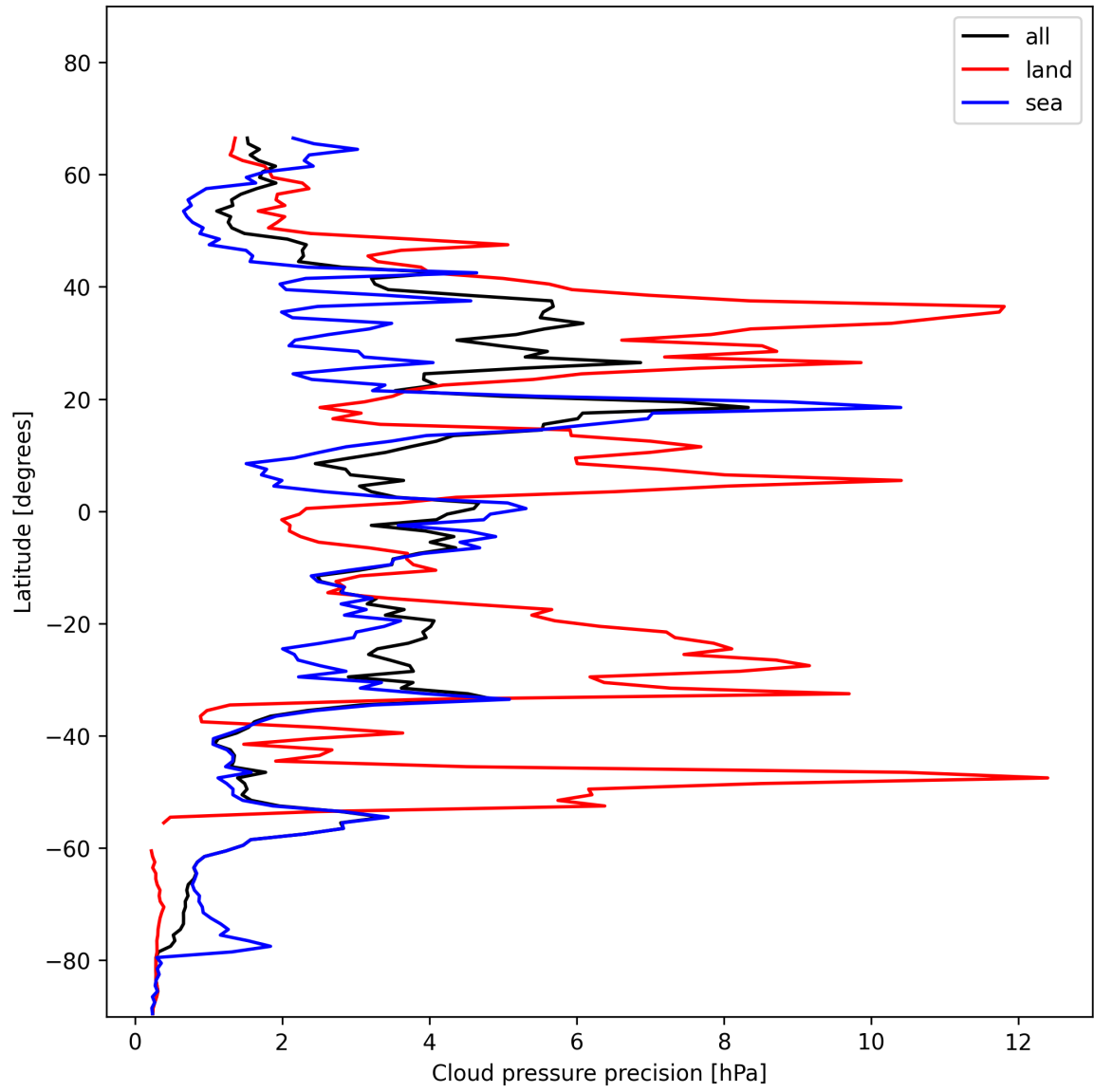
Figure 14: Zonal average of "Cloud pressure precision" for 2025-11-28 to 2025-11-30.
