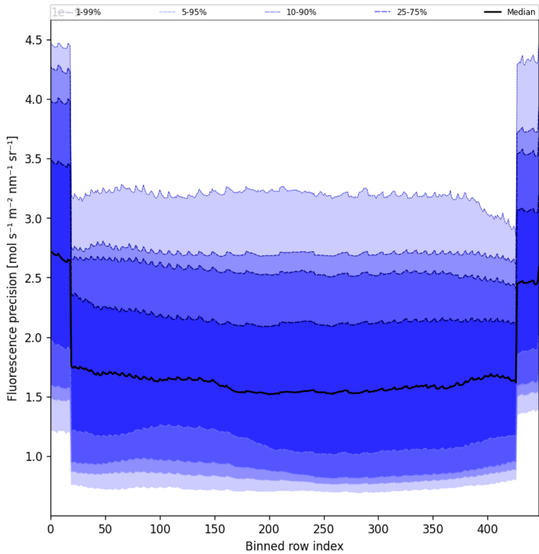
Figure 58: Along track statistics of “Fluorescence precision” for 2025-11-28 to 2025-11-30
