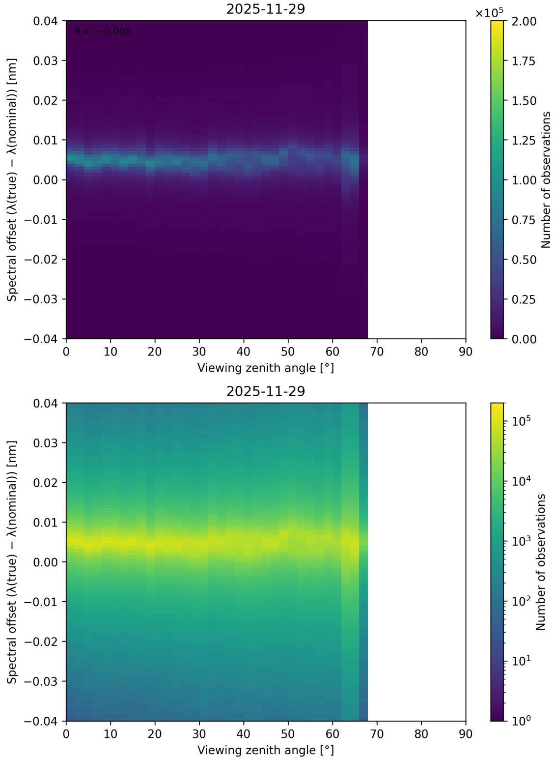
Figure 128: Scatter density plot of “Viewing zenith angle” against “Spectral offset ( \lambda_{\text{true}} - \lambda_{\text{nominal}} )” for 2025-11-28 to 2025-11-30.
