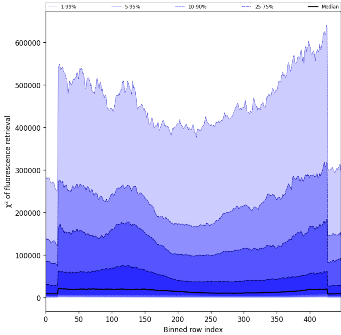
Figure 59: Along track statistics of “ \chi^2 of fluorescence retrieval” for 2025-11-28 to 2025-11-30
