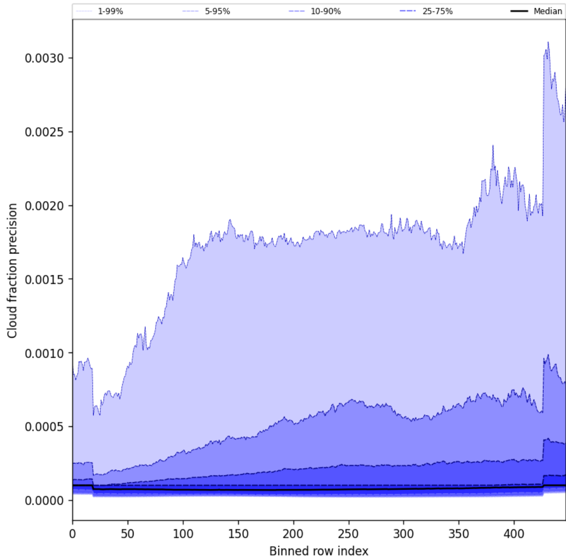
Figure 50: Along track statistics of “Cloud fraction precision” for 2025-11-28 to 2025-11-30
