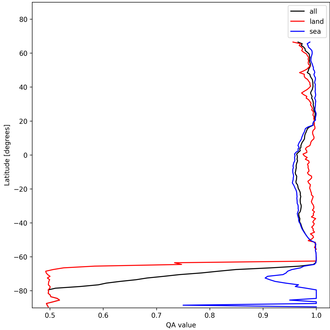
Figure 12: Zonal average of “QA value” for 2025-11-28 to 2025-11-30.
