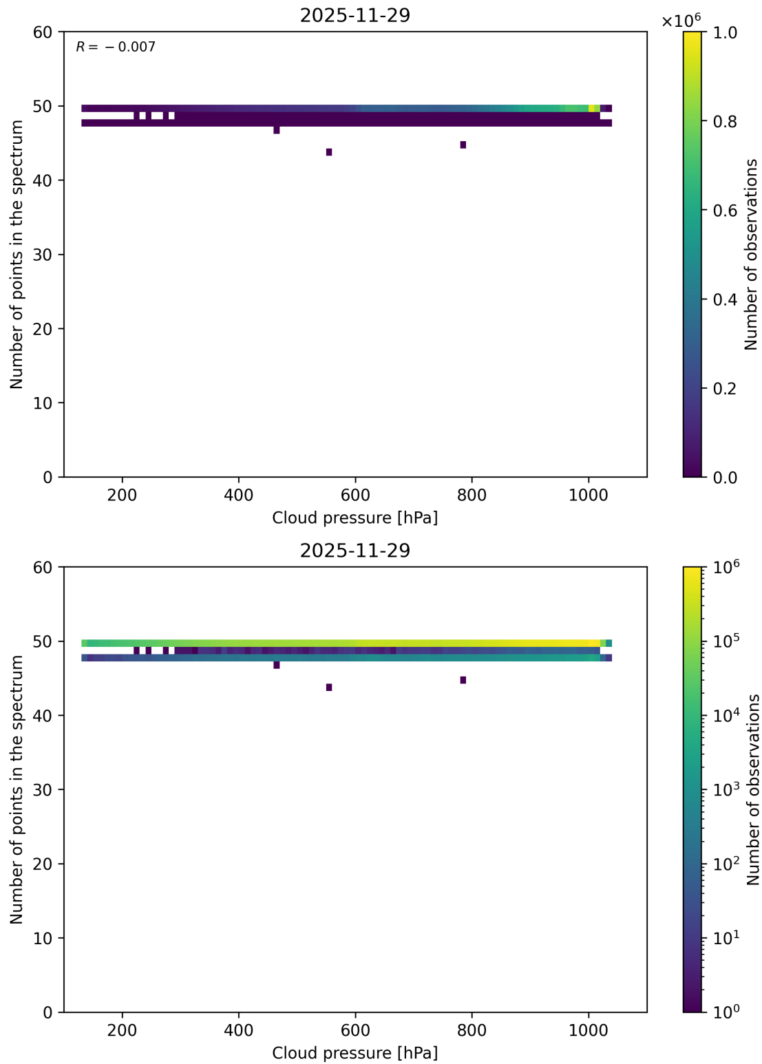
Figure 82: Scatter density plot of “Cloud pressure” against “Number of points in the spectrum” for 2025-11-28 to 2025-11-30.
