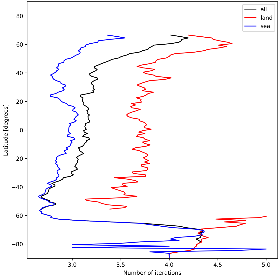
Figure 22: Zonal average of “Number of iterations” for 2025-11-28 to 2025-11-30.
