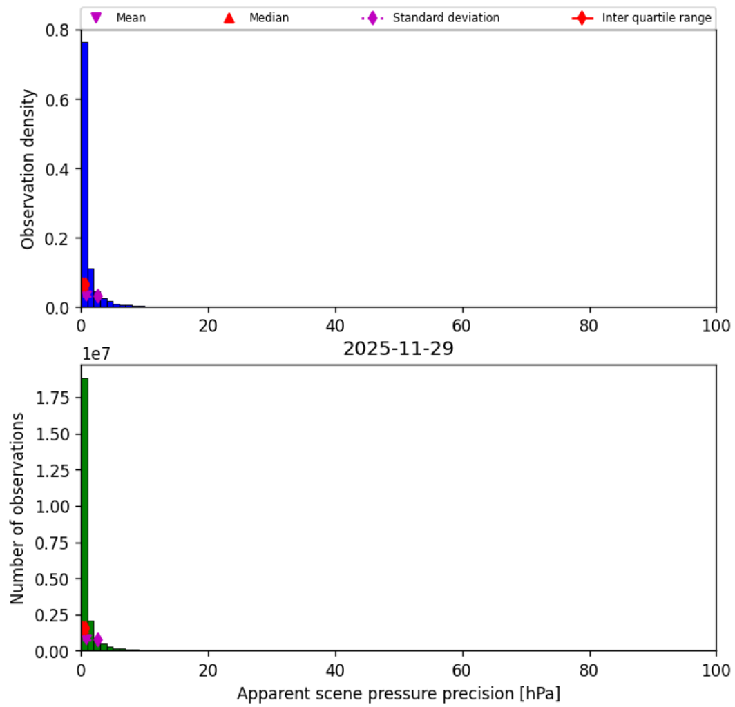
Figure 37: Histogram of “Apparent scene pressure precision” for 2025-11-28 to 2025-11-30
