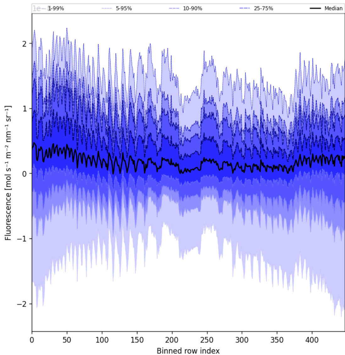
Figure 57: Along track statistics of “Fluorescence” for 2025-11-28 to 2025-11-30
