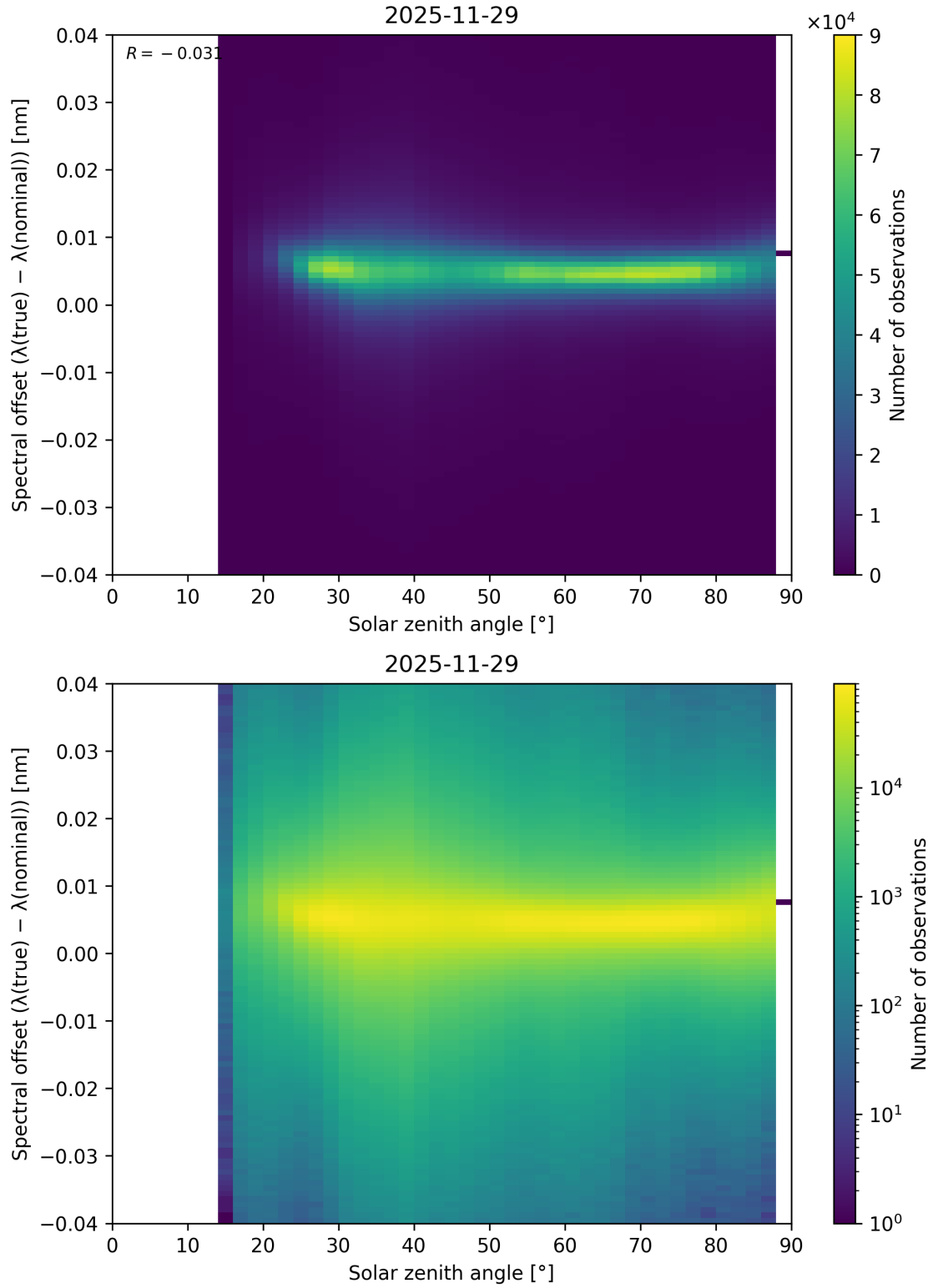
Figure 117: Scatter density plot of “Solar zenith angle” against “Spectral offset ( \lambda_{\text{true}} - \lambda_{\text{nominal}} )” for 2025-11-28 to 2025-11-30.
