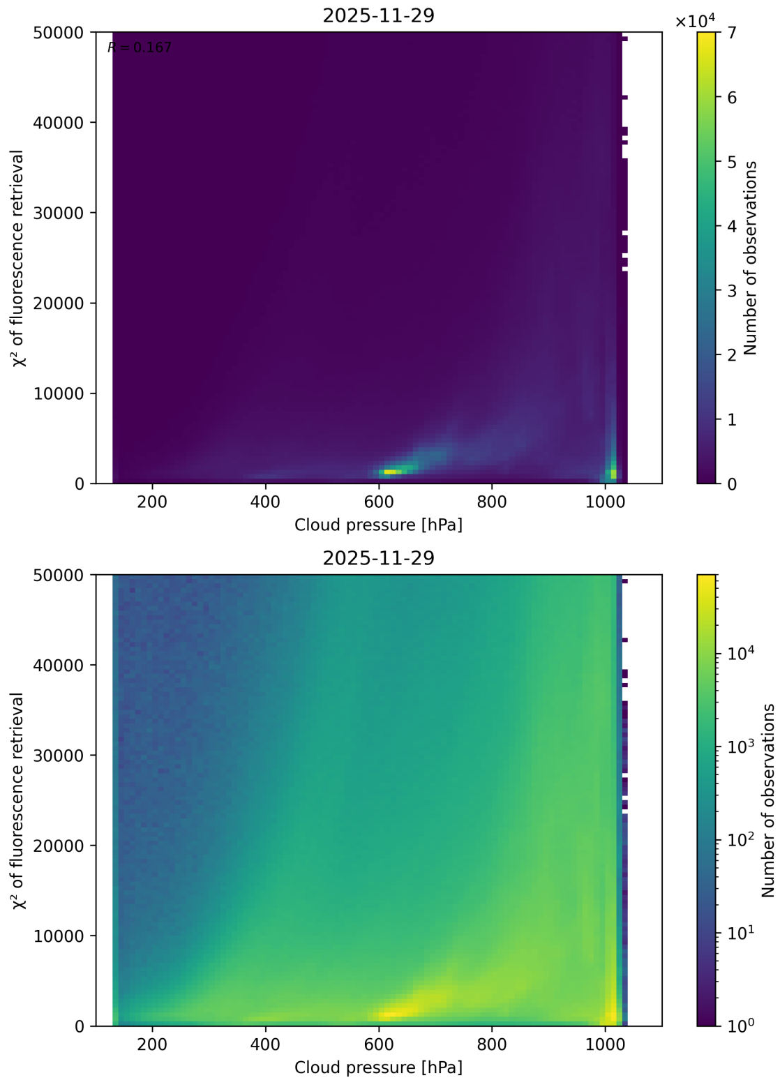
Figure 78: Scatter density plot of “Cloud pressure” against “ \chi^2 of fluorescence retrieval” for 2025-11-28 to 2025-11-30.
