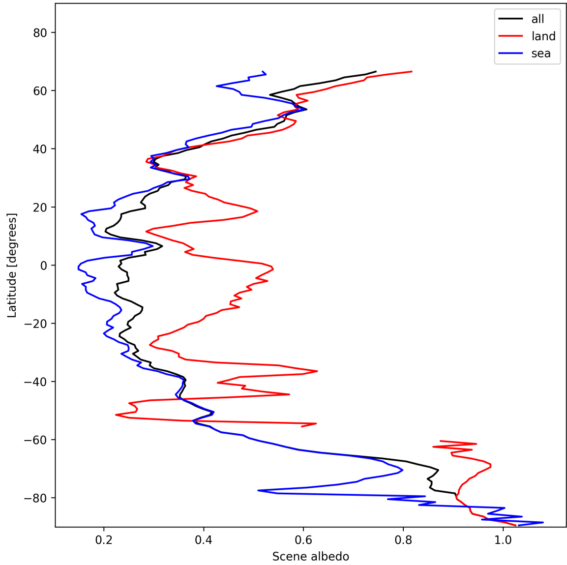
Figure 17: Zonal average of “Scene albedo” for 2025-11-28 to 2025-11-30.
