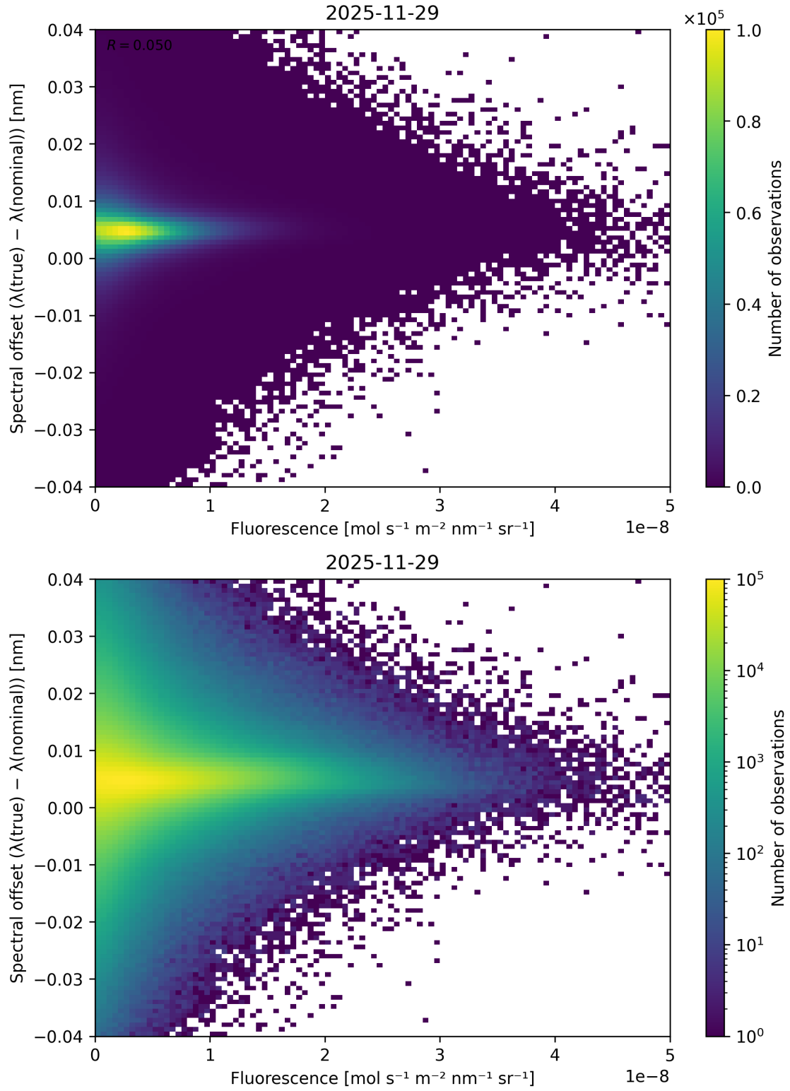
Figure 87: Scatter density plot of “Fluorescence” against “Spectral offset ( \lambda_{\text{true}} - \lambda_{\text{nominal}} )” for 2025-11-28 to 2025-11-30.
