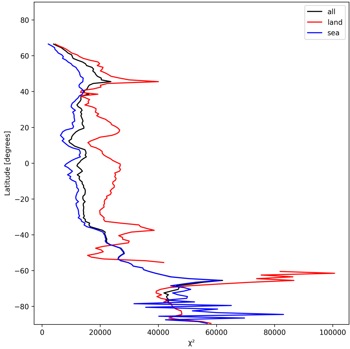
Figure 21: Zonal average of “ \chi^2 ” for 2025-11-28 to 2025-11-30.
