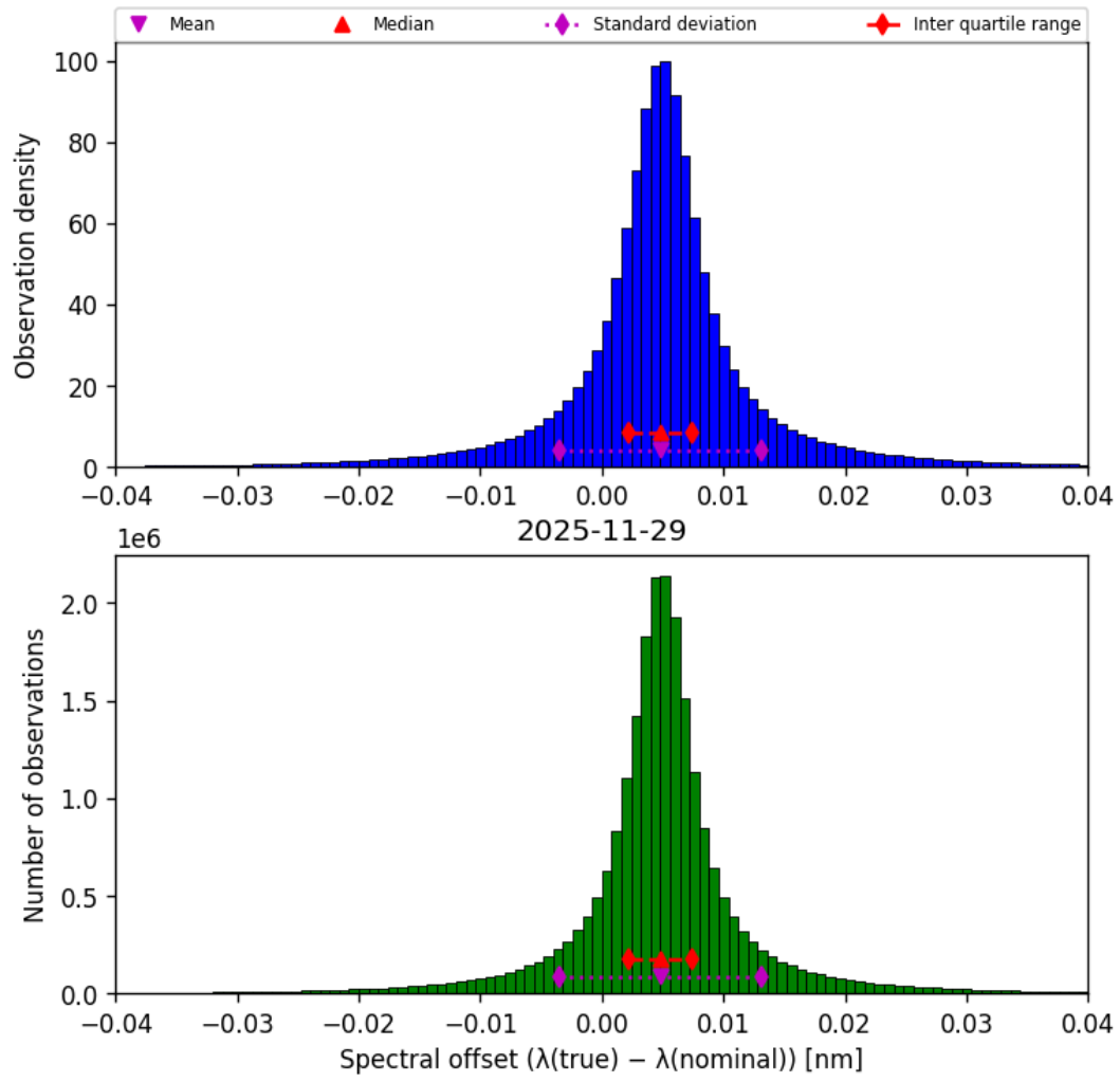
Figure 45: Histogram of “Spectral offset ( \lambda_{\text{true}} - \lambda_{\text{nominal}} )” for 2025-11-28 to 2025-11-30
