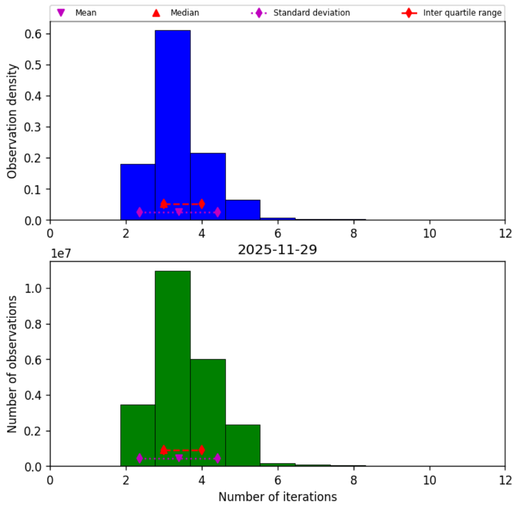
Figure 39: Histogram of “Number of iterations” for 2025-11-28 to 2025-11-30
