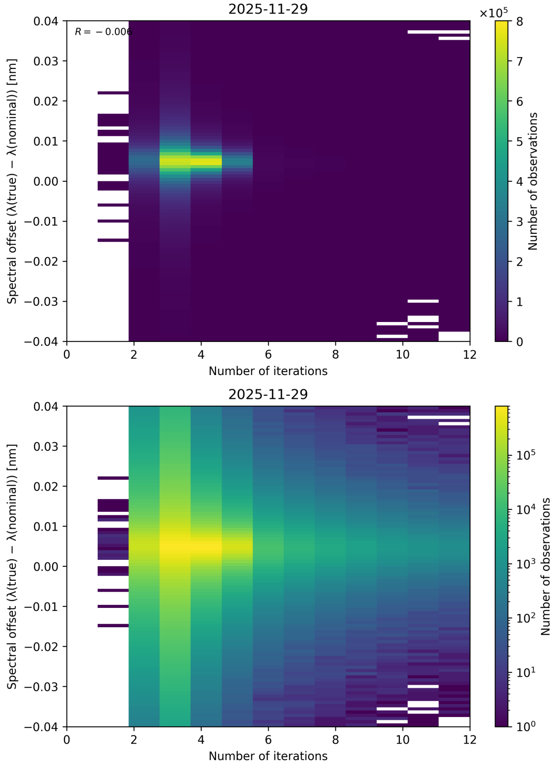
Figure 100: Scatter density plot of “Number of iterations” against “Spectral offset ( \lambda_{\text{true}} - \lambda_{\text{nominal}} )” for 2025-11-28 to 2025-11-30.
