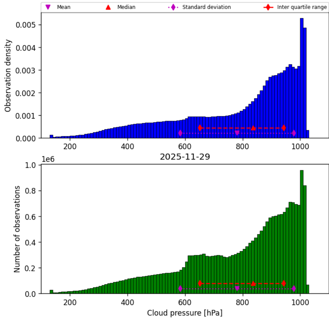
Figure 30: Histogram of “Cloud pressure” for 2025-11-28 to 2025-11-30
