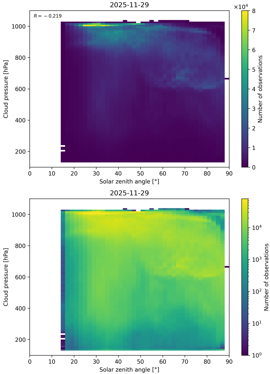
Figure 111: Scatter density plot of “Solar zenith angle” against “Cloud pressure” for 2025-11-28 to 2025-11-30.
