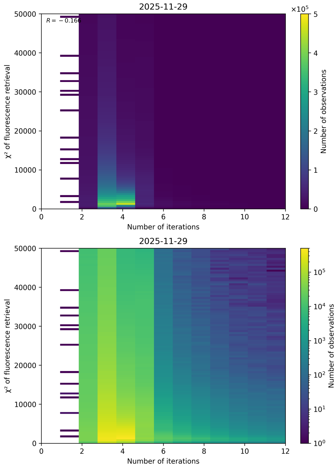
Figure 97: Scatter density plot of “Number of iterations” against “ \chi^2 of fluorescence retrieval” for 2025-11-28 to 2025-11-30.
