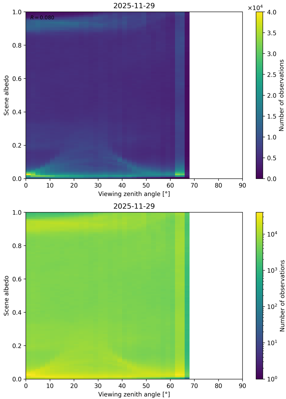
Figure 126: Scatter density plot of “Viewing zenith angle” against “Scene albedo” for 2025-11-28 to 2025-11-30.
