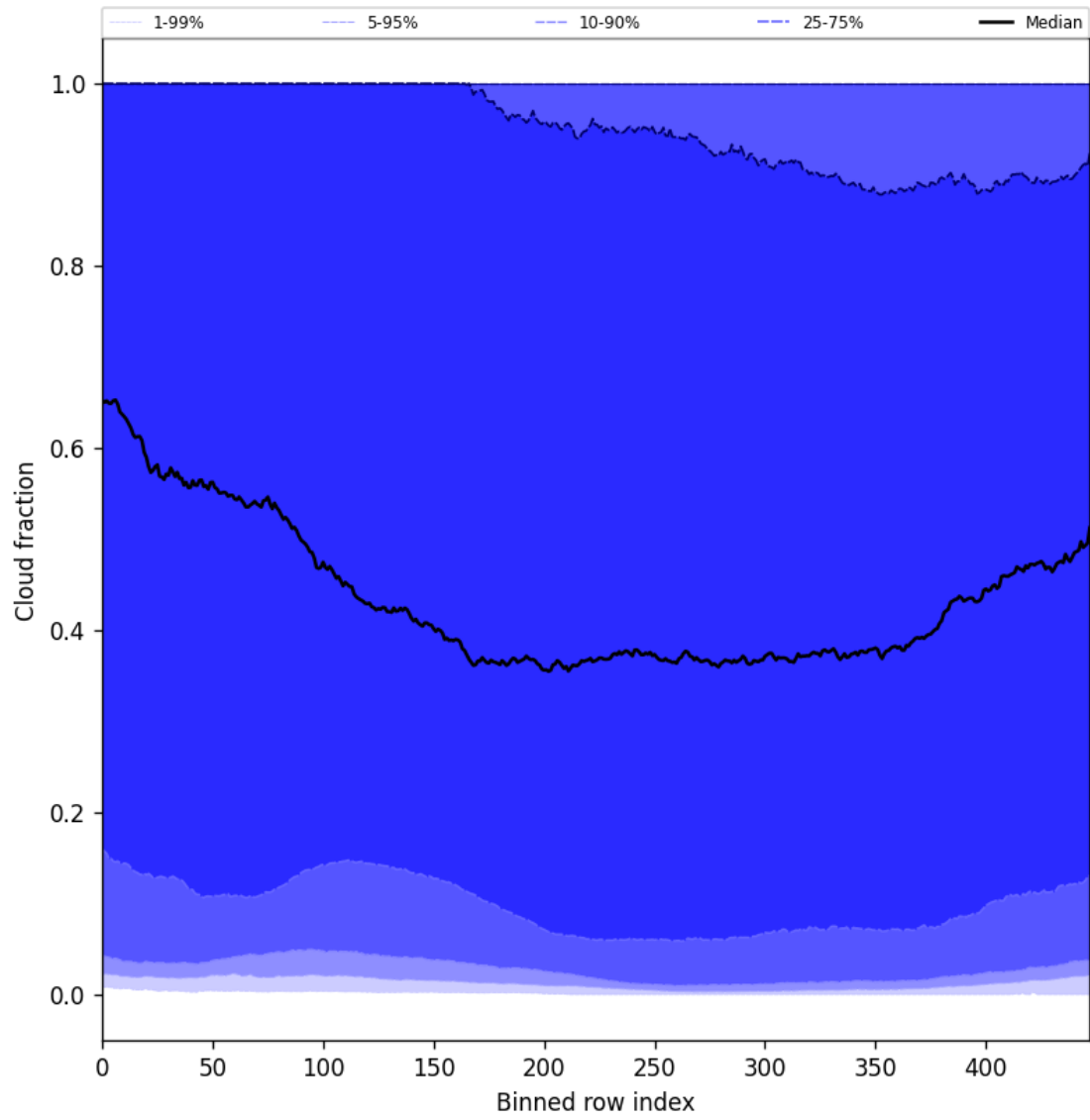
Figure 49: Along track statistics of “Cloud fraction” for 2025-11-28 to 2025-11-30
