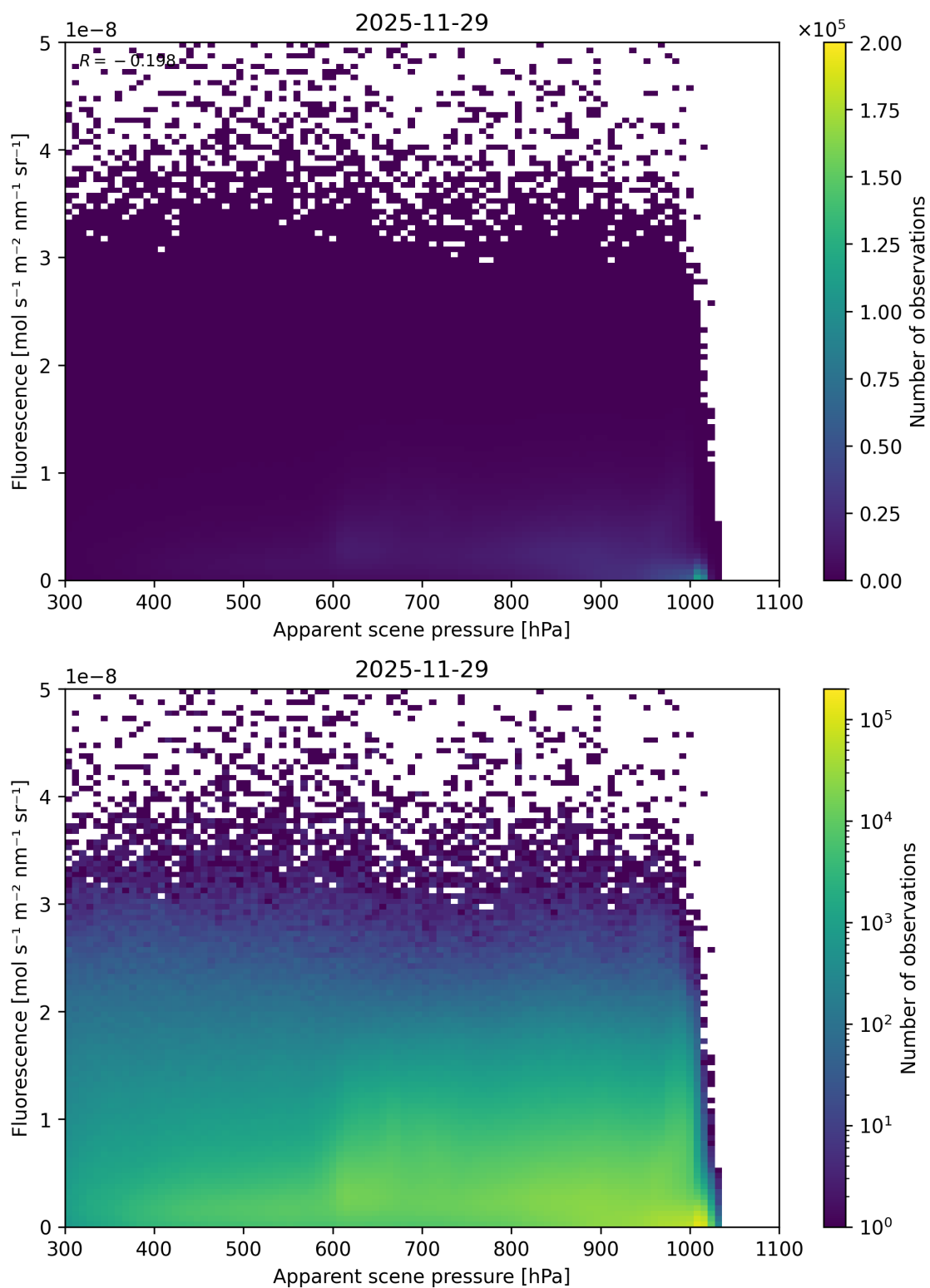
Figure 64: Scatter density plot of “Apparent scene pressure” against “Fluorescence” for 2025-11-28 to 2025-11-30.
