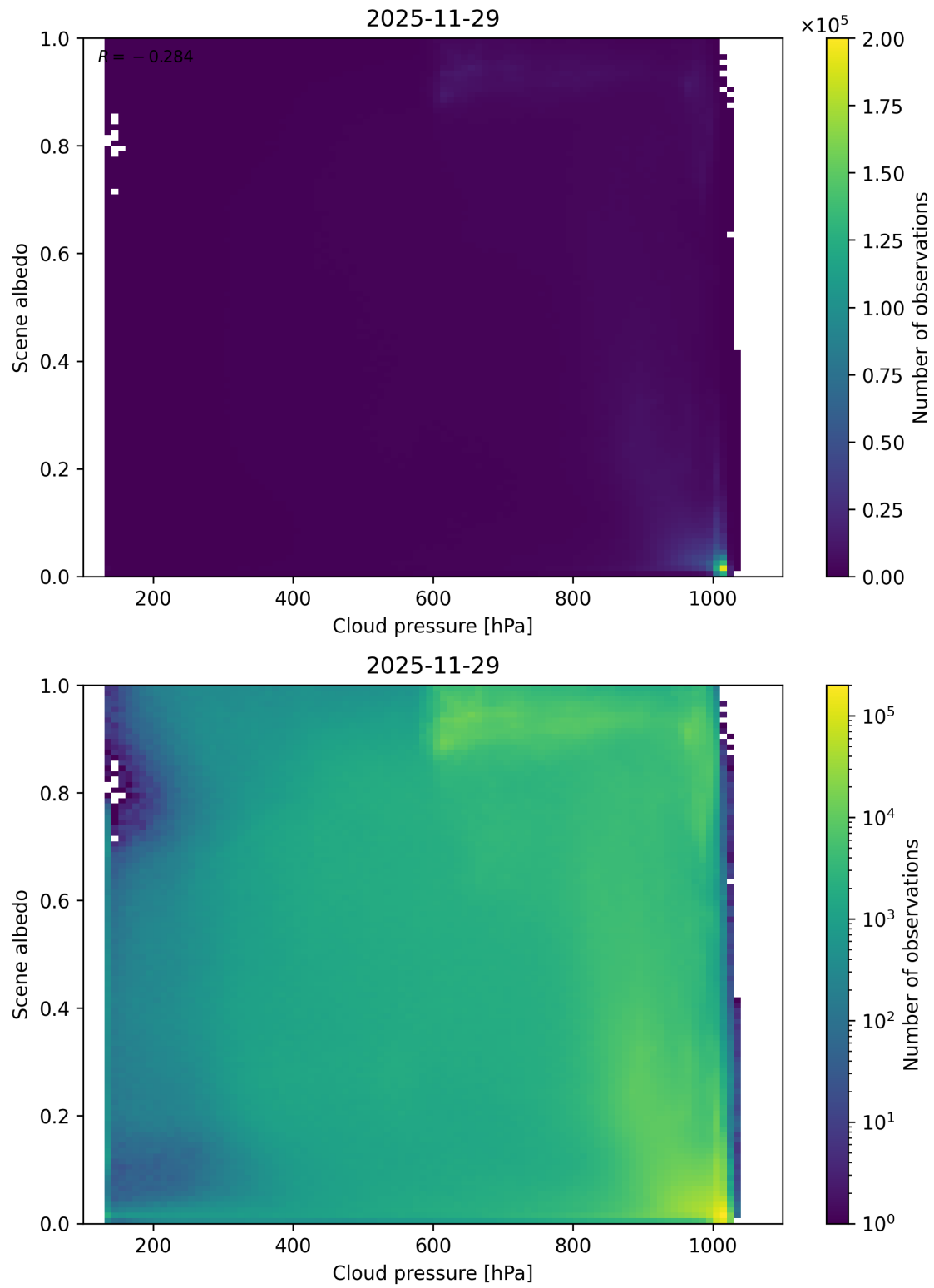
Figure 83: Scatter density plot of “Cloud pressure” against “Scene albedo” for 2025-11-28 to 2025-11-30.
