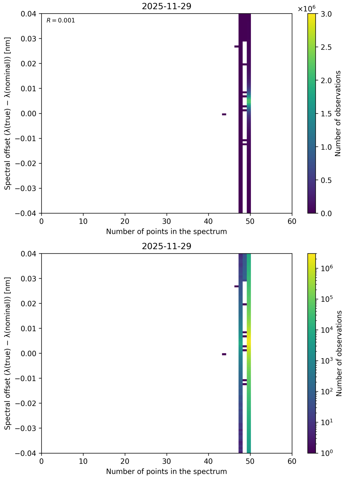
Figure 101: Scatter density plot of “Number of points in the spectrum” against “Spectral offset ( \lambda_{\text{true}} - \lambda_{\text{nominal}} )” for 2025-11-28 to 2025-11-30.
