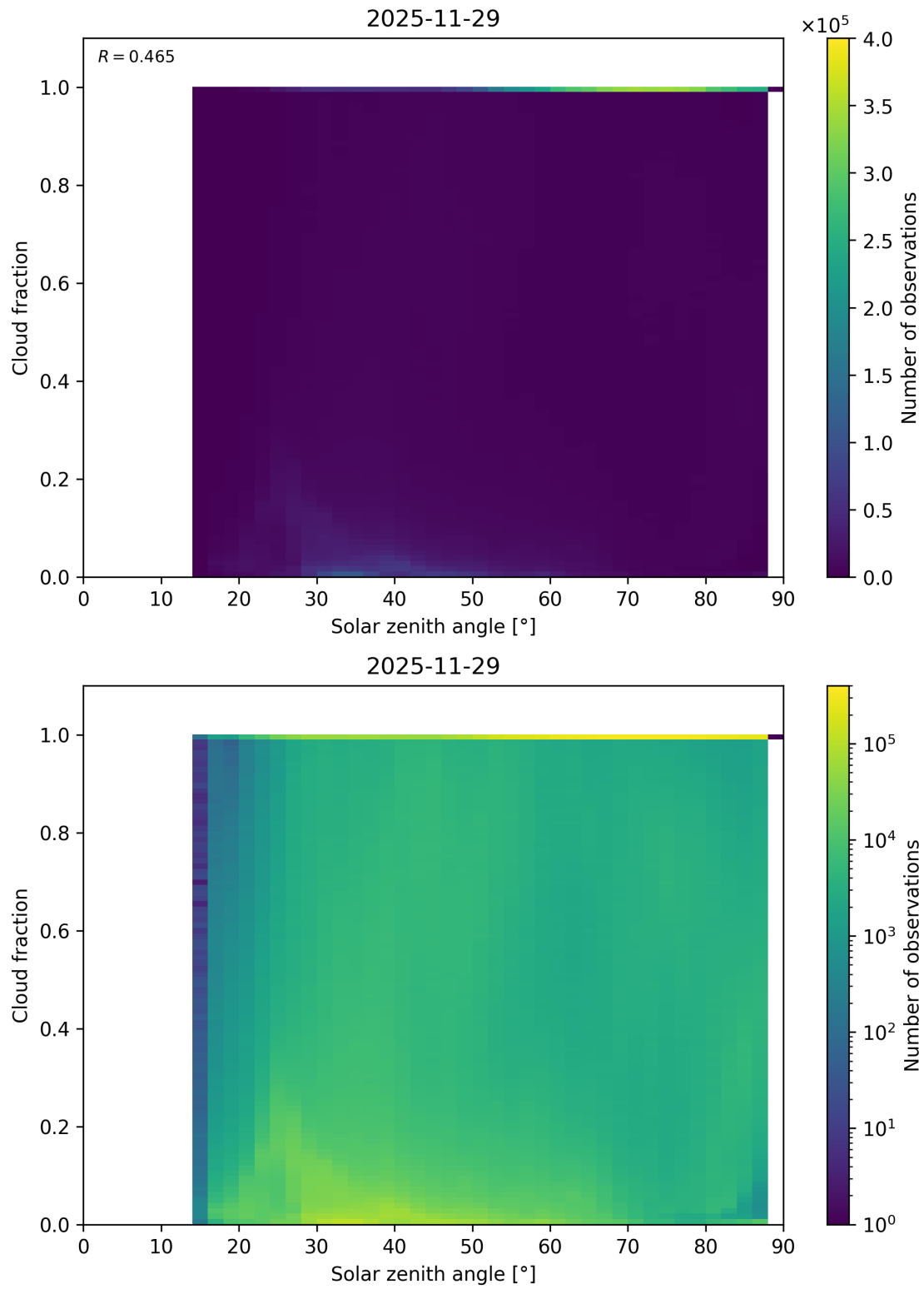
Figure 110: Scatter density plot of “Solar zenith angle” against “Cloud fraction” for 2025-11-28 to 2025-11-30.
