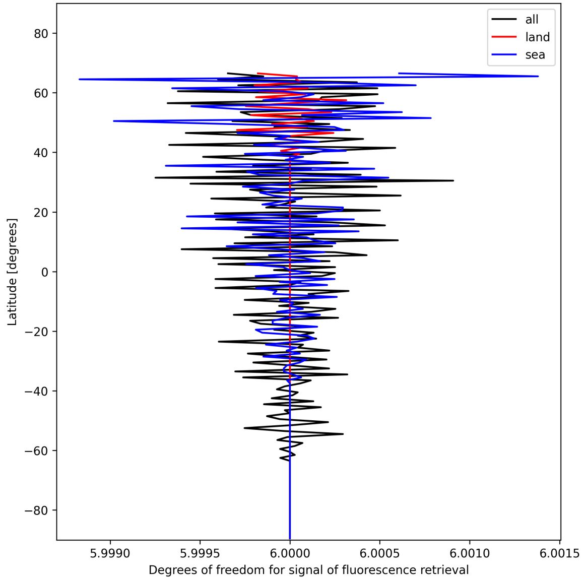
Figure 26: Zonal average of “Degrees of freedom for signal of fluorescence retrieval” for 2025-11-28 to 2025-11-30.
