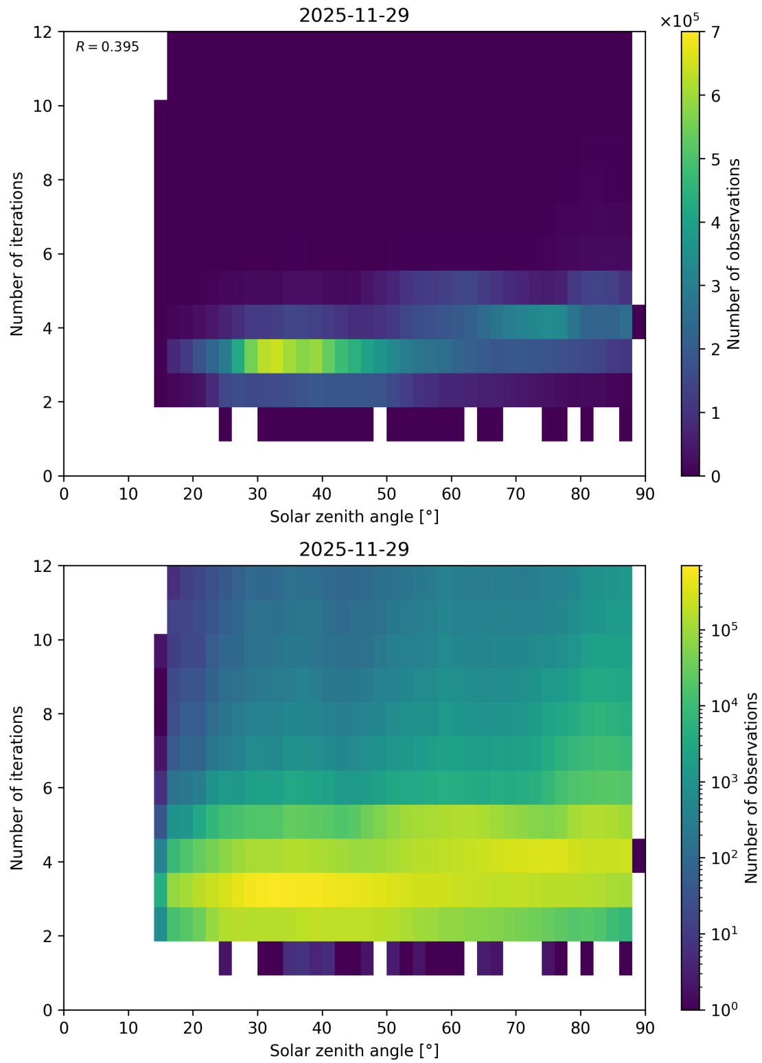
Figure 114: Scatter density plot of “Solar zenith angle” against “Number of iterations” for 2025-11-28 to 2025-11-30.
