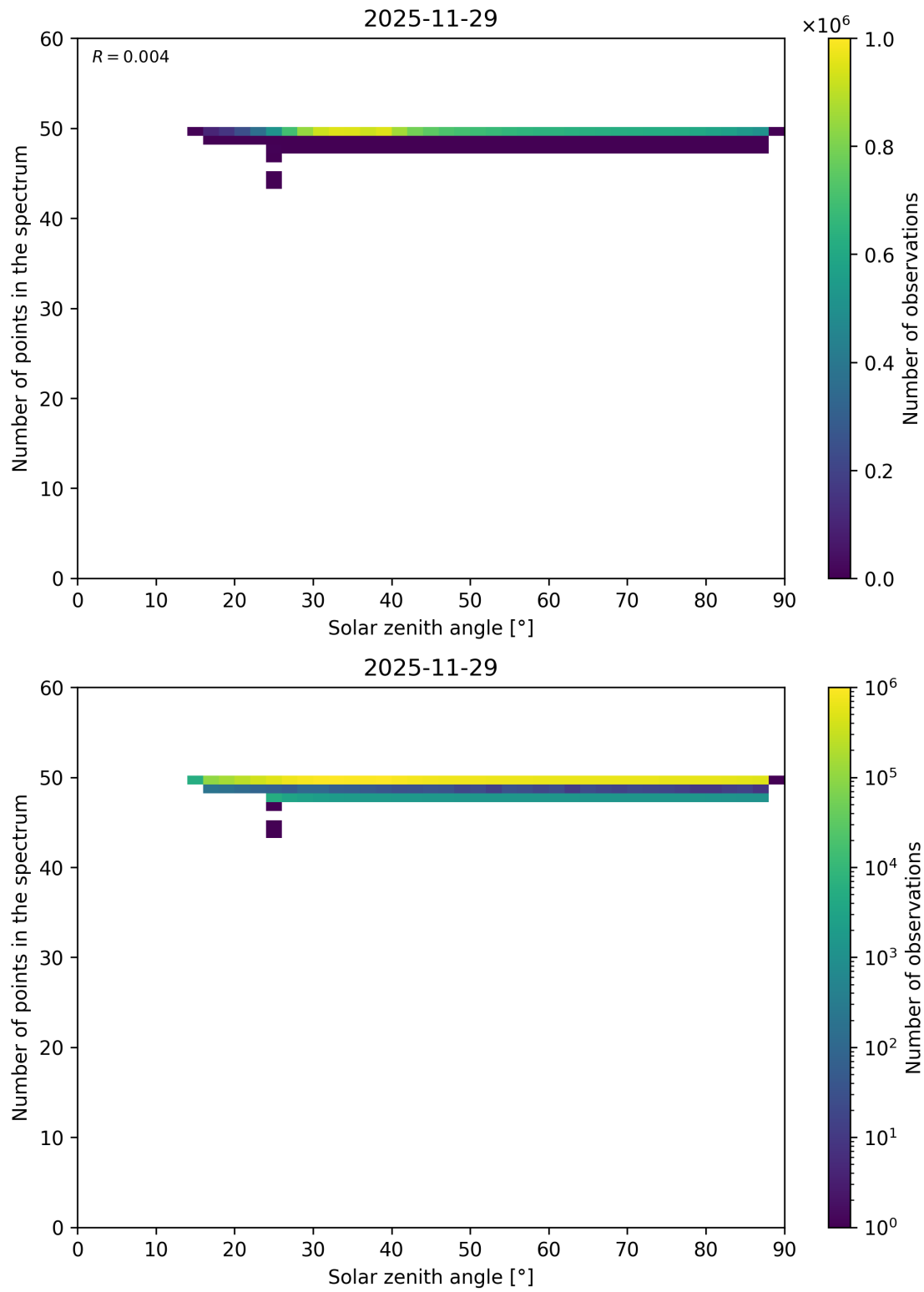
Figure 115: Scatter density plot of “Solar zenith angle” against “Number of points in the spectrum” for 2025-11-28 to 2025-11-30.
