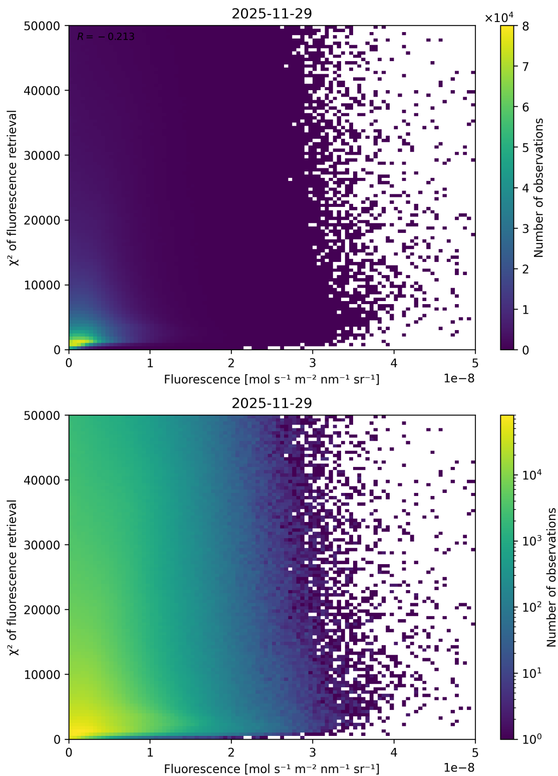
Figure 85: Scatter density plot of “Fluorescence” against “ \chi^2 of fluorescence retrieval” for 2025-11-28 to 2025-11-30.
