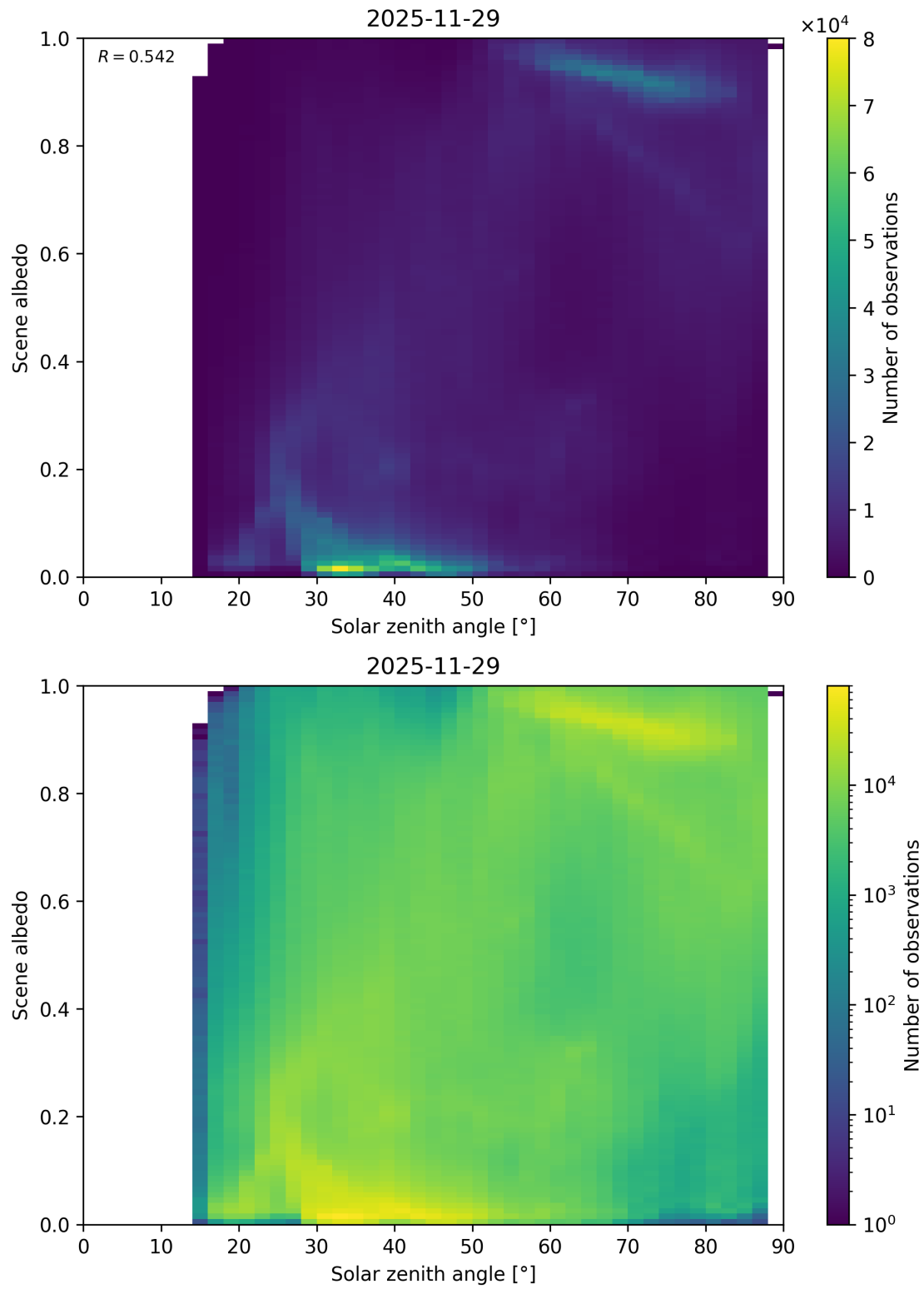
Figure 116: Scatter density plot of “Solar zenith angle” against “Scene albedo” for 2025-11-28 to 2025-11-30.
