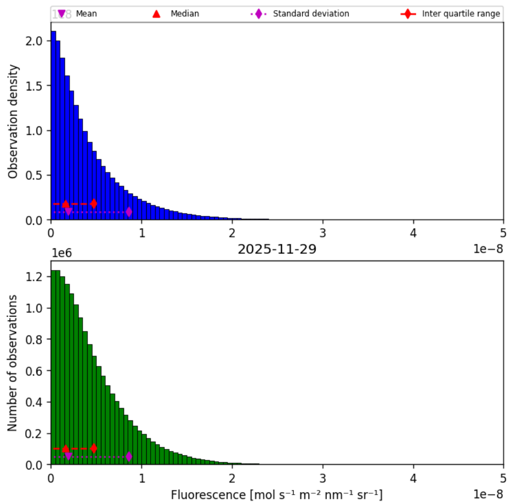
Figure 40: Histogram of “Fluorescence” for 2025-11-28 to 2025-11-30
