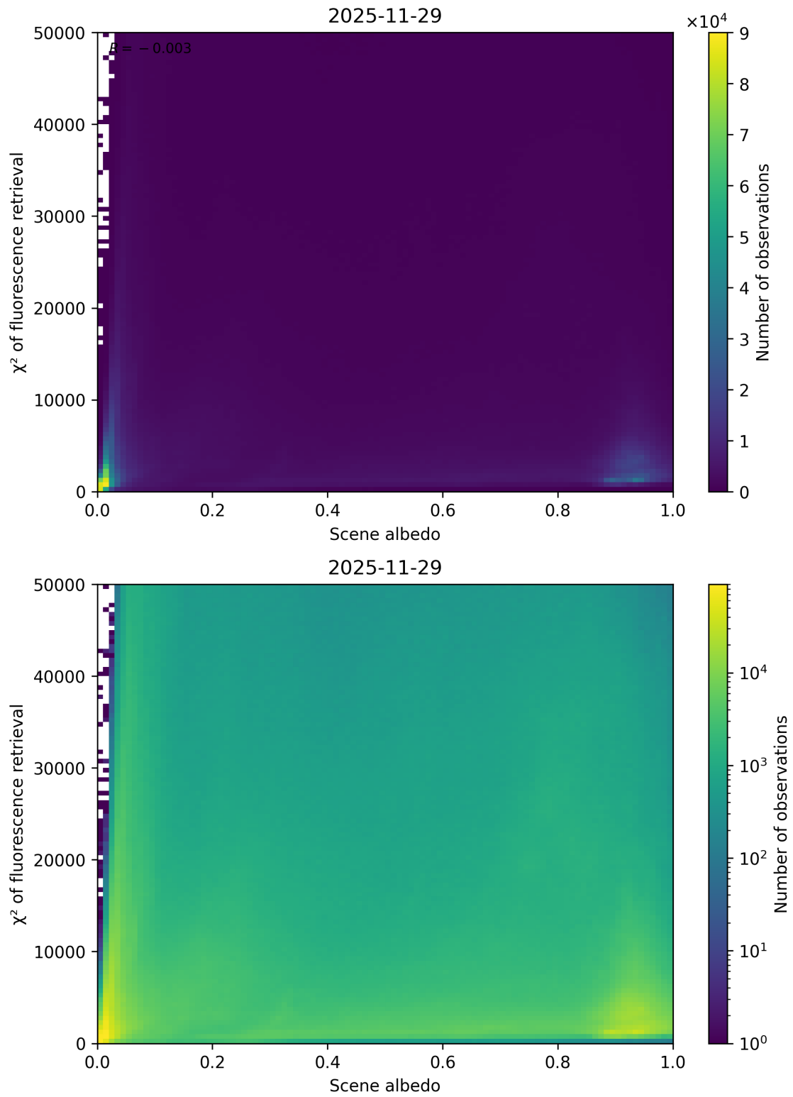
Figure 103: Scatter density plot of “Scene albedo” against “ \chi^2 of fluorescence retrieval” for 2025-11-28 to 2025-11-30.
