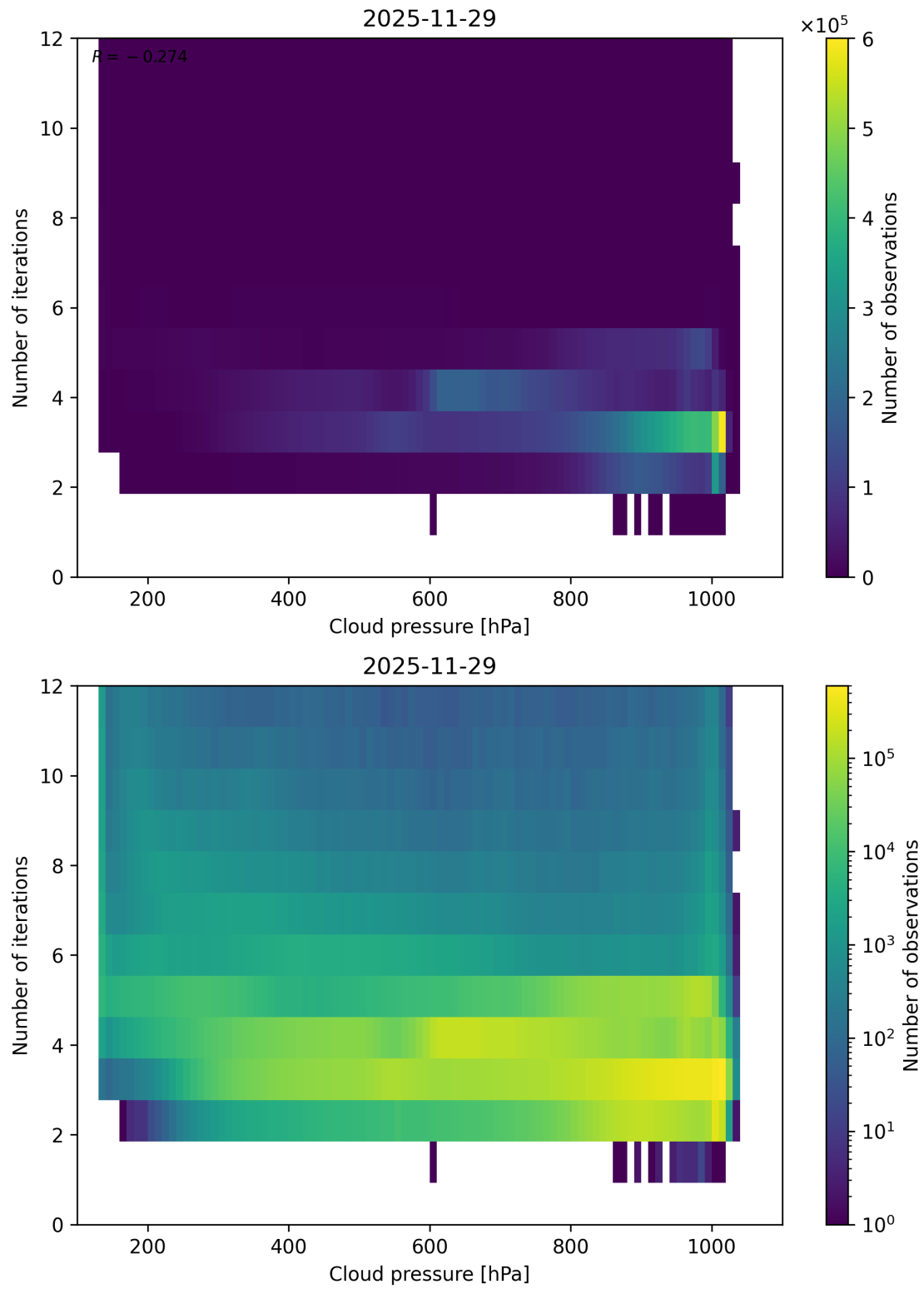
Figure 81: Scatter density plot of “Cloud pressure” against “Number of iterations” for 2025-11-28 to 2025-11-30.
