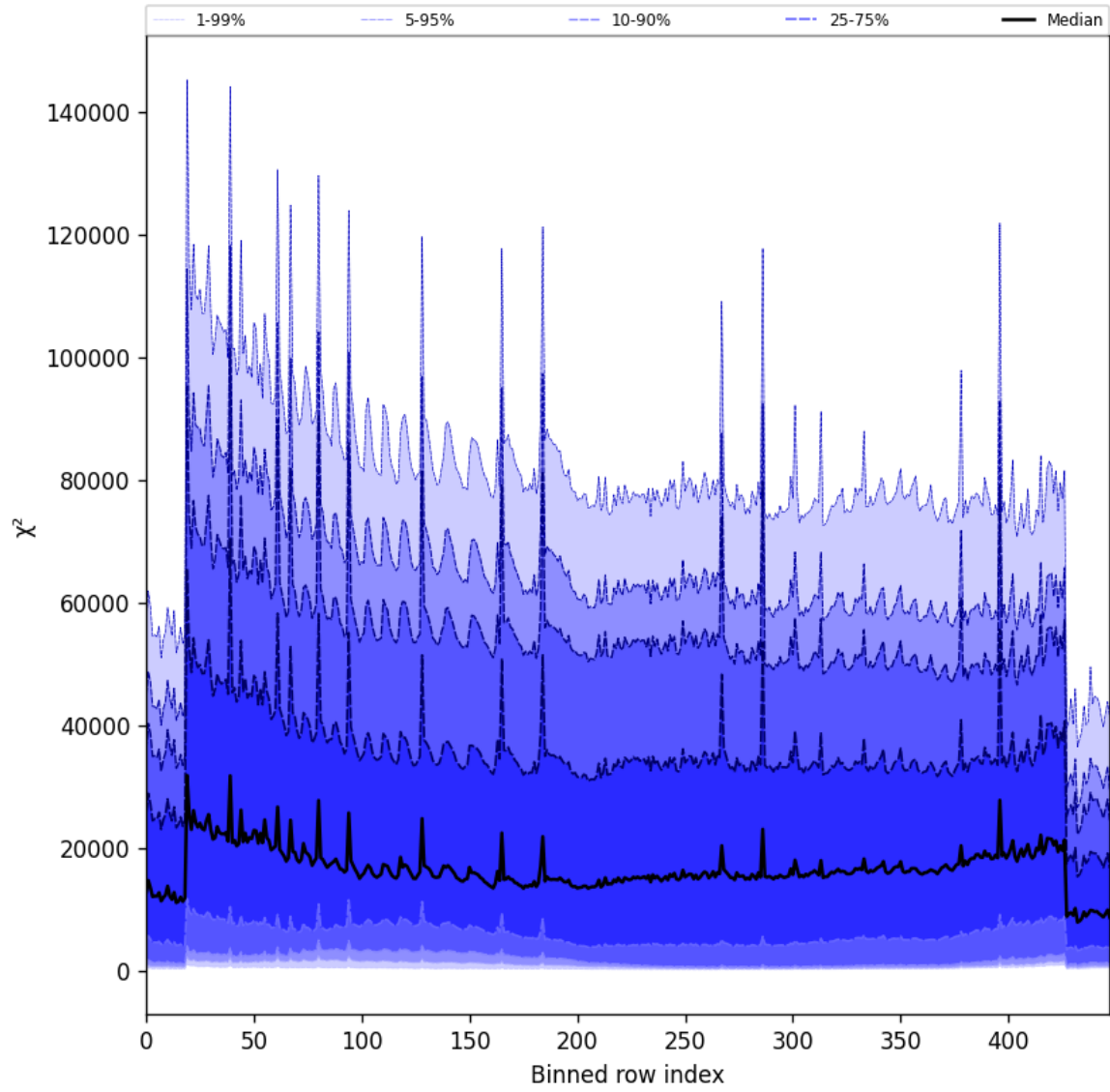
Figure 55: Along track statistics of “ \chi^2 ” for 2025-11-28 to 2025-11-30
