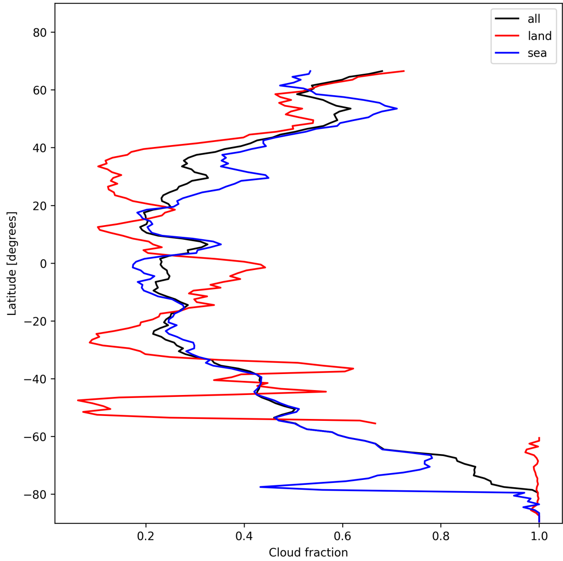
Figure 15: Zonal average of “Cloud fraction” for 2025-11-28 to 2025-11-30.
