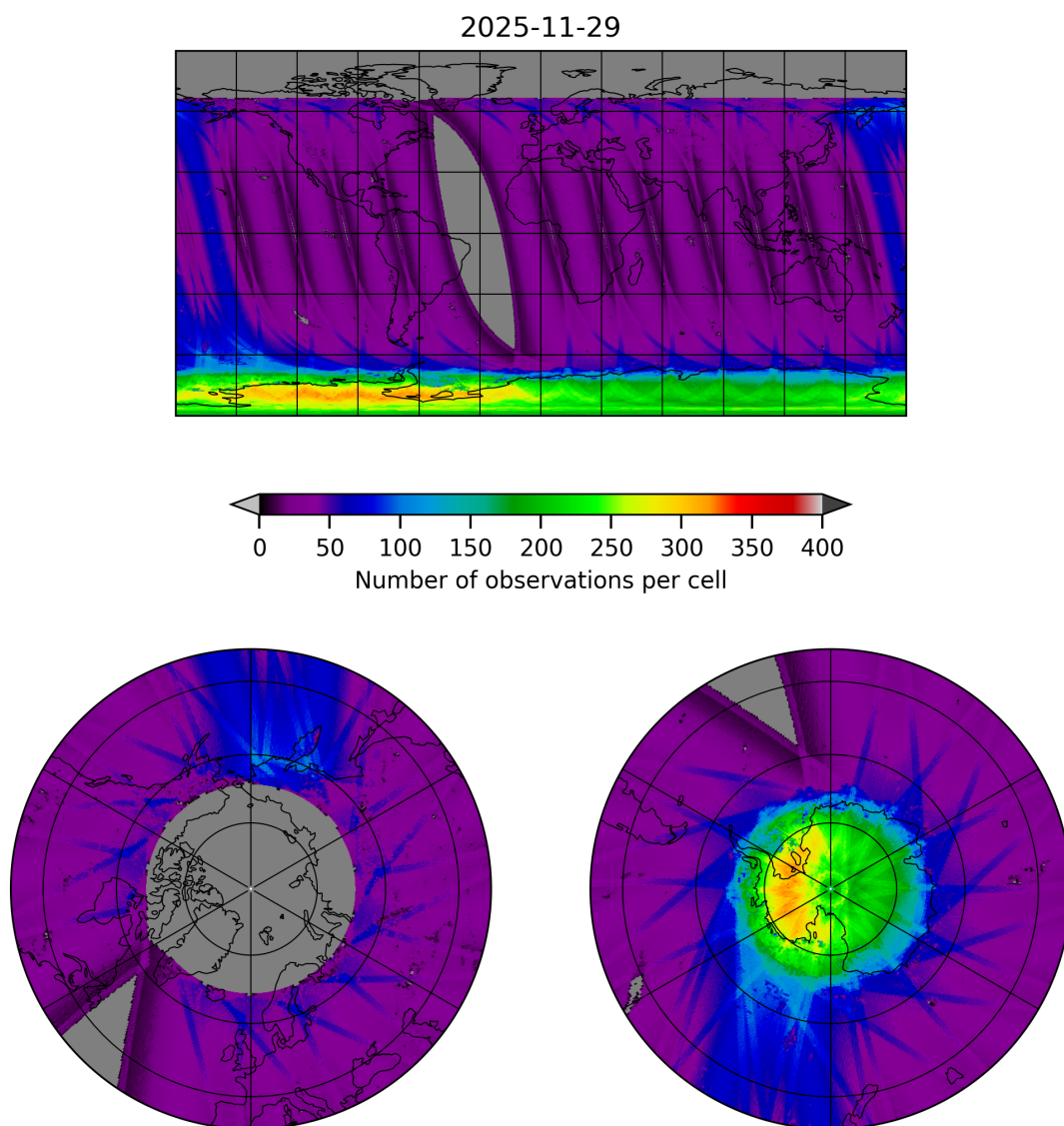
Figure 11: Map of the number of observations for 2025-11-28 to 2025-11-30
