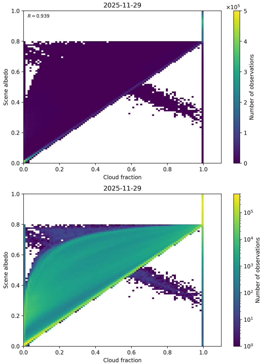
Figure 75: Scatter density plot of “Cloud fraction” against “Scene albedo” for 2025-11-28 to 2025-11-30.
