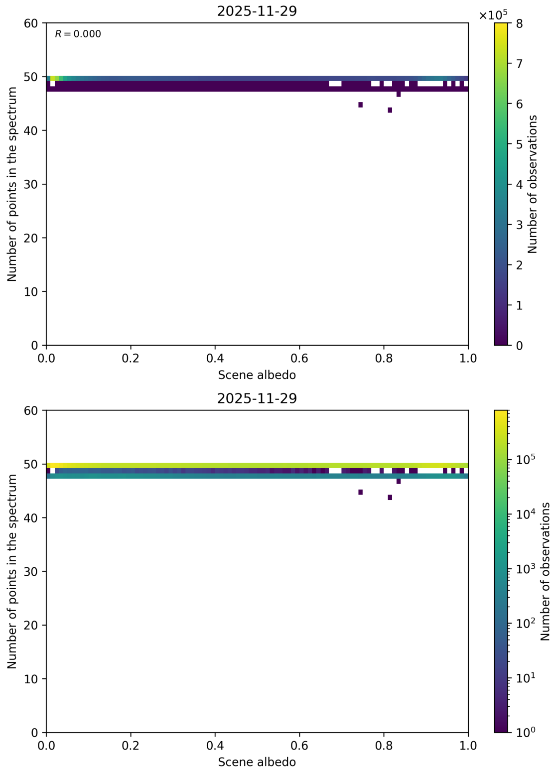
Figure 106: Scatter density plot of “Scene albedo” against “Number of points in the spectrum” for 2025-11-28 to 2025-11-30.
