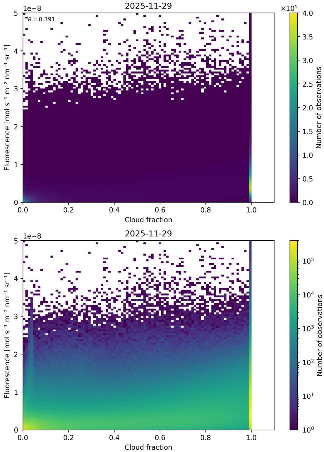
Figure 72: Scatter density plot of “Cloud fraction” against “Fluorescence” for 2025-11-28 to 2025-11-30.
