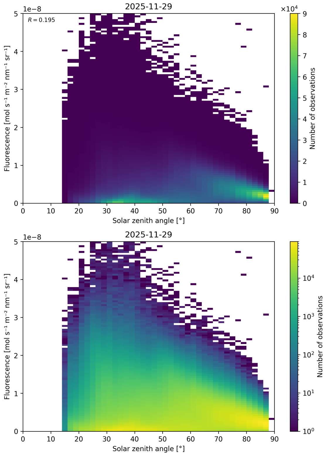
Figure 112: Scatter density plot of “Solar zenith angle” against “Fluorescence” for 2025-11-28 to 2025-11-30.
