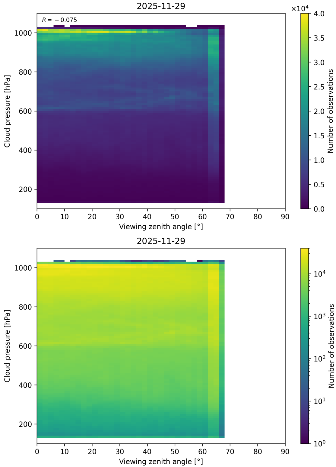
Figure 121: Scatter density plot of “Viewing zenith angle” against “Cloud pressure” for 2025-11-28 to 2025-11-30.
