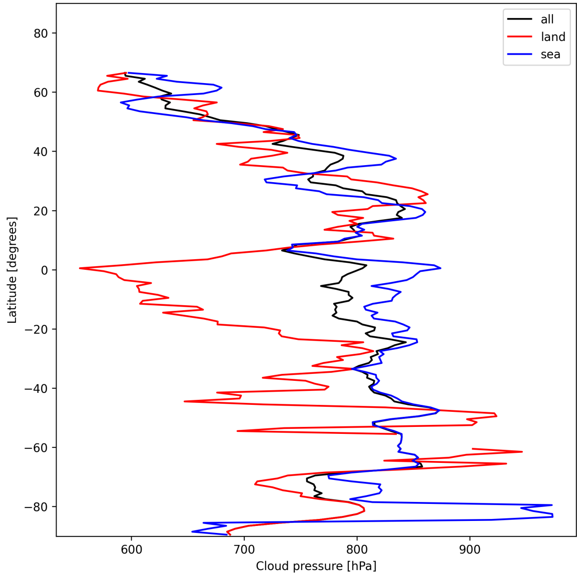
Figure 13: Zonal average of “Cloud pressure” for 2025-11-28 to 2025-11-30.
