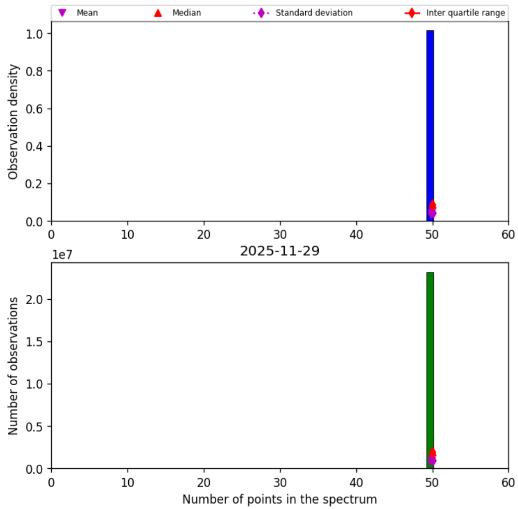
Figure 44: Histogram of “Number of points in the spectrum” for 2025-11-28 to 2025-11-30
