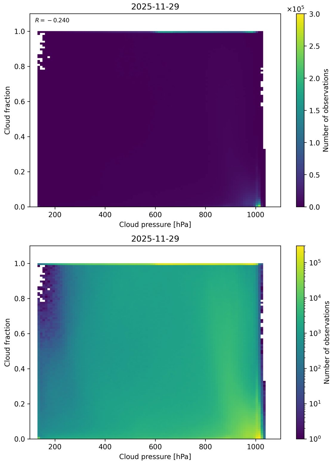
Figure 79: Scatter density plot of “Cloud pressure” against “Cloud fraction” for 2025-11-28 to 2025-11-30.
