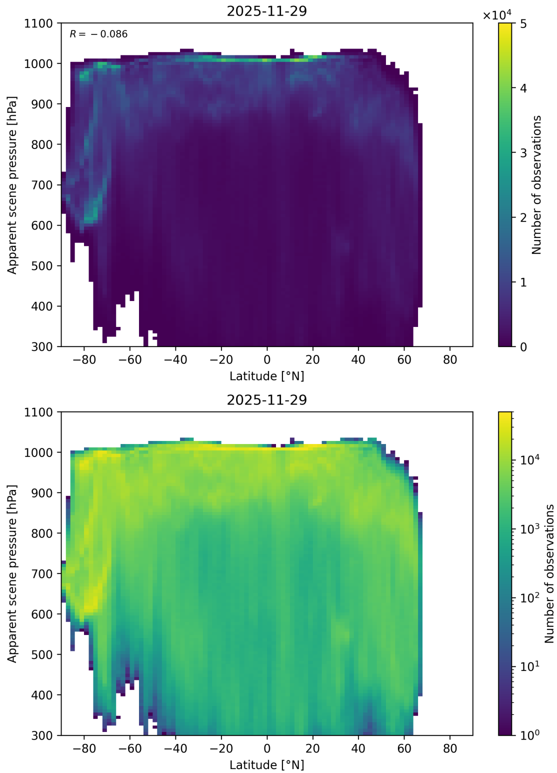
Figure 88: Scatter density plot of “Latitude” against “Apparent scene pressure” for 2025-11-28 to 2025-11-30.
