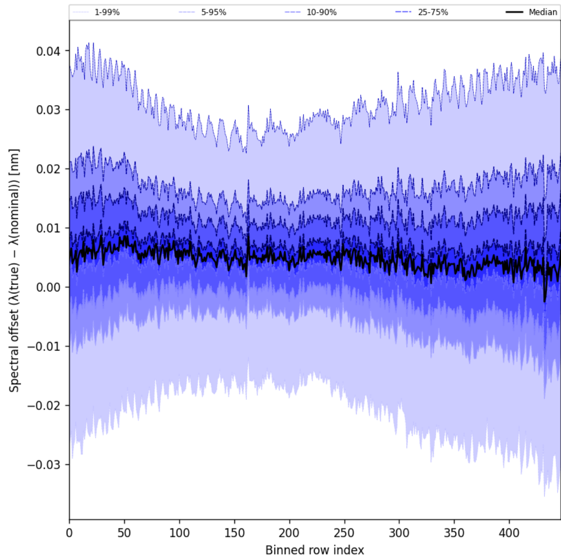
Figure 62: Along track statistics of “Spectral offset ( \lambda_{\text{true}} - \lambda_{\text{nominal}} )” for 2025-11-28 to 2025-11-30
