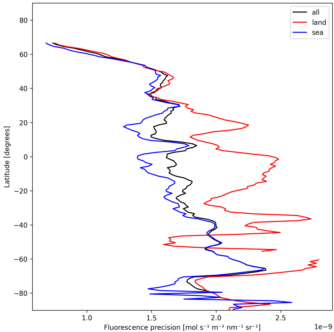
Figure 24: Zonal average of “Fluorescence precision” for 2025-11-28 to 2025-11-30.
