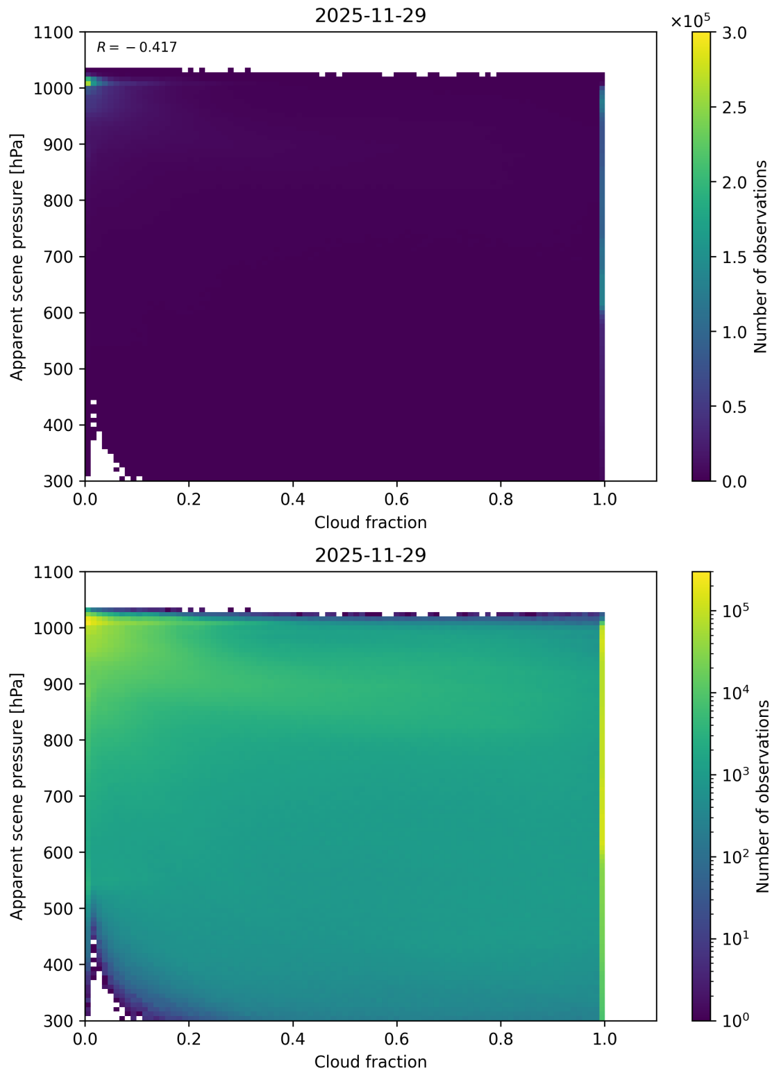
Figure 70: Scatter density plot of “Cloud fraction” against “Apparent scene pressure” for 2025-11-28 to 2025-11-30.
