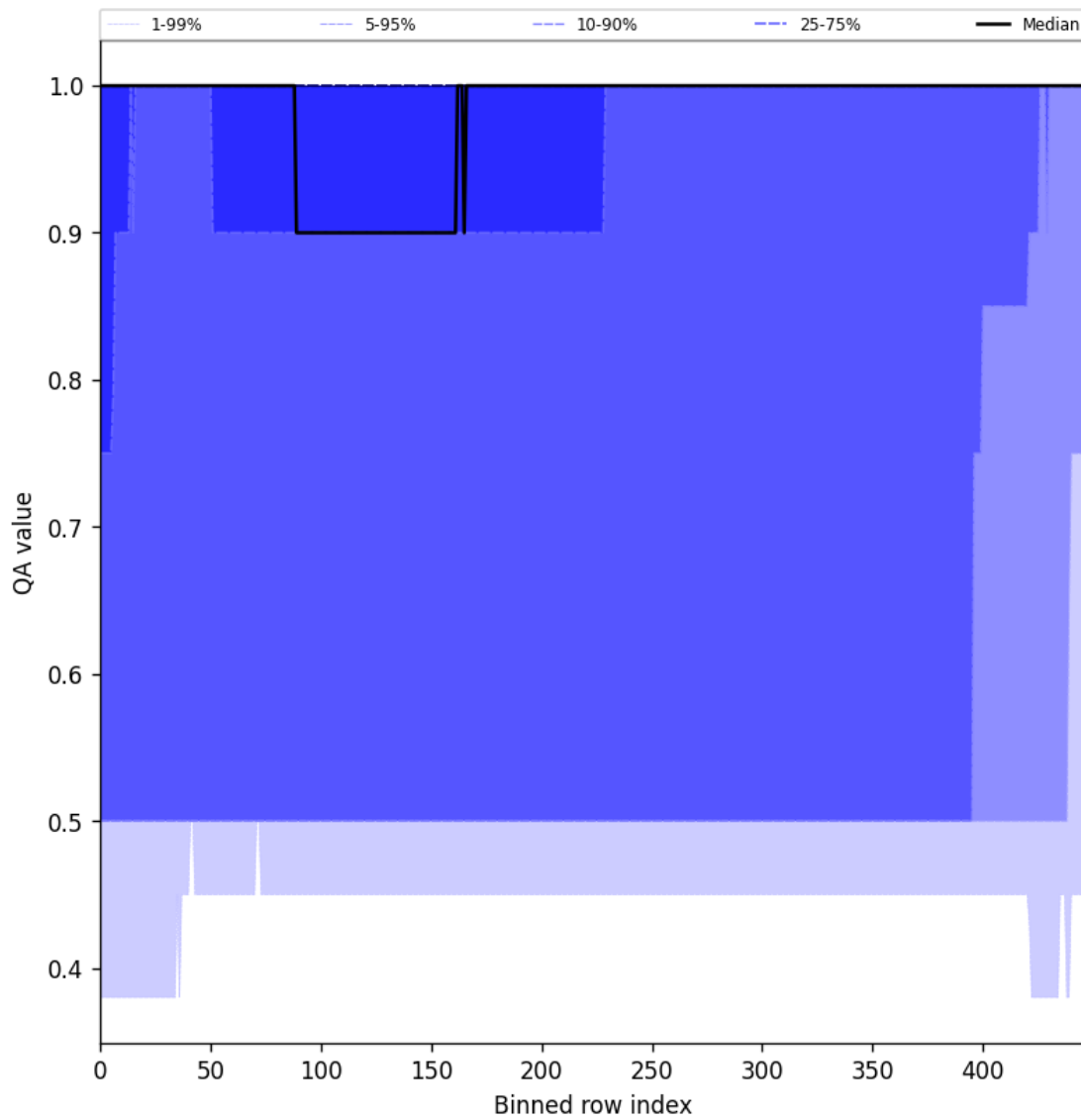
Figure 46: Along track statistics of “QA value” for 2025-11-28 to 2025-11-30
