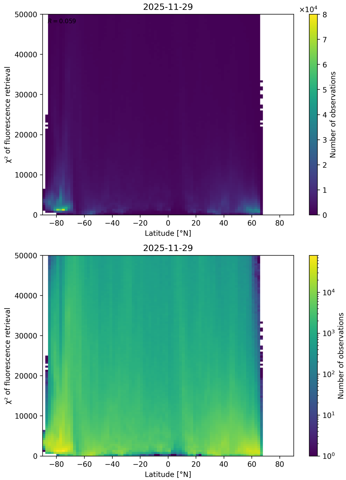
Figure 89: Scatter density plot of “Latitude” against “ \chi^2 of fluorescence retrieval” for 2025-11-28 to 2025-11-30.
