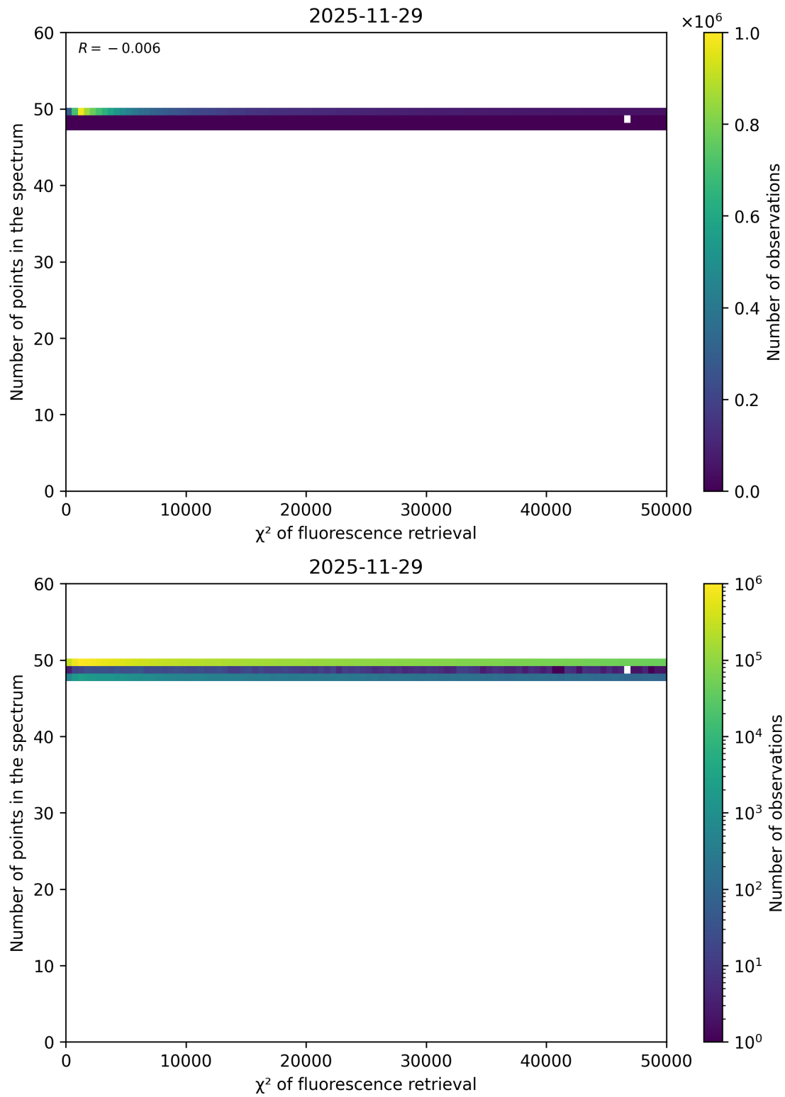
Figure 68: Scatter density plot of " \chi^2 of fluorescence retrieval" against "Number of points in the spectrum" for 2025-11-28 to 2025-11-30.
