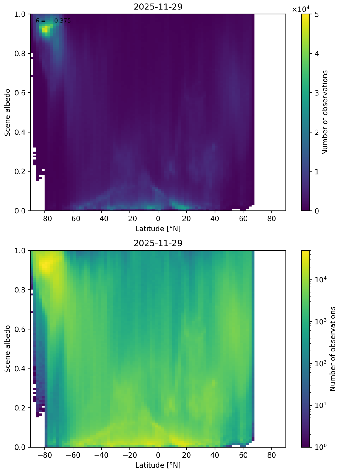
Figure 95: Scatter density plot of “Latitude” against “Scene albedo” for 2025-11-28 to 2025-11-30.
