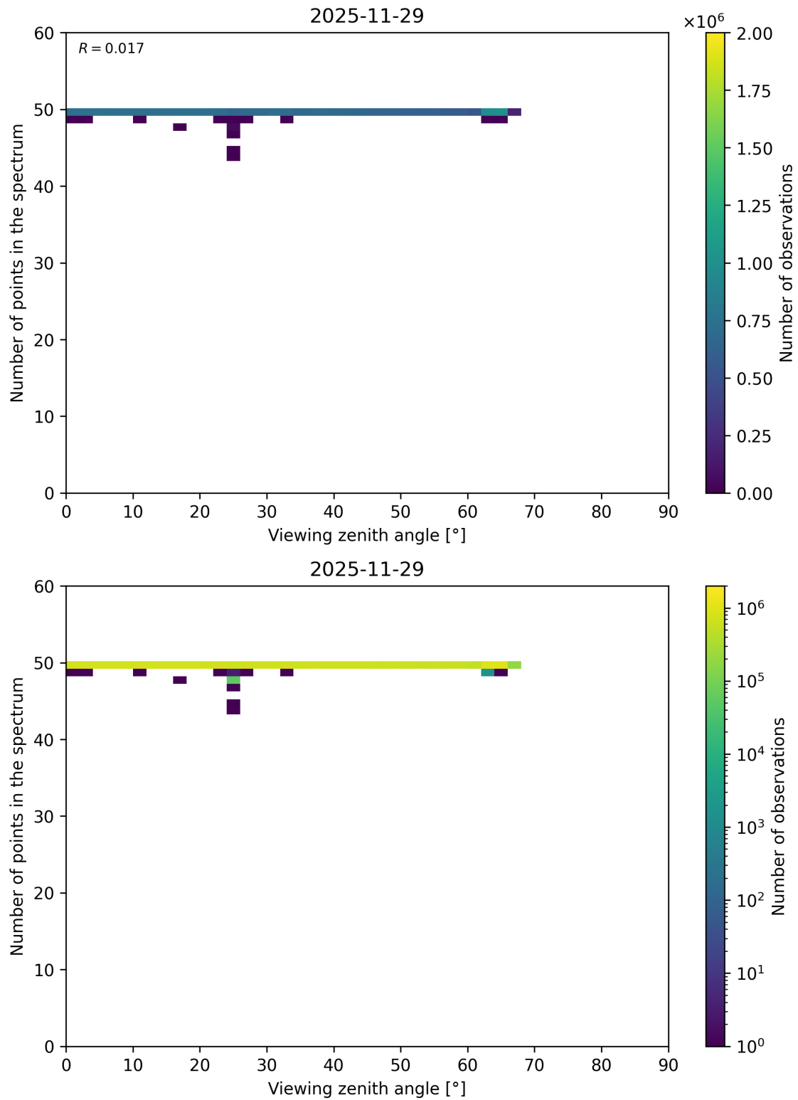
Figure 125: Scatter density plot of “Viewing zenith angle” against “Number of points in the spectrum” for 2025-11-28 to 2025-11-30.
