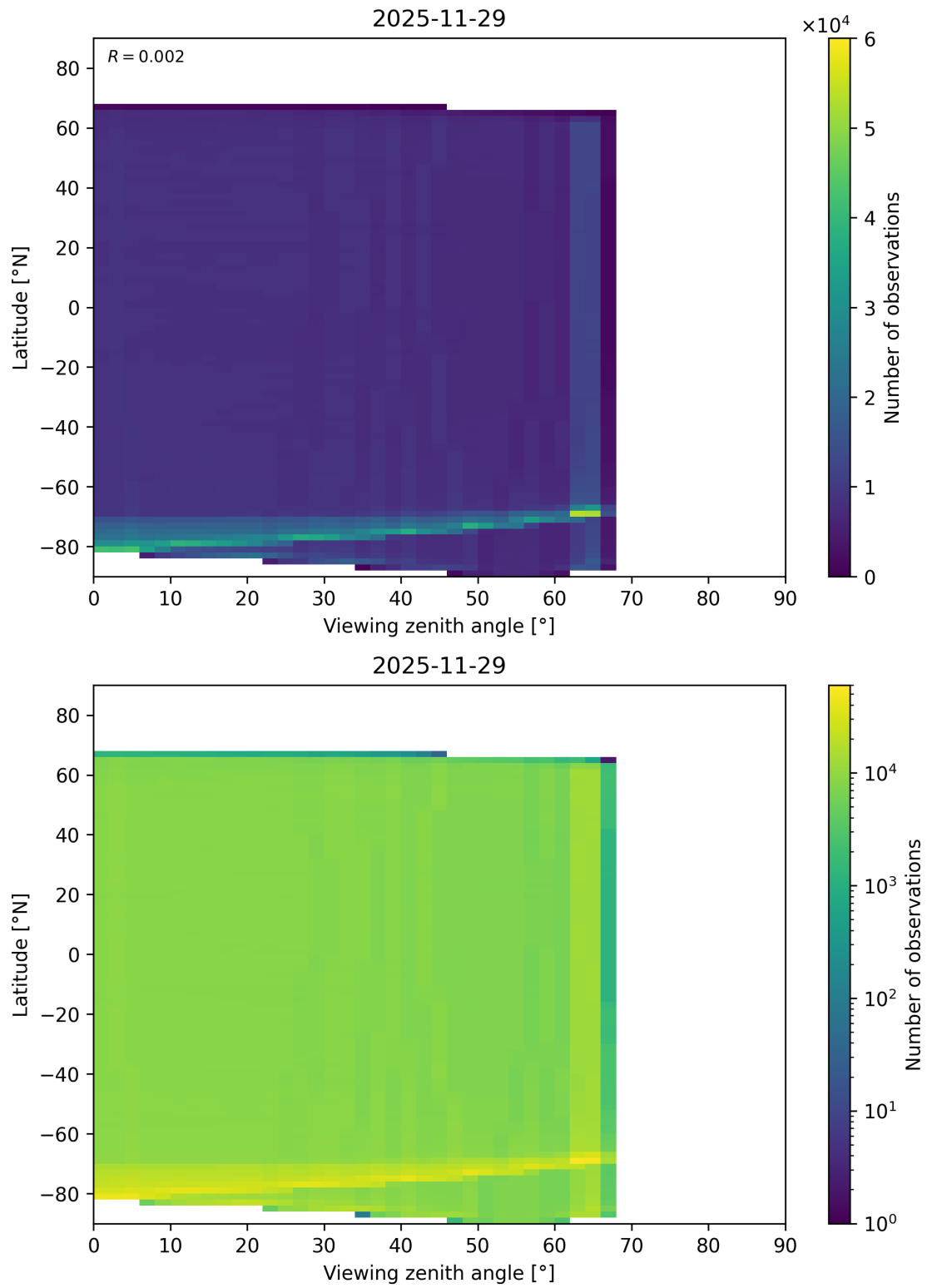
Figure 123: Scatter density plot of “Viewing zenith angle” against “Latitude” for 2025-11-28 to 2025-11-30.
