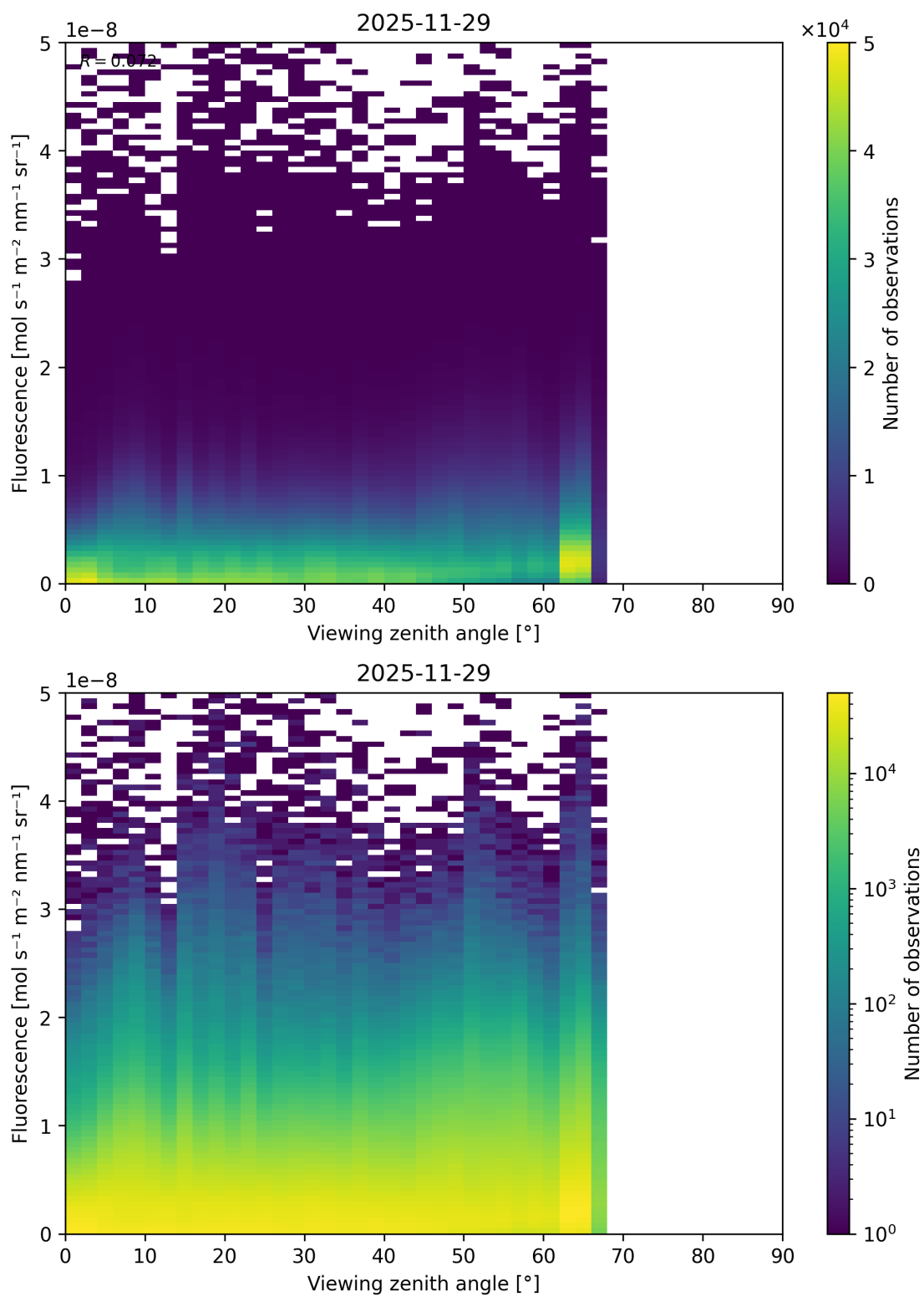
Figure 122: Scatter density plot of “Viewing zenith angle” against “Fluorescence” for 2025-11-28 to 2025-11-30.
