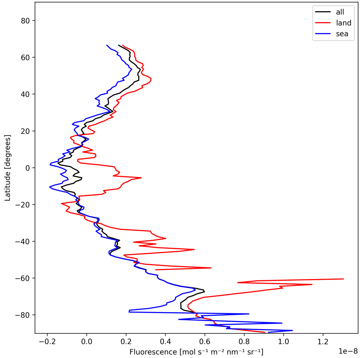
Figure 23: Zonal average of “Fluorescence” for 2025-11-28 to 2025-11-30.
