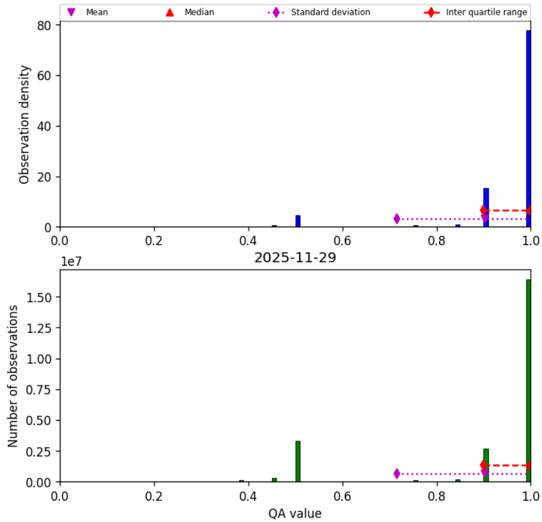
Figure 29: Histogram of “QA value” for 2025-11-28 to 2025-11-30
