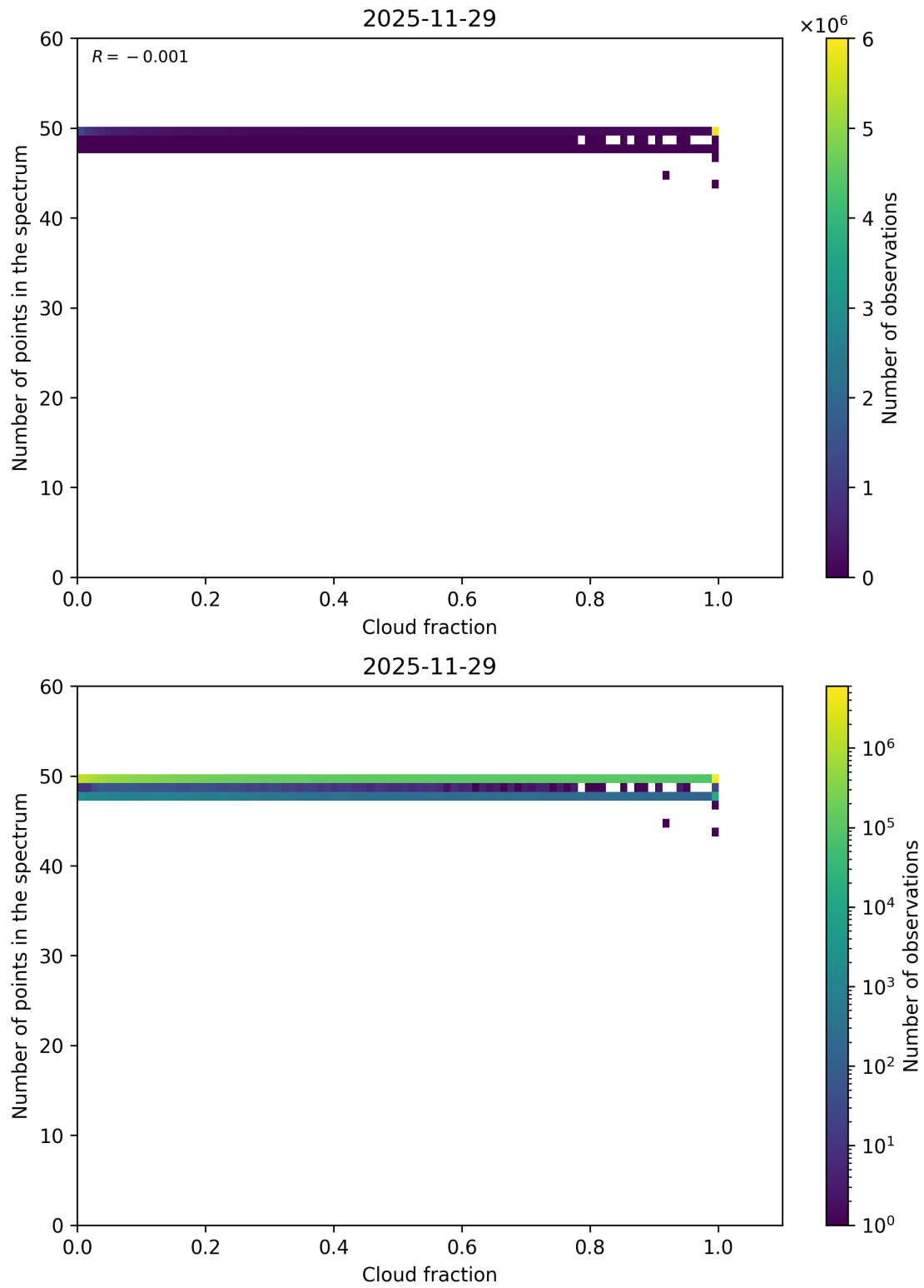
Figure 74: Scatter density plot of “Cloud fraction” against “Number of points in the spectrum” for 2025-11-28 to 2025-11-30.
