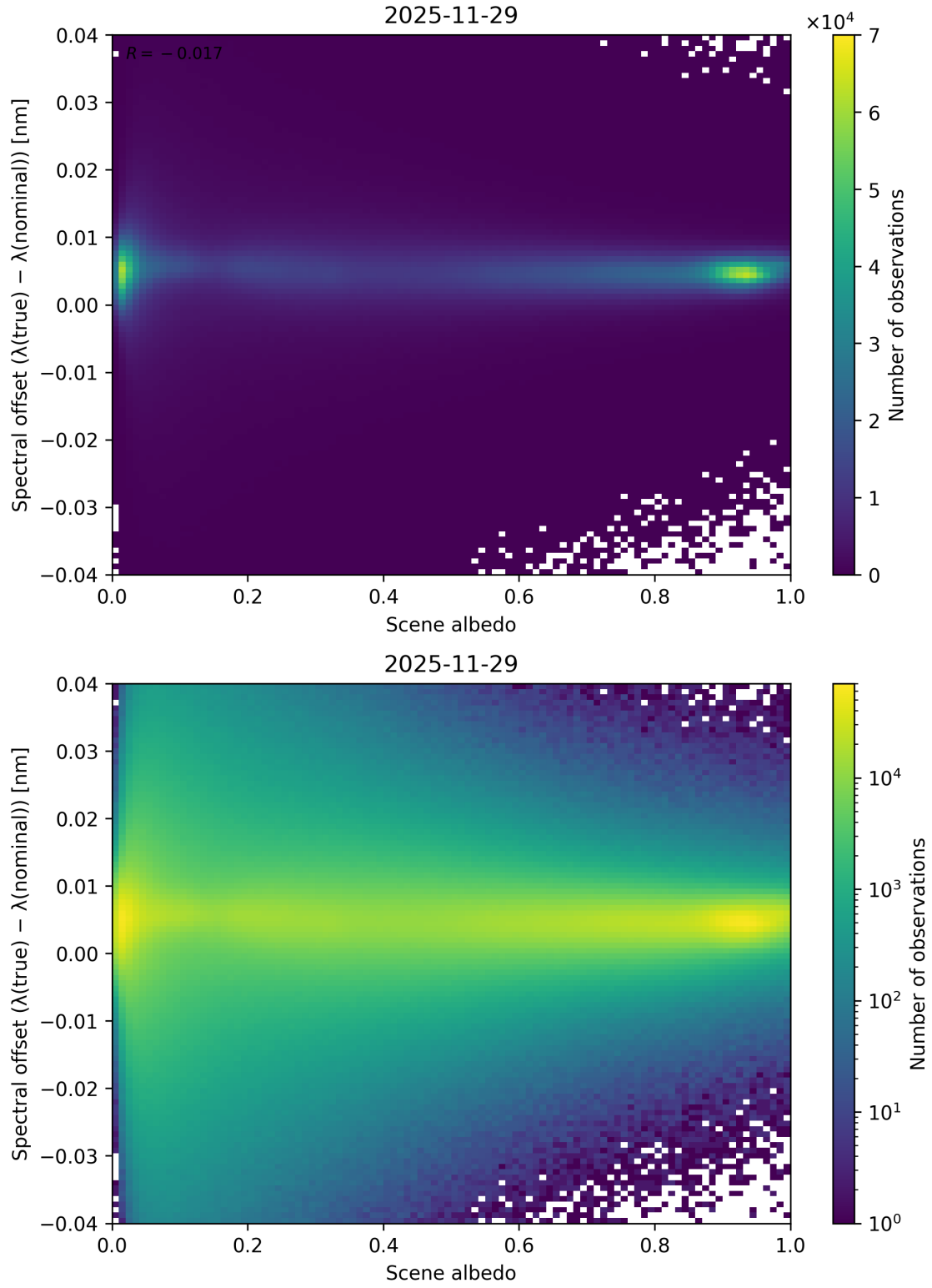
Figure 107: Scatter density plot of “Scene albedo” against “Spectral offset ( \lambda_{\text{true}} - \lambda_{\text{nominal}} )” for 2025-11-28 to 2025-11-30.
