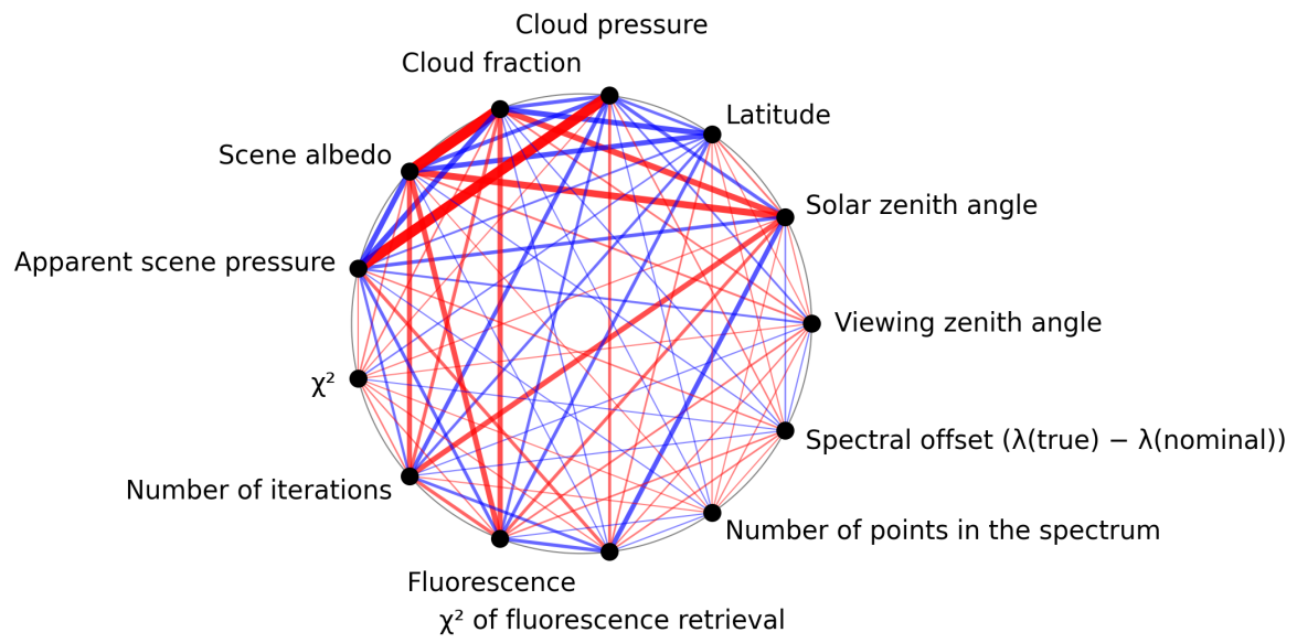
Figure 1: Map of correlation graph for 2025-11-28 to 2025-11-30.
