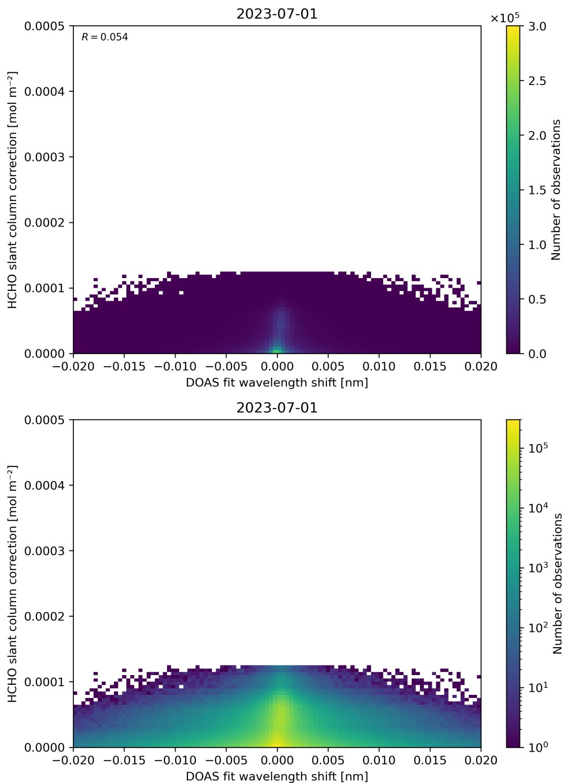
Figure 67: Scatter density plot of “DOAS fit wavelength shift” against “HCHO slant column correction” for 2023-06-30 to 2023-07-02.
