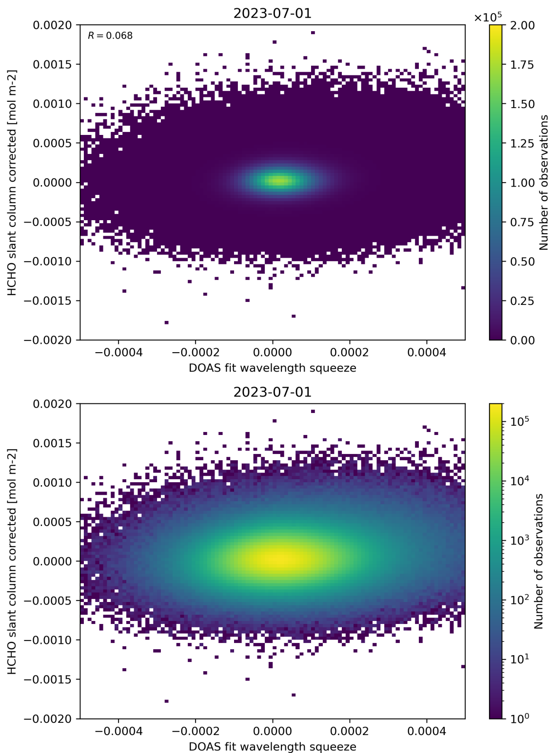
Figure 69: Scatter density plot of “DOAS fit wavelength squeeze” against “HCHO slant column corrected” for 2023-06-30 to 2023-07-02.
