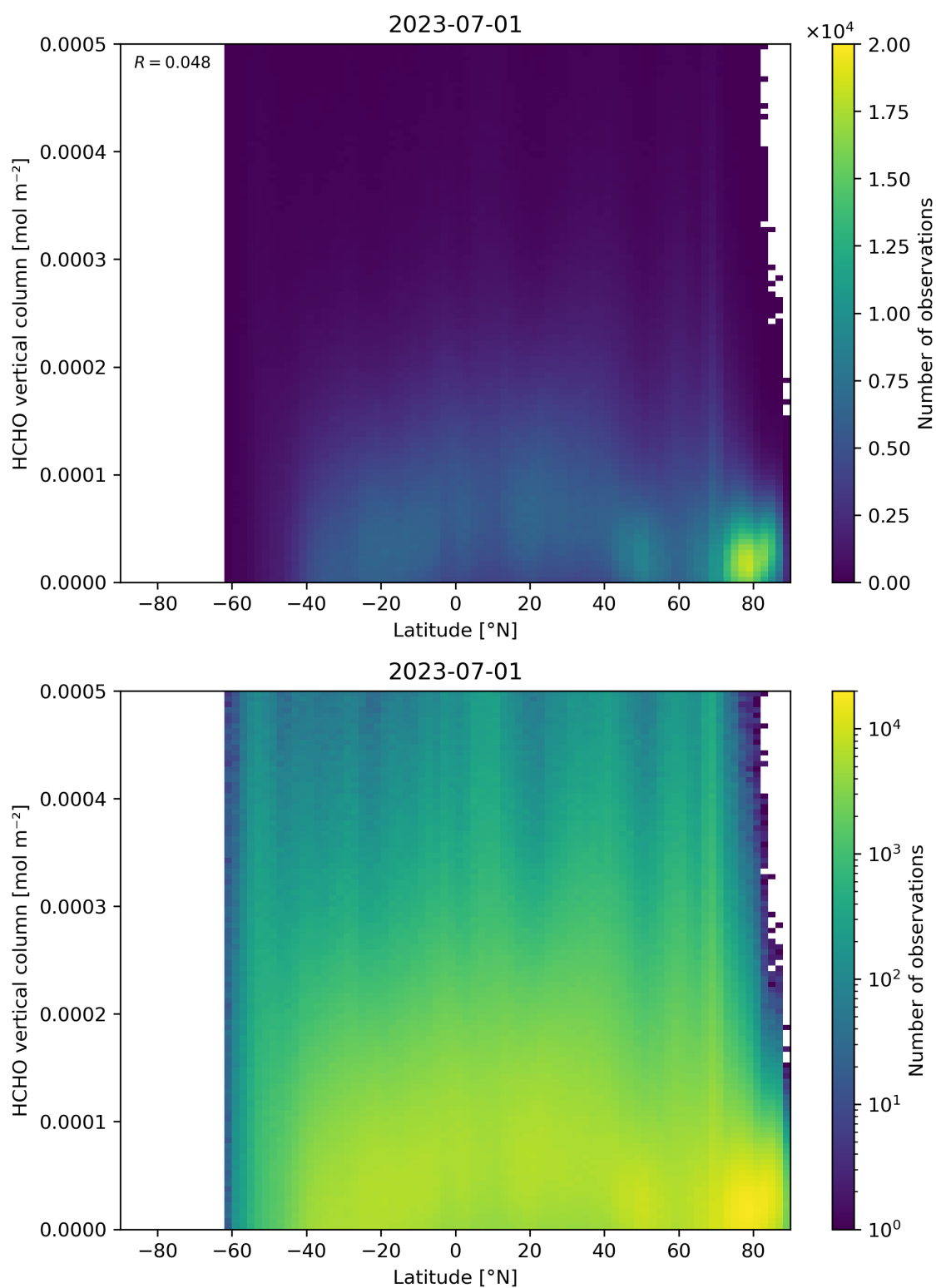
Figure 163: Scatter density plot of “Latitude” against “HCHO vertical column” for 2023-06-30 to 2023-07-02.
