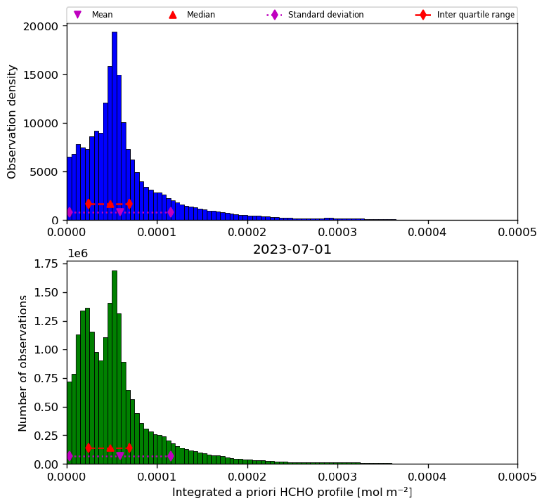
Figure 43: Histogram of “Integrated a priori HCHO profile” for 2023-06-30 to 2023-07-02
