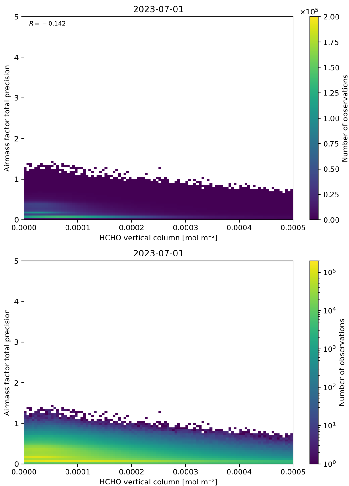
Figure 132: Scatter density plot of “HCHO vertical column” against “Airmass factor total precision” for 2023-06-30 to 2023-07-02.
