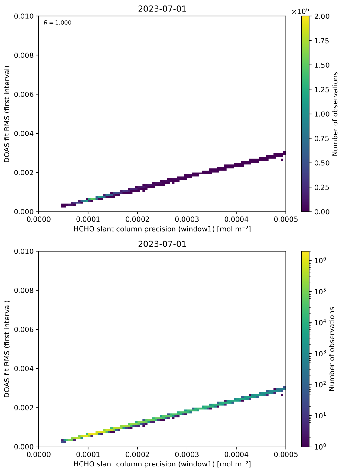
Figure 88: Scatter density plot of “HCHO slant column precision (window1)” against “DOAS fit RMS (first interval)” for 2023-06-30 to 2023-07-02.
