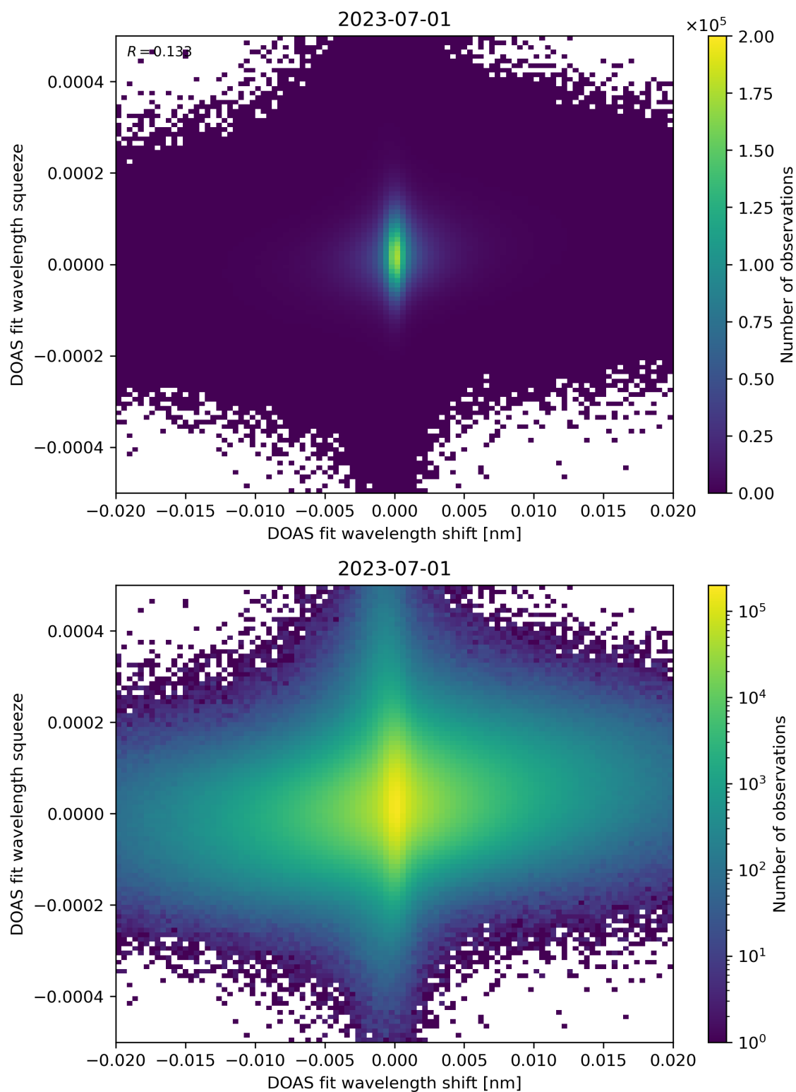
Figure 65: Scatter density plot of “DOAS fit wavelength shift” against “DOAS fit wavelength squeeze” for 2023-06-30 to 2023-07-02.
