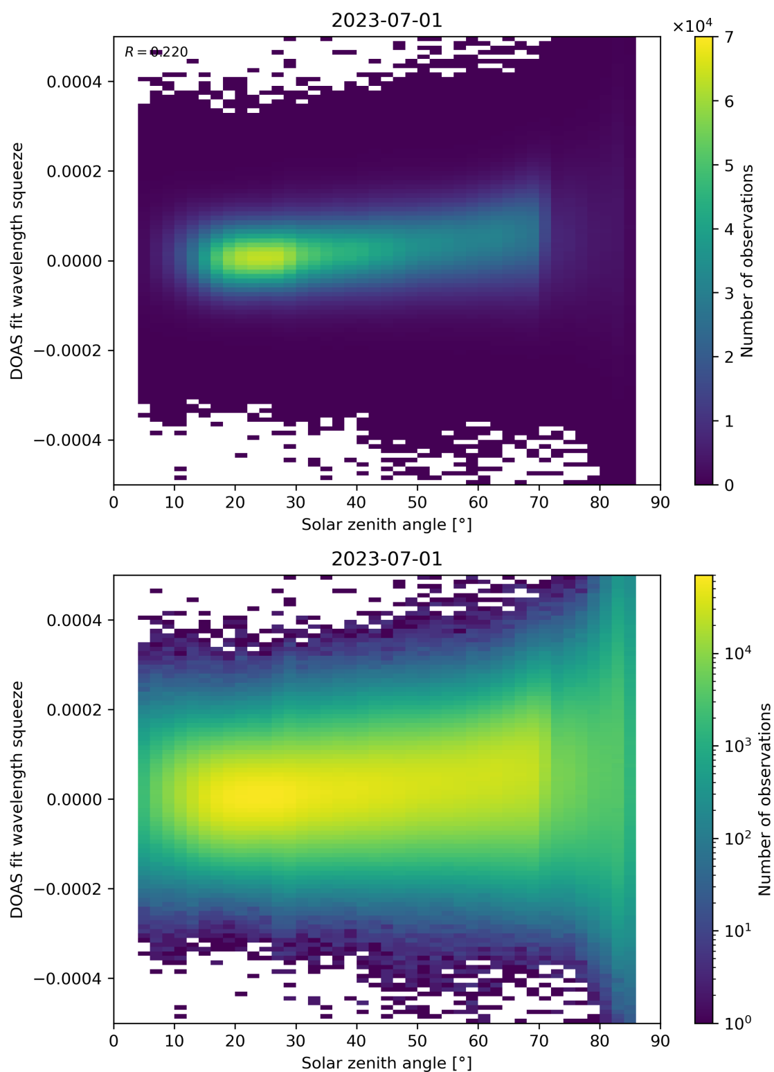
Figure 169: Scatter density plot of “Solar zenith angle” against “DOAS fit wavelength squeeze” for 2023-06-30 to 2023-07-02.
