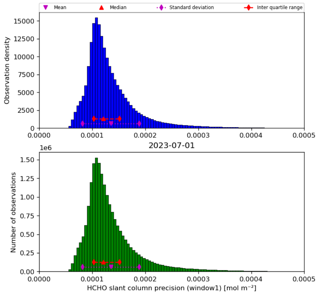
Figure 39: Histogram of “HCHO slant column precision (window1)” for 2023-06-30 to 2023-07-02
