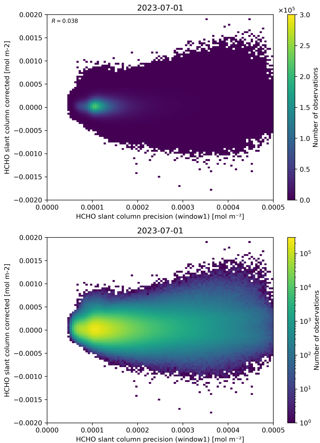
Figure 92: Scatter density plot of “HCHO slant column precision (window1)” against “HCHO slant column corrected” for 2023-06-30 to 2023-07-02.
