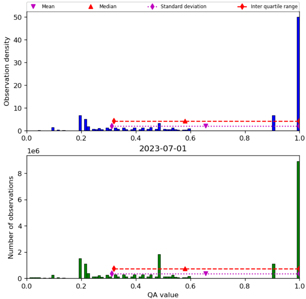
Figure 34: Histogram of “QA value” for 2023-06-30 to 2023-07-02
