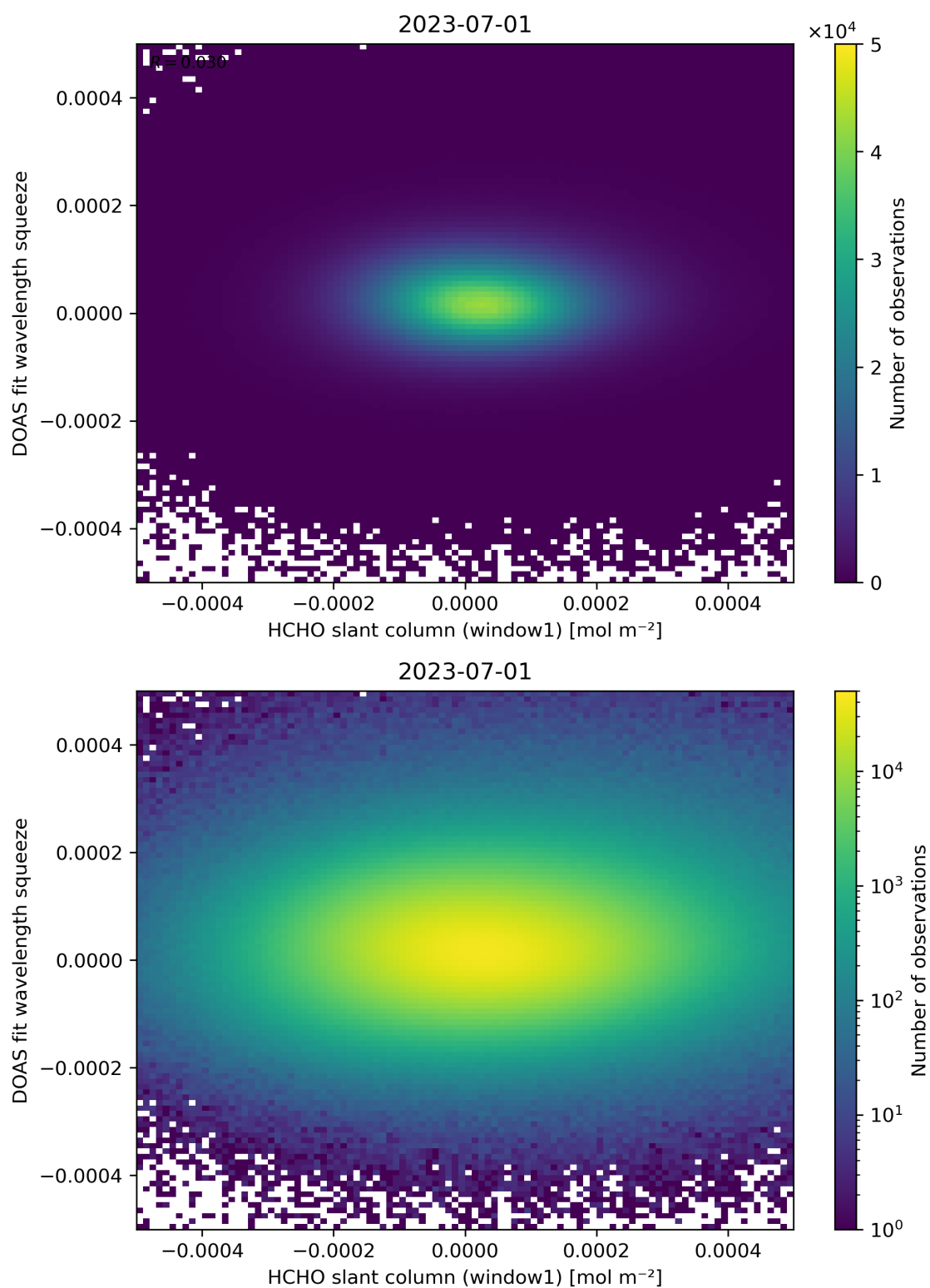
Figure 80: Scatter density plot of “HCHO slant column (window1)” against “DOAS fit wavelength squeeze” for 2023-06-30 to 2023-07-02.
