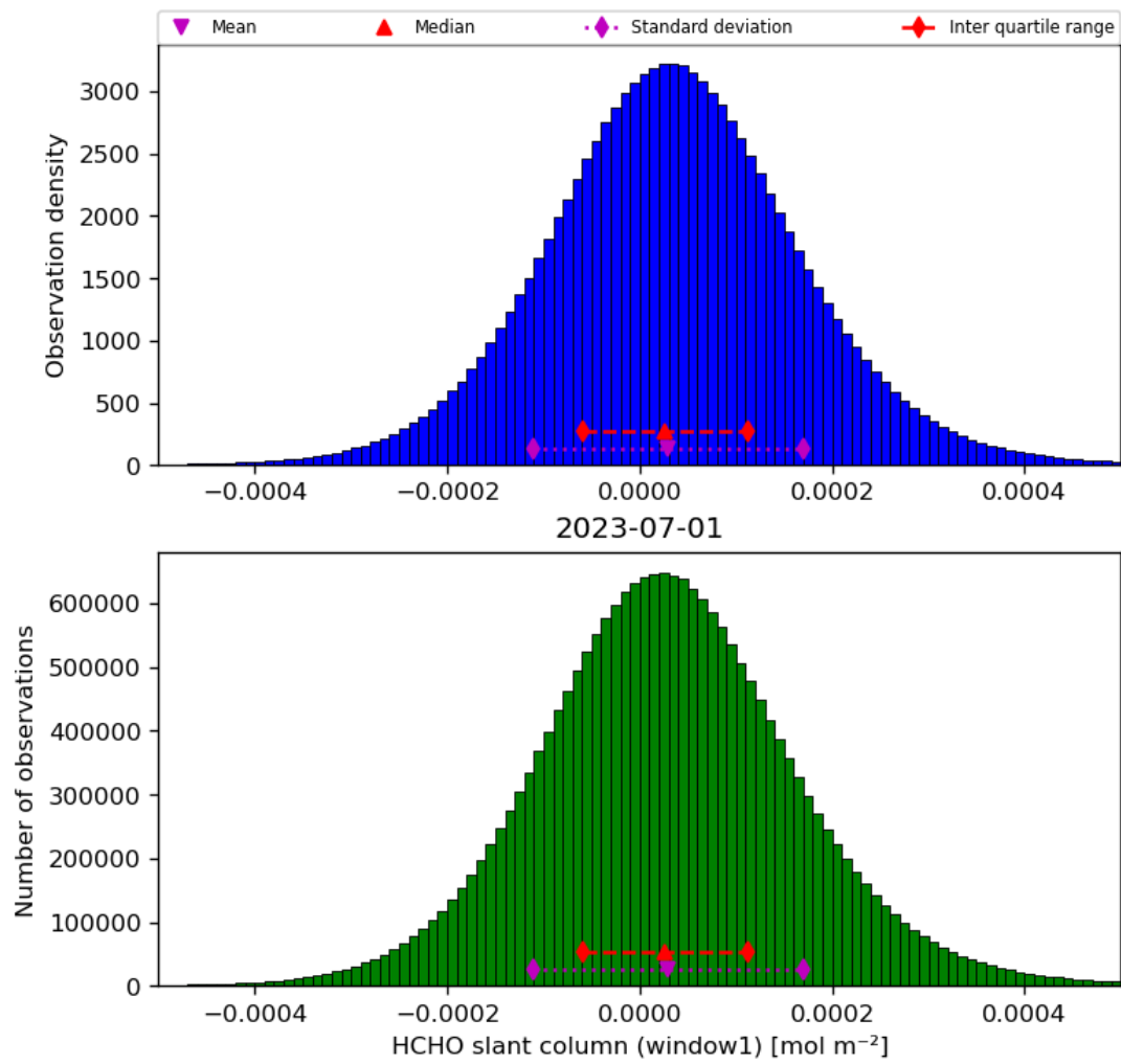
Figure 38: Histogram of “HCHO slant column (window1)” for 2023-06-30 to 2023-07-02
