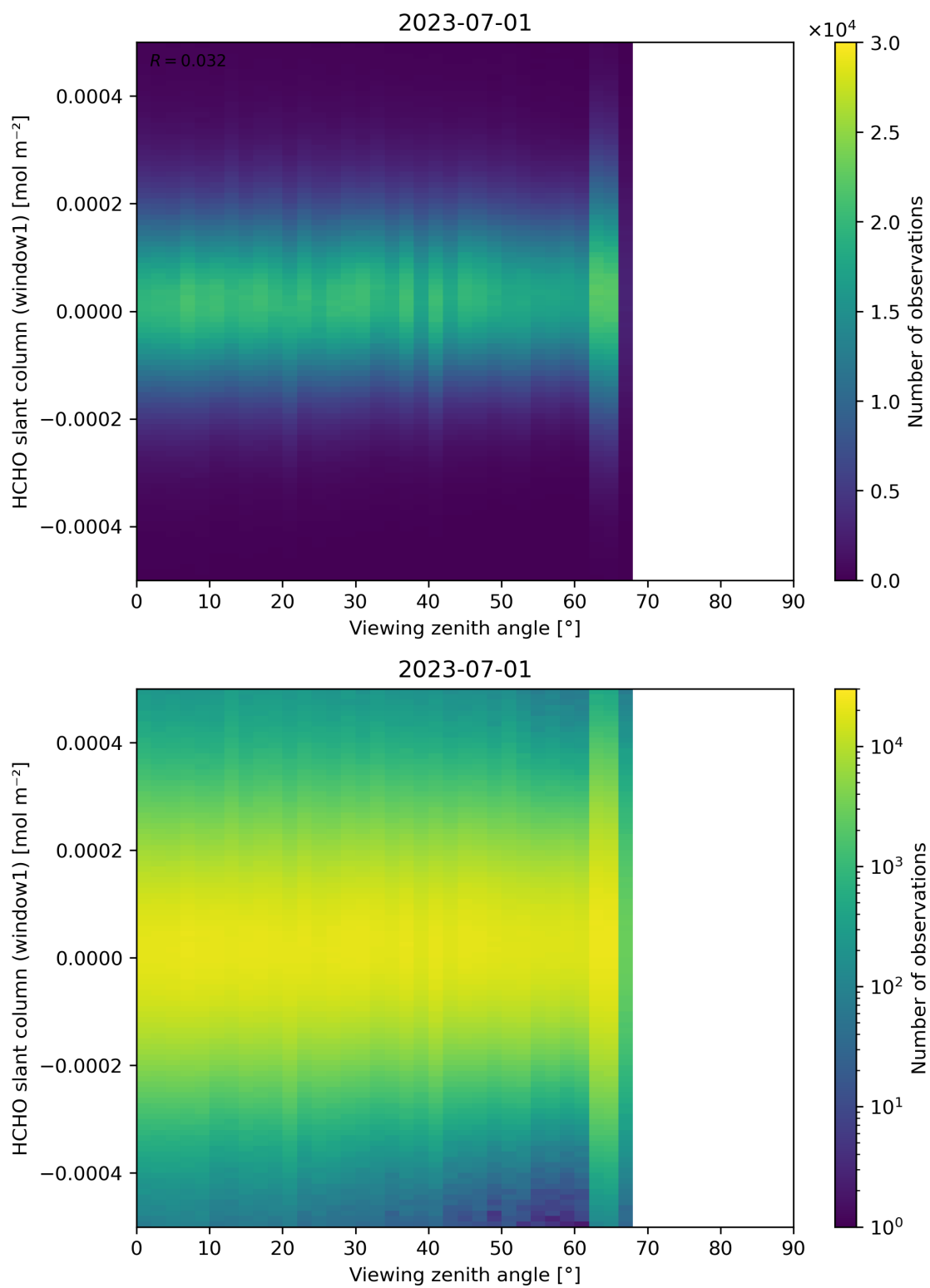
Figure 188: Scatter density plot of “Viewing zenith angle” against “HCHO slant column (window1)” for 2023-06-30 to 2023-07-02.
