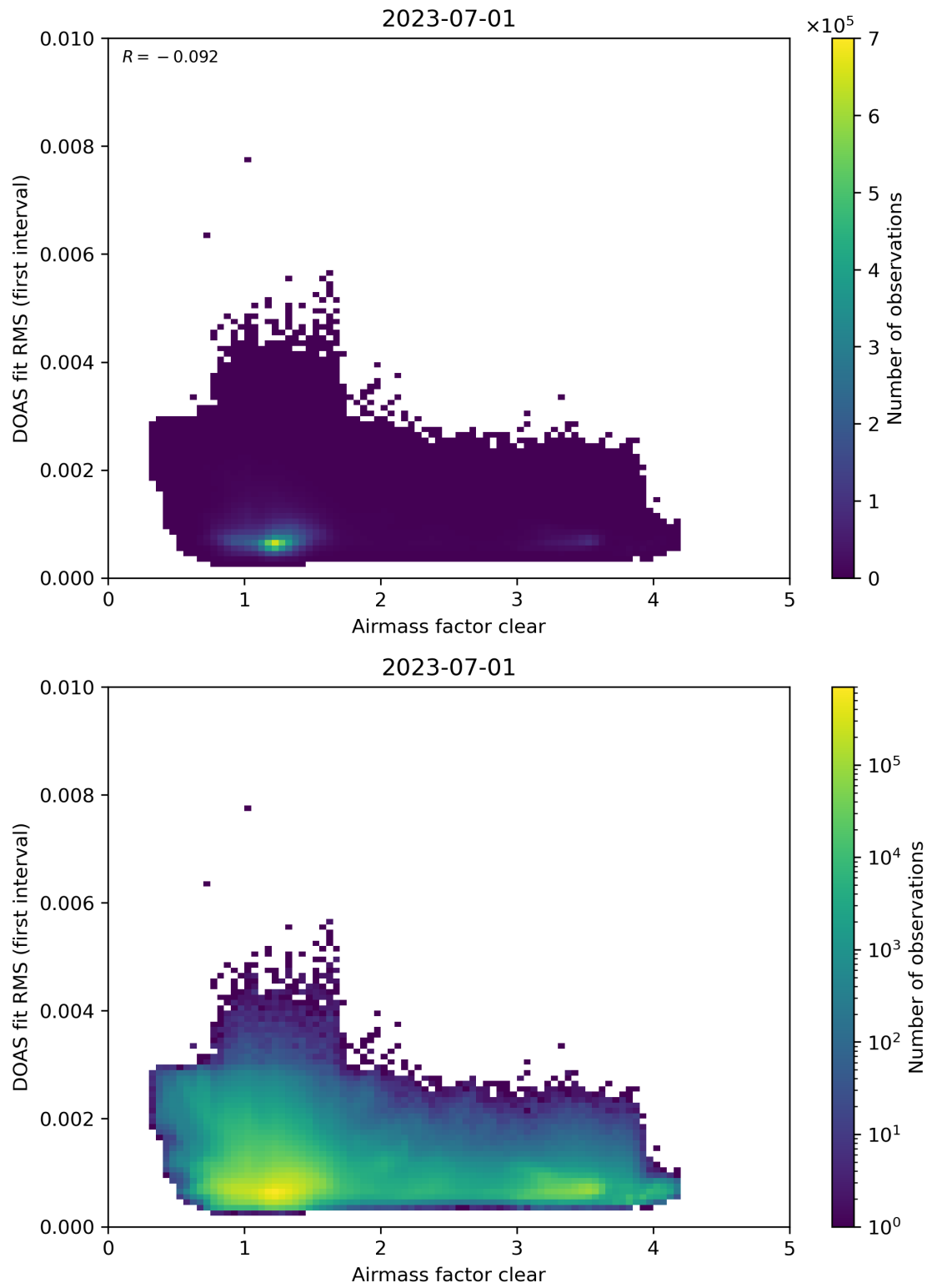
Figure 71: Scatter density plot of “Airmass factor clear” against “DOAS fit RMS (first interval)” for 2023-06-30 to 2023-07-02.
