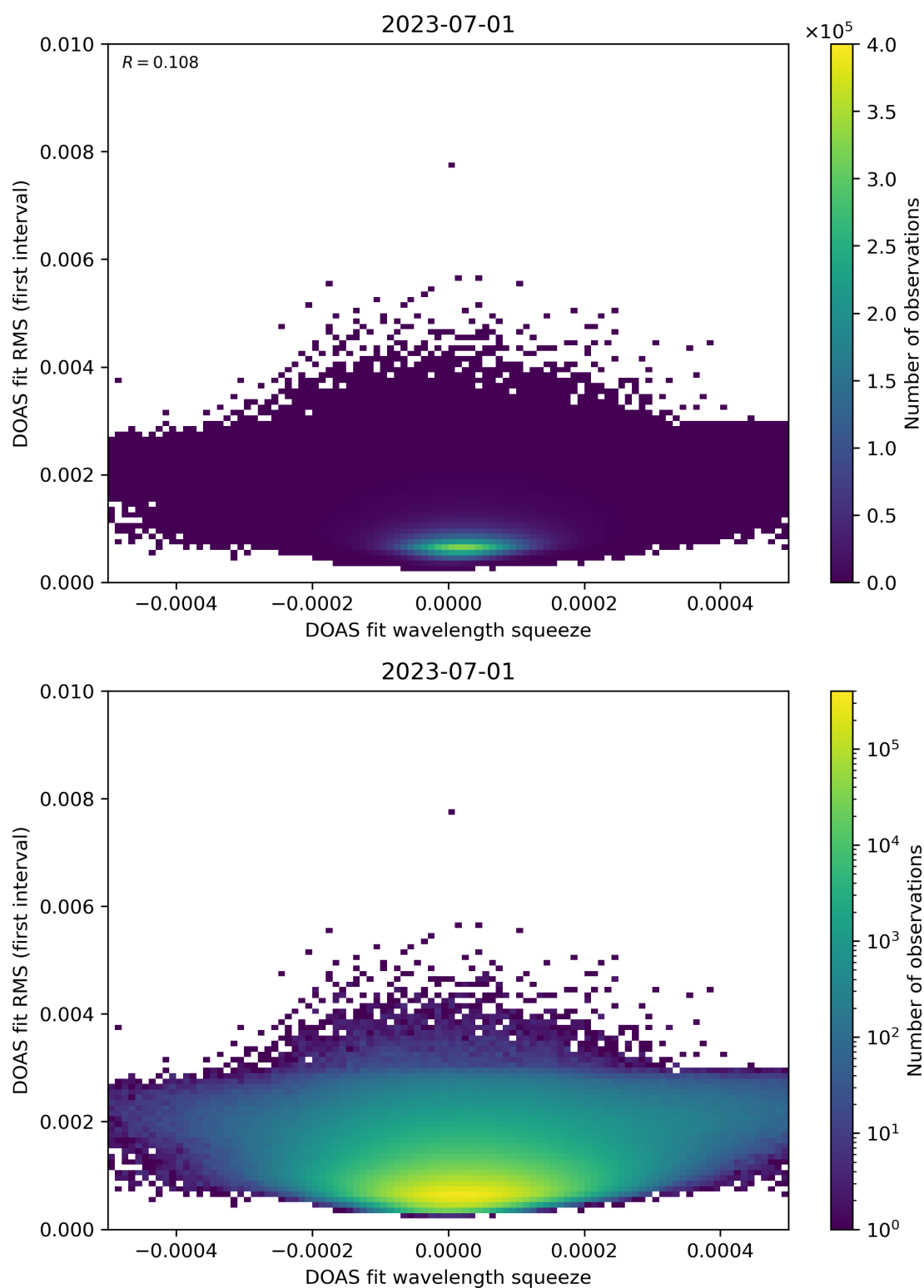
Figure 68: Scatter density plot of “DOAS fit wavelength squeeze” against “DOAS fit RMS (first interval)” for 2023-06-30 to 2023-07-02.
