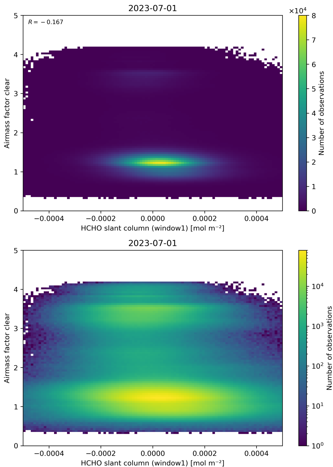
Figure 81: Scatter density plot of “HCHO slant column (window1)” against “Airmass factor clear” for 2023-06-30 to 2023-07-02.
