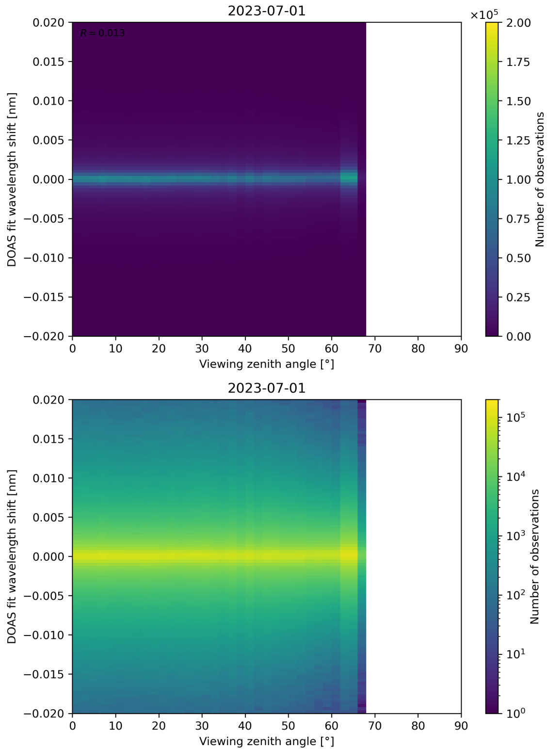
Figure 183: Scatter density plot of “Viewing zenith angle” against “DOAS fit wavelength shift” for 2023-06-30 to 2023-07-02.
