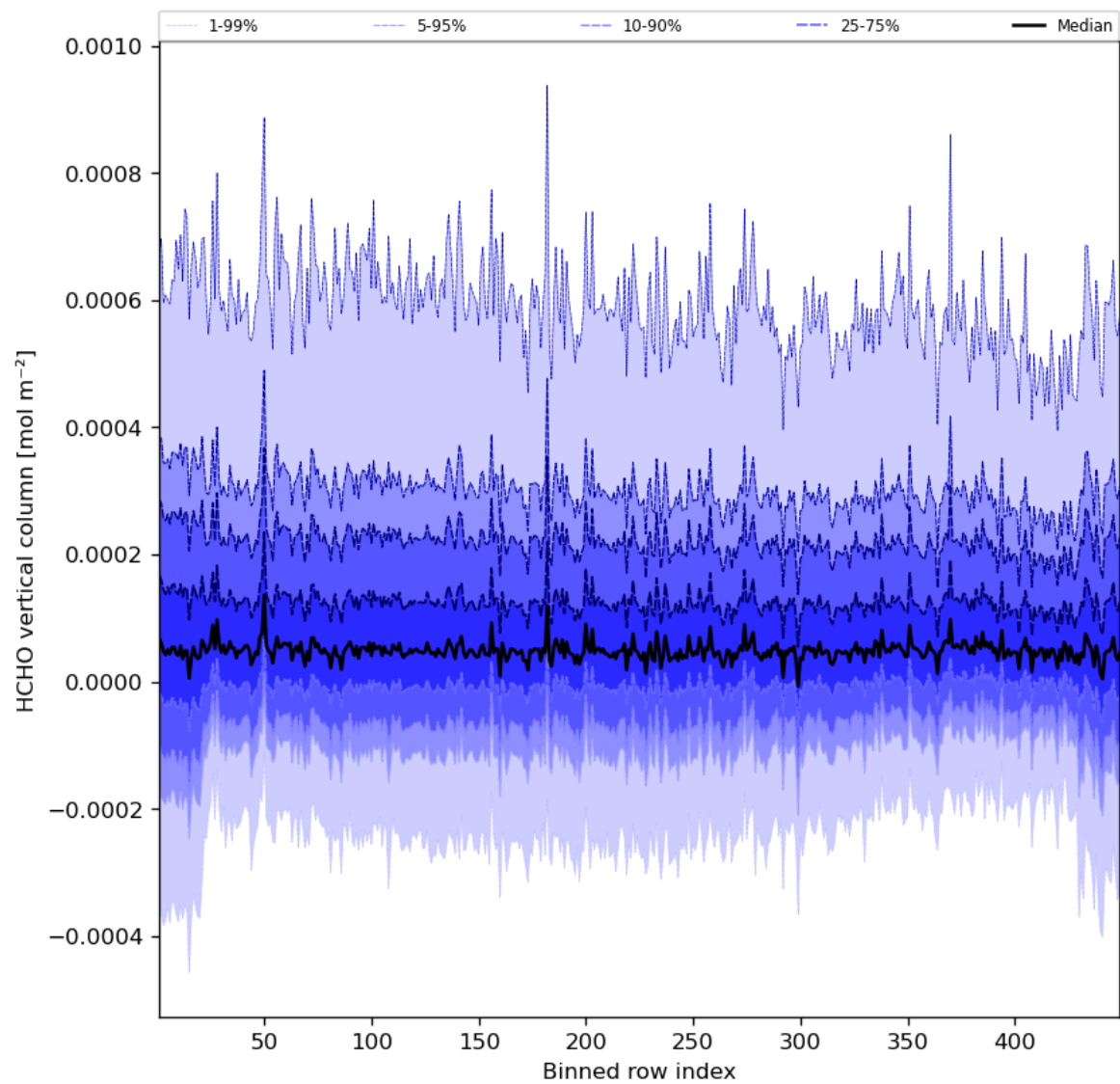
Figure 49: Along track statistics of “HCHO vertical column” for 2023-06-30 to 2023-07-02
