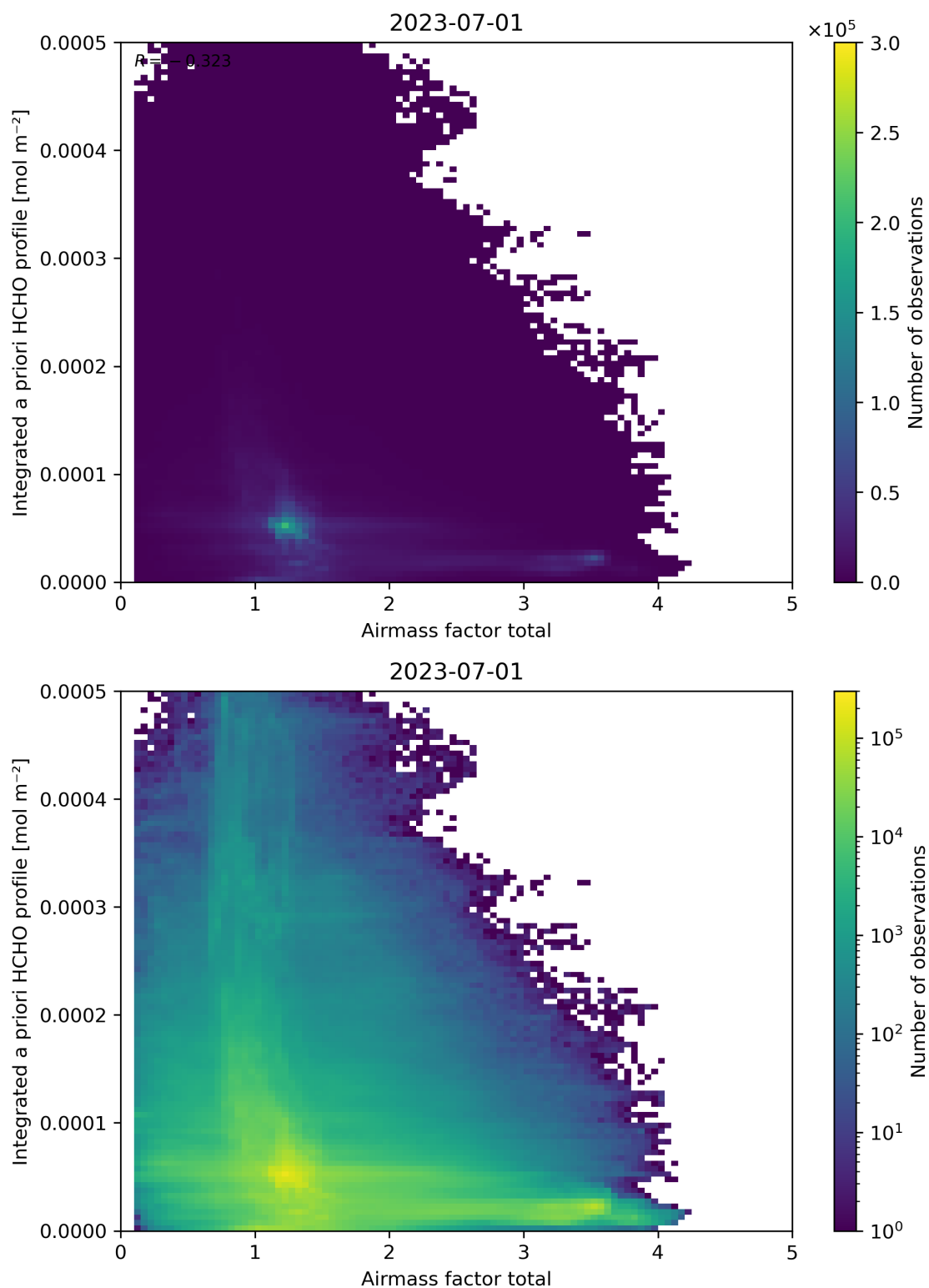
Figure 104: Scatter density plot of “Air mass factor total” against “Integrated a priori HCHO profile” for 2023-06-30 to 2023-07-02.
