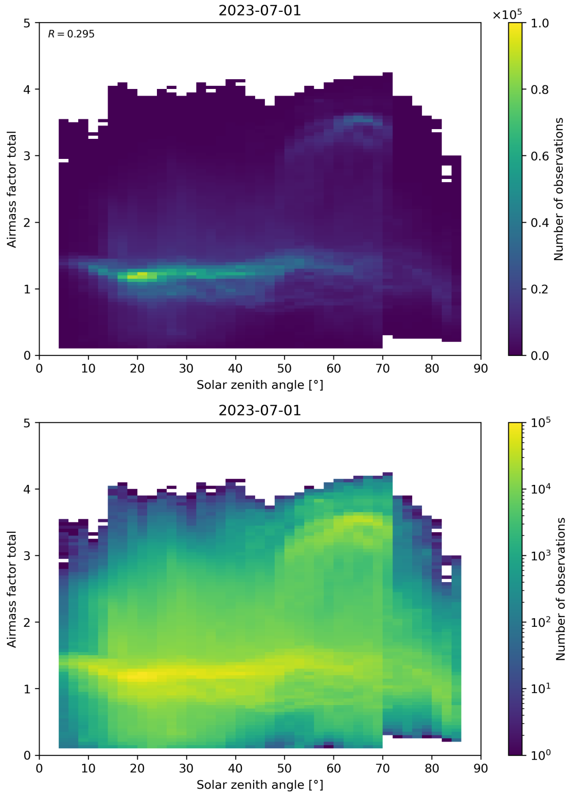
Figure 175: Scatter density plot of “Solar zenith angle” against “Airmass factor total” for 2023-06-30 to 2023-07-02.
