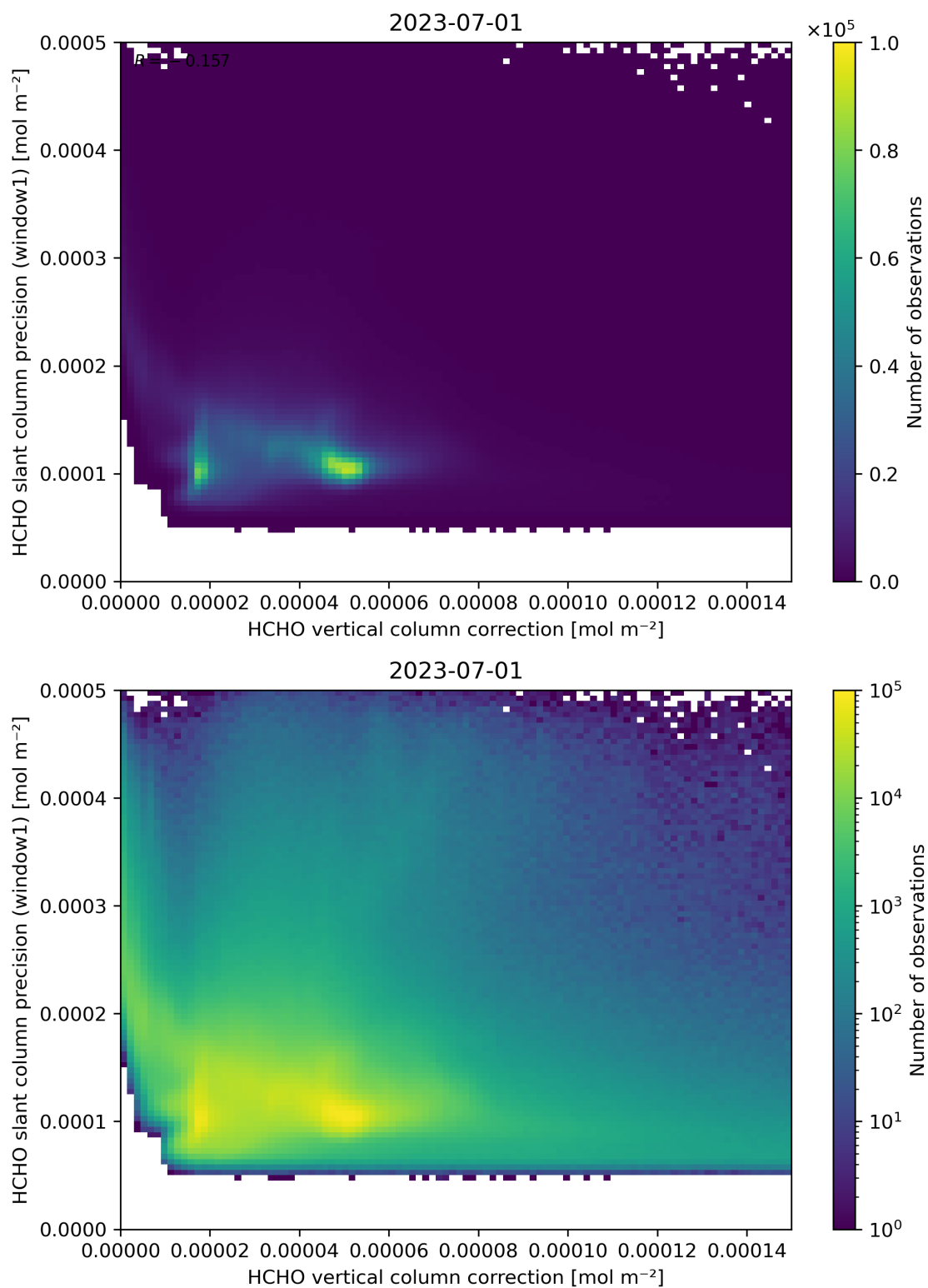
Figure 119: Scatter density plot of “HCHO vertical column correction” against “HCHO slant column precision (window1)” for 2023-06-30 to 2023-07-02.
