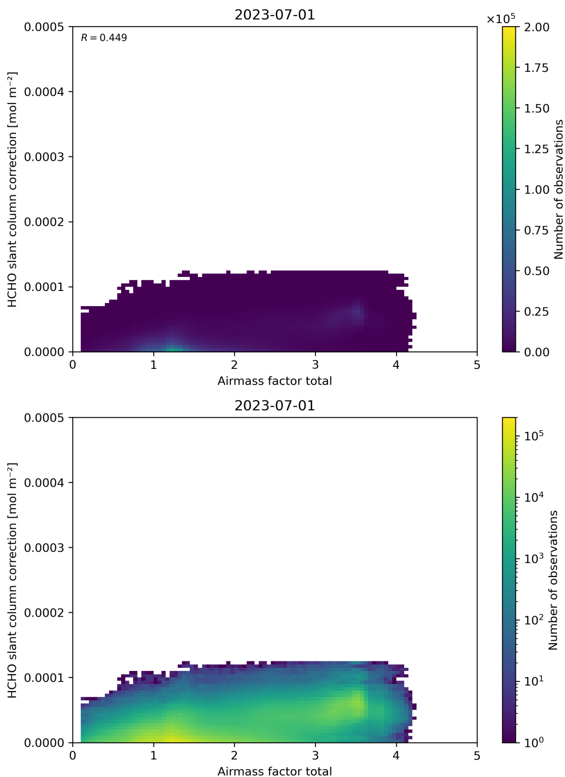
Figure 102: Scatter density plot of “Airmass factor total” against “HCHO slant column correction” for 2023-06-30 to 2023-07-02.
