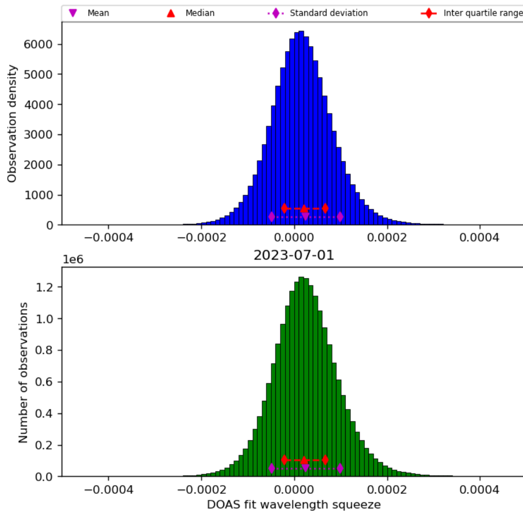
Figure 45: Histogram of “DOAS fit wavelength squeeze” for 2023-06-30 to 2023-07-02
