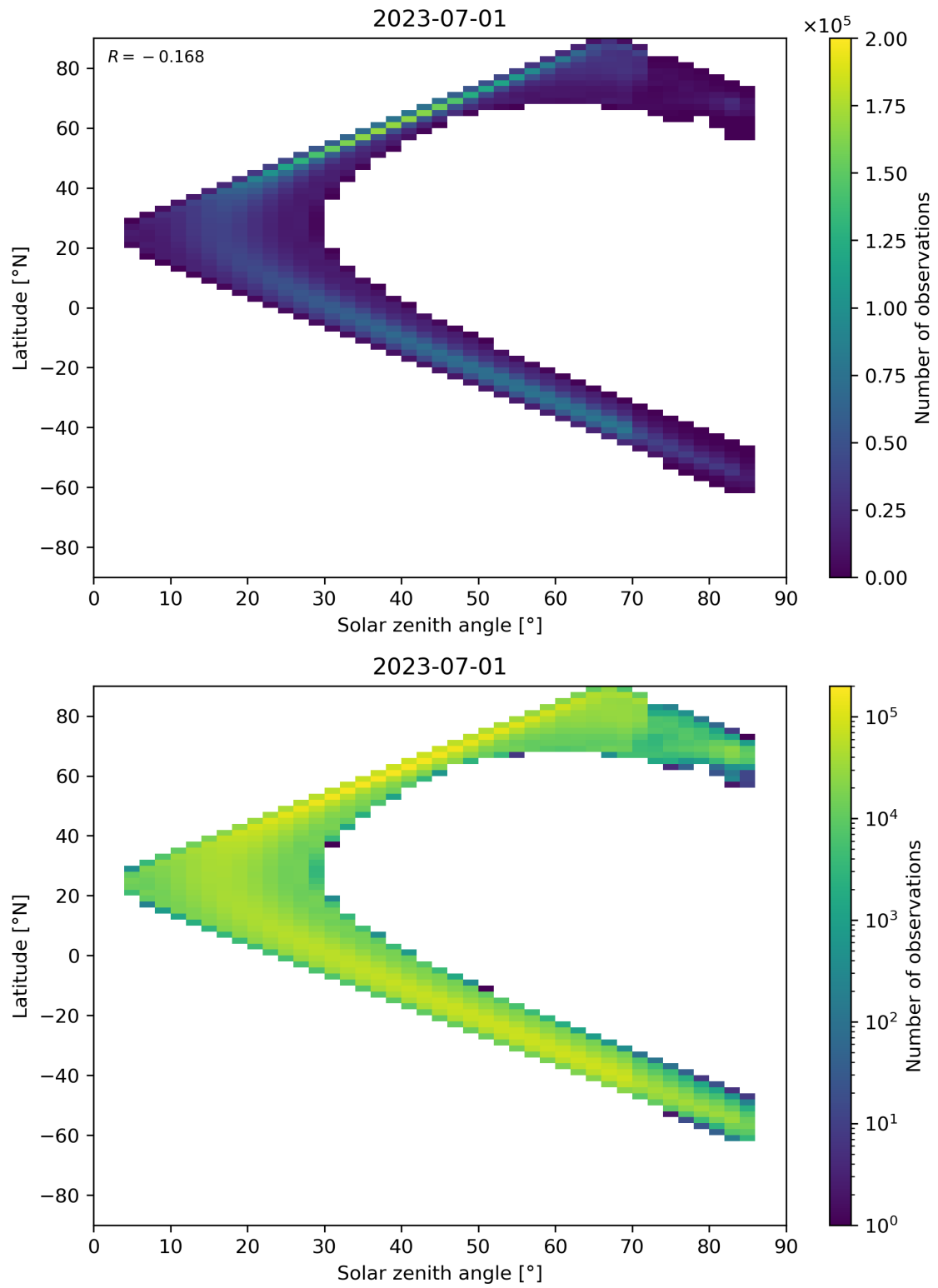
Figure 181: Scatter density plot of “Solar zenith angle” against “Latitude” for 2023-06-30 to 2023-07-02.
