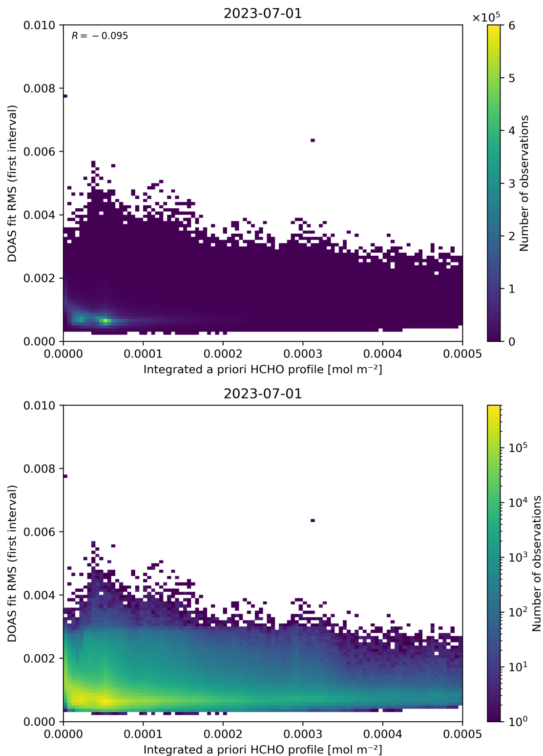
Figure 148: Scatter density plot of “Integrated a priori HCHO profile” against “DOAS fit RMS (first interval)” for 2023-06-30 to 2023-07-02.
