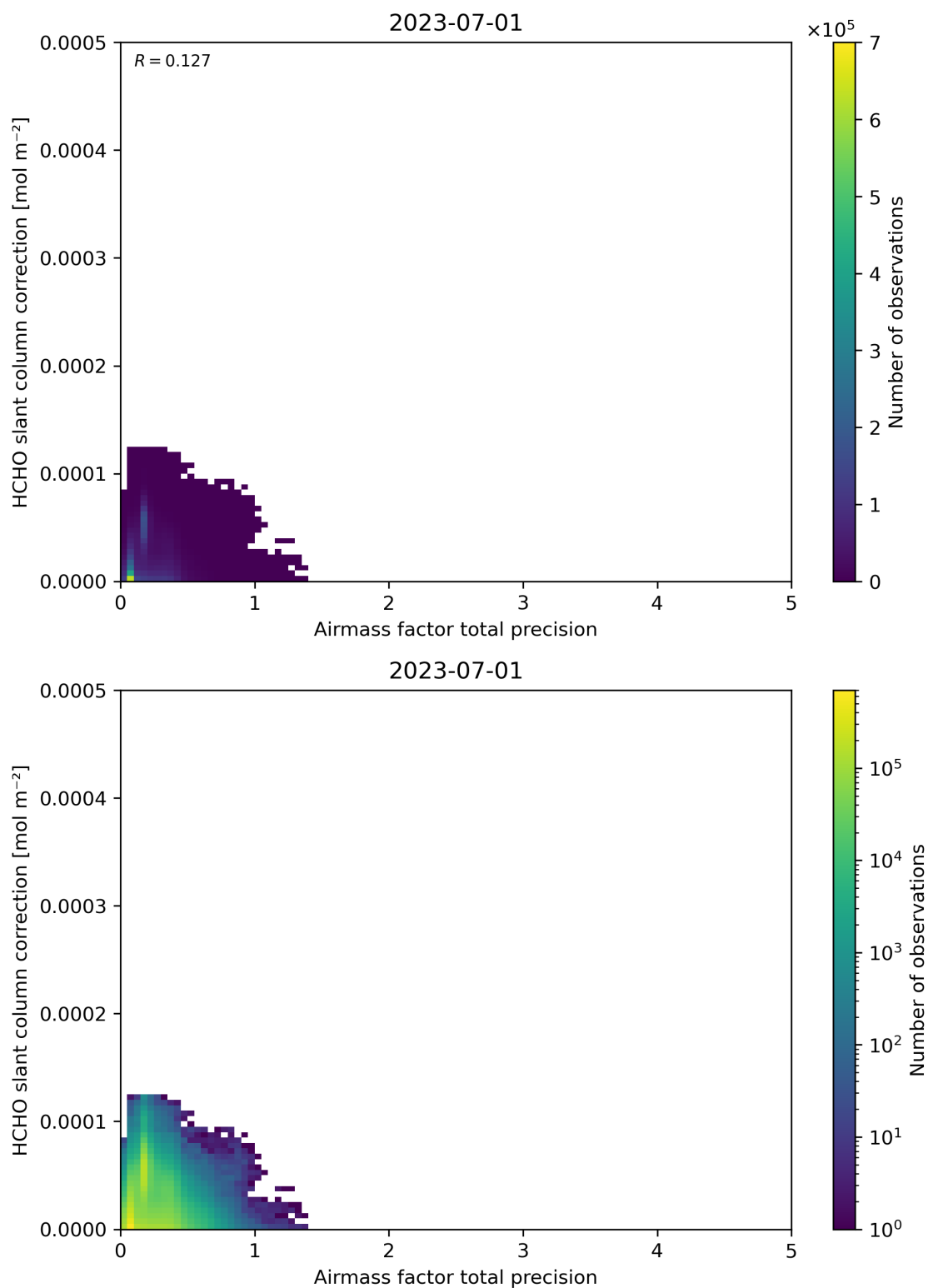
Figure 110: Scatter density plot of “Airmass factor total precision” against “HCHO slant column correction” for 2023-06-30 to 2023-07-02.
