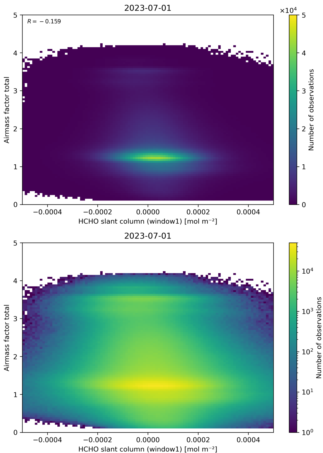
Figure 85: Scatter density plot of “HCHO slant column (window1)” against “Airmass factor total” for 2023-06-30 to 2023-07-02.
