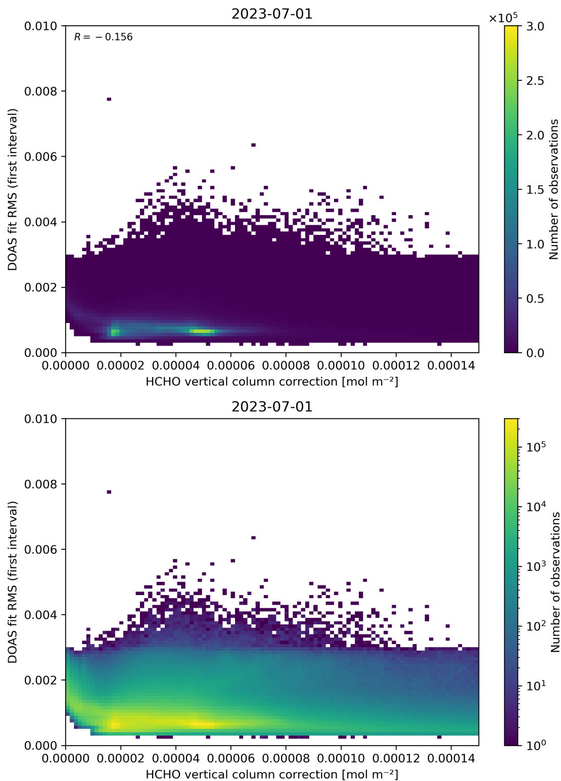
Figure 112: Scatter density plot of “HCHO vertical column correction” against “DOAS fit RMS (first interval)” for 2023-06-30 to 2023-07-02.
