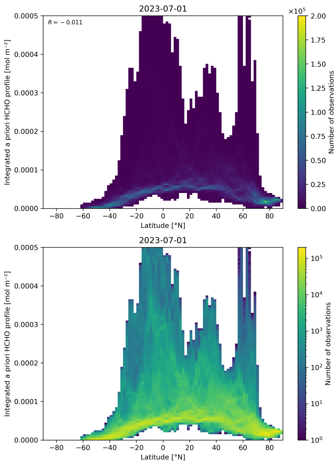
Figure 166: Scatter density plot of “Latitude” against “Integrated a priori HCHO profile” for 2023-06-30 to 2023-07-02.
