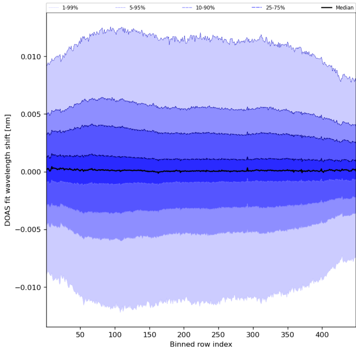
Figure 58: Along track statistics of “DOAS fit wavelength shift” for 2023-06-30 to 2023-07-02
