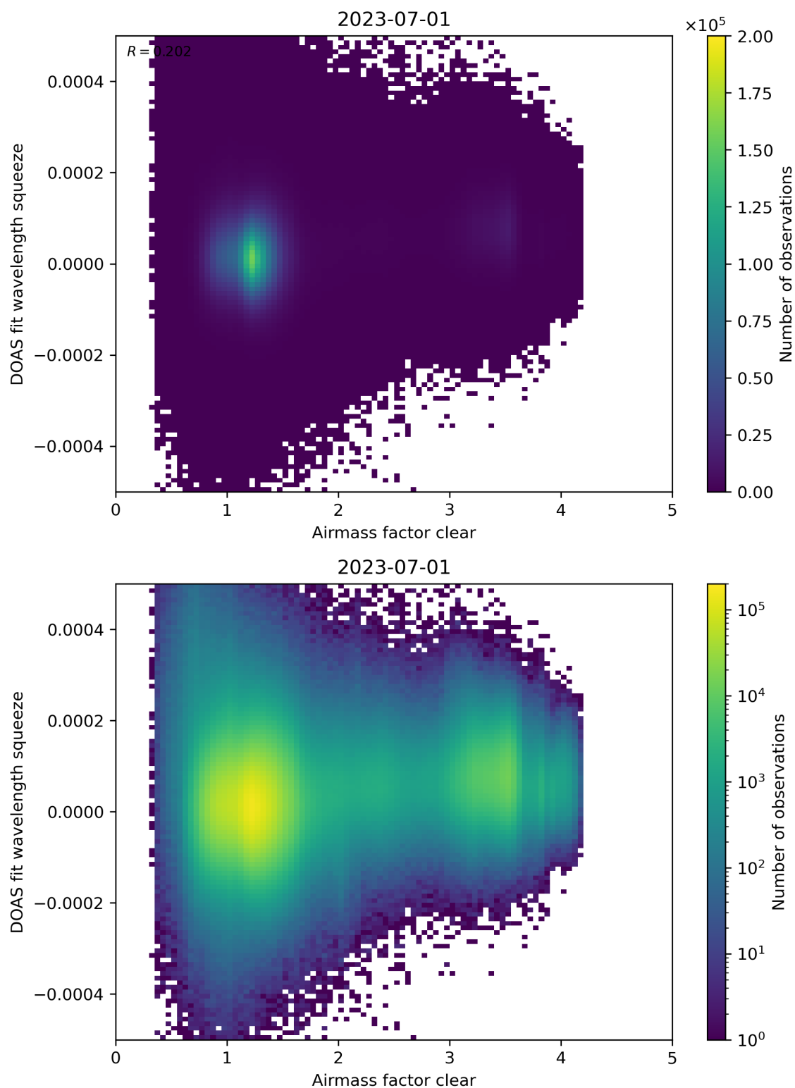
Figure 73: Scatter density plot of “Airmass factor clear” against “DOAS fit wavelength squeeze” for 2023-06-30 to 2023-07-02.
