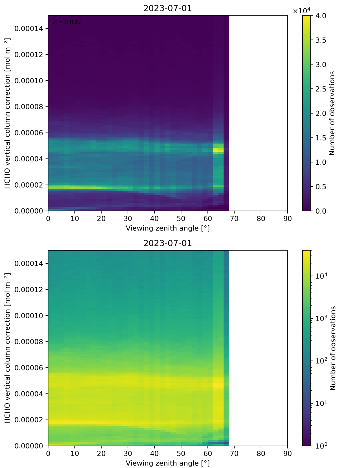
Figure 193: Scatter density plot of “Viewing zenith angle” against “HCHO vertical column correction” for 2023-06-30 to 2023-07-02.
