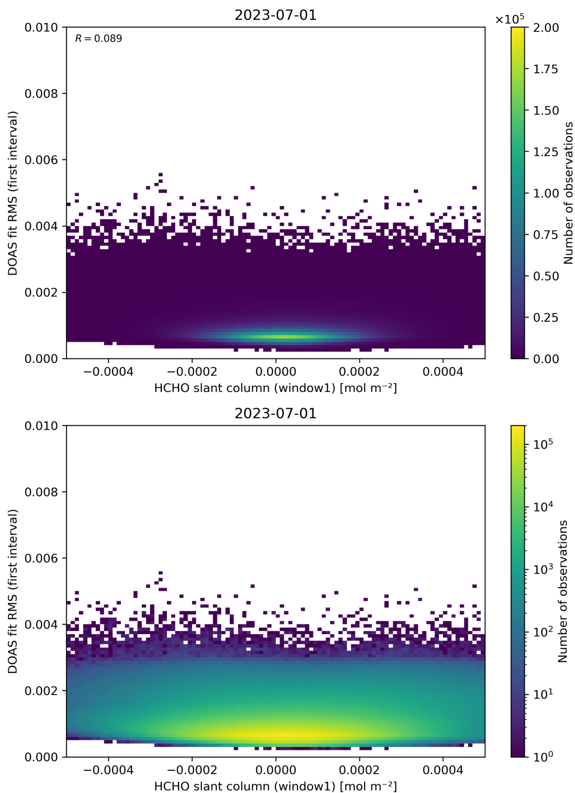
Figure 78: Scatter density plot of “HCHO slant column (window1)” against “DOAS fit RMS (first interval)” for 2023-06-30 to 2023-07-02.
