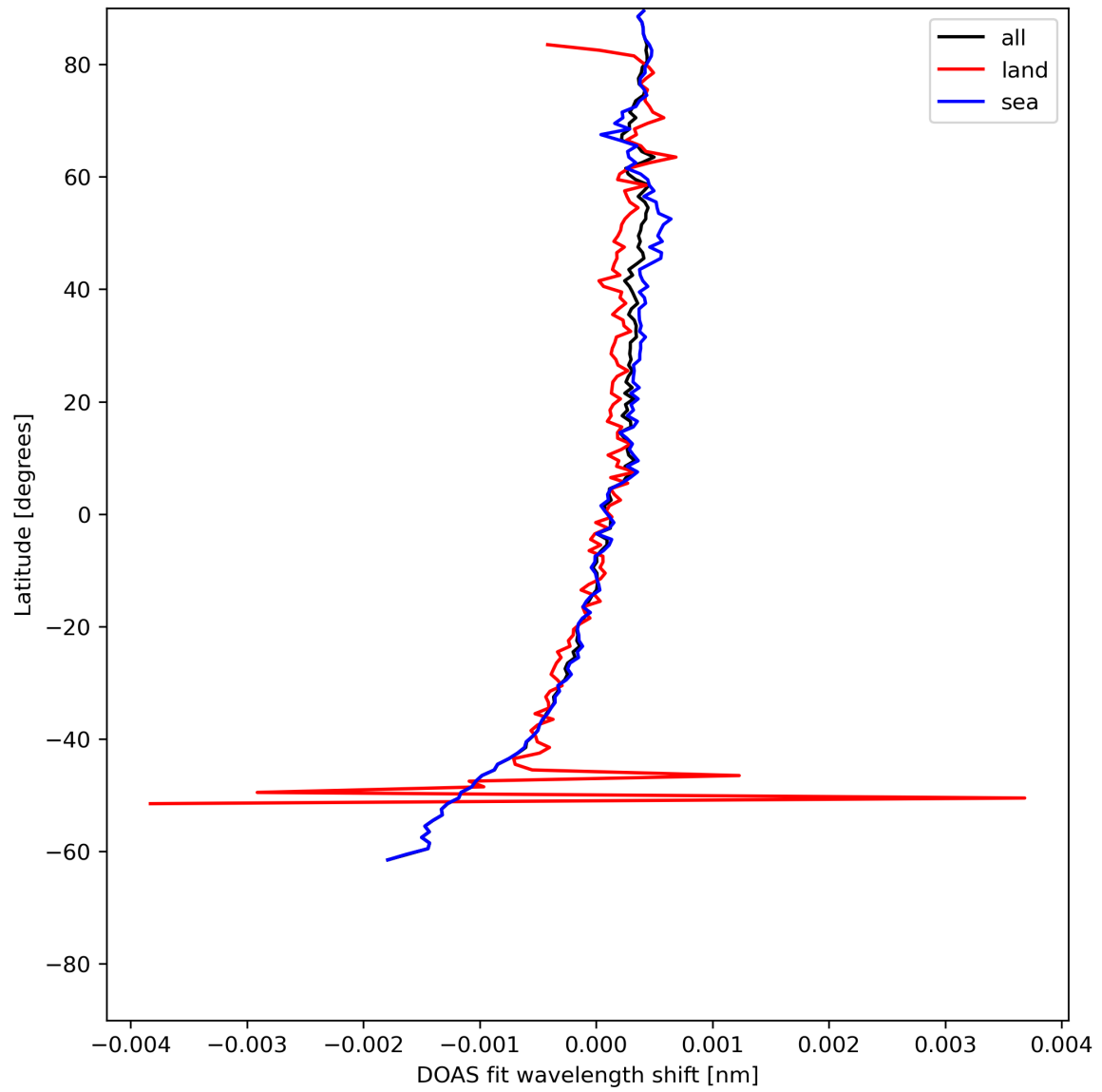
Figure 30: Zonal average of “DOAS fit wavelength shift” for 2023-06-30 to 2023-07-02.
