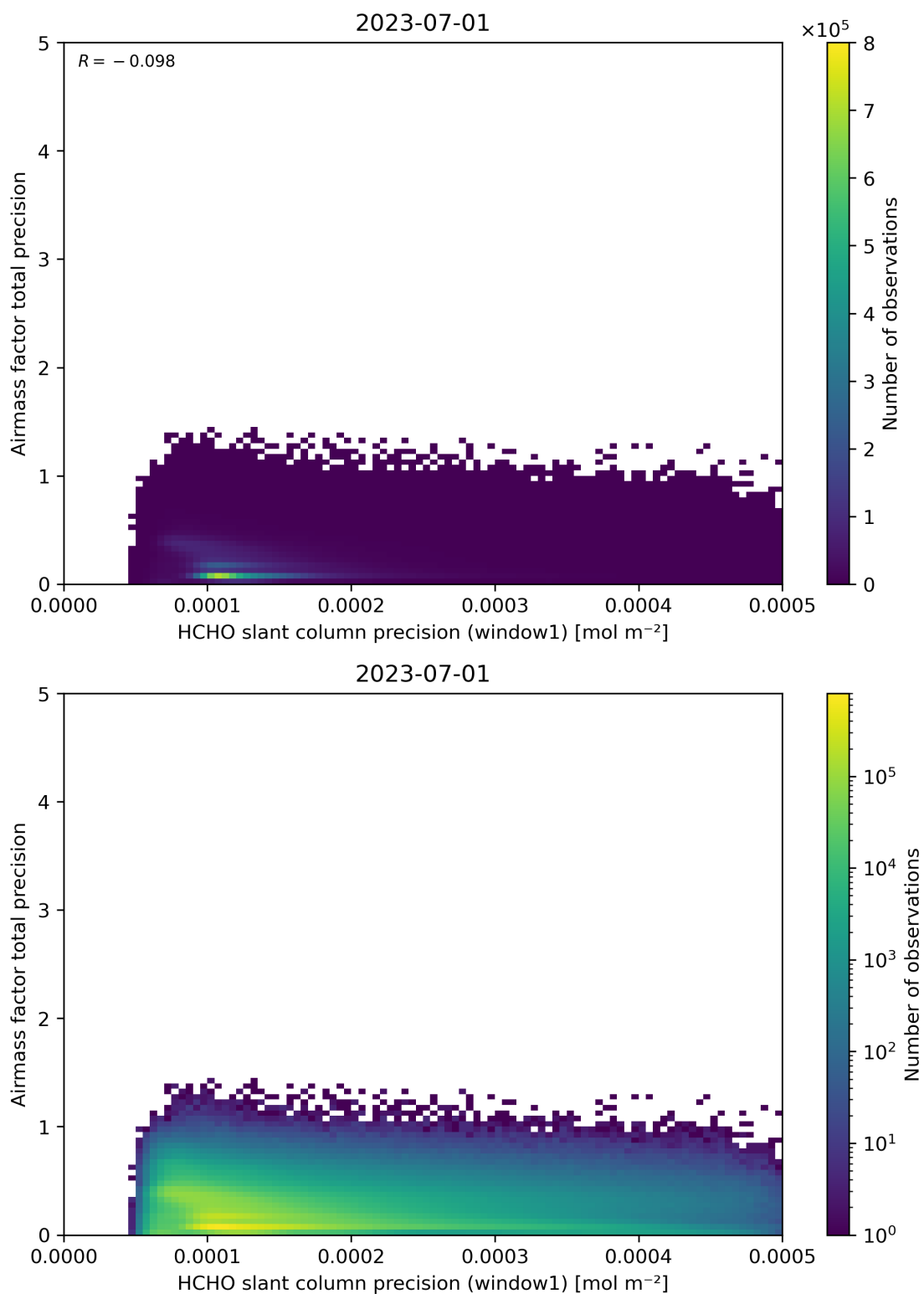
Figure 95: Scatter density plot of “HCHO slant column precision (window1)” against “Airmass factor total precision” for 2023-06-30 to 2023-07-02.
