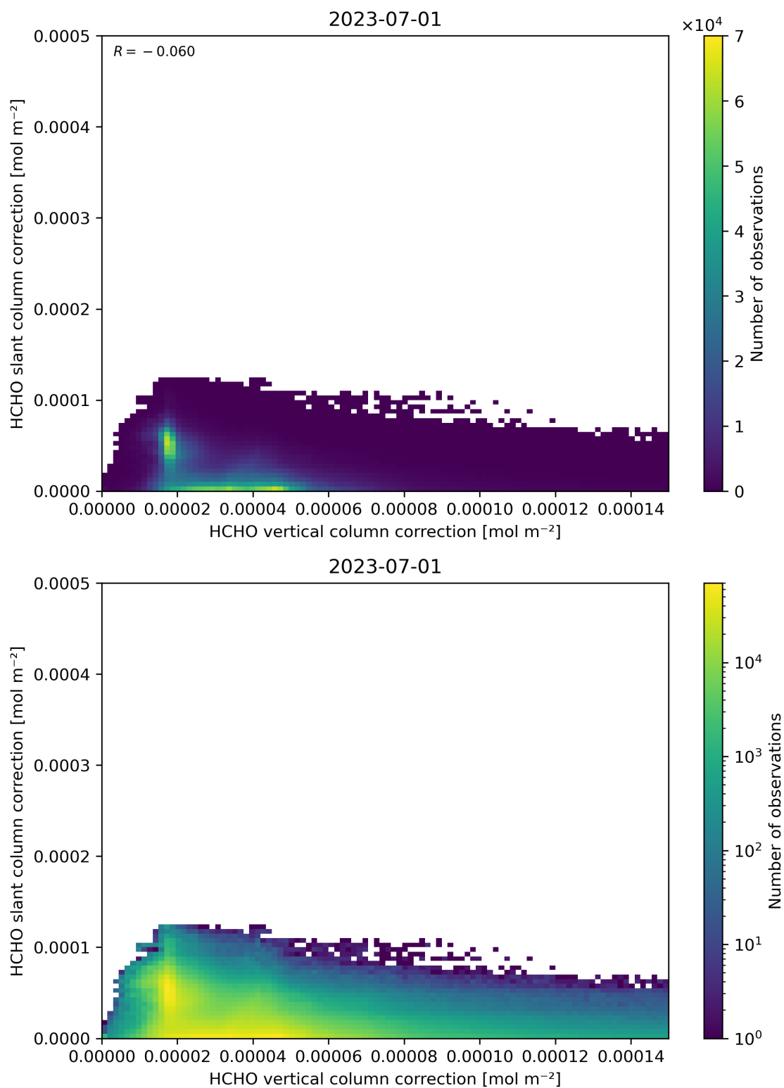
Figure 117: Scatter density plot of “HCHO vertical column correction” against “HCHO slant column correction” for 2023-06-30 to 2023-07-02.
