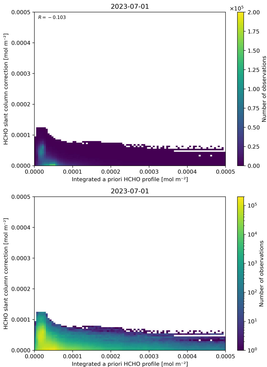
Figure 152: Scatter density plot of “Integrated a priori HCHO profile” against “HCHO slant column correction” for 2023-06-30 to 2023-07-02.
