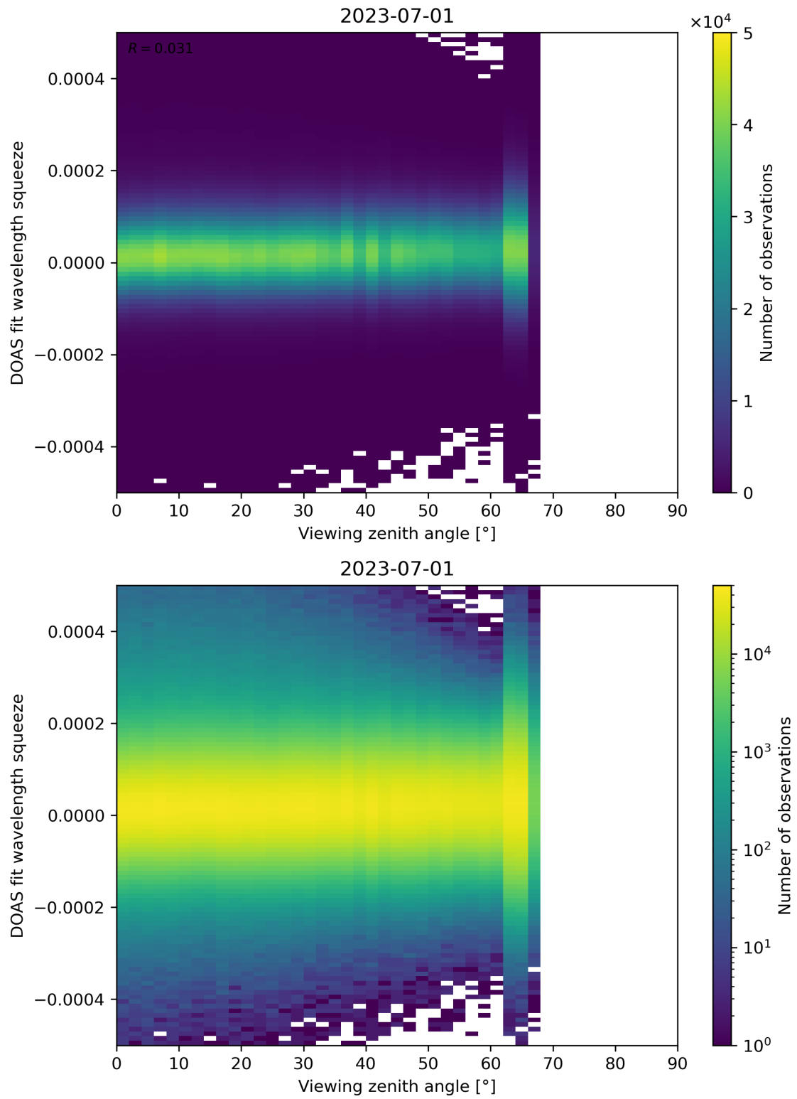
Figure 184: Scatter density plot of “Viewing zenith angle” against “DOAS fit wavelength squeeze” for 2023-06-30 to 2023-07-02.
