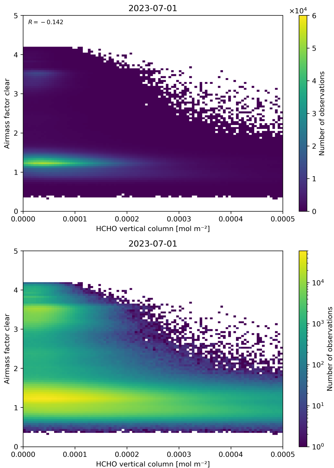
Figure 126: Scatter density plot of “HCHO vertical column” against “Airmass factor clear” for 2023-06-30 to 2023-07-02.
