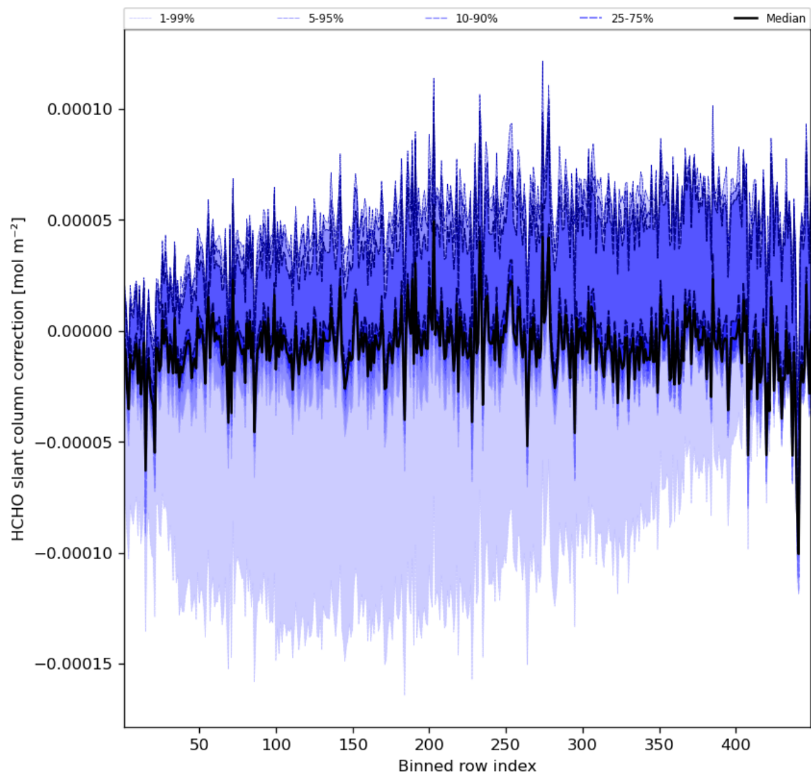
Figure 61: Along track statistics of “HCHO slant column correction” for 2023-06-30 to 2023-07-02
