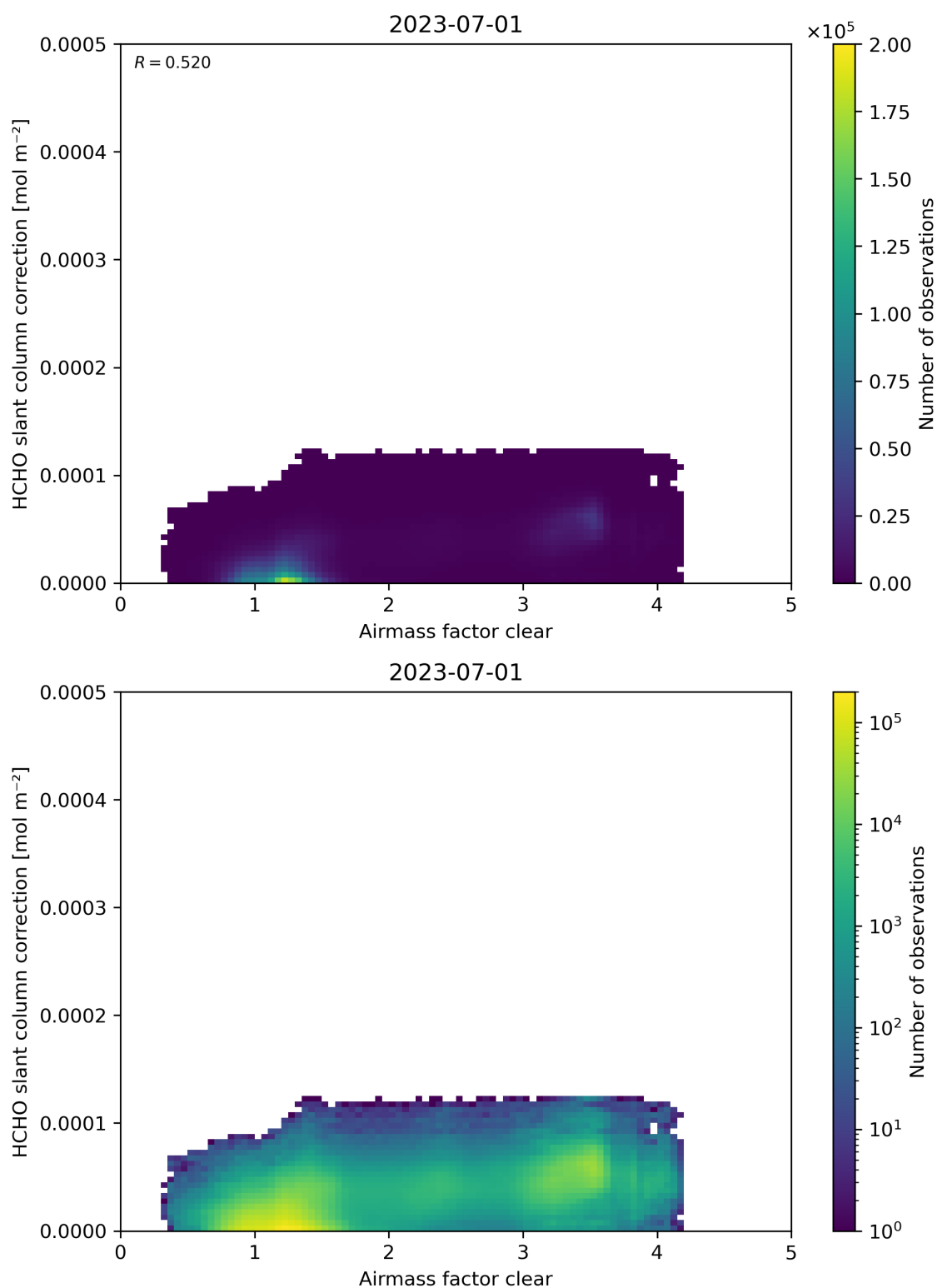
Figure 75: Scatter density plot of “Airmass factor clear” against “HCHO slant column correction” for 2023-06-30 to 2023-07-02.
