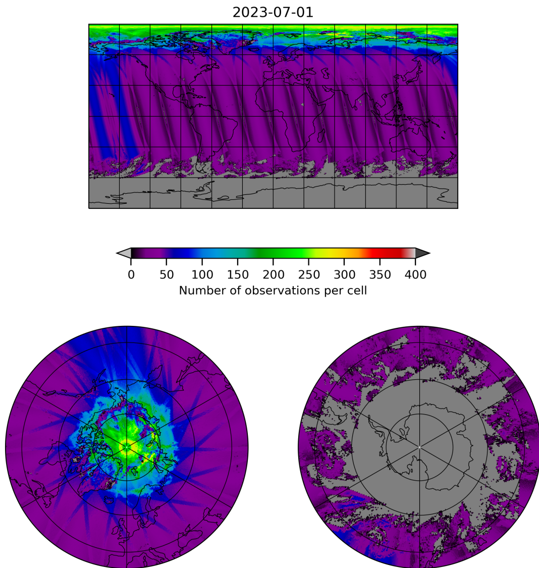
Figure 19: Map of the number of observations for 2023-06-30 to 2023-07-02
