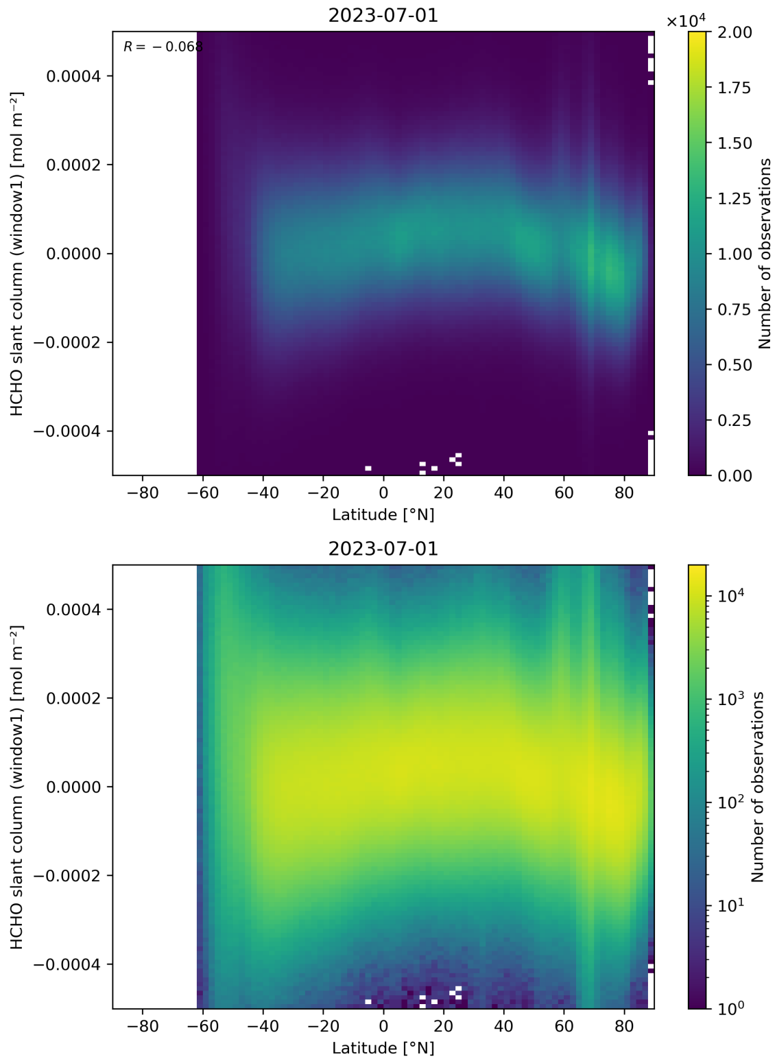
Figure 159: Scatter density plot of “Latitude” against “HCHO slant column (window1)” for 2023-06-30 to 2023-07-02.
