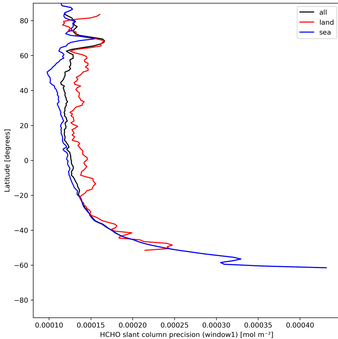
Figure 25: Zonal average of “HCHO slant column precision (window1)” for 2023-06-30 to 2023-07-02.
