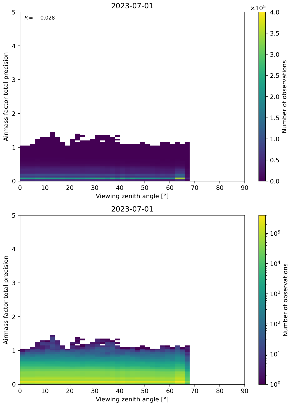
Figure 191: Scatter density plot of “Viewing zenith angle” against “Airmass factor total precision” for 2023-06-30 to 2023-07-02.
