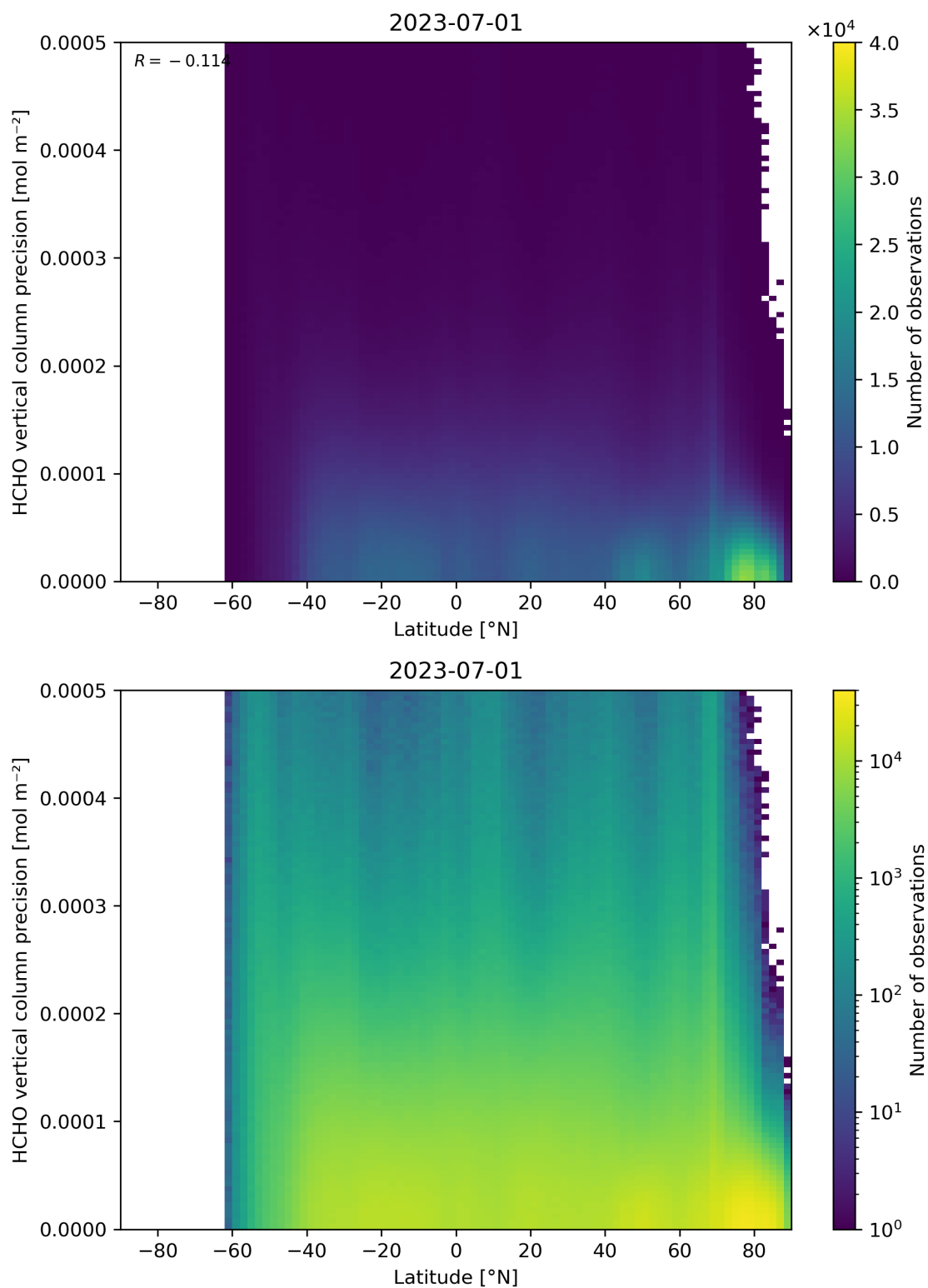
Figure 165: Scatter density plot of “Latitude” against “HCHO vertical column precision” for 2023-06-30 to 2023-07-02.
