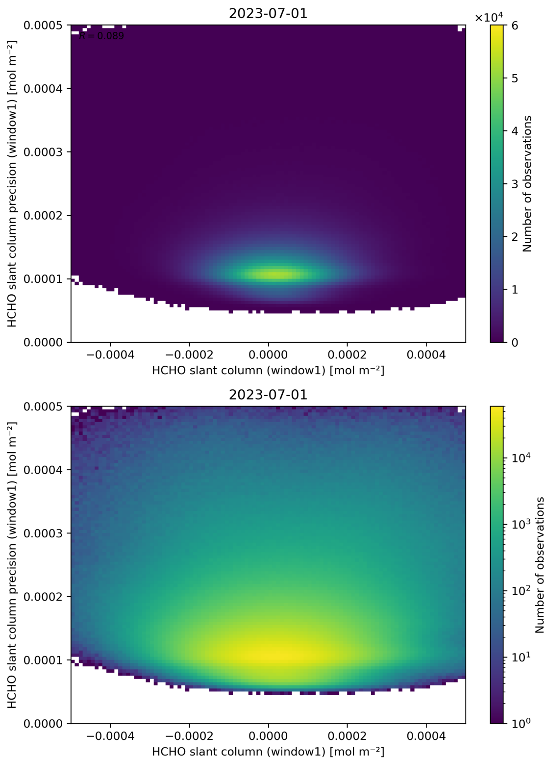
Figure 84: Scatter density plot of “HCHO slant column (window1)” against “HCHO slant column precision (window1)” for 2023-06-30 to 2023-07-02.
