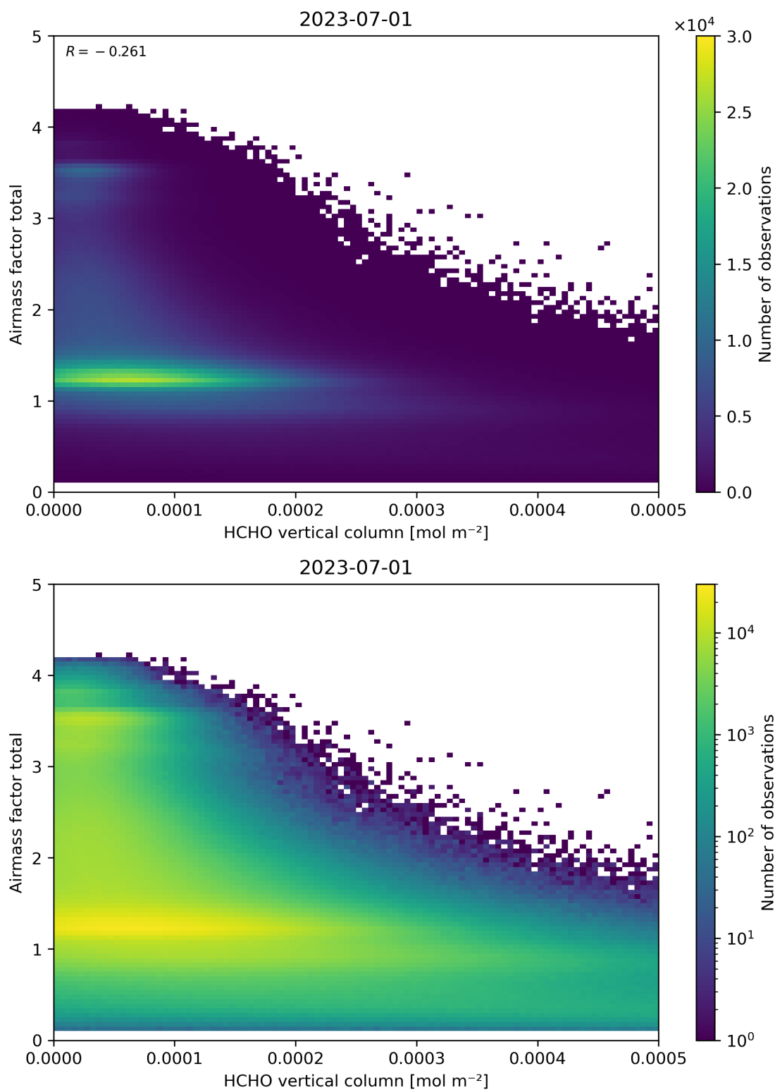
Figure 131: Scatter density plot of “HCHO vertical column” against “Airmass factor total” for 2023-06-30 to 2023-07-02.
