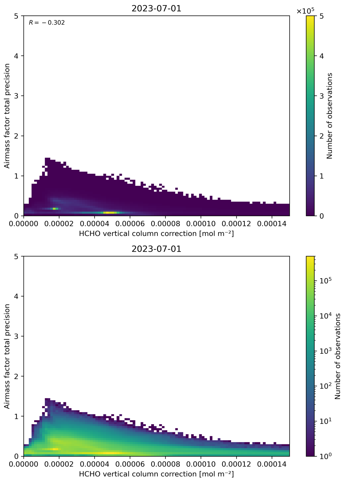
Figure 121: Scatter density plot of “HCHO vertical column correction” against “Airmass factor total precision” for 2023-06-30 to 2023-07-02.
