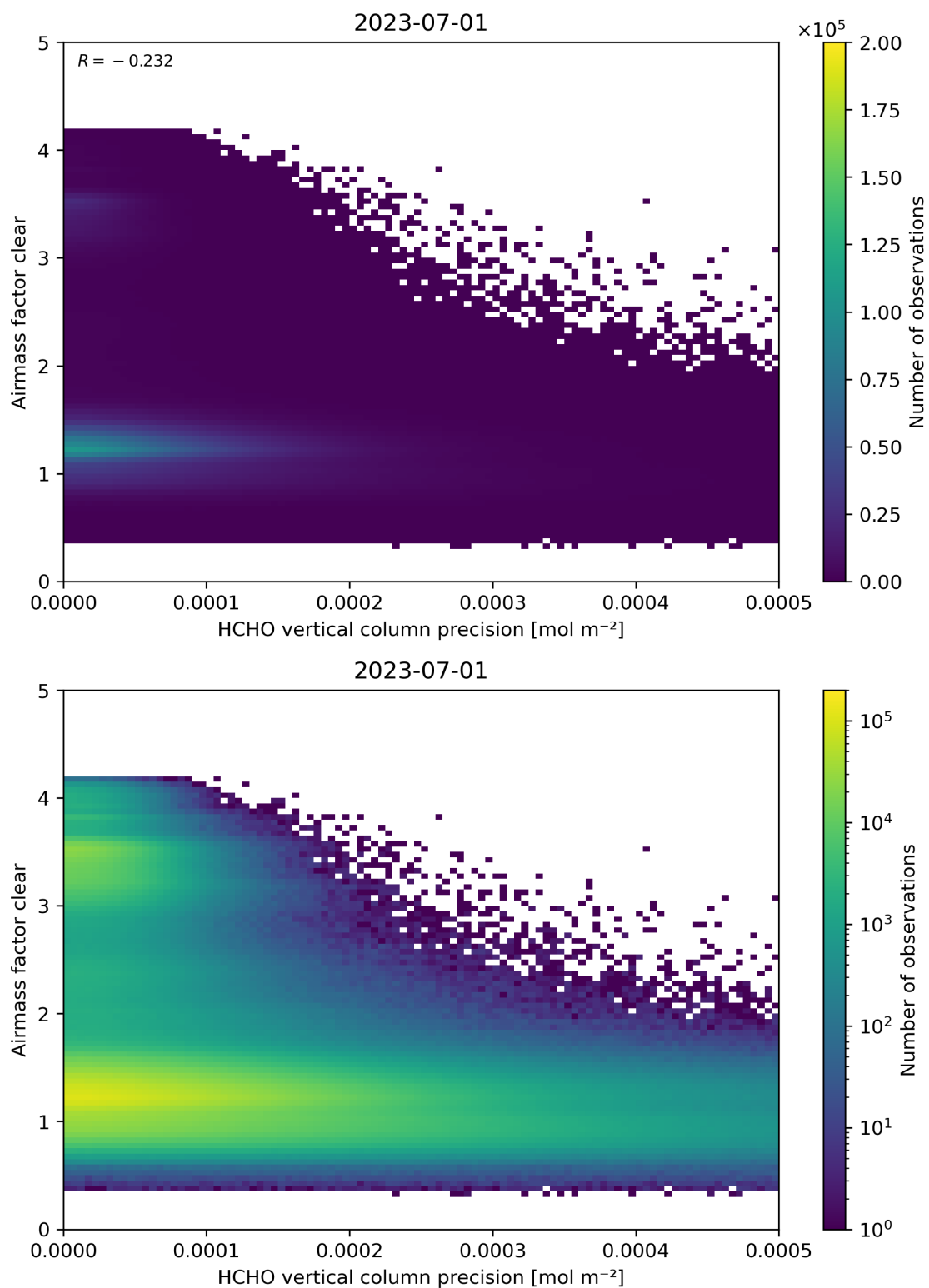
Figure 139: Scatter density plot of “HCHO vertical column precision” against “Airmass factor clear” for 2023-06-30 to 2023-07-02.
