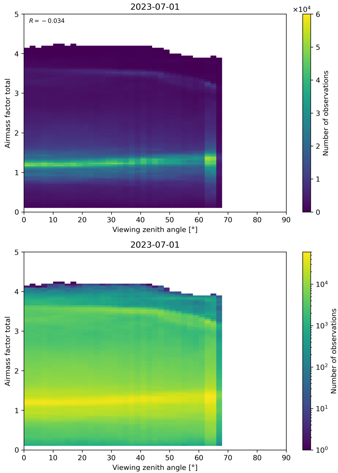
Figure 190: Scatter density plot of “Viewing zenith angle” against “Airmass factor total” for 2023-06-30 to 2023-07-02.
