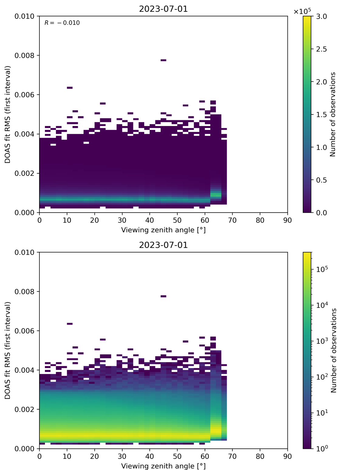
Figure 182: Scatter density plot of “Viewing zenith angle” against “DOAS fit RMS (first interval)” for 2023-06-30 to 2023-07-02.
