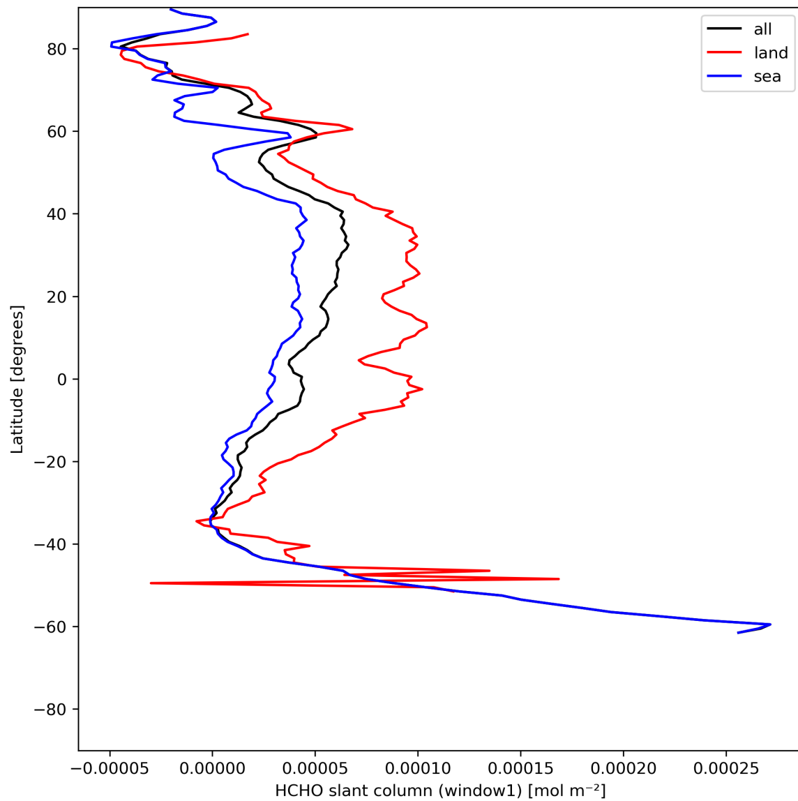
Figure 24: Zonal average of “HCHO slant column (window1)” for 2023-06-30 to 2023-07-02.
