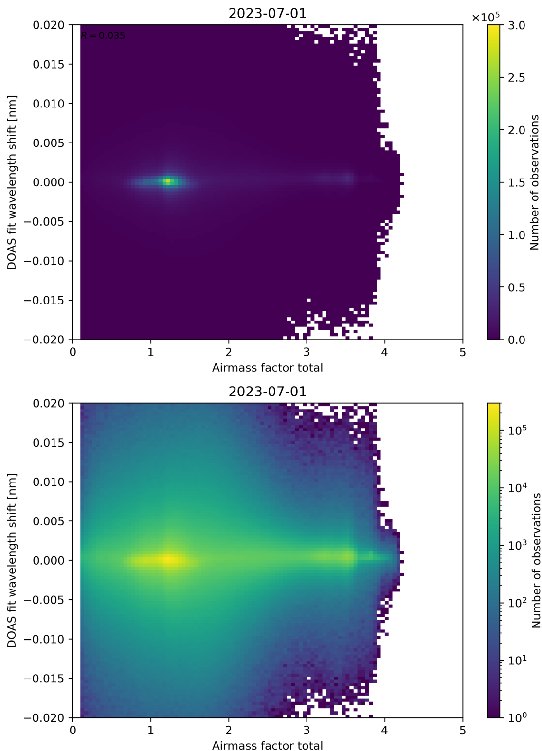
Figure 98: Scatter density plot of “Airmass factor total” against “DOAS fit wavelength shift” for 2023-06-30 to 2023-07-02.
