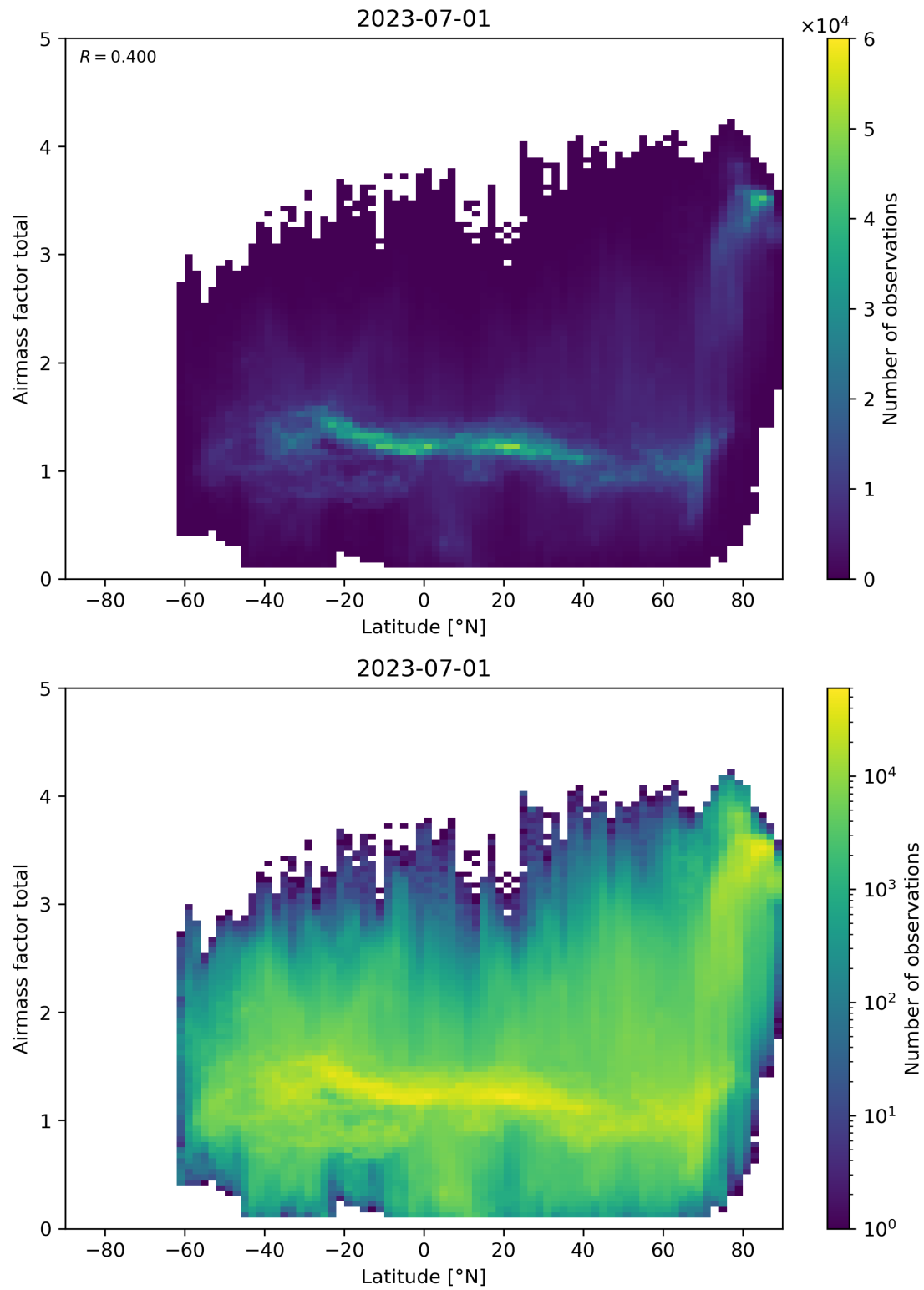
Figure 161: Scatter density plot of “Latitude” against “Airmass factor total” for 2023-06-30 to 2023-07-02.
