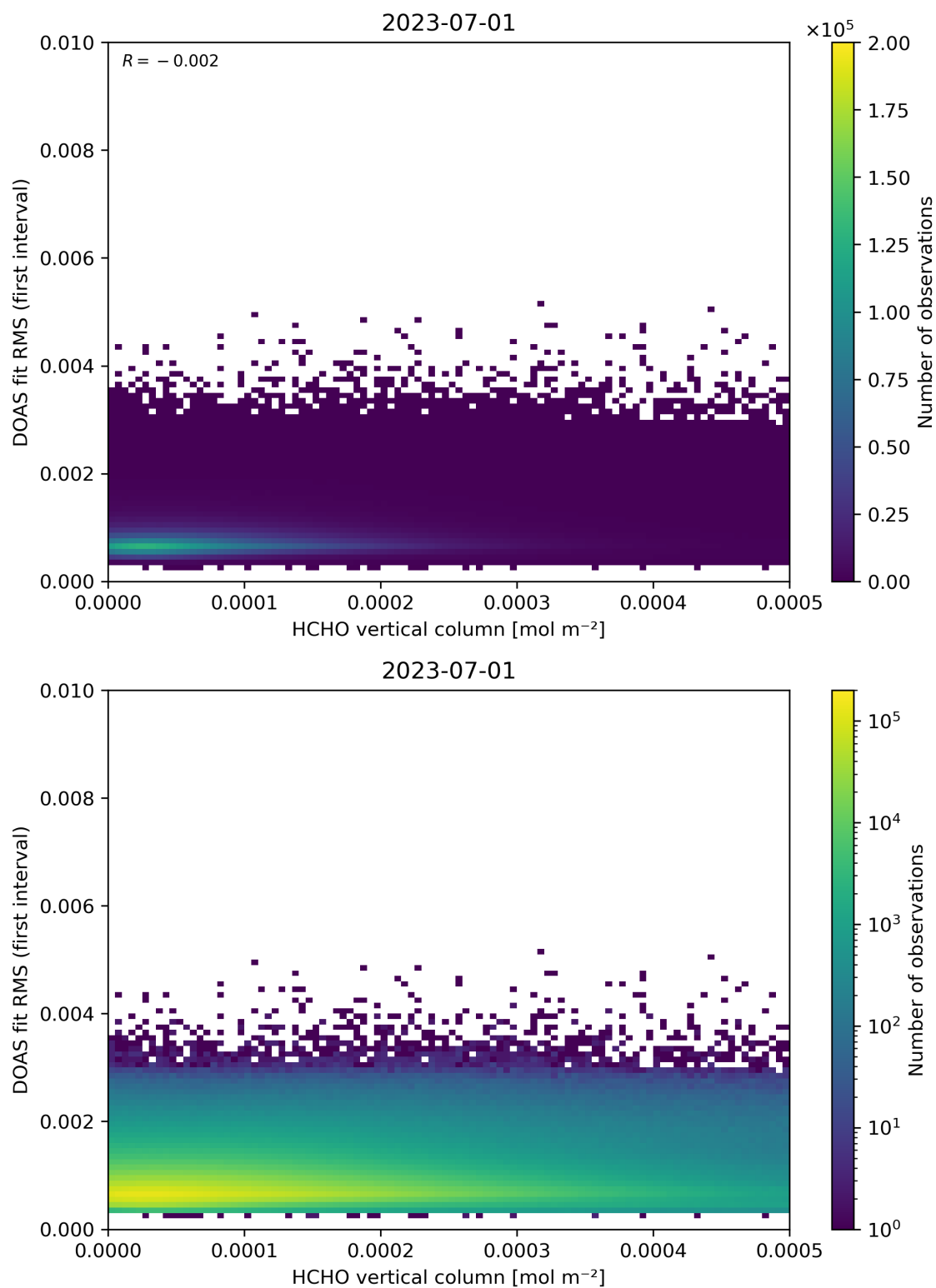
Figure 123: Scatter density plot of “HCHO vertical column” against “DOAS fit RMS (first interval)” for 2023-06-30 to 2023-07-02.
