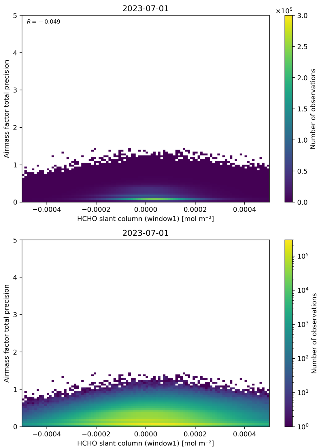
Figure 86: Scatter density plot of “HCHO slant column (window1)” against “Airmass factor total precision” for 2023-06-30 to 2023-07-02.
