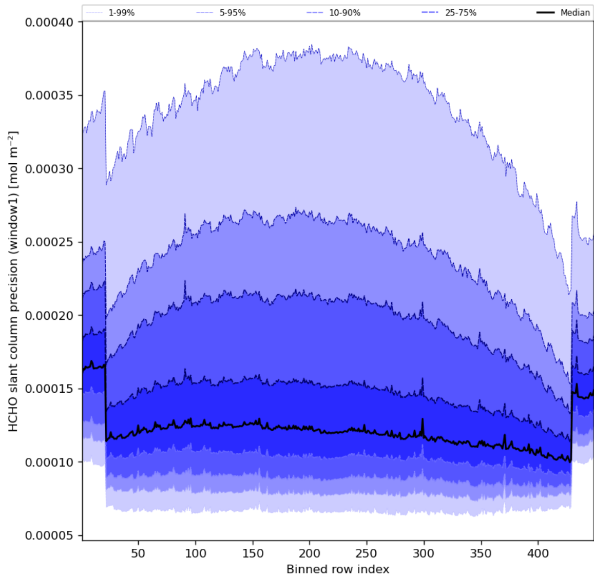
Figure 53: Along track statistics of “HCHO slant column precision (window1)” for 2023-06-30 to 2023-07-02
