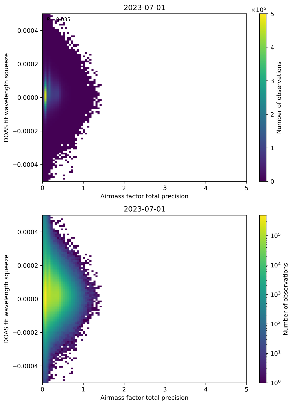
Figure 107: Scatter density plot of “Airmass factor total precision” against “DOAS fit wavelength squeeze” for 2023-06-30 to 2023-07-02.
