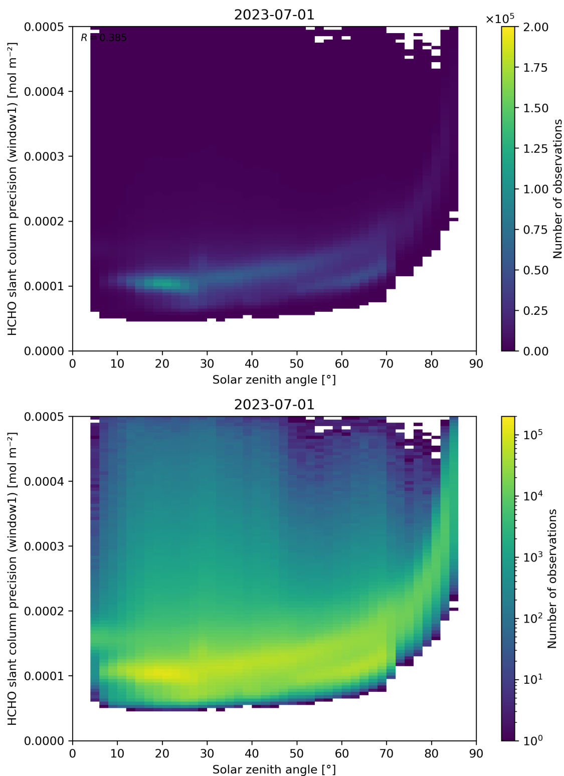
Figure 174: Scatter density plot of “Solar zenith angle” against “HCHO slant column precision (window1)” for 2023-06-30 to 2023-07-02.
