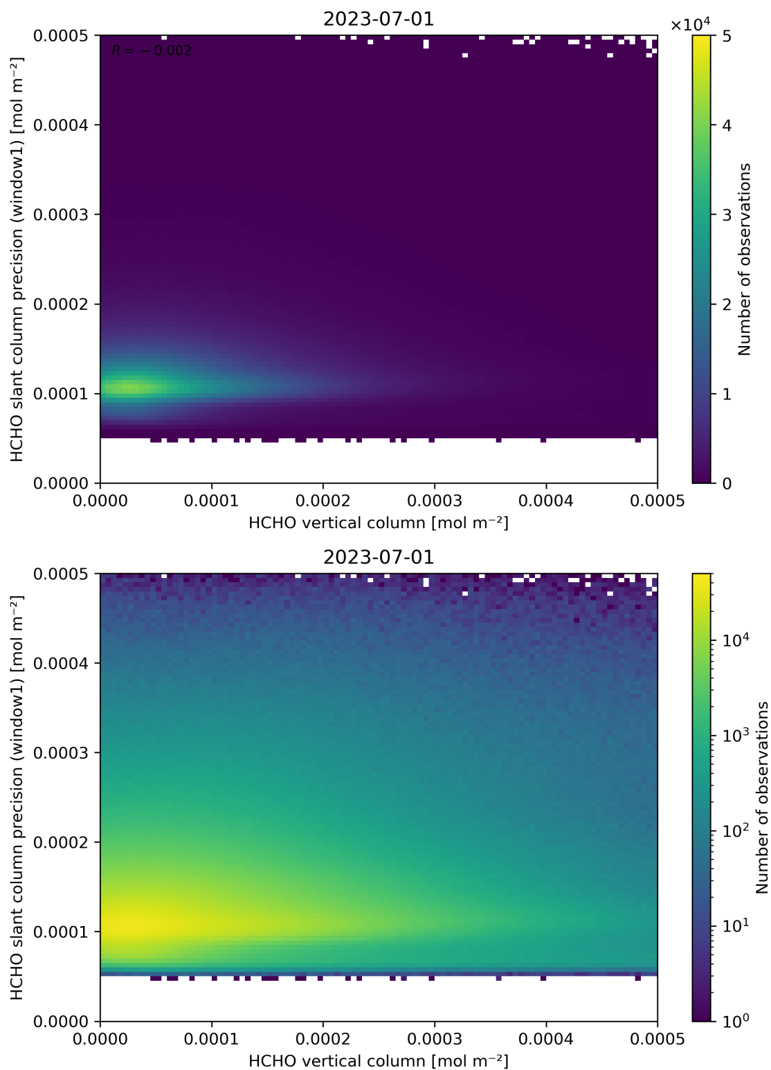
Figure 130: Scatter density plot of “HCHO vertical column” against “HCHO slant column precision (window1)” for 2023-06-30 to 2023-07-02.
