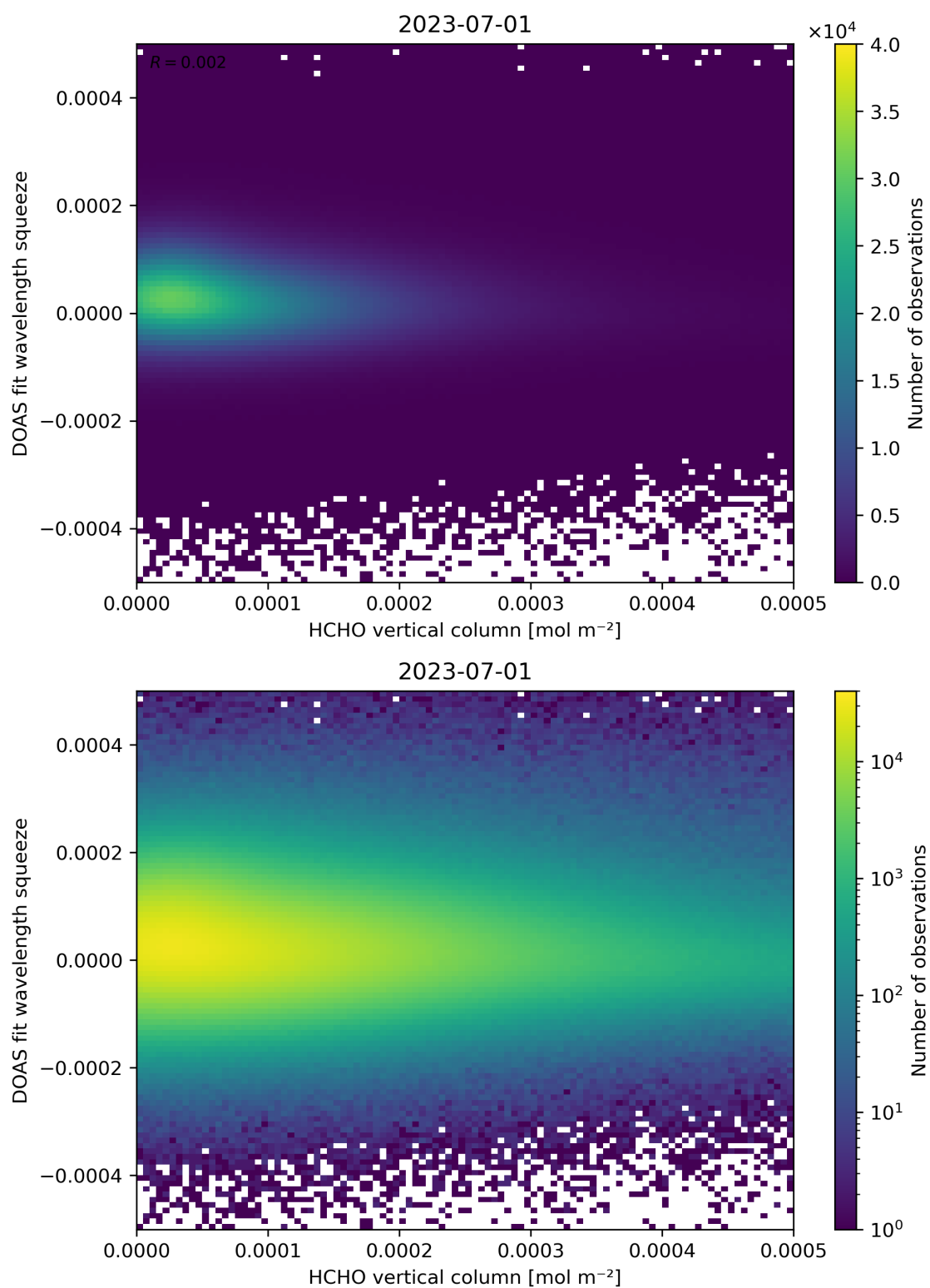
Figure 125: Scatter density plot of “HCHO vertical column” against “DOAS fit wavelength squeeze” for 2023-06-30 to 2023-07-02.
