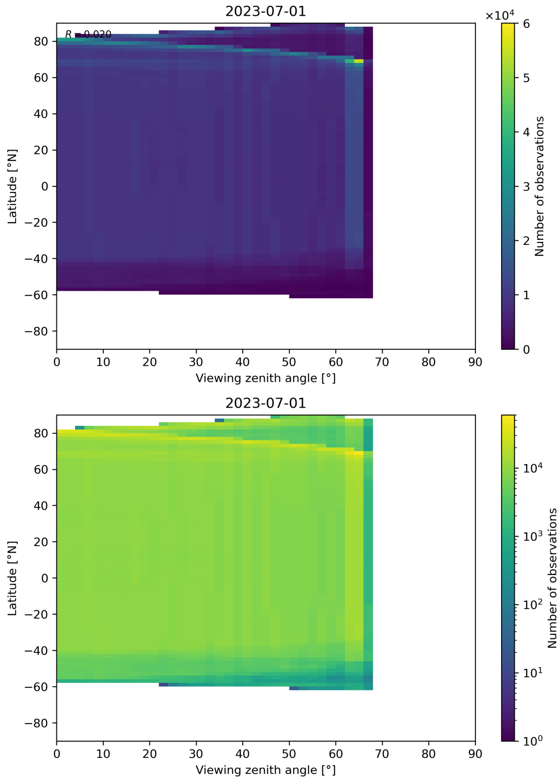
Figure 196: Scatter density plot of “Viewing zenith angle” against “Latitude” for 2023-06-30 to 2023-07-02.
