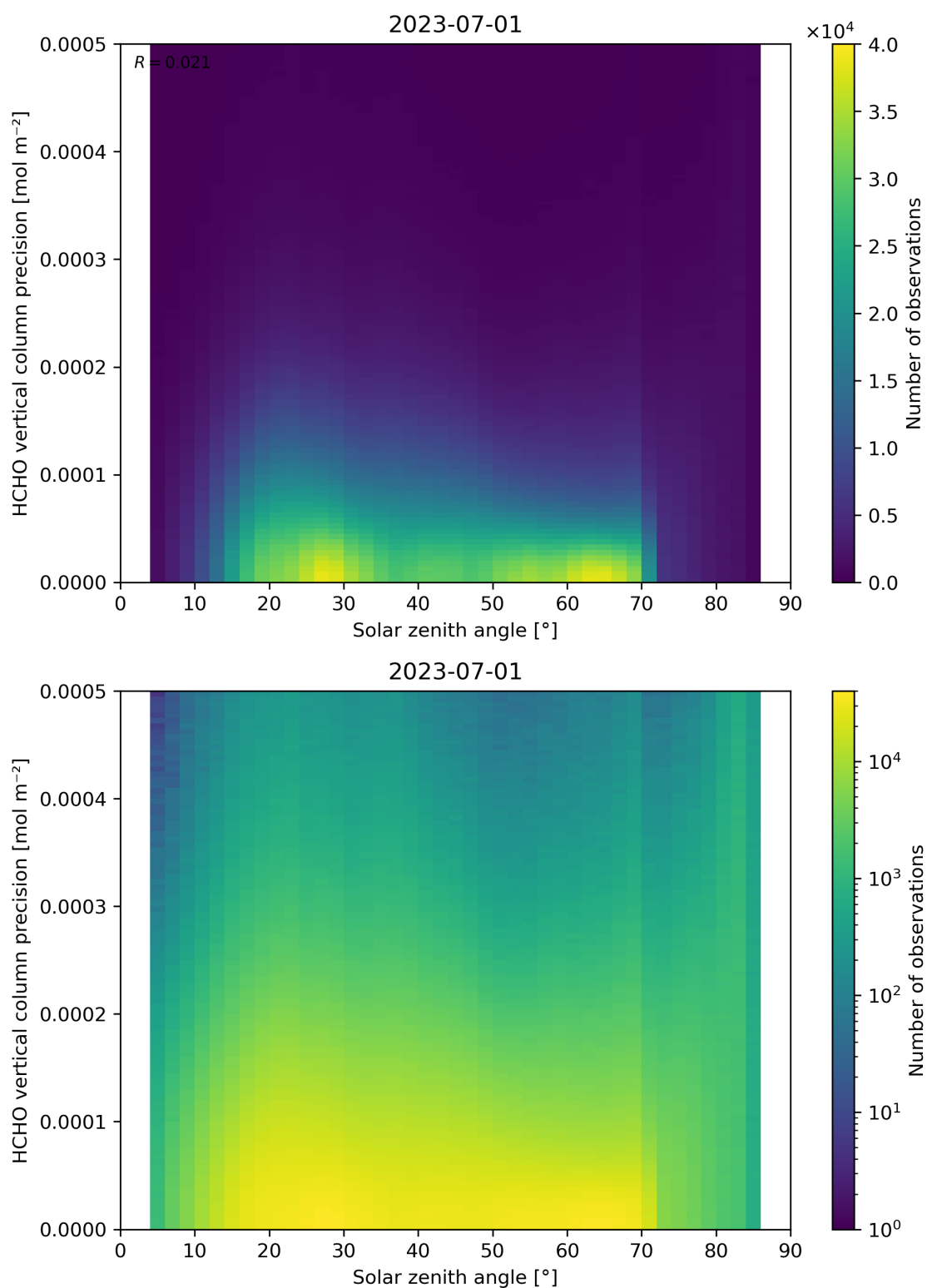
Figure 179: Scatter density plot of “Solar zenith angle” against “HCHO vertical column precision” for 2023-06-30 to 2023-07-02.
