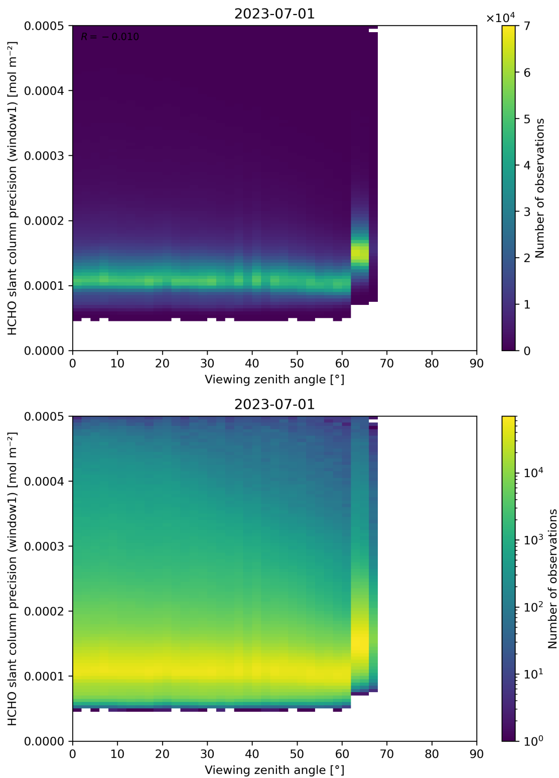
Figure 189: Scatter density plot of “Viewing zenith angle” against “HCHO slant column precision (window1)” for 2023-06-30 to 2023-07-02.
