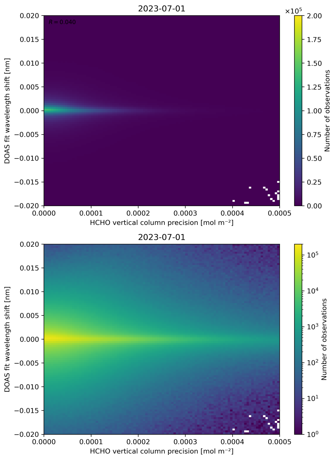
Figure 137: Scatter density plot of “HCHO vertical column precision” against “DOAS fit wavelength shift” for 2023-06-30 to 2023-07-02.
