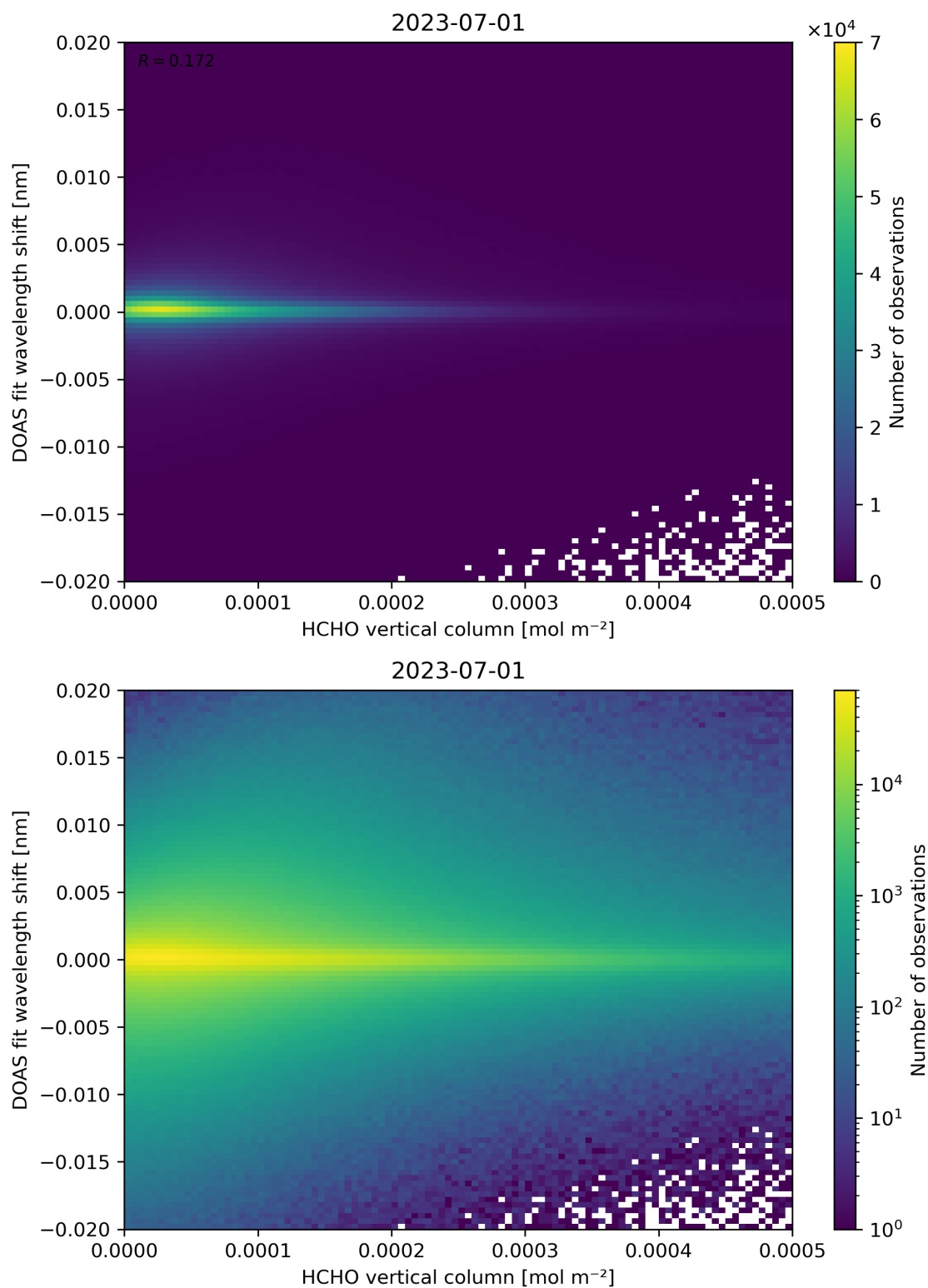
Figure 124: Scatter density plot of “HCHO vertical column” against “DOAS fit wavelength shift” for 2023-06-30 to 2023-07-02.
