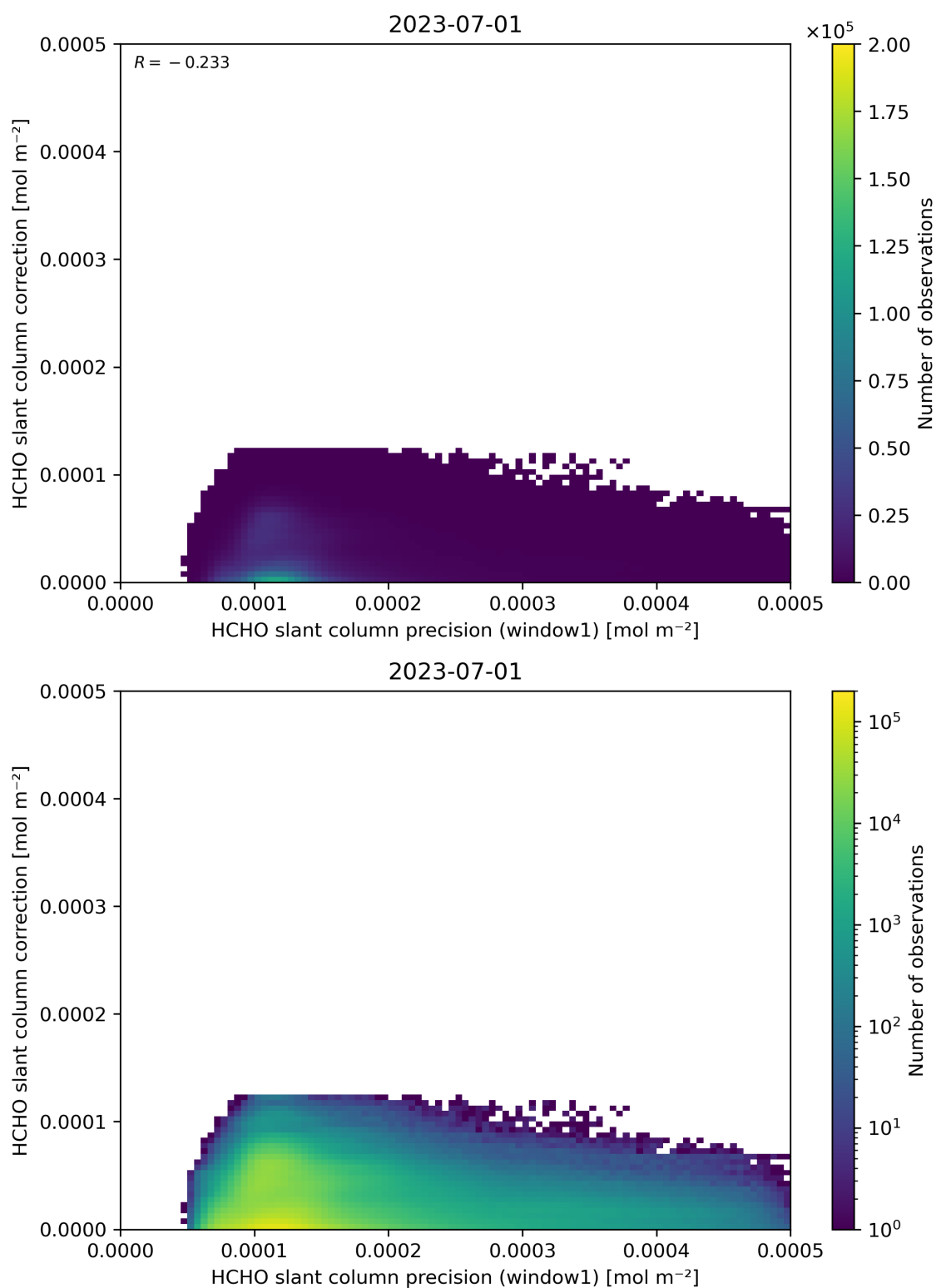
Figure 93: Scatter density plot of “HCHO slant column precision (window1)” against “HCHO slant column correction” for 2023-06-30 to 2023-07-02.
