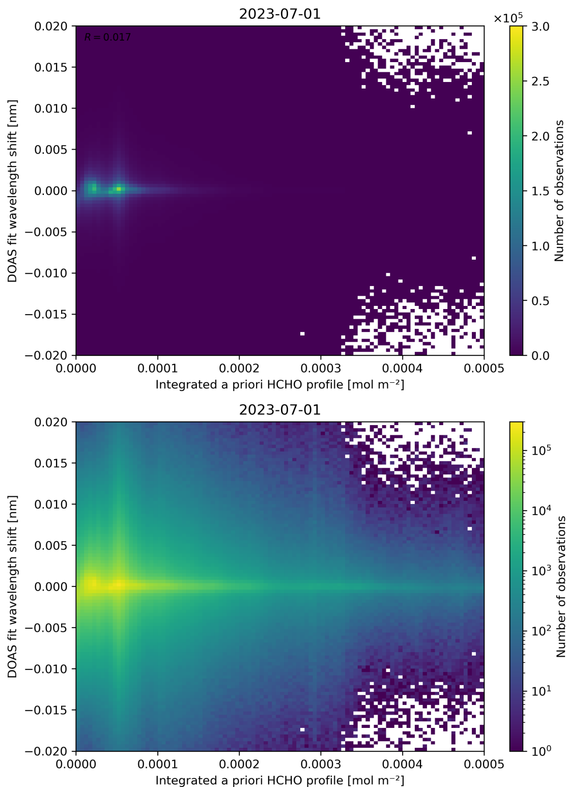
Figure 149: Scatter density plot of “Integrated a priori HCHO profile” against “DOAS fit wavelength shift” for 2023-06-30 to 2023-07-02.
