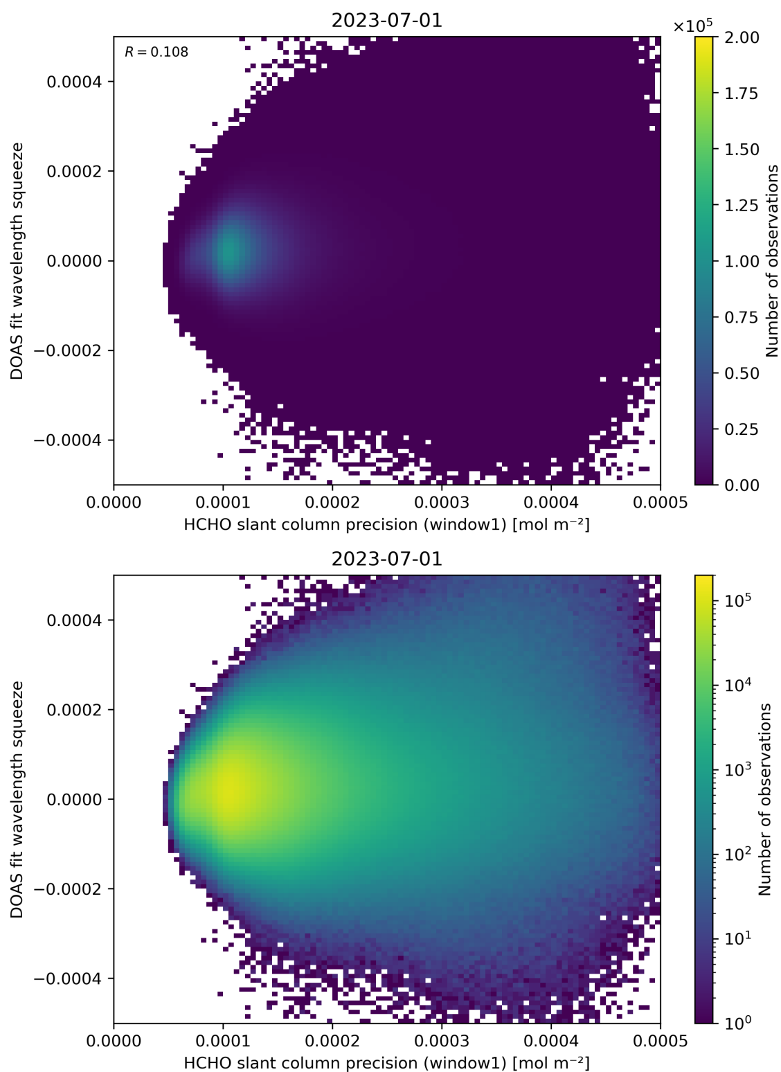
Figure 90: Scatter density plot of “HCHO slant column precision (window1)” against “DOAS fit wavelength squeeze” for 2023-06-30 to 2023-07-02.
