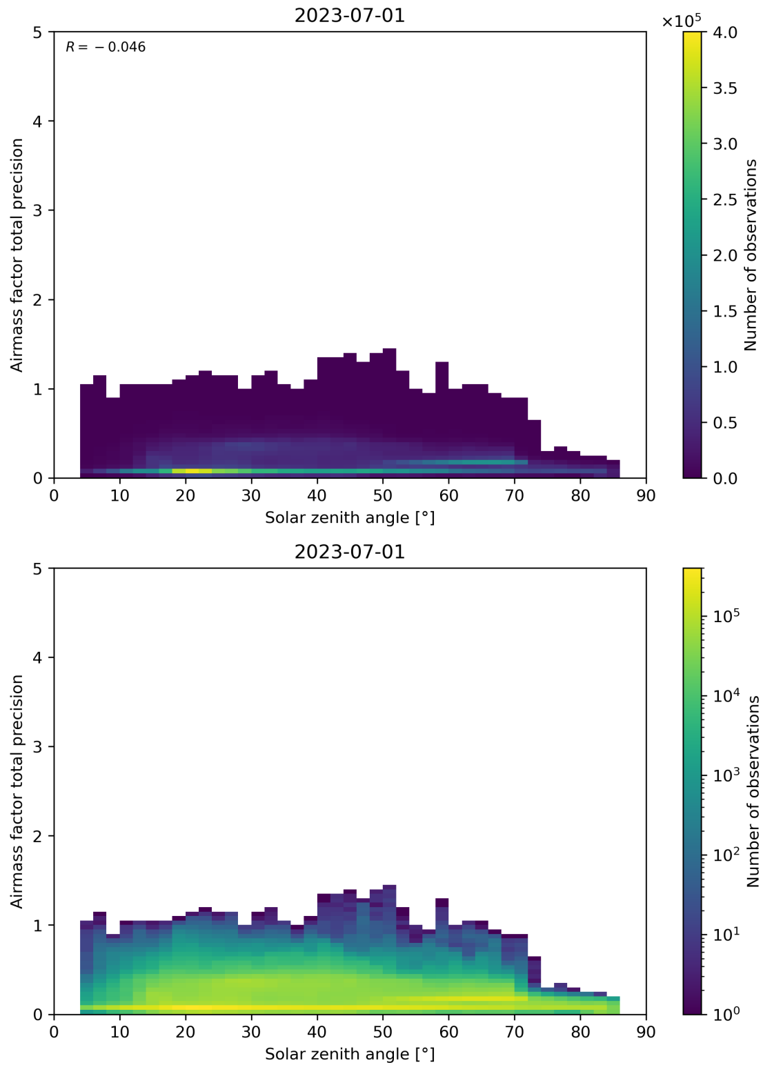
Figure 176: Scatter density plot of “Solar zenith angle” against “Airmass factor total precision” for 2023-06-30 to 2023-07-02.
