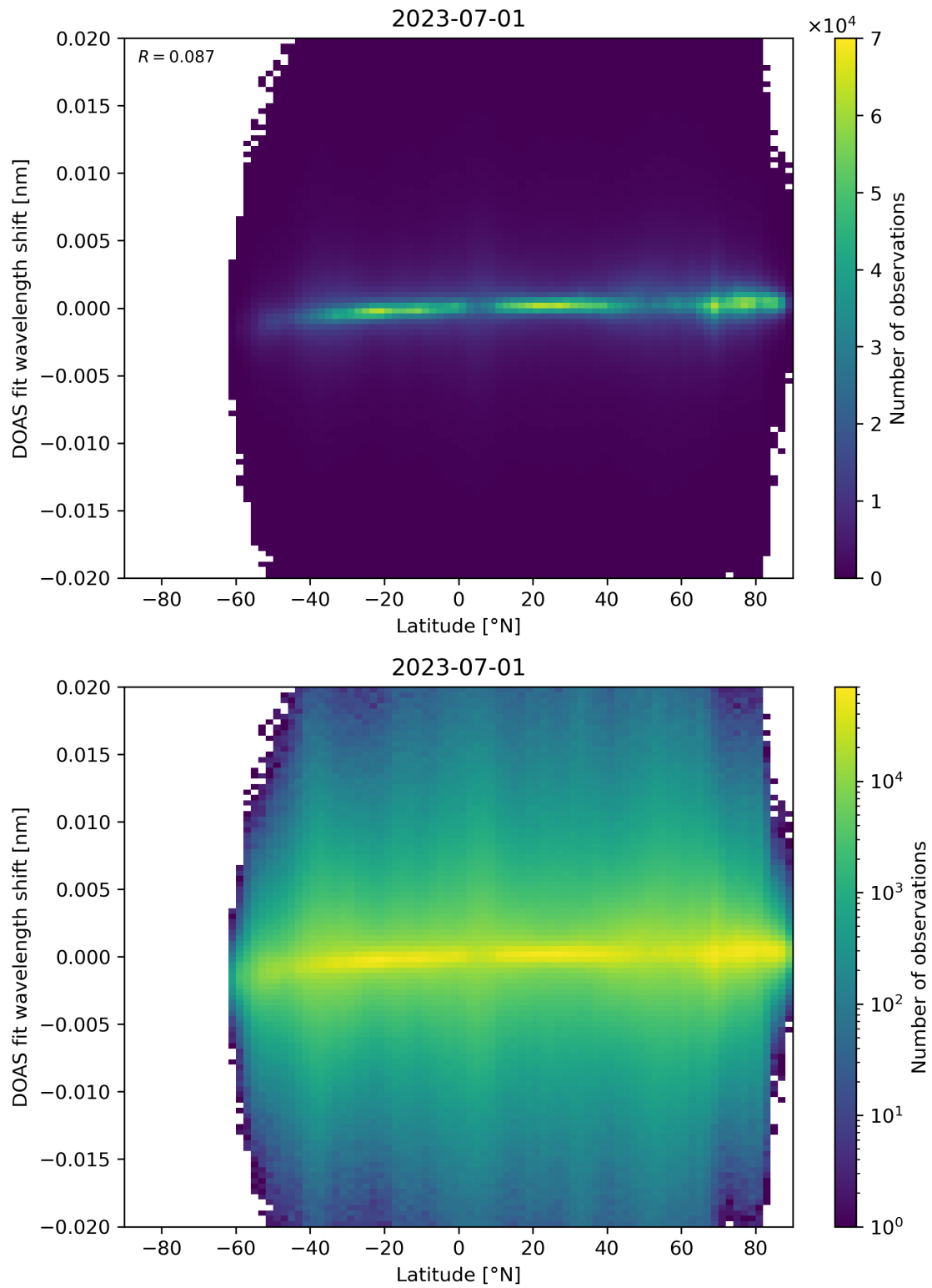
Figure 154: Scatter density plot of “Latitude” against “DOAS fit wavelength shift” for 2023-06-30 to 2023-07-02.
