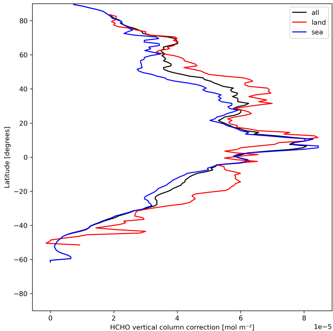
Figure 23: Zonal average of "HCHO vertical column correction" for 2023-06-30 to 2023-07-02.
