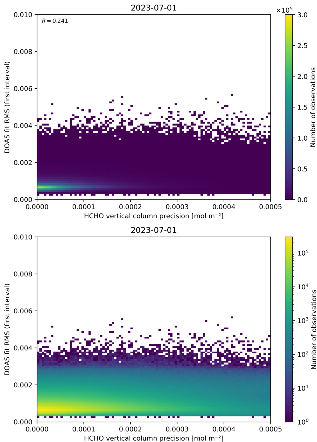
Figure 136: Scatter density plot of “HCHO vertical column precision” against “DOAS fit RMS (first interval)” for 2023-06-30 to 2023-07-02.
