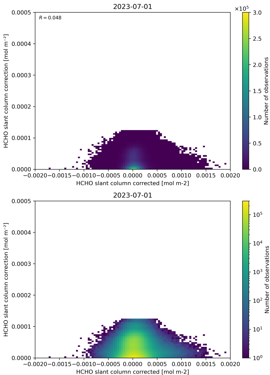
Figure 77: Scatter density plot of “HCHO slant column corrected” against “HCHO slant column correction” for 2023-06-30 to 2023-07-02.
