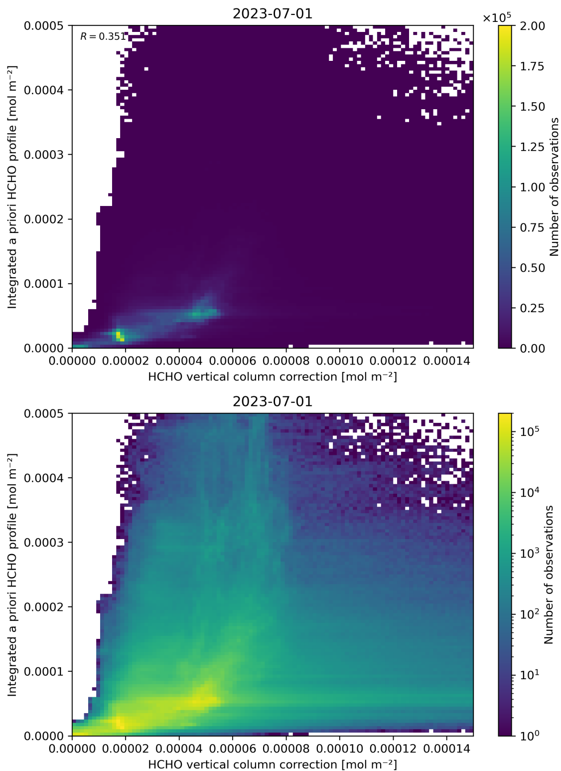
Figure 122: Scatter density plot of “HCHO vertical column correction” against “Integrated a priori HCHO profile” for 2023-06-30 to 2023-07-02.
