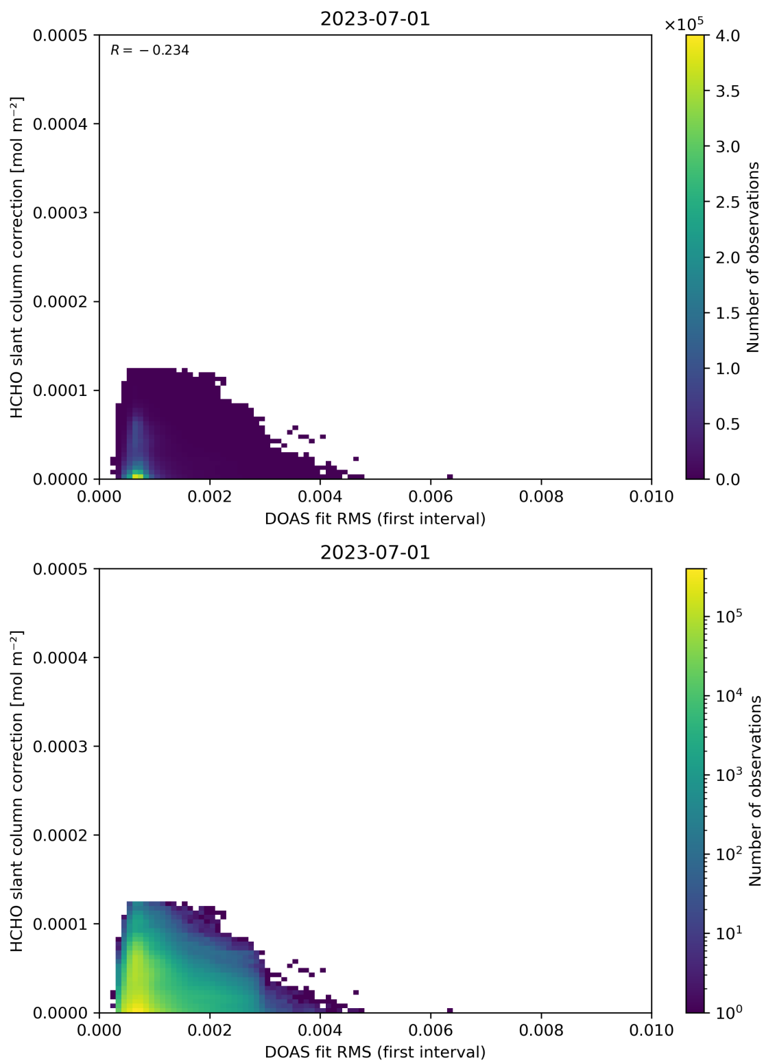
Figure 63: Scatter density plot of “DOAS fit RMS (first interval)” against “HCHO slant column correction” for 2023-06-30 to 2023-07-02.
