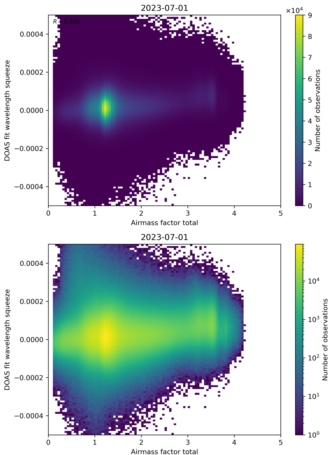
Figure 99: Scatter density plot of “Airmass factor total” against “DOAS fit wavelength squeeze” for 2023-06-30 to 2023-07-02.
