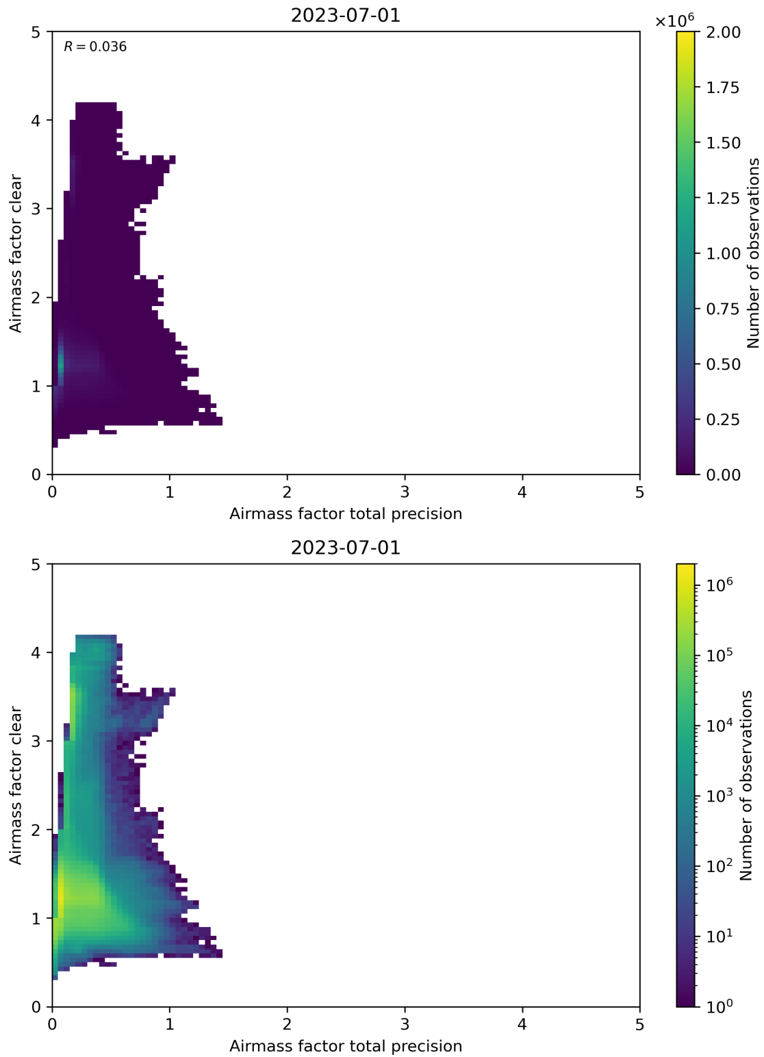
Figure 108: Scatter density plot of “Airmass factor total precision” against “Airmass factor clear” for 2023-06-30 to 2023-07-02.
