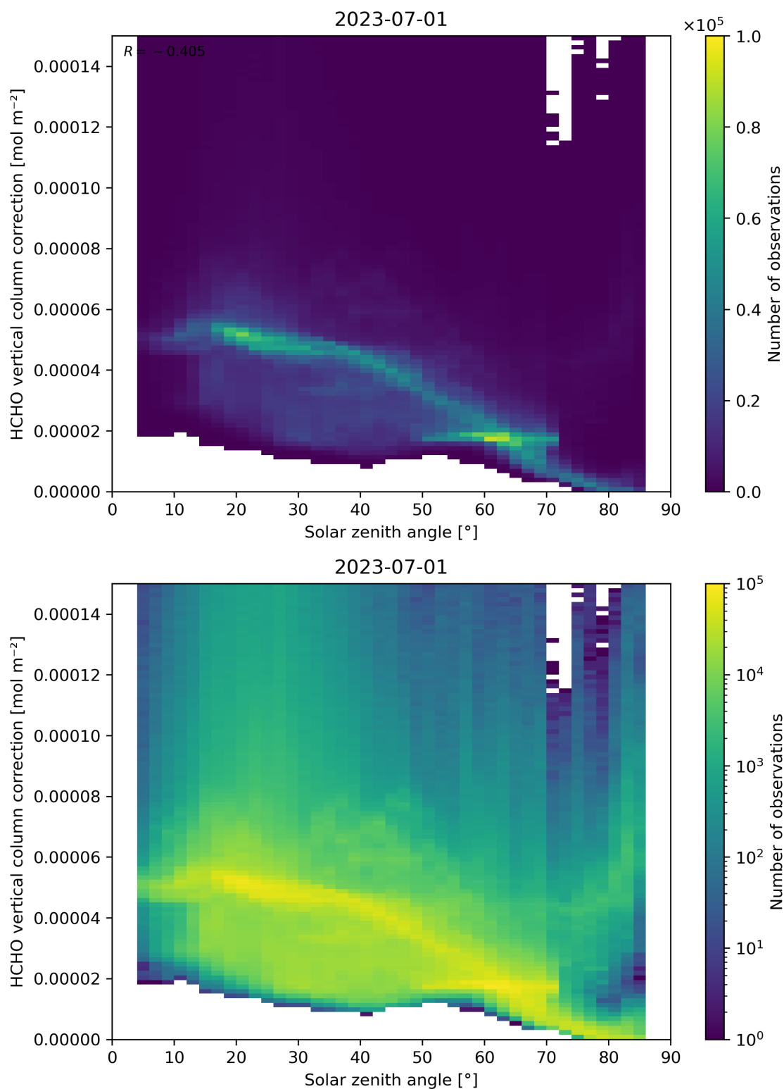
Figure 178: Scatter density plot of “Solar zenith angle” against “HCHO vertical column correction” for 2023-06-30 to 2023-07-02.
