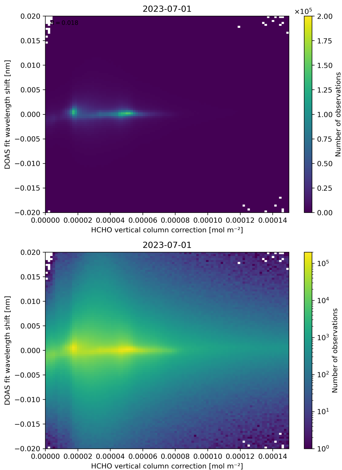
Figure 113: Scatter density plot of “HCHO vertical column correction” against “DOAS fit wavelength shift” for 2023-06-30 to 2023-07-02.
