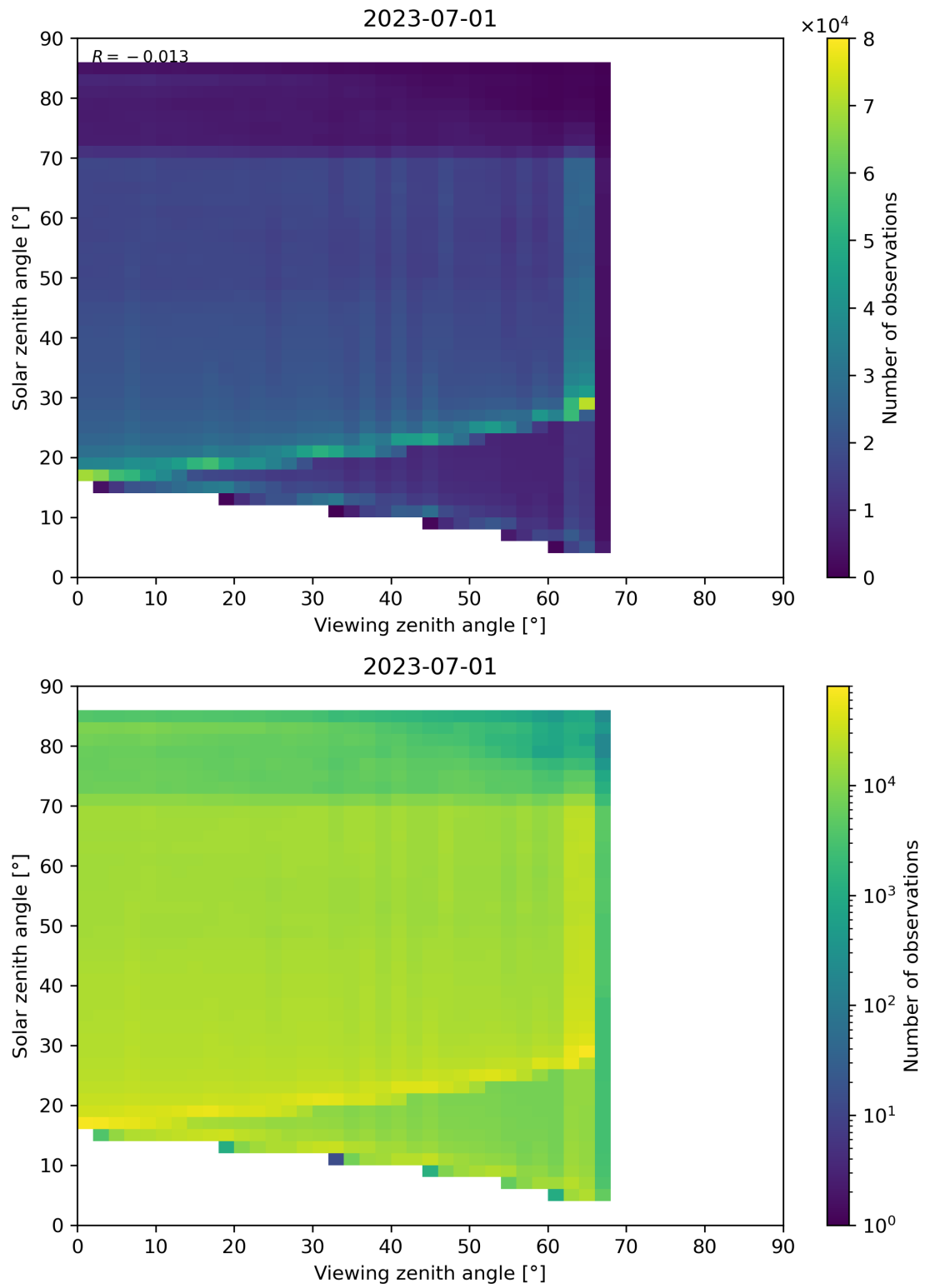
Figure 197: Scatter density plot of “Viewing zenith angle” against “Solar zenith angle” for 2023-06-30 to 2023-07-02.
