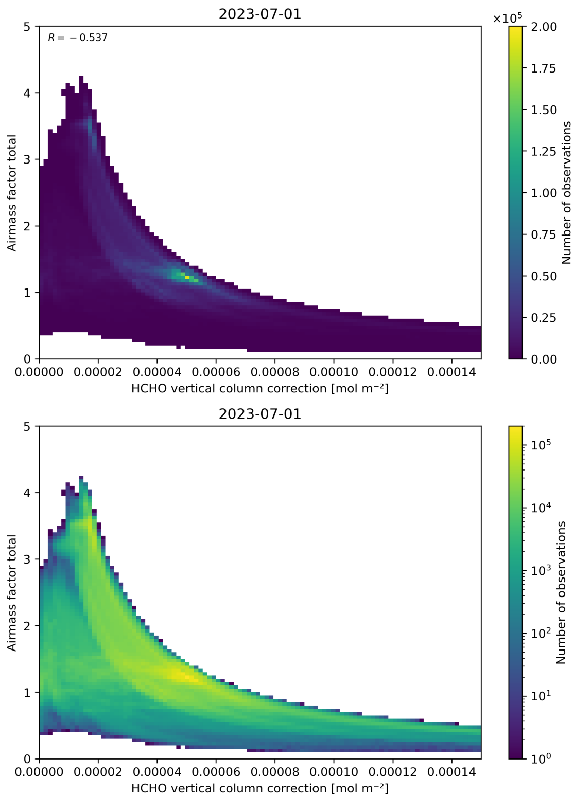
Figure 120: Scatter density plot of “HCHO vertical column correction” against “Airmass factor total” for 2023-06-30 to 2023-07-02.
