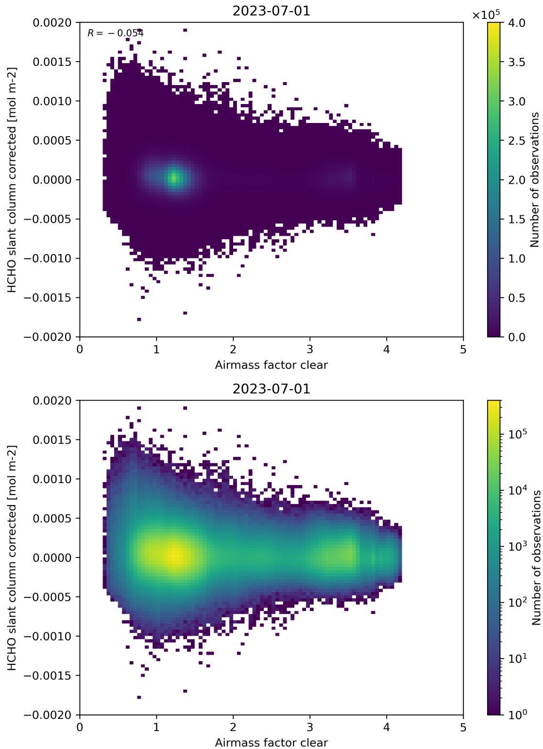
Figure 74: Scatter density plot of “Airmass factor clear” against “HCHO slant column corrected” for 2023-06-30 to 2023-07-02.
