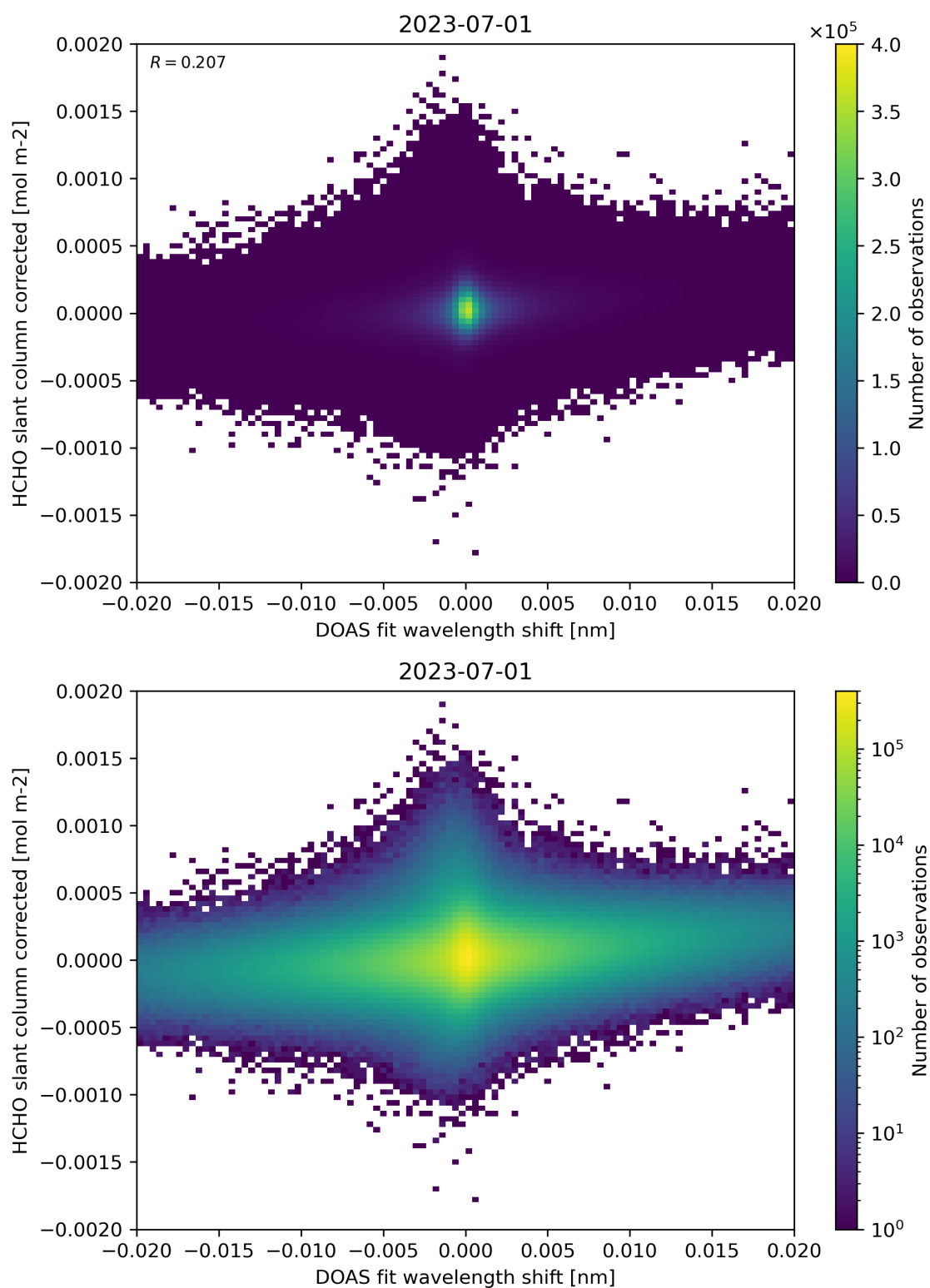
Figure 66: Scatter density plot of “DOAS fit wavelength shift” against “HCHO slant column corrected” for 2023-06-30 to 2023-07-02.
