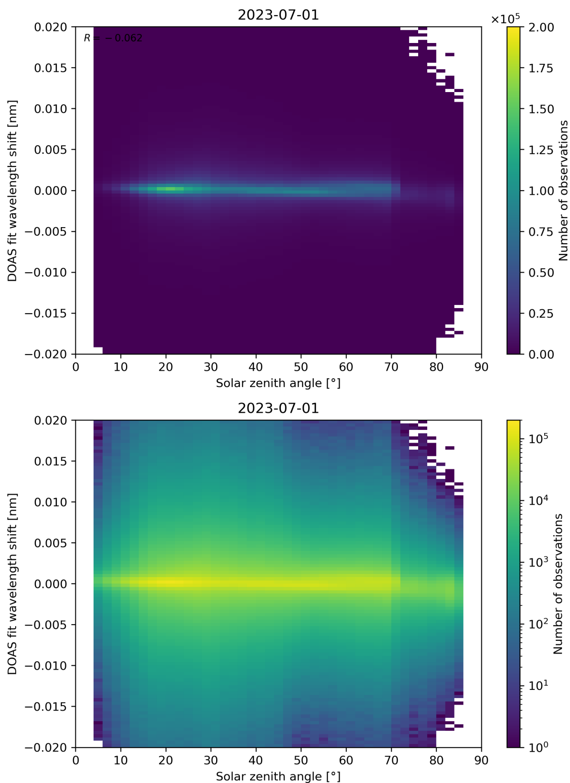
Figure 168: Scatter density plot of “Solar zenith angle” against “DOAS fit wavelength shift” for 2023-06-30 to 2023-07-02.
