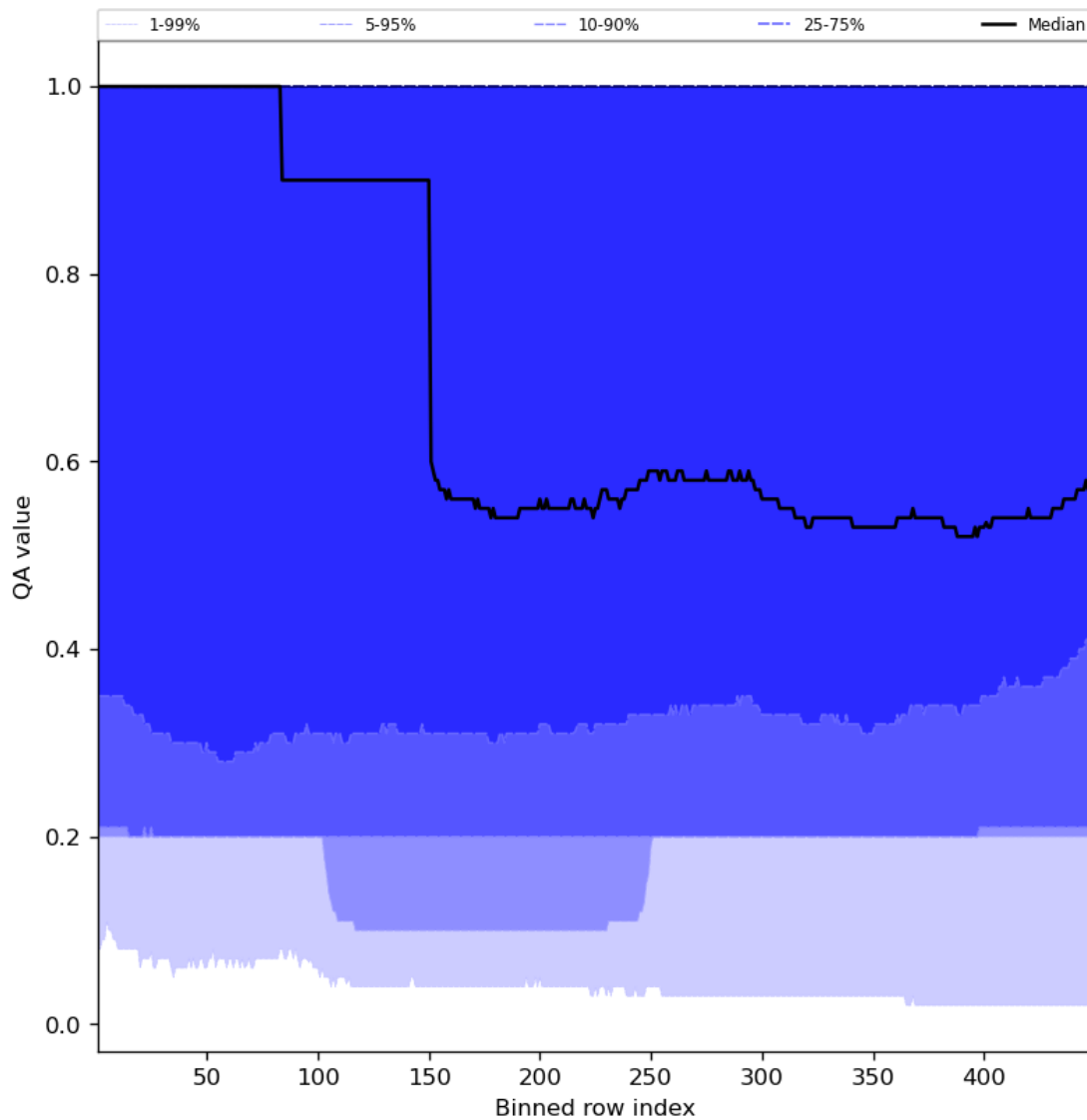
Figure 48: Along track statistics of “QA value” for 2023-06-30 to 2023-07-02
