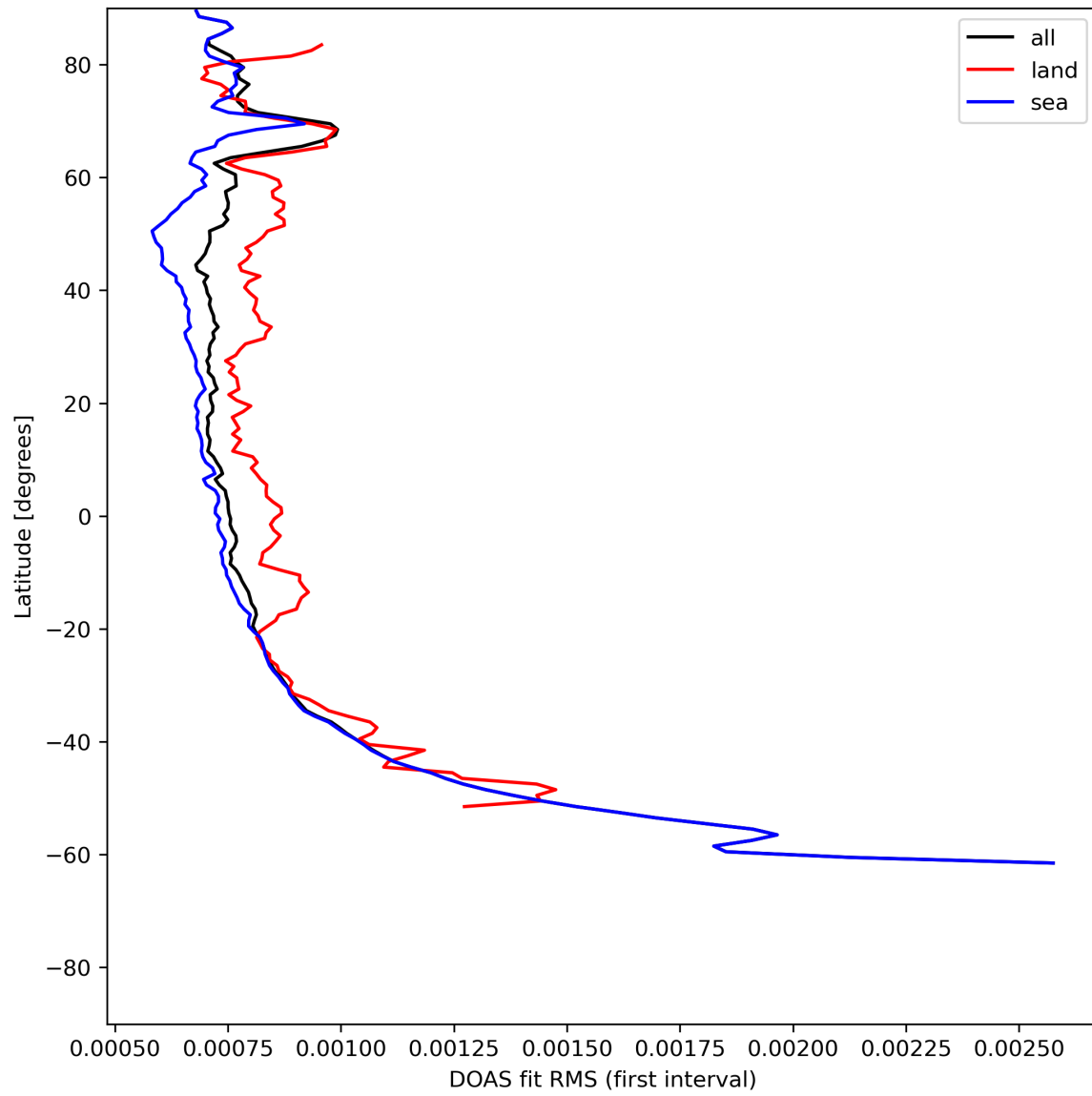
Figure 32: Zonal average of “DOAS fit RMS (first interval)” for 2023-06-30 to 2023-07-02.
