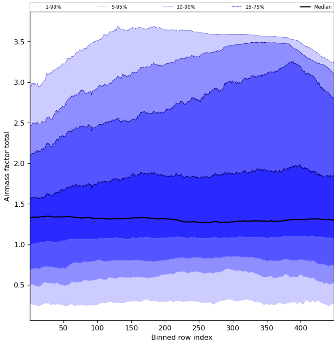
Figure 54: Along track statistics of “Airmass factor total” for 2023-06-30 to 2023-07-02
