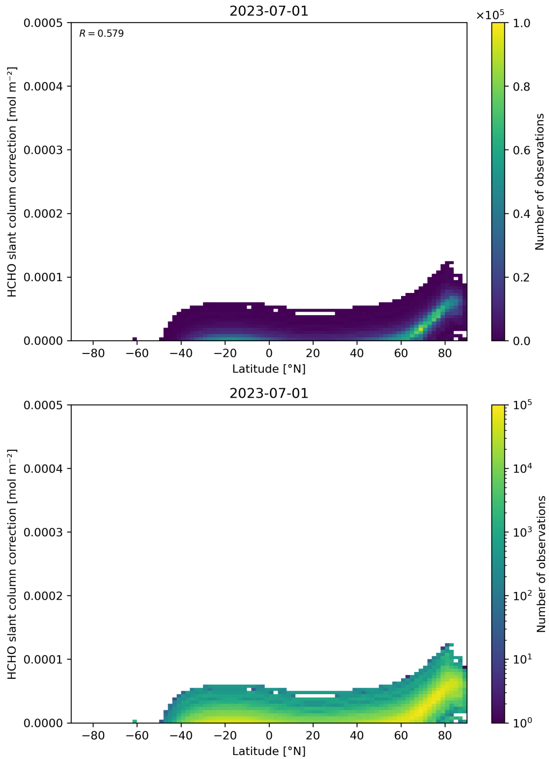
Figure 158: Scatter density plot of “Latitude” against “HCHO slant column correction” for 2023-06-30 to 2023-07-02.
