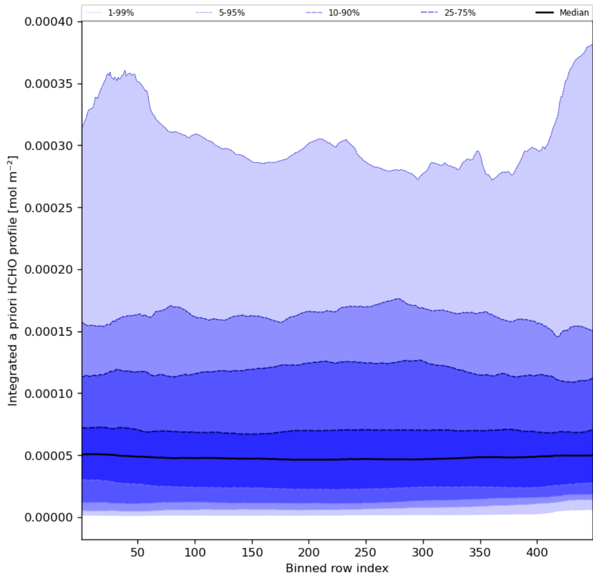
Figure 57: Along track statistics of “Integrated a priori HCHO profile” for 2023-06-30 to 2023-07-02
