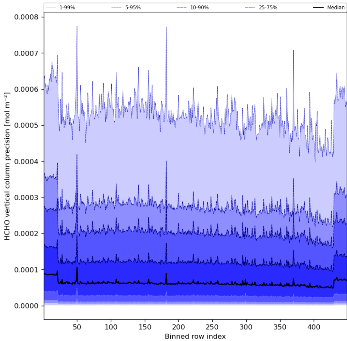
Figure 50: Along track statistics of “HCHO vertical column precision” for 2023-06-30 to 2023-07-02
