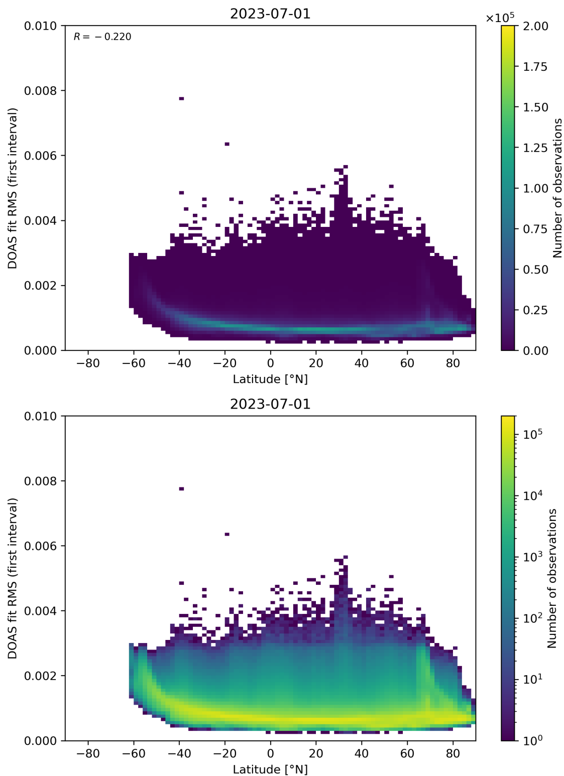
Figure 153: Scatter density plot of “Latitude” against “DOAS fit RMS (first interval)” for 2023-06-30 to 2023-07-02.
