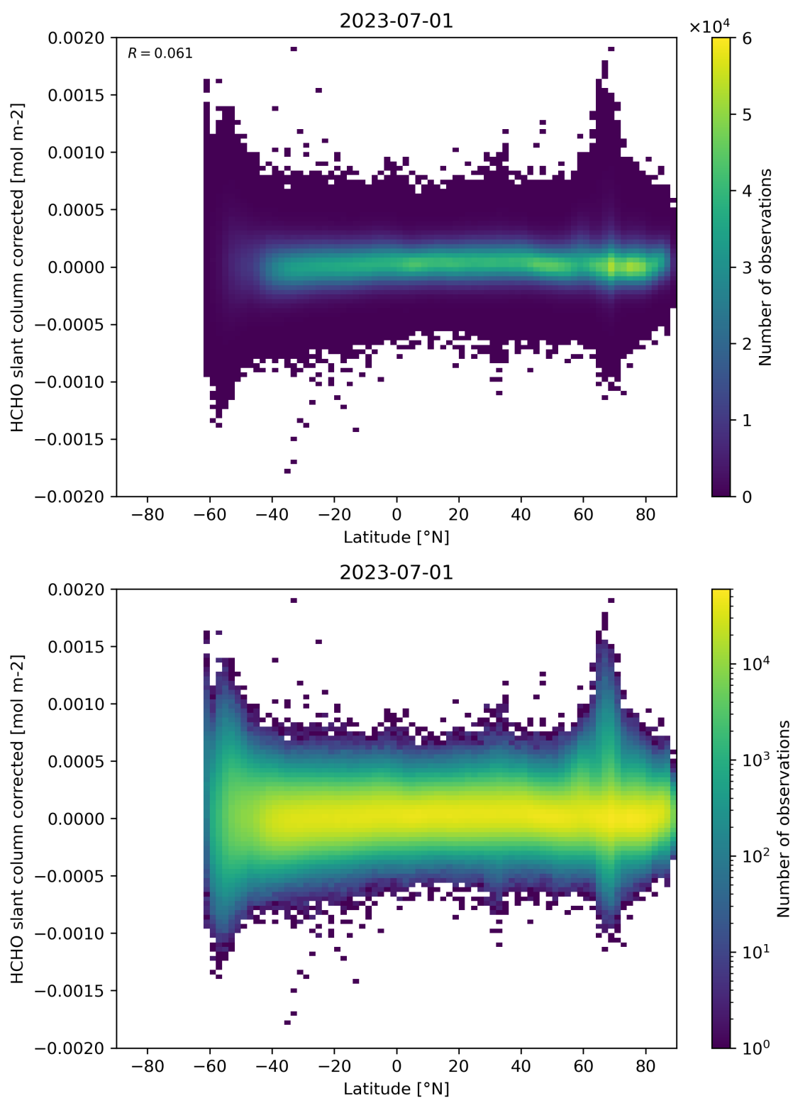
Figure 157: Scatter density plot of “Latitude” against “HCHO slant column corrected” for 2023-06-30 to 2023-07-02.
