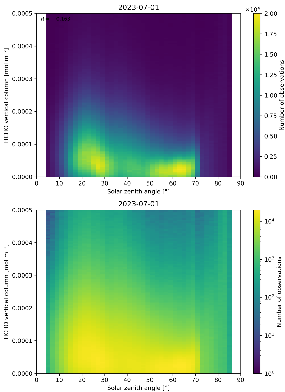
Figure 177: Scatter density plot of “Solar zenith angle” against “HCHO vertical column” for 2023-06-30 to 2023-07-02.
