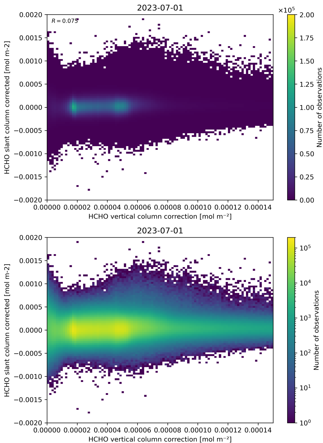
Figure 116: Scatter density plot of “HCHO vertical column correction” against “HCHO slant column corrected” for 2023-06-30 to 2023-07-02.
