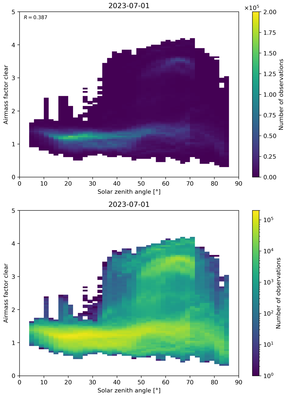
Figure 170: Scatter density plot of “Solar zenith angle” against “Airmass factor clear” for 2023-06-30 to 2023-07-02.
