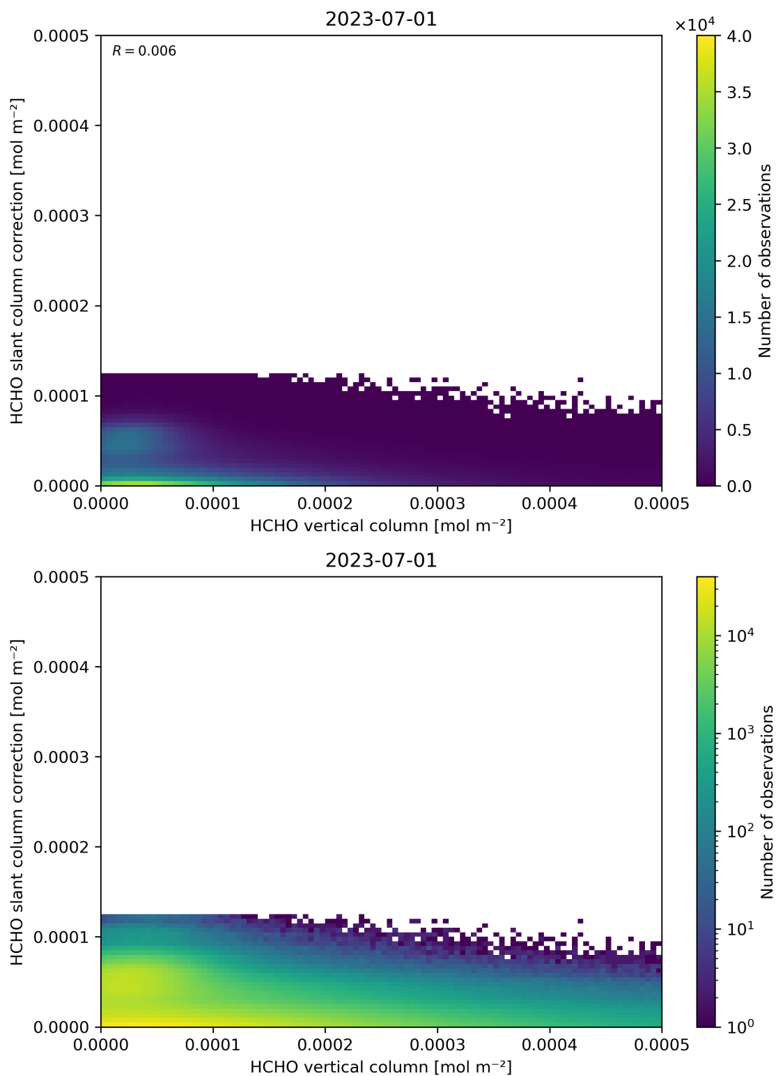
Figure 128: Scatter density plot of “HCHO vertical column” against “HCHO slant column correction” for 2023-06-30 to 2023-07-02.
