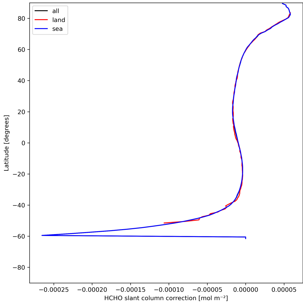
Figure 33: Zonal average of “HCHO slant column correction” for 2023-06-30 to 2023-07-02.
