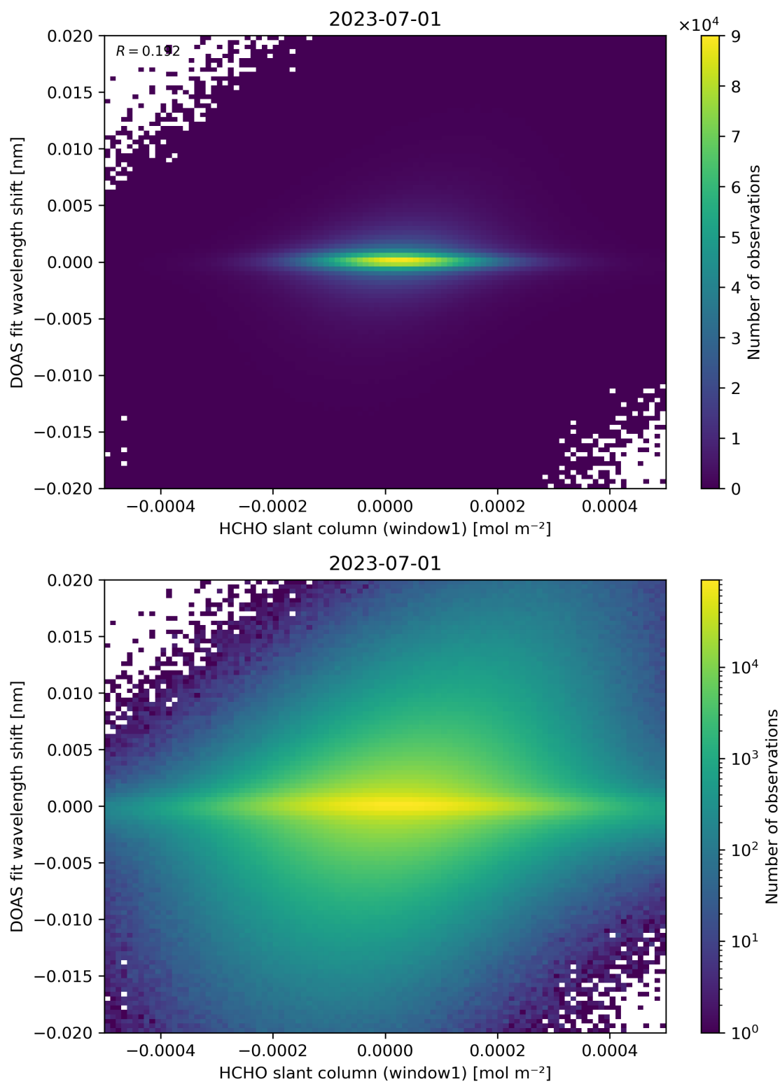
Figure 79: Scatter density plot of “HCHO slant column (window1)” against “DOAS fit wavelength shift” for 2023-06-30 to 2023-07-02.
