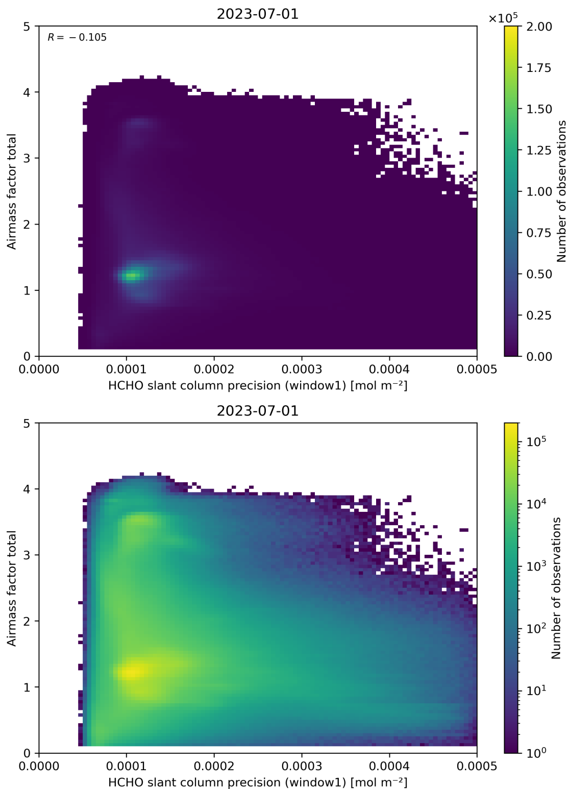
Figure 94: Scatter density plot of “HCHO slant column precision (window1)” against “Airmass factor total” for 2023-06-30 to 2023-07-02.
