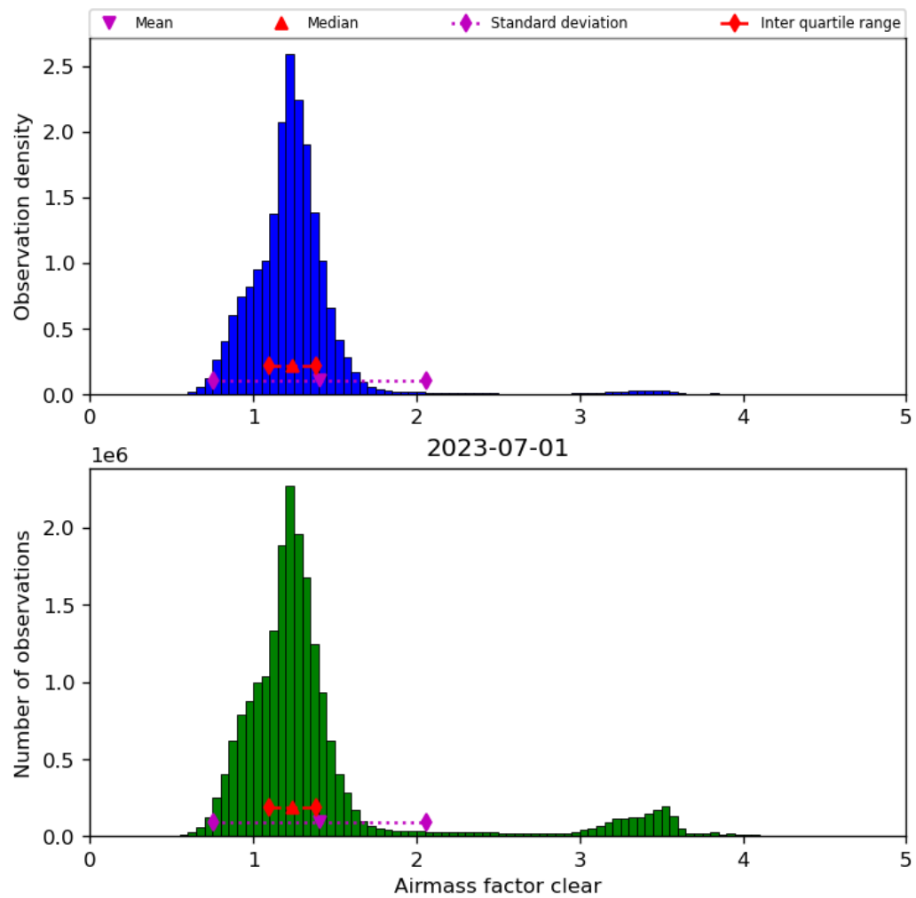
Figure 42: Histogram of “Airmass factor clear” for 2023-06-30 to 2023-07-02
