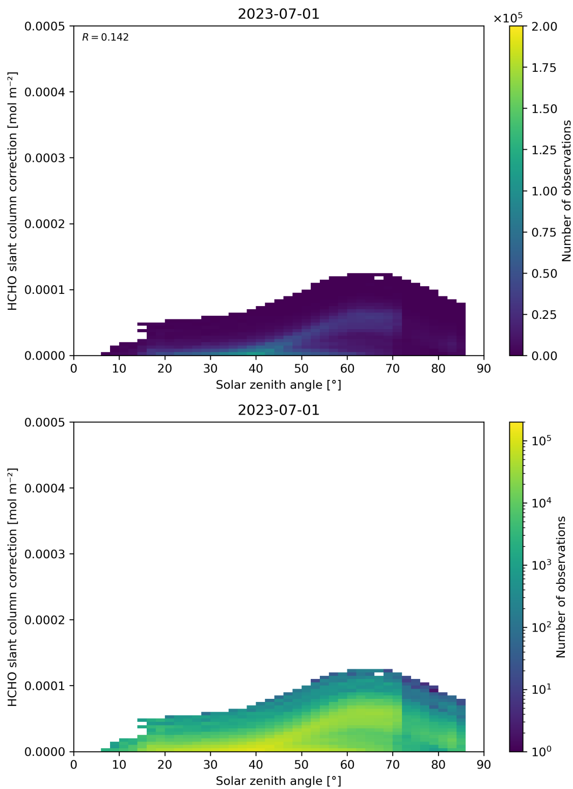
Figure 172: Scatter density plot of “Solar zenith angle” against “HCHO slant column correction” for 2023-06-30 to 2023-07-02.
