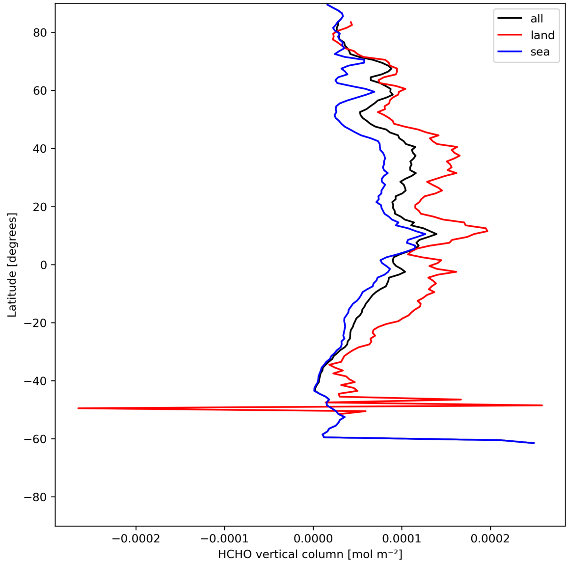
Figure 21: Zonal average of “HCHO vertical column” for 2023-06-30 to 2023-07-02.
