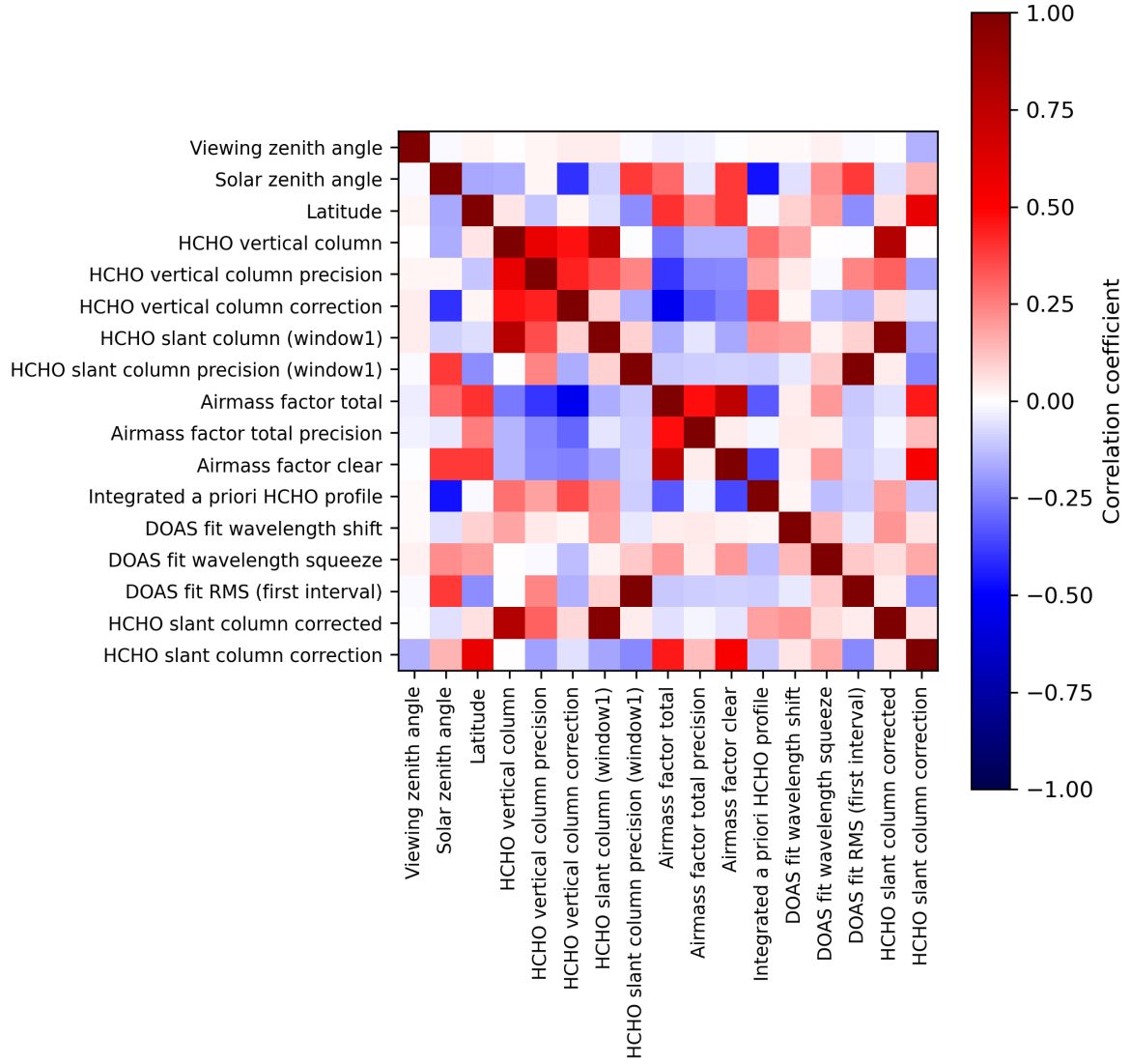
Figure 2: Map of correlation matrix for 2023-06-30 to 2023-07-02.
