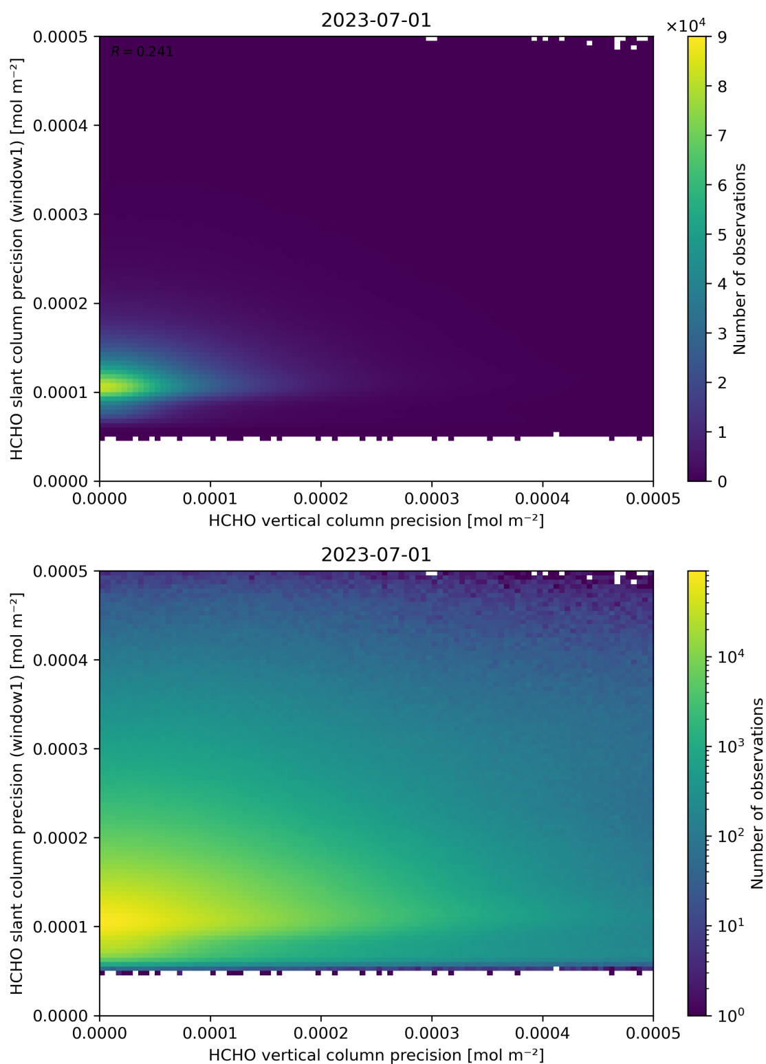
Figure 143: Scatter density plot of “HCHO vertical column precision” against “HCHO slant column precision (window1)” for 2023-06-30 to 2023-07-02.
