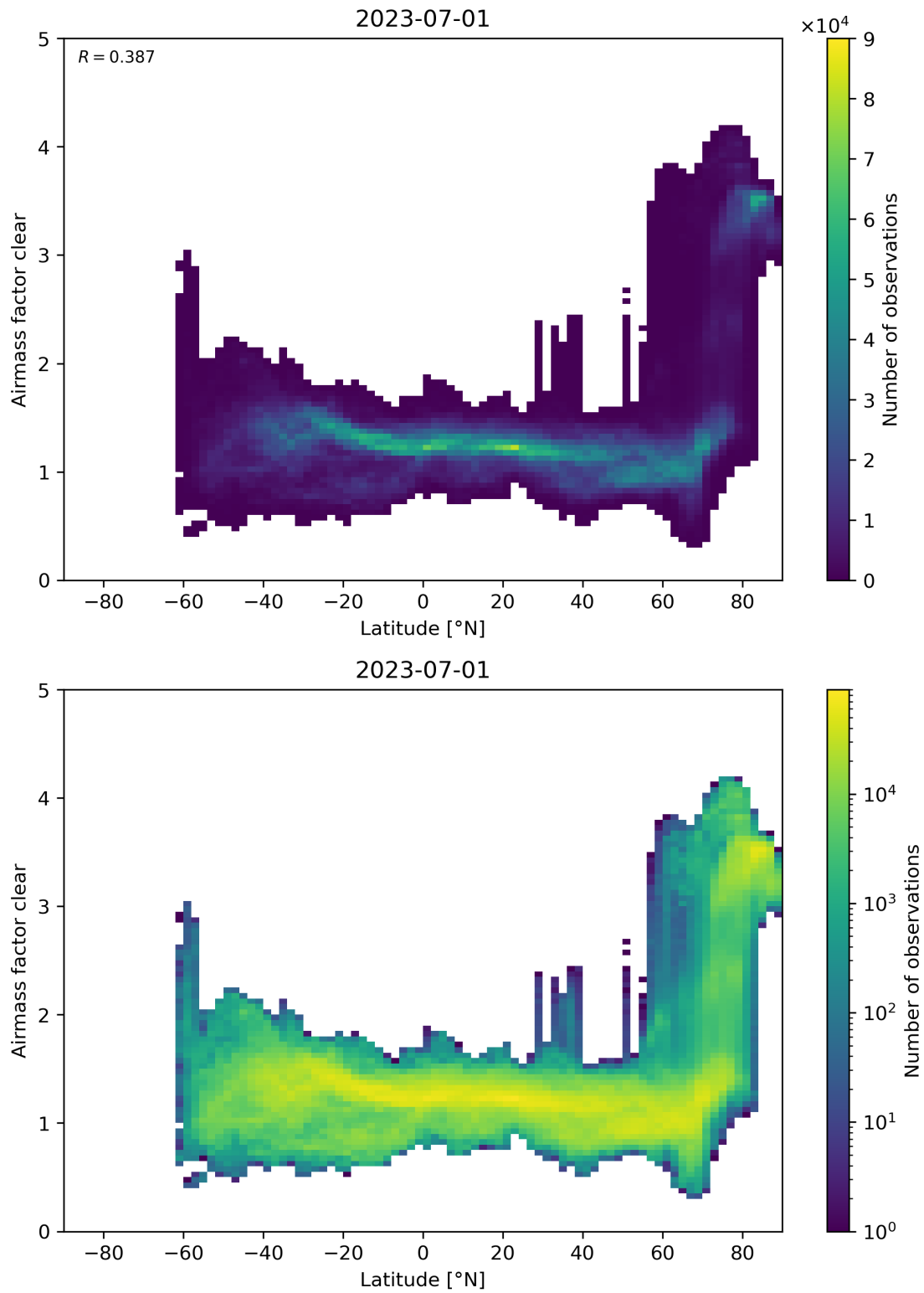
Figure 156: Scatter density plot of “Latitude” against “Airmass factor clear” for 2023-06-30 to 2023-07-02.
