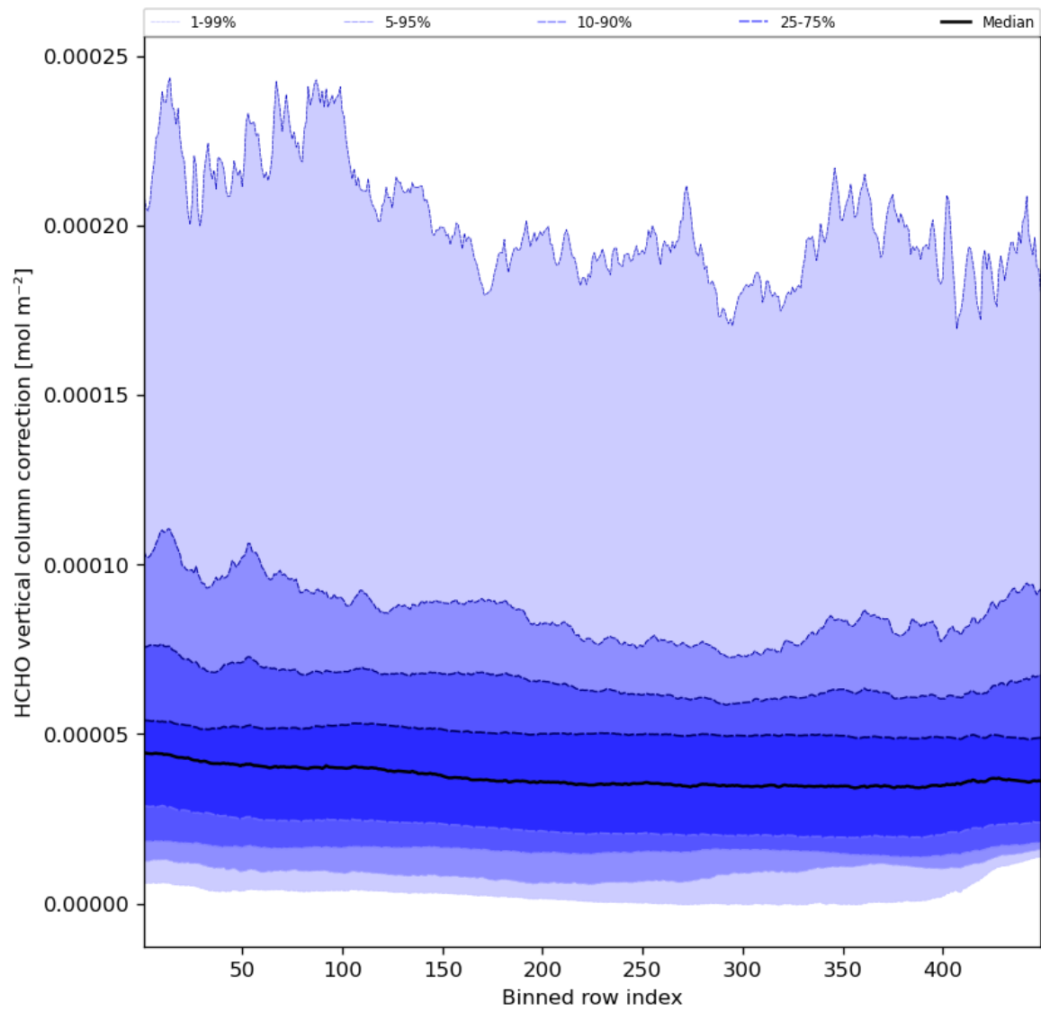
Figure 51: Along track statistics of “HCHO vertical column correction” for 2023-06-30 to 2023-07-02
