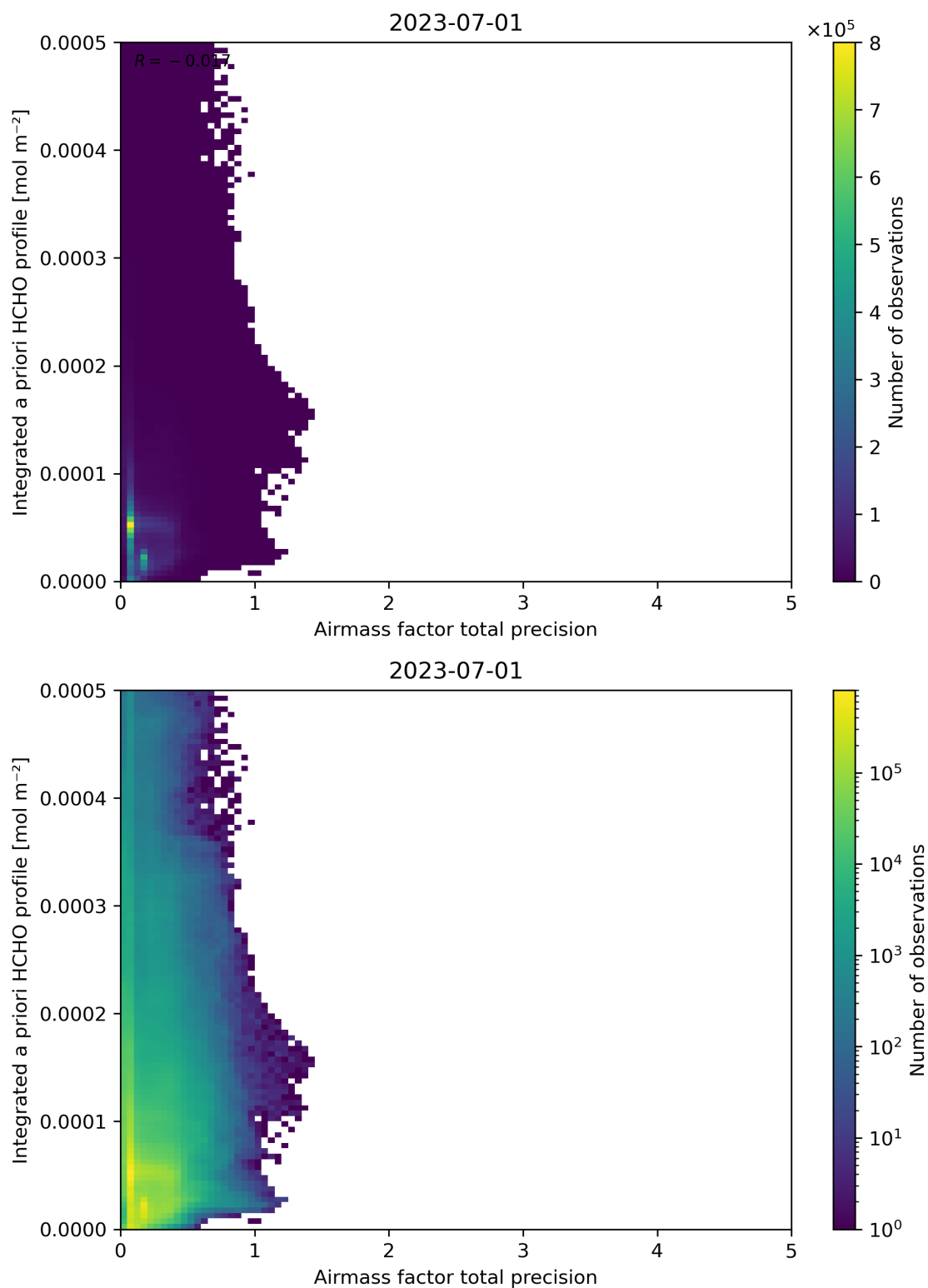
Figure 111: Scatter density plot of “Airmass factor total precision” against “Integrated a priori HCHO profile” for 2023-06-30 to 2023-07-02.
