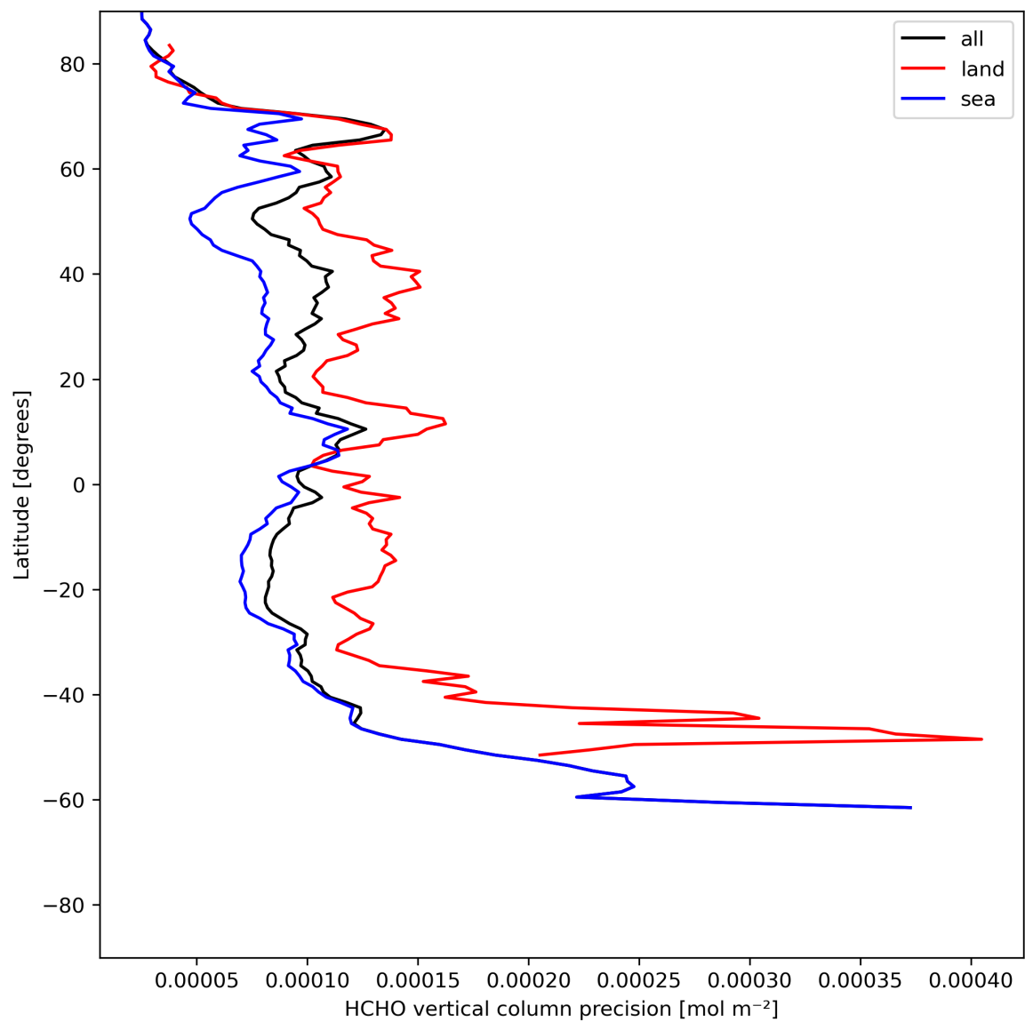
Figure 22: Zonal average of “HCHO vertical column precision” for 2023-06-30 to 2023-07-02.
