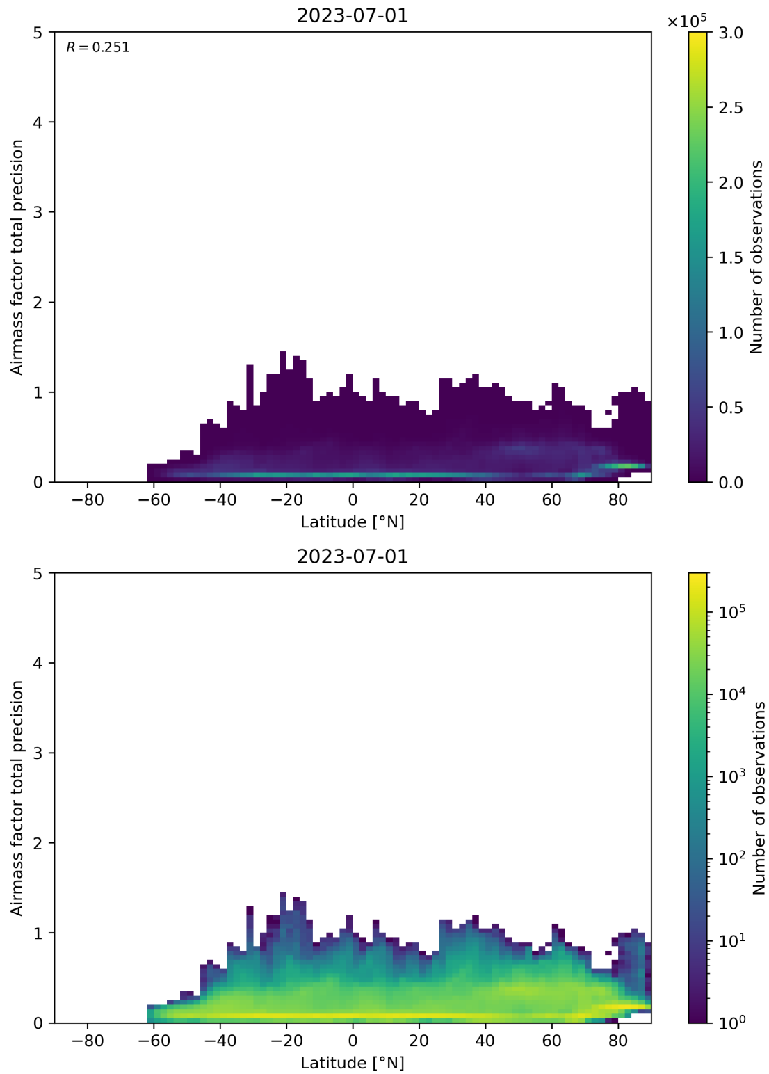
Figure 162: Scatter density plot of “Latitude” against “Airmass factor total precision” for 2023-06-30 to 2023-07-02.
