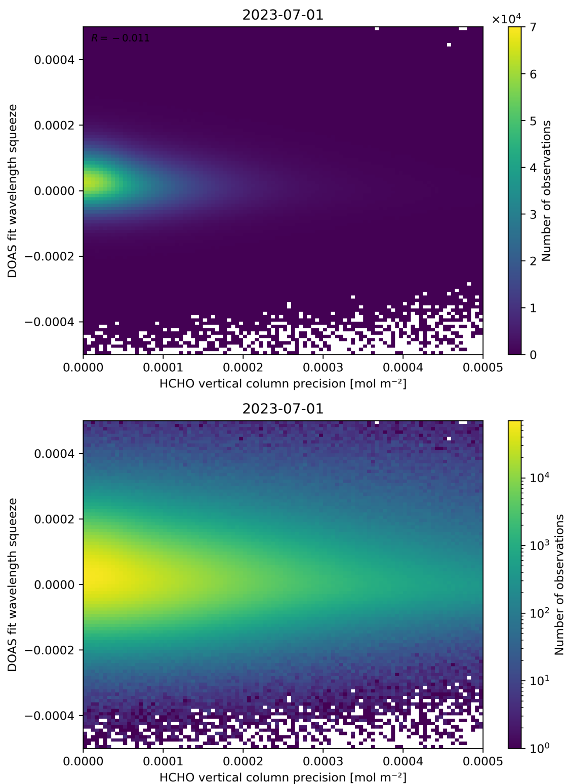
Figure 138: Scatter density plot of “HCHO vertical column precision” against “DOAS fit wavelength squeeze” for 2023-06-30 to 2023-07-02.
