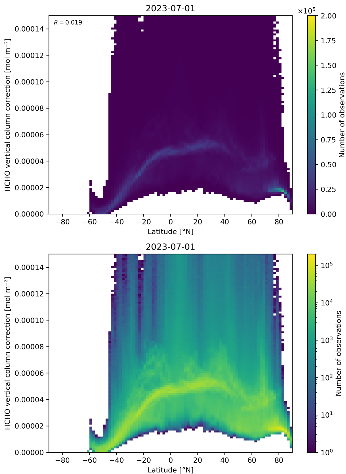
Figure 164: Scatter density plot of “Latitude” against “HCHO vertical column correction” for 2023-06-30 to 2023-07-02.
