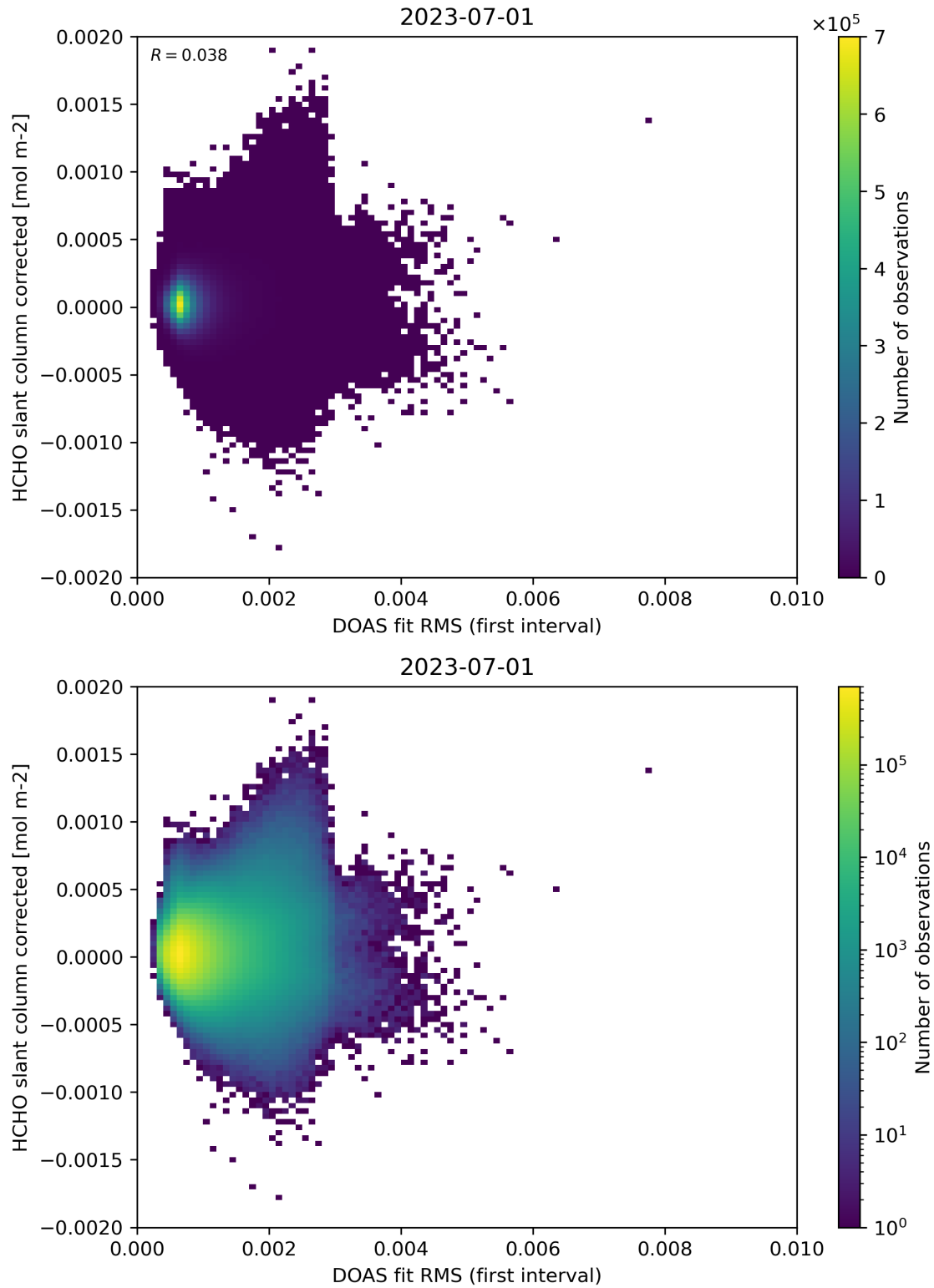
Figure 62: Scatter density plot of “DOAS fit RMS (first interval)” against “HCHO slant column corrected” for 2023-06-30 to 2023-07-02.
