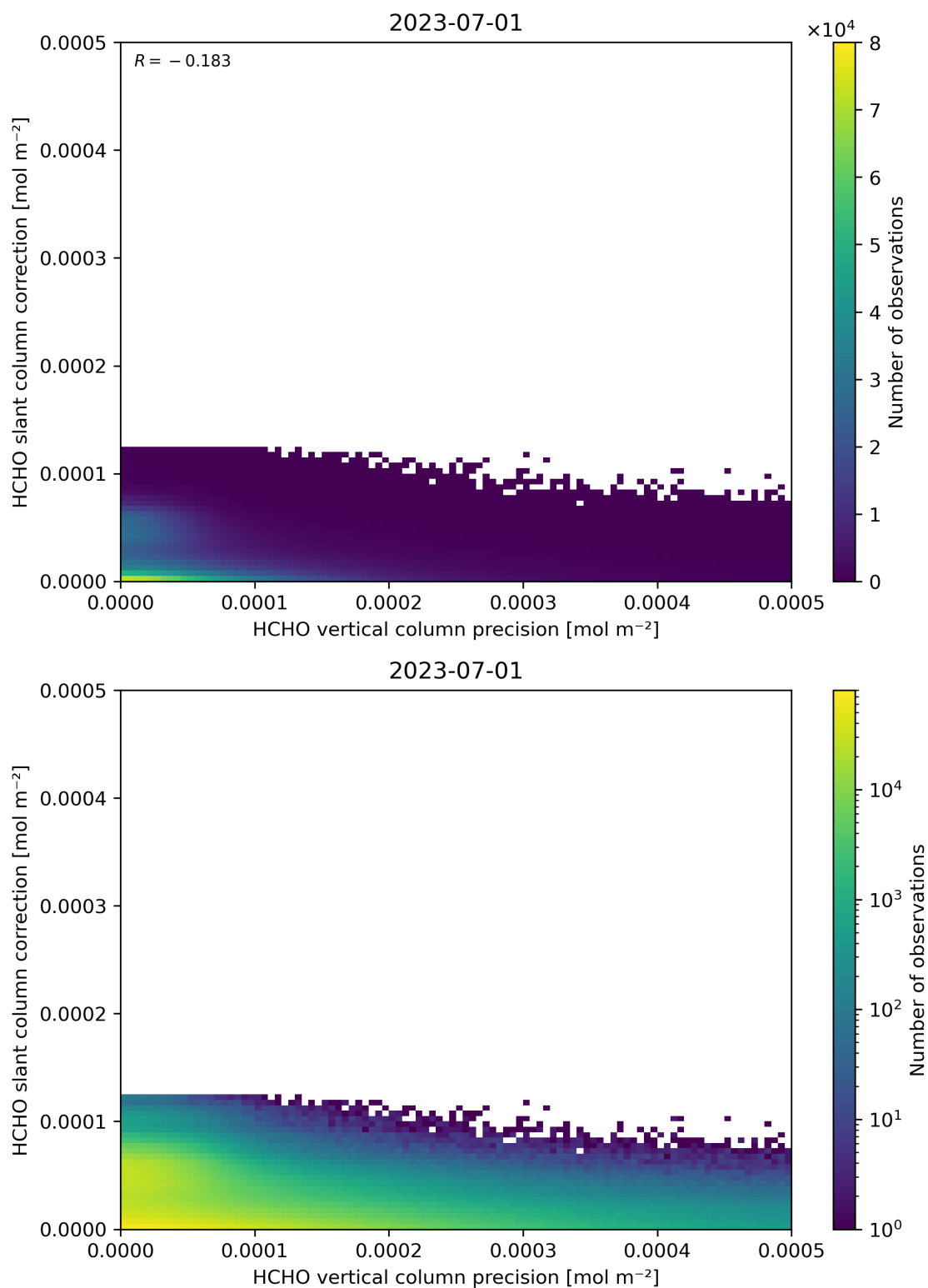
Figure 141: Scatter density plot of “HCHO vertical column precision” against “HCHO slant column correction” for 2023-06-30 to 2023-07-02.
