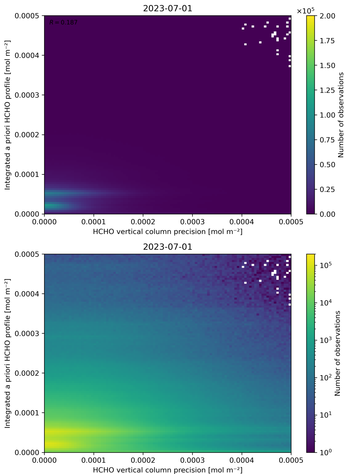
Figure 147: Scatter density plot of “HCHO vertical column precision” against “Integrated a priori HCHO profile” for 2023-06-30 to 2023-07-02.
