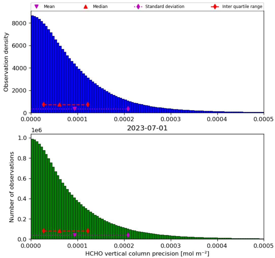
Figure 36: Histogram of “HCHO vertical column precision” for 2023-06-30 to 2023-07-02
