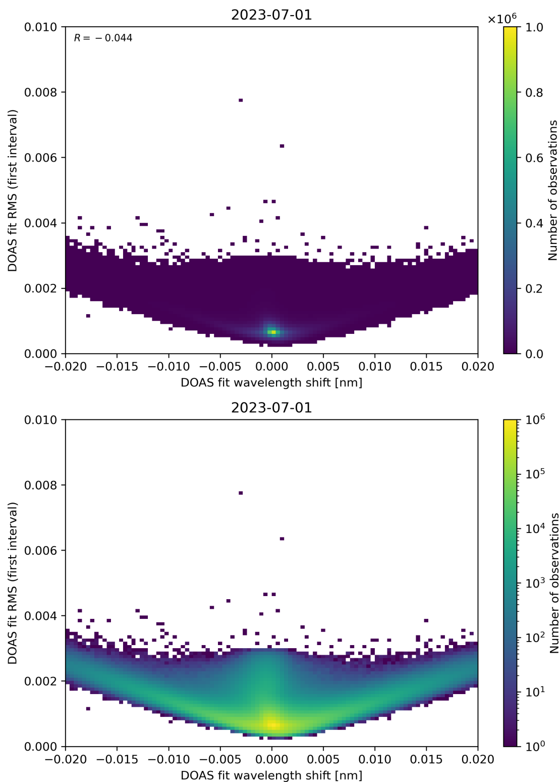
Figure 64: Scatter density plot of “DOAS fit wavelength shift” against “DOAS fit RMS (first interval)” for 2023-06-30 to 2023-07-02.
