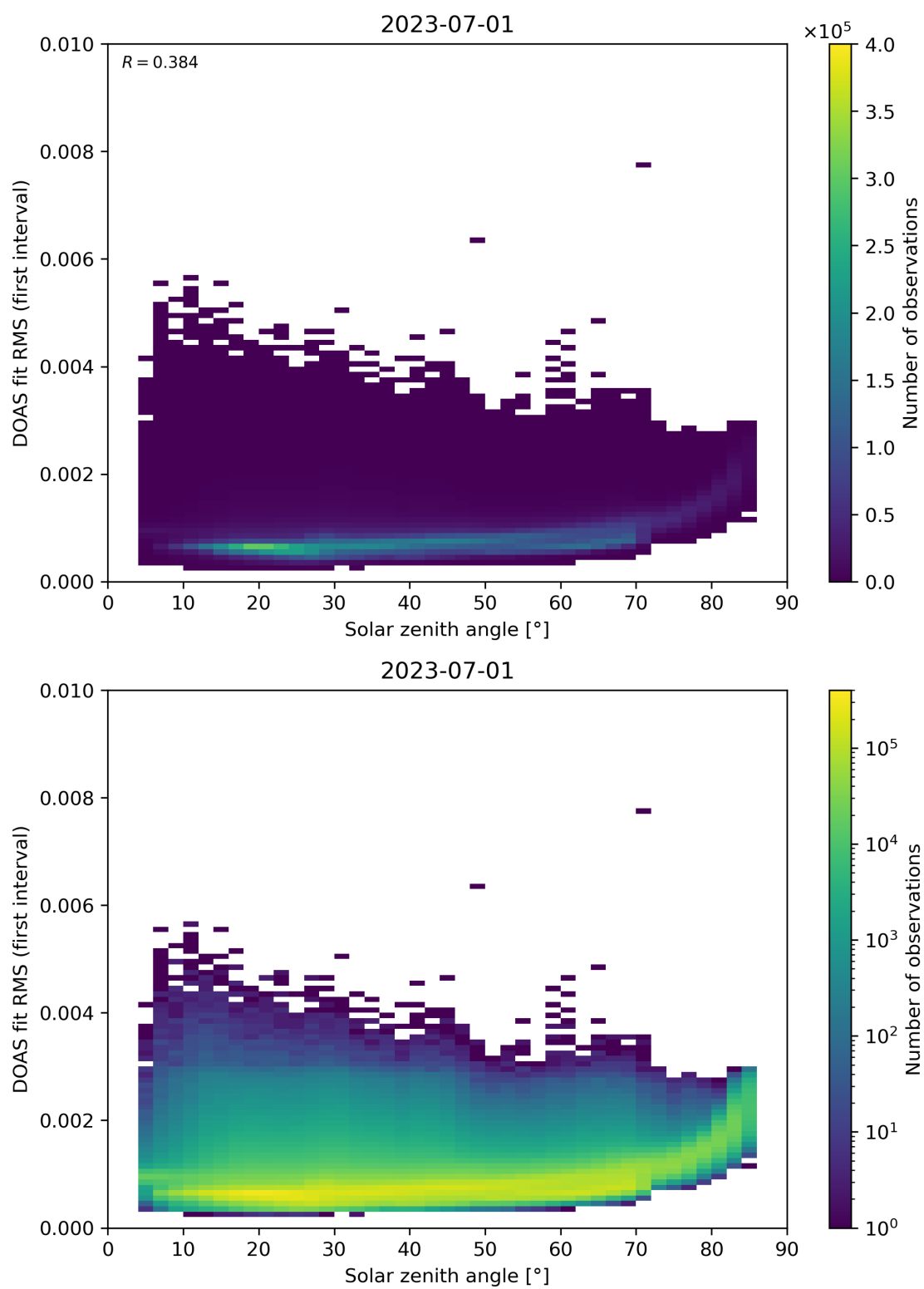
Figure 167: Scatter density plot of “Solar zenith angle” against “DOAS fit RMS (first interval)” for 2023-06-30 to 2023-07-02.
