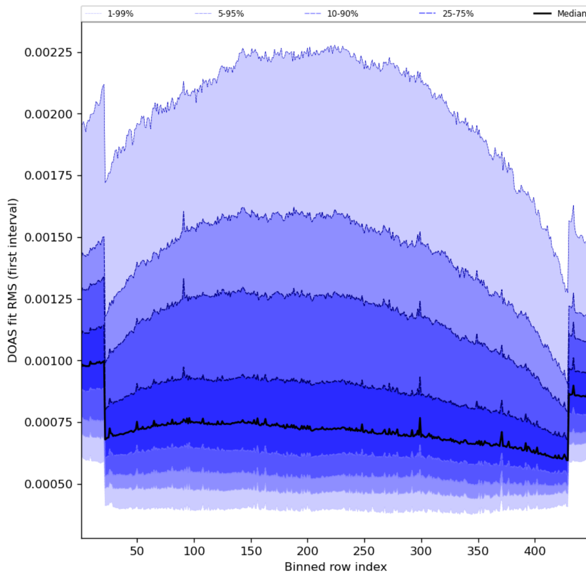
Figure 60: Along track statistics of “DOAS fit RMS (first interval)” for 2023-06-30 to 2023-07-02
