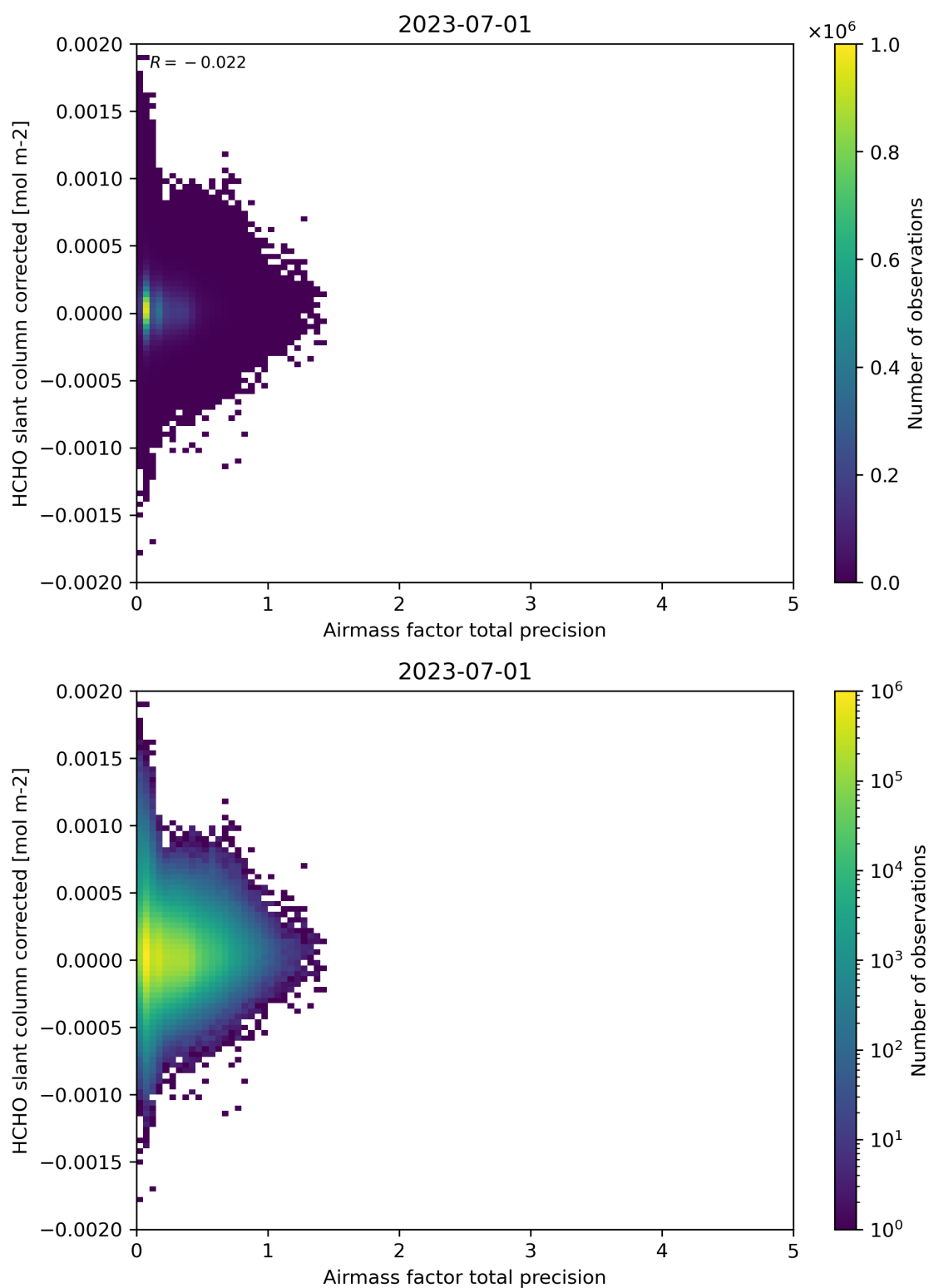
Figure 109: Scatter density plot of “Airmass factor total precision” against “HCHO slant column corrected” for 2023-06-30 to 2023-07-02.
