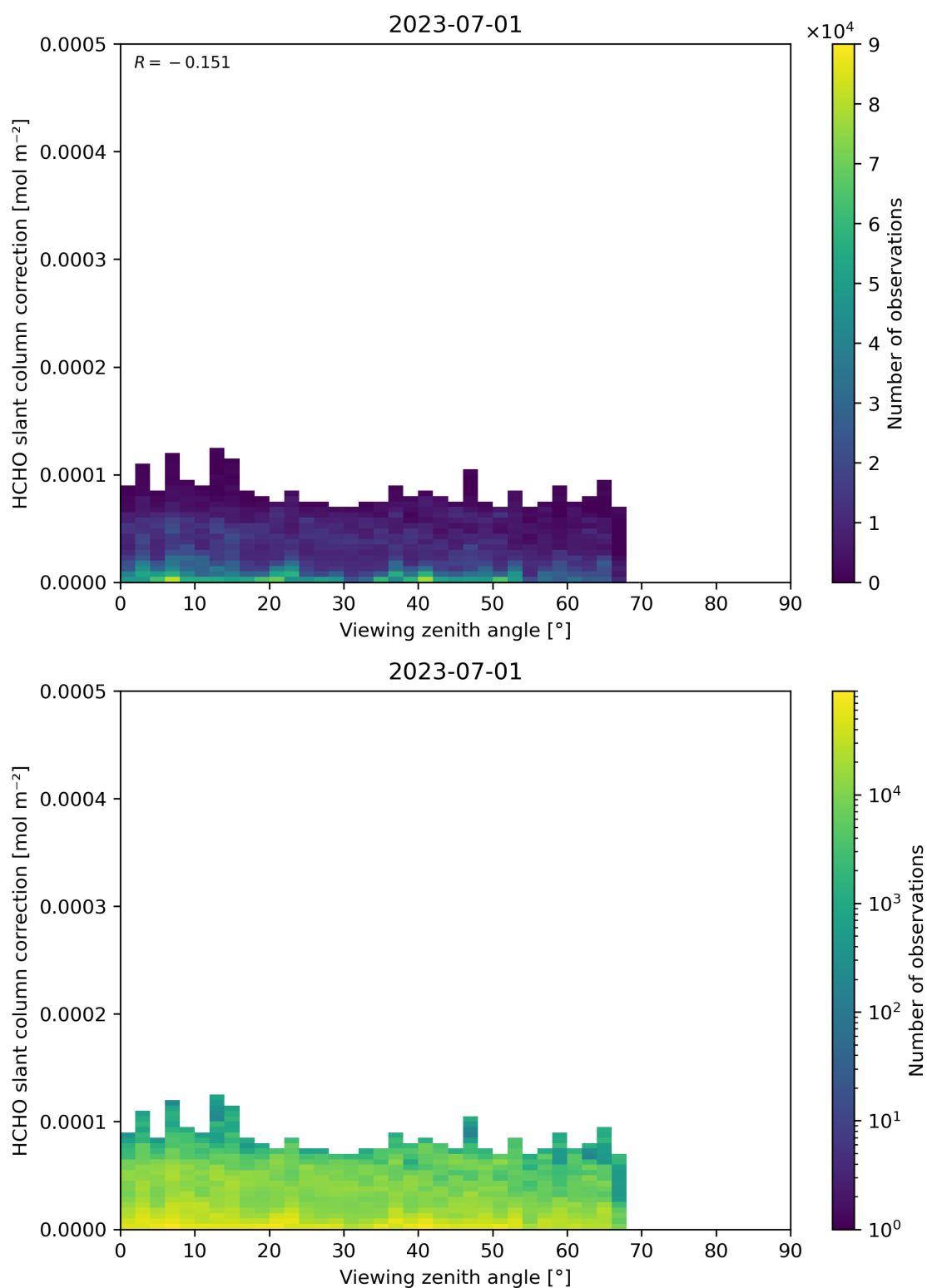
Figure 187: Scatter density plot of “Viewing zenith angle” against “HCHO slant column correction” for 2023-06-30 to 2023-07-02.
