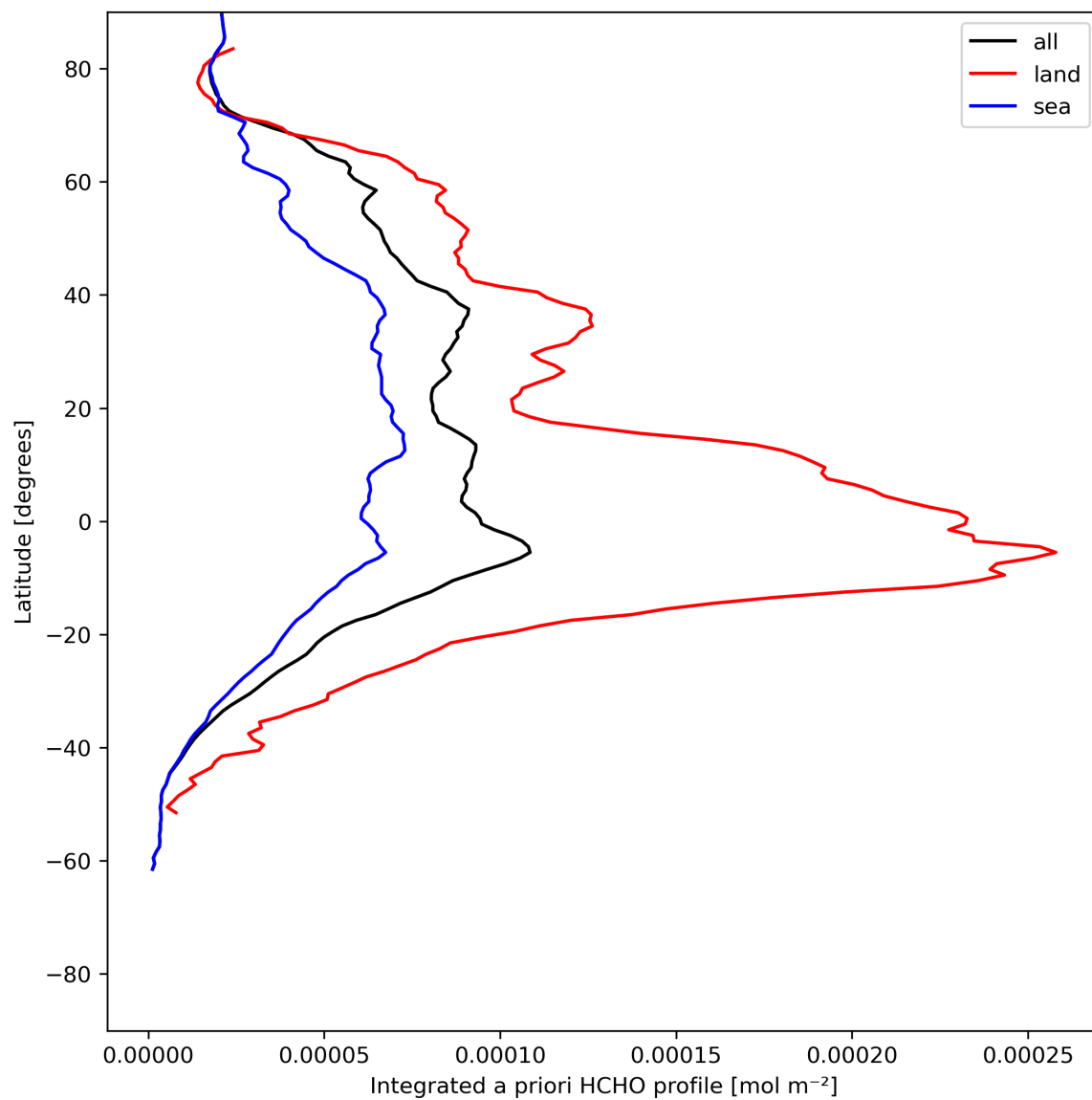
Figure 29: Zonal average of “Integrated a priori HCHO profile” for 2023-06-30 to 2023-07-02.
