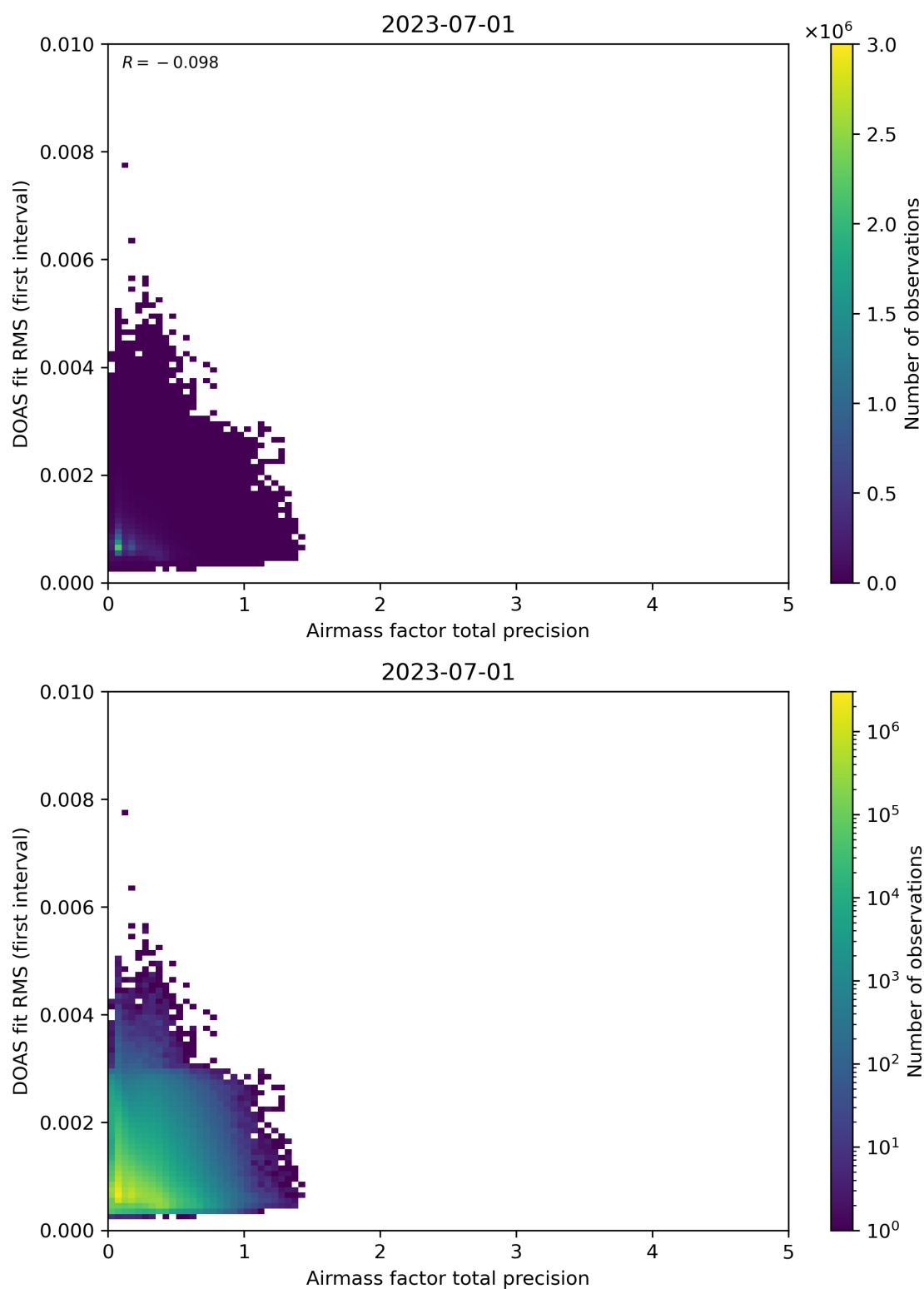
Figure 105: Scatter density plot of “Airmass factor total precision” against “DOAS fit RMS (first interval)” for 2023-06-30 to 2023-07-02.
