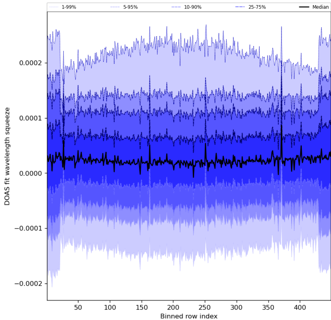
Figure 59: Along track statistics of “DOAS fit wavelength squeeze” for 2023-06-30 to 2023-07-02
