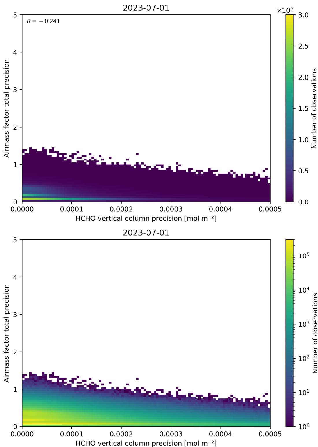
Figure 145: Scatter density plot of “HCHO vertical column precision” against “Airmass factor total precision” for 2023-06-30 to 2023-07-02.
