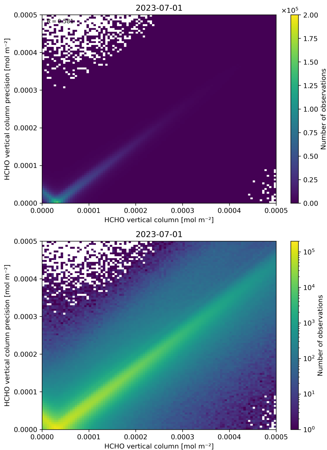
Figure 134: Scatter density plot of “HCHO vertical column” against “HCHO vertical column precision” for 2023-06-30 to 2023-07-02.
