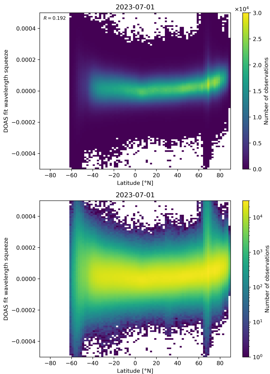
Figure 155: Scatter density plot of “Latitude” against “DOAS fit wavelength squeeze” for 2023-06-30 to 2023-07-02.
