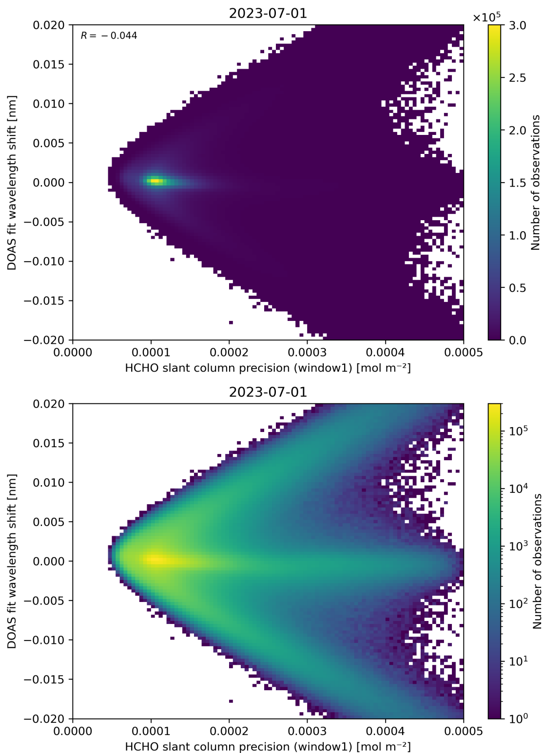
Figure 89: Scatter density plot of “HCHO slant column precision (window1)” against “DOAS fit wavelength shift” for 2023-06-30 to 2023-07-02.
