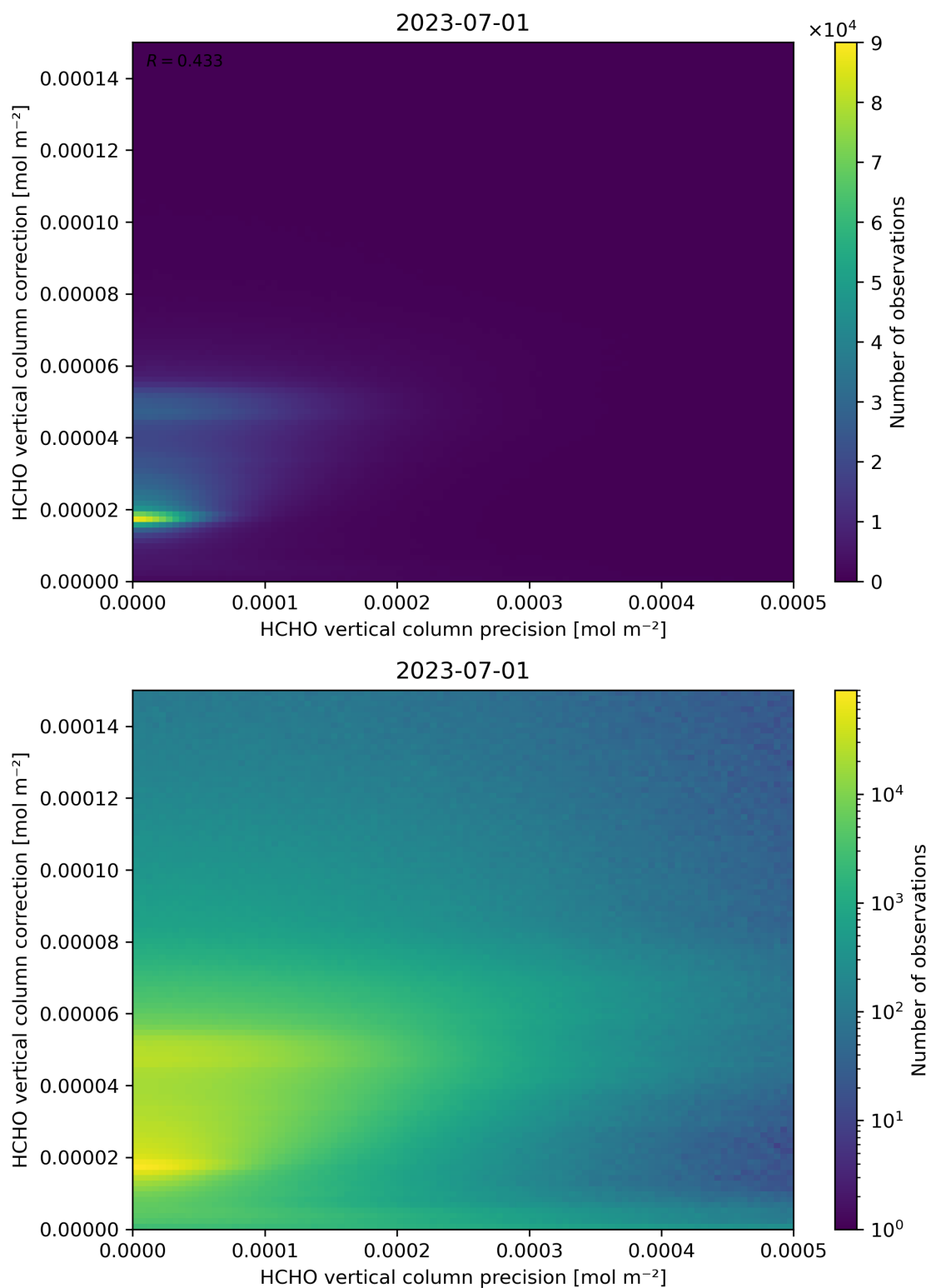
Figure 146: Scatter density plot of “HCHO vertical column precision” against “HCHO vertical column correction” for 2023-06-30 to 2023-07-02.
