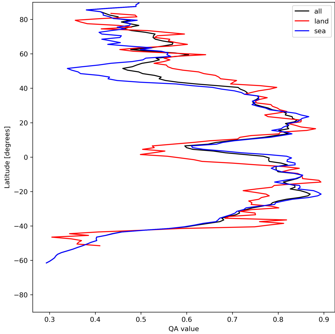
Figure 20: Zonal average of “QA value” for 2023-06-30 to 2023-07-02.
