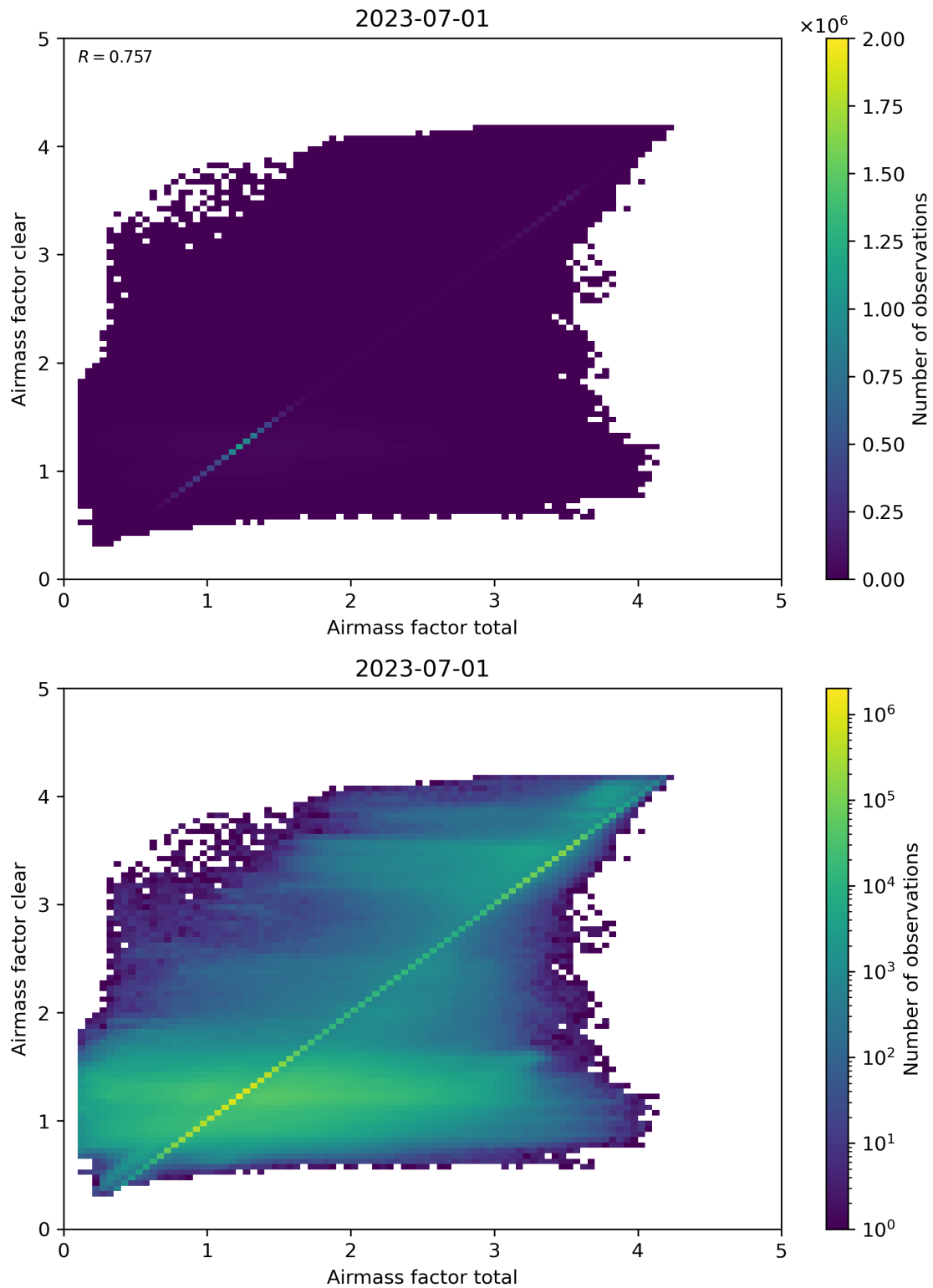
Figure 100: Scatter density plot of “Airmass factor total” against “Airmass factor clear” for 2023-06-30 to 2023-07-02.
