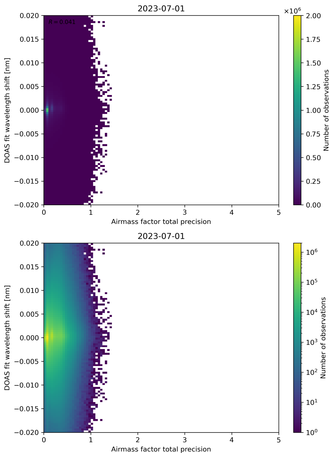
Figure 106: Scatter density plot of “Airmass factor total precision” against “DOAS fit wavelength shift” for 2023-06-30 to 2023-07-02.
