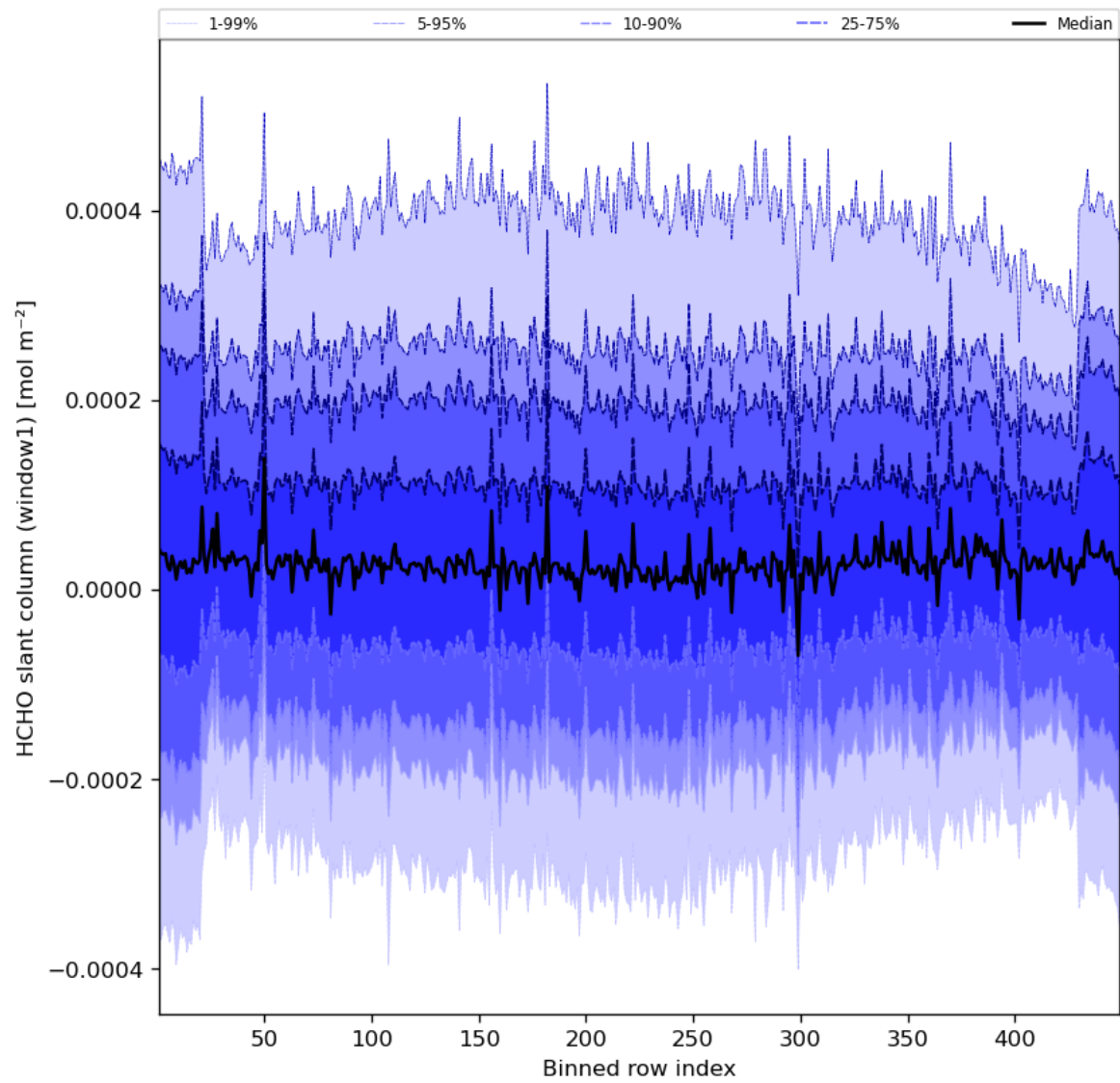
Figure 52: Along track statistics of “HCHO slant column (window1)” for 2023-06-30 to 2023-07-02
