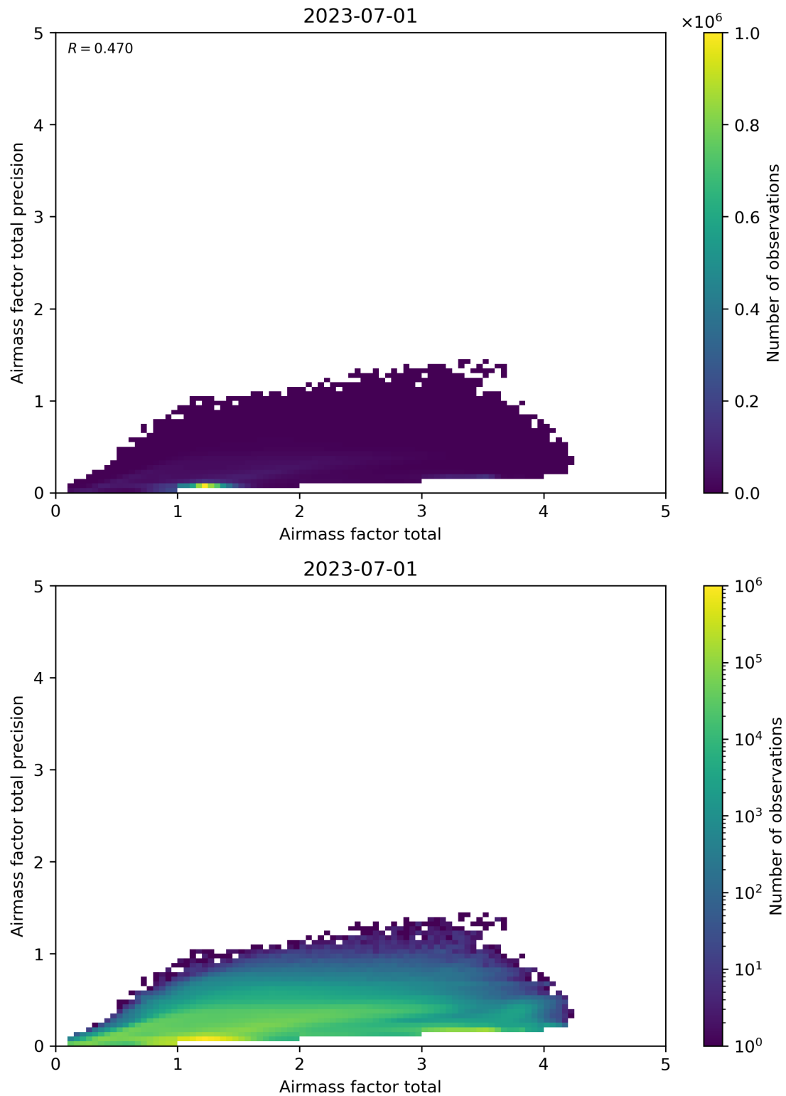
Figure 103: Scatter density plot of “Airmass factor total” against “Airmass factor total precision” for 2023-06-30 to 2023-07-02.
