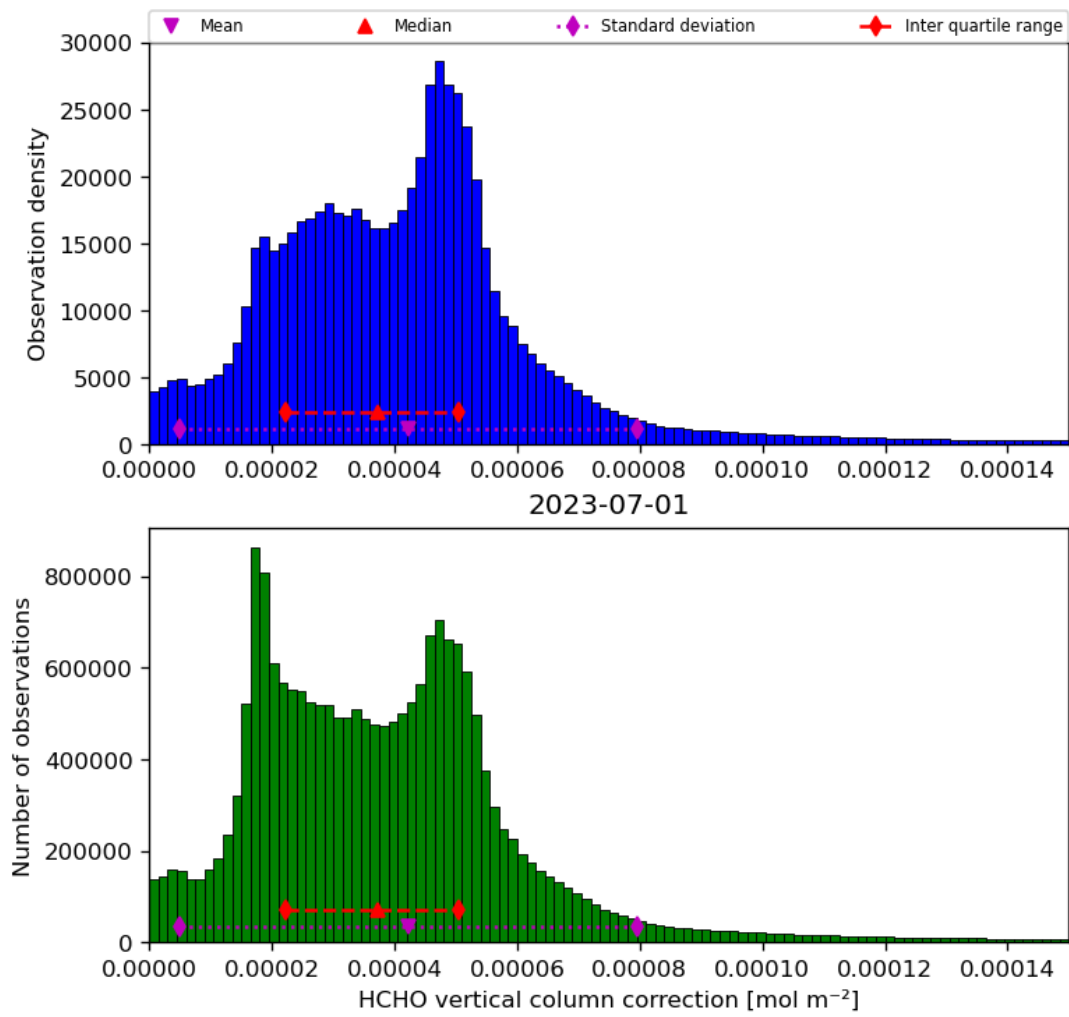
Figure 37: Histogram of “HCHO vertical column correction” for 2023-06-30 to 2023-07-02
