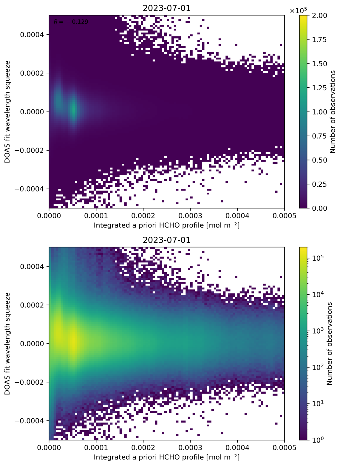
Figure 150: Scatter density plot of “Integrated a priori HCHO profile” against “DOAS fit wavelength squeeze” for 2023-06-30 to 2023-07-02.
