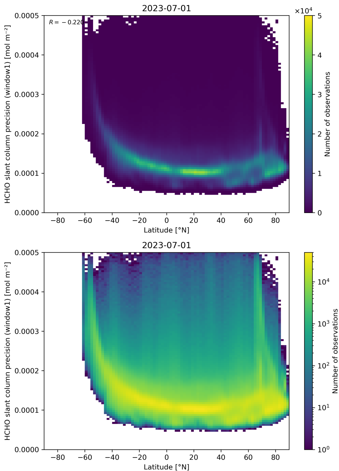
Figure 160: Scatter density plot of “Latitude” against “HCHO slant column precision (window1)” for 2023-06-30 to 2023-07-02.
