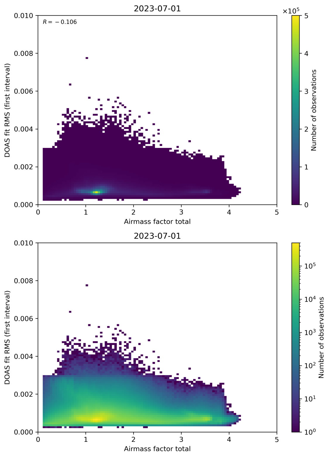
Figure 97: Scatter density plot of “Airmass factor total” against “DOAS fit RMS (first interval)” for 2023-06-30 to 2023-07-02.
