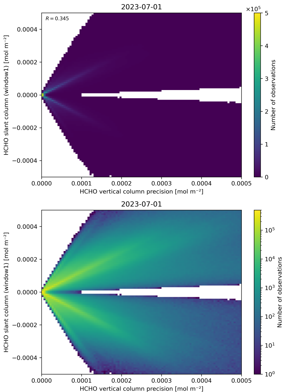
Figure 142: Scatter density plot of “HCHO vertical column precision” against “HCHO slant column (window1)” for 2023-06-30 to 2023-07-02.
