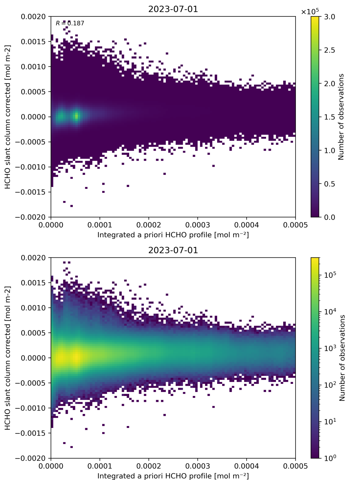
Figure 151: Scatter density plot of “Integrated a priori HCHO profile” against “HCHO slant column corrected” for 2023-06-30 to 2023-07-02.
