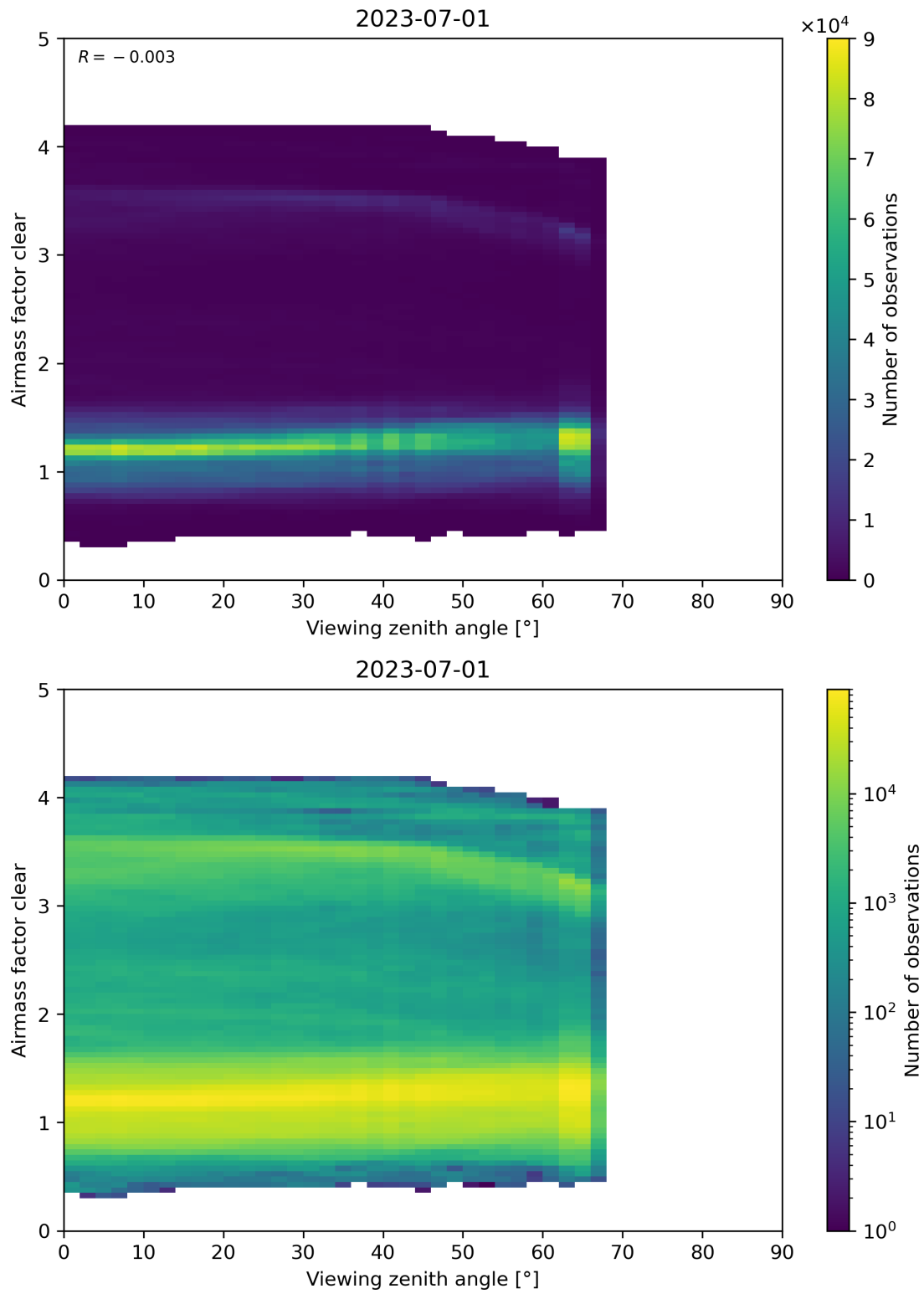
Figure 185: Scatter density plot of “Viewing zenith angle” against “Airmass factor clear” for 2023-06-30 to 2023-07-02.
