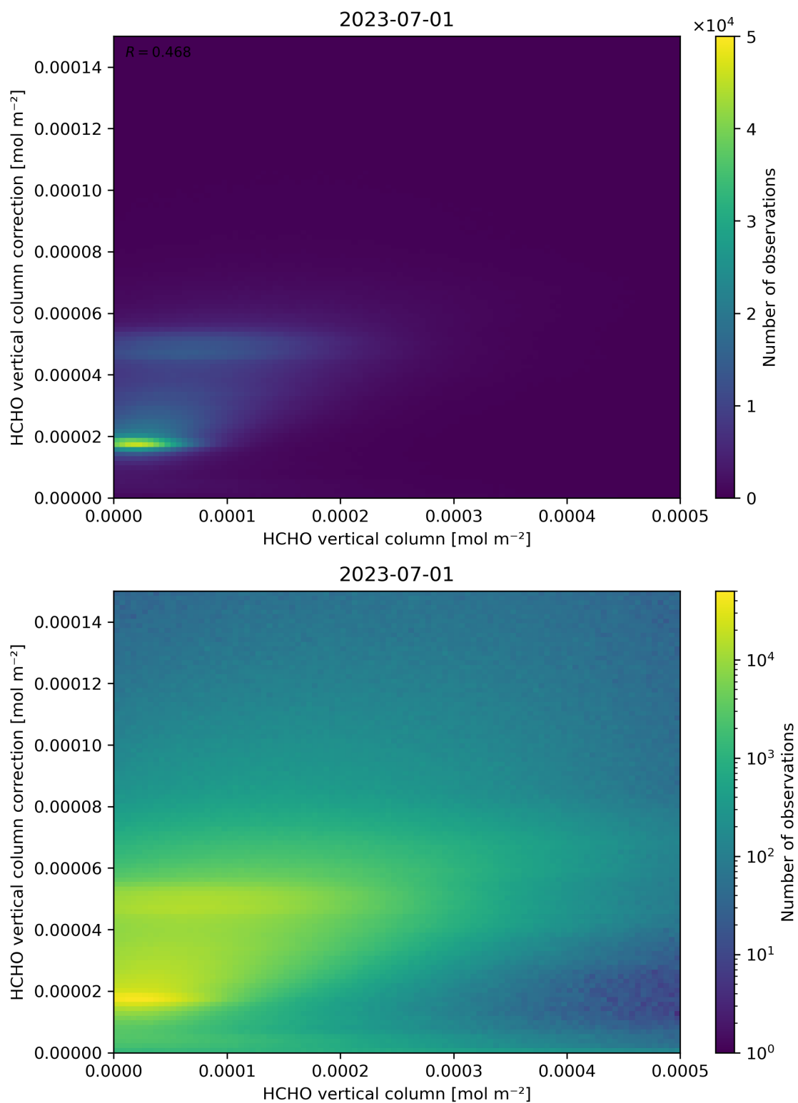
Figure 133: Scatter density plot of “HCHO vertical column” against “HCHO vertical column correction” for 2023-06-30 to 2023-07-02.
