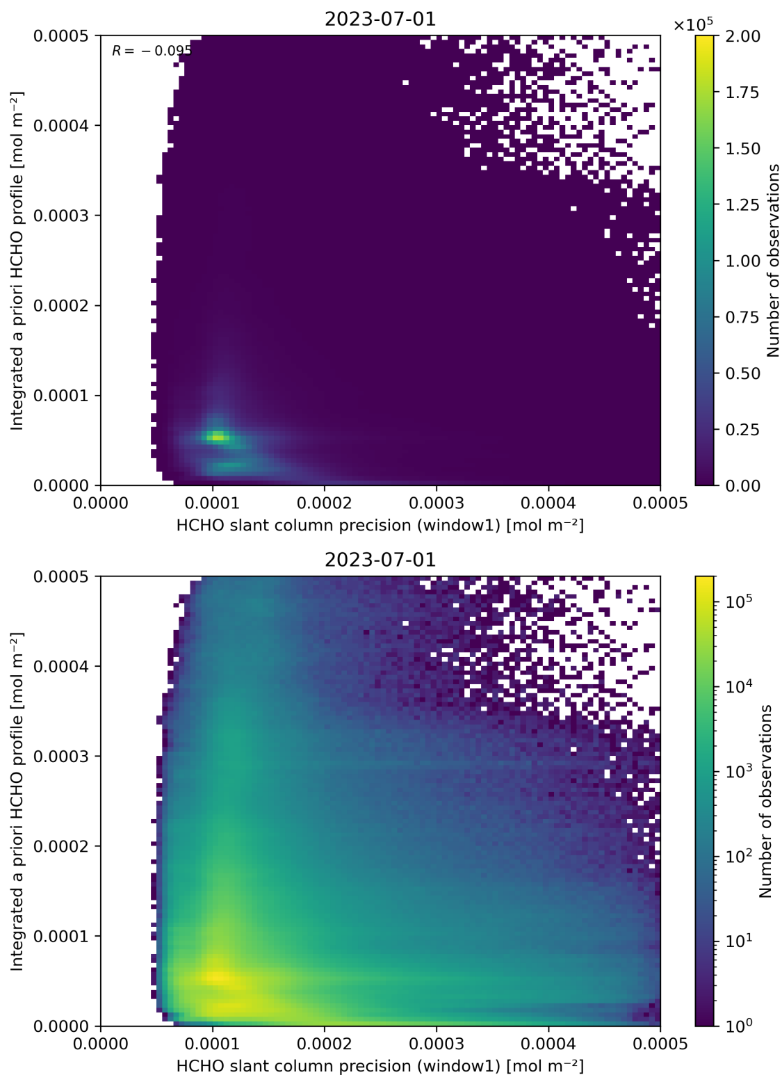
Figure 96: Scatter density plot of “HCHO slant column precision (window1)” against “Integrated a priori HCHO profile” for 2023-06-30 to 2023-07-02.
