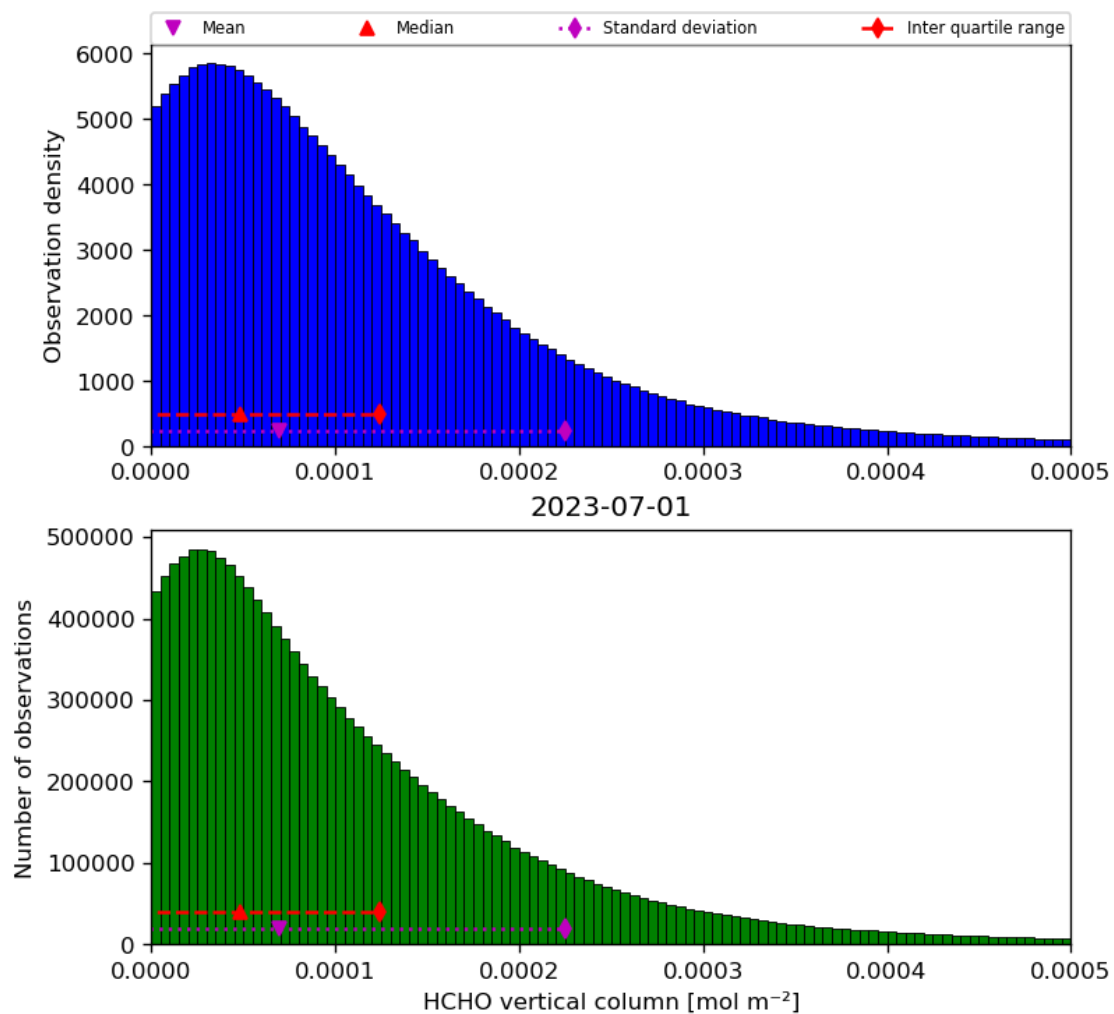
Figure 35: Histogram of “HCHO vertical column” for 2023-06-30 to 2023-07-02
