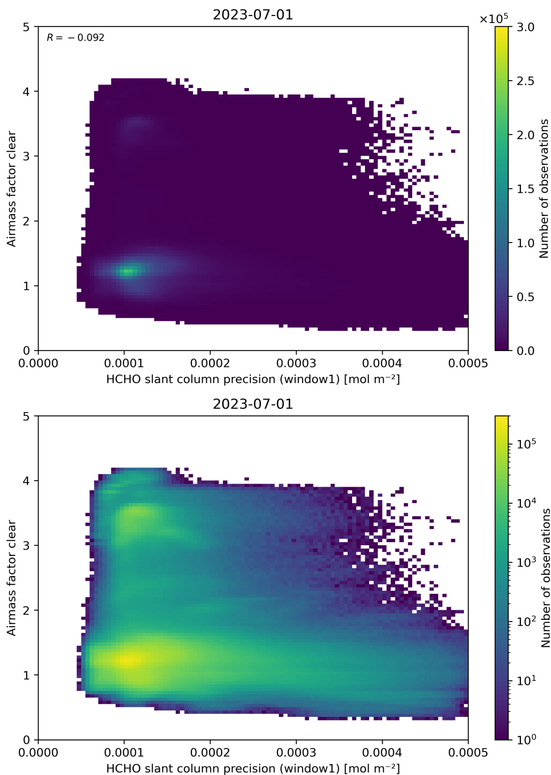
Figure 91: Scatter density plot of “HCHO slant column precision (window1)” against “Airmass factor clear” for 2023-06-30 to 2023-07-02.
