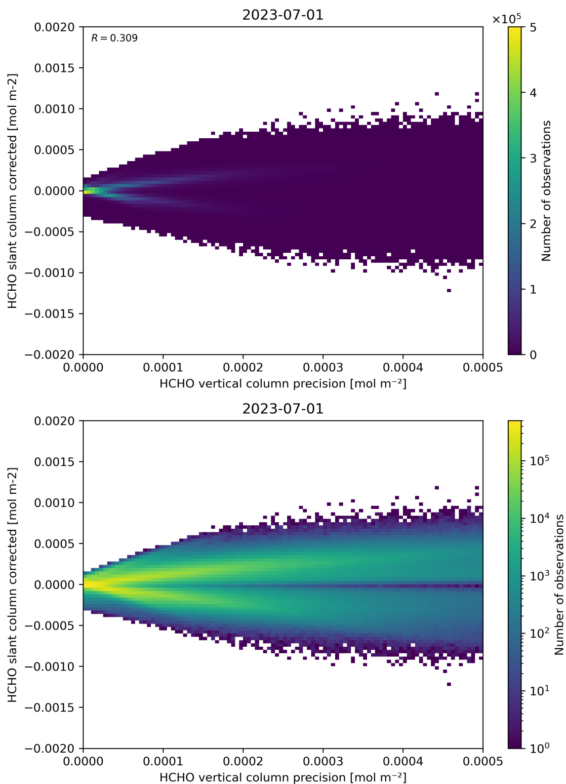
Figure 140: Scatter density plot of “HCHO vertical column precision” against “HCHO slant column corrected” for 2023-06-30 to 2023-07-02.
