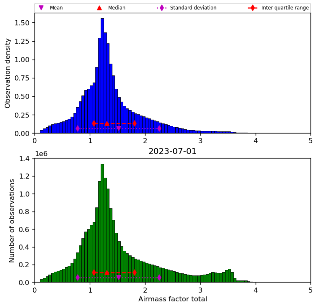
Figure 40: Histogram of “Airmass factor total” for 2023-06-30 to 2023-07-02
