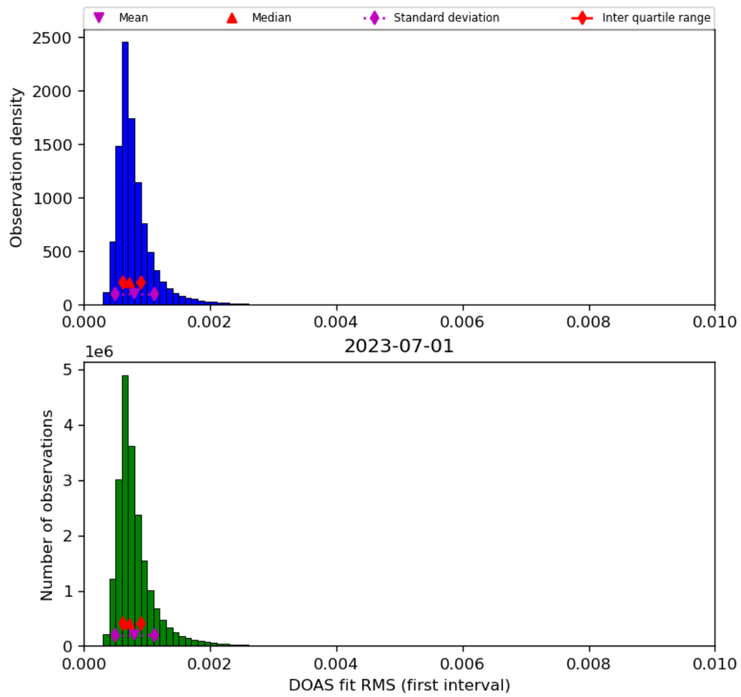
Figure 46: Histogram of “DOAS fit RMS (first interval)” for 2023-06-30 to 2023-07-02
