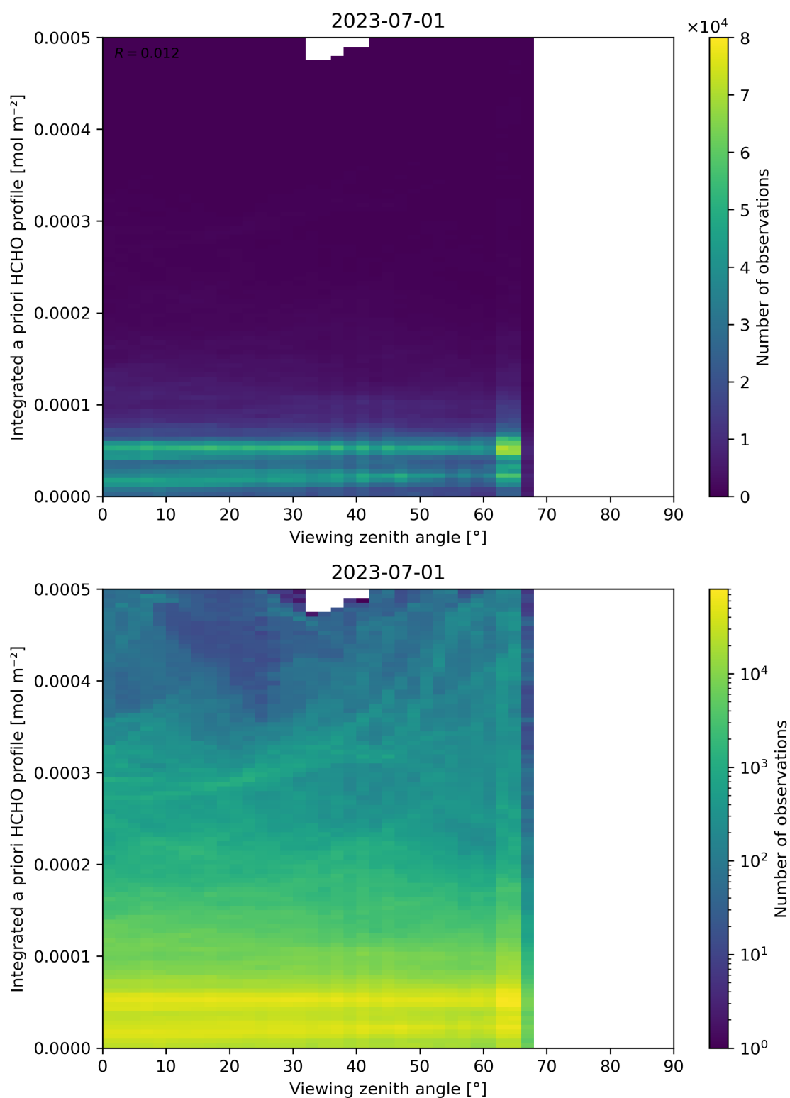
Figure 195: Scatter density plot of “Viewing zenith angle” against “Integrated a priori HCHO profile” for 2023-06-30 to 2023-07-02.
