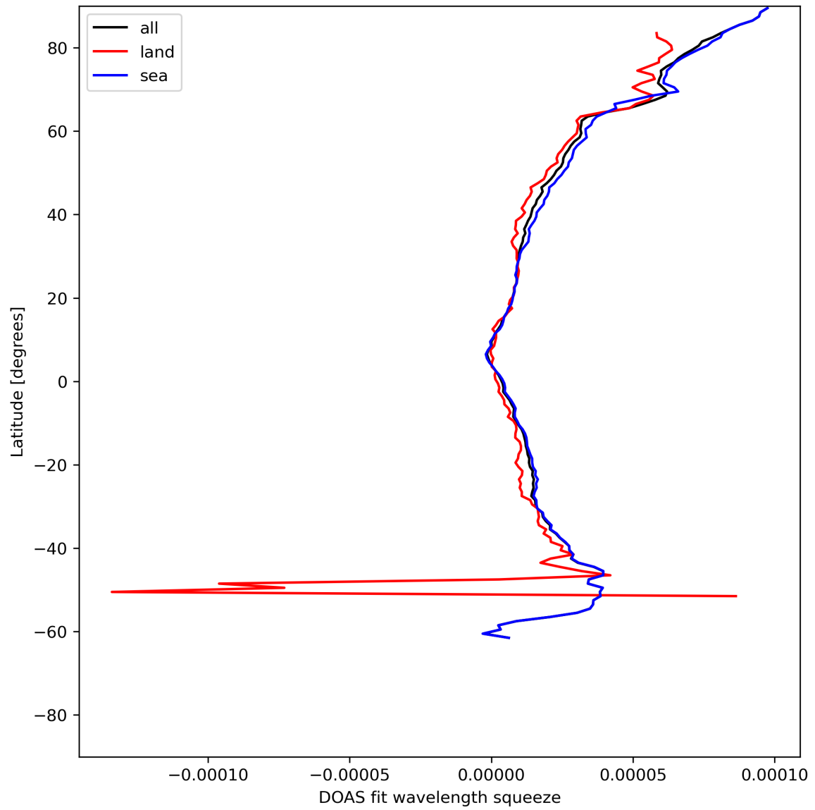
Figure 31: Zonal average of “DOAS fit wavelength squeeze” for 2023-06-30 to 2023-07-02.
