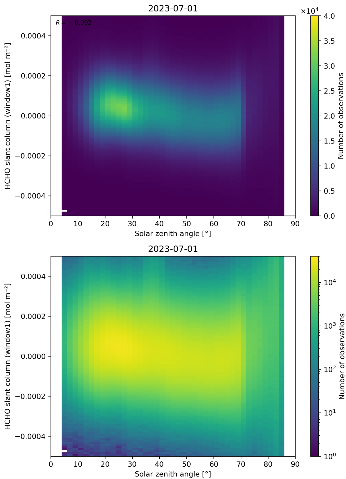
Figure 173: Scatter density plot of “Solar zenith angle” against “HCHO slant column (window1)” for 2023-06-30 to 2023-07-02.
