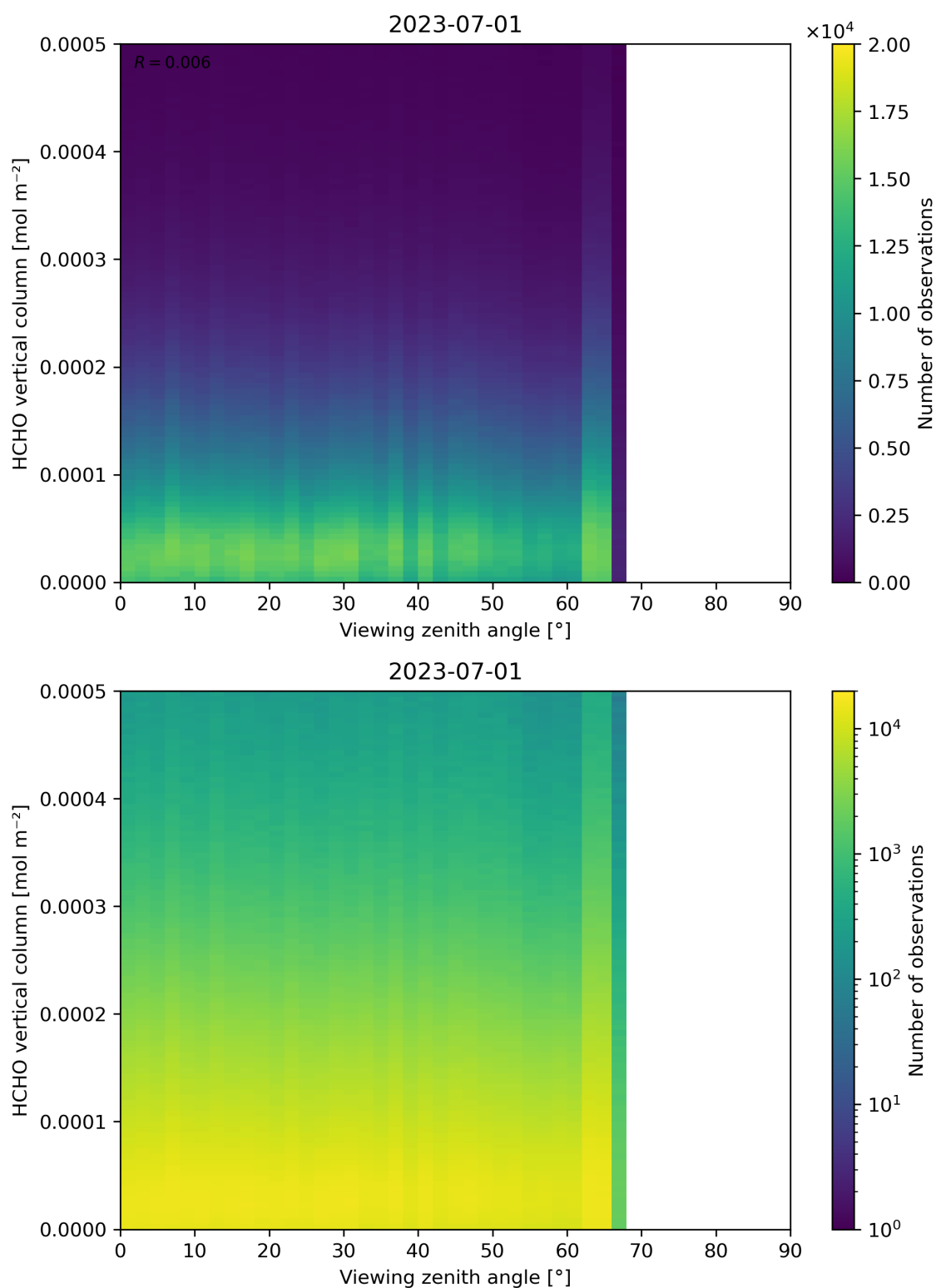
Figure 192: Scatter density plot of “Viewing zenith angle” against “HCHO vertical column” for 2023-06-30 to 2023-07-02.
