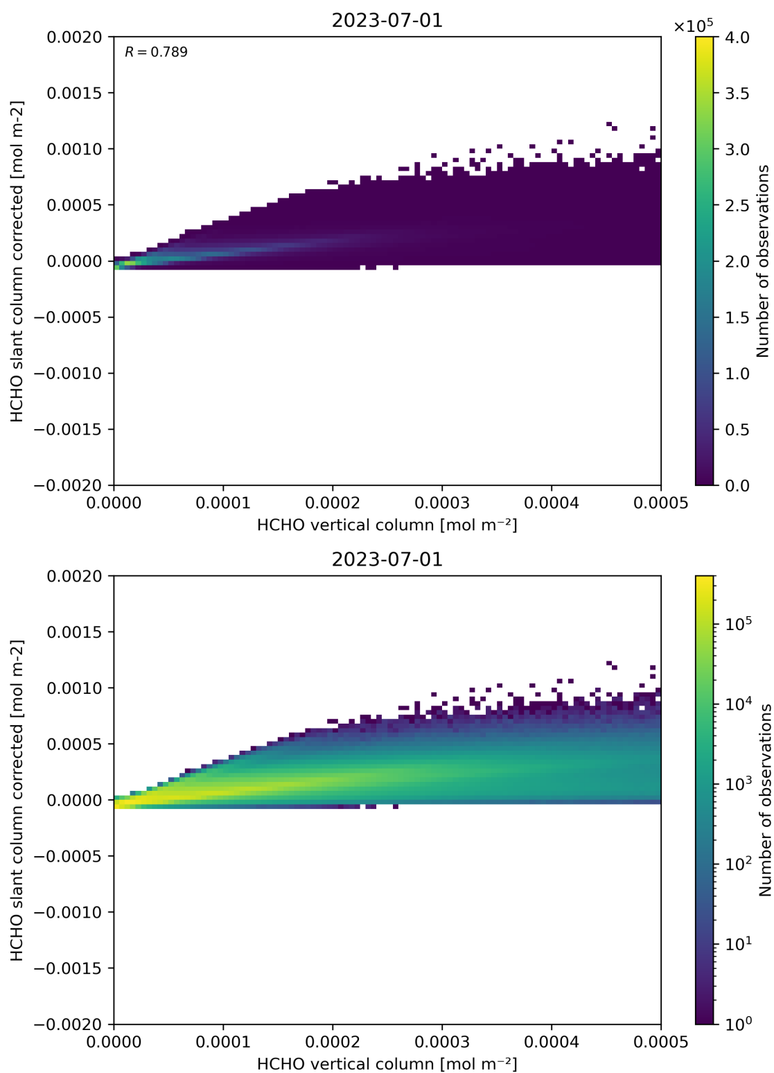
Figure 127: Scatter density plot of “HCHO vertical column” against “HCHO slant column corrected” for 2023-06-30 to 2023-07-02.
