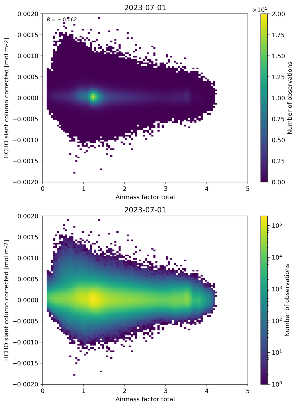
Figure 101: Scatter density plot of “Airmass factor total” against “HCHO slant column corrected” for 2023-06-30 to 2023-07-02.
