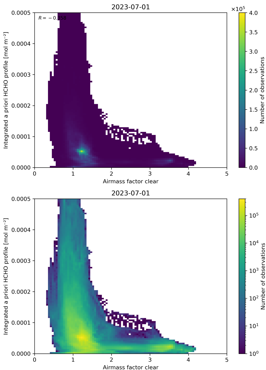
Figure 76: Scatter density plot of “Airmass factor clear” against “Integrated a priori HCHO profile” for 2023-06-30 to 2023-07-02.
