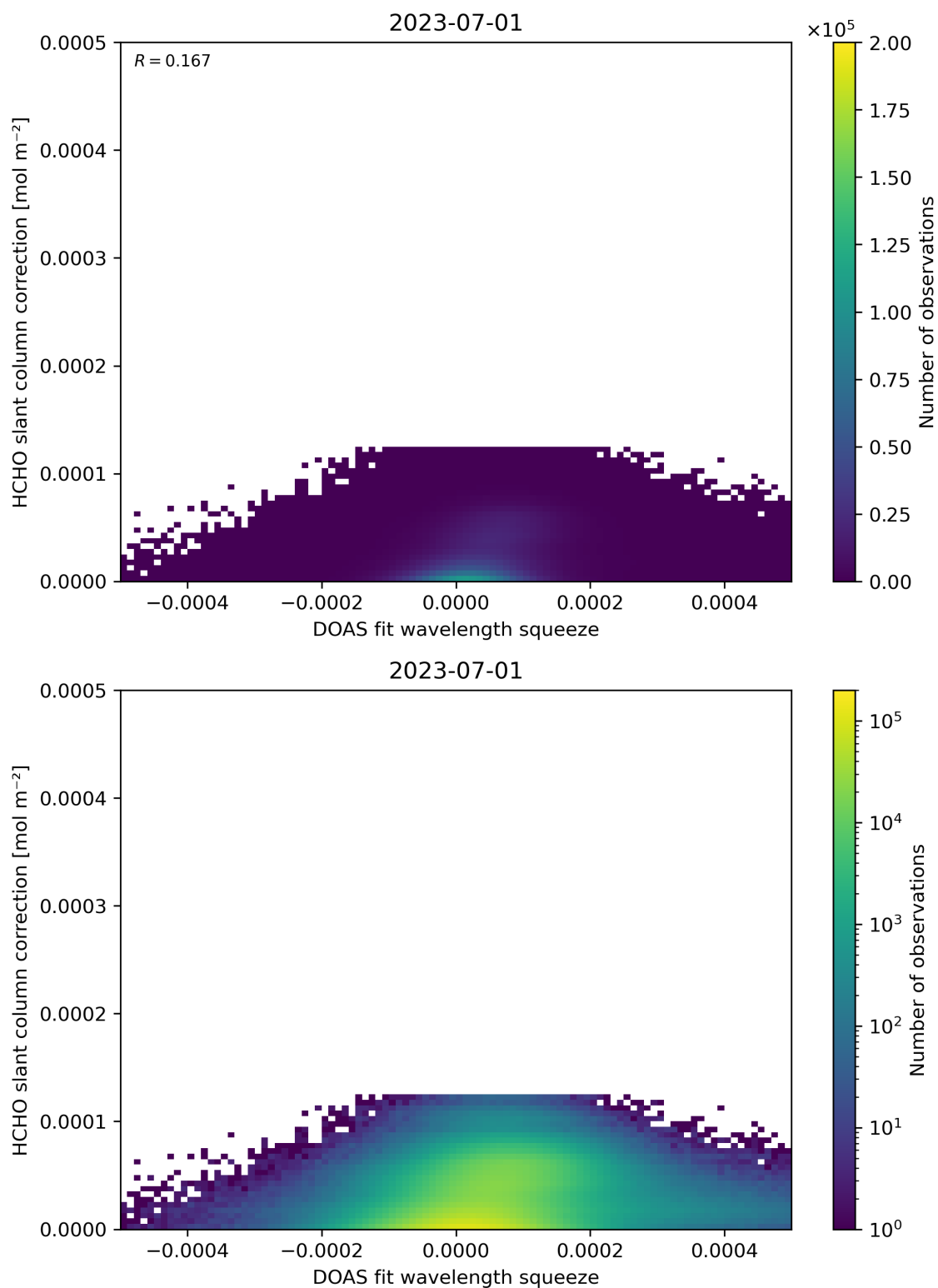
Figure 70: Scatter density plot of “DOAS fit wavelength squeeze” against “HCHO slant column correction” for 2023-06-30 to 2023-07-02.
