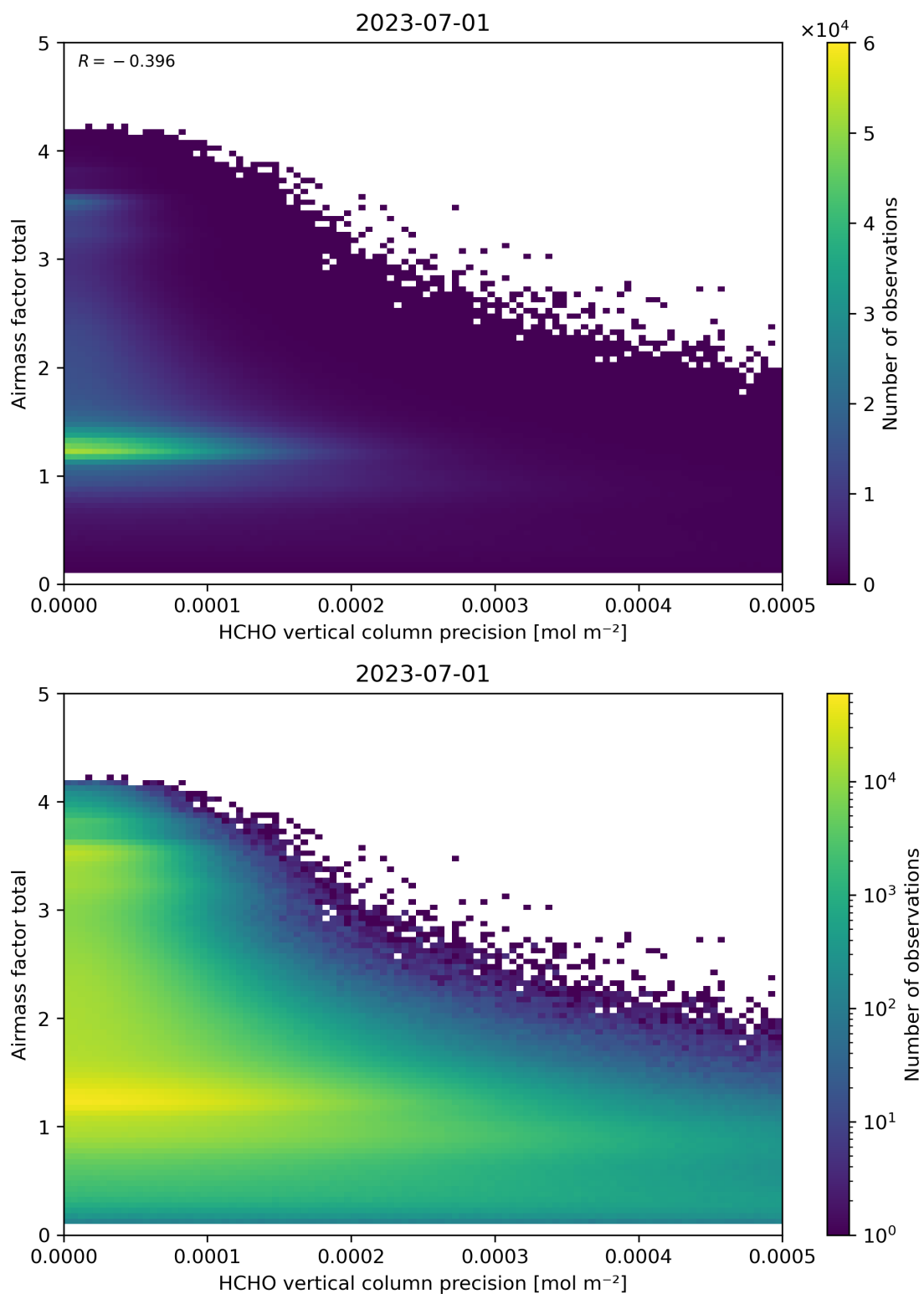
Figure 144: Scatter density plot of “HCHO vertical column precision” against “Airmass factor total” for 2023-06-30 to 2023-07-02.
