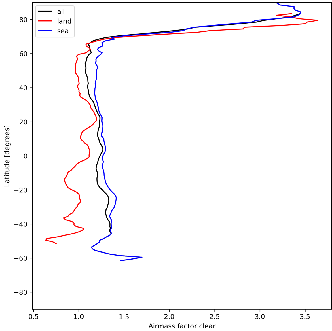
Figure 28: Zonal average of “Airmass factor clear” for 2023-06-30 to 2023-07-02.
