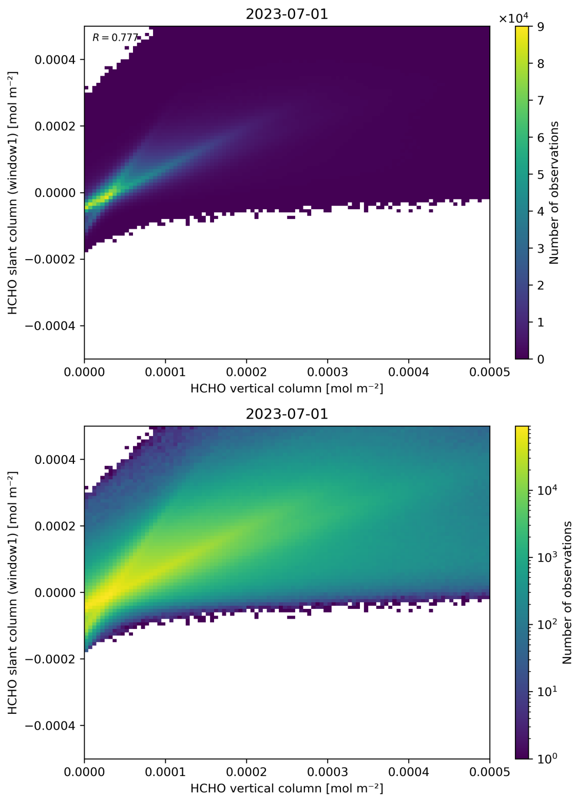
Figure 129: Scatter density plot of “HCHO vertical column” against “HCHO slant column (window1)” for 2023-06-30 to 2023-07-02.
