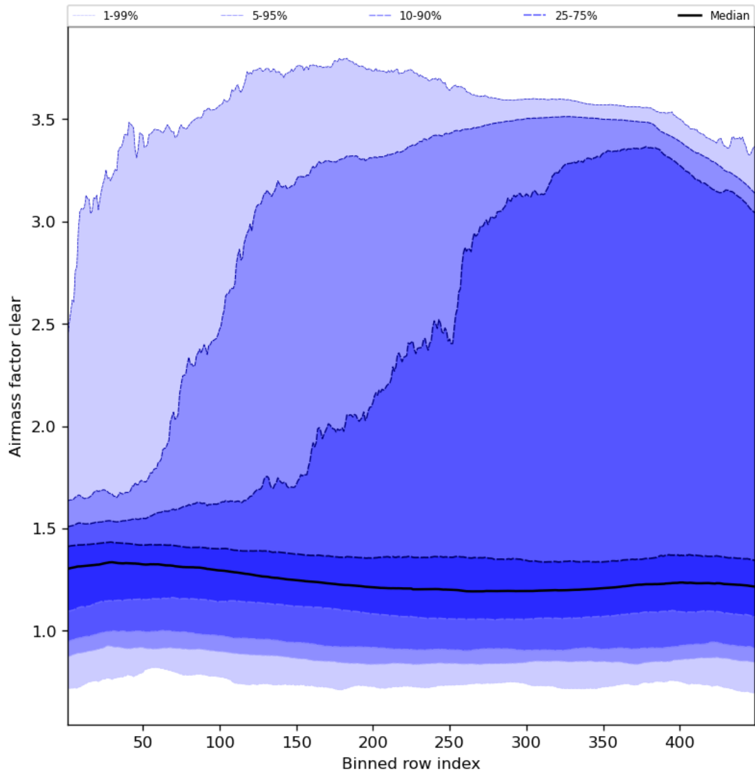
Figure 56: Along track statistics of “Airmass factor clear” for 2023-06-30 to 2023-07-02
