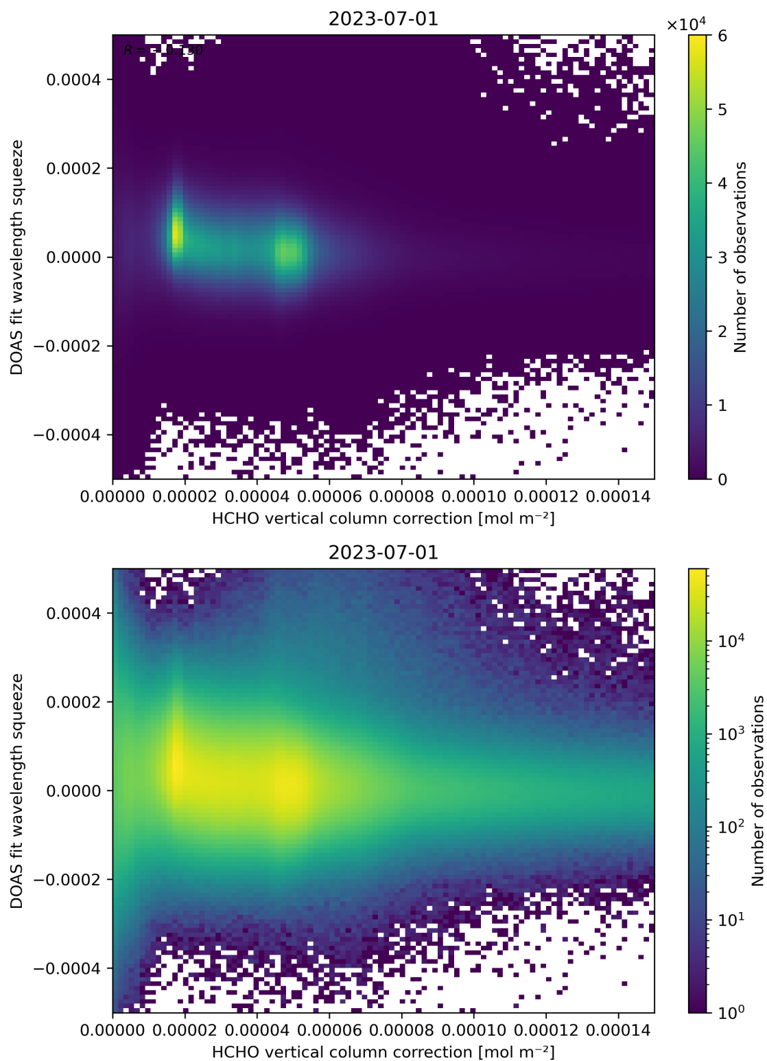
Figure 114: Scatter density plot of “HCHO vertical column correction” against “DOAS fit wavelength squeeze” for 2023-06-30 to 2023-07-02.
