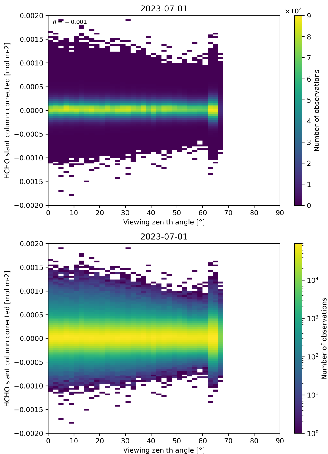
Figure 186: Scatter density plot of “Viewing zenith angle” against “HCHO slant column corrected” for 2023-06-30 to 2023-07-02.
