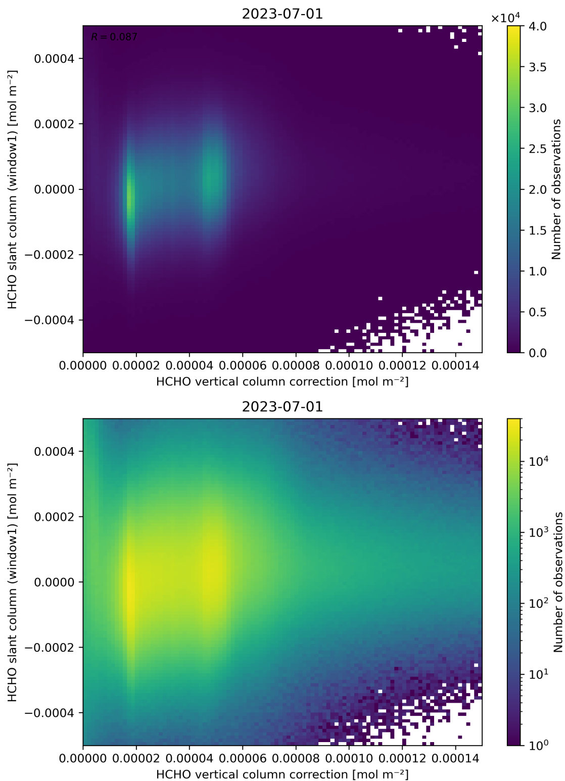
Figure 118: Scatter density plot of “HCHO vertical column correction” against “HCHO slant column (window1)” for 2023-06-30 to 2023-07-02.
