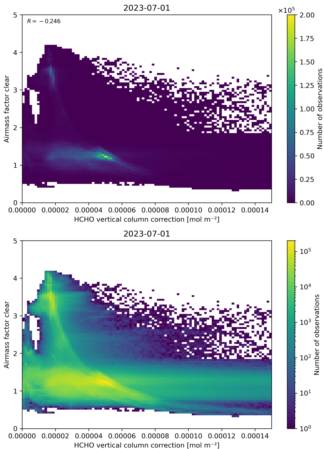
Figure 115: Scatter density plot of “HCHO vertical column correction” against “Airmass factor clear” for 2023-06-30 to 2023-07-02.
