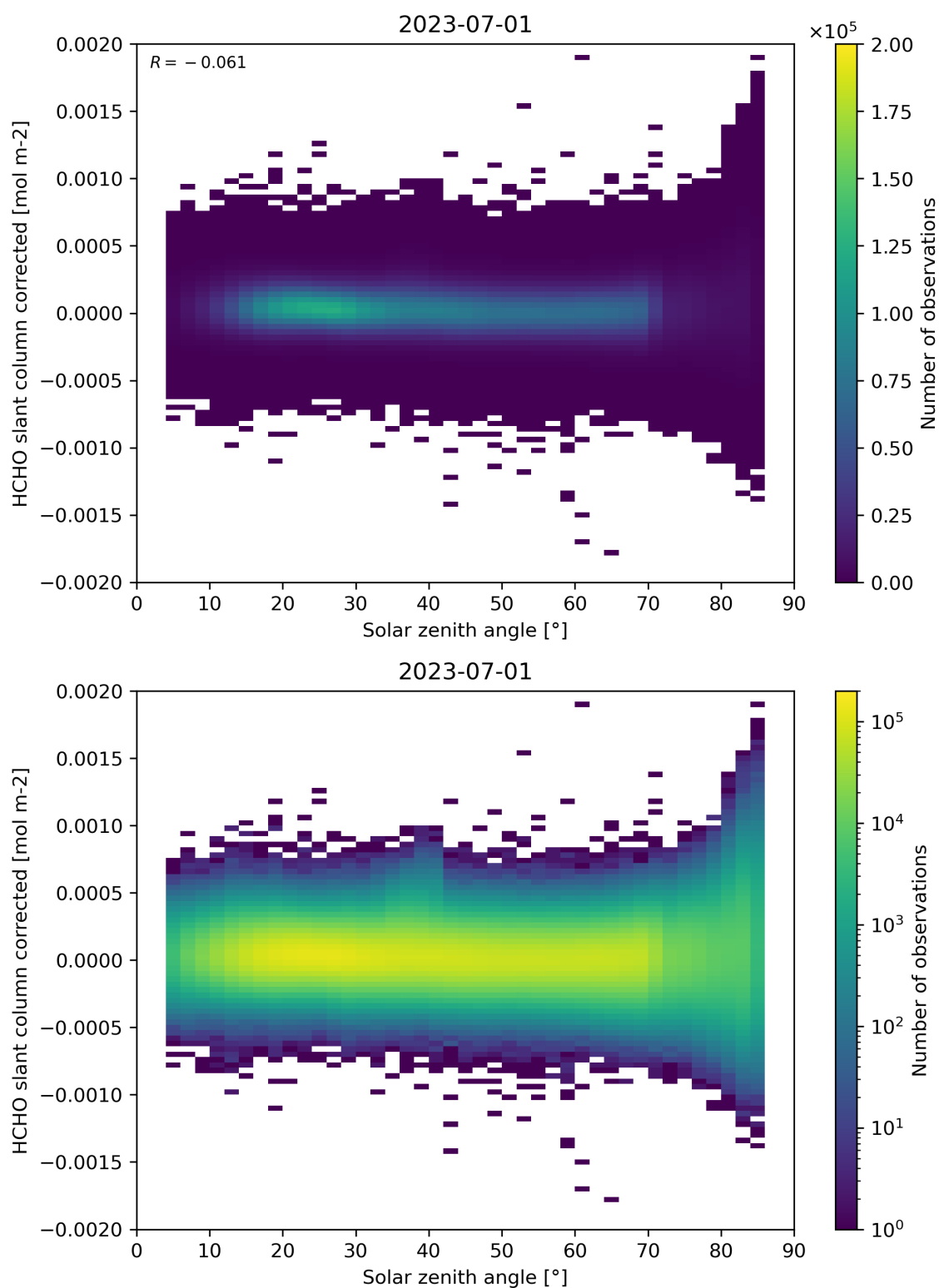
Figure 171: Scatter density plot of “Solar zenith angle” against “HCHO slant column corrected” for 2023-06-30 to 2023-07-02.
