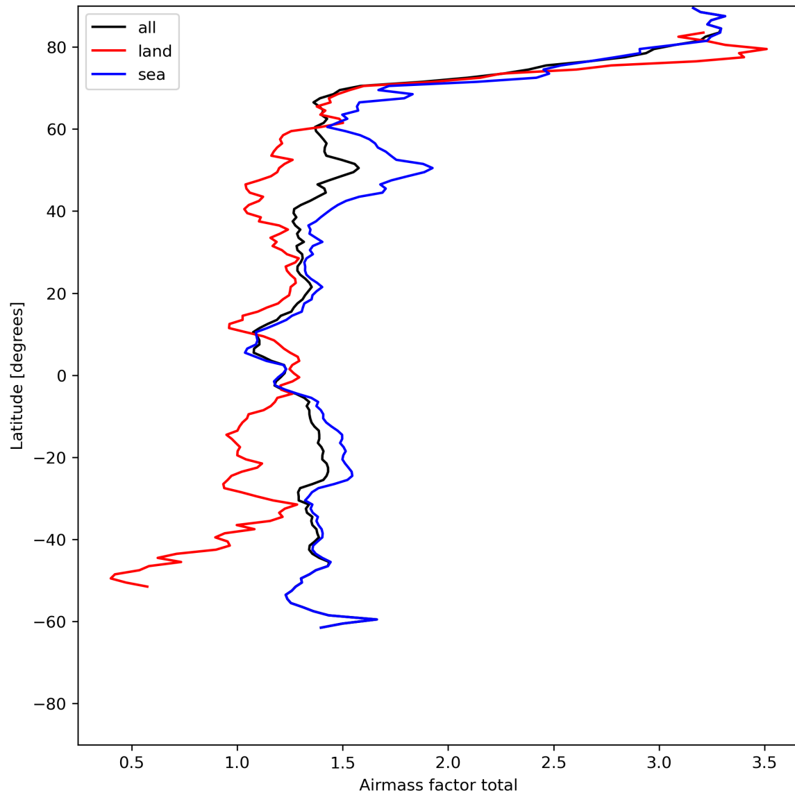
Figure 26: Zonal average of “Airmass factor total” for 2023-06-30 to 2023-07-02.
