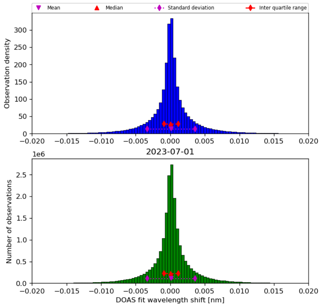
Figure 44: Histogram of “DOAS fit wavelength shift” for 2023-06-30 to 2023-07-02
