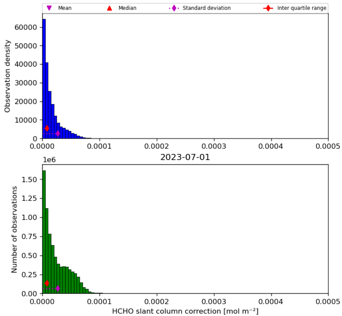
Figure 47: Histogram of “HCHO slant column correction” for 2023-06-30 to 2023-07-02
