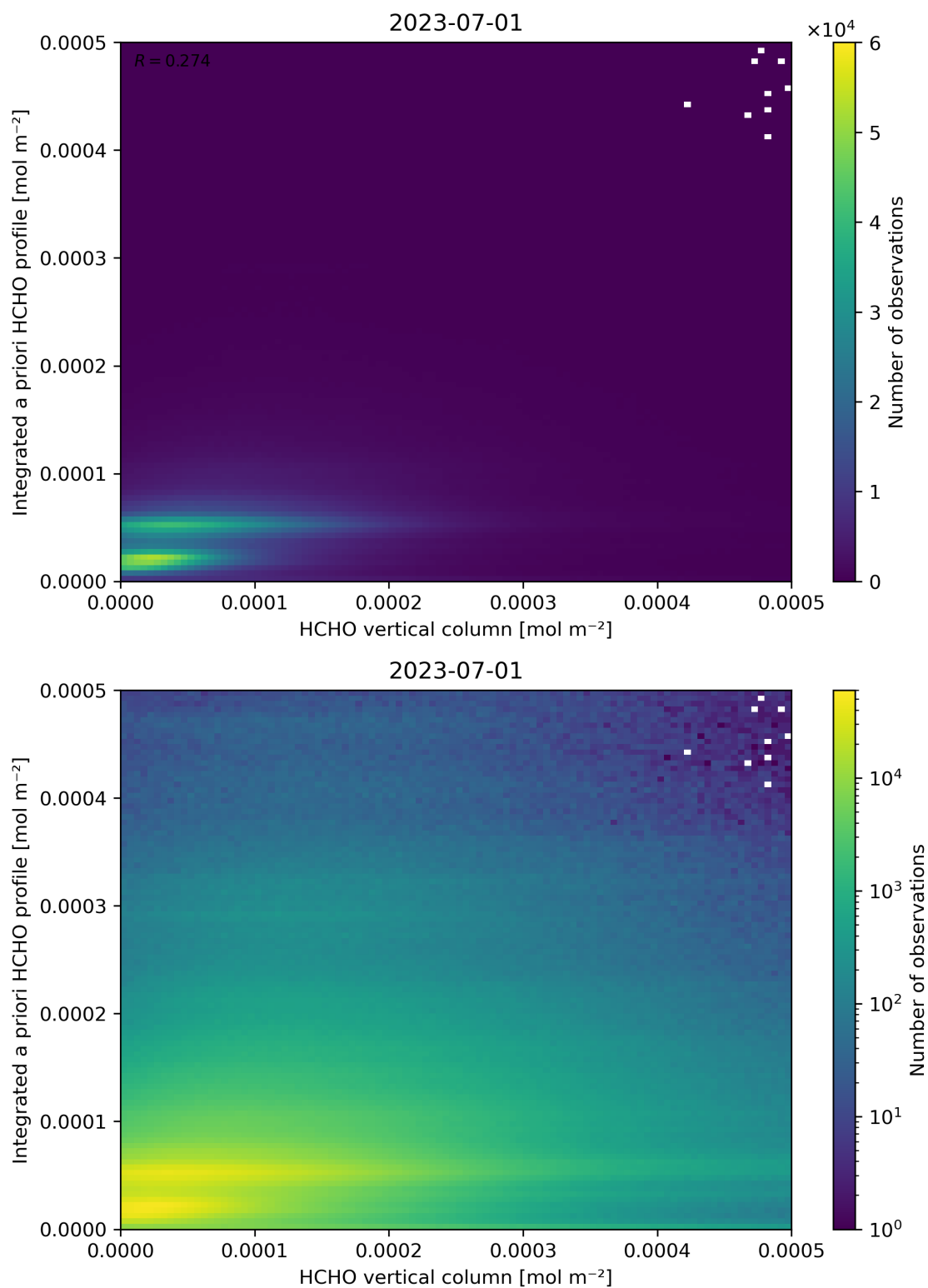
Figure 135: Scatter density plot of “HCHO vertical column” against “Integrated a priori HCHO profile” for 2023-06-30 to 2023-07-02.
