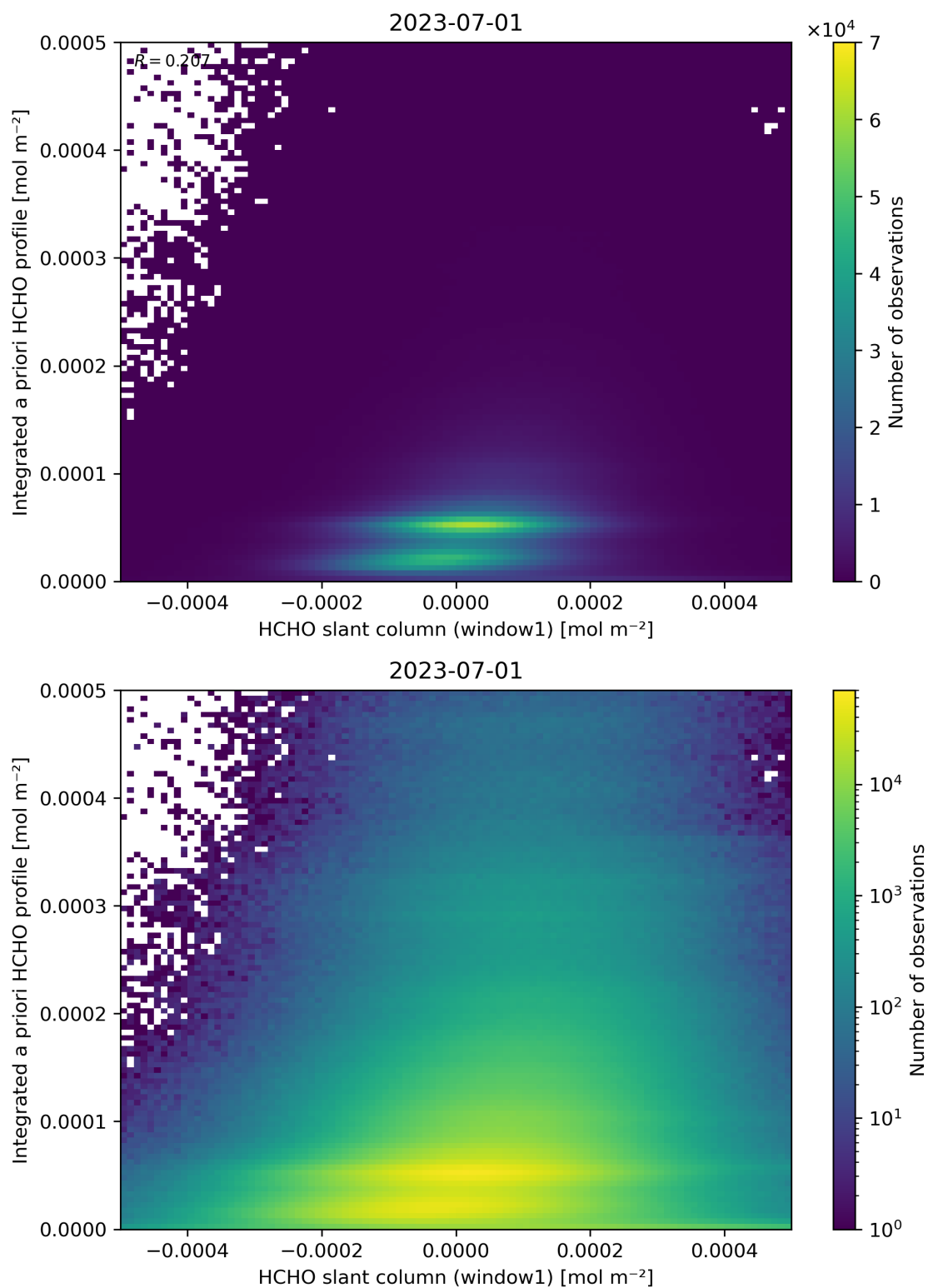
Figure 87: Scatter density plot of “HCHO slant column (window1)” against “Integrated a priori HCHO profile” for 2023-06-30 to 2023-07-02.
