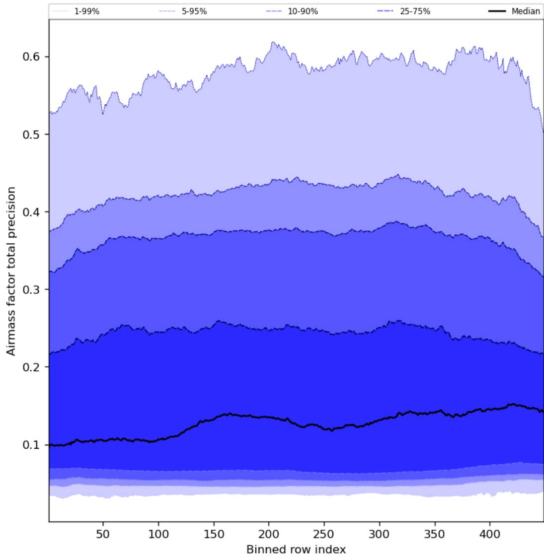
Figure 55: Along track statistics of “Airmass factor total precision” for 2023-06-30 to 2023-07-02
