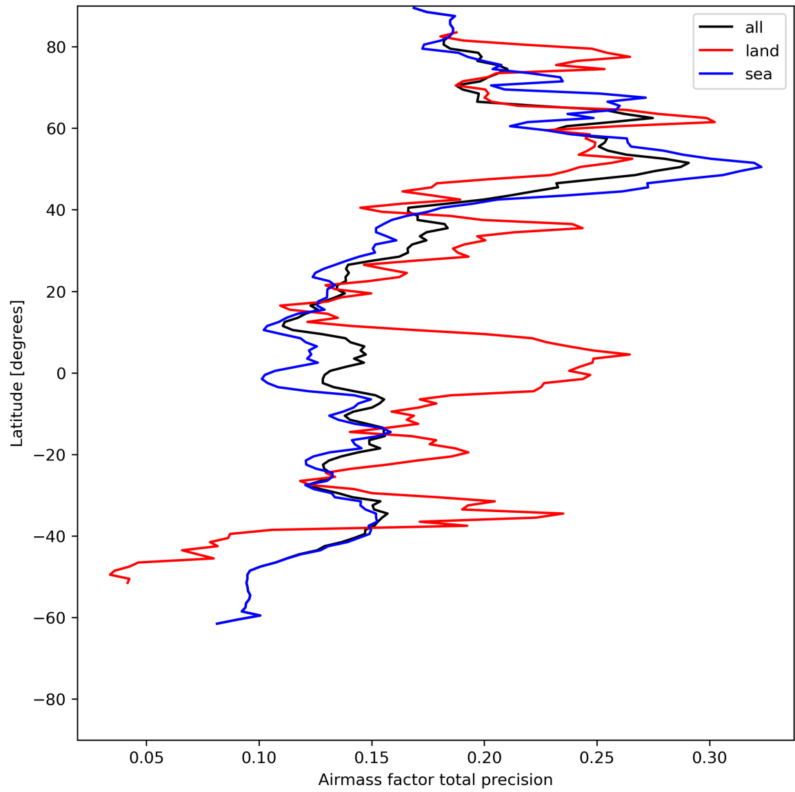
Figure 27: Zonal average of “Airmass factor total precision” for 2023-06-30 to 2023-07-02.
