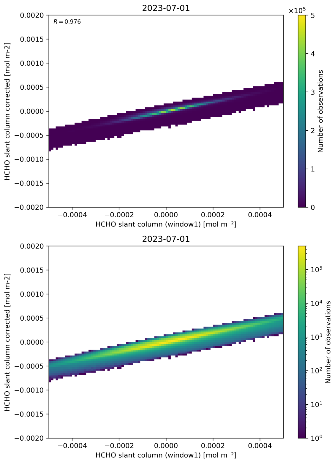
Figure 82: Scatter density plot of “HCHO slant column (window1)” against “HCHO slant column corrected” for 2023-06-30 to 2023-07-02.
