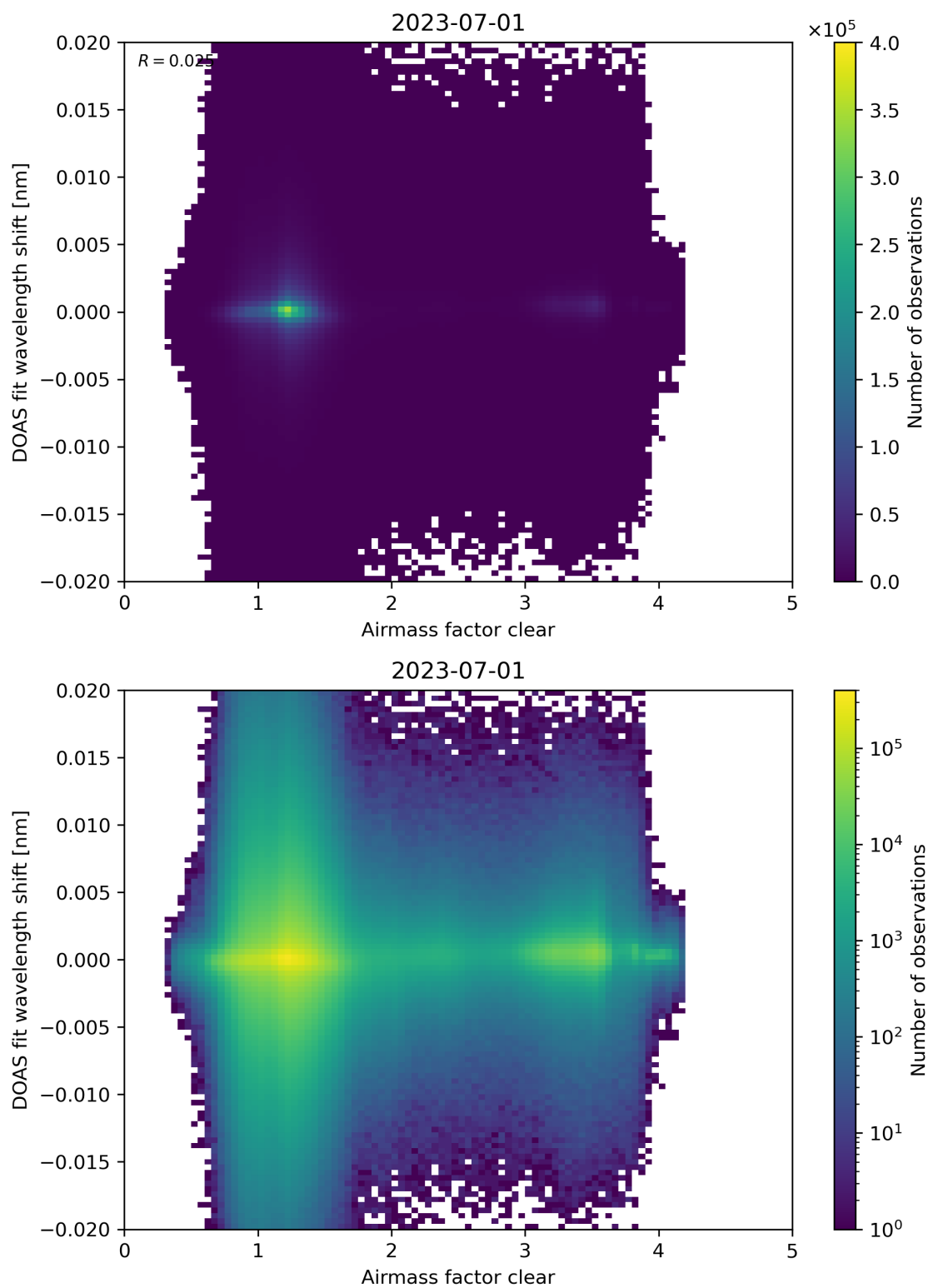
Figure 72: Scatter density plot of “Airmass factor clear” against “DOAS fit wavelength shift” for 2023-06-30 to 2023-07-02.
