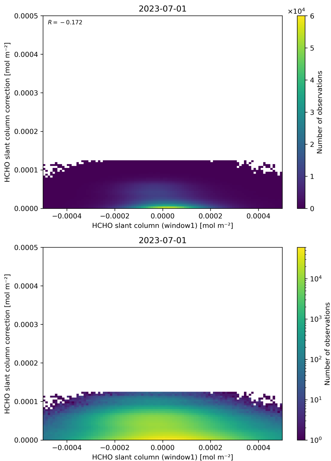
Figure 83: Scatter density plot of “HCHO slant column (window1)” against “HCHO slant column correction” for 2023-06-30 to 2023-07-02.
