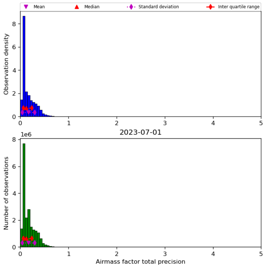
Figure 41: Histogram of “Airmass factor total precision” for 2023-06-30 to 2023-07-02
