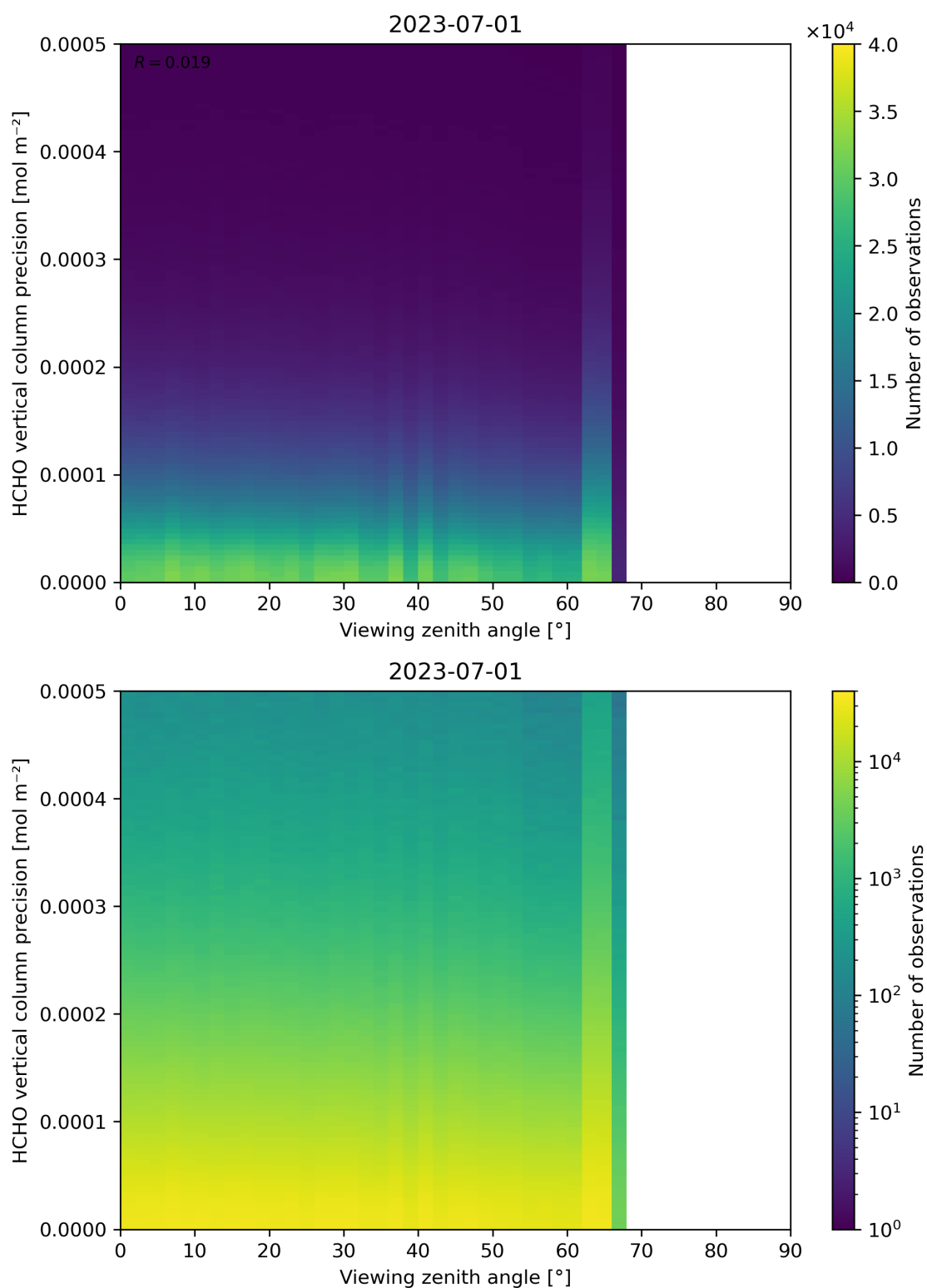
Figure 194: Scatter density plot of “Viewing zenith angle” against “HCHO vertical column precision” for 2023-06-30 to 2023-07-02.
