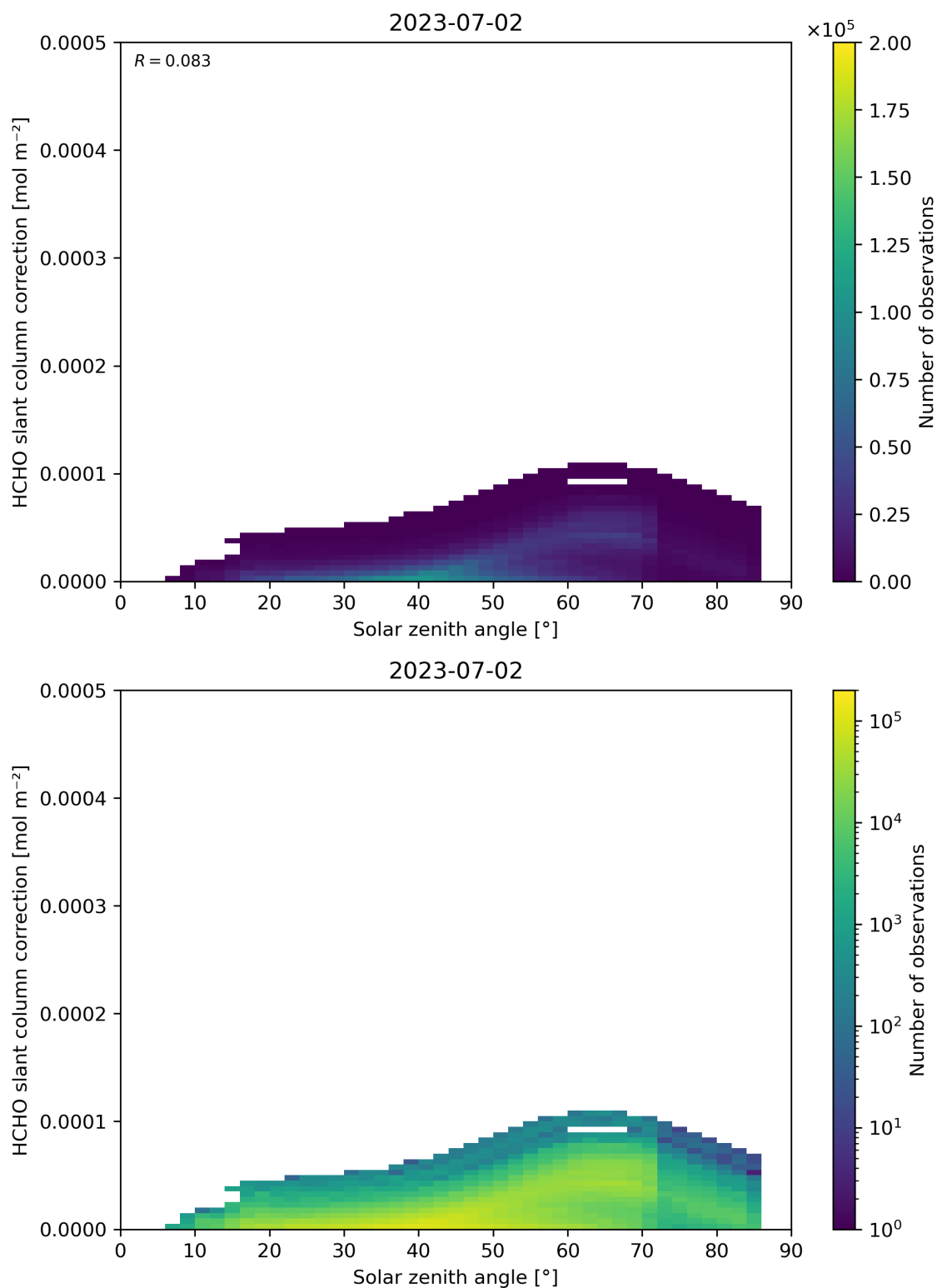
Figure 172: Scatter density plot of “Solar zenith angle” against “HCHO slant column correction” for 2023-07-01 to 2023-07-03.
