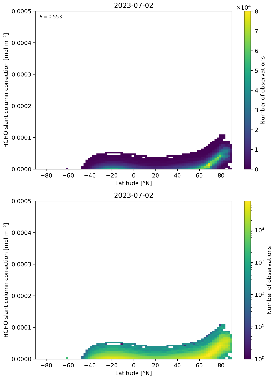
Figure 158: Scatter density plot of “Latitude” against “HCHO slant column correction” for 2023-07-01 to 2023-07-03.
