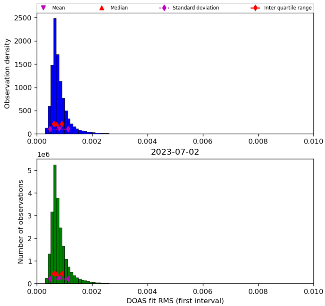
Figure 46: Histogram of “DOAS fit RMS (first interval)” for 2023-07-01 to 2023-07-03
