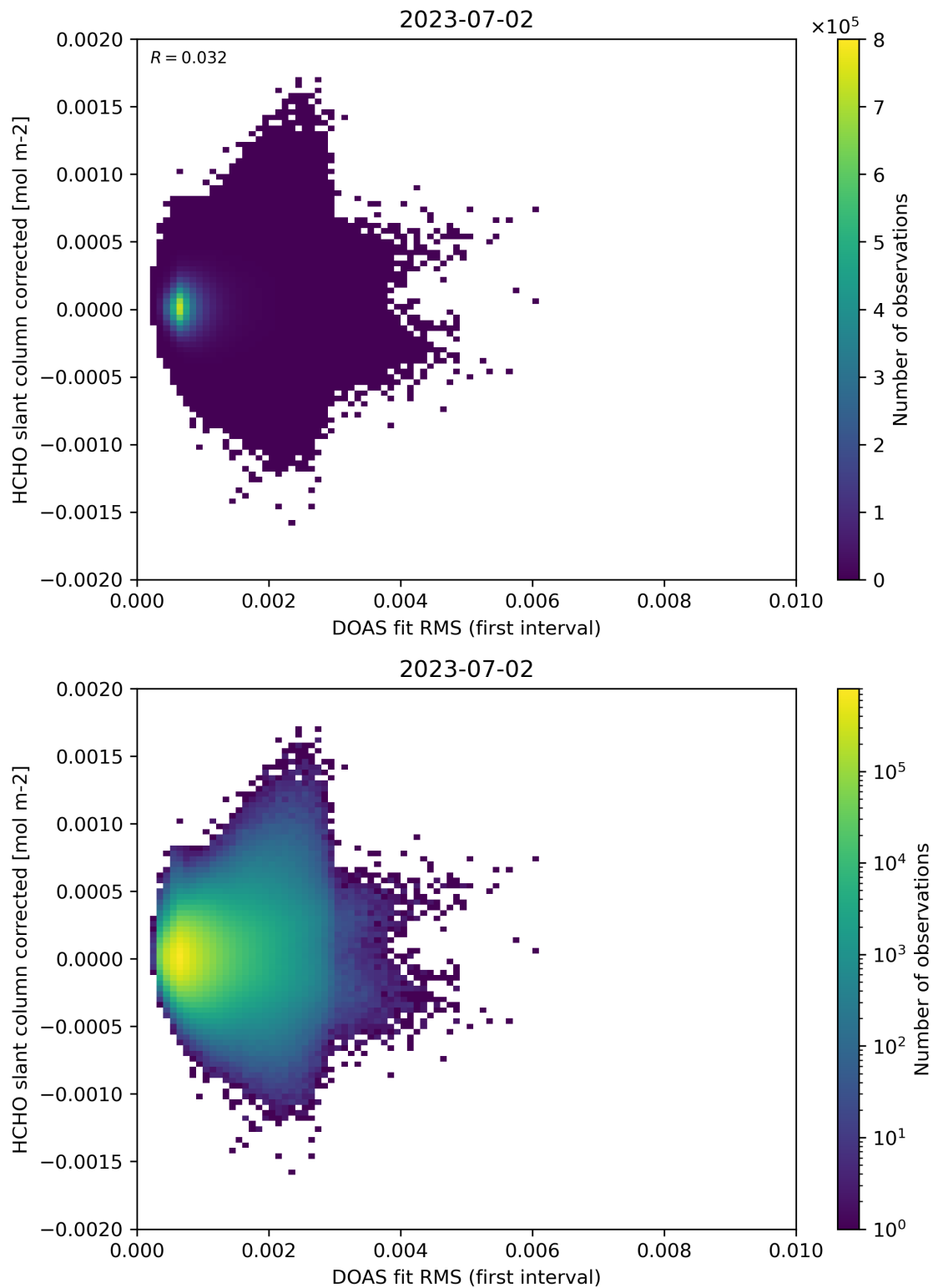
Figure 62: Scatter density plot of “DOAS fit RMS (first interval)” against “HCHO slant column corrected” for 2023-07-01 to 2023-07-03.
