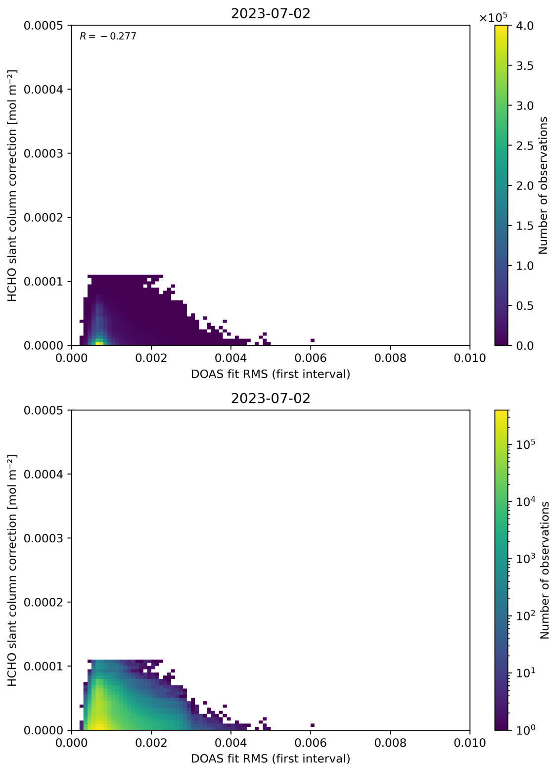
Figure 63: Scatter density plot of “DOAS fit RMS (first interval)” against “HCHO slant column correction” for 2023-07-01 to 2023-07-03.
