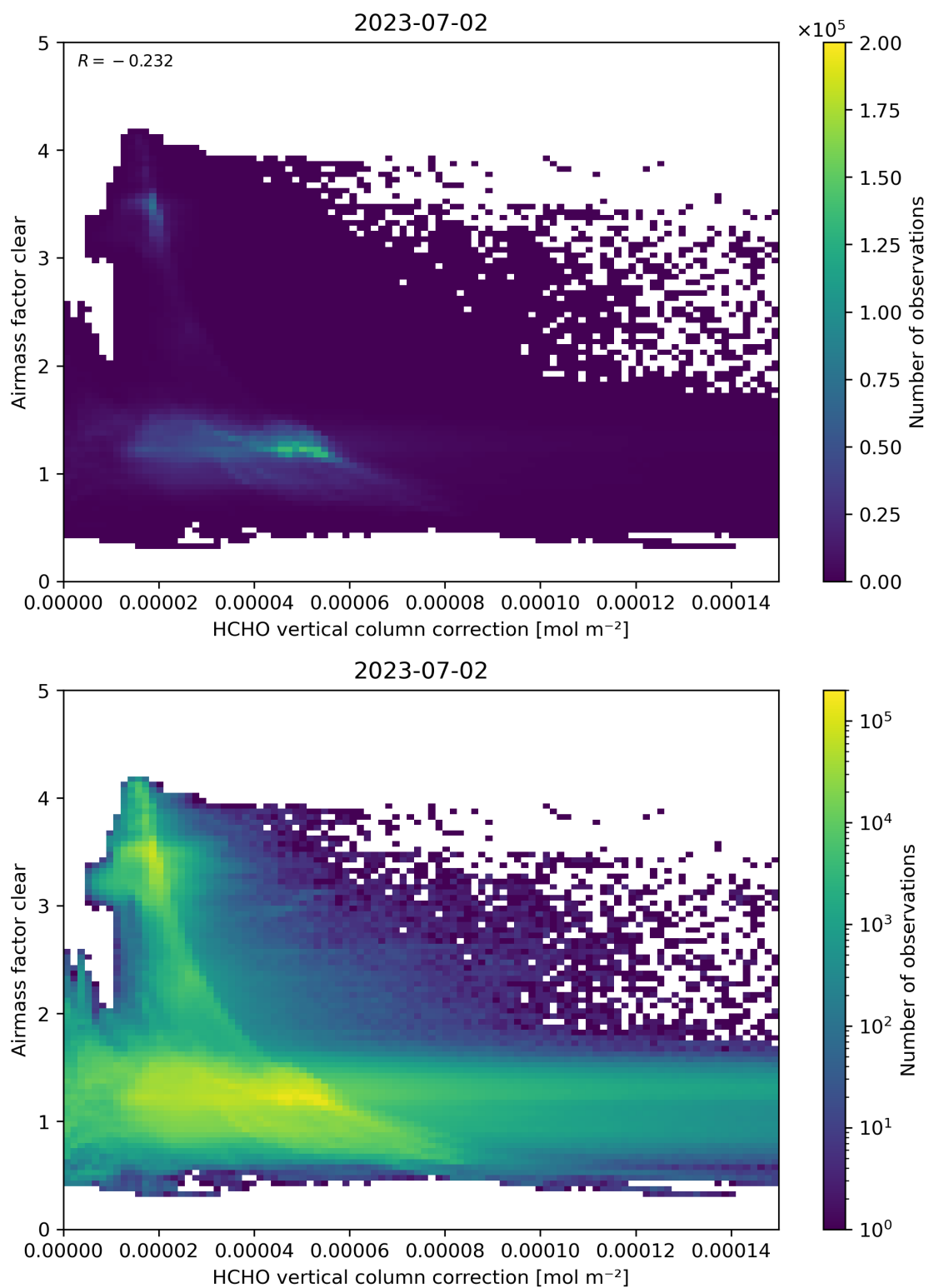
Figure 115: Scatter density plot of “HCHO vertical column correction” against “Airmass factor clear” for 2023-07-01 to 2023-07-03.
