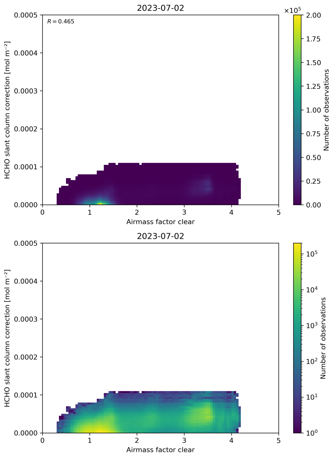
Figure 75: Scatter density plot of “Airmass factor clear” against “HCHO slant column correction” for 2023-07-01 to 2023-07-03.
