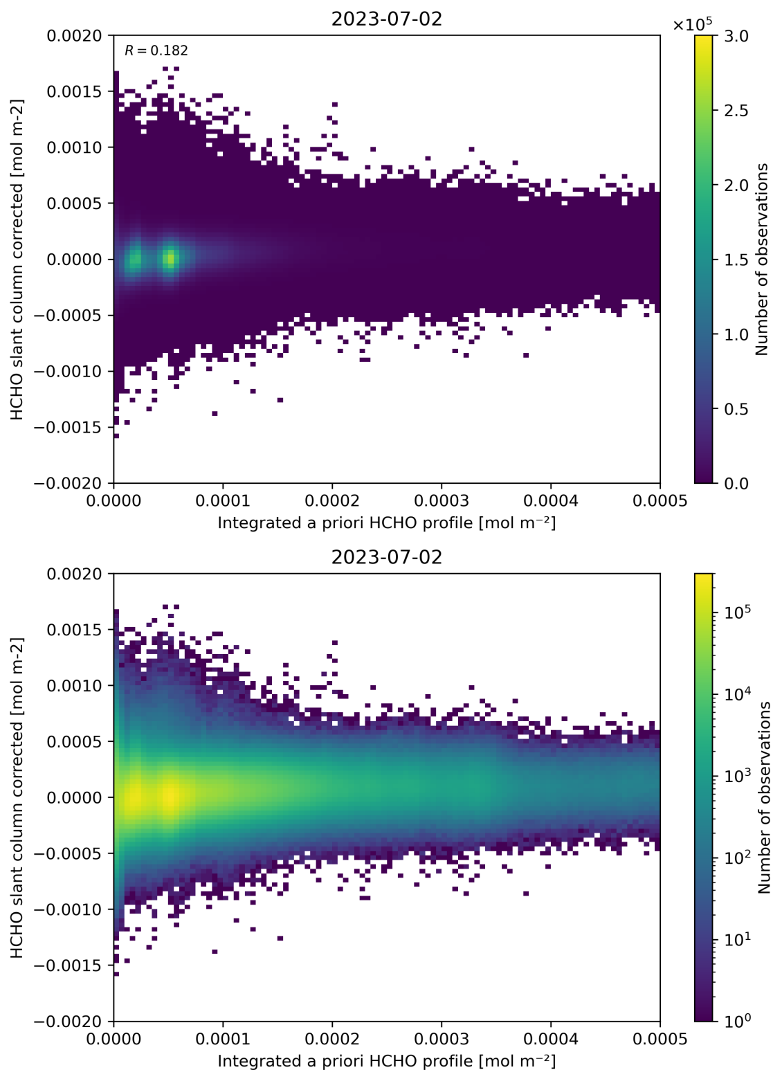
Figure 151: Scatter density plot of “Integrated a priori HCHO profile” against “HCHO slant column corrected” for 2023-07-01 to 2023-07-03.
