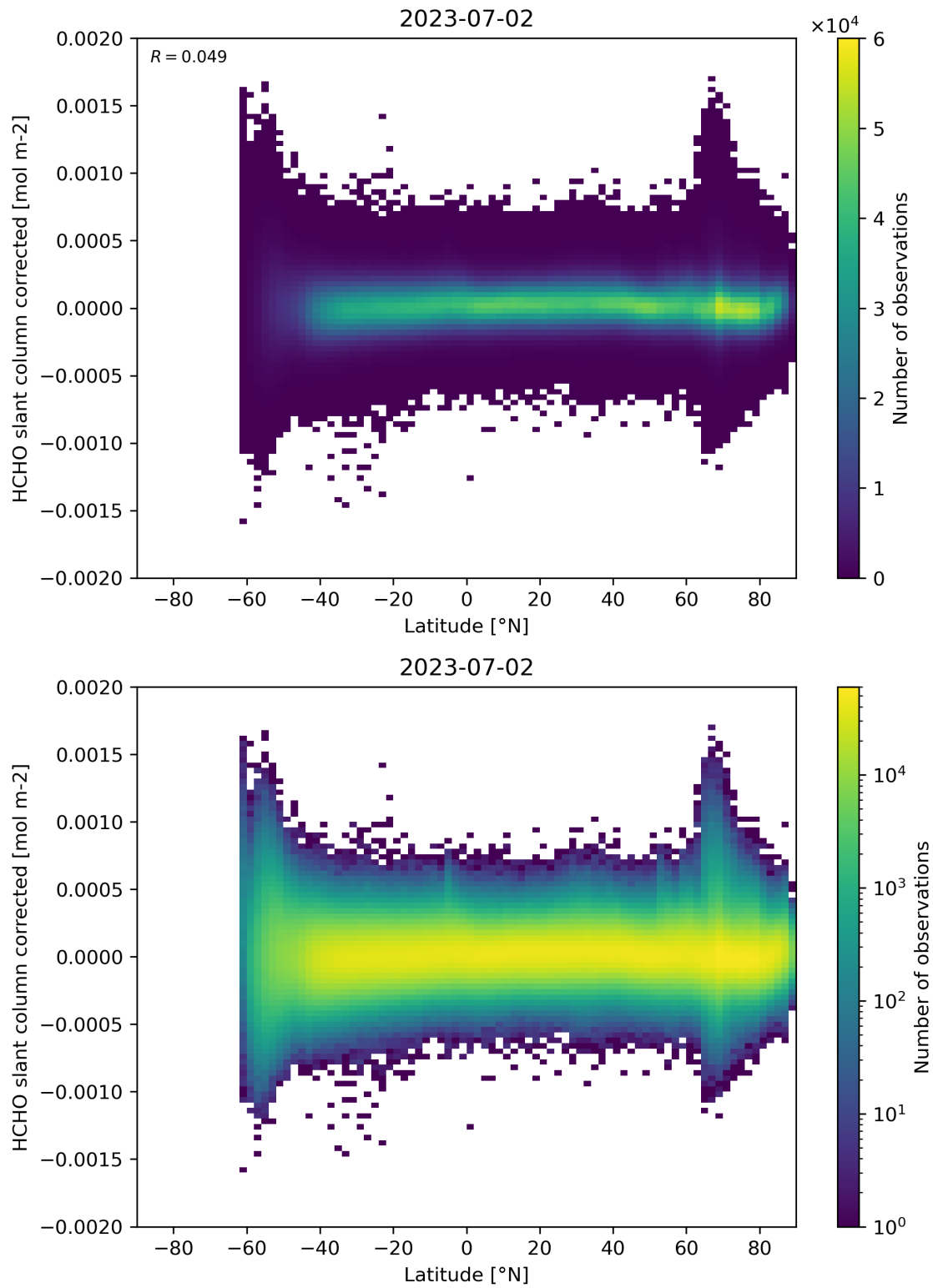
Figure 157: Scatter density plot of “Latitude” against “HCHO slant column corrected” for 2023-07-01 to 2023-07-03.
