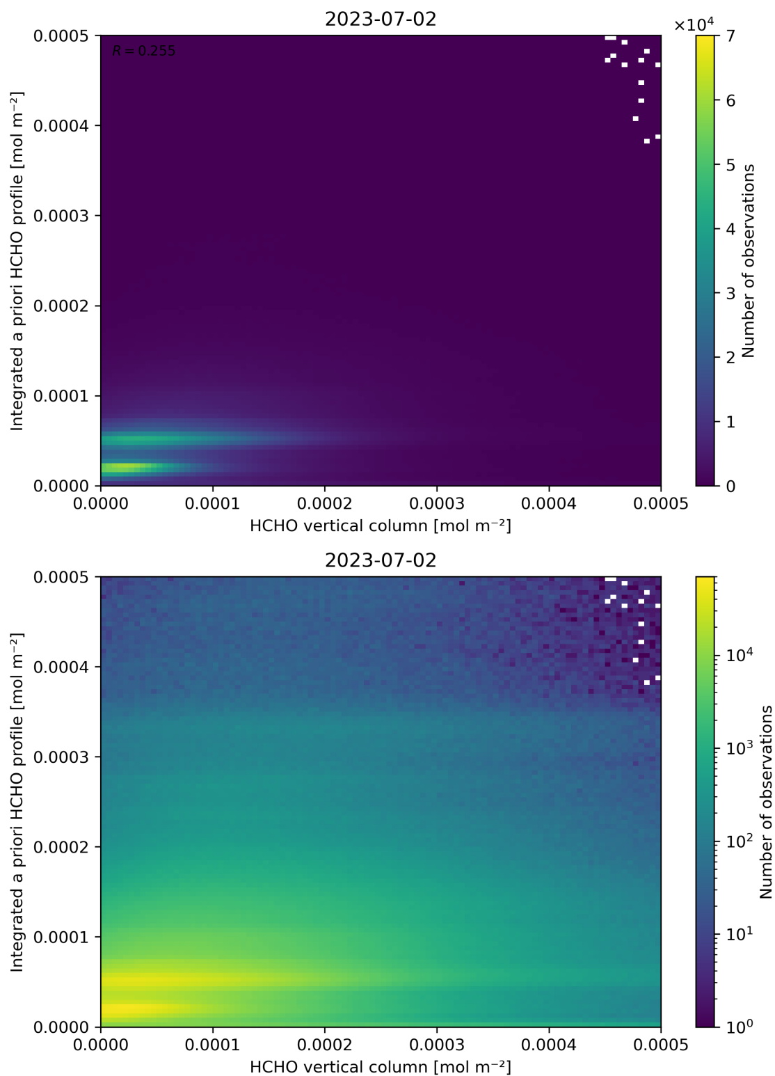
Figure 135: Scatter density plot of “HCHO vertical column” against “Integrated a priori HCHO profile” for 2023-07-01 to 2023-07-03.
