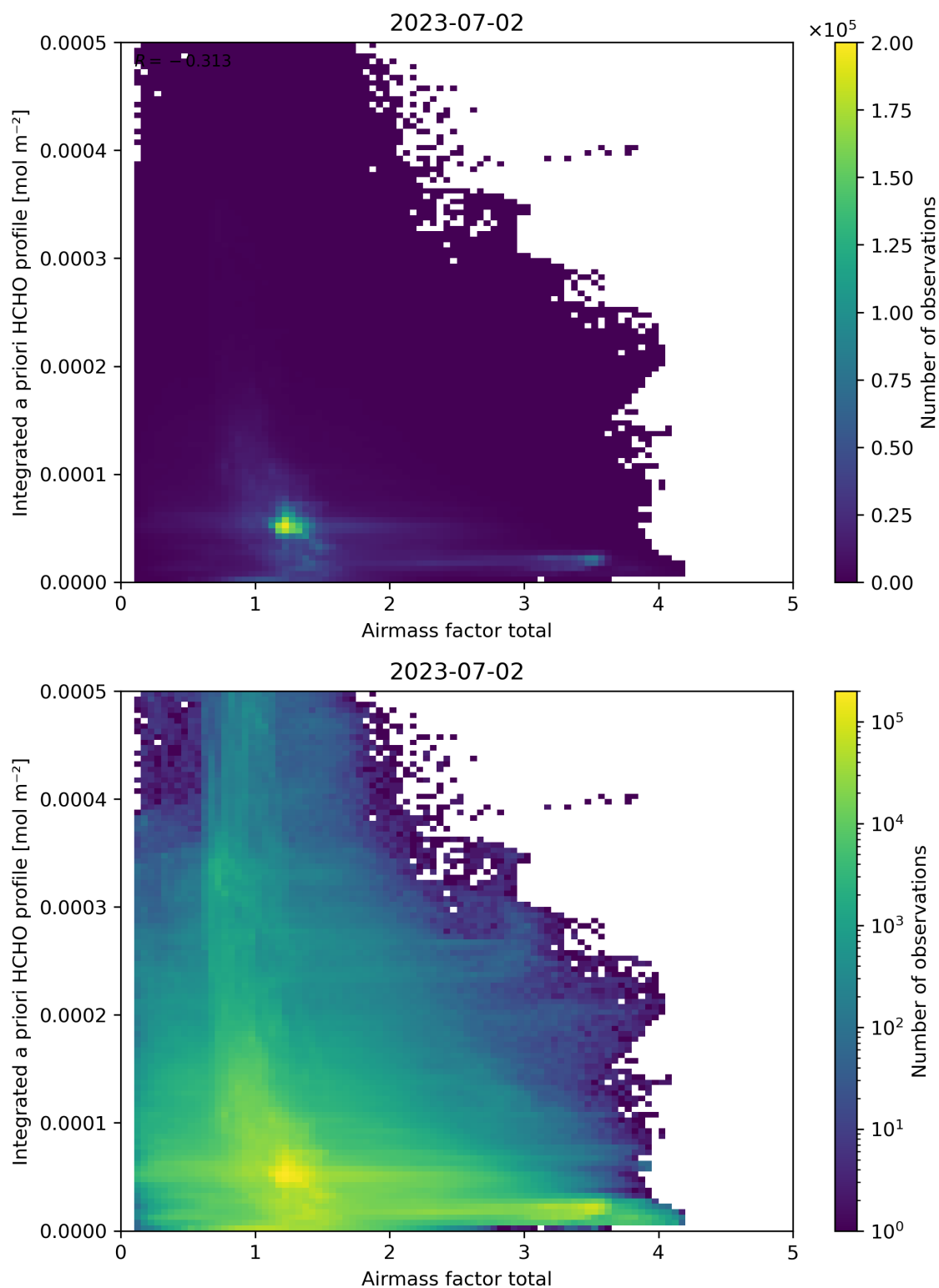
Figure 104: Scatter density plot of “Airmass factor total” against “Integrated a priori HCHO profile” for 2023-07-01 to 2023-07-03.
