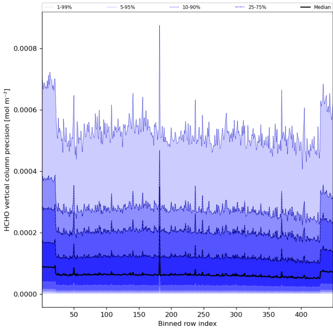
Figure 50: Along track statistics of “HCHO vertical column precision” for 2023-07-01 to 2023-07-03
