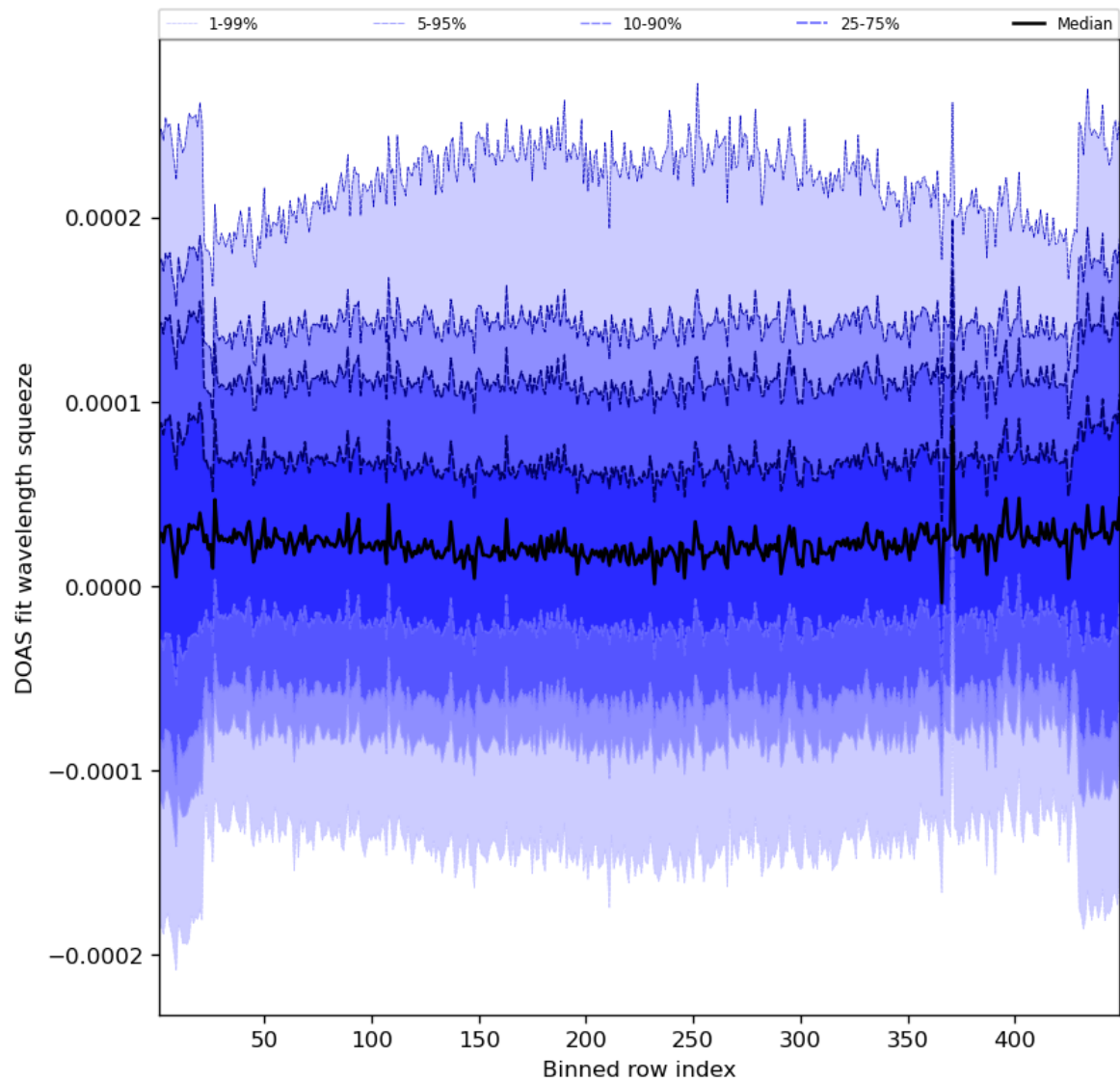
Figure 59: Along track statistics of “DOAS fit wavelength squeeze” for 2023-07-01 to 2023-07-03
