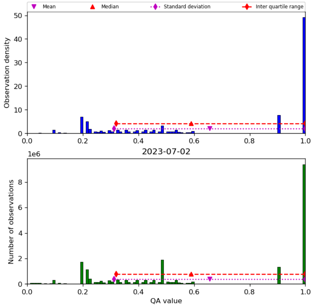
Figure 34: Histogram of “QA value” for 2023-07-01 to 2023-07-03
