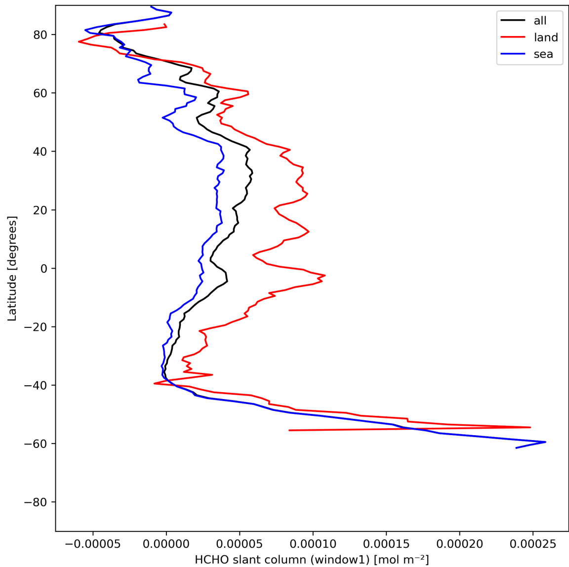
Figure 24: Zonal average of “HCHO slant column (window1)” for 2023-07-01 to 2023-07-03.
