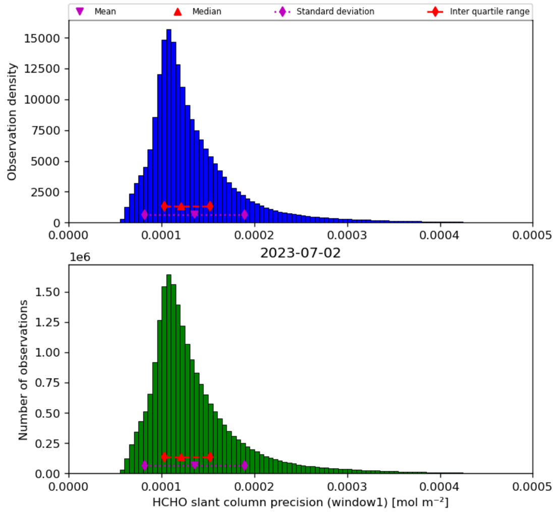
Figure 39: Histogram of “HCHO slant column precision (window1)” for 2023-07-01 to 2023-07-03
