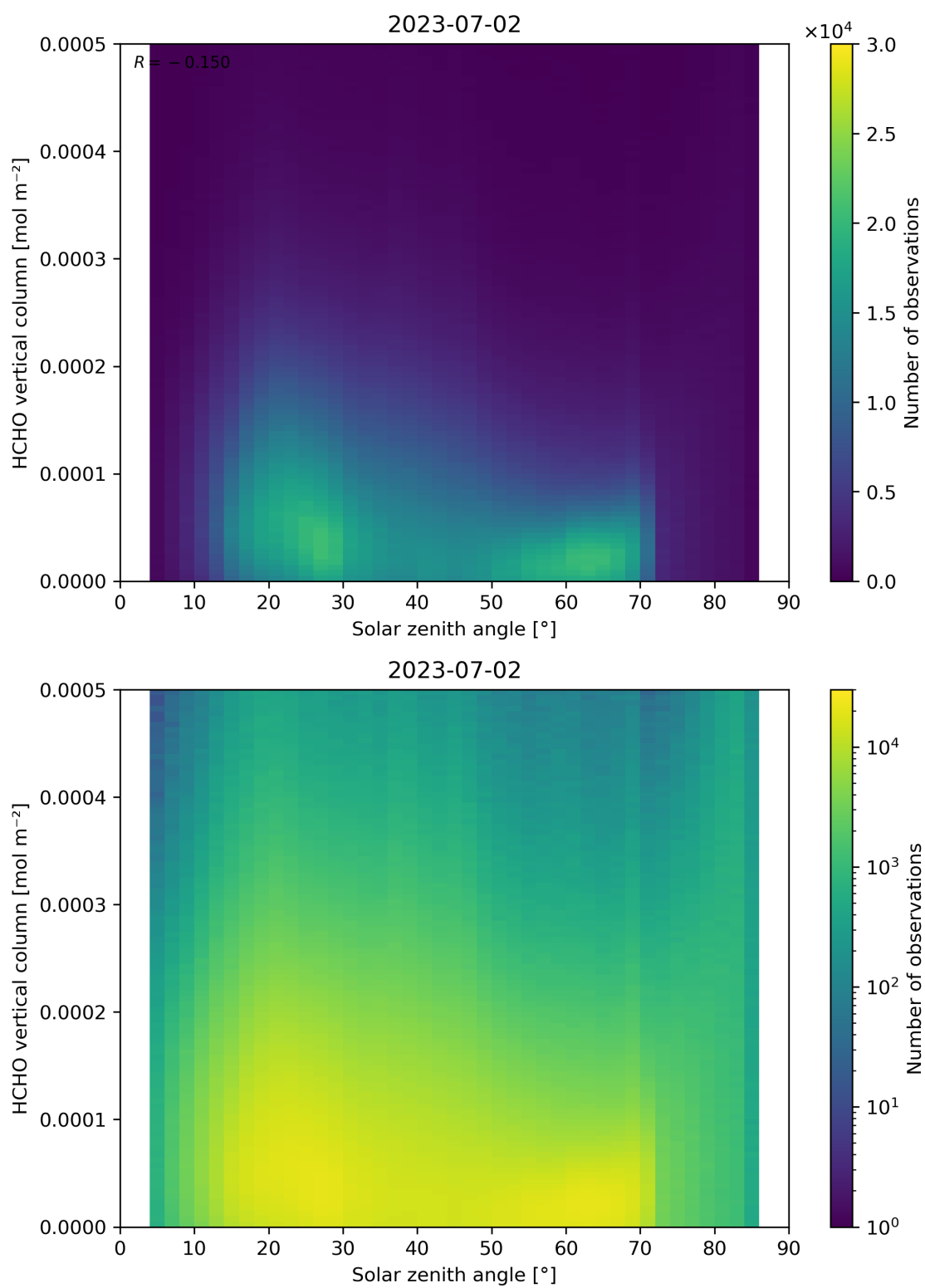
Figure 177: Scatter density plot of “Solar zenith angle” against “HCHO vertical column” for 2023-07-01 to 2023-07-03.
