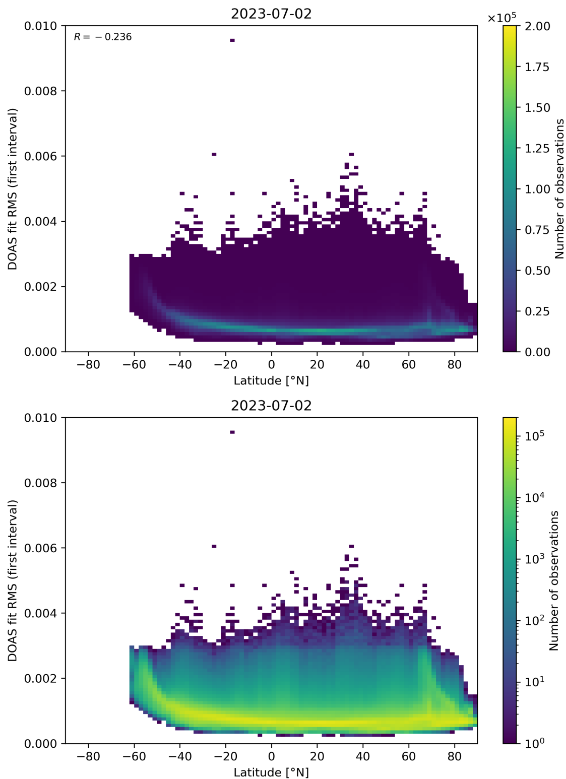
Figure 153: Scatter density plot of “Latitude” against “DOAS fit RMS (first interval)” for 2023-07-01 to 2023-07-03.
