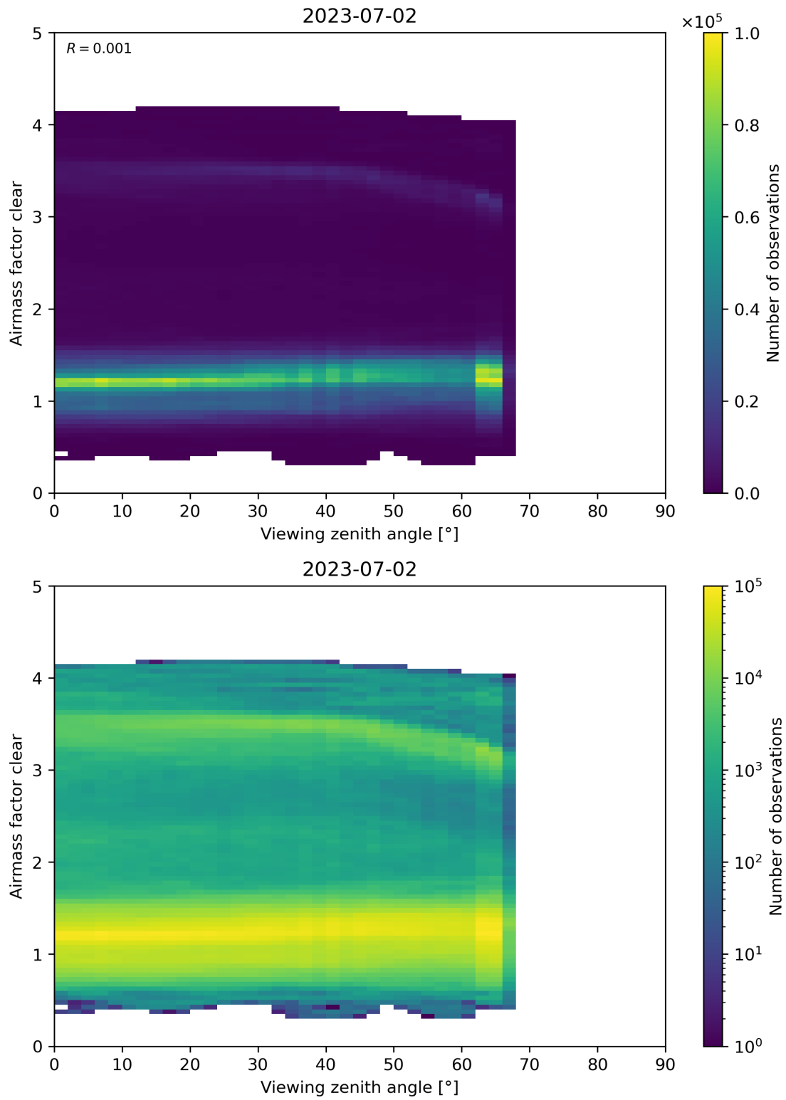
Figure 185: Scatter density plot of “Viewing zenith angle” against “Airmass factor clear” for 2023-07-01 to 2023-07-03.
