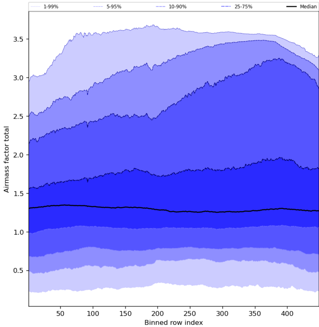
Figure 54: Along track statistics of “Airmass factor total” for 2023-07-01 to 2023-07-03
