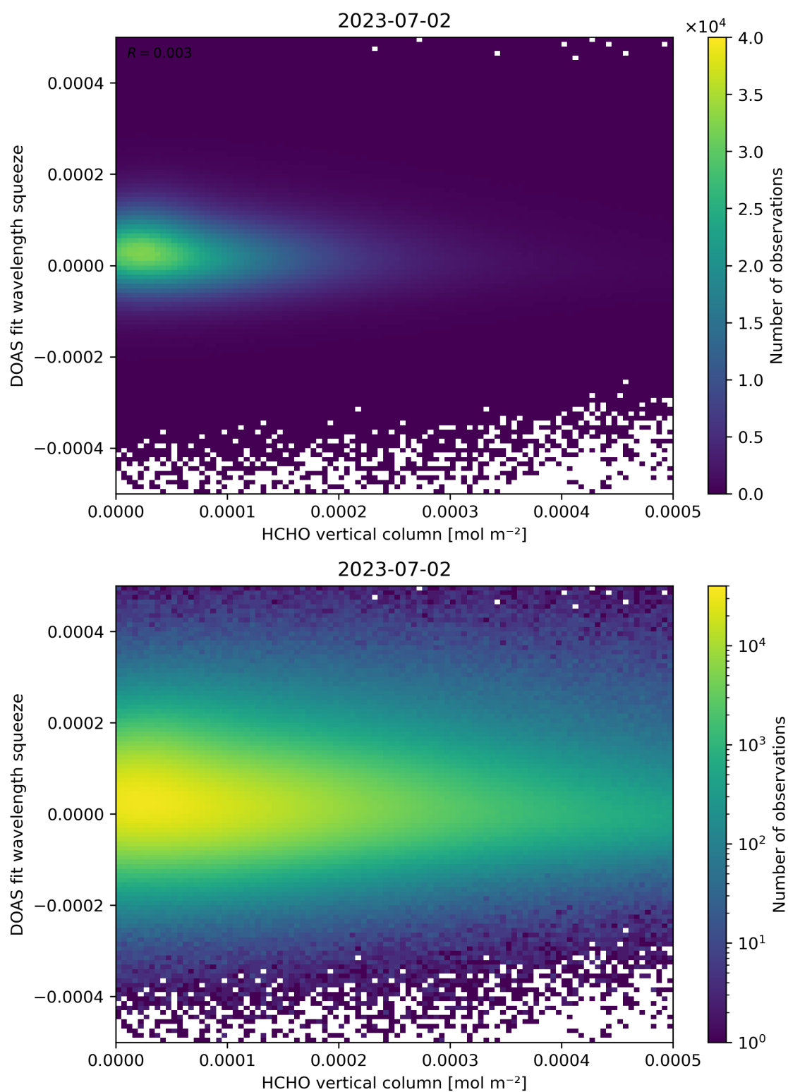
Figure 125: Scatter density plot of “HCHO vertical column” against “DOAS fit wavelength squeeze” for 2023-07-01 to 2023-07-03.
