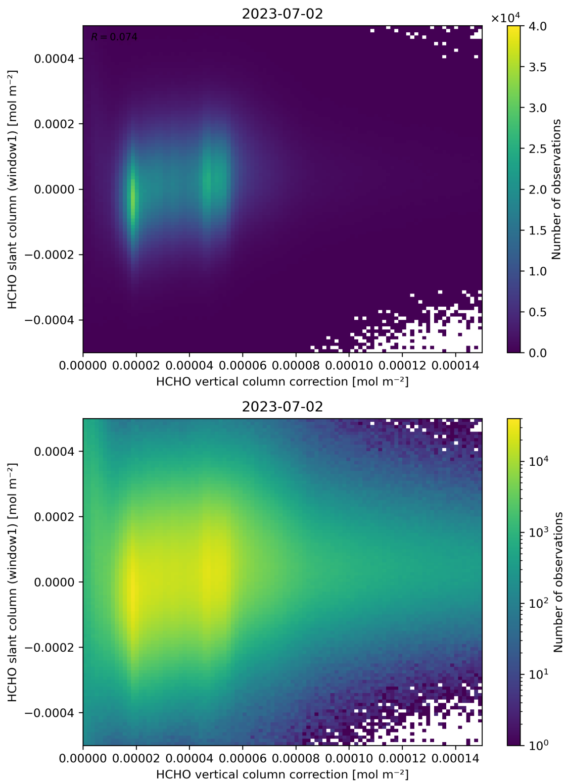
Figure 118: Scatter density plot of “HCHO vertical column correction” against “HCHO slant column (window1)” for 2023-07-01 to 2023-07-03.
