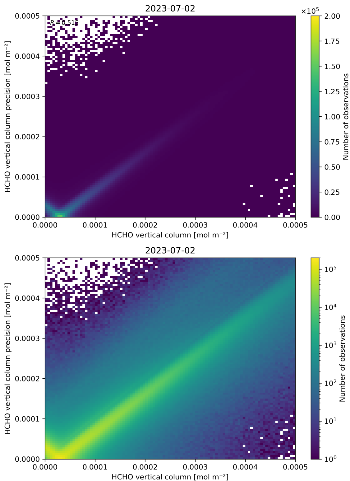
Figure 134: Scatter density plot of “HCHO vertical column” against “HCHO vertical column precision” for 2023-07-01 to 2023-07-03.
