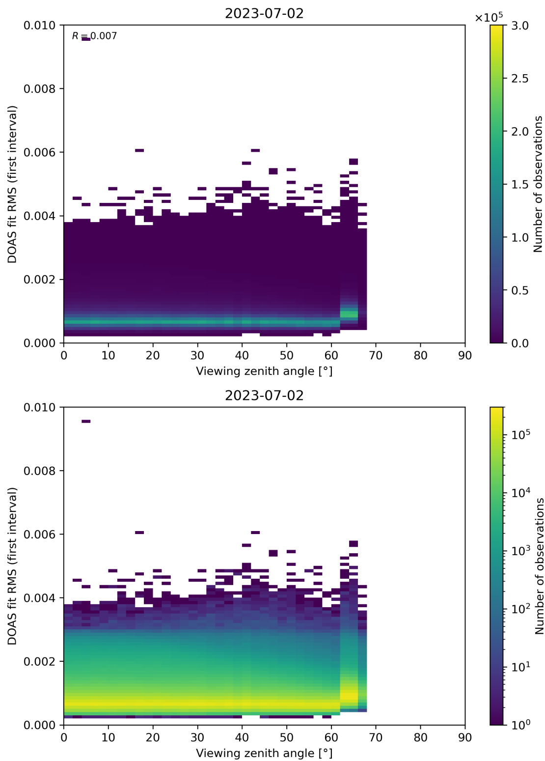
Figure 182: Scatter density plot of “Viewing zenith angle” against “DOAS fit RMS (first interval)” for 2023-07-01 to 2023-07-03.
