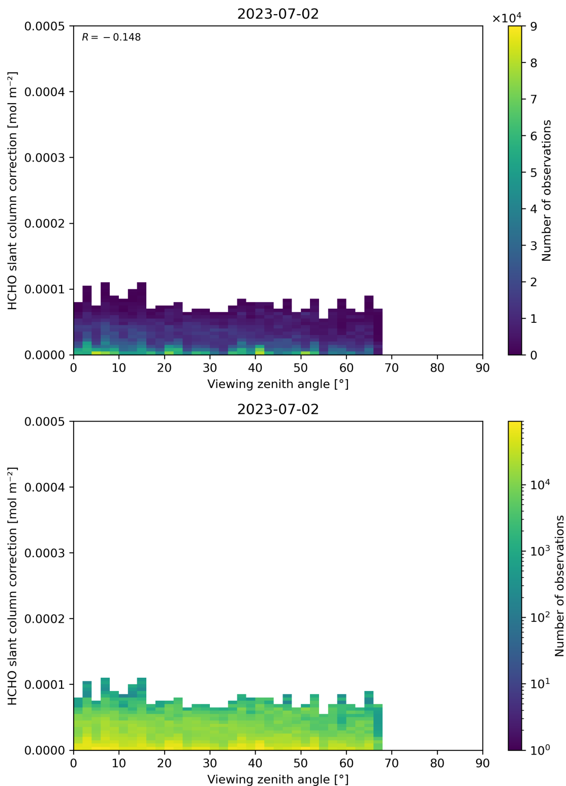
Figure 187: Scatter density plot of “Viewing zenith angle” against “HCHO slant column correction” for 2023-07-01 to 2023-07-03.
