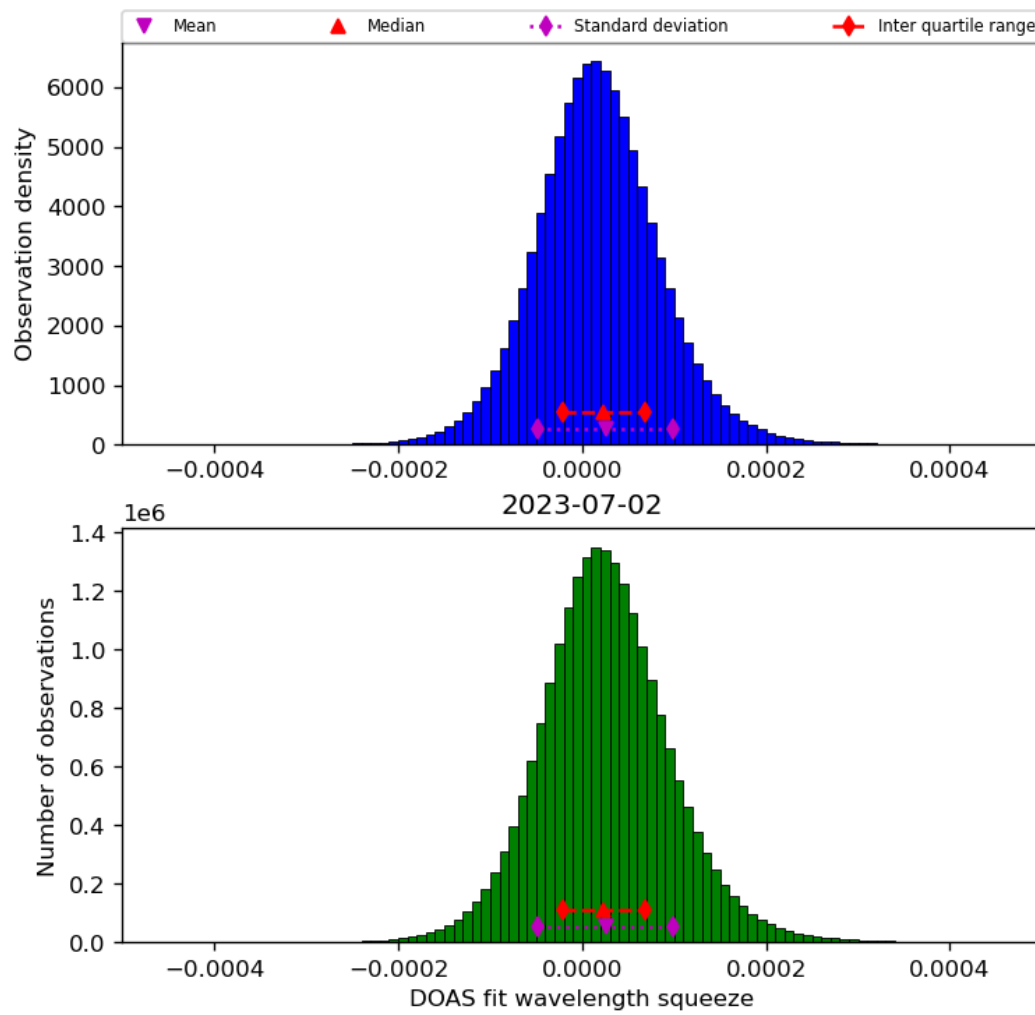
Figure 45: Histogram of “DOAS fit wavelength squeeze” for 2023-07-01 to 2023-07-03
