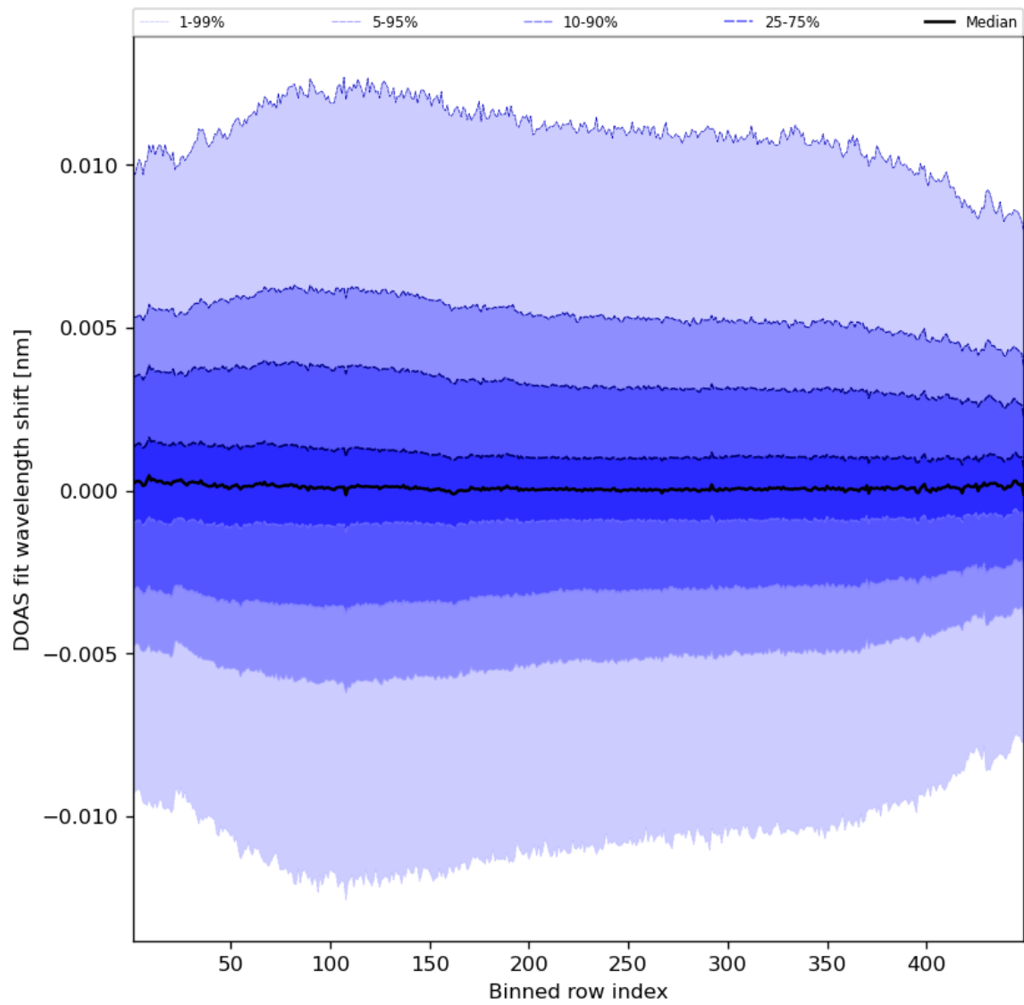
Figure 58: Along track statistics of “DOAS fit wavelength shift” for 2023-07-01 to 2023-07-03
