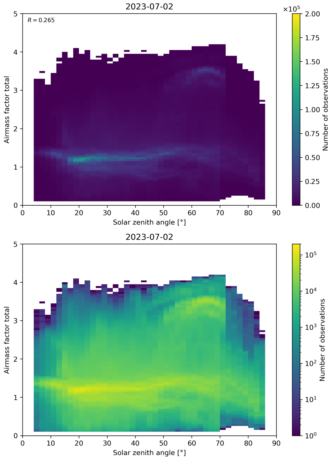
Figure 175: Scatter density plot of “Solar zenith angle” against “Airmass factor total” for 2023-07-01 to 2023-07-03.
