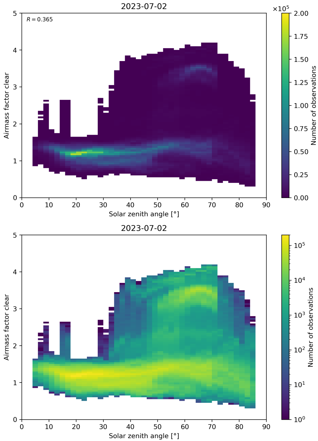
Figure 170: Scatter density plot of “Solar zenith angle” against “Airmass factor clear” for 2023-07-01 to 2023-07-03.
