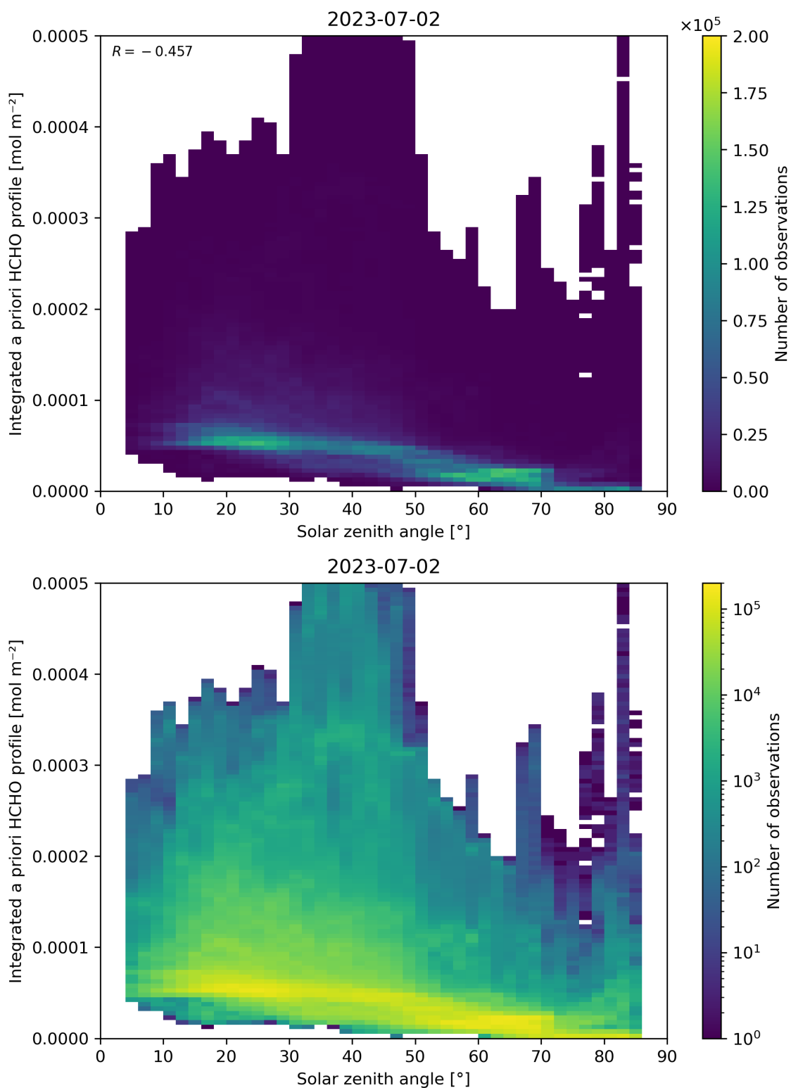
Figure 180: Scatter density plot of “Solar zenith angle” against “Integrated a priori HCHO profile” for 2023-07-01 to 2023-07-03.
