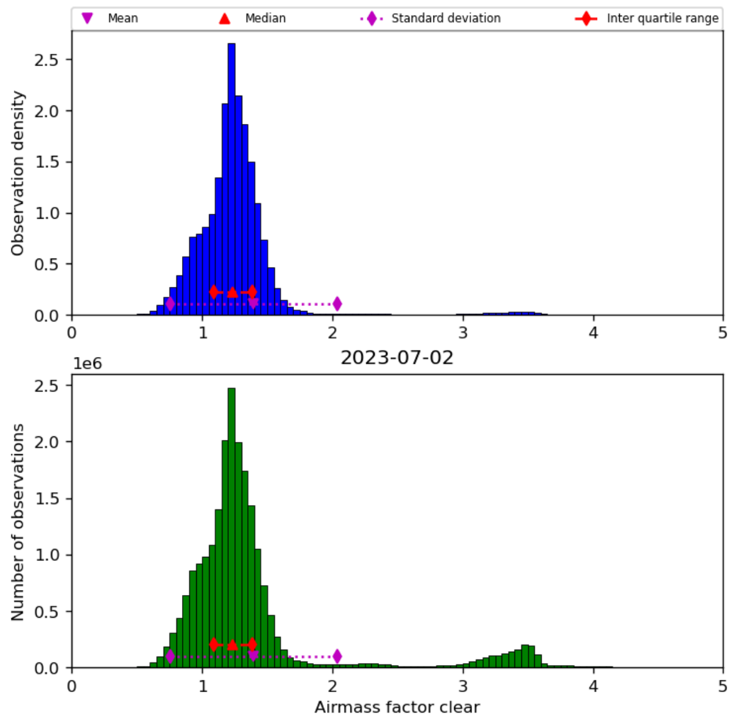
Figure 42: Histogram of “Airmass factor clear” for 2023-07-01 to 2023-07-03
