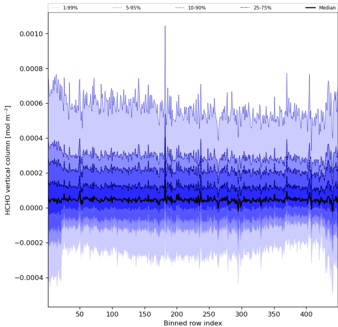
Figure 49: Along track statistics of “HCHO vertical column” for 2023-07-01 to 2023-07-03
