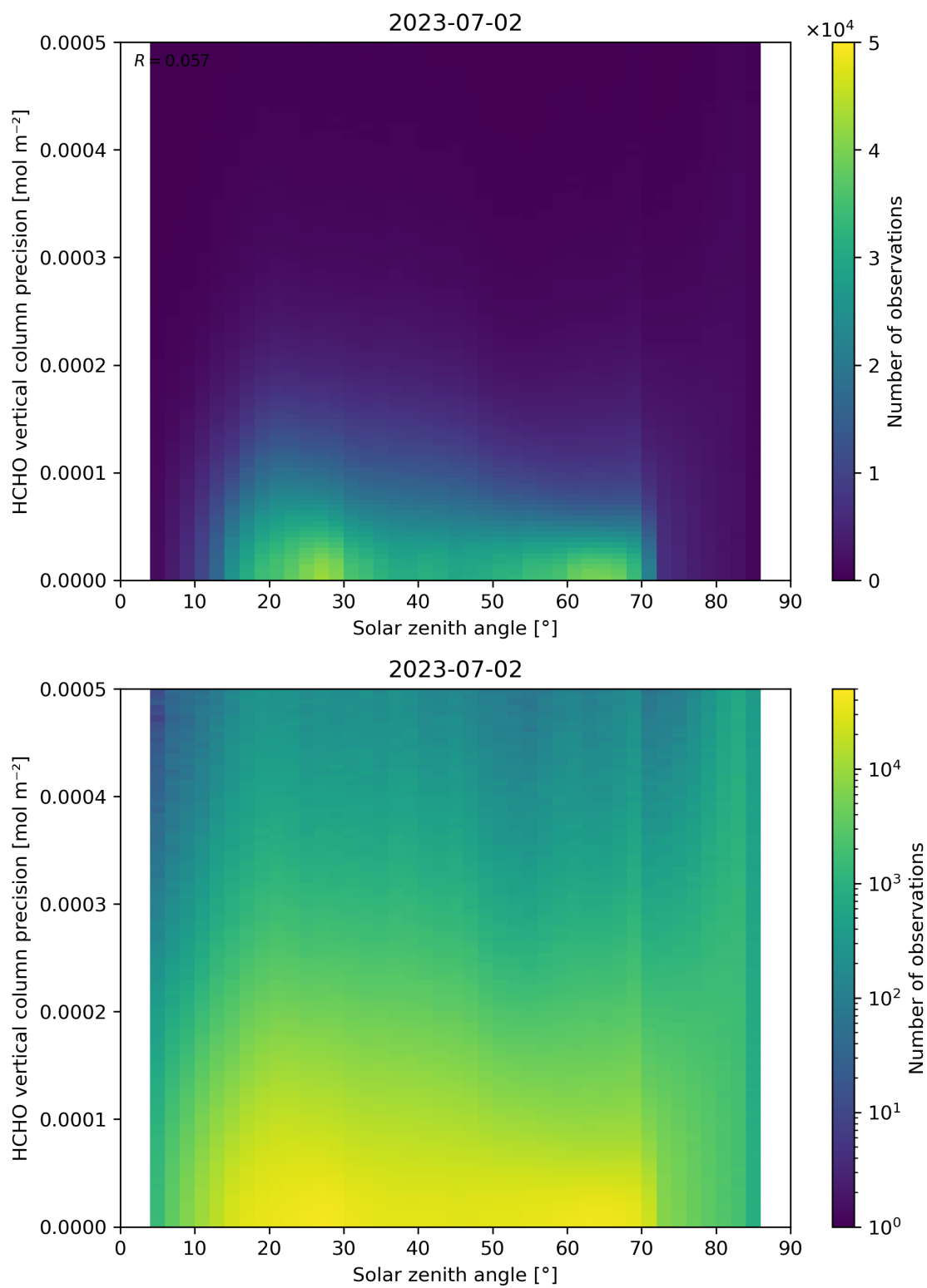
Figure 179: Scatter density plot of “Solar zenith angle” against “HCHO vertical column precision” for 2023-07-01 to 2023-07-03.
