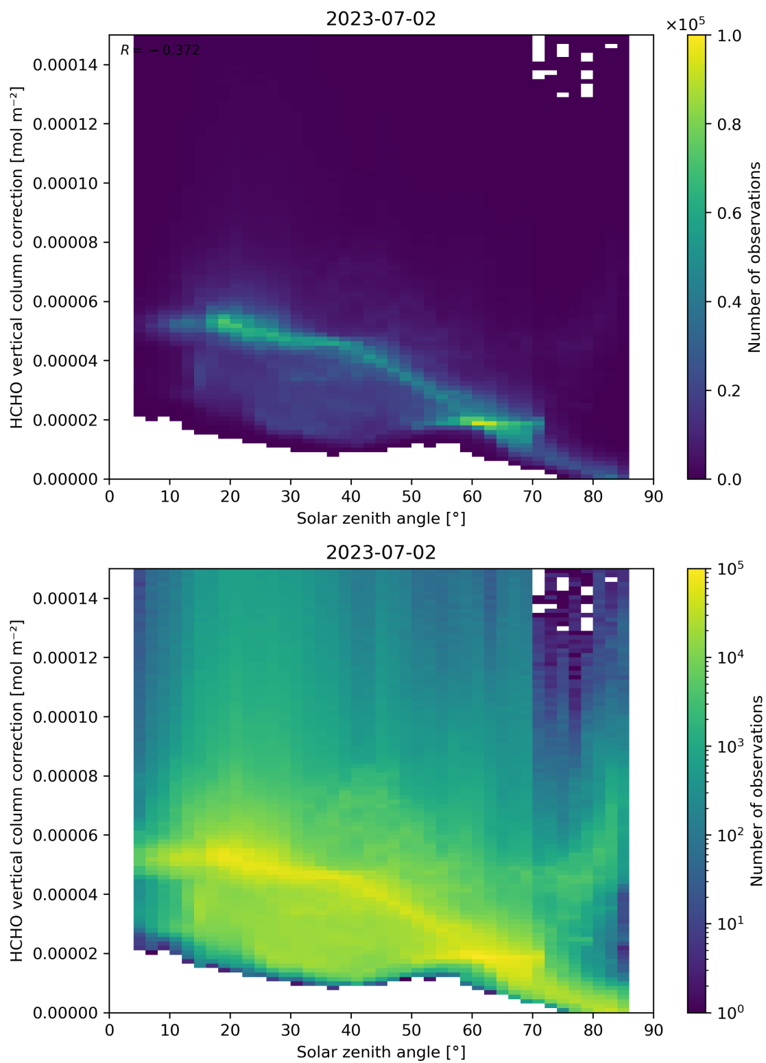
Figure 178: Scatter density plot of “Solar zenith angle” against “HCHO vertical column correction” for 2023-07-01 to 2023-07-03.
