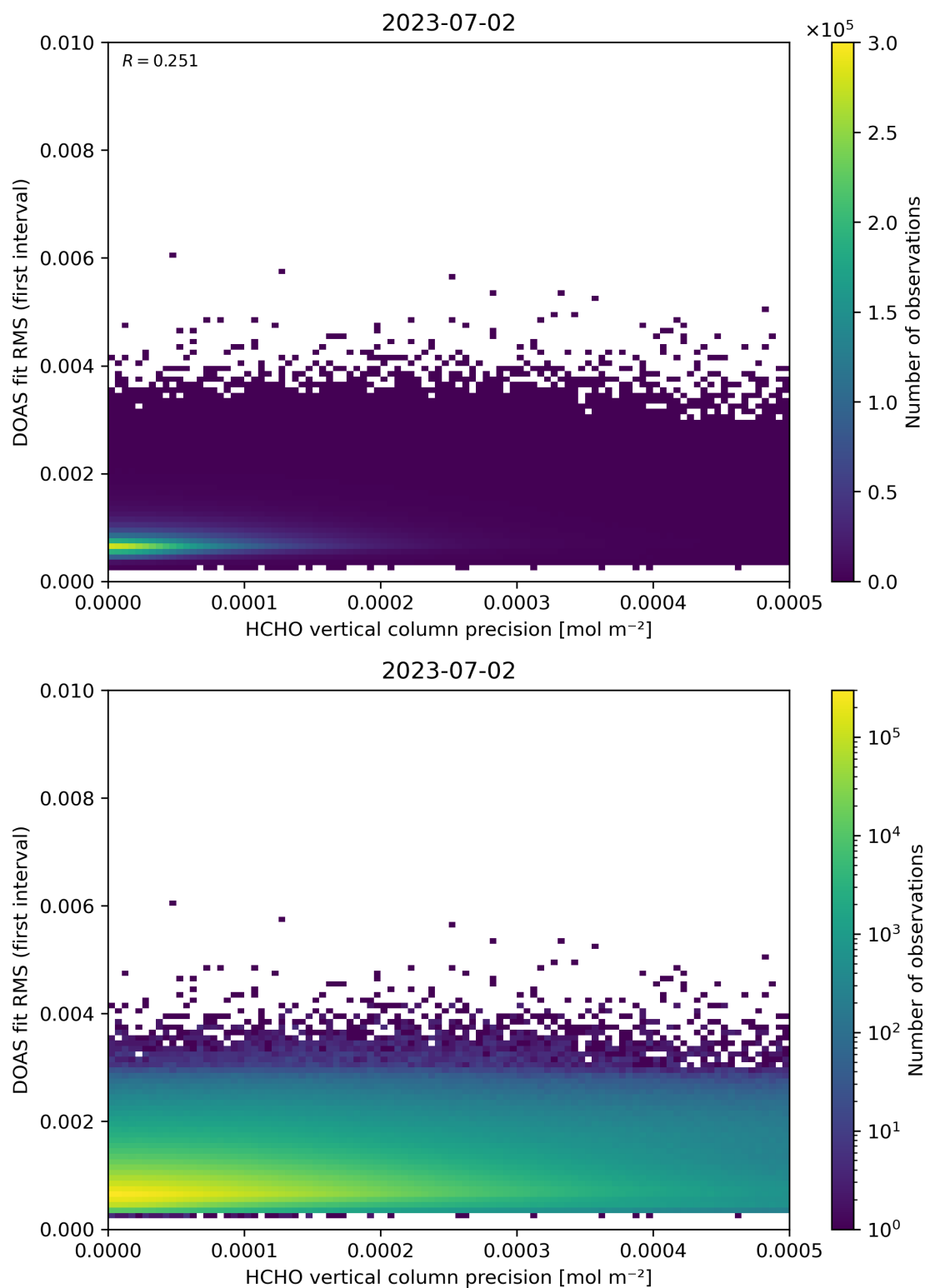
Figure 136: Scatter density plot of “HCHO vertical column precision” against “DOAS fit RMS (first interval)” for 2023-07-01 to 2023-07-03.
