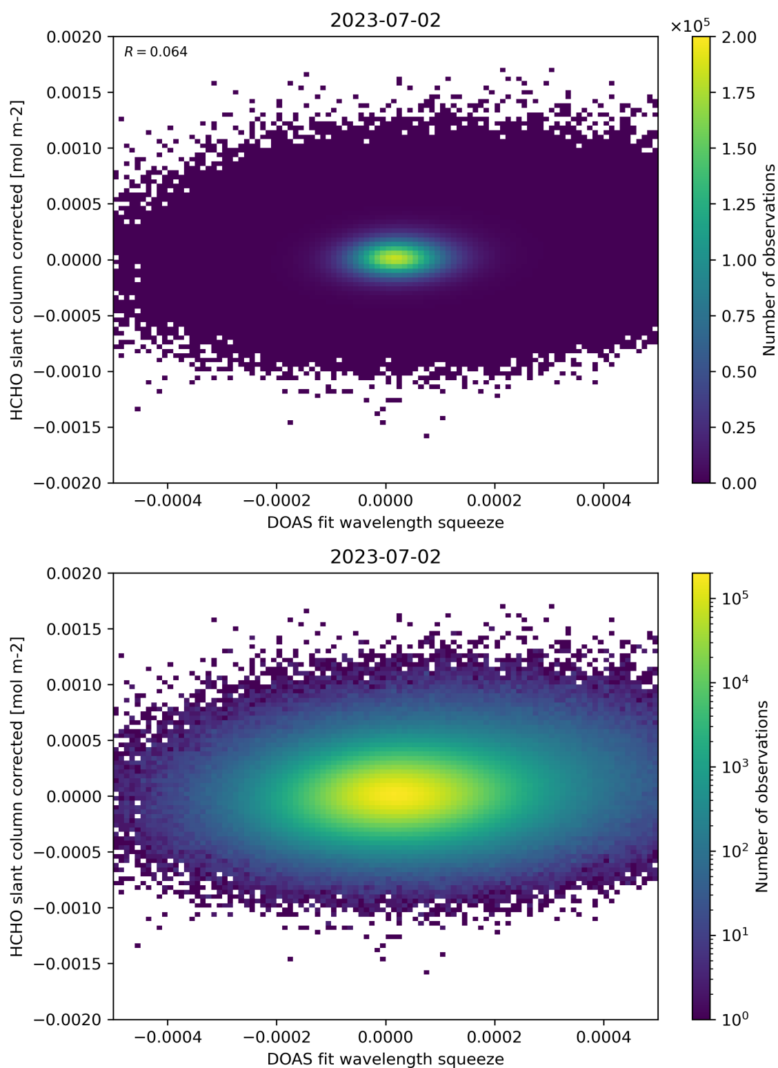
Figure 69: Scatter density plot of “DOAS fit wavelength squeeze” against “HCHO slant column corrected” for 2023-07-01 to 2023-07-03.
