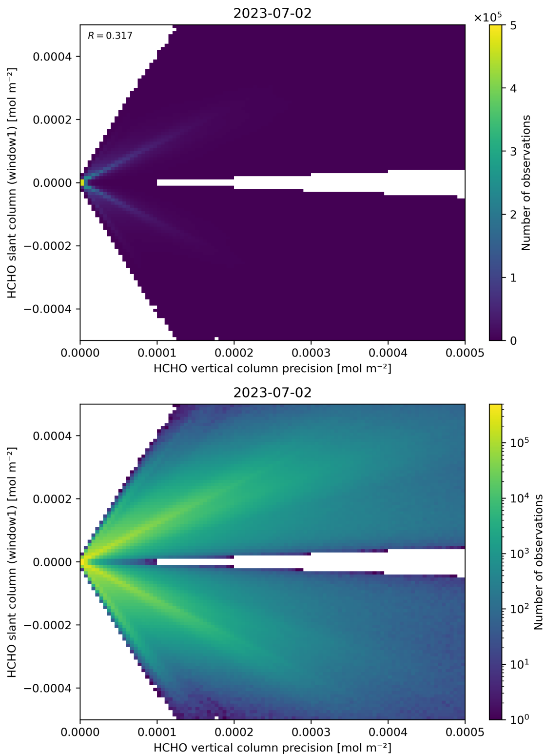
Figure 142: Scatter density plot of “HCHO vertical column precision” against “HCHO slant column (window1)” for 2023-07-01 to 2023-07-03.
