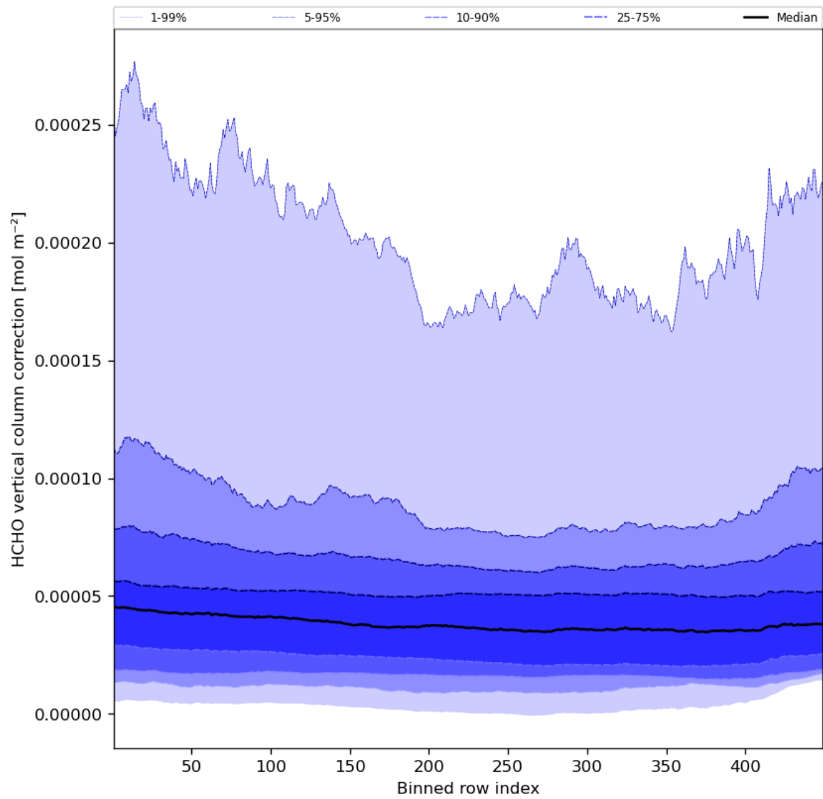
Figure 51: Along track statistics of “HCHO vertical column correction” for 2023-07-01 to 2023-07-03
