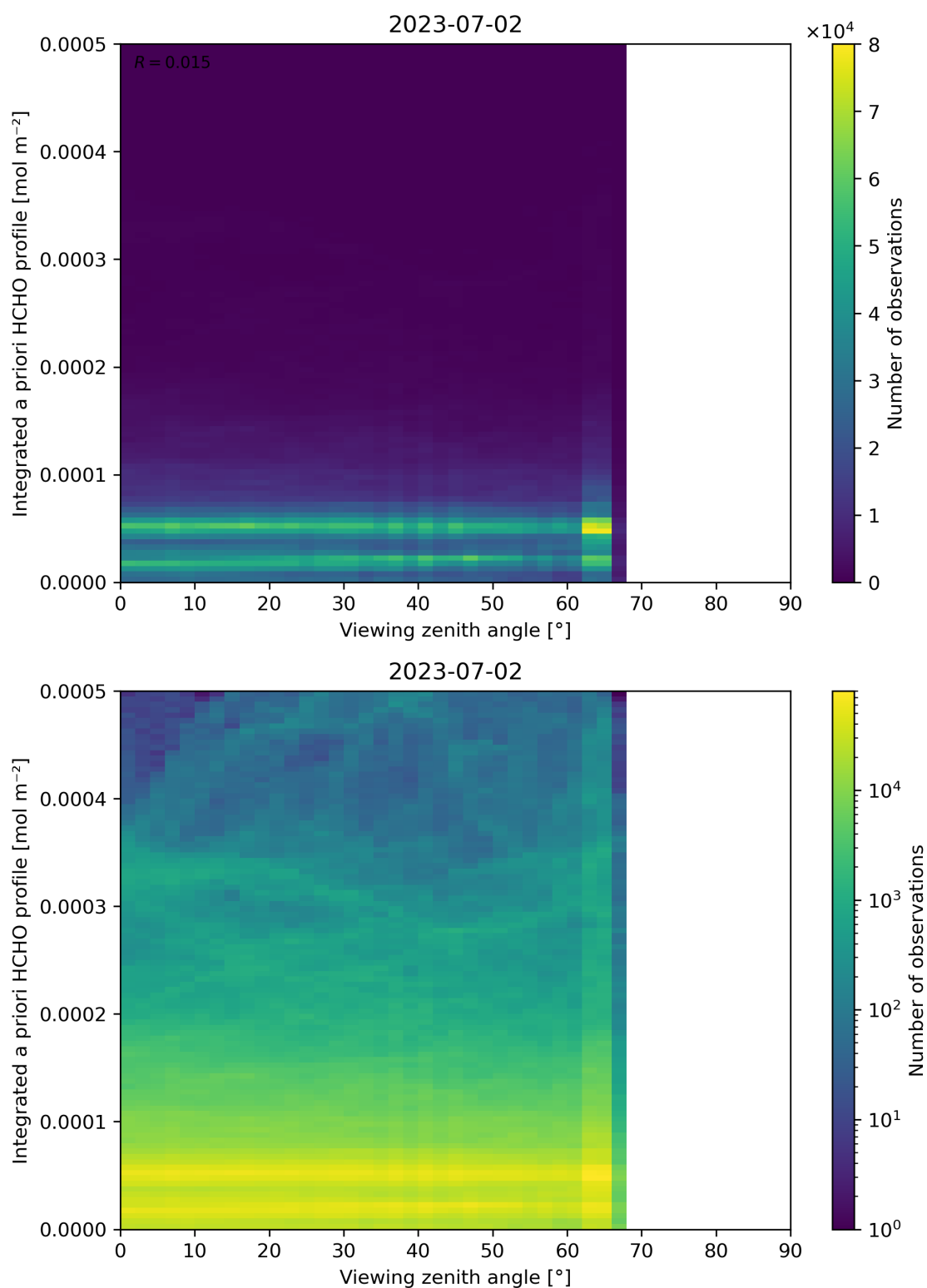
Figure 195: Scatter density plot of “Viewing zenith angle” against “Integrated a priori HCHO profile” for 2023-07-01 to 2023-07-03.
