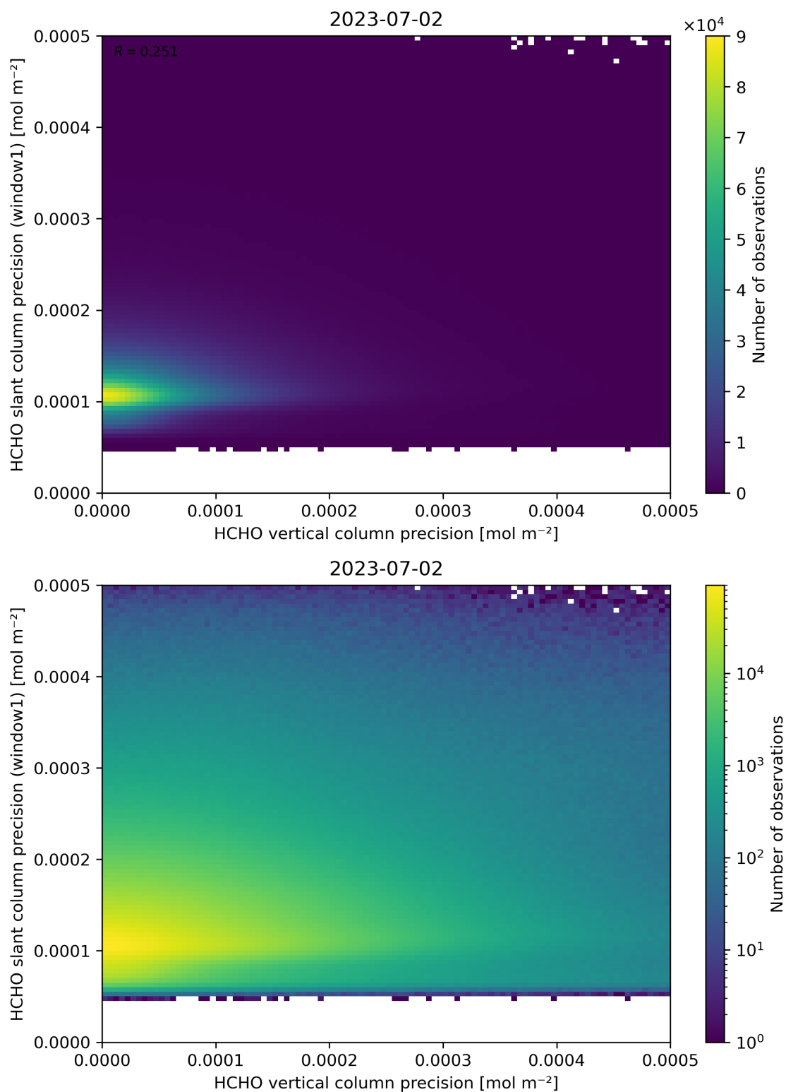
Figure 143: Scatter density plot of “HCHO vertical column precision” against “HCHO slant column precision (window1)” for 2023-07-01 to 2023-07-03.
