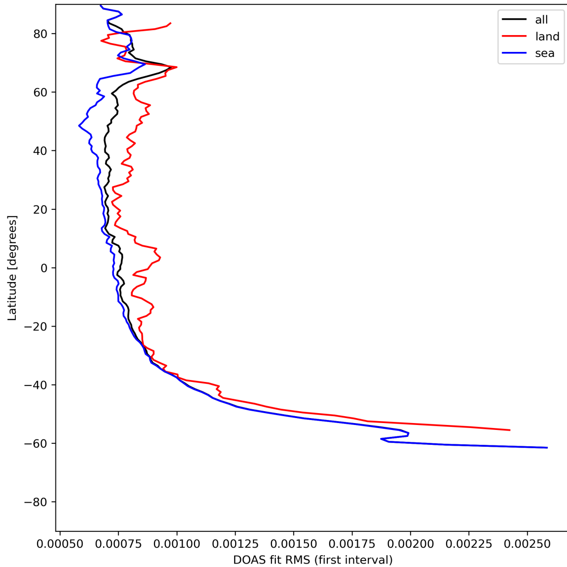
Figure 32: Zonal average of “DOAS fit RMS (first interval)” for 2023-07-01 to 2023-07-03.
