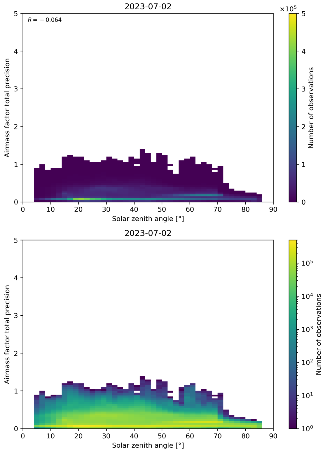
Figure 176: Scatter density plot of “Solar zenith angle” against “Airmass factor total precision” for 2023-07-01 to 2023-07-03.
