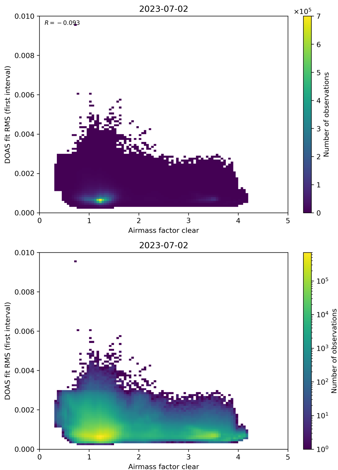
Figure 71: Scatter density plot of “Airmass factor clear” against “DOAS fit RMS (first interval)” for 2023-07-01 to 2023-07-03.
