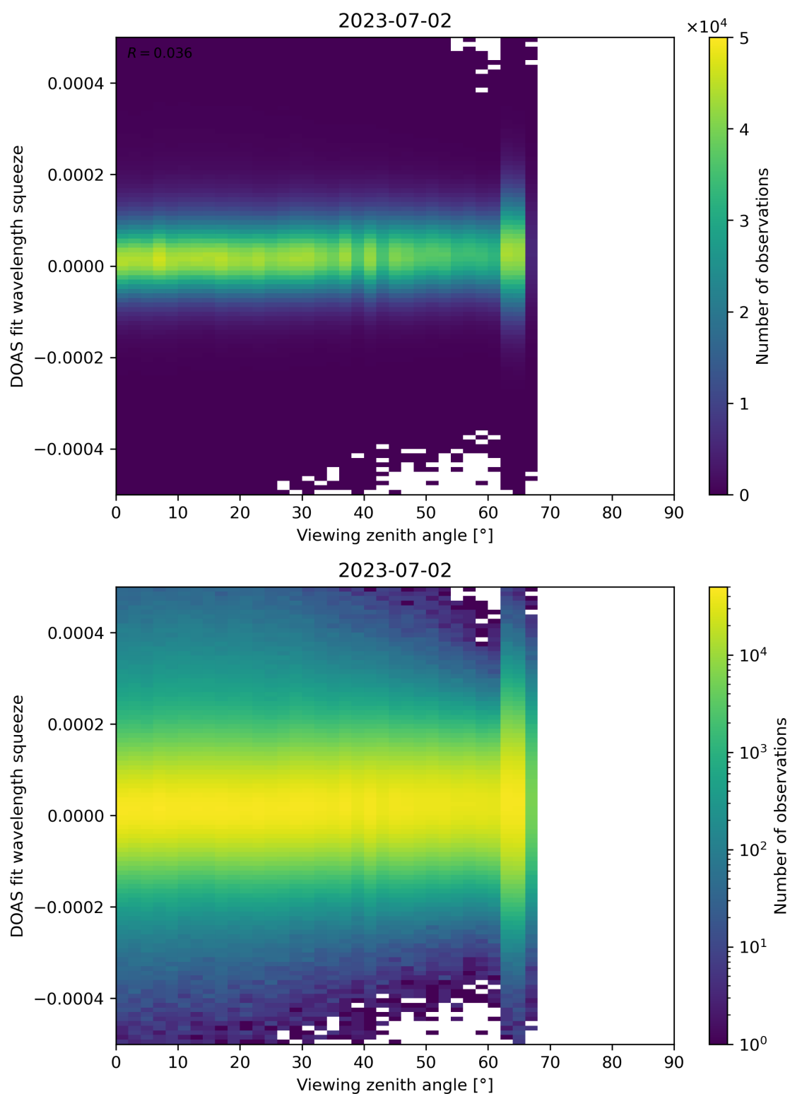
Figure 184: Scatter density plot of “Viewing zenith angle” against “DOAS fit wavelength squeeze” for 2023-07-01 to 2023-07-03.
