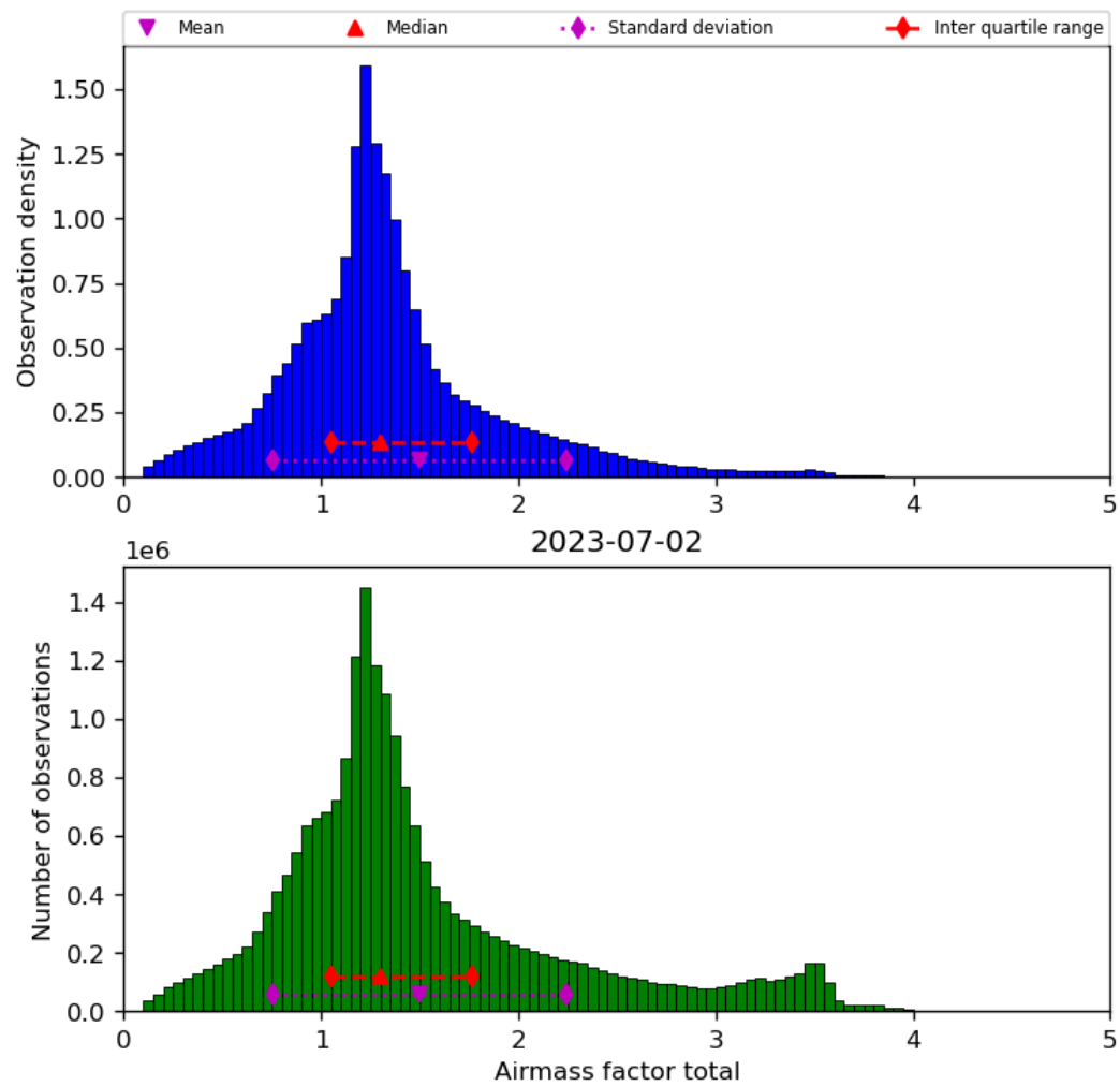
Figure 40: Histogram of “Airmass factor total” for 2023-07-01 to 2023-07-03
