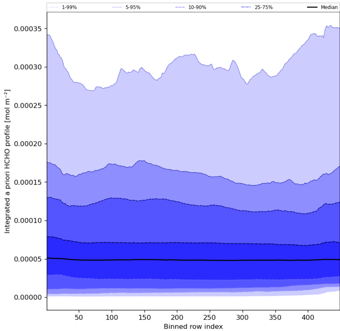
Figure 57: Along track statistics of “Integrated a priori HCHO profile” for 2023-07-01 to 2023-07-03
