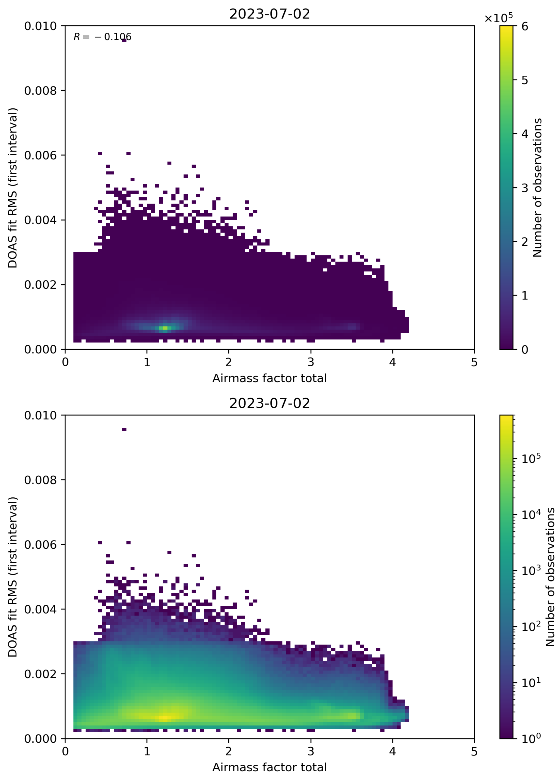
Figure 97: Scatter density plot of “Airmass factor total” against “DOAS fit RMS (first interval)” for 2023-07-01 to 2023-07-03.
