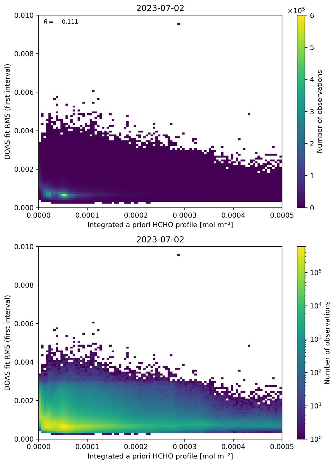
Figure 148: Scatter density plot of “Integrated a priori HCHO profile” against “DOAS fit RMS (first interval)” for 2023-07-01 to 2023-07-03.
