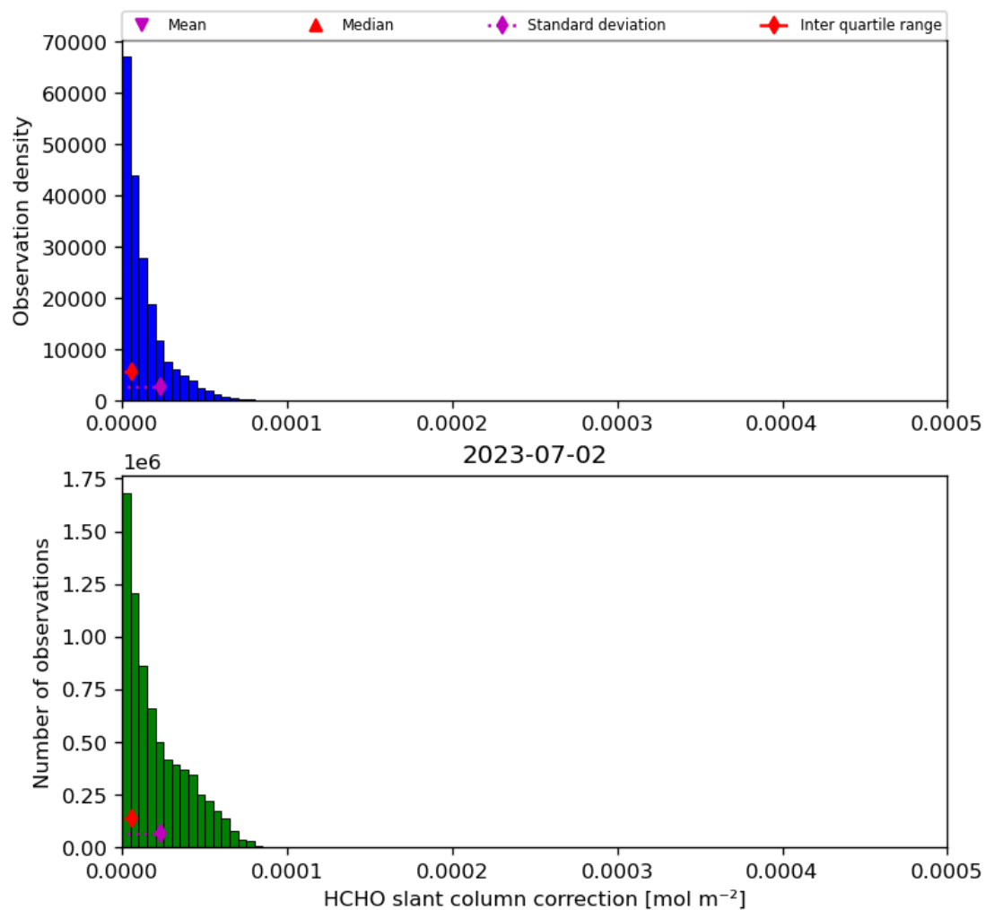
Figure 47: Histogram of “HCHO slant column correction” for 2023-07-01 to 2023-07-03
