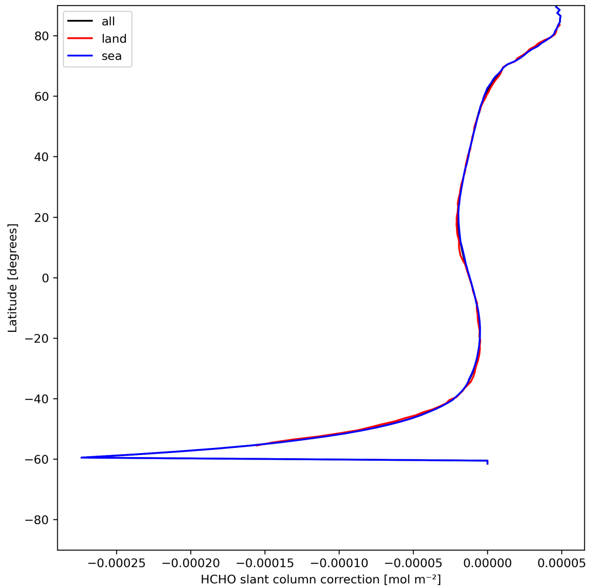
Figure 33: Zonal average of “HCHO slant column correction” for 2023-07-01 to 2023-07-03.
