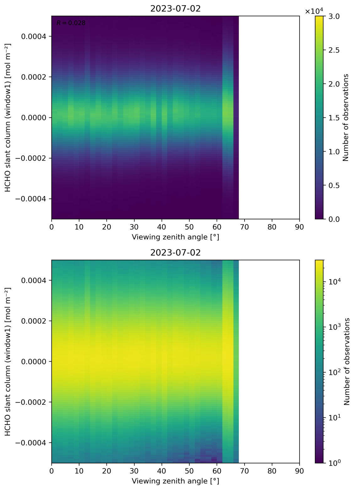
Figure 188: Scatter density plot of “Viewing zenith angle” against “HCHO slant column (window1)” for 2023-07-01 to 2023-07-03.
