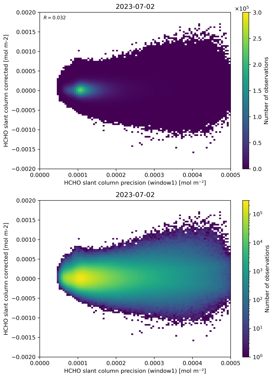
Figure 92: Scatter density plot of “HCHO slant column precision (window1)” against “HCHO slant column corrected” for 2023-07-01 to 2023-07-03.
