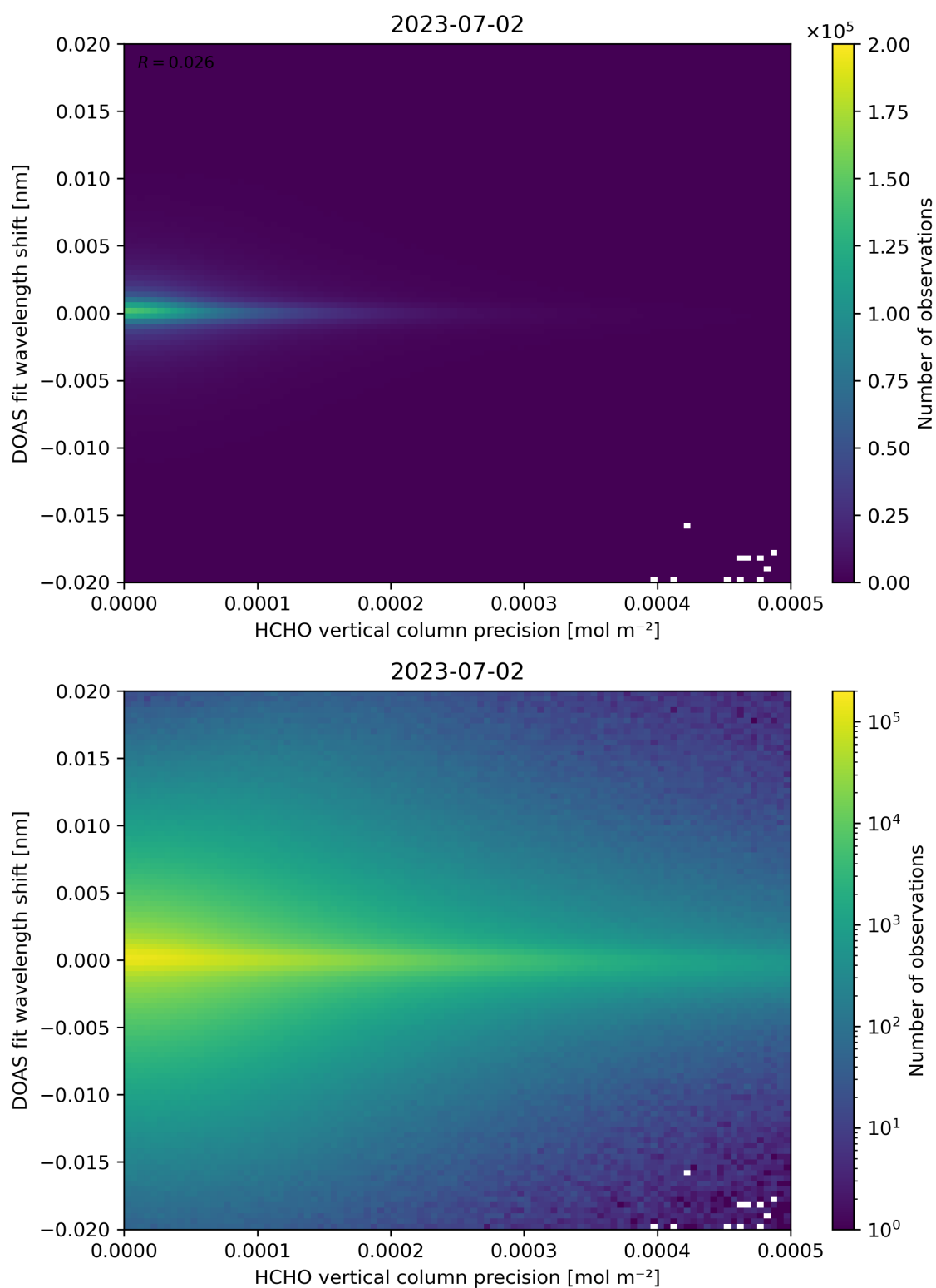
Figure 137: Scatter density plot of “HCHO vertical column precision” against “DOAS fit wavelength shift” for 2023-07-01 to 2023-07-03.
