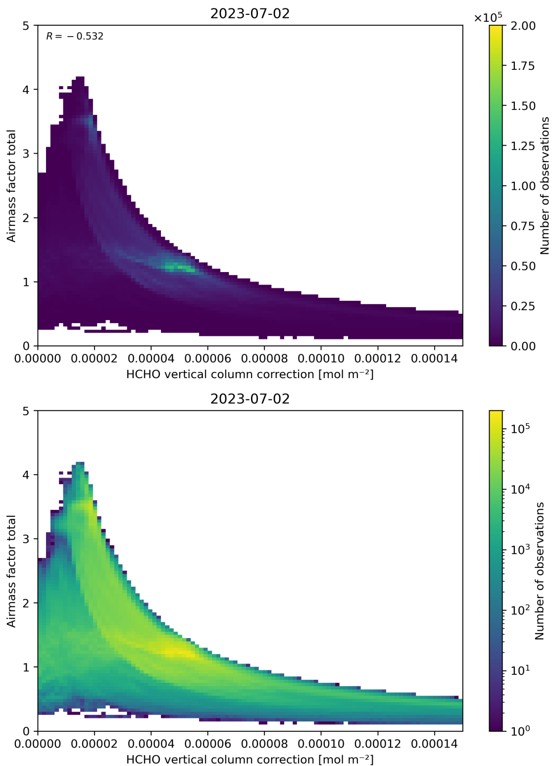
Figure 120: Scatter density plot of “HCHO vertical column correction” against “Airmass factor total” for 2023-07-01 to 2023-07-03.
