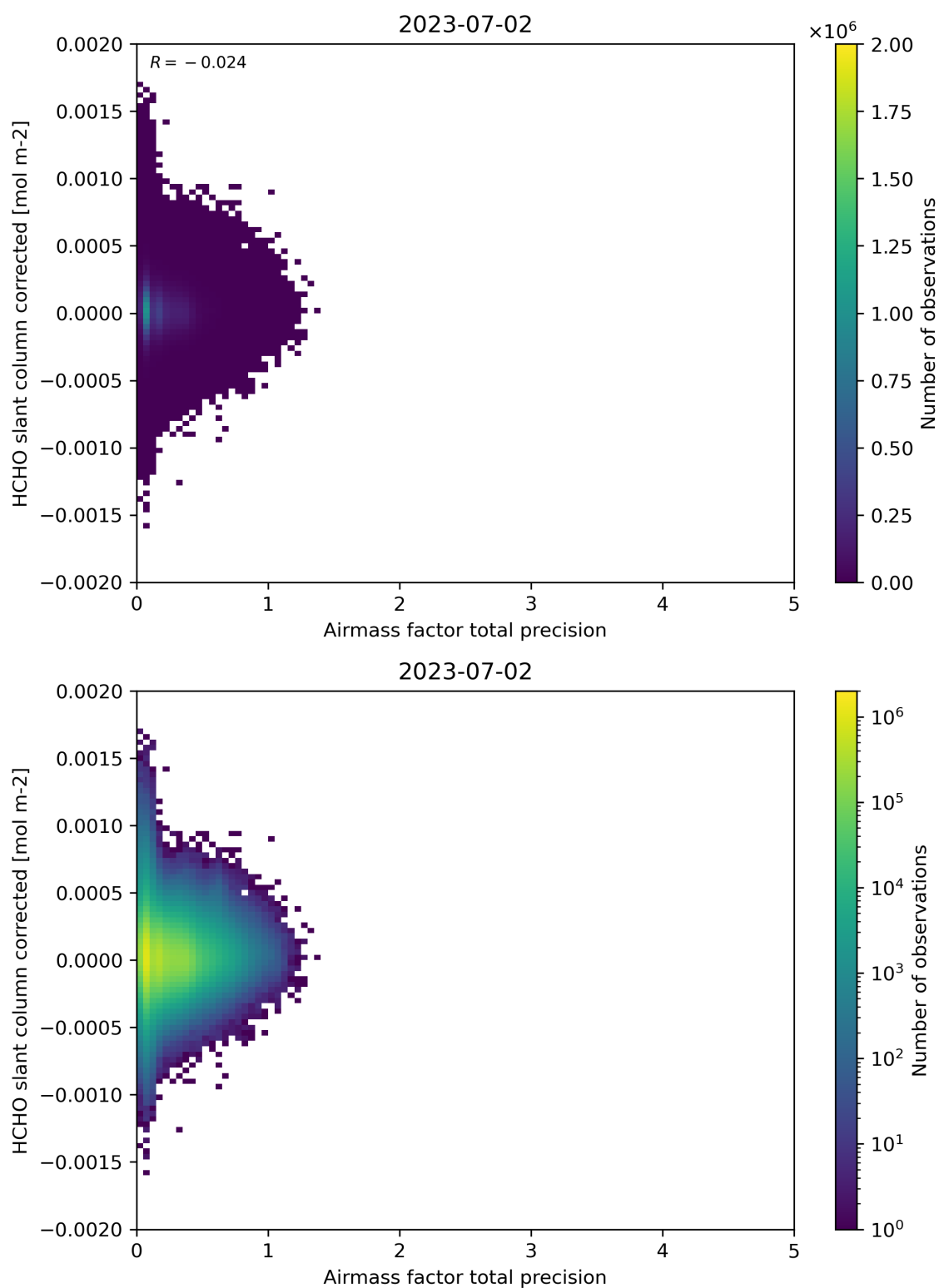
Figure 109: Scatter density plot of “Airmass factor total precision” against “HCHO slant column corrected” for 2023-07-01 to 2023-07-03.
