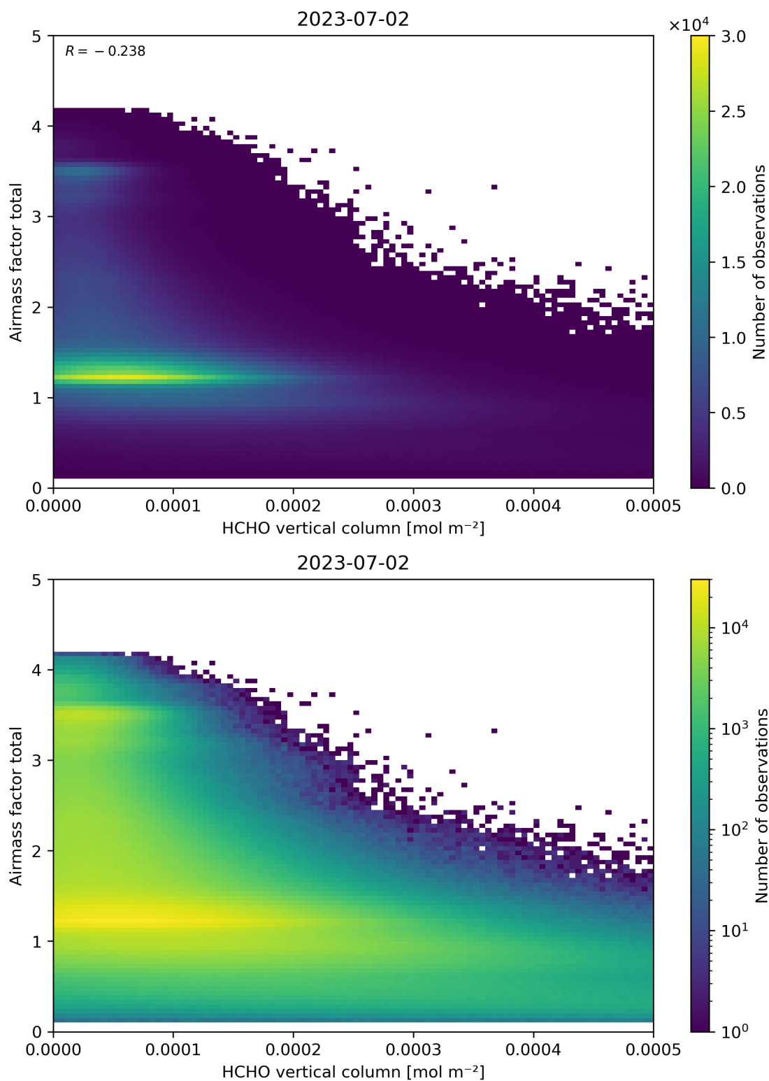
Figure 131: Scatter density plot of “HCHO vertical column” against “Airmass factor total” for 2023-07-01 to 2023-07-03.
