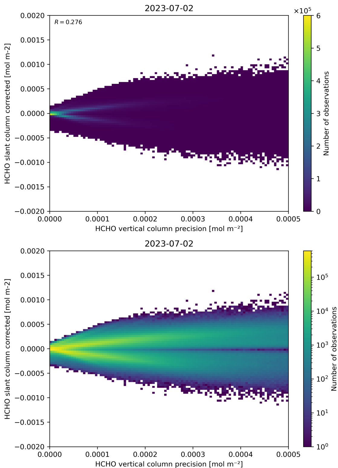
Figure 140: Scatter density plot of “HCHO vertical column precision” against “HCHO slant column corrected” for 2023-07-01 to 2023-07-03.
