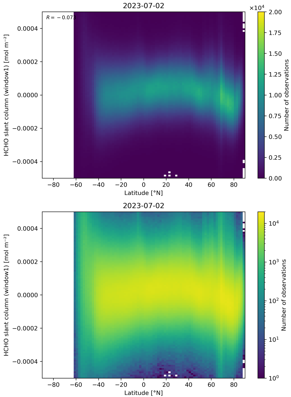
Figure 159: Scatter density plot of “Latitude” against “HCHO slant column (window1)” for 2023-07-01 to 2023-07-03.
