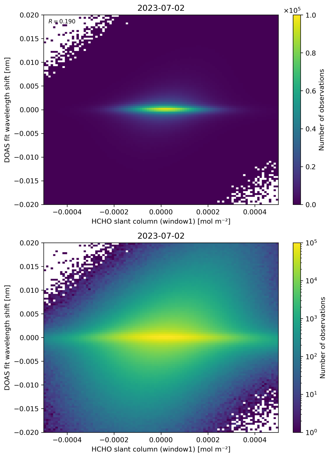
Figure 79: Scatter density plot of “HCHO slant column (window1)” against “DOAS fit wavelength shift” for 2023-07-01 to 2023-07-03.
