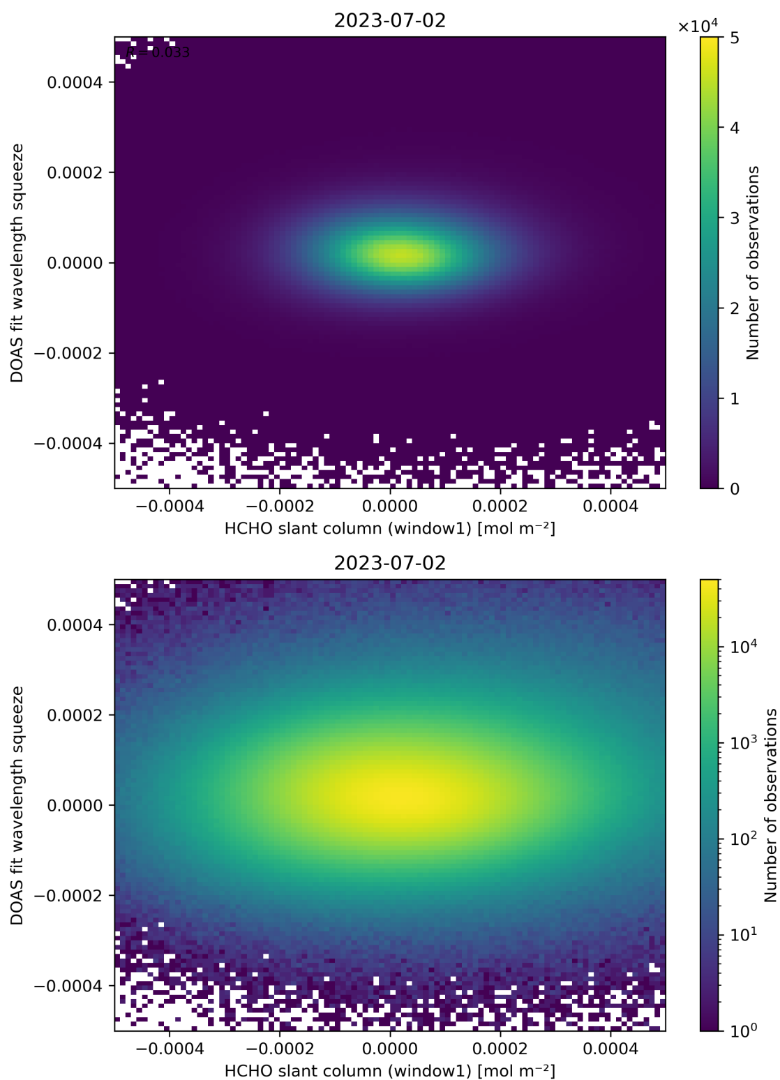
Figure 80: Scatter density plot of “HCHO slant column (window1)” against “DOAS fit wavelength squeeze” for 2023-07-01 to 2023-07-03.
