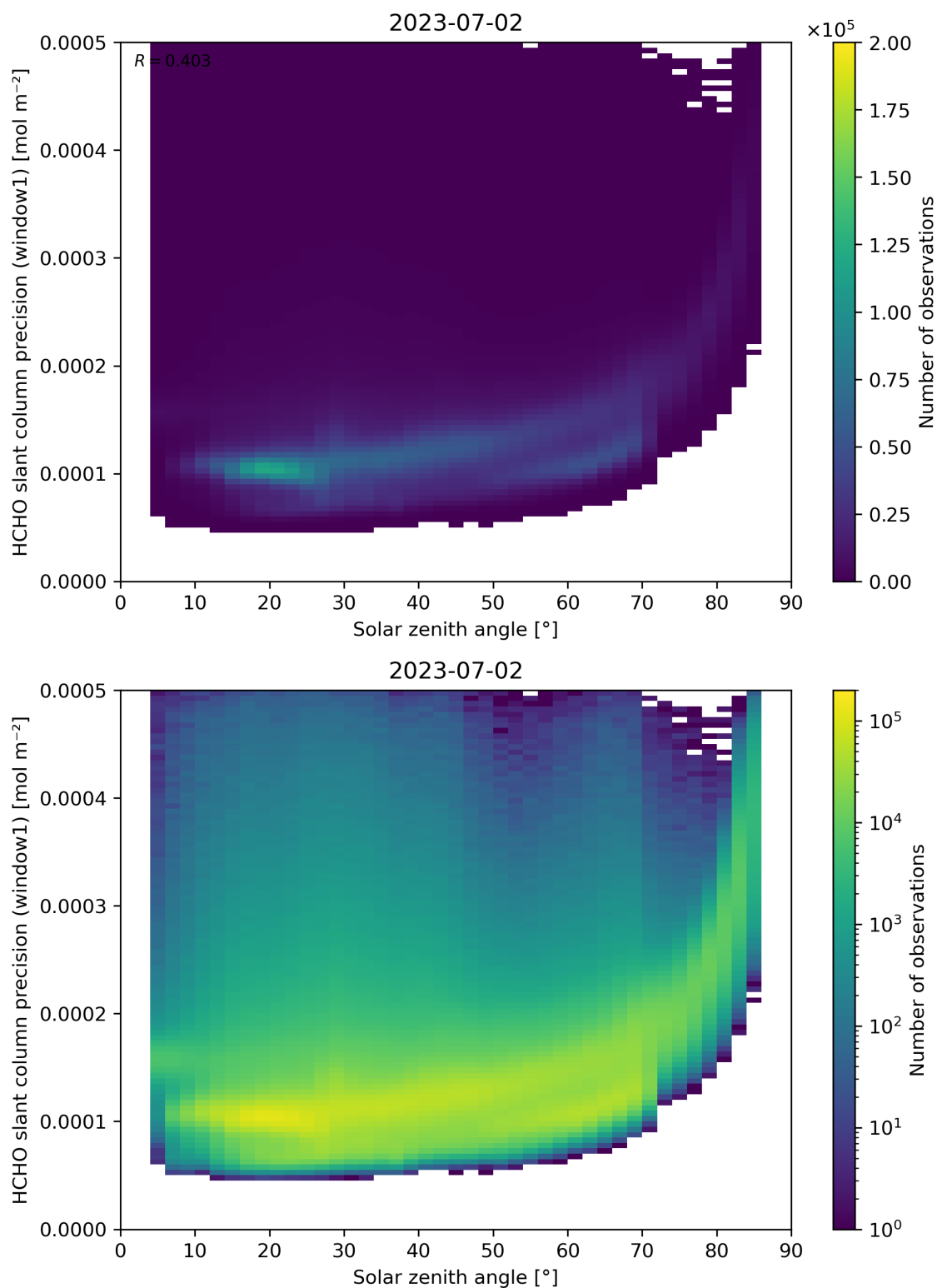
Figure 174: Scatter density plot of “Solar zenith angle” against “HCHO slant column precision (window1)” for 2023-07-01 to 2023-07-03.
