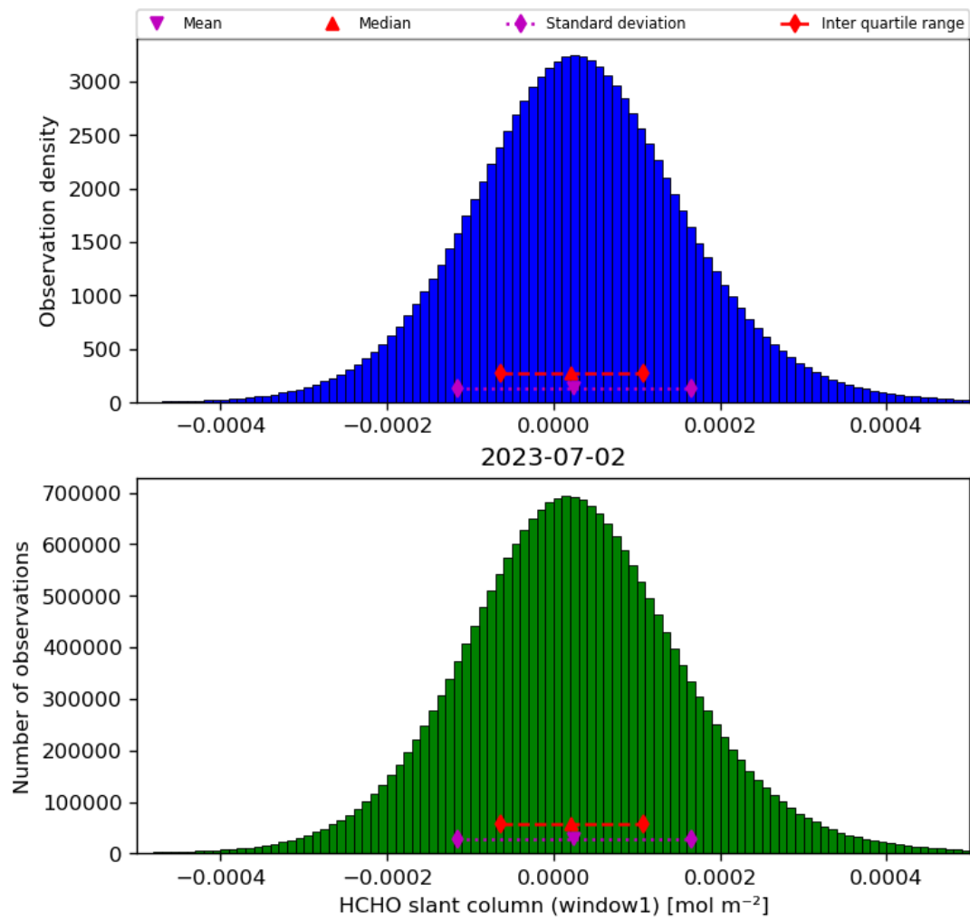
Figure 38: Histogram of “HCHO slant column (window1)” for 2023-07-01 to 2023-07-03
