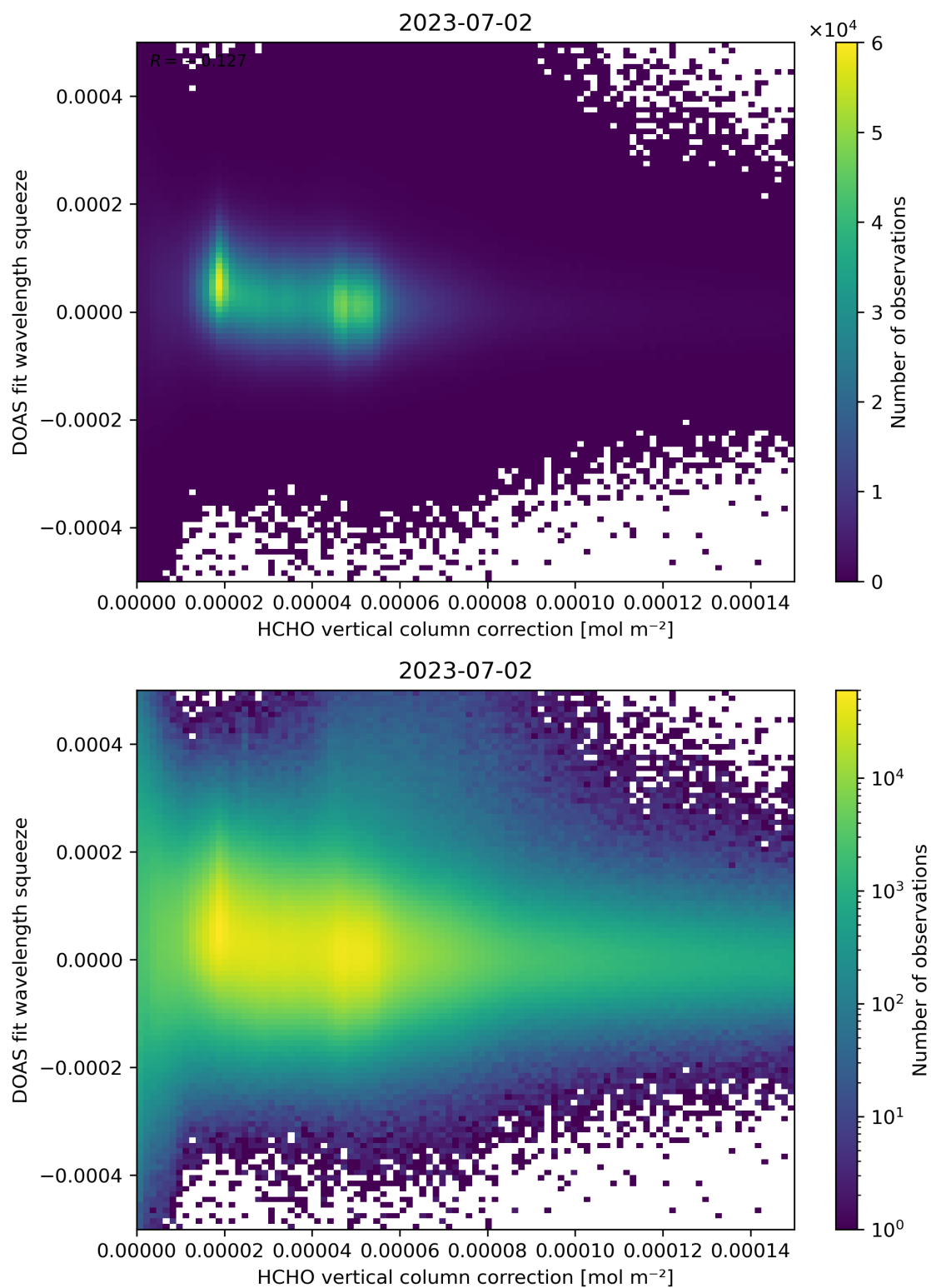
Figure 114: Scatter density plot of “HCHO vertical column correction” against “DOAS fit wavelength squeeze” for 2023-07-01 to 2023-07-03.
