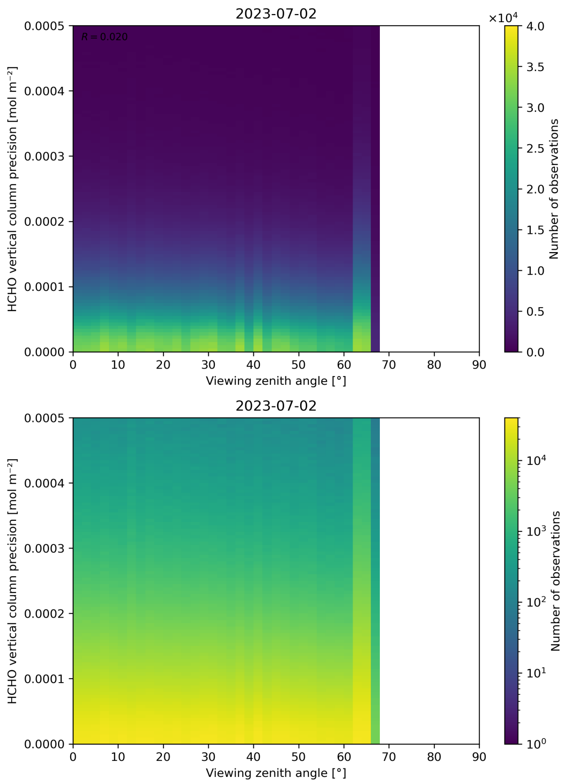
Figure 194: Scatter density plot of “Viewing zenith angle” against “HCHO vertical column precision” for 2023-07-01 to 2023-07-03.
