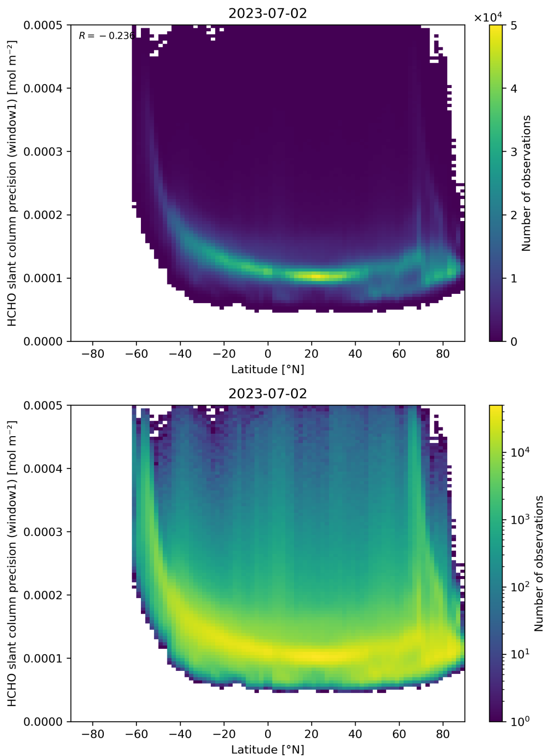
Figure 160: Scatter density plot of “Latitude” against “HCHO slant column precision (window1)” for 2023-07-01 to 2023-07-03.
