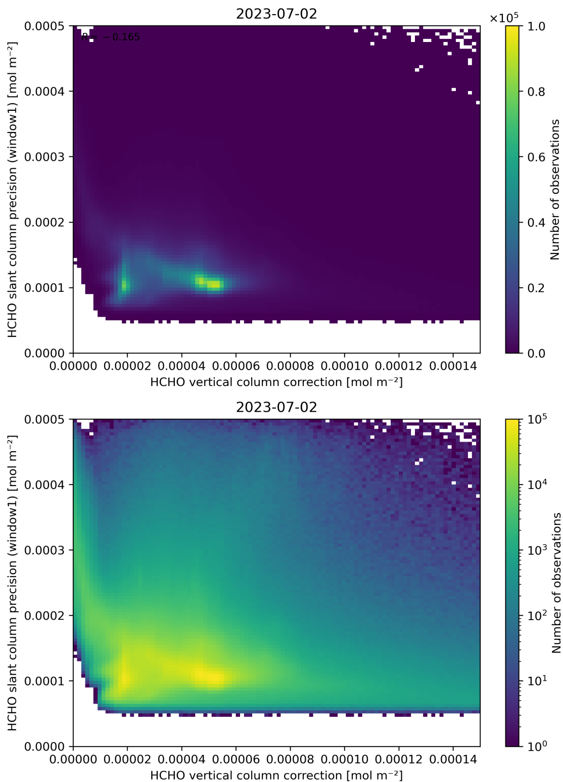
Figure 119: Scatter density plot of “HCHO vertical column correction” against “HCHO slant column precision (window1)” for 2023-07-01 to 2023-07-03.
