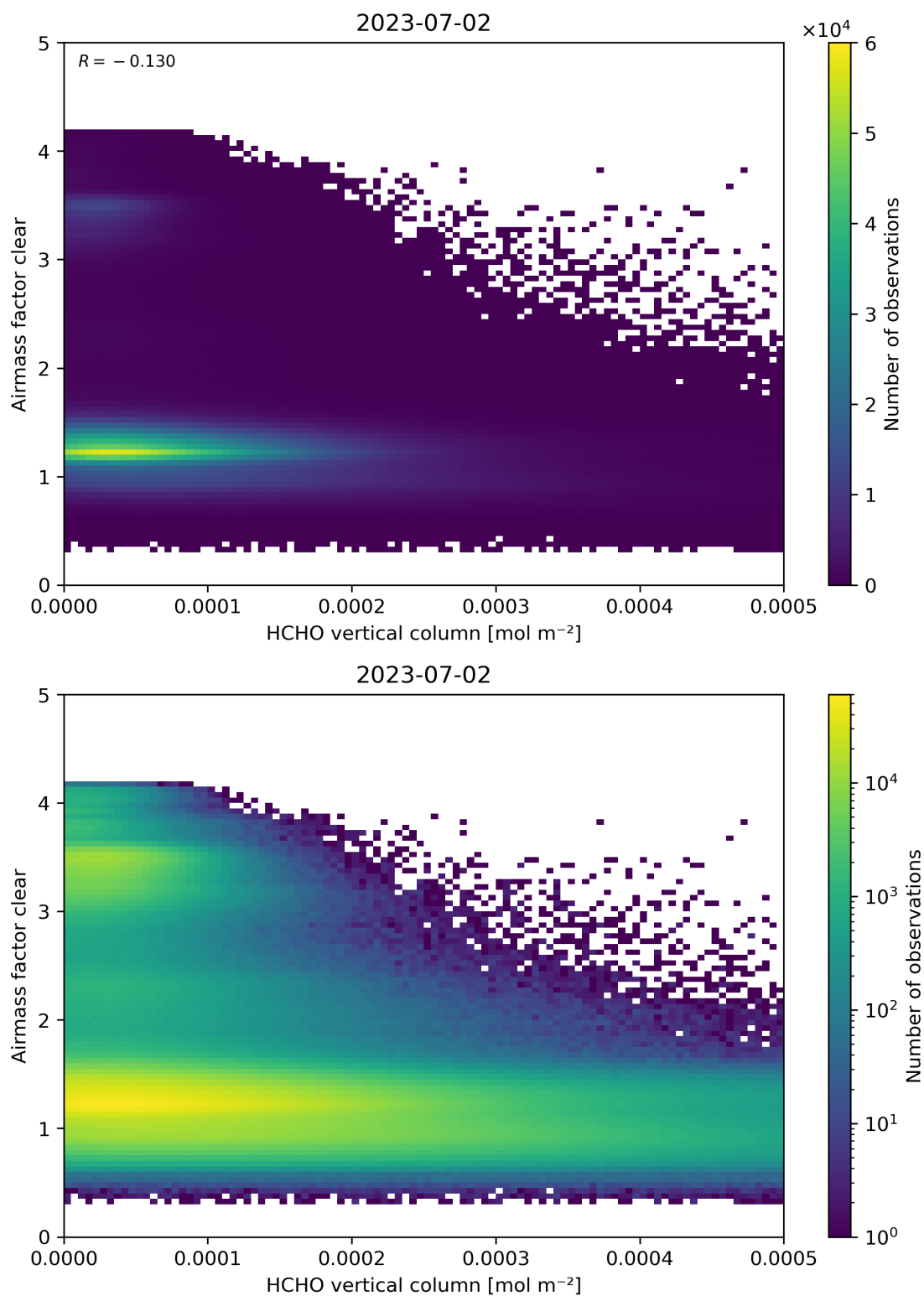
Figure 126: Scatter density plot of “HCHO vertical column” against “Airmass factor clear” for 2023-07-01 to 2023-07-03.
