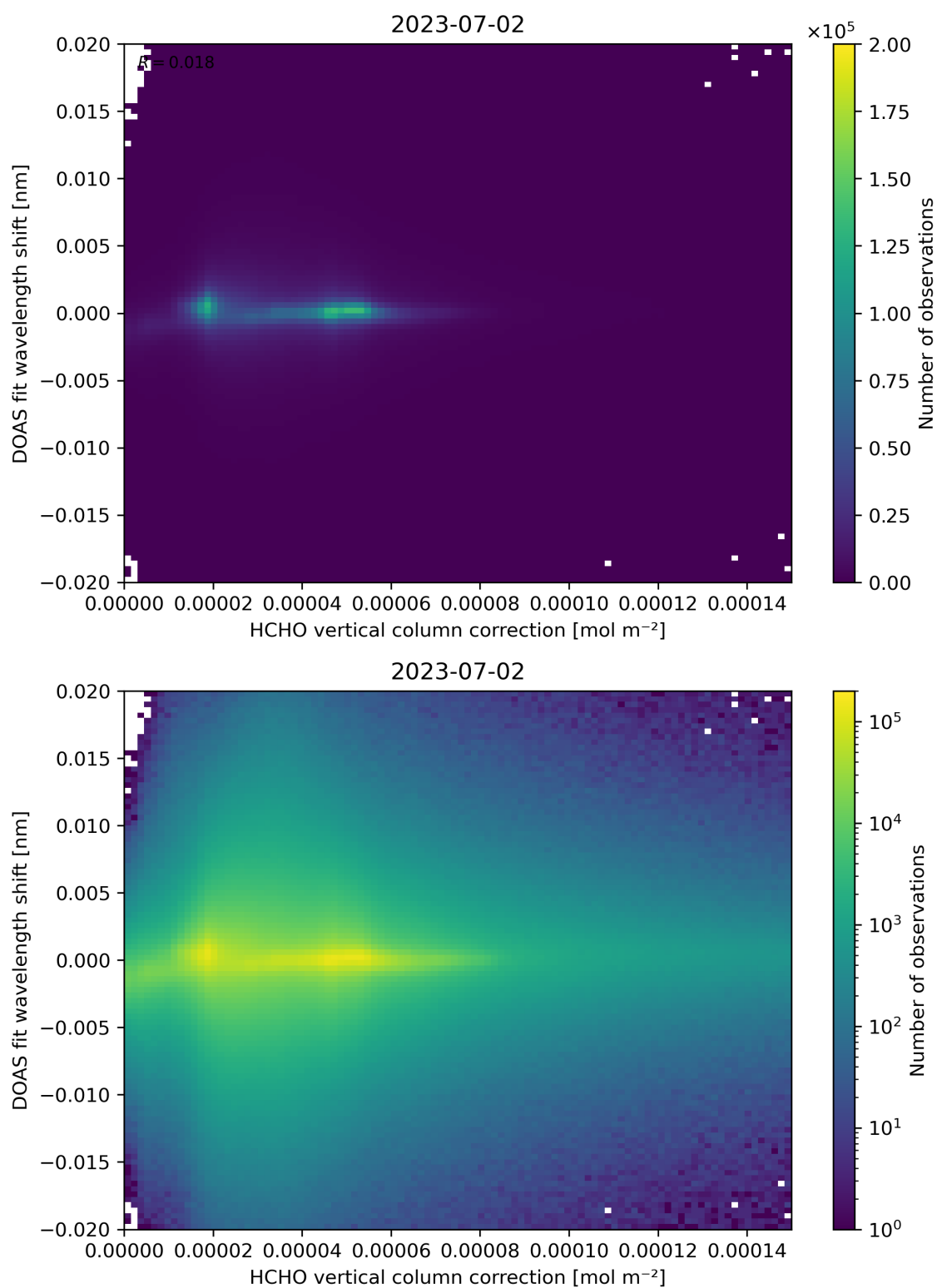
Figure 113: Scatter density plot of “HCHO vertical column correction” against “DOAS fit wavelength shift” for 2023-07-01 to 2023-07-03.
