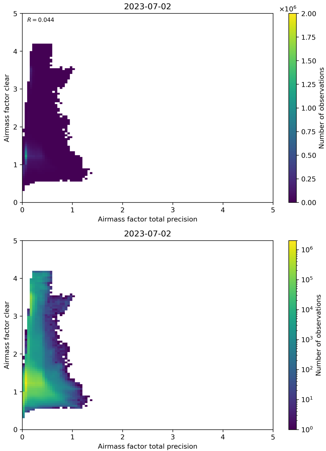
Figure 108: Scatter density plot of “Airmass factor total precision” against “Airmass factor clear” for 2023-07-01 to 2023-07-03.
