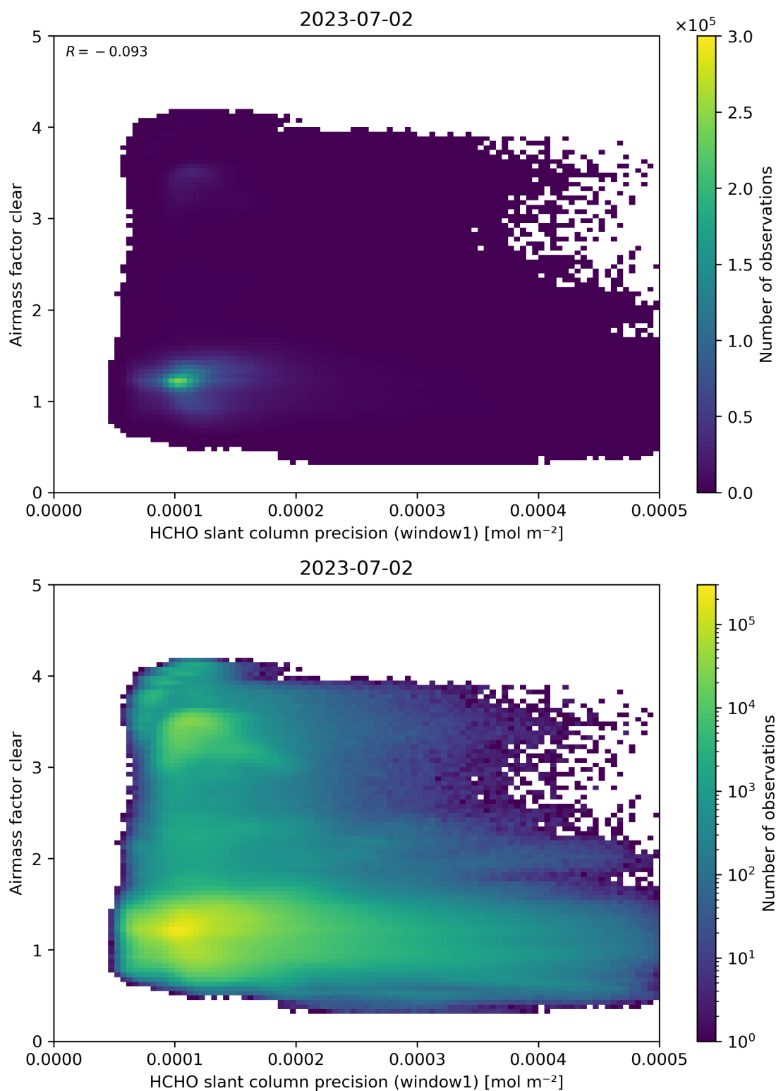
Figure 91: Scatter density plot of “HCHO slant column precision (window1)” against “Airmass factor clear” for 2023-07-01 to 2023-07-03.
