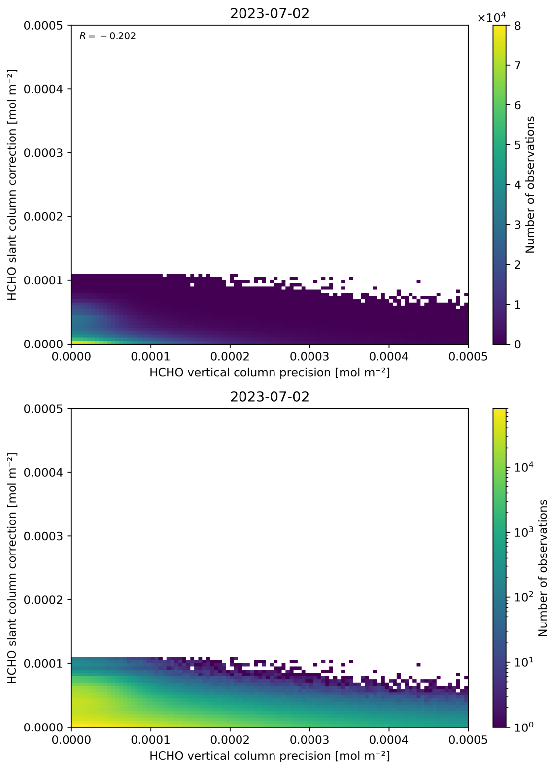
Figure 141: Scatter density plot of “HCHO vertical column precision” against “HCHO slant column correction” for 2023-07-01 to 2023-07-03.
