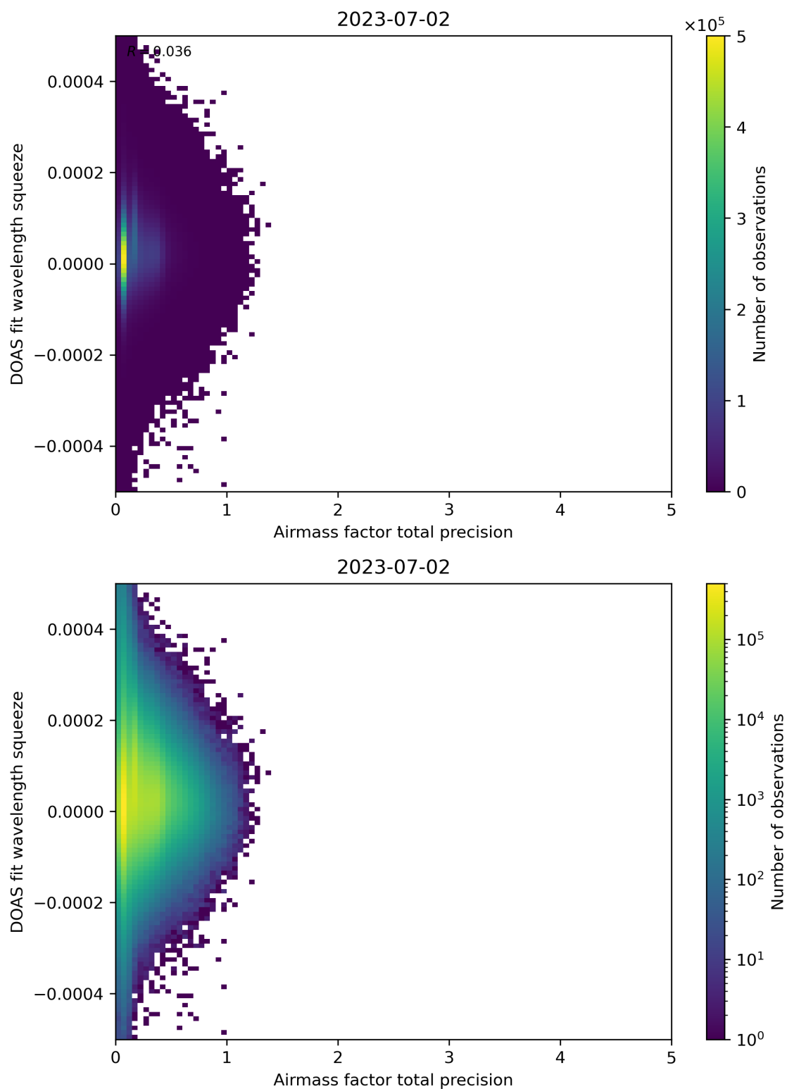
Figure 107: Scatter density plot of “Airmass factor total precision” against “DOAS fit wavelength squeeze” for 2023-07-01 to 2023-07-03.
