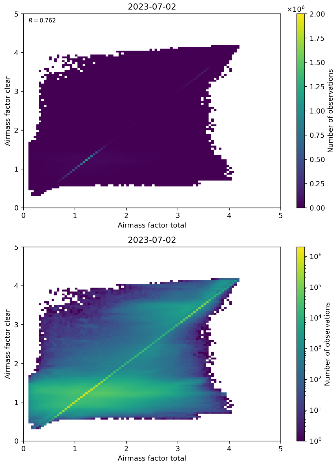
Figure 100: Scatter density plot of “Airmass factor total” against “Airmass factor clear” for 2023-07-01 to 2023-07-03.
