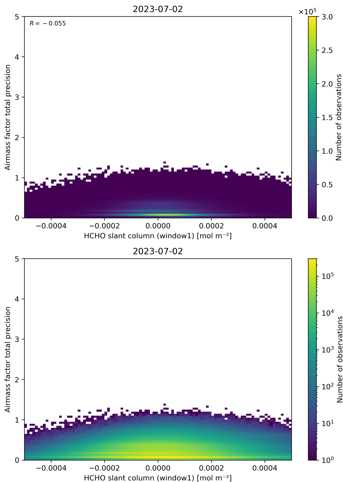
Figure 86: Scatter density plot of “HCHO slant column (window1)” against “Airmass factor total precision” for 2023-07-01 to 2023-07-03.
