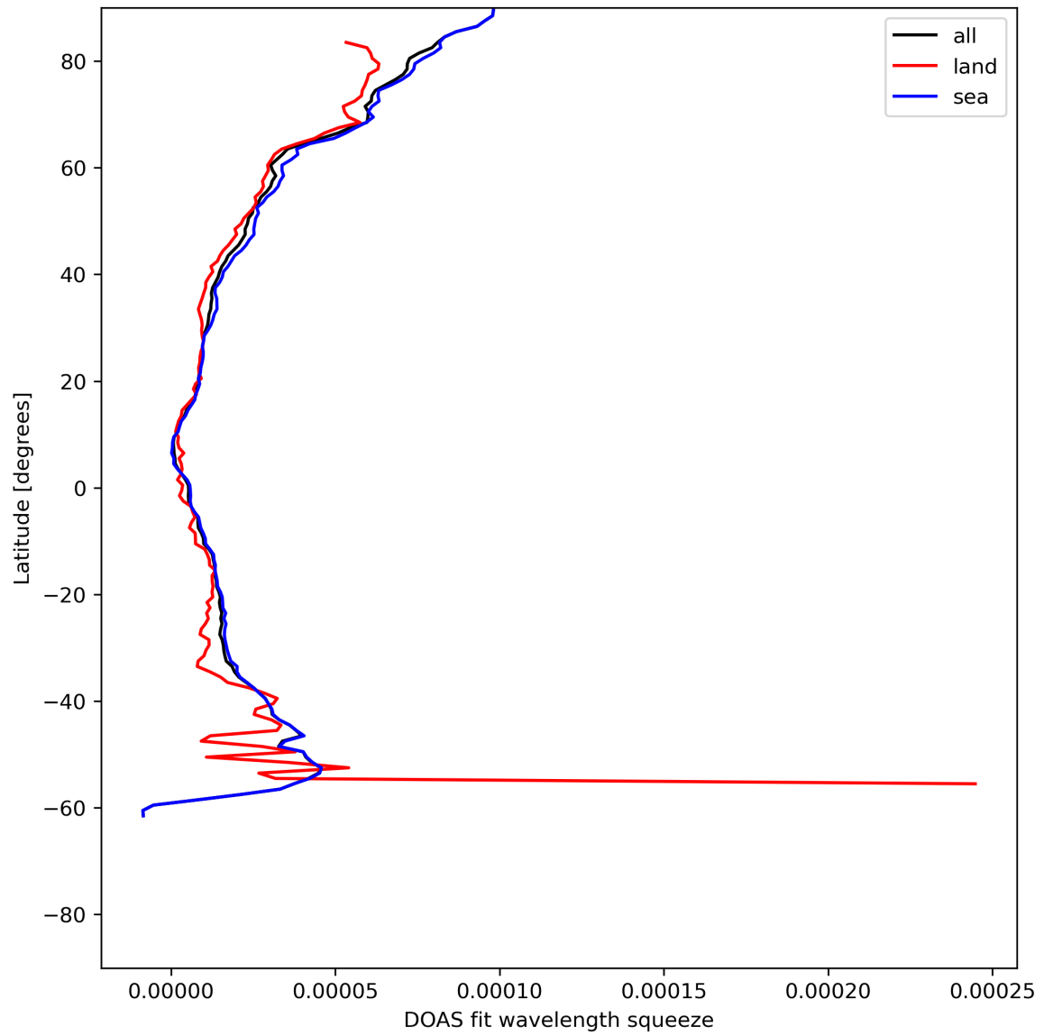
Figure 31: Zonal average of “DOAS fit wavelength squeeze” for 2023-07-01 to 2023-07-03.
