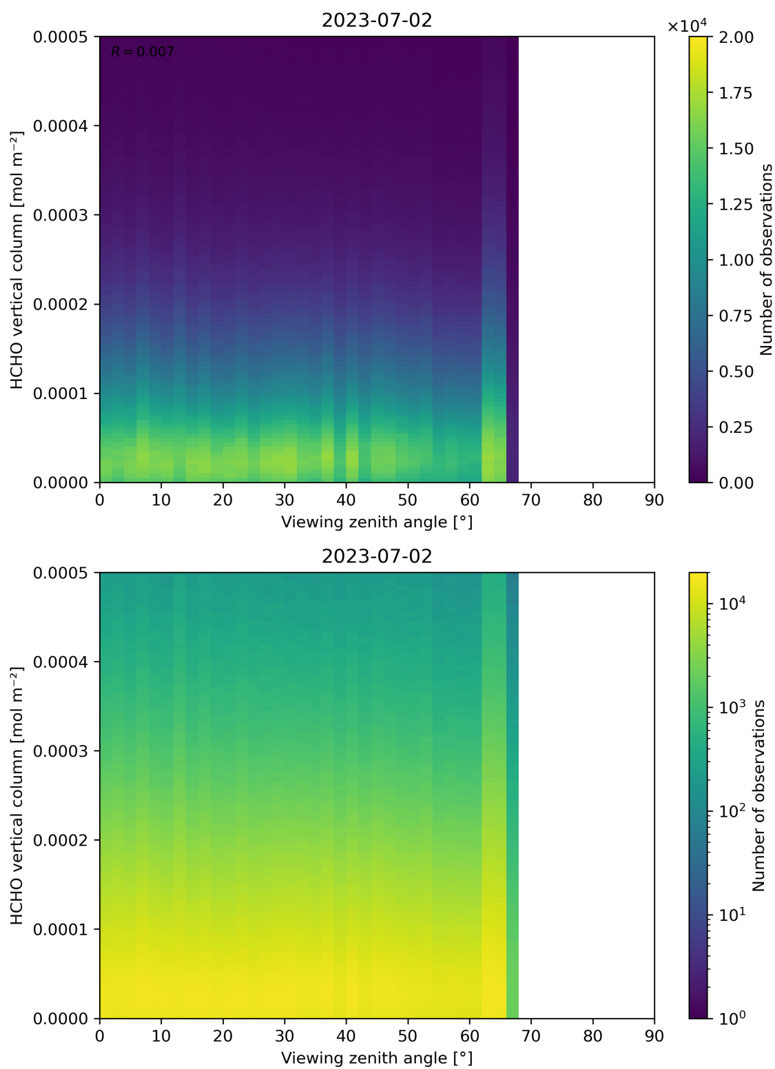
Figure 192: Scatter density plot of “Viewing zenith angle” against “HCHO vertical column” for 2023-07-01 to 2023-07-03.
