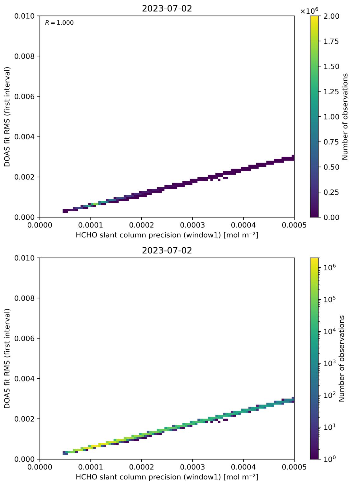
Figure 88: Scatter density plot of “HCHO slant column precision (window1)” against “DOAS fit RMS (first interval)” for 2023-07-01 to 2023-07-03.
