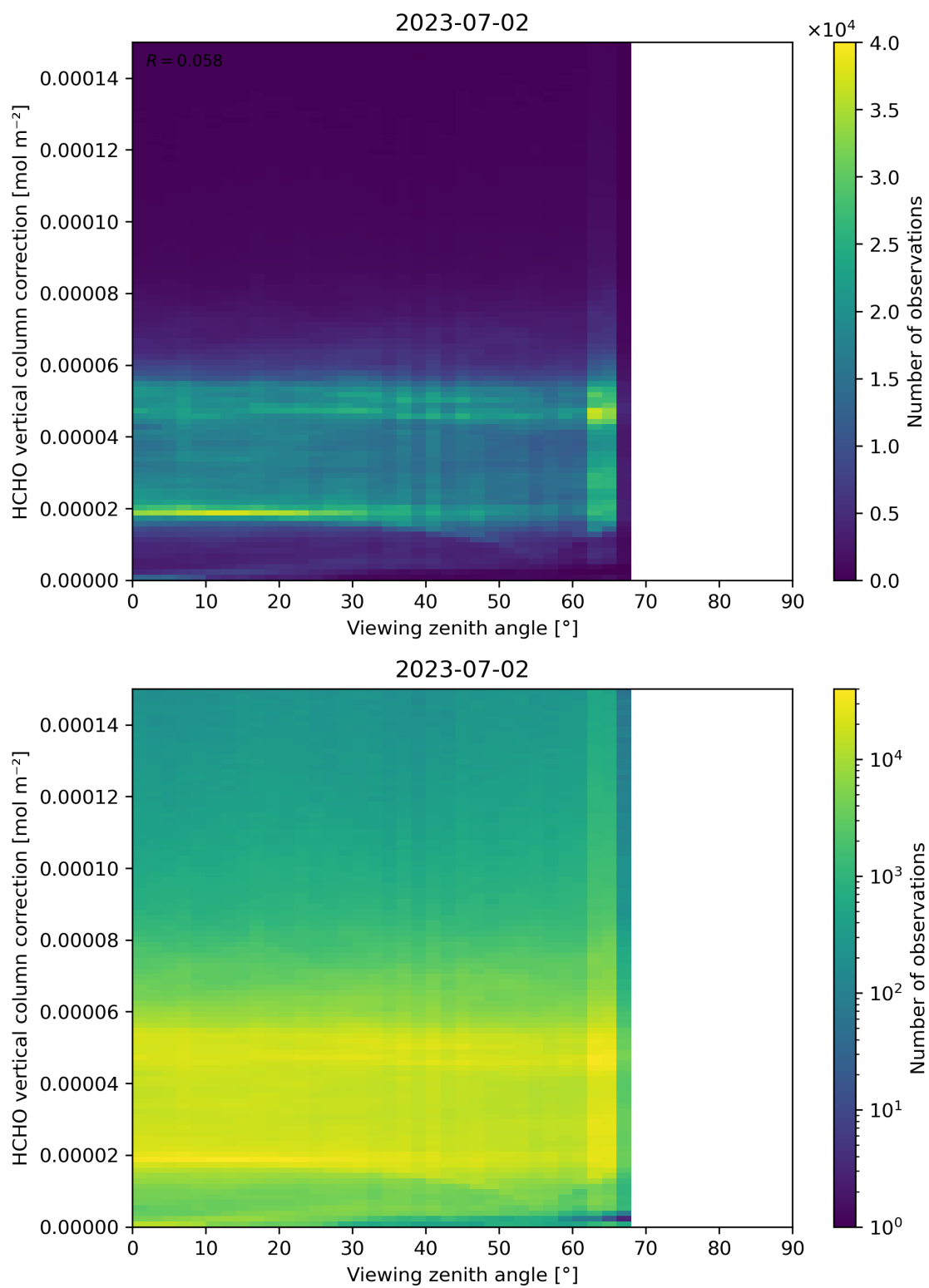
Figure 193: Scatter density plot of “Viewing zenith angle” against “HCHO vertical column correction” for 2023-07-01 to 2023-07-03.
