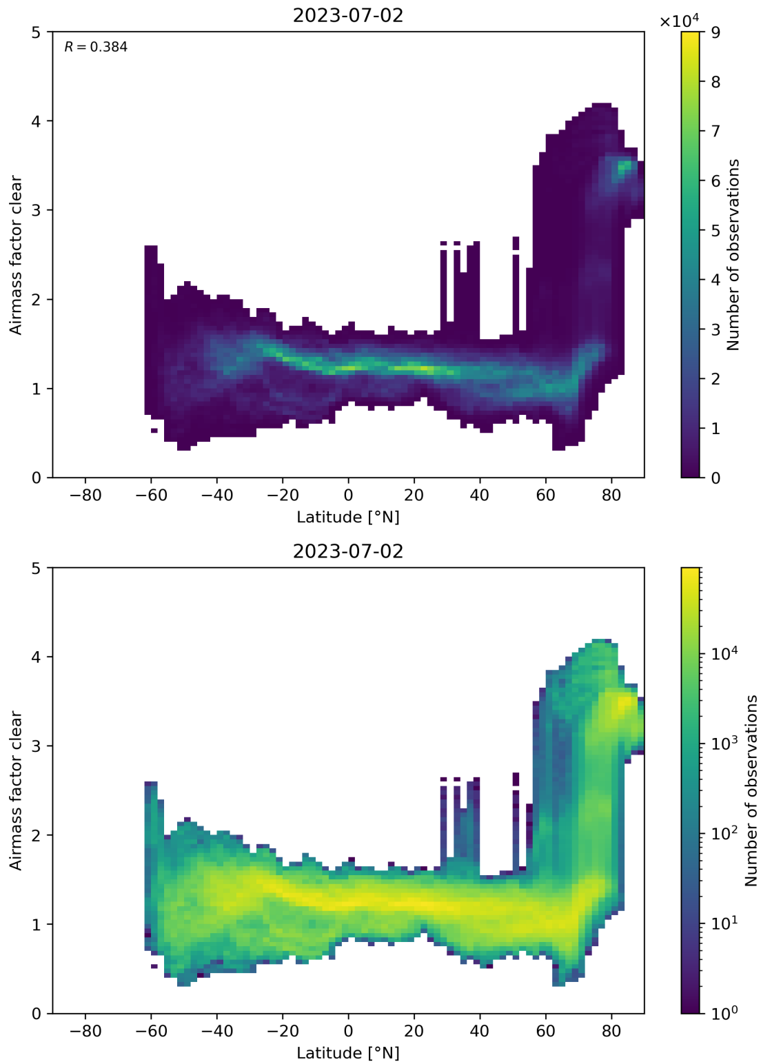
Figure 156: Scatter density plot of “Latitude” against “Airmass factor clear” for 2023-07-01 to 2023-07-03.
