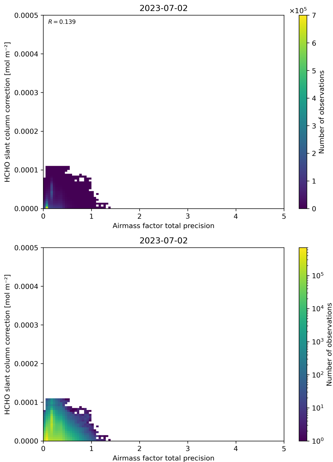
Figure 110: Scatter density plot of “Airmass factor total precision” against “HCHO slant column correction” for 2023-07-01 to 2023-07-03.
