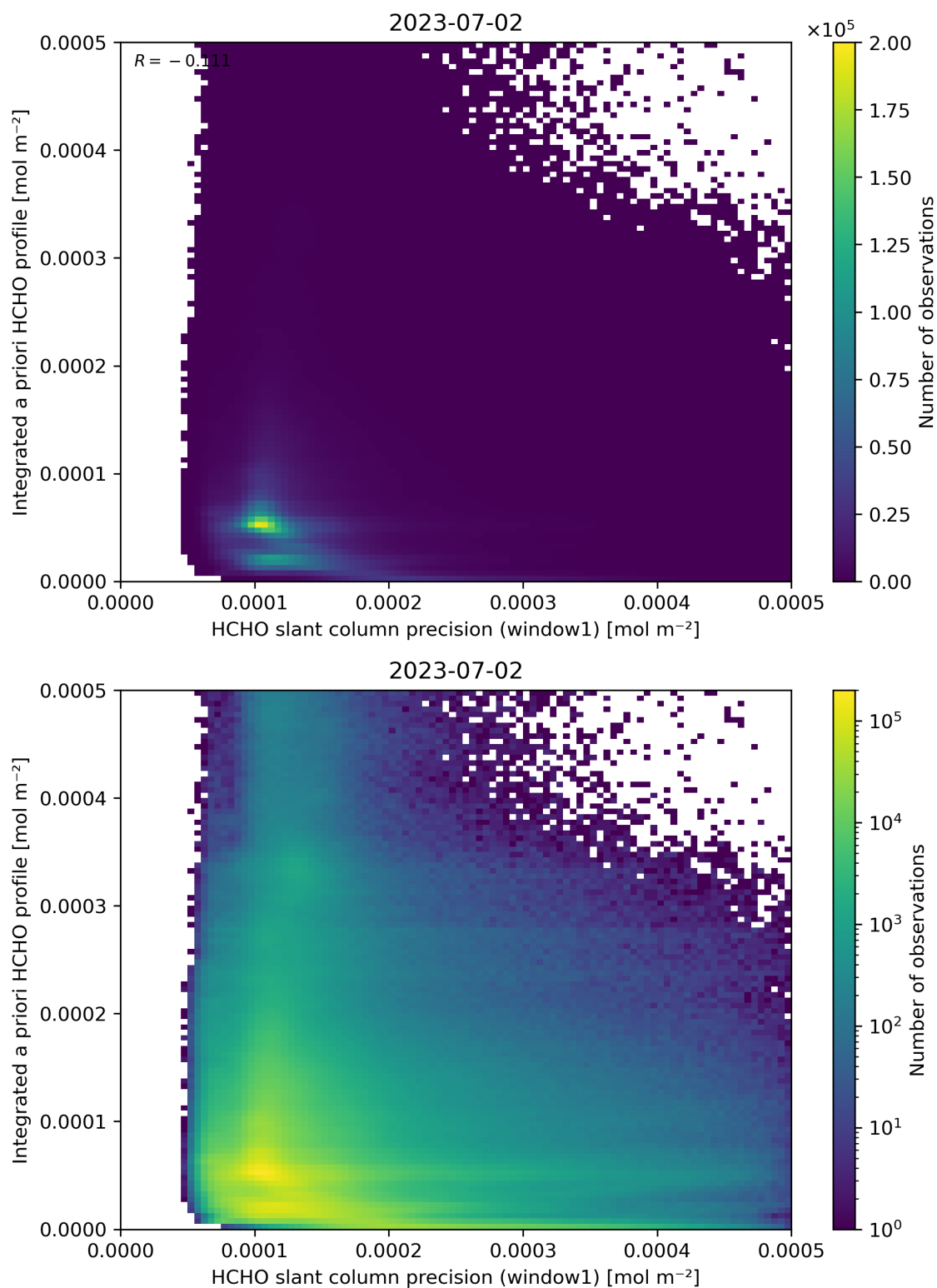
Figure 96: Scatter density plot of “HCHO slant column precision (window1)” against “Integrated a priori HCHO profile” for 2023-07-01 to 2023-07-03.
