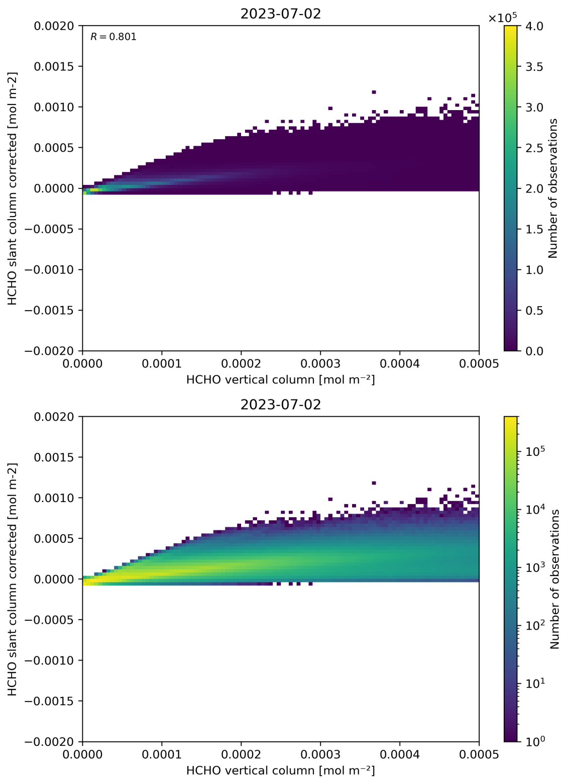
Figure 127: Scatter density plot of “HCHO vertical column” against “HCHO slant column corrected” for 2023-07-01 to 2023-07-03.
