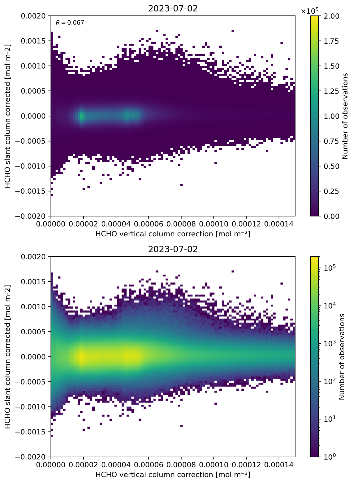
Figure 116: Scatter density plot of “HCHO vertical column correction” against “HCHO slant column corrected” for 2023-07-01 to 2023-07-03.
