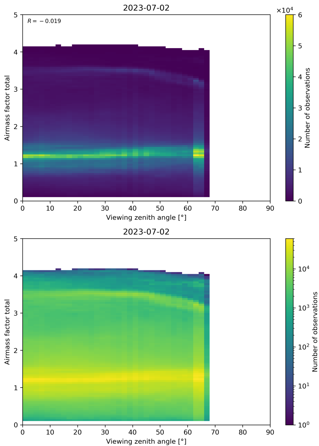
Figure 190: Scatter density plot of “Viewing zenith angle” against “Airmass factor total” for 2023-07-01 to 2023-07-03.
