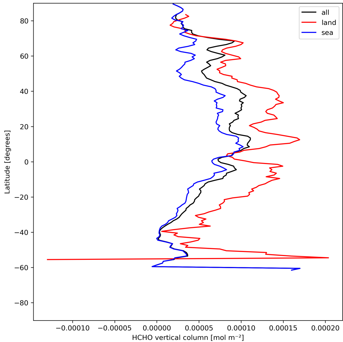
Figure 21: Zonal average of “HCHO vertical column” for 2023-07-01 to 2023-07-03.
