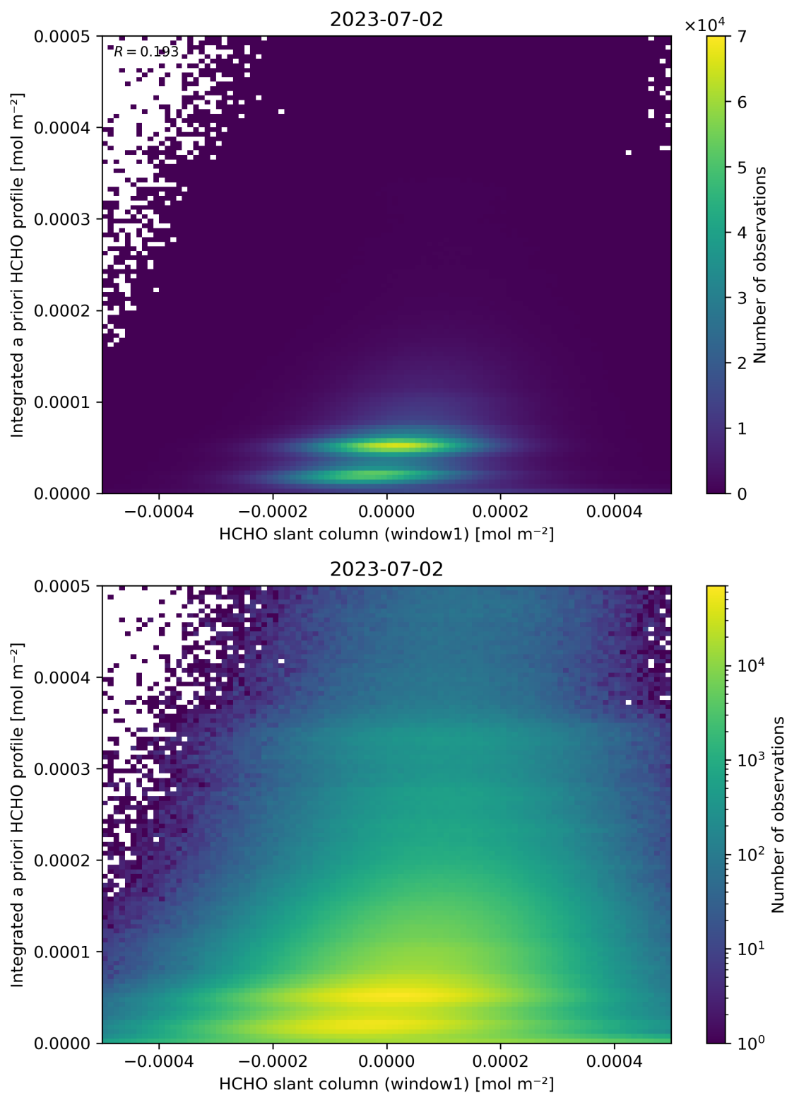
Figure 87: Scatter density plot of “HCHO slant column (window1)” against “Integrated a priori HCHO profile” for 2023-07-01 to 2023-07-03.
