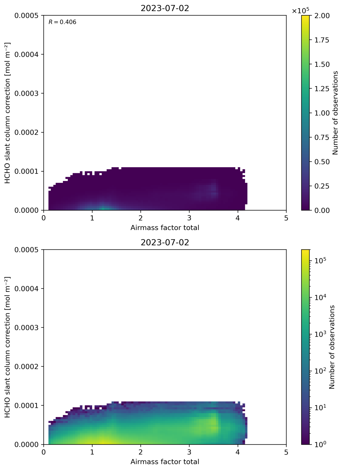
Figure 102: Scatter density plot of “Airmass factor total” against “HCHO slant column correction” for 2023-07-01 to 2023-07-03.
