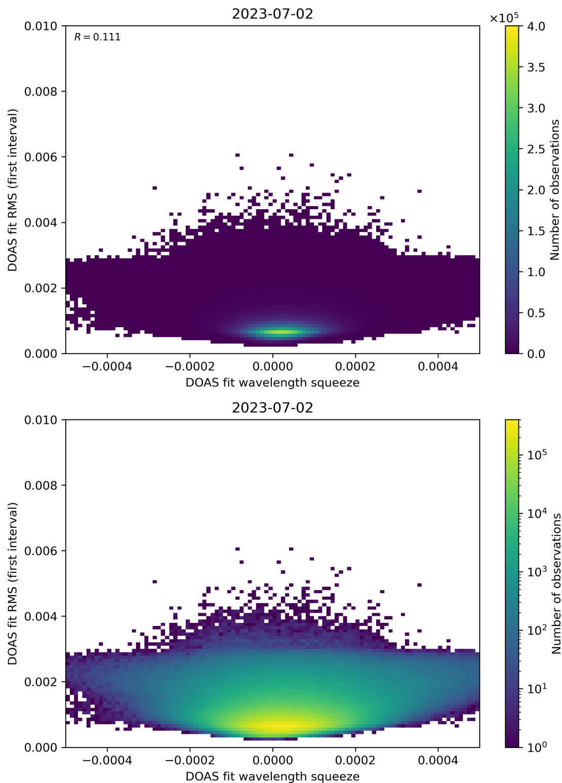
Figure 68: Scatter density plot of “DOAS fit wavelength squeeze” against “DOAS fit RMS (first interval)” for 2023-07-01 to 2023-07-03.
