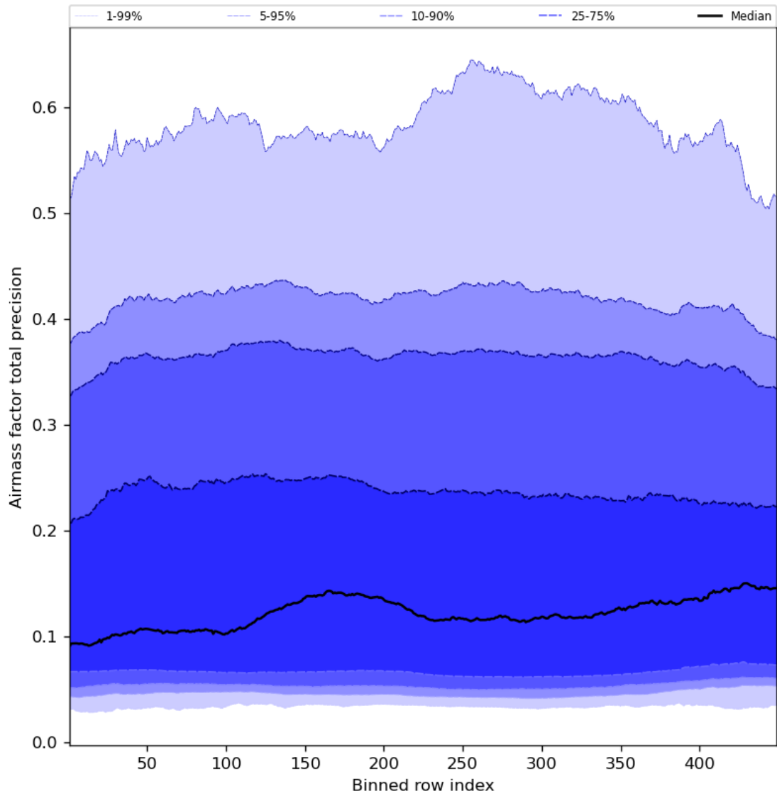
Figure 55: Along track statistics of “Airmass factor total precision” for 2023-07-01 to 2023-07-03
