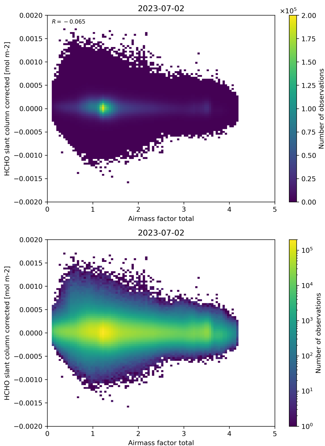
Figure 101: Scatter density plot of “Airmass factor total” against “HCHO slant column corrected” for 2023-07-01 to 2023-07-03.
