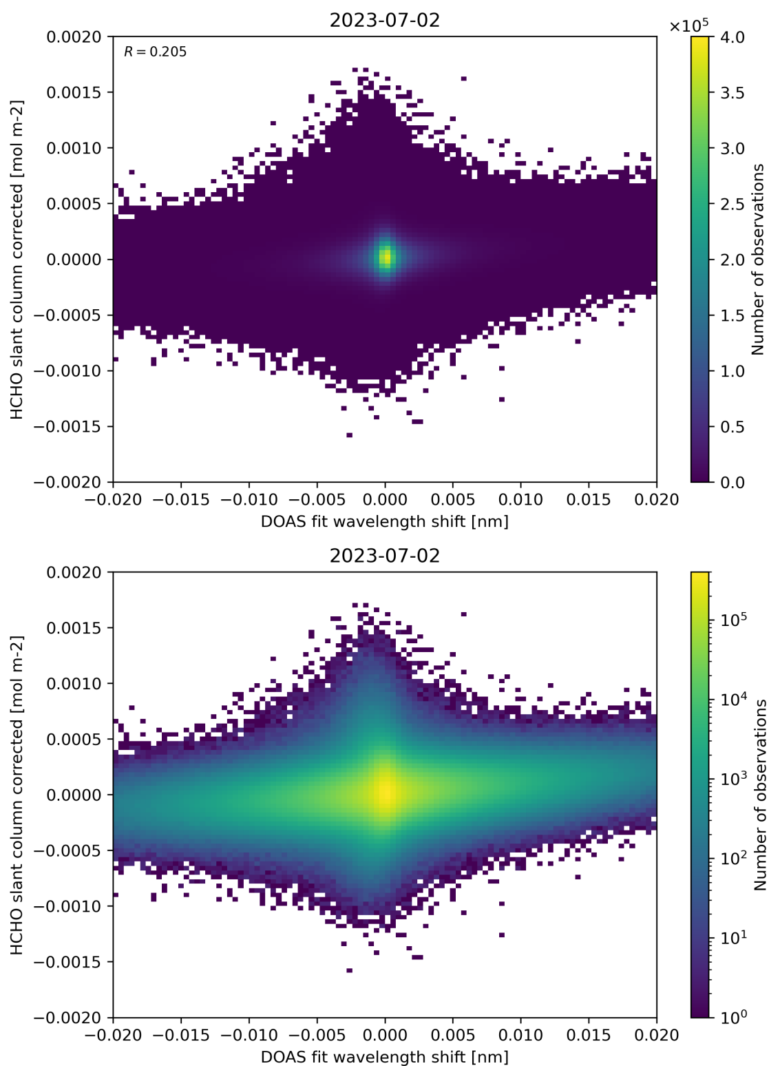
Figure 66: Scatter density plot of “DOAS fit wavelength shift” against “HCHO slant column corrected” for 2023-07-01 to 2023-07-03.
