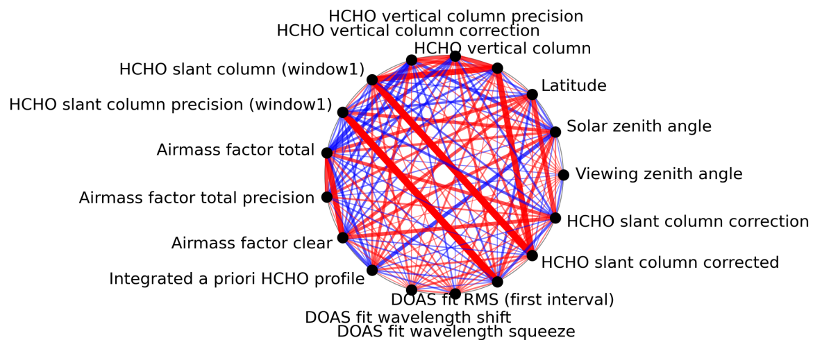
Figure 1: Map of correlation graph for 2023-07-01 to 2023-07-03.
