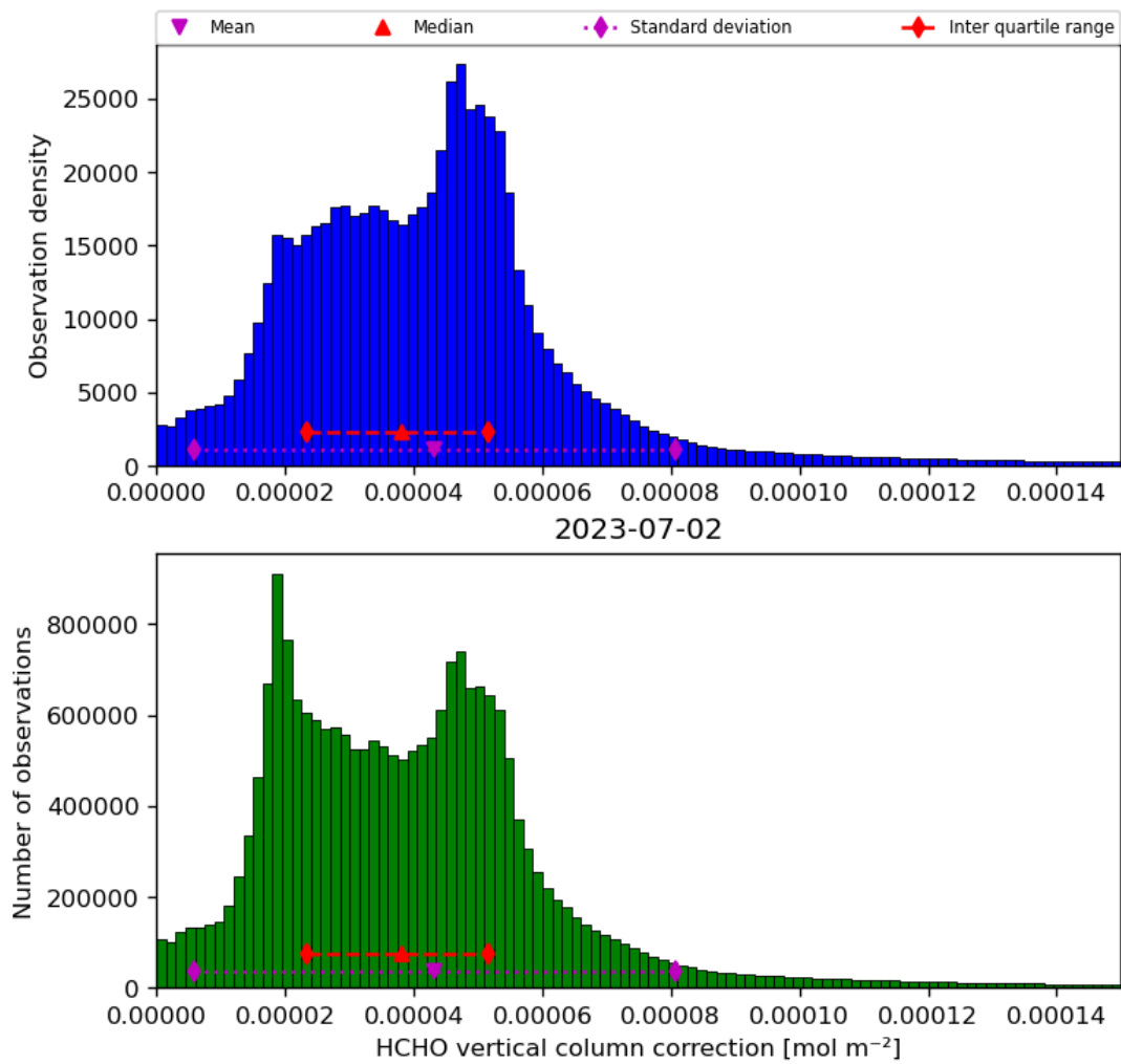
Figure 37: Histogram of “HCHO vertical column correction” for 2023-07-01 to 2023-07-03
