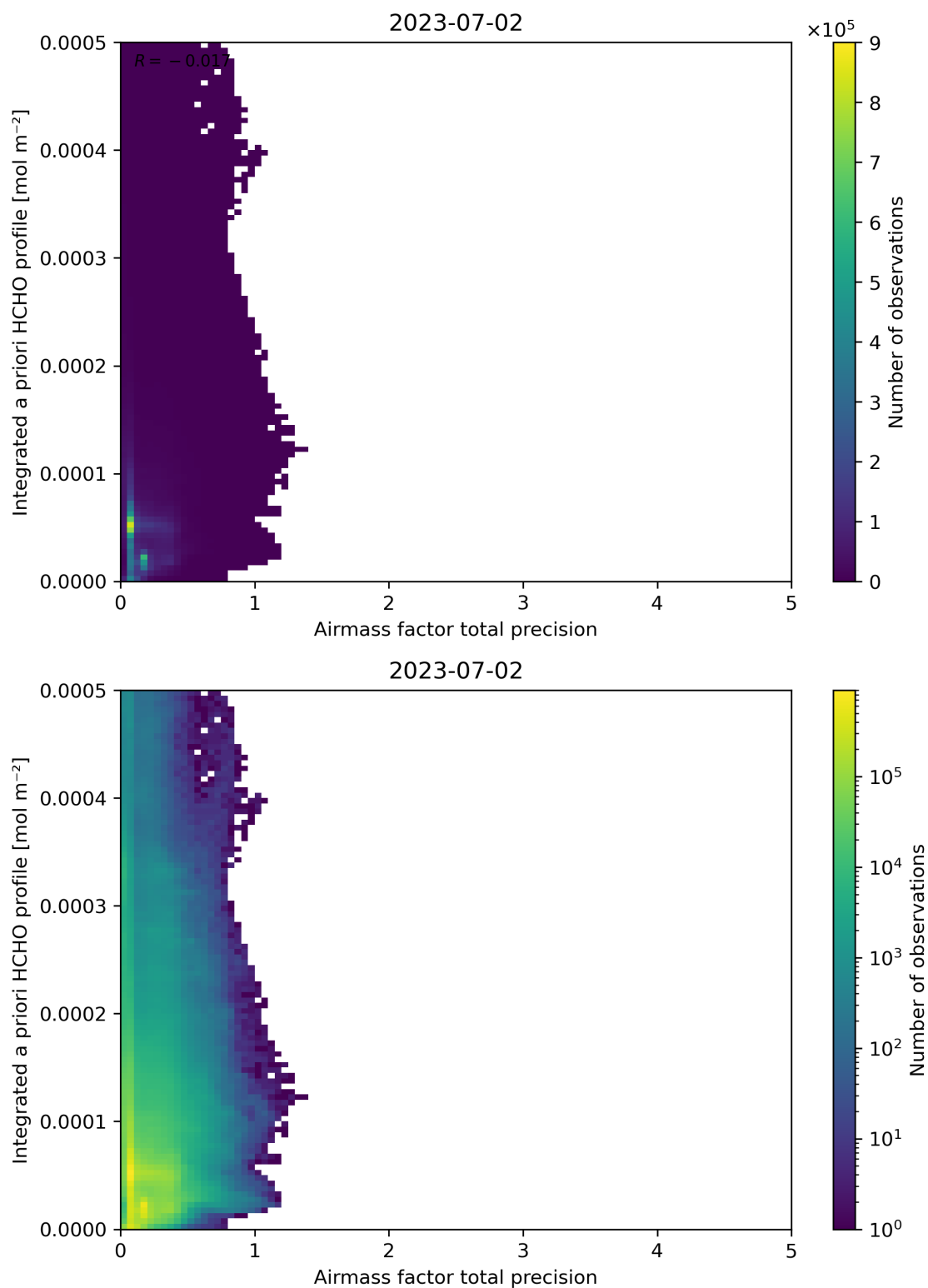
Figure 111: Scatter density plot of “Airmass factor total precision” against “Integrated a priori HCHO profile” for 2023-07-01 to 2023-07-03.
