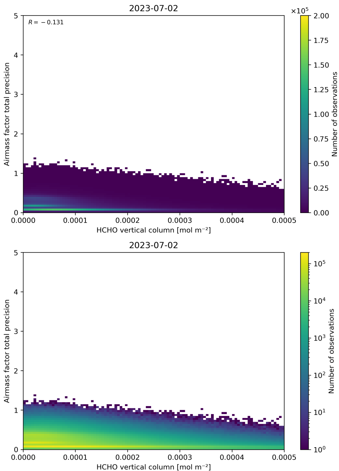
Figure 132: Scatter density plot of “HCHO vertical column” against “Airmass factor total precision” for 2023-07-01 to 2023-07-03.
