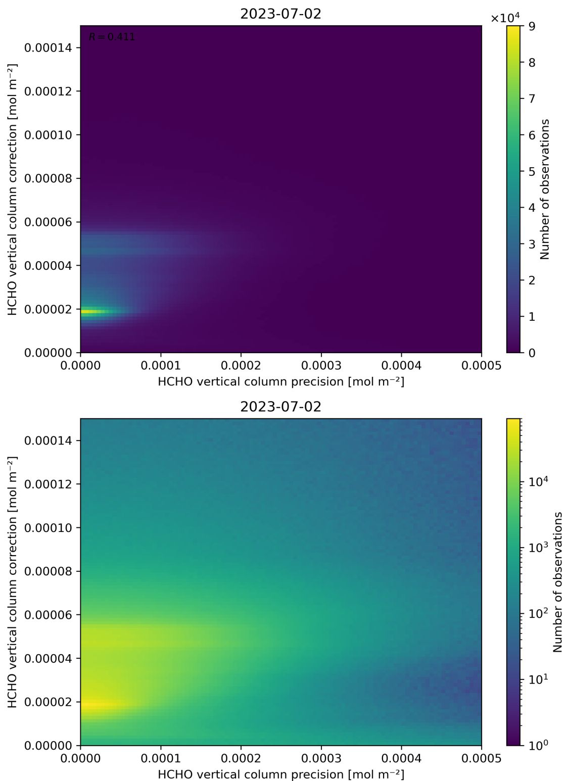
Figure 146: Scatter density plot of “HCHO vertical column precision” against “HCHO vertical column correction” for 2023-07-01 to 2023-07-03.
