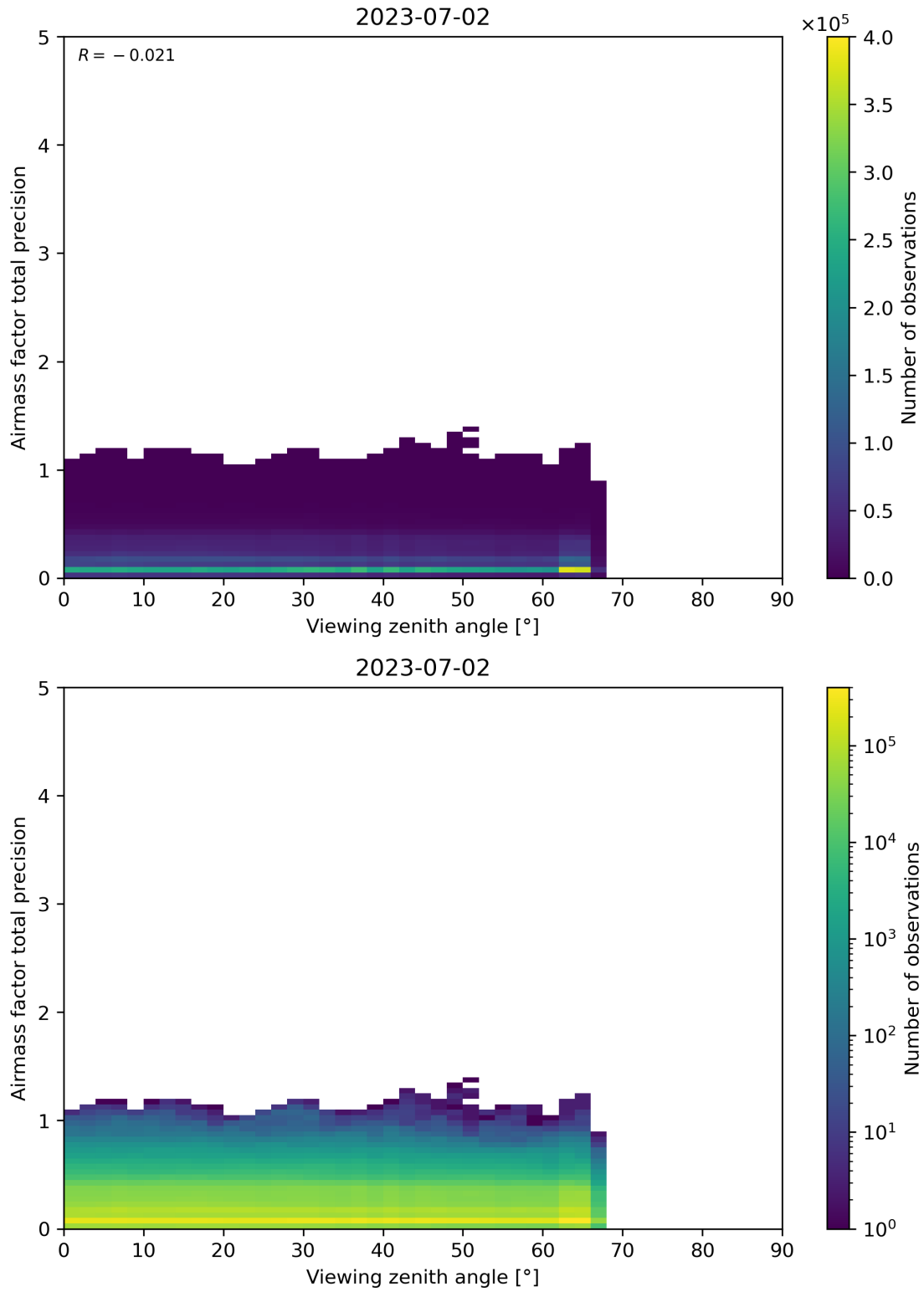
Figure 191: Scatter density plot of “Viewing zenith angle” against “Airmass factor total precision” for 2023-07-01 to 2023-07-03.
