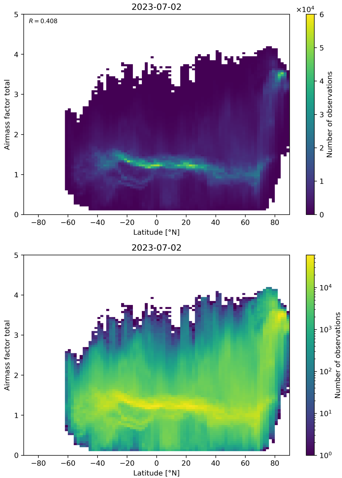
Figure 161: Scatter density plot of “Latitude” against “Airmass factor total” for 2023-07-01 to 2023-07-03.
