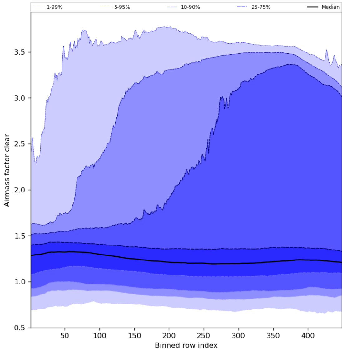
Figure 56: Along track statistics of “Airmass factor clear” for 2023-07-01 to 2023-07-03
