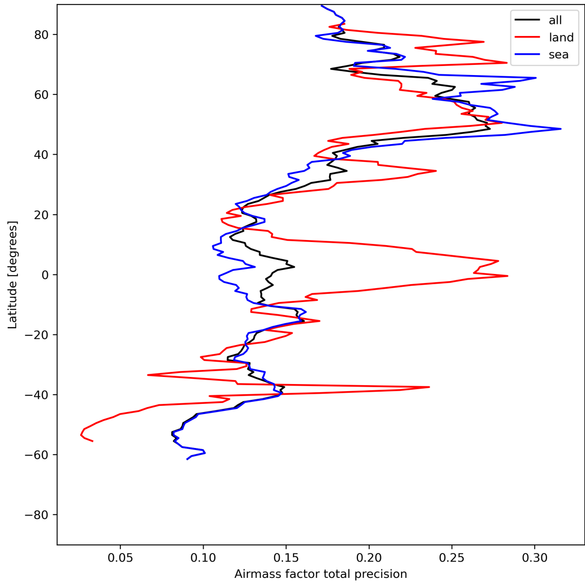
Figure 27: Zonal average of “Airmass factor total precision” for 2023-07-01 to 2023-07-03.
