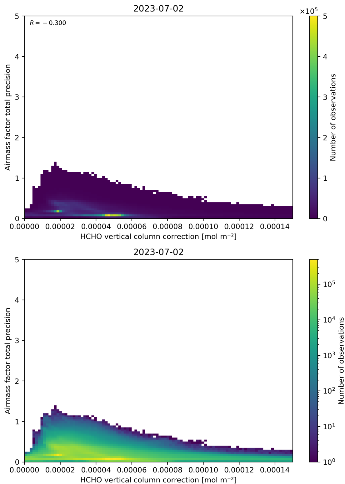
Figure 121: Scatter density plot of “HCHO vertical column correction” against “Airmass factor total precision” for 2023-07-01 to 2023-07-03.
