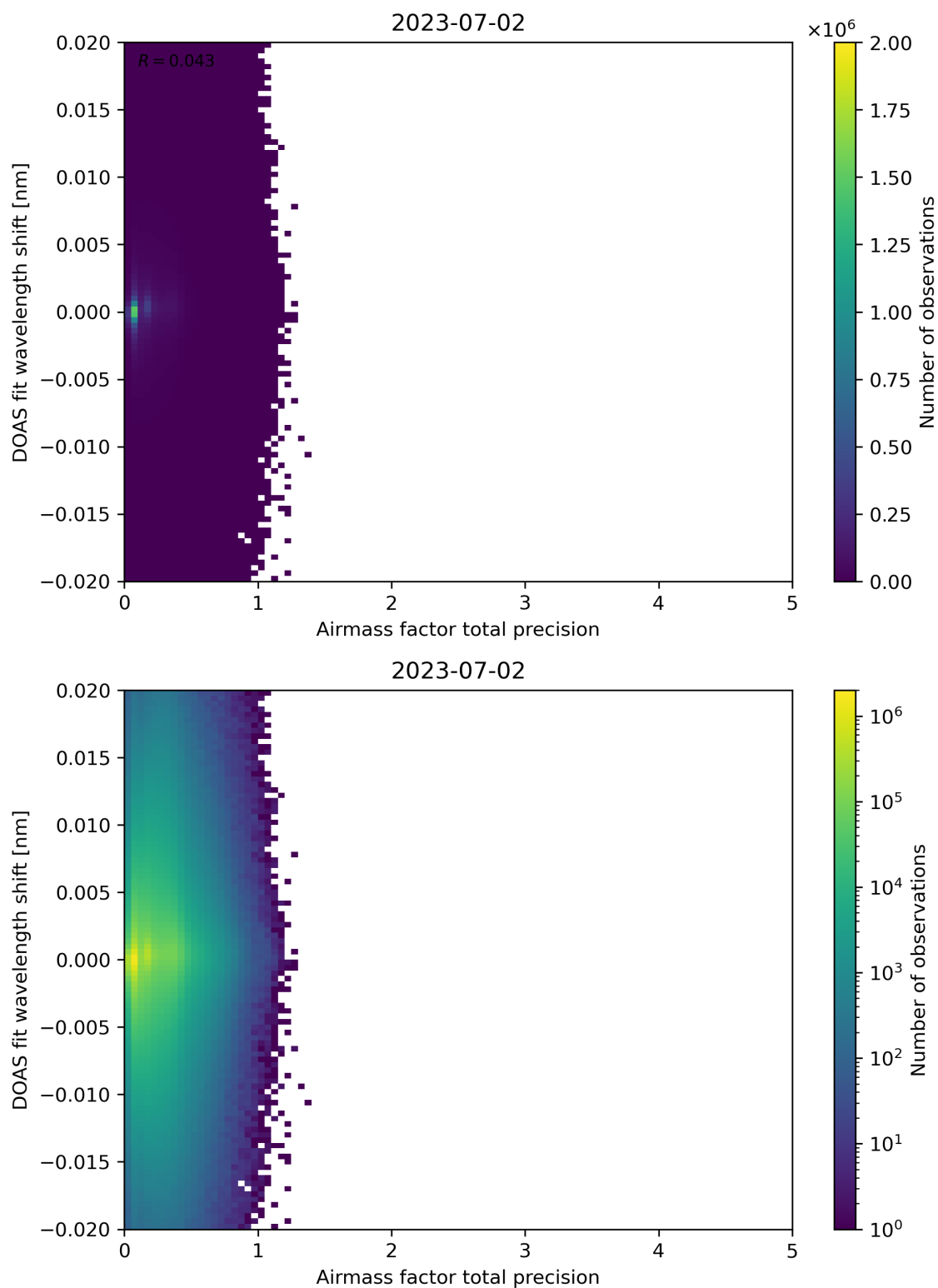
Figure 106: Scatter density plot of “Airmass factor total precision” against “DOAS fit wavelength shift” for 2023-07-01 to 2023-07-03.
