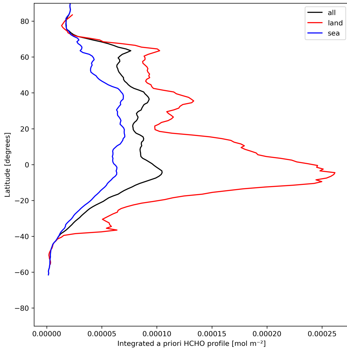
Figure 29: Zonal average of “Integrated a priori HCHO profile” for 2023-07-01 to 2023-07-03.
