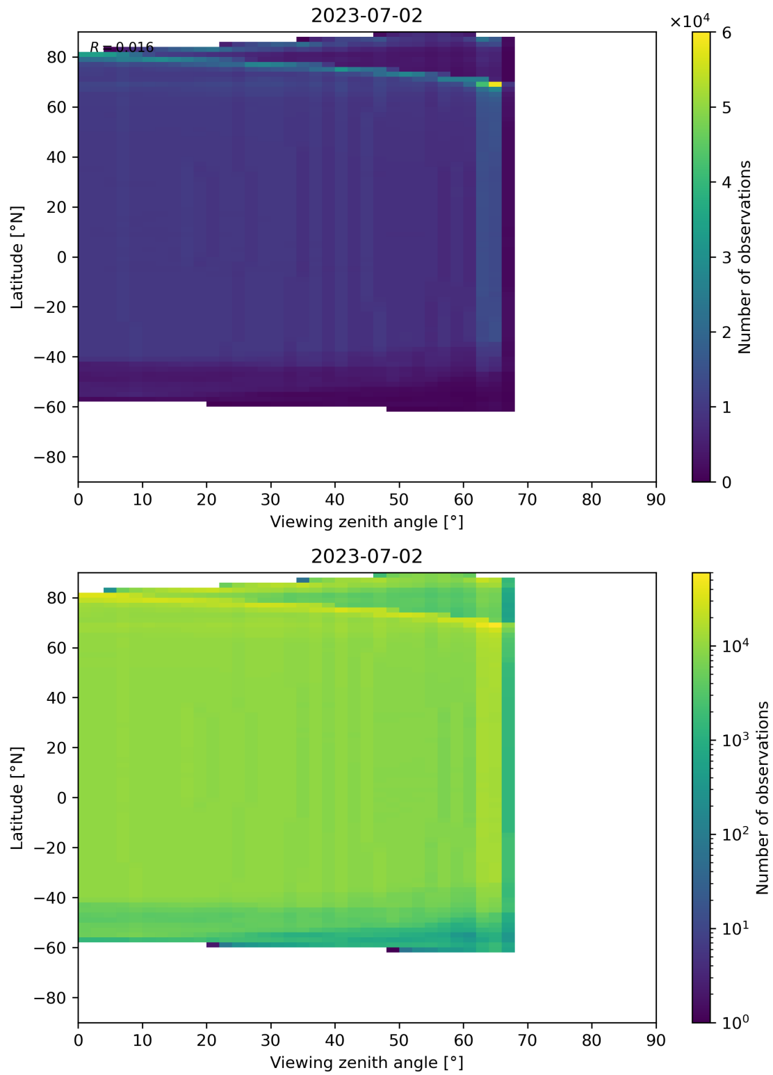
Figure 196: Scatter density plot of “Viewing zenith angle” against “Latitude” for 2023-07-01 to 2023-07-03.
