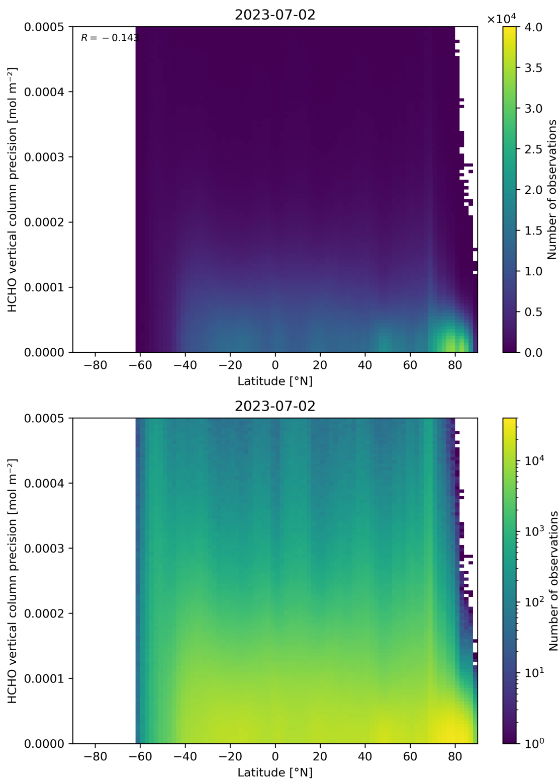
Figure 165: Scatter density plot of “Latitude” against “HCHO vertical column precision” for 2023-07-01 to 2023-07-03.
