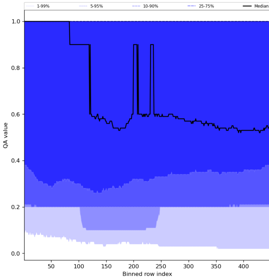
Figure 48: Along track statistics of “QA value” for 2023-07-01 to 2023-07-03
