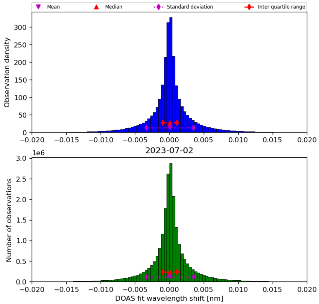
Figure 44: Histogram of “DOAS fit wavelength shift” for 2023-07-01 to 2023-07-03
