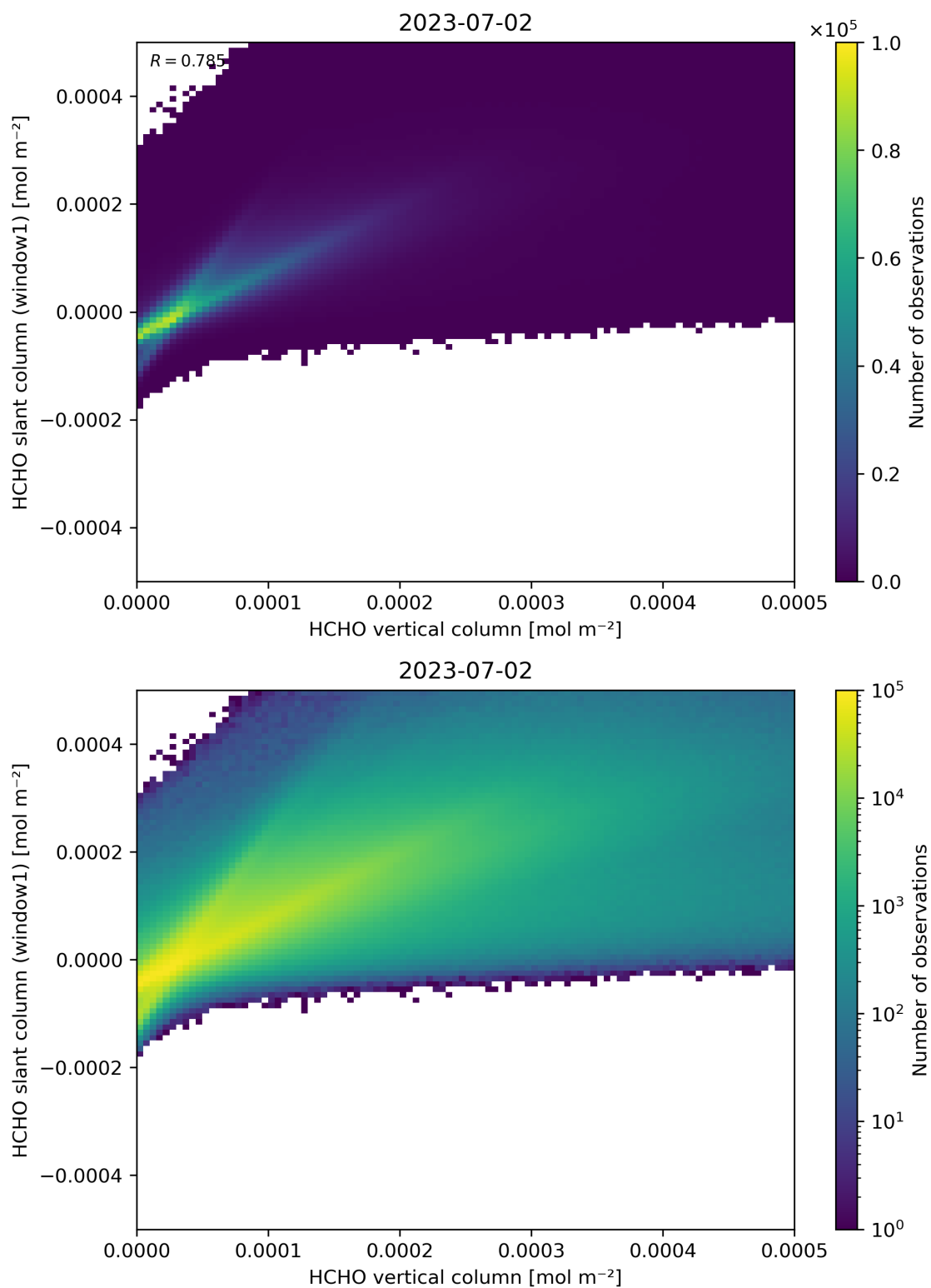
Figure 129: Scatter density plot of “HCHO vertical column” against “HCHO slant column (window1)” for 2023-07-01 to 2023-07-03.
