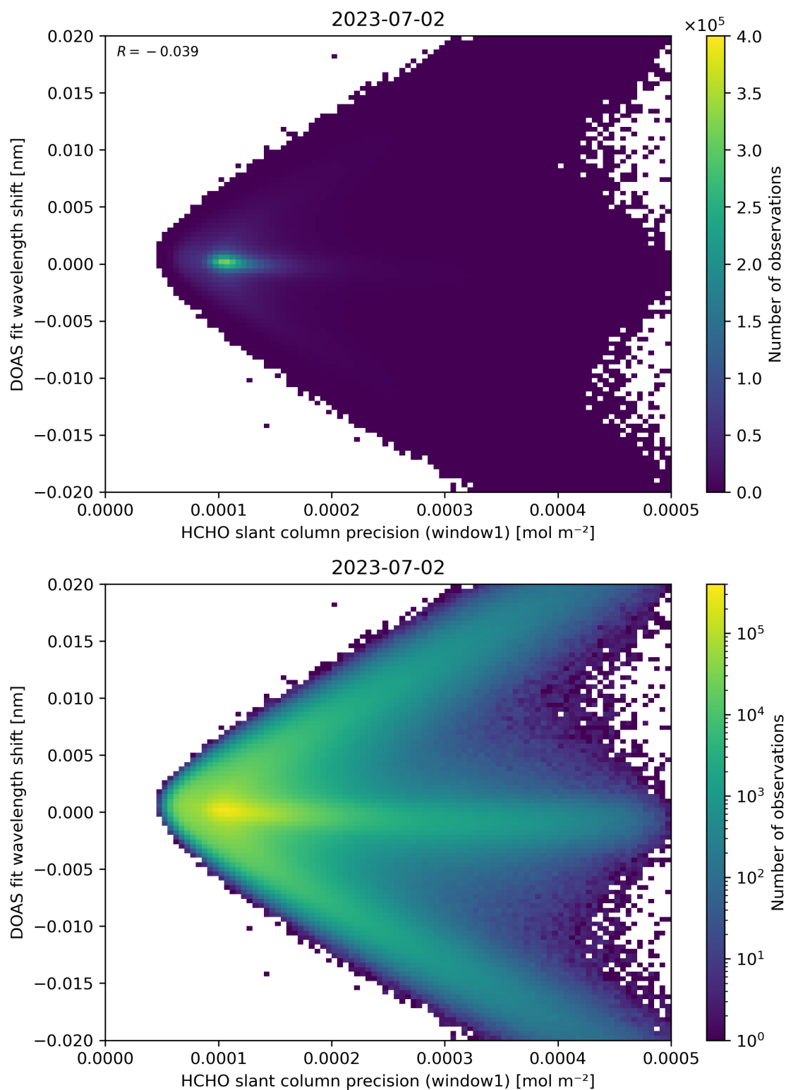
Figure 89: Scatter density plot of “HCHO slant column precision (window1)” against “DOAS fit wavelength shift” for 2023-07-01 to 2023-07-03.
