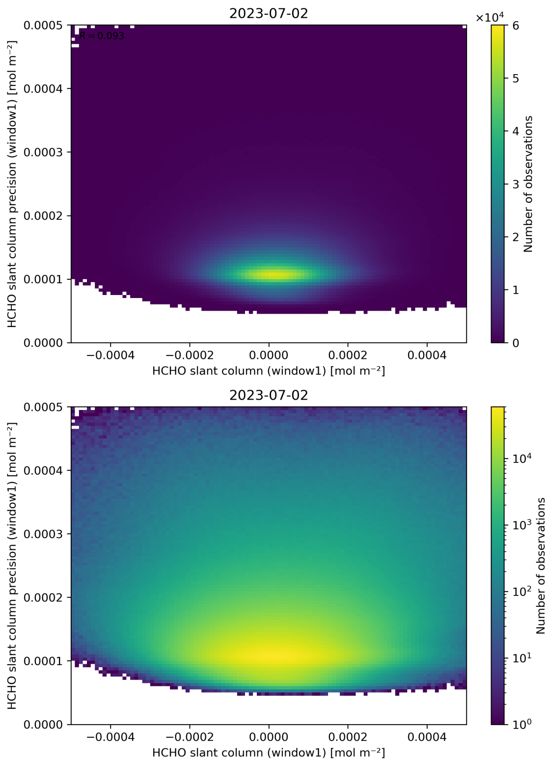
Figure 84: Scatter density plot of “HCHO slant column (window1)” against “HCHO slant column precision (window1)” for 2023-07-01 to 2023-07-03.
