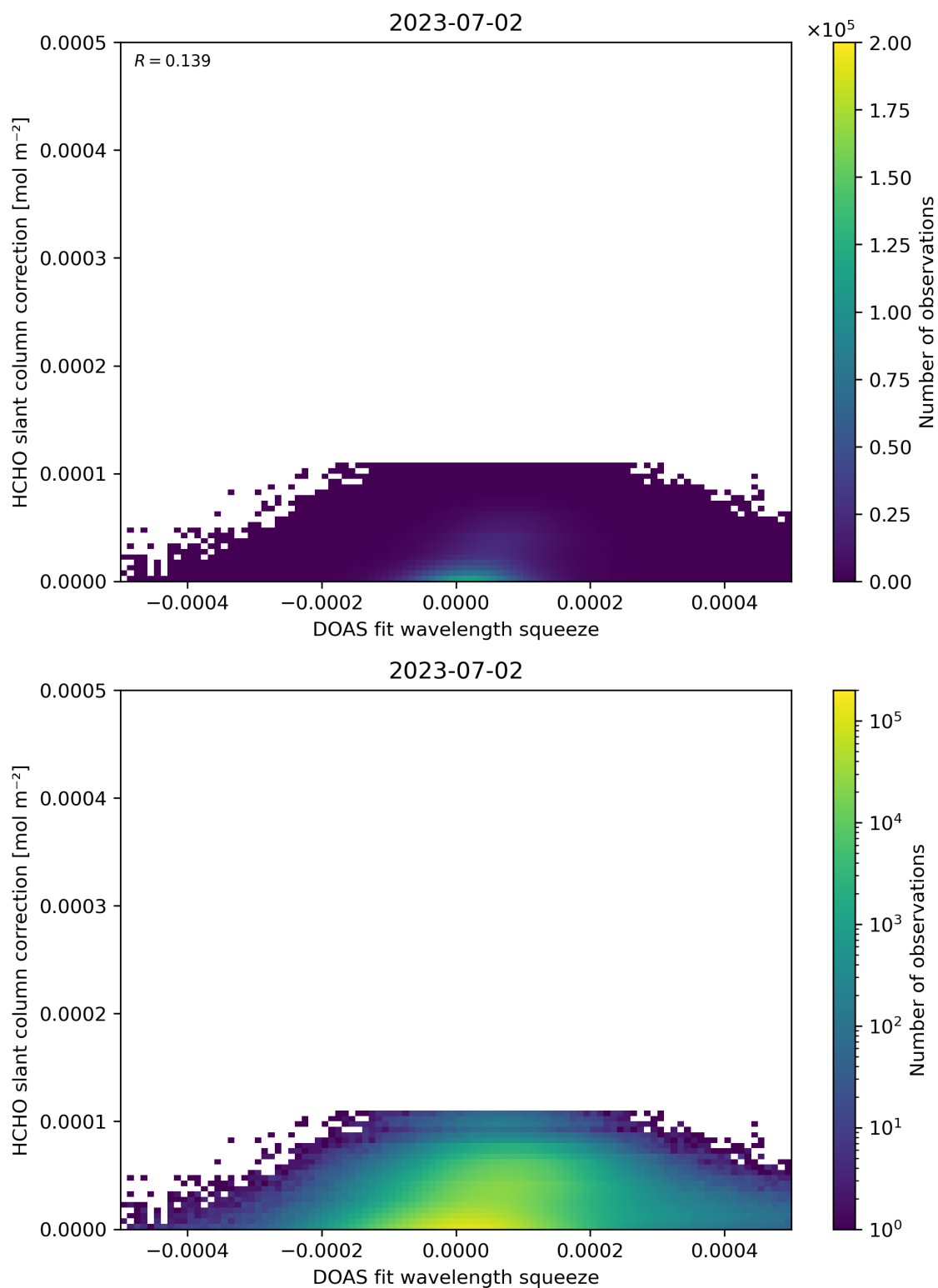
Figure 70: Scatter density plot of “DOAS fit wavelength squeeze” against “HCHO slant column correction” for 2023-07-01 to 2023-07-03.
