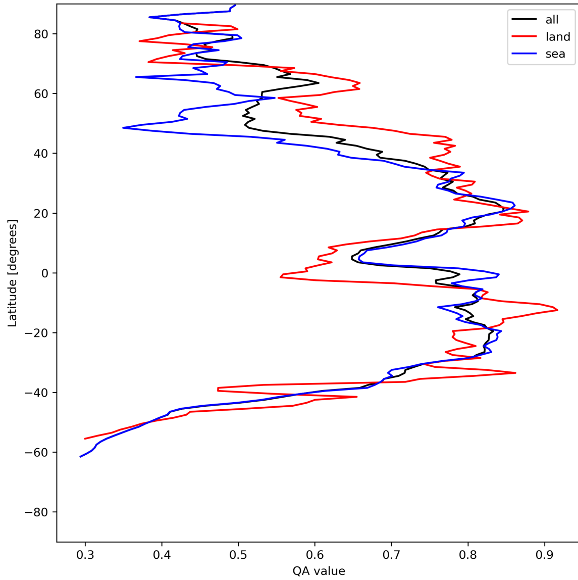
Figure 20: Zonal average of “QA value” for 2023-07-01 to 2023-07-03.
