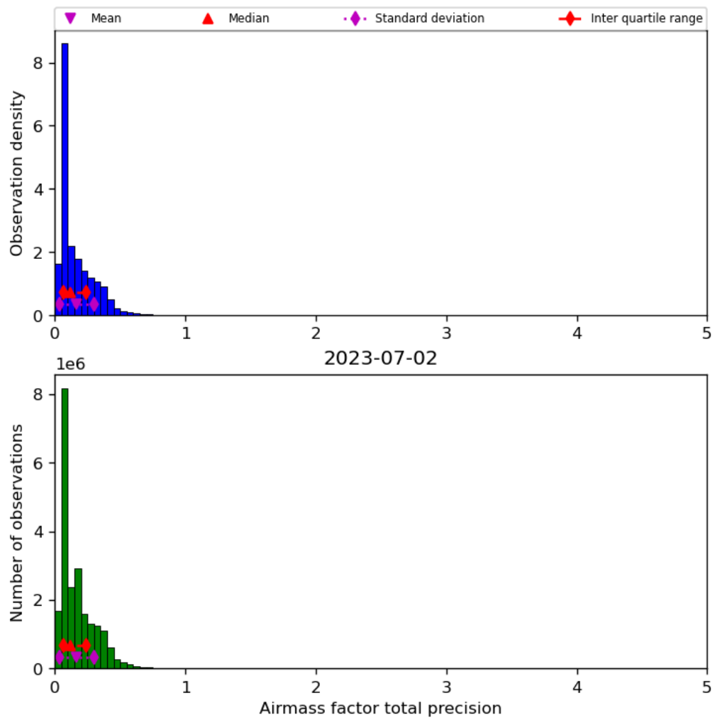
Figure 41: Histogram of “Airmass factor total precision” for 2023-07-01 to 2023-07-03
