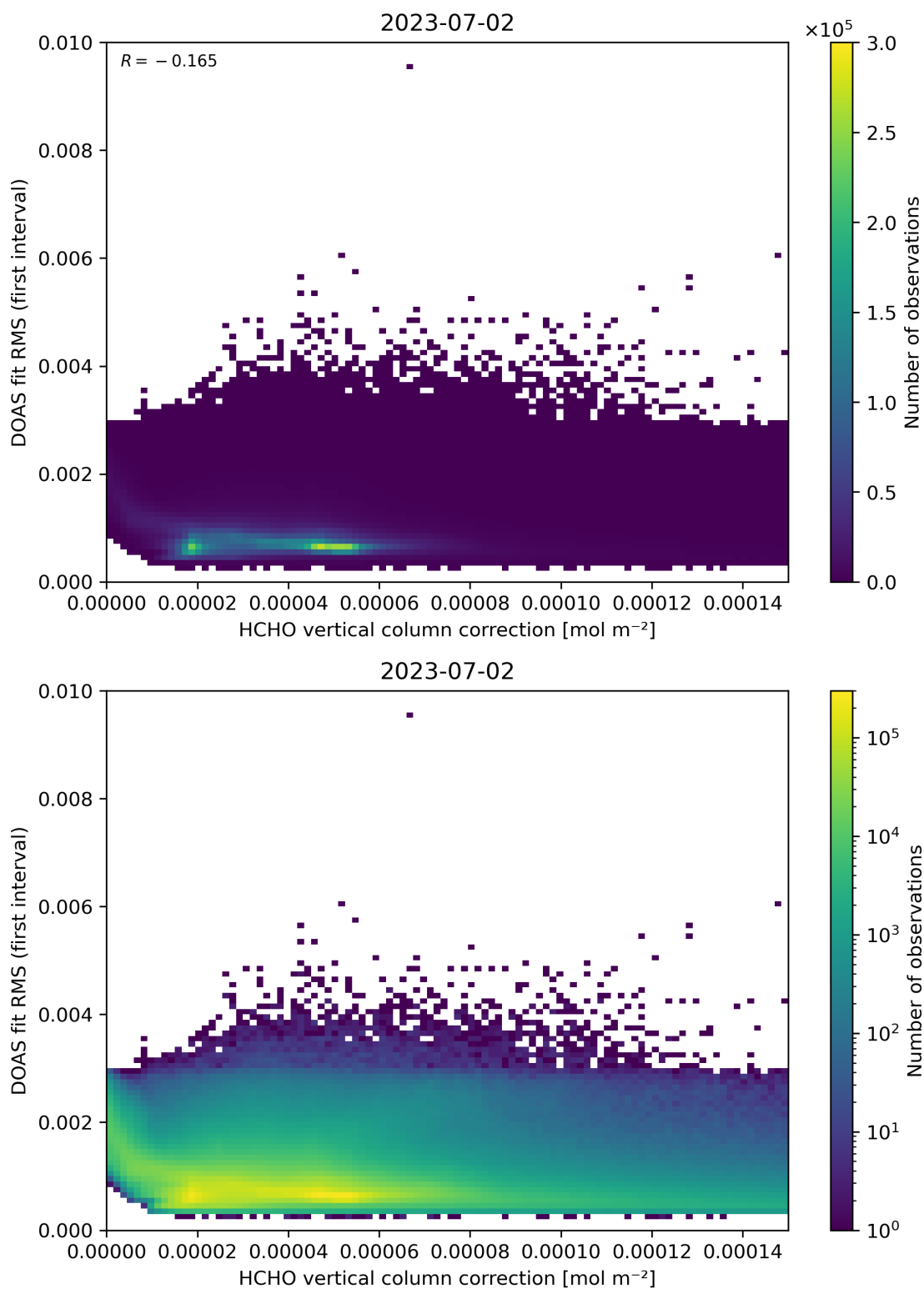
Figure 112: Scatter density plot of “HCHO vertical column correction” against “DOAS fit RMS (first interval)” for 2023-07-01 to 2023-07-03.
