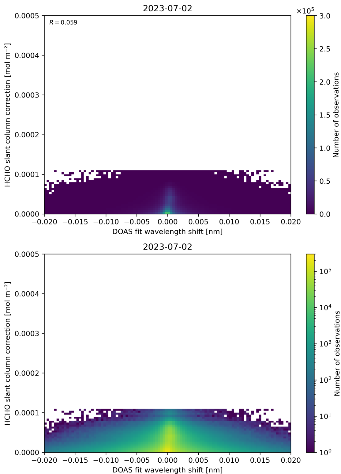
Figure 67: Scatter density plot of “DOAS fit wavelength shift” against “HCHO slant column correction” for 2023-07-01 to 2023-07-03.
