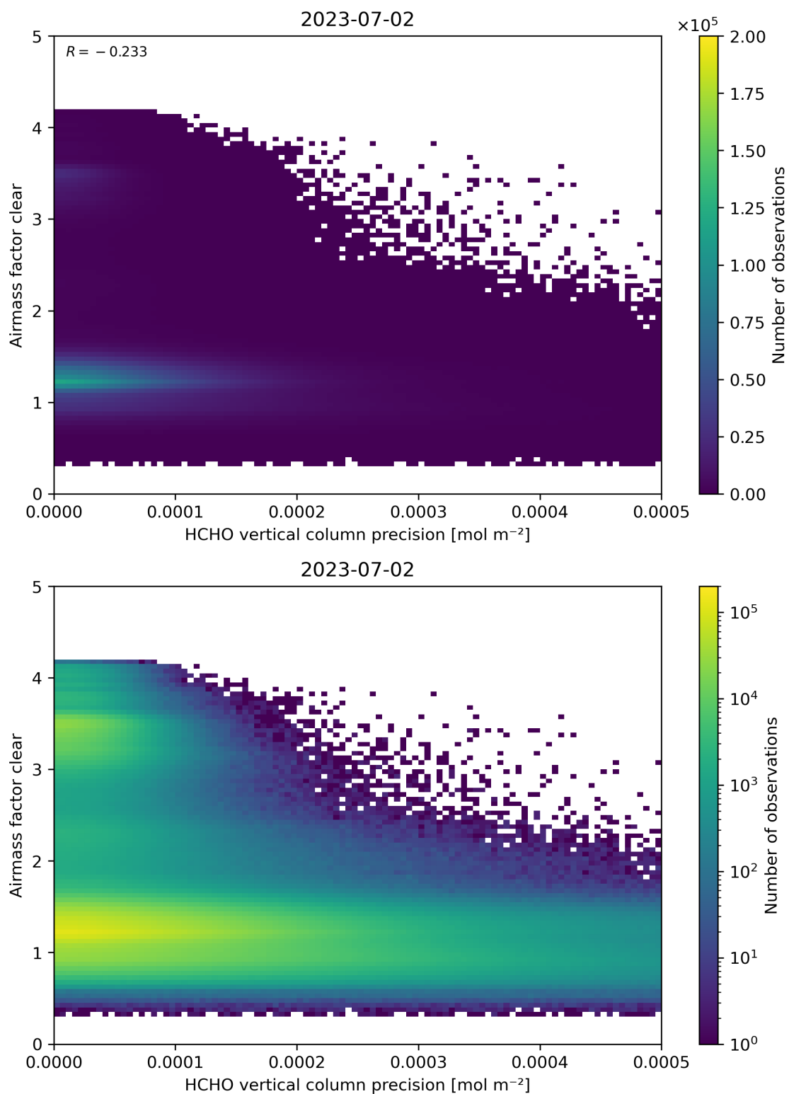
Figure 139: Scatter density plot of “HCHO vertical column precision” against “Airmass factor clear” for 2023-07-01 to 2023-07-03.
