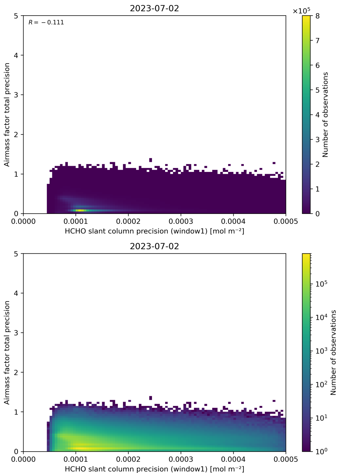
Figure 95: Scatter density plot of “HCHO slant column precision (window1)” against “Airmass factor total precision” for 2023-07-01 to 2023-07-03.
