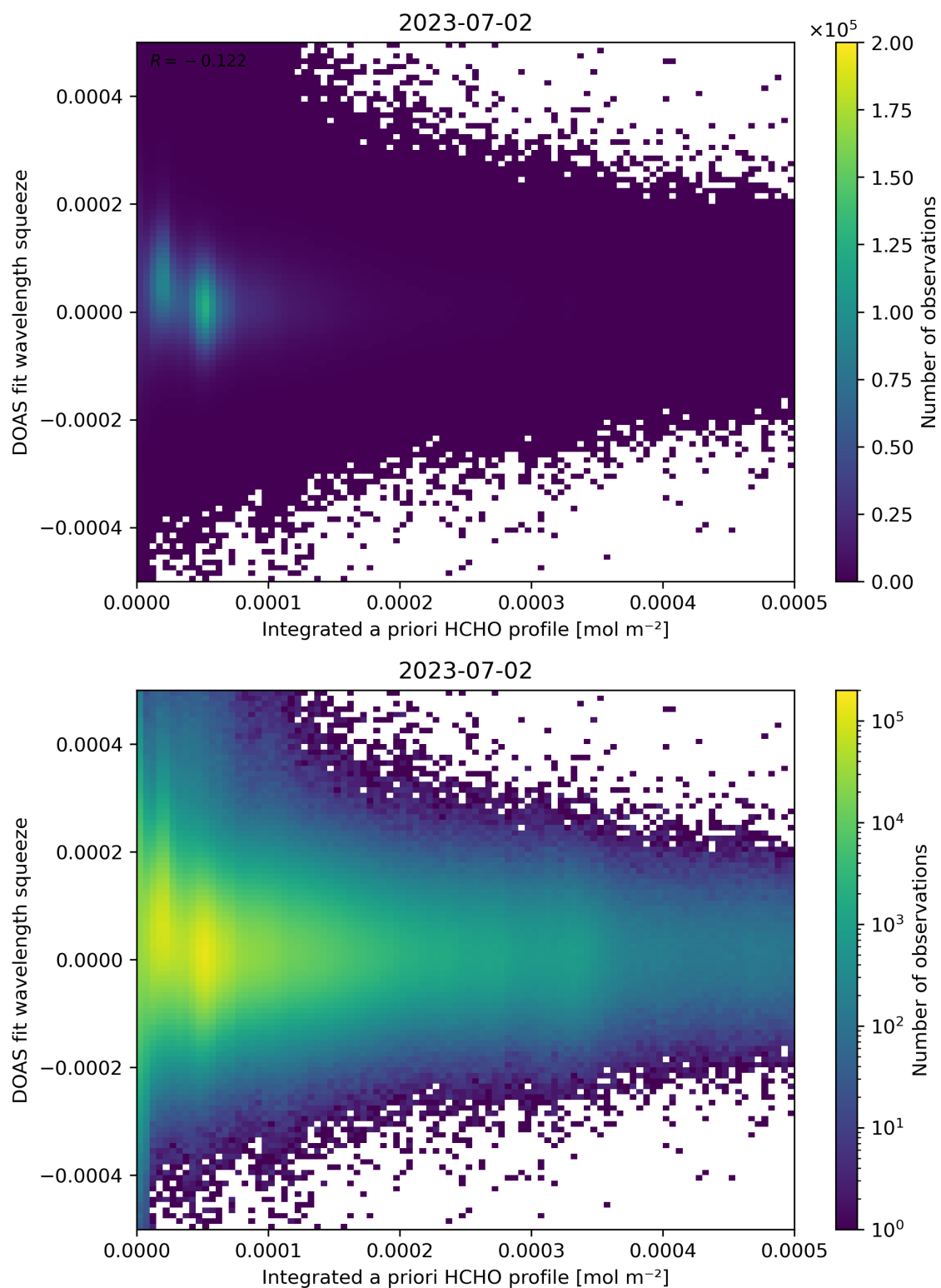
Figure 150: Scatter density plot of “Integrated a priori HCHO profile” against “DOAS fit wavelength squeeze” for 2023-07-01 to 2023-07-03.
