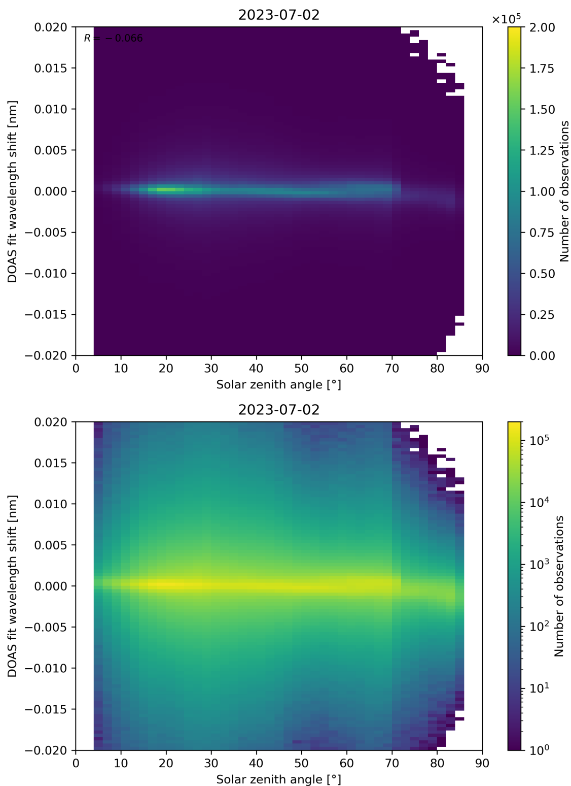
Figure 168: Scatter density plot of “Solar zenith angle” against “DOAS fit wavelength shift” for 2023-07-01 to 2023-07-03.
