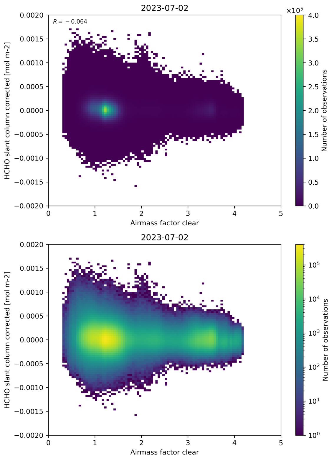
Figure 74: Scatter density plot of “Airmass factor clear” against “HCHO slant column corrected” for 2023-07-01 to 2023-07-03.
