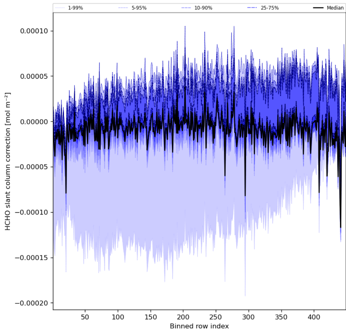
Figure 61: Along track statistics of “HCHO slant column correction” for 2023-07-01 to 2023-07-03
