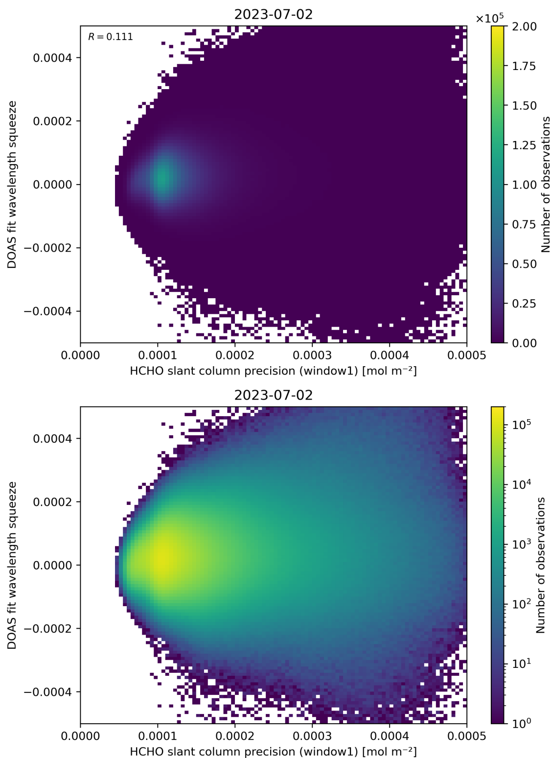
Figure 90: Scatter density plot of “HCHO slant column precision (window1)” against “DOAS fit wavelength squeeze” for 2023-07-01 to 2023-07-03.
