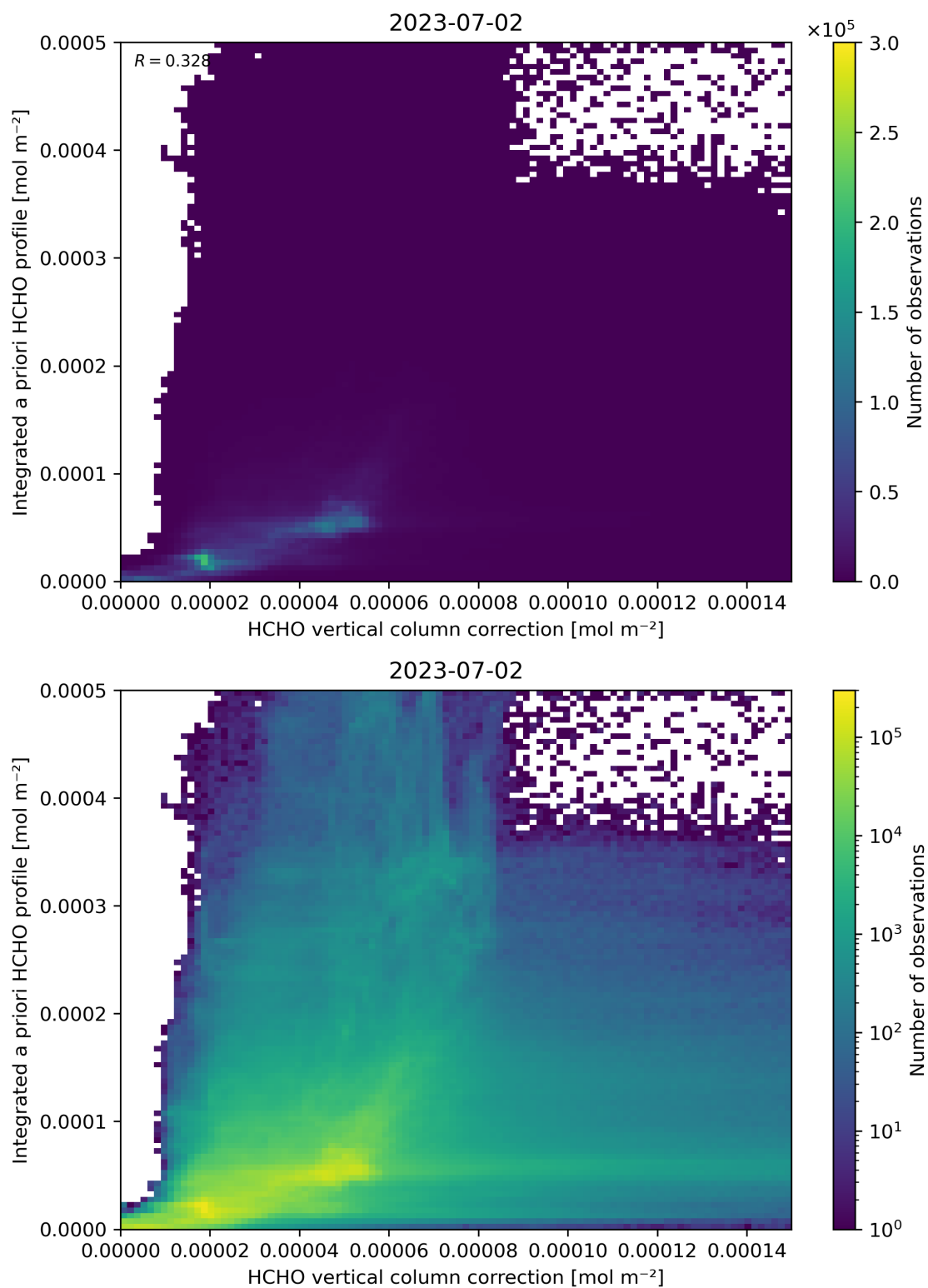
Figure 122: Scatter density plot of “HCHO vertical column correction” against “Integrated a priori HCHO profile” for 2023-07-01 to 2023-07-03.
