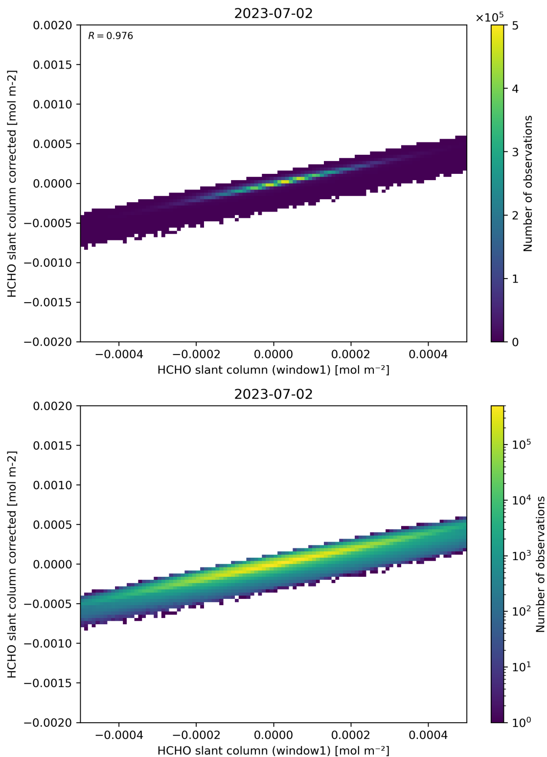
Figure 82: Scatter density plot of “HCHO slant column (window1)” against “HCHO slant column corrected” for 2023-07-01 to 2023-07-03.
