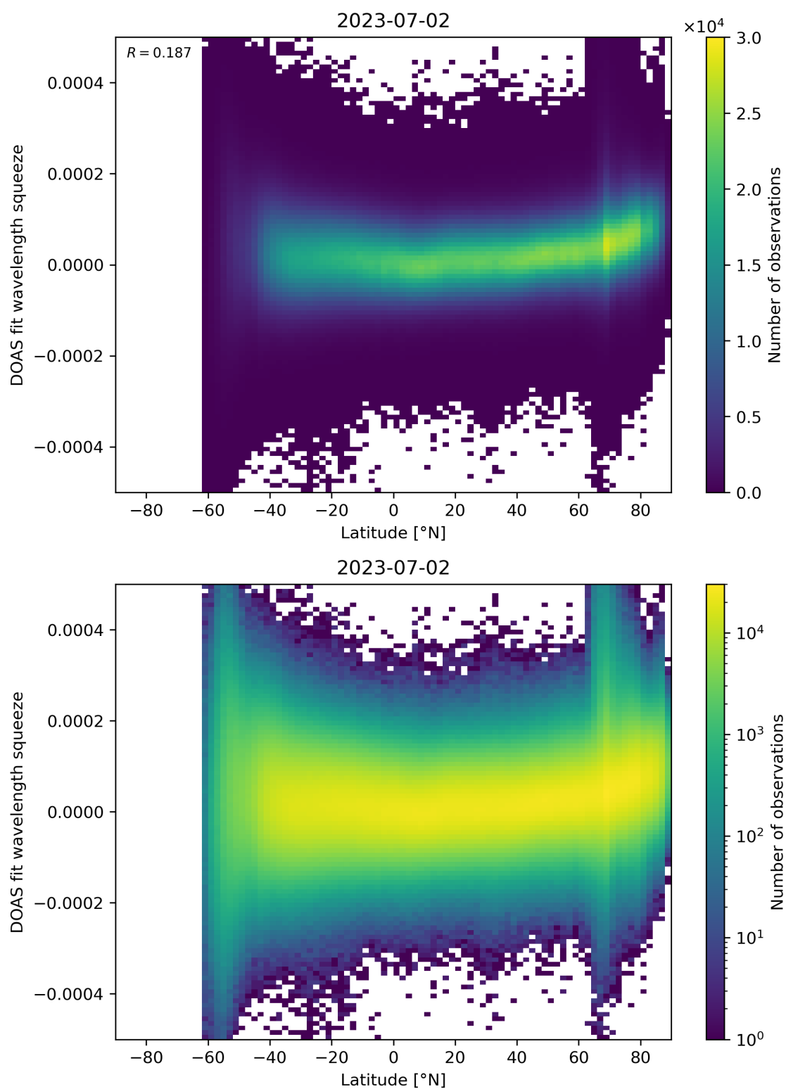
Figure 155: Scatter density plot of “Latitude” against “DOAS fit wavelength squeeze” for 2023-07-01 to 2023-07-03.
