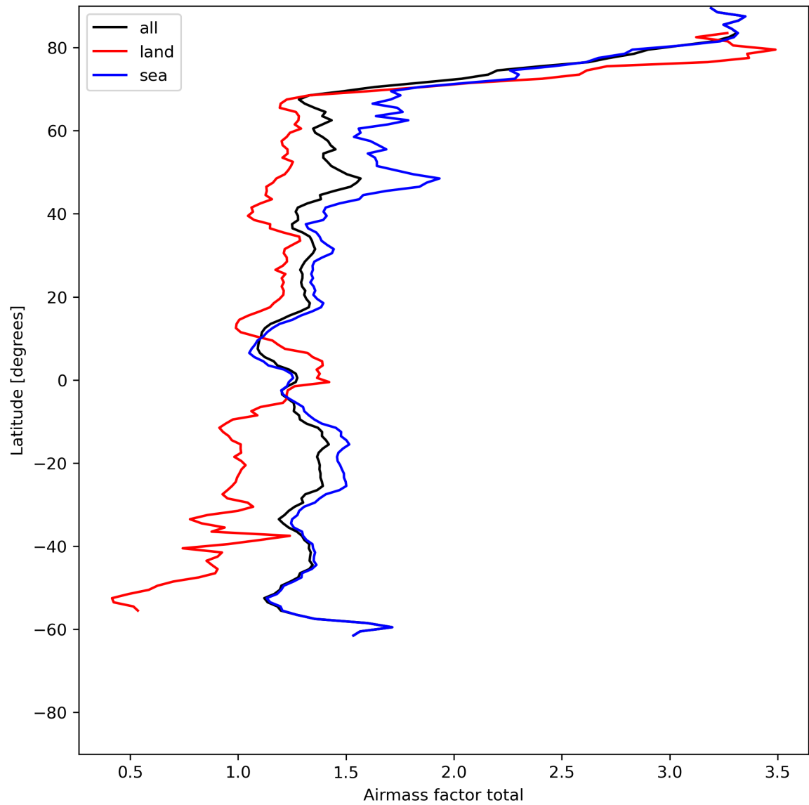
Figure 26: Zonal average of “Airmass factor total” for 2023-07-01 to 2023-07-03.
