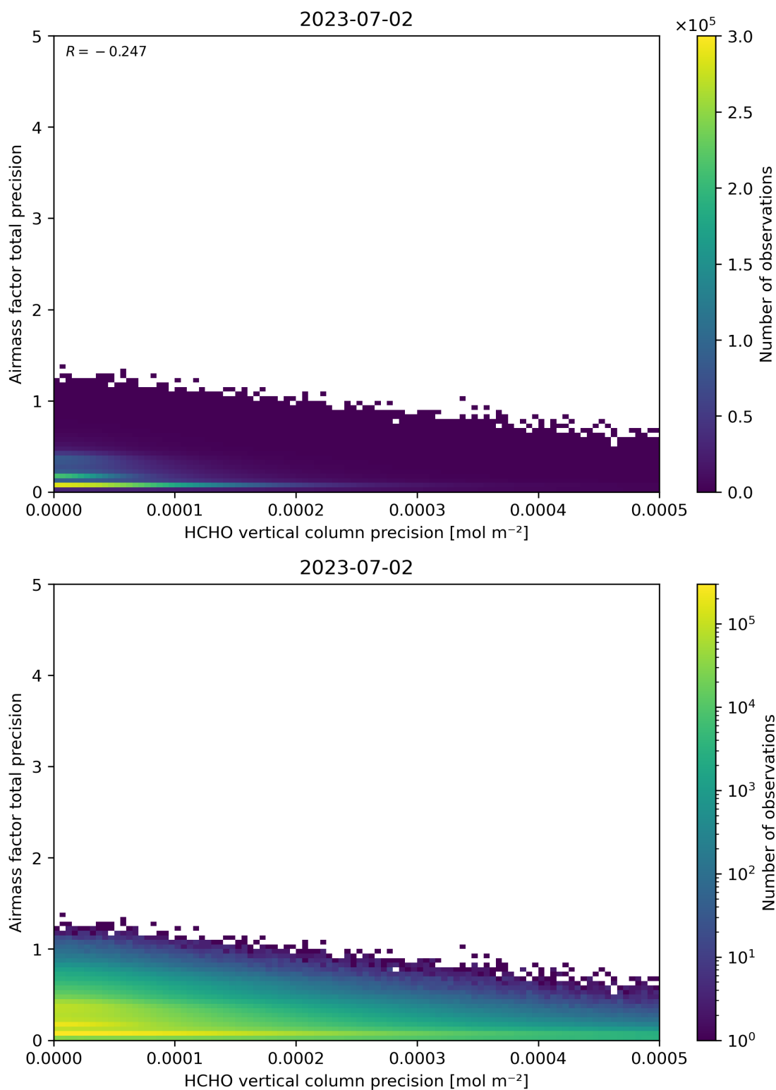
Figure 145: Scatter density plot of “HCHO vertical column precision” against “Airmass factor total precision” for 2023-07-01 to 2023-07-03.
