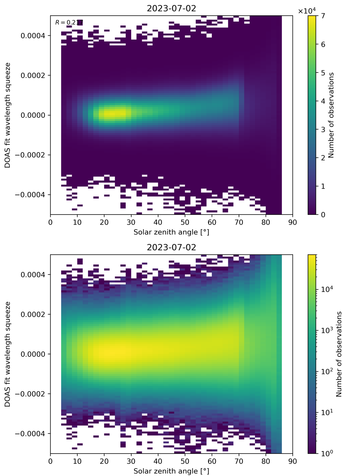
Figure 169: Scatter density plot of “Solar zenith angle” against “DOAS fit wavelength squeeze” for 2023-07-01 to 2023-07-03.
