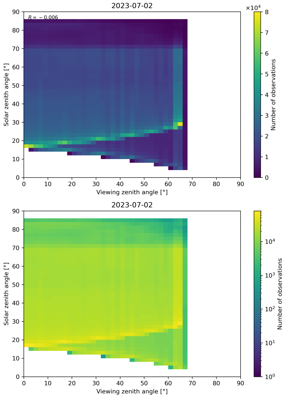
Figure 197: Scatter density plot of “Viewing zenith angle” against “Solar zenith angle” for 2023-07-01 to 2023-07-03.
