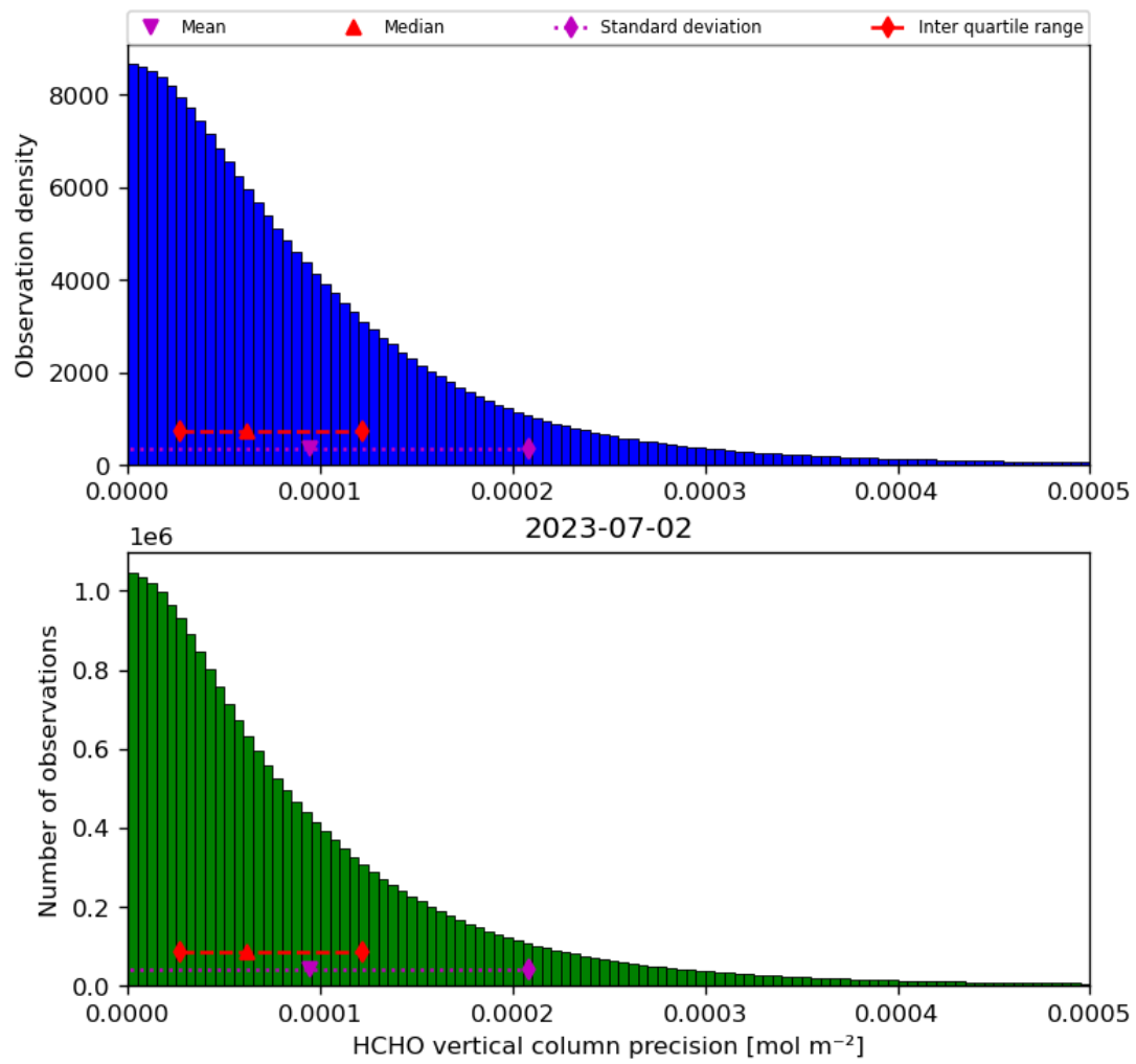
Figure 36: Histogram of “HCHO vertical column precision” for 2023-07-01 to 2023-07-03
