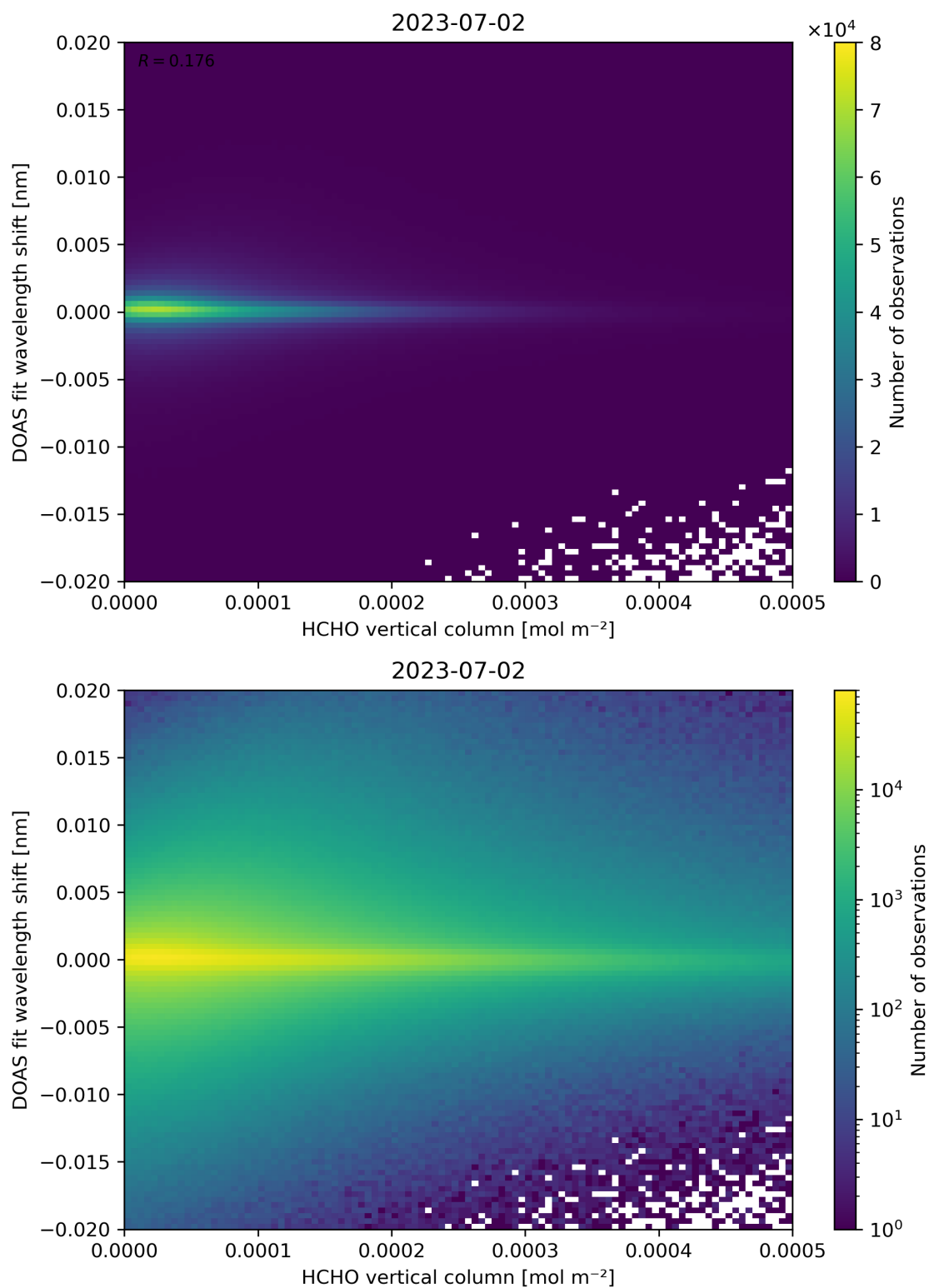
Figure 124: Scatter density plot of “HCHO vertical column” against “DOAS fit wavelength shift” for 2023-07-01 to 2023-07-03.
