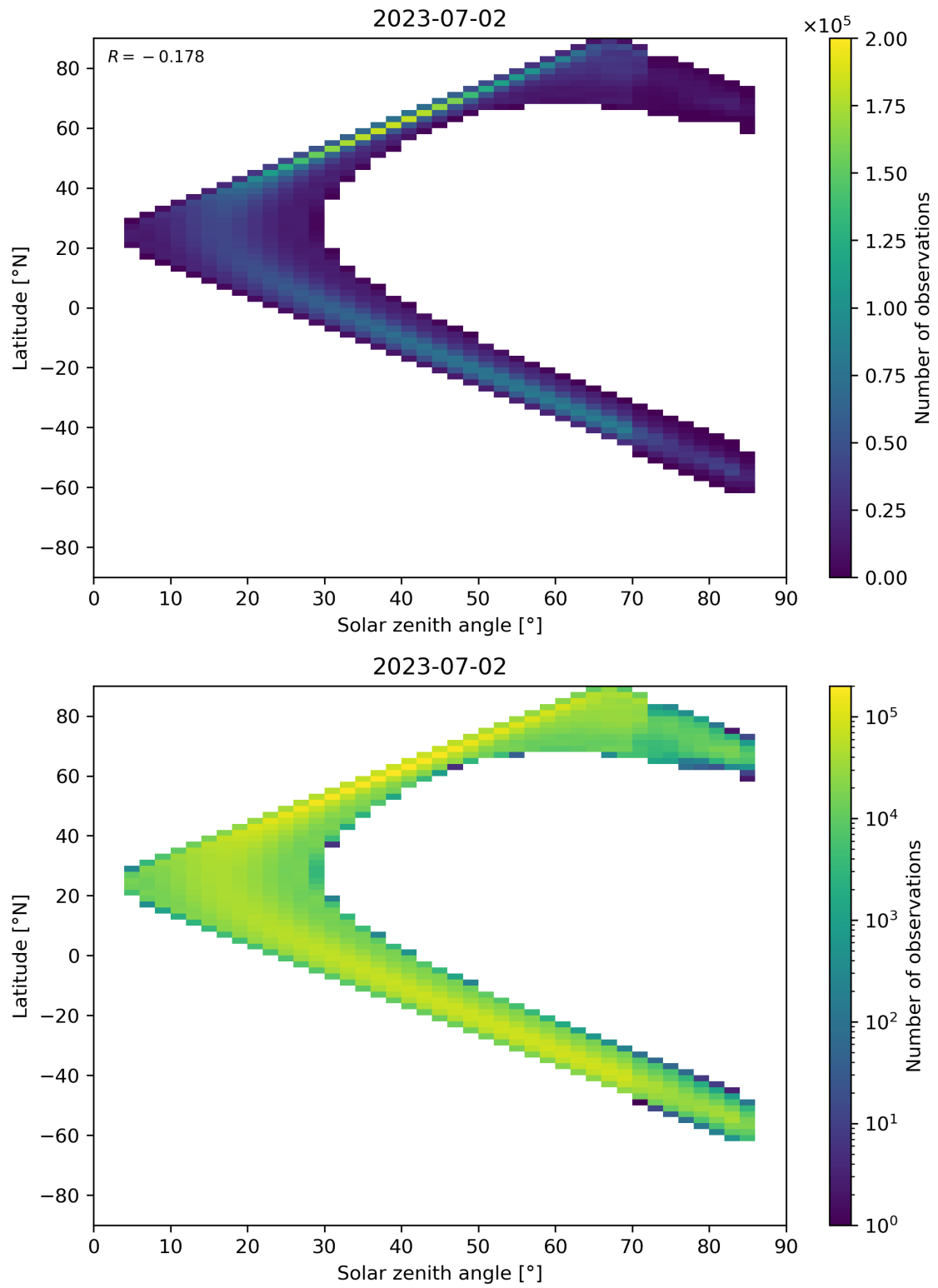
Figure 181: Scatter density plot of “Solar zenith angle” against “Latitude” for 2023-07-01 to 2023-07-03.
