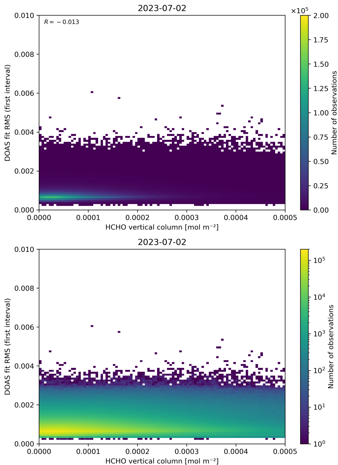
Figure 123: Scatter density plot of “HCHO vertical column” against “DOAS fit RMS (first interval)” for 2023-07-01 to 2023-07-03.
