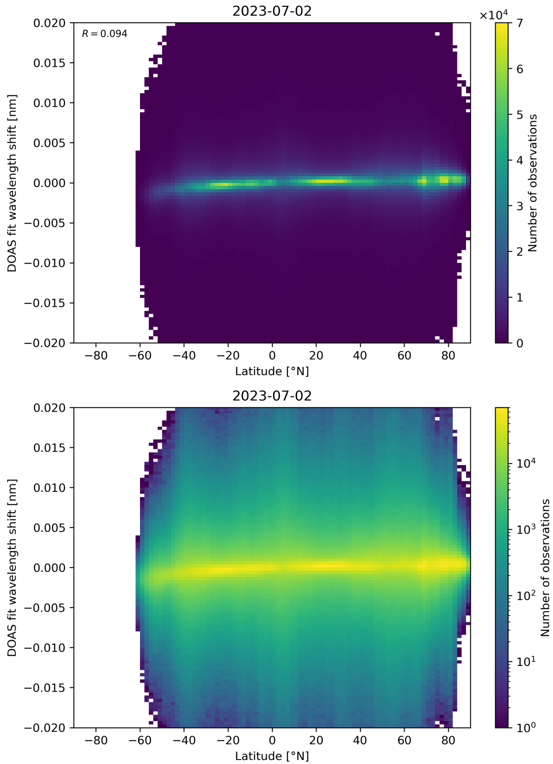
Figure 154: Scatter density plot of “Latitude” against “DOAS fit wavelength shift” for 2023-07-01 to 2023-07-03.
