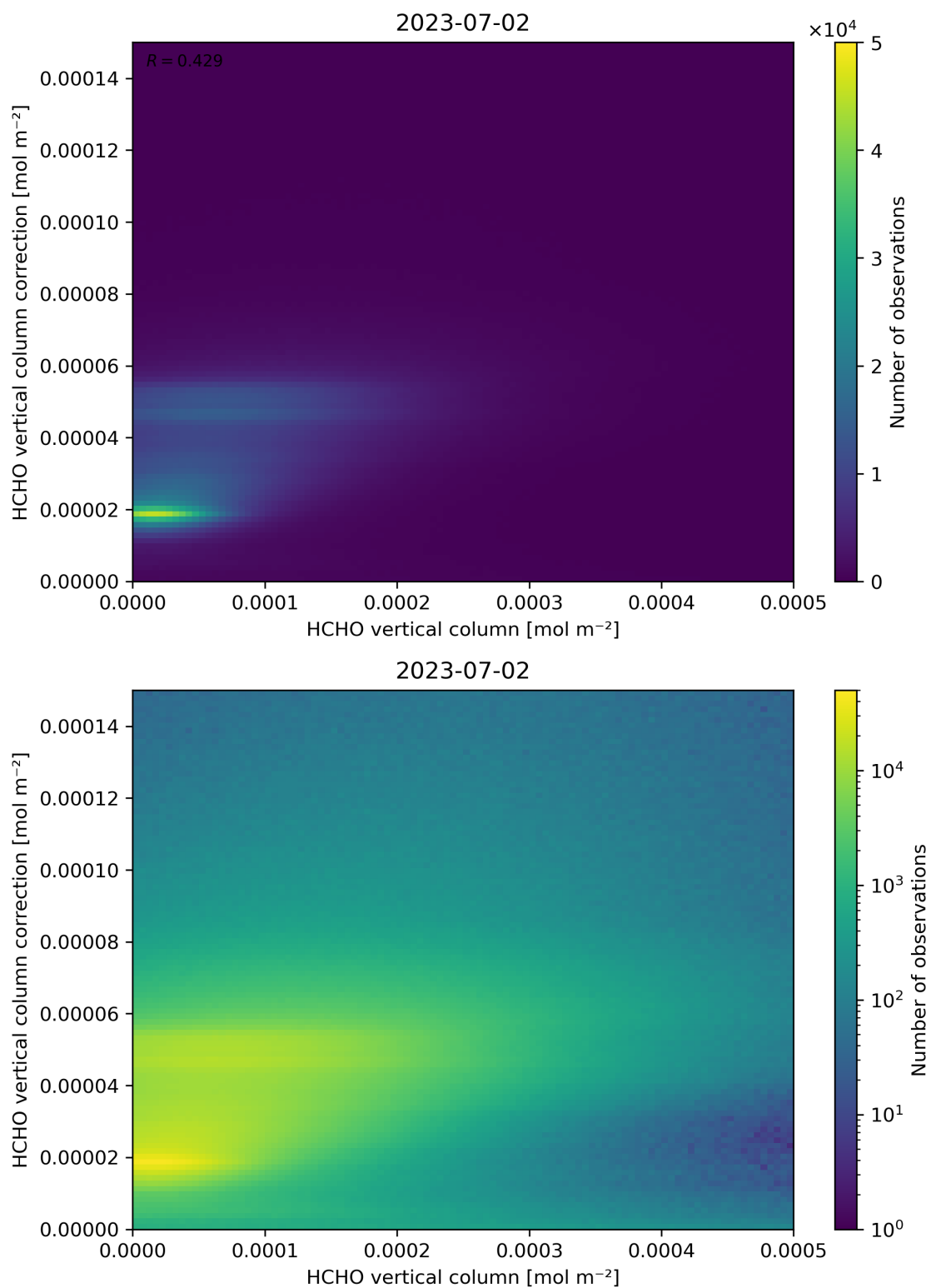
Figure 133: Scatter density plot of “HCHO vertical column” against “HCHO vertical column correction” for 2023-07-01 to 2023-07-03.
