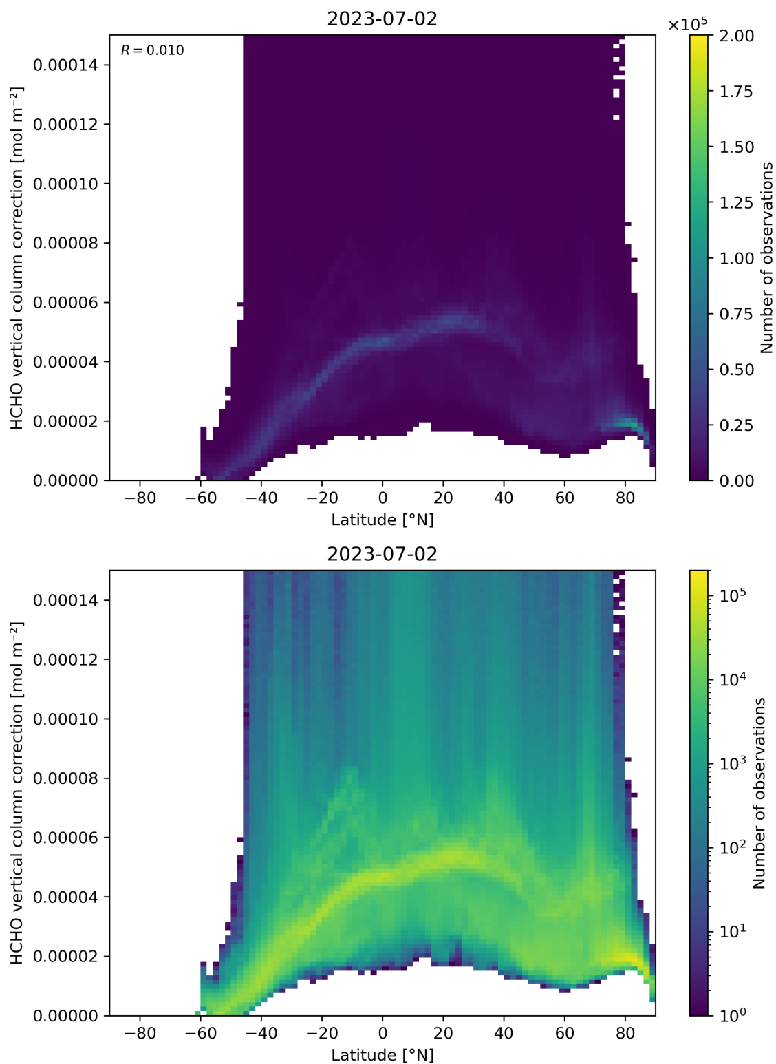
Figure 164: Scatter density plot of “Latitude” against “HCHO vertical column correction” for 2023-07-01 to 2023-07-03.
