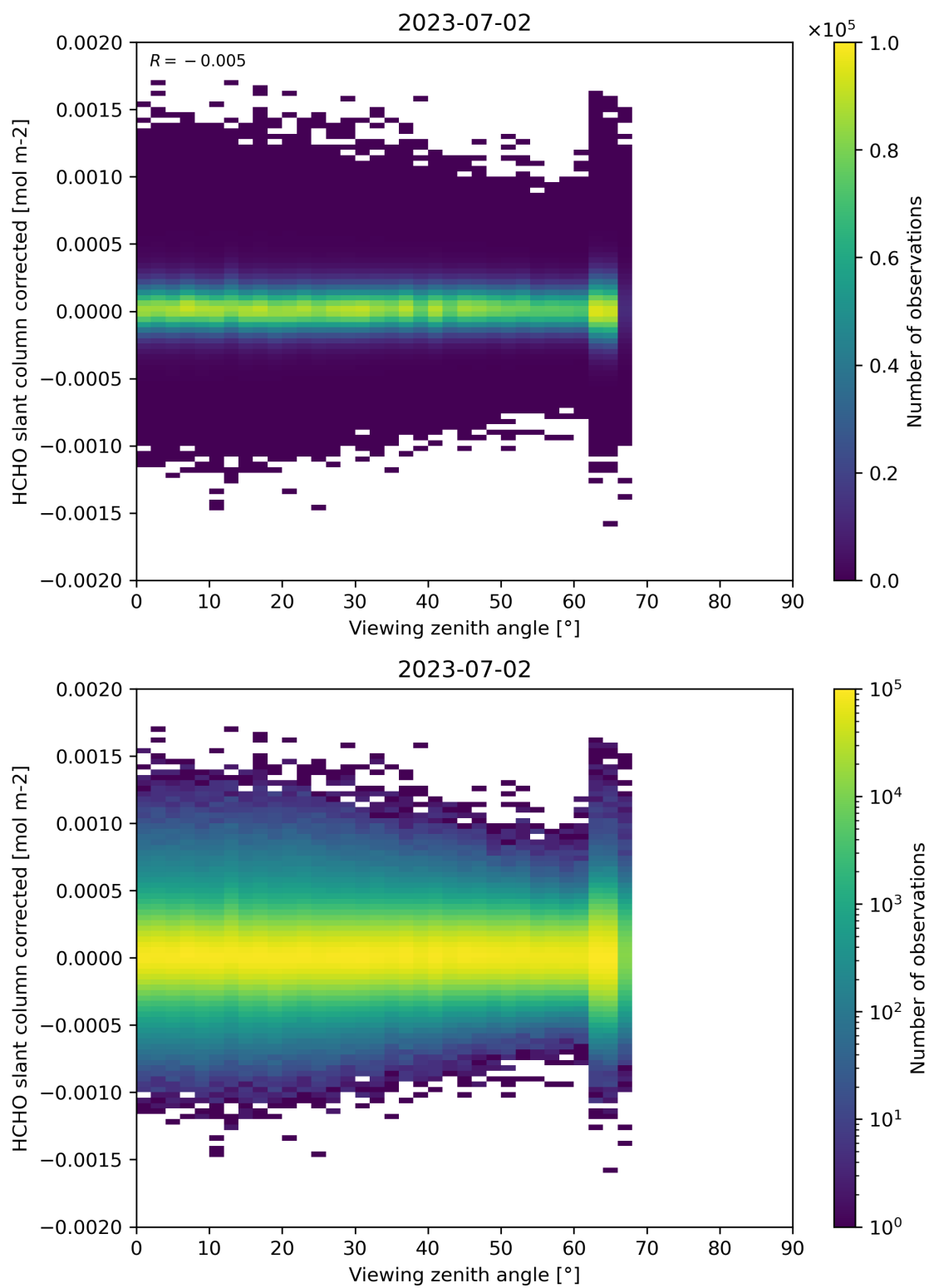
Figure 186: Scatter density plot of “Viewing zenith angle” against “HCHO slant column corrected” for 2023-07-01 to 2023-07-03.
