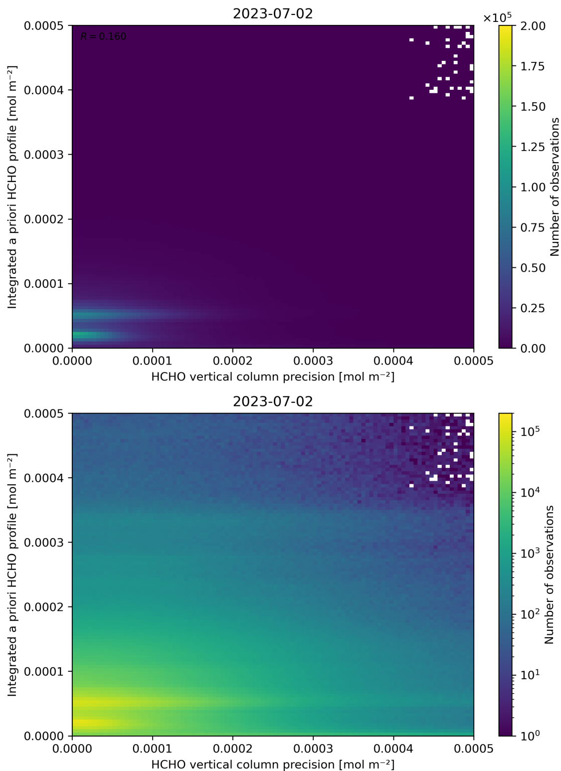
Figure 147: Scatter density plot of “HCHO vertical column precision” against “Integrated a priori HCHO profile” for 2023-07-01 to 2023-07-03.
