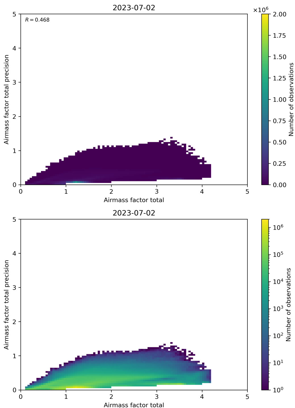
Figure 103: Scatter density plot of “Airmass factor total” against “Airmass factor total precision” for 2023-07-01 to 2023-07-03.
