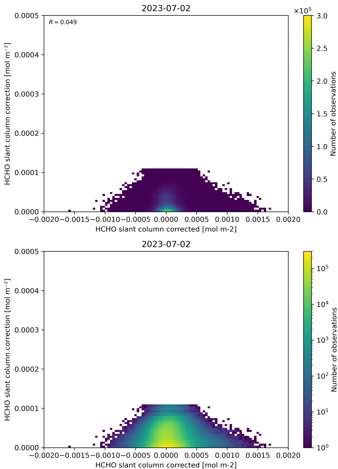
Figure 77: Scatter density plot of “HCHO slant column corrected” against “HCHO slant column correction” for 2023-07-01 to 2023-07-03.
