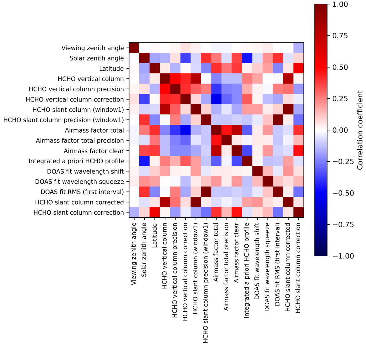
Figure 2: Map of correlation matrix for 2023-07-01 to 2023-07-03.
