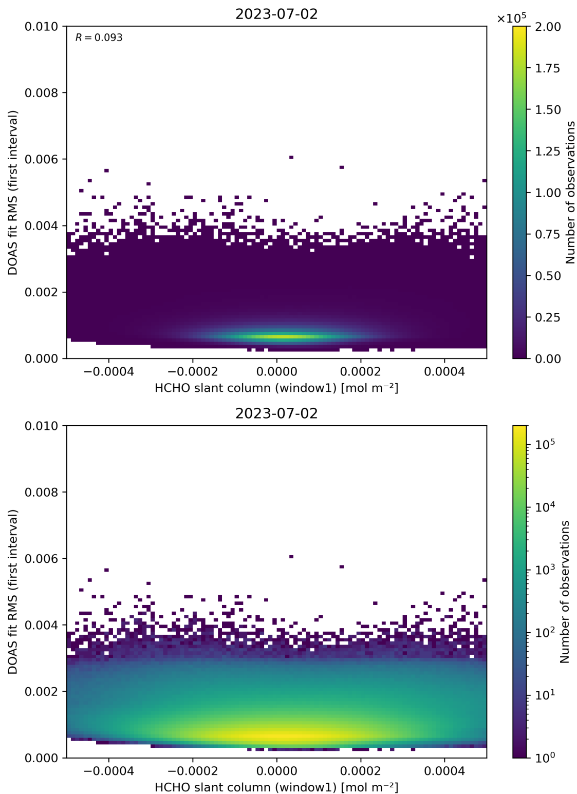
Figure 78: Scatter density plot of “HCHO slant column (window1)” against “DOAS fit RMS (first interval)” for 2023-07-01 to 2023-07-03.
