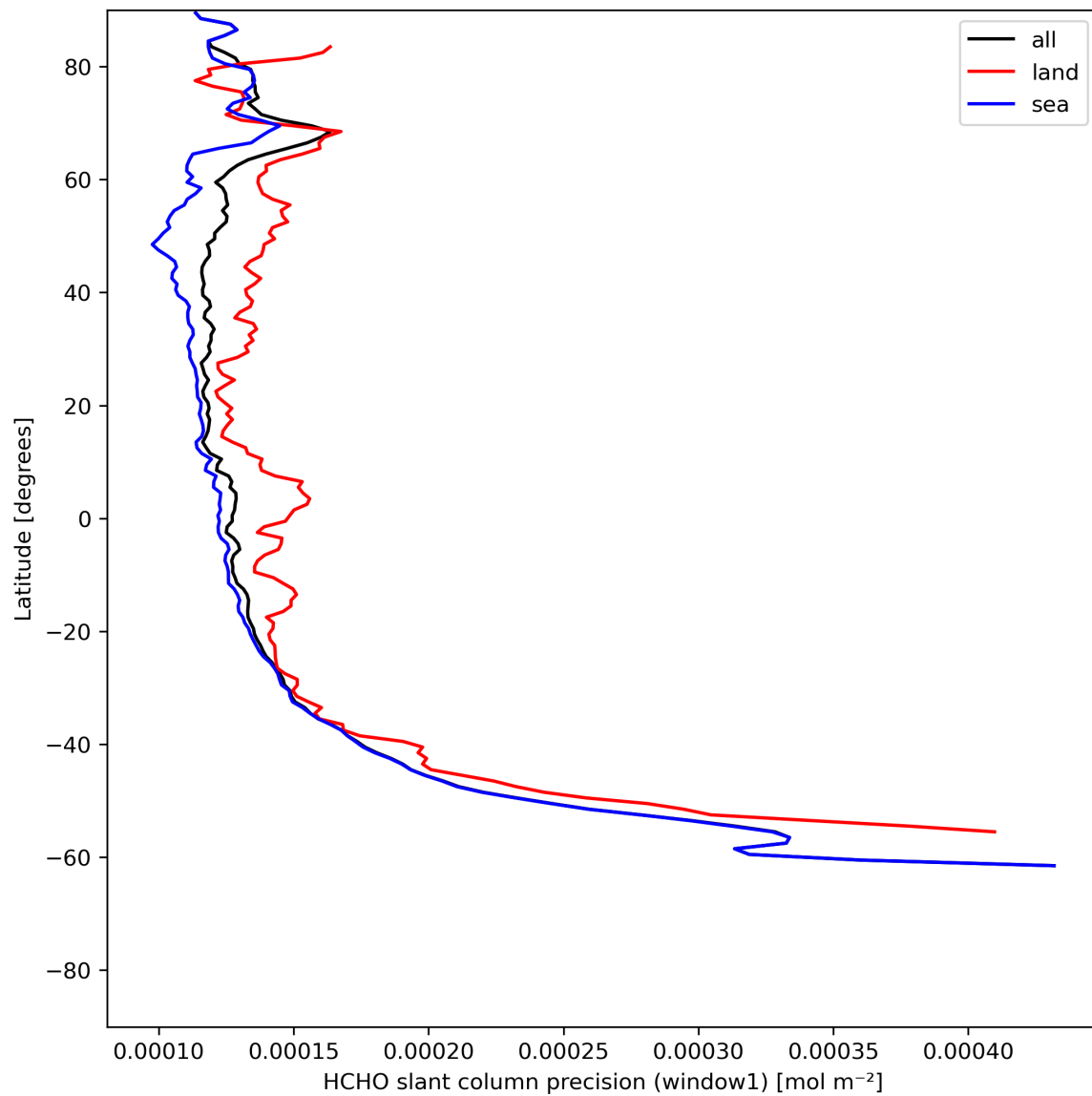
Figure 25: Zonal average of “HCHO slant column precision (window1)” for 2023-07-01 to 2023-07-03.
