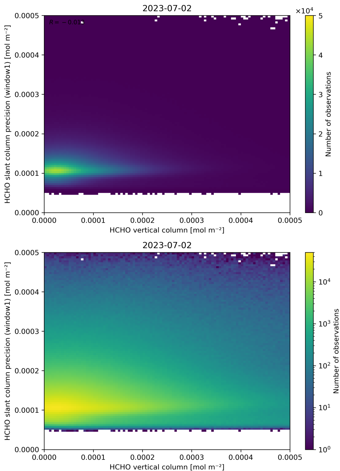
Figure 130: Scatter density plot of “HCHO vertical column” against “HCHO slant column precision (window1)” for 2023-07-01 to 2023-07-03.
