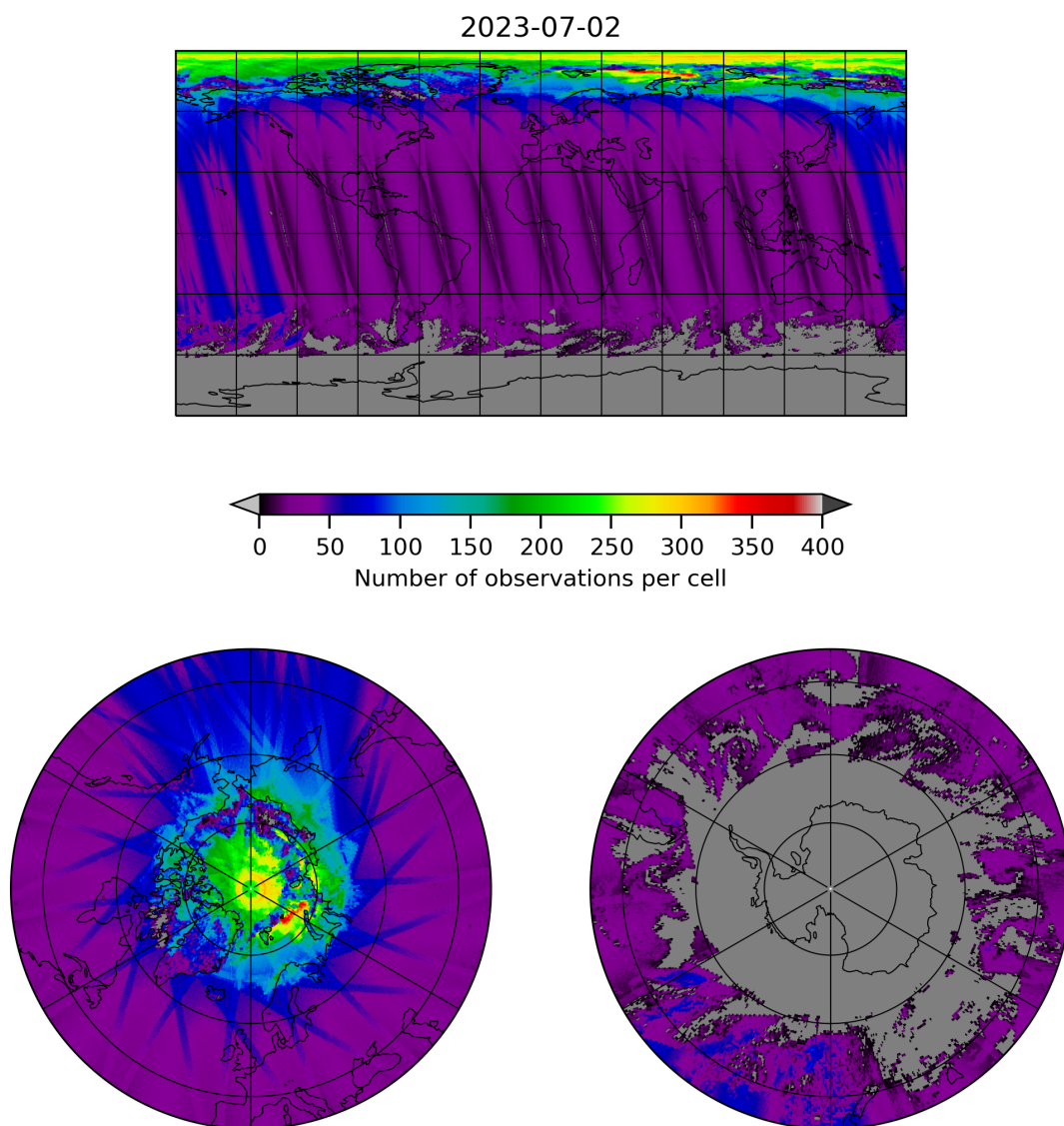
Figure 19: Map of the number of observations for 2023-07-01 to 2023-07-03
