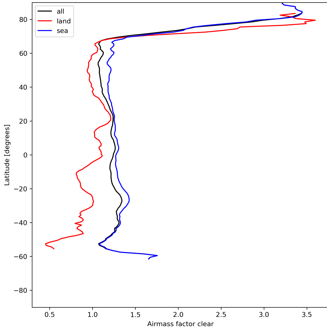
Figure 28: Zonal average of “Airmass factor clear” for 2023-07-01 to 2023-07-03.
