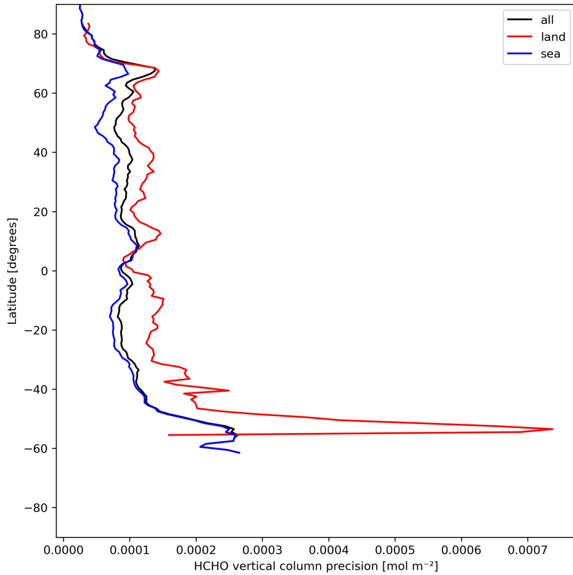
Figure 22: Zonal average of “HCHO vertical column precision” for 2023-07-01 to 2023-07-03.
