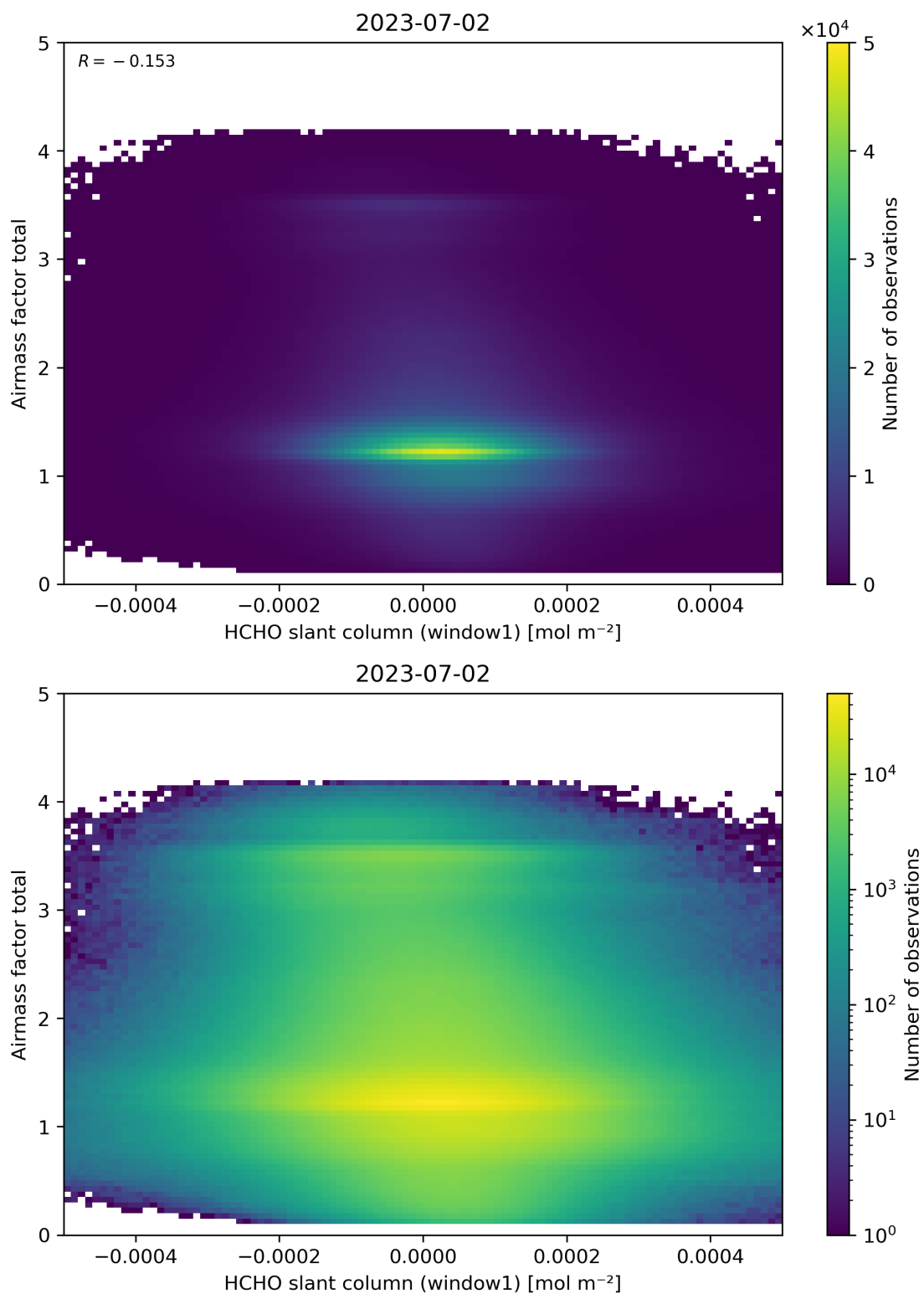
Figure 85: Scatter density plot of “HCHO slant column (window1)” against “Airmass factor total” for 2023-07-01 to 2023-07-03.
