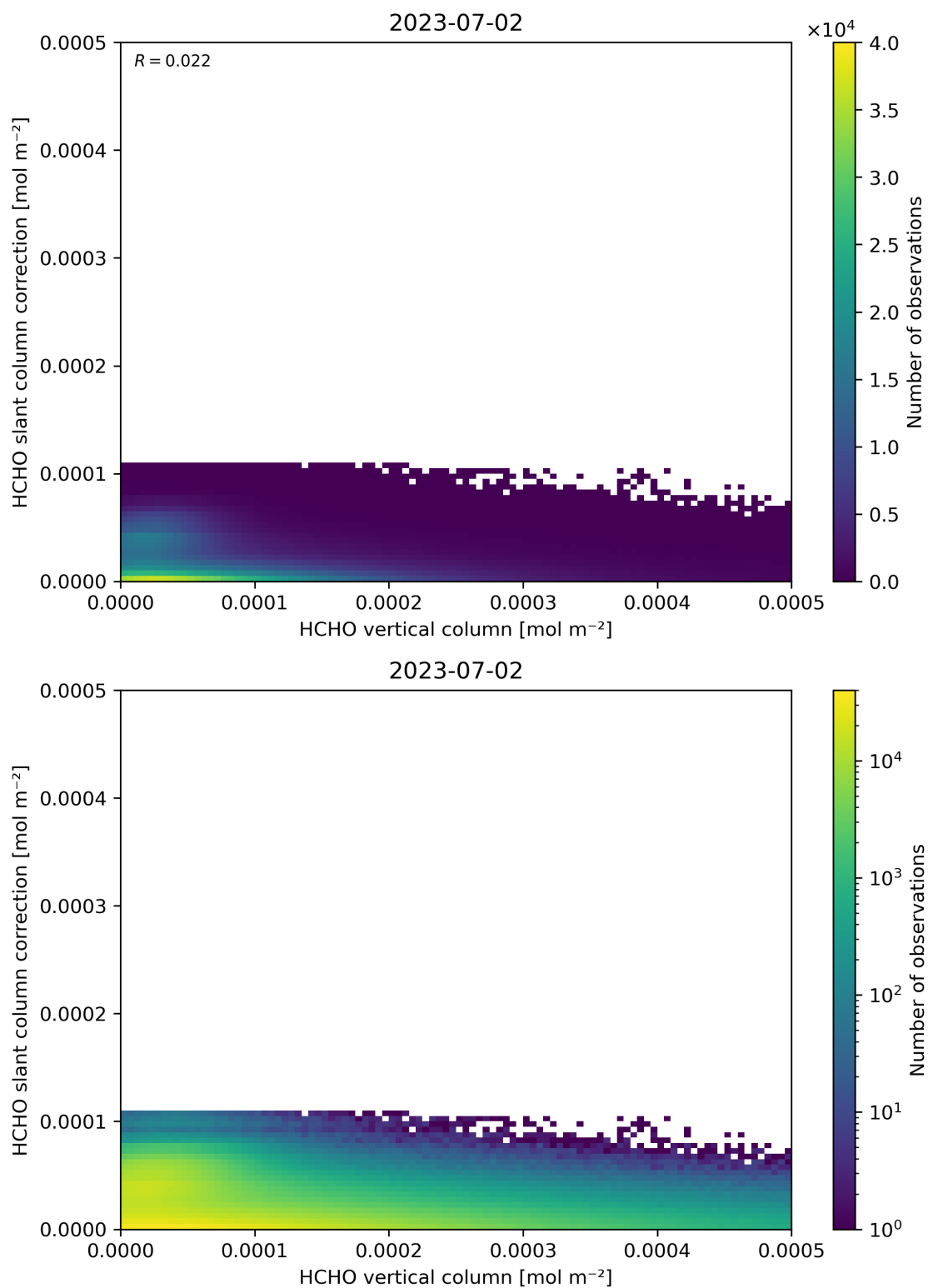
Figure 128: Scatter density plot of “HCHO vertical column” against “HCHO slant column correction” for 2023-07-01 to 2023-07-03.
