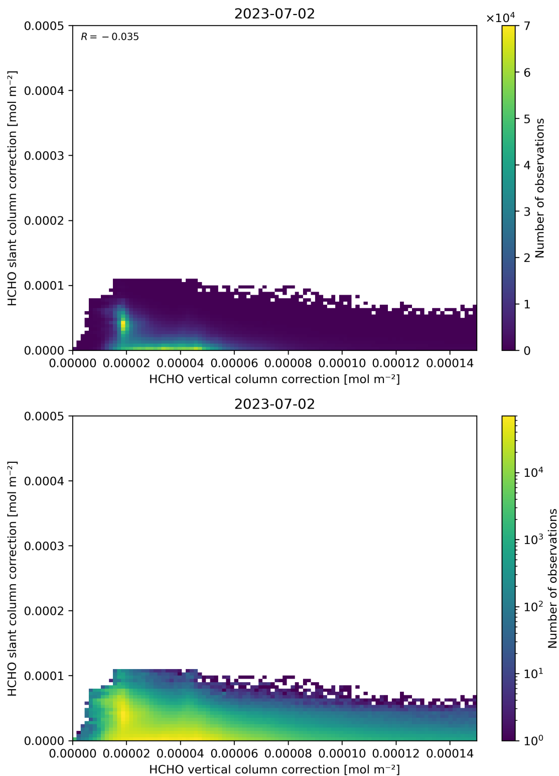
Figure 117: Scatter density plot of “HCHO vertical column correction” against “HCHO slant column correction” for 2023-07-01 to 2023-07-03.
