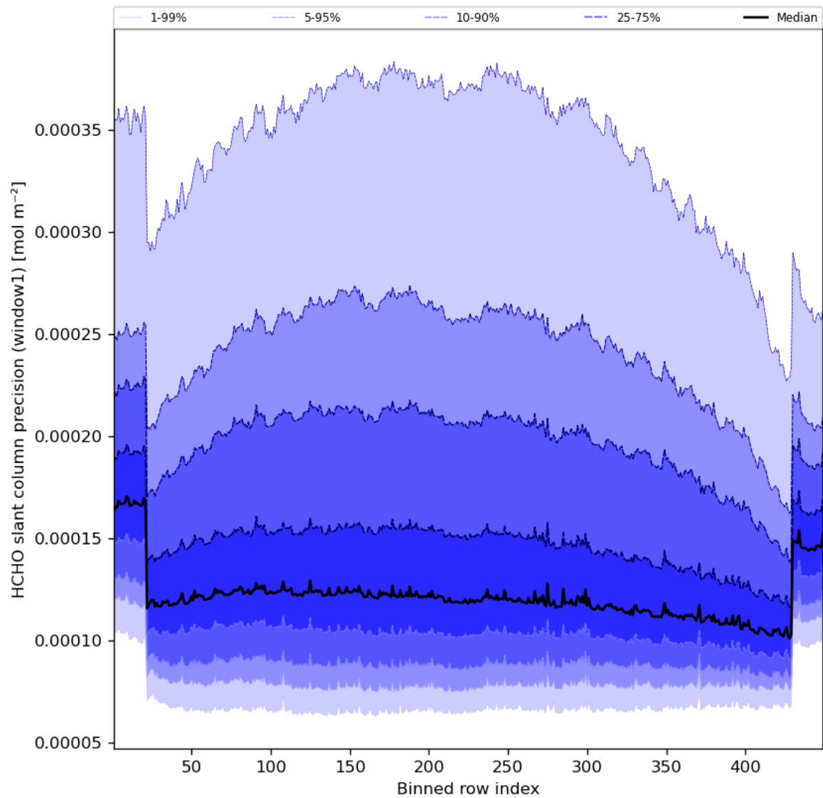
Figure 53: Along track statistics of “HCHO slant column precision (window1)” for 2023-07-01 to 2023-07-03
