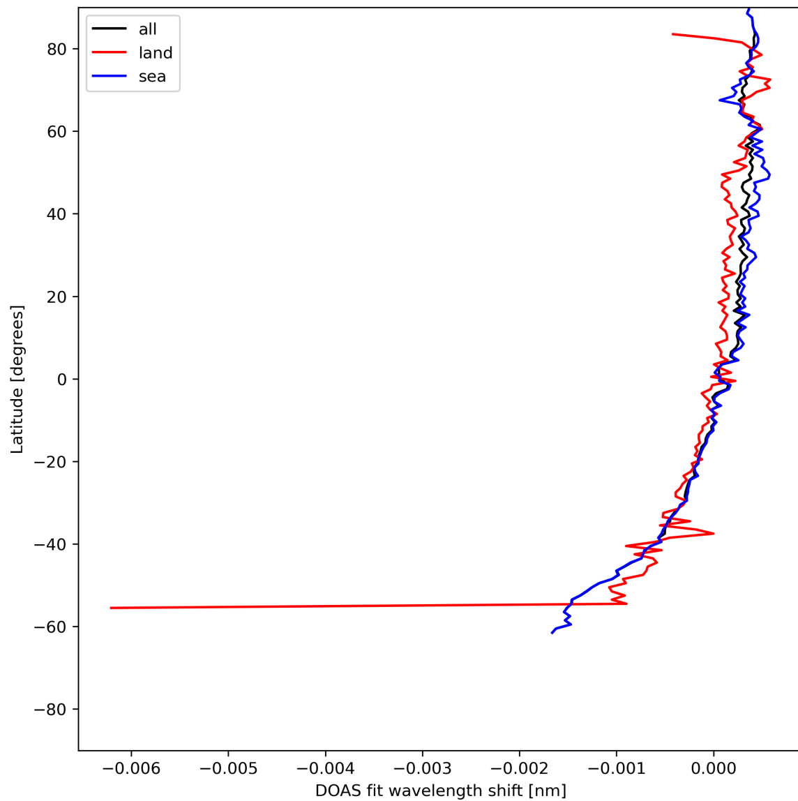
Figure 30: Zonal average of “DOAS fit wavelength shift” for 2023-07-01 to 2023-07-03.
