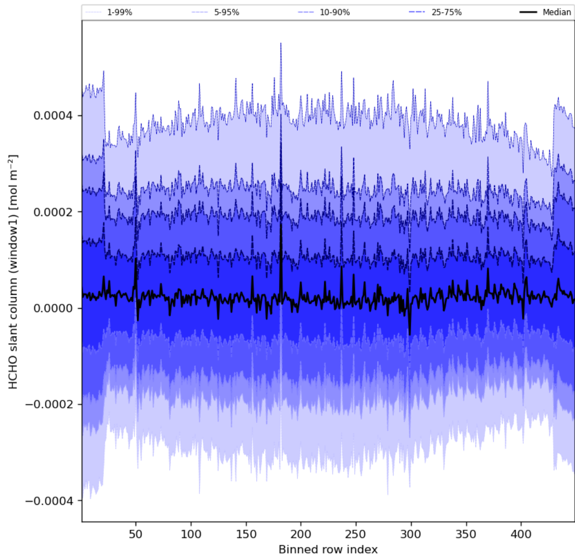
Figure 52: Along track statistics of “HCHO slant column (window1)” for 2023-07-01 to 2023-07-03
