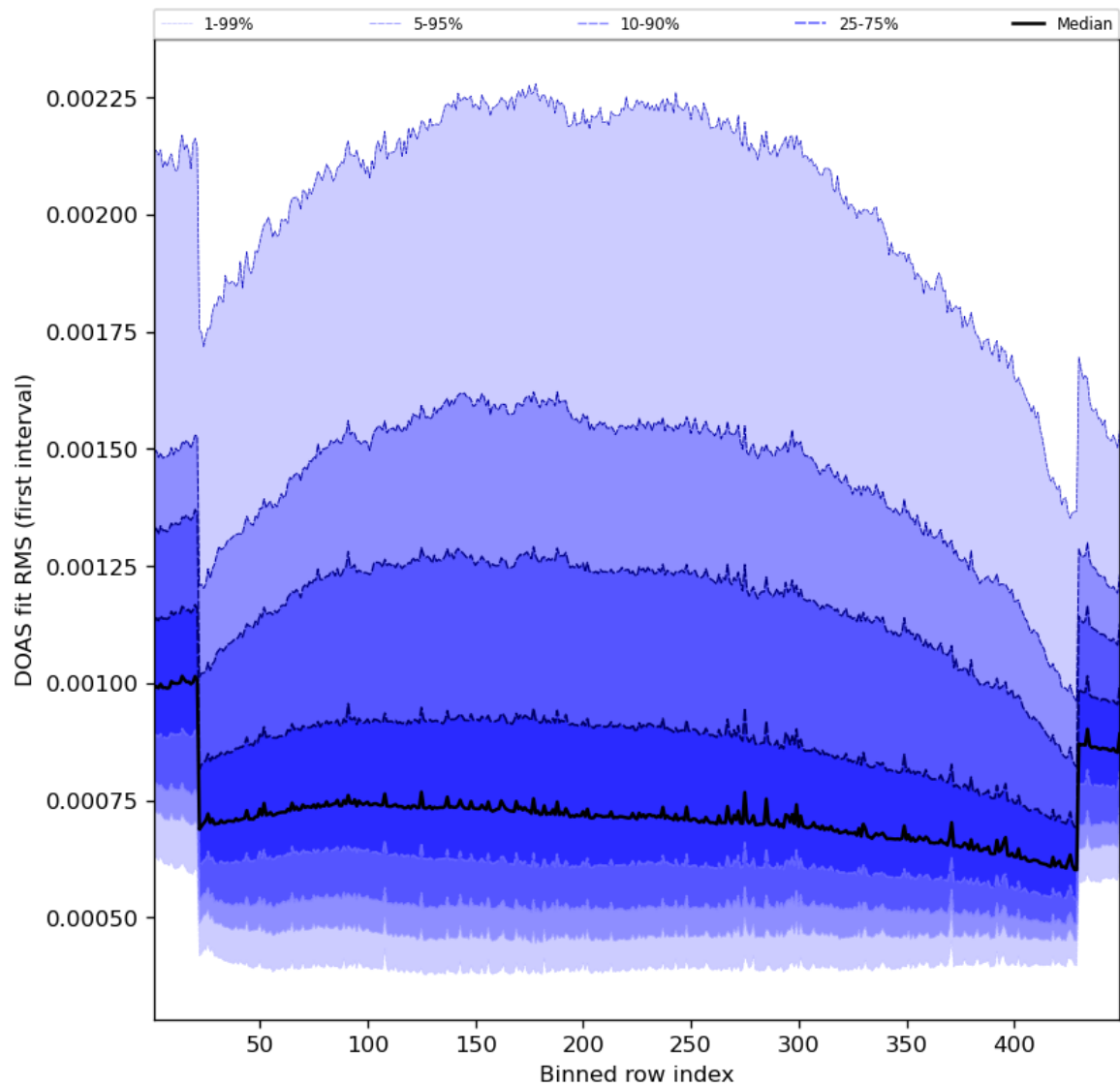
Figure 60: Along track statistics of “DOAS fit RMS (first interval)” for 2023-07-01 to 2023-07-03
