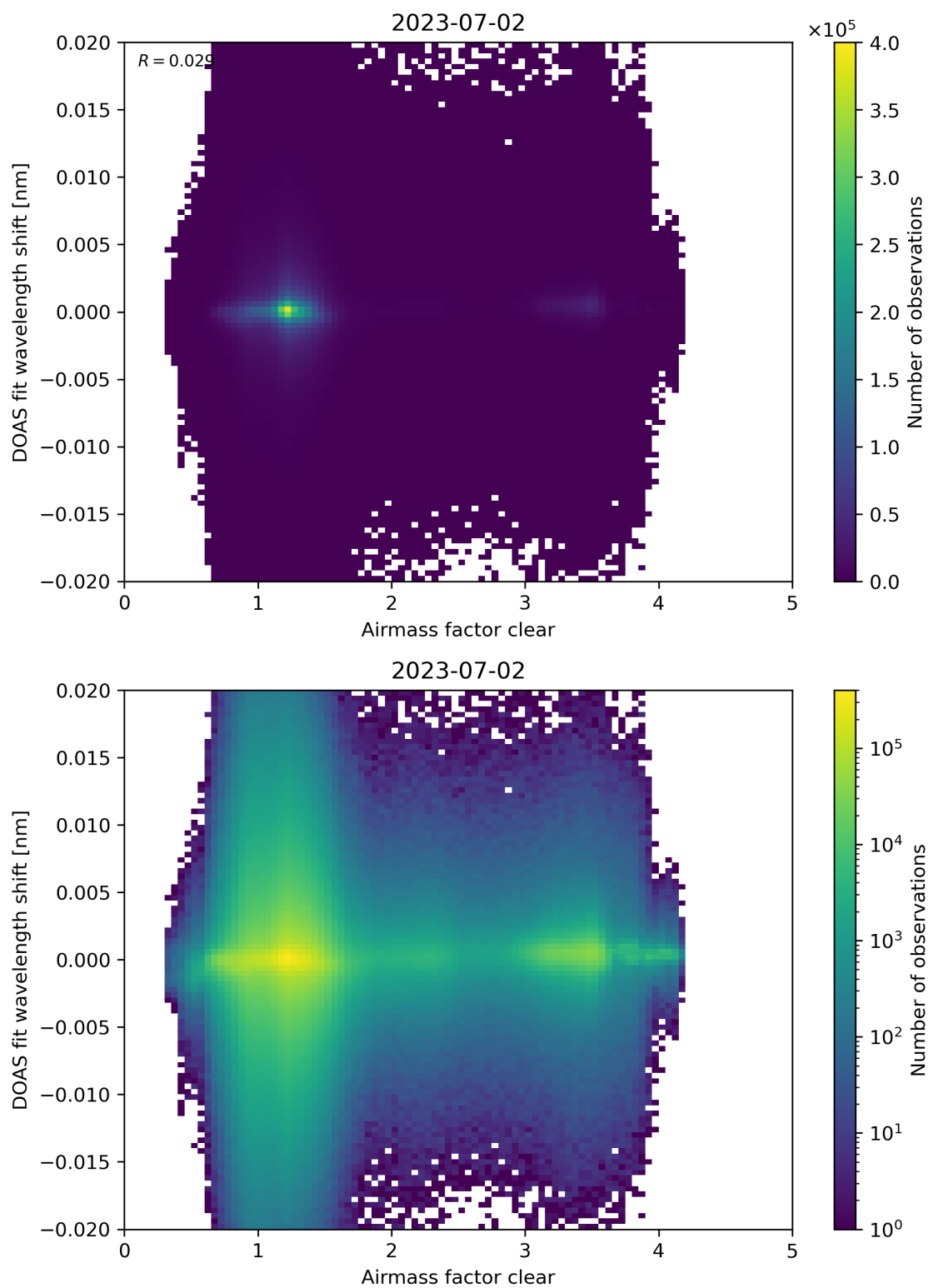
Figure 72: Scatter density plot of “Airmass factor clear” against “DOAS fit wavelength shift” for 2023-07-01 to 2023-07-03.
