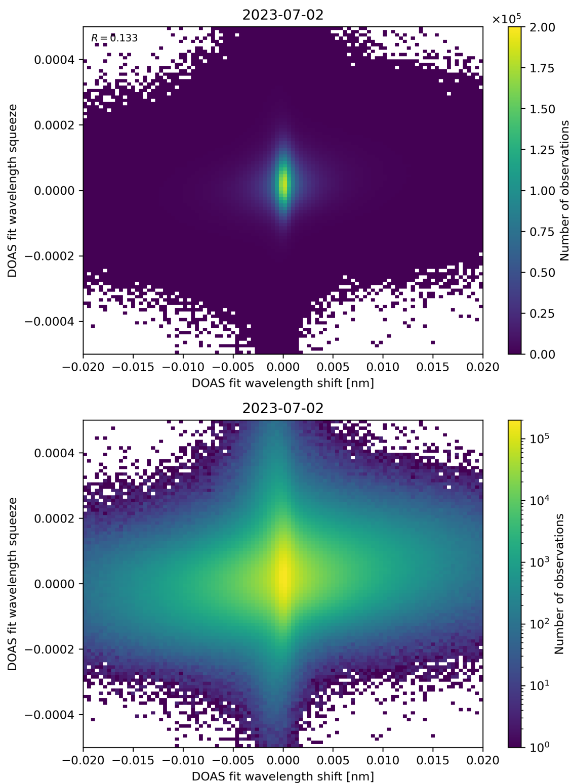
Figure 65: Scatter density plot of “DOAS fit wavelength shift” against “DOAS fit wavelength squeeze” for 2023-07-01 to 2023-07-03.
