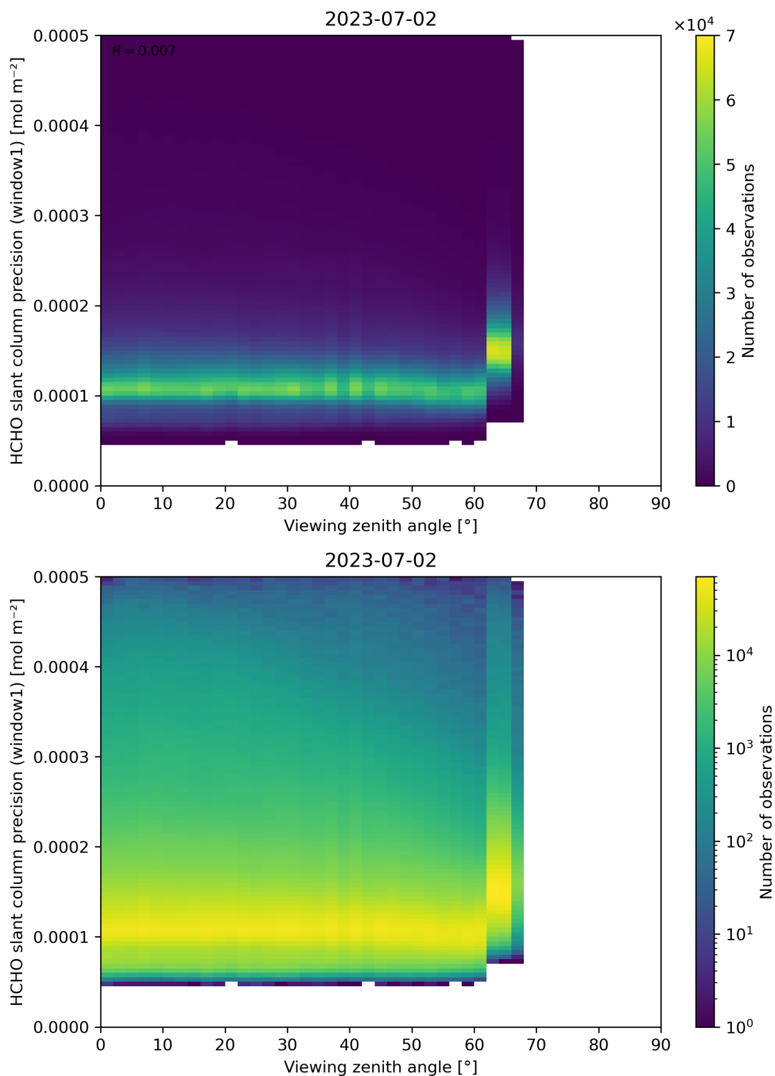
Figure 189: Scatter density plot of “Viewing zenith angle” against “HCHO slant column precision (window1)” for 2023-07-01 to 2023-07-03.
