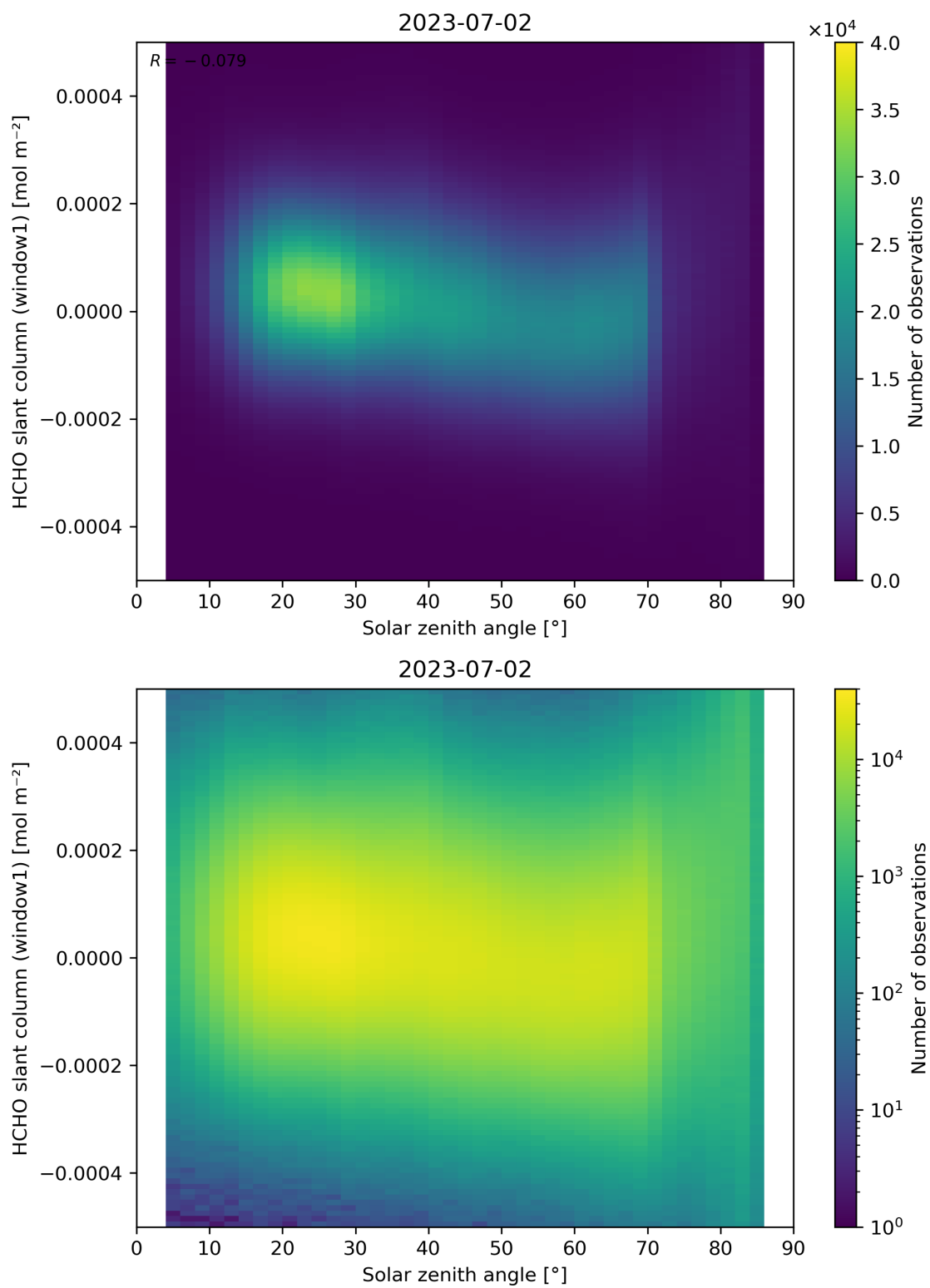
Figure 173: Scatter density plot of “Solar zenith angle” against “HCHO slant column (window1)” for 2023-07-01 to 2023-07-03.
