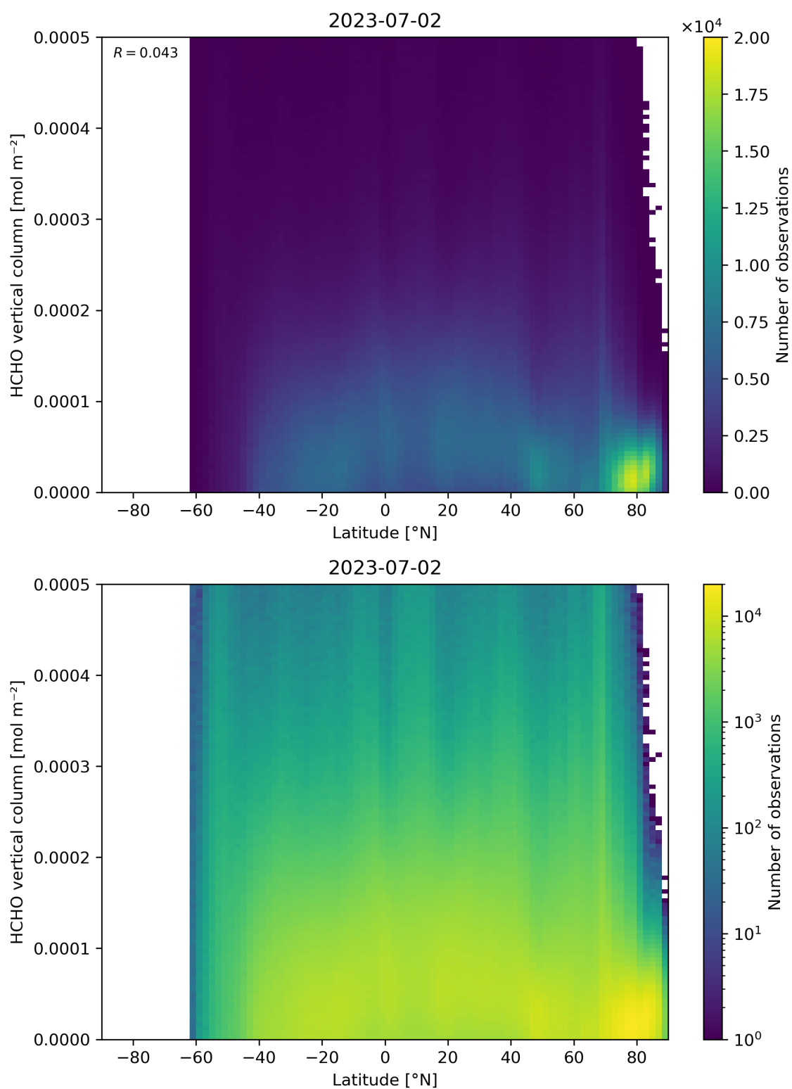
Figure 163: Scatter density plot of “Latitude” against “HCHO vertical column” for 2023-07-01 to 2023-07-03.
