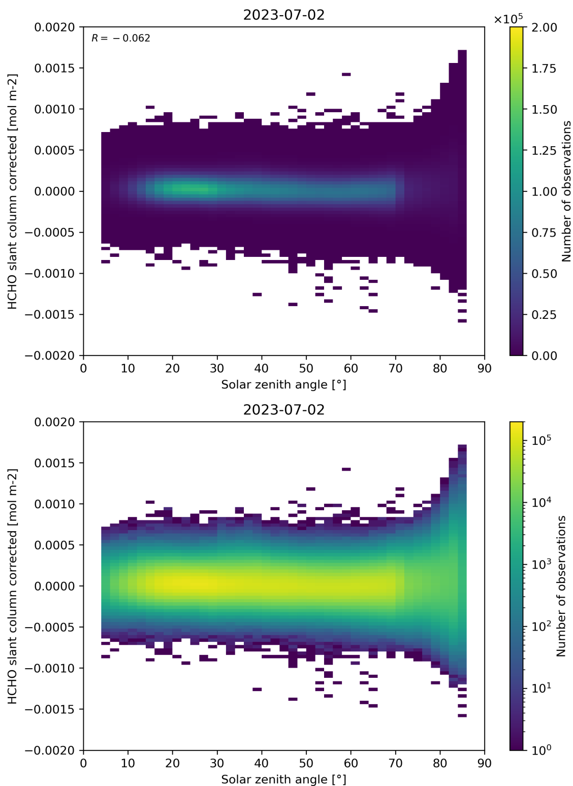
Figure 171: Scatter density plot of “Solar zenith angle” against “HCHO slant column corrected” for 2023-07-01 to 2023-07-03.
