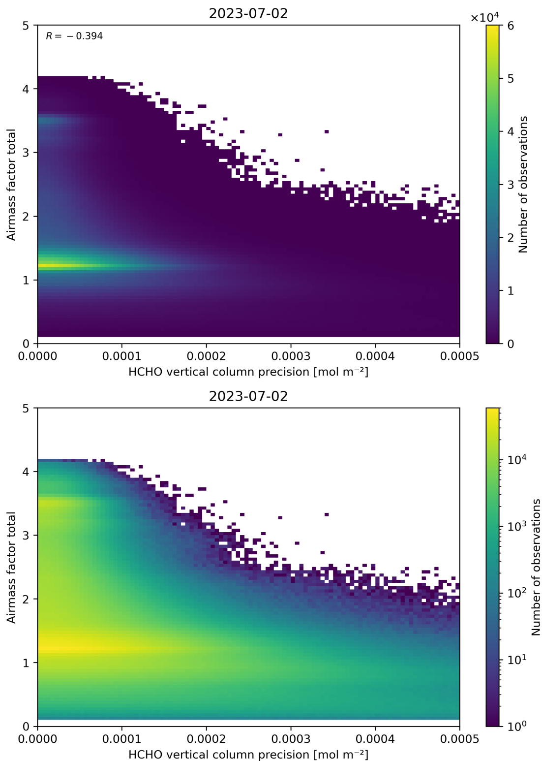
Figure 144: Scatter density plot of “HCHO vertical column precision” against “Airmass factor total” for 2023-07-01 to 2023-07-03.
