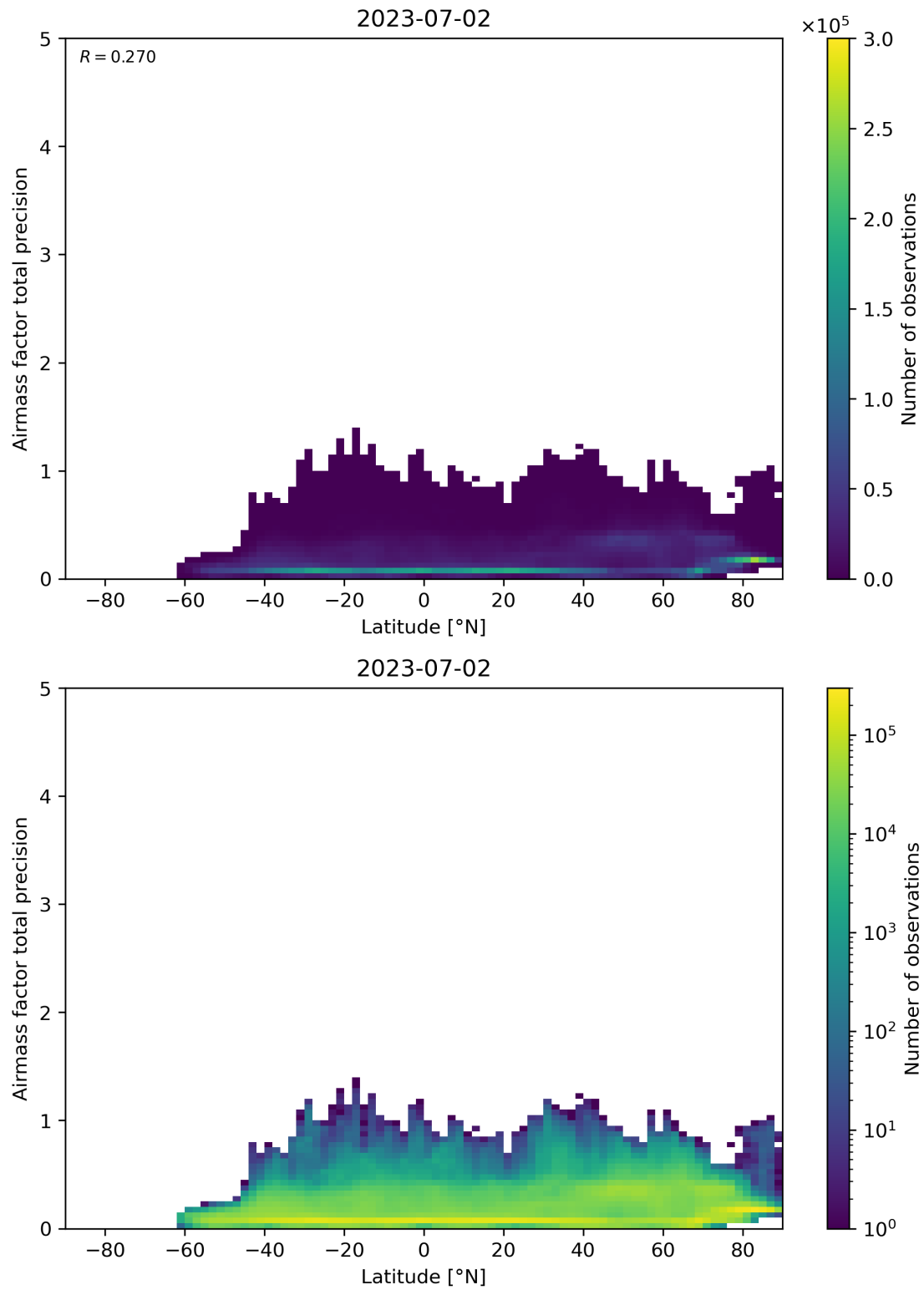
Figure 162: Scatter density plot of “Latitude” against “Airmass factor total precision” for 2023-07-01 to 2023-07-03.
