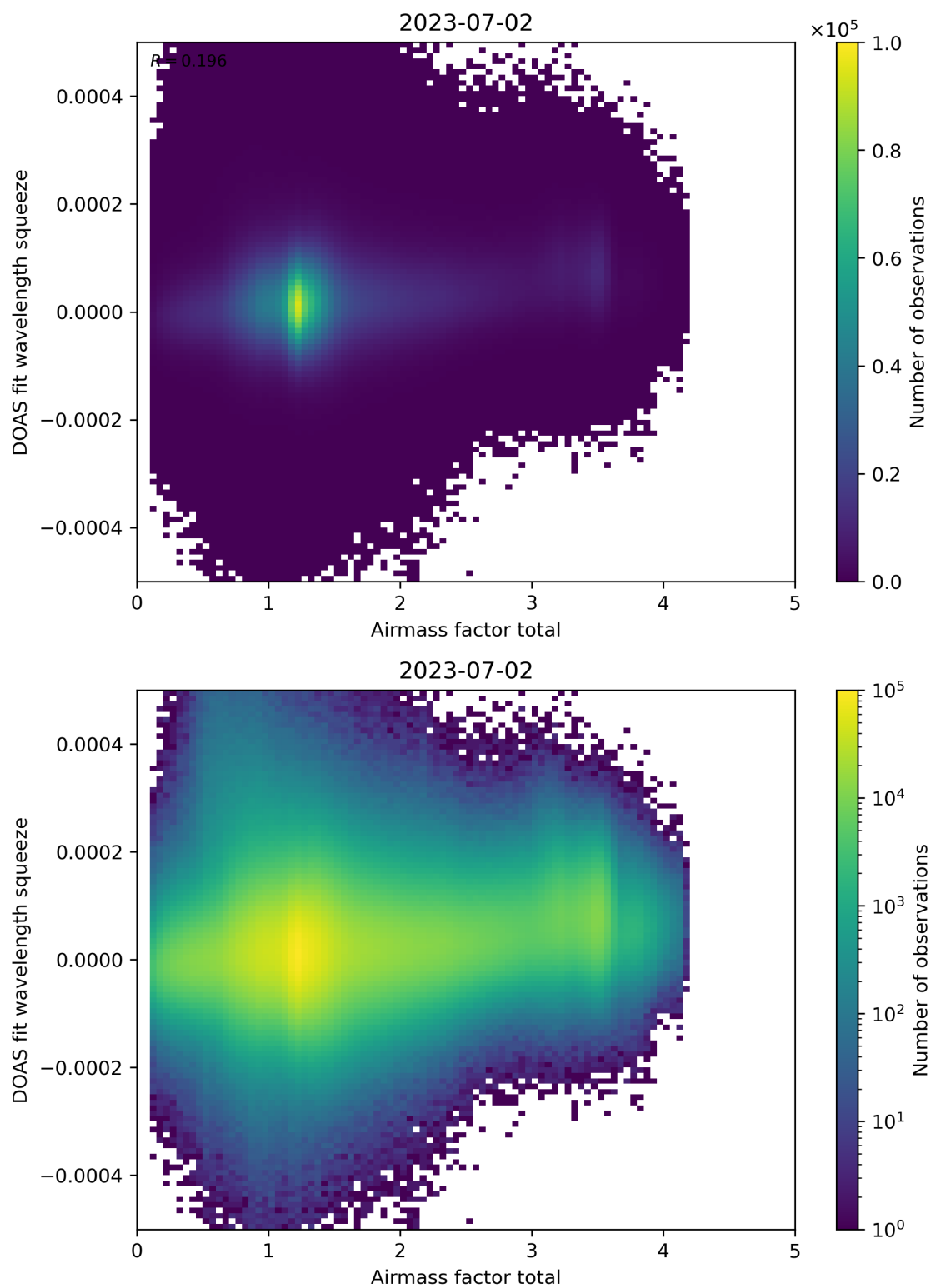
Figure 99: Scatter density plot of “Airmass factor total” against “DOAS fit wavelength squeeze” for 2023-07-01 to 2023-07-03.
