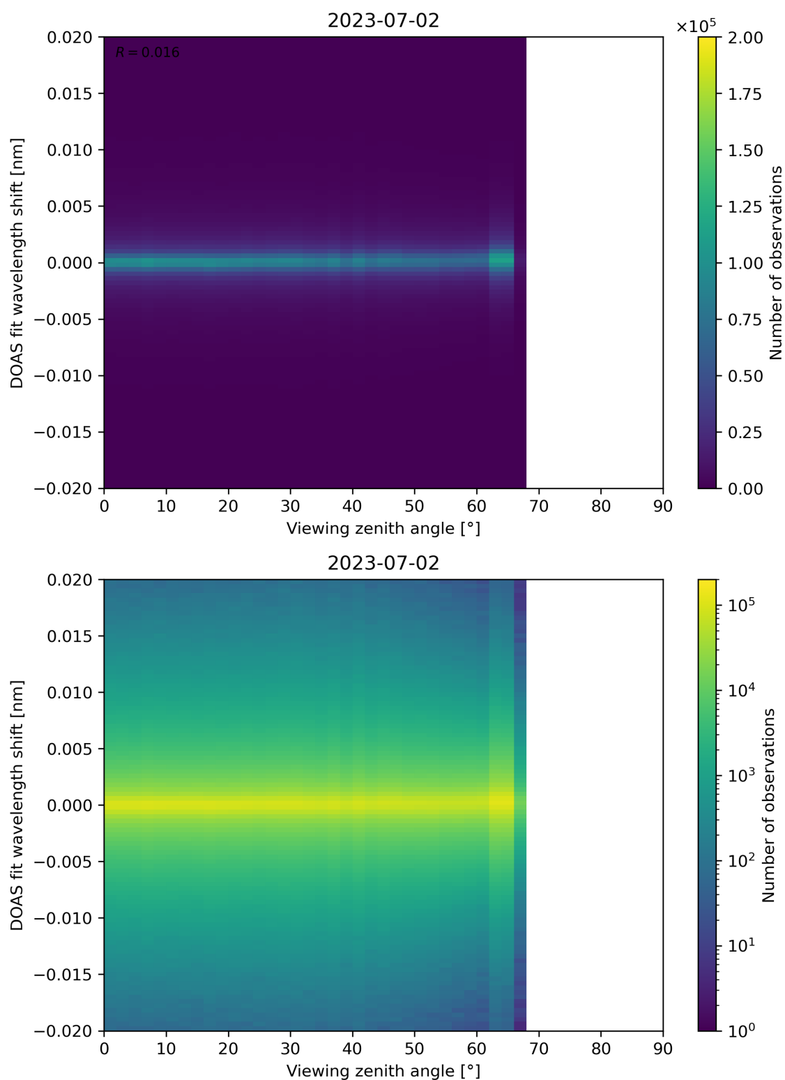
Figure 183: Scatter density plot of “Viewing zenith angle” against “DOAS fit wavelength shift” for 2023-07-01 to 2023-07-03.
