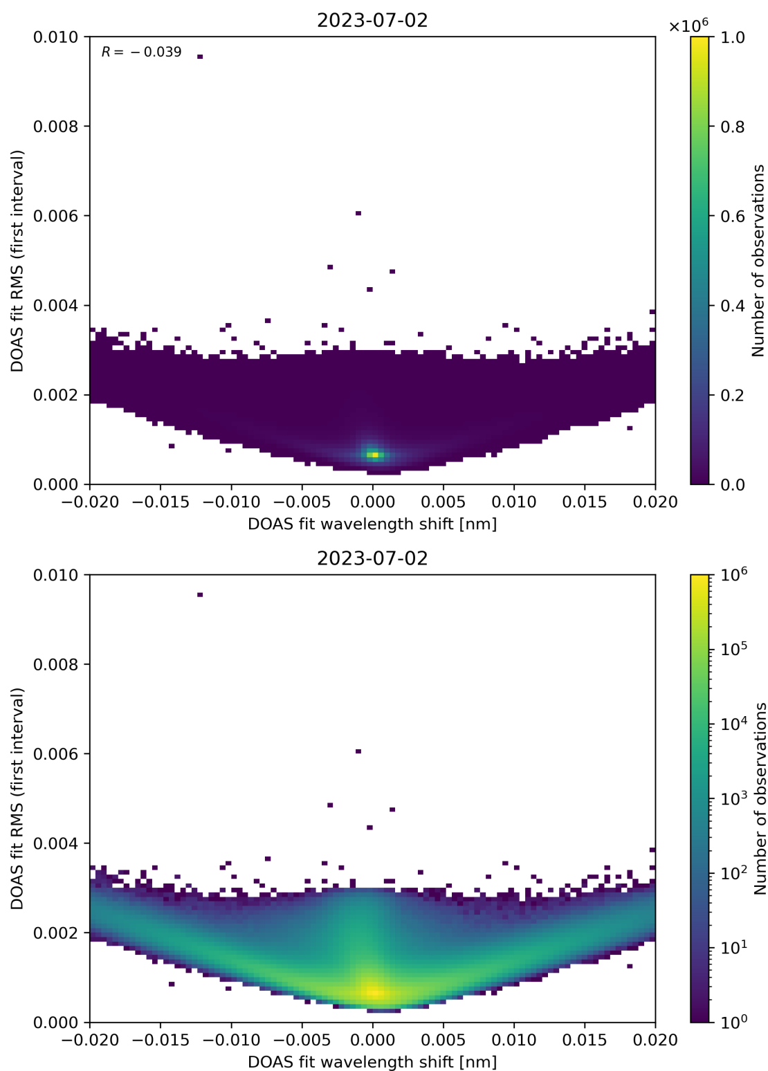
Figure 64: Scatter density plot of “DOAS fit wavelength shift” against “DOAS fit RMS (first interval)” for 2023-07-01 to 2023-07-03.
