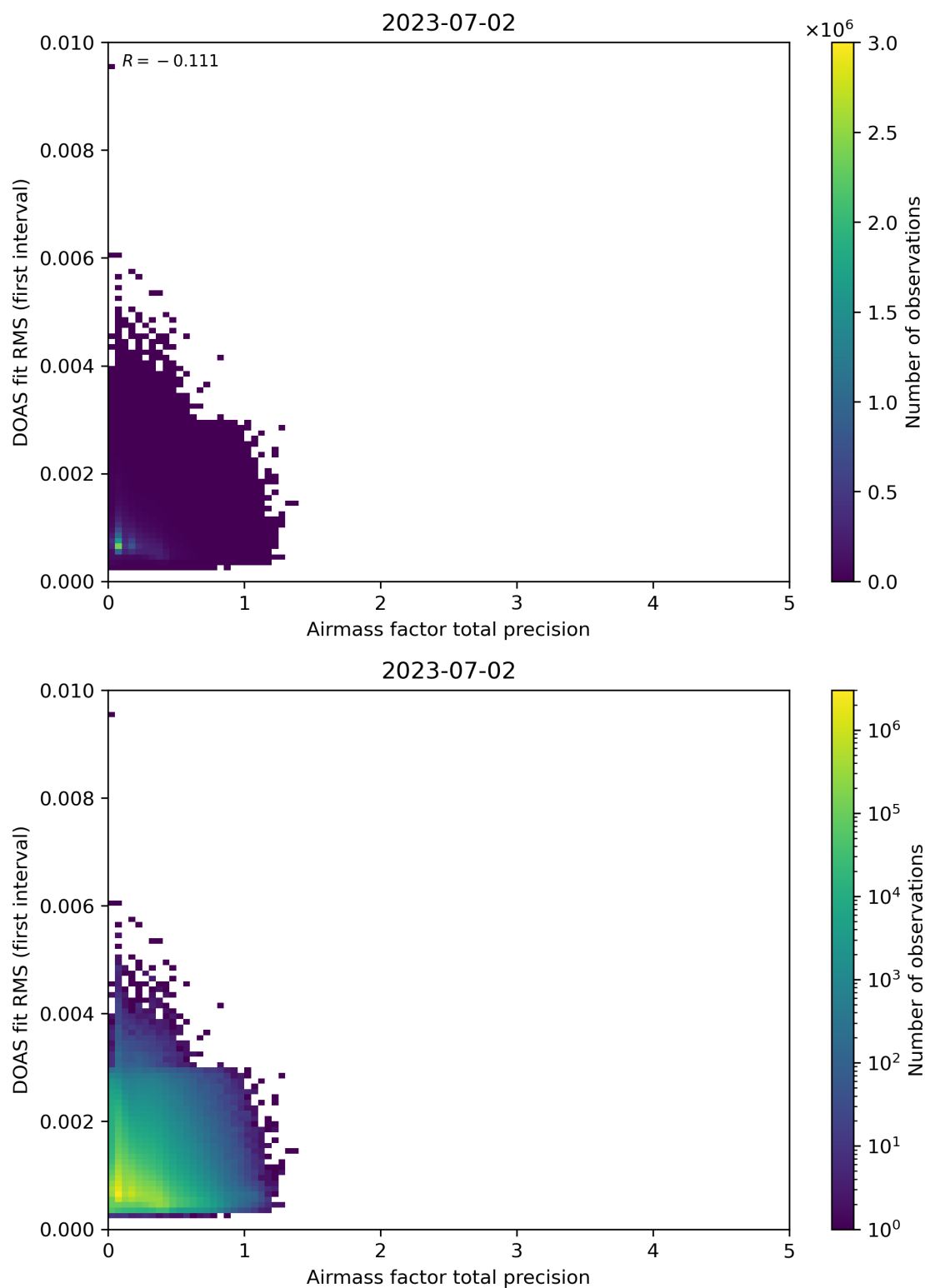
Figure 105: Scatter density plot of “Airmass factor total precision” against “DOAS fit RMS (first interval)” for 2023-07-01 to 2023-07-03.
