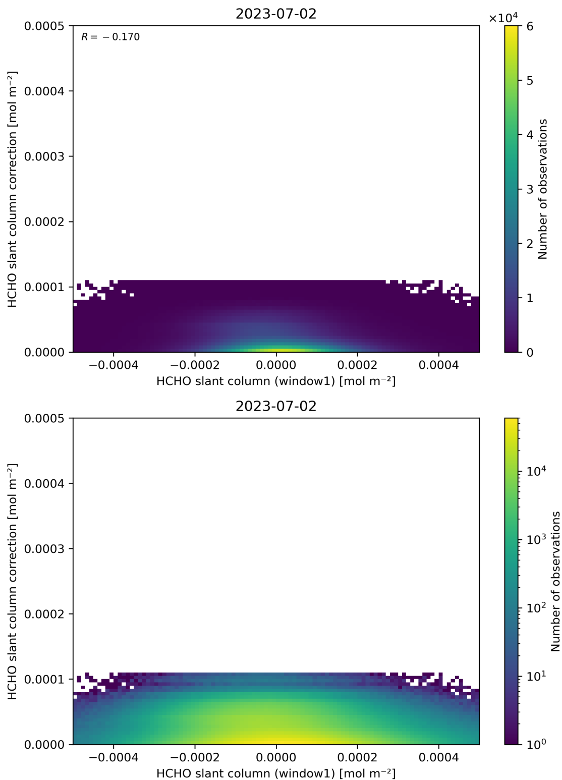
Figure 83: Scatter density plot of “HCHO slant column (window1)” against “HCHO slant column correction” for 2023-07-01 to 2023-07-03.
