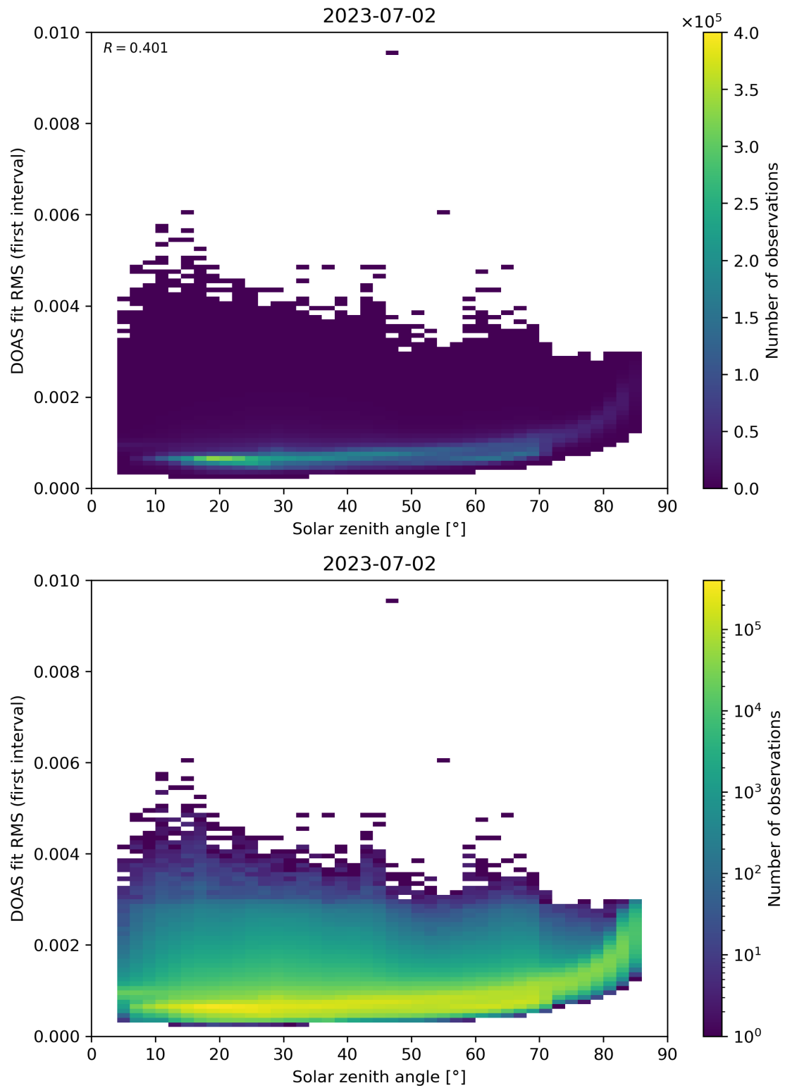
Figure 167: Scatter density plot of “Solar zenith angle” against “DOAS fit RMS (first interval)” for 2023-07-01 to 2023-07-03.
