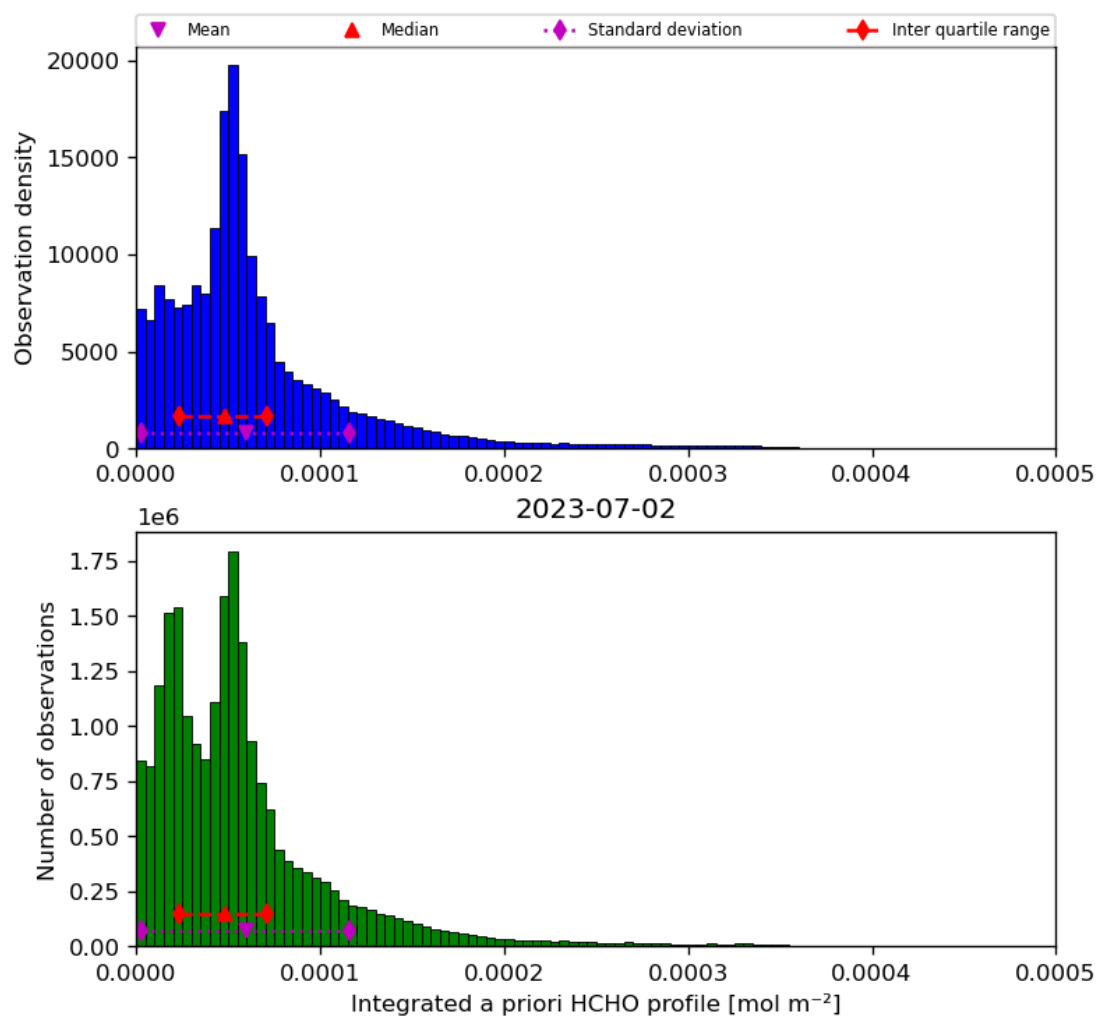
Figure 43: Histogram of “Integrated a priori HCHO profile” for 2023-07-01 to 2023-07-03
