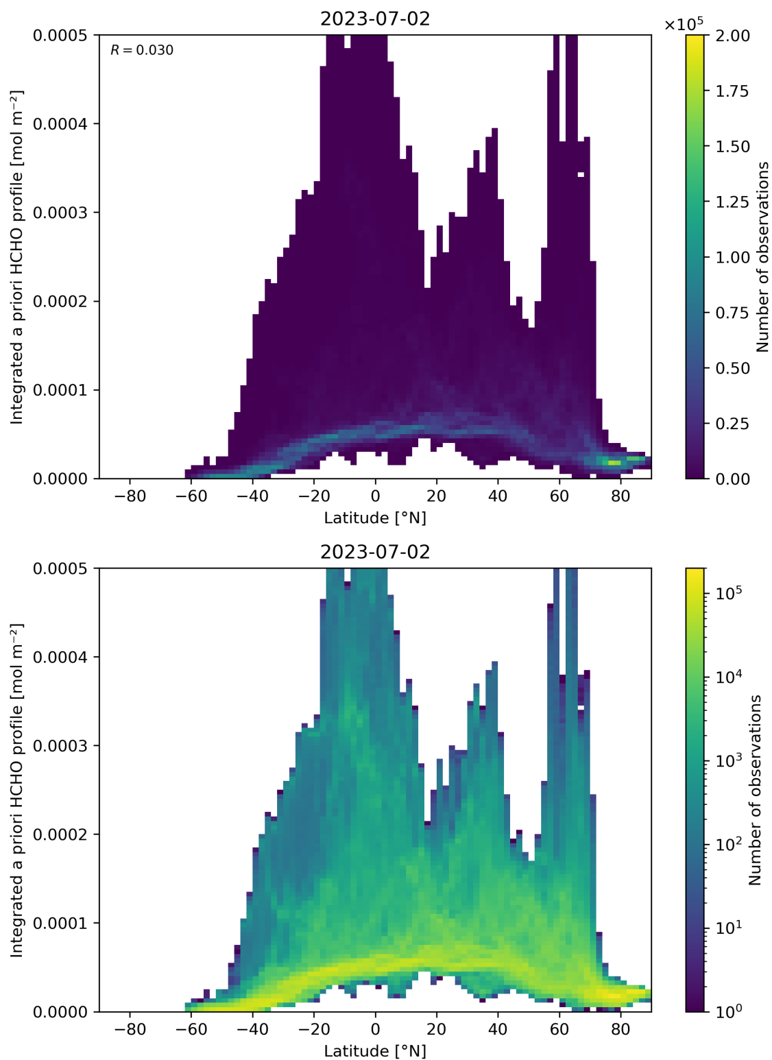
Figure 166: Scatter density plot of “Latitude” against “Integrated a priori HCHO profile” for 2023-07-01 to 2023-07-03.
