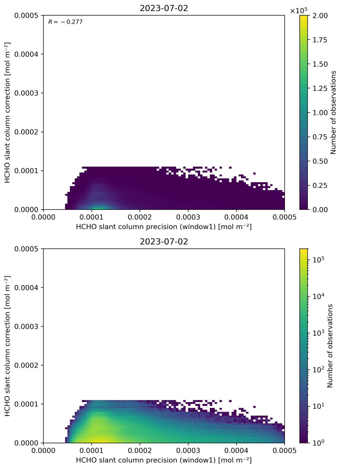
Figure 93: Scatter density plot of “HCHO slant column precision (window1)” against “HCHO slant column correction” for 2023-07-01 to 2023-07-03.
