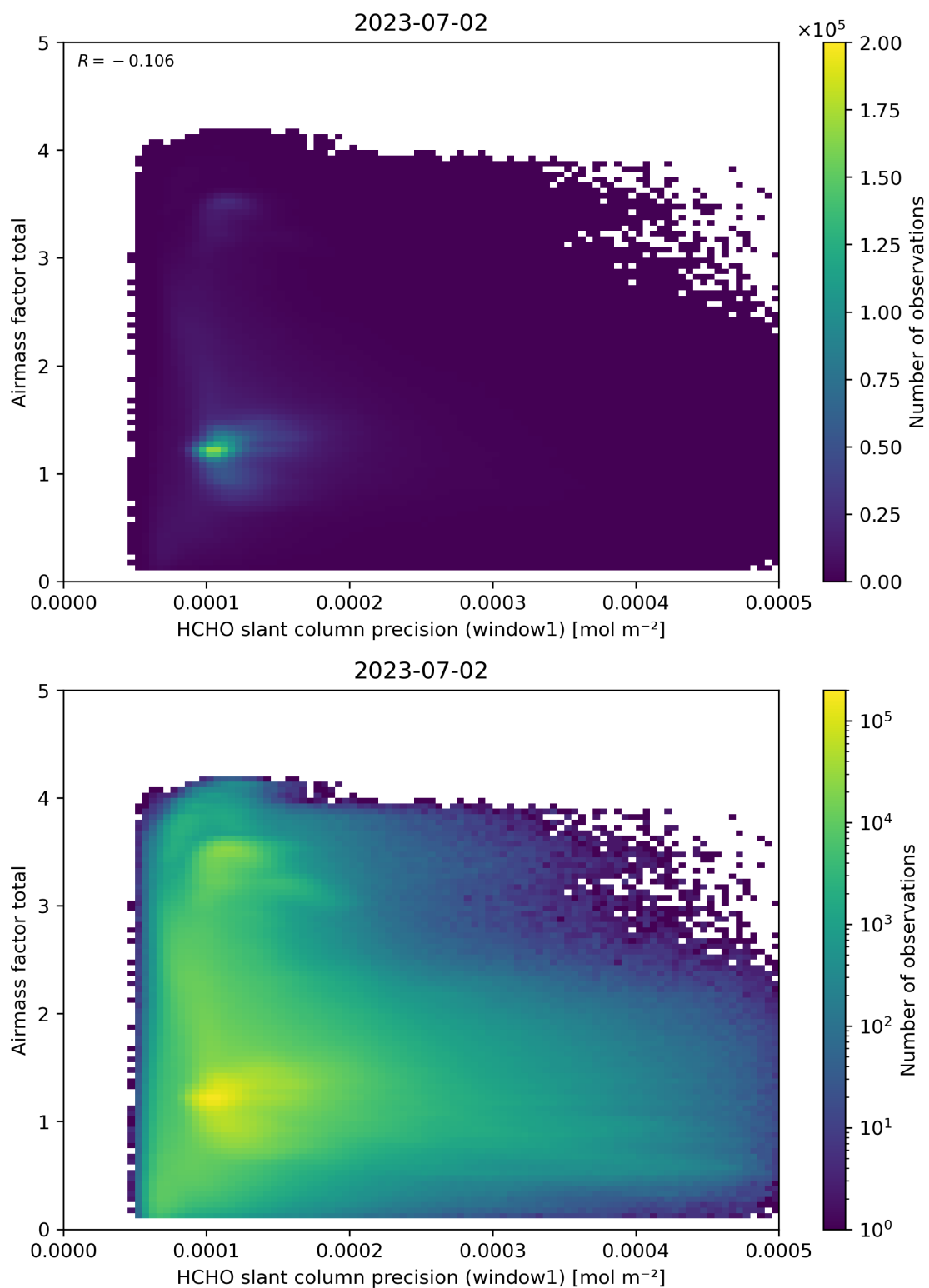
Figure 94: Scatter density plot of “HCHO slant column precision (window1)” against “Airmass factor total” for 2023-07-01 to 2023-07-03.
