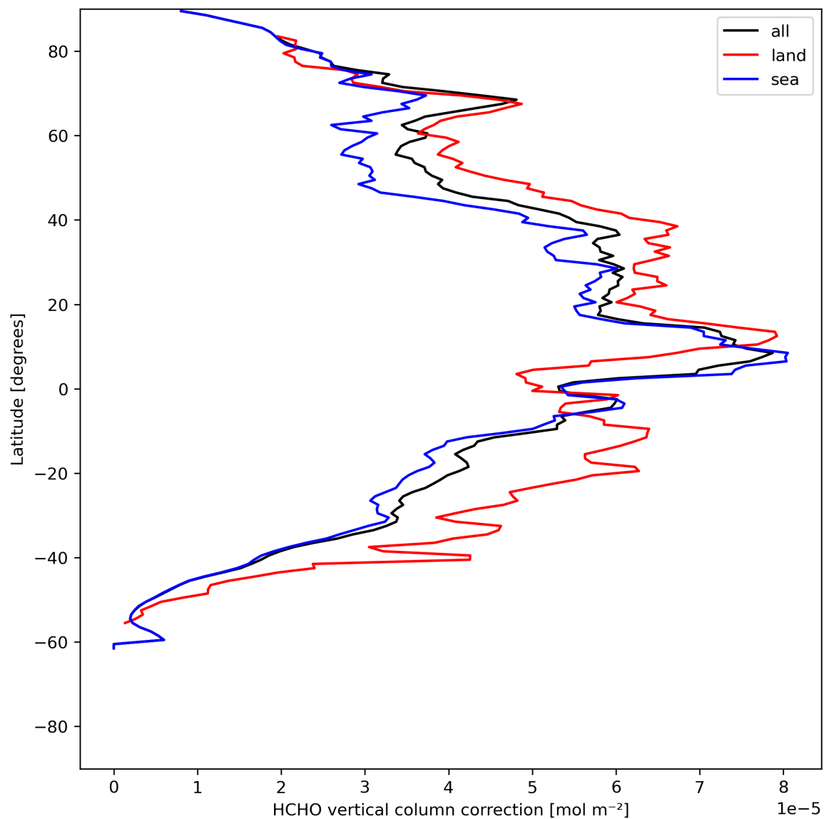
Figure 23: Zonal average of “HCHO vertical column correction” for 2023-07-01 to 2023-07-03.
