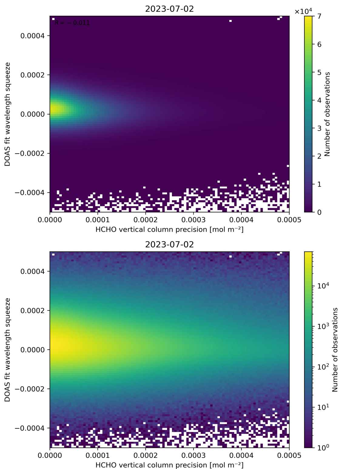
Figure 138: Scatter density plot of “HCHO vertical column precision” against “DOAS fit wavelength squeeze” for 2023-07-01 to 2023-07-03.
