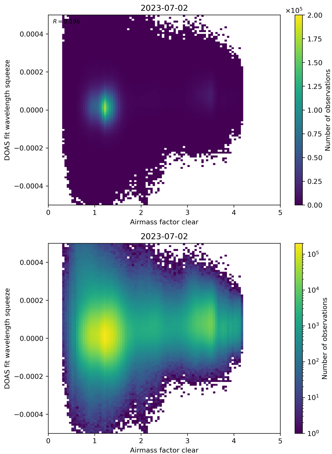
Figure 73: Scatter density plot of “Airmass factor clear” against “DOAS fit wavelength squeeze” for 2023-07-01 to 2023-07-03.
