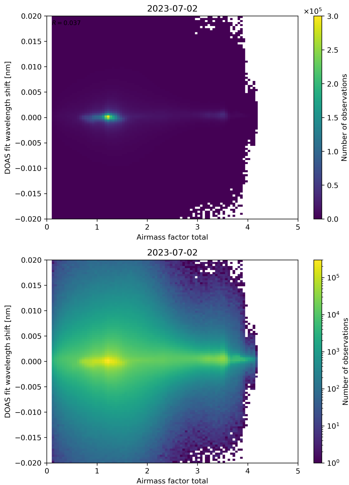
Figure 98: Scatter density plot of “Airmass factor total” against “DOAS fit wavelength shift” for 2023-07-01 to 2023-07-03.
