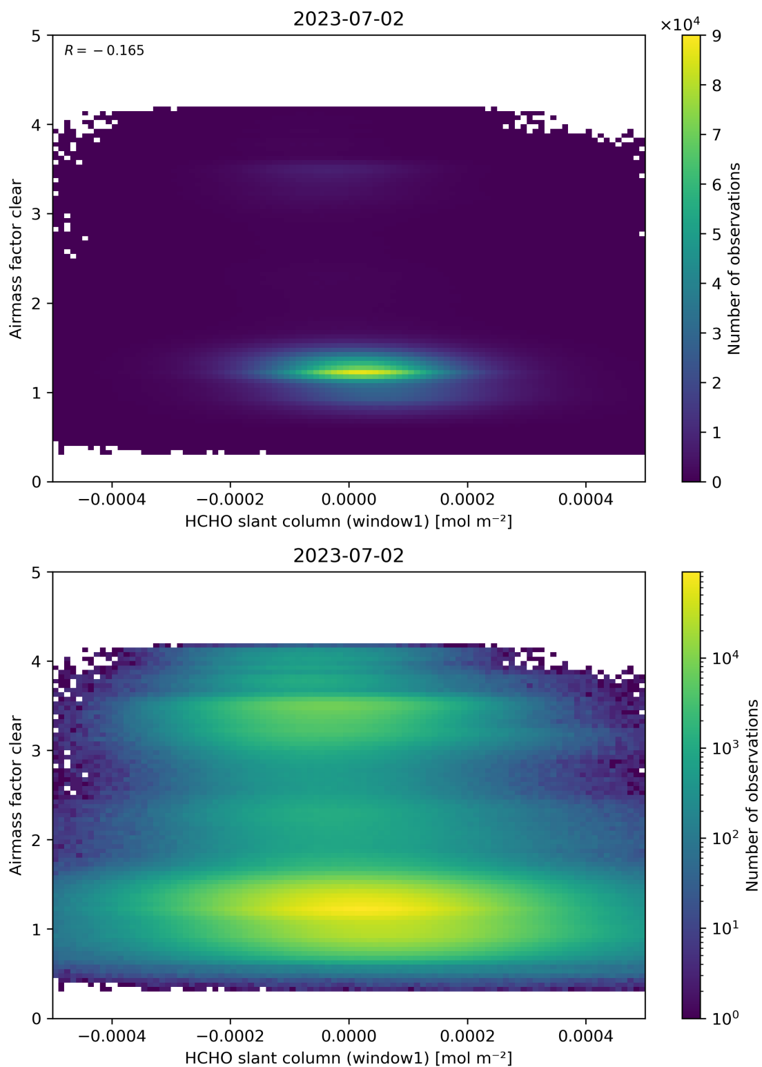
Figure 81: Scatter density plot of “HCHO slant column (window1)” against “Airmass factor clear” for 2023-07-01 to 2023-07-03.
