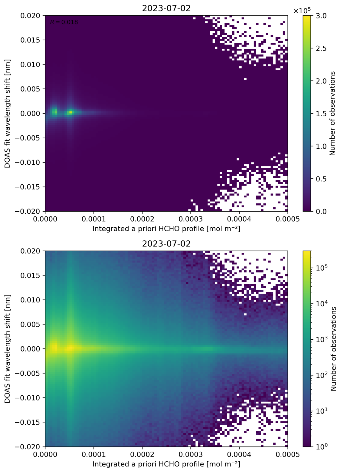
Figure 149: Scatter density plot of “Integrated a priori HCHO profile” against “DOAS fit wavelength shift” for 2023-07-01 to 2023-07-03.
