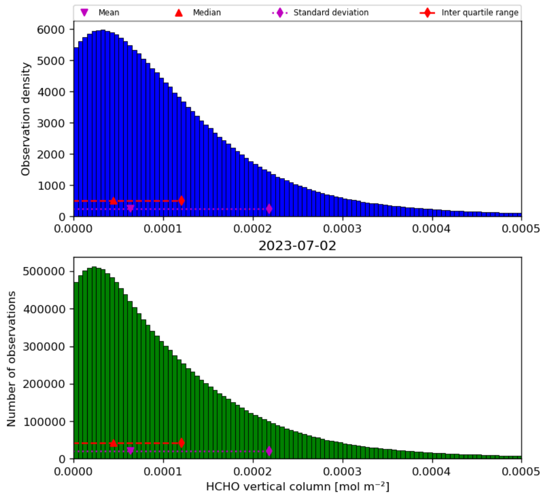
Figure 35: Histogram of “HCHO vertical column” for 2023-07-01 to 2023-07-03
