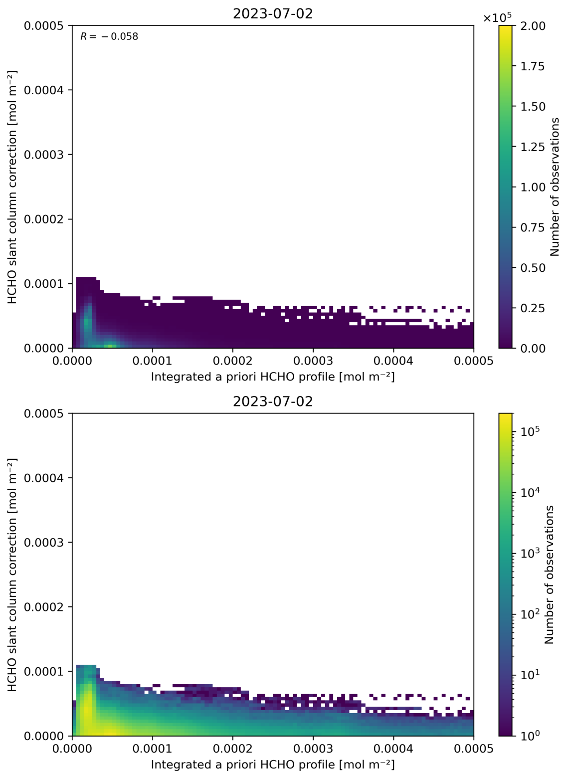
Figure 152: Scatter density plot of “Integrated a priori HCHO profile” against “HCHO slant column correction” for 2023-07-01 to 2023-07-03.
