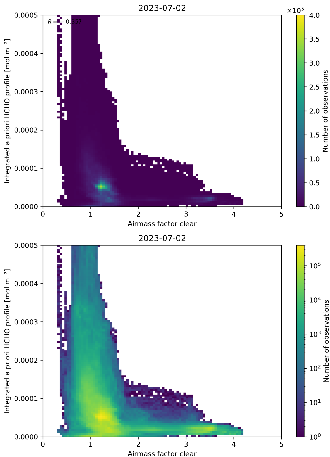
Figure 76: Scatter density plot of “Airmass factor clear” against “Integrated a priori HCHO profile” for 2023-07-01 to 2023-07-03.
