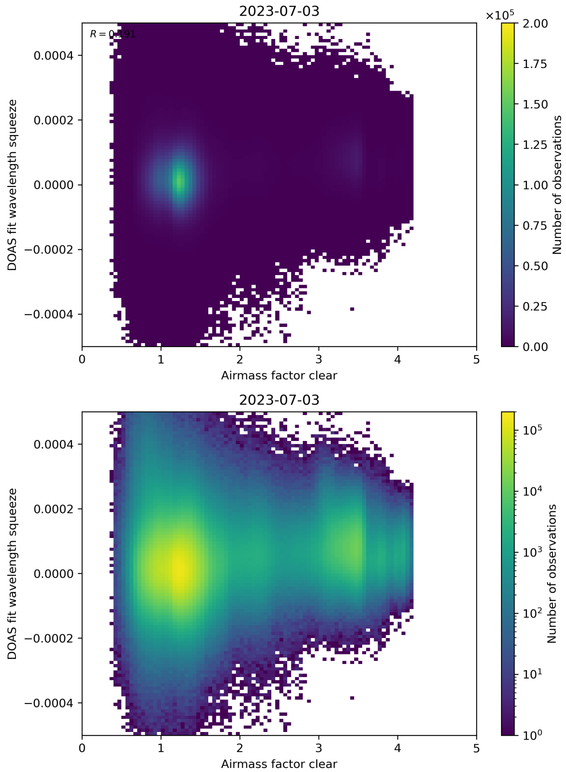
Figure 73: Scatter density plot of “Airmass factor clear” against “DOAS fit wavelength squeeze” for 2023-07-03 to 2023-07-04.
