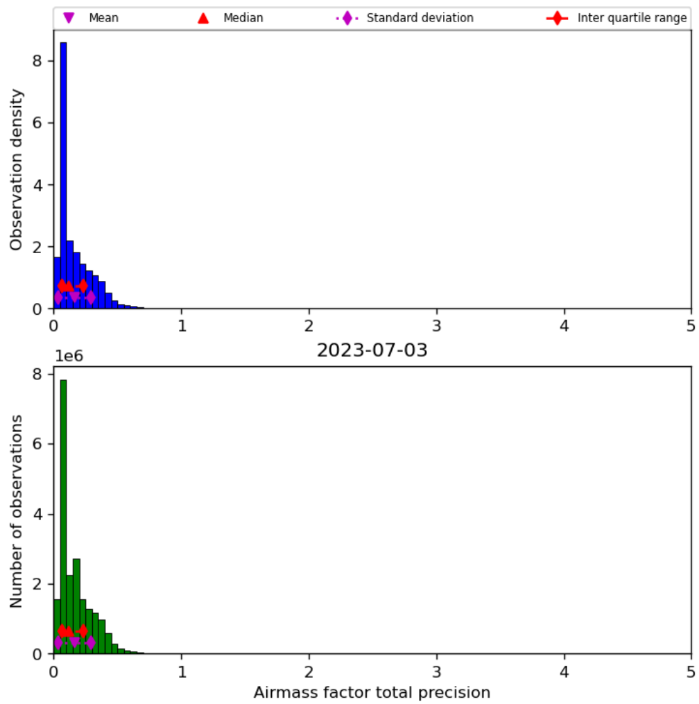
Figure 41: Histogram of “Airmass factor total precision” for 2023-07-03 to 2023-07-04
