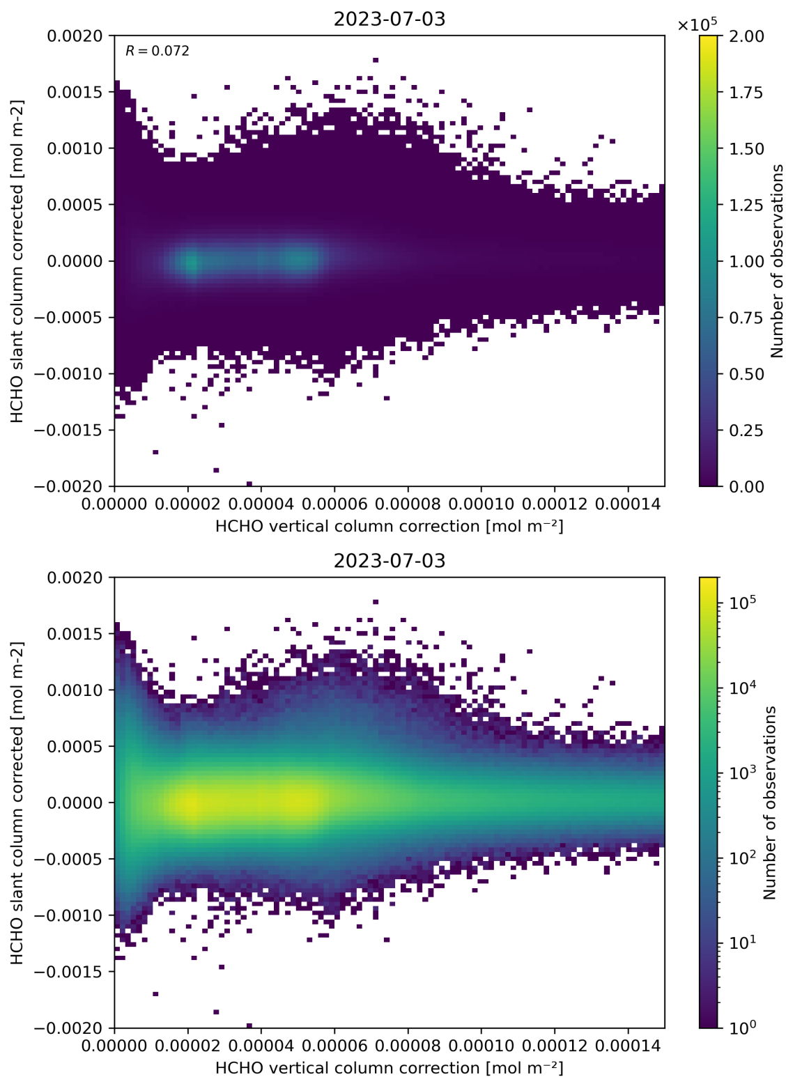
Figure 116: Scatter density plot of “HCHO vertical column correction” against “HCHO slant column corrected” for 2023-07-03 to 2023-07-04.
