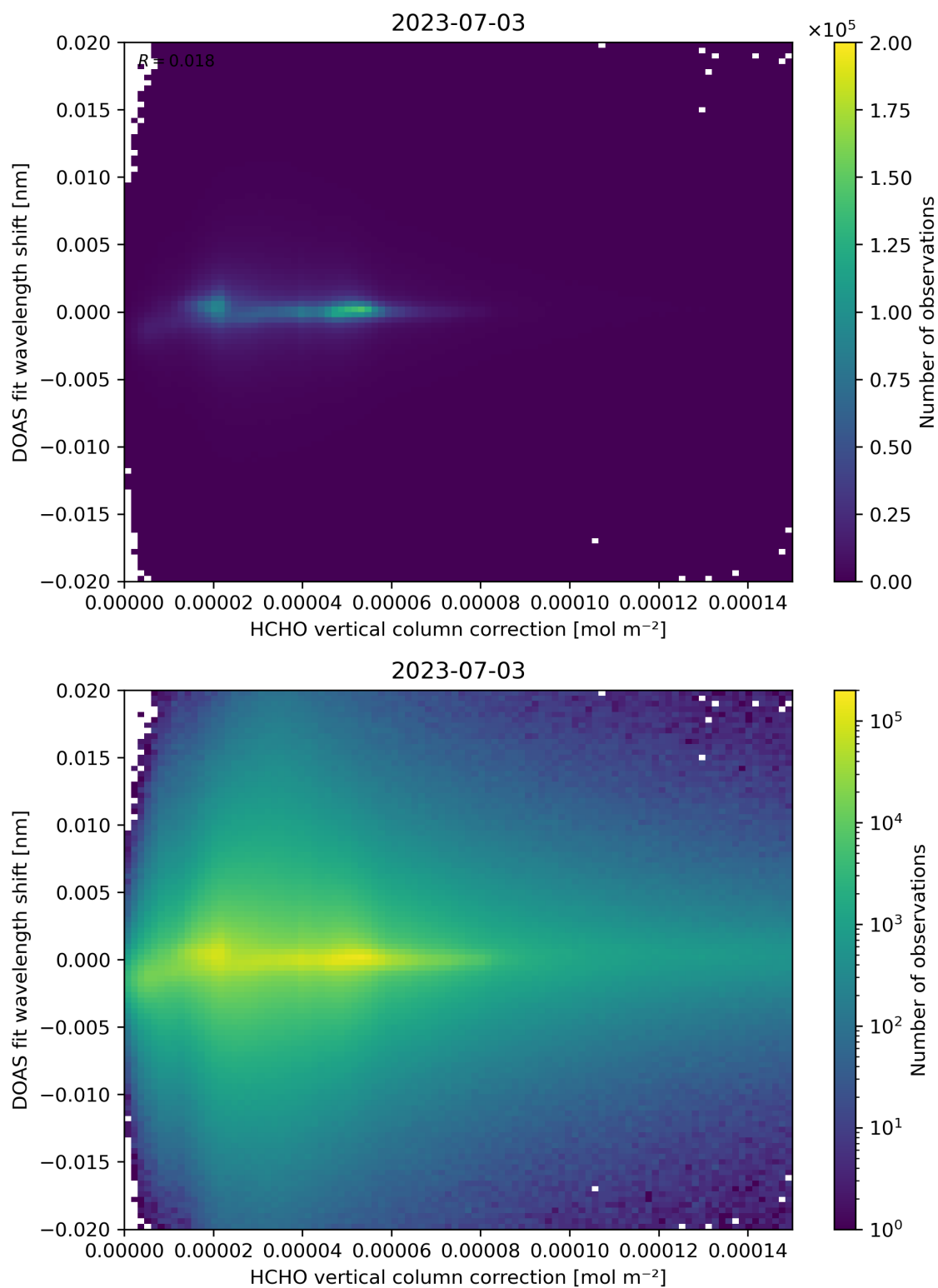
Figure 113: Scatter density plot of “HCHO vertical column correction” against “DOAS fit wavelength shift” for 2023-07-03 to 2023-07-04.
