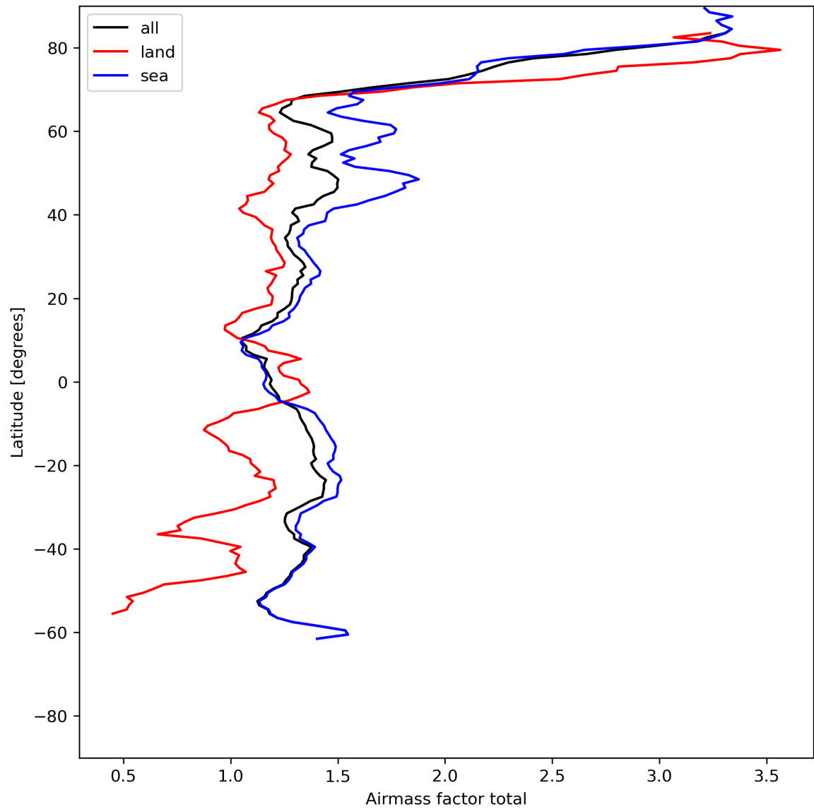
Figure 26: Zonal average of “Airmass factor total” for 2023-07-03 to 2023-07-04.
