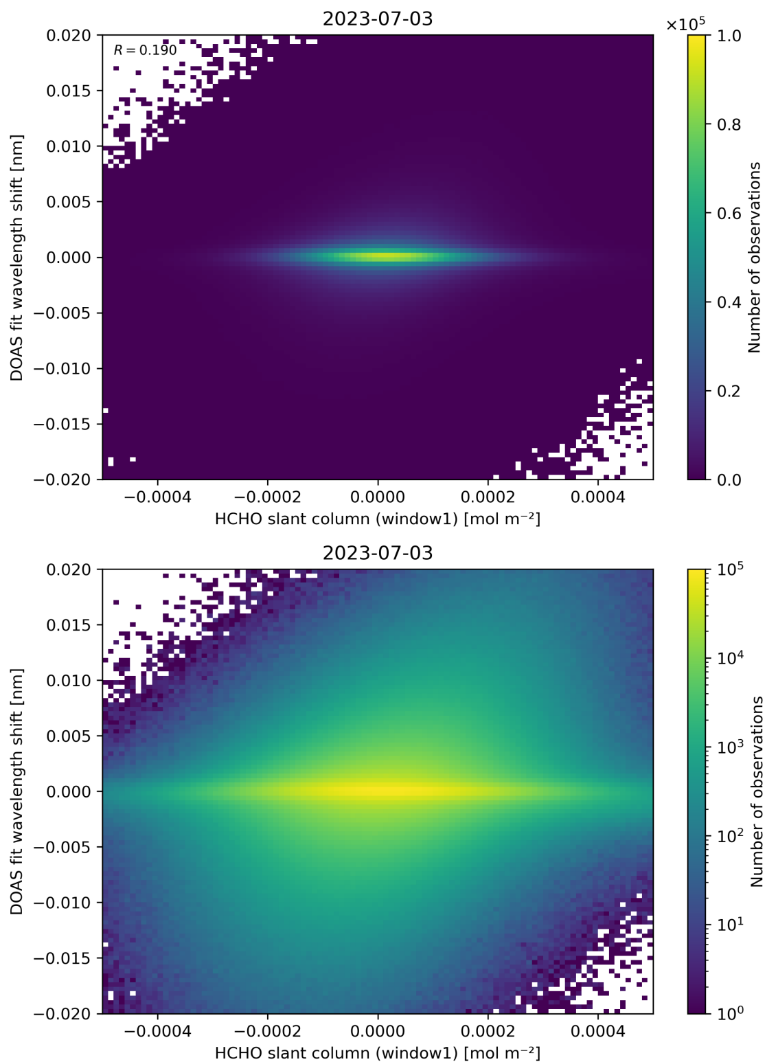
Figure 79: Scatter density plot of “HCHO slant column (window1)” against “DOAS fit wavelength shift” for 2023-07-03 to 2023-07-04.
