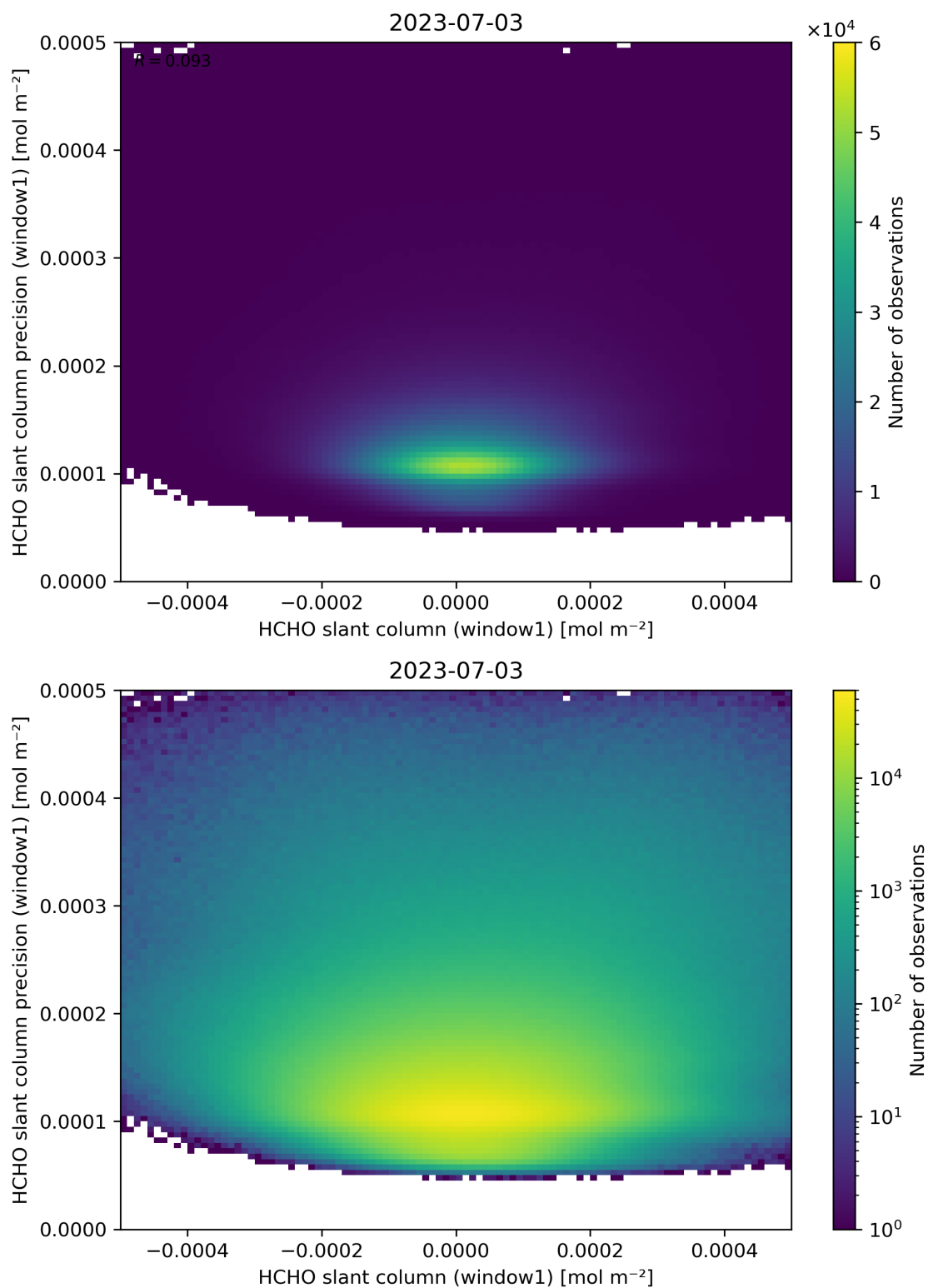
Figure 84: Scatter density plot of “HCHO slant column (window1)” against “HCHO slant column precision (window1)” for 2023-07-03 to 2023-07-04.
