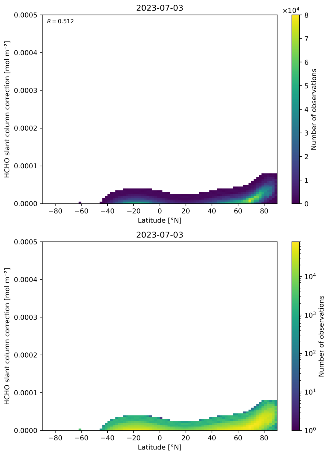
Figure 158: Scatter density plot of “Latitude” against “HCHO slant column correction” for 2023-07-03 to 2023-07-04.
