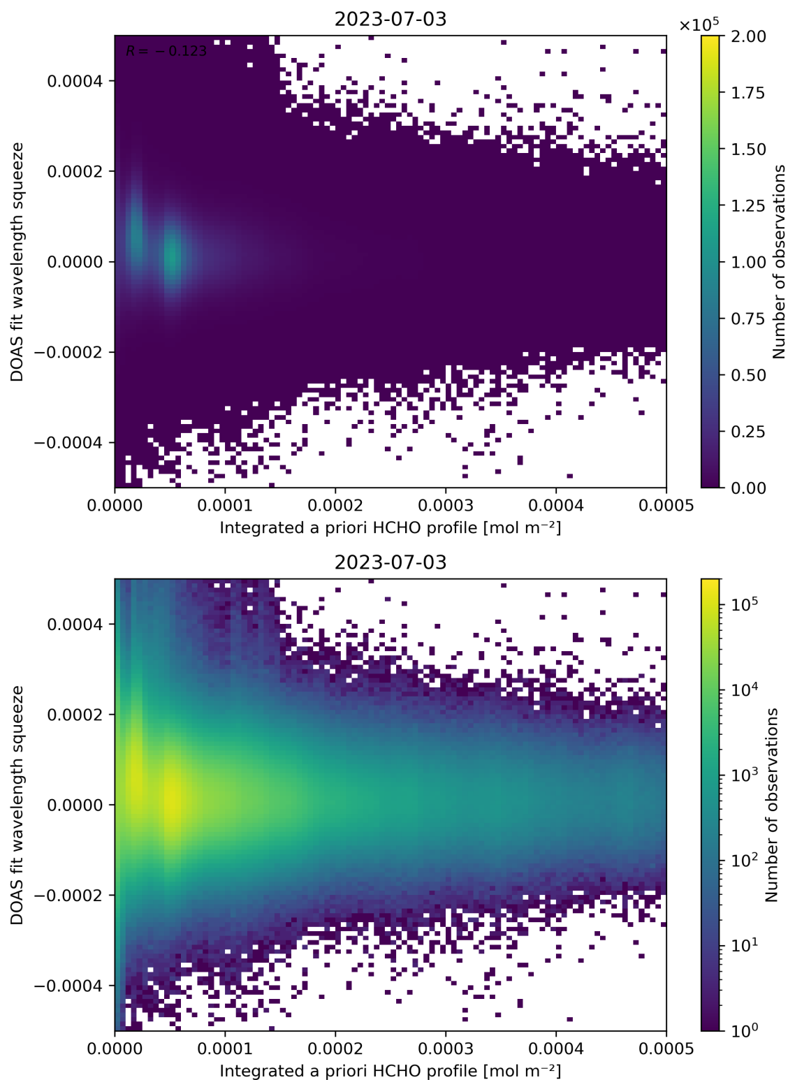
Figure 150: Scatter density plot of “Integrated a priori HCHO profile” against “DOAS fit wavelength squeeze” for 2023-07-03 to 2023-07-04.
