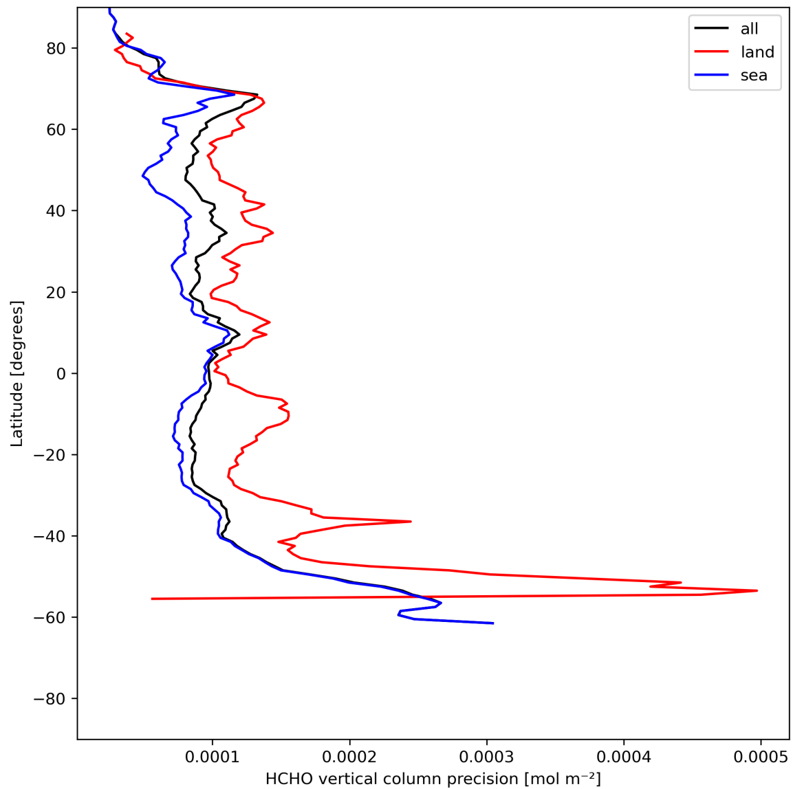
Figure 22: Zonal average of “HCHO vertical column precision” for 2023-07-03 to 2023-07-04.
