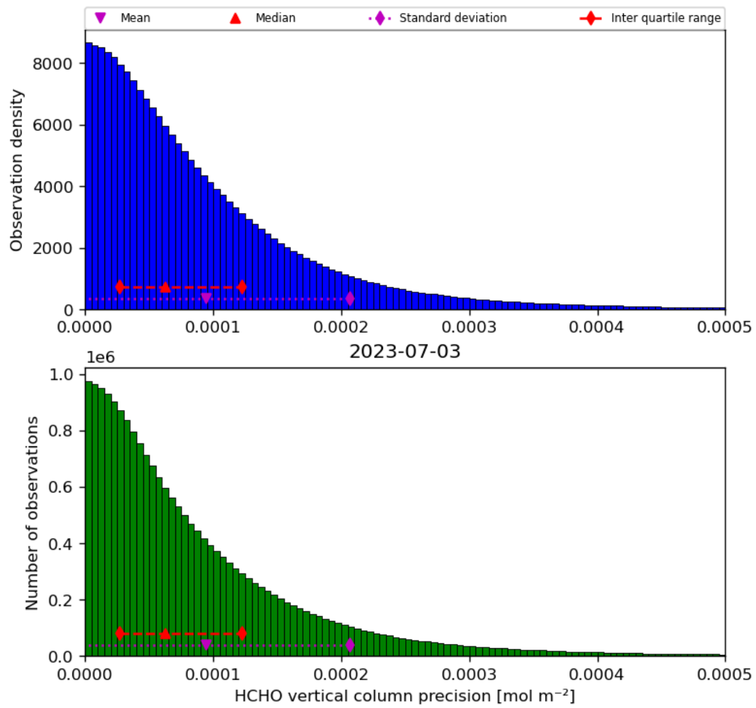
Figure 36: Histogram of “HCHO vertical column precision” for 2023-07-03 to 2023-07-04
