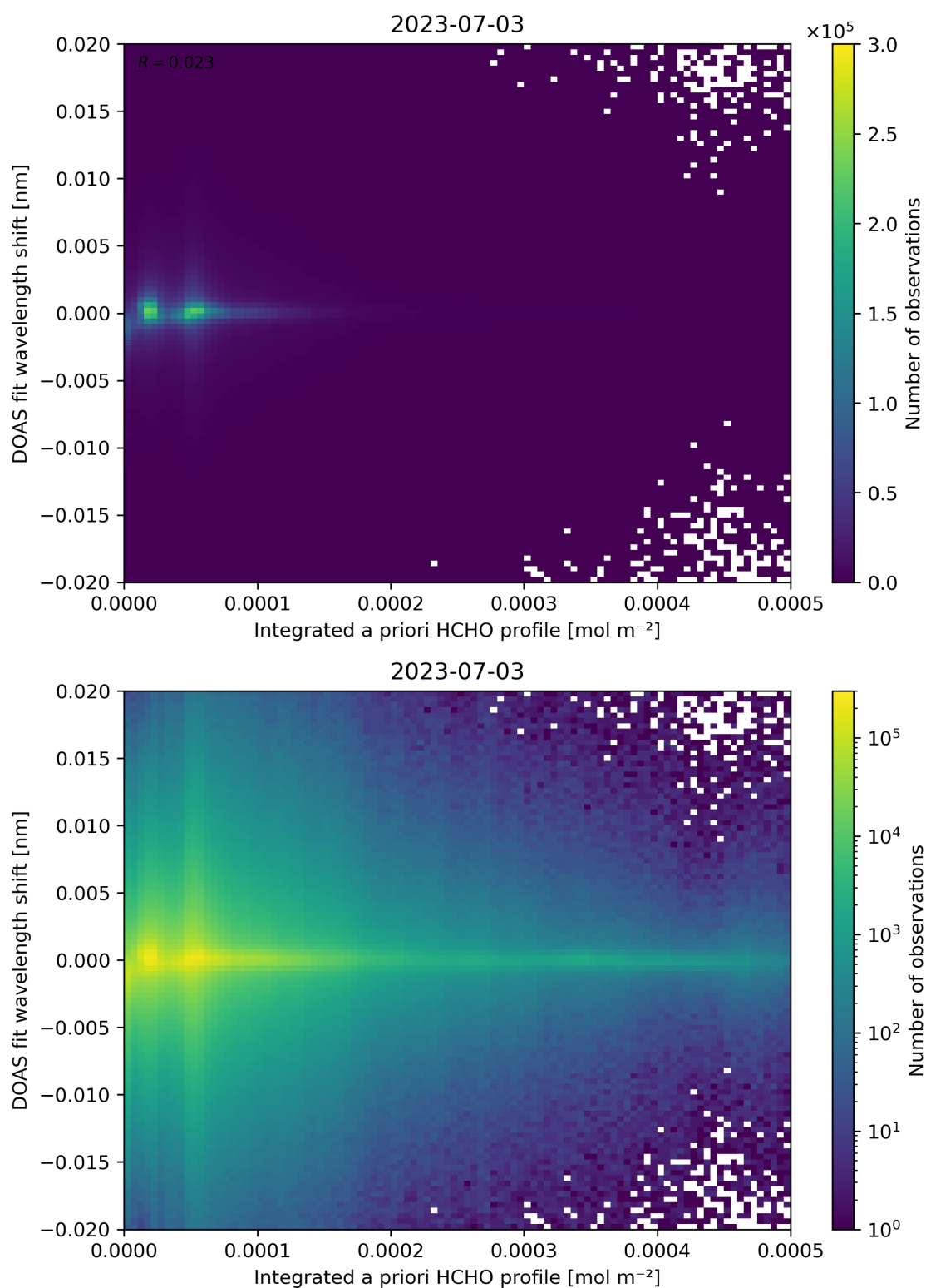
Figure 149: Scatter density plot of “Integrated a priori HCHO profile” against “DOAS fit wavelength shift” for 2023-07-03 to 2023-07-04.
