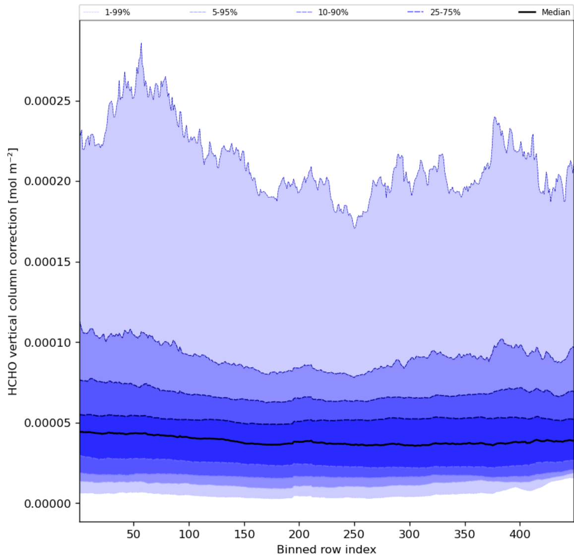
Figure 51: Along track statistics of “HCHO vertical column correction” for 2023-07-03 to 2023-07-04
