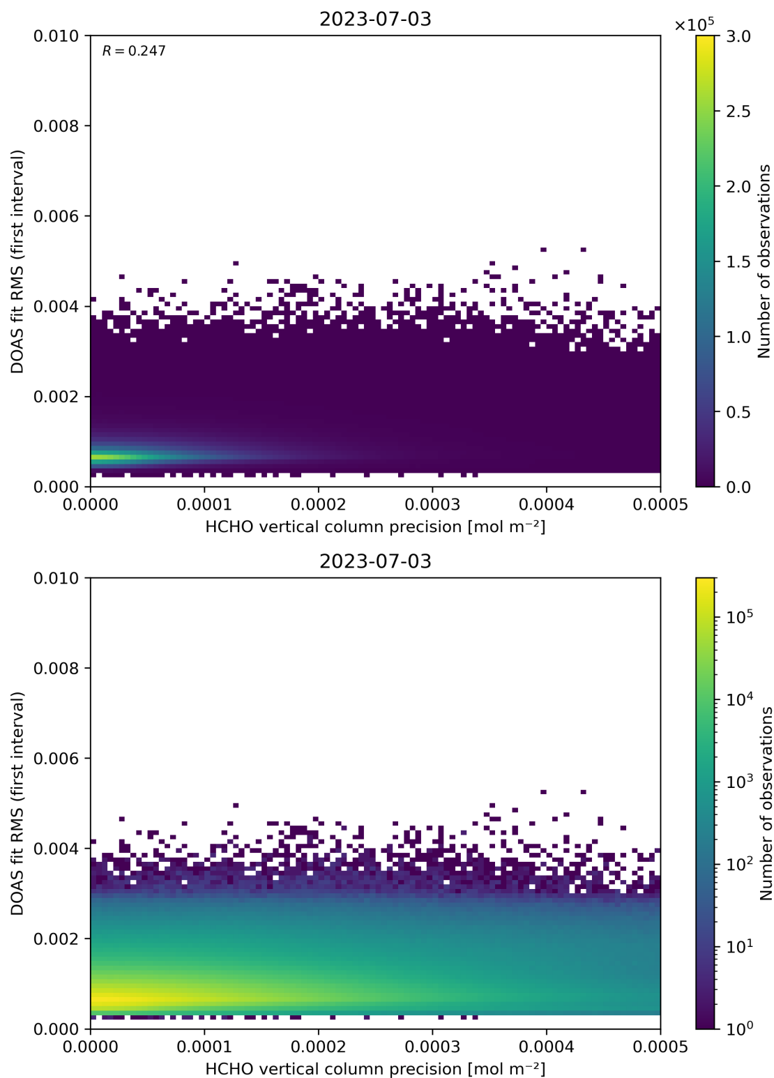
Figure 136: Scatter density plot of “HCHO vertical column precision” against “DOAS fit RMS (first interval)” for 2023-07-03 to 2023-07-04.
