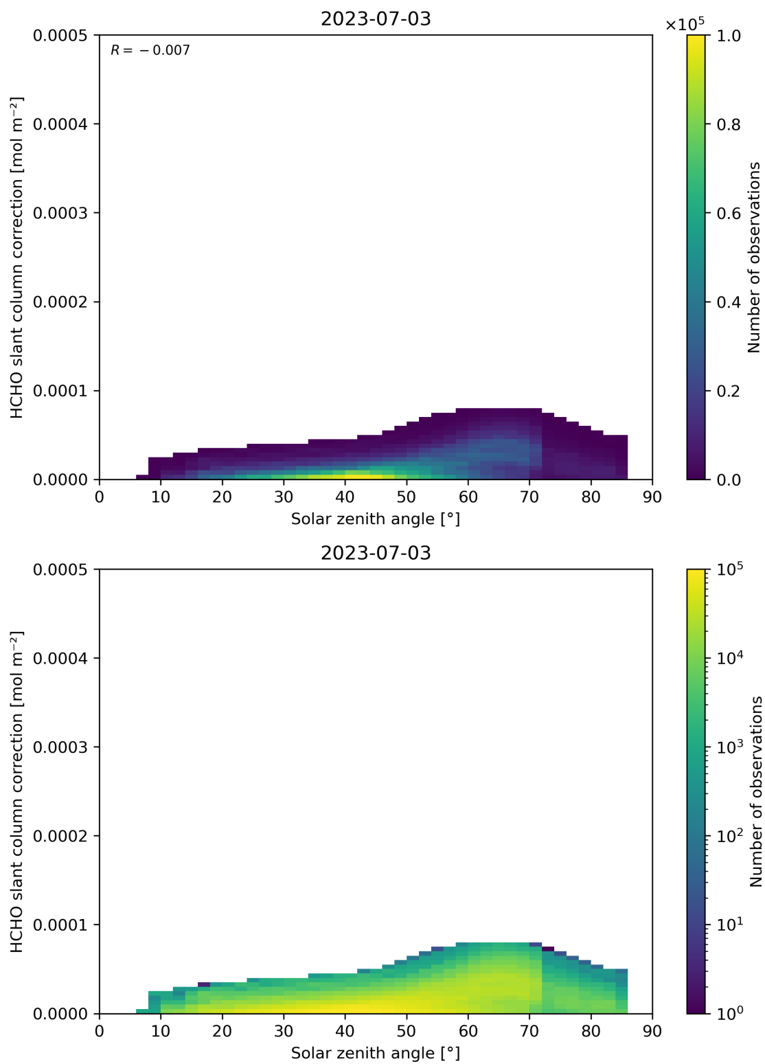
Figure 172: Scatter density plot of “Solar zenith angle” against “HCHO slant column correction” for 2023-07-03 to 2023-07-04.
