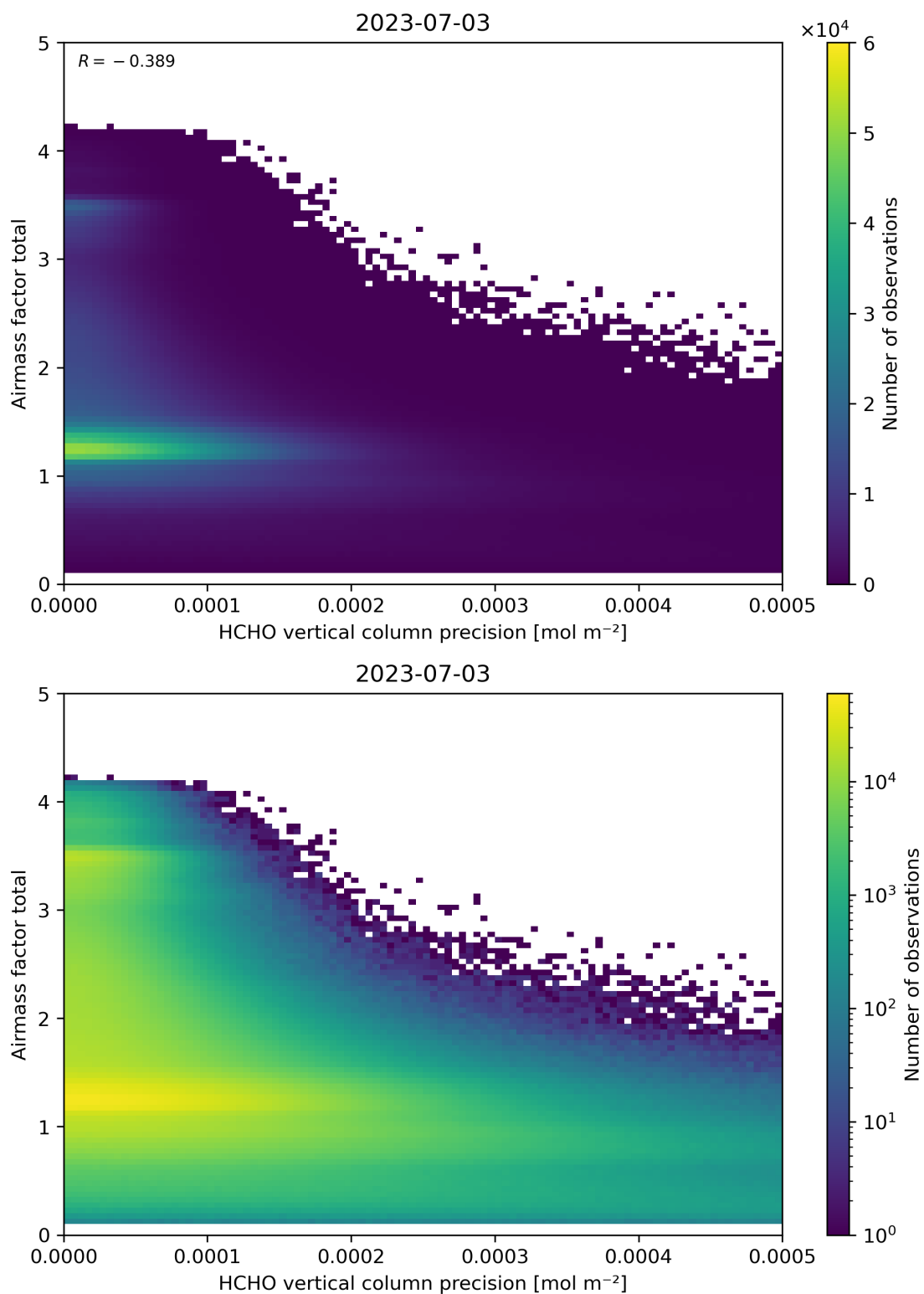
Figure 144: Scatter density plot of “HCHO vertical column precision” against “Airmass factor total” for 2023-07-03 to 2023-07-04.
