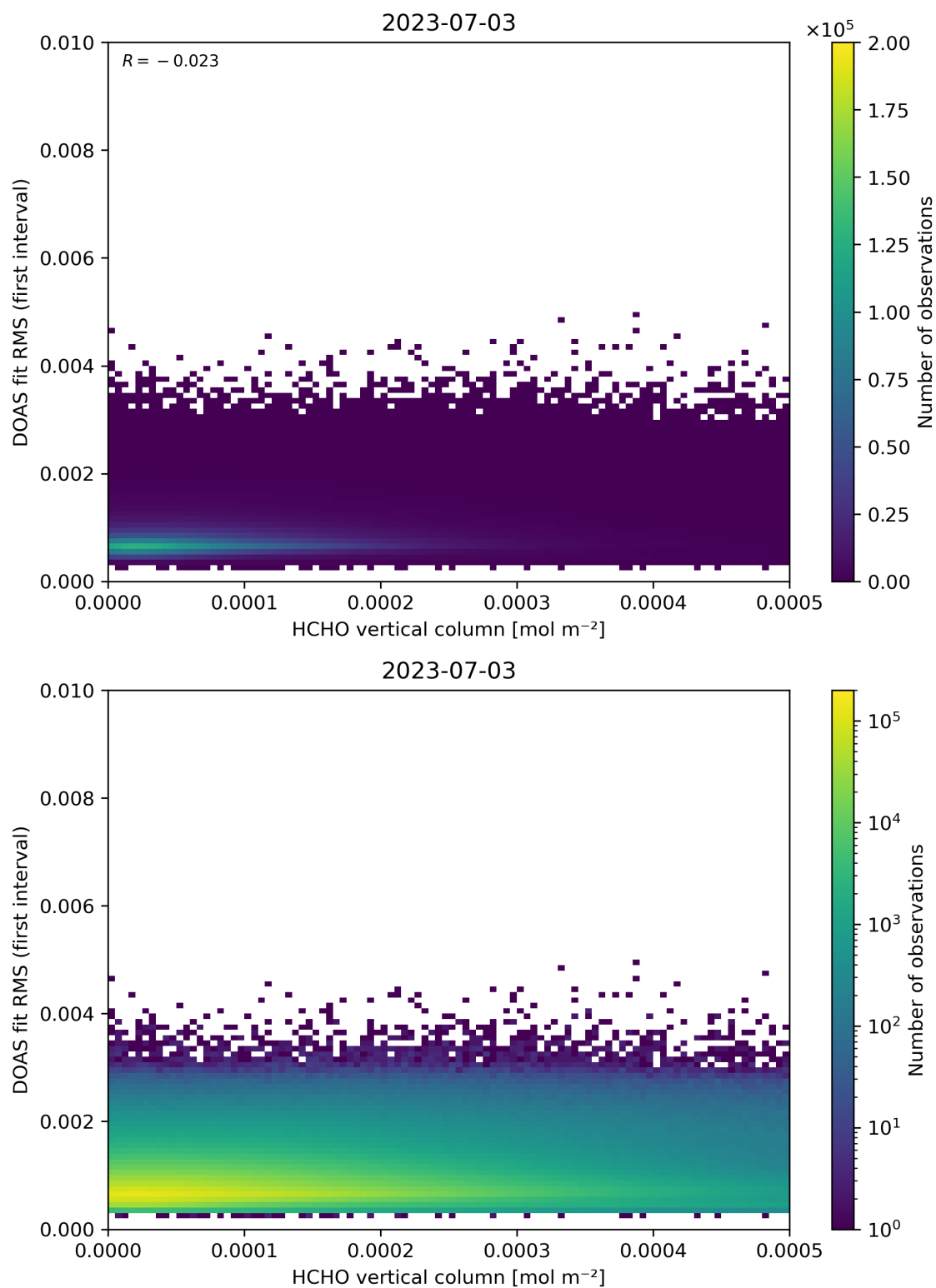
Figure 123: Scatter density plot of “HCHO vertical column” against “DOAS fit RMS (first interval)” for 2023-07-03 to 2023-07-04.
