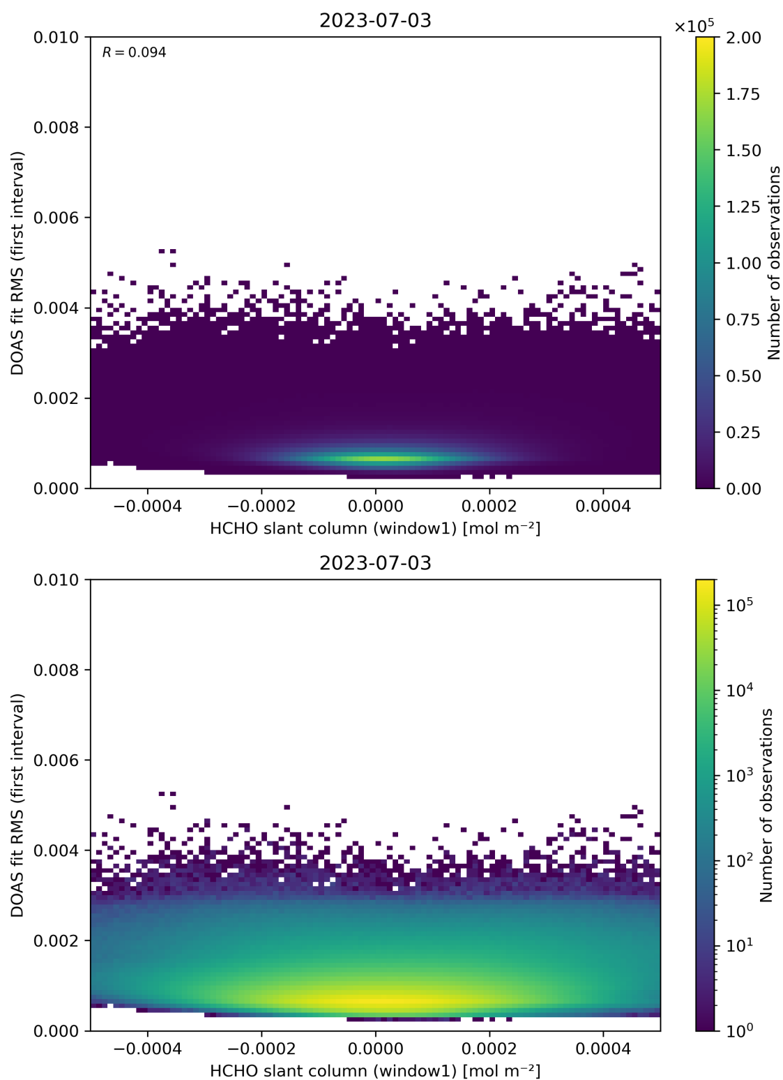
Figure 78: Scatter density plot of “HCHO slant column (window1)” against “DOAS fit RMS (first interval)” for 2023-07-03 to 2023-07-04.
