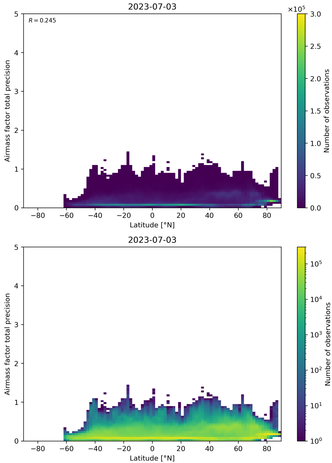
Figure 162: Scatter density plot of “Latitude” against “Airmass factor total precision” for 2023-07-03 to 2023-07-04.
