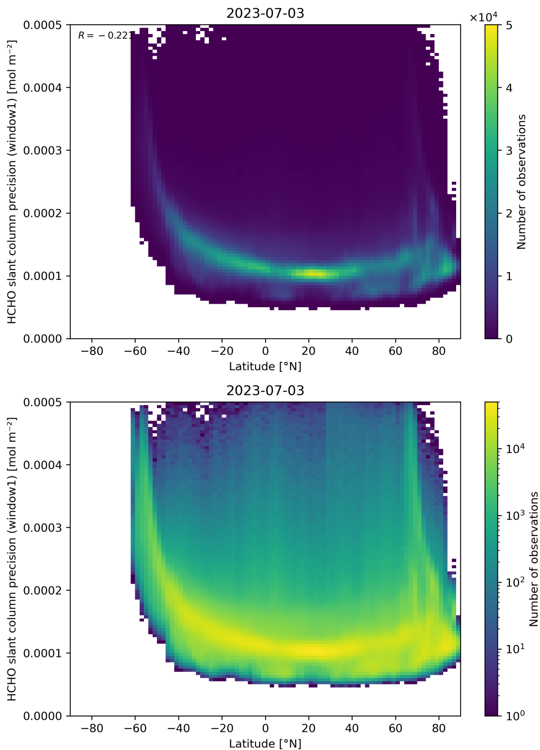
Figure 160: Scatter density plot of “Latitude” against “HCHO slant column precision (window1)” for 2023-07-03 to 2023-07-04.
