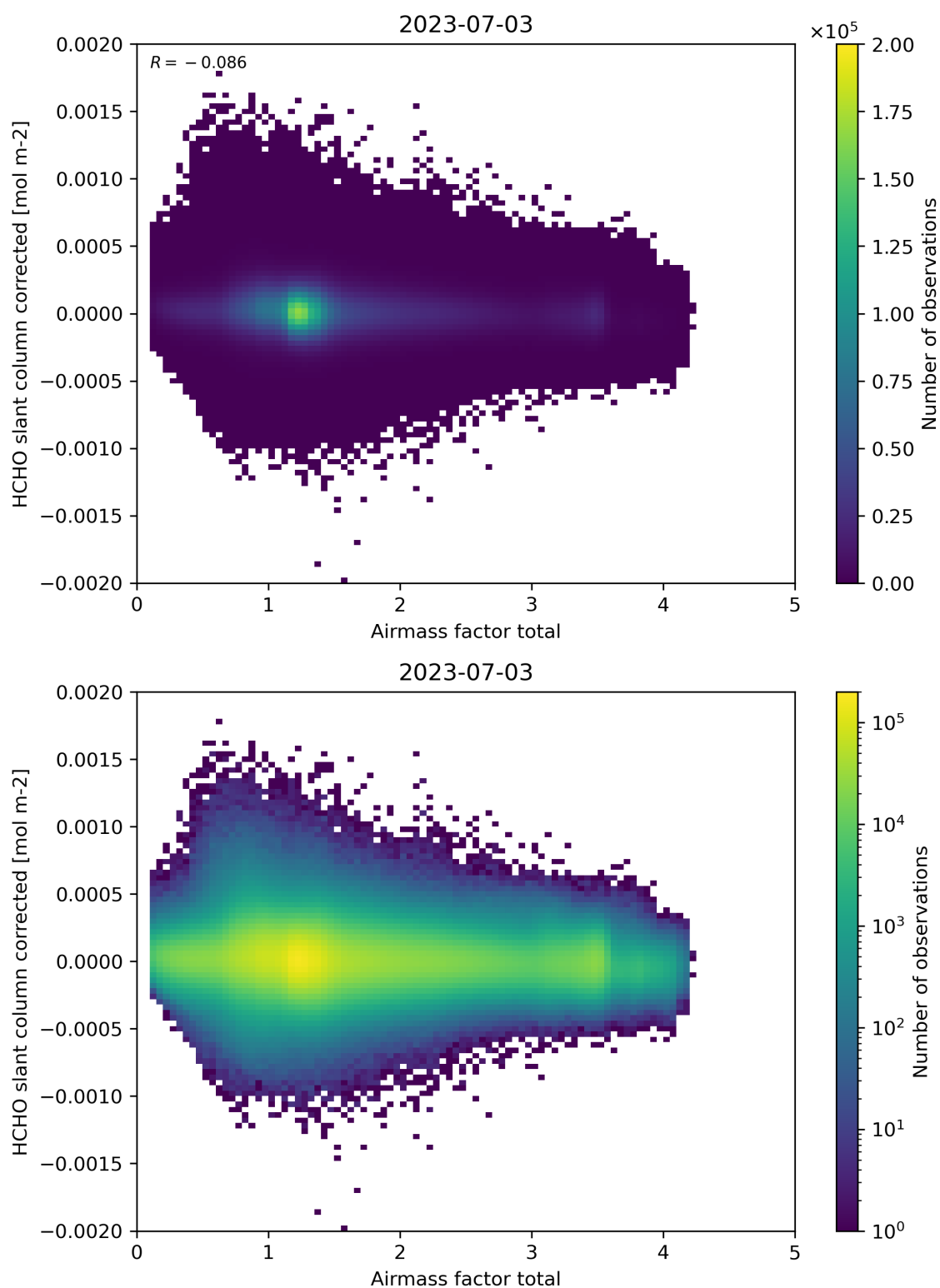
Figure 101: Scatter density plot of “Airmass factor total” against “HCHO slant column corrected” for 2023-07-03 to 2023-07-04.
