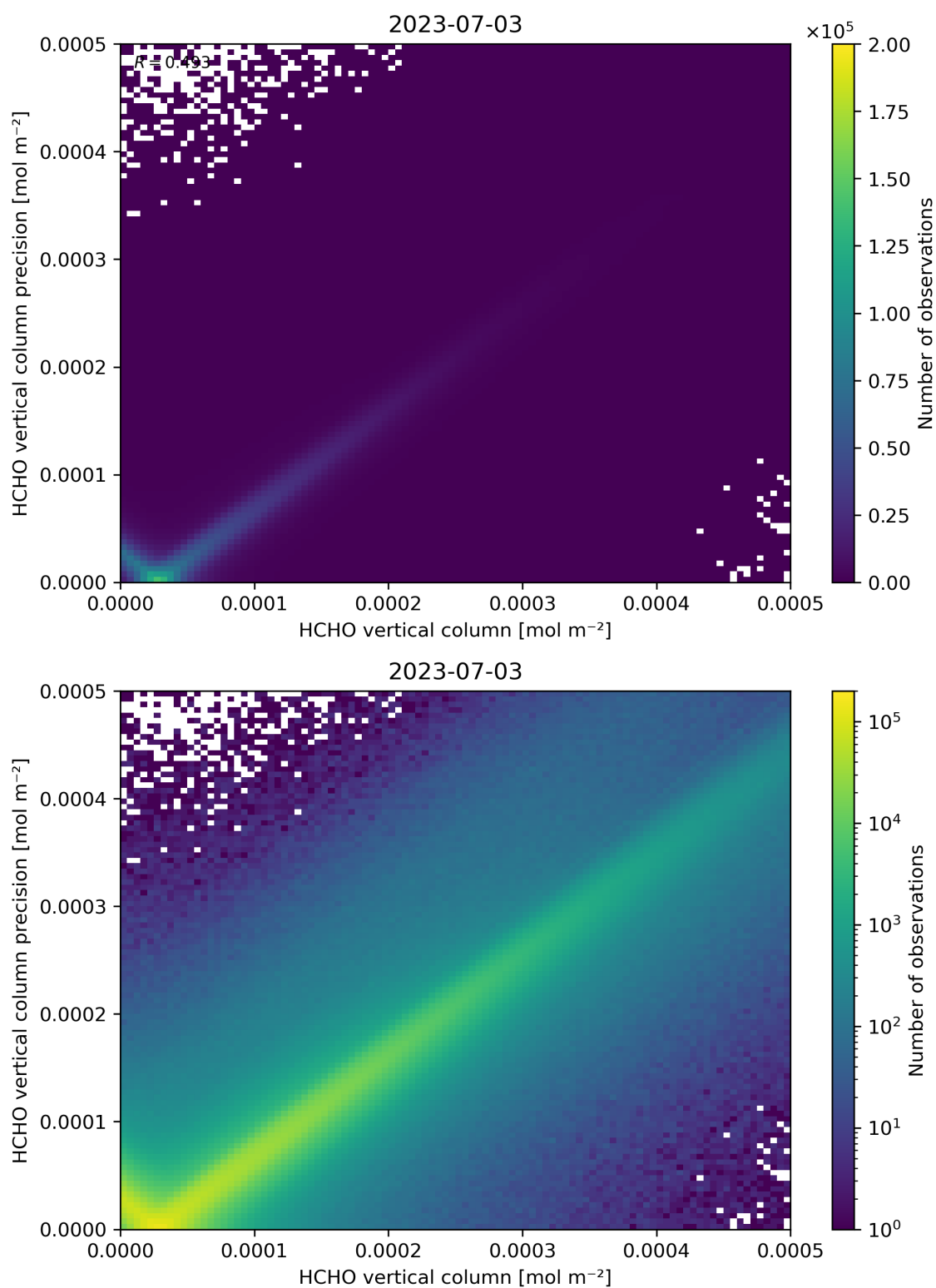
Figure 134: Scatter density plot of “HCHO vertical column” against “HCHO vertical column precision” for 2023-07-03 to 2023-07-04.
