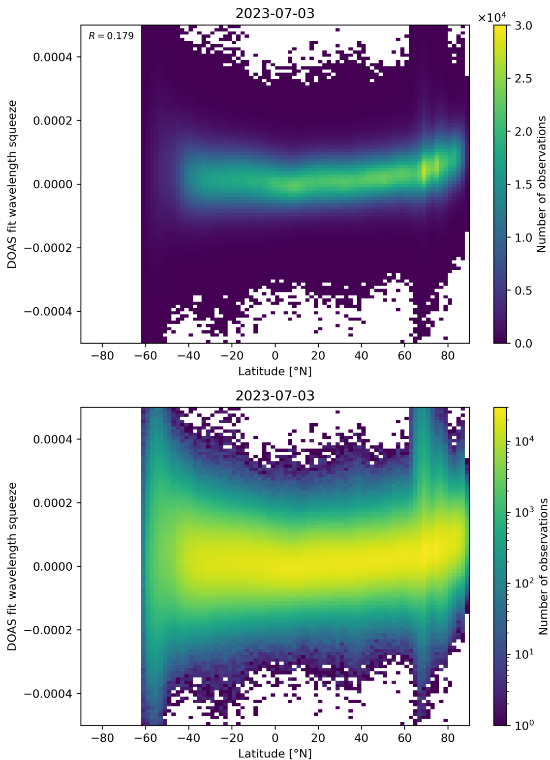
Figure 155: Scatter density plot of “Latitude” against “DOAS fit wavelength squeeze” for 2023-07-03 to 2023-07-04.
