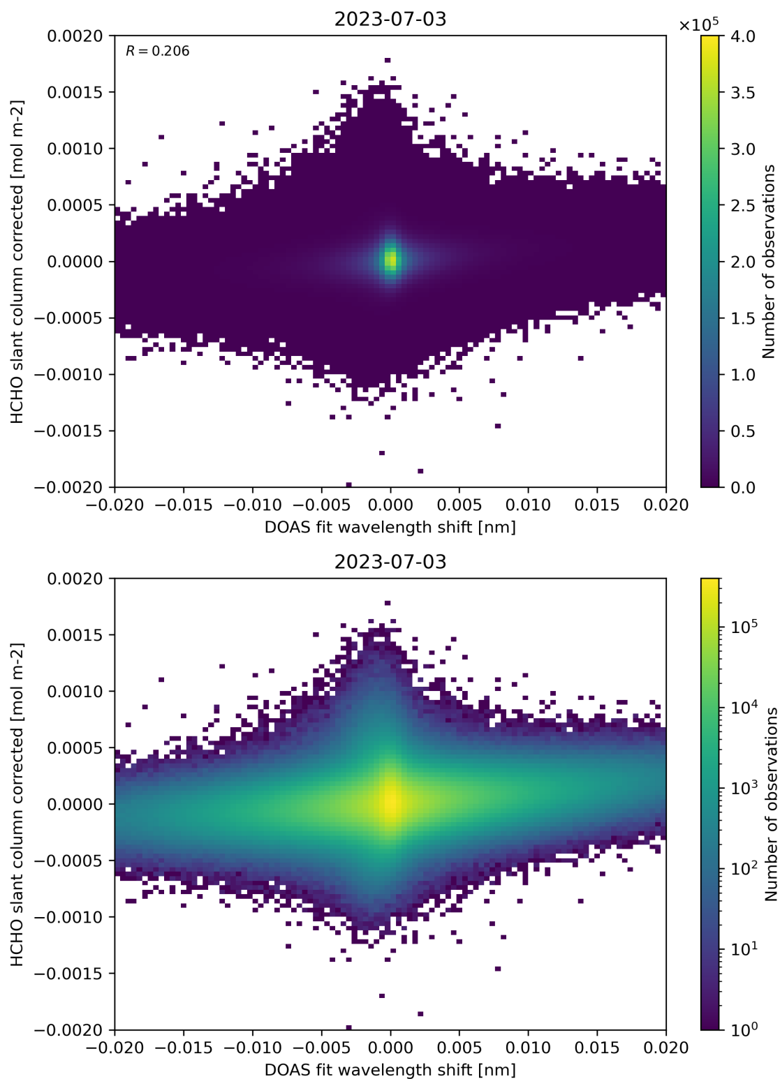
Figure 66: Scatter density plot of “DOAS fit wavelength shift” against “HCHO slant column corrected” for 2023-07-03 to 2023-07-04.
