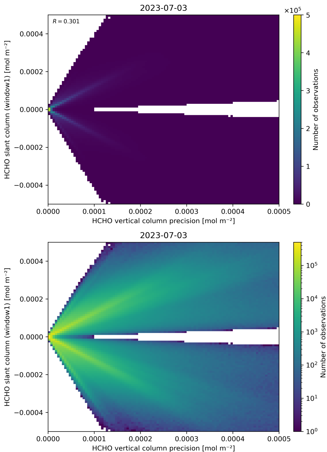
Figure 142: Scatter density plot of “HCHO vertical column precision” against “HCHO slant column (window1)” for 2023-07-03 to 2023-07-04.
