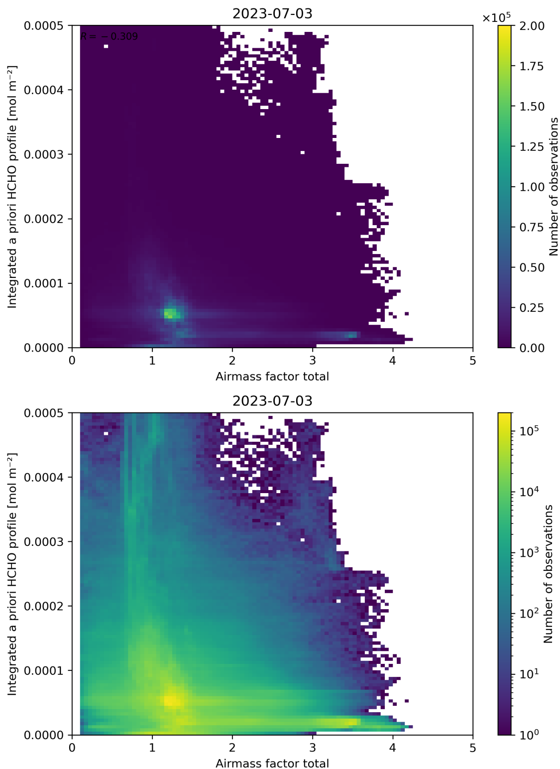
Figure 104: Scatter density plot of “Airmass factor total” against “Integrated a priori HCHO profile” for 2023-07-03 to 2023-07-04.
