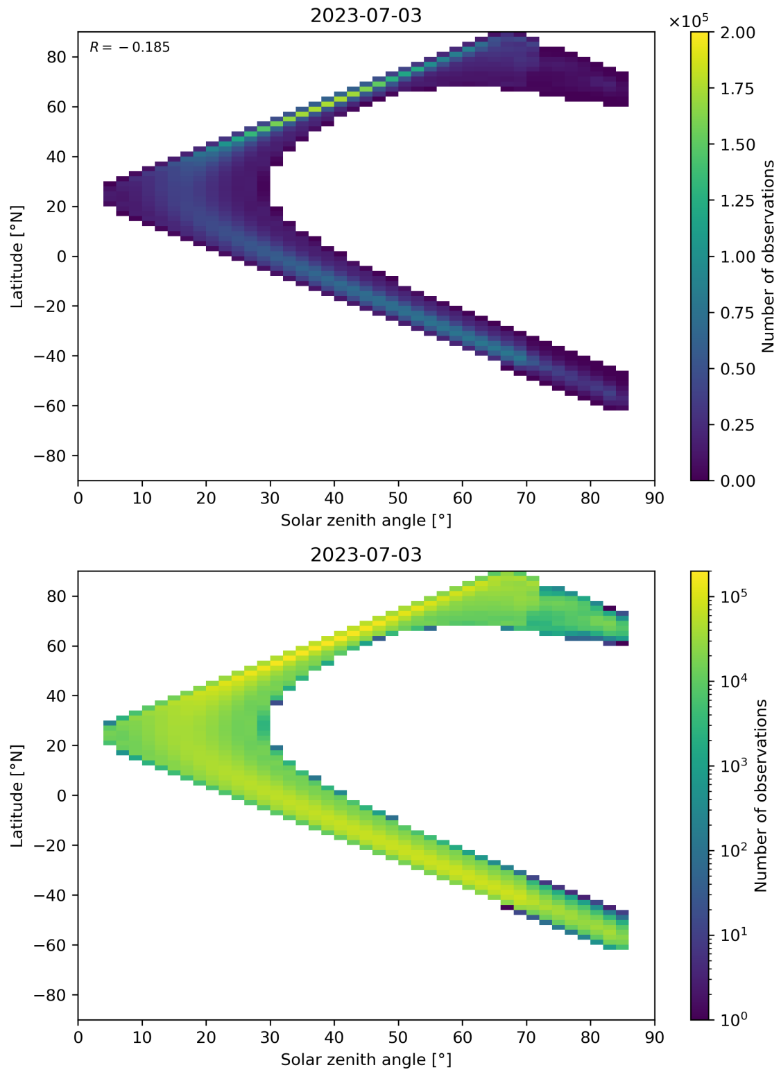
Figure 181: Scatter density plot of “Solar zenith angle” against “Latitude” for 2023-07-03 to 2023-07-04.
