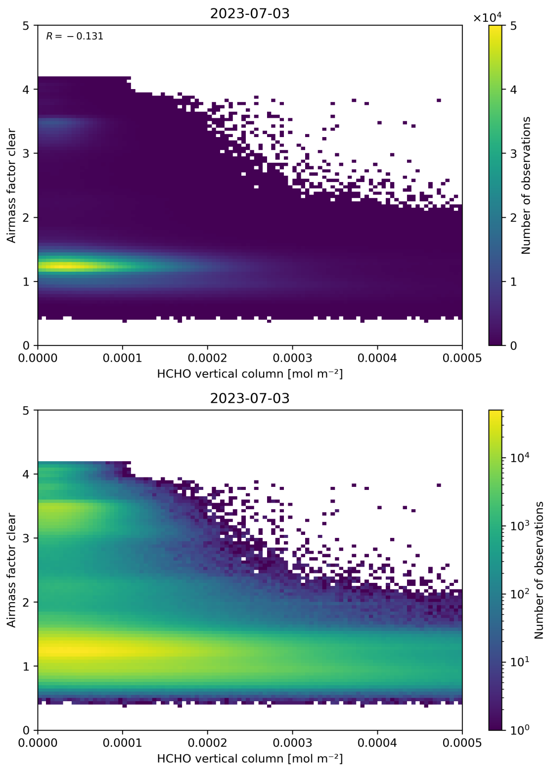
Figure 126: Scatter density plot of “HCHO vertical column” against “Airmass factor clear” for 2023-07-03 to 2023-07-04.
