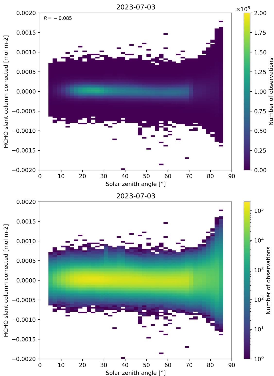
Figure 171: Scatter density plot of “Solar zenith angle” against “HCHO slant column corrected” for 2023-07-03 to 2023-07-04.
