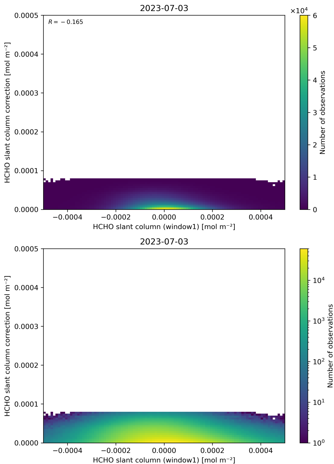
Figure 83: Scatter density plot of “HCHO slant column (window1)” against “HCHO slant column correction” for 2023-07-03 to 2023-07-04.
