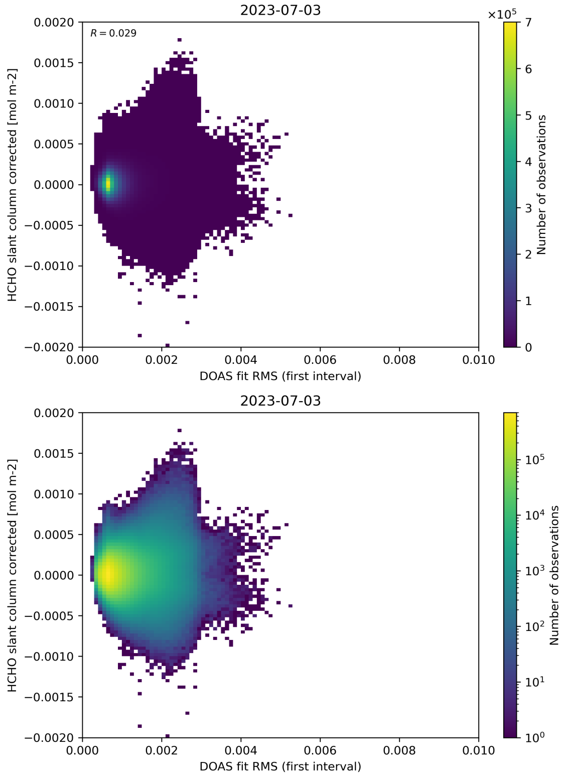
Figure 62: Scatter density plot of “DOAS fit RMS (first interval)” against “HCHO slant column corrected” for 2023-07-03 to 2023-07-04.
