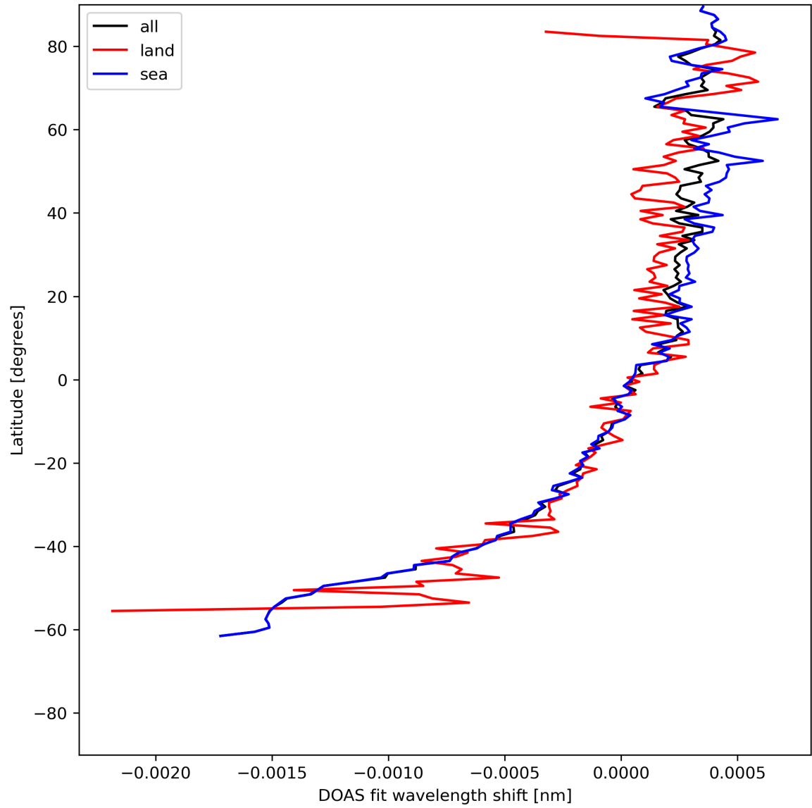
Figure 30: Zonal average of “DOAS fit wavelength shift” for 2023-07-03 to 2023-07-04.
