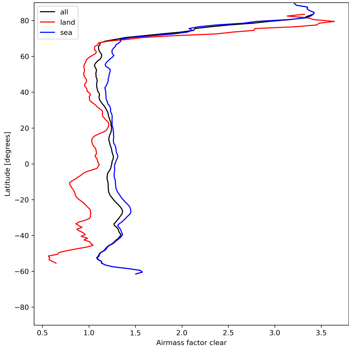
Figure 28: Zonal average of “Airmass factor clear” for 2023-07-03 to 2023-07-04.
