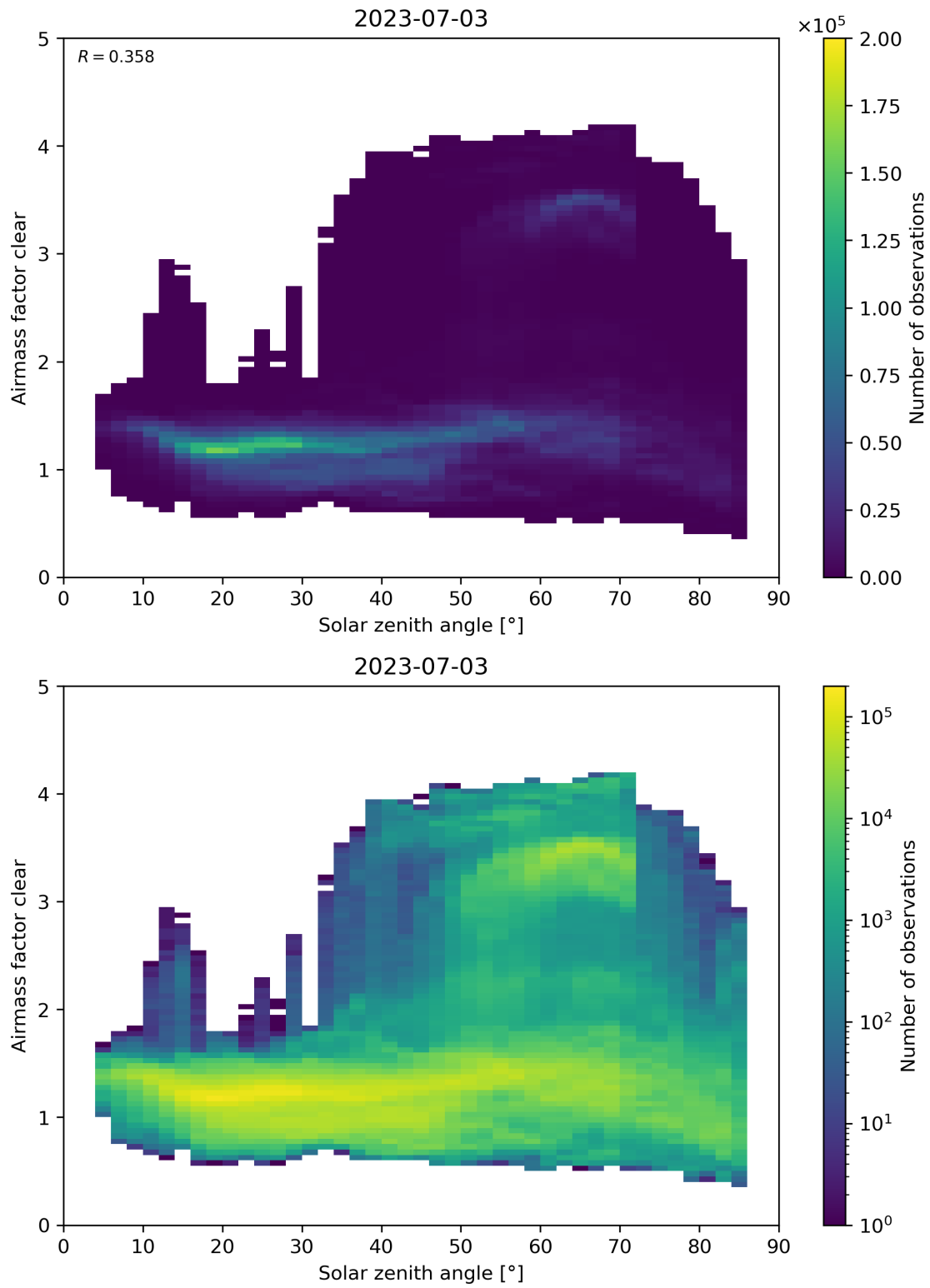
Figure 170: Scatter density plot of “Solar zenith angle” against “Airmass factor clear” for 2023-07-03 to 2023-07-04.
