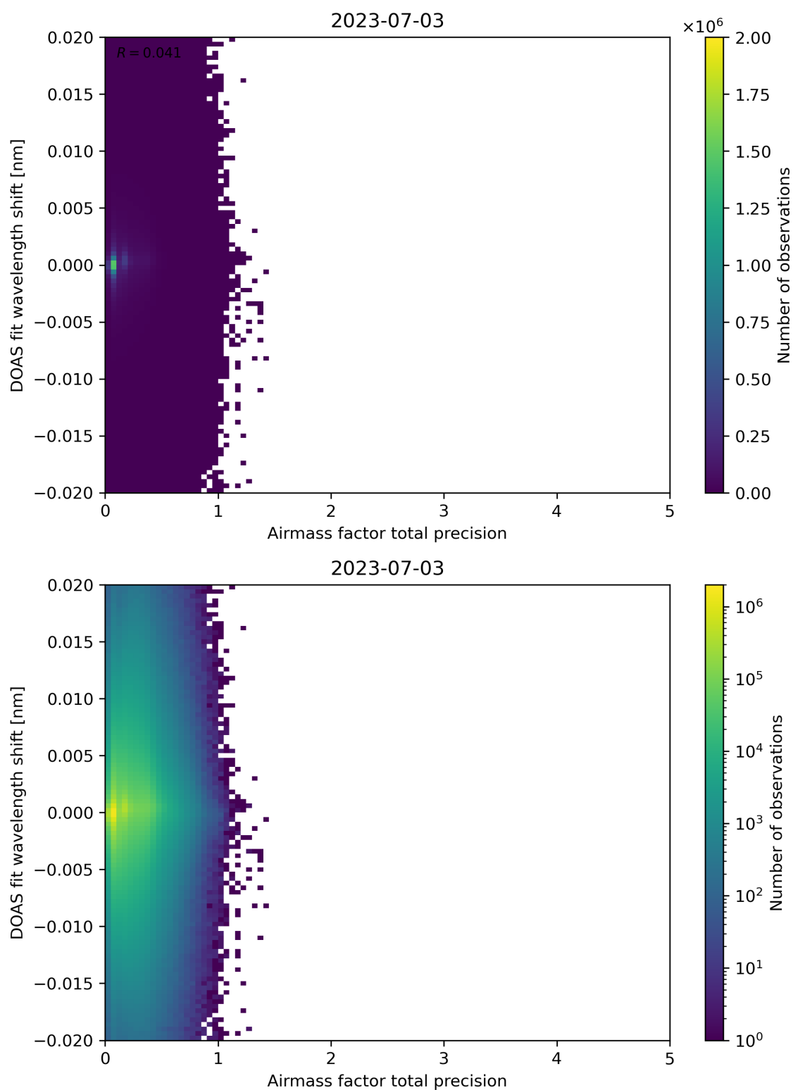
Figure 106: Scatter density plot of “Airmass factor total precision” against “DOAS fit wavelength shift” for 2023-07-03 to 2023-07-04.
