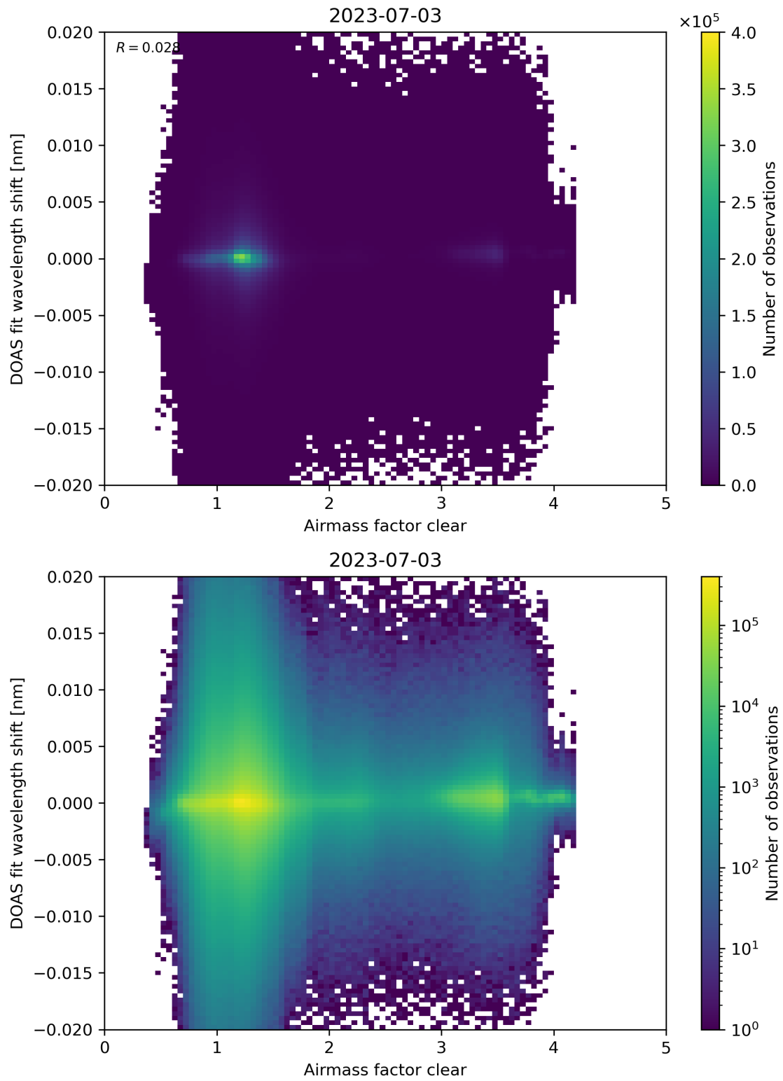
Figure 72: Scatter density plot of “Airmass factor clear” against “DOAS fit wavelength shift” for 2023-07-03 to 2023-07-04.
