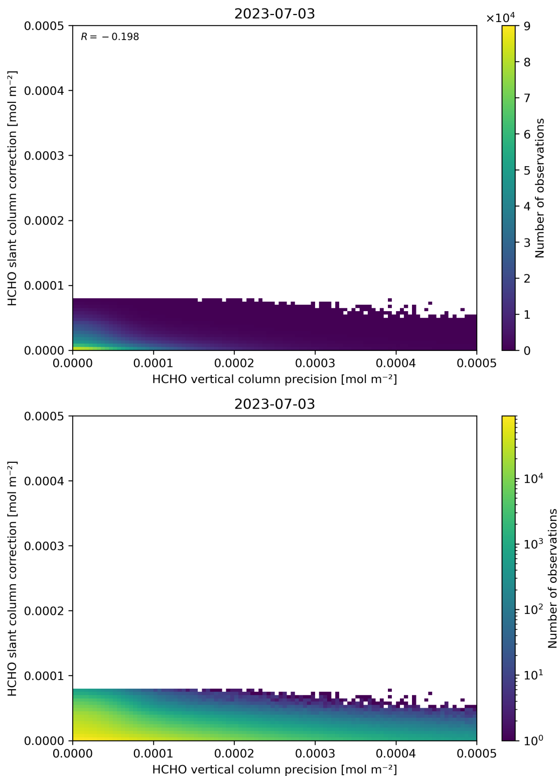
Figure 141: Scatter density plot of “HCHO vertical column precision” against “HCHO slant column correction” for 2023-07-03 to 2023-07-04.
