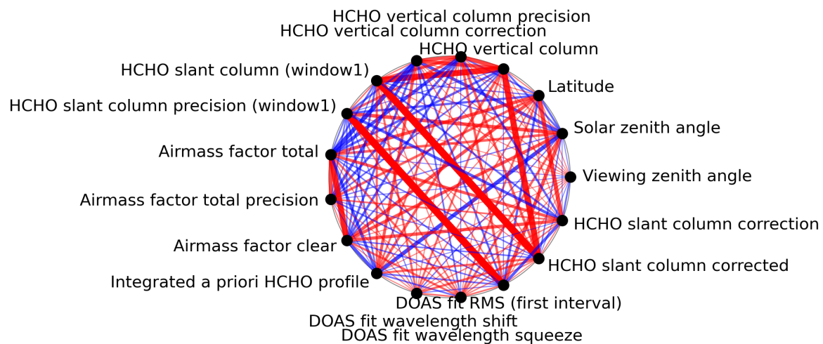
Figure 1: Map of correlation graph for 2023-07-03 to 2023-07-04.
