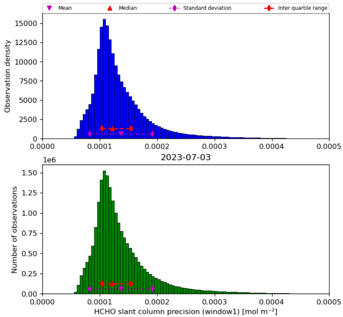
Figure 39: Histogram of “HCHO slant column precision (window1)” for 2023-07-03 to 2023-07-04
