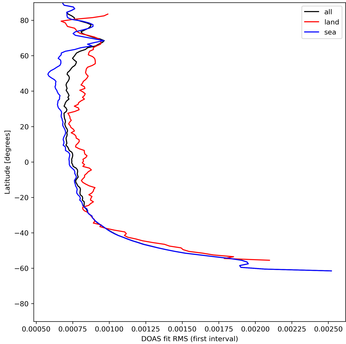
Figure 32: Zonal average of “DOAS fit RMS (first interval)” for 2023-07-03 to 2023-07-04.
