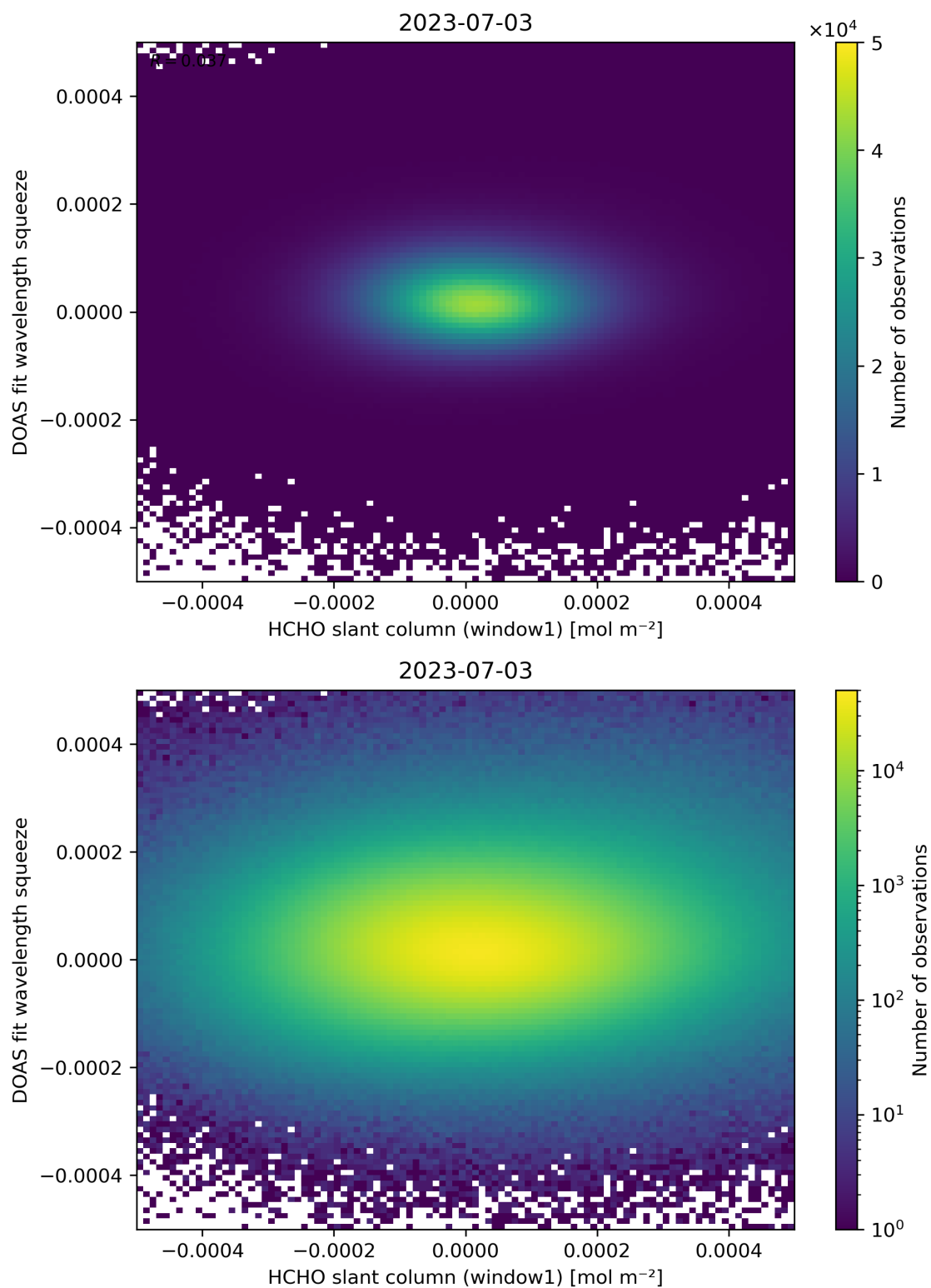
Figure 80: Scatter density plot of “HCHO slant column (window1)” against “DOAS fit wavelength squeeze” for 2023-07-03 to 2023-07-04.
