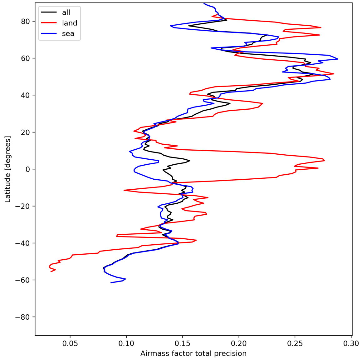
Figure 27: Zonal average of “Airmass factor total precision” for 2023-07-03 to 2023-07-04.
