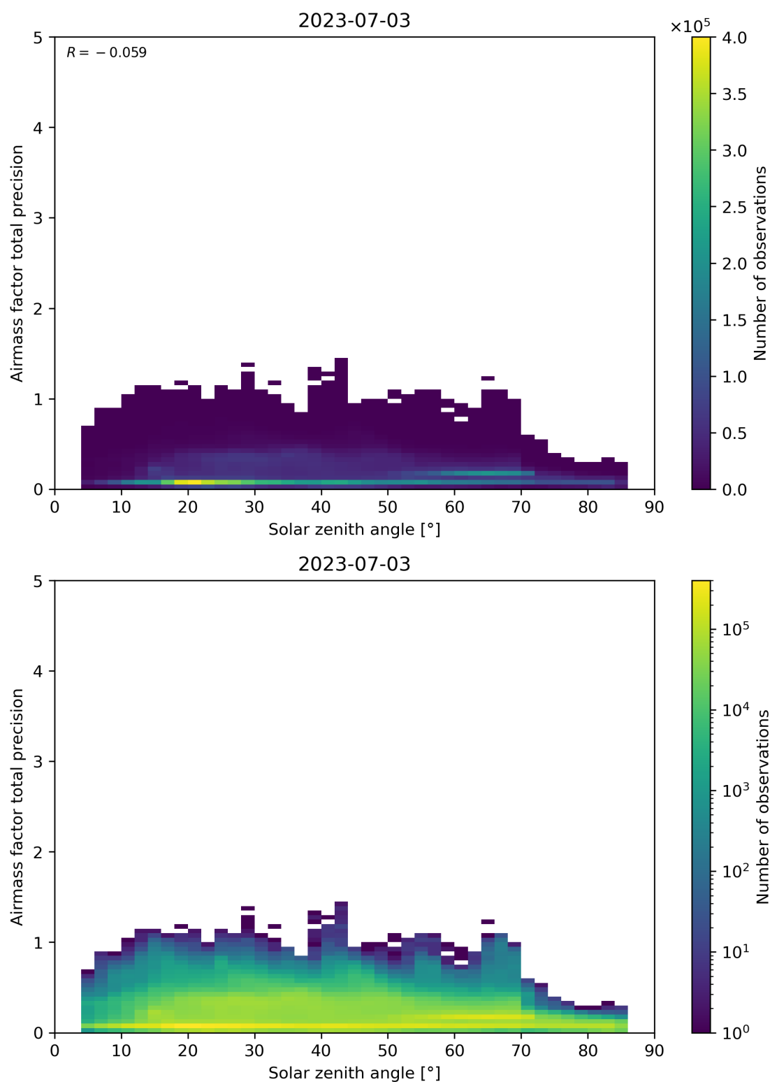
Figure 176: Scatter density plot of “Solar zenith angle” against “Airmass factor total precision” for 2023-07-03 to 2023-07-04.
