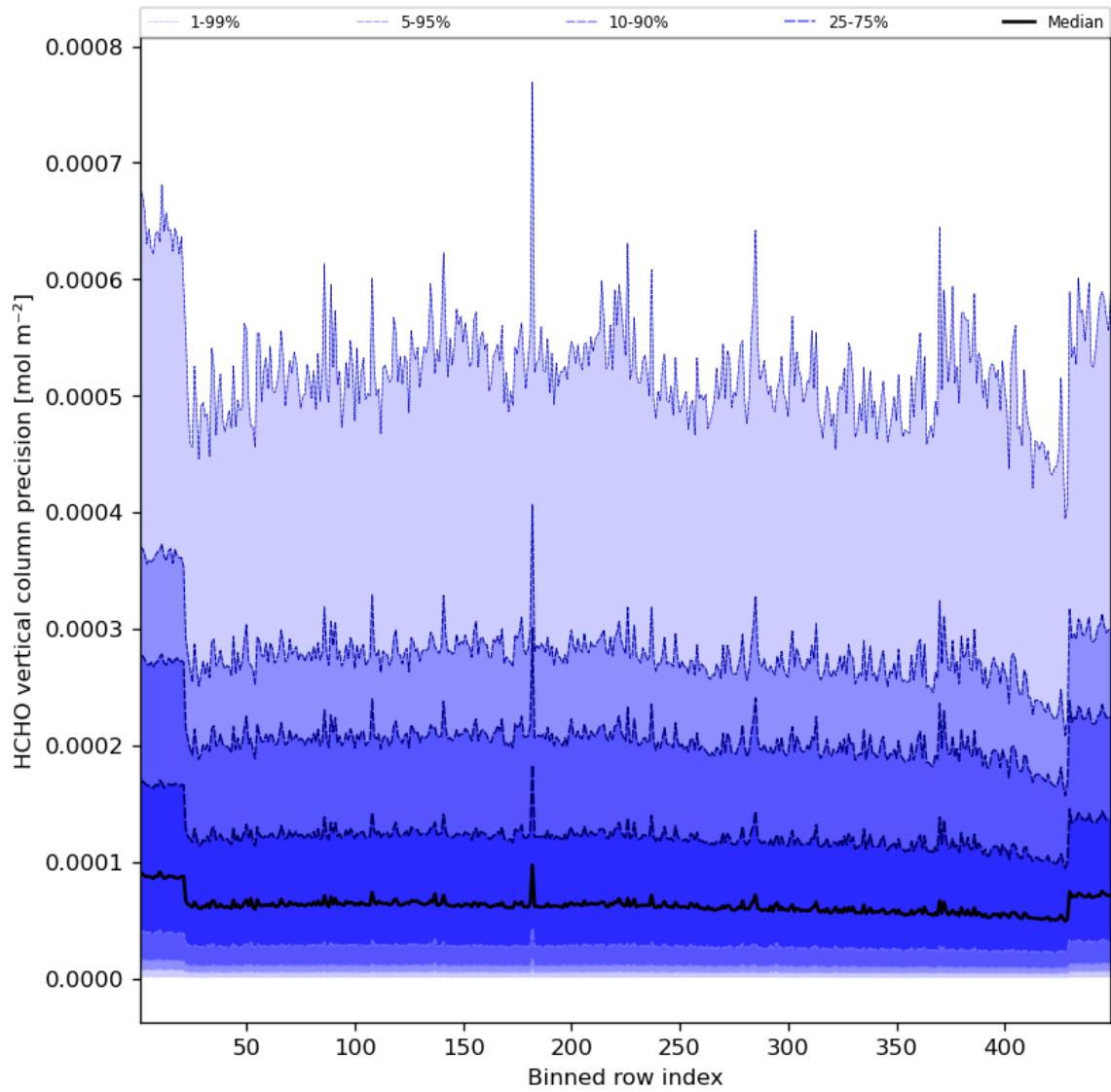
Figure 50: Along track statistics of “HCHO vertical column precision” for 2023-07-03 to 2023-07-04
