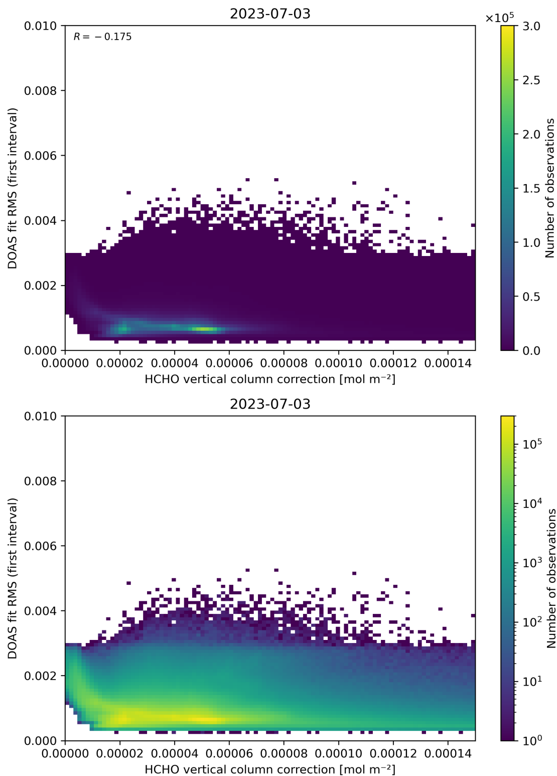
Figure 112: Scatter density plot of “HCHO vertical column correction” against “DOAS fit RMS (first interval)” for 2023-07-03 to 2023-07-04.
