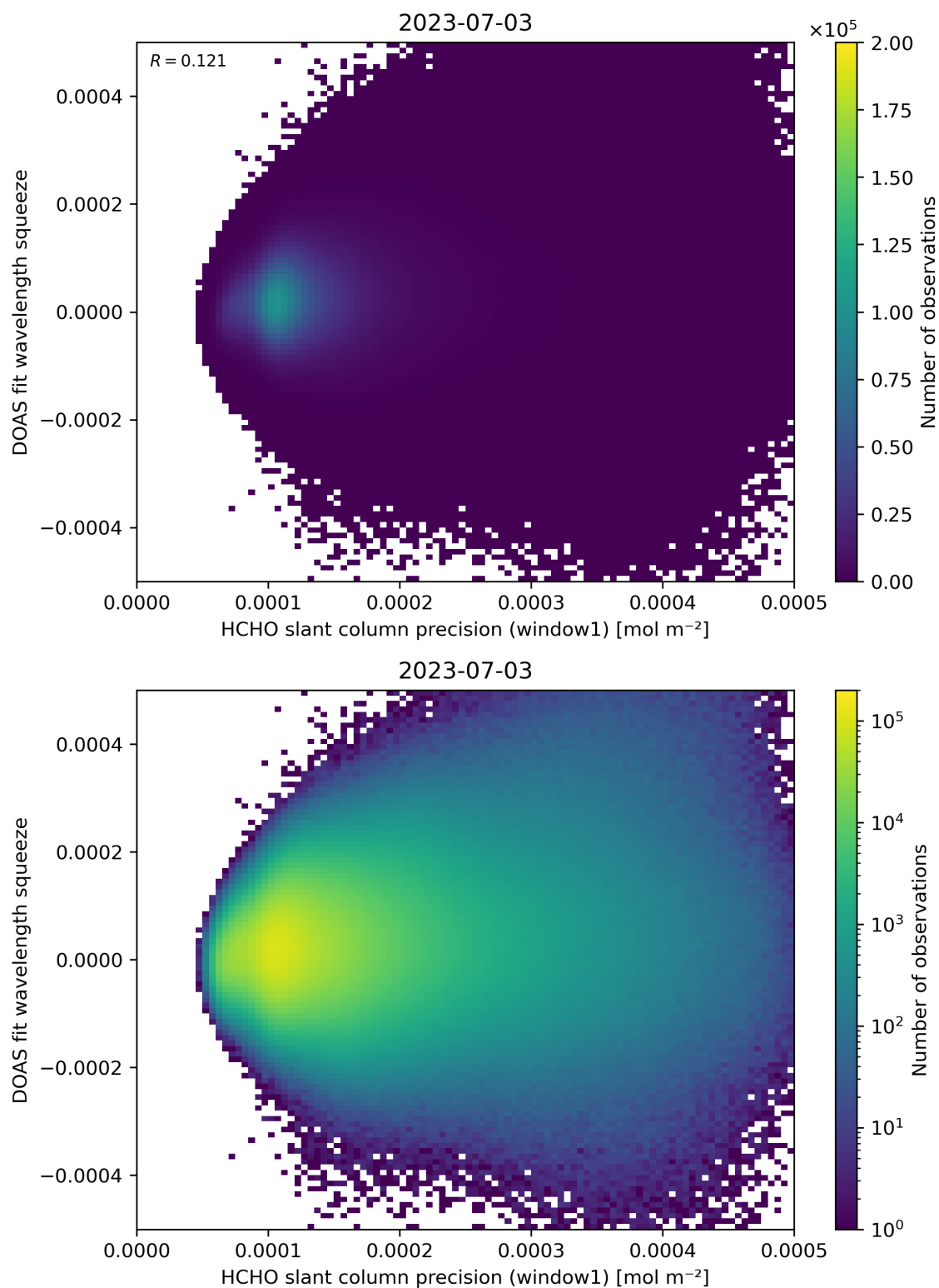
Figure 90: Scatter density plot of “HCHO slant column precision (window1)” against “DOAS fit wavelength squeeze” for 2023-07-03 to 2023-07-04.
