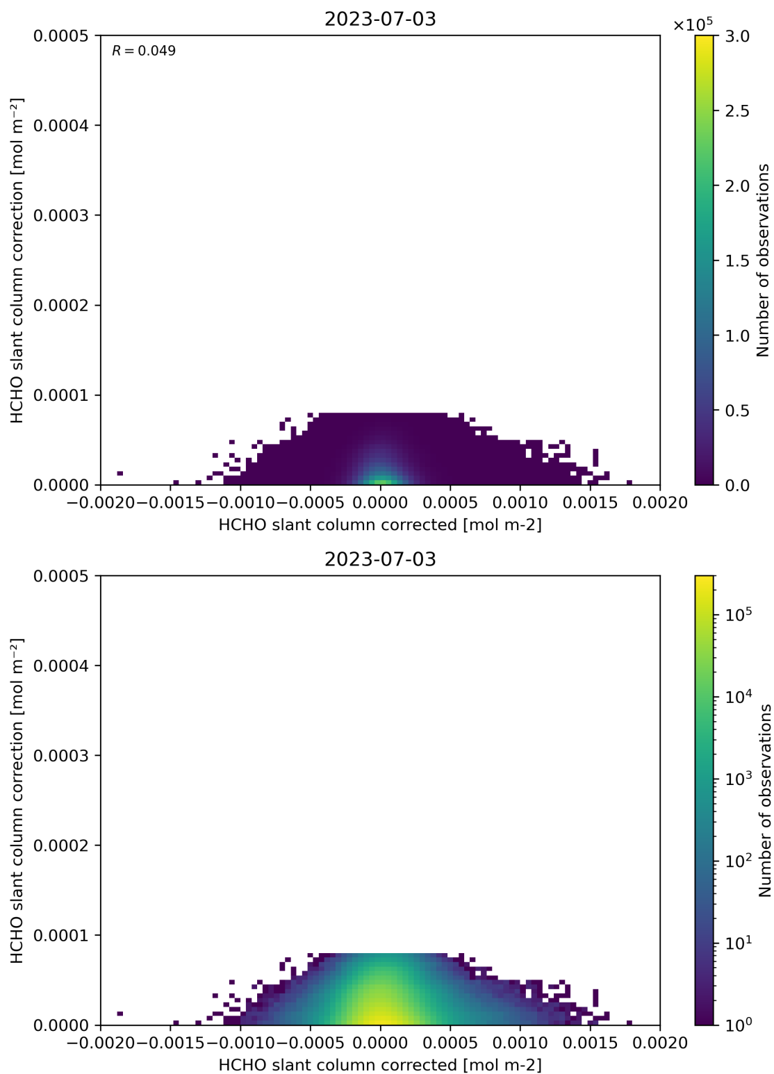
Figure 77: Scatter density plot of “HCHO slant column corrected” against “HCHO slant column correction” for 2023-07-03 to 2023-07-04.
