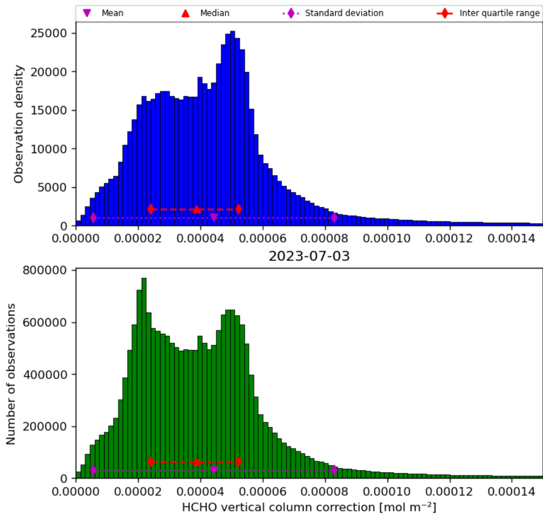
Figure 37: Histogram of “HCHO vertical column correction” for 2023-07-03 to 2023-07-04
