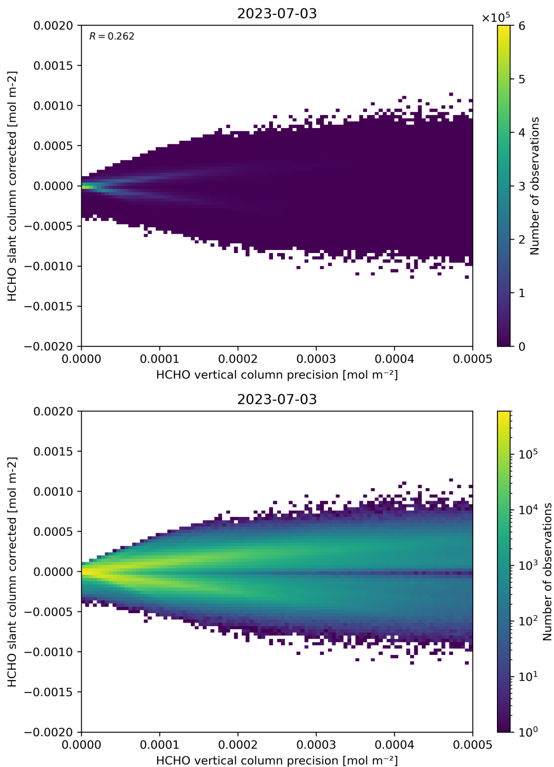
Figure 140: Scatter density plot of “HCHO vertical column precision” against “HCHO slant column corrected” for 2023-07-03 to 2023-07-04.
