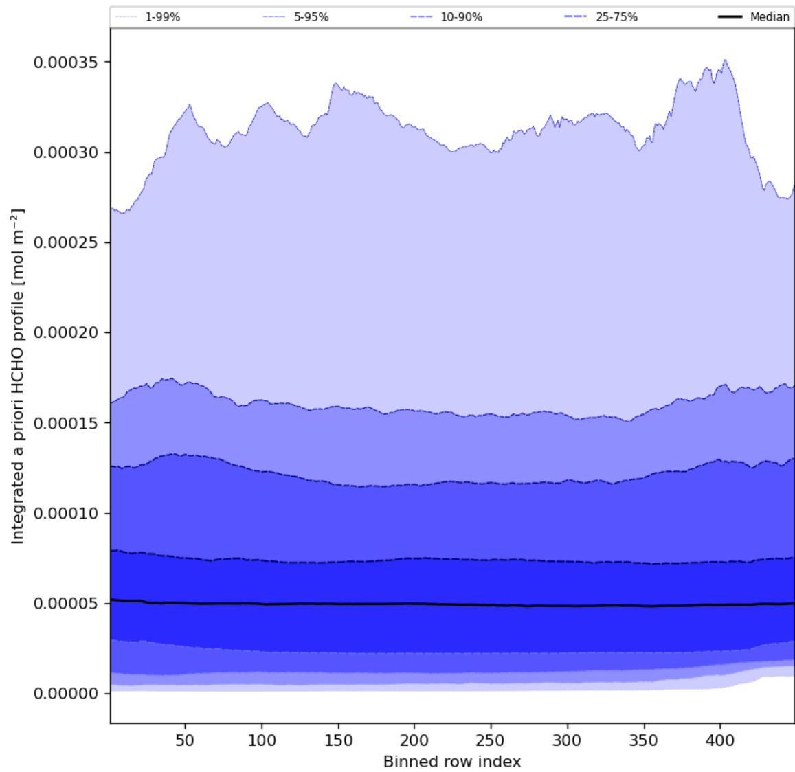
Figure 57: Along track statistics of "Integrated a priori HCHO profile" for 2023-07-03 to 2023-07-04
