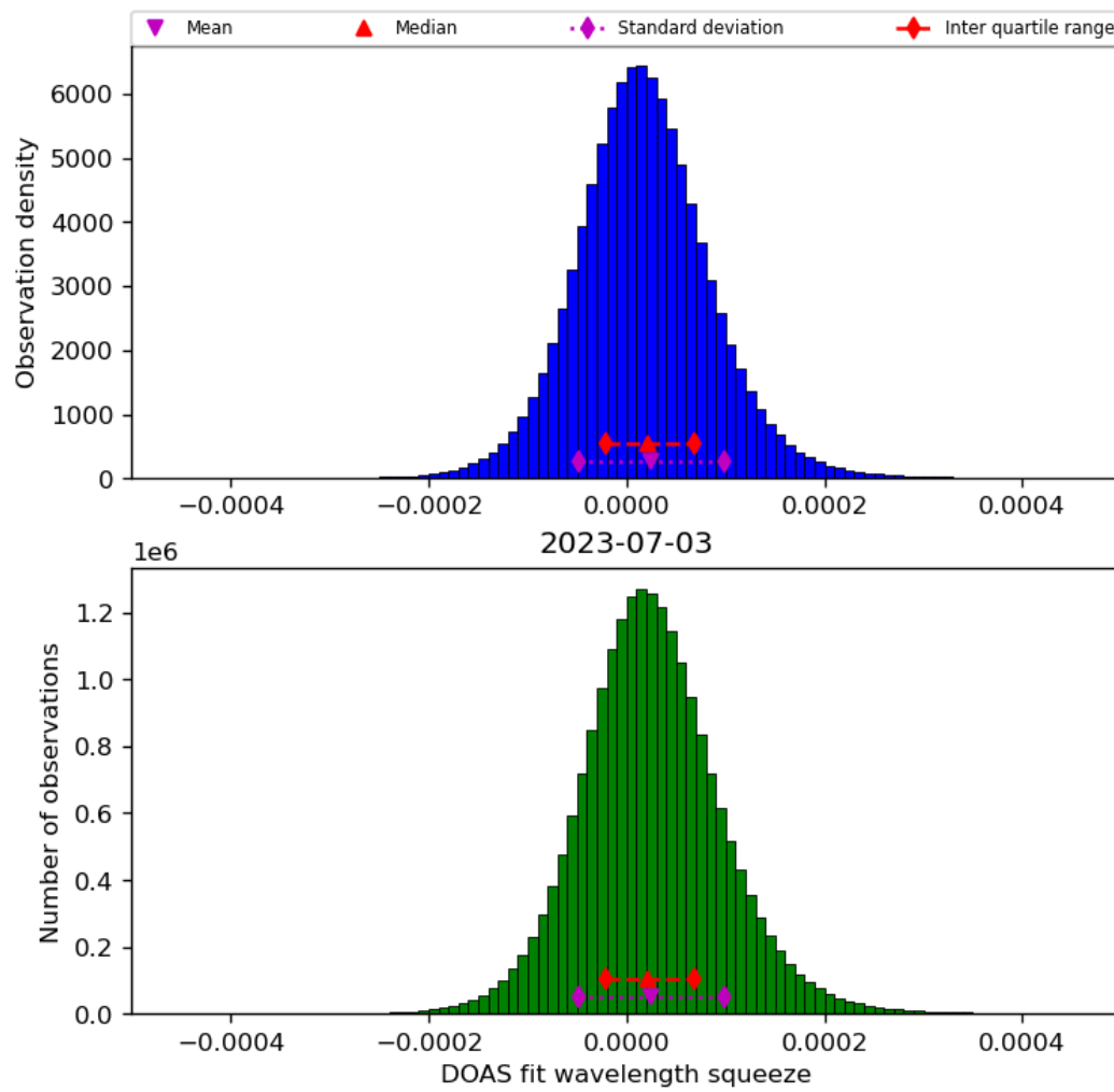
Figure 45: Histogram of “DOAS fit wavelength squeeze” for 2023-07-03 to 2023-07-04
