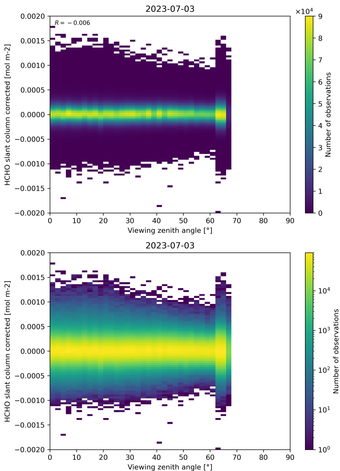
Figure 186: Scatter density plot of “Viewing zenith angle” against “HCHO slant column corrected” for 2023-07-03 to 2023-07-04.
