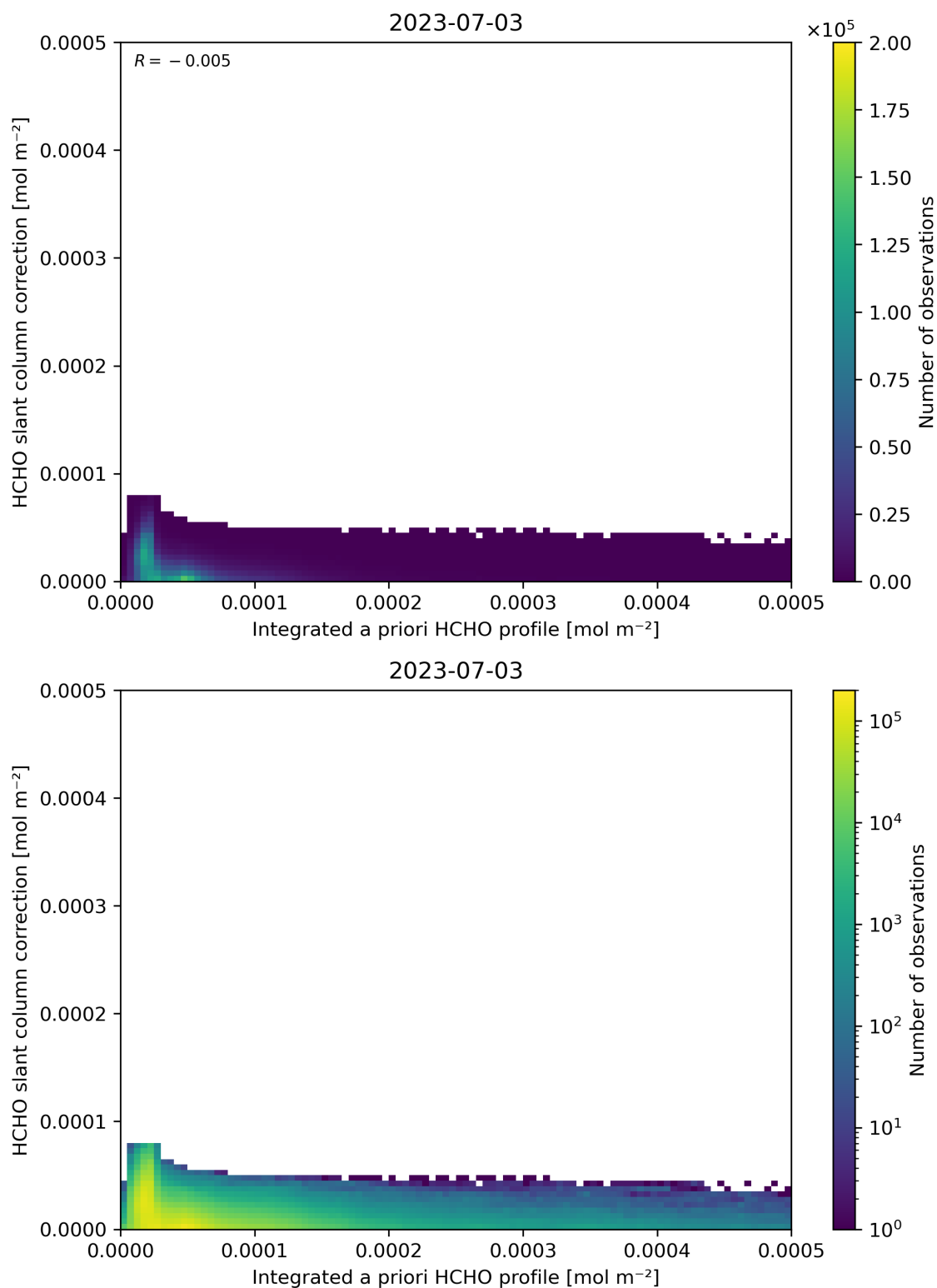
Figure 152: Scatter density plot of “Integrated a priori HCHO profile” against “HCHO slant column correction” for 2023-07-03 to 2023-07-04.
