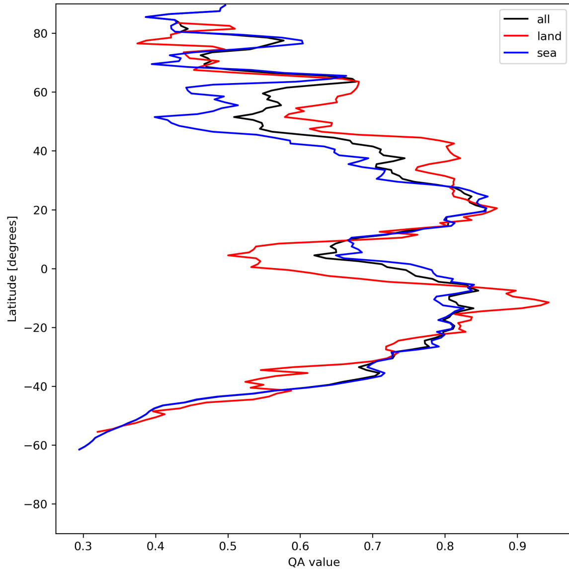
Figure 20: Zonal average of “QA value” for 2023-07-03 to 2023-07-04.
