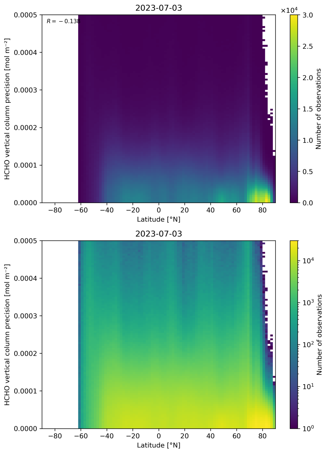
Figure 165: Scatter density plot of “Latitude” against “HCHO vertical column precision” for 2023-07-03 to 2023-07-04.
