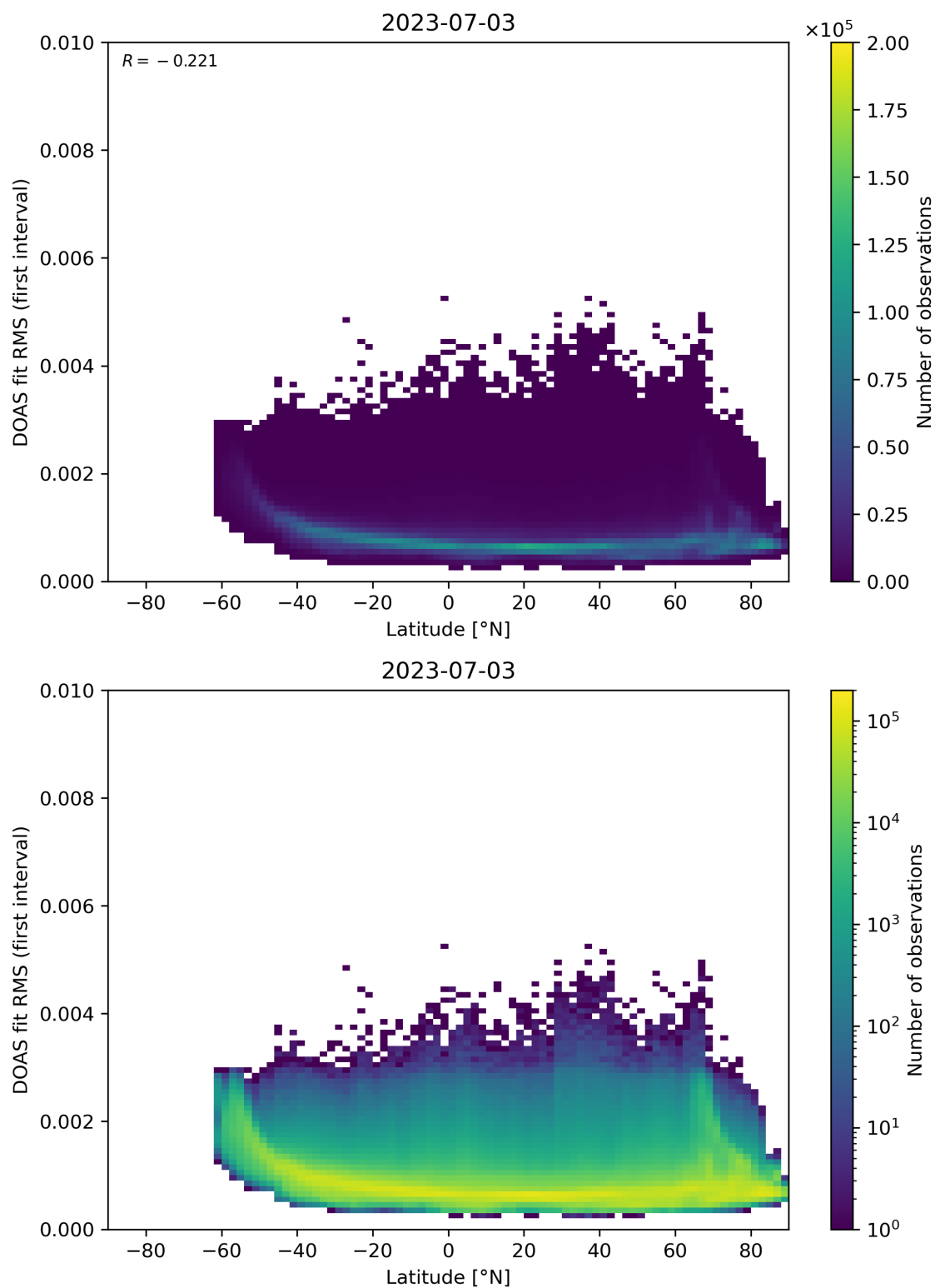
Figure 153: Scatter density plot of “Latitude” against “DOAS fit RMS (first interval)” for 2023-07-03 to 2023-07-04.
