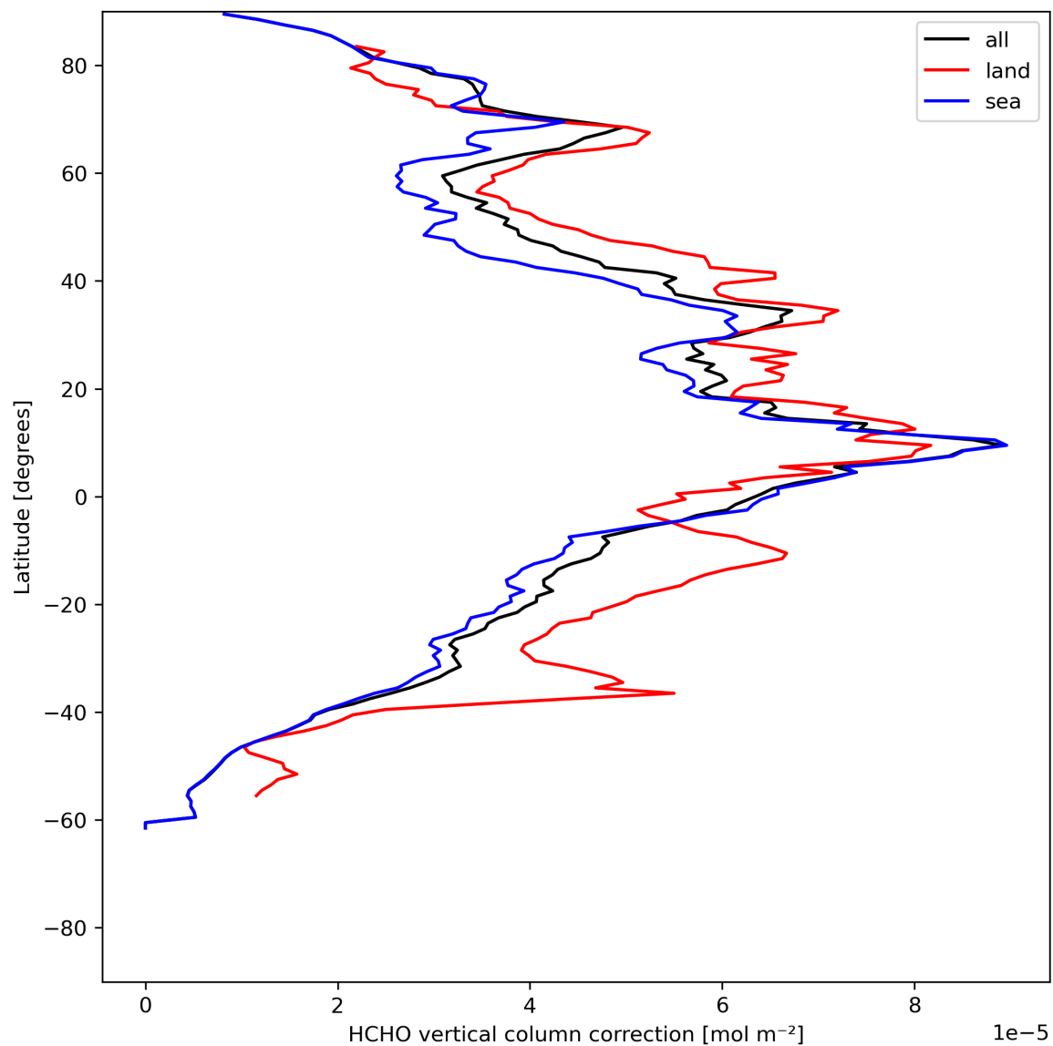
Figure 23: Zonal average of “HCHO vertical column correction” for 2023-07-03 to 2023-07-04.
