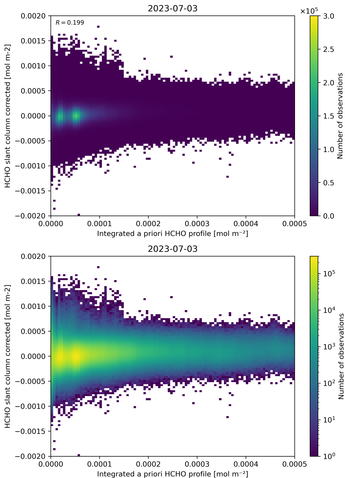
Figure 151: Scatter density plot of “Integrated a priori HCHO profile” against “HCHO slant column corrected” for 2023-07-03 to 2023-07-04.
