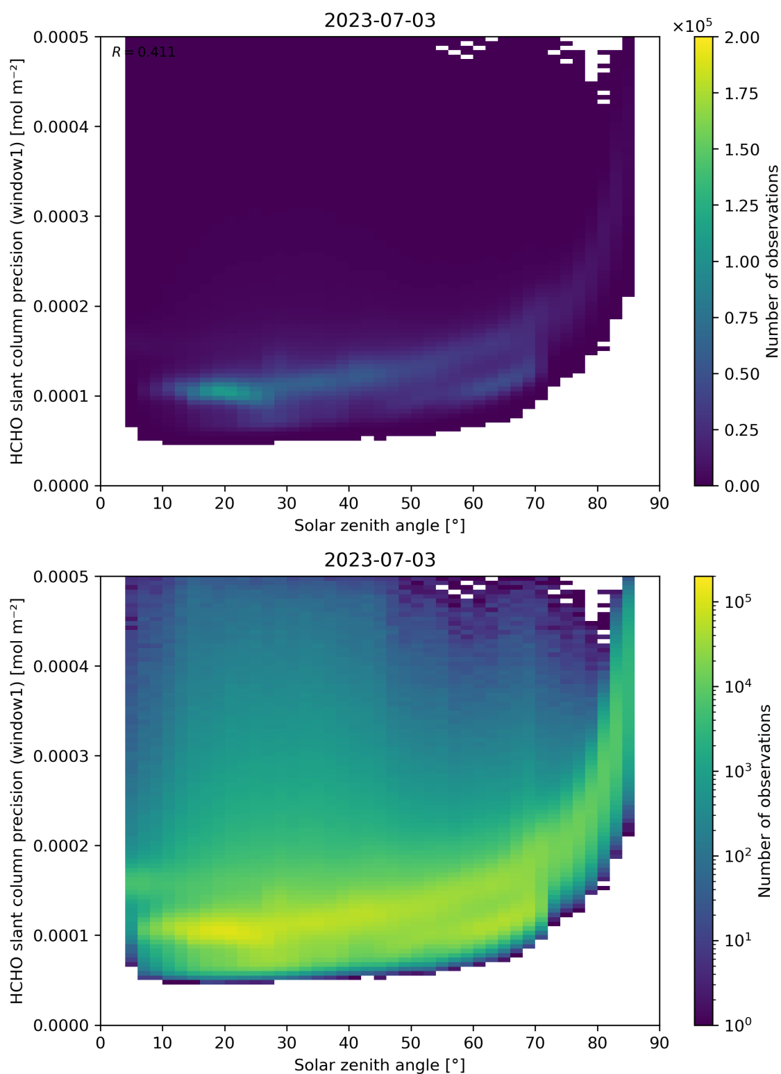
Figure 174: Scatter density plot of “Solar zenith angle” against “HCHO slant column precision (window1)” for 2023-07-03 to 2023-07-04.
