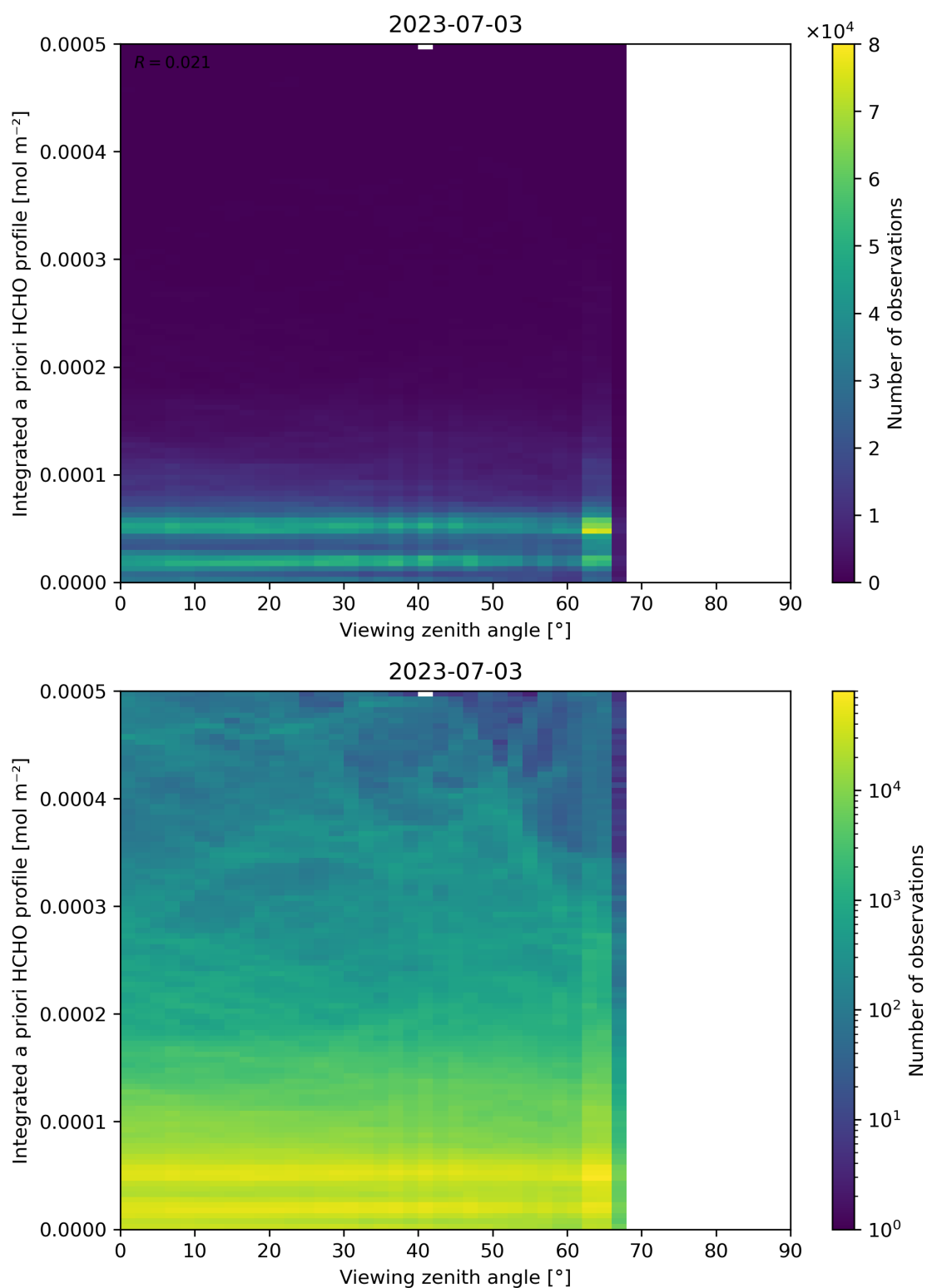
Figure 195: Scatter density plot of “Viewing zenith angle” against “Integrated a priori HCHO profile” for 2023-07-03 to 2023-07-04.
