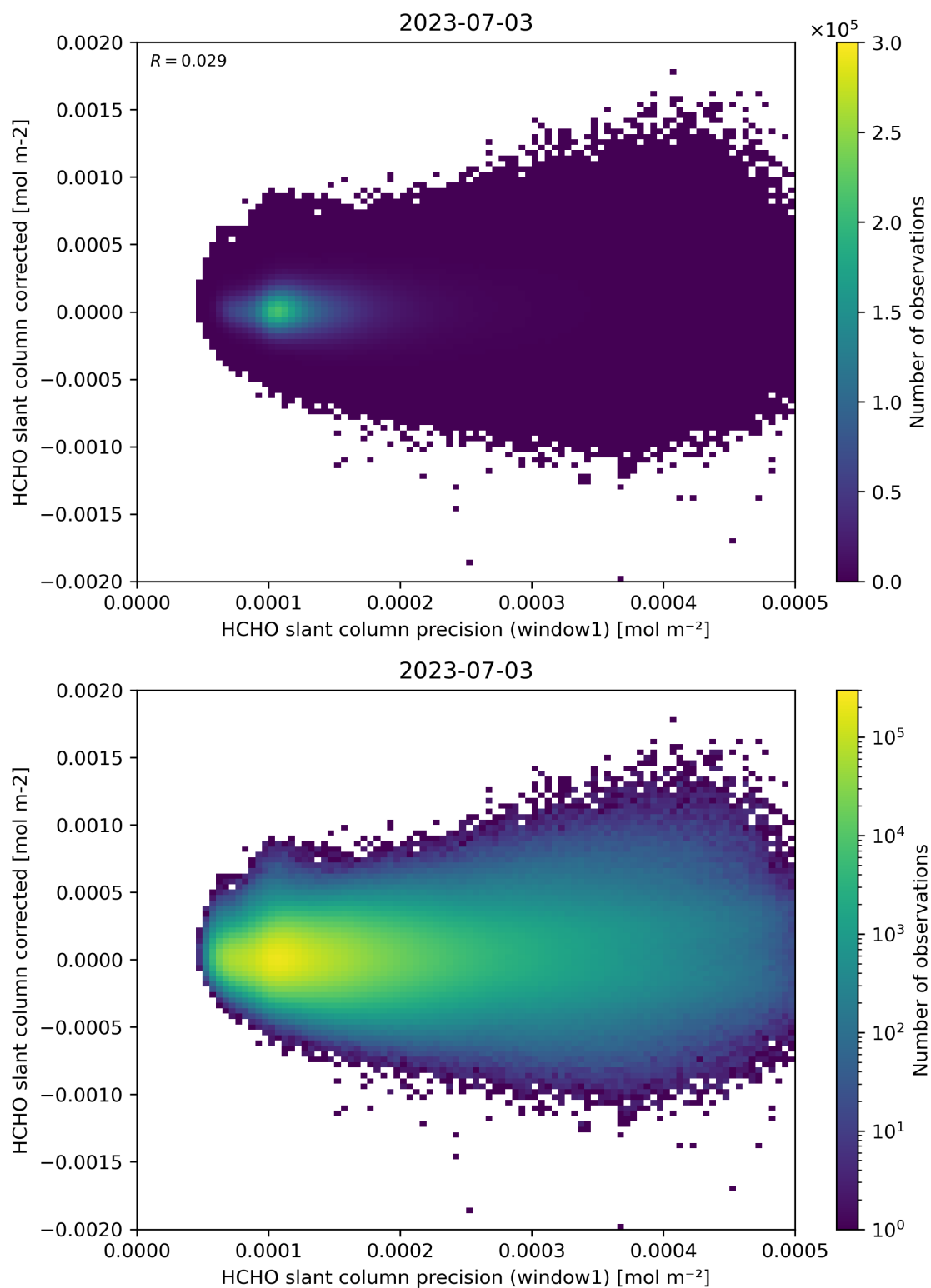
Figure 92: Scatter density plot of “HCHO slant column precision (window1)” against “HCHO slant column corrected” for 2023-07-03 to 2023-07-04.
