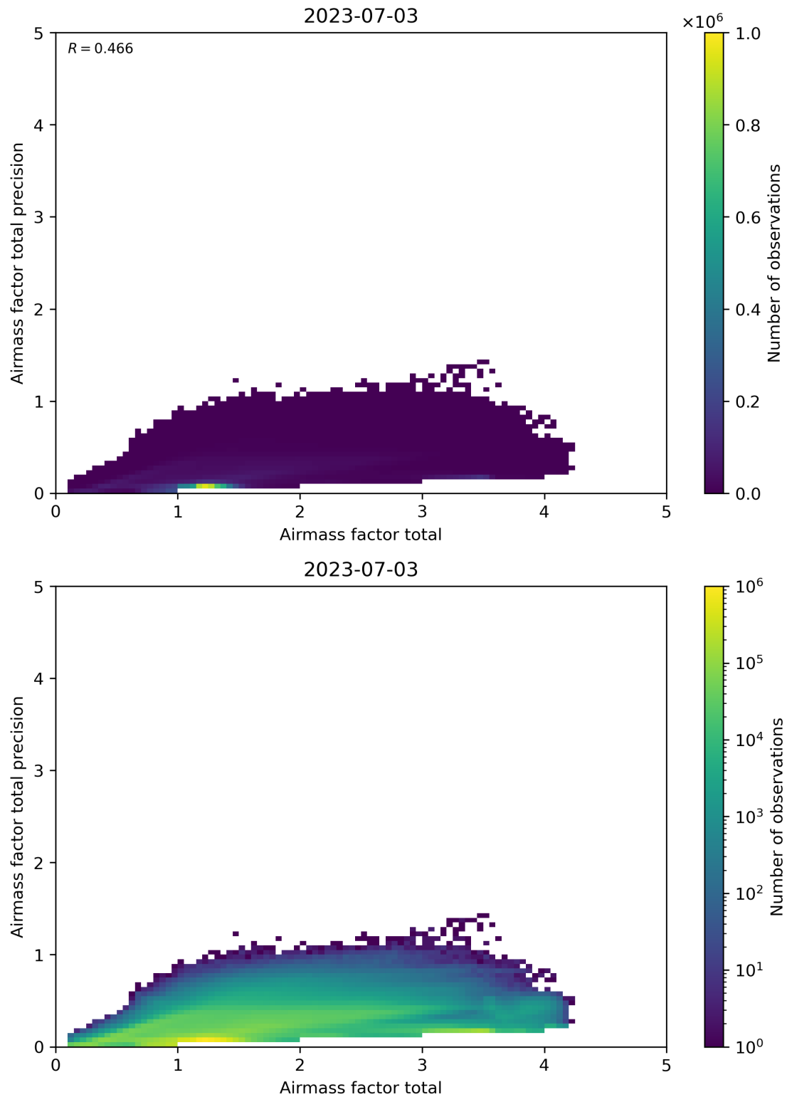
Figure 103: Scatter density plot of “Airmass factor total” against “Airmass factor total precision” for 2023-07-03 to 2023-07-04.
