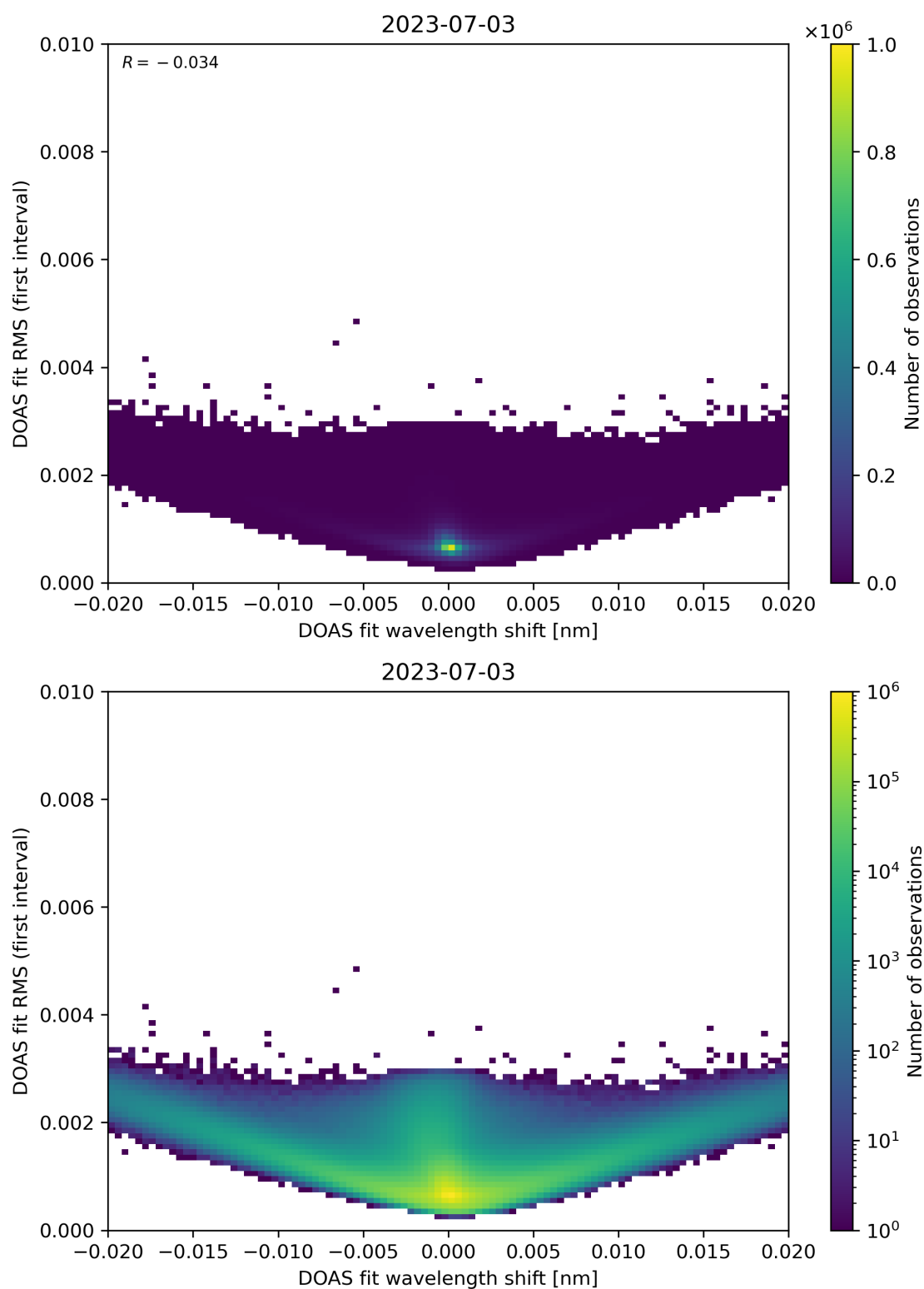
Figure 64: Scatter density plot of “DOAS fit wavelength shift” against “DOAS fit RMS (first interval)” for 2023-07-03 to 2023-07-04.
