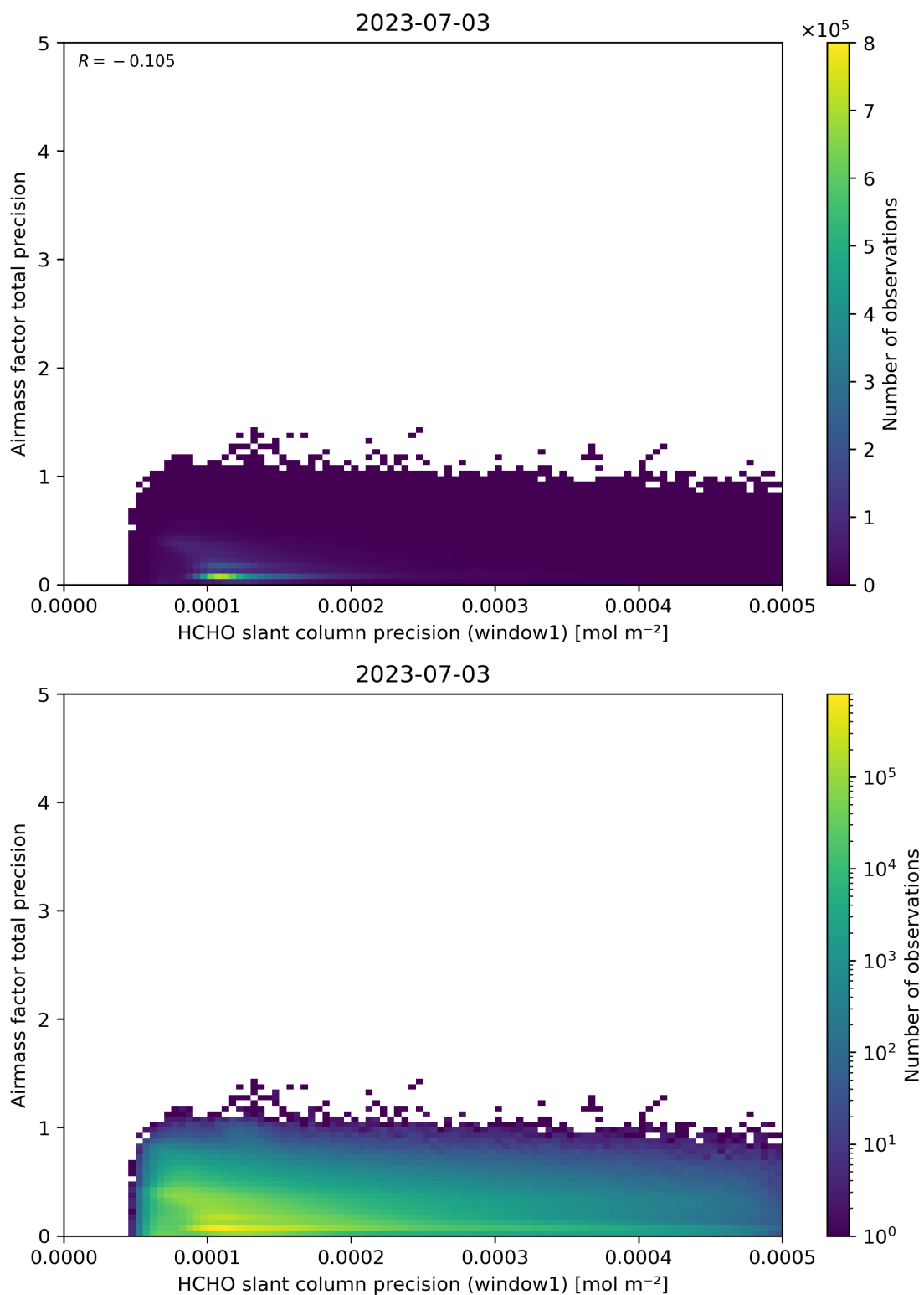
Figure 95: Scatter density plot of “HCHO slant column precision (window1)” against “Airmass factor total precision” for 2023-07-03 to 2023-07-04.
