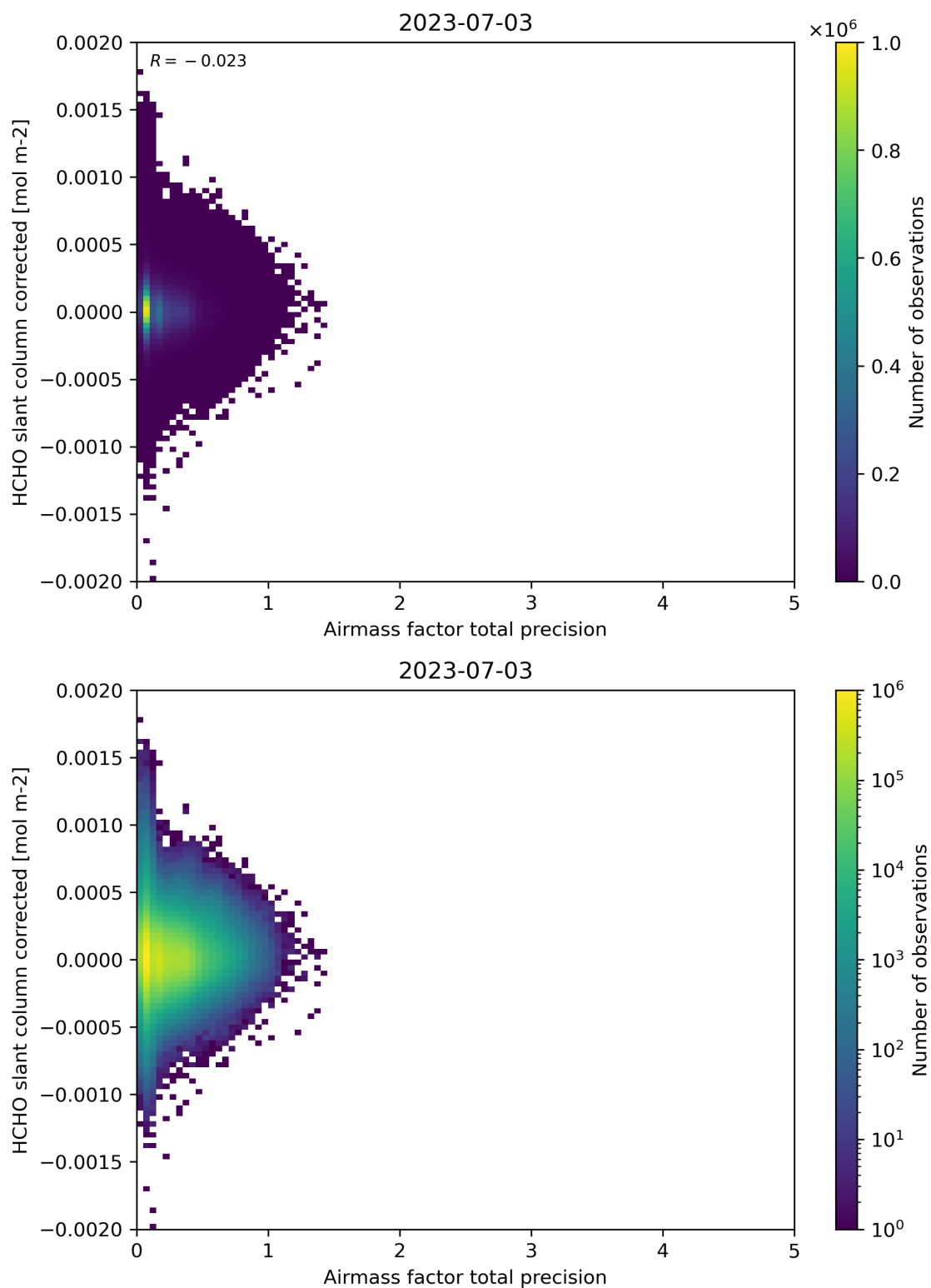
Figure 109: Scatter density plot of “Airmass factor total precision” against “HCHO slant column corrected” for 2023-07-03 to 2023-07-04.
