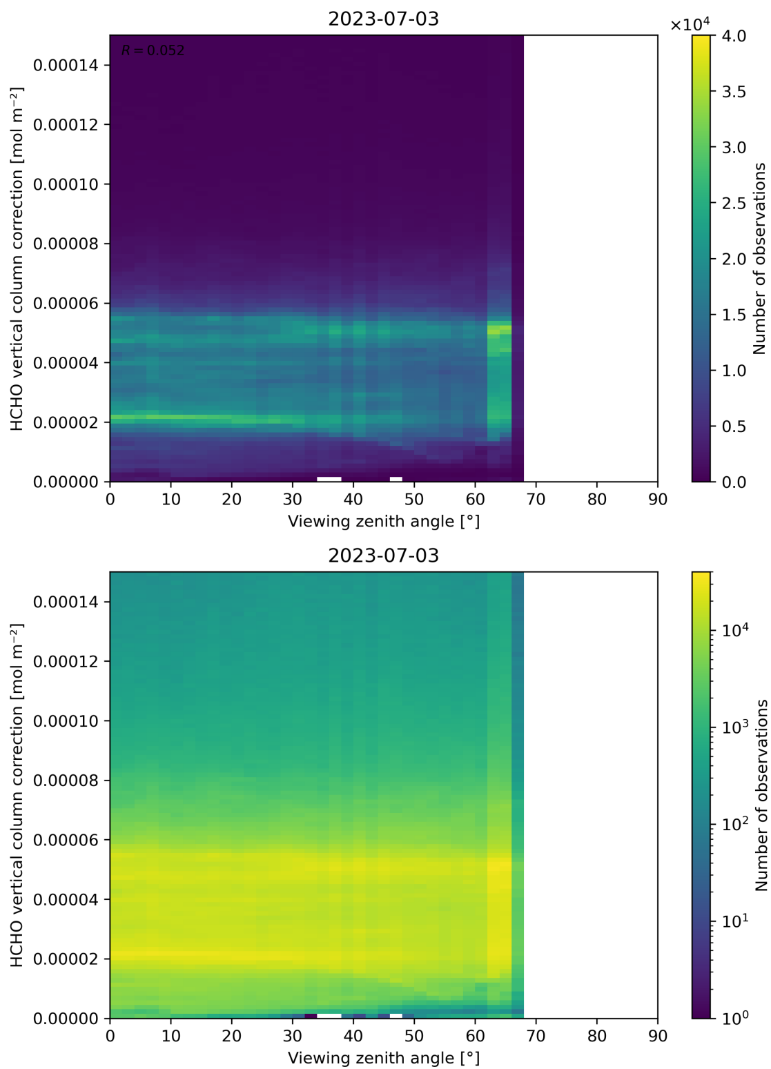
Figure 193: Scatter density plot of “Viewing zenith angle” against “HCHO vertical column correction” for 2023-07-03 to 2023-07-04.
