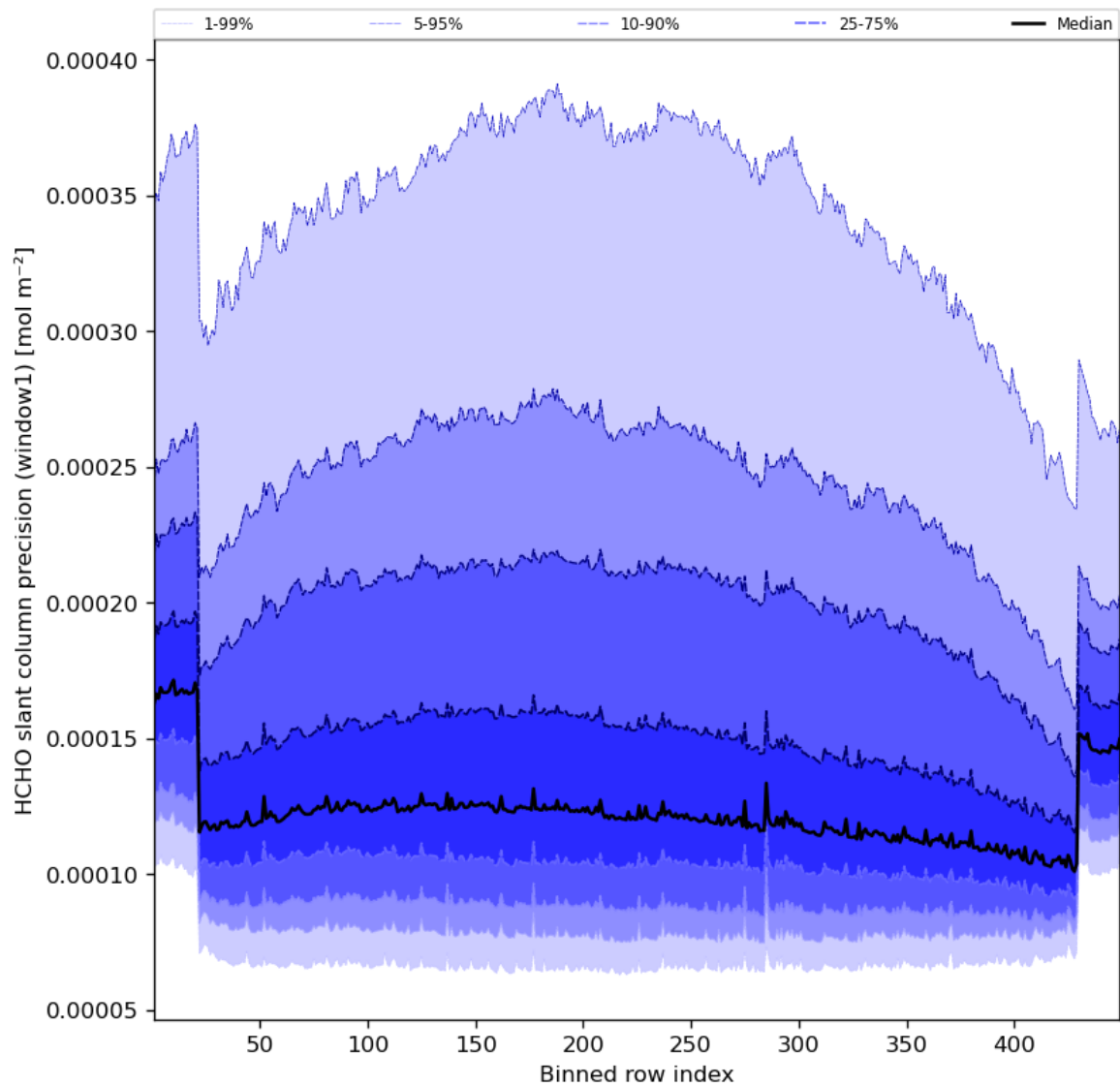
Figure 53: Along track statistics of “HCHO slant column precision (window1)” for 2023-07-03 to 2023-07-04
