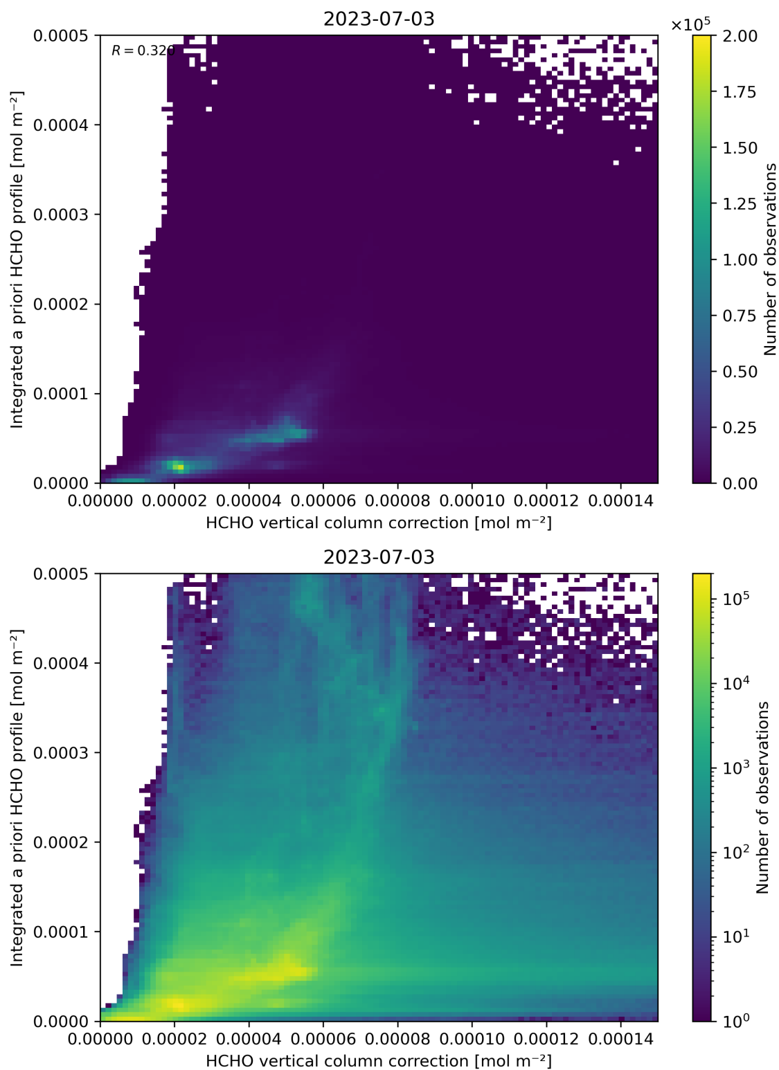
Figure 122: Scatter density plot of “HCHO vertical column correction” against “Integrated a priori HCHO profile” for 2023-07-03 to 2023-07-04.
