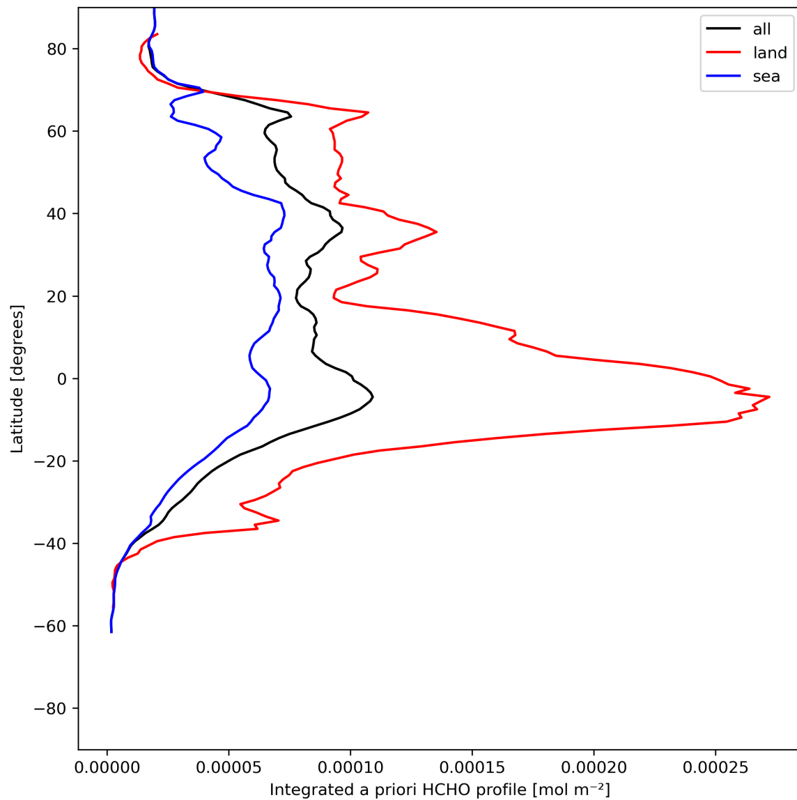
Figure 29: Zonal average of “Integrated a priori HCHO profile” for 2023-07-03 to 2023-07-04.
