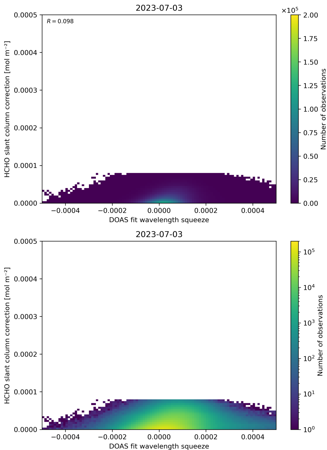
Figure 70: Scatter density plot of “DOAS fit wavelength squeeze” against “HCHO slant column correction” for 2023-07-03 to 2023-07-04.
