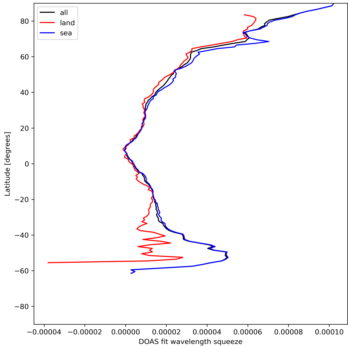
Figure 31: Zonal average of “DOAS fit wavelength squeeze” for 2023-07-03 to 2023-07-04.
