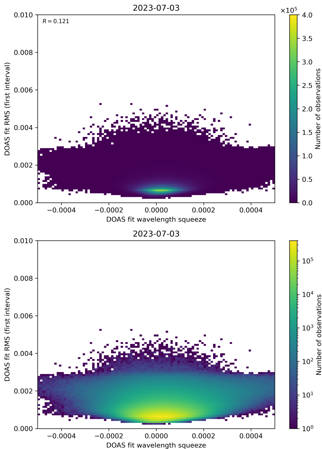
Figure 68: Scatter density plot of “DOAS fit wavelength squeeze” against “DOAS fit RMS (first interval)” for 2023-07-03 to 2023-07-04.
