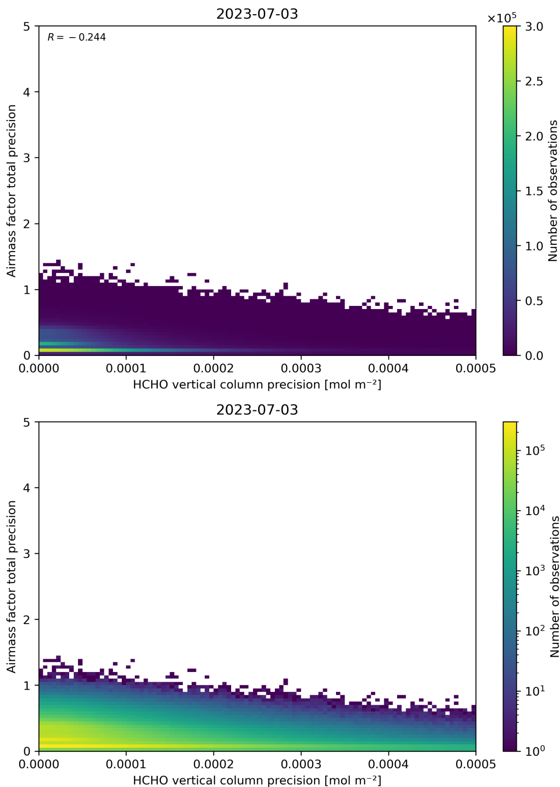
Figure 145: Scatter density plot of “HCHO vertical column precision” against “Airmass factor total precision” for 2023-07-03 to 2023-07-04.
