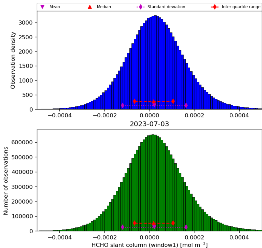
Figure 38: Histogram of “HCHO slant column (window1)” for 2023-07-03 to 2023-07-04
