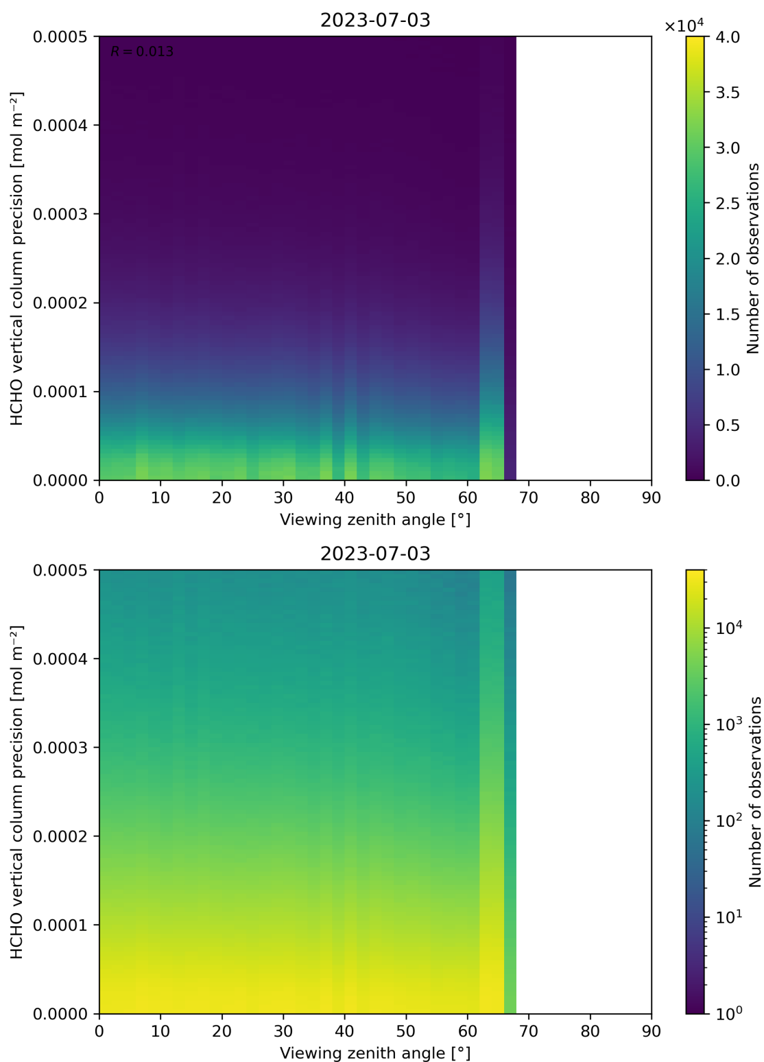
Figure 194: Scatter density plot of “Viewing zenith angle” against “HCHO vertical column precision” for 2023-07-03 to 2023-07-04.
