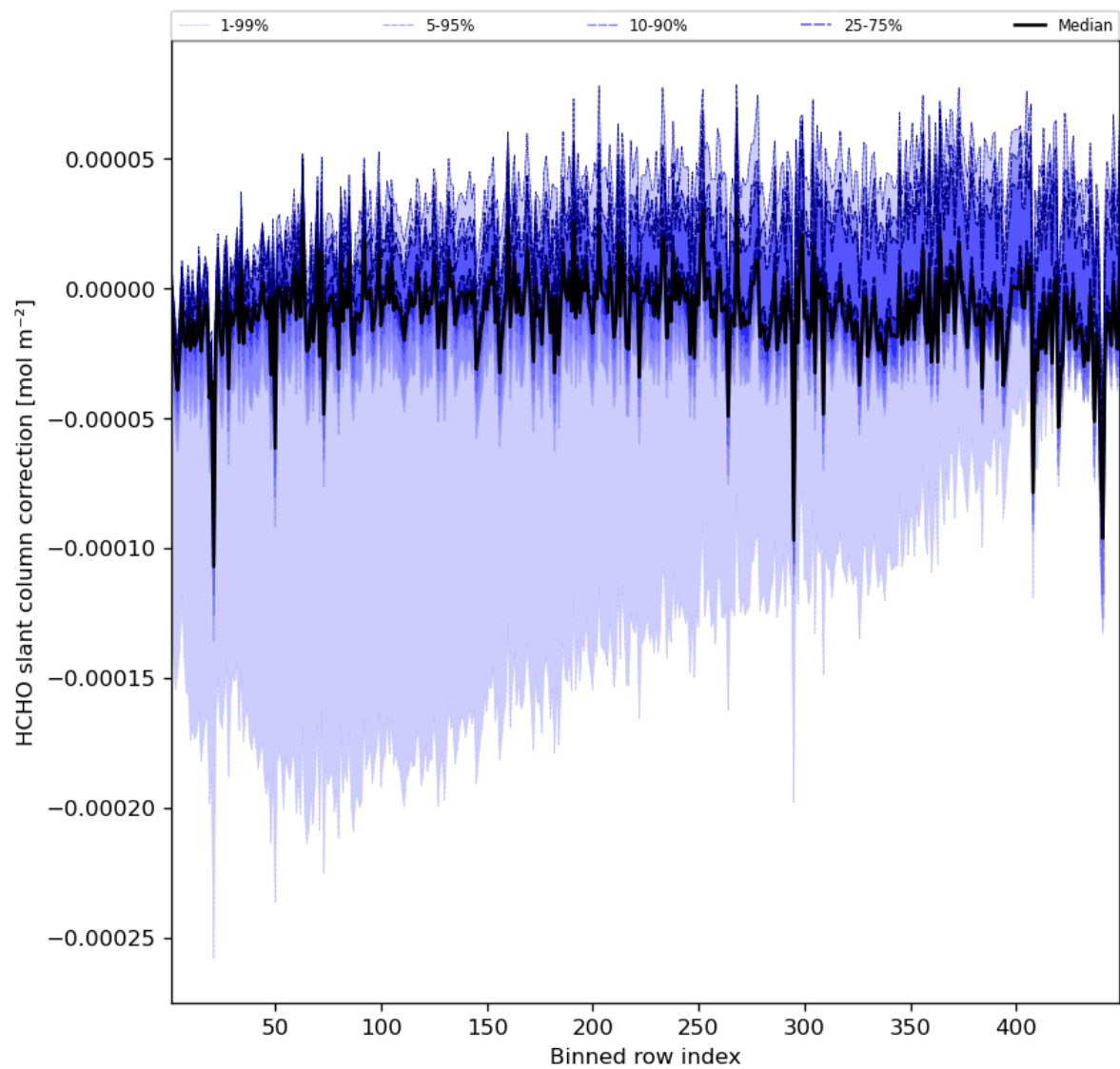
Figure 61: Along track statistics of “HCHO slant column correction” for 2023-07-03 to 2023-07-04
