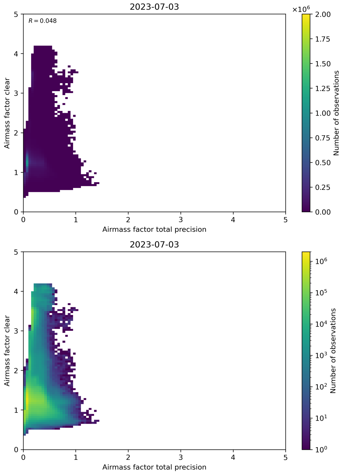
Figure 108: Scatter density plot of “Airmass factor total precision” against “Airmass factor clear” for 2023-07-03 to 2023-07-04.
