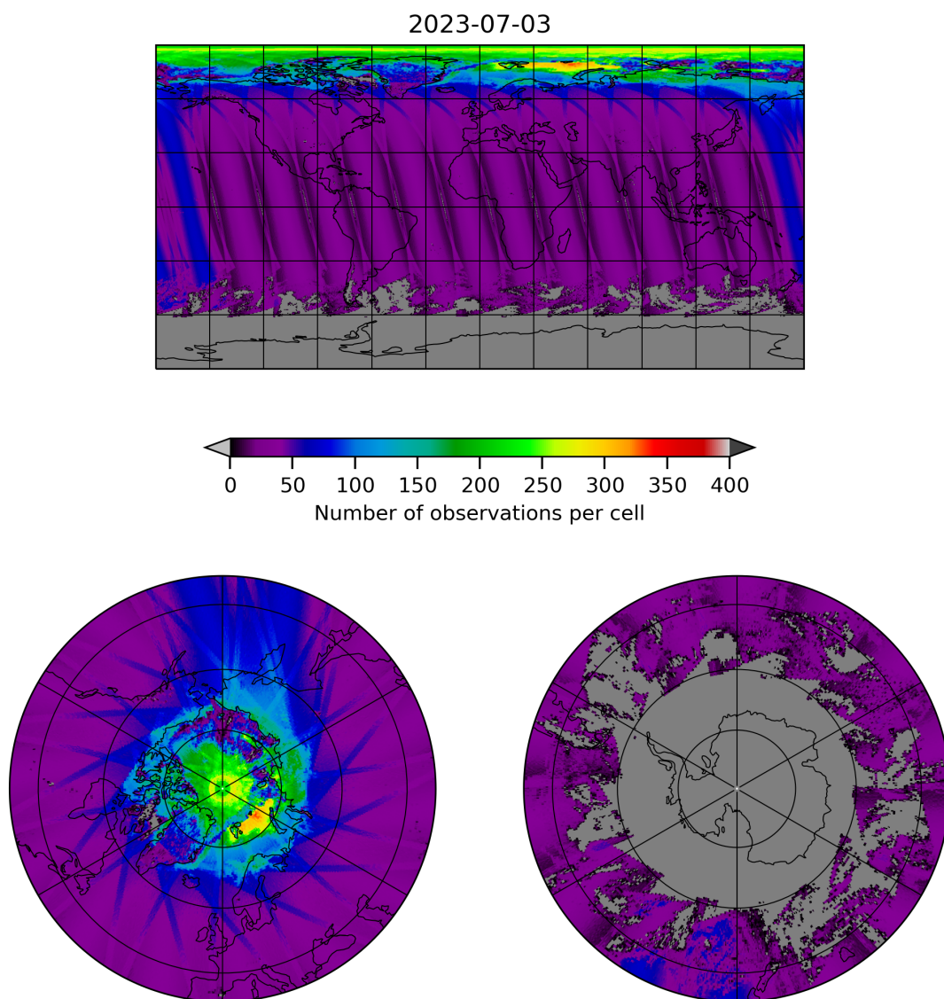
Figure 19: Map of the number of observations for 2023-07-03 to 2023-07-04
