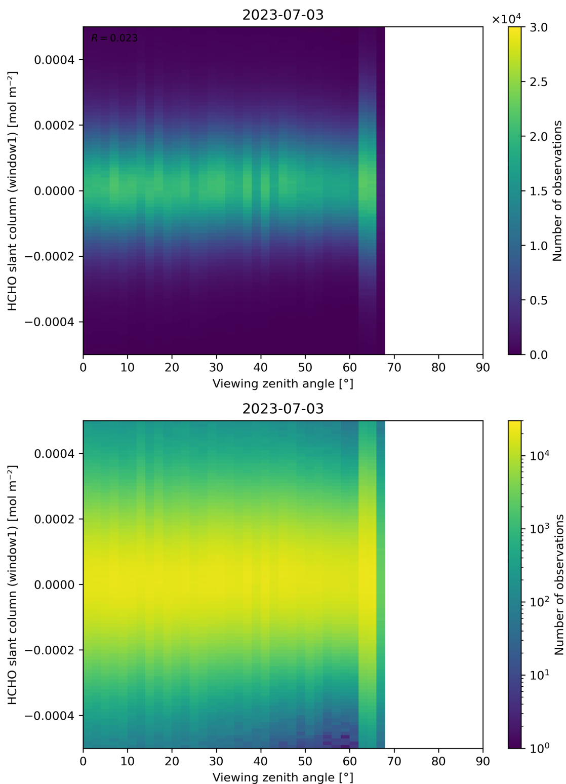
Figure 188: Scatter density plot of “Viewing zenith angle” against “HCHO slant column (window1)” for 2023-07-03 to 2023-07-04.
