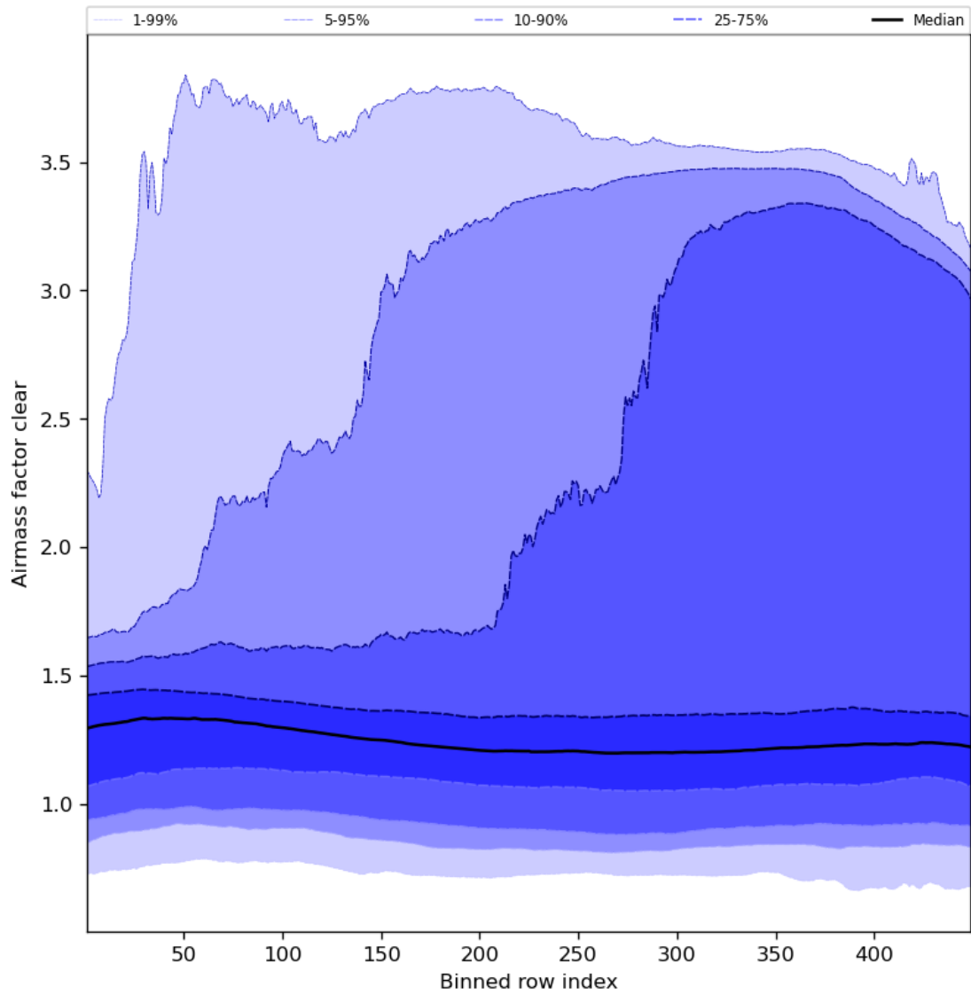
Figure 56: Along track statistics of “Airmass factor clear” for 2023-07-03 to 2023-07-04
