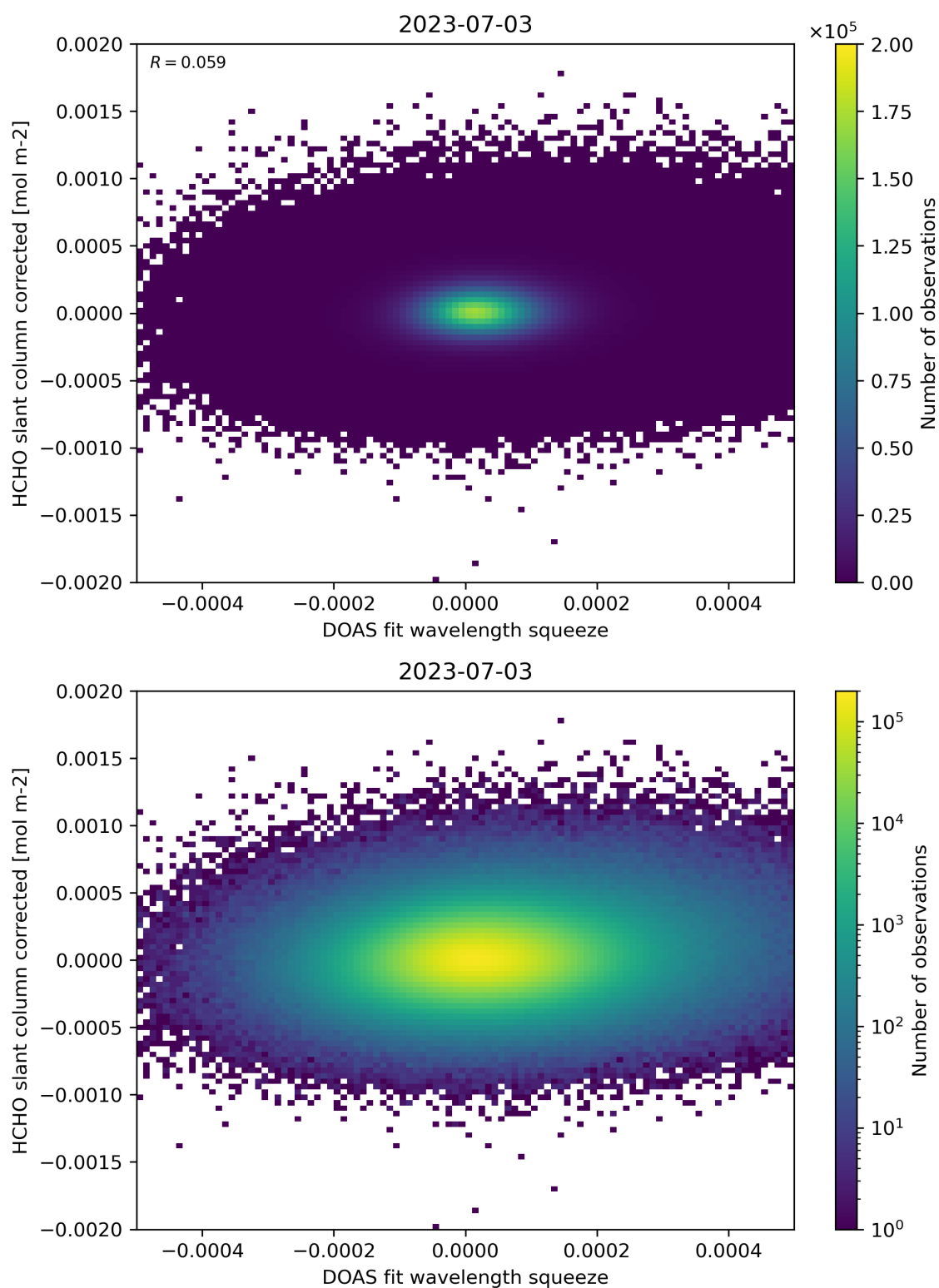
Figure 69: Scatter density plot of “DOAS fit wavelength squeeze” against “HCHO slant column corrected” for 2023-07-03 to 2023-07-04.
