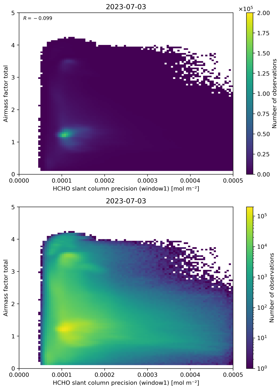
Figure 94: Scatter density plot of “HCHO slant column precision (window1)” against “Airmass factor total” for 2023-07-03 to 2023-07-04.
