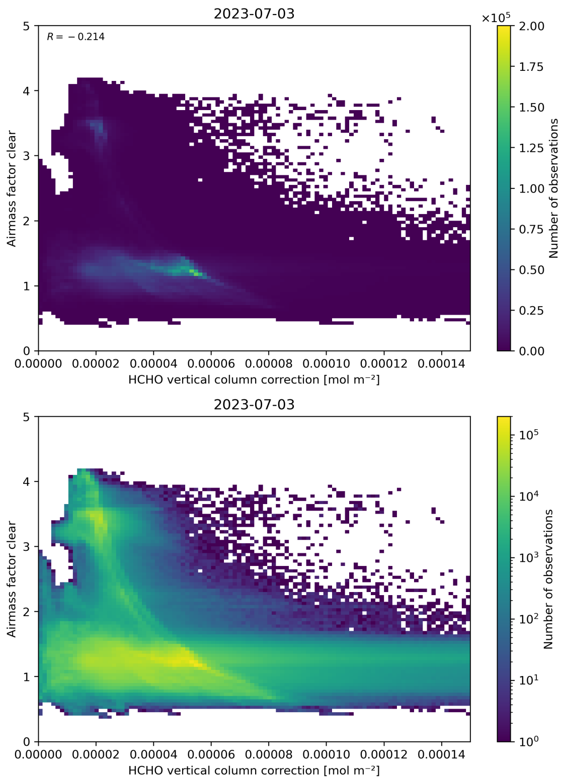
Figure 115: Scatter density plot of “HCHO vertical column correction” against “Air mass factor clear” for 2023-07-03 to 2023-07-04.
