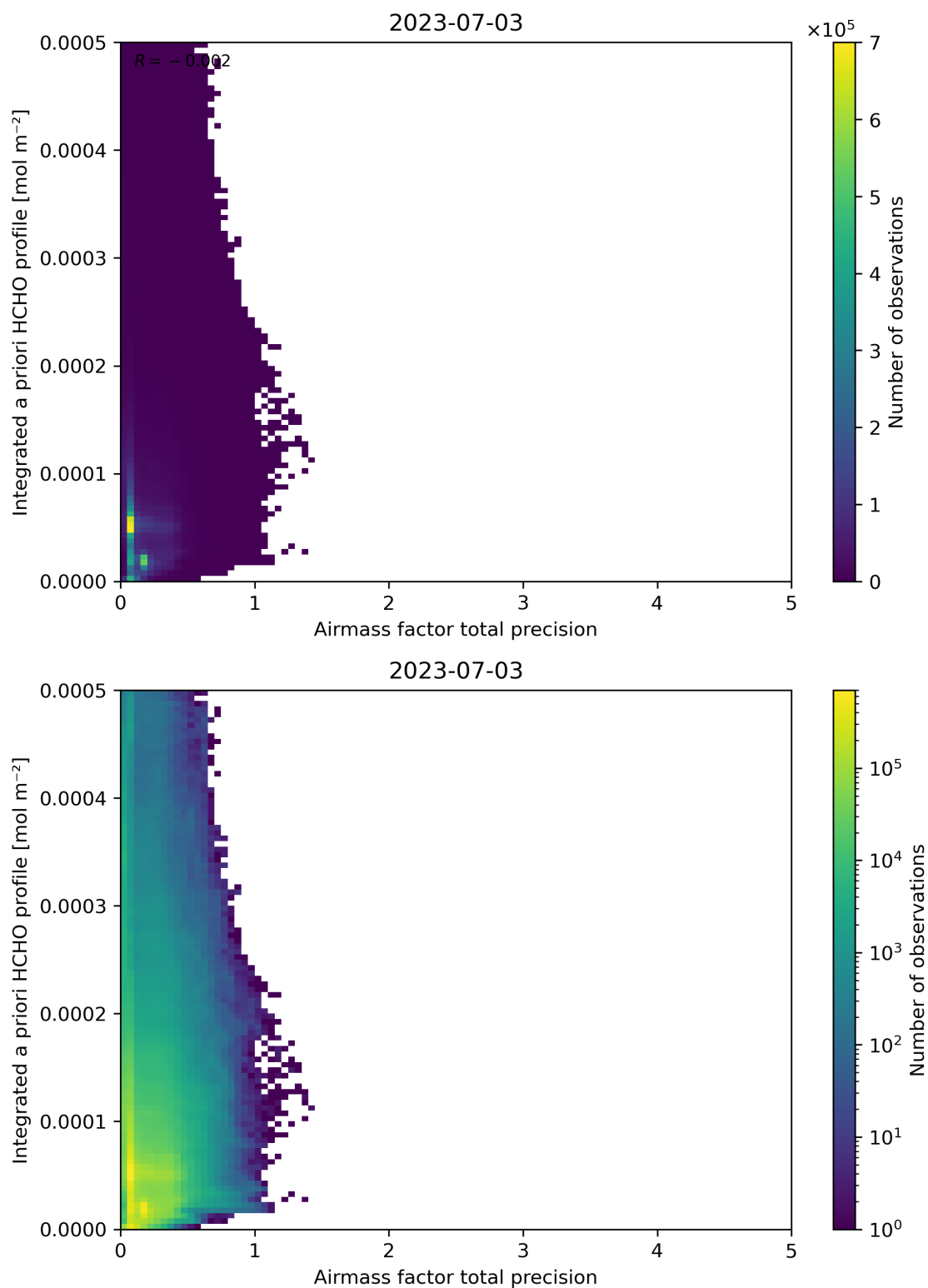
Figure 111: Scatter density plot of “Airmass factor total precision” against “Integrated a priori HCHO profile” for 2023-07-03 to 2023-07-04.
