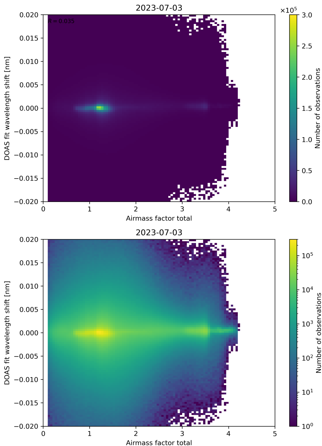
Figure 98: Scatter density plot of “Airmass factor total” against “DOAS fit wavelength shift” for 2023-07-03 to 2023-07-04.
