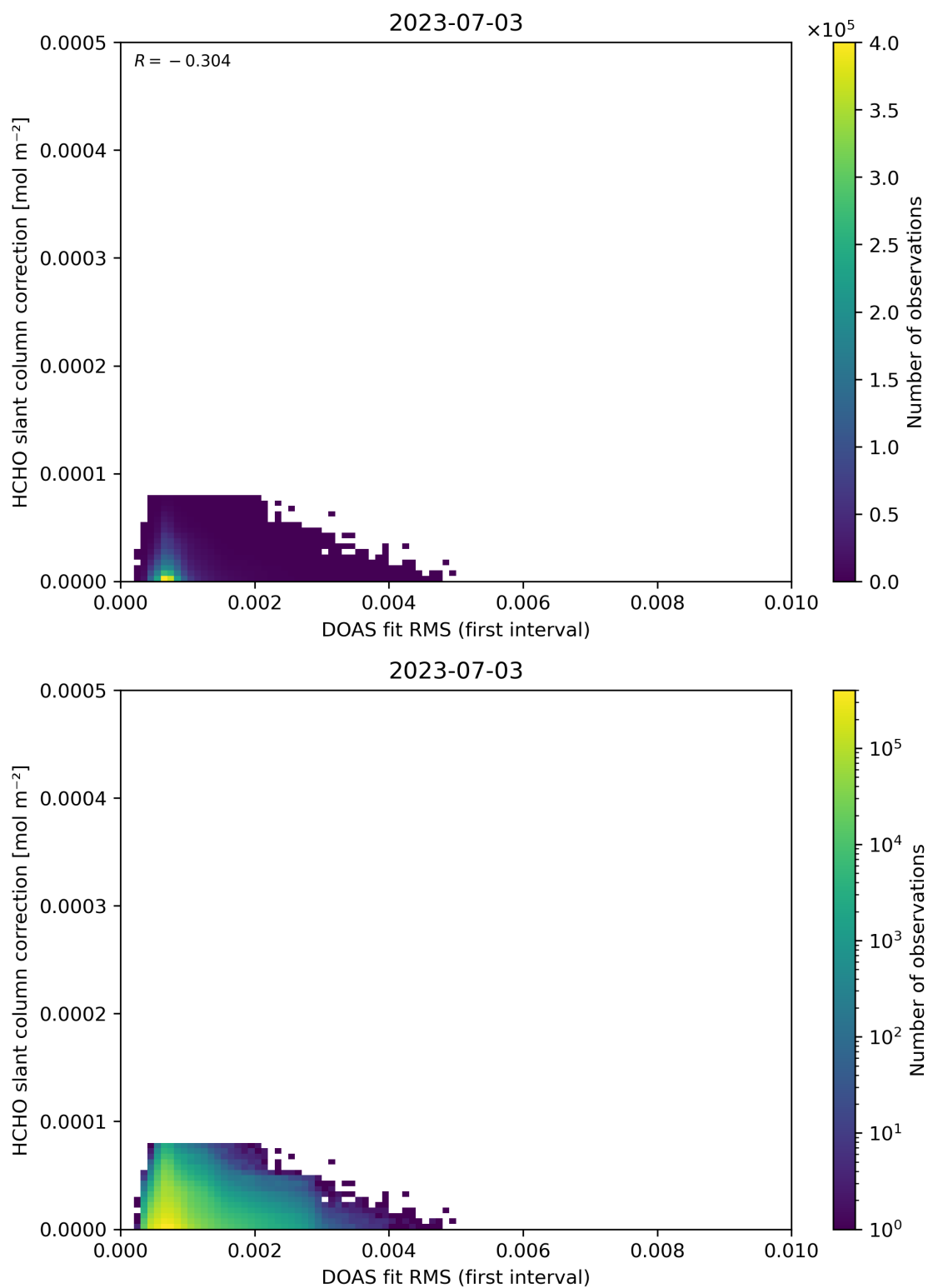
Figure 63: Scatter density plot of “DOAS fit RMS (first interval)” against “HCHO slant column correction” for 2023-07-03 to 2023-07-04.
