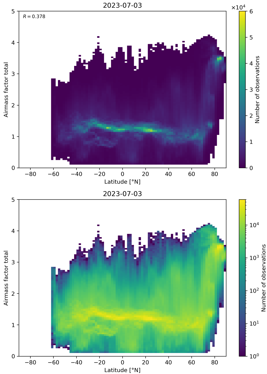
Figure 161: Scatter density plot of “Latitude” against “Airmass factor total” for 2023-07-03 to 2023-07-04.
