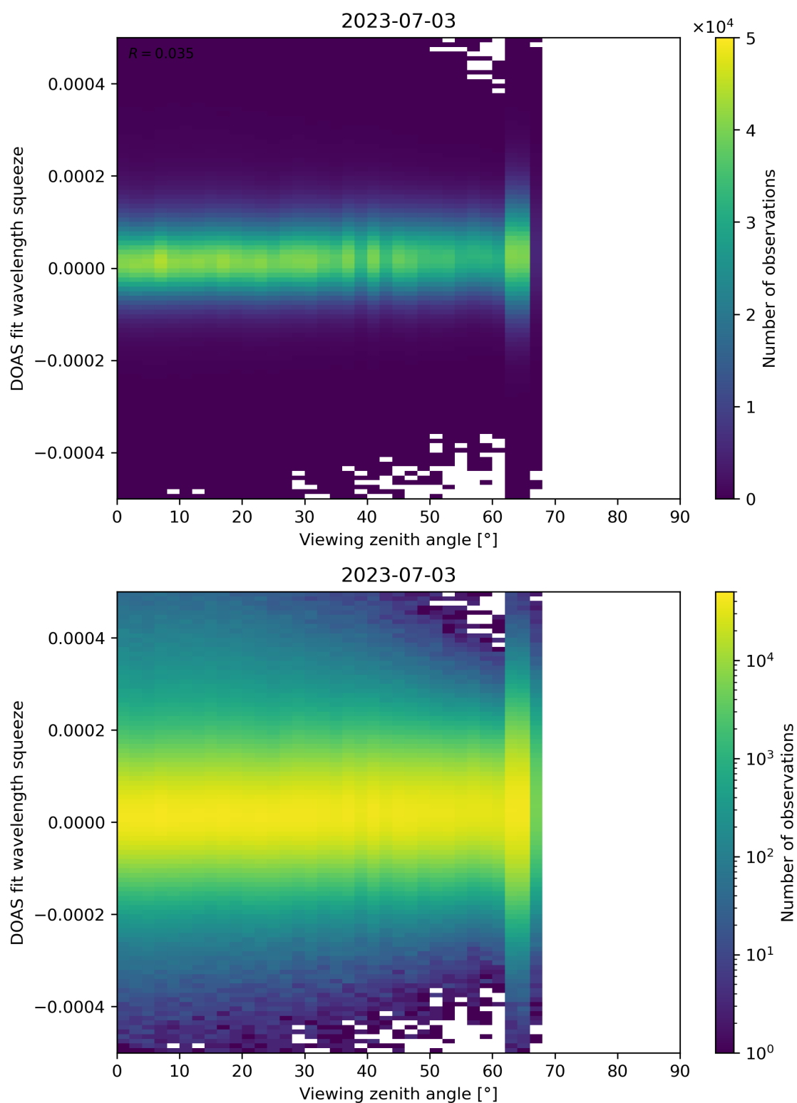
Figure 184: Scatter density plot of “Viewing zenith angle” against “DOAS fit wavelength squeeze” for 2023-07-03 to 2023-07-04.
