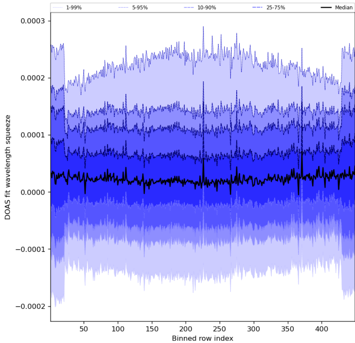
Figure 59: Along track statistics of “DOAS fit wavelength squeeze” for 2023-07-03 to 2023-07-04
