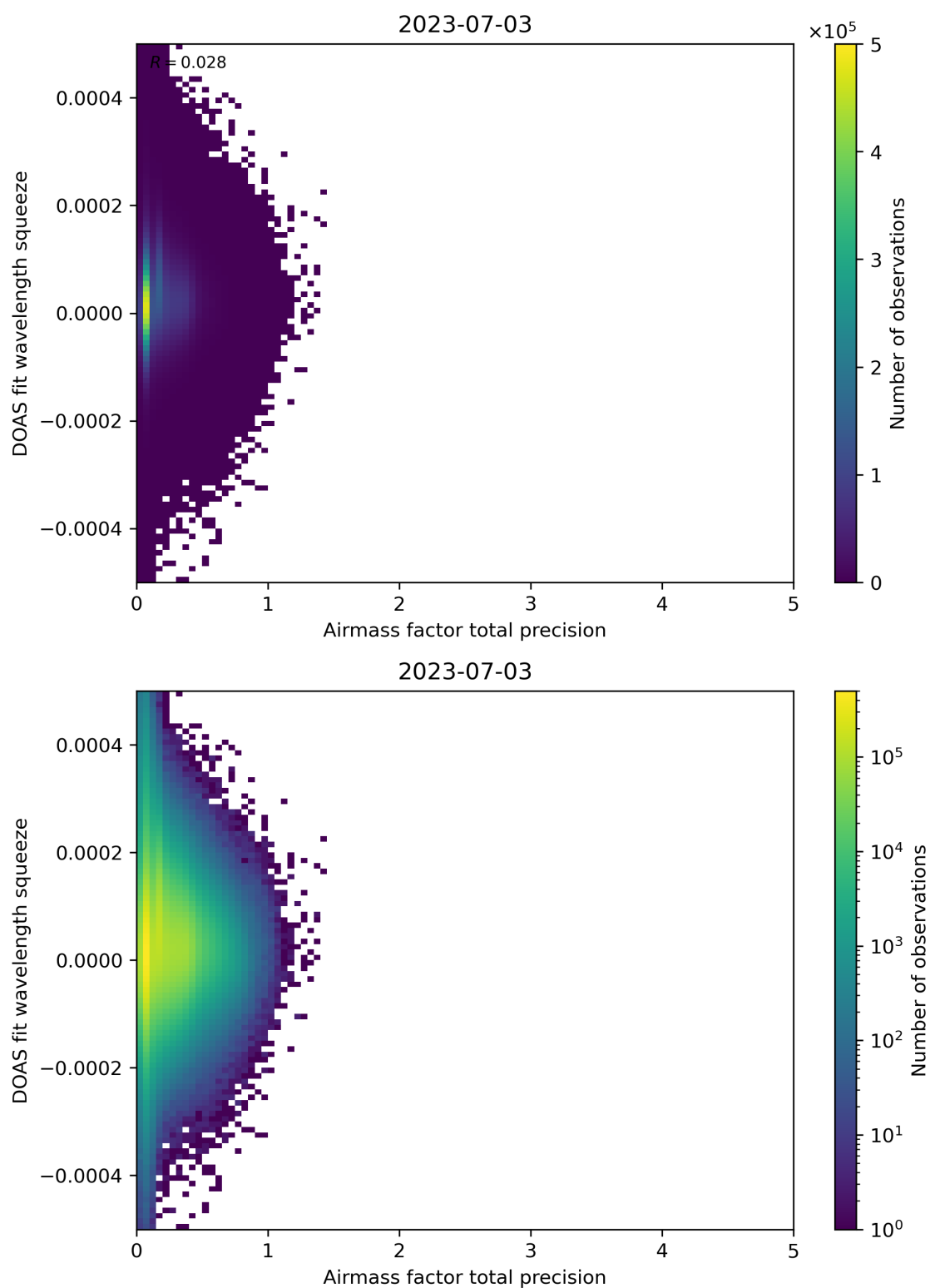
Figure 107: Scatter density plot of “Airmass factor total precision” against “DOAS fit wavelength squeeze” for 2023-07-03 to 2023-07-04.
