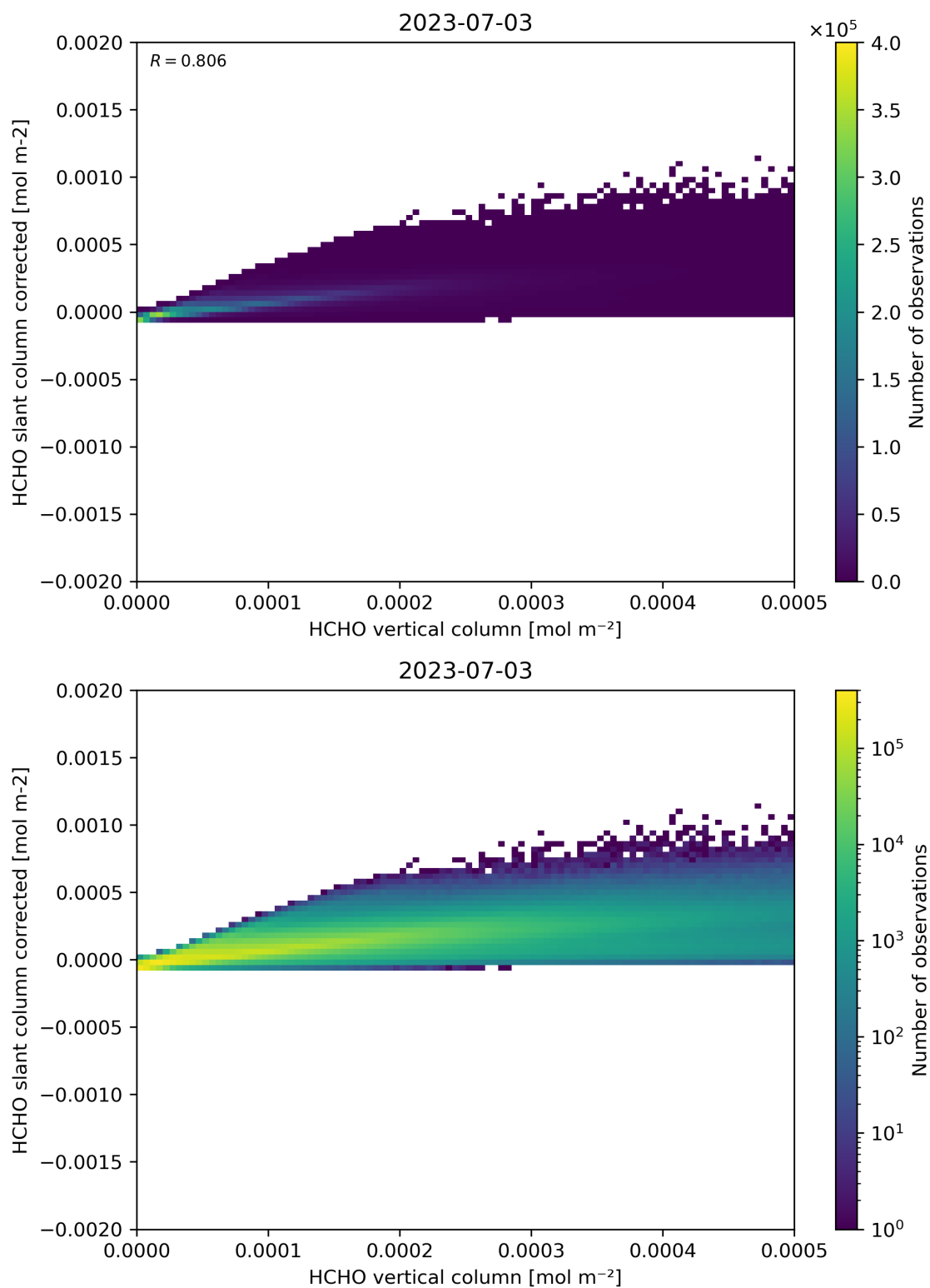
Figure 127: Scatter density plot of “HCHO vertical column” against “HCHO slant column corrected” for 2023-07-03 to 2023-07-04.
