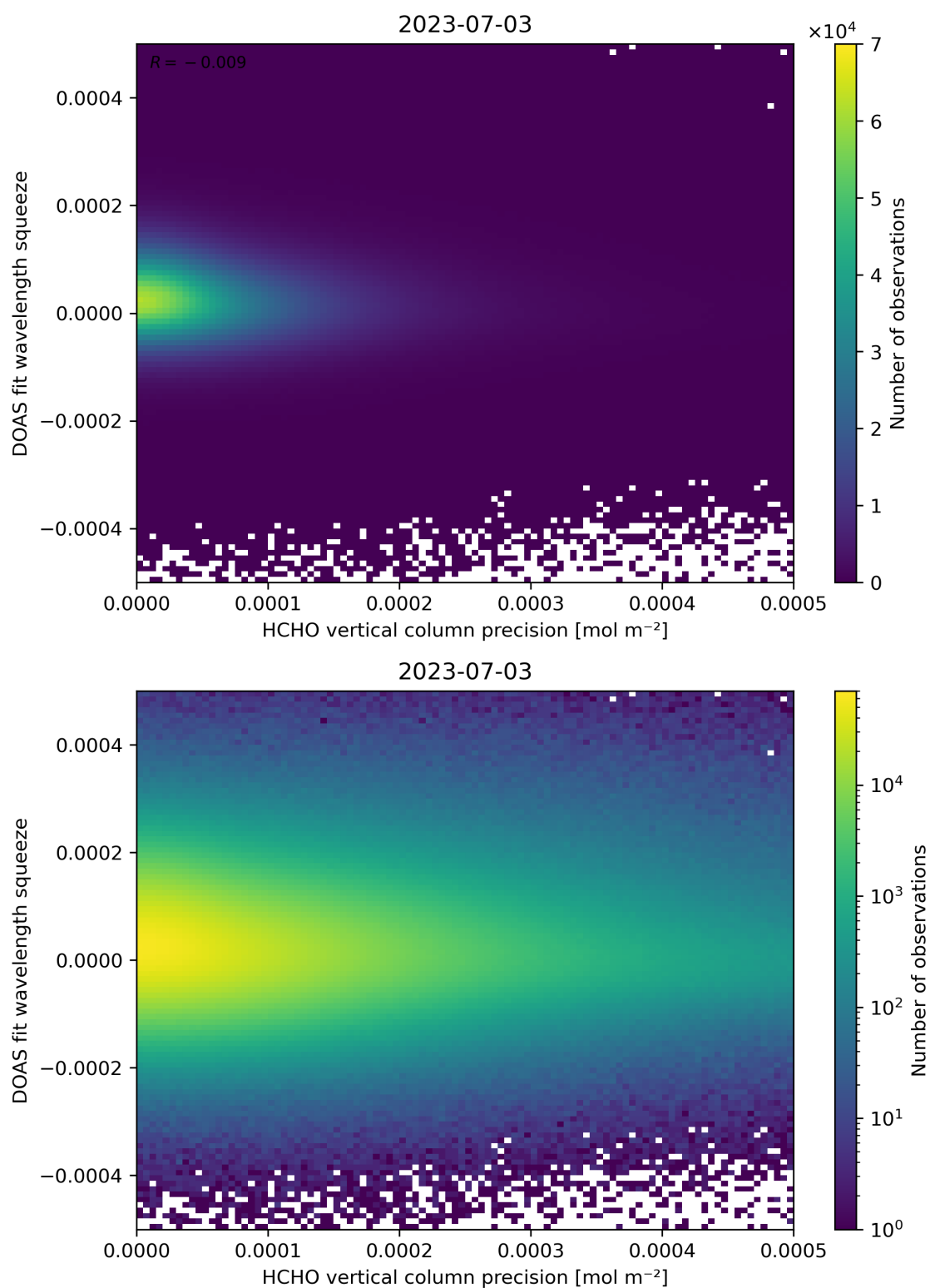
Figure 138: Scatter density plot of “HCHO vertical column precision” against “DOAS fit wavelength squeeze” for 2023-07-03 to 2023-07-04.
