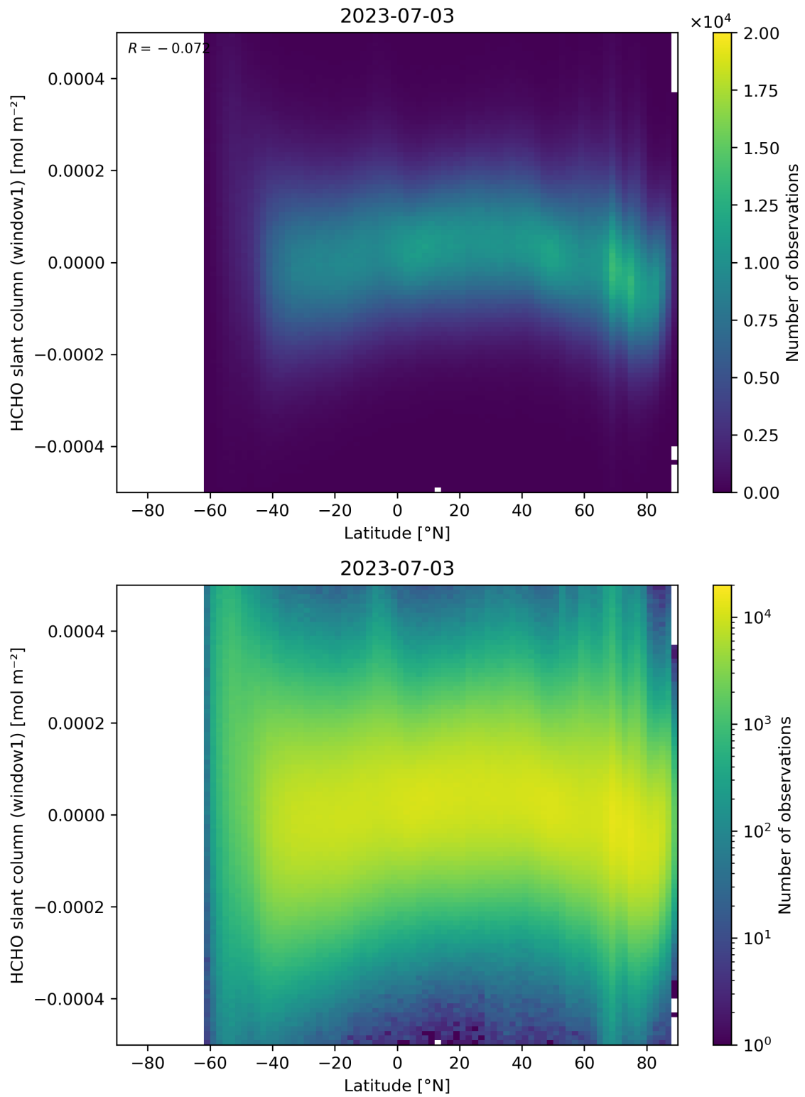
Figure 159: Scatter density plot of “Latitude” against “HCHO slant column (window1)” for 2023-07-03 to 2023-07-04.
