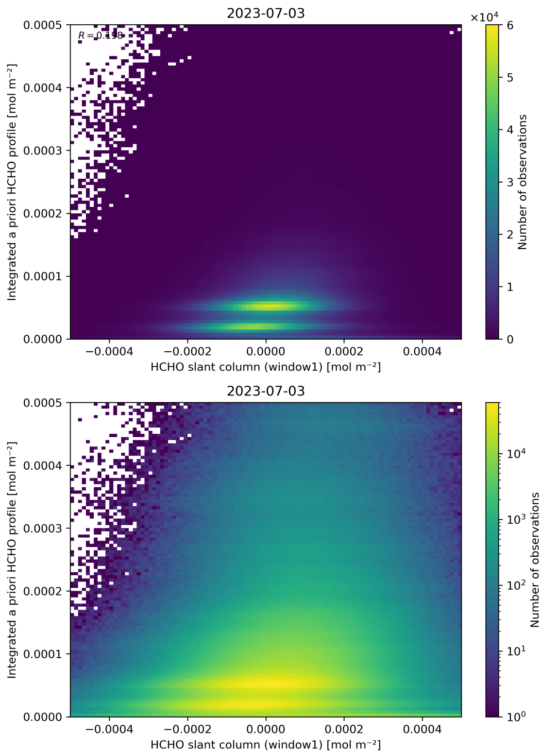
Figure 87: Scatter density plot of “HCHO slant column (window1)” against “Integrated a priori HCHO profile” for 2023-07-03 to 2023-07-04.
