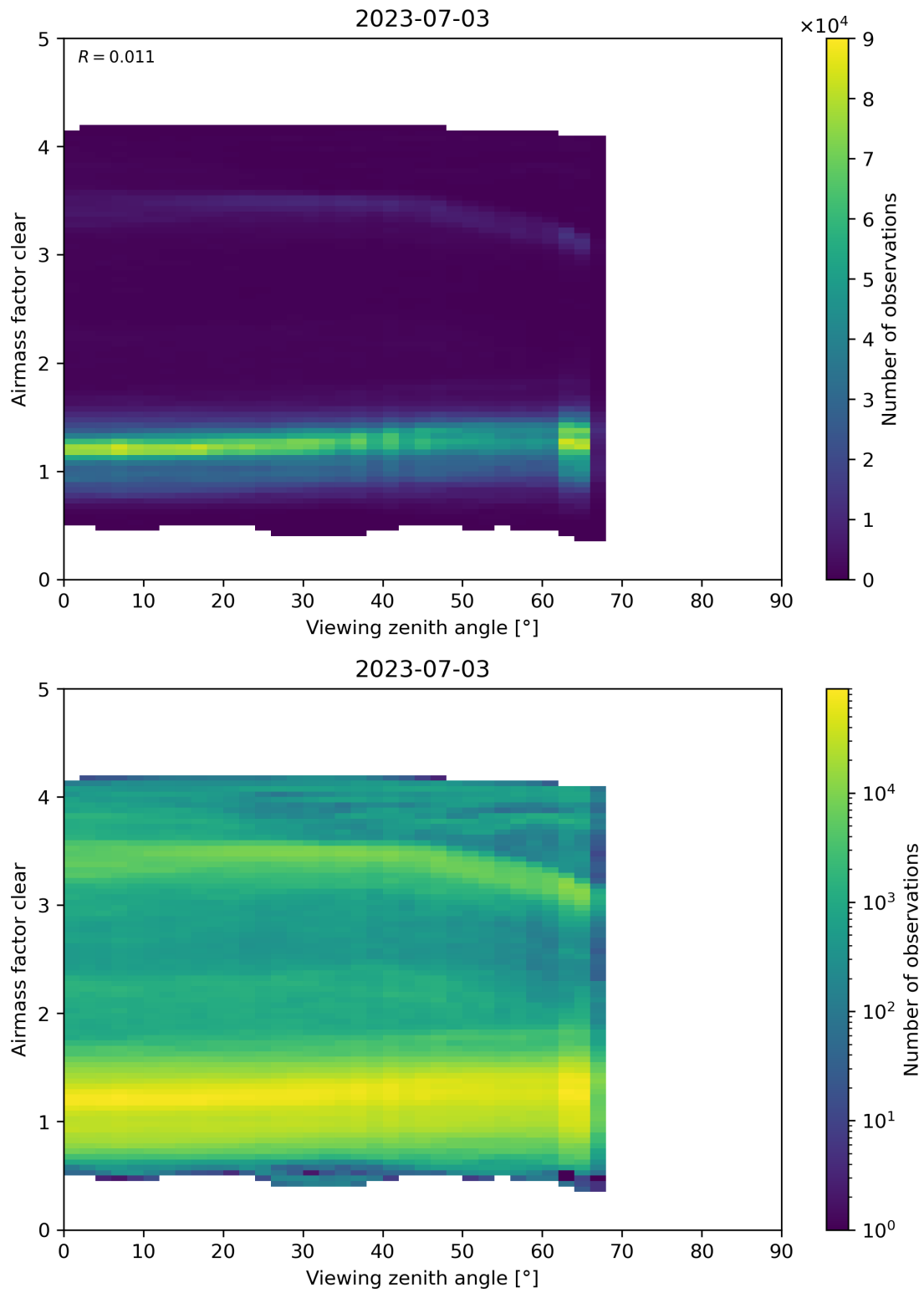
Figure 185: Scatter density plot of “Viewing zenith angle” against “Airmass factor clear” for 2023-07-03 to 2023-07-04.
