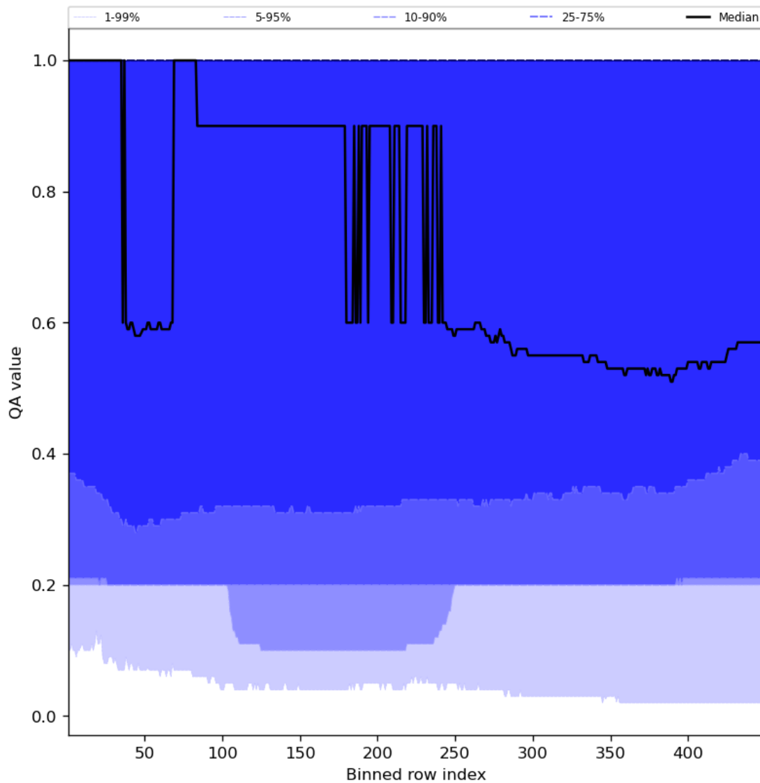
Figure 48: Along track statistics of “QA value” for 2023-07-03 to 2023-07-04
