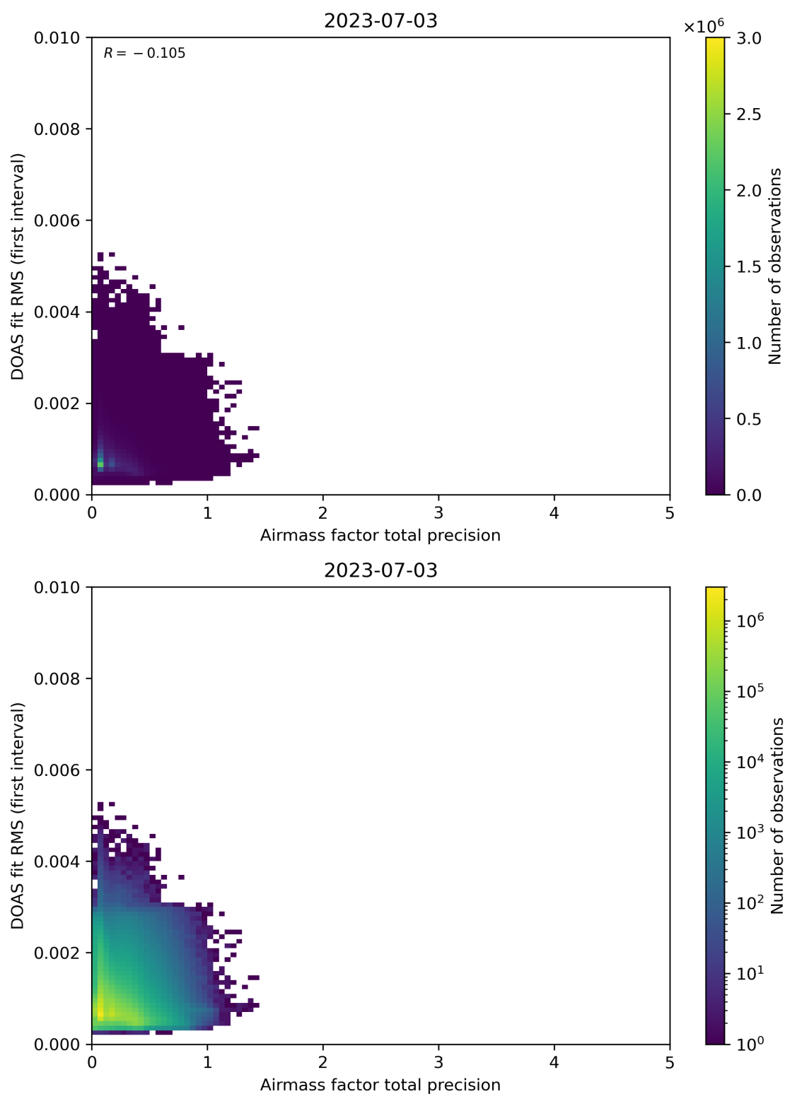
Figure 105: Scatter density plot of “Airmass factor total precision” against “DOAS fit RMS (first interval)” for 2023-07-03 to 2023-07-04.
