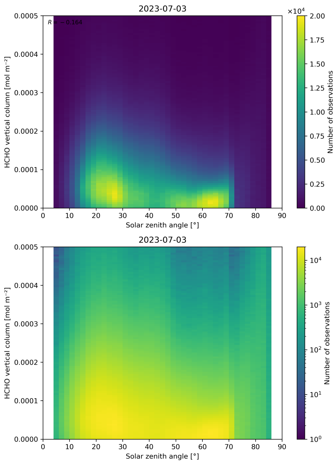
Figure 177: Scatter density plot of “Solar zenith angle” against “HCHO vertical column” for 2023-07-03 to 2023-07-04.
