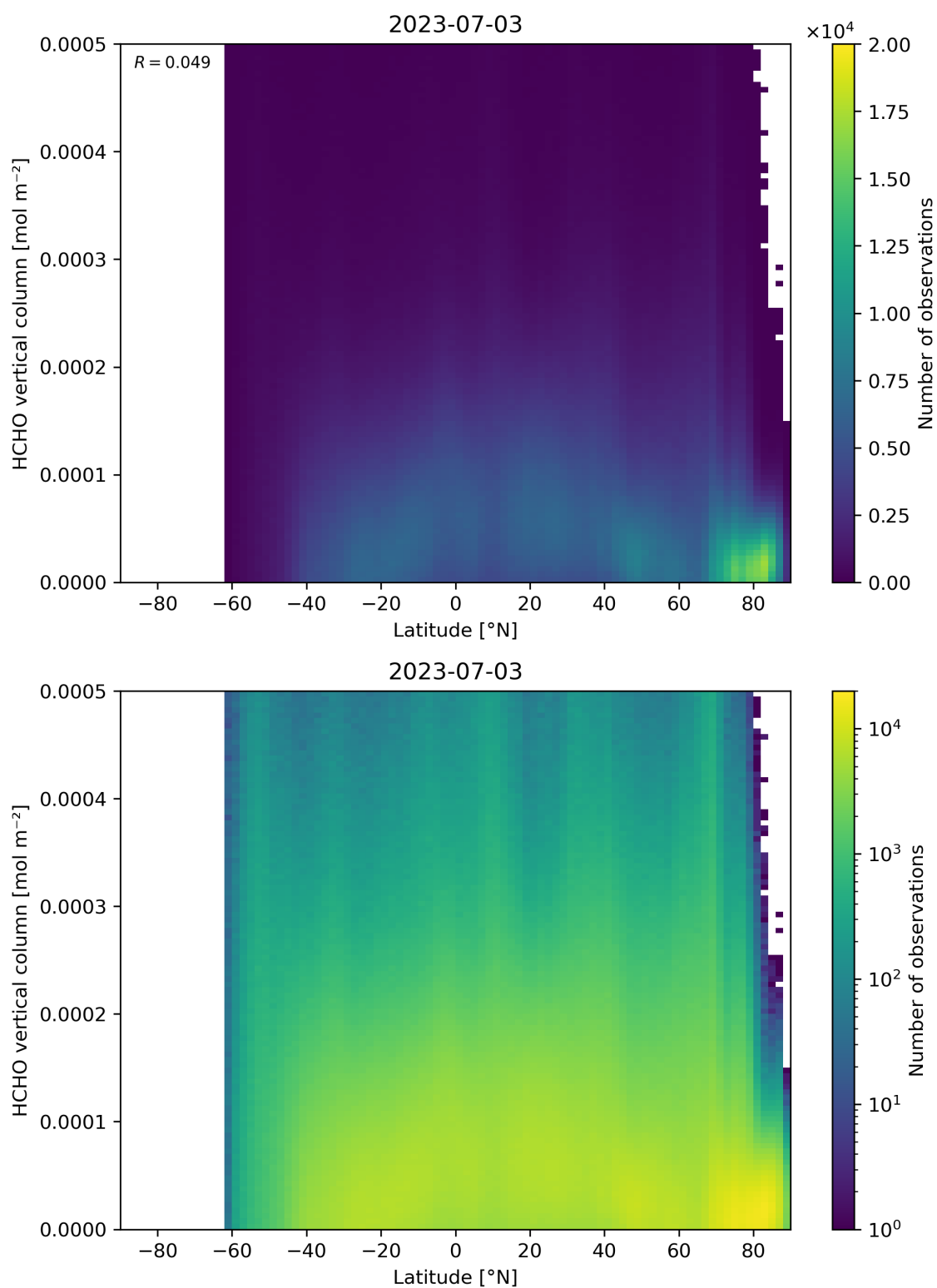
Figure 163: Scatter density plot of “Latitude” against “HCHO vertical column” for 2023-07-03 to 2023-07-04.
