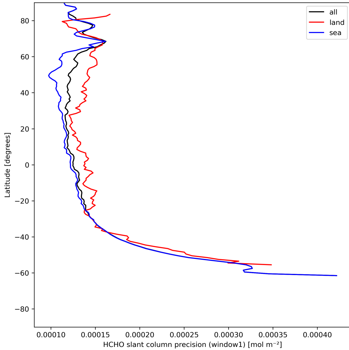
Figure 25: Zonal average of "HCHO slant column precision (window1)" for 2023-07-03 to 2023-07-04.
