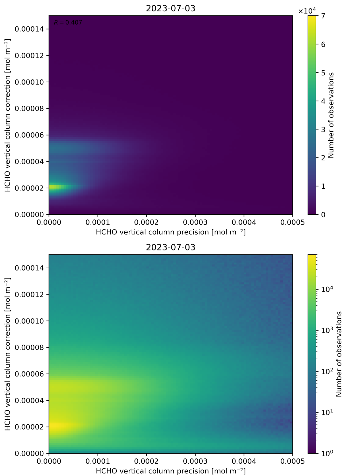
Figure 146: Scatter density plot of “HCHO vertical column precision” against “HCHO vertical column correction” for 2023-07-03 to 2023-07-04.
