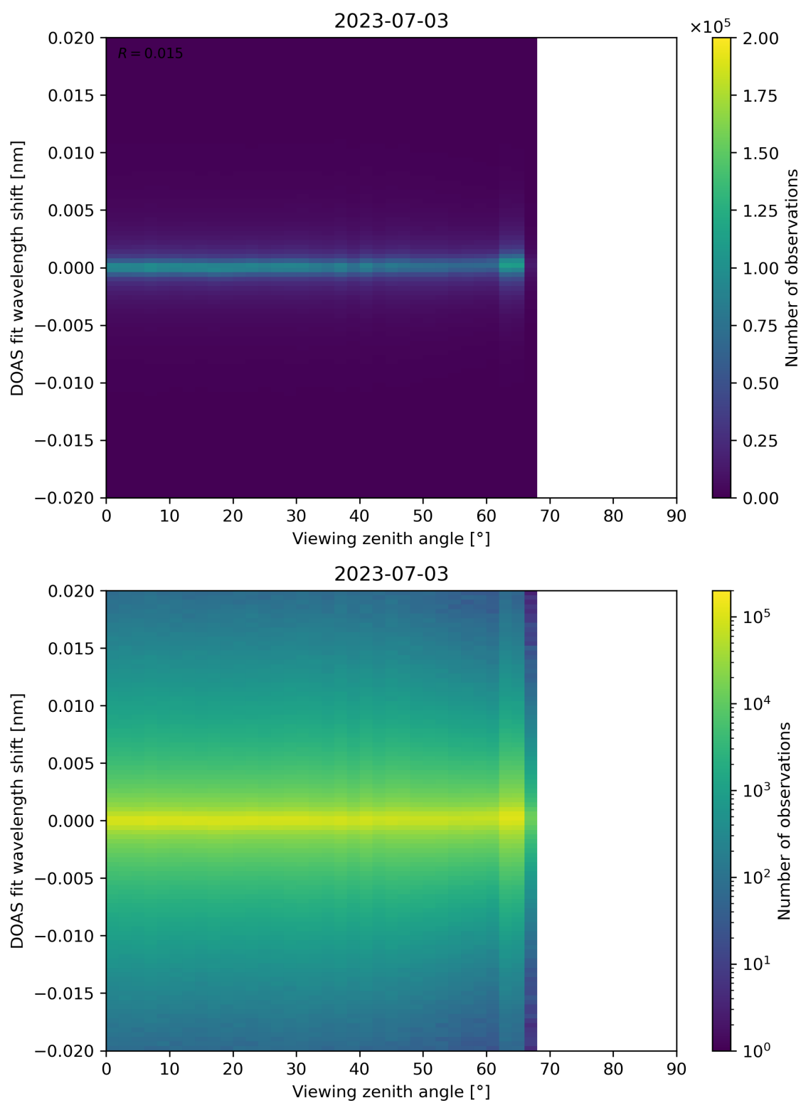
Figure 183: Scatter density plot of “Viewing zenith angle” against “DOAS fit wavelength shift” for 2023-07-03 to 2023-07-04.
