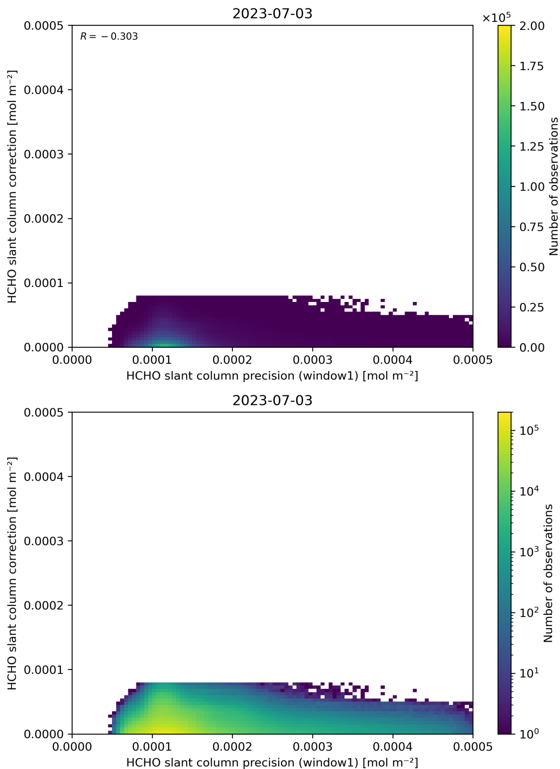
Figure 93: Scatter density plot of “HCHO slant column precision (window1)” against “HCHO slant column correction” for 2023-07-03 to 2023-07-04.
