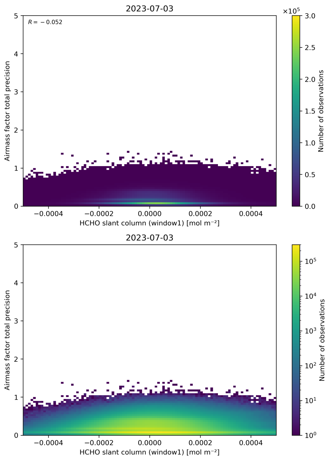
Figure 86: Scatter density plot of “HCHO slant column (window1)” against “Air mass factor total precision” for 2023-07-03 to 2023-07-04.
