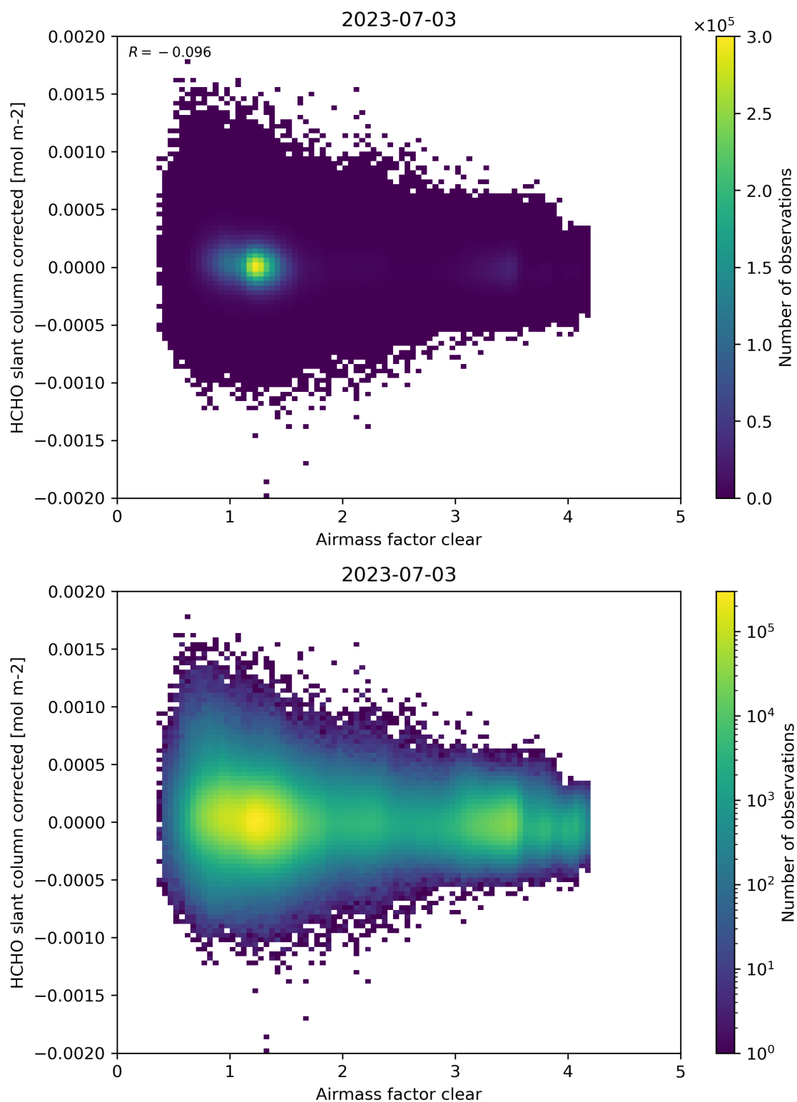
Figure 74: Scatter density plot of “Airmass factor clear” against “HCHO slant column corrected” for 2023-07-03 to 2023-07-04.
