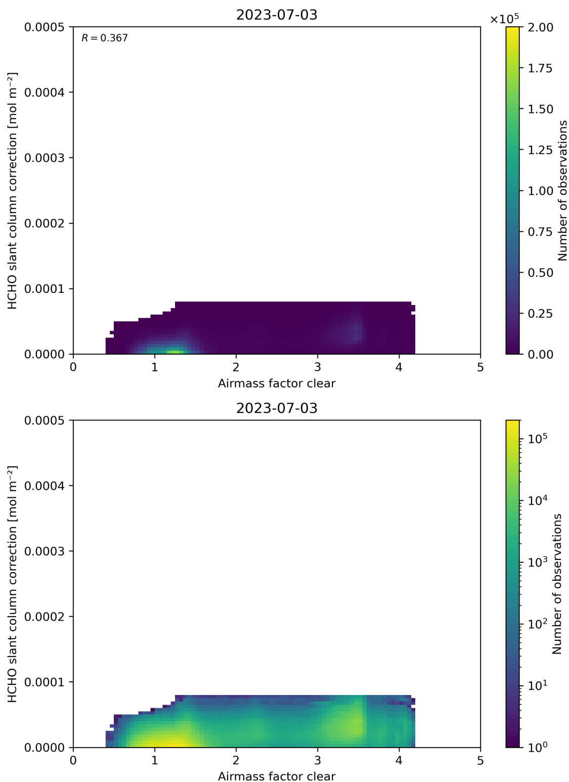
Figure 75: Scatter density plot of “Airmass factor clear” against “HCHO slant column correction” for 2023-07-03 to 2023-07-04.
