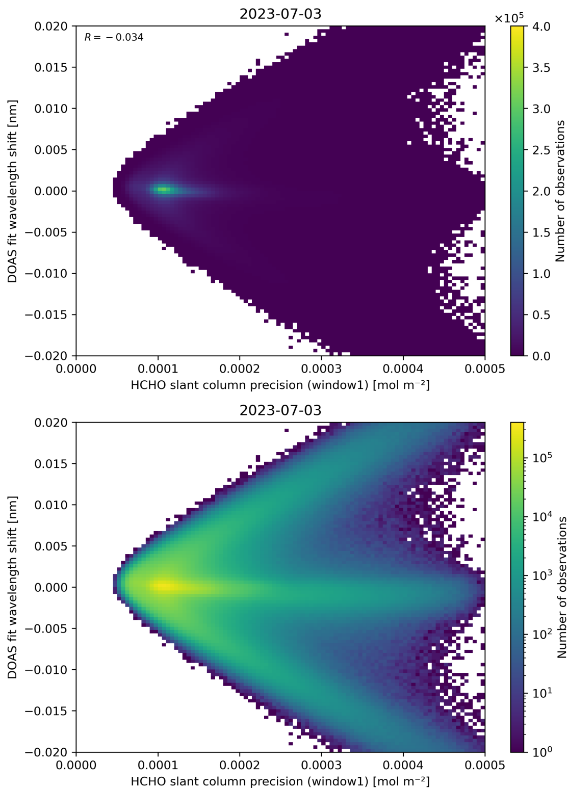
Figure 89: Scatter density plot of “HCHO slant column precision (window1)” against “DOAS fit wavelength shift” for 2023-07-03 to 2023-07-04.
