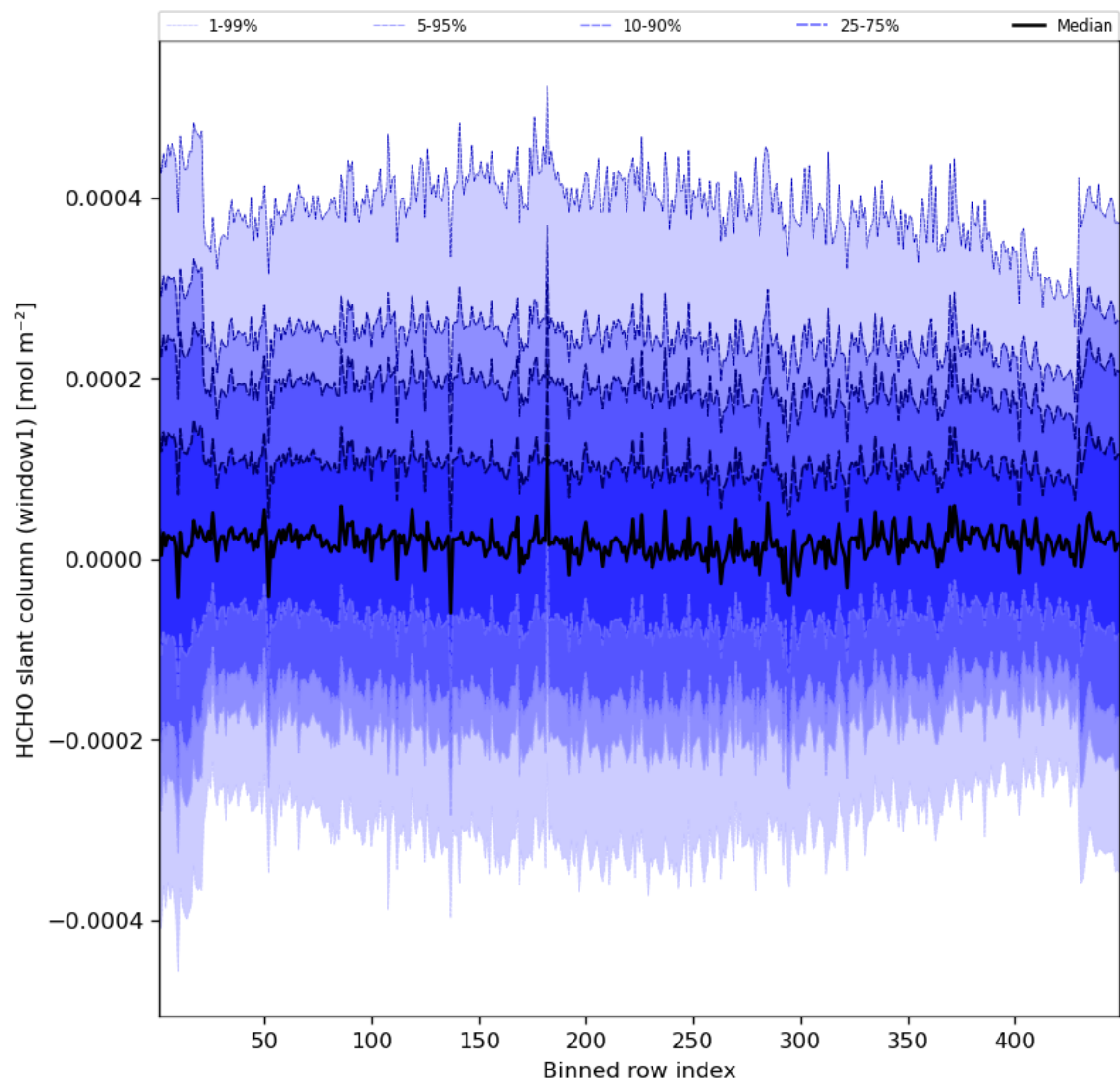
Figure 52: Along track statistics of “HCHO slant column (window1)” for 2023-07-03 to 2023-07-04
