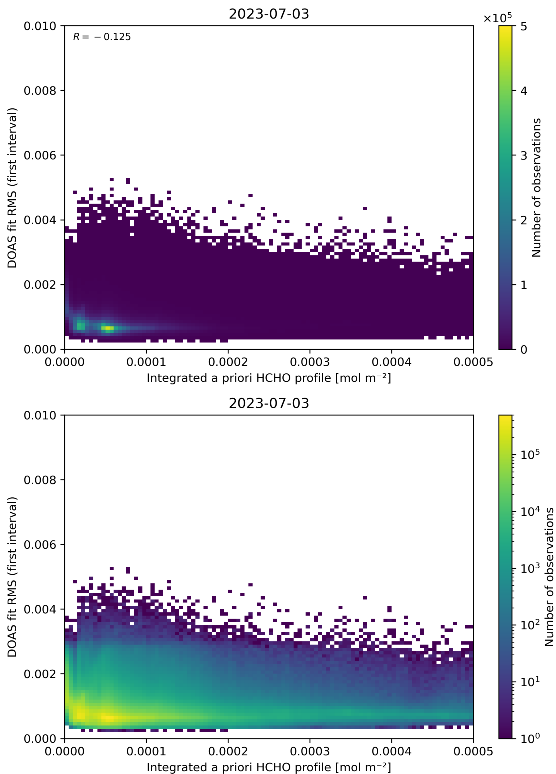
Figure 148: Scatter density plot of “Integrated a priori HCHO profile” against “DOAS fit RMS (first interval)” for 2023-07-03 to 2023-07-04.
