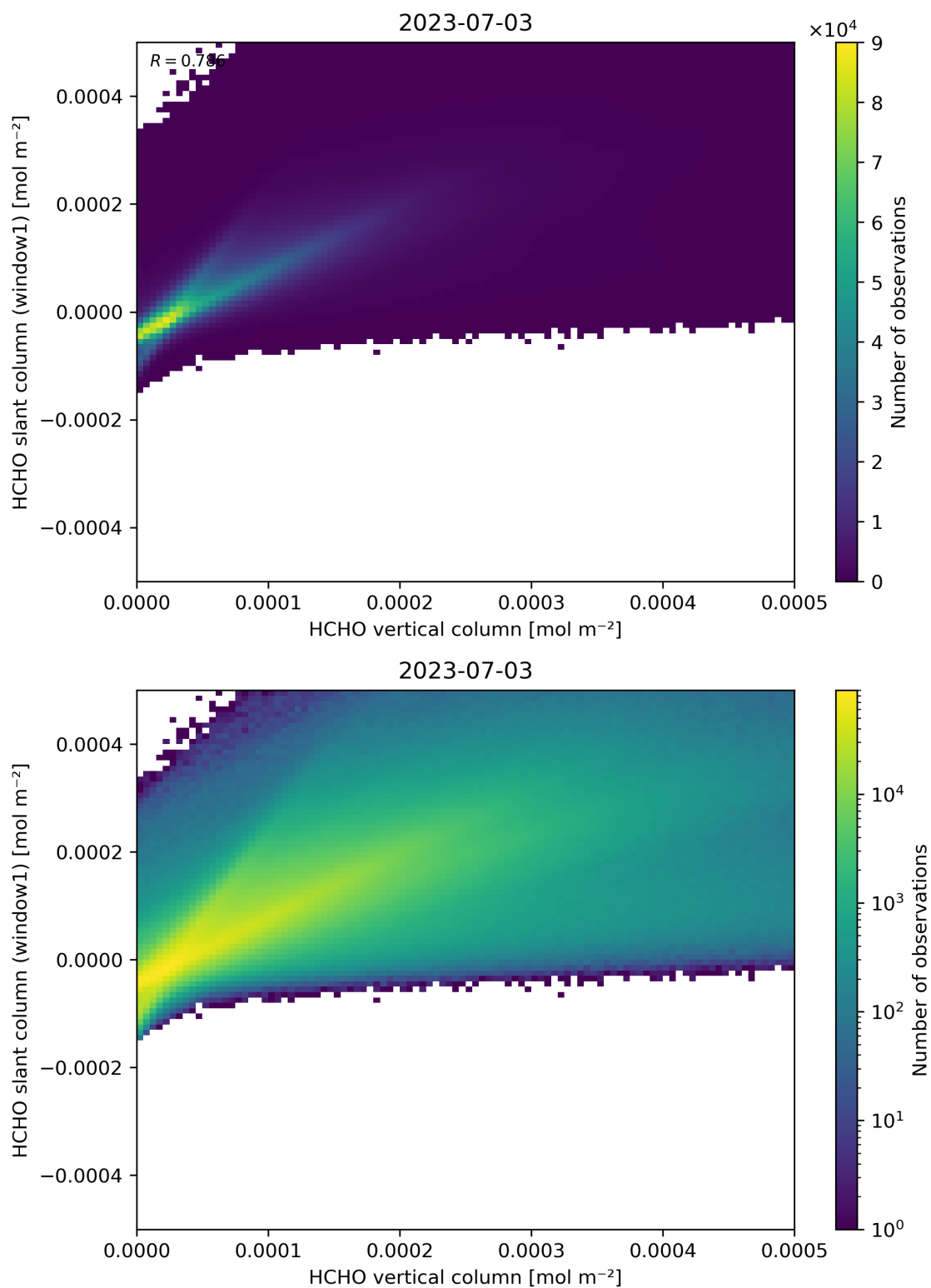
Figure 129: Scatter density plot of “HCHO vertical column” against “HCHO slant column (window1)” for 2023-07-03 to 2023-07-04.
