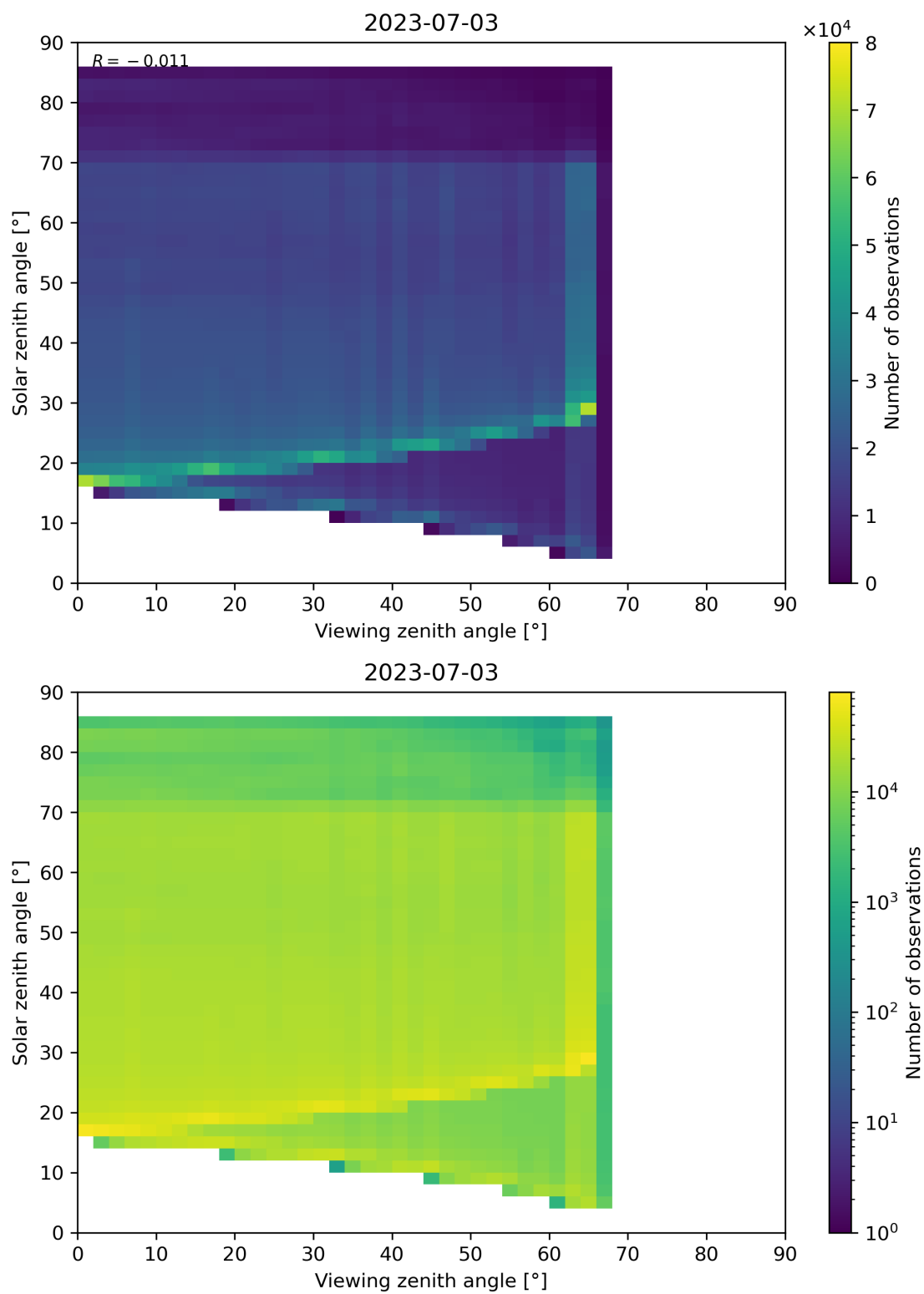
Figure 197: Scatter density plot of “Viewing zenith angle” against “Solar zenith angle” for 2023-07-03 to 2023-07-04.
