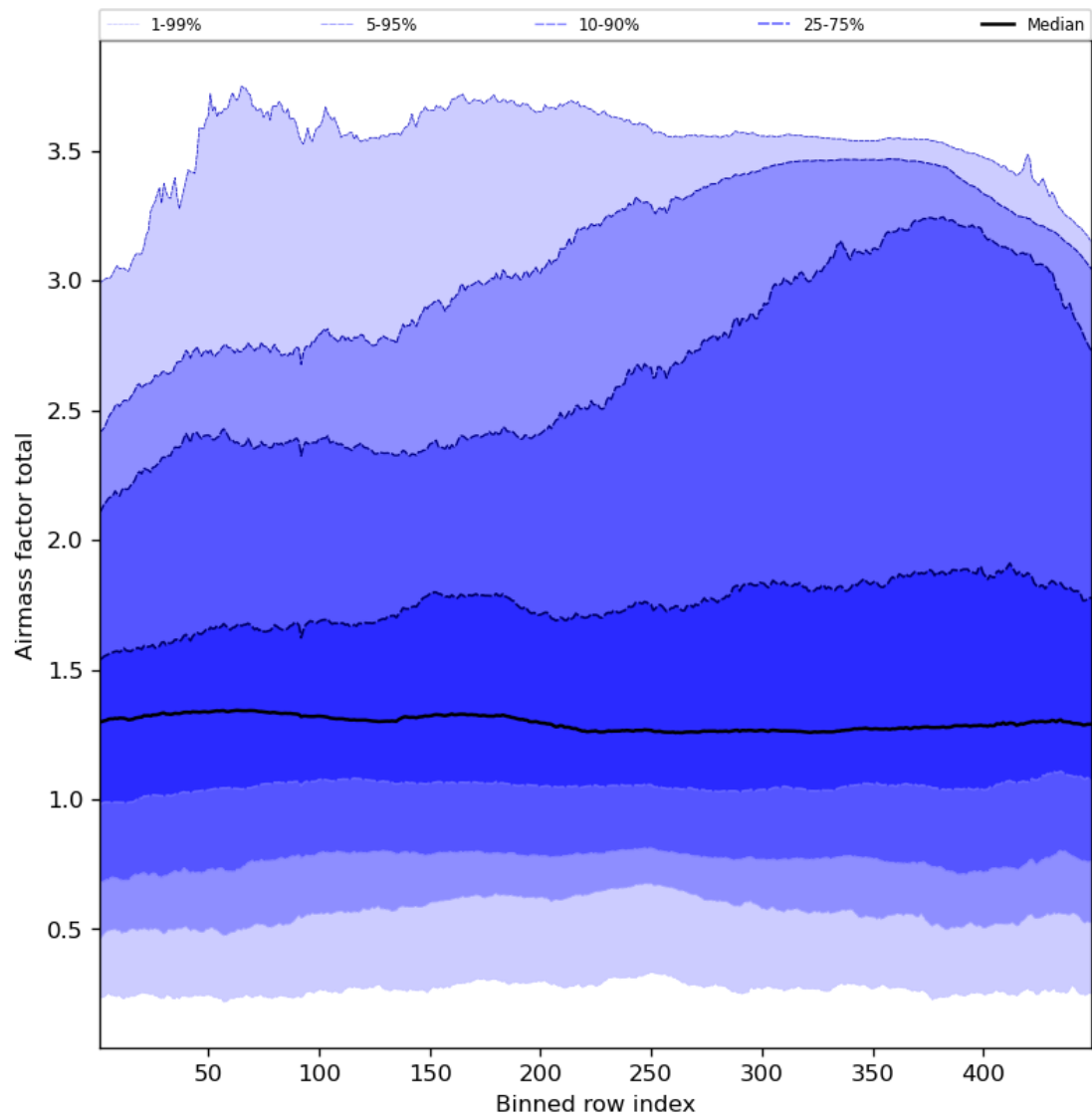
Figure 54: Along track statistics of “Airmass factor total” for 2023-07-03 to 2023-07-04
