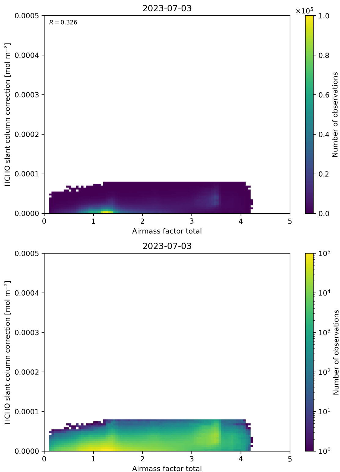
Figure 102: Scatter density plot of “Airmass factor total” against “HCHO slant column correction” for 2023-07-03 to 2023-07-04.
