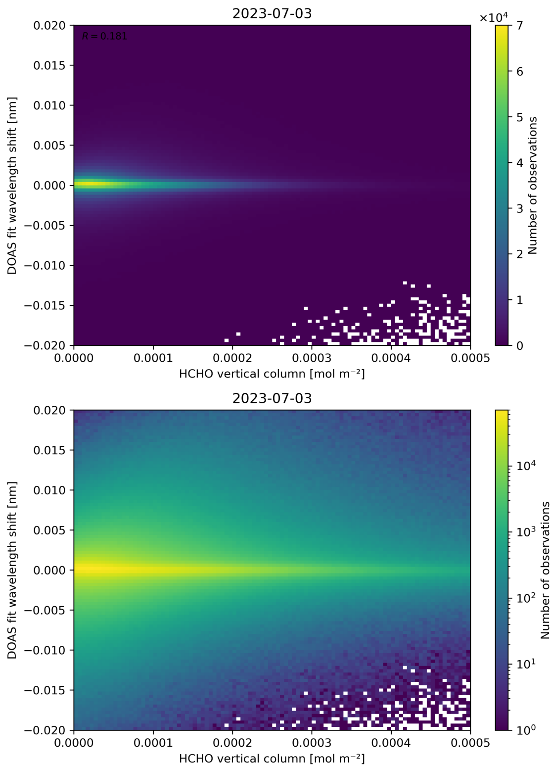
Figure 124: Scatter density plot of “HCHO vertical column” against “DOAS fit wavelength shift” for 2023-07-03 to 2023-07-04.
