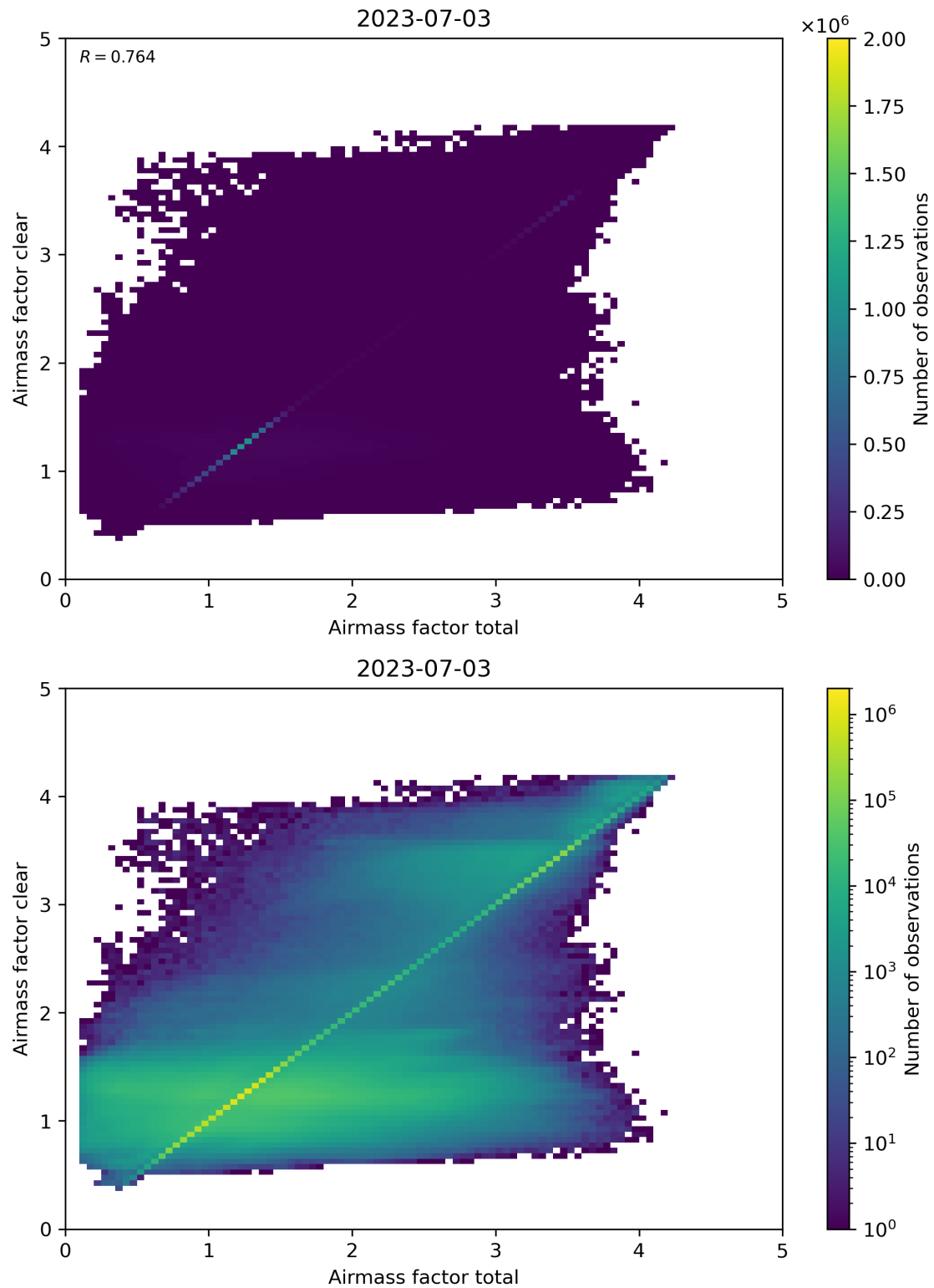
Figure 100: Scatter density plot of “Airmass factor total” against “Airmass factor clear” for 2023-07-03 to 2023-07-04.
