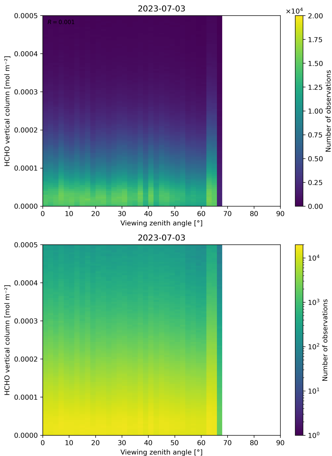
Figure 192: Scatter density plot of “Viewing zenith angle” against “HCHO vertical column” for 2023-07-03 to 2023-07-04.
