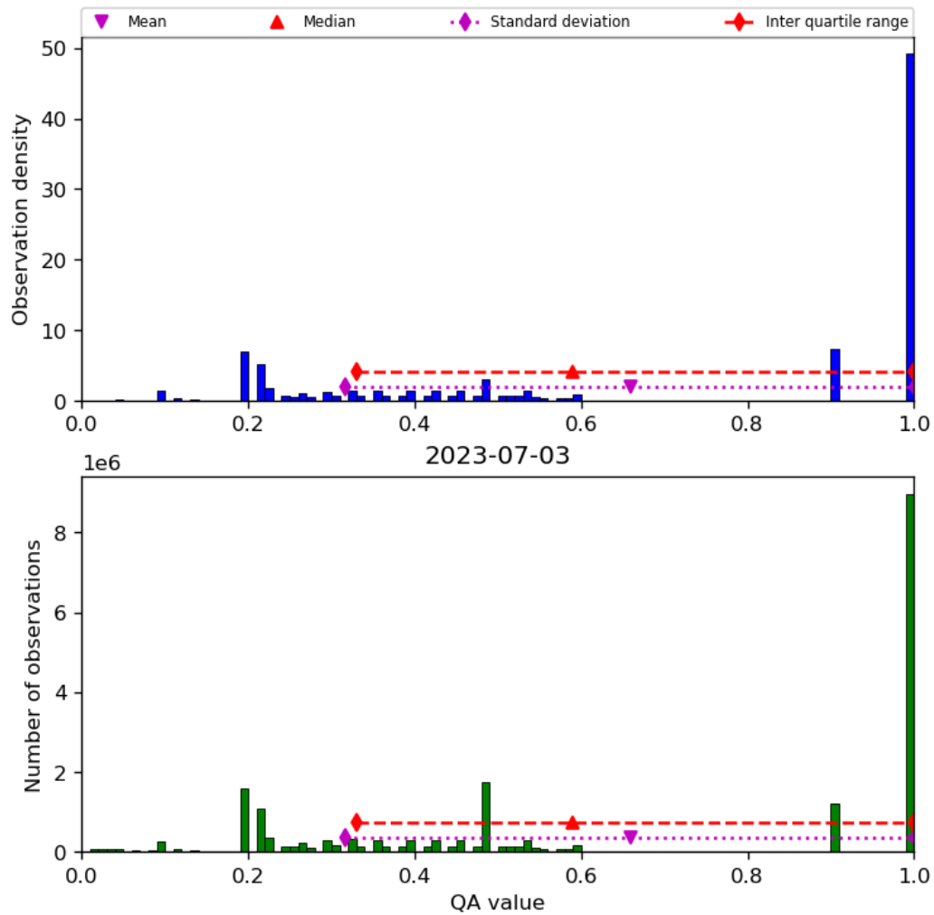
Figure 34: Histogram of “QA value” for 2023-07-03 to 2023-07-04
