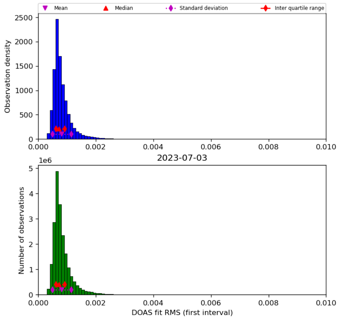
Figure 46: Histogram of “DOAS fit RMS (first interval)” for 2023-07-03 to 2023-07-04
