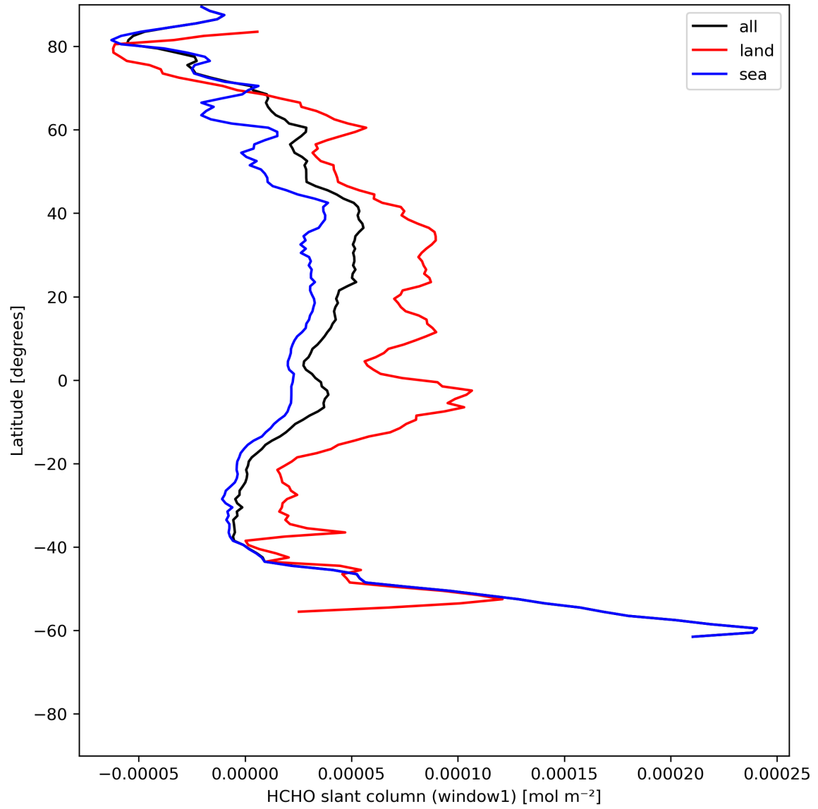
Figure 24: Zonal average of “HCHO slant column (window1)” for 2023-07-03 to 2023-07-04.
