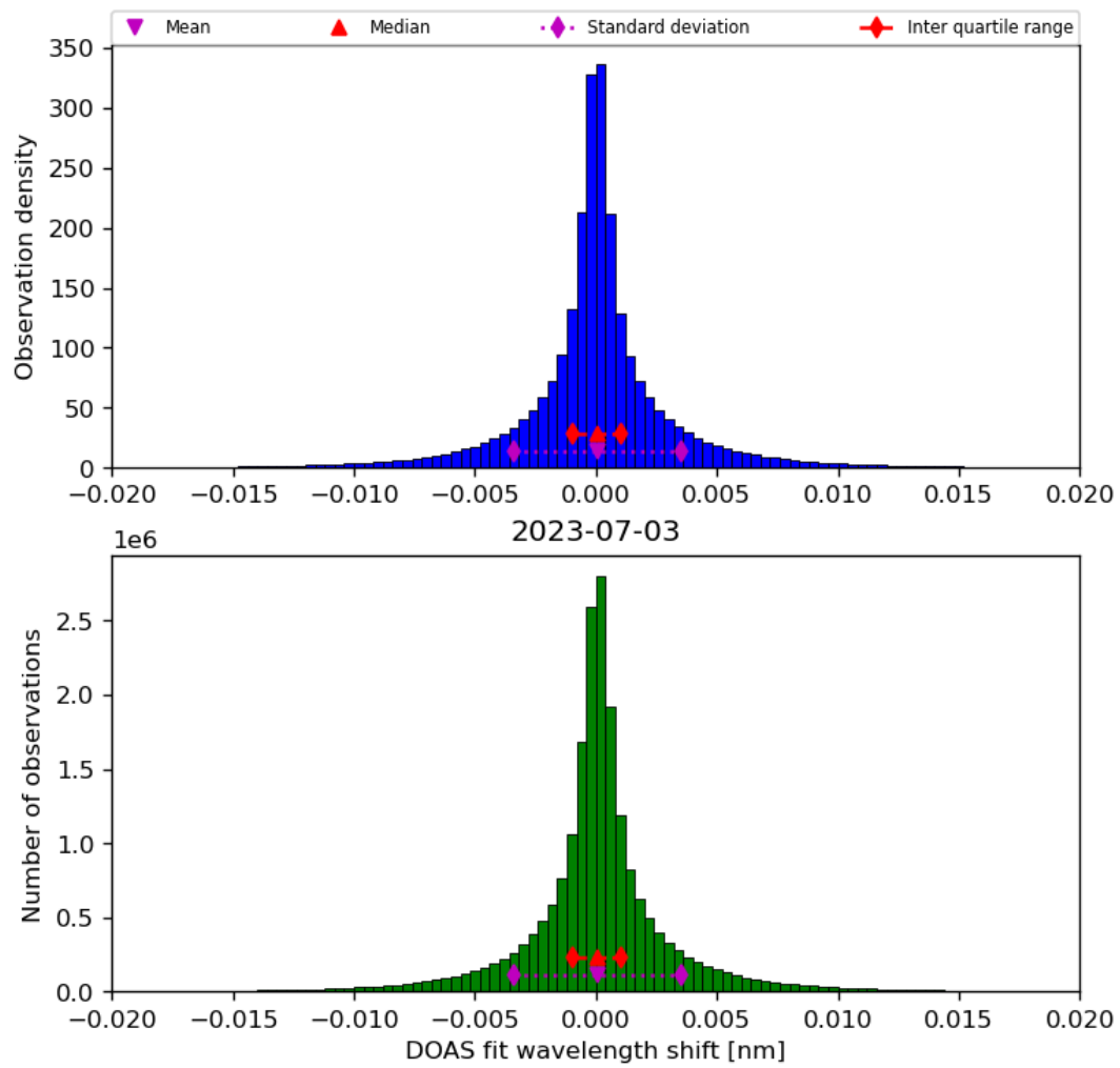
Figure 44: Histogram of “DOAS fit wavelength shift” for 2023-07-03 to 2023-07-04
