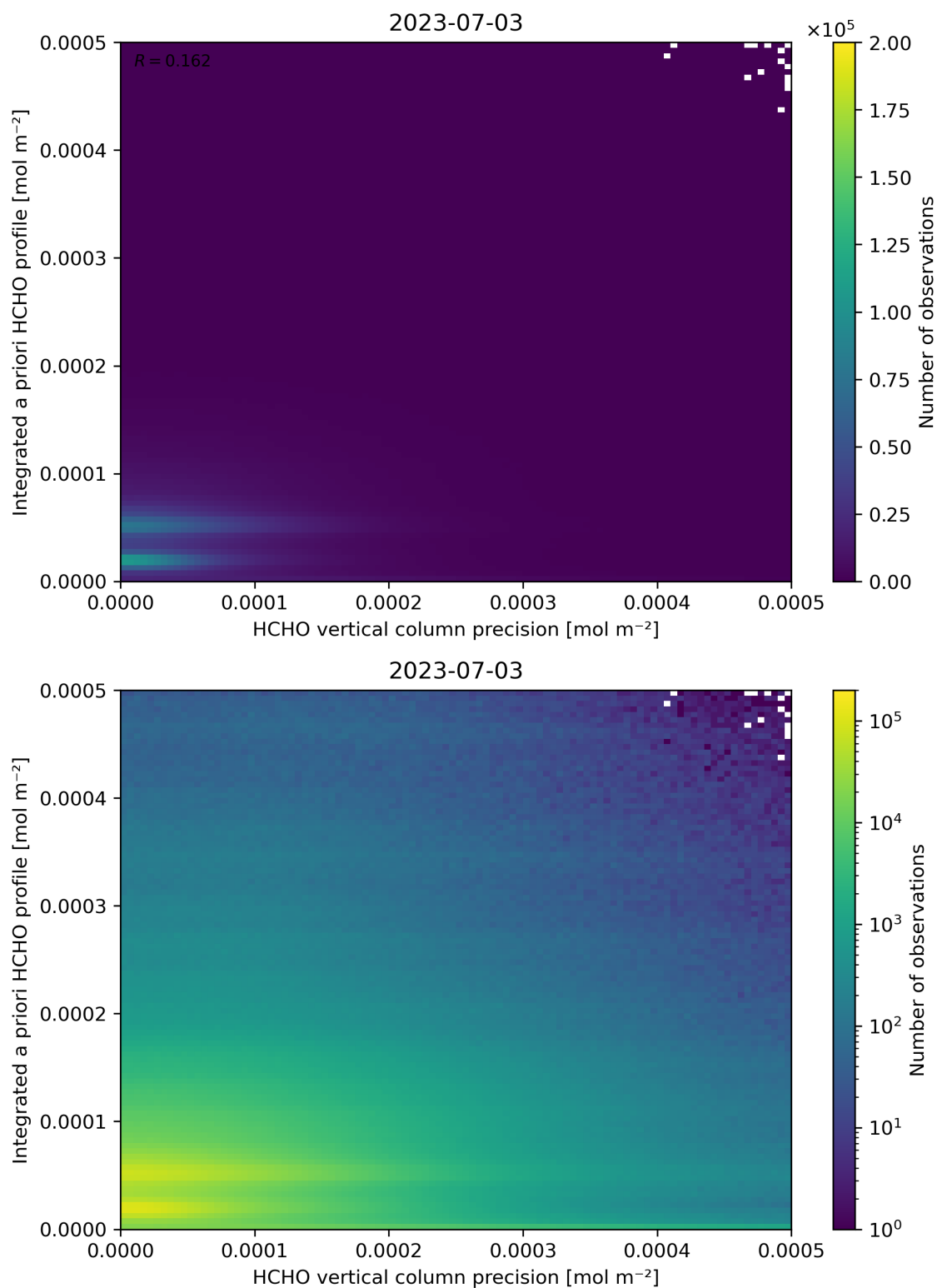
Figure 147: Scatter density plot of “HCHO vertical column precision” against “Integrated a priori HCHO profile” for 2023-07-03 to 2023-07-04.
