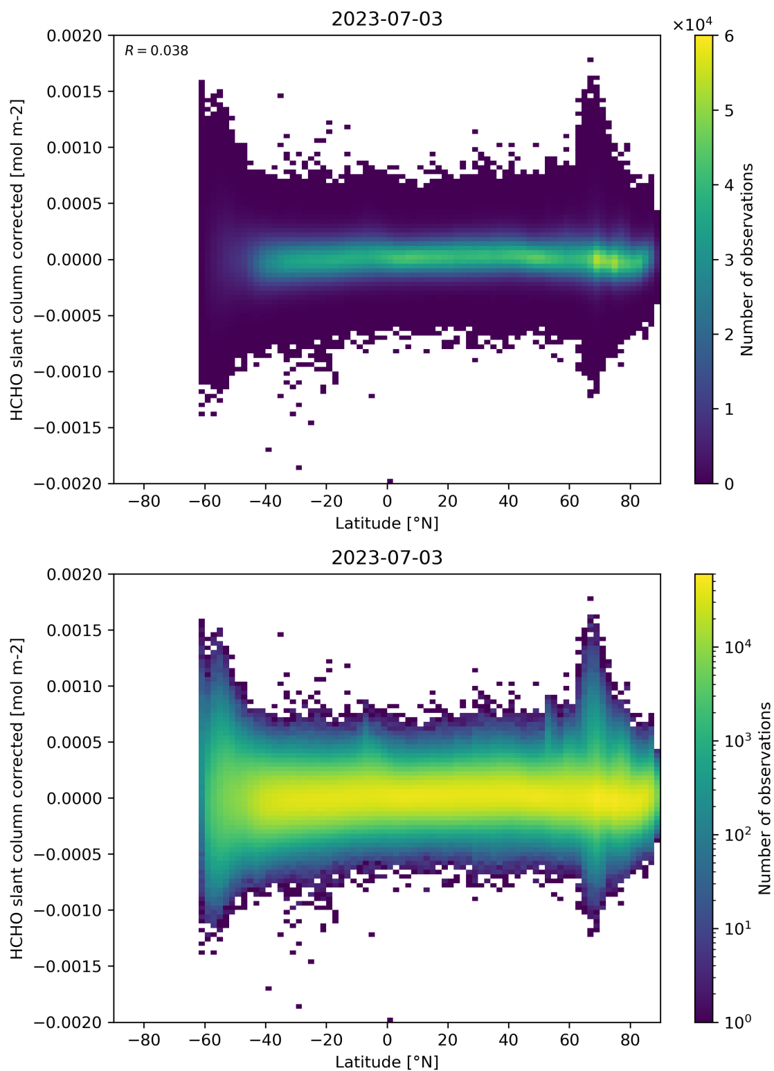
Figure 157: Scatter density plot of “Latitude” against “HCHO slant column corrected” for 2023-07-03 to 2023-07-04.
