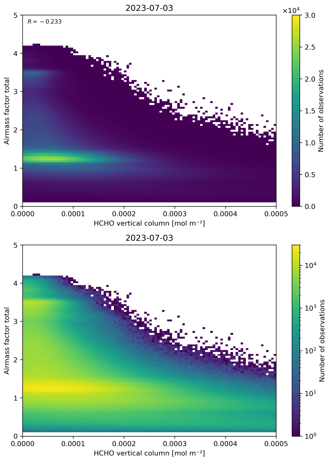
Figure 131: Scatter density plot of “HCHO vertical column” against “Airmass factor total” for 2023-07-03 to 2023-07-04.
