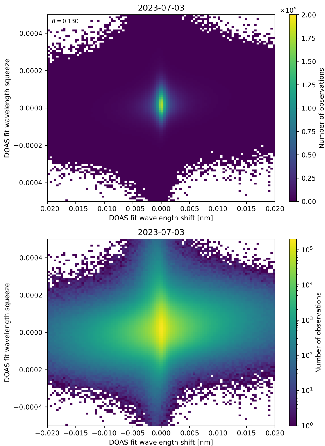
Figure 65: Scatter density plot of “DOAS fit wavelength shift” against “DOAS fit wavelength squeeze” for 2023-07-03 to 2023-07-04.
