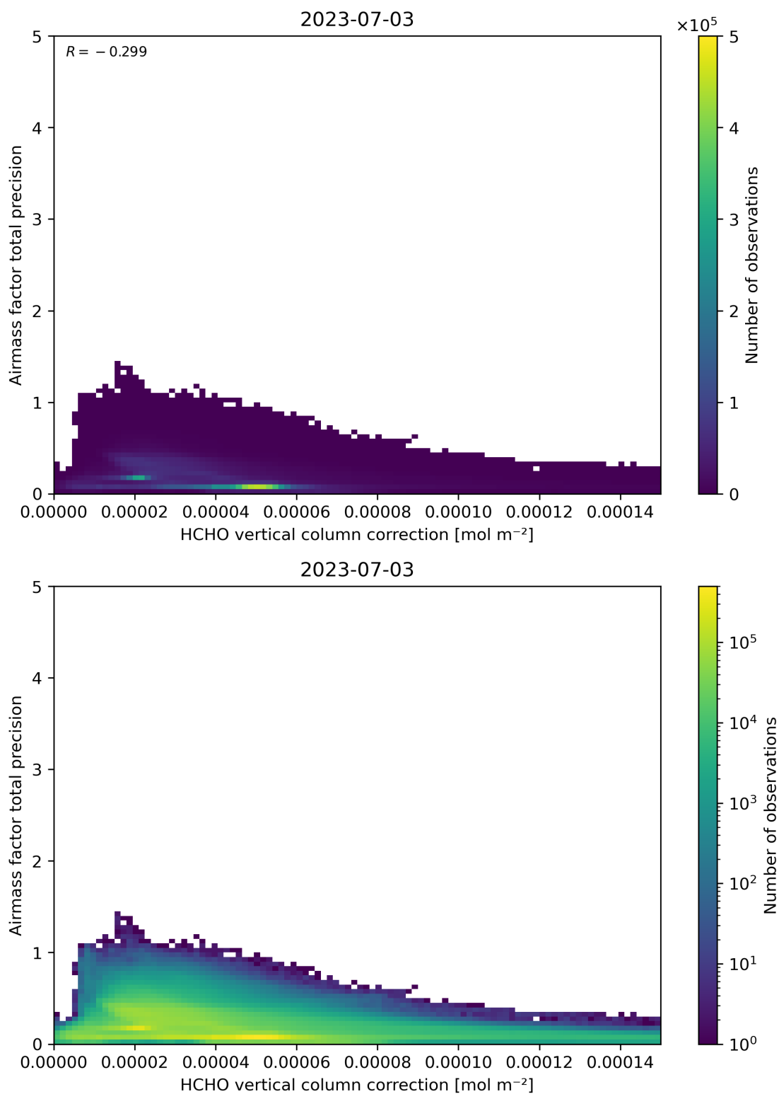
Figure 121: Scatter density plot of “HCHO vertical column correction” against “Airmass factor total precision” for 2023-07-03 to 2023-07-04.
