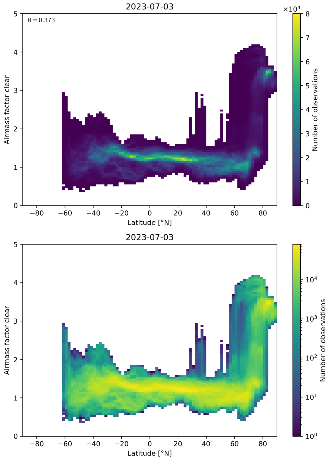
Figure 156: Scatter density plot of “Latitude” against “Airmass factor clear” for 2023-07-03 to 2023-07-04.
