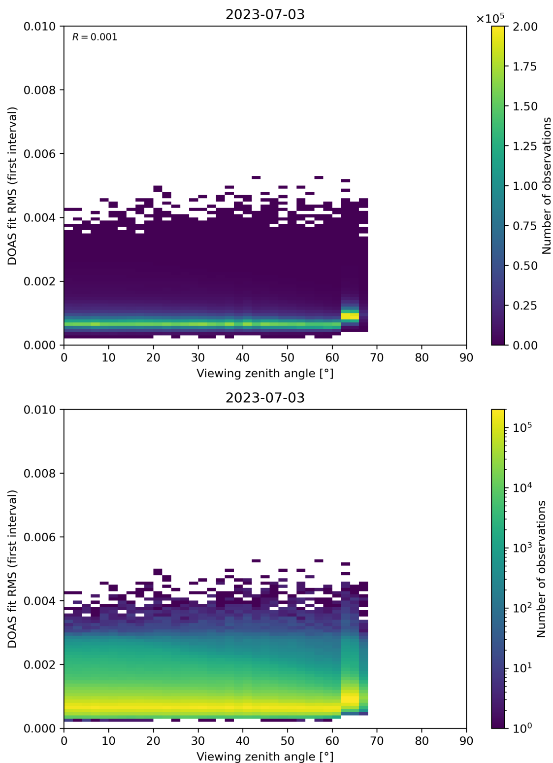
Figure 182: Scatter density plot of “Viewing zenith angle” against “DOAS fit RMS (first interval)” for 2023-07-03 to 2023-07-04.
