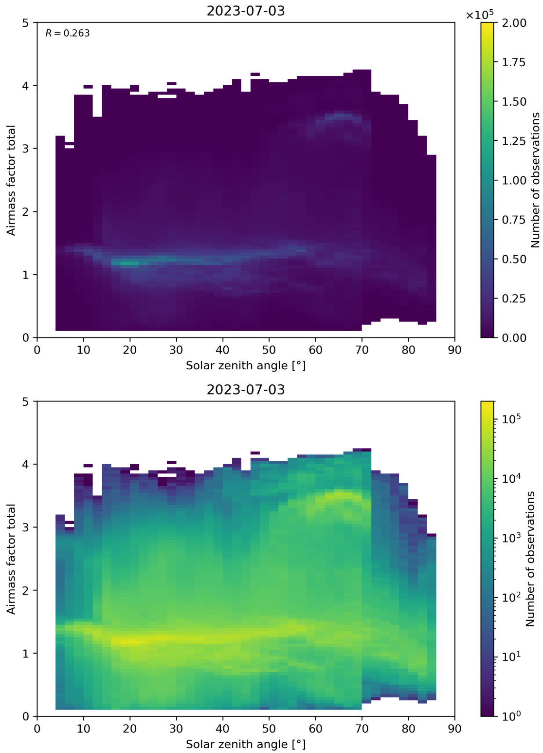
Figure 175: Scatter density plot of “Solar zenith angle” against “Airmass factor total” for 2023-07-03 to 2023-07-04.
