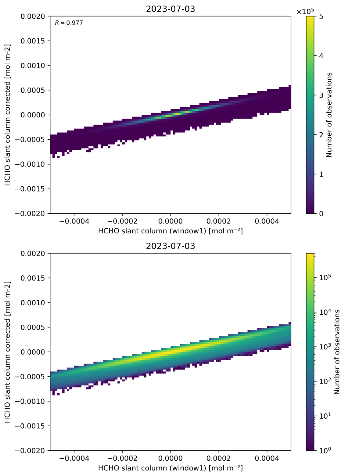
Figure 82: Scatter density plot of “HCHO slant column (window1)” against “HCHO slant column corrected” for 2023-07-03 to 2023-07-04.
