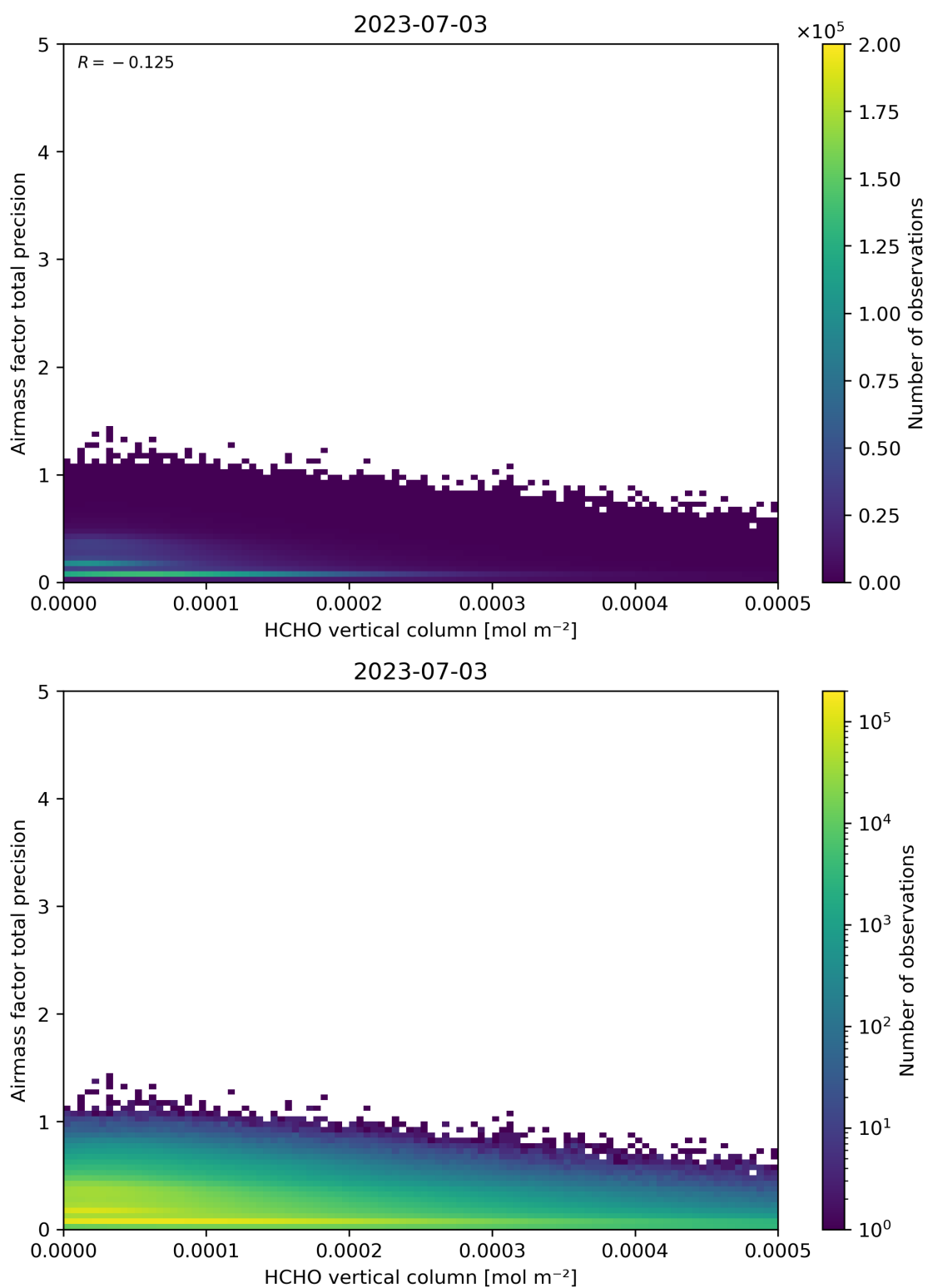
Figure 132: Scatter density plot of “HCHO vertical column” against “Airmass factor total precision” for 2023-07-03 to 2023-07-04.
