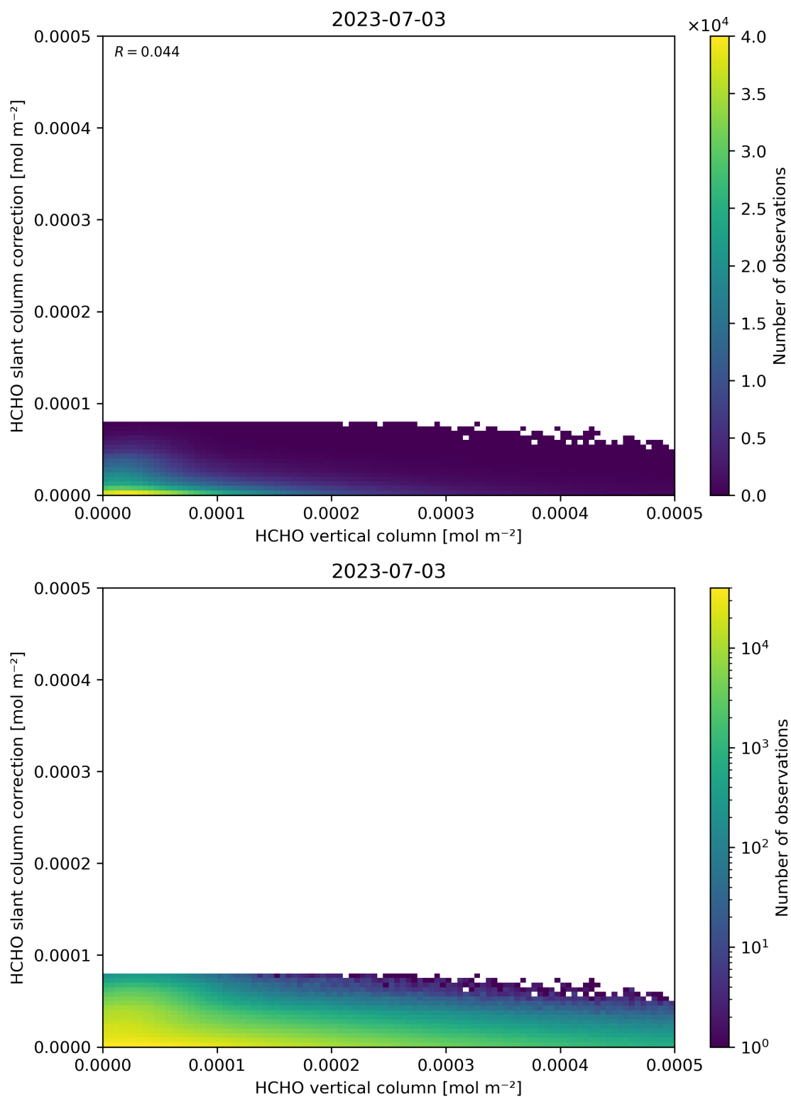
Figure 128: Scatter density plot of “HCHO vertical column” against “HCHO slant column correction” for 2023-07-03 to 2023-07-04.
