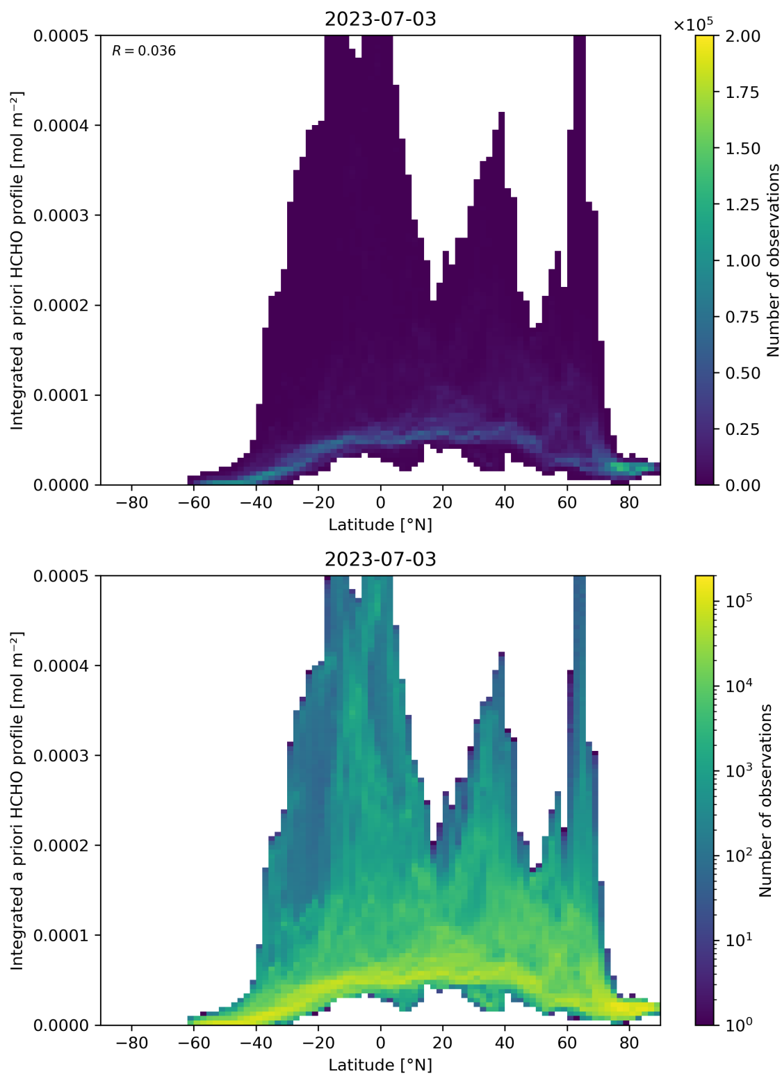
Figure 166: Scatter density plot of “Latitude” against “Integrated a priori HCHO profile” for 2023-07-03 to 2023-07-04.
