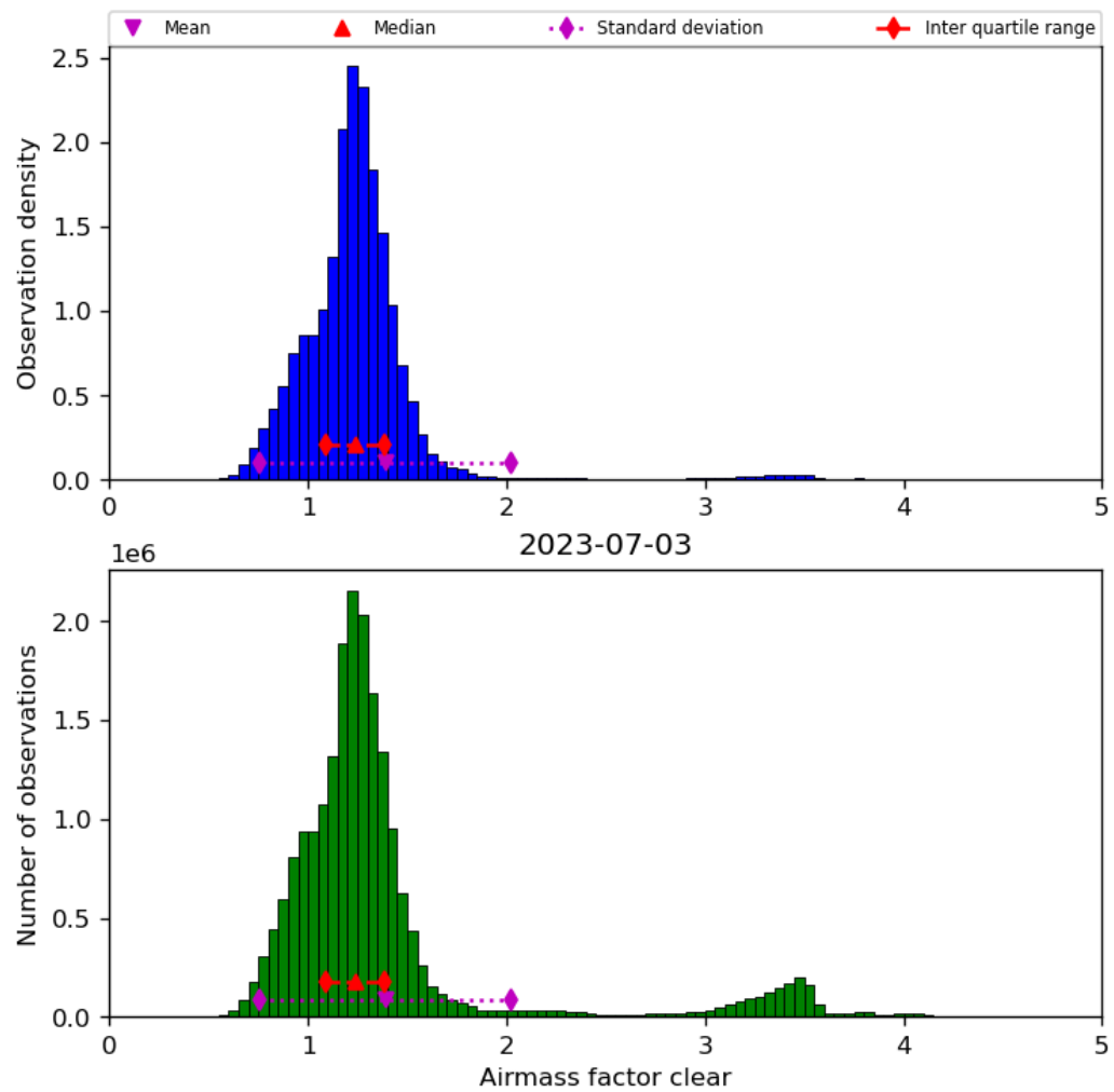
Figure 42: Histogram of “Airmass factor clear” for 2023-07-03 to 2023-07-04
