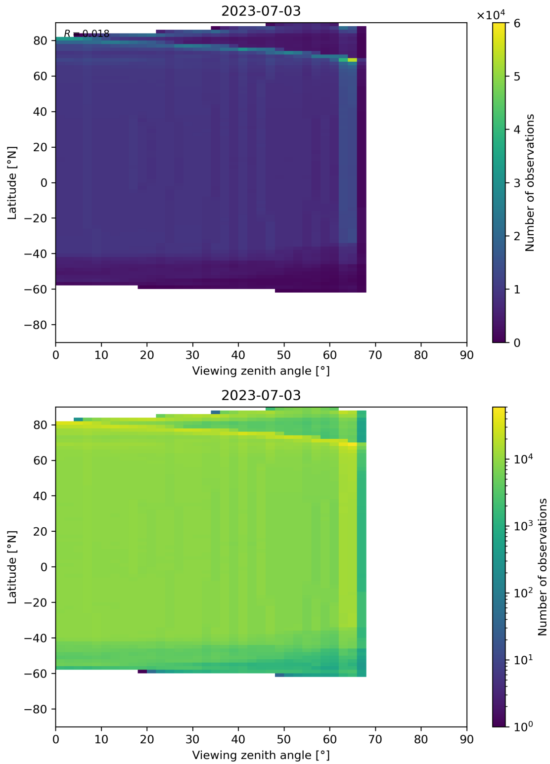
Figure 196: Scatter density plot of “Viewing zenith angle” against “Latitude” for 2023-07-03 to 2023-07-04.
