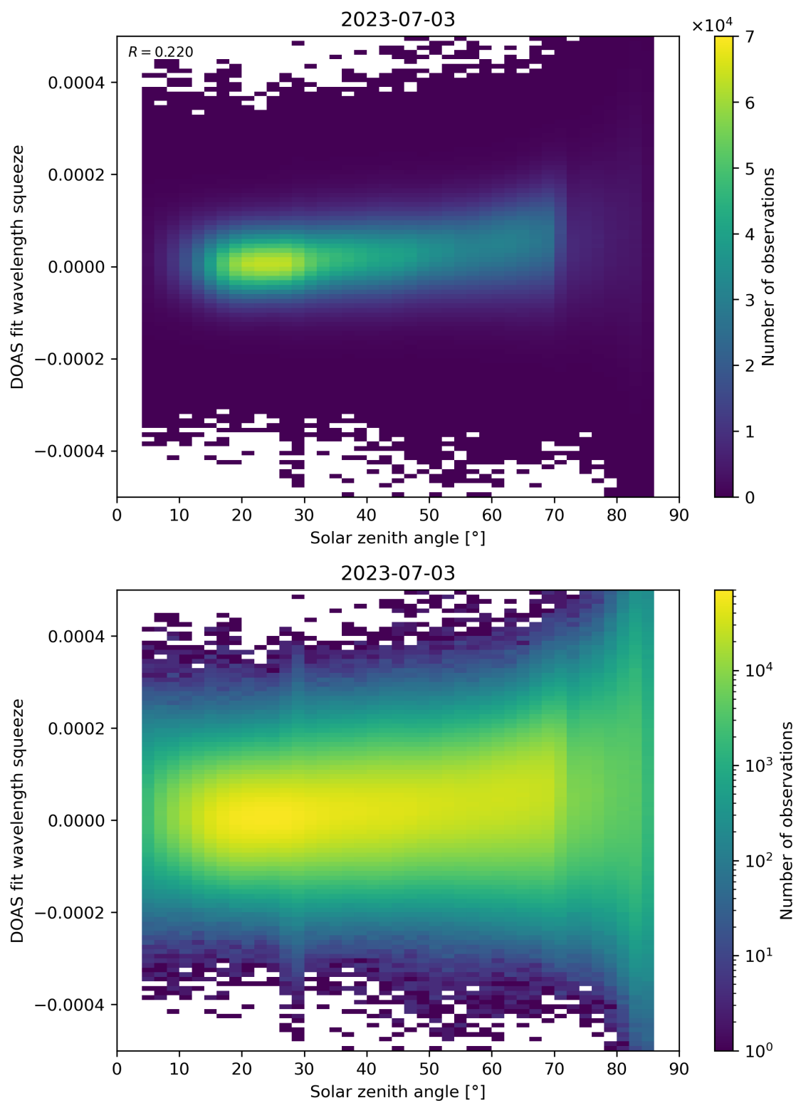
Figure 169: Scatter density plot of “Solar zenith angle” against “DOAS fit wavelength squeeze” for 2023-07-03 to 2023-07-04.
