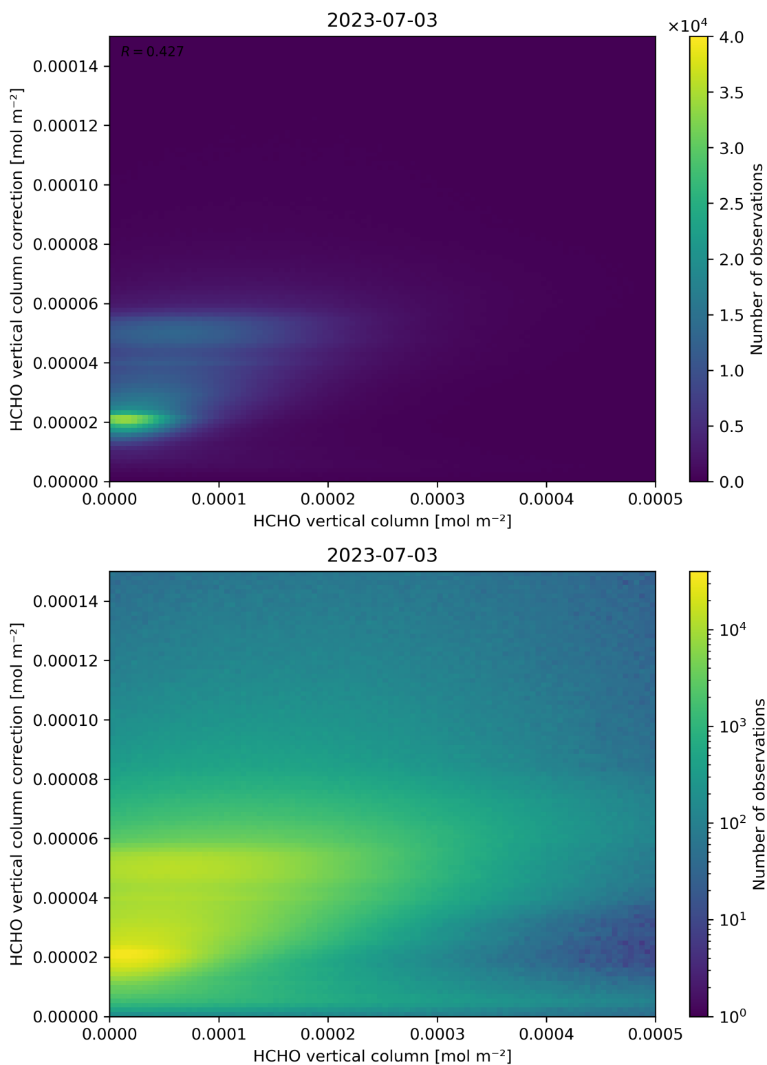
Figure 133: Scatter density plot of “HCHO vertical column” against “HCHO vertical column correction” for 2023-07-03 to 2023-07-04.
