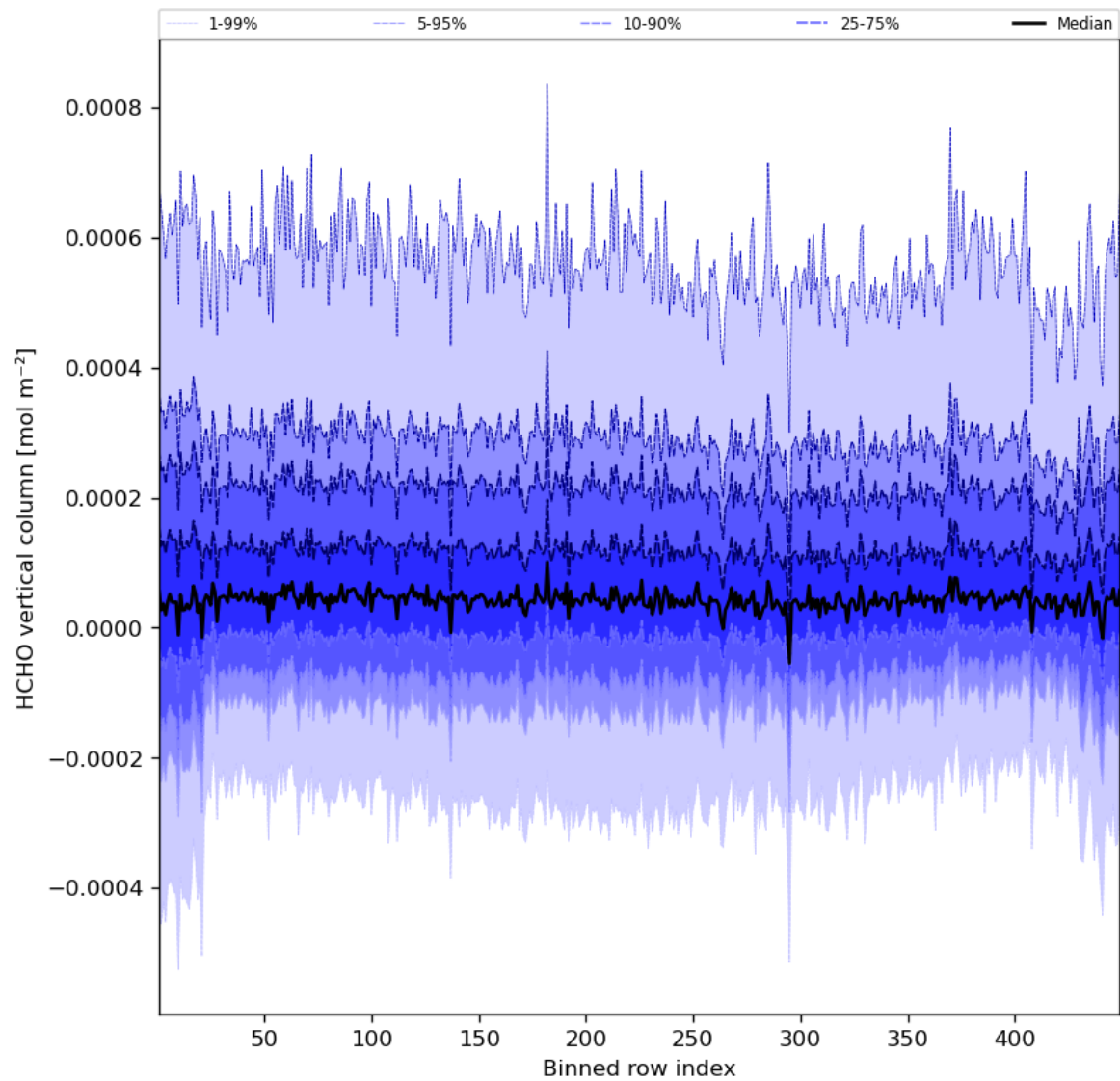
Figure 49: Along track statistics of “HCHO vertical column” for 2023-07-03 to 2023-07-04
