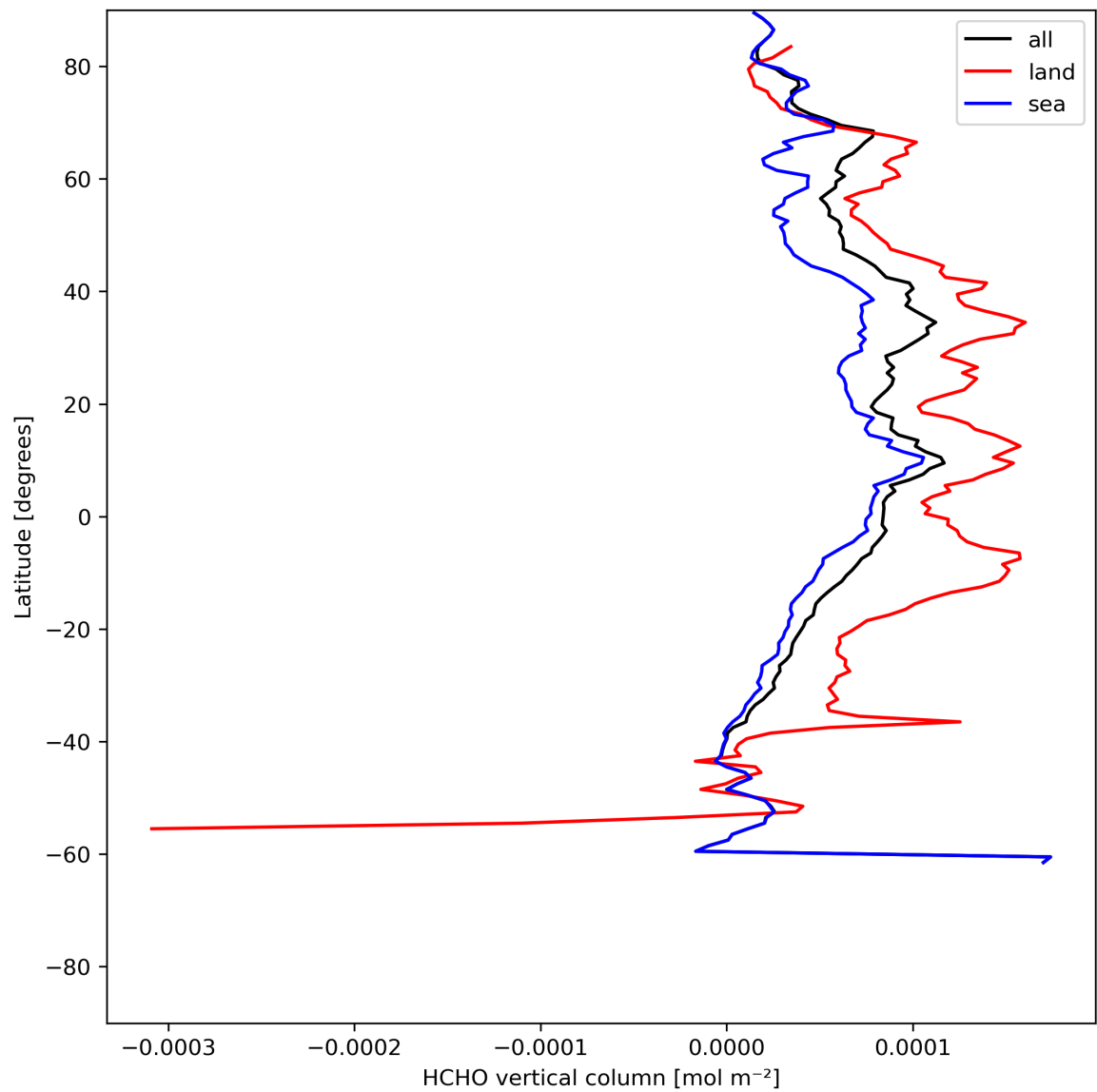
Figure 21: Zonal average of “HCHO vertical column” for 2023-07-03 to 2023-07-04.
