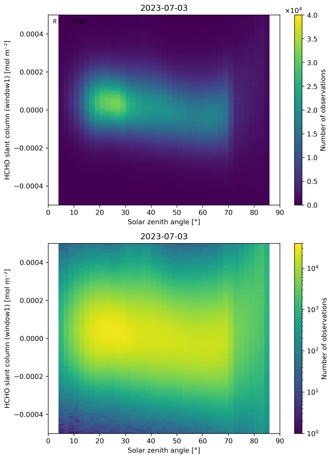
Figure 173: Scatter density plot of “Solar zenith angle” against “HCHO slant column (window1)” for 2023-07-03 to 2023-07-04.
