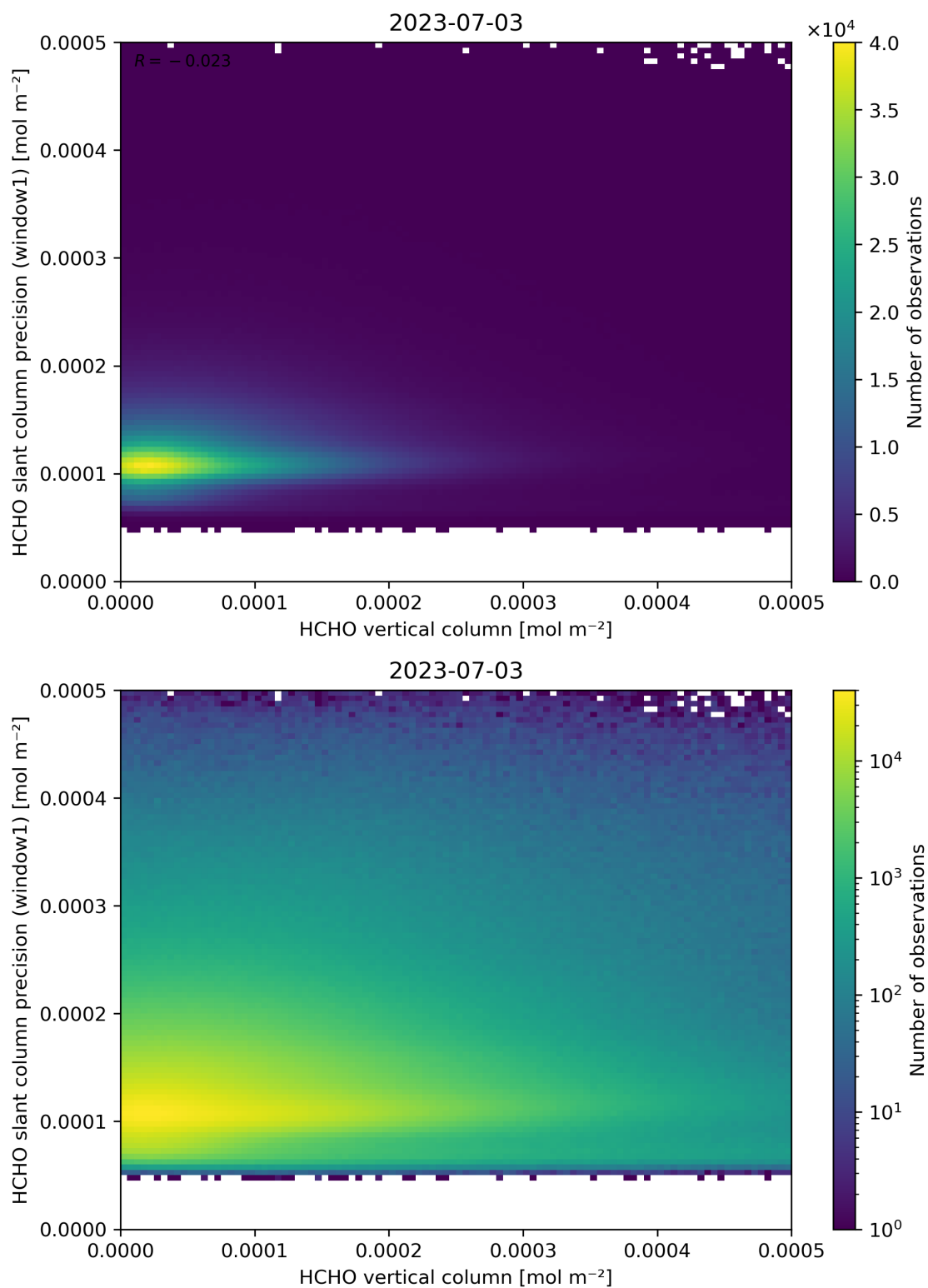
Figure 130: Scatter density plot of “HCHO vertical column” against “HCHO slant column precision (window1)” for 2023-07-03 to 2023-07-04.
