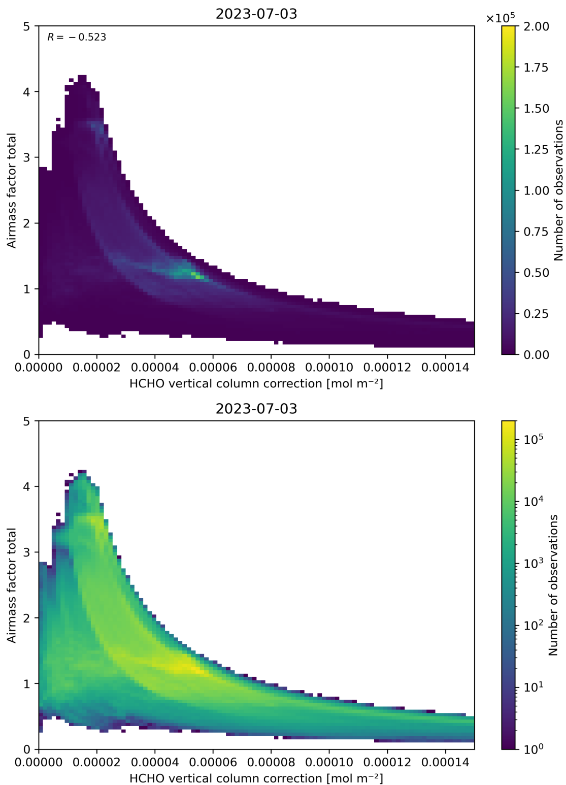
Figure 120: Scatter density plot of “HCHO vertical column correction” against “Airmass factor total” for 2023-07-03 to 2023-07-04.
