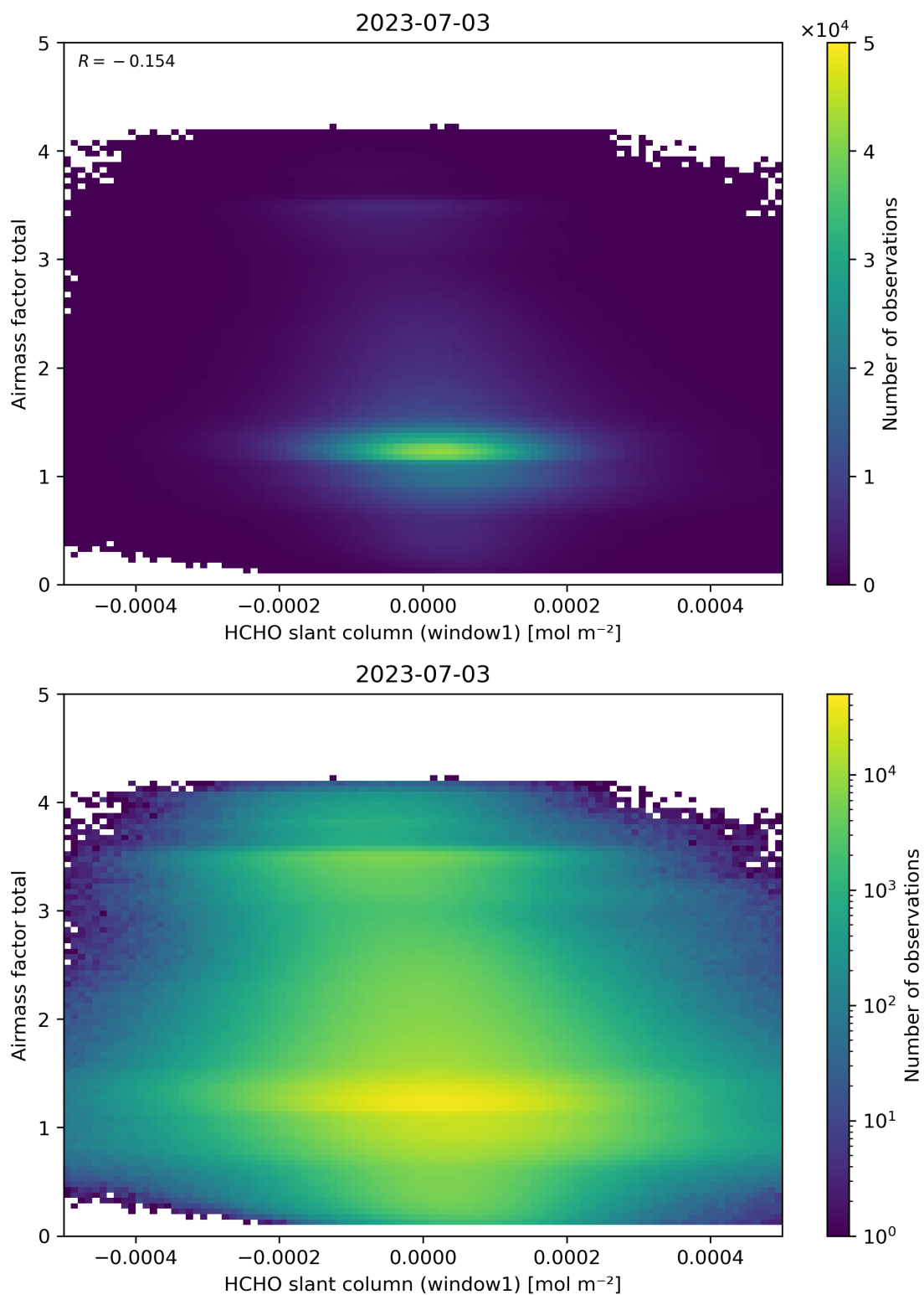
Figure 85: Scatter density plot of “HCHO slant column (window1)” against “Airmass factor total” for 2023-07-03 to 2023-07-04.
