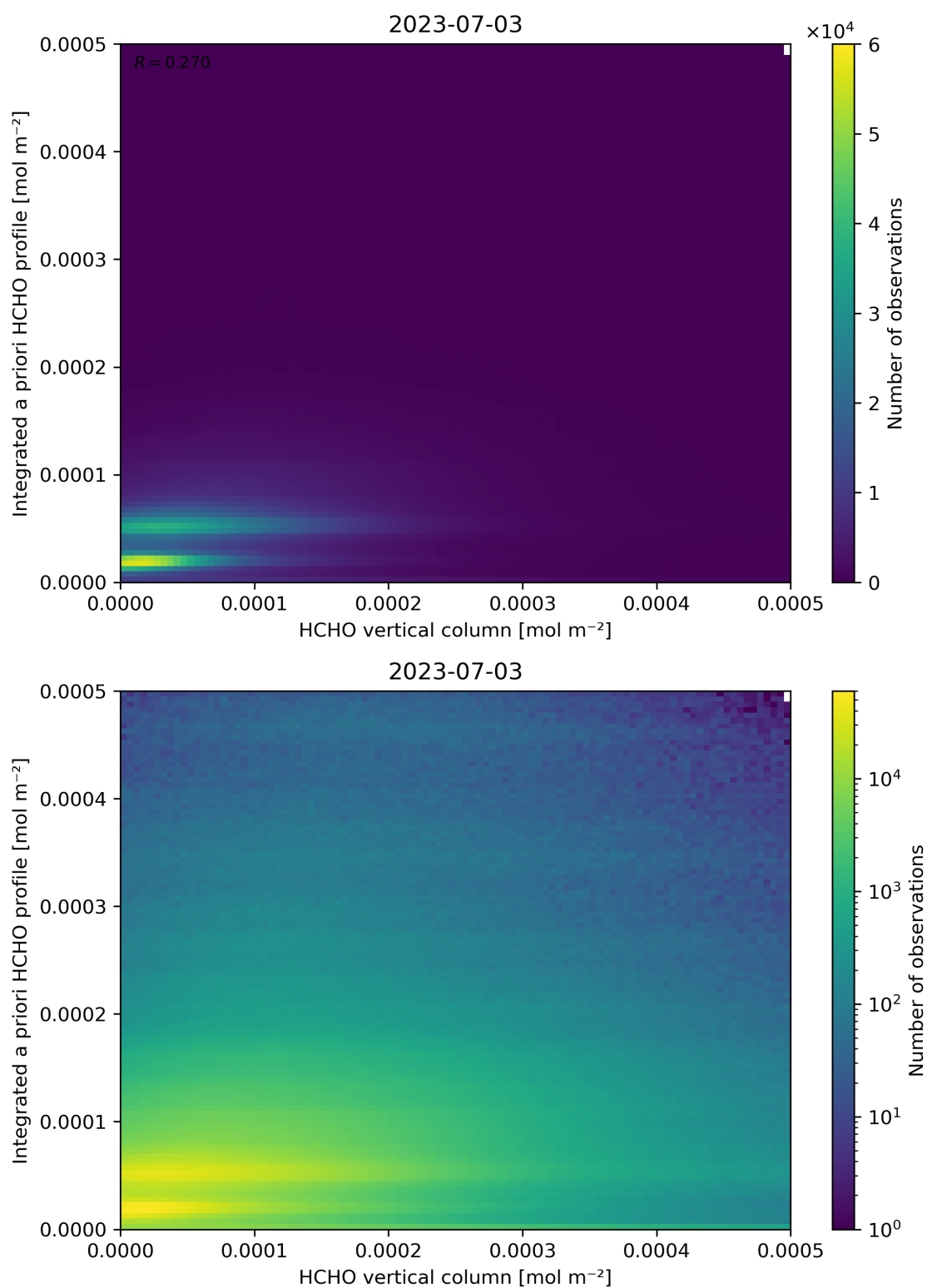
Figure 135: Scatter density plot of “HCHO vertical column” against “Integrated a priori HCHO profile” for 2023-07-03 to 2023-07-04.
