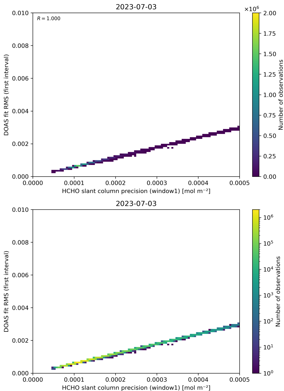
Figure 88: Scatter density plot of “HCHO slant column precision (window1)” against “DOAS fit RMS (first interval)” for 2023-07-03 to 2023-07-04.
