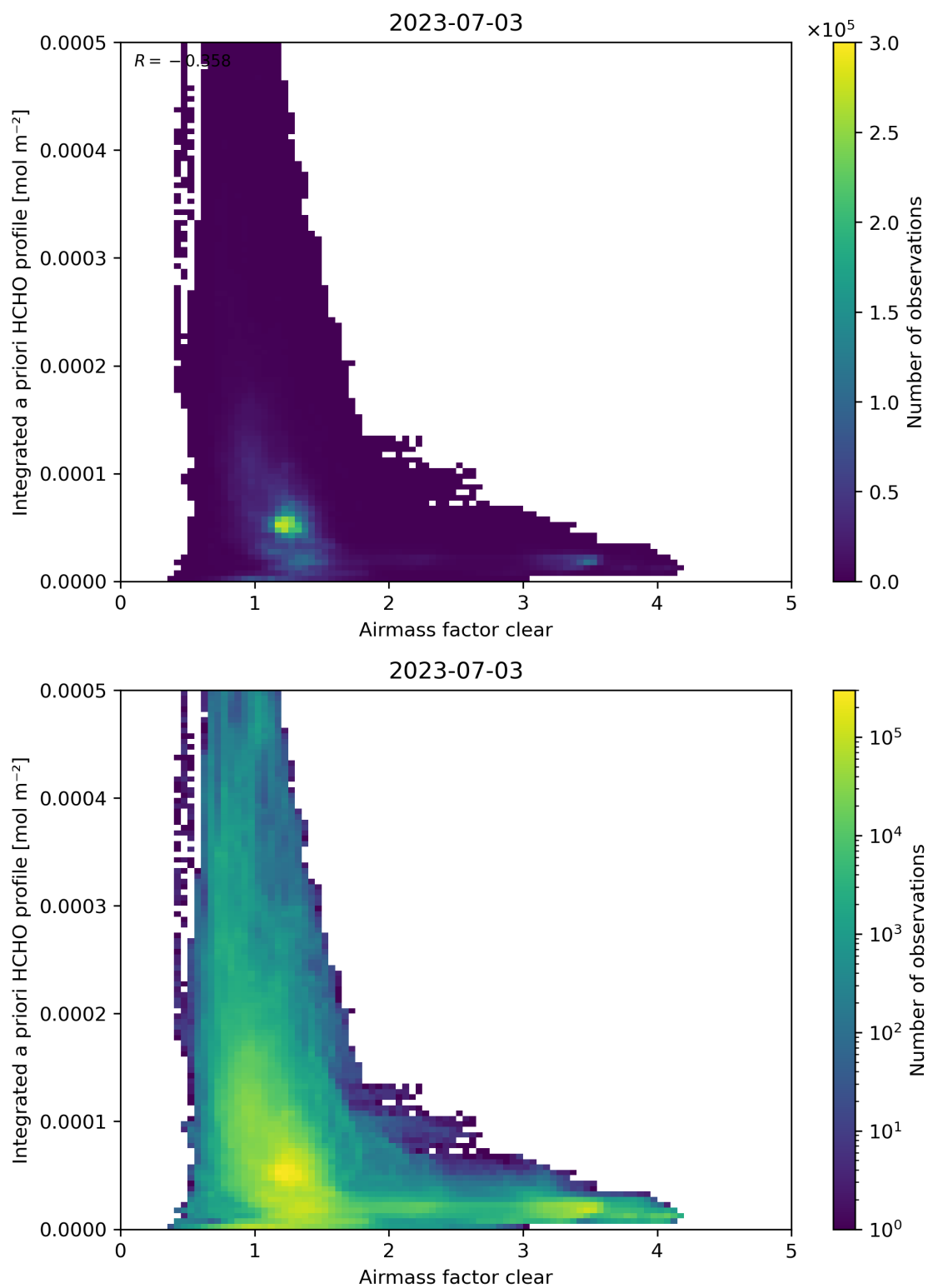
Figure 76: Scatter density plot of “Airmass factor clear” against “Integrated a priori HCHO profile” for 2023-07-03 to 2023-07-04.
