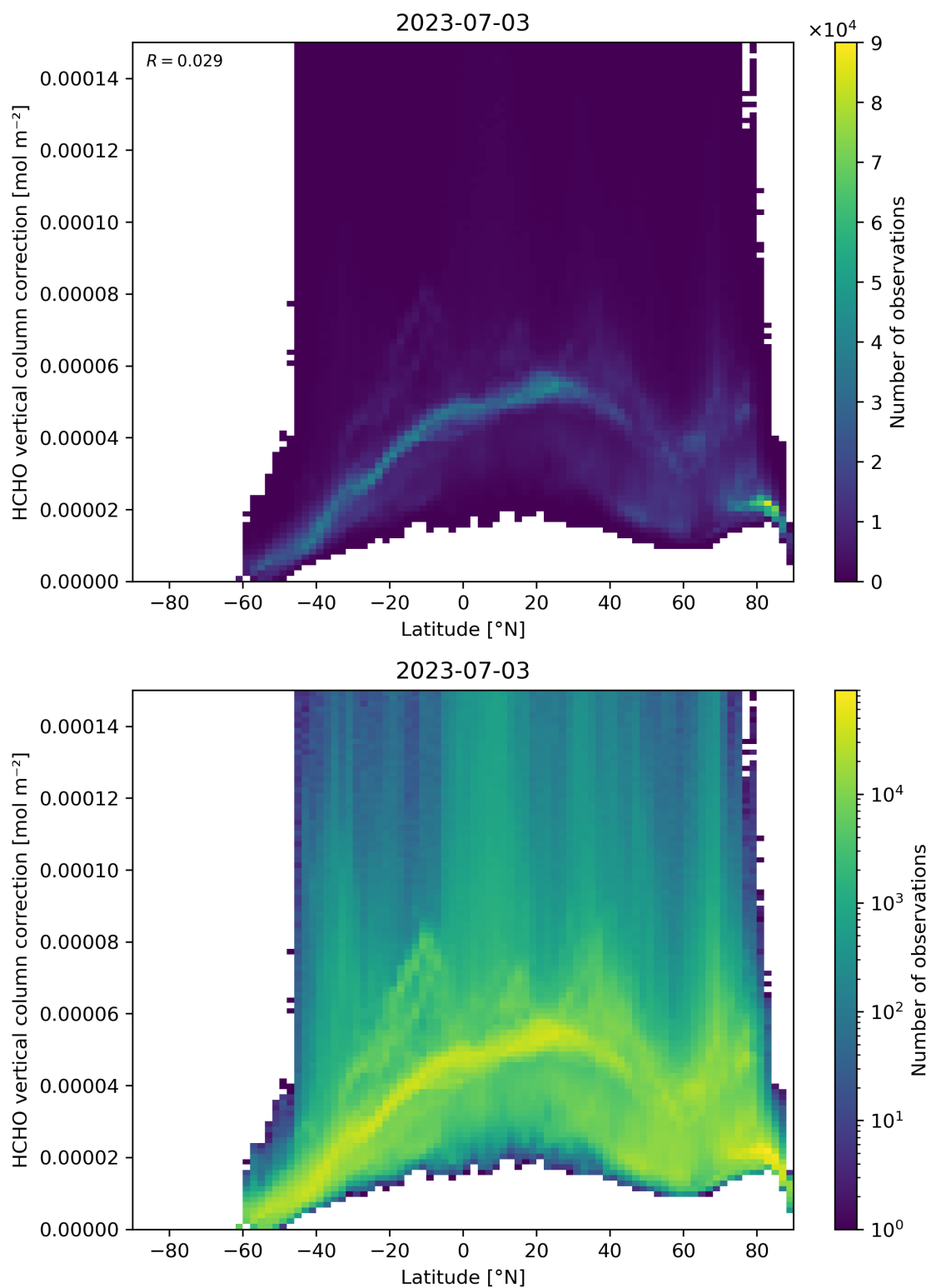
Figure 164: Scatter density plot of “Latitude” against “HCHO vertical column correction” for 2023-07-03 to 2023-07-04.
