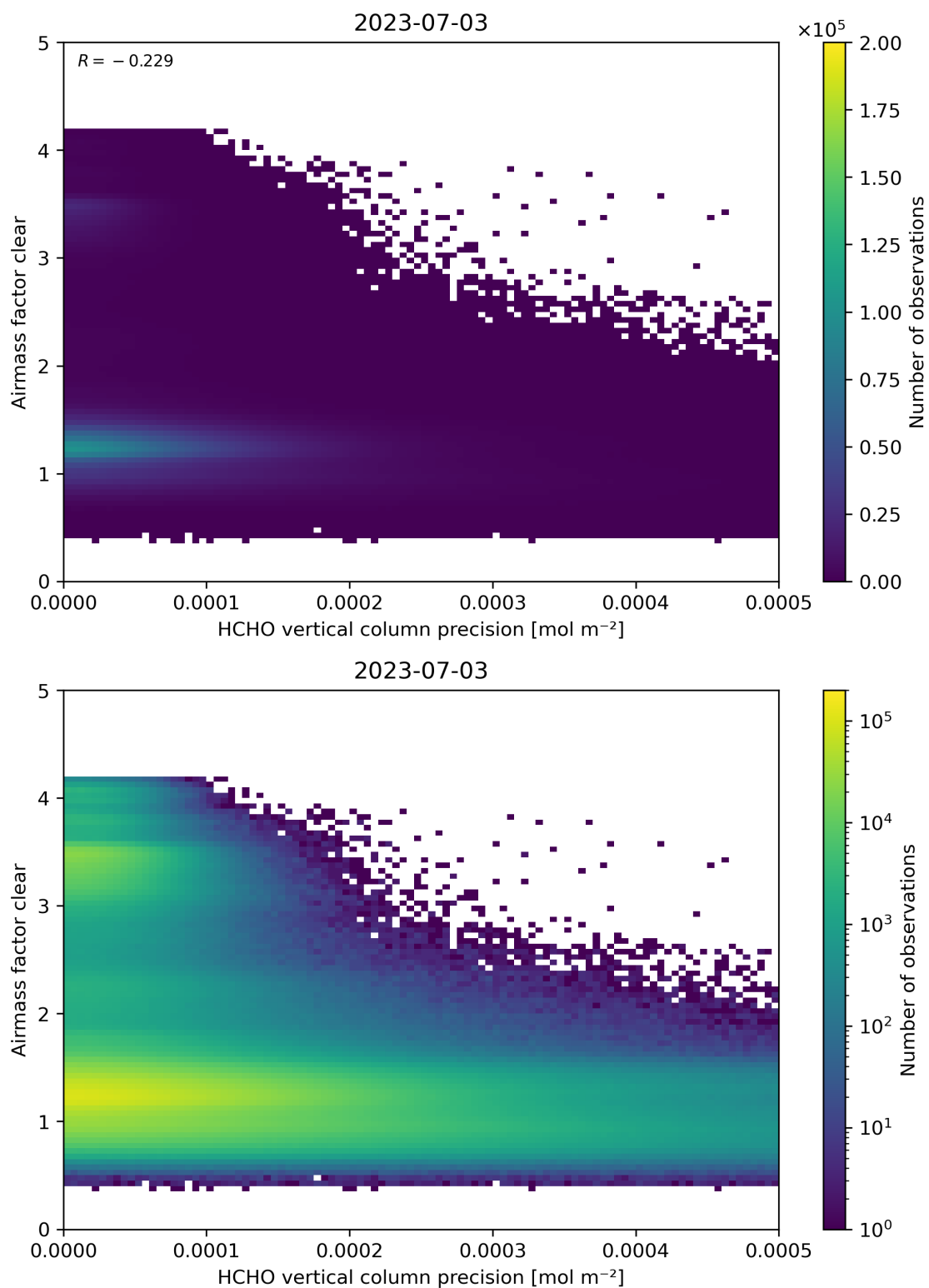
Figure 139: Scatter density plot of “HCHO vertical column precision” against “Airmass factor clear” for 2023-07-03 to 2023-07-04.
