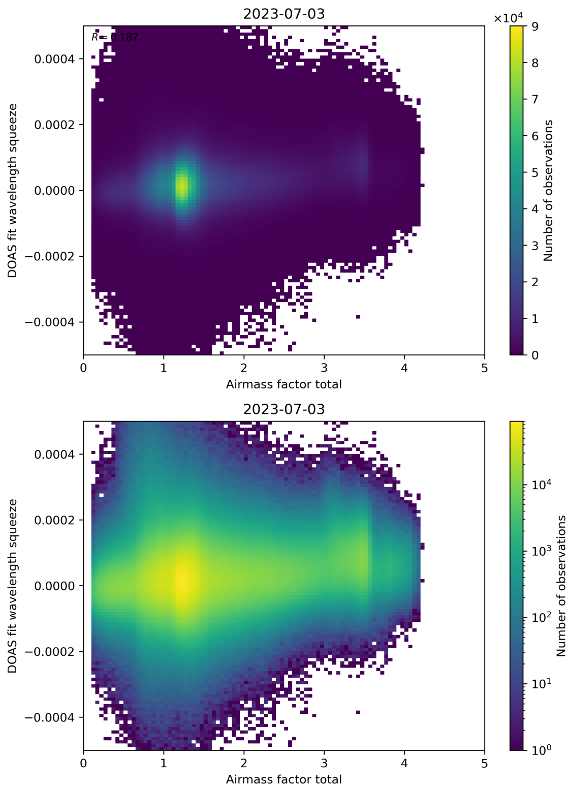
Figure 99: Scatter density plot of “Airmass factor total” against “DOAS fit wavelength squeeze” for 2023-07-03 to 2023-07-04.
