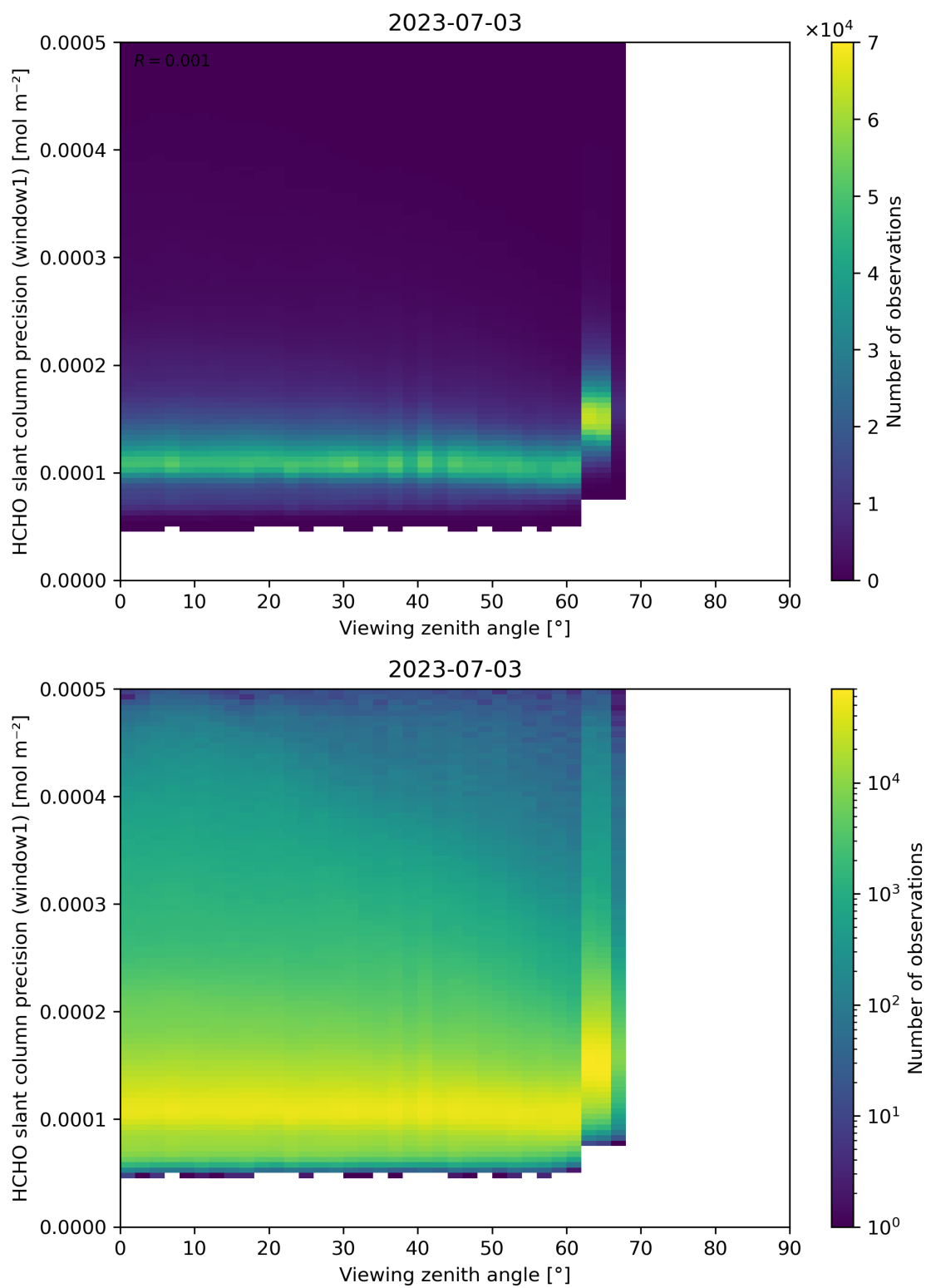
Figure 189: Scatter density plot of “Viewing zenith angle” against “HCHO slant column precision (window1)” for 2023-07-03 to 2023-07-04.
