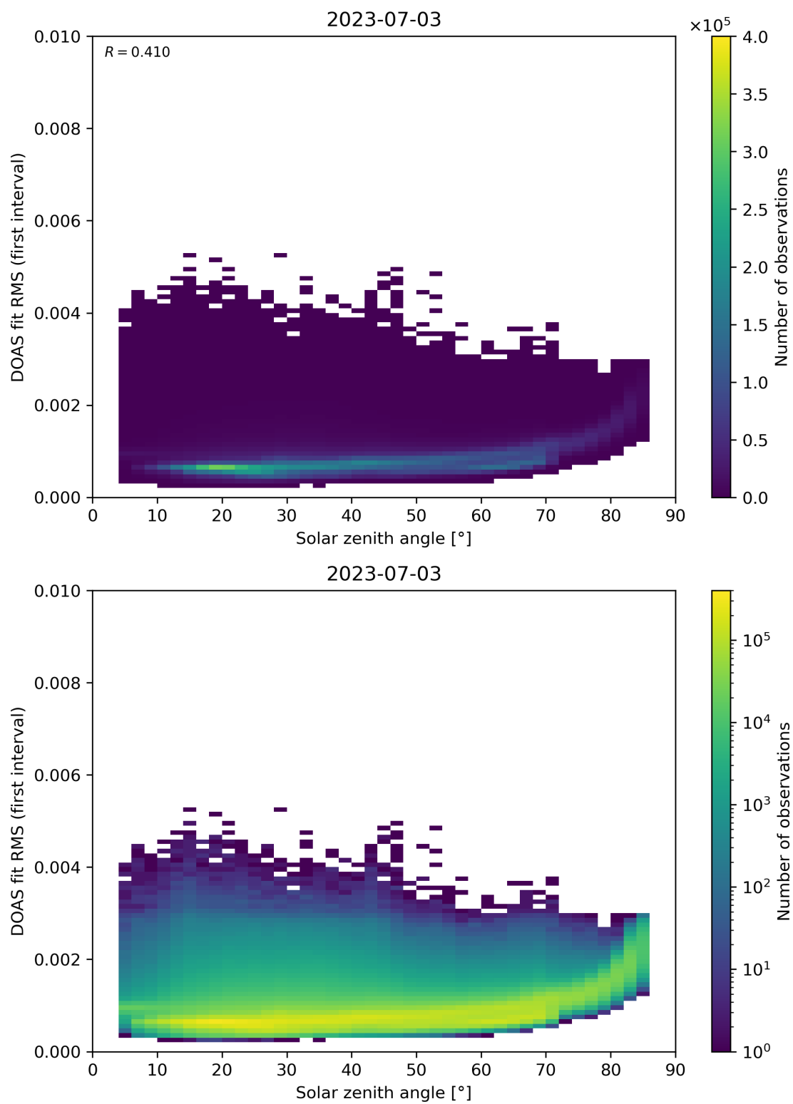
Figure 167: Scatter density plot of “Solar zenith angle” against “DOAS fit RMS (first interval)” for 2023-07-03 to 2023-07-04.
