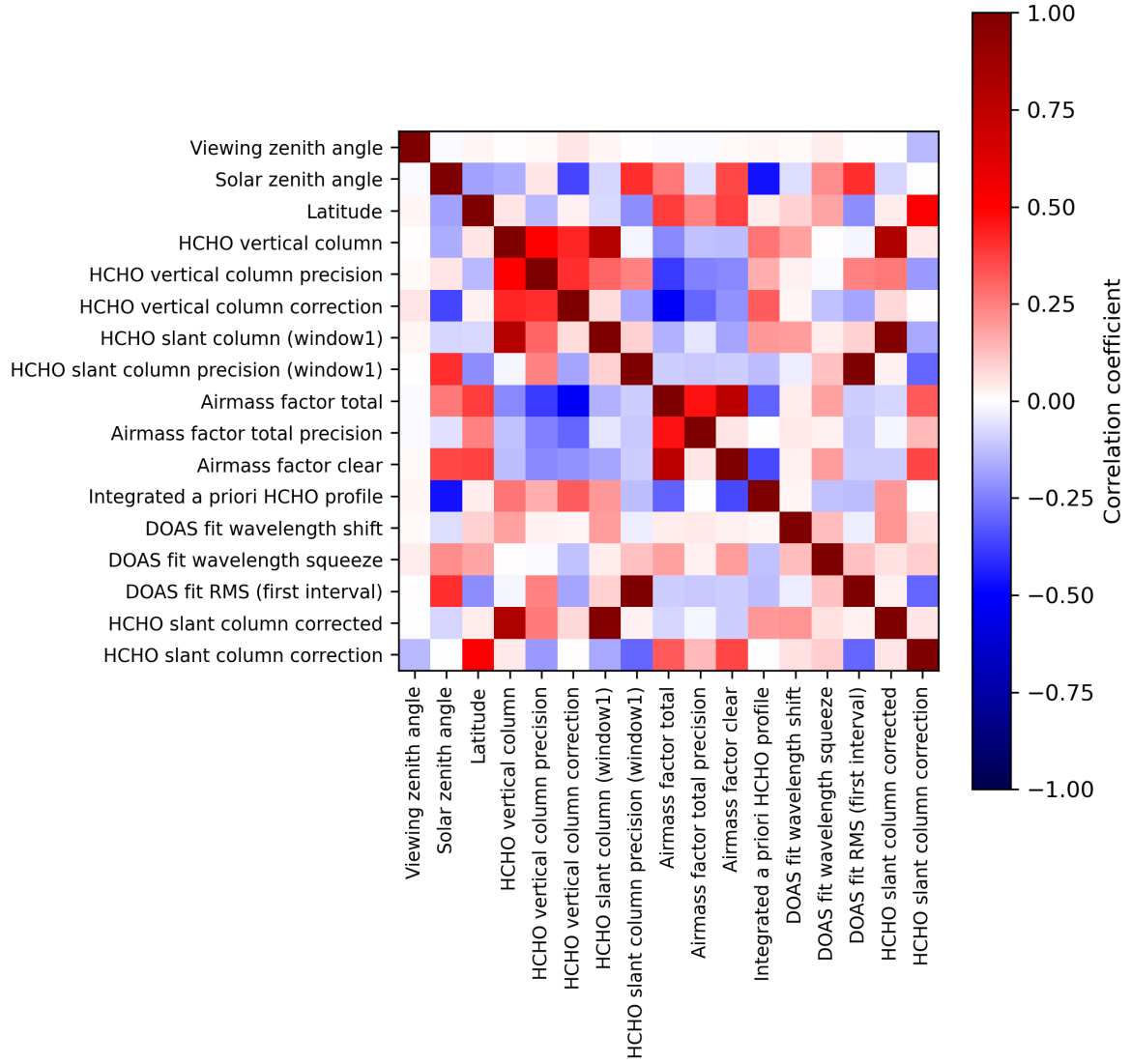
Figure 2: Map of correlation matrix for 2023-07-03 to 2023-07-04.
