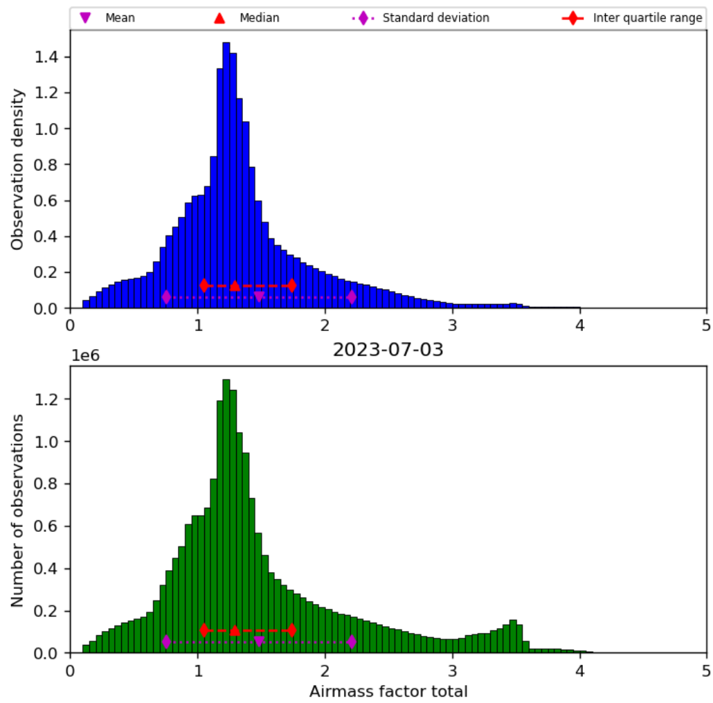
Figure 40: Histogram of “Airmass factor total” for 2023-07-03 to 2023-07-04
