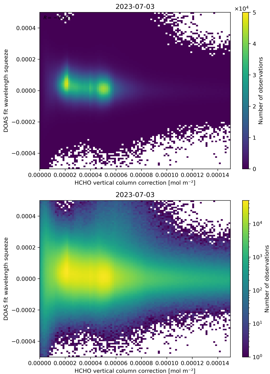
Figure 114: Scatter density plot of “HCHO vertical column correction” against “DOAS fit wavelength squeeze” for 2023-07-03 to 2023-07-04.
