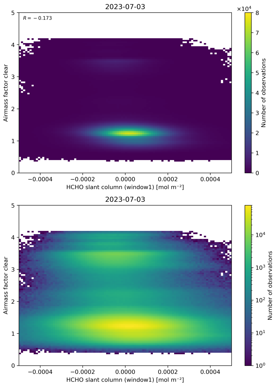
Figure 81: Scatter density plot of “HCHO slant column (window1)” against “Airmass factor clear” for 2023-07-03 to 2023-07-04.
