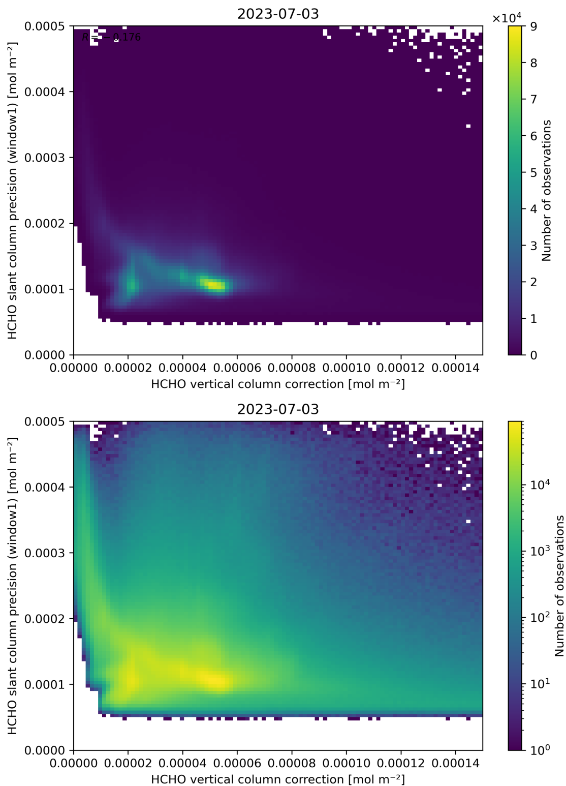
Figure 119: Scatter density plot of “HCHO vertical column correction” against “HCHO slant column precision (window1)” for 2023-07-03 to 2023-07-04.
