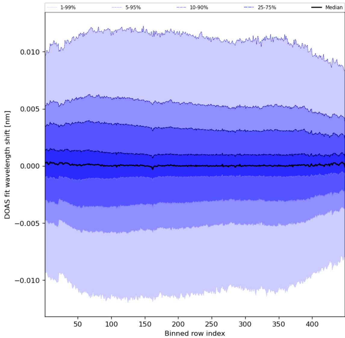
Figure 58: Along track statistics of “DOAS fit wavelength shift” for 2023-07-03 to 2023-07-04
