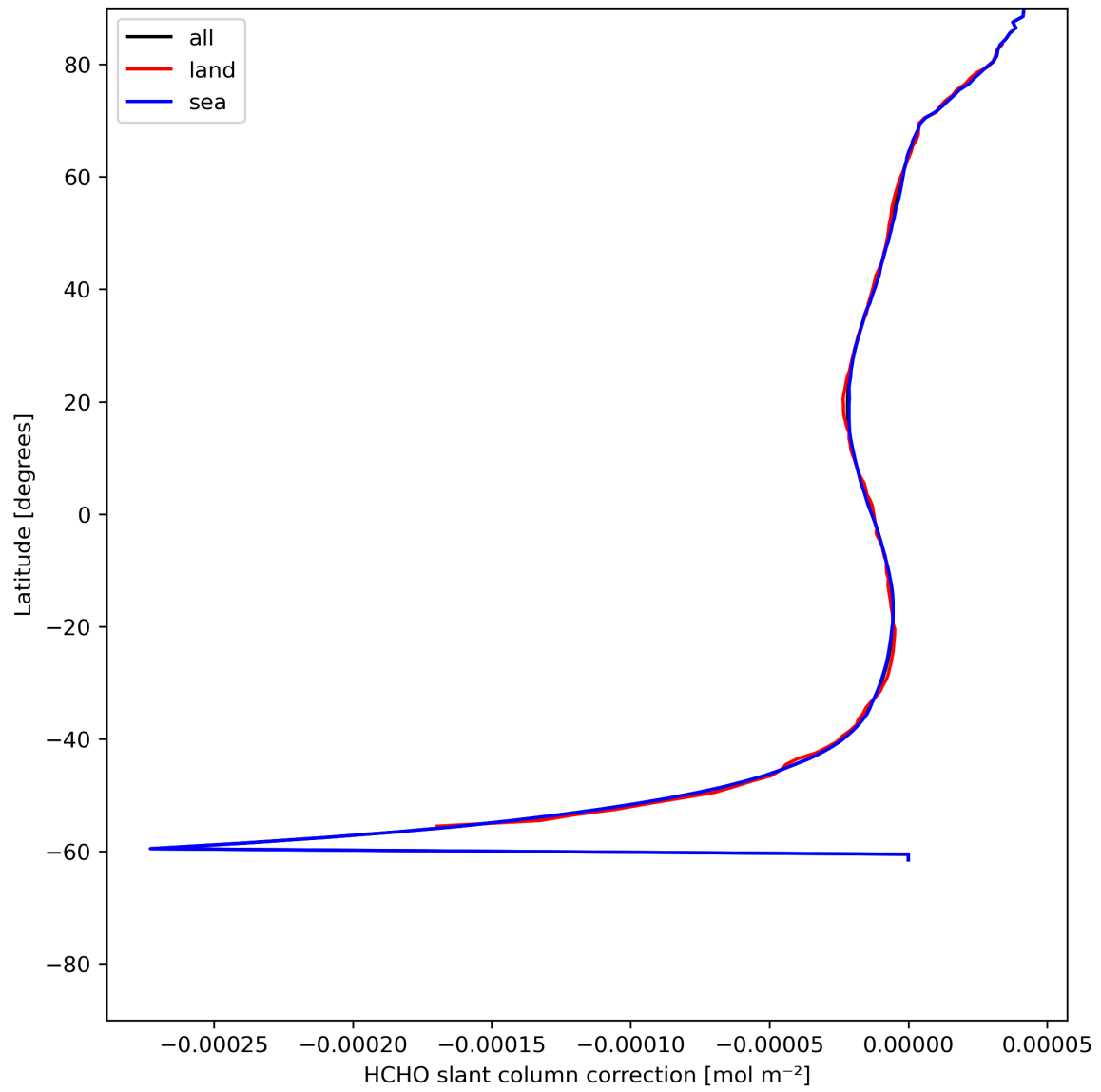
Figure 33: Zonal average of “HCHO slant column correction” for 2023-07-03 to 2023-07-04.
