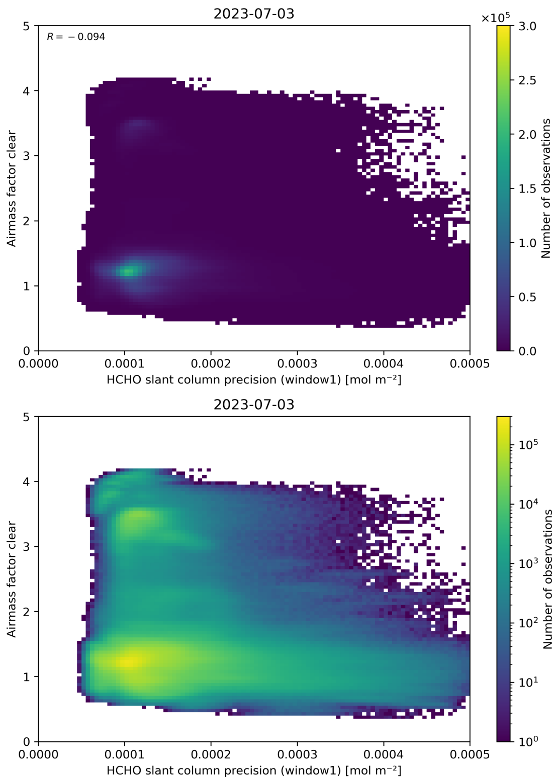
Figure 91: Scatter density plot of “HCHO slant column precision (window1)” against “Airmass factor clear” for 2023-07-03 to 2023-07-04.
