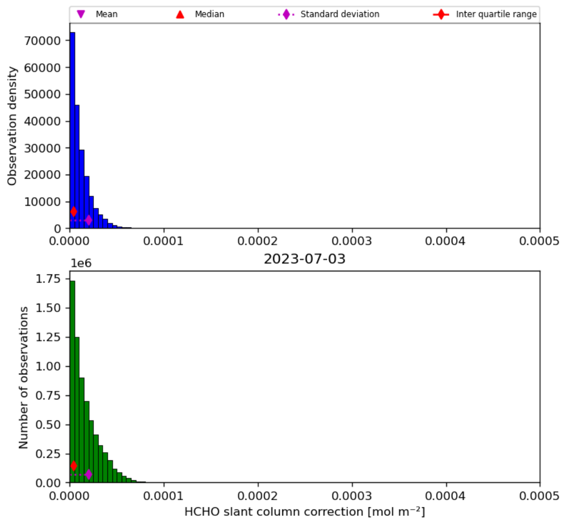
Figure 47: Histogram of “HCHO slant column correction” for 2023-07-03 to 2023-07-04
