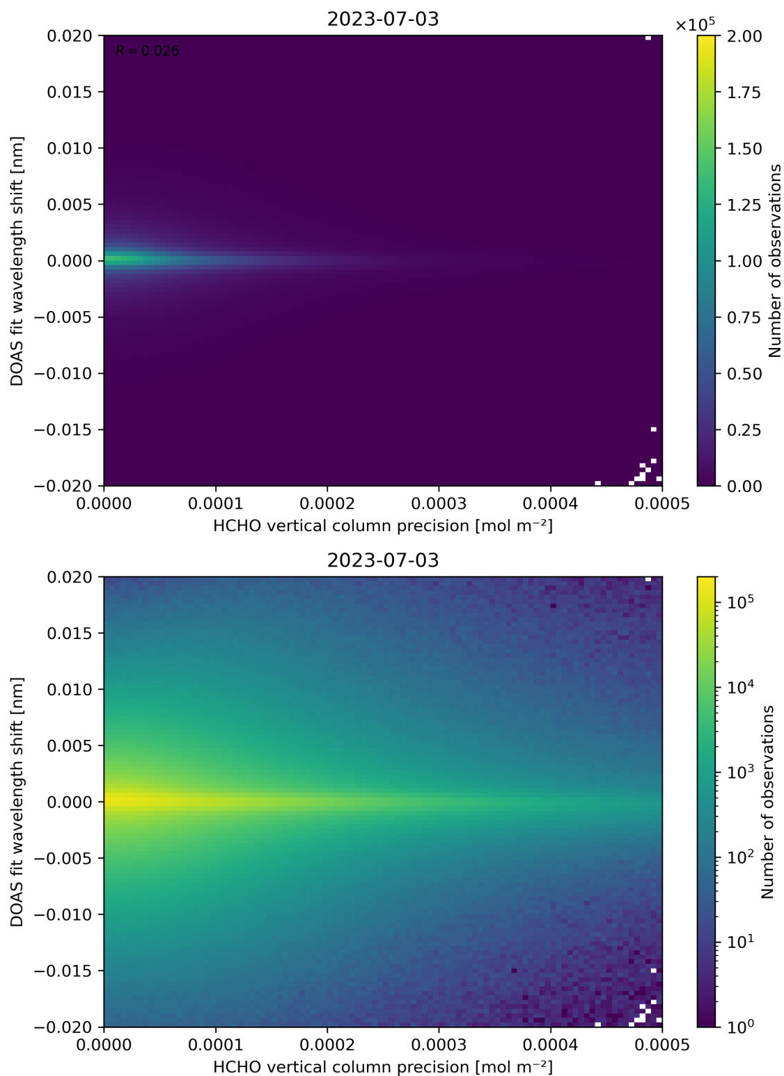
Figure 137: Scatter density plot of “HCHO vertical column precision” against “DOAS fit wavelength shift” for 2023-07-03 to 2023-07-04.
