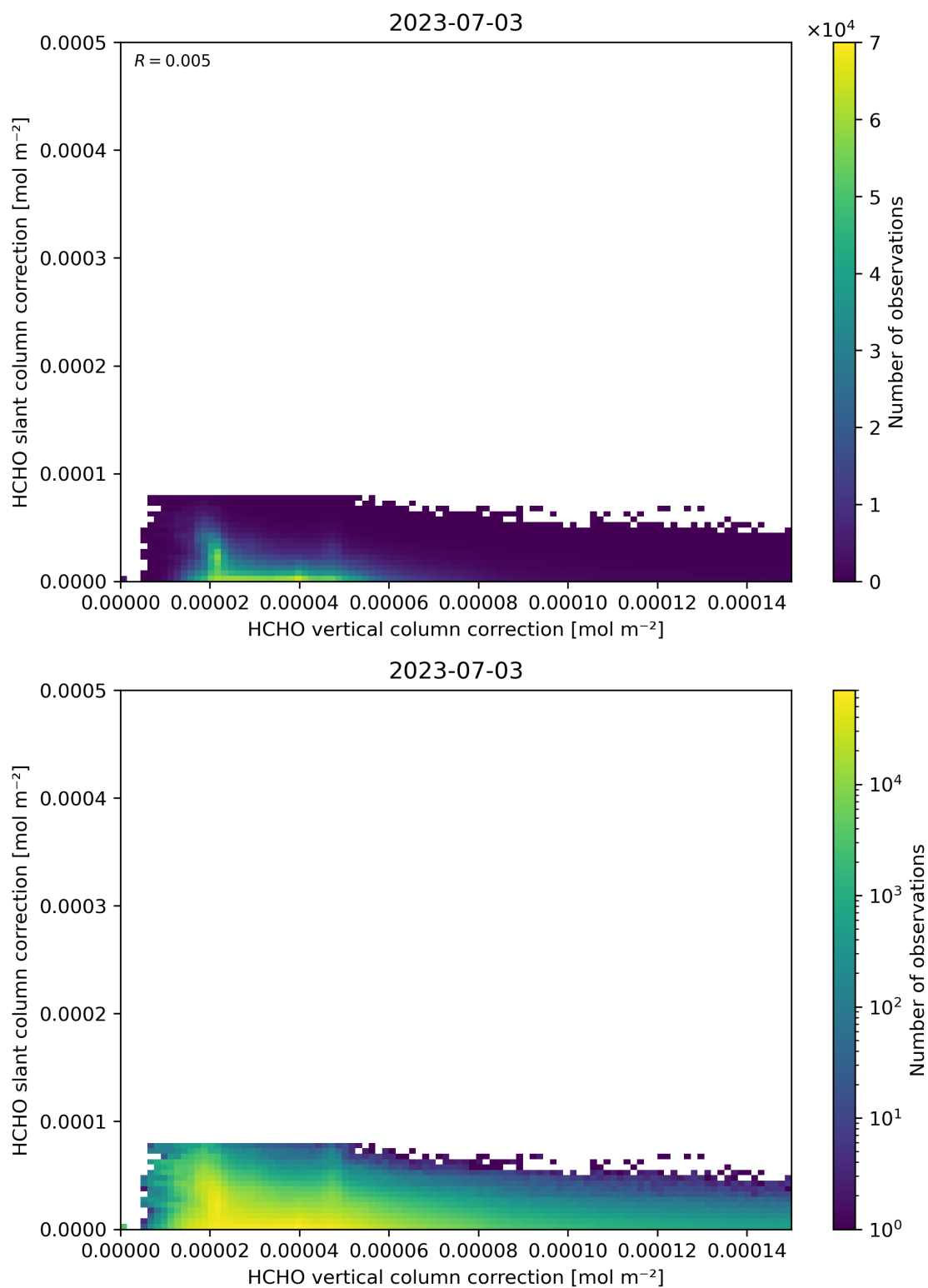
Figure 117: Scatter density plot of “HCHO vertical column correction” against “HCHO slant column correction” for 2023-07-03 to 2023-07-04.
