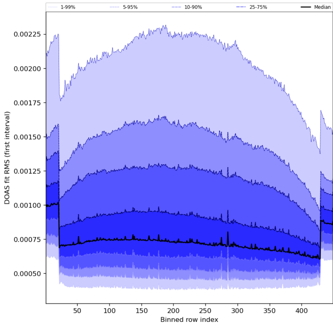
Figure 60: Along track statistics of “DOAS fit RMS (first interval)” for 2023-07-03 to 2023-07-04
