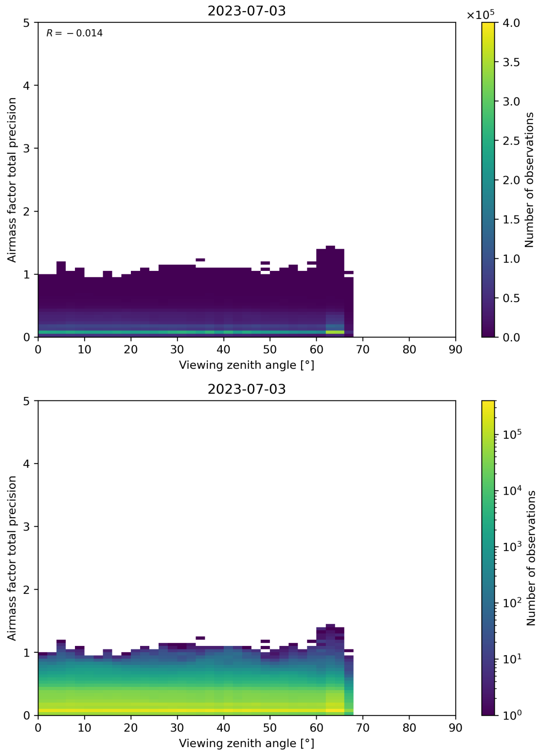
Figure 191: Scatter density plot of “Viewing zenith angle” against “Airmass factor total precision” for 2023-07-03 to 2023-07-04.
