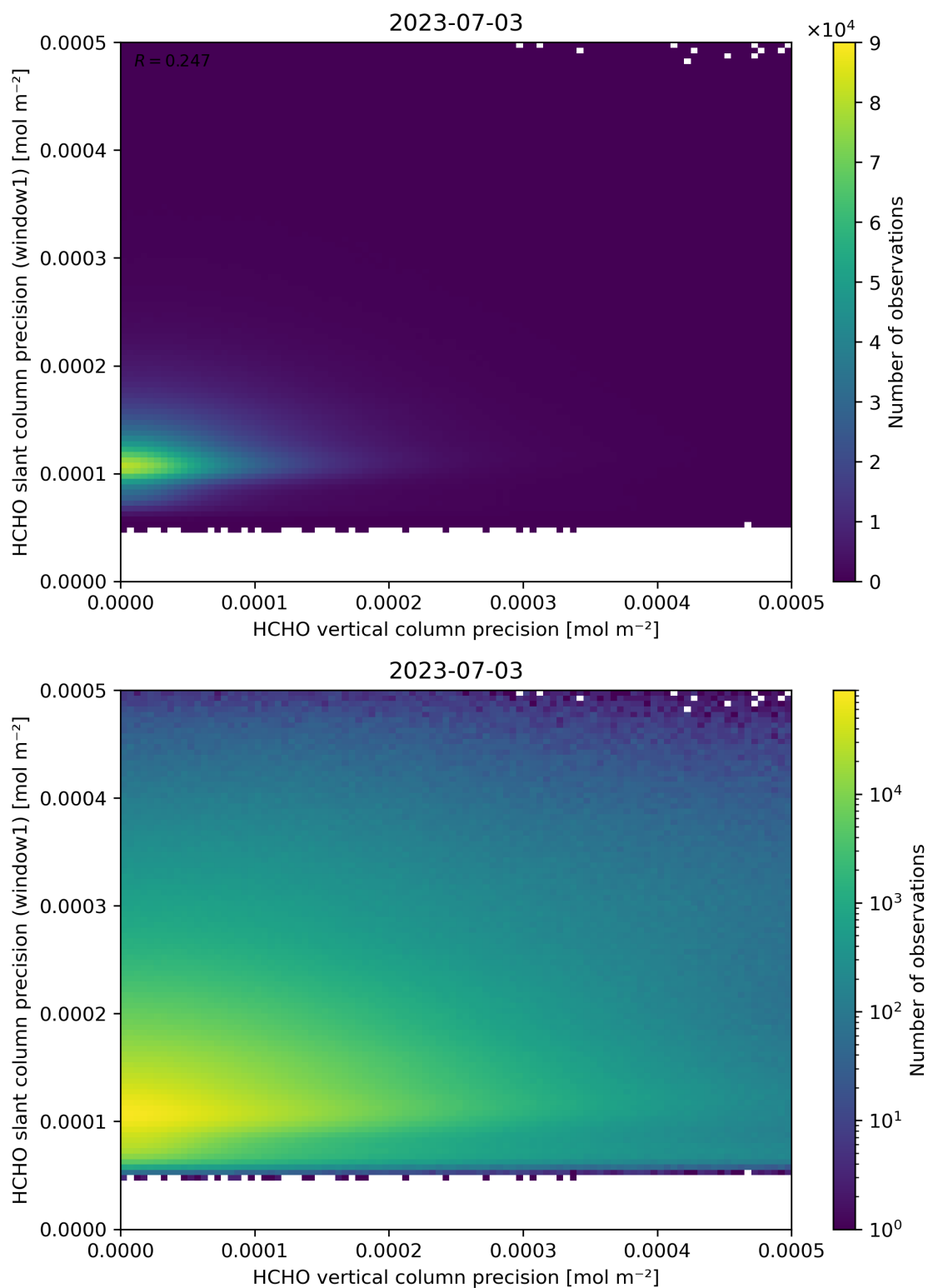
Figure 143: Scatter density plot of “HCHO vertical column precision” against “HCHO slant column precision (window1)” for 2023-07-03 to 2023-07-04.
