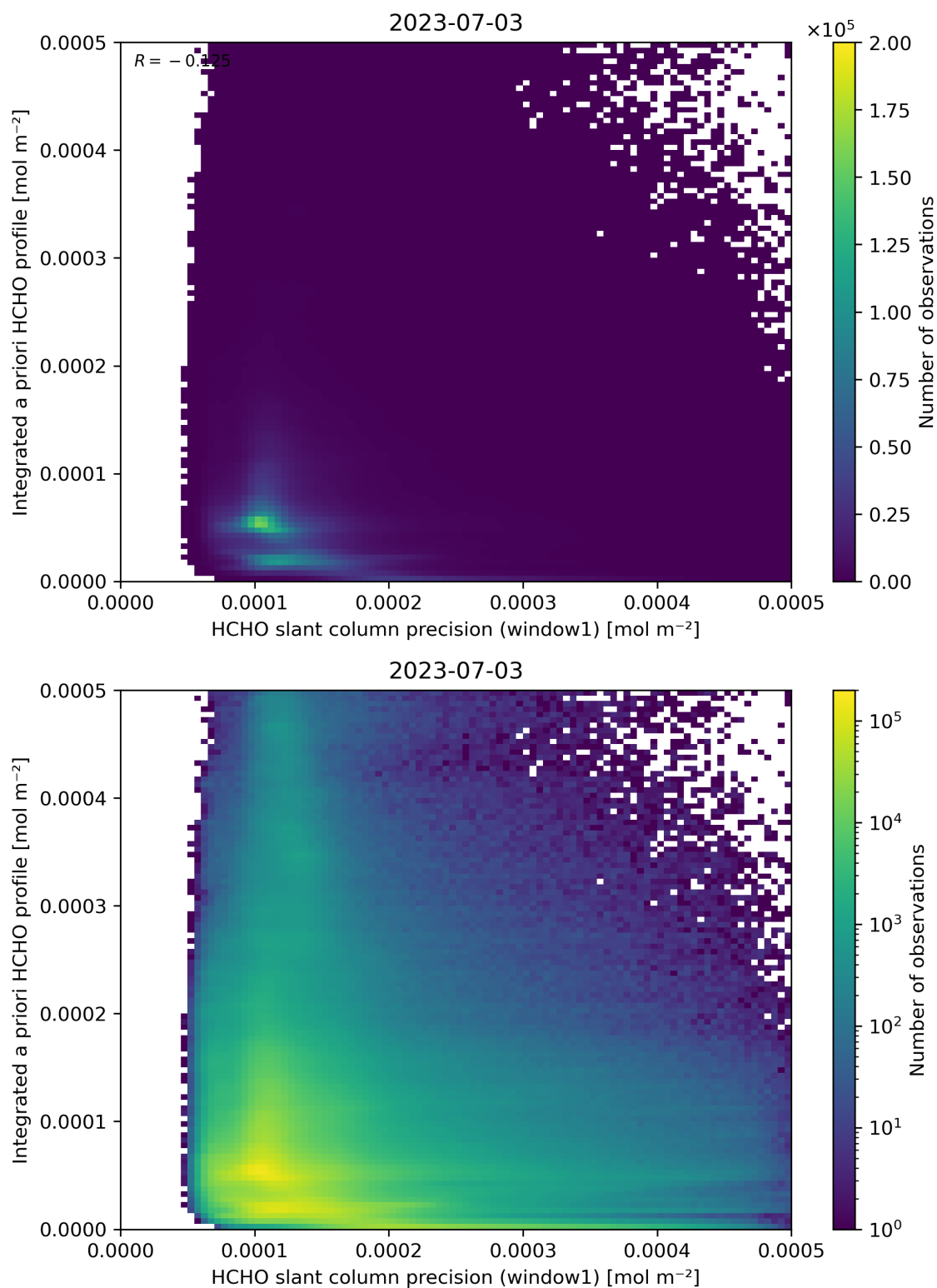
Figure 96: Scatter density plot of “HCHO slant column precision (window1)” against “Integrated a priori HCHO profile” for 2023-07-03 to 2023-07-04.
