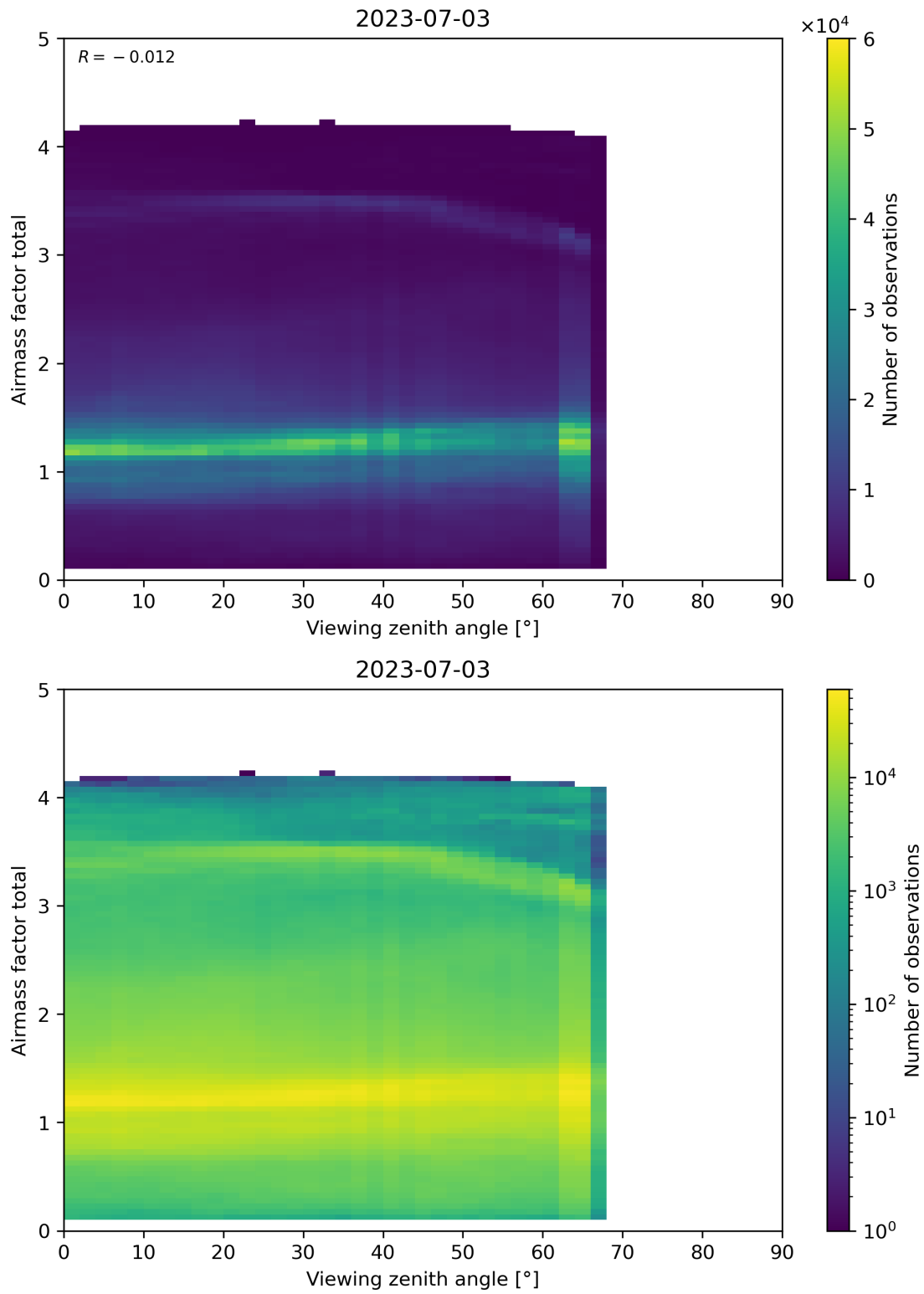
Figure 190: Scatter density plot of “Viewing zenith angle” against “Airmass factor total” for 2023-07-03 to 2023-07-04.
