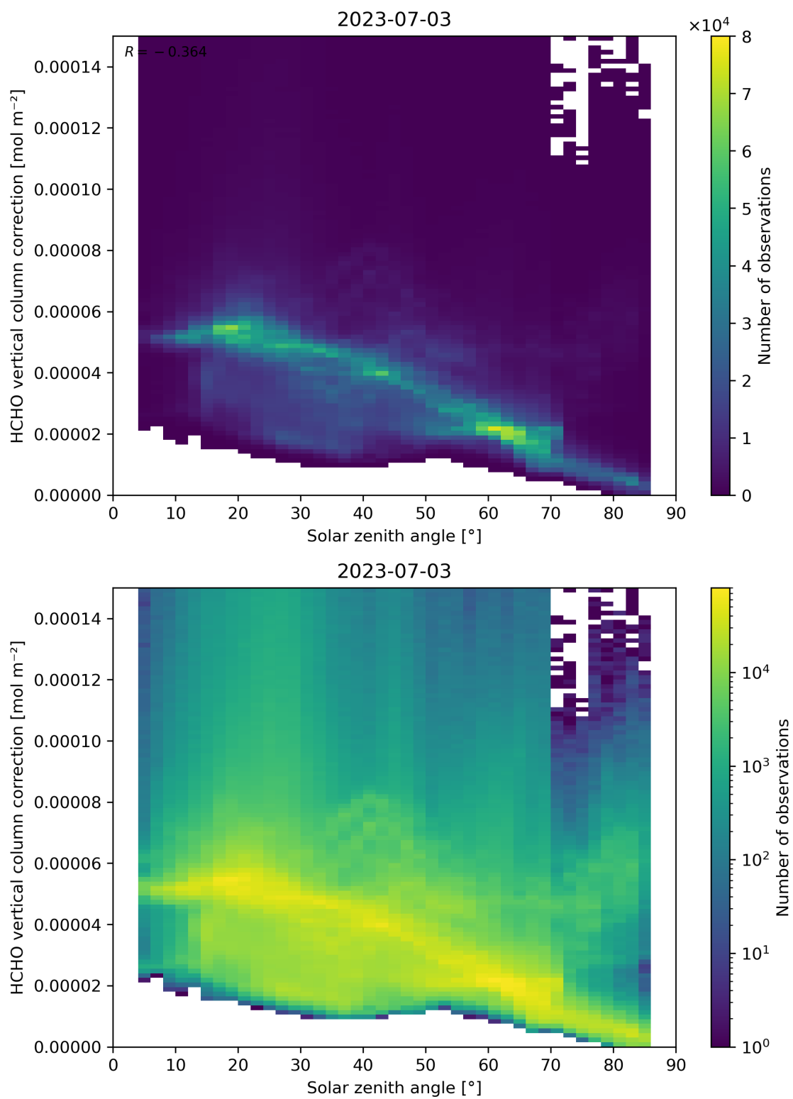
Figure 178: Scatter density plot of “Solar zenith angle” against “HCHO vertical column correction” for 2023-07-03 to 2023-07-04.
