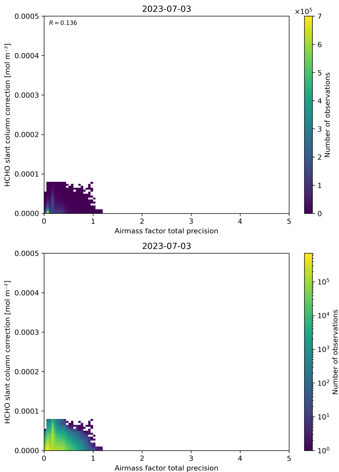
Figure 110: Scatter density plot of “Airmass factor total precision” against “HCHO slant column correction” for 2023-07-03 to 2023-07-04.
