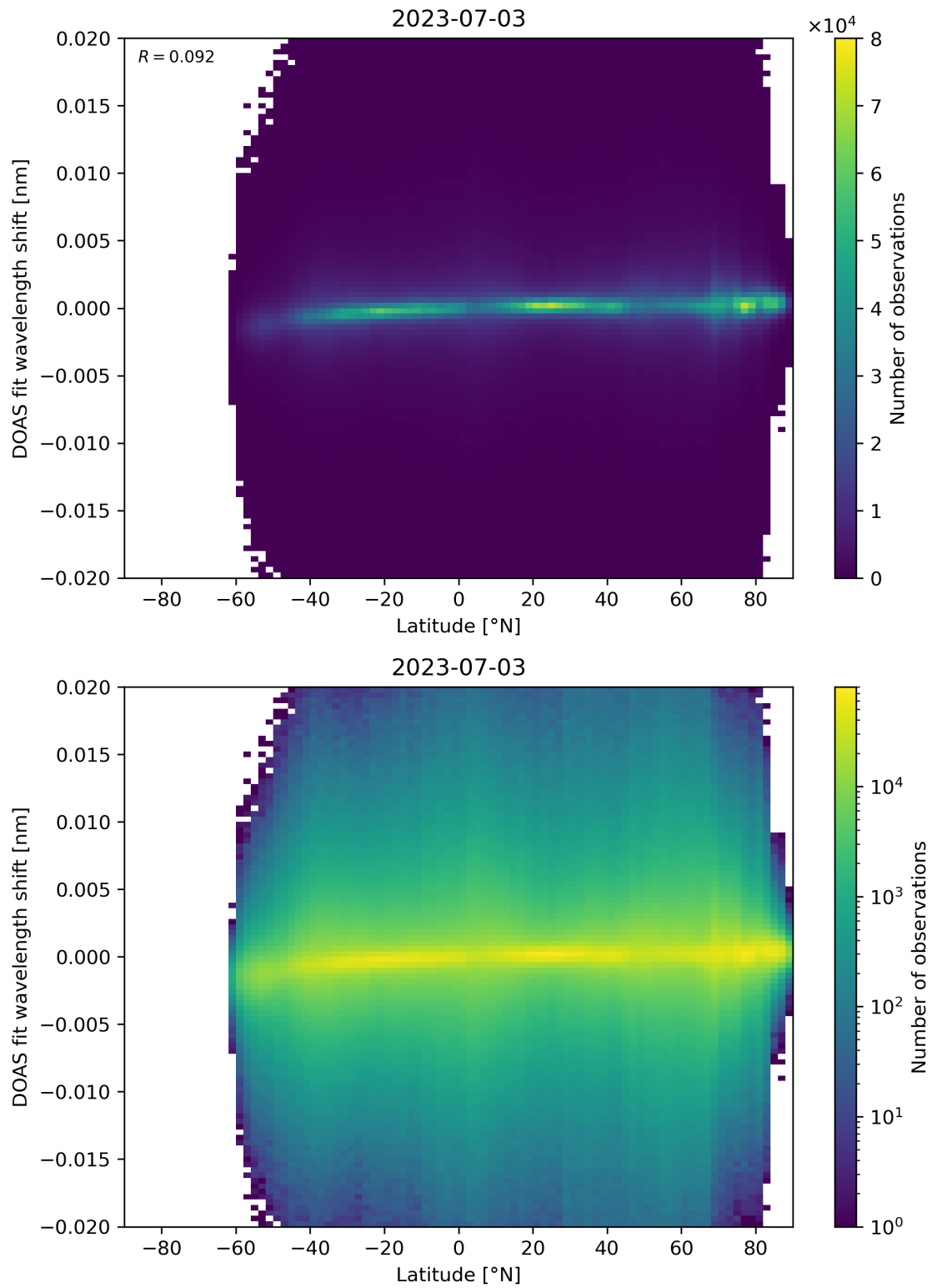
Figure 154: Scatter density plot of “Latitude” against “DOAS fit wavelength shift” for 2023-07-03 to 2023-07-04.
