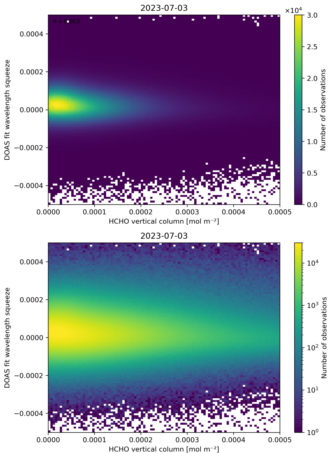
Figure 125: Scatter density plot of “HCHO vertical column” against “DOAS fit wavelength squeeze” for 2023-07-03 to 2023-07-04.
