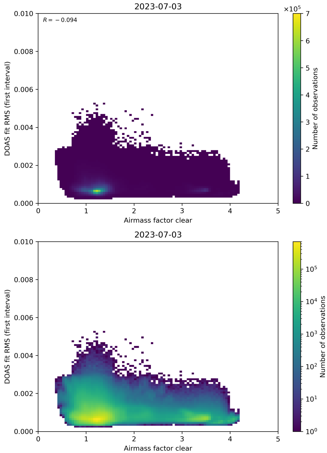
Figure 71: Scatter density plot of “Airmass factor clear” against “DOAS fit RMS (first interval)” for 2023-07-03 to 2023-07-04.
