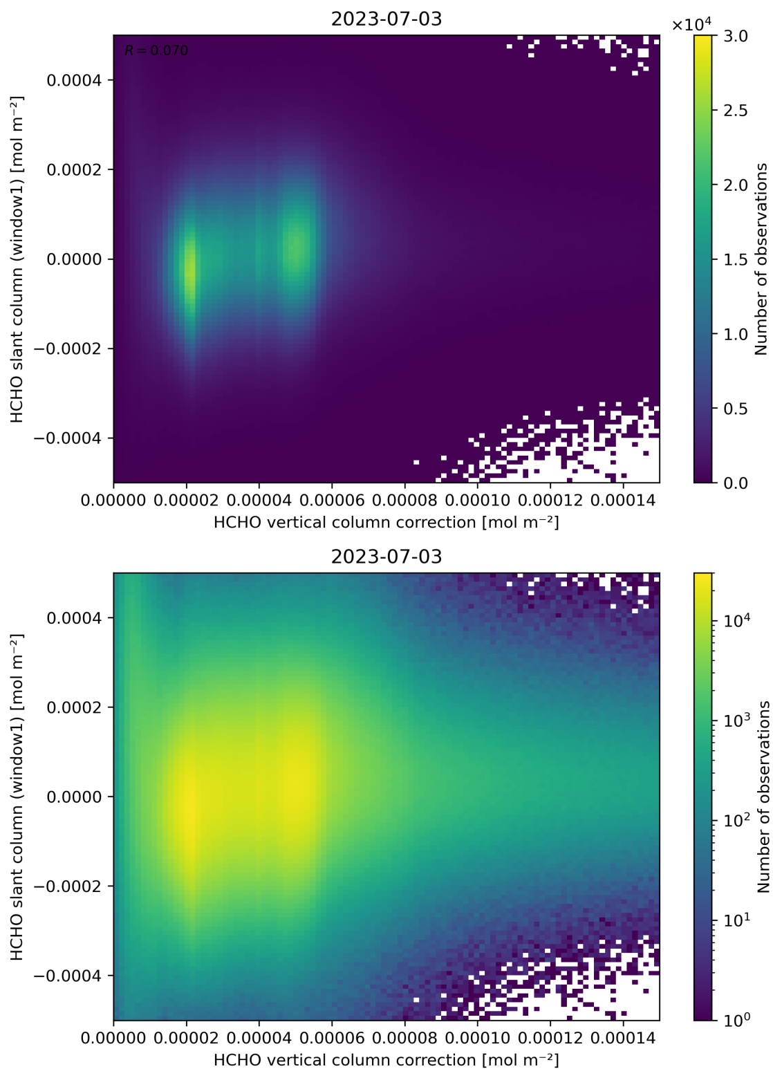
Figure 118: Scatter density plot of “HCHO vertical column correction” against “HCHO slant column (window1)” for 2023-07-03 to 2023-07-04.
