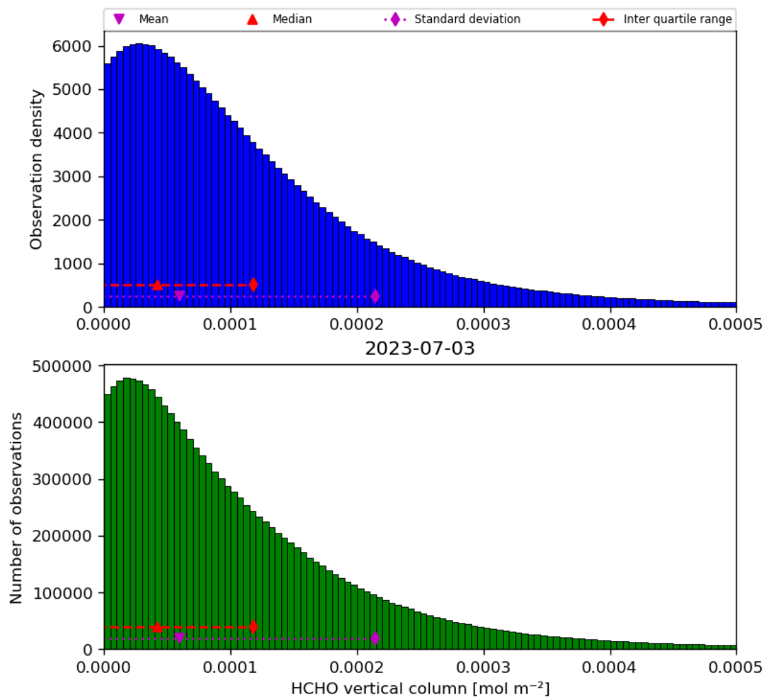
Figure 35: Histogram of “HCHO vertical column” for 2023-07-03 to 2023-07-04
