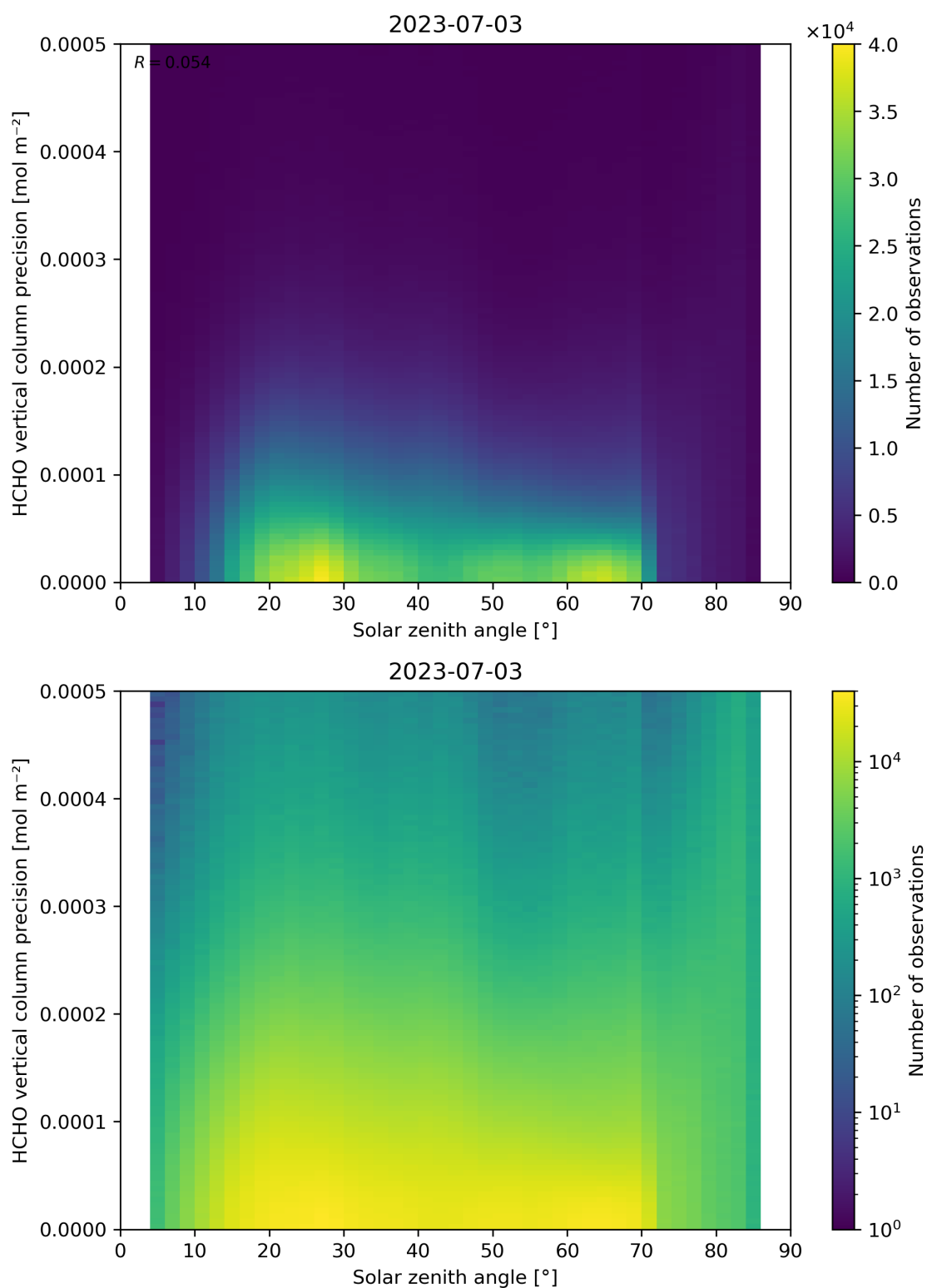
Figure 179: Scatter density plot of “Solar zenith angle” against “HCHO vertical column precision” for 2023-07-03 to 2023-07-04.
