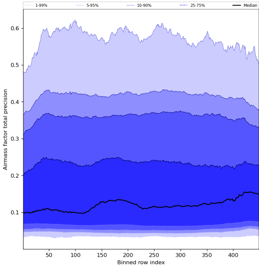
Figure 55: Along track statistics of “Airmass factor total precision” for 2023-07-03 to 2023-07-04
