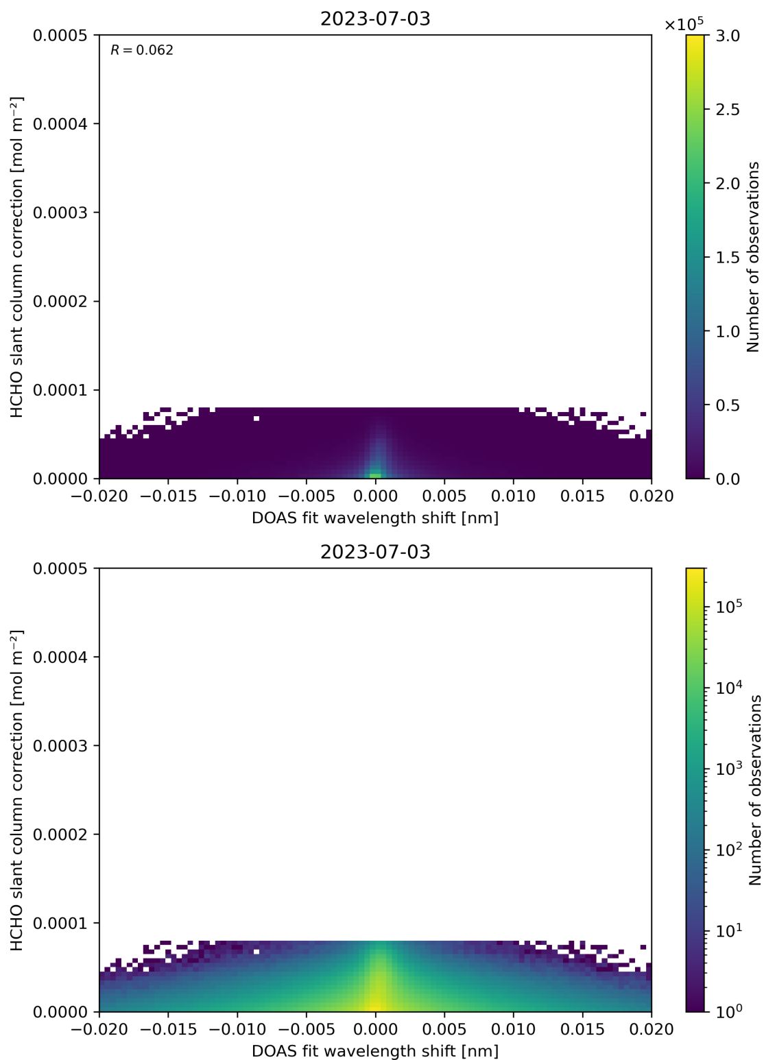
Figure 67: Scatter density plot of “DOAS fit wavelength shift” against “HCHO slant column correction” for 2023-07-03 to 2023-07-04.
