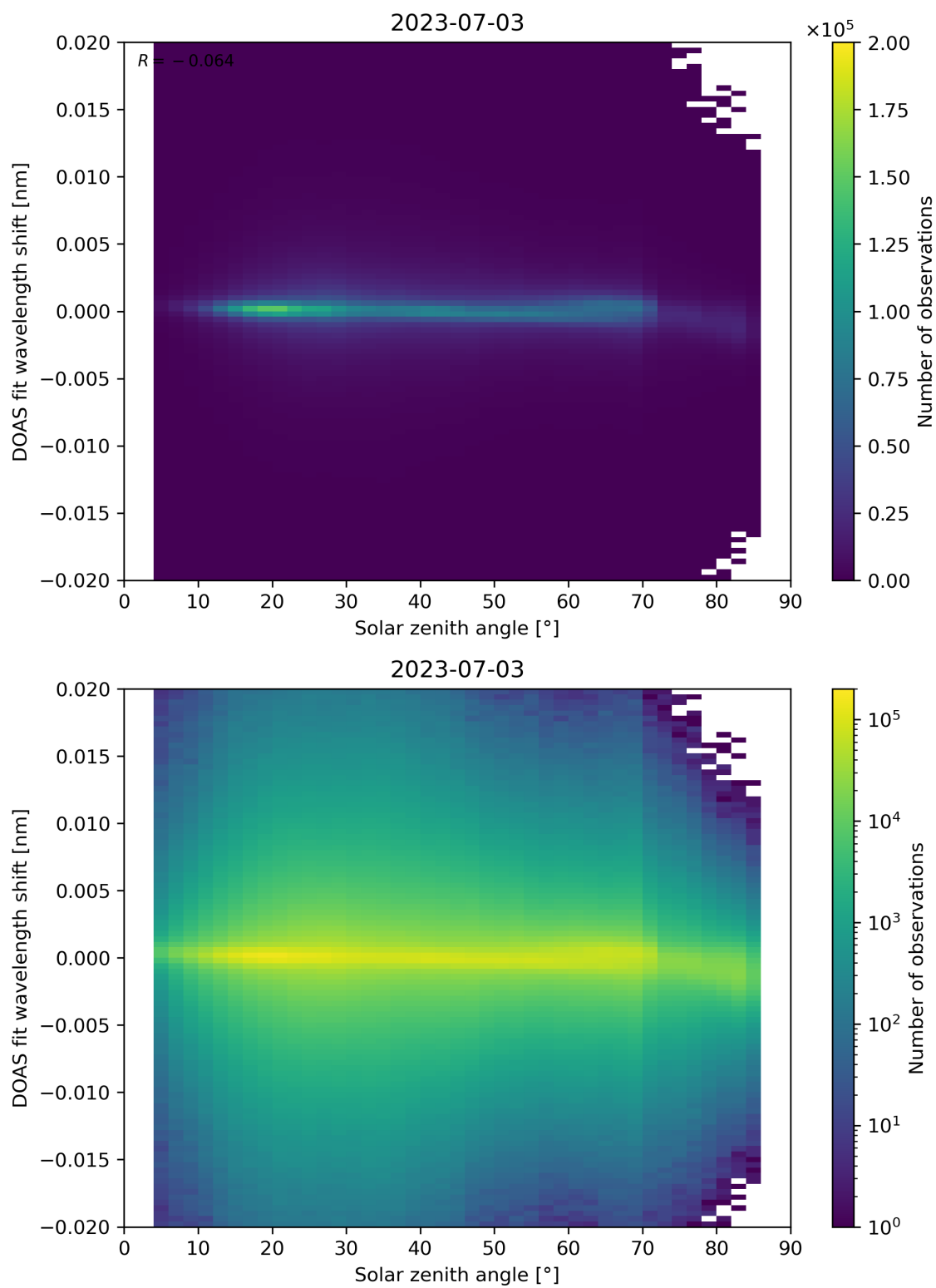
Figure 168: Scatter density plot of “Solar zenith angle” against “DOAS fit wavelength shift” for 2023-07-03 to 2023-07-04.
