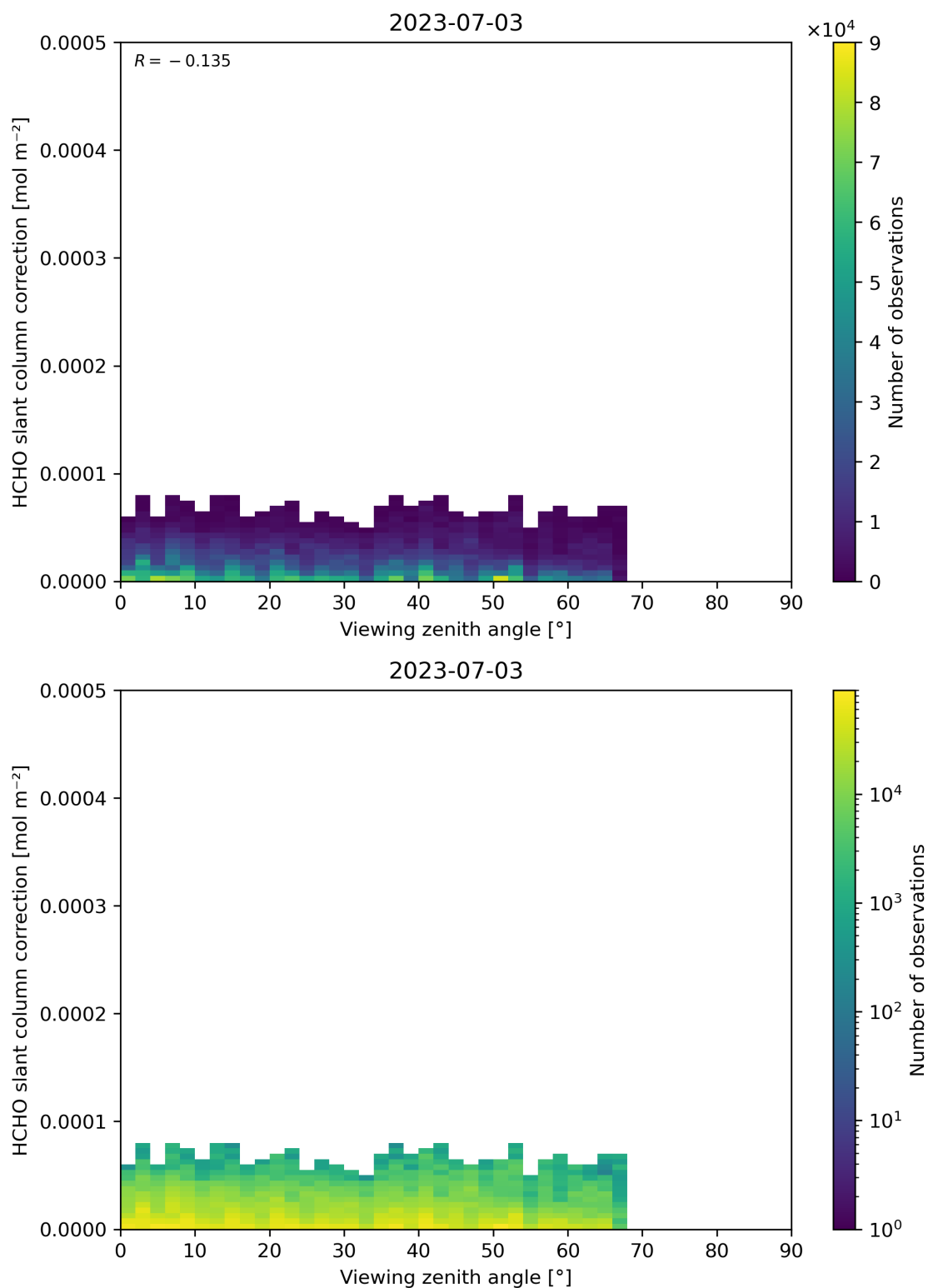
Figure 187: Scatter density plot of “Viewing zenith angle” against “HCHO slant column correction” for 2023-07-03 to 2023-07-04.
