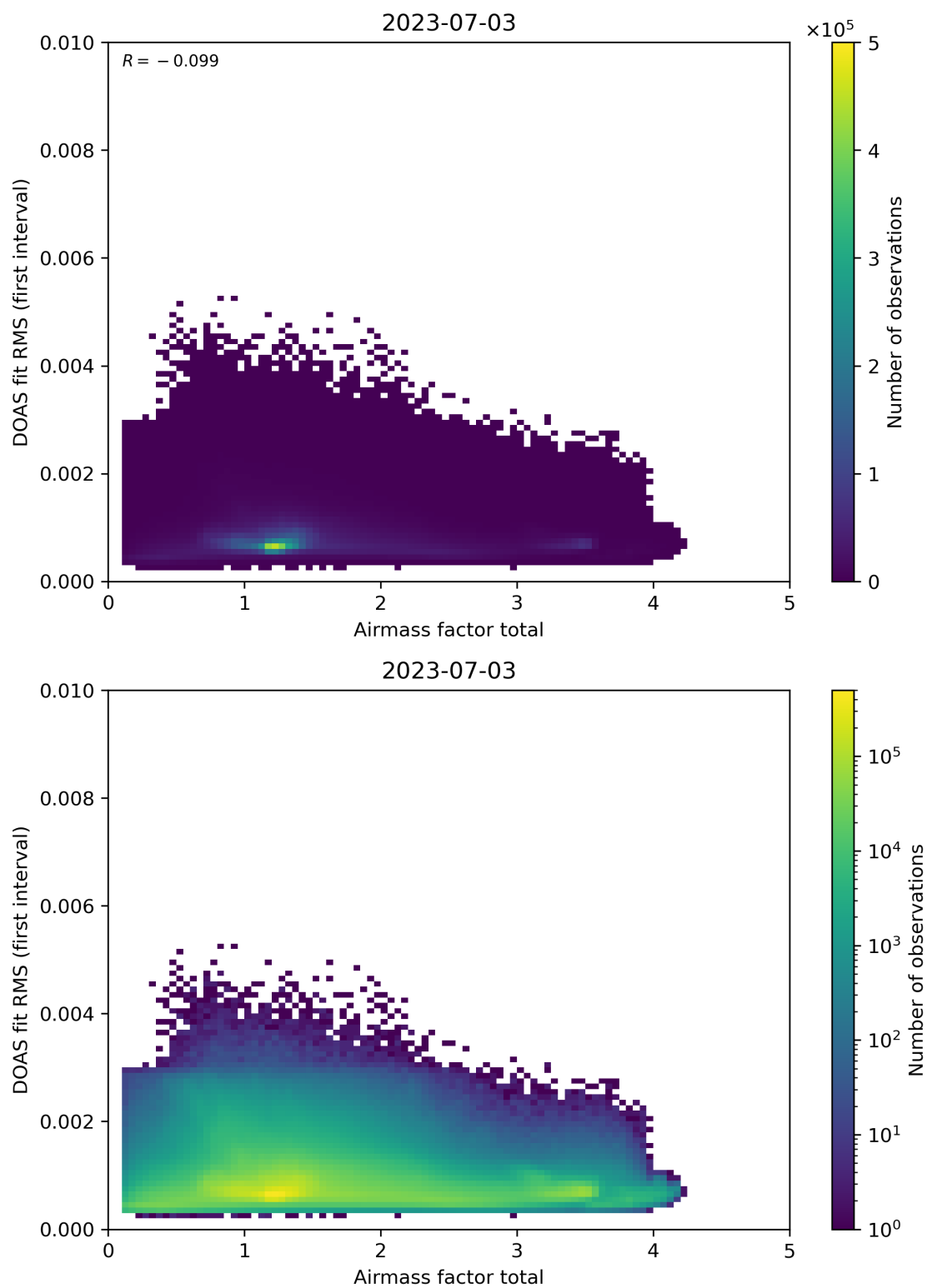
Figure 97: Scatter density plot of “Airmass factor total” against “DOAS fit RMS (first interval)” for 2023-07-03 to 2023-07-04.
