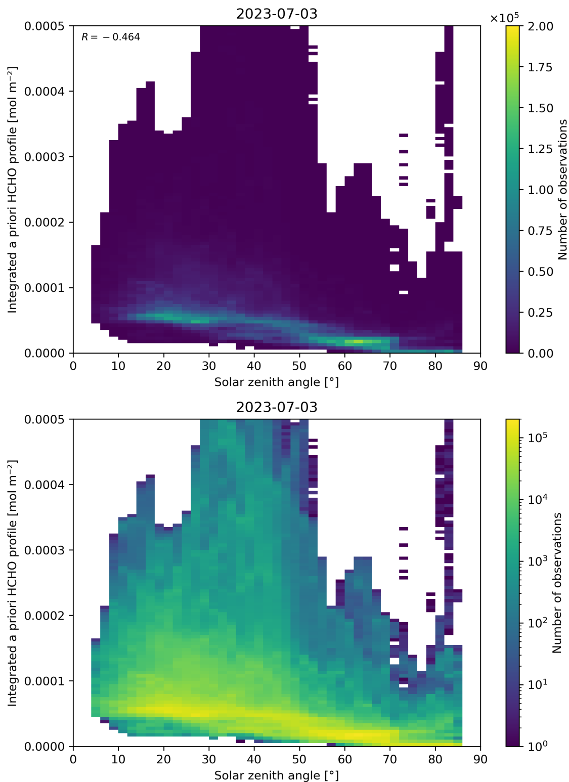
Figure 180: Scatter density plot of “Solar zenith angle” against “Integrated a priori HCHO profile” for 2023-07-03 to 2023-07-04.
