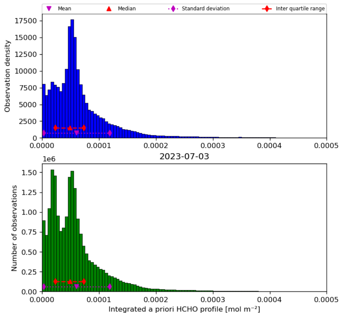
Figure 43: Histogram of “Integrated a priori HCHO profile” for 2023-07-03 to 2023-07-04
